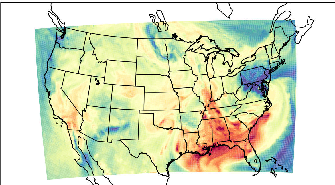
WRF (2023-09-24_20:00:00)
