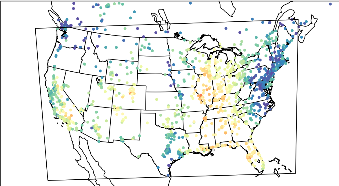
AirNOW (2023-09-23_17:00:00)
