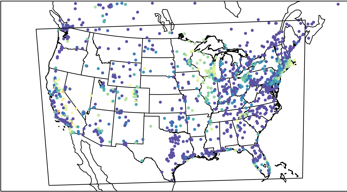
AirNOW (2023-09-24_11:00:00)
