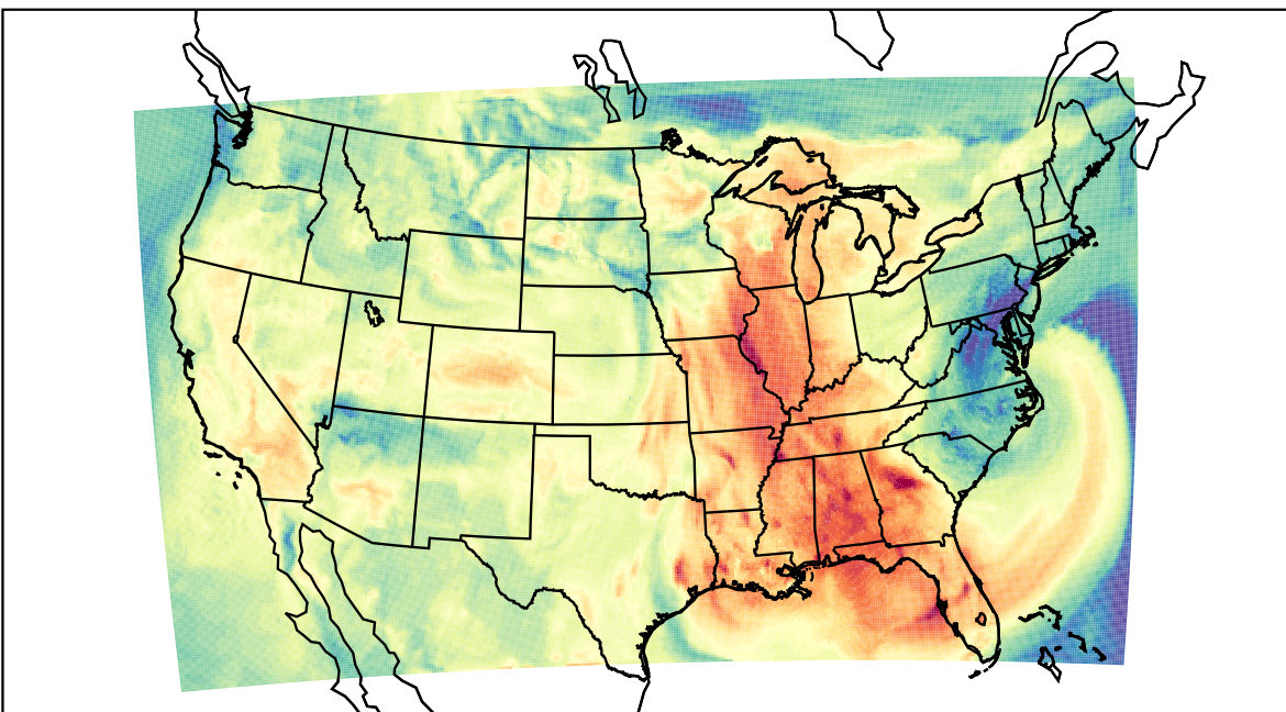
WRF (2023-09-23_19:00:00)
