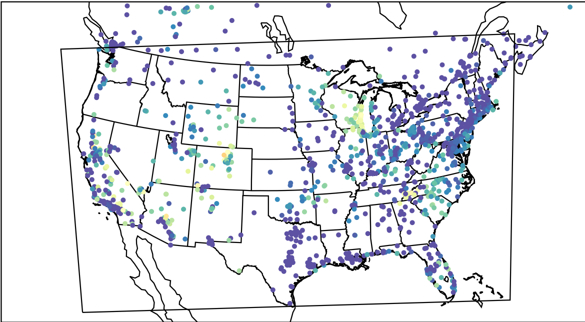
AirNOW (2023-09-23_11:00:00)
