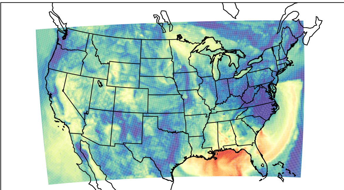
WRF (2023-09-24_10:00:00)
