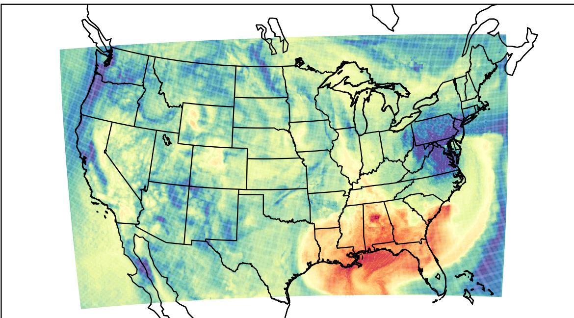
WRF (2023-09-24_16:00:00)
