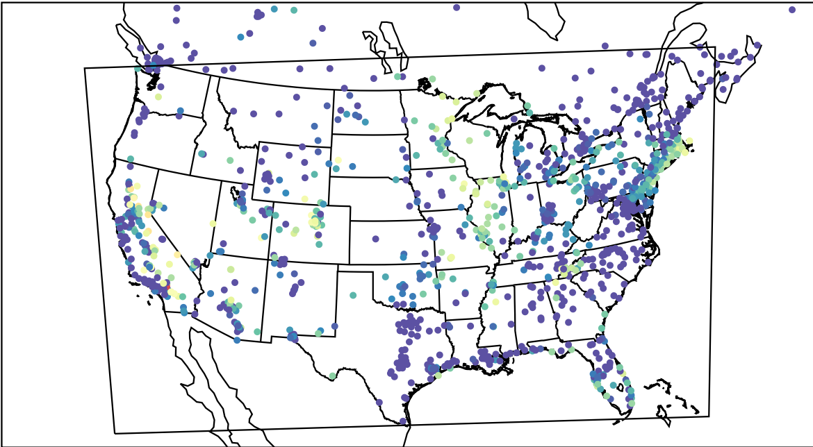
AirNOW (2023-09-24_10:00:00)
