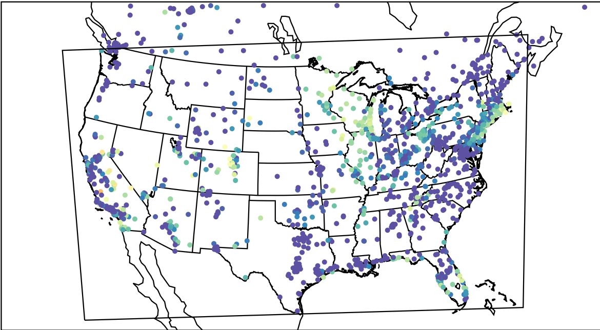
AirNOW (2023-09-24_12:00:00)
