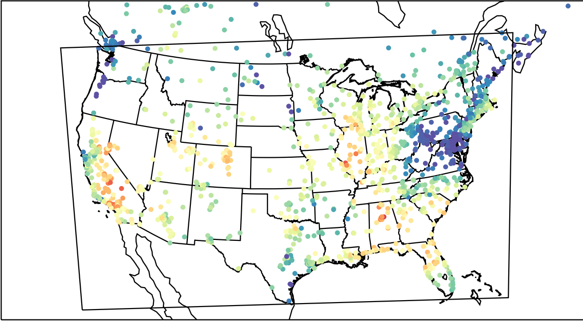
AirNOW (2023-09-24_19:00:00)
