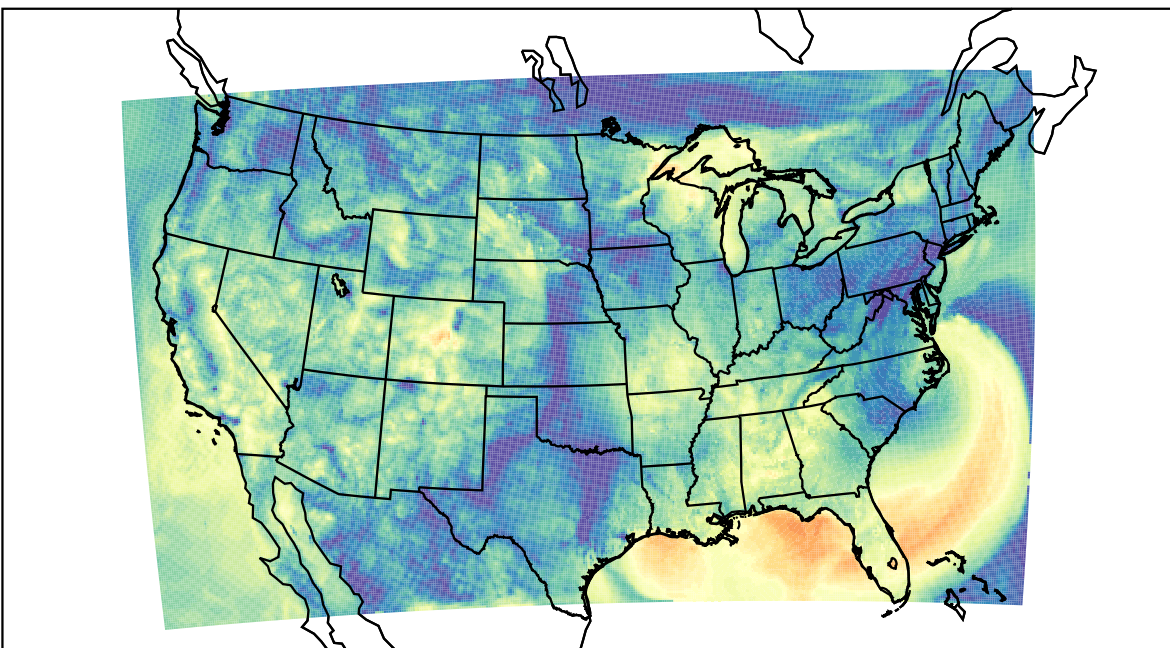
WRF (2023-09-23_14:00:00)
