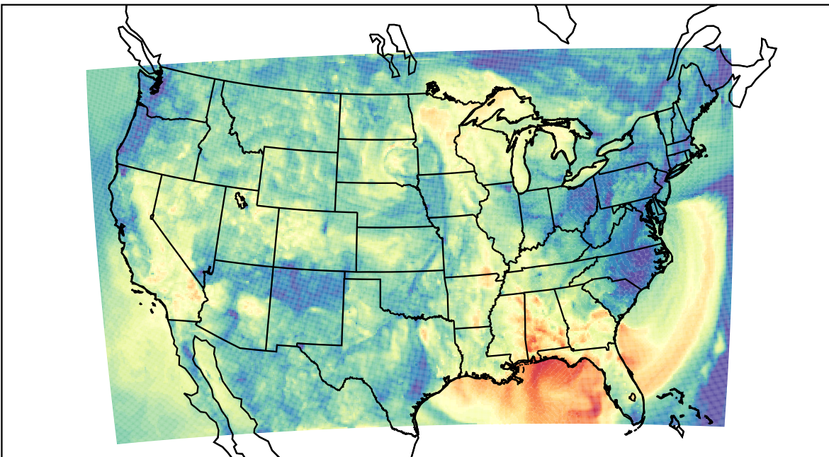
WRF (2023-09-24_04:00:00)
