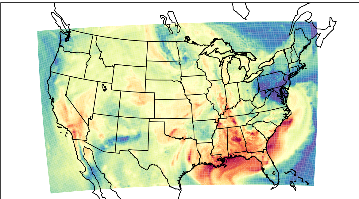
WRF (2023-09-24_22:00:00)
