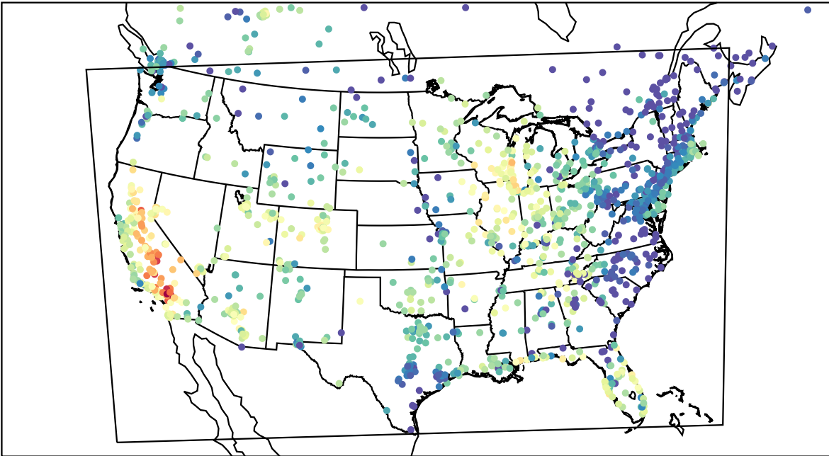
AirNOW (2023-09-24_01:00:00)
