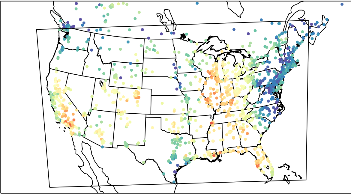
AirNOW (2023-09-23_19:00:00)
