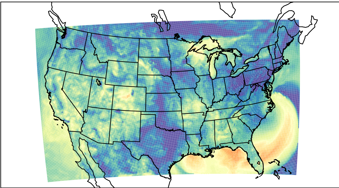
WRF (2023-09-23_13:00:00)
