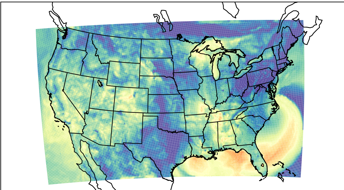
WRF (2023-09-23_12:00:00)
