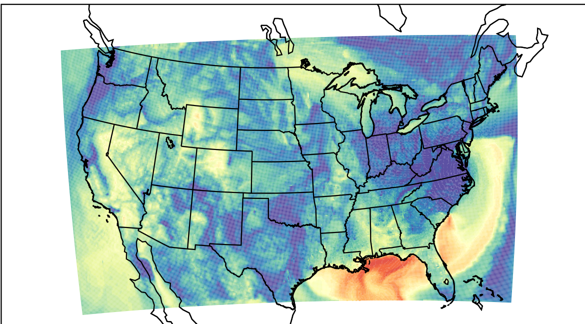
WRF (2023-09-24_13:00:00)
