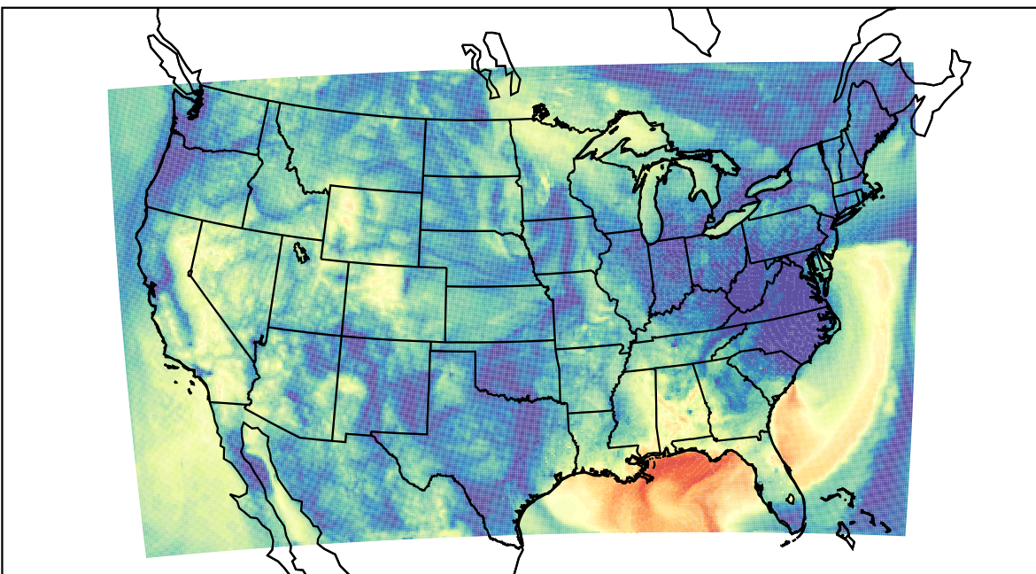
WRF (2023-09-24_12:00:00)
