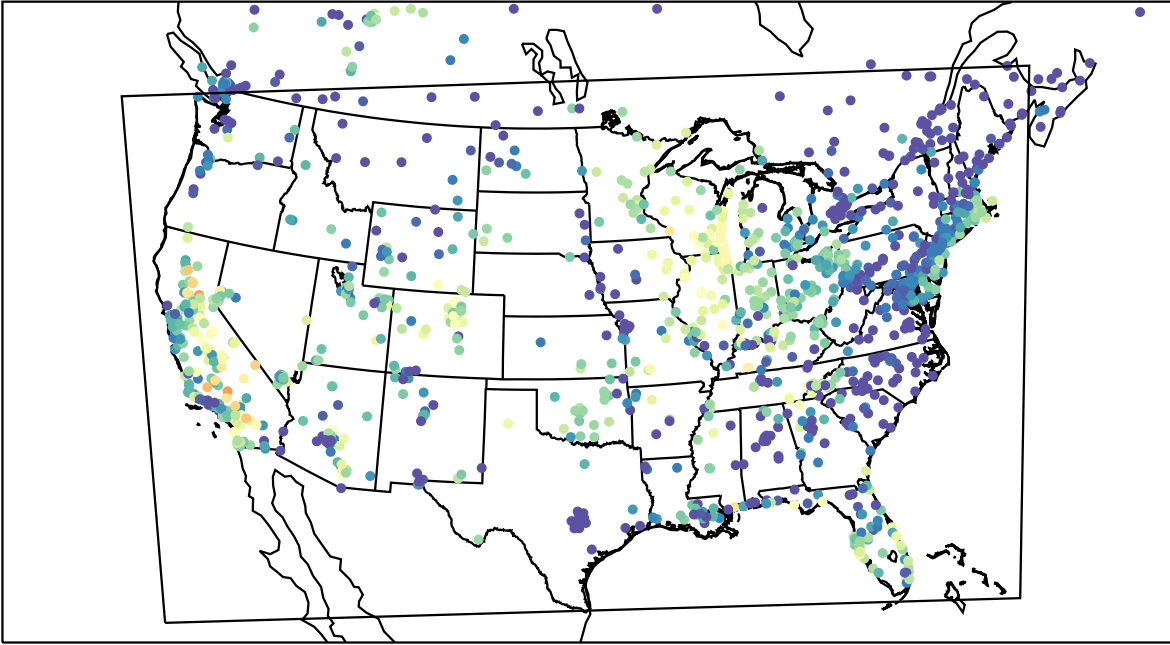
AirNOW (2023-09-24_04:00:00)
