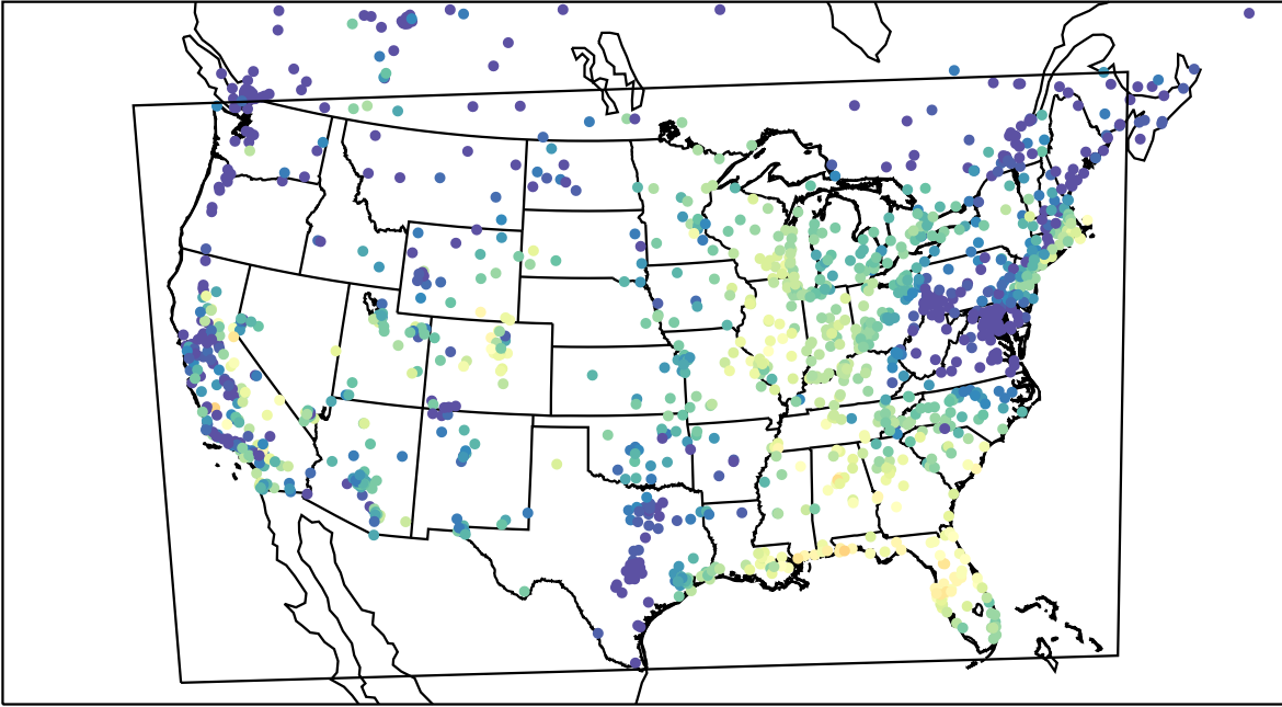
AirNOW (2023-09-24_15:00:00)
