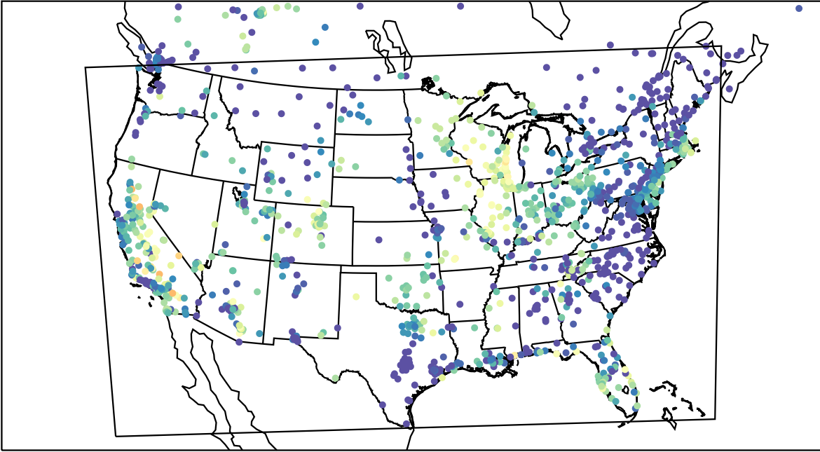
AirNOW (2023-09-24_05:00:00)
