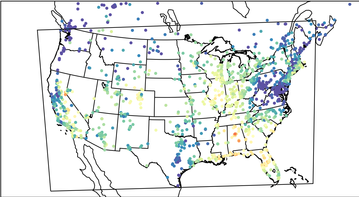
AirNOW (2023-09-24_16:00:00)
