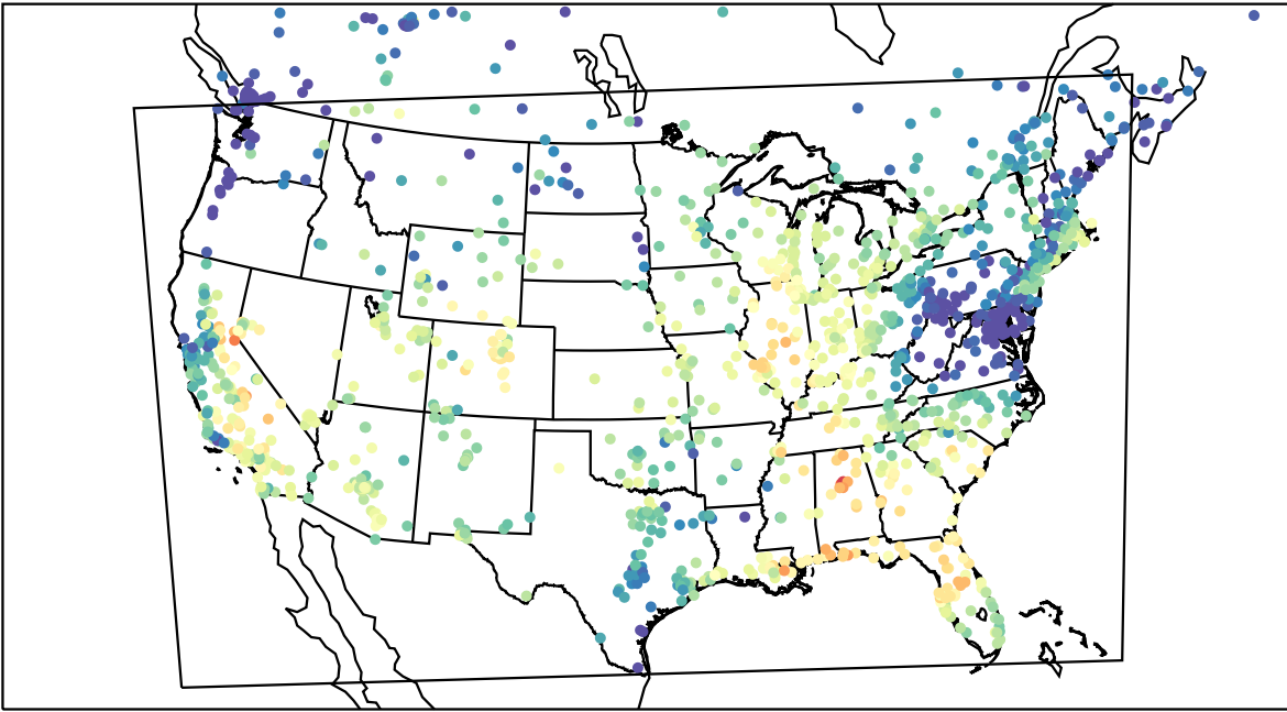
AirNOW (2023-09-24_17:00:00)
