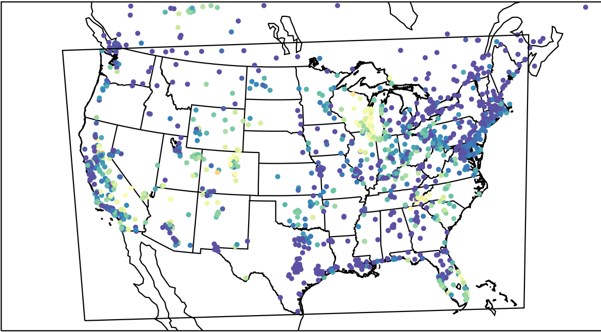
AirNOW (2023-09-23_08:00:00)
