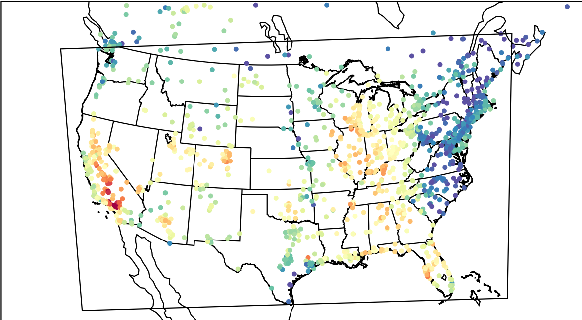
AirNOW (2023-09-23_22:00:00)
