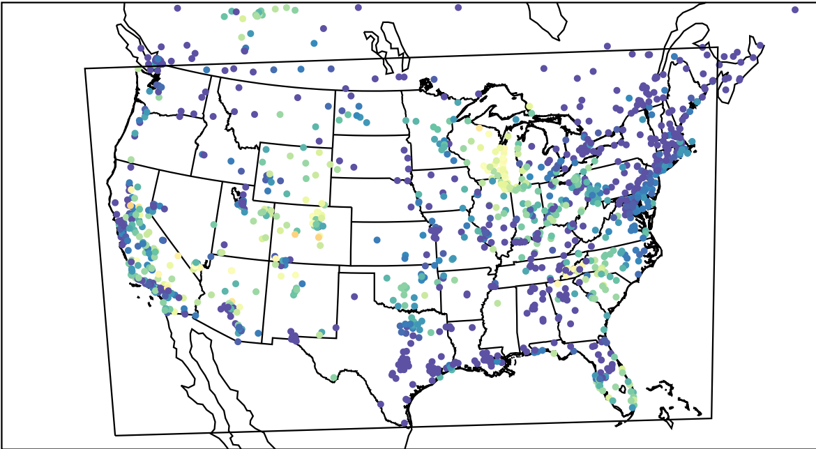
AirNOW (2023-09-23_07:00:00)
