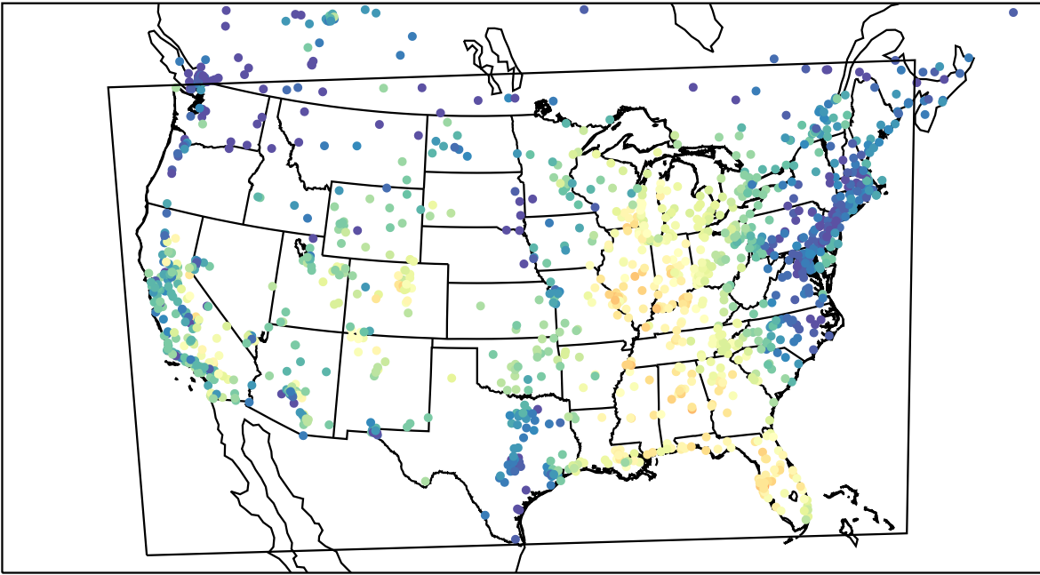
AirNOW (2023-09-23_16:00:00)
