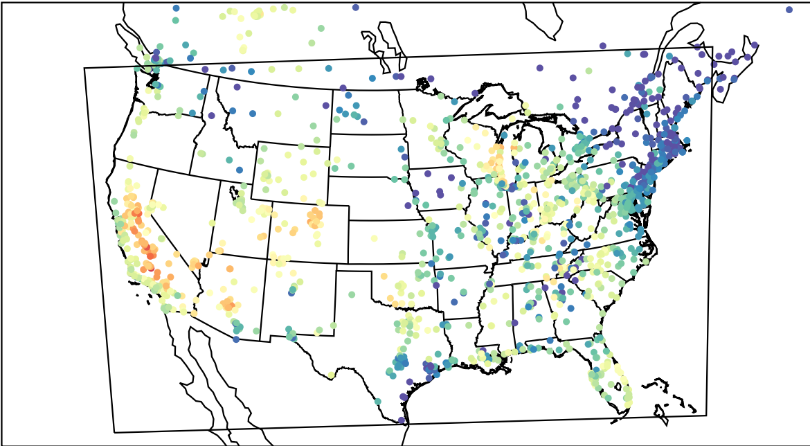
AirNOW (2023-09-23_00:00:00)
