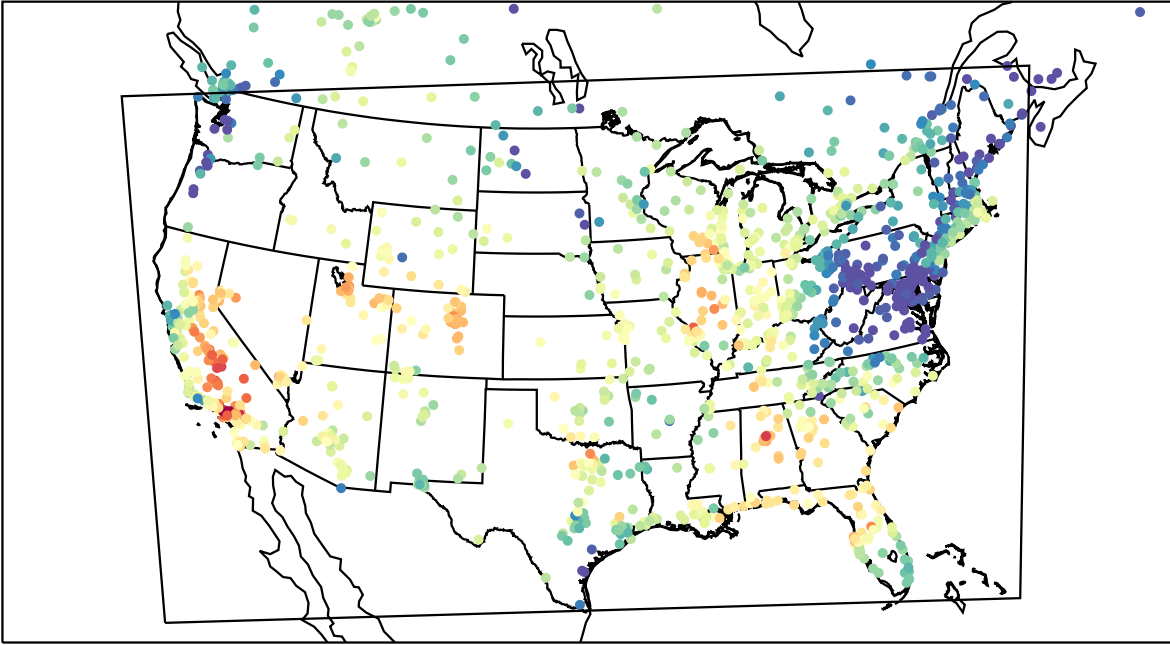
AirNOW (2023-09-24_21:00:00)
