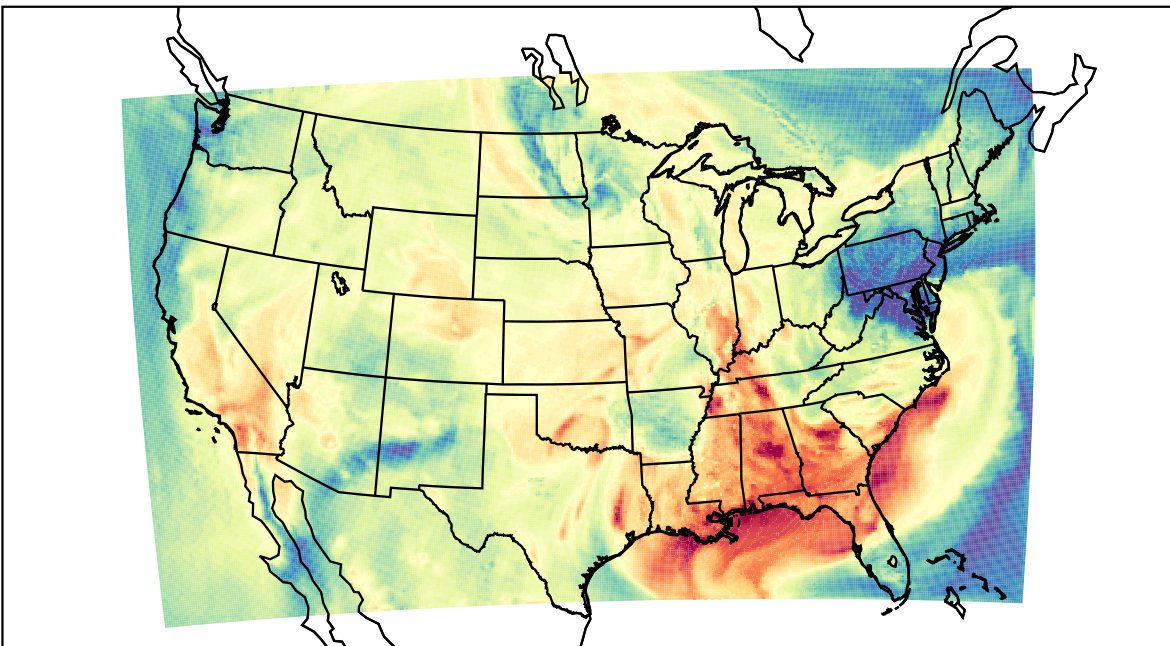
WRF (2023-09-24_21:00:00)
