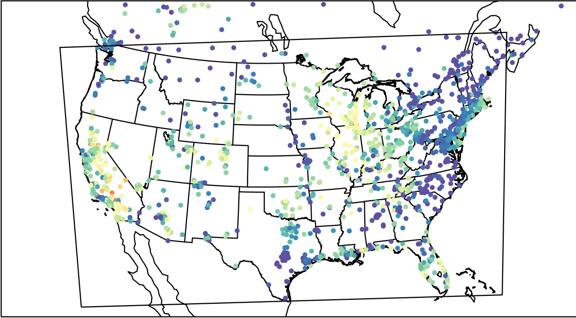
AirNOW (2023-09-24_03:00:00)
