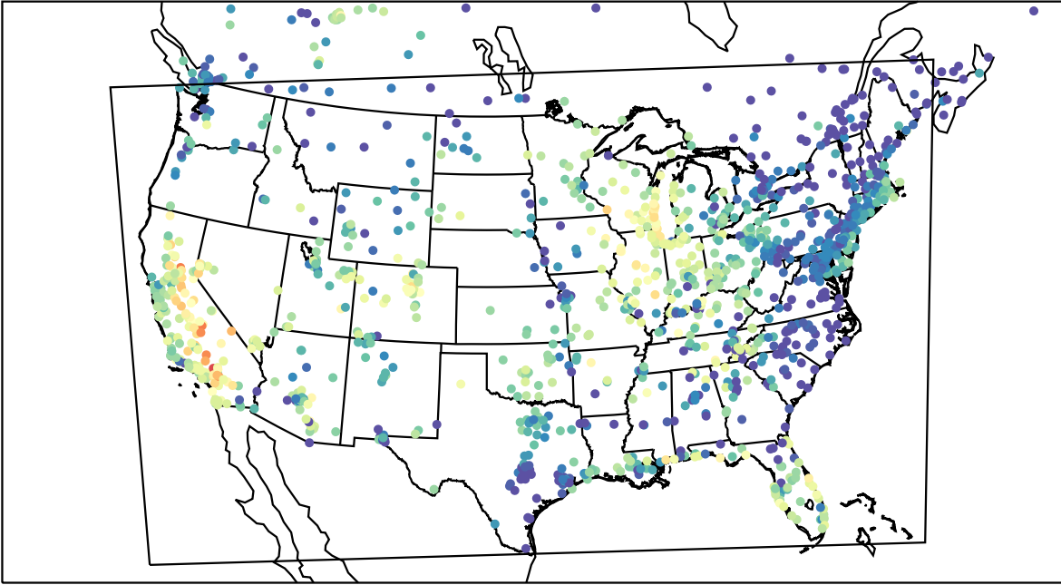
AirNOW (2023-09-24_02:00:00)
