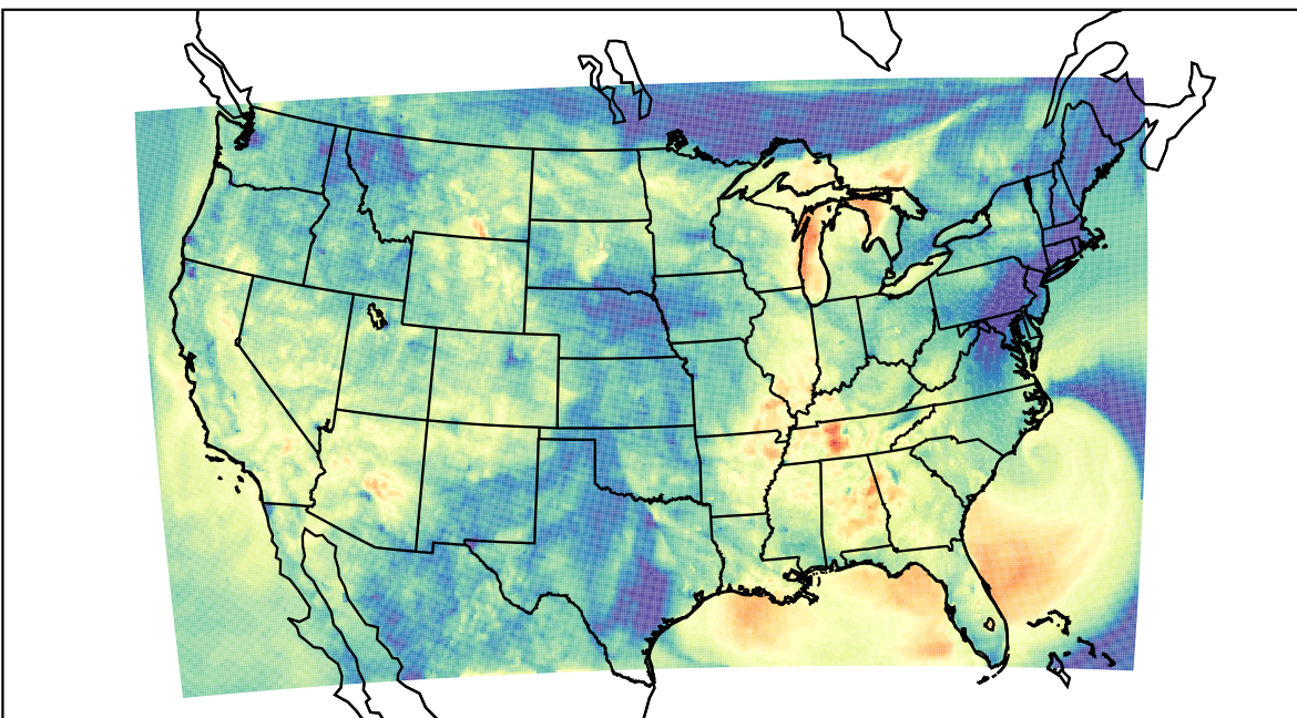
WRF (2023-09-23_04:00:00)
