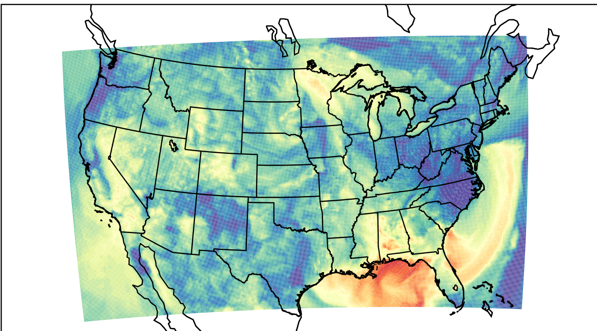
WRF (2023-09-24_08:00:00)
