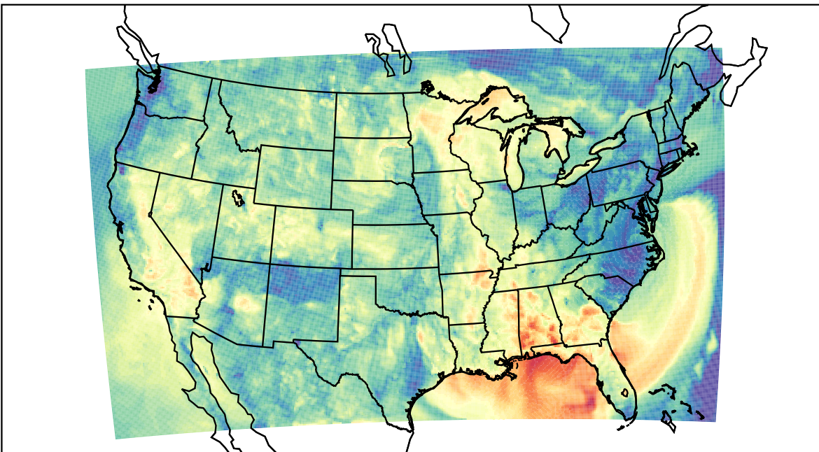
WRF (2023-09-24_03:00:00)
