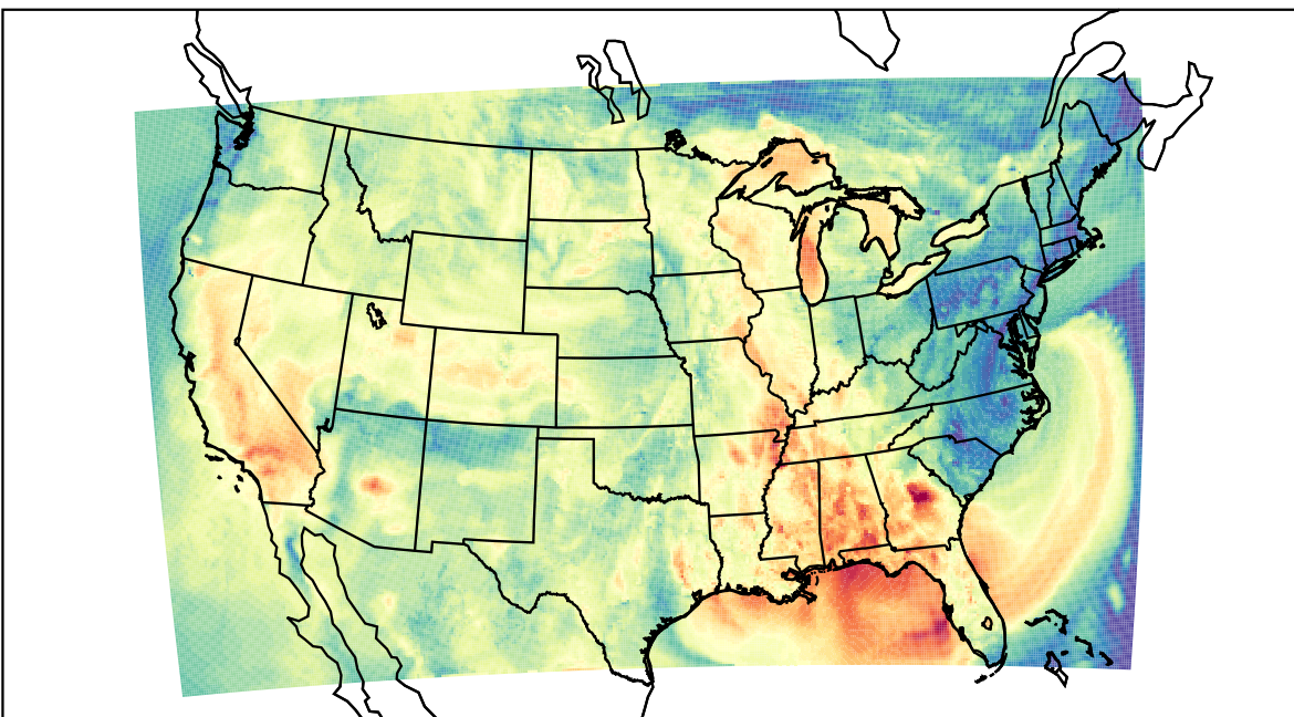
WRF (2023-09-24_00:00:00)
