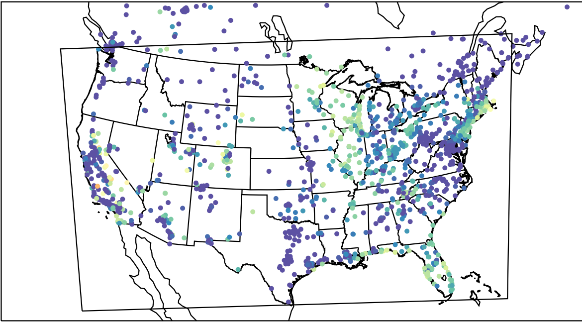
AirNOW (2023-09-24_13:00:00)
