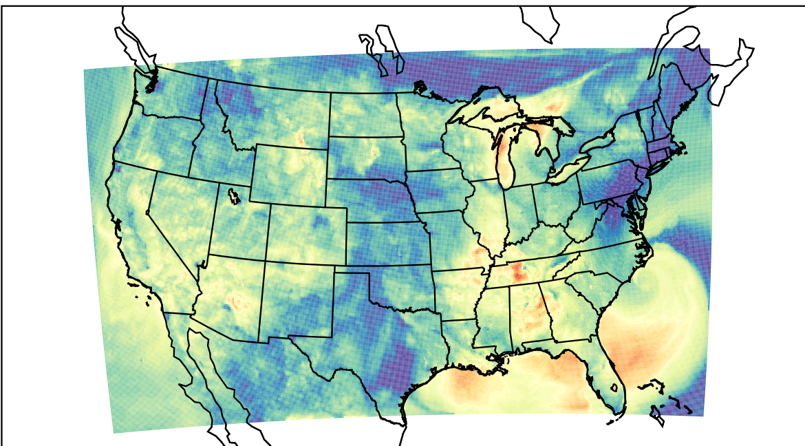
WRF (2023-09-23_05:00:00)
