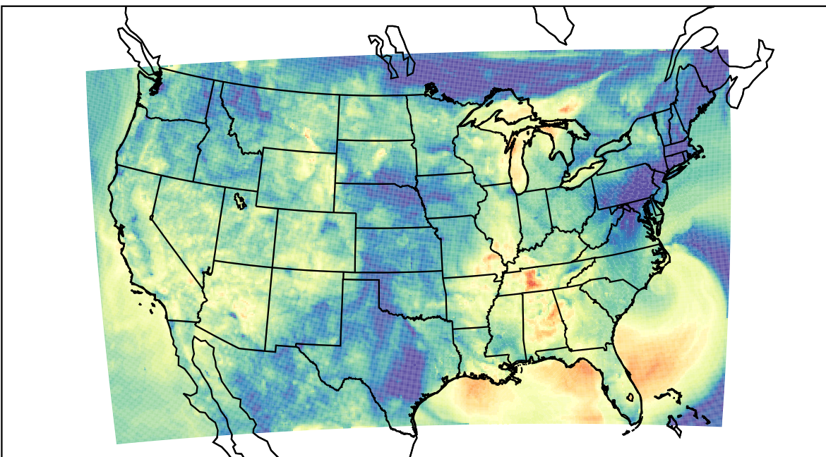
WRF (2023-09-23_06:00:00)
