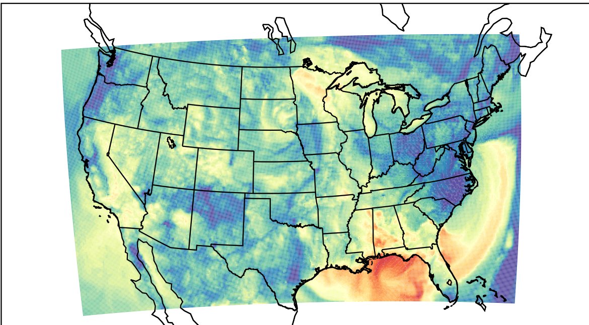
WRF (2023-09-24_06:00:00)
