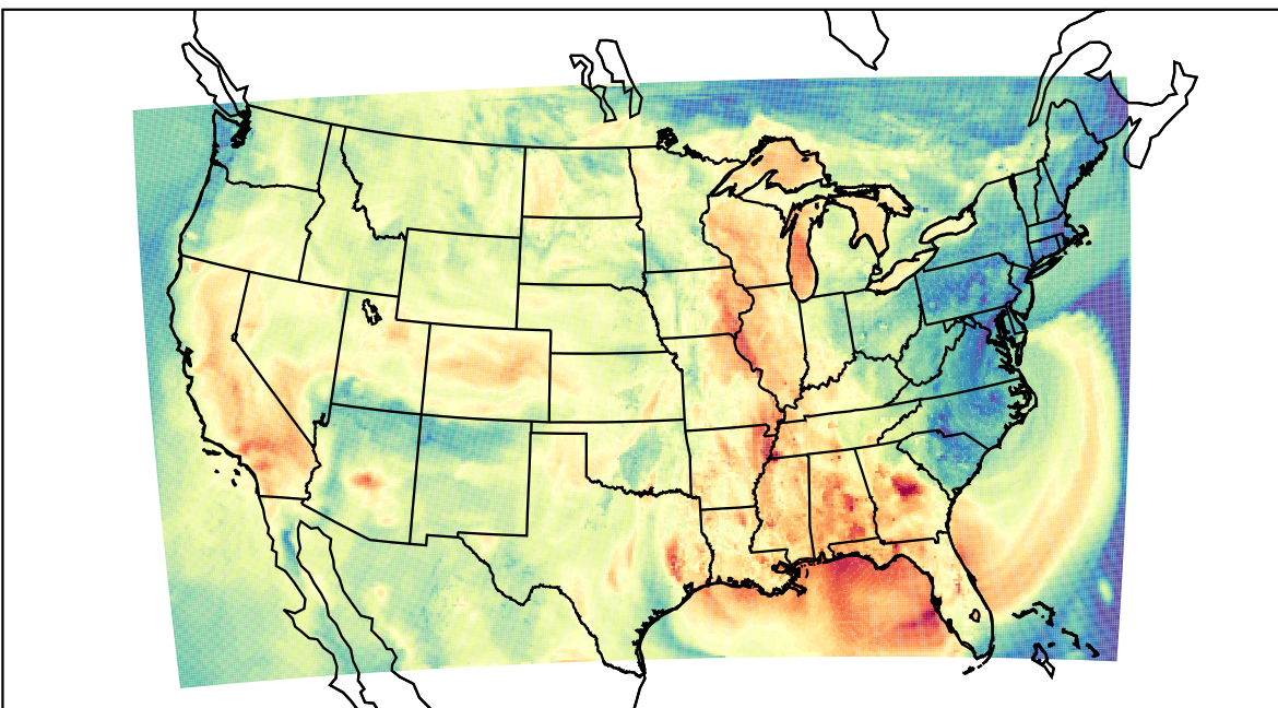
WRF (2023-09-23_23:00:00)
