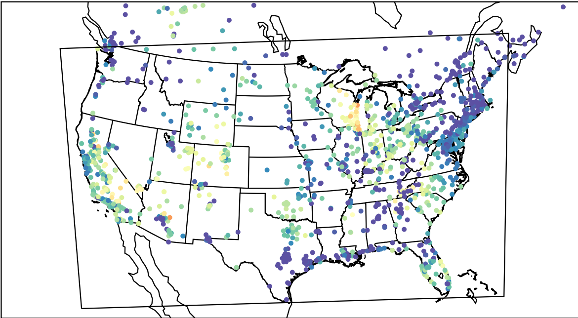
AirNOW (2023-09-23_04:00:00)
