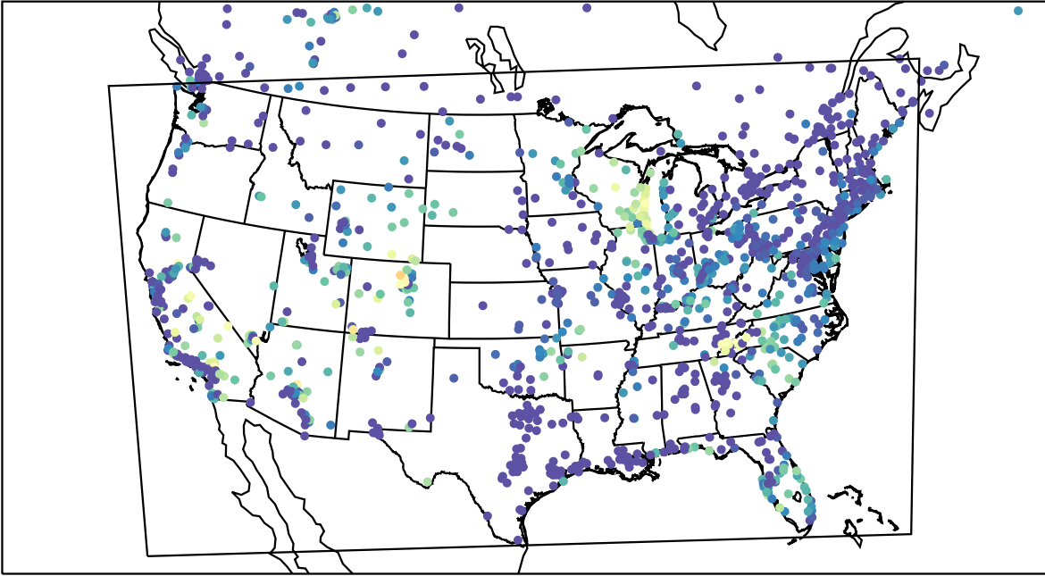
AirNOW (2023-09-23_12:00:00)
