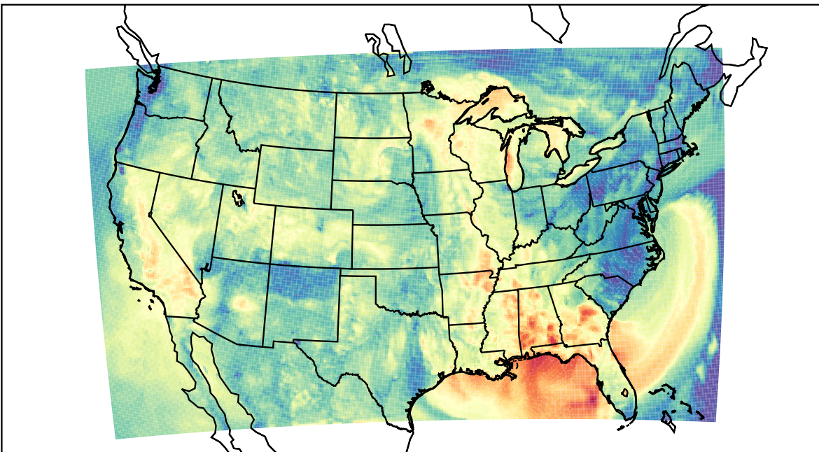
WRF (2023-09-24_02:00:00)
