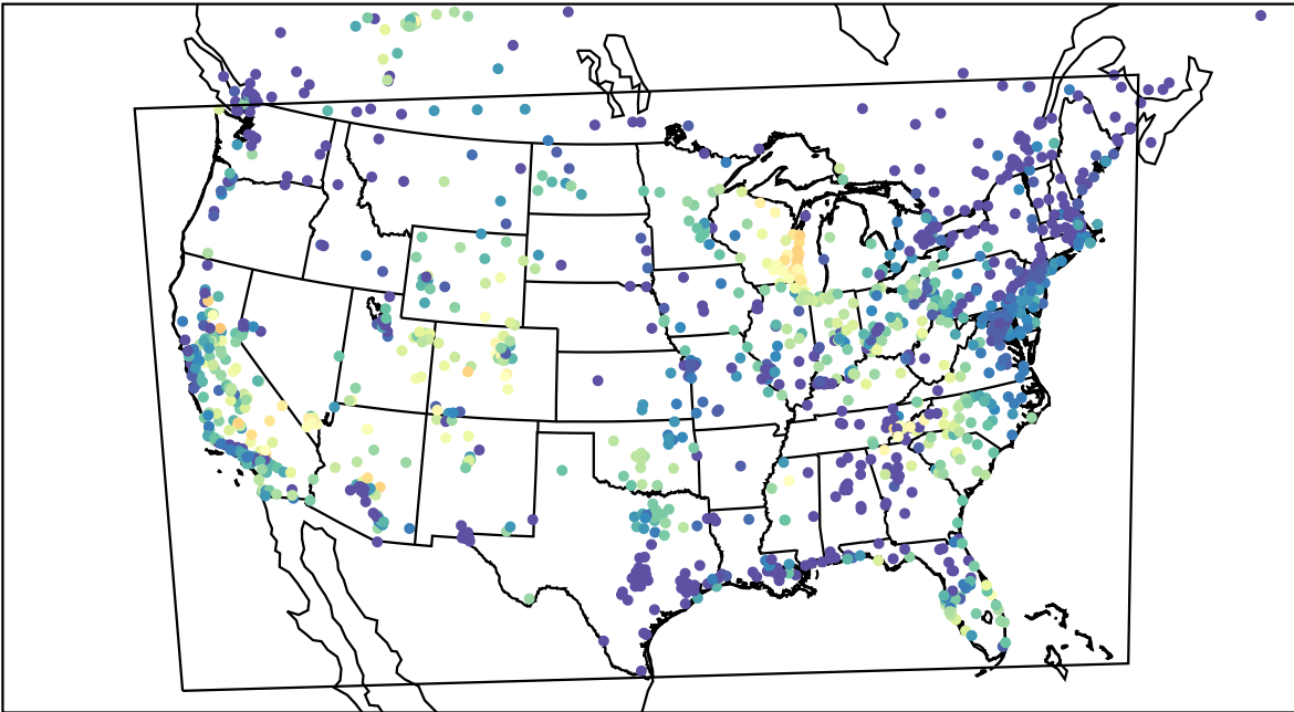
AirNOW (2023-09-23_05:00:00)
