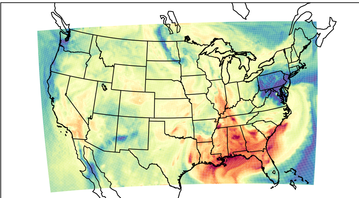
WRF (2023-09-24_19:00:00)
