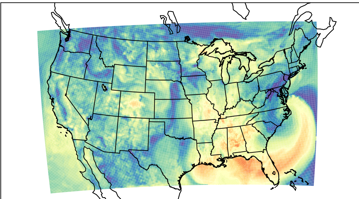
WRF (2023-09-23_15:00:00)
