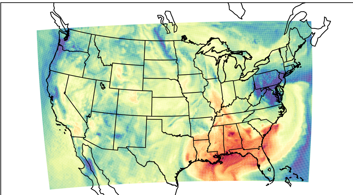
WRF (2023-09-24_17:00:00)
