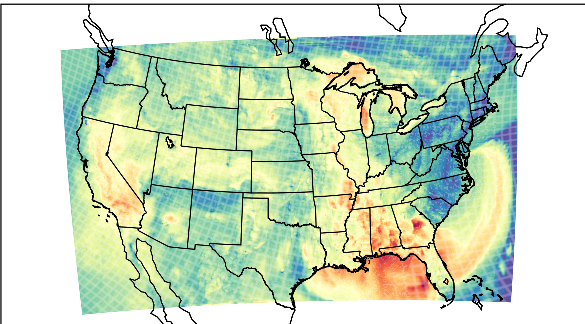
WRF (2023-09-24_01:00:00)
