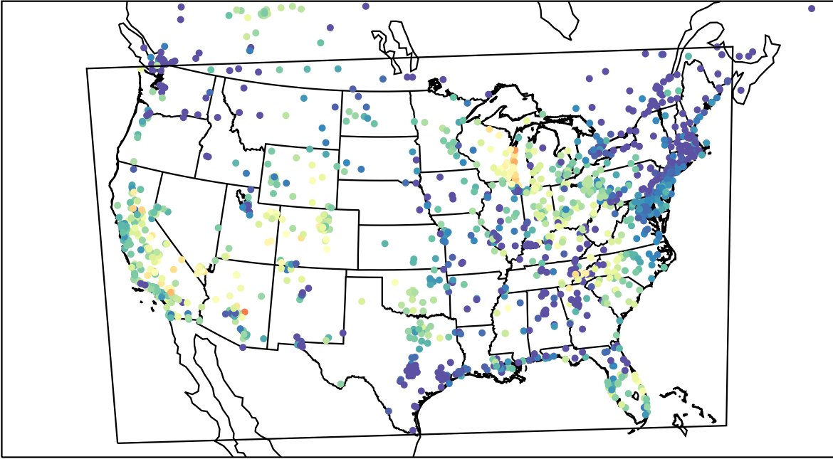
AirNOW (2023-09-23_03:00:00)
