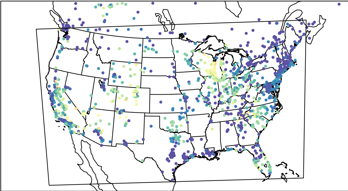
AirNOW (2023-09-23_06:00:00)
