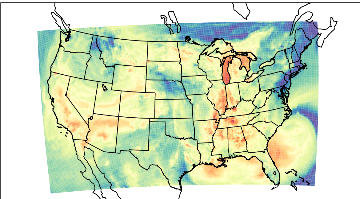
WRF (2023-09-23_00:00:00)
