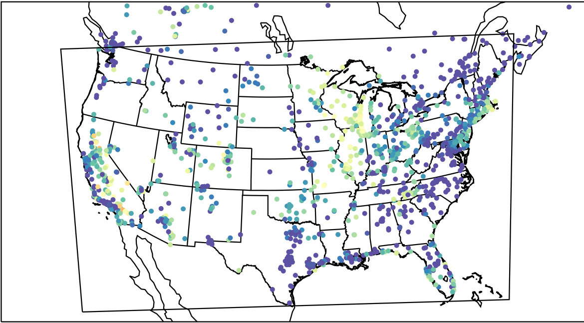
AirNOW (2023-09-24_07:00:00)
