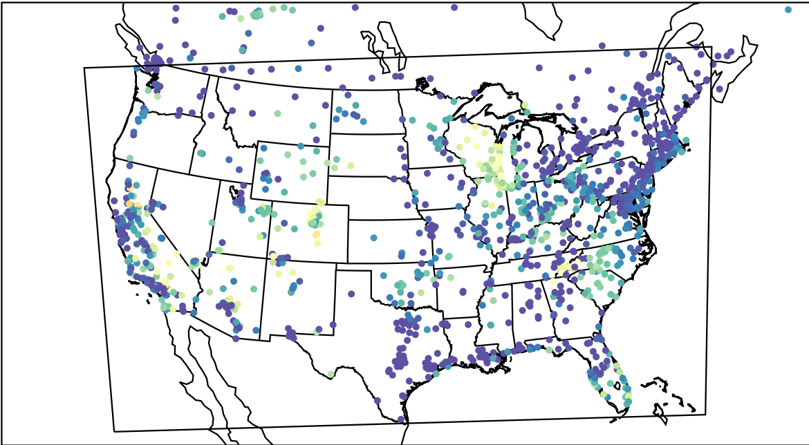
AirNOW (2023-09-23_09:00:00)
