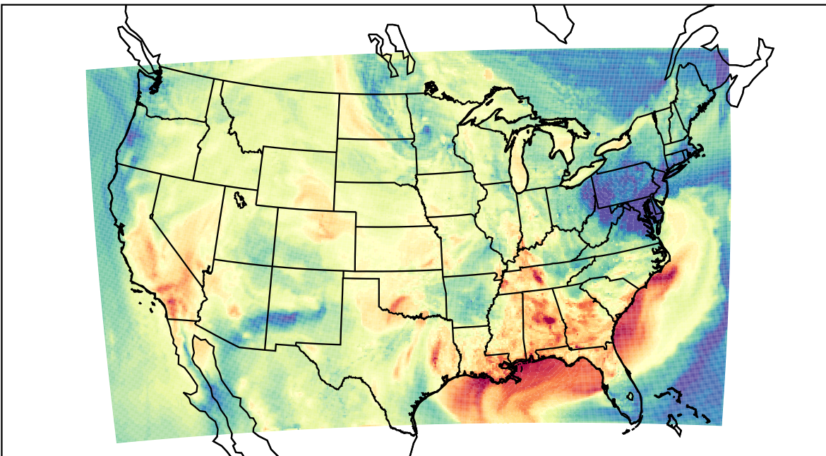
WRF (2023-09-24_23:00:00)
