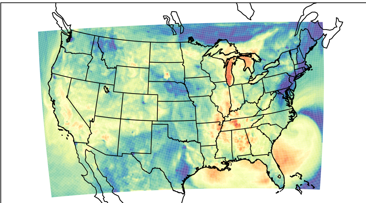
WRF (2023-09-23_02:00:00)
