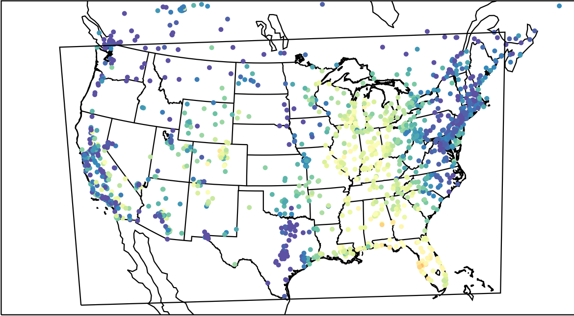
AirNOW (2023-09-23_15:00:00)
