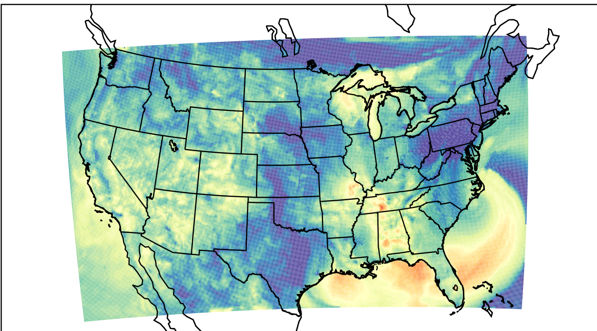
WRF (2023-09-23_10:00:00)
