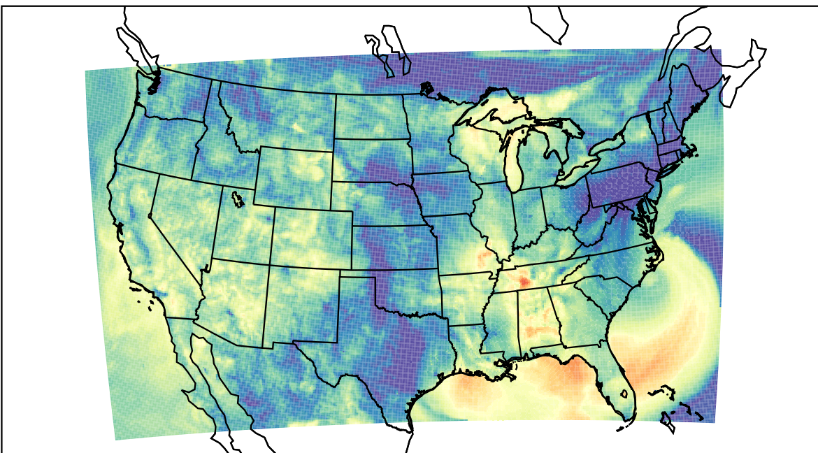
WRF (2023-09-23_09:00:00)
