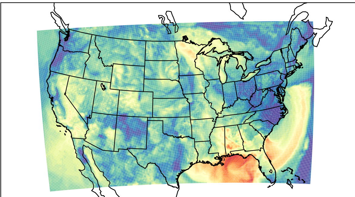
WRF (2023-09-24_07:00:00)
