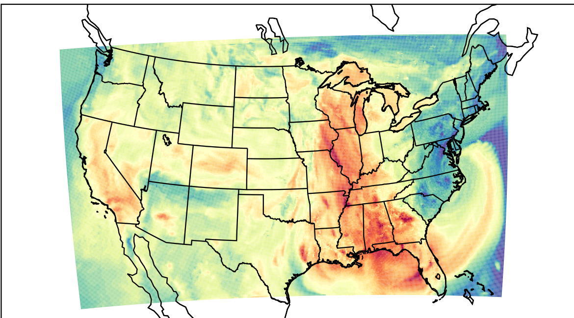
WRF (2023-09-23_22:00:00)
