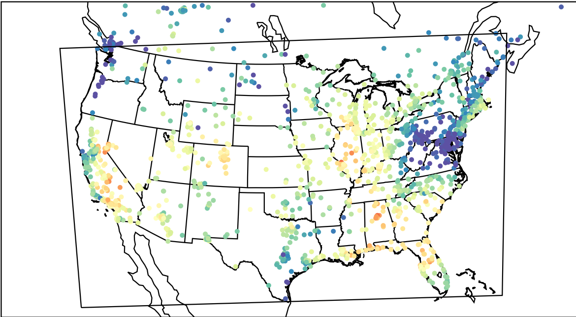
AirNOW (2023-09-24_18:00:00)
