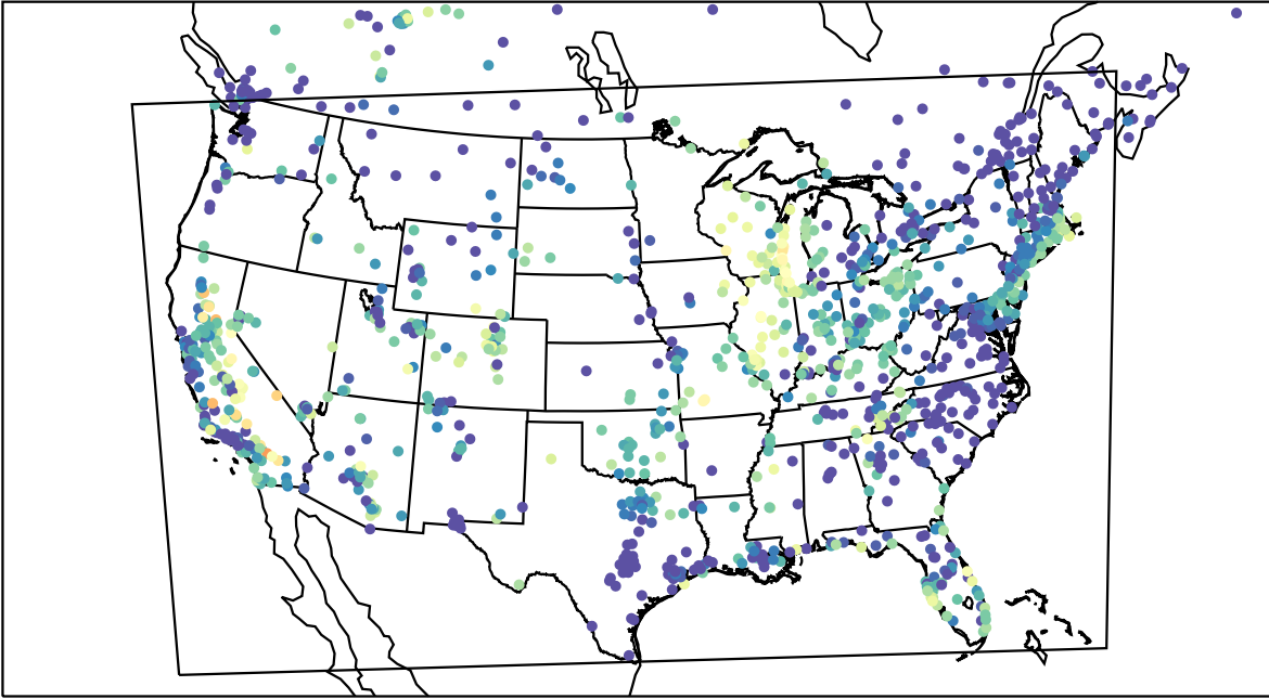
AirNOW (2023-09-24_06:00:00)
