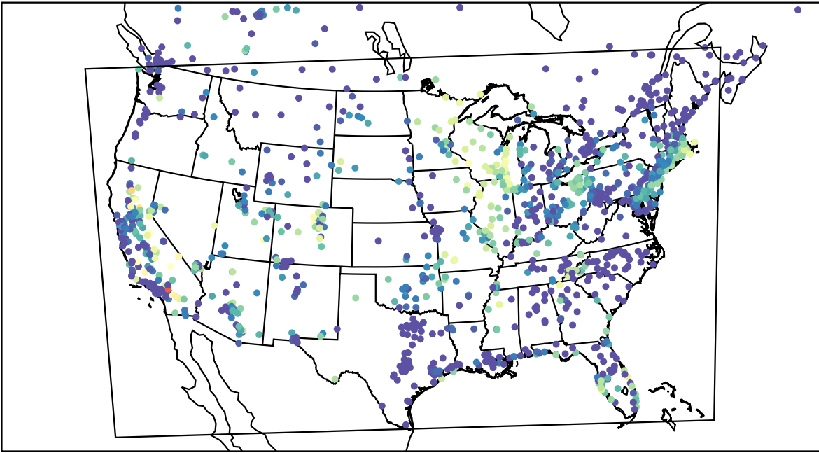
AirNOW (2023-09-24_09:00:00)
