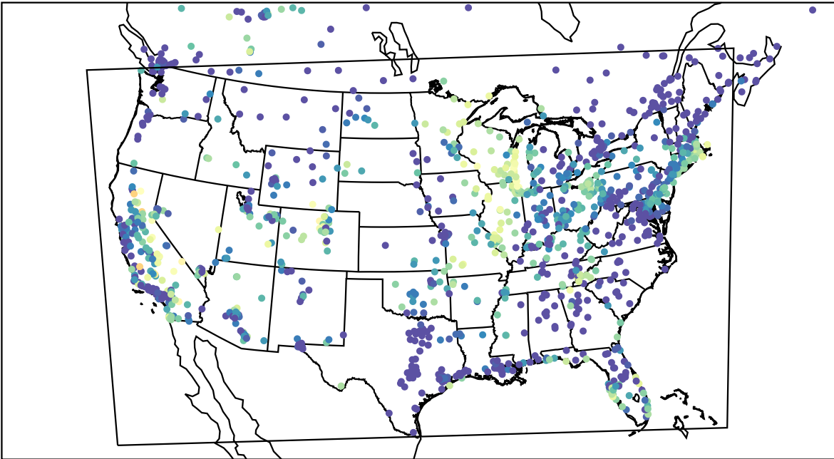
AirNOW (2023-09-24_08:00:00)
