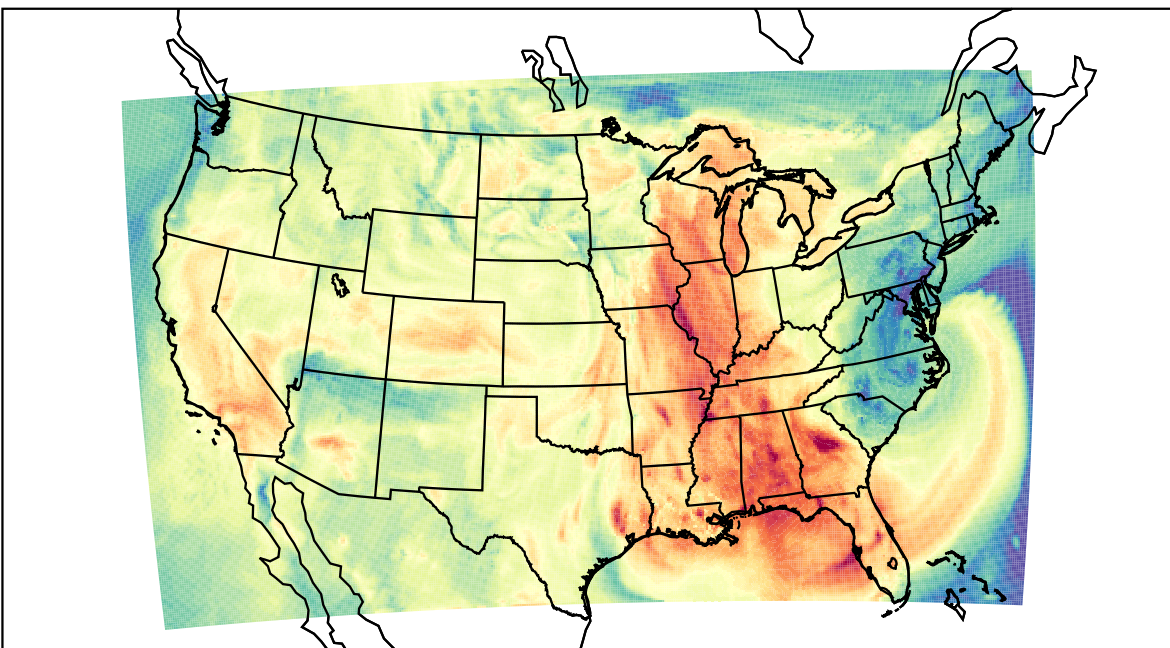
WRF (2023-09-23_21:00:00)
