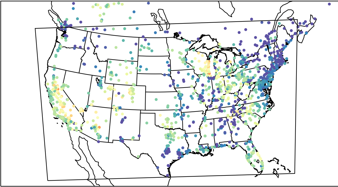
AirNOW (2023-09-23_02:00:00)
