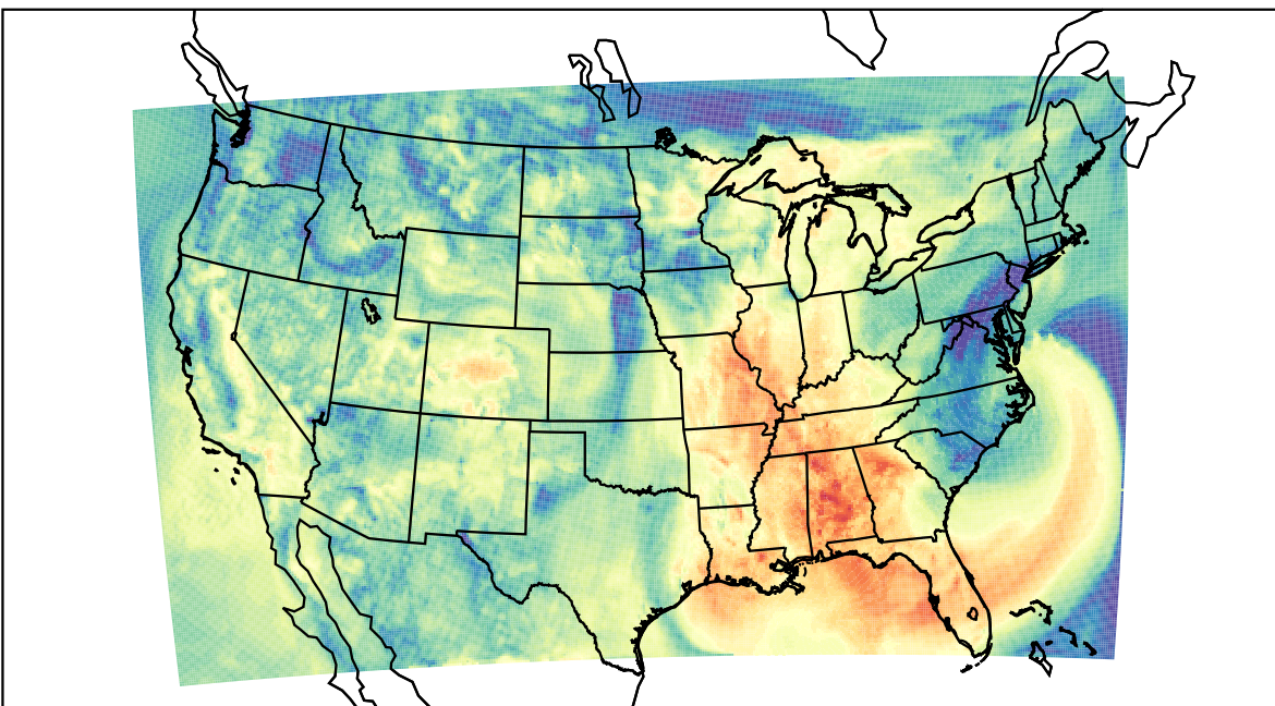
WRF (2023-09-23_16:00:00)
