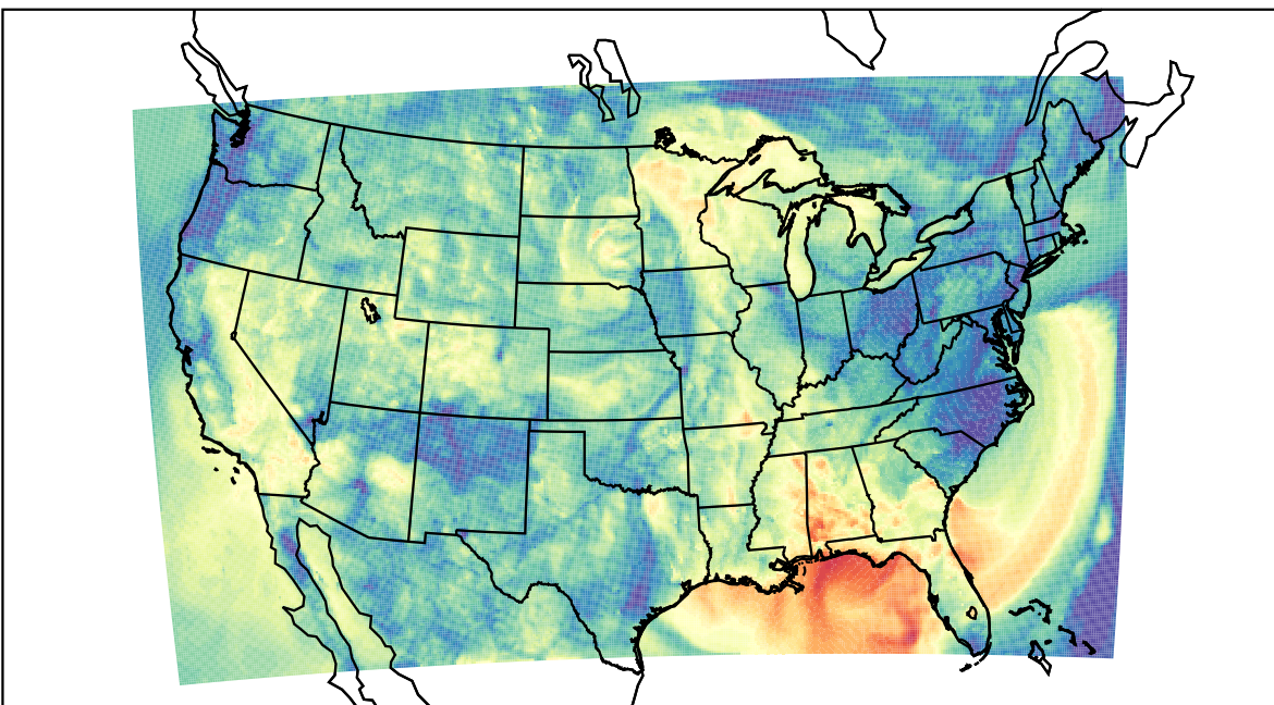
WRF (2023-09-24_05:00:00)
