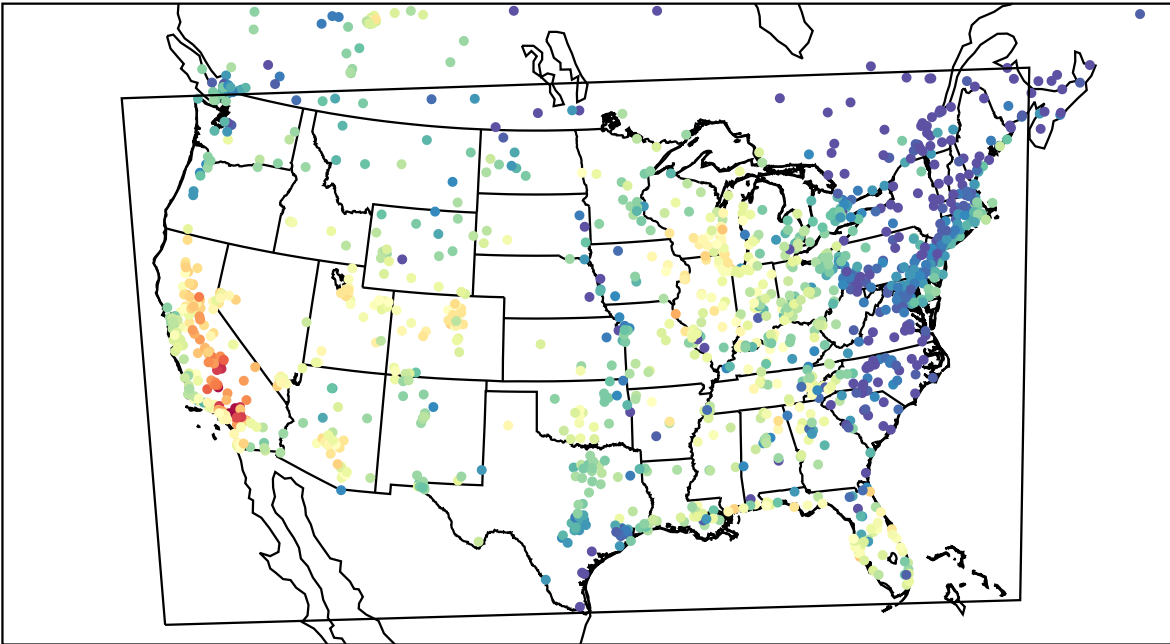
AirNOW (2023-09-24_00:00:00)
