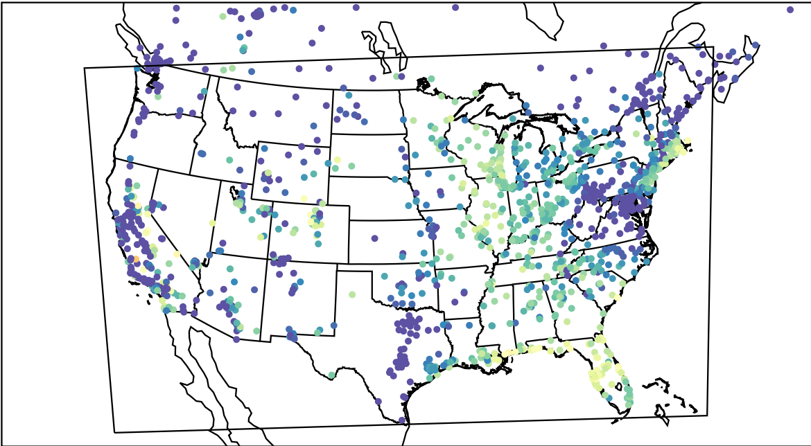
AirNOW (2023-09-24_14:00:00)
