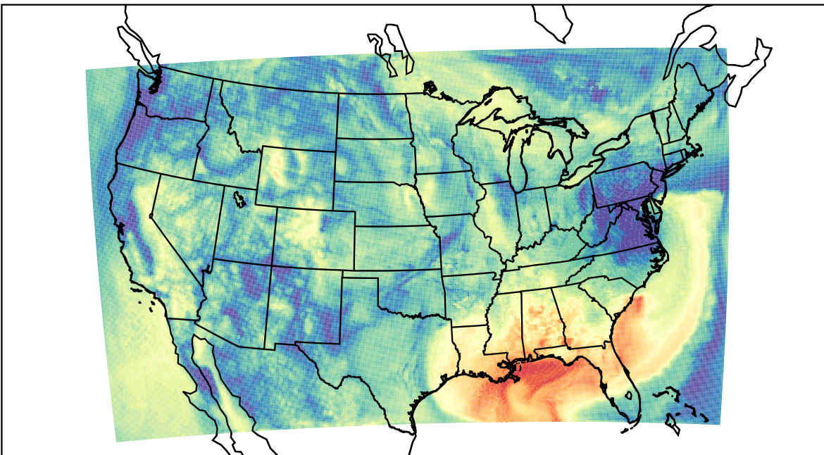
WRF (2023-09-24_15:00:00)
