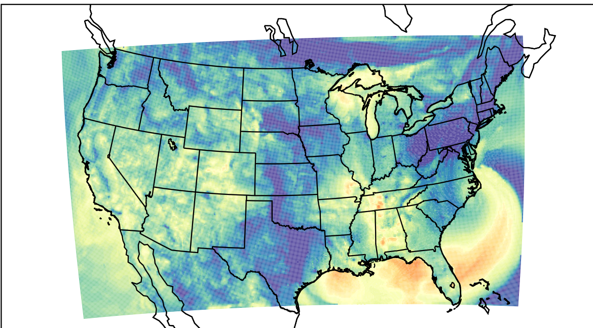
WRF (2023-09-23_11:00:00)
