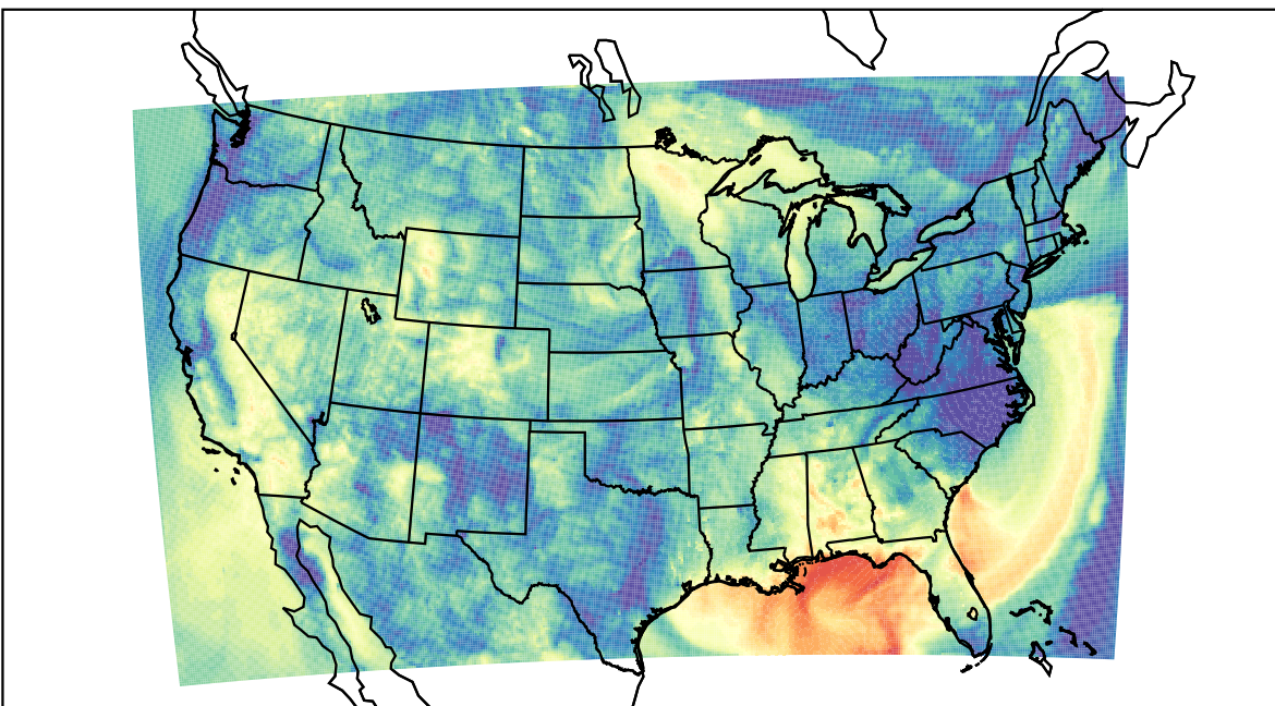
WRF (2023-09-24_09:00:00)
