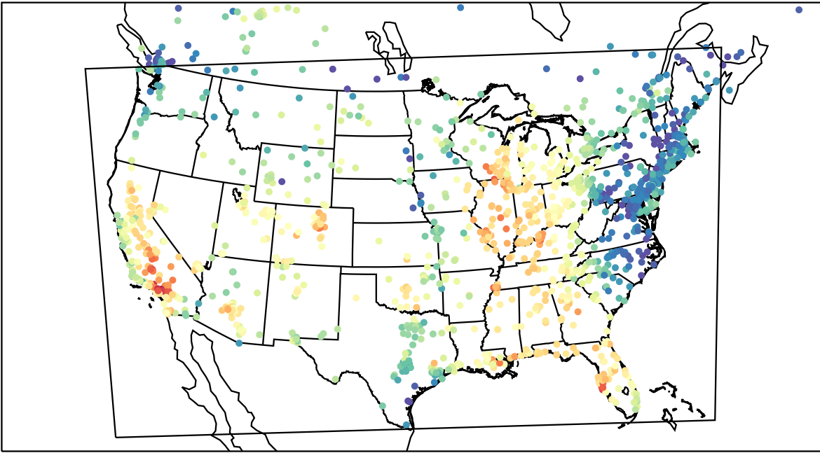
AirNOW (2023-09-23_20:00:00)
