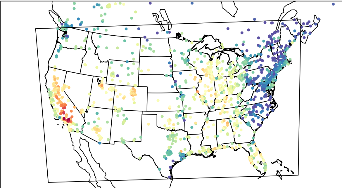
AirNOW (2023-09-23_23:00:00)
