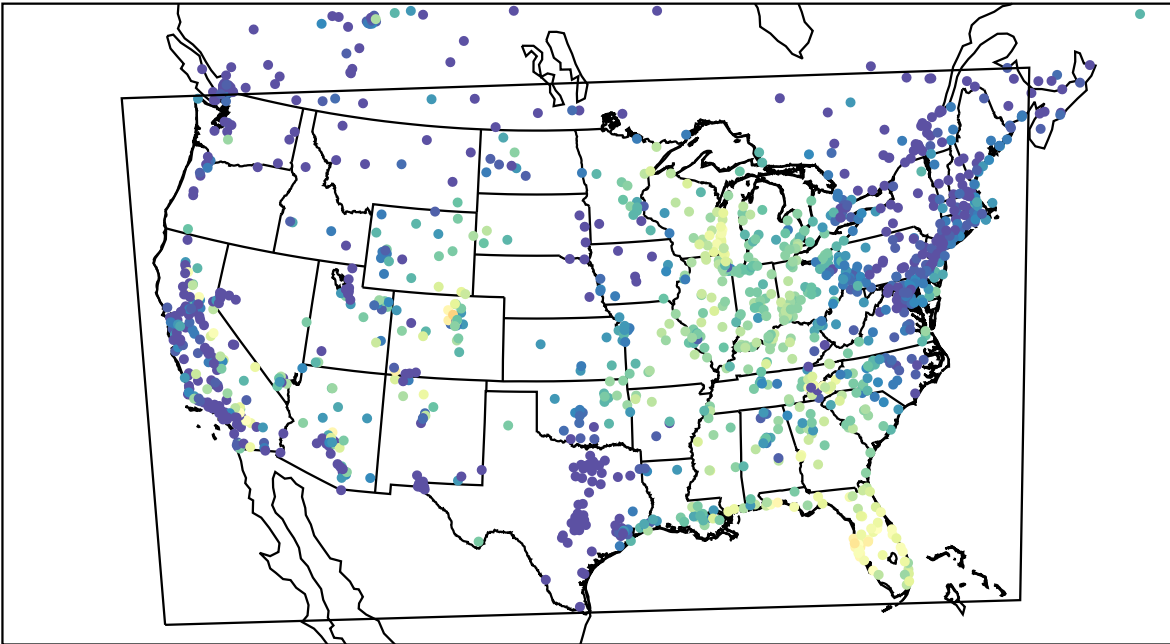
AirNOW (2023-09-23_14:00:00)
