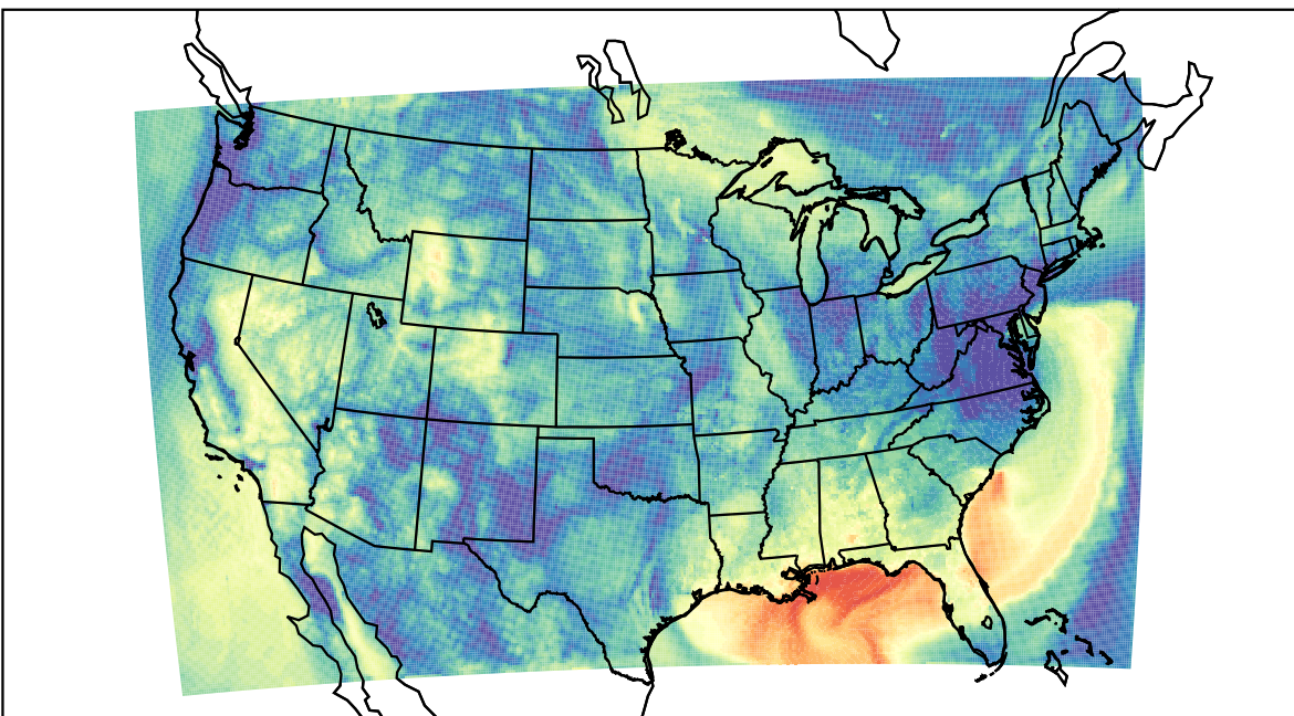
WRF (2023-09-24_14:00:00)
