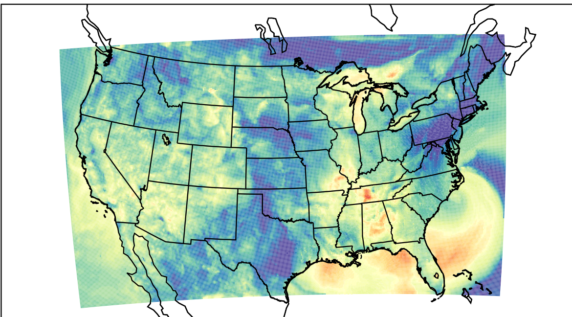
WRF (2023-09-23_07:00:00)
