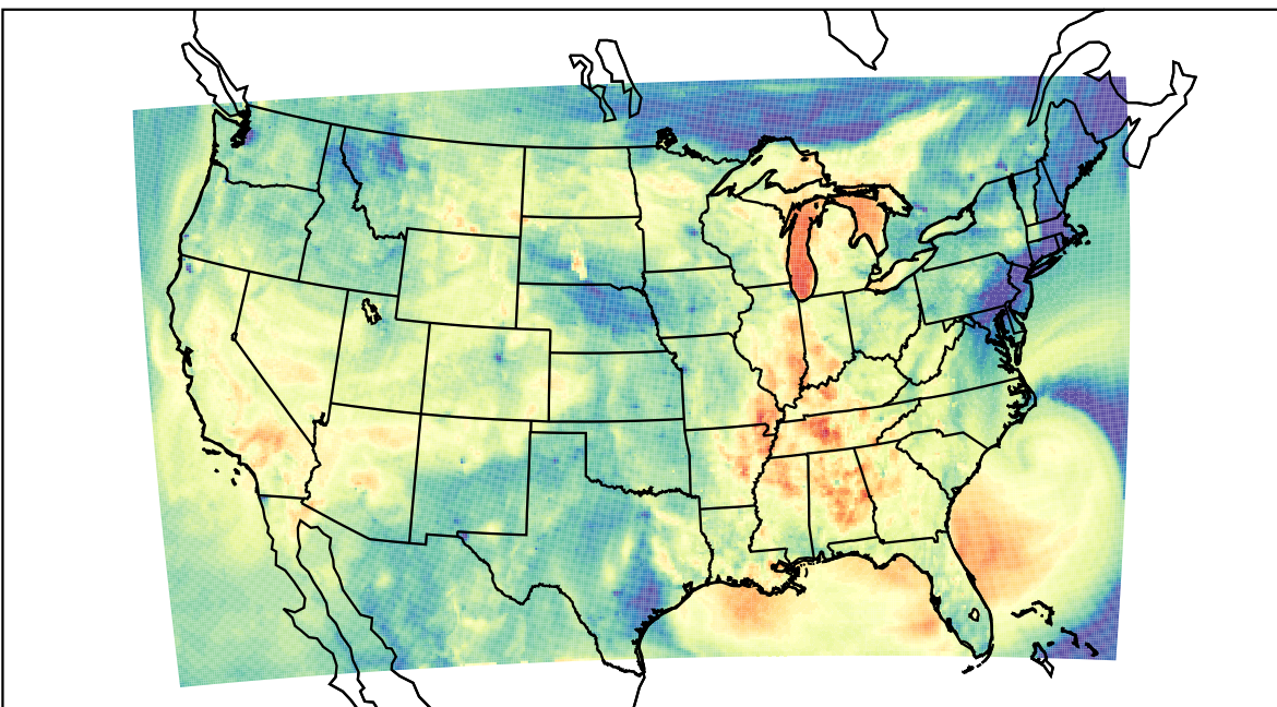
WRF (2023-09-23_01:00:00)
