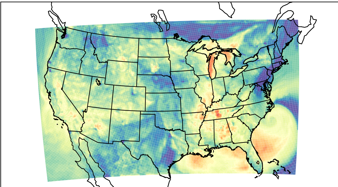
WRF (2023-09-23_03:00:00)
