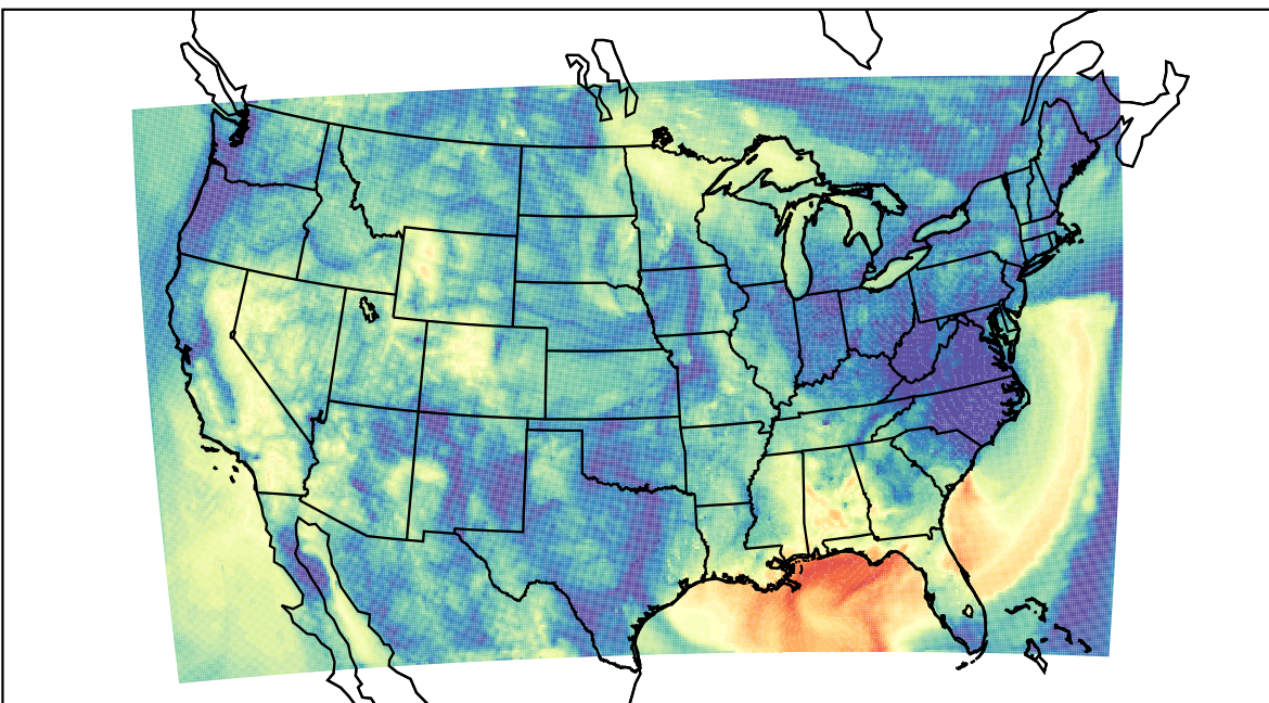
WRF (2023-09-24_11:00:00)
