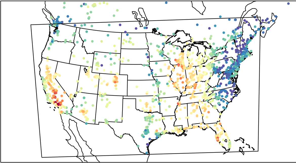
AirNOW (2023-09-23_21:00:00)
