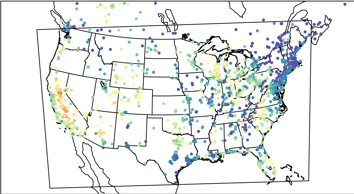
AirNOW (2023-09-23_01:00:00)
