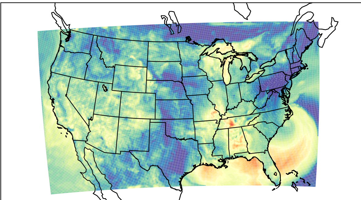
WRF (2023-09-23_08:00:00)
