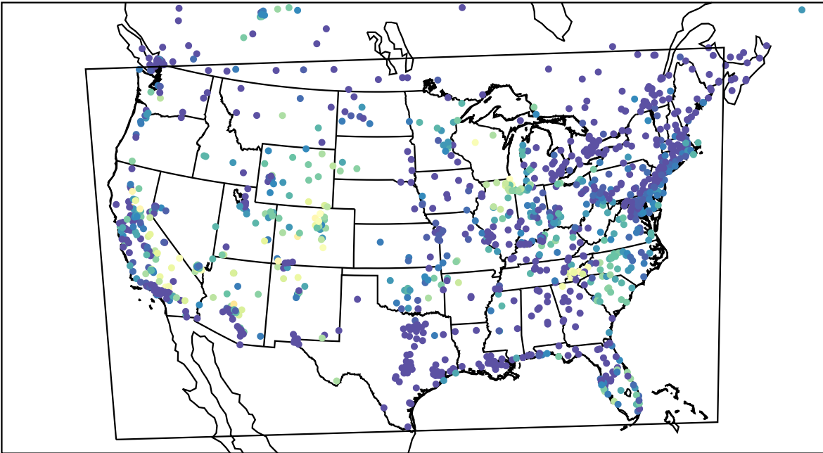
AirNOW (2023-09-23_10:00:00)
