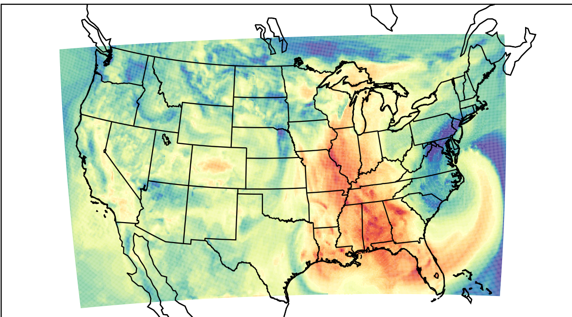
WRF (2023-09-23_17:00:00)
