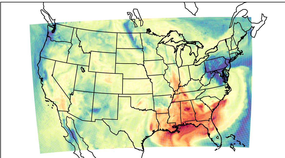
WRF (2023-09-24_18:00:00)
