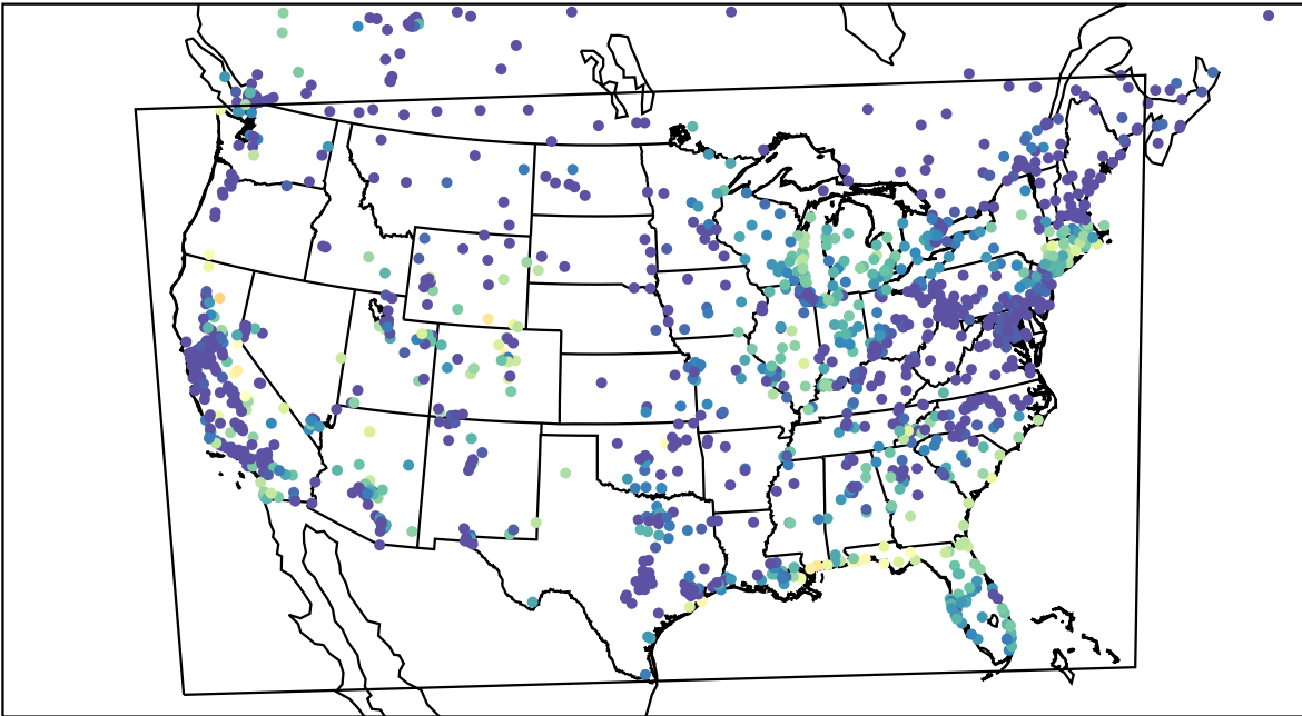
AirNOW (2023-09-25_14:00:00)
