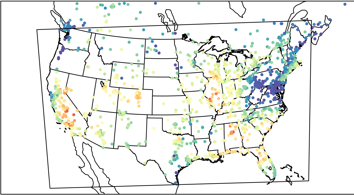
AirNOW (2023-09-24_19:00:00)
