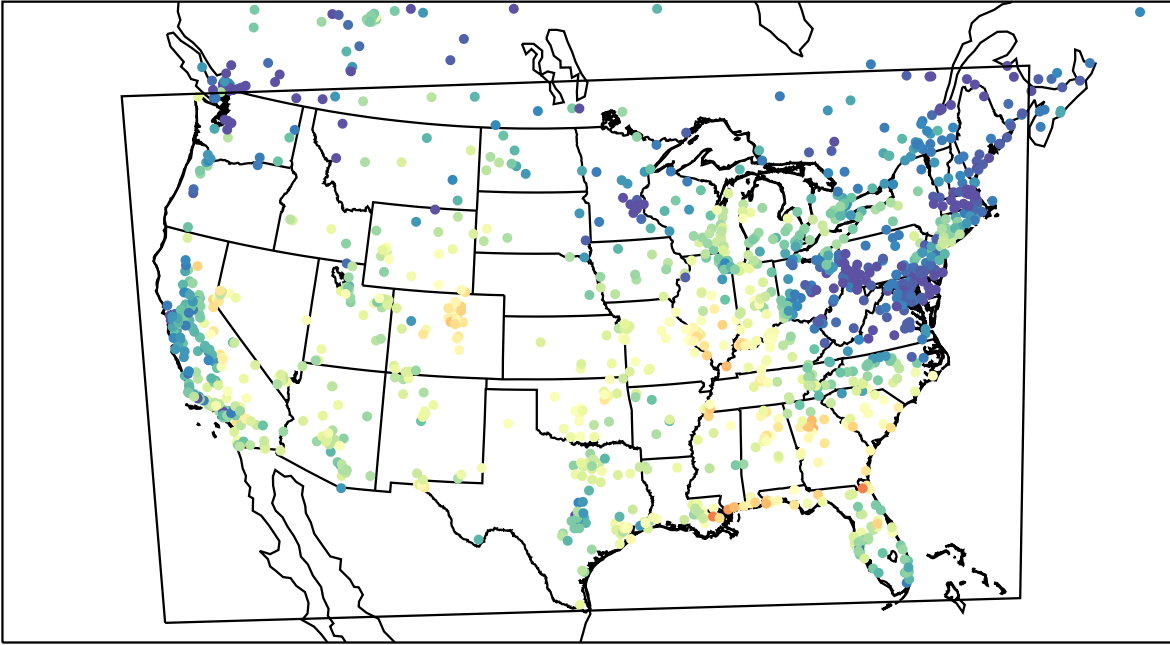
AirNOW (2023-09-25_17:00:00)
