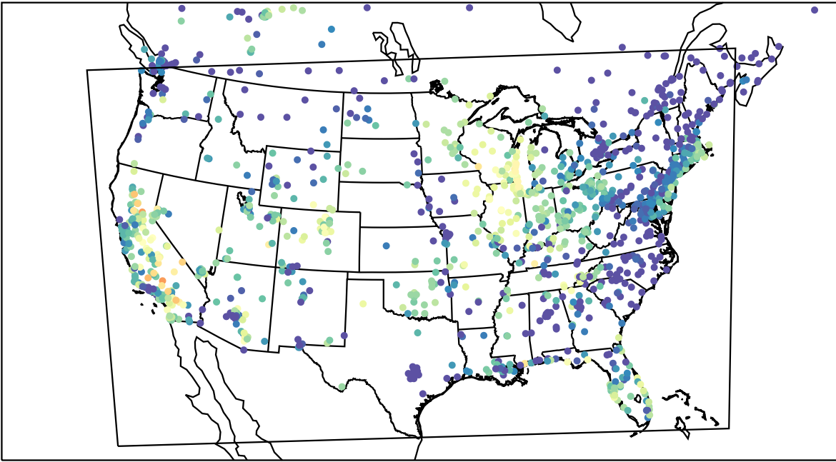
AirNOW (2023-09-24_04:00:00)
