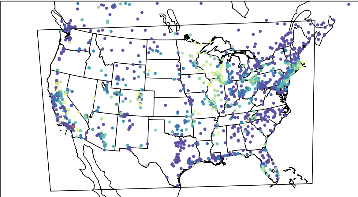
AirNOW (2023-09-24_09:00:00)
