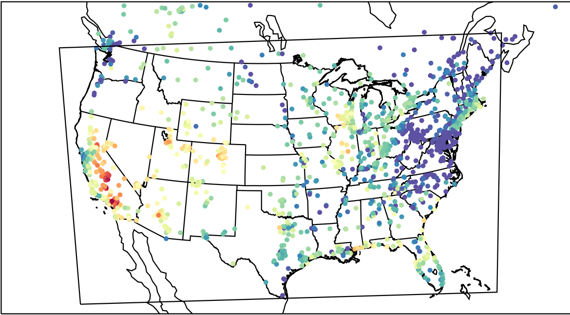
AirNOW (2023-09-25_00:00:00)
