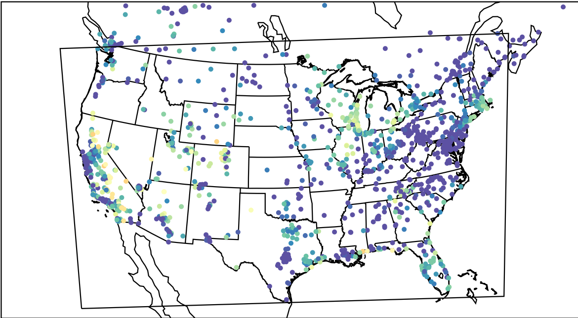
AirNOW (2023-09-25_05:00:00)
