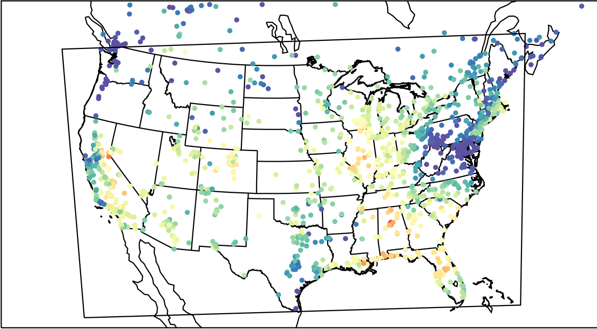
AirNOW (2023-09-24_17:00:00)
