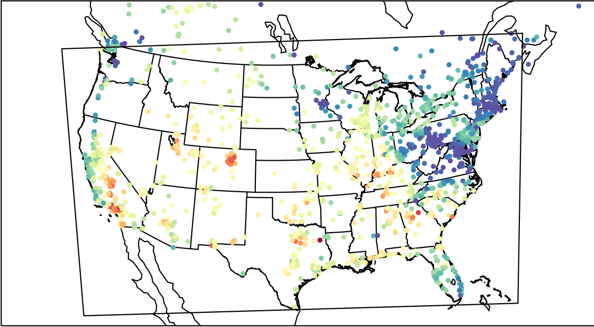
AirNOW (2023-09-25_21:00:00)
