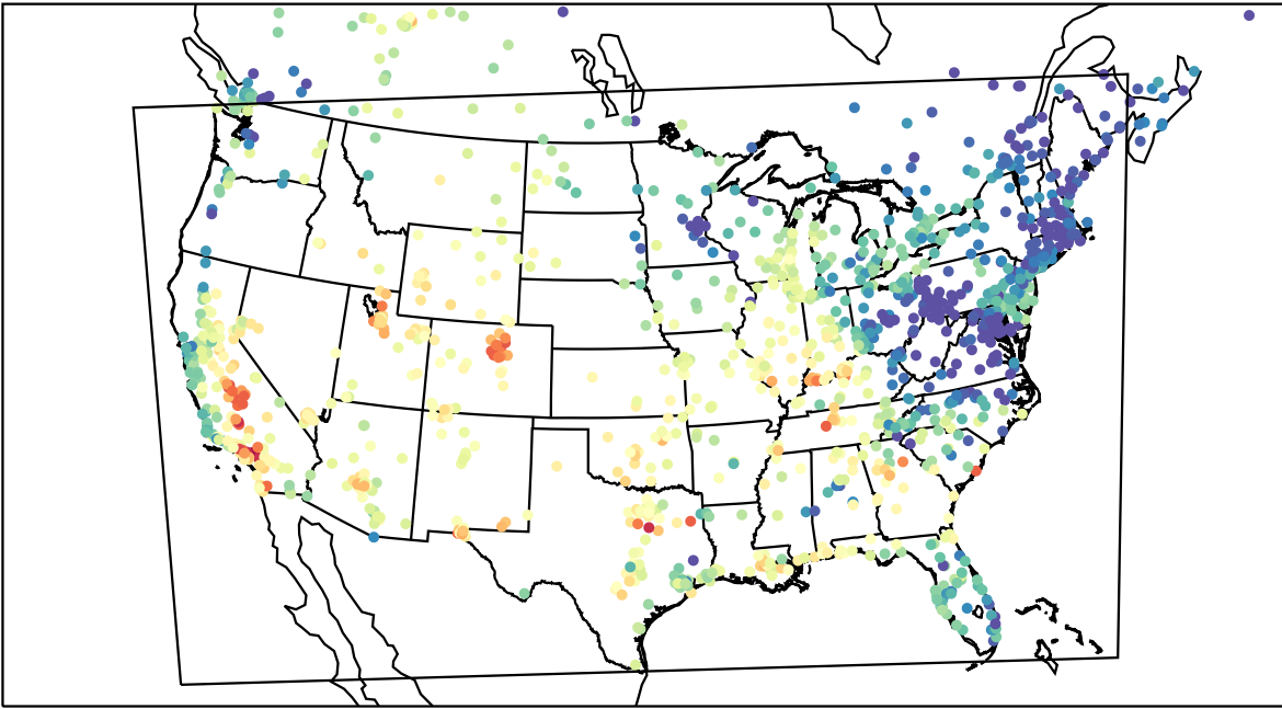
AirNOW (2023-09-25_22:00:00)
