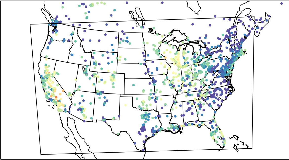
AirNOW (2023-09-24_03:00:00)
