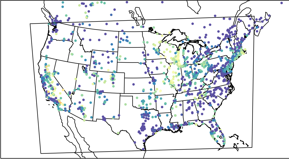
AirNOW (2023-09-24_07:00:00)
