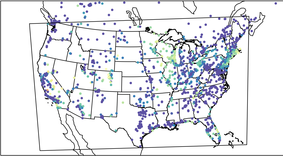
AirNOW (2023-09-24_12:00:00)
