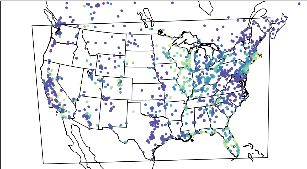
AirNOW (2023-09-24_13:00:00)
