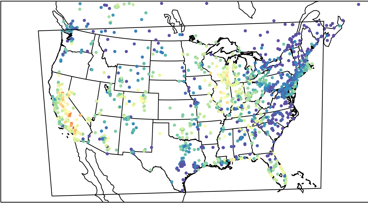
AirNOW (2023-09-24_02:00:00)
