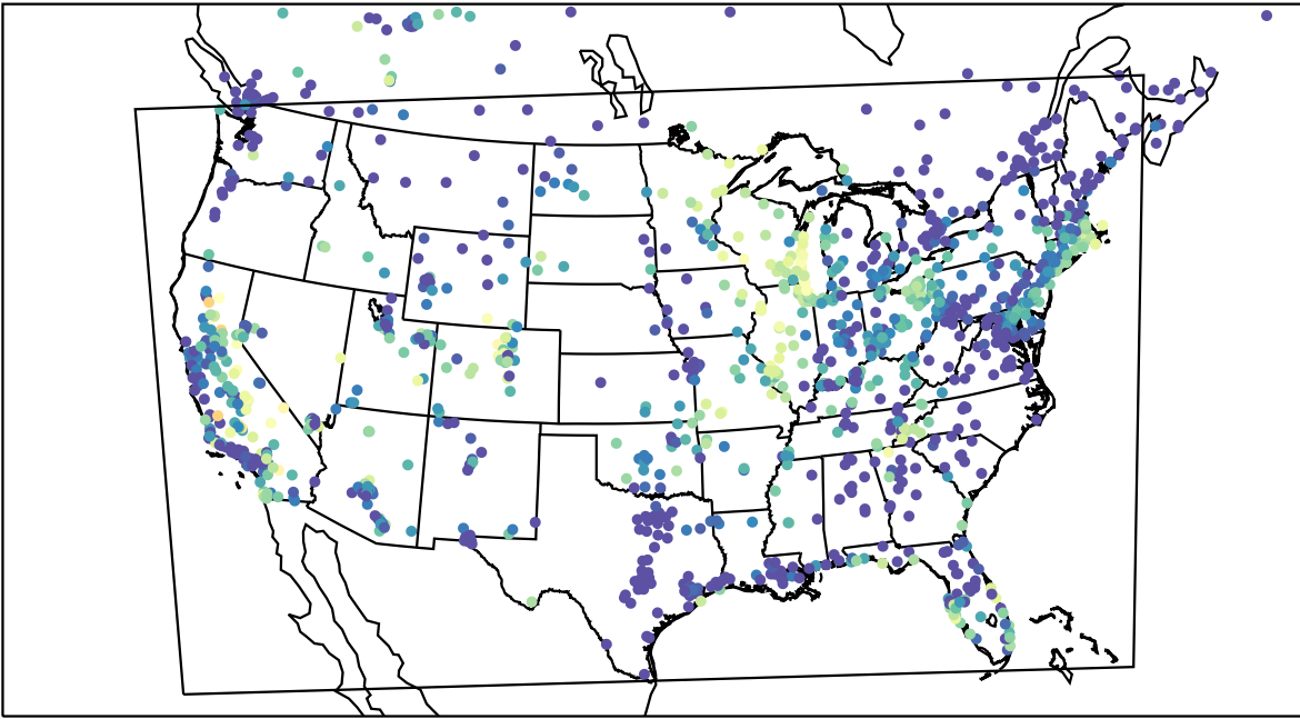
AirNOW (2023-09-24_08:00:00)
