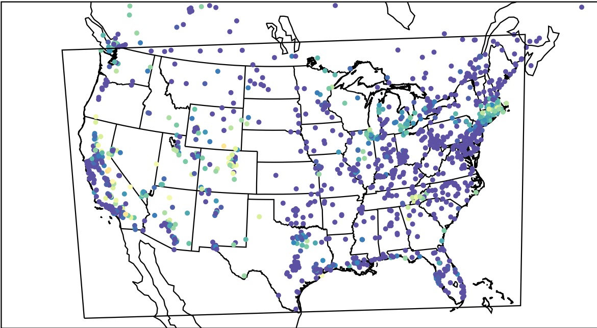
AirNOW (2023-09-25_10:00:00)
