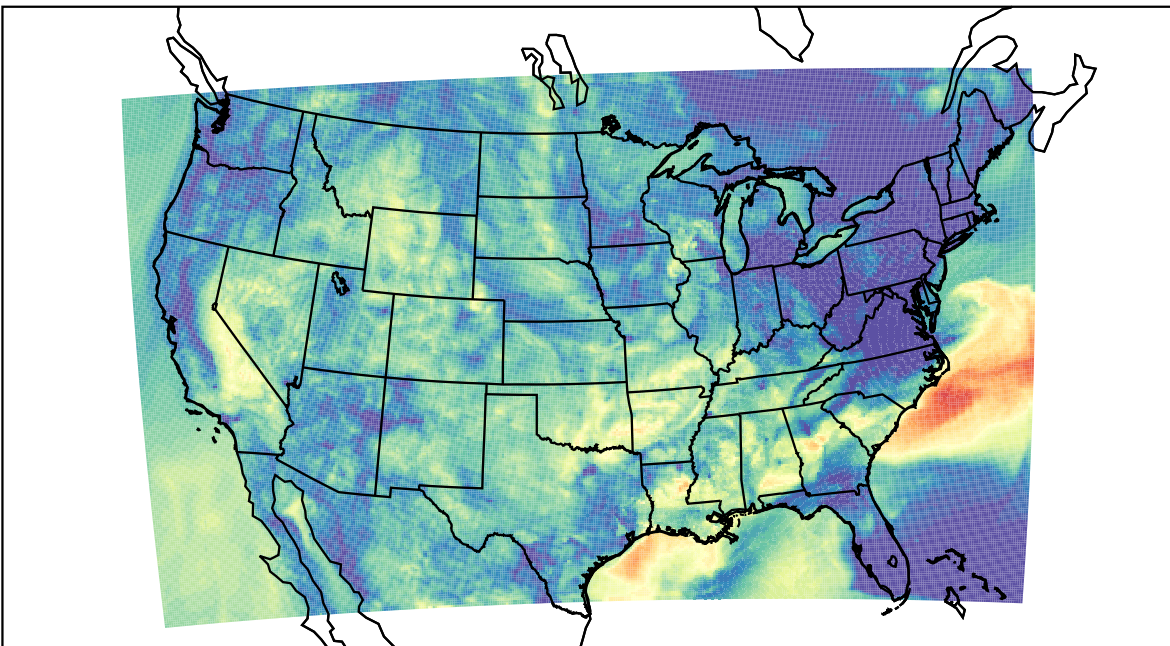
WRF (2023-09-26_11:00:00)
