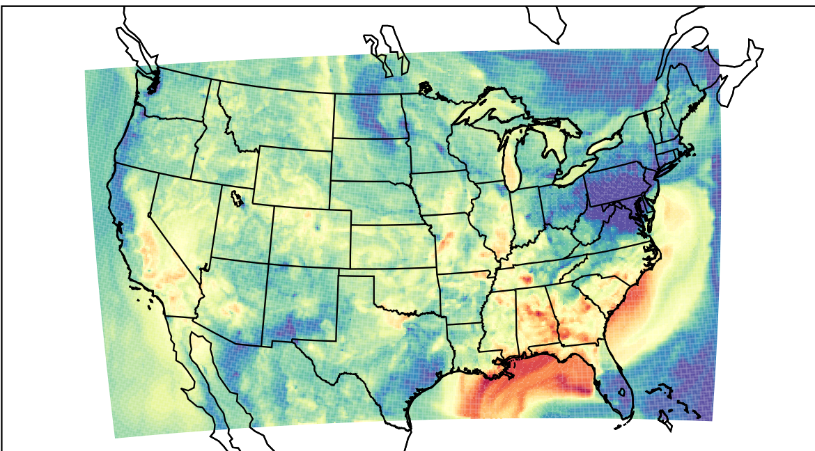
WRF (2023-09-25_02:00:00)
