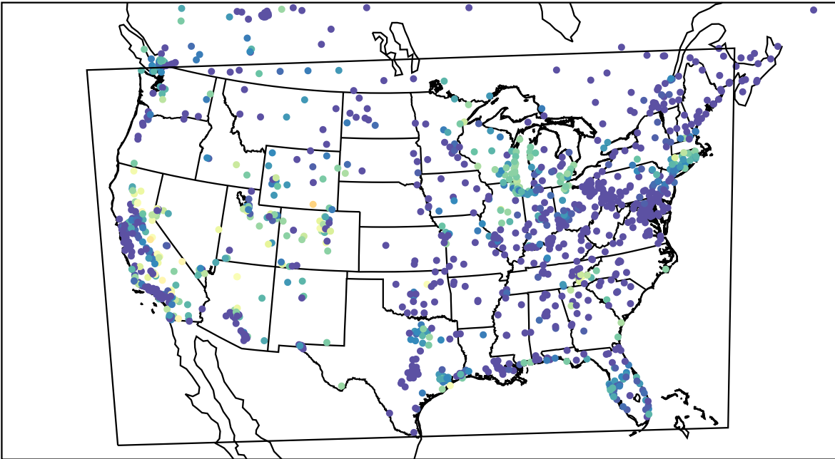
AirNOW (2023-09-25_08:00:00)
