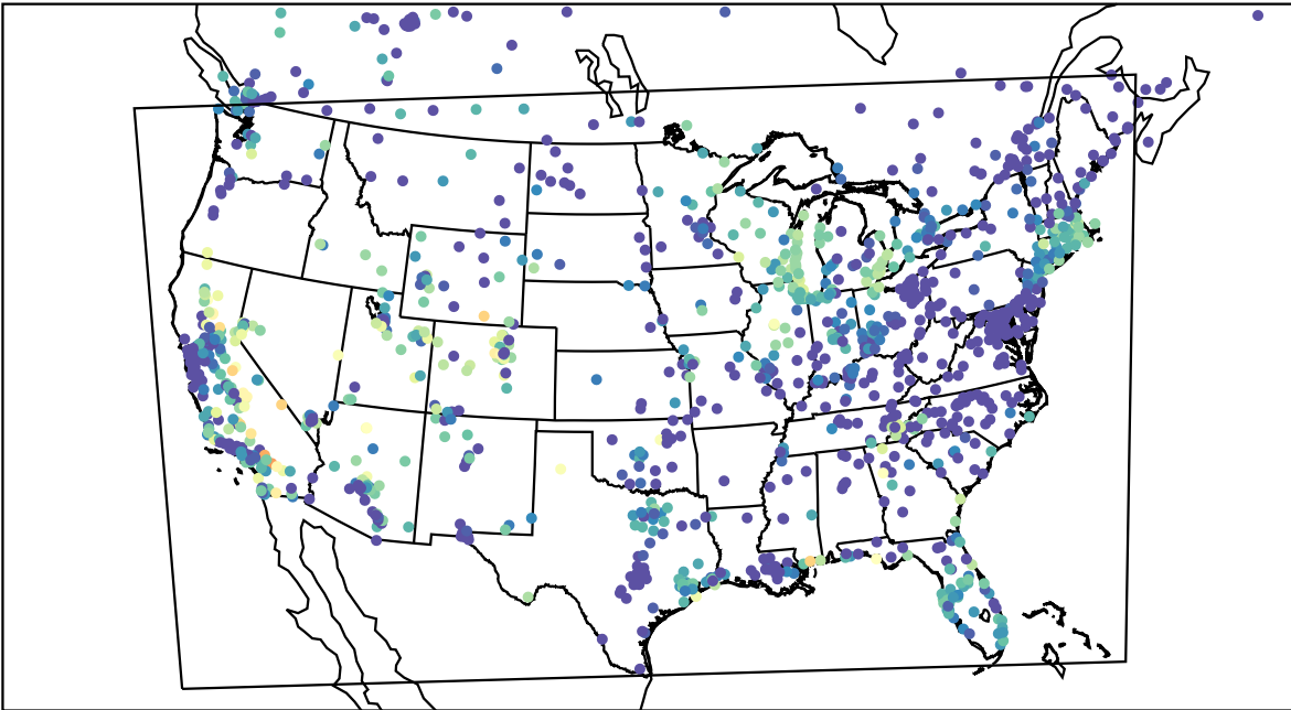
AirNOW (2023-09-25_06:00:00)
