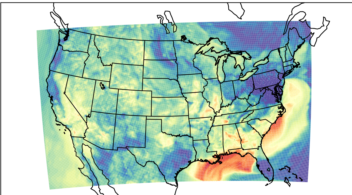
WRF (2023-09-25_05:00:00)
