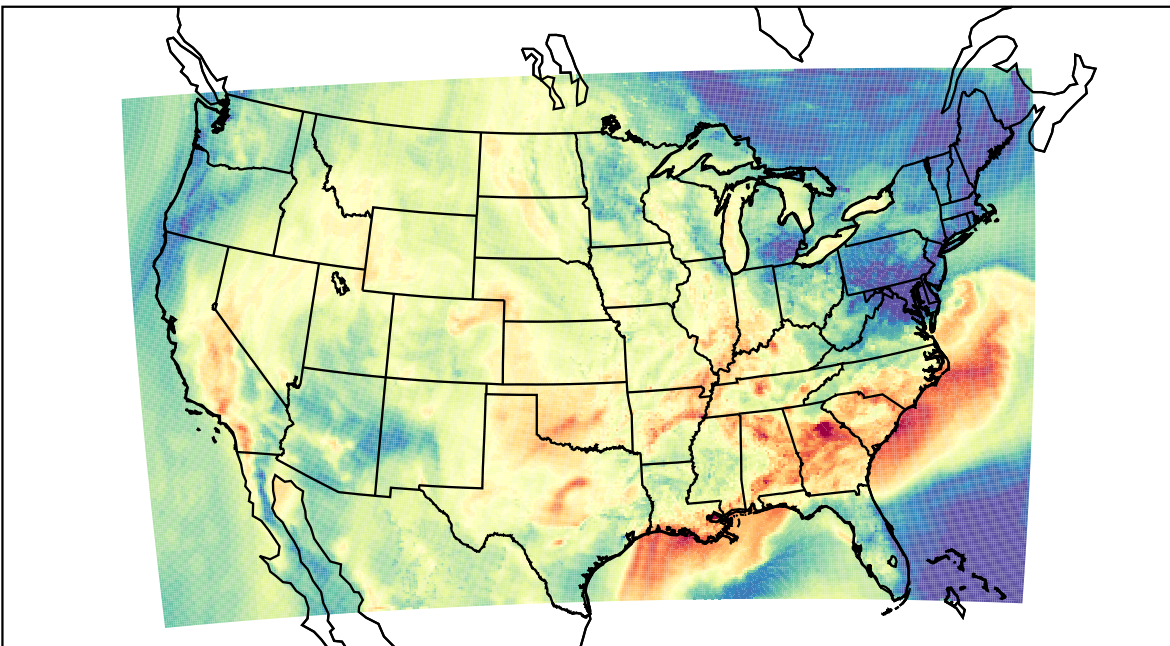
WRF (2023-09-25_23:00:00)
