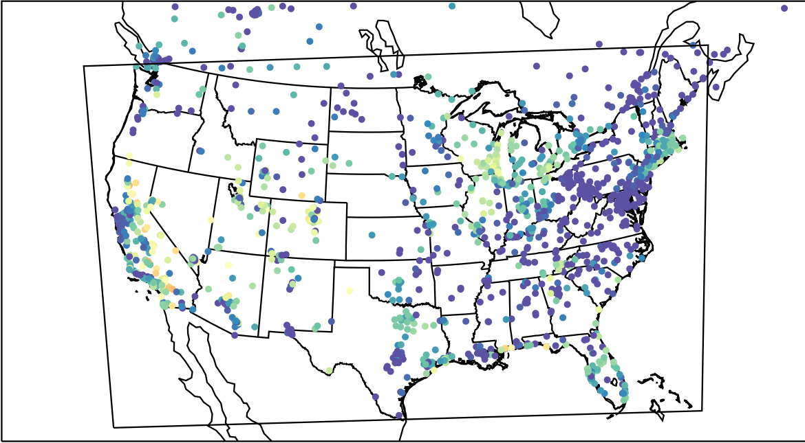
AirNOW (2023-09-25_04:00:00)
