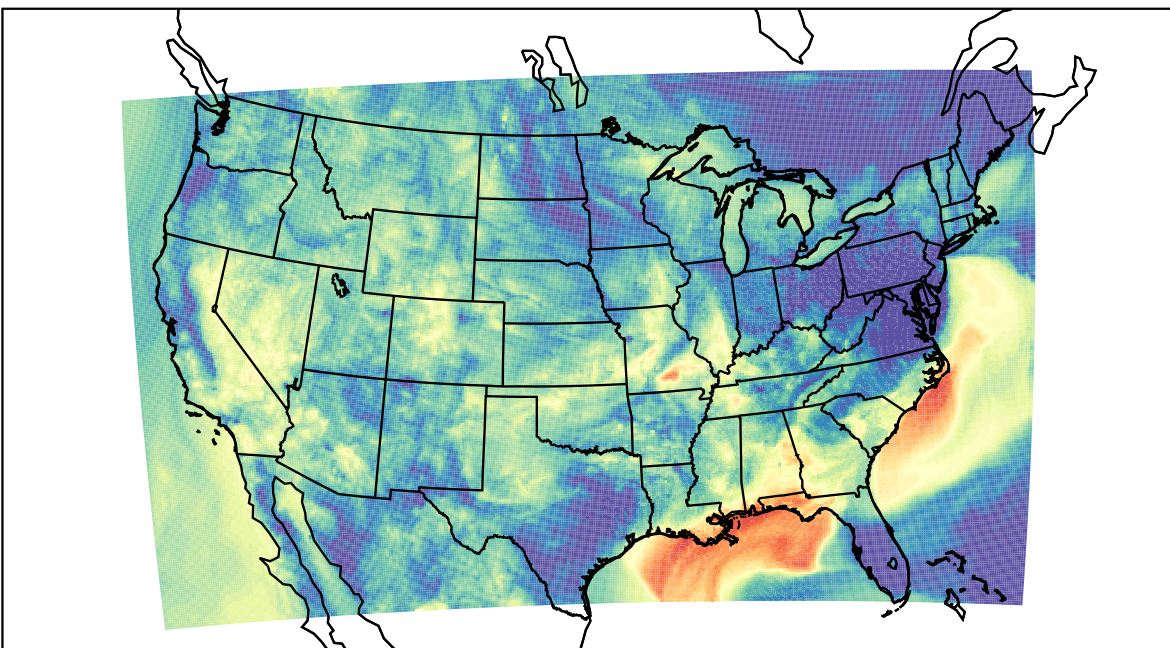
WRF (2023-09-25_09:00:00)
