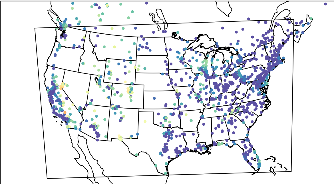
AirNOW (2023-09-26_07:00:00)
