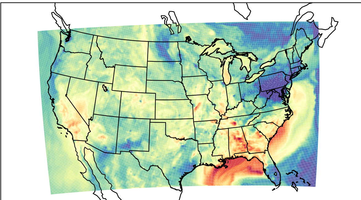
WRF (2023-09-25_01:00:00)
