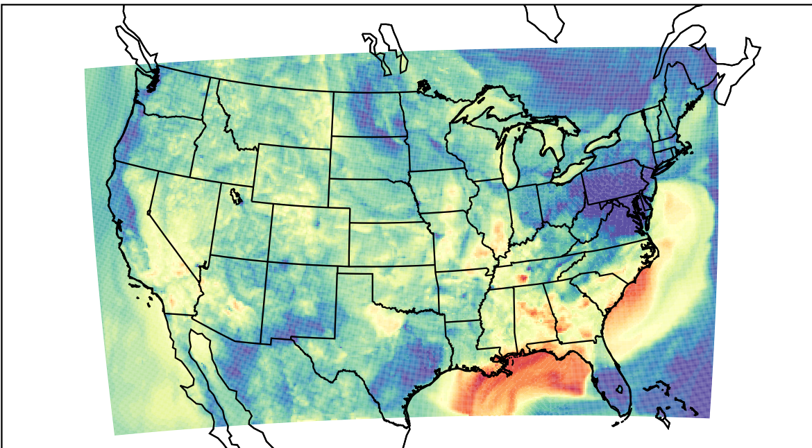
WRF (2023-09-25_04:00:00)
