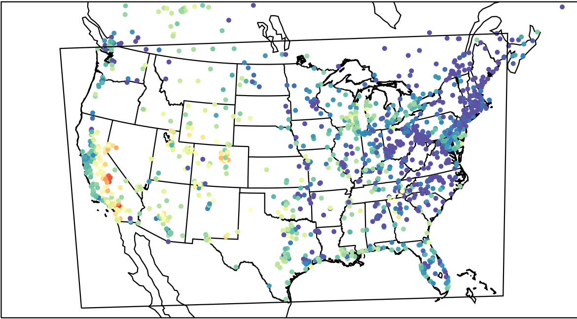
AirNOW (2023-09-26_01:00:00)
