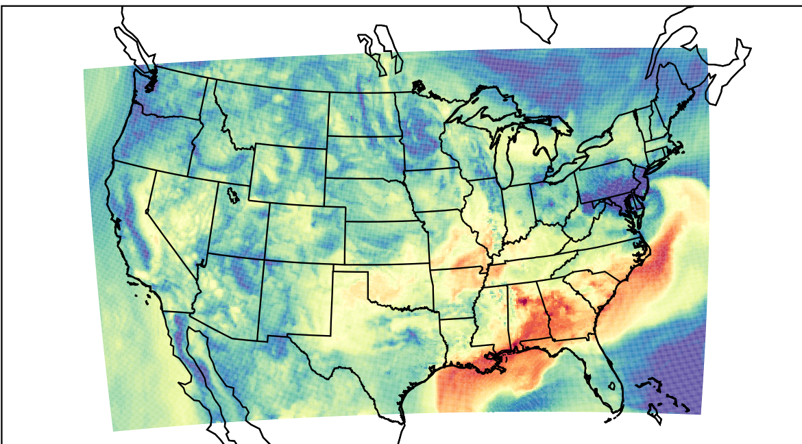
WRF (2023-09-25_16:00:00)
