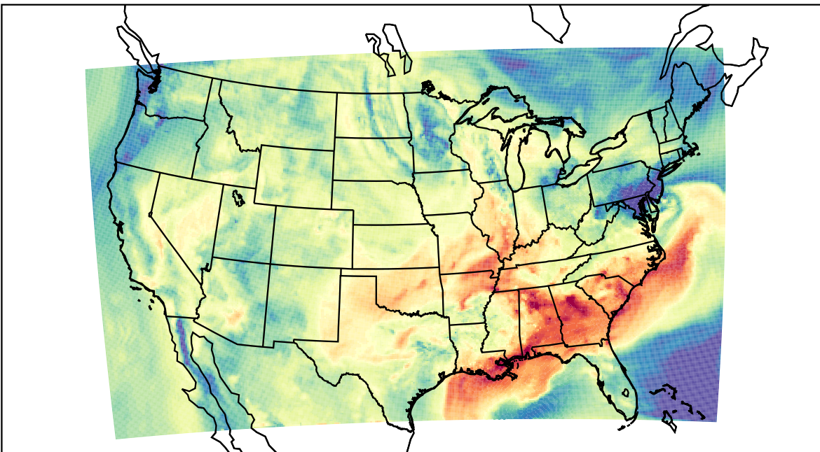
WRF (2023-09-25_18:00:00)
