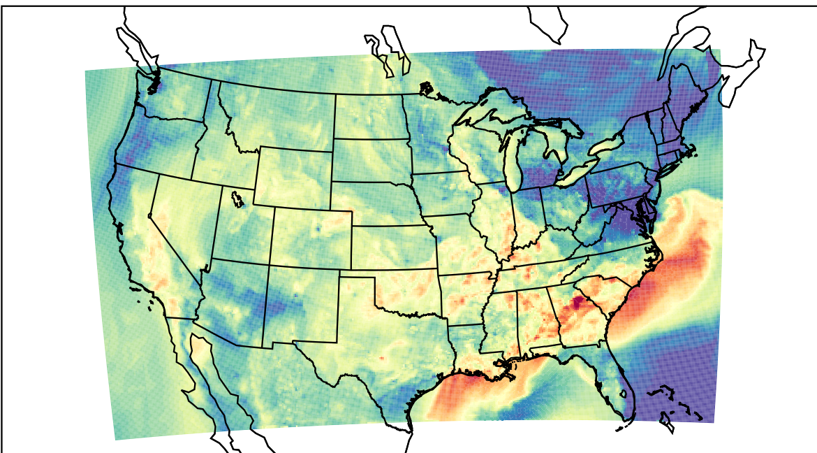
WRF (2023-09-26_01:00:00)
