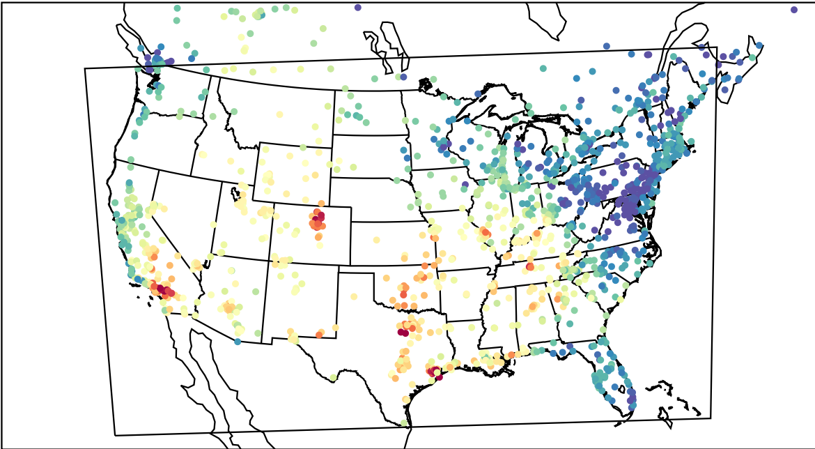
AirNOW (2023-09-26_21:00:00)
