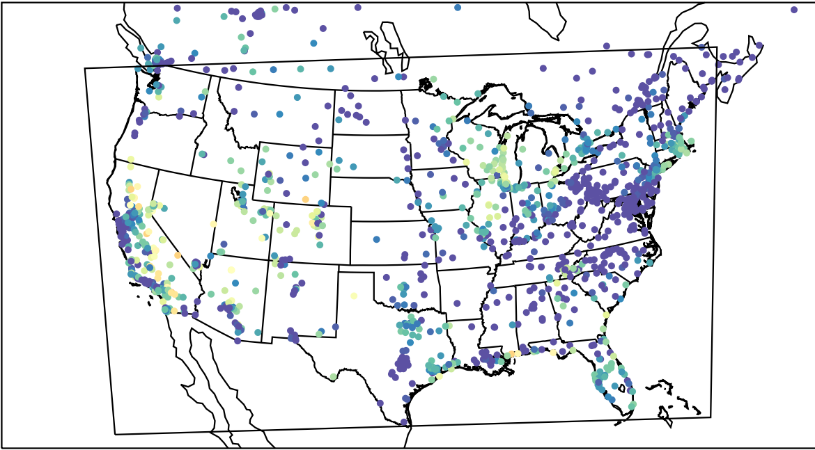
AirNOW (2023-09-25_05:00:00)
