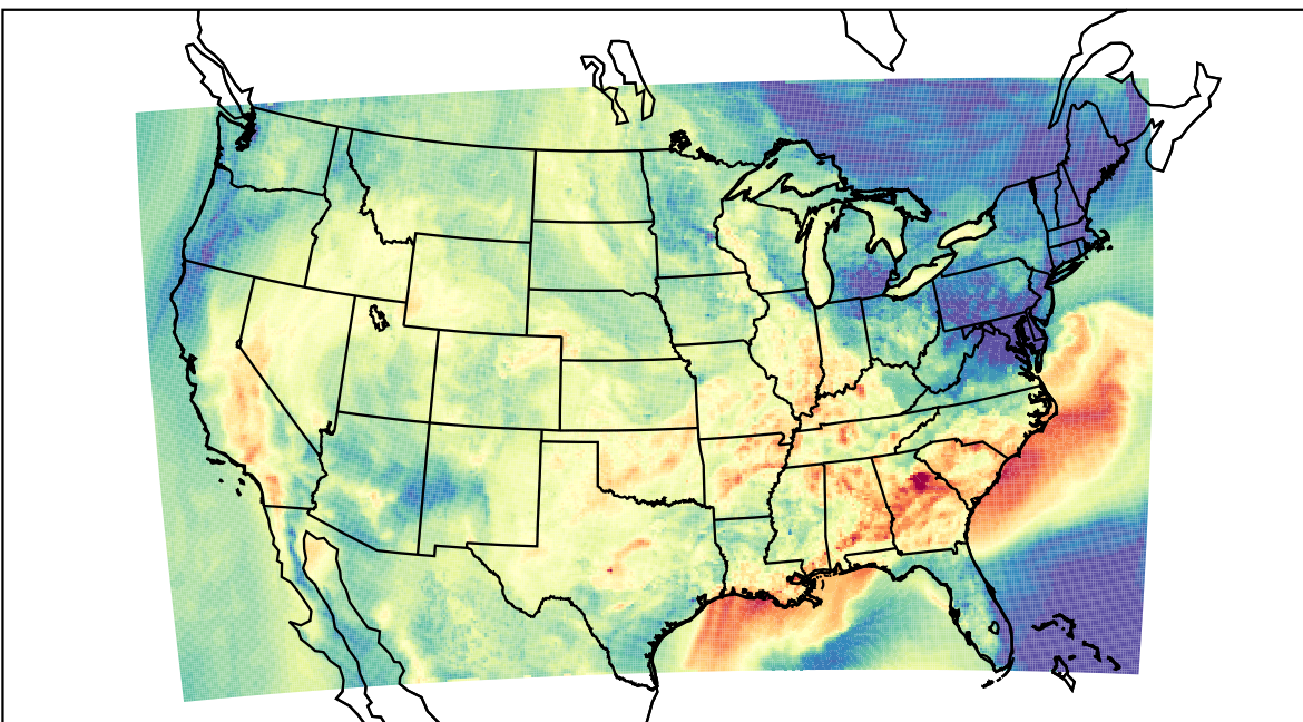
WRF (2023-09-26_00:00:00)
