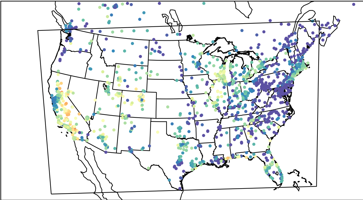
AirNOW (2023-09-25_02:00:00)
