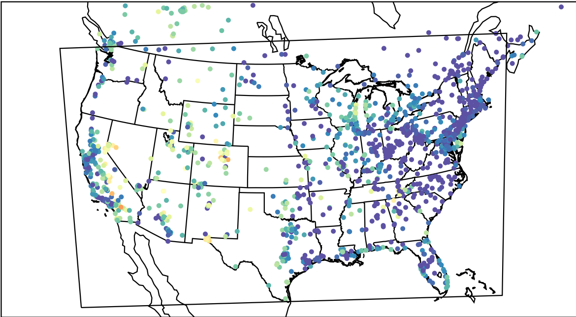
AirNOW (2023-09-26_04:00:00)
