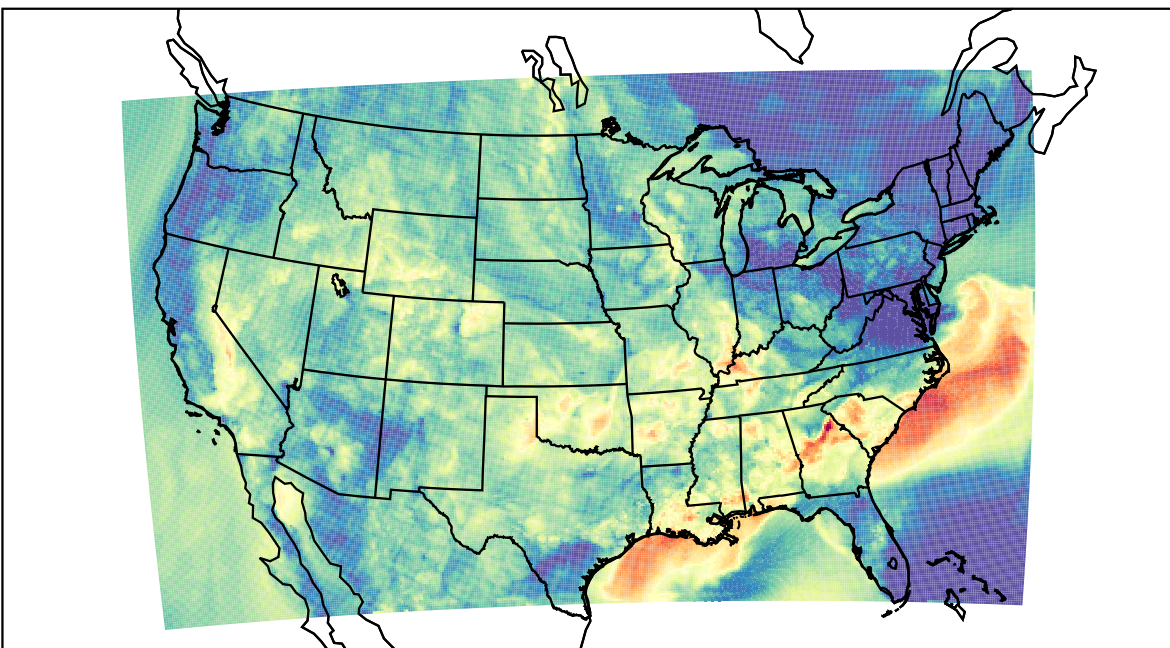
WRF (2023-09-26_04:00:00)
