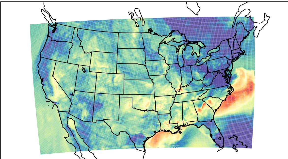
WRF (2023-09-26_06:00:00)
