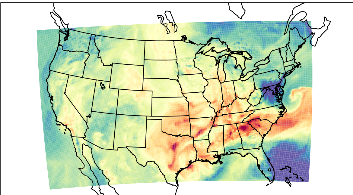
WRF (2023-09-26_21:00:00)
