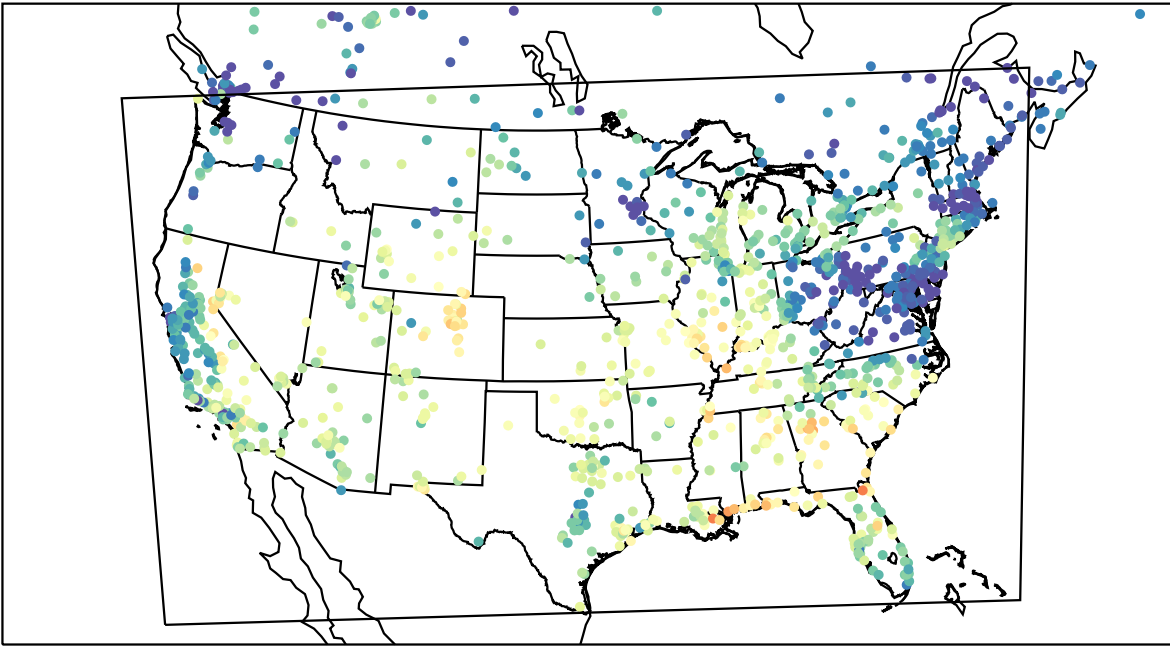
AirNOW (2023-09-25_17:00:00)
