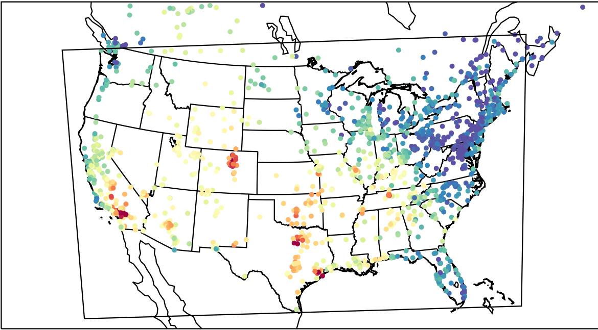
AirNOW (2023-09-26_22:00:00)
