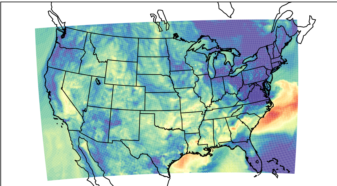
WRF (2023-09-26_09:00:00)
