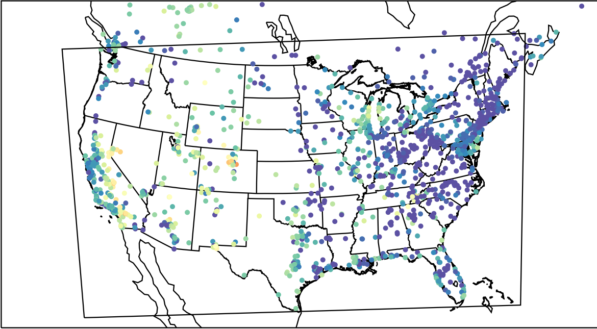
AirNOW (2023-09-26_03:00:00)
