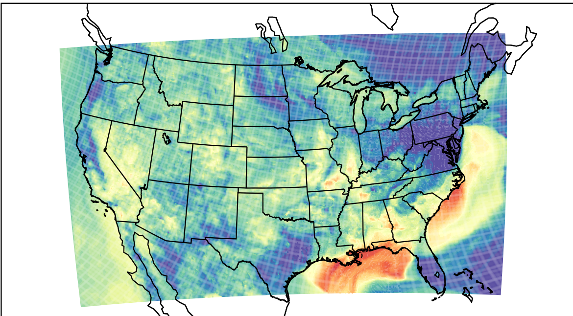
WRF (2023-09-25_07:00:00)
