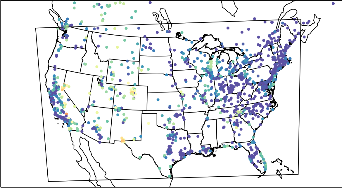
AirNOW (2023-09-26_06:00:00)
