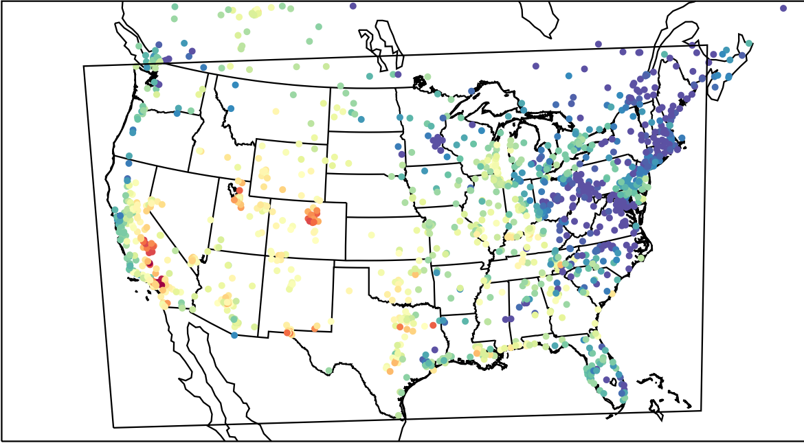
AirNOW (2023-09-25_23:00:00)
