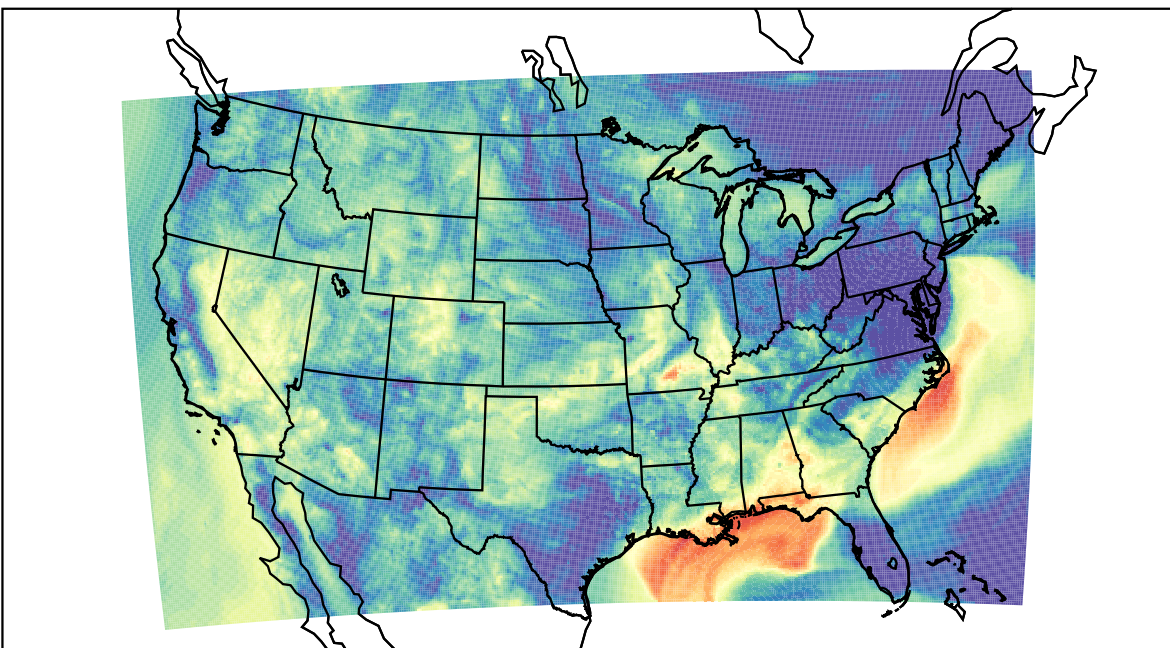
WRF (2023-09-25_10:00:00)
