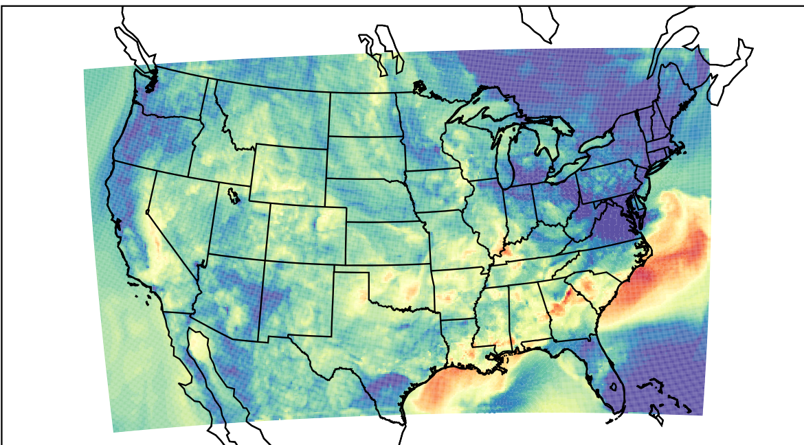
WRF (2023-09-26_05:00:00)
