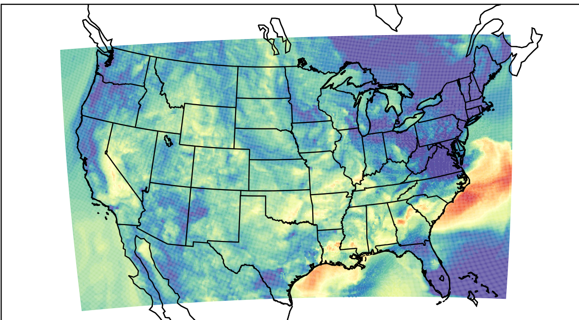
WRF (2023-09-26_08:00:00)
