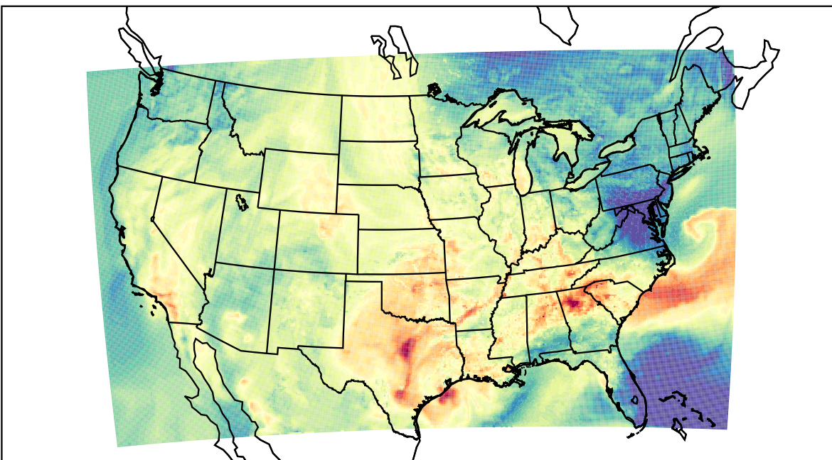
WRF (2023-09-26_23:00:00)
