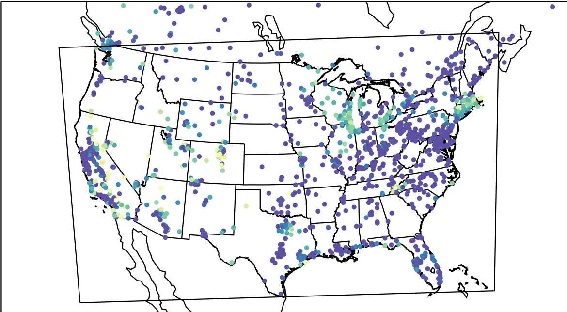
AirNOW (2023-09-25_09:00:00)
