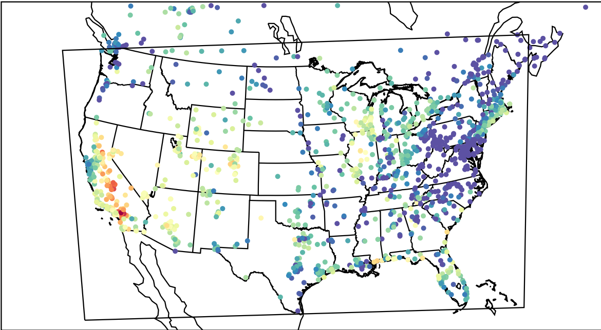
AirNOW (2023-09-25_01:00:00)
