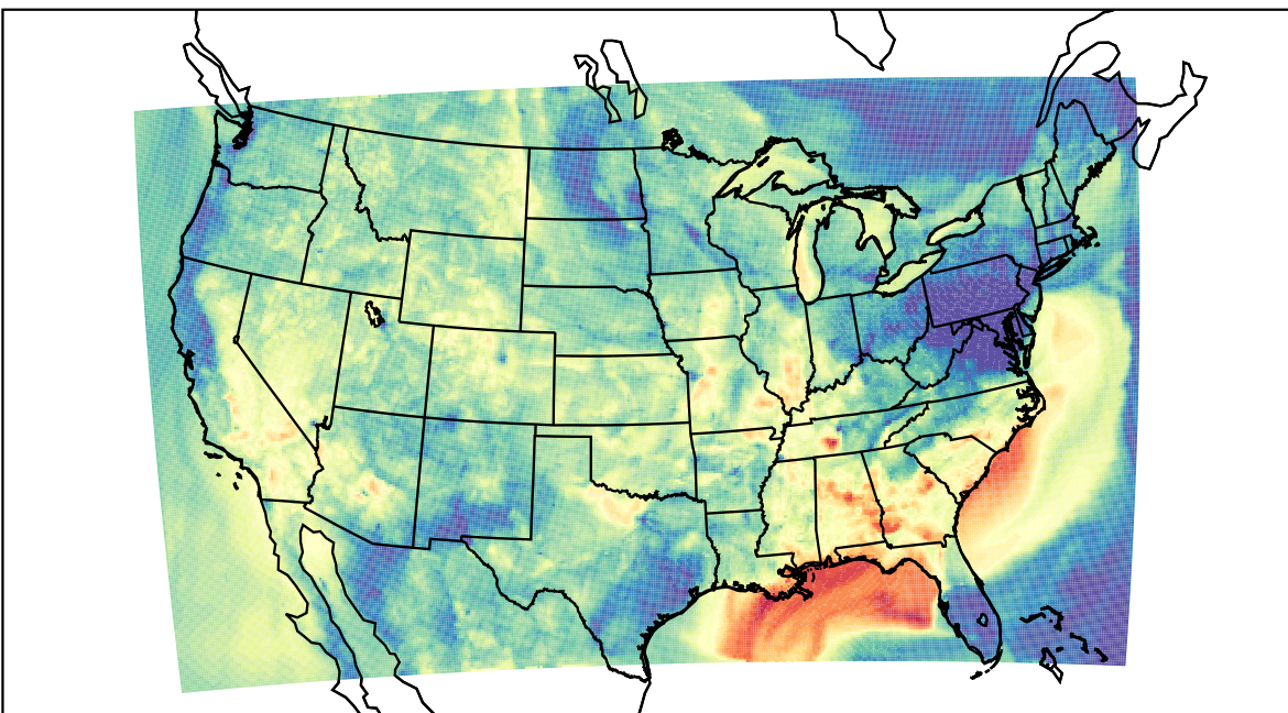
WRF (2023-09-25_03:00:00)
