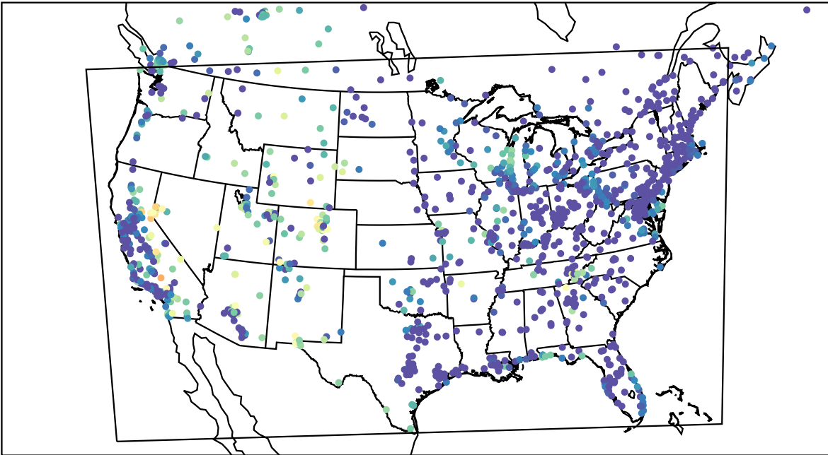
AirNOW (2023-09-26_08:00:00)
