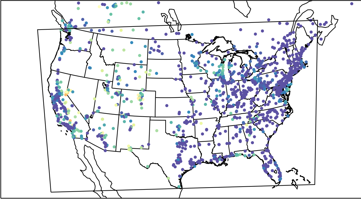
AirNOW (2023-09-26_09:00:00)
