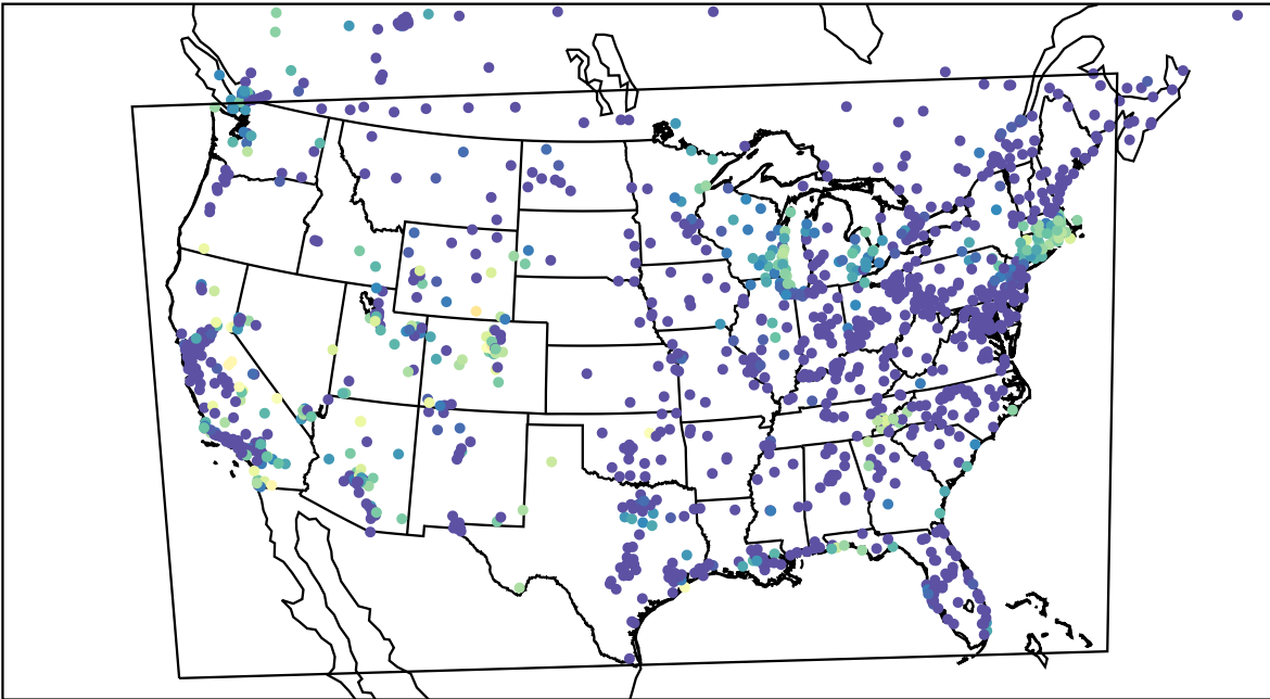
AirNOW (2023-09-25_12:00:00)
