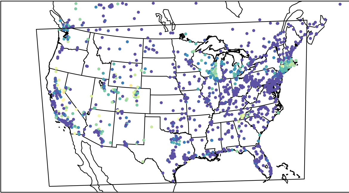
AirNOW (2023-09-25_11:00:00)
