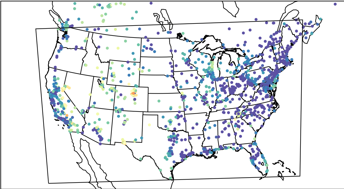
AirNOW (2023-09-26_05:00:00)
