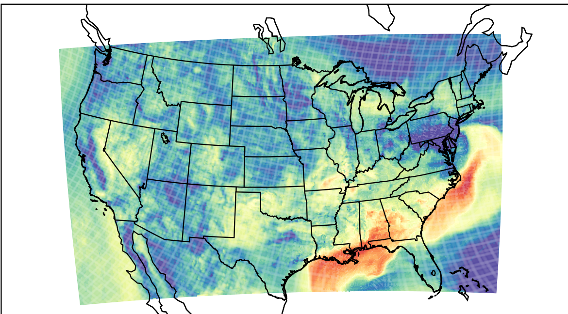
WRF (2023-09-25_15:00:00)
