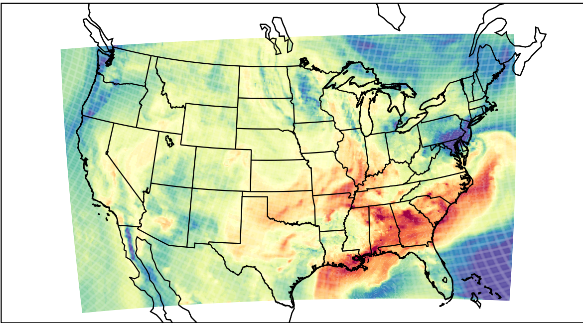
WRF (2023-09-25_19:00:00)
