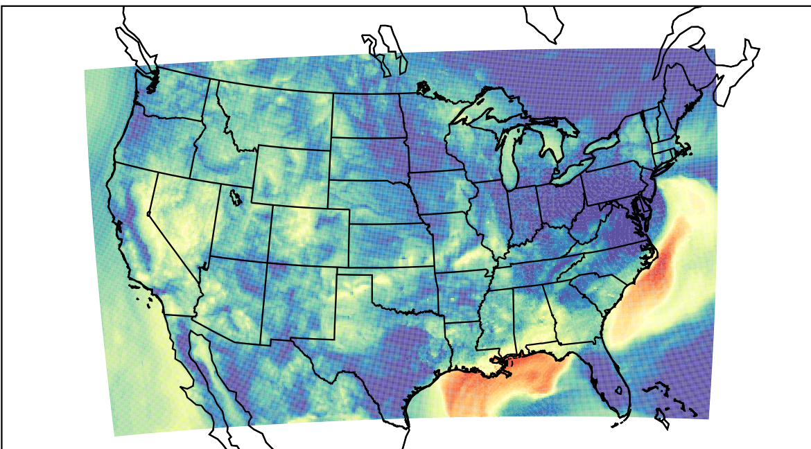
WRF (2023-09-25_13:00:00)
