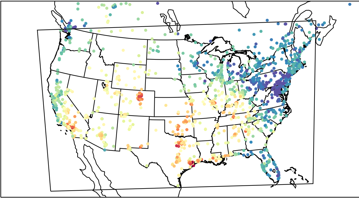
AirNOW (2023-09-26_20:00:00)
