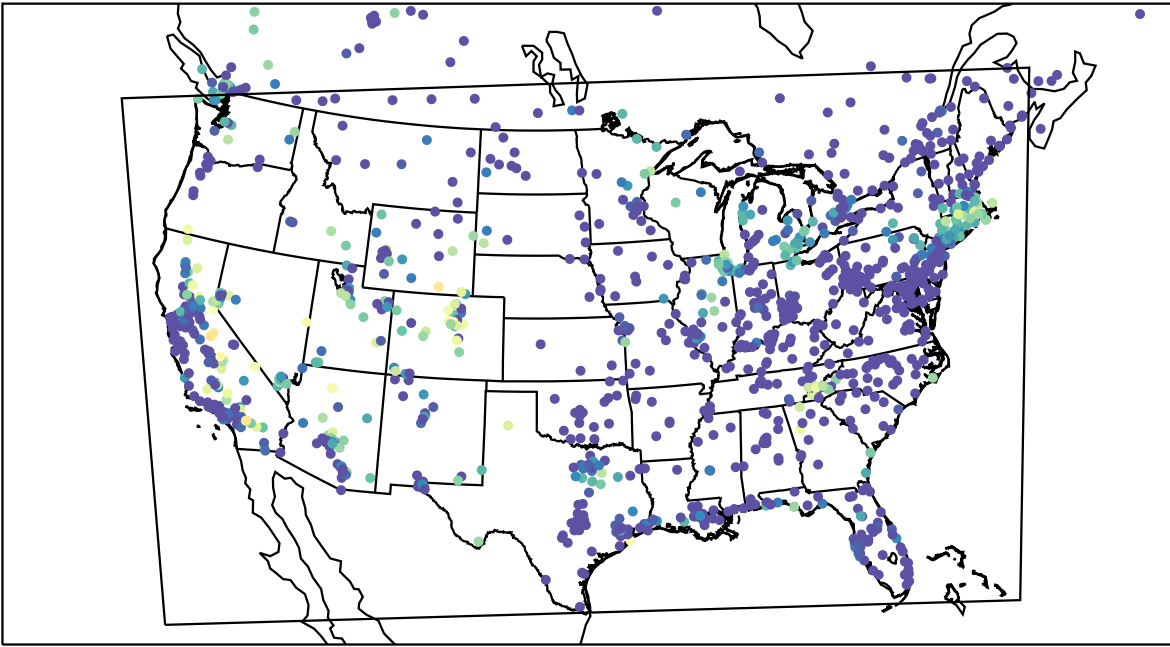
AirNOW (2023-09-25_10:00:00)
