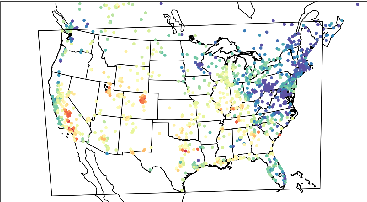
AirNOW (2023-09-25_22:00:00)
