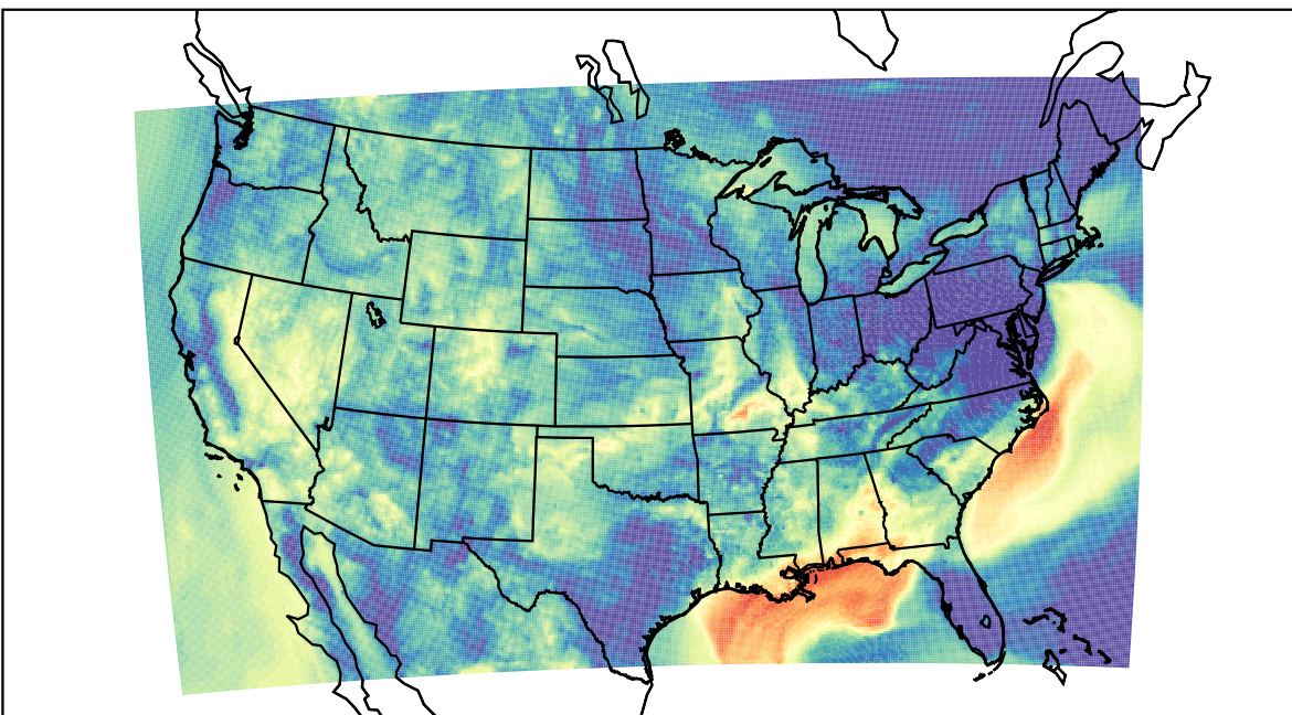
WRF (2023-09-25_11:00:00)
