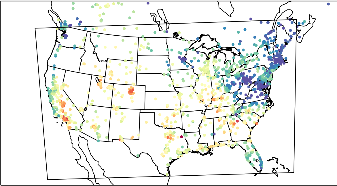
AirNOW (2023-09-25_21:00:00)
