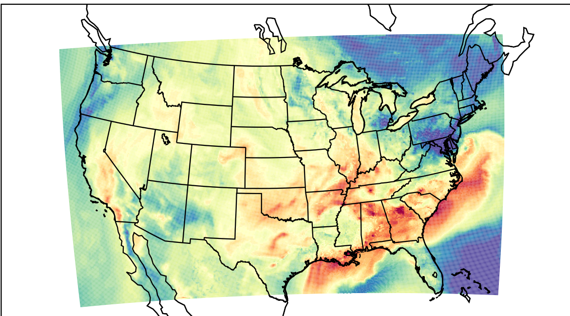
WRF (2023-09-25_22:00:00)
