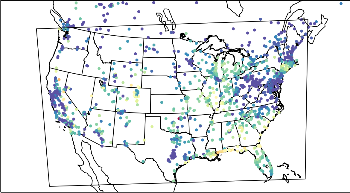
AirNOW (2023-09-25_15:00:00)
