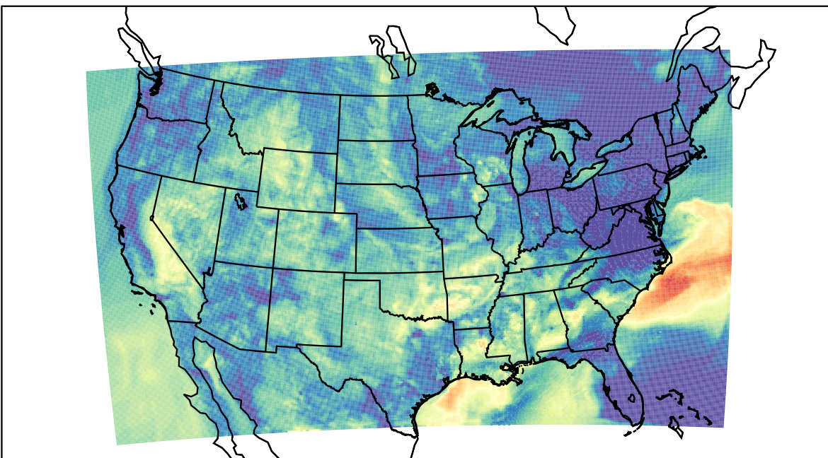
WRF (2023-09-26_12:00:00)
