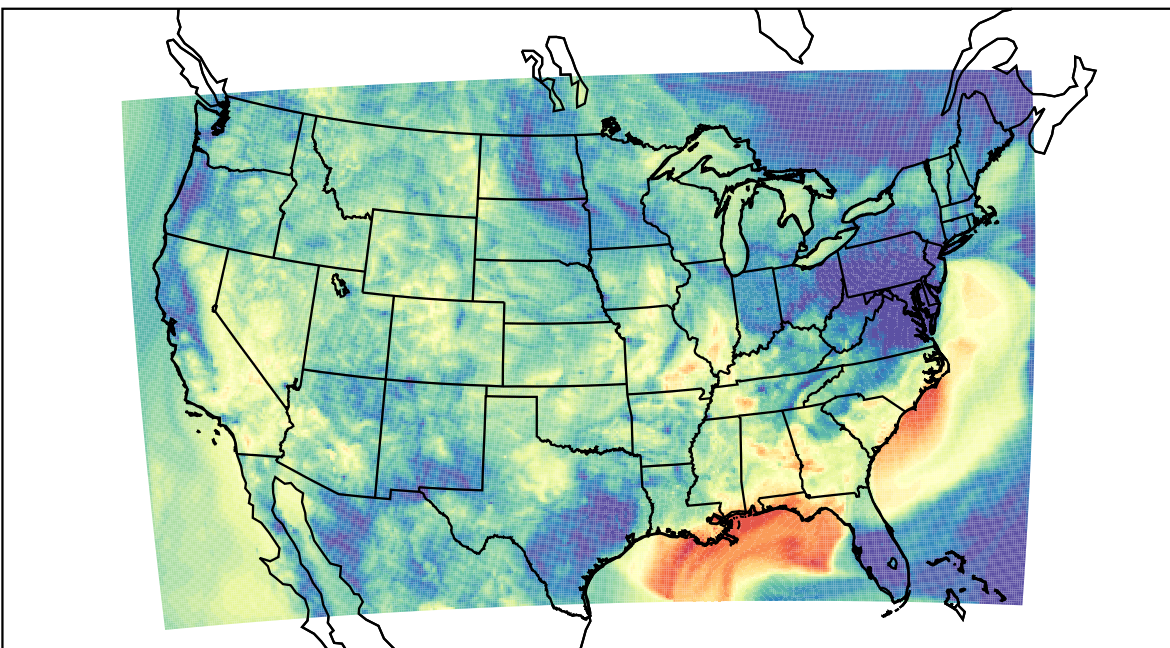
WRF (2023-09-25_06:00:00)
