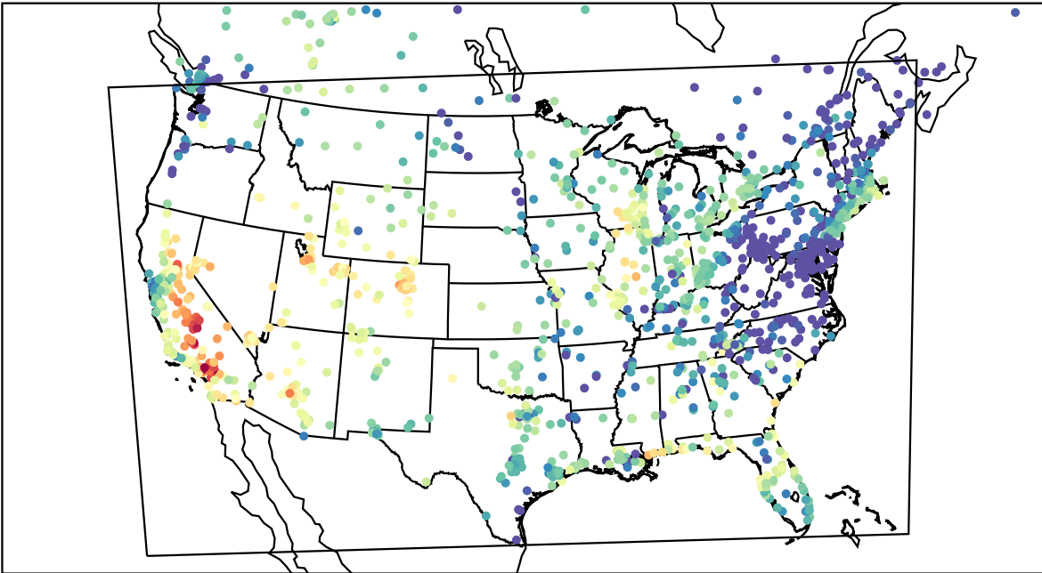
AirNOW (2023-09-25_00:00:00)
