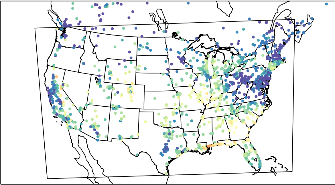
AirNOW (2023-09-25_16:00:00)
