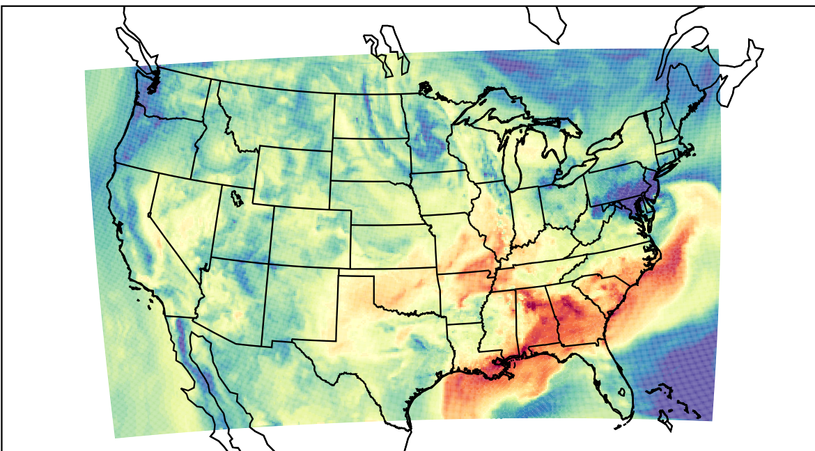
WRF (2023-09-25_17:00:00)
