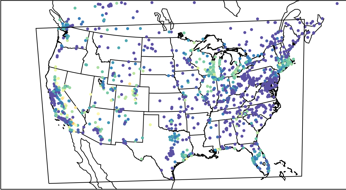
AirNOW (2023-09-25_07:00:00)
