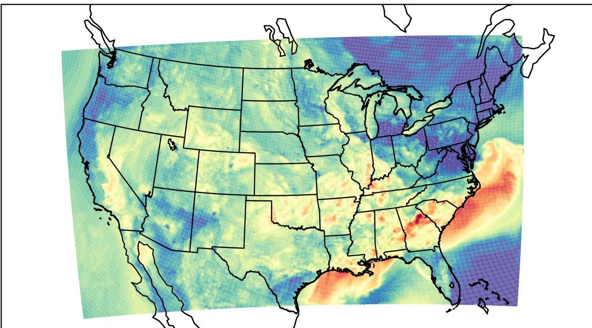
WRF (2023-09-26_02:00:00)
