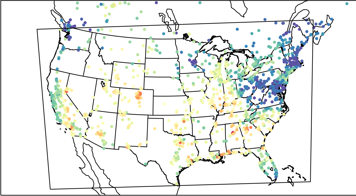
AirNOW (2023-09-25_19:00:00)
