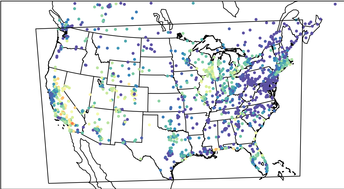
AirNOW (2023-09-25_03:00:00)
