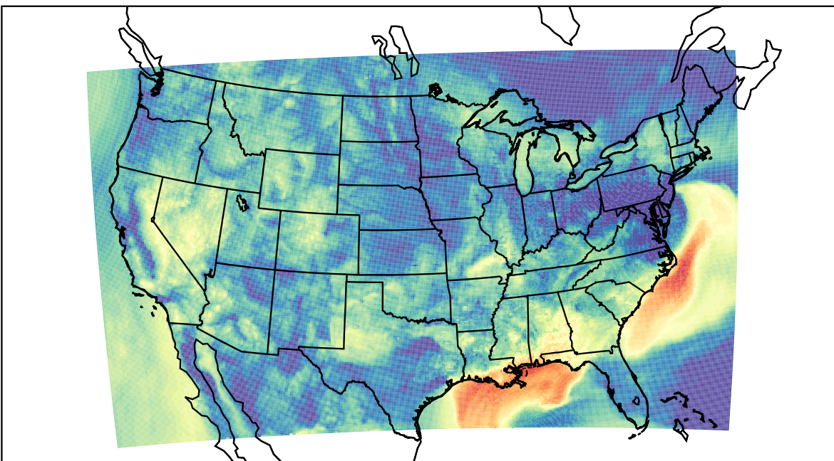
WRF (2023-09-25_14:00:00)
