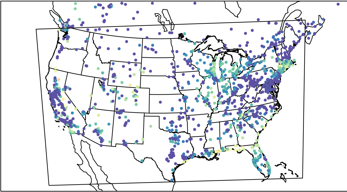
AirNOW (2023-09-25_14:00:00)
