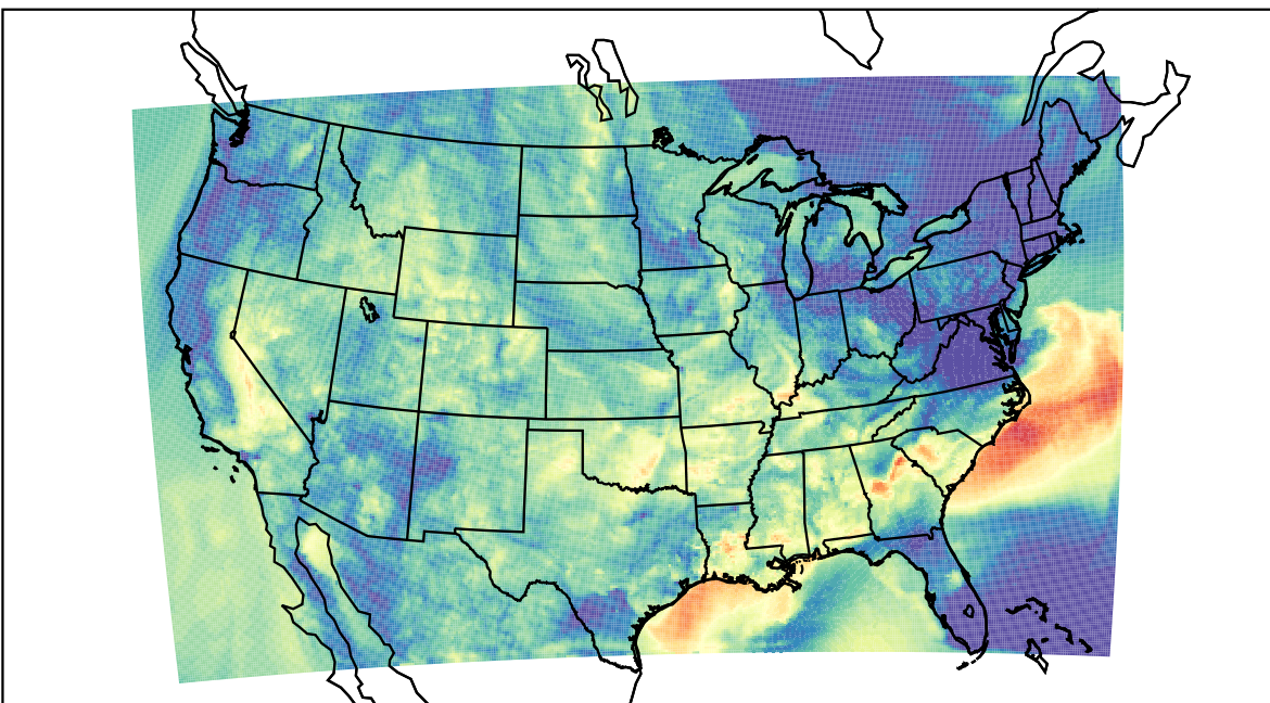
WRF (2023-09-26_07:00:00)
