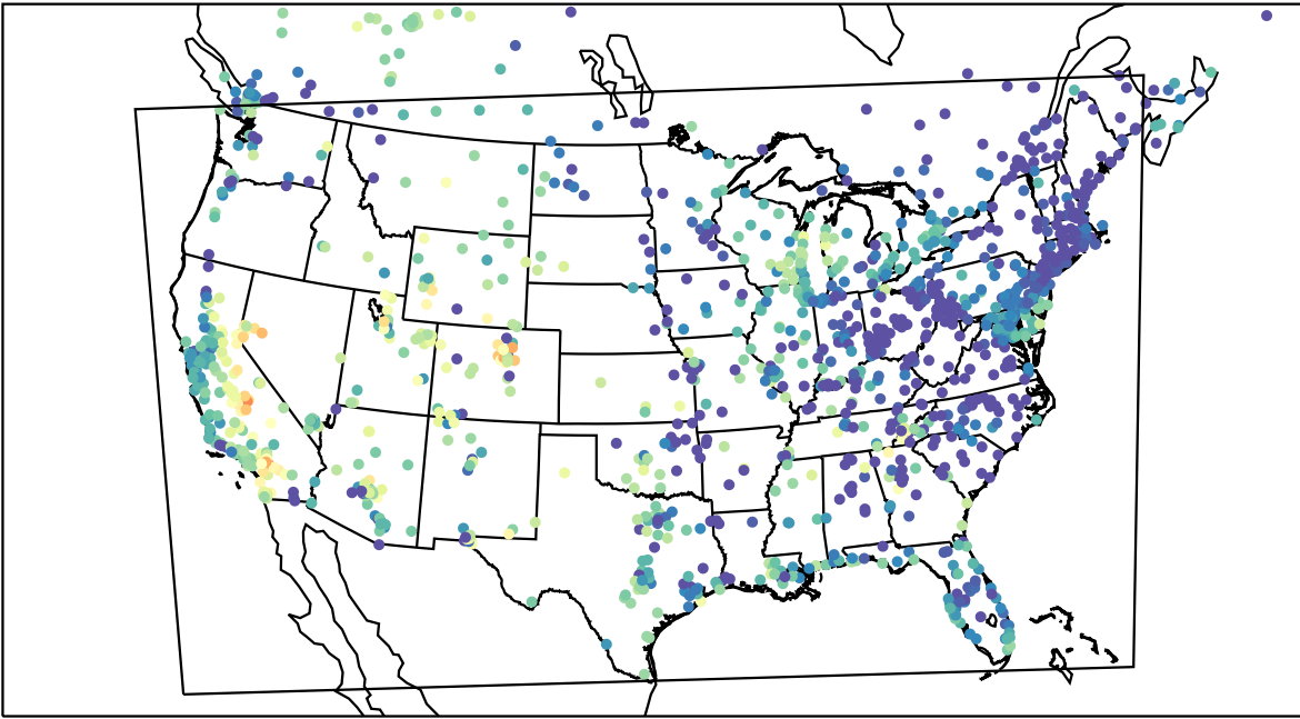
AirNOW (2023-09-26_02:00:00)
