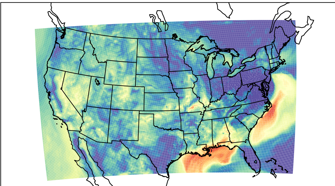
WRF (2023-09-25_12:00:00)
