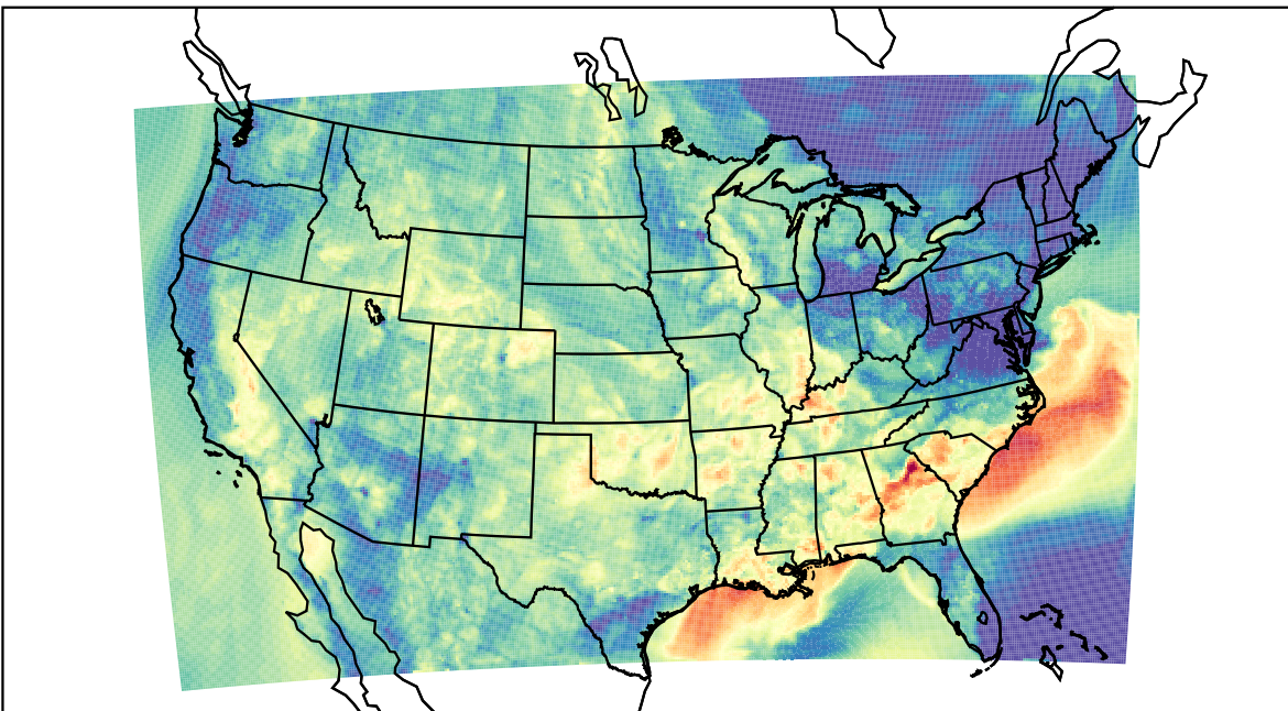
WRF (2023-09-26_03:00:00)
