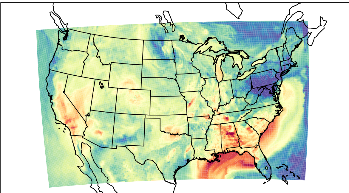
WRF (2023-09-25_00:00:00)
