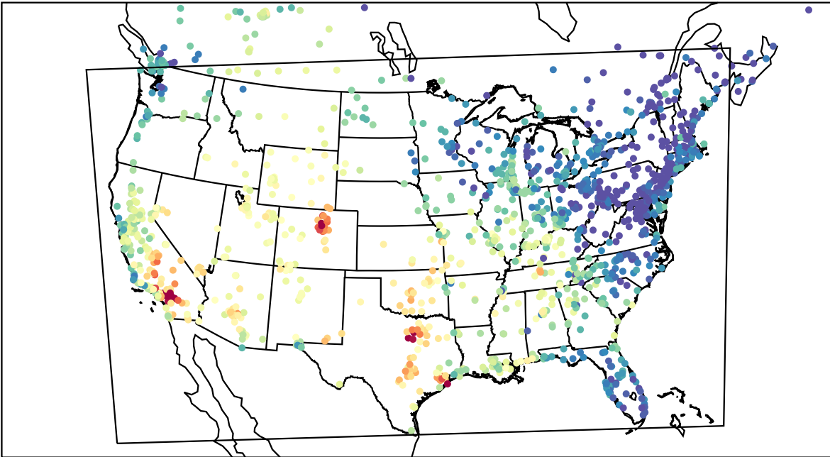
AirNOW (2023-09-26_23:00:00)
