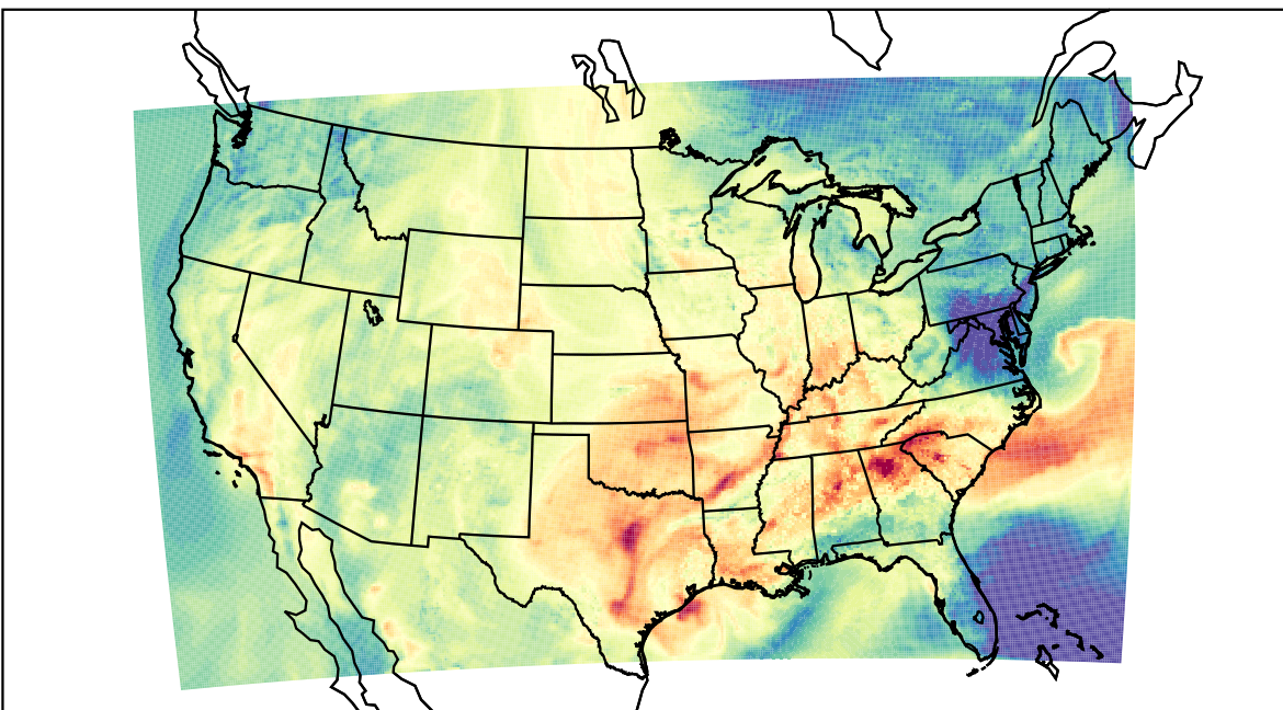
WRF (2023-09-26_22:00:00)
