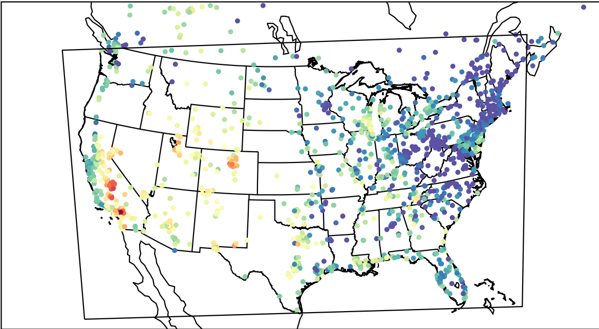
AirNOW (2023-09-26_00:00:00)
