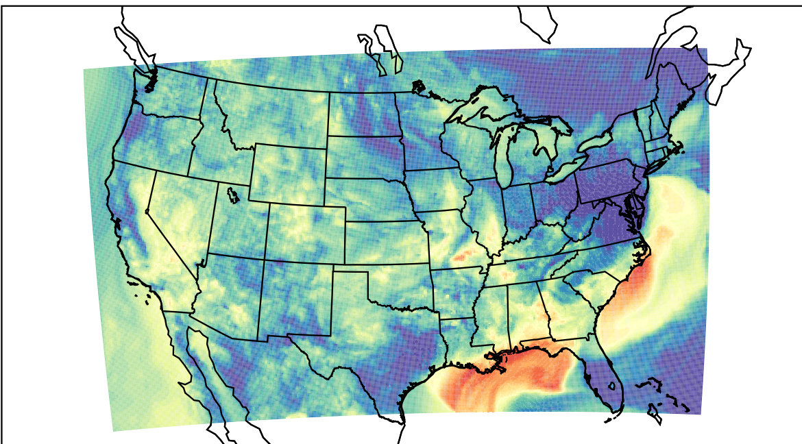
WRF (2023-09-25_08:00:00)
