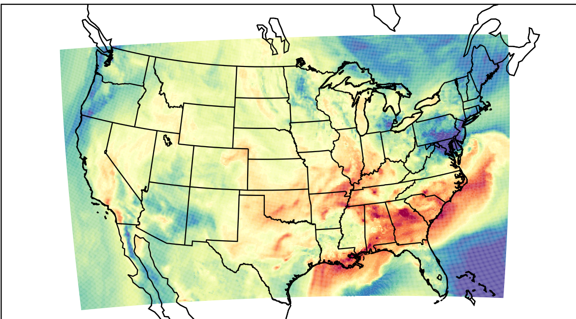
WRF (2023-09-25_21:00:00)
