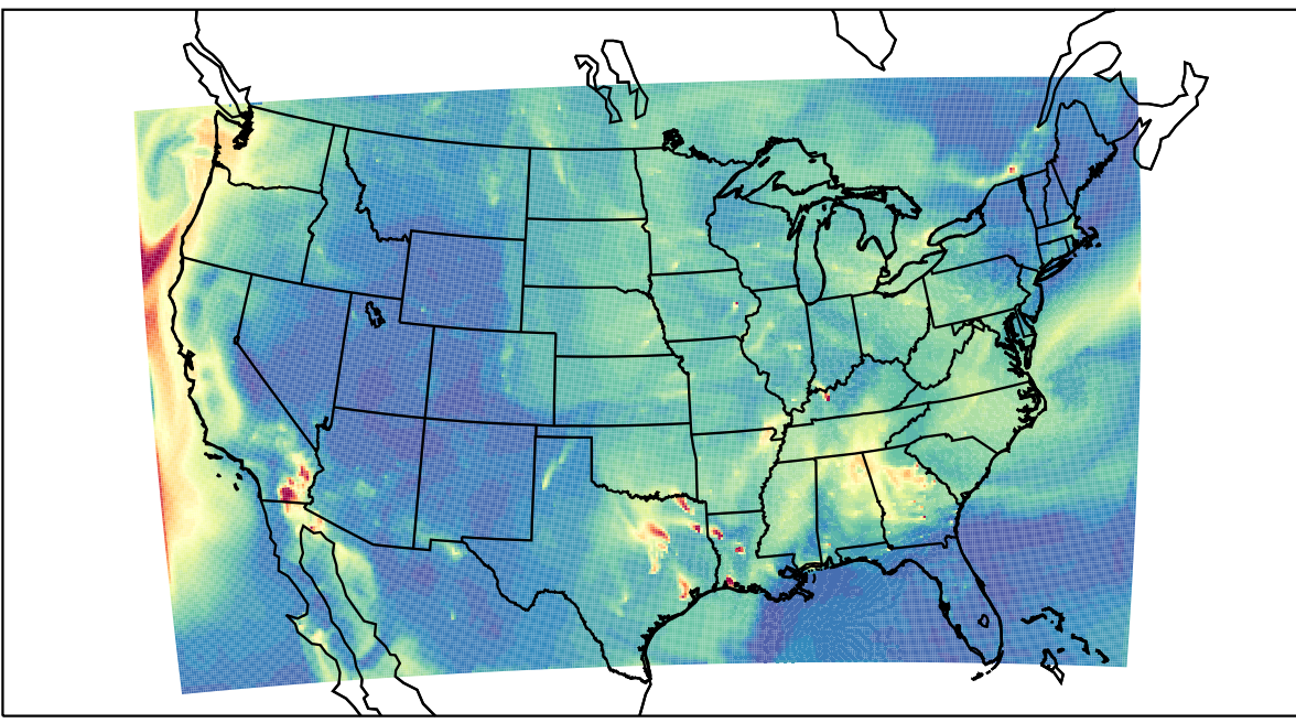
WRF 2023-09-27_10:00:00
