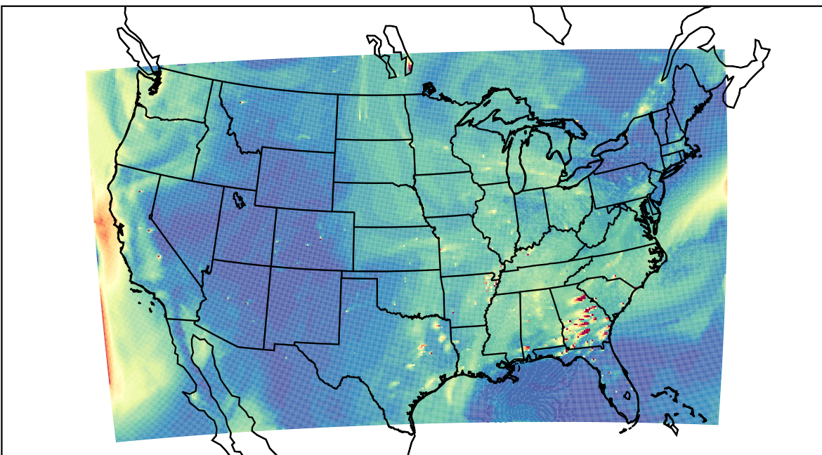
WRF 2023-09-27_22:00:00
