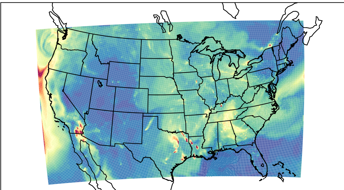
WRF 2023-09-27_13:00:00
