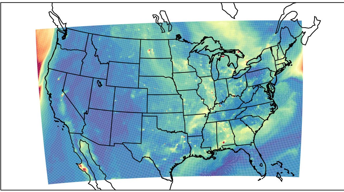
WRF 2023-09-26_00:00:00
