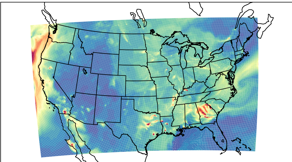
WRF 2023-09-27_05:00:00
