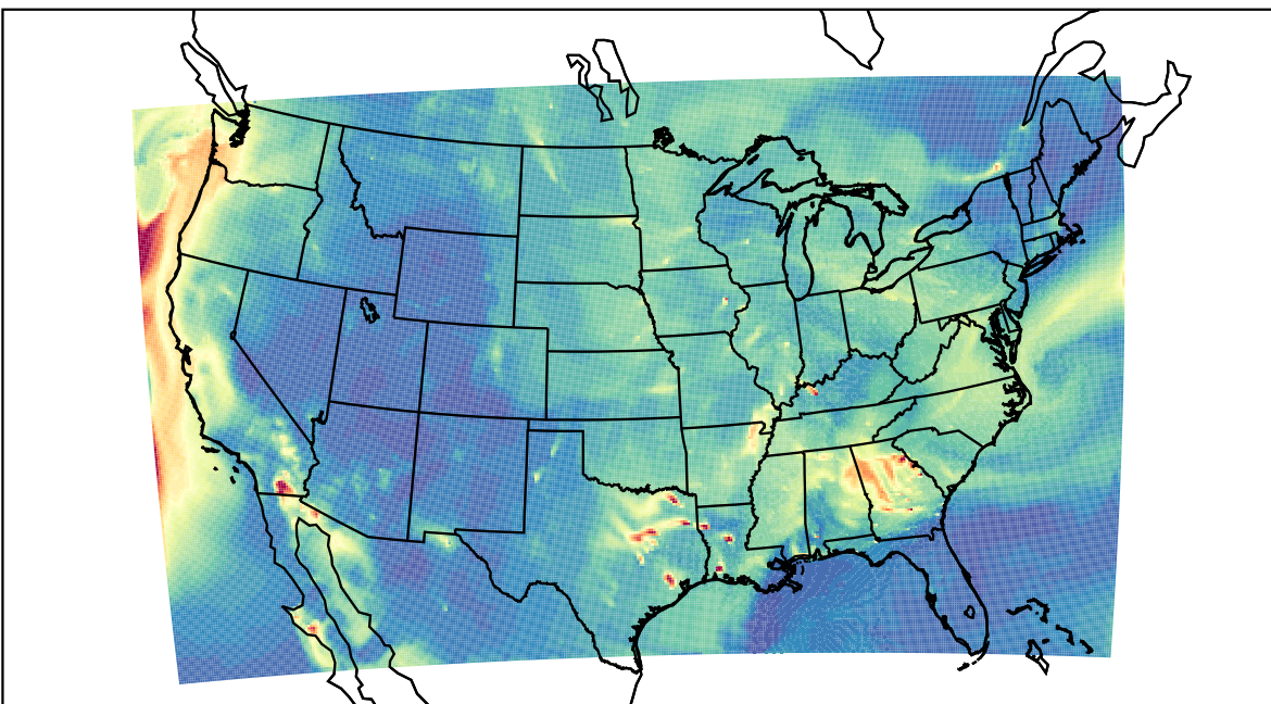
WRF 2023-09-27_07:00:00
