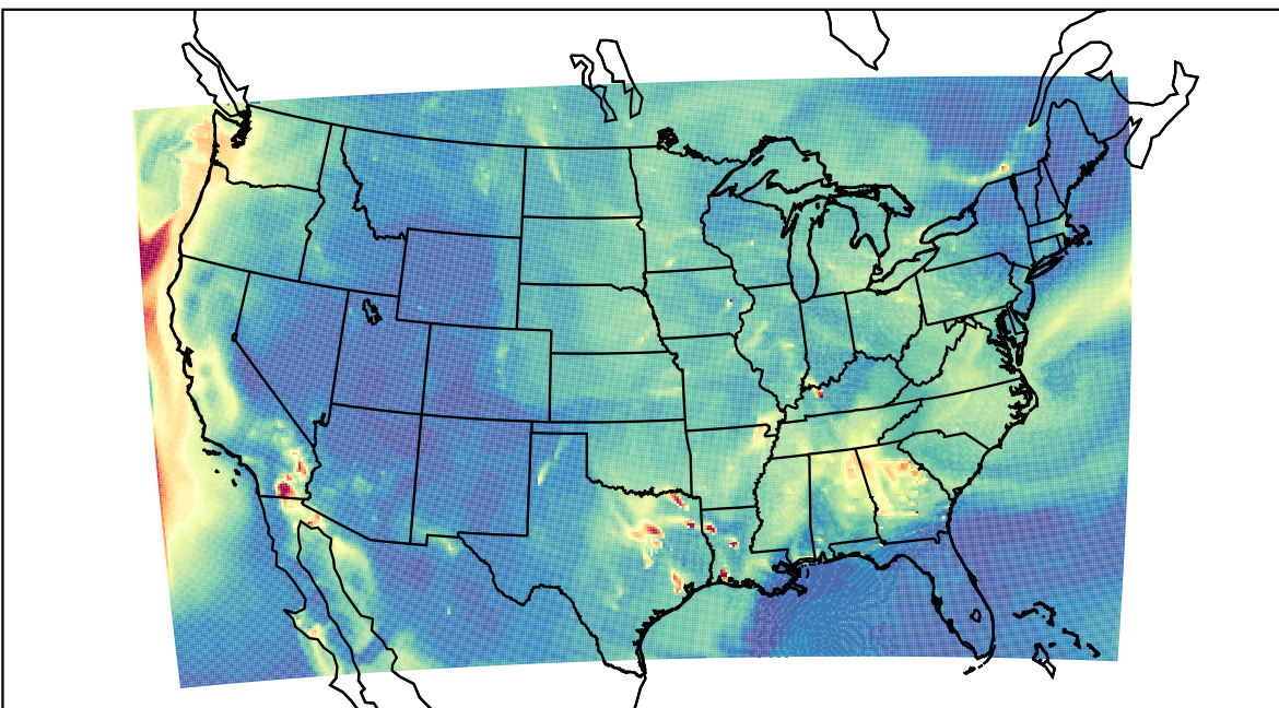
WRF 2023-09-27_09:00:00
