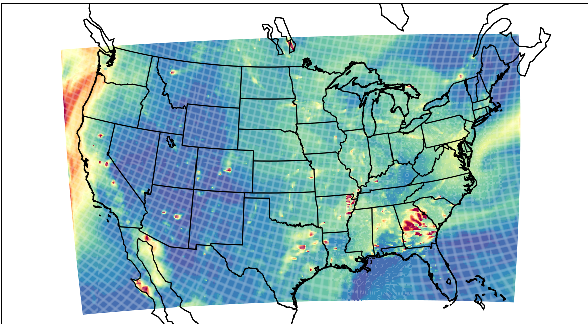
WRF 2023-09-27_02:00:00
