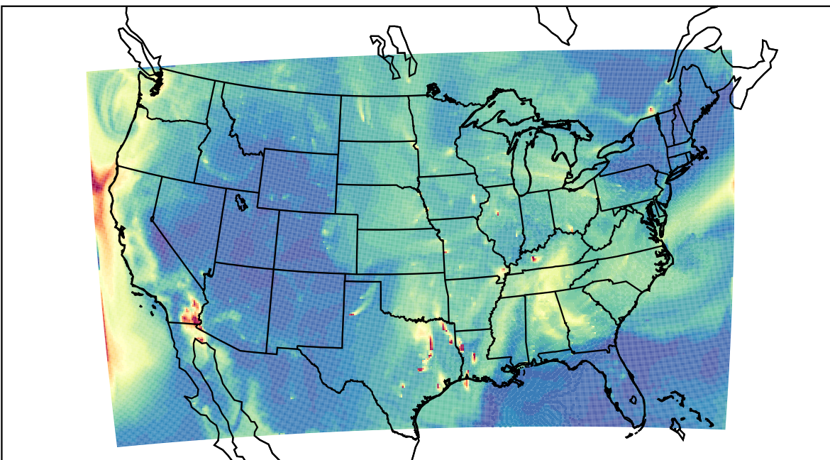
WRF 2023-09-27_15:00:00
