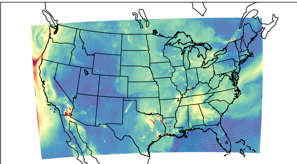
WRF 2023-09-27_12:00:00
