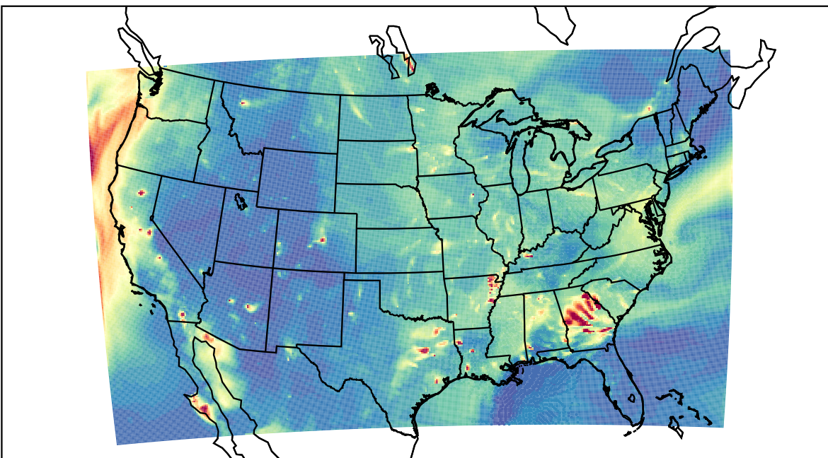
WRF 2023-09-27_03:00:00
