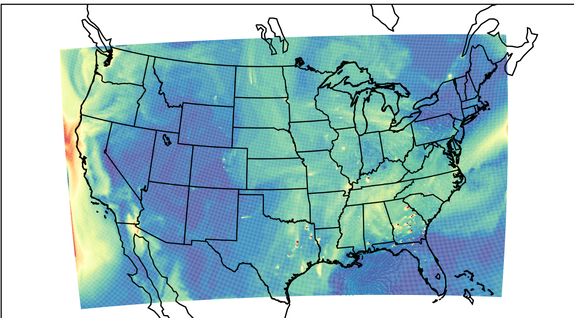
WRF 2023-09-27_18:00:00
