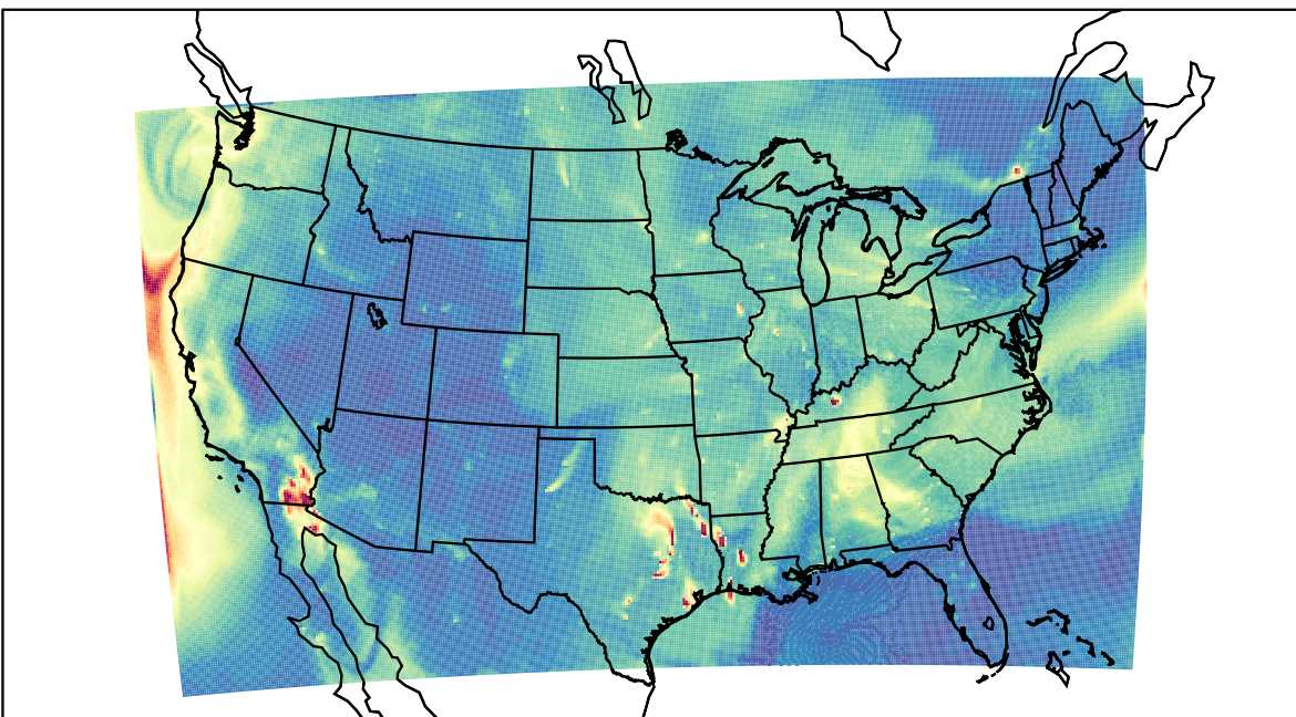
WRF 2023-09-27_14:00:00
