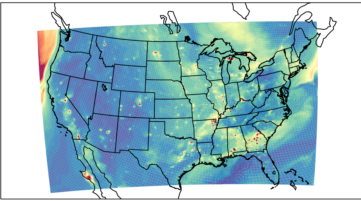
WRF 2023-09-26_02:00:00
