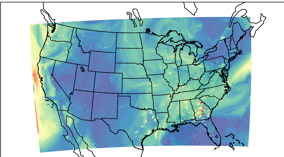
WRF 2023-09-27_21:00:00
