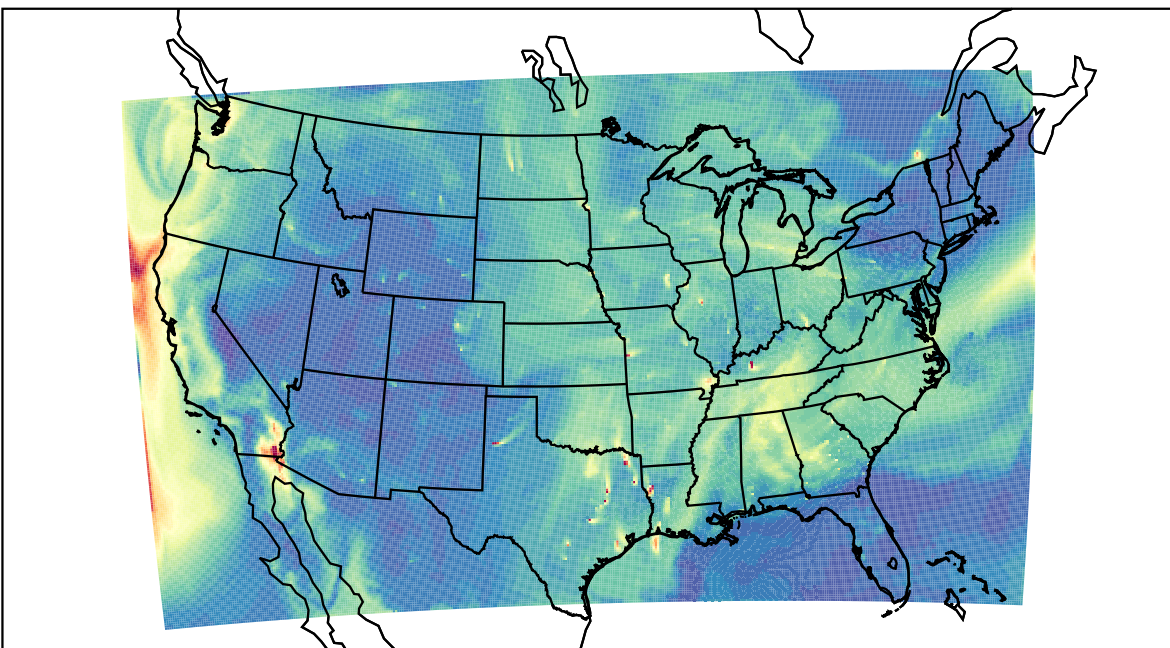
WRF 2023-09-27_16:00:00
