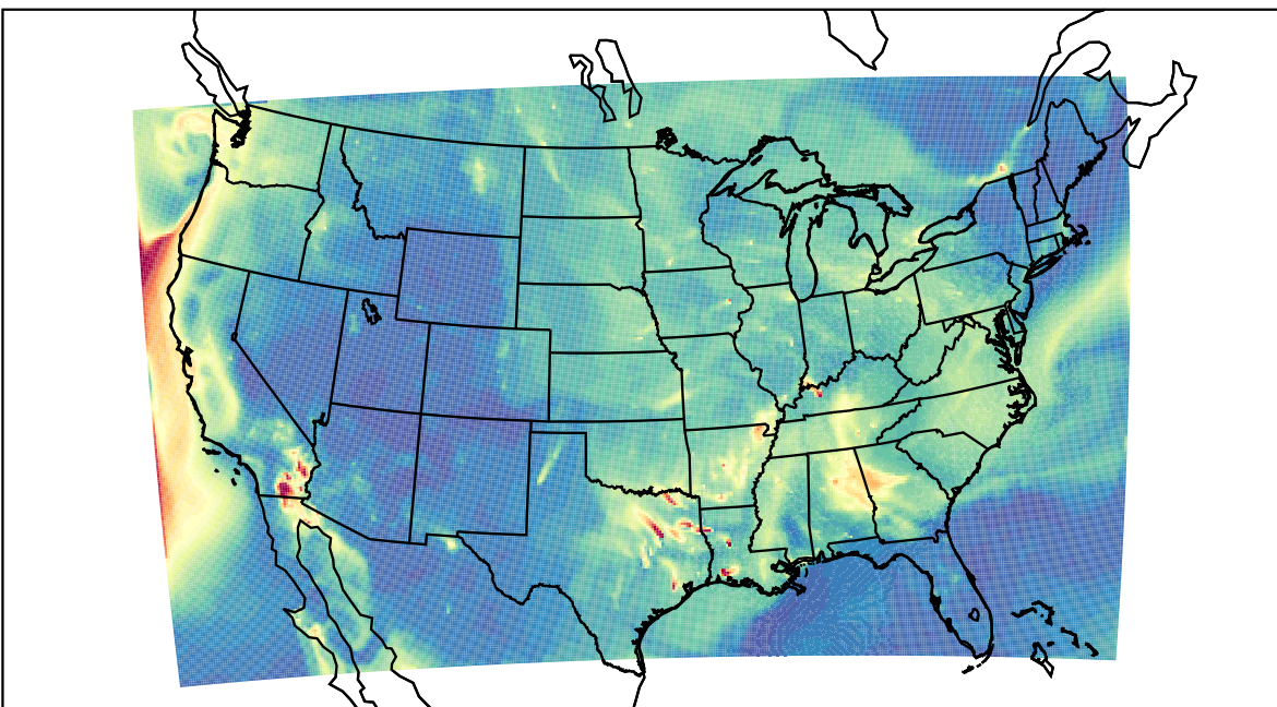
WRF 2023-09-27_10:00:00
