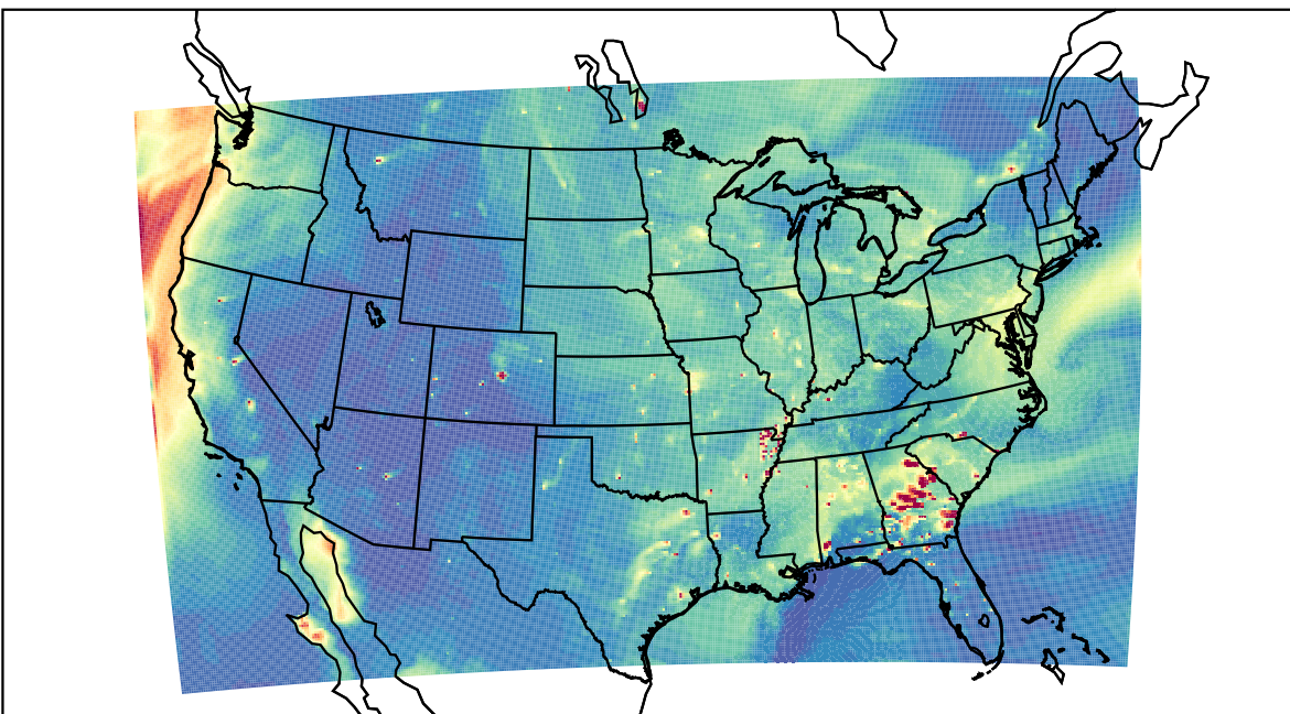
WRF 2023-09-27_00:00:00
