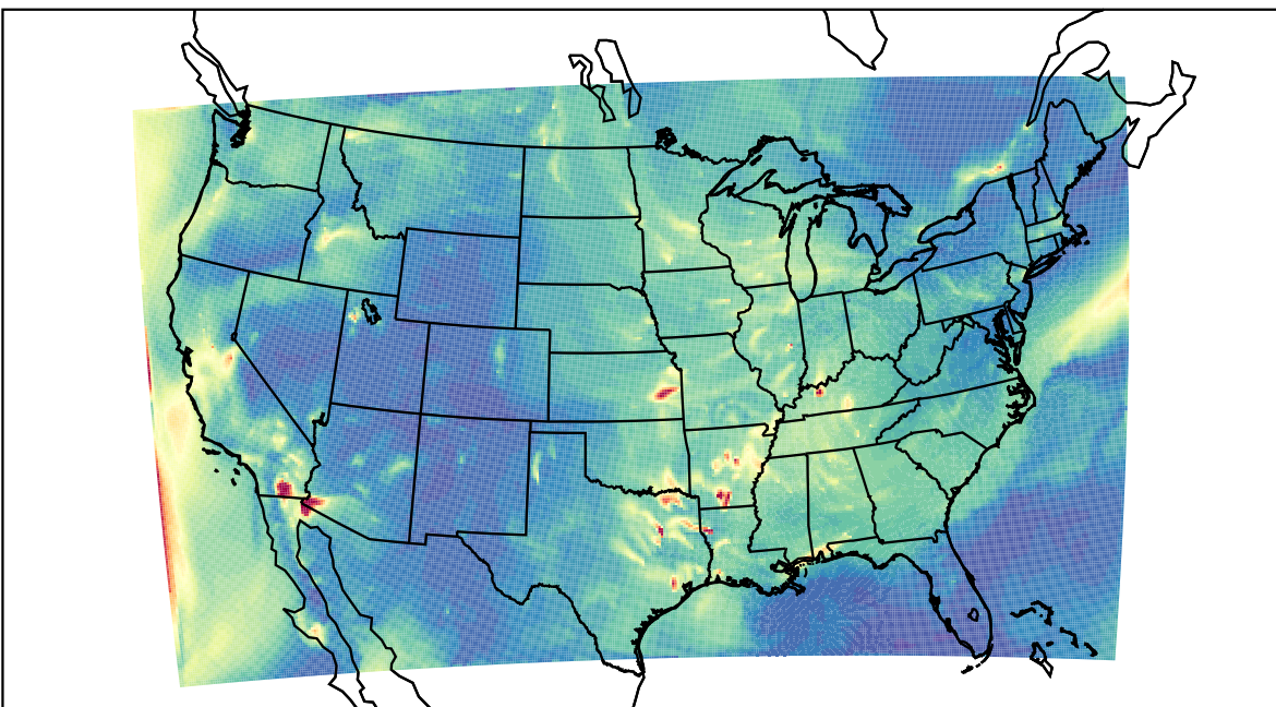
WRF 2023-09-28_05:00:00
