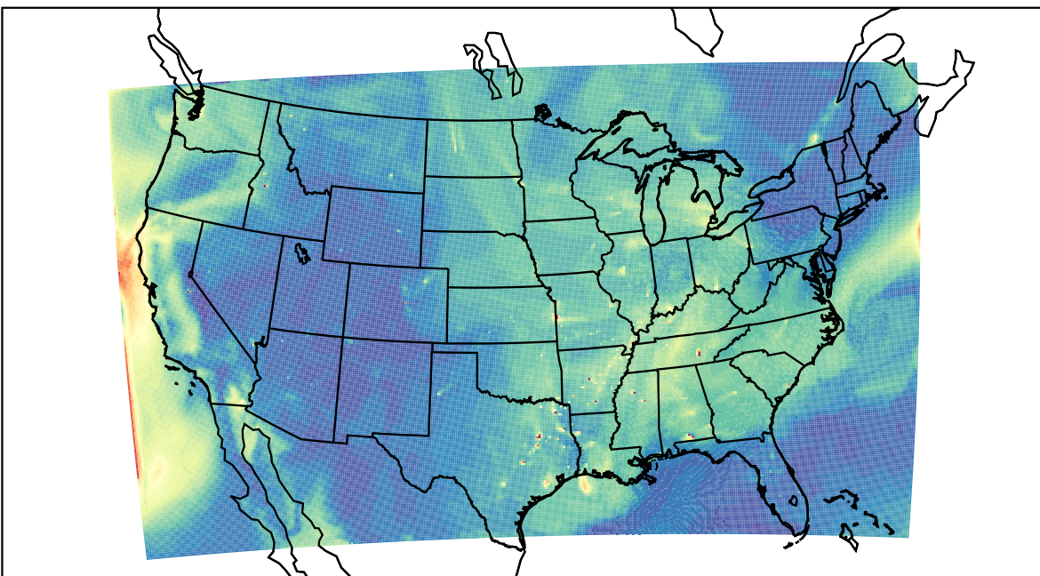
WRF 2023-09-27_19:00:00
