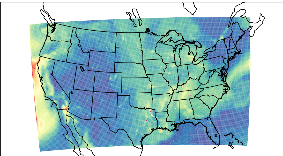
WRF 2023-09-27_17:00:00
