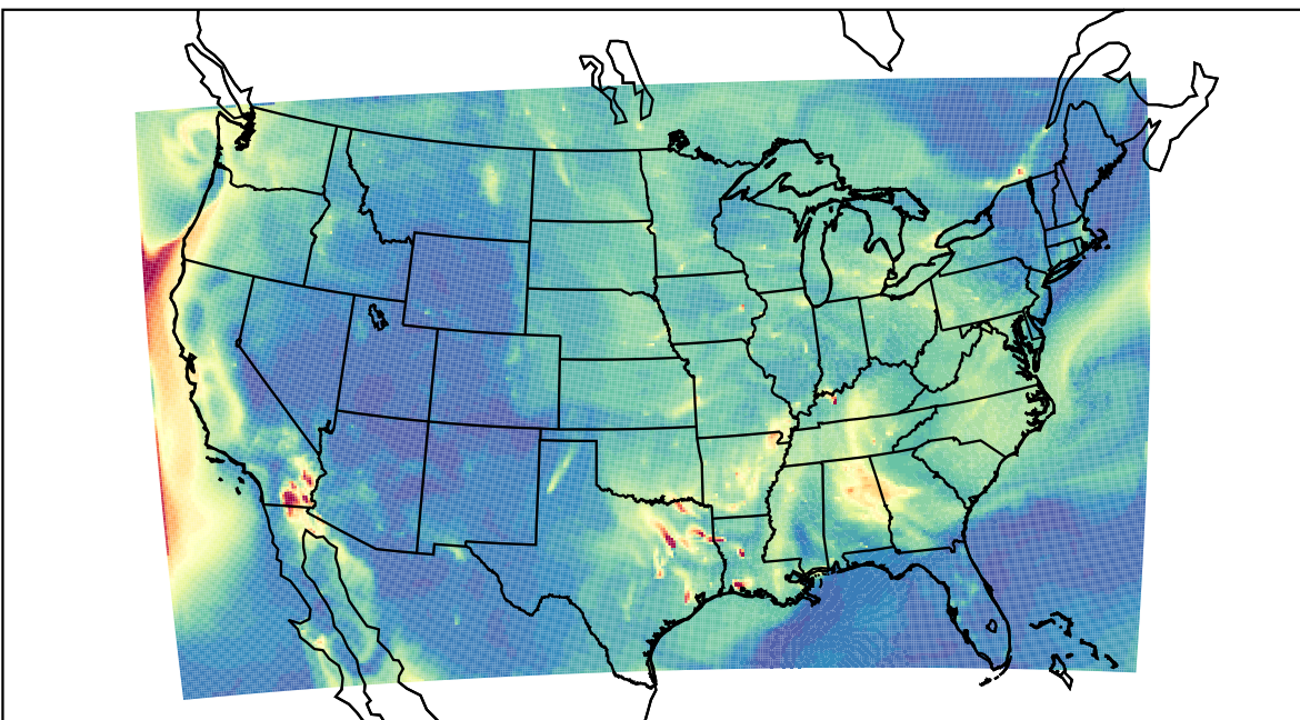
WRF 2023-09-27_11:00:00
