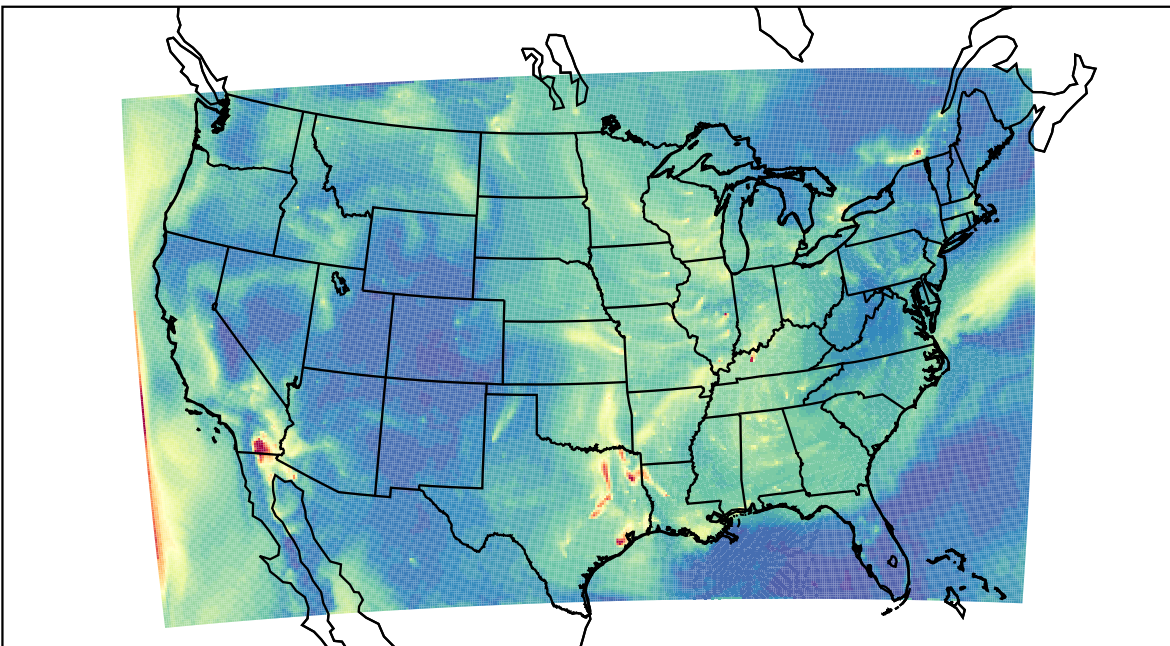
WRF 2023-09-28_12:00:00
