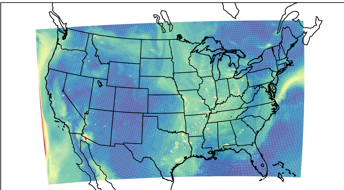
WRF 2023-09-28_21:00:00
