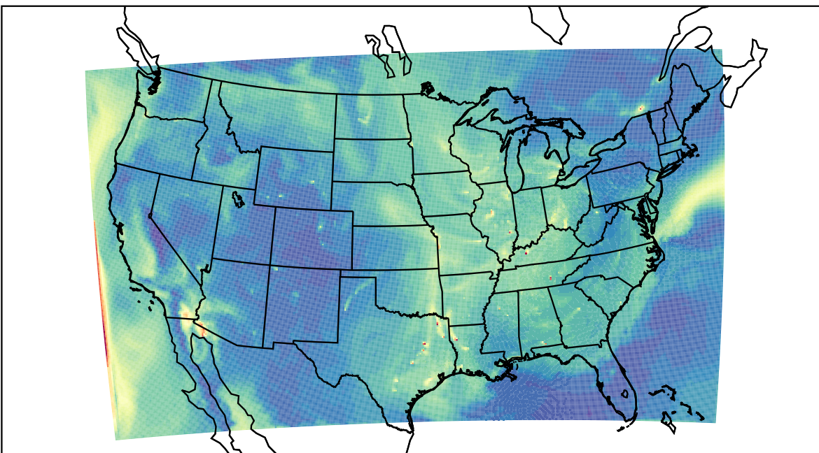
WRF 2023-09-28_17:00:00
