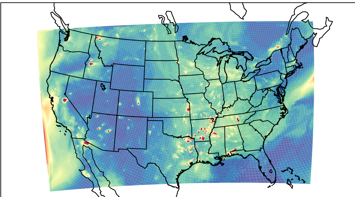
WRF 2023-09-28_02:00:00
