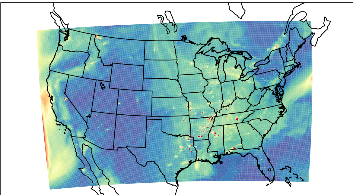
WRF 2023-09-27_23:00:00
