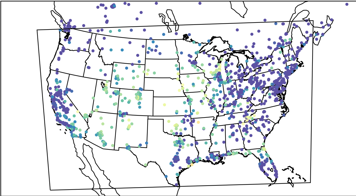
AirNOW (2023-10-01_08:00:00)
