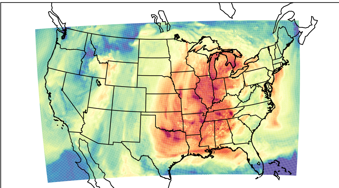
WRF (2023-10-01_22:00:00)
