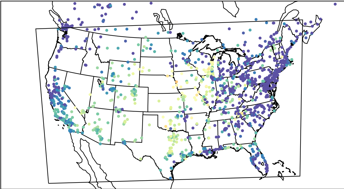
AirNOW (2023-10-01_03:00:00)
