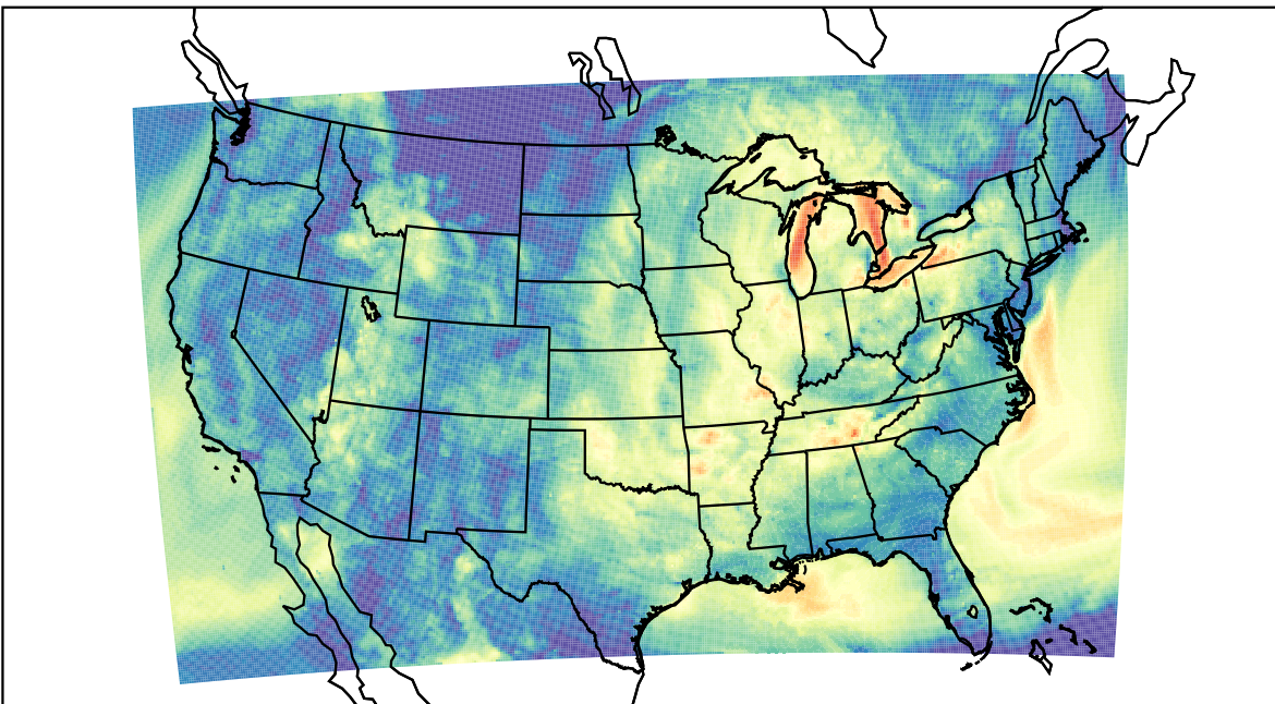
WRF (2023-10-02_09:00:00)
