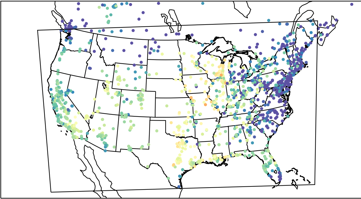
AirNOW (2023-10-02_00:00:00)
