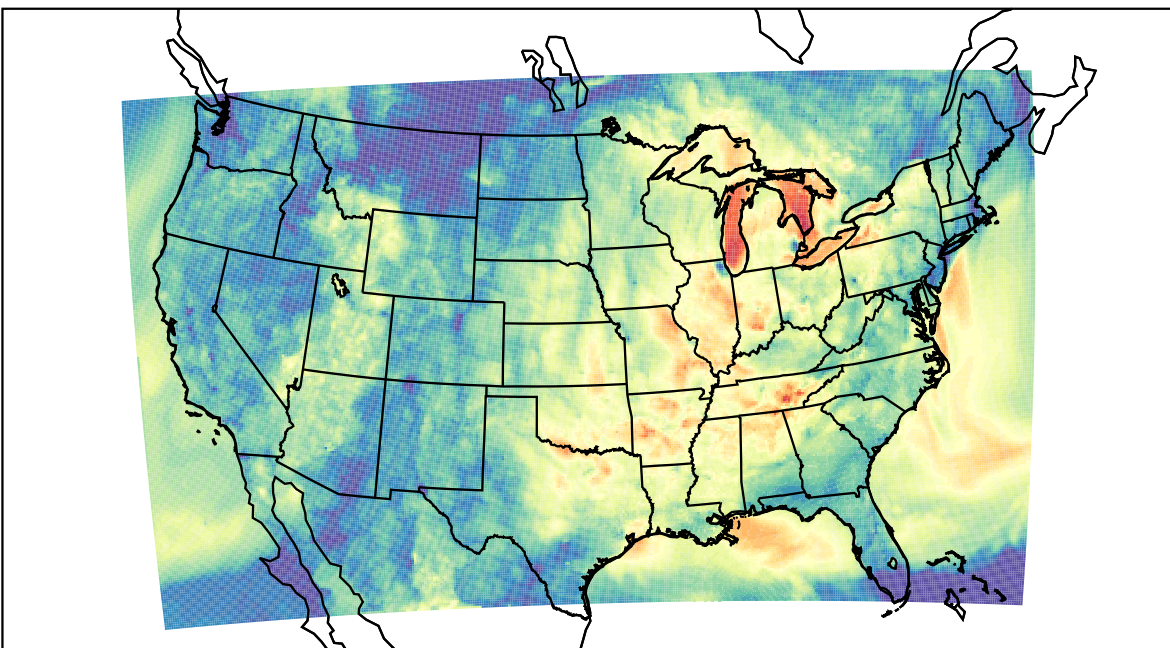
WRF (2023-10-02_04:00:00)
