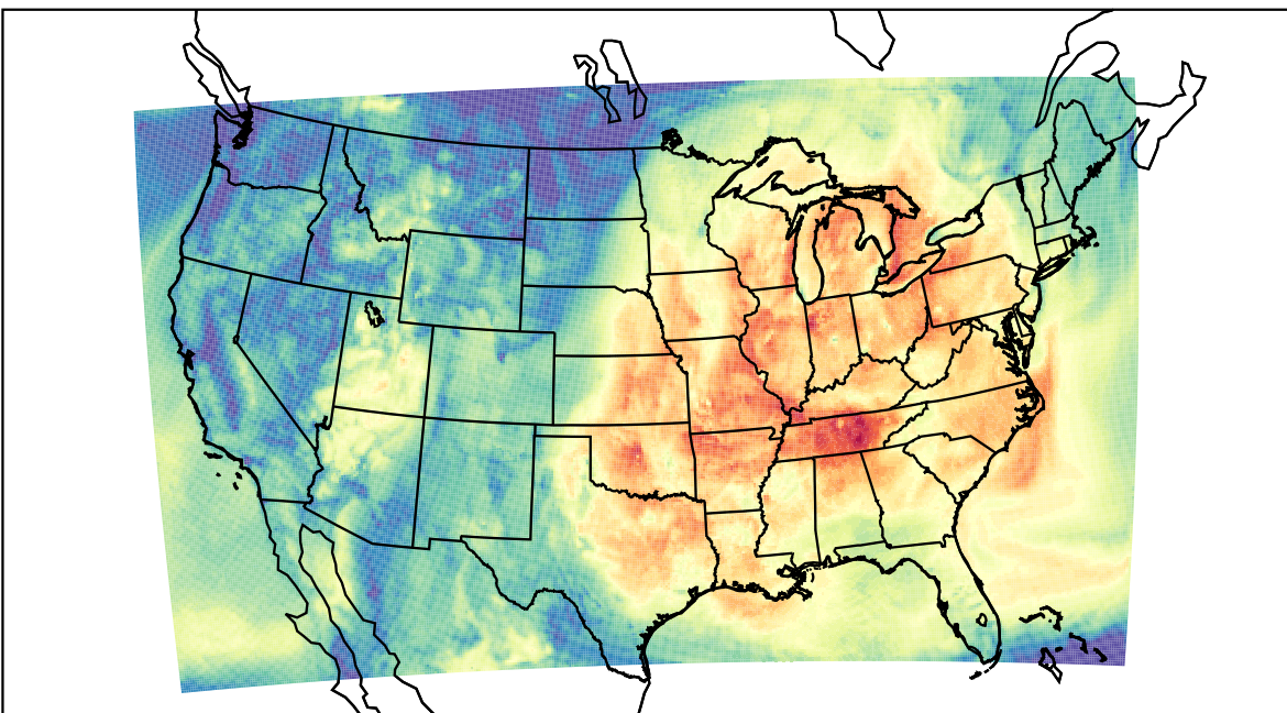
WRF (2023-10-02_16:00:00)
