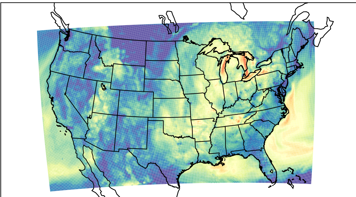
WRF (2023-10-02_11:00:00)
