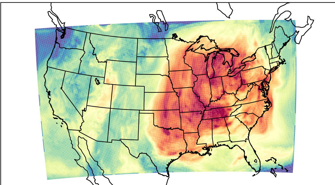
WRF (2023-10-02_20:00:00)
