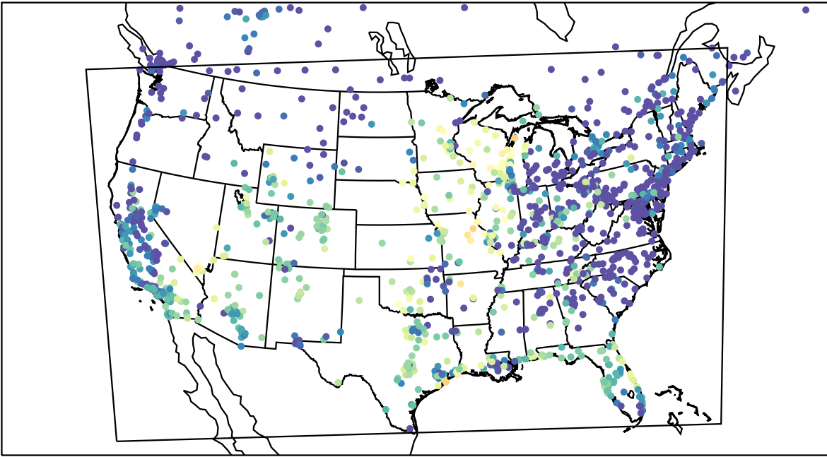
AirNOW (2023-10-02_03:00:00)
