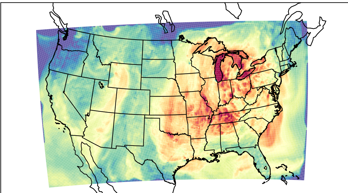
WRF (2023-10-03_00:00:00)
