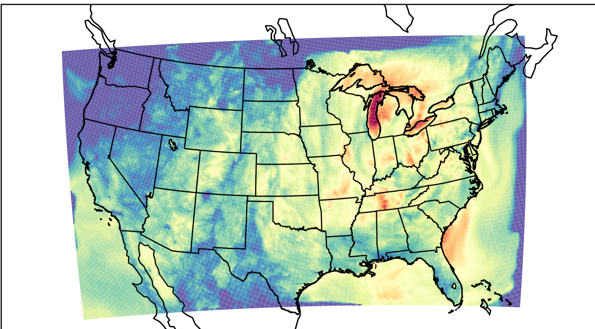
WRF (2023-10-03_07:00:00)
