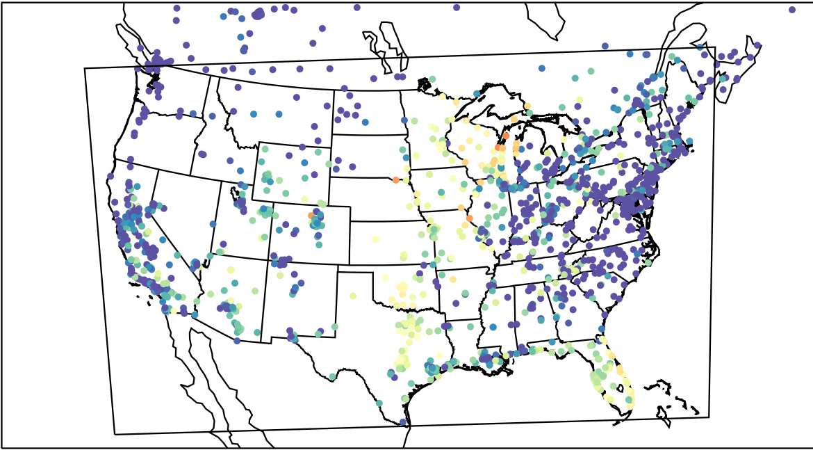
AirNOW (2023-10-03_04:00:00)
