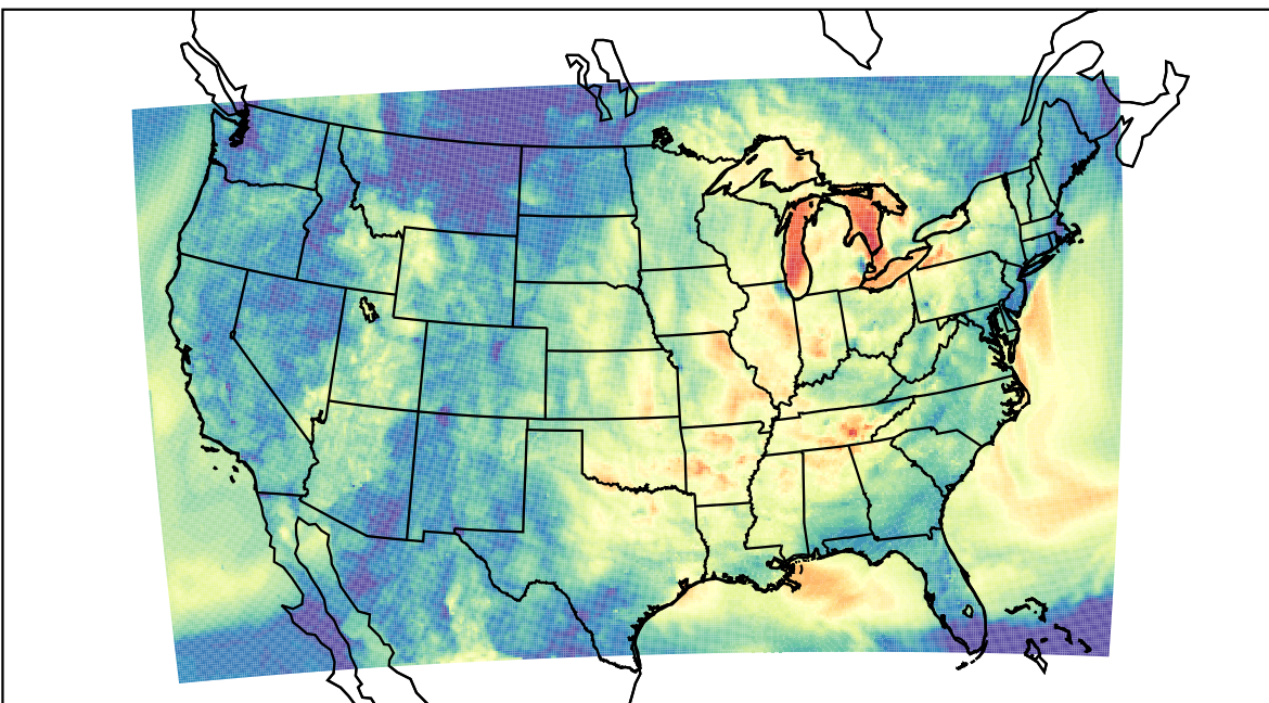
WRF (2023-10-02_05:00:00)
