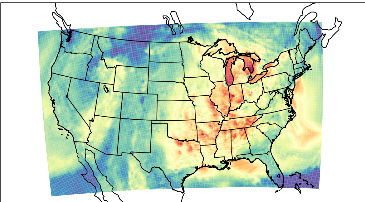
WRF (2023-10-02_01:00:00)
