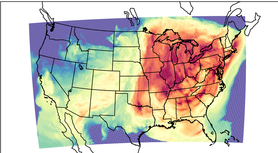
WRF (2023-10-03_21:00:00)
