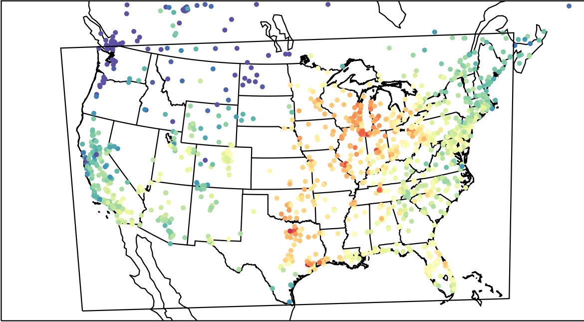
AirNOW (2023-10-02_19:00:00)
