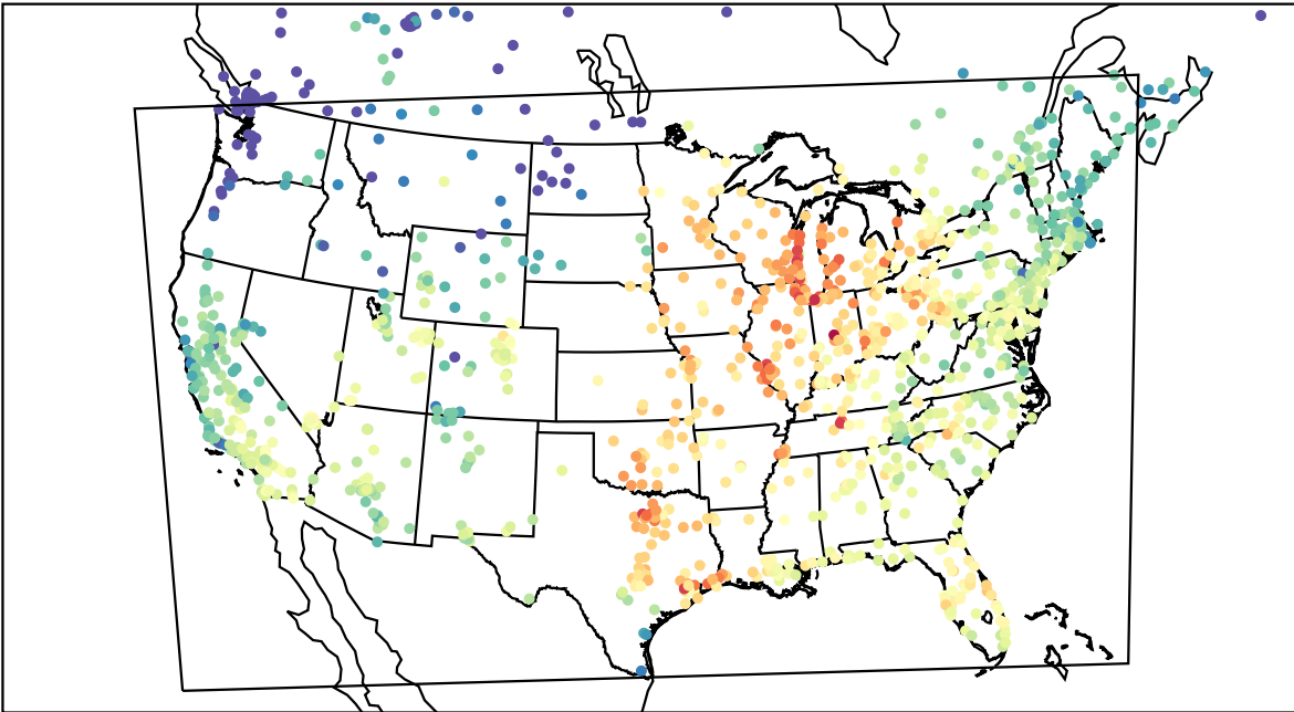
AirNOW (2023-10-02_20:00:00)
