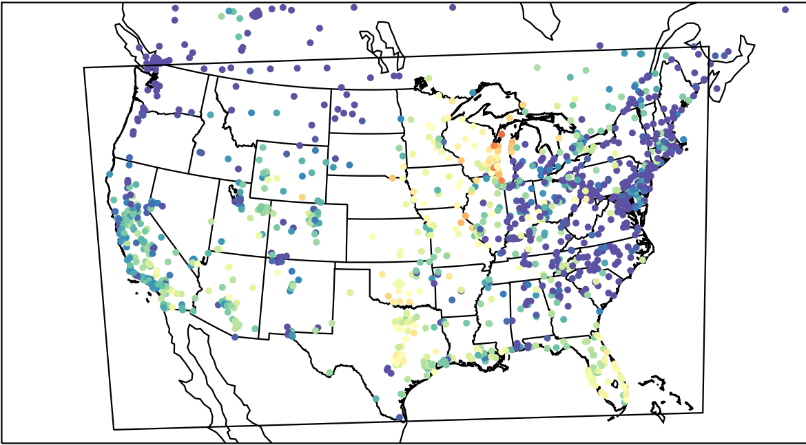
AirNOW (2023-10-03_02:00:00)
