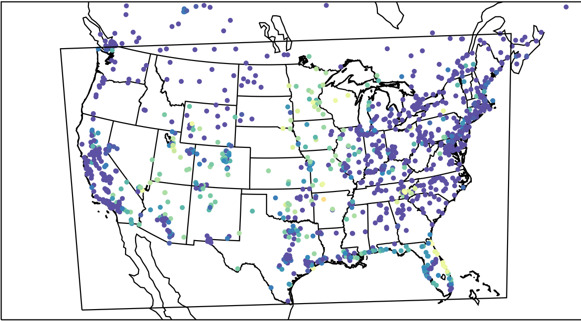
AirNOW (2023-10-02_10:00:00)
