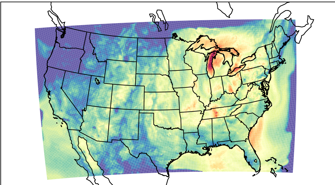
WRF (2023-10-03_08:00:00)
