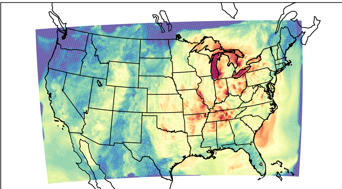
WRF (2023-10-03_02:00:00)
