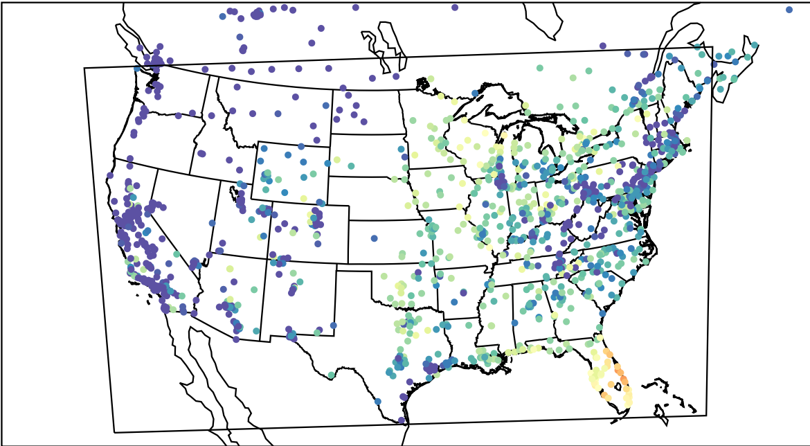
AirNOW (2023-10-03_14:00:00)
