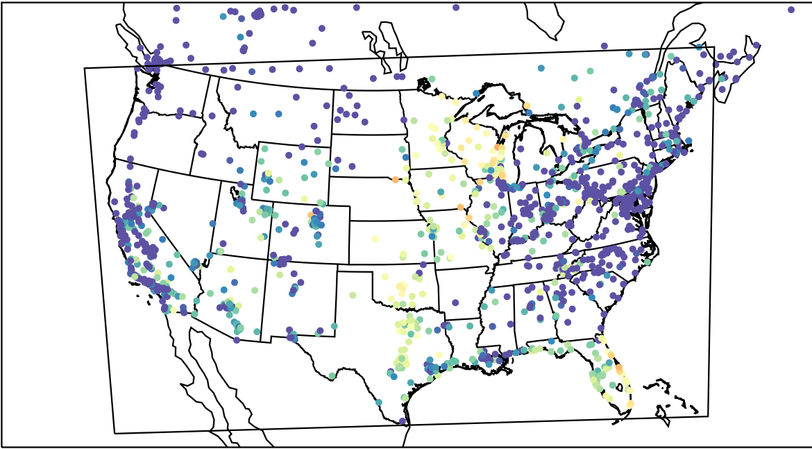
AirNOW (2023-10-03_05:00:00)
