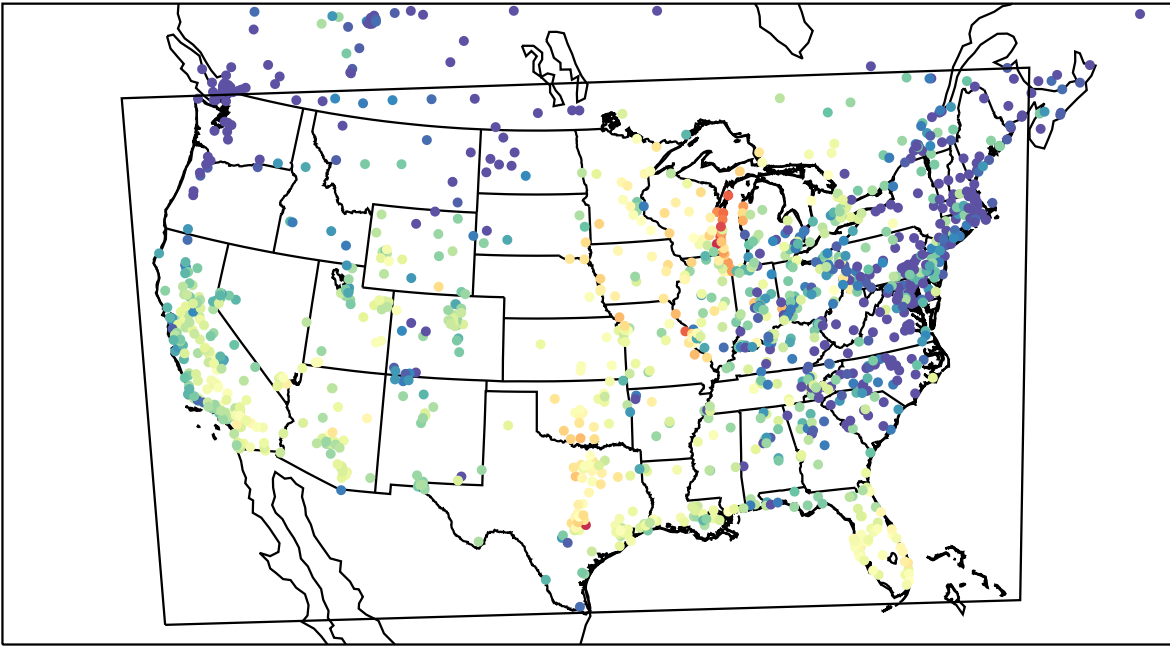
AirNOW (2023-10-03_00:00:00)
