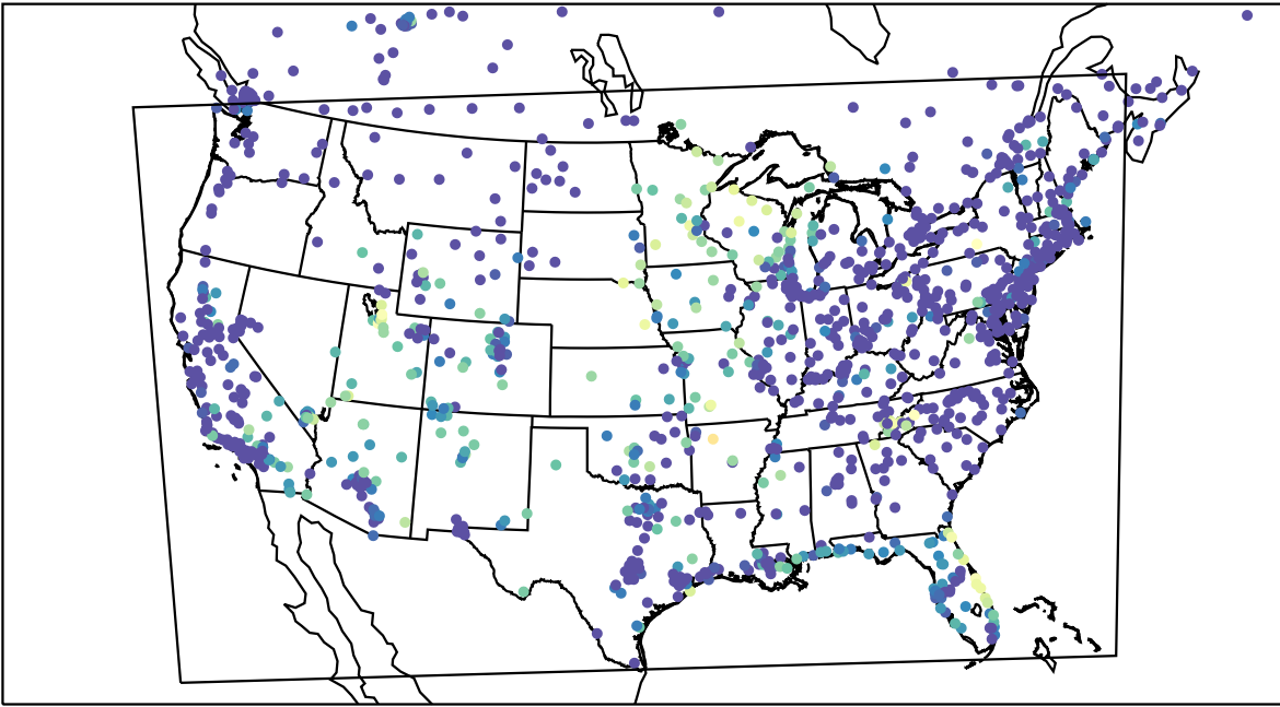
AirNOW (2023-10-02_11:00:00)
