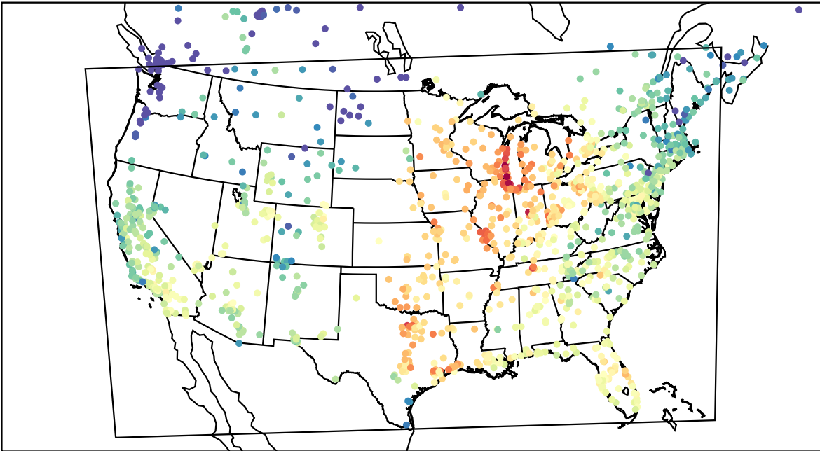
AirNOW (2023-10-02_21:00:00)
