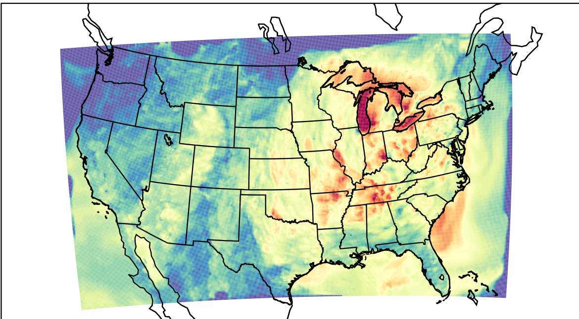
WRF (2023-10-03_03:00:00)
