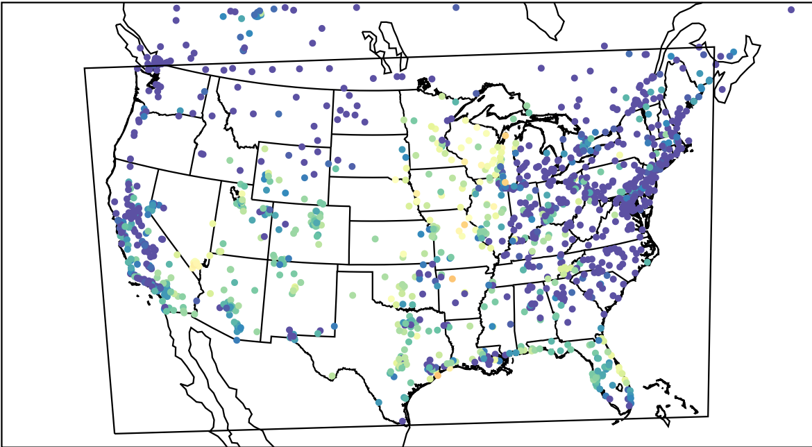
AirNOW (2023-10-02_04:00:00)
