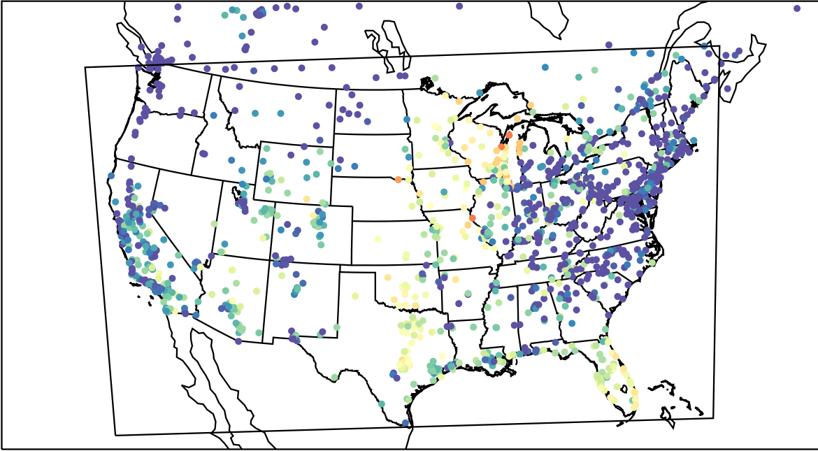
AirNOW (2023-10-03_03:00:00)
