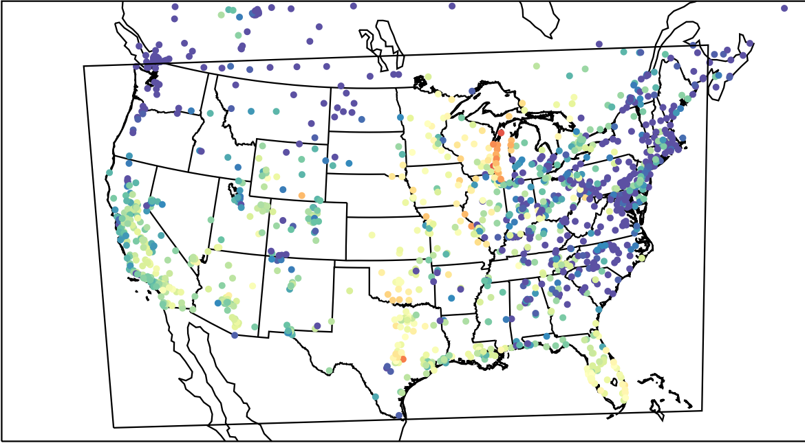
AirNOW (2023-10-03_01:00:00)
