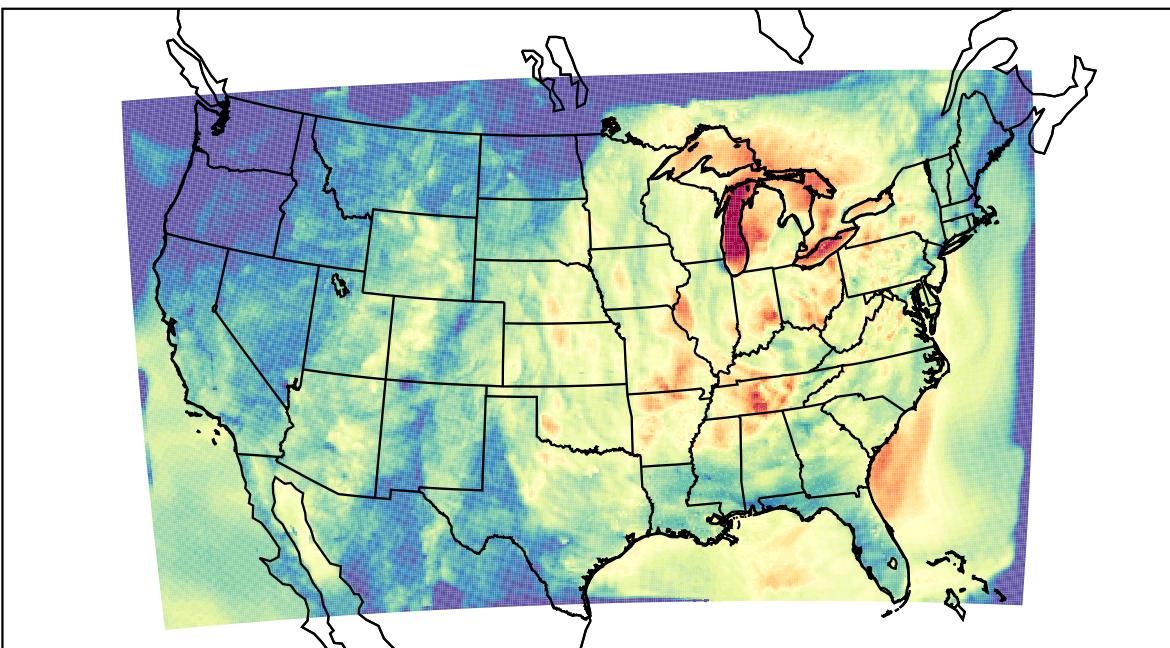
WRF (2023-10-03_05:00:00)
