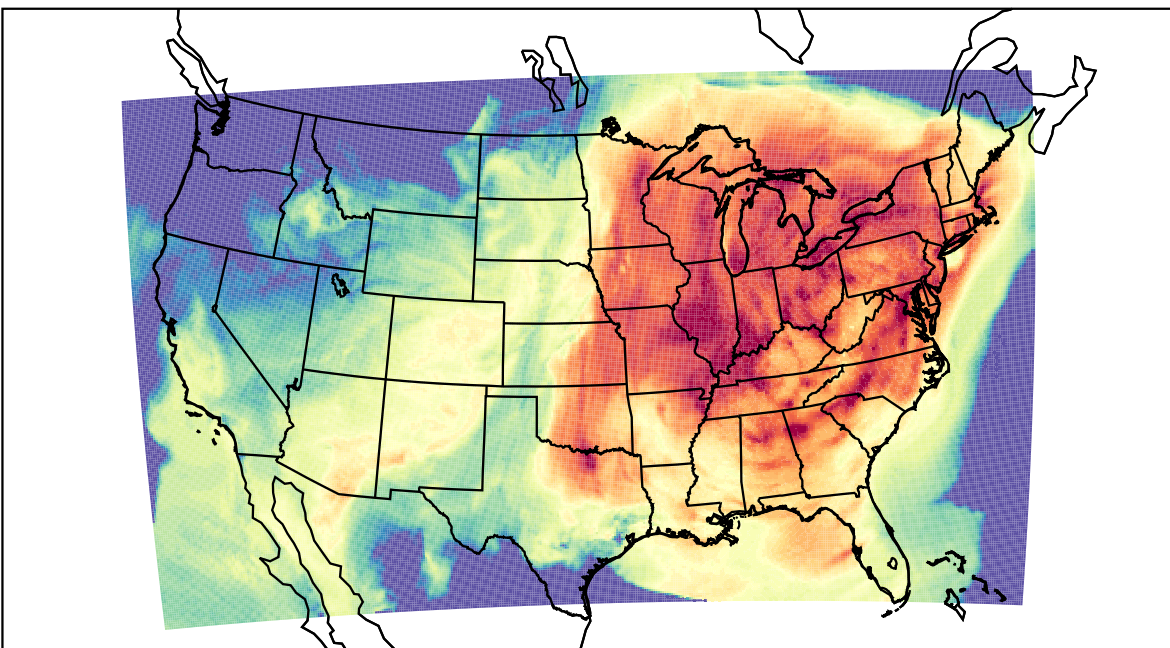
WRF (2023-10-03_19:00:00)
