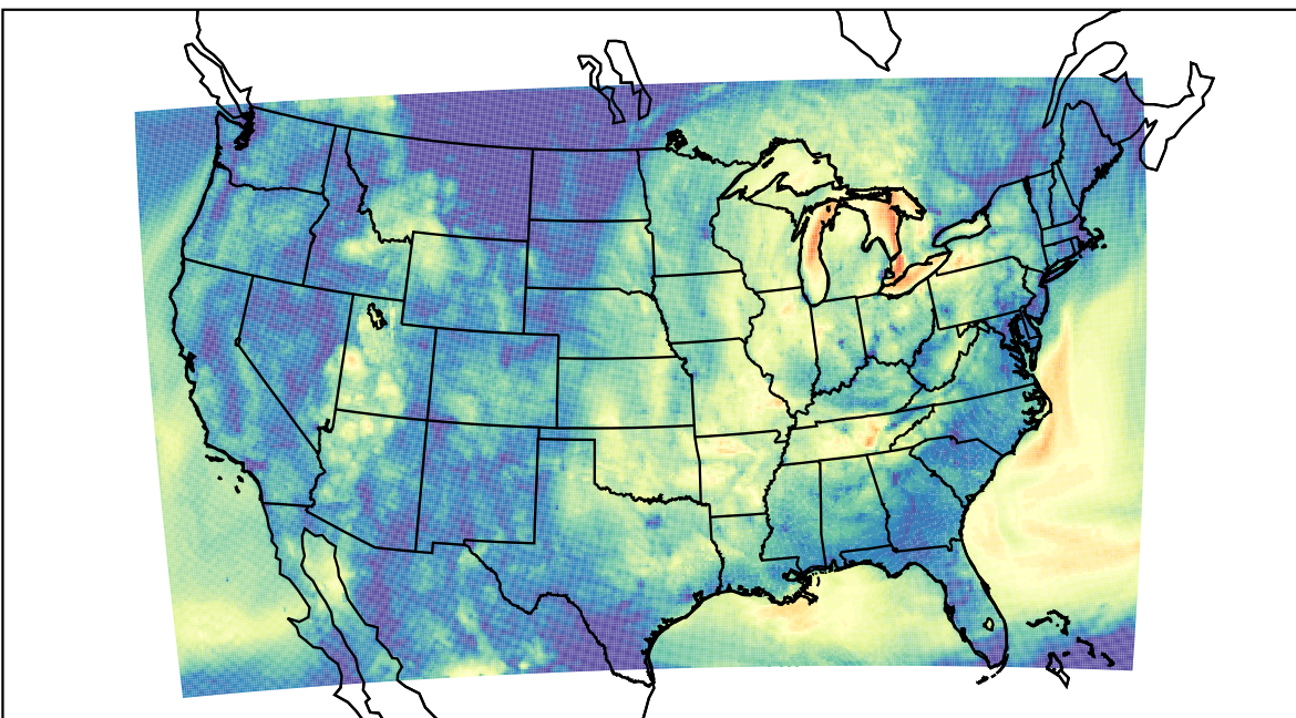
WRF (2023-10-02_12:00:00)
