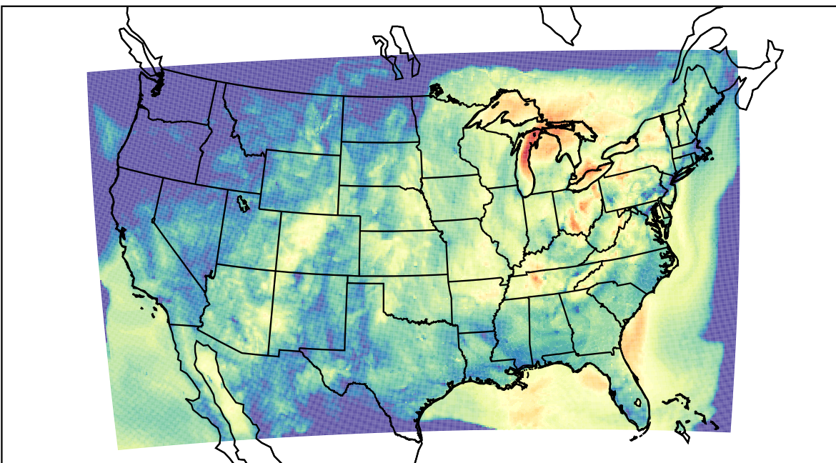
WRF (2023-10-03_11:00:00)
