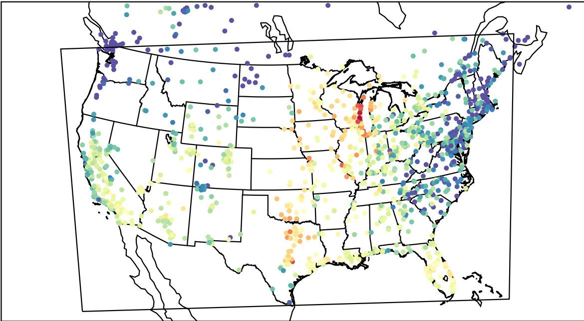
AirNOW (2023-10-02_23:00:00)
