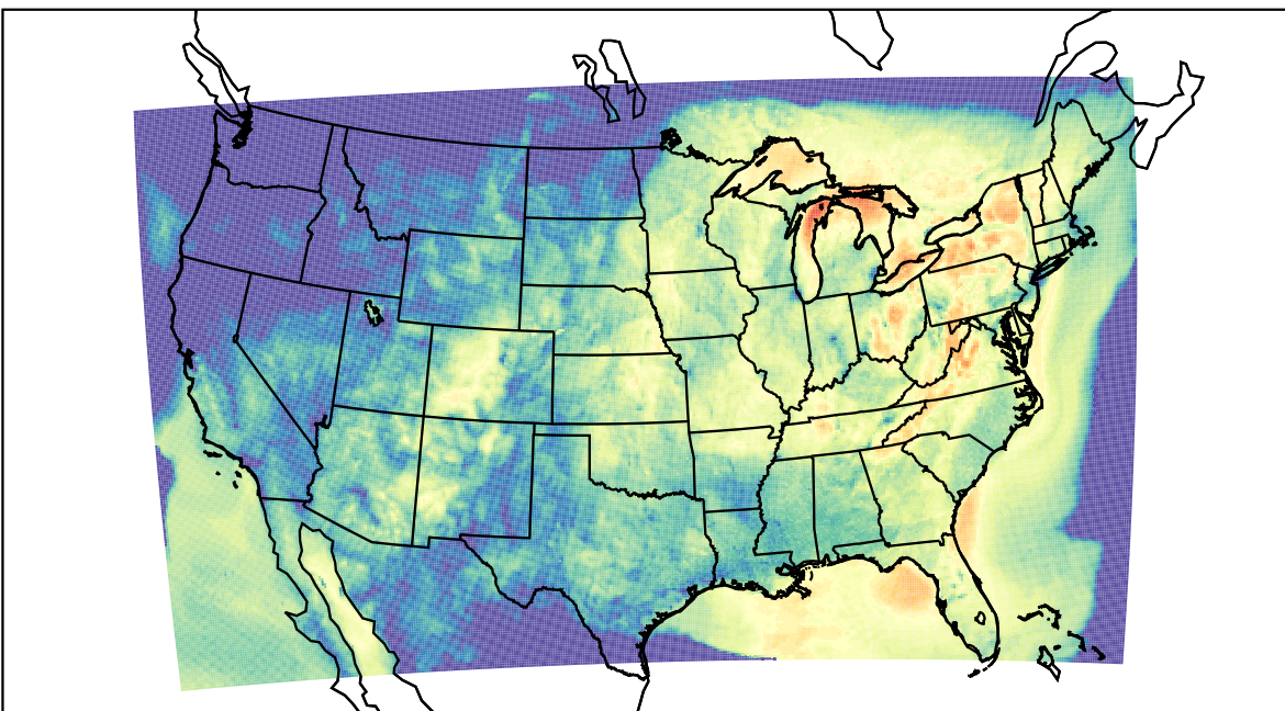
WRF (2023-10-03_14:00:00)
