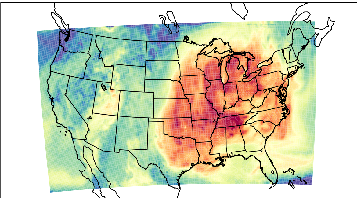
WRF (2023-10-02_18:00:00)
