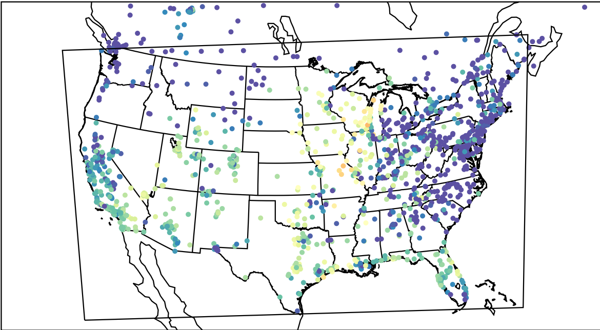
AirNOW (2023-10-02_02:00:00)
