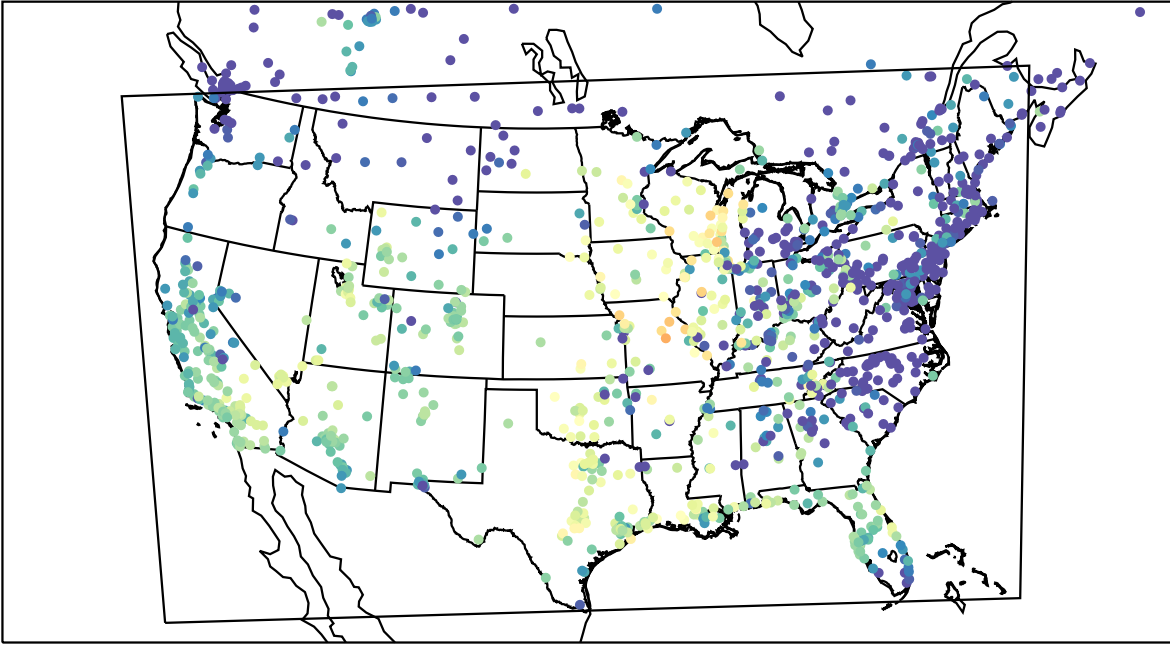
AirNOW (2023-10-02_01:00:00)
