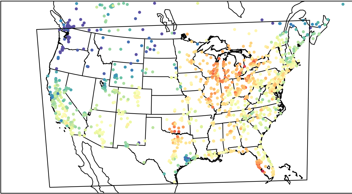
AirNOW (2023-10-03_19:00:00)
