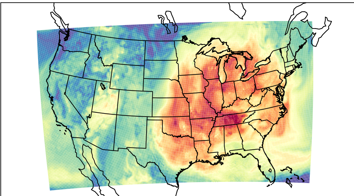
WRF (2023-10-02_17:00:00)
