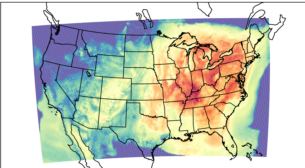
WRF (2023-10-03_16:00:00)
