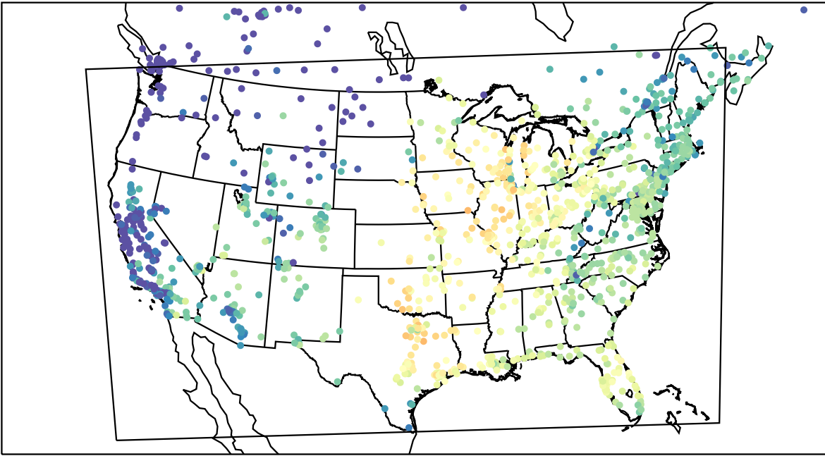
AirNOW (2023-10-02_16:00:00)
