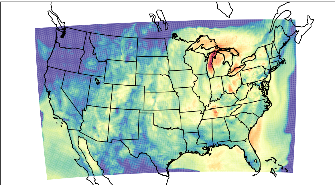
WRF (2023-10-03_09:00:00)
