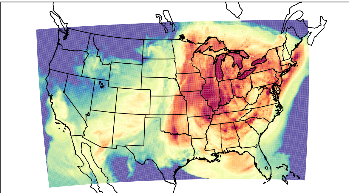
WRF (2023-10-03_22:00:00)
