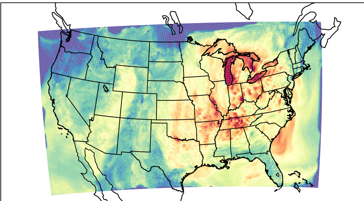
WRF (2023-10-03_01:00:00)
