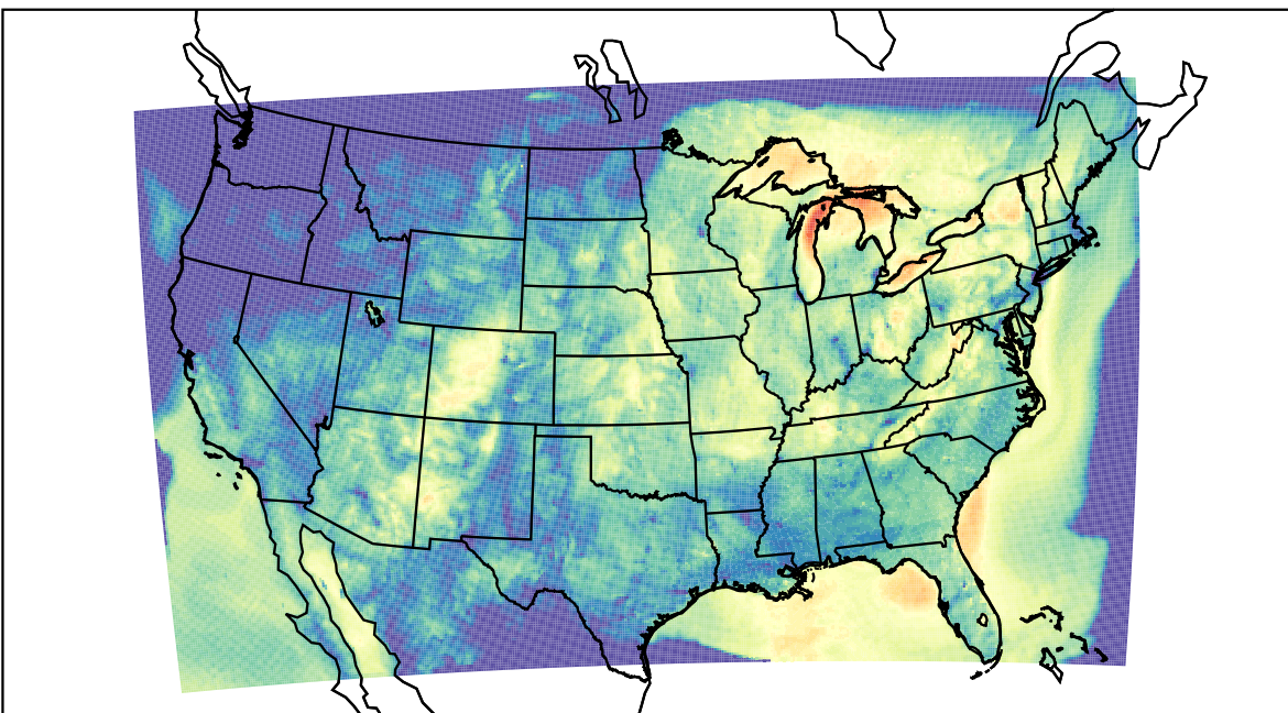
WRF (2023-10-03_13:00:00)
