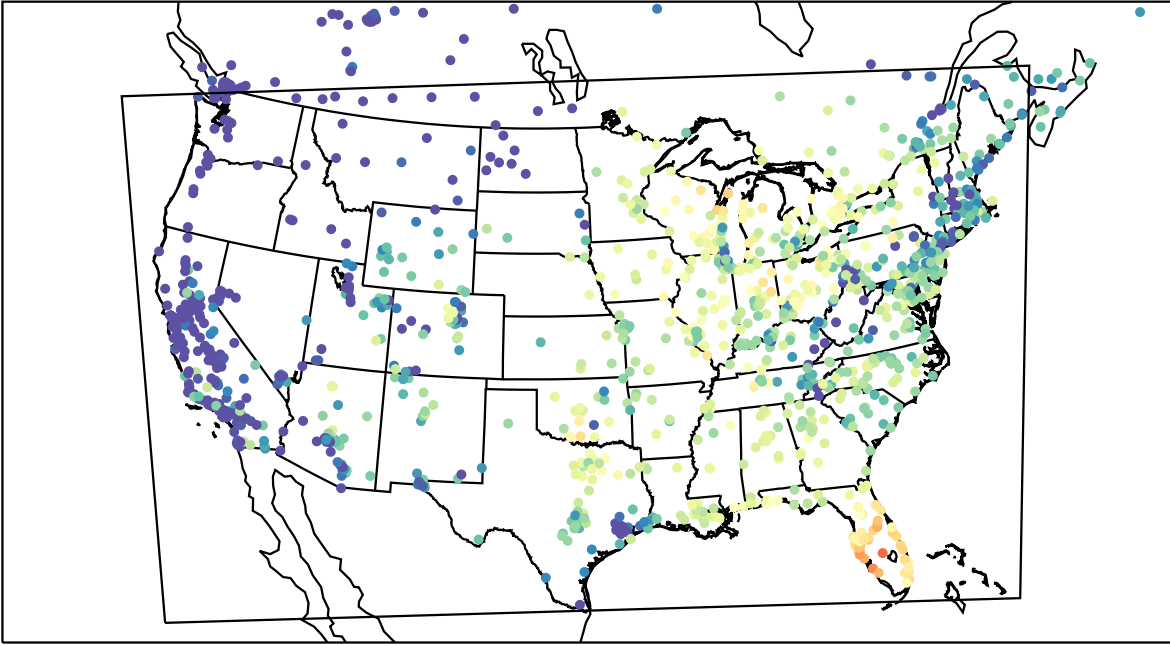
AirNOW (2023-10-03_15:00:00)
