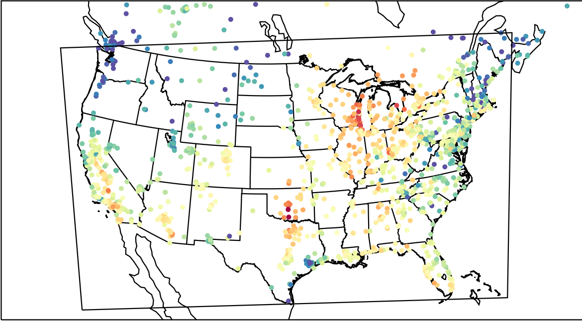
AirNOW (2023-10-03_22:00:00)
