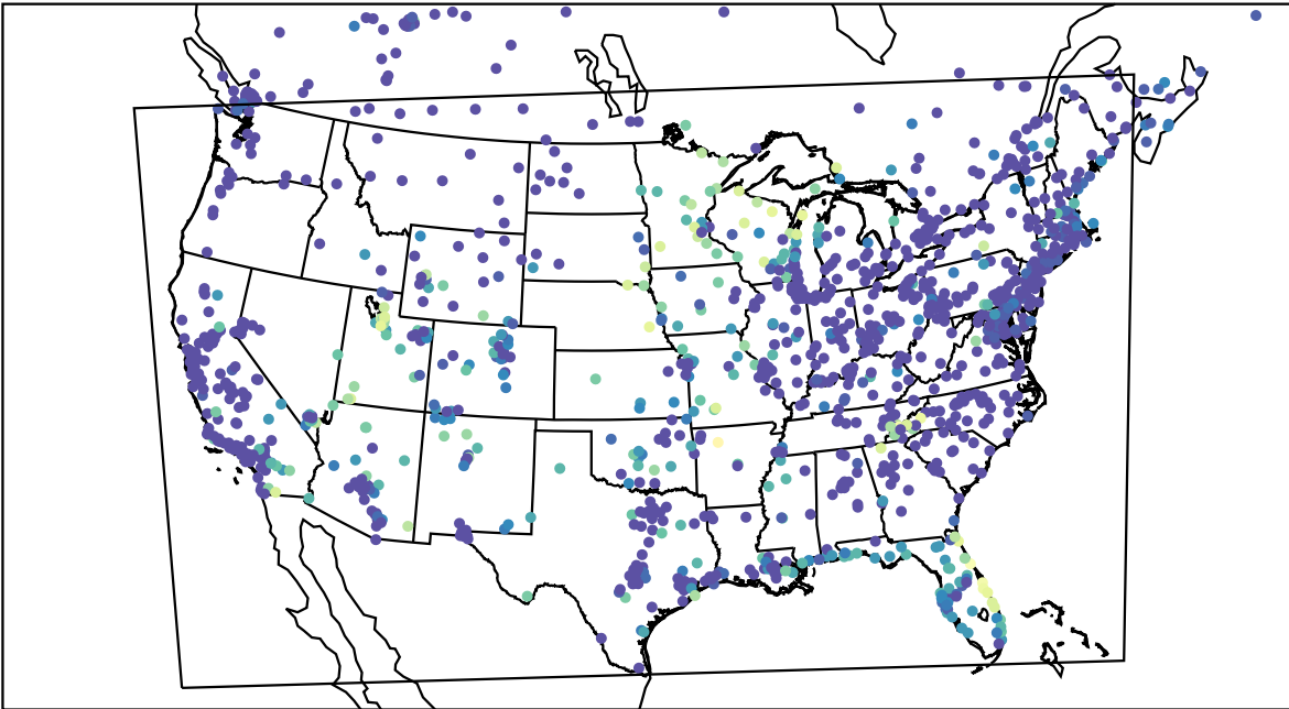
AirNOW (2023-10-02_12:00:00)
