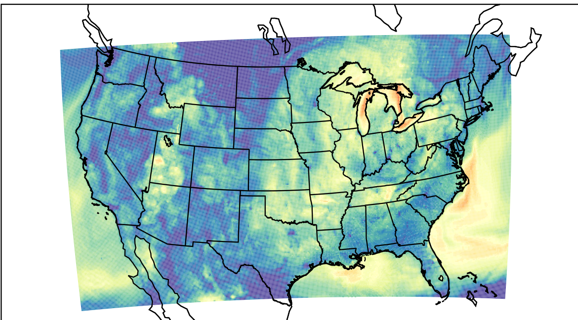
WRF (2023-10-02_13:00:00)
