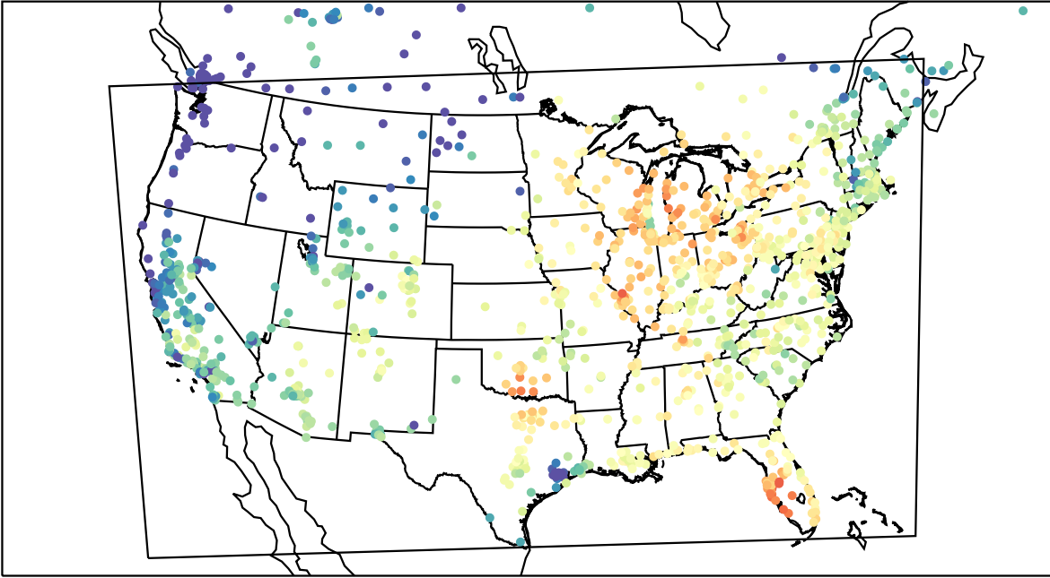
AirNOW (2023-10-03_17:00:00)
