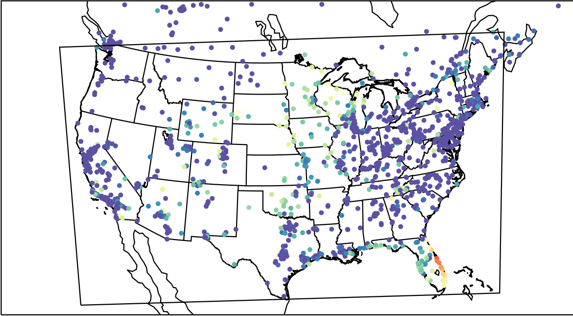
AirNOW (2023-10-03_12:00:00)
