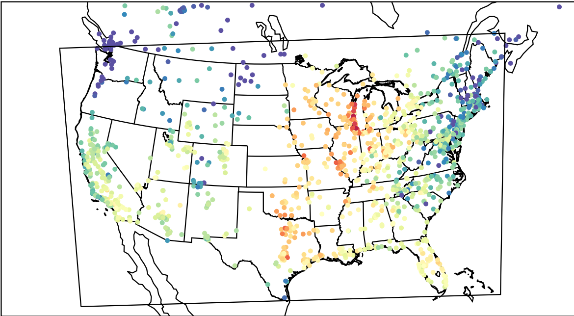
AirNOW (2023-10-02_22:00:00)
