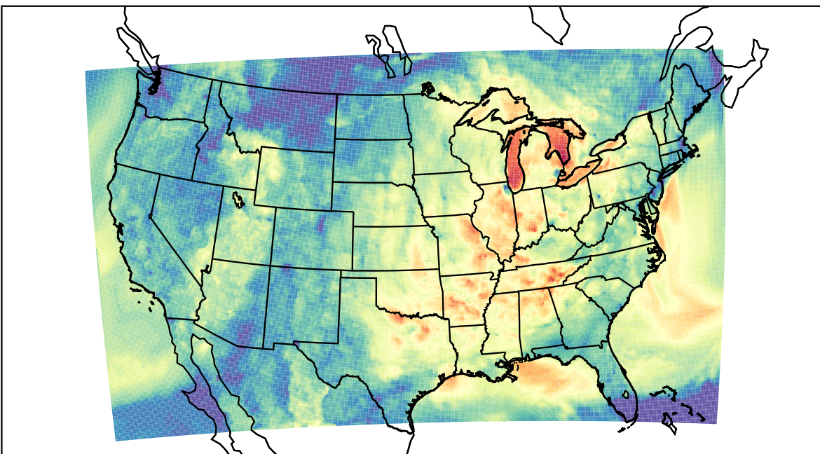
WRF (2023-10-02_03:00:00)
