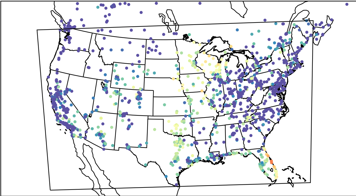
AirNOW (2023-10-03_07:00:00)
