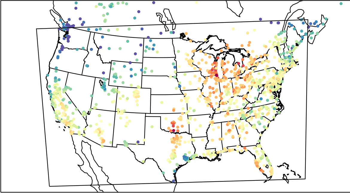
AirNOW (2023-10-03_21:00:00)
