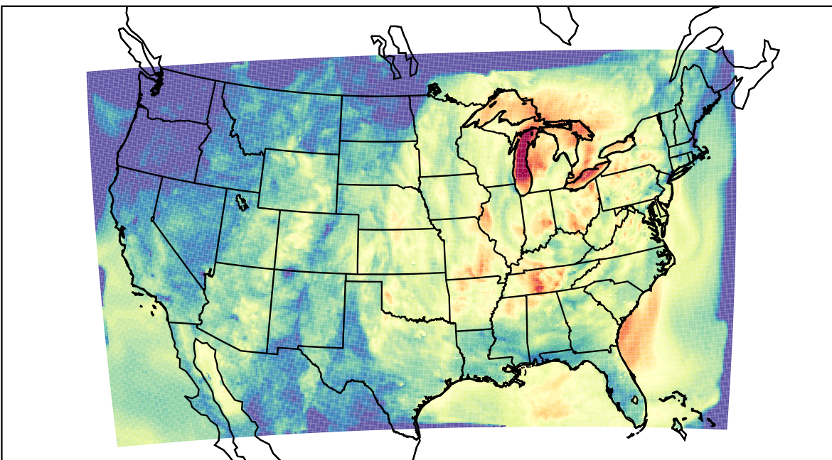
WRF (2023-10-03_06:00:00)
