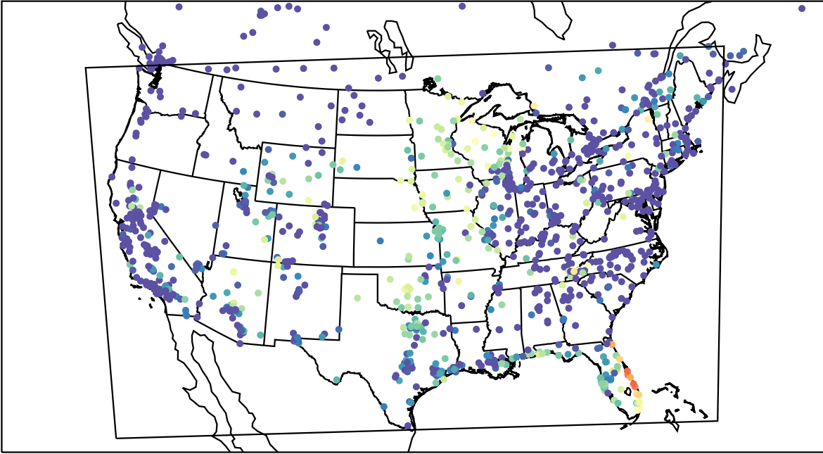
AirNOW (2023-10-03_10:00:00)
