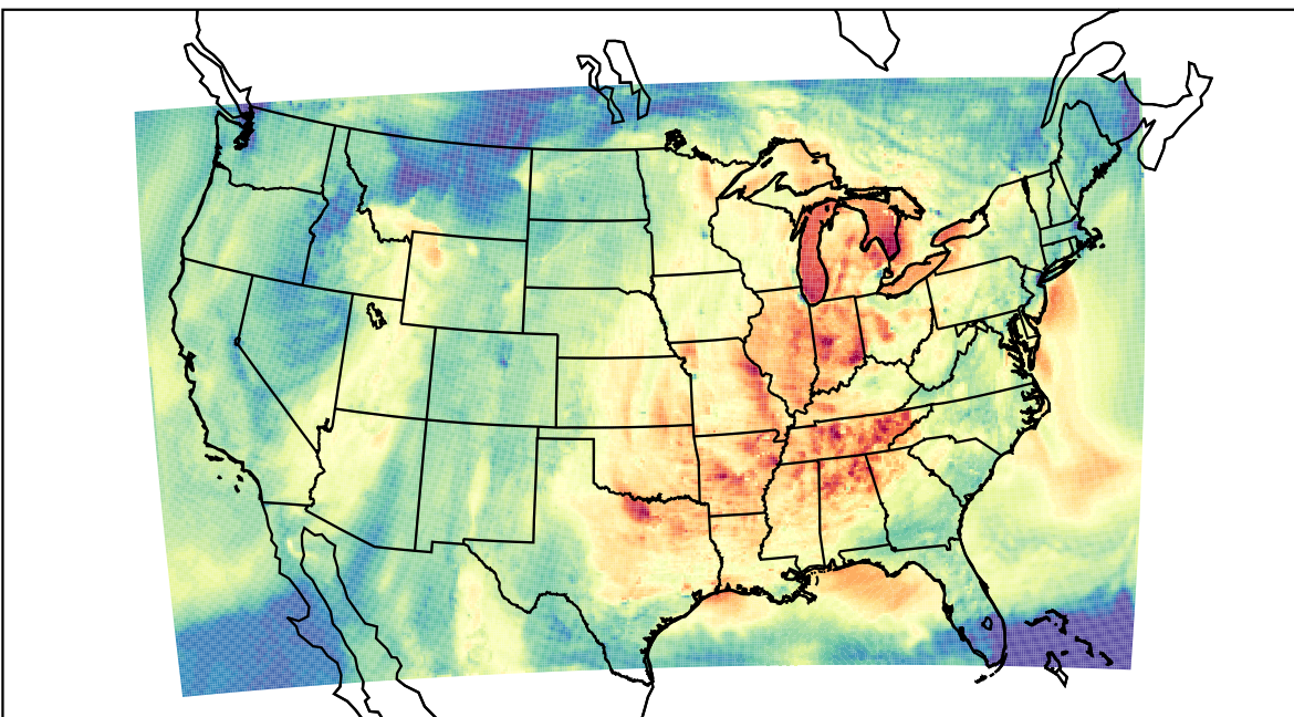
WRF (2023-10-02_00:00:00)
