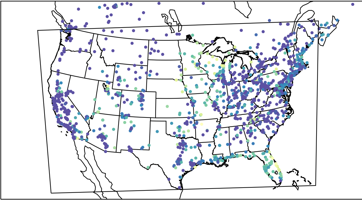
AirNOW (2023-10-02_13:00:00)
