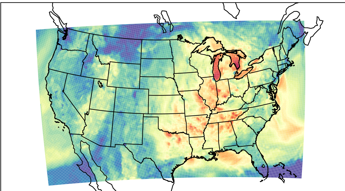
WRF (2023-10-02_02:00:00)
