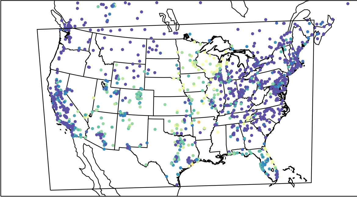
AirNOW (2023-10-02_07:00:00)
