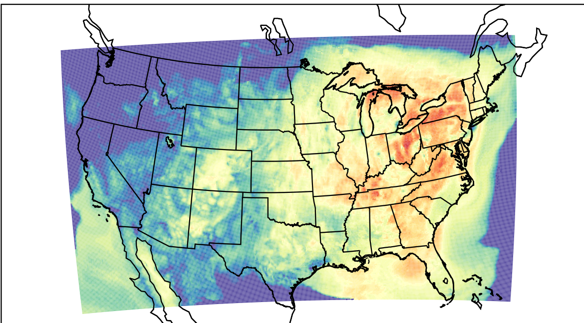
WRF (2023-10-03_15:00:00)
