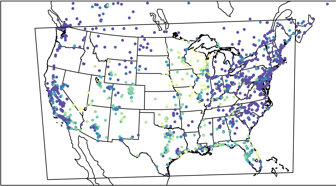
AirNOW (2023-10-02_05:00:00)
