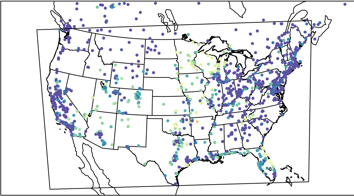
AirNOW (2023-10-02_08:00:00)
