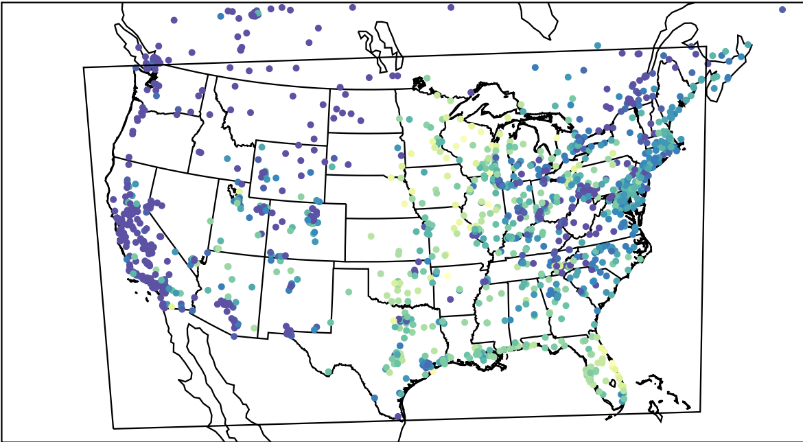
AirNOW (2023-10-02_14:00:00)
