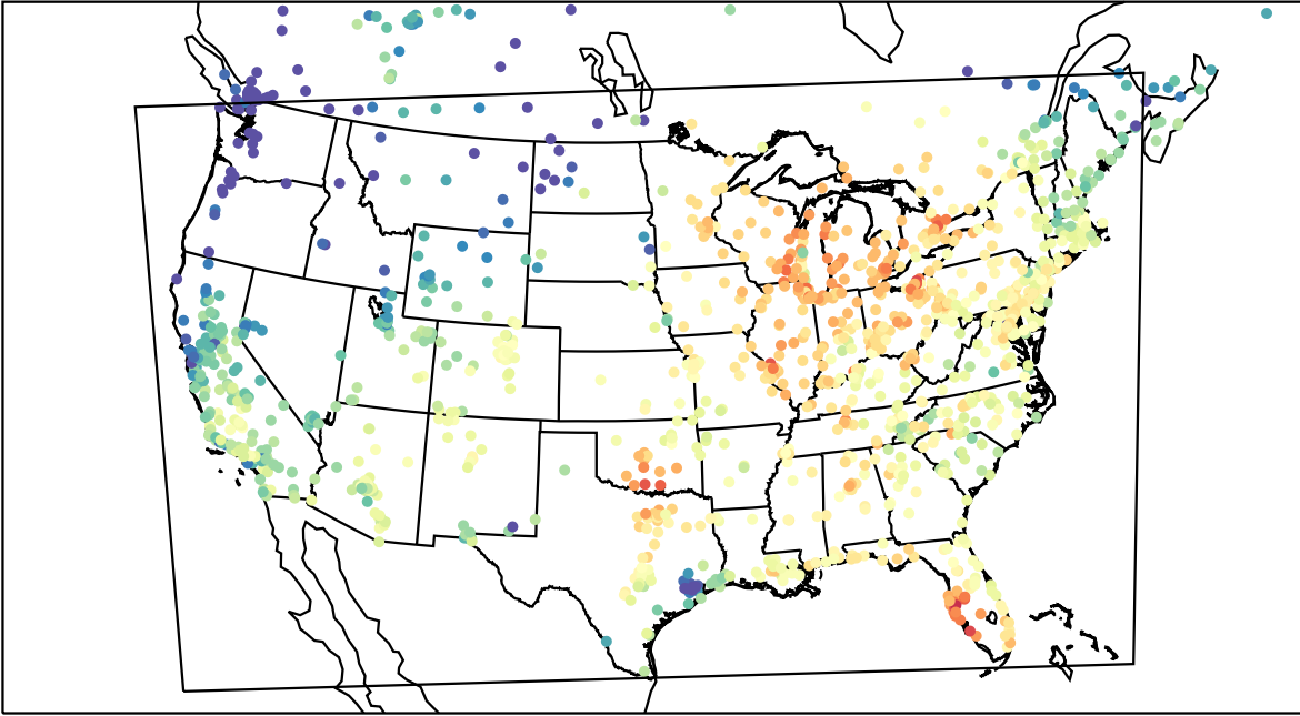
AirNOW (2023-10-03_18:00:00)
