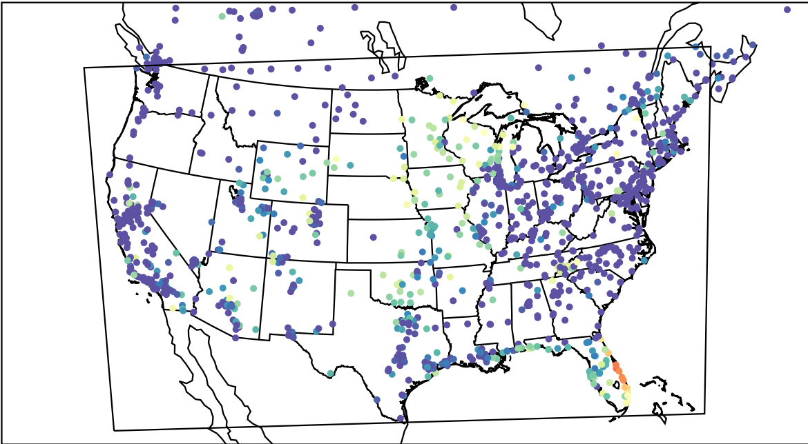
AirNOW (2023-10-03_11:00:00)
