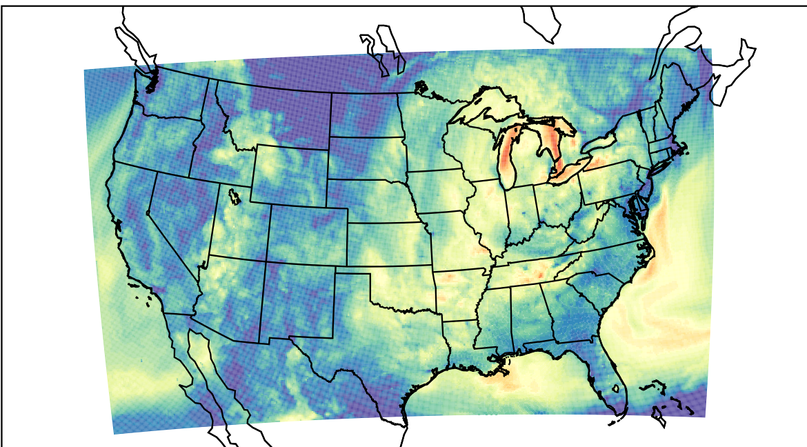
WRF (2023-10-02_10:00:00)
