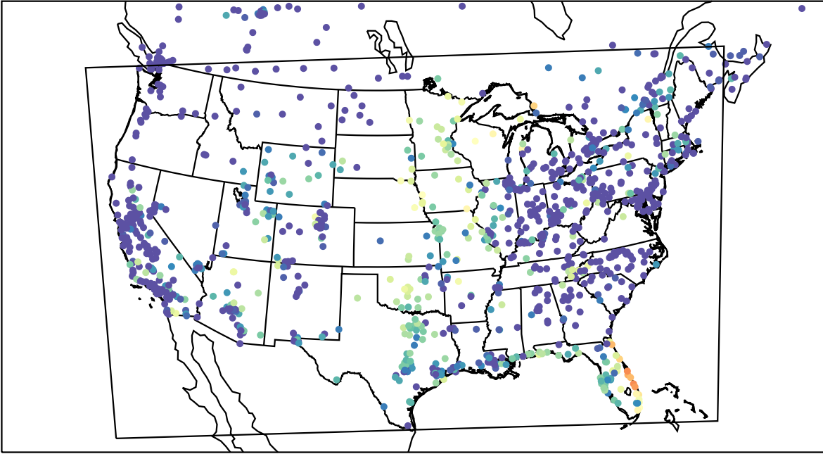
AirNOW (2023-10-03_09:00:00)
