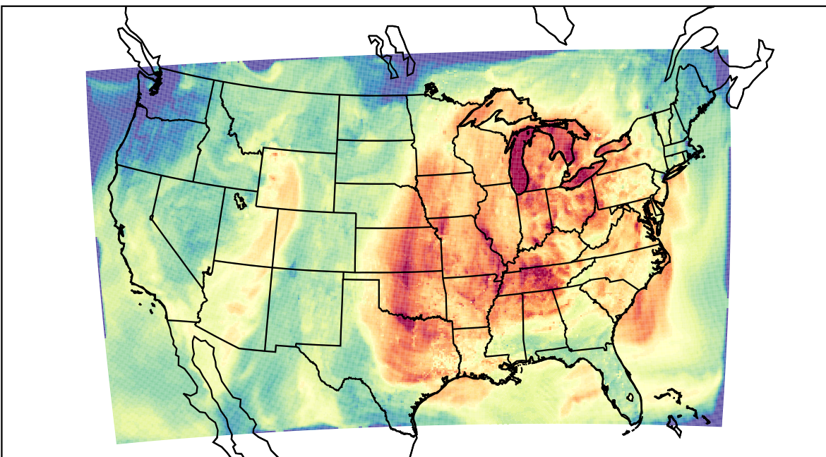
WRF (2023-10-02_23:00:00)
