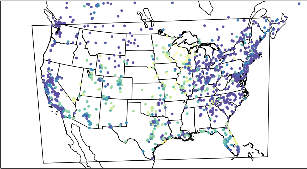
AirNOW (2023-10-02_06:00:00)
