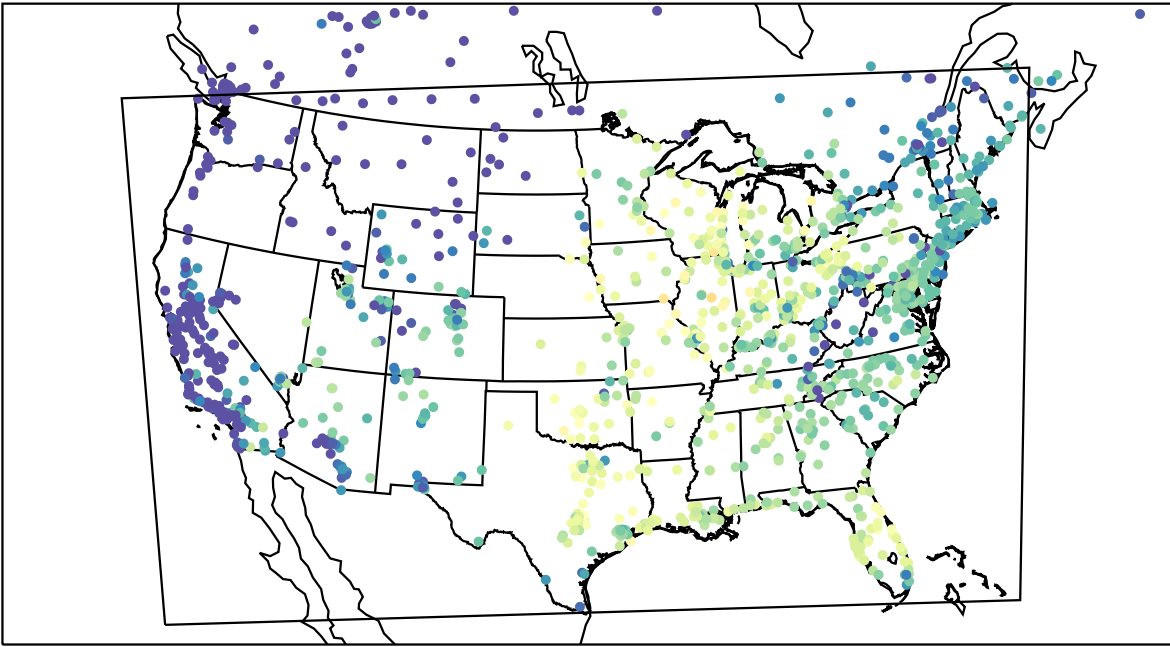
AirNOW (2023-10-02_15:00:00)
