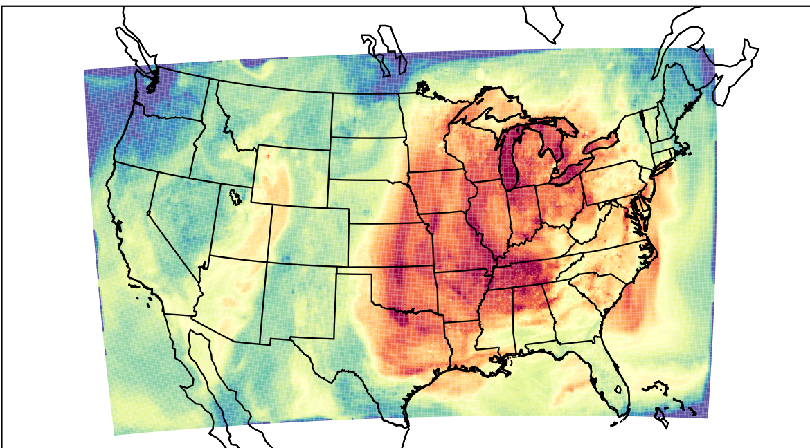
WRF (2023-10-02_22:00:00)
