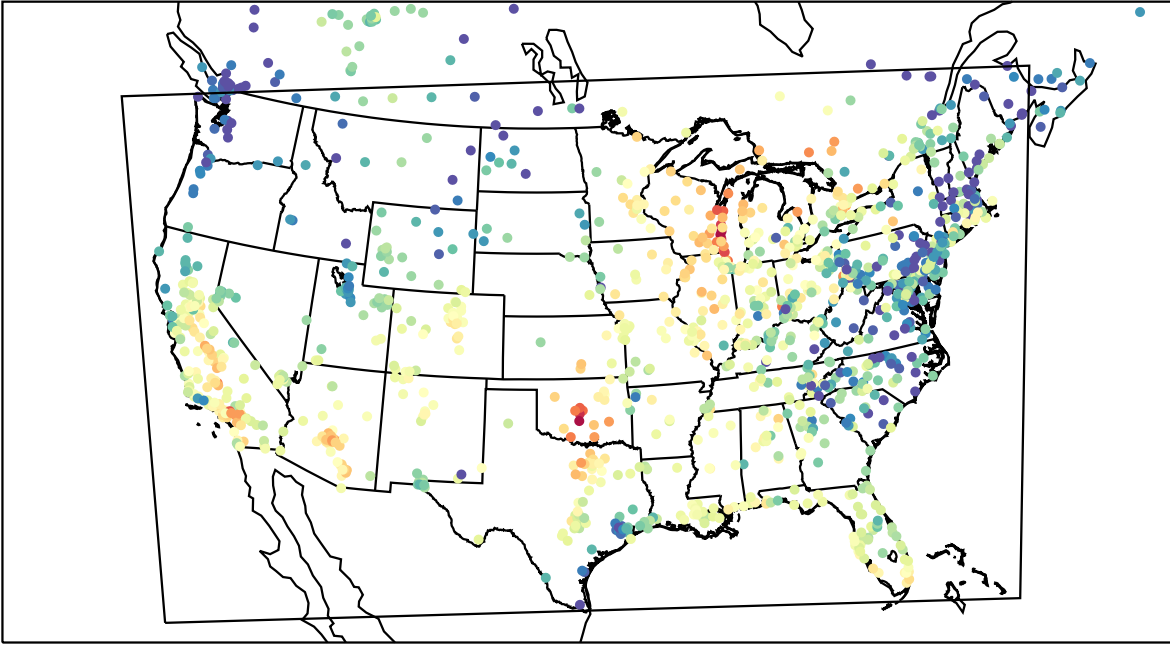
AirNOW (2023-10-03_23:00:00)
