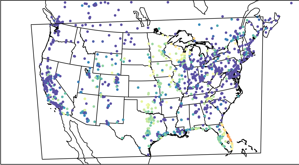
AirNOW (2023-10-03_08:00:00)
