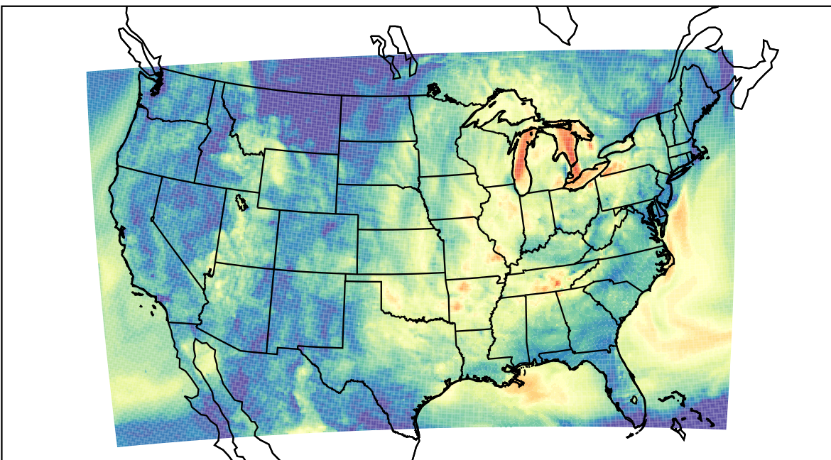
WRF (2023-10-02_08:00:00)
