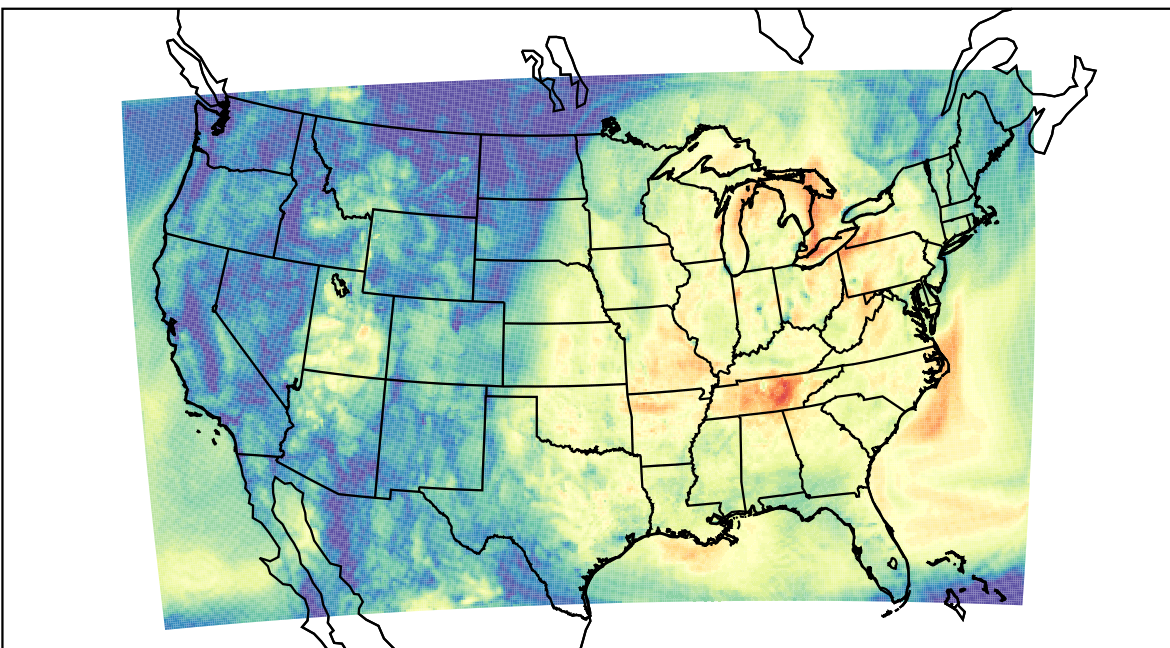
WRF (2023-10-02_15:00:00)
