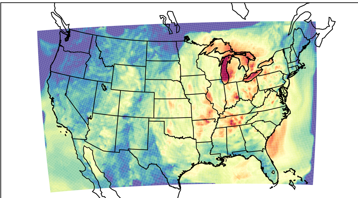
WRF (2023-10-03_04:00:00)
