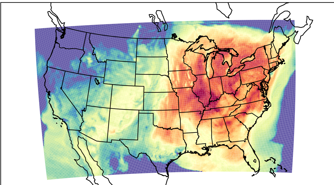
WRF (2023-10-03_17:00:00)
