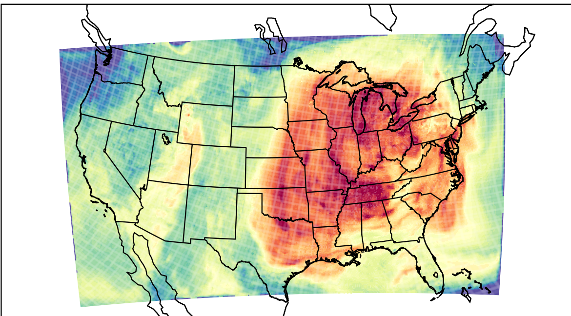
WRF (2023-10-02_21:00:00)
