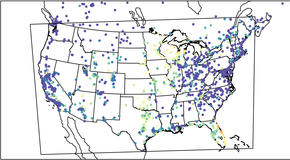
AirNOW (2023-10-03_06:00:00)
