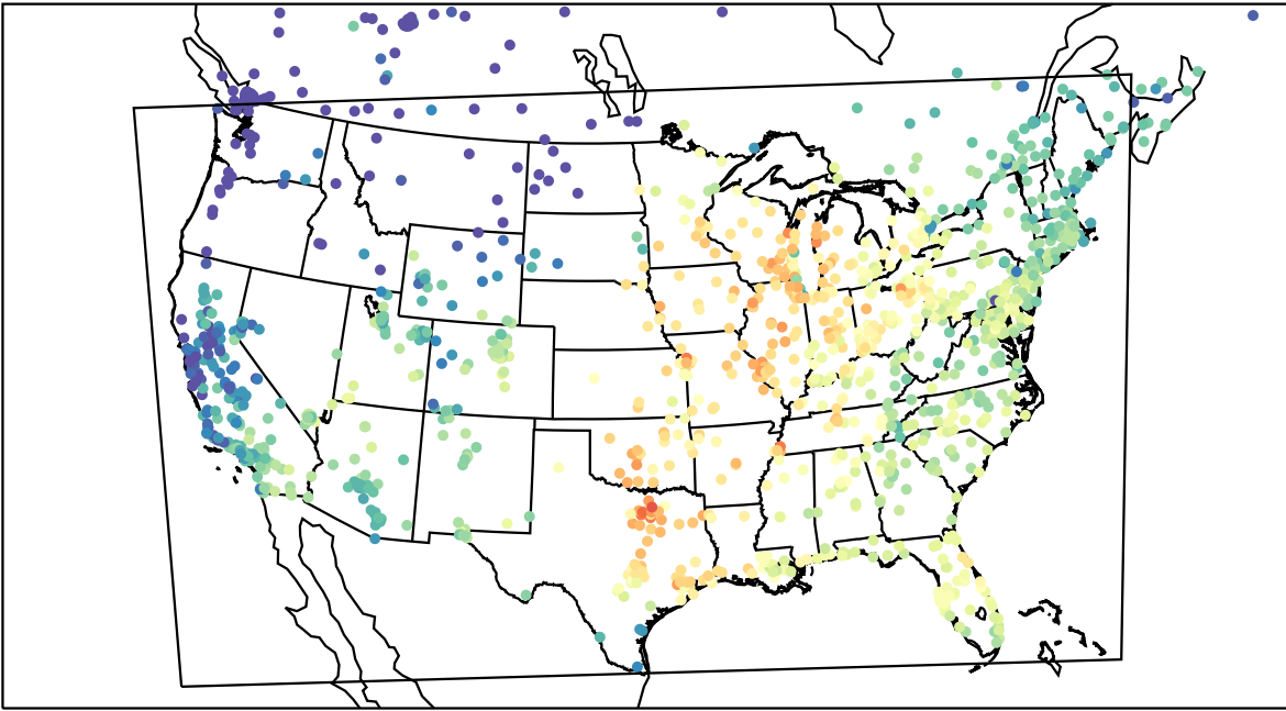
AirNOW (2023-10-02_17:00:00)
