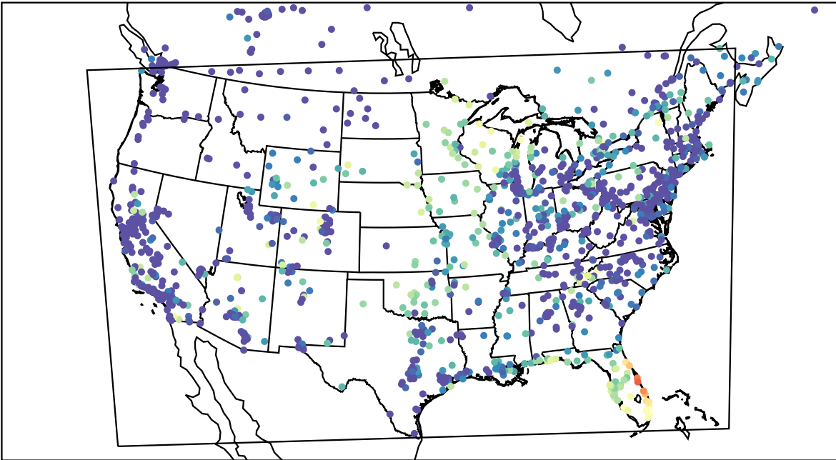
AirNOW (2023-10-03_13:00:00)
