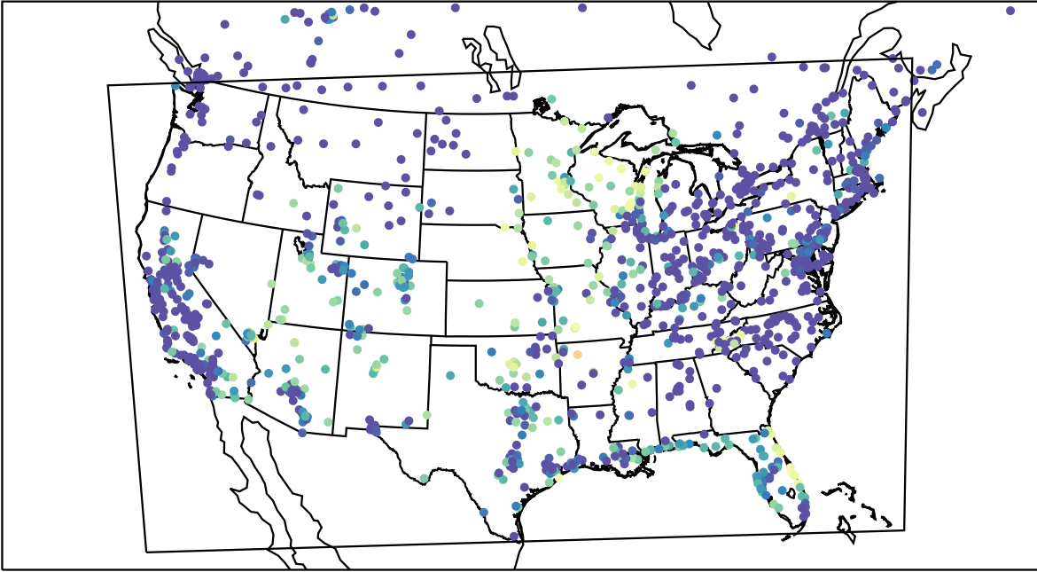
AirNOW (2023-10-02_09:00:00)
