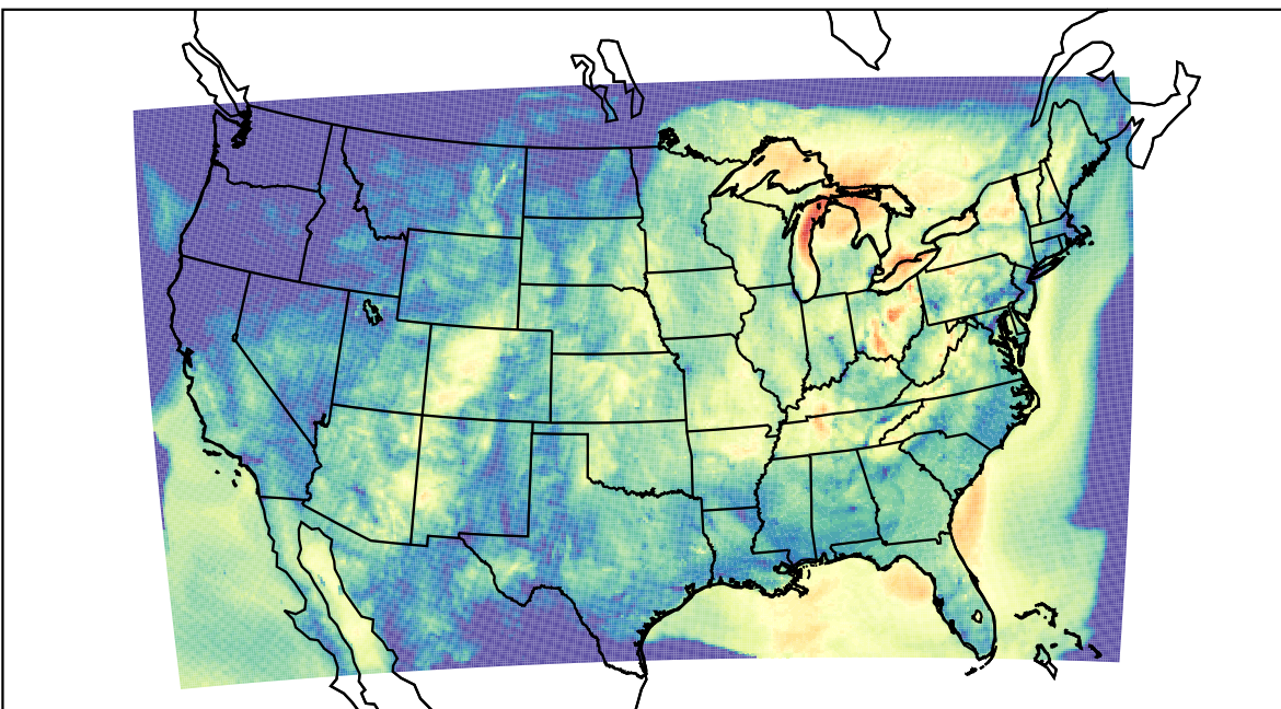
WRF (2023-10-03_12:00:00)
