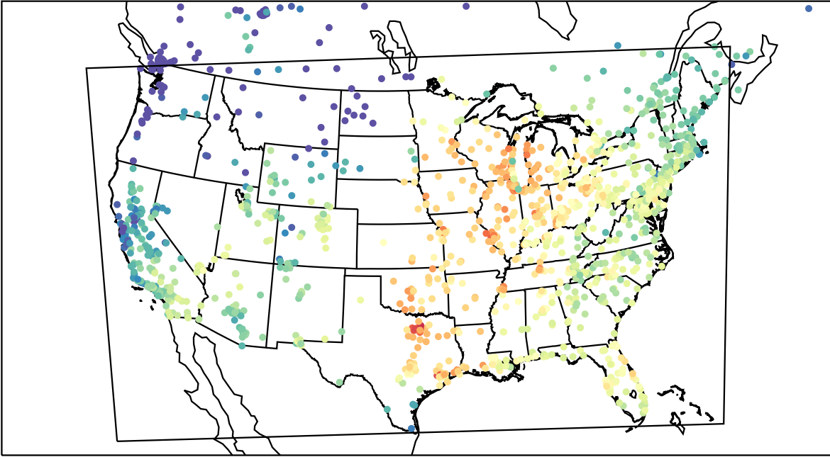
AirNOW (2023-10-02_18:00:00)
