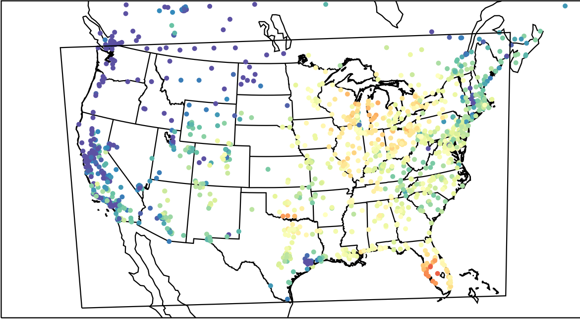
AirNOW (2023-10-03_16:00:00)
