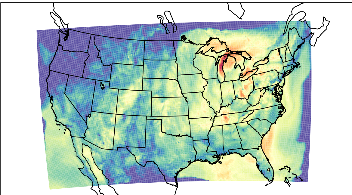
WRF (2023-10-03_10:00:00)
