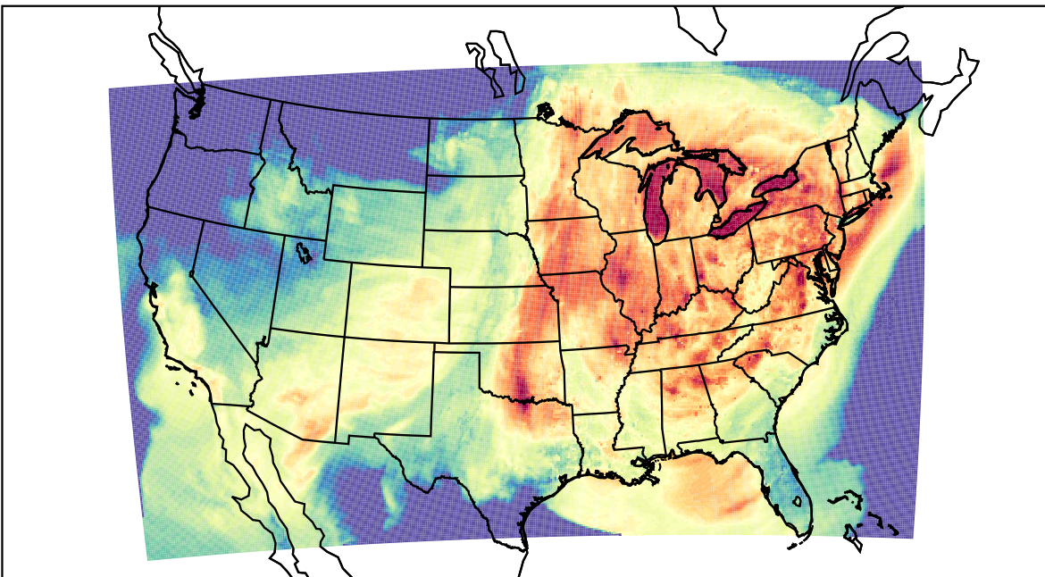
WRF (2023-10-03_23:00:00)
