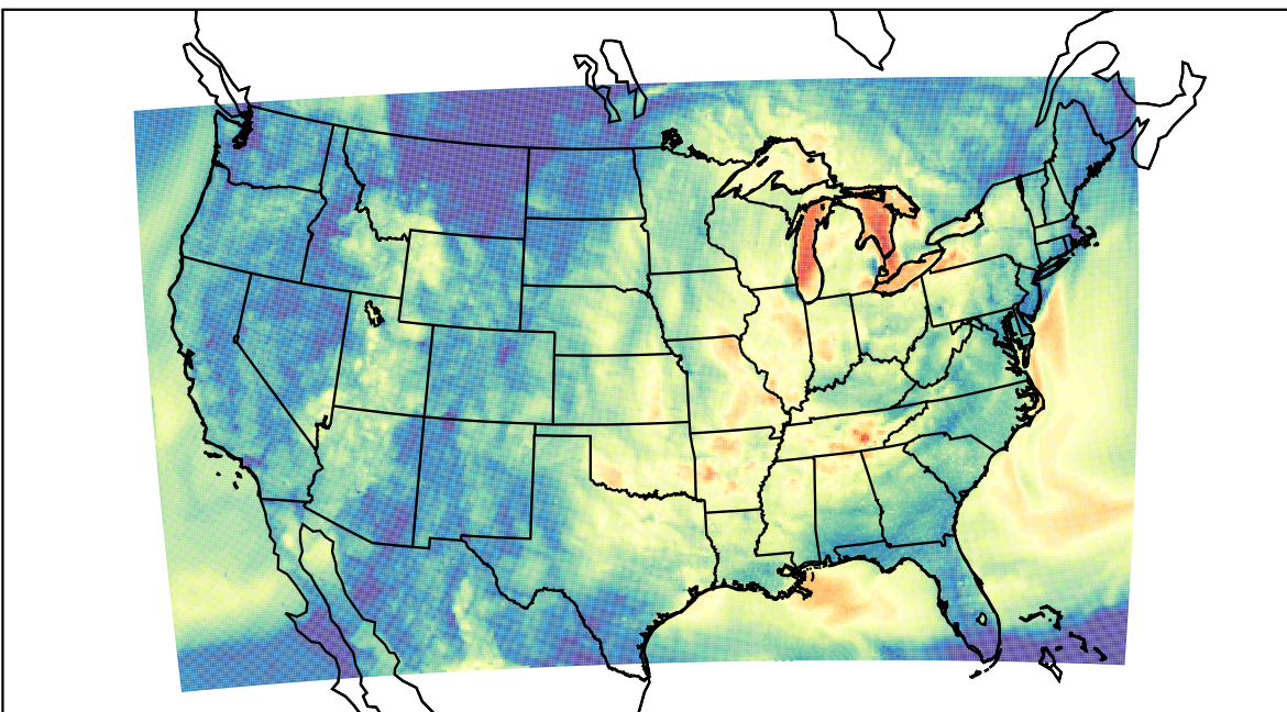
WRF (2023-10-02_06:00:00)
