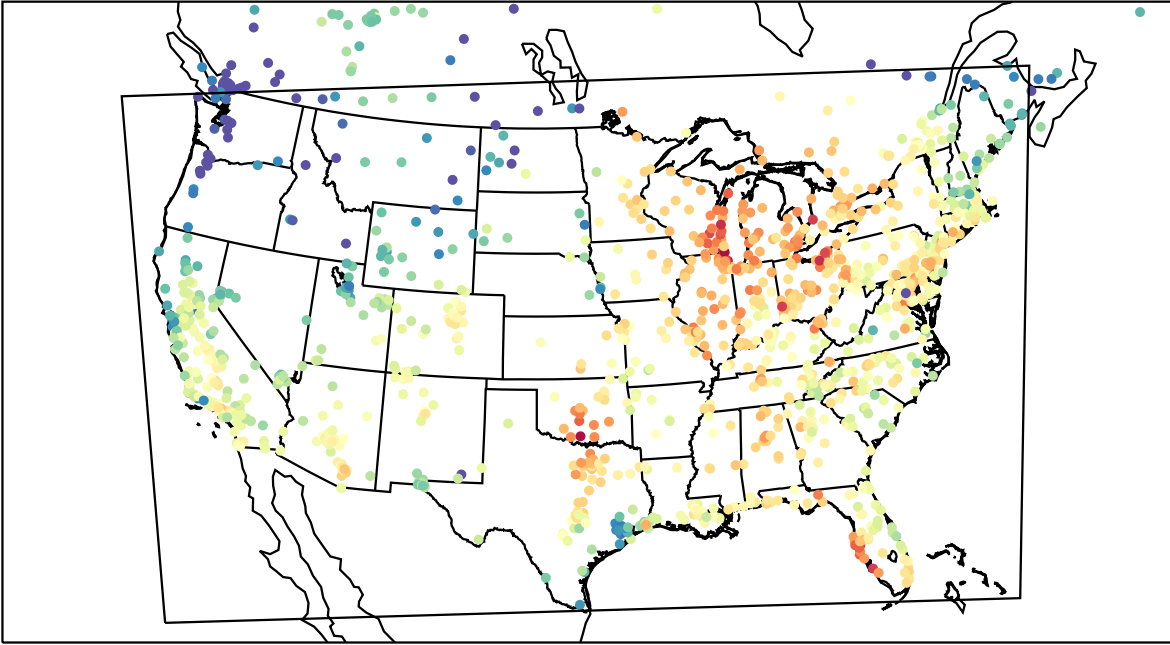
AirNOW (2023-10-03_20:00:00)
