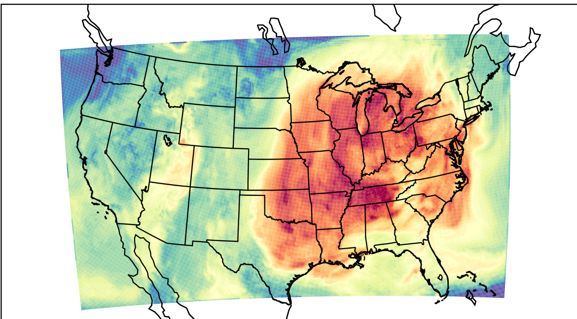
WRF (2023-10-02_19:00:00)
