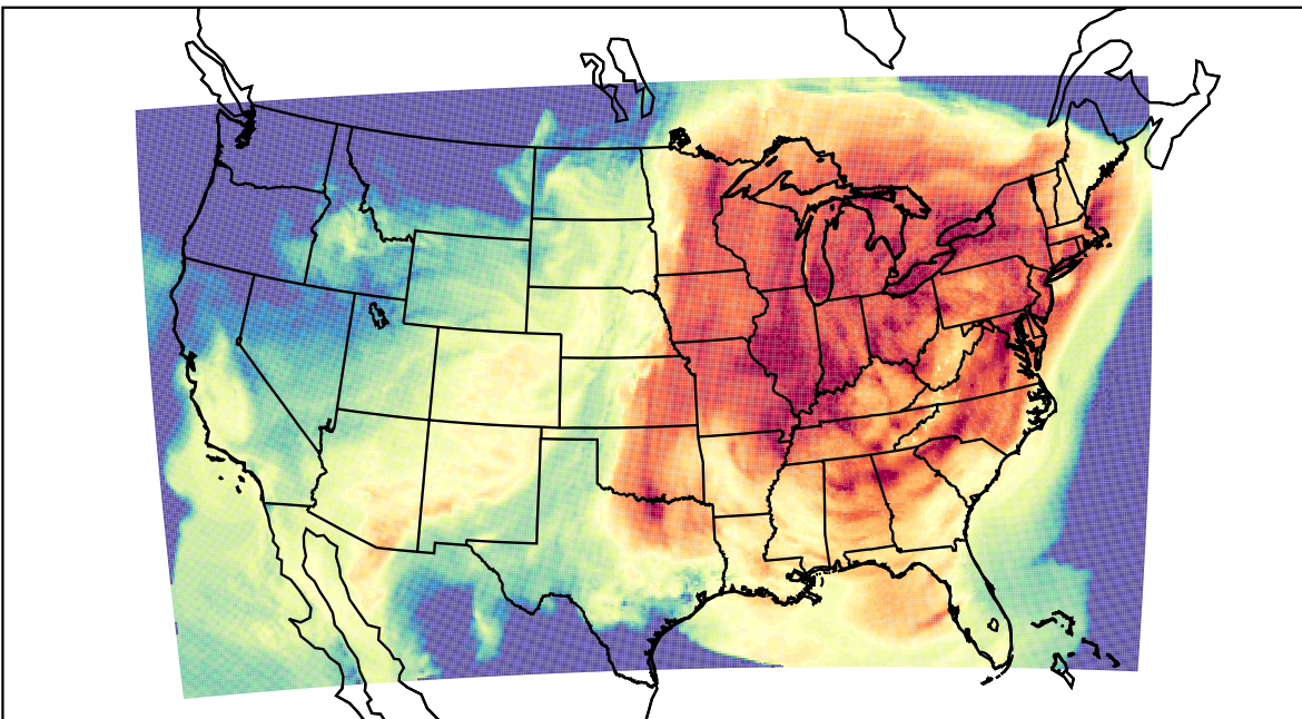
WRF (2023-10-03_20:00:00)
