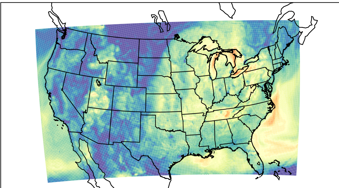
WRF (2023-10-02_14:00:00)
