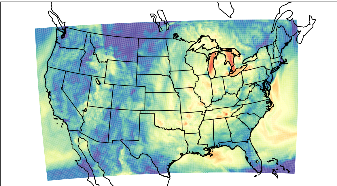
WRF (2023-10-02_07:00:00)
