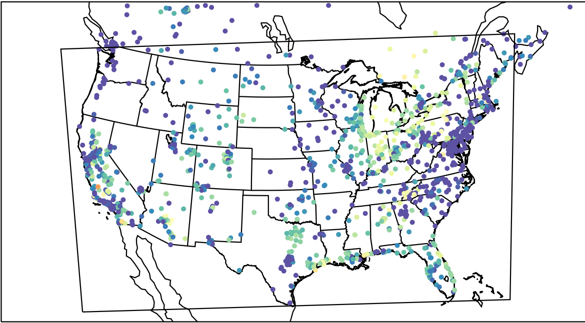
AirNOW (2023-10-05_05:00:00)
