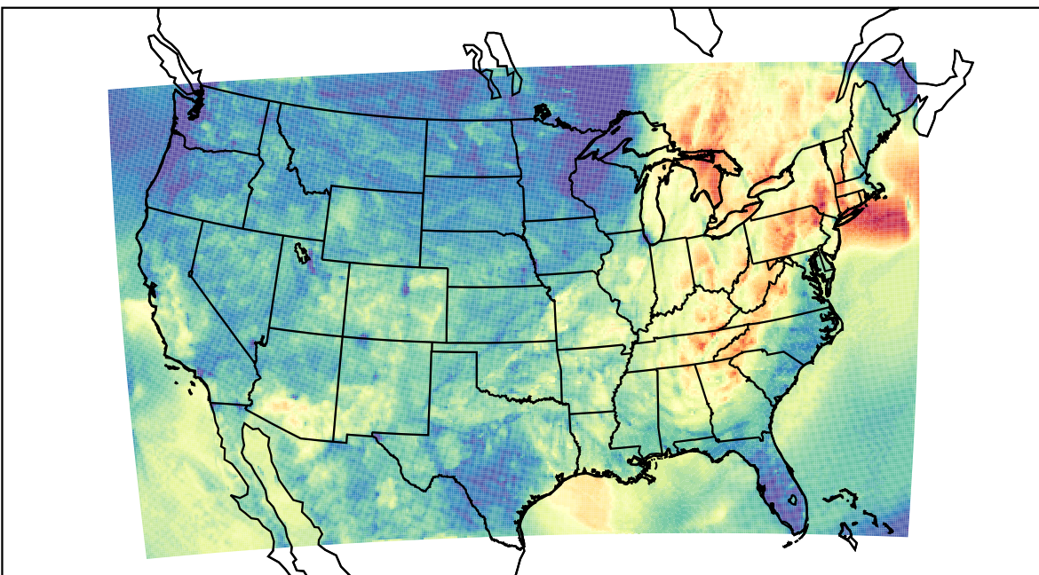
WRF (2023-10-05_03:00:00)
