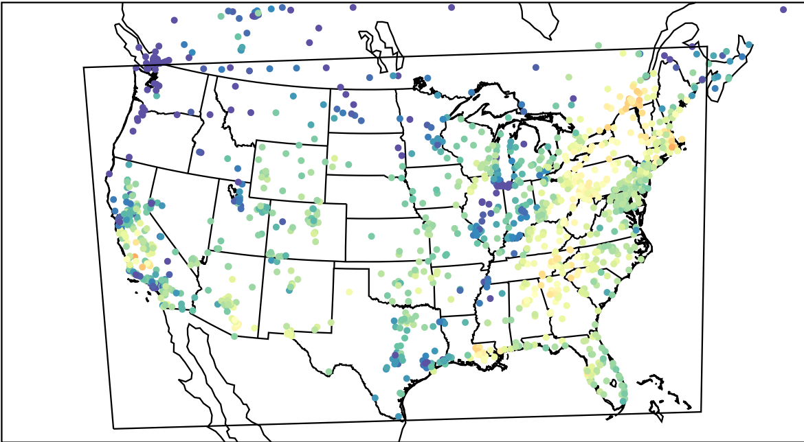
AirNOW (2023-10-05_17:00:00)
