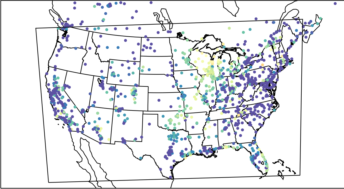
AirNOW (2023-10-04_09:00:00)
