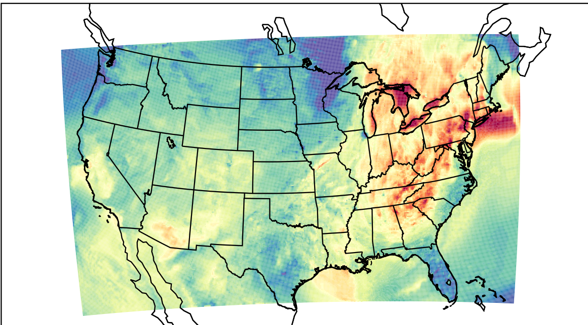
WRF (2023-10-05_00:00:00)
