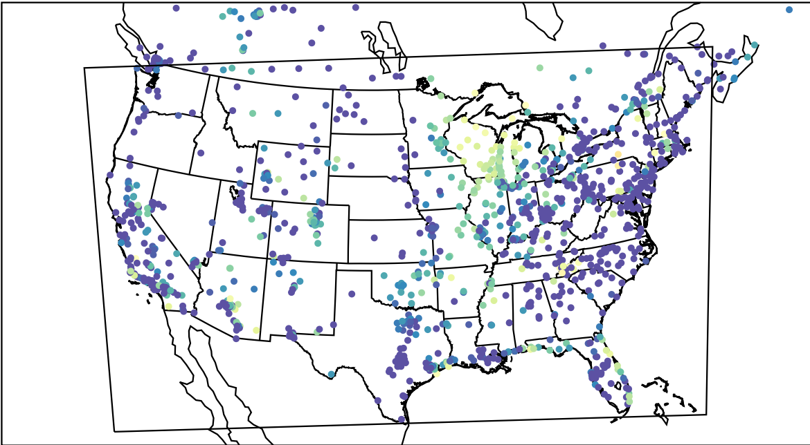
AirNOW (2023-10-04_11:00:00)
