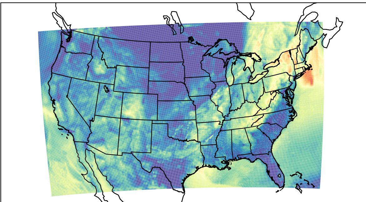
WRF (2023-10-05_12:00:00)
