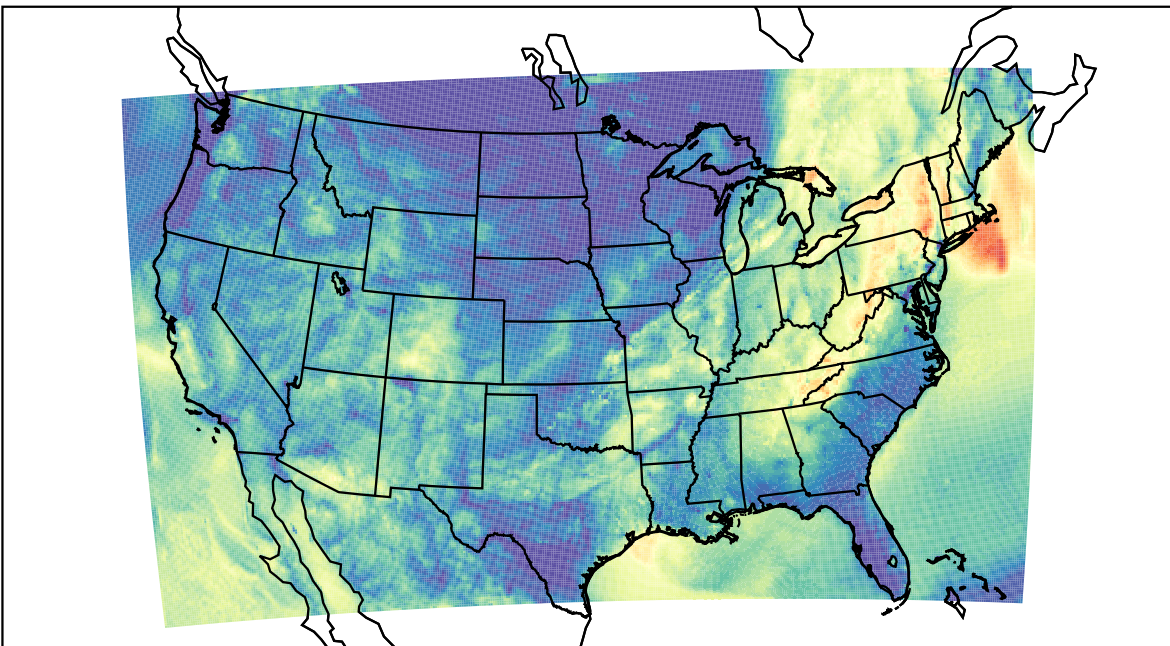
WRF (2023-10-05_10:00:00)
