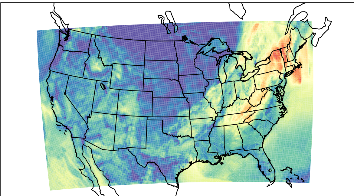
WRF (2023-10-05_14:00:00)
