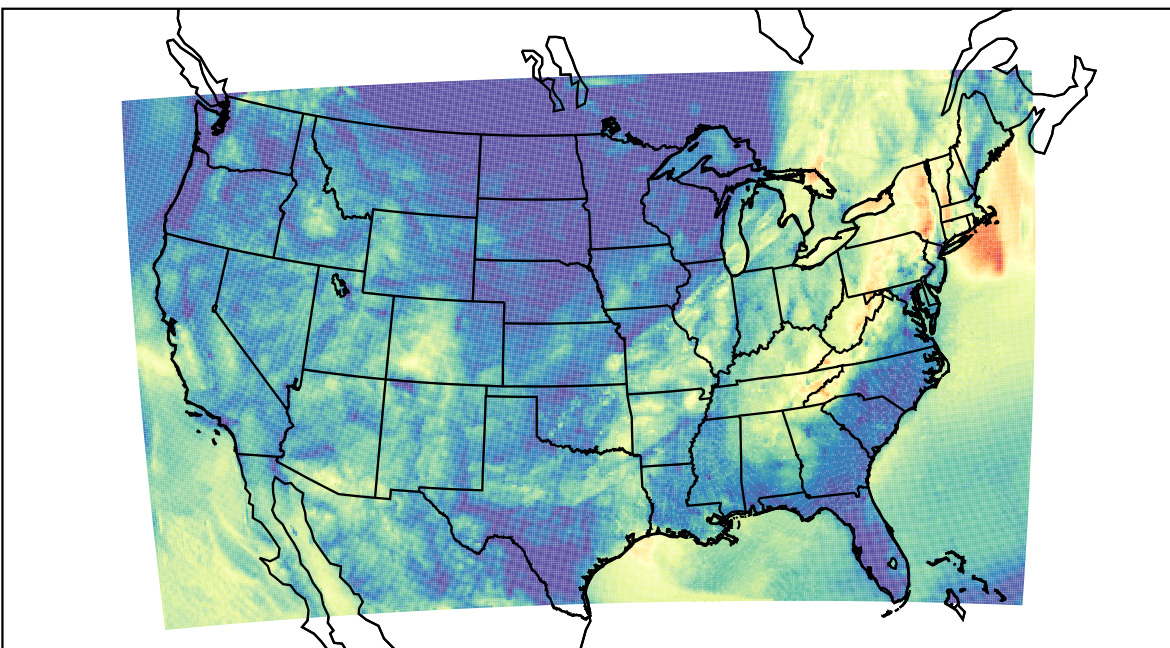
WRF (2023-10-05_11:00:00)
