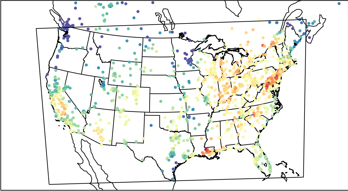
AirNOW (2023-10-04_19:00:00)
