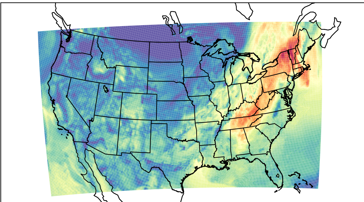
WRF (2023-10-05_15:00:00)
