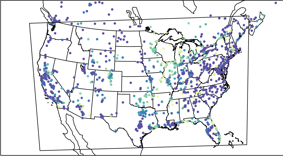
AirNOW (2023-10-04_10:00:00)
