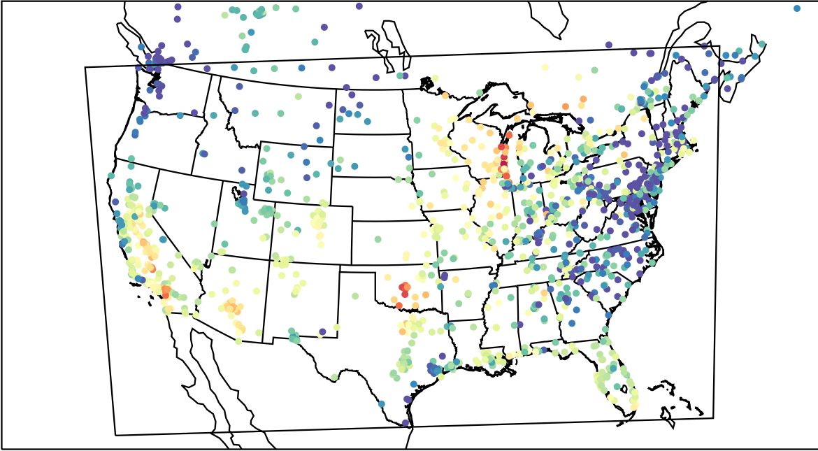
AirNOW (2023-10-04_00:00:00)
