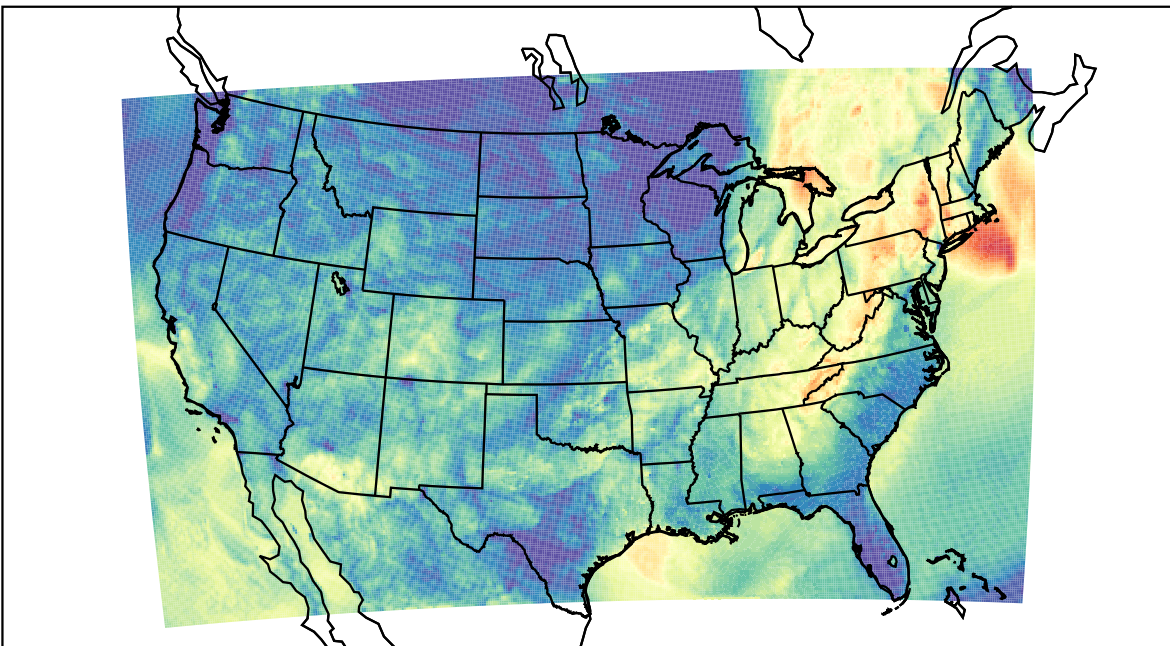
WRF (2023-10-05_07:00:00)
