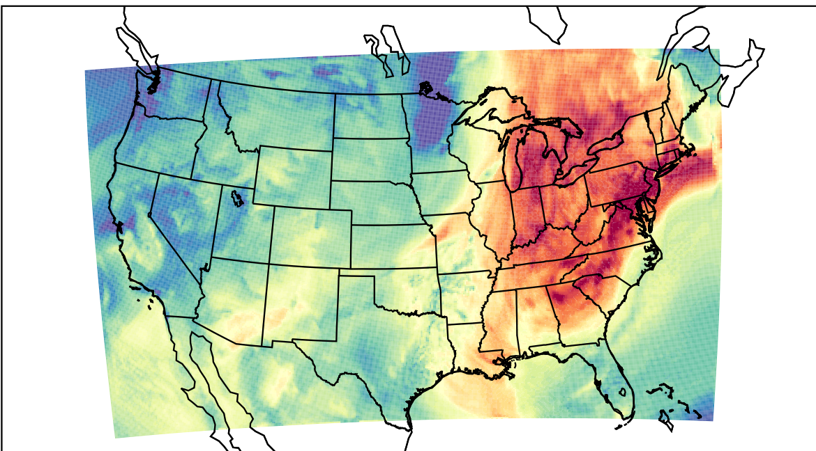
WRF (2023-10-04_18:00:00)
