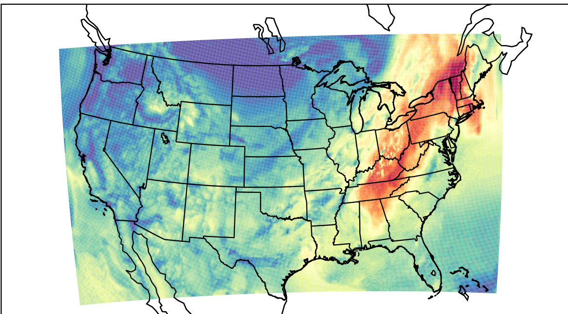
WRF (2023-10-05_16:00:00)
