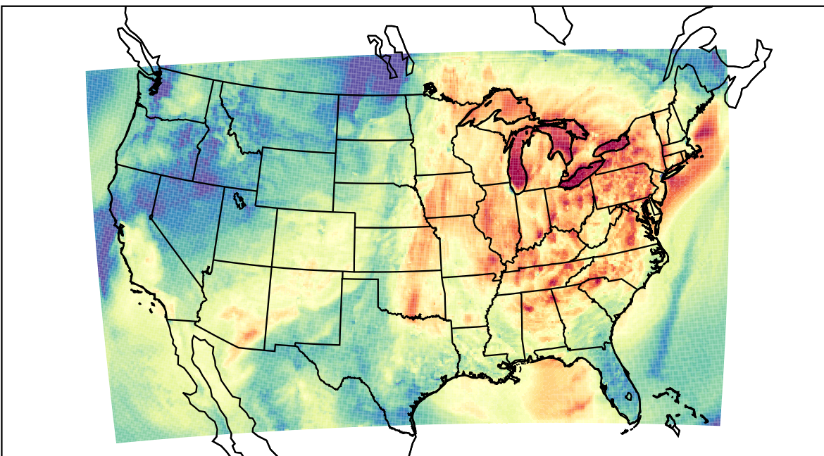
WRF (2023-10-04_00:00:00)
