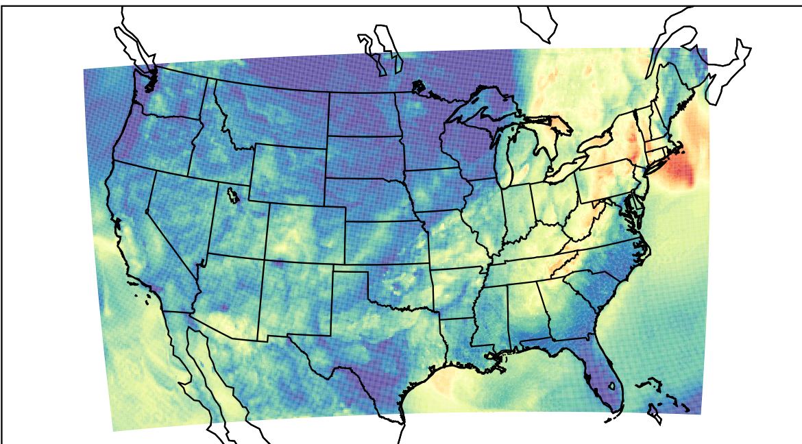
WRF (2023-10-05_08:00:00)
