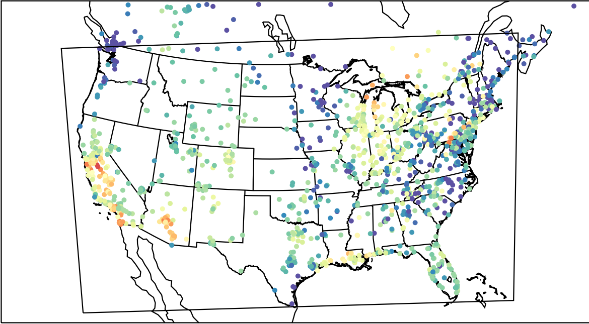
AirNOW (2023-10-05_00:00:00)
