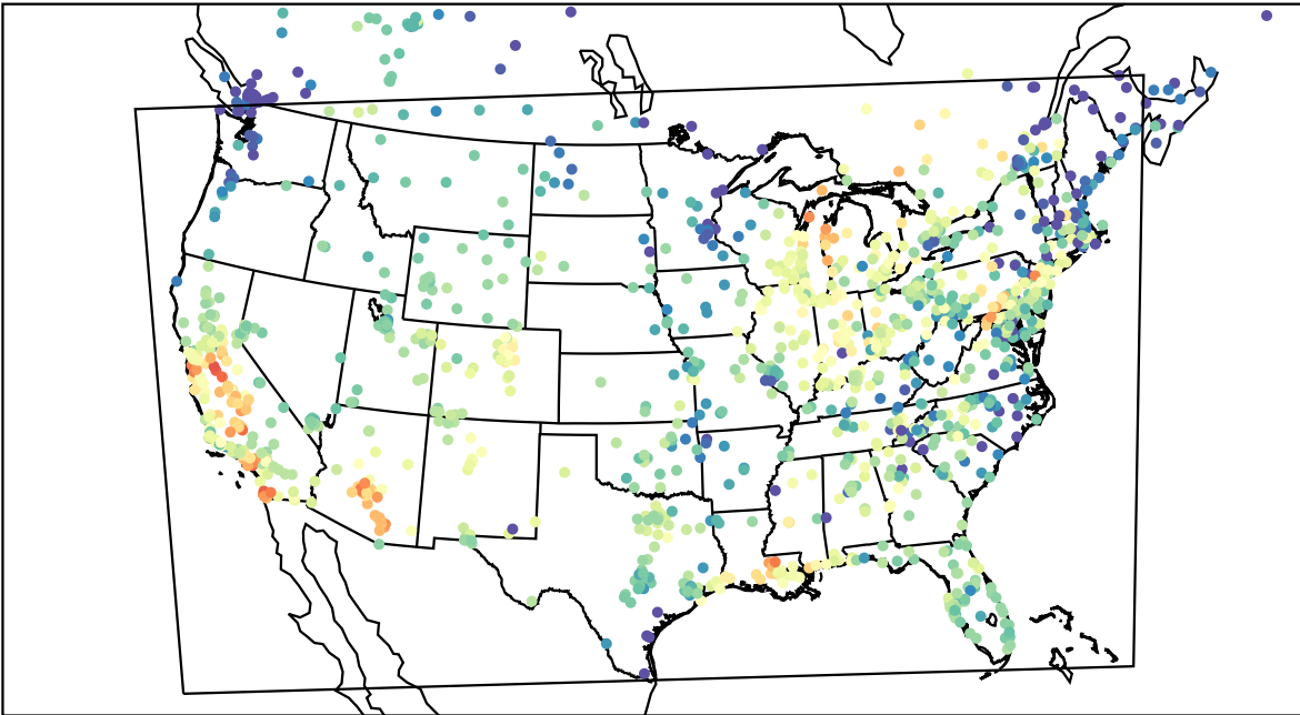
AirNOW (2023-10-04_23:00:00)
