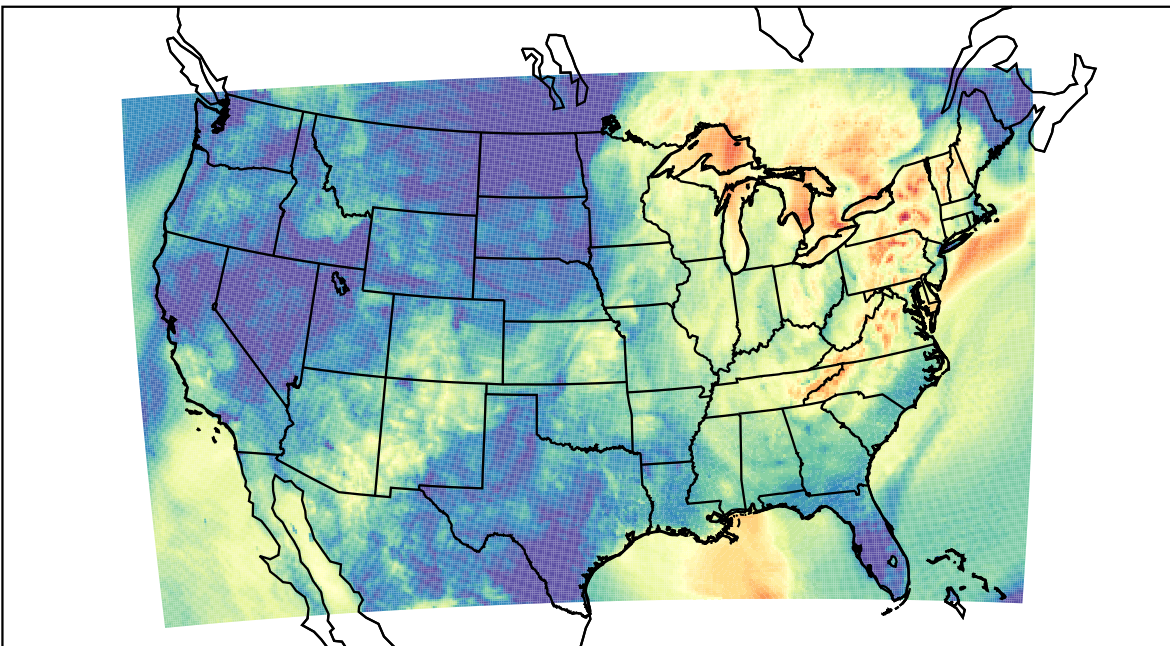
WRF (2023-10-04_09:00:00)
