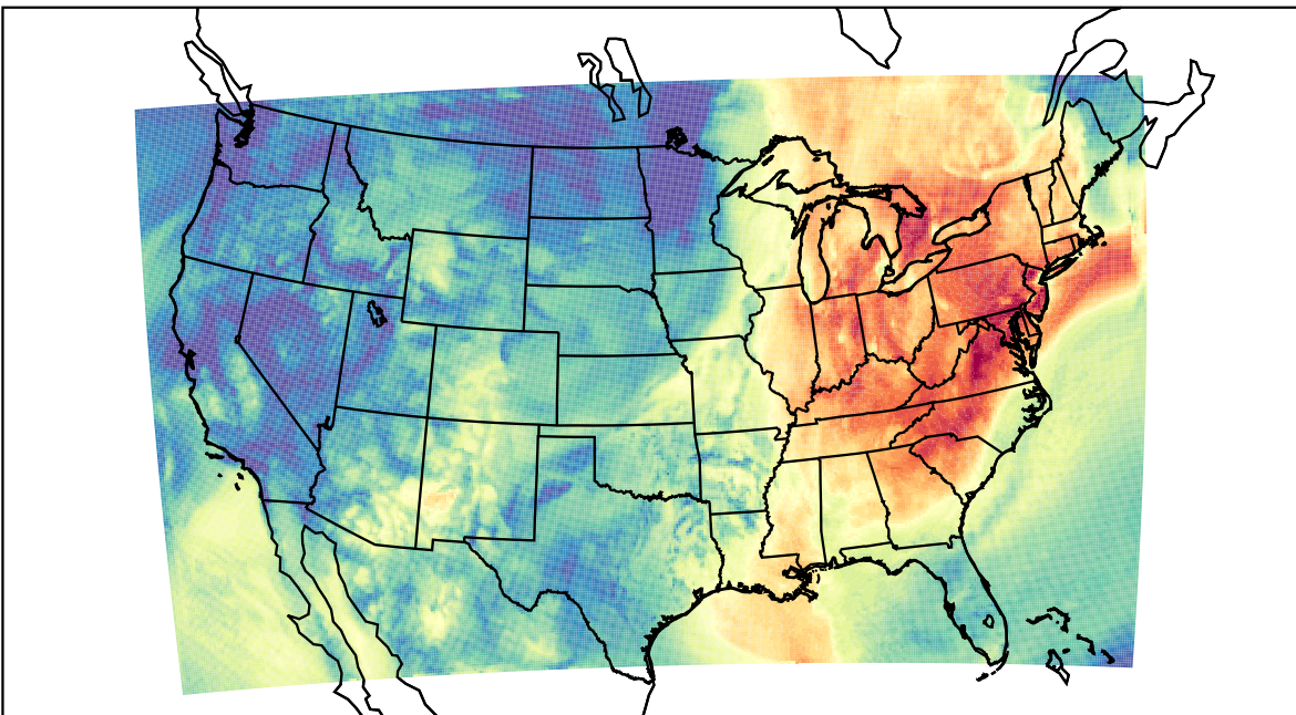
WRF (2023-10-04_16:00:00)
