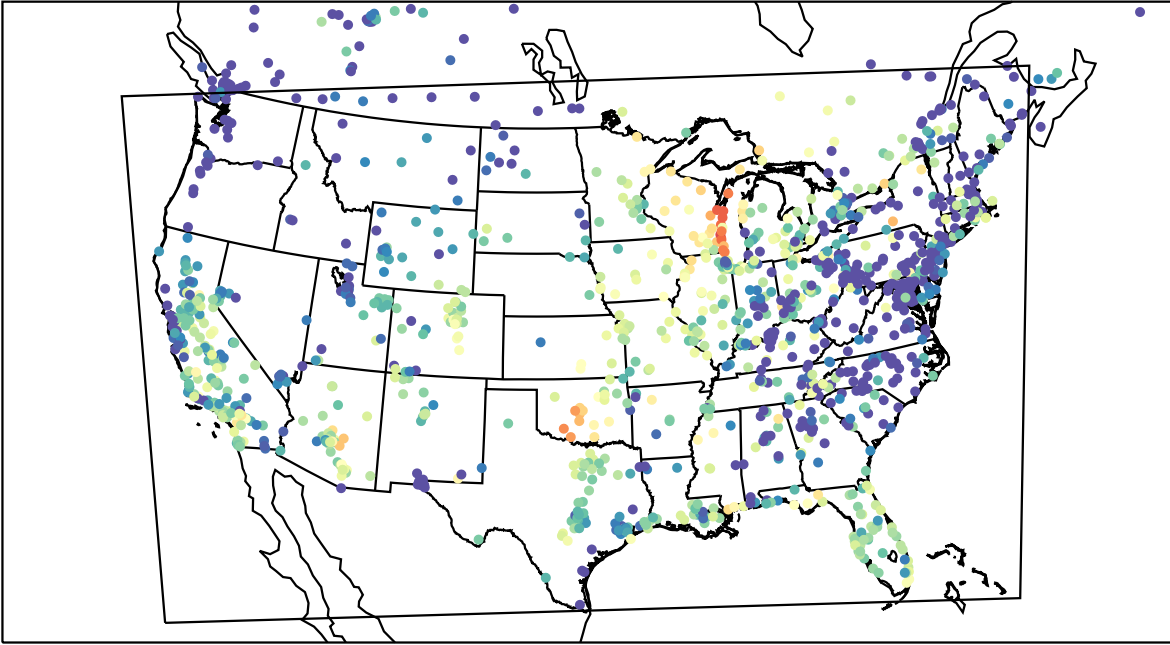
AirNOW (2023-10-04_02:00:00)
