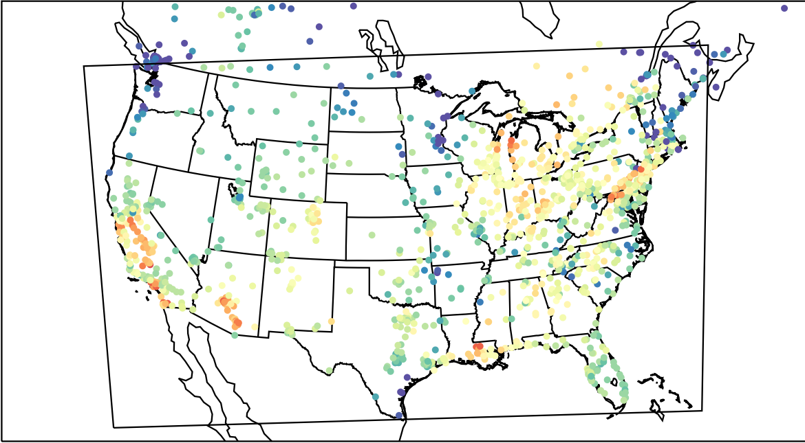
AirNOW (2023-10-04_22:00:00)
