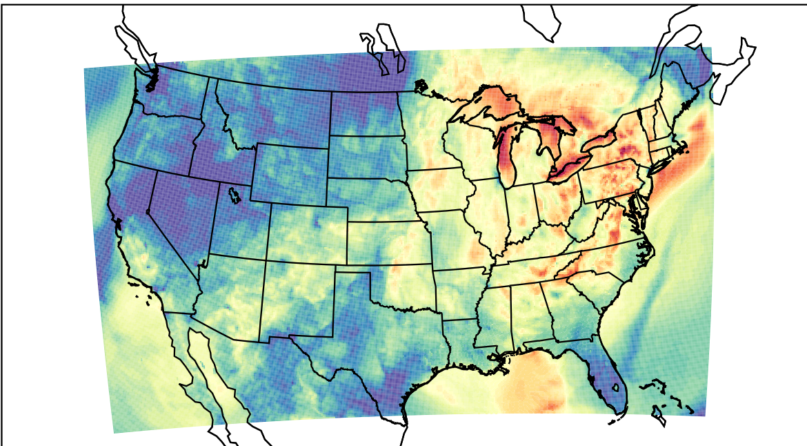
WRF (2023-10-04_04:00:00)
