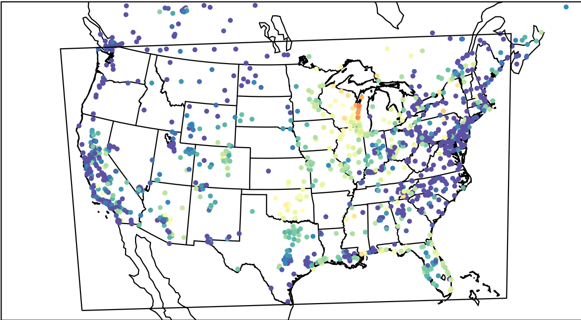
AirNOW (2023-10-04_05:00:00)
