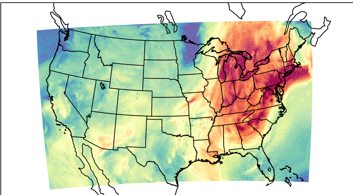
WRF (2023-10-04_20:00:00)
