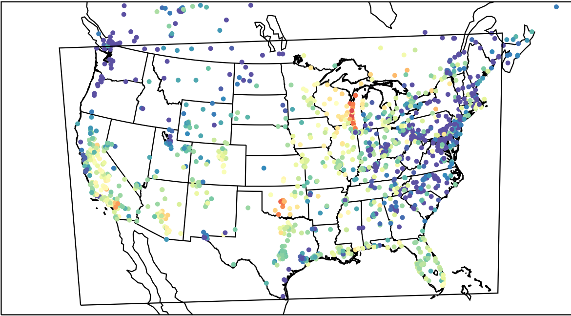
AirNOW (2023-10-04_01:00:00)
