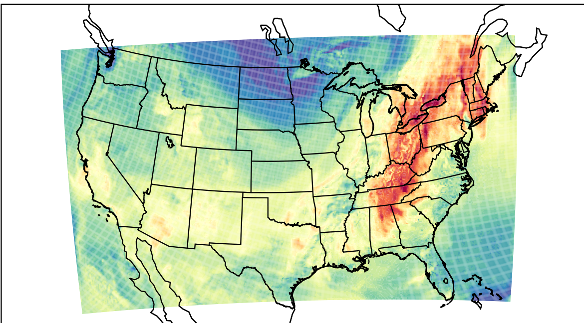
WRF (2023-10-05_21:00:00)
