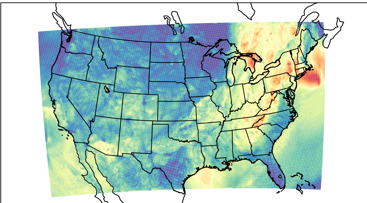
WRF (2023-10-05_05:00:00)
