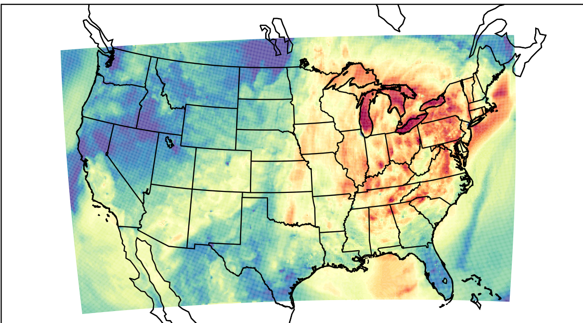
WRF (2023-10-04_01:00:00)
