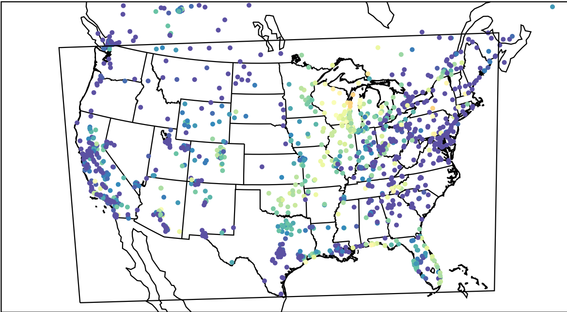
AirNOW (2023-10-04_08:00:00)
