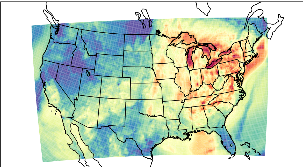
WRF (2023-10-04_02:00:00)
