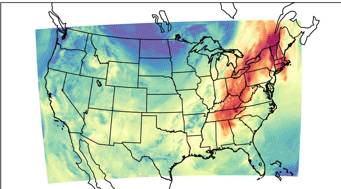
WRF (2023-10-05_18:00:00)
