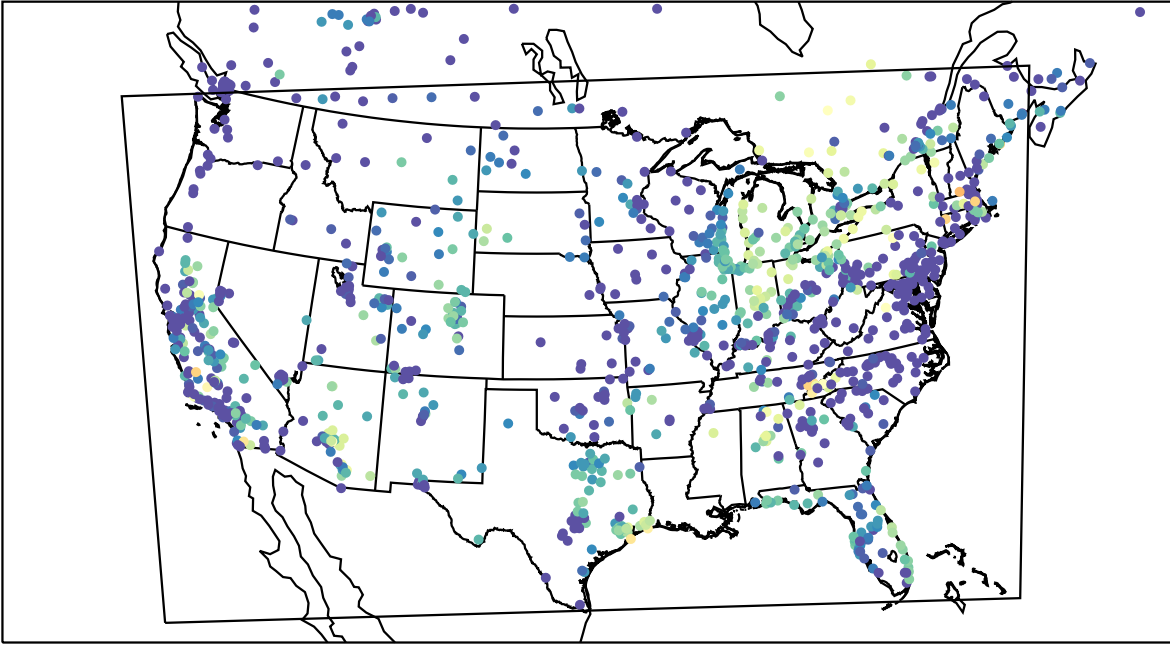
AirNOW (2023-10-05_07:00:00)
