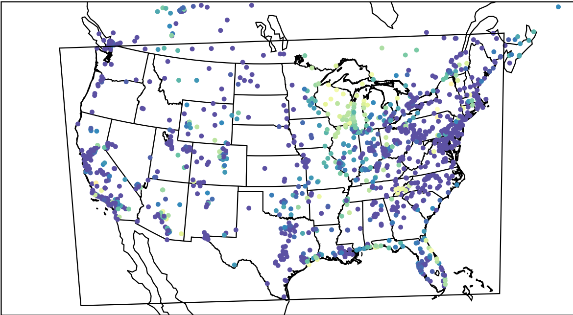
AirNOW (2023-10-04_12:00:00)
