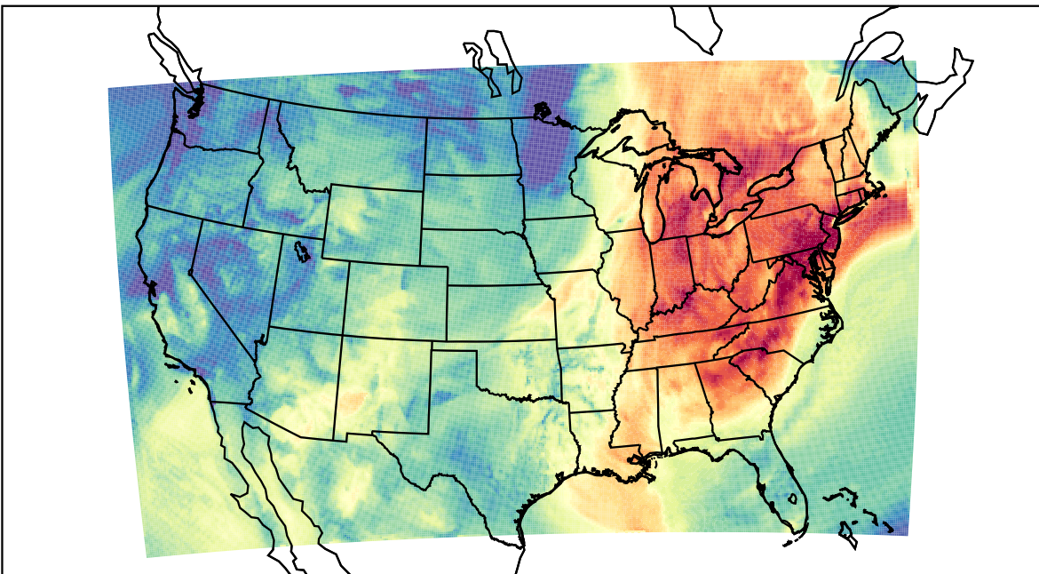
WRF (2023-10-04_17:00:00)
