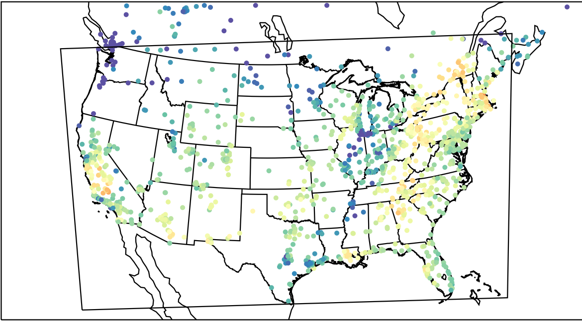
AirNOW (2023-10-05_18:00:00)
