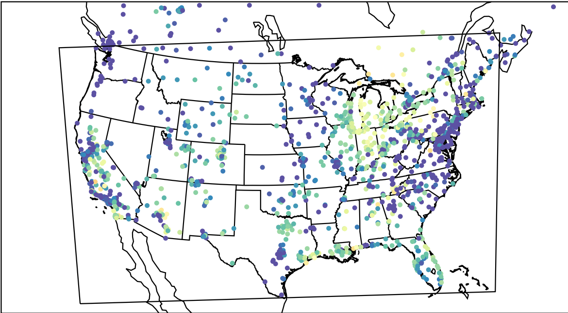
AirNOW (2023-10-05_04:00:00)
