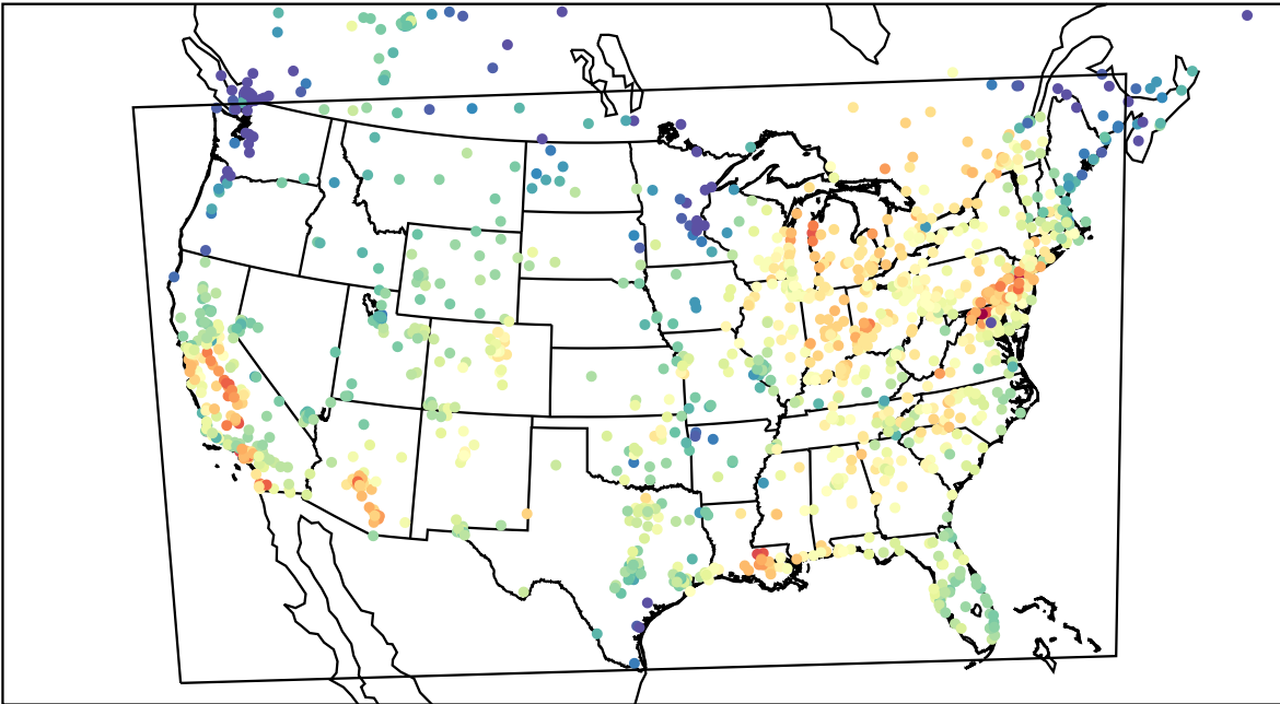
AirNOW (2023-10-04_21:00:00)
