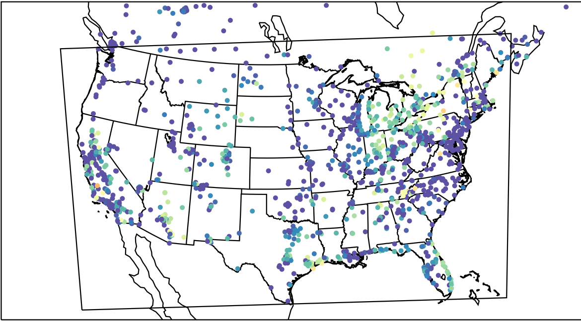
AirNOW (2023-10-05_09:00:00)
