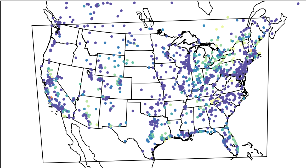
AirNOW (2023-10-05_11:00:00)
