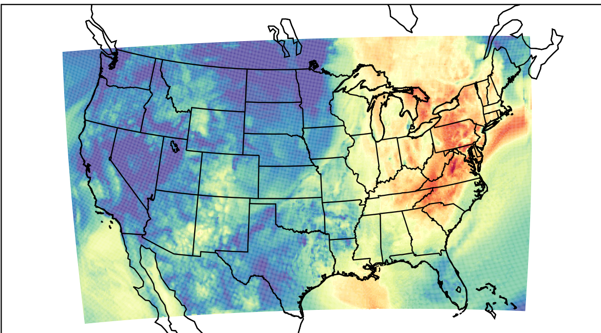
WRF (2023-10-04_15:00:00)
