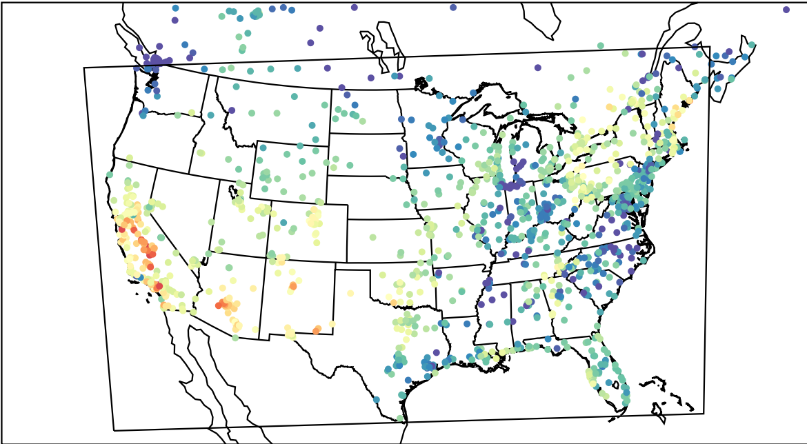
AirNOW (2023-10-05_23:00:00)
