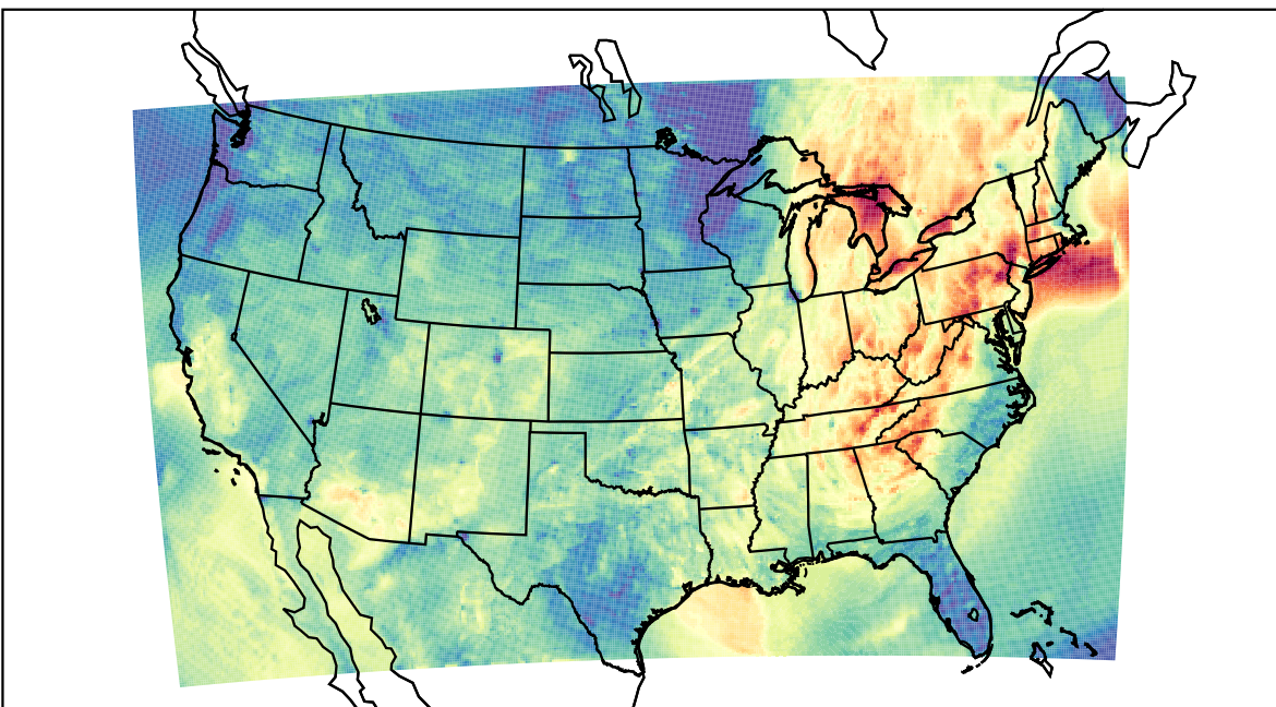
WRF (2023-10-05_01:00:00)
