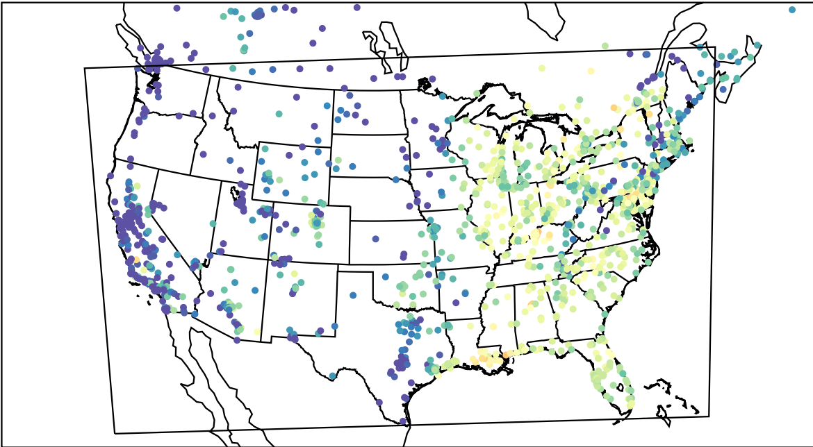
AirNOW (2023-10-04_15:00:00)
