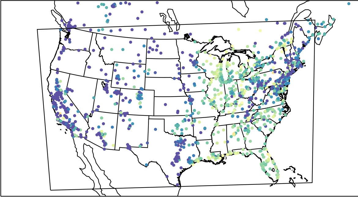
AirNOW (2023-10-04_14:00:00)
