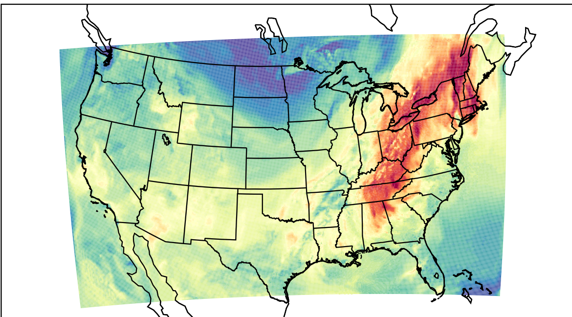
WRF (2023-10-05_20:00:00)
