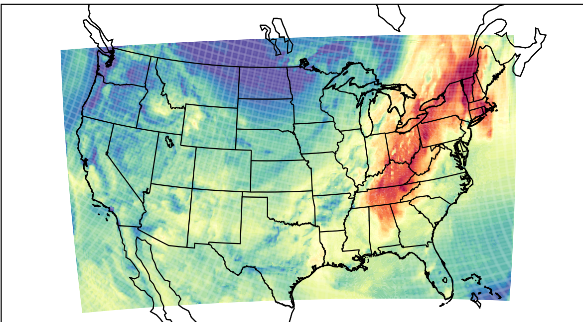
WRF (2023-10-05_17:00:00)
