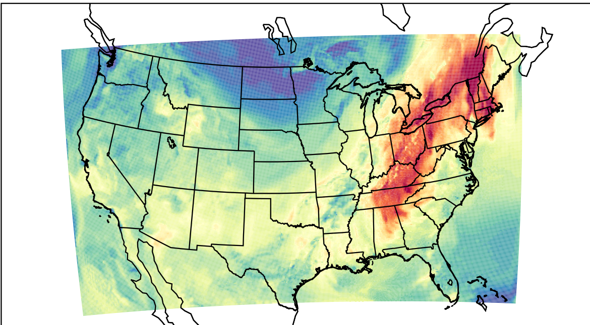
WRF (2023-10-05_19:00:00)
