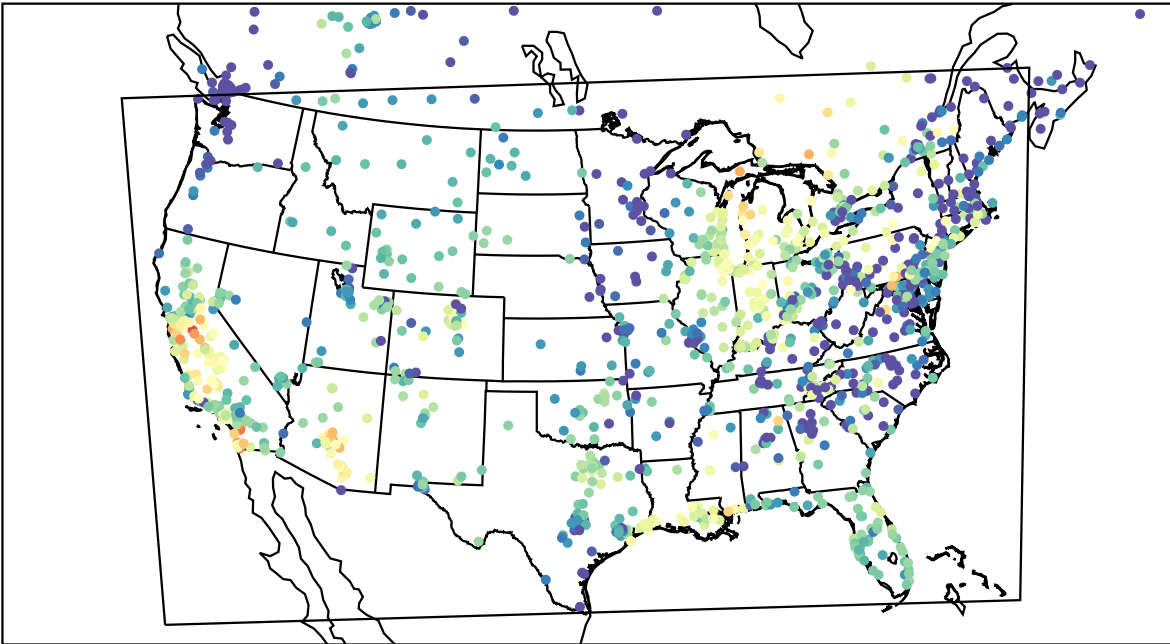
AirNOW (2023-10-05_01:00:00)
