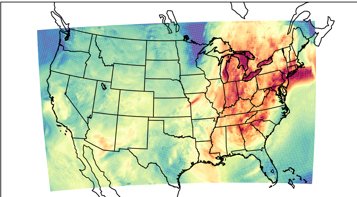
WRF (2023-10-04_22:00:00)
