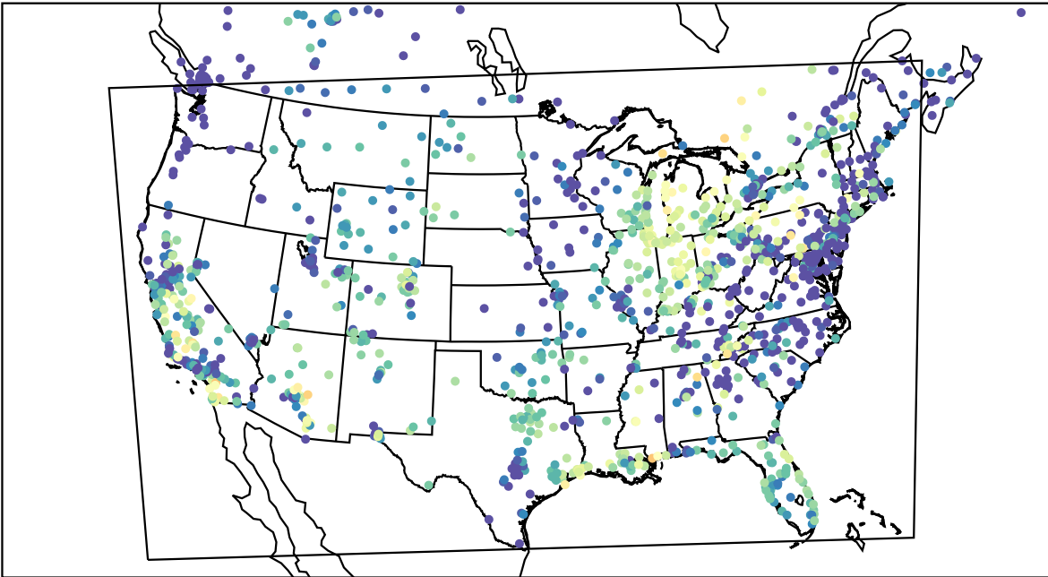
AirNOW (2023-10-05_03:00:00)
