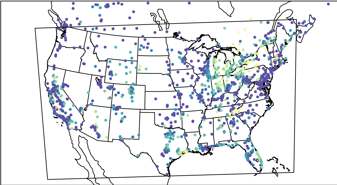
AirNOW (2023-10-05_08:00:00)
