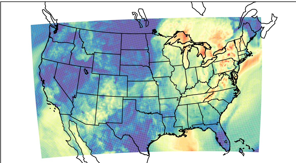
WRF (2023-10-04_10:00:00)
