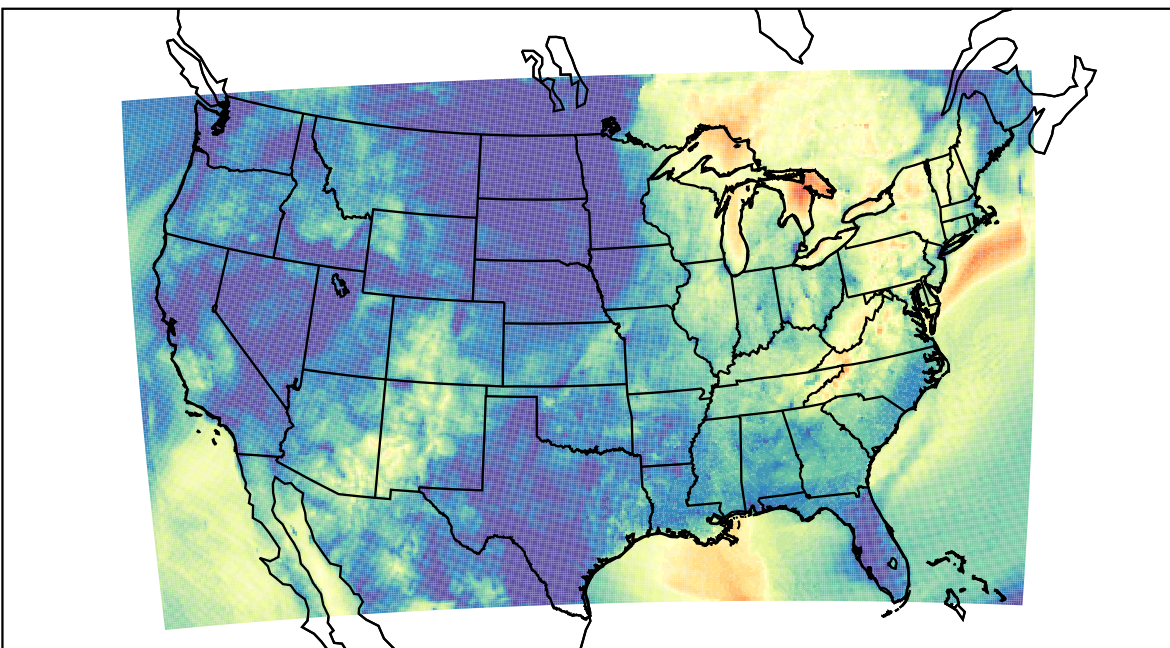
WRF (2023-10-04_13:00:00)
