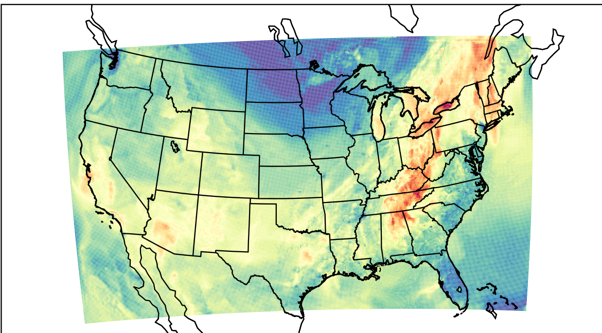
WRF (2023-10-05_23:00:00)
