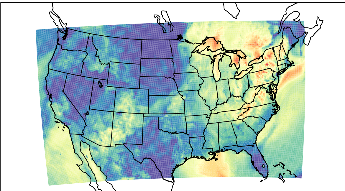
WRF (2023-10-04_11:00:00)
