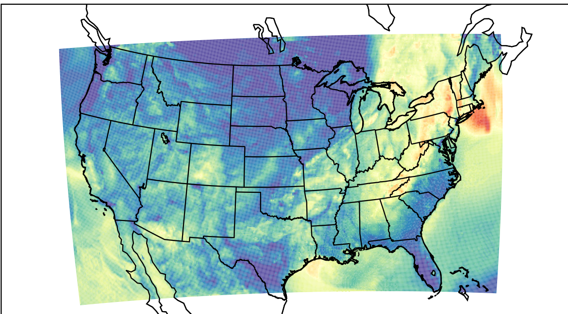
WRF (2023-10-05_09:00:00)
