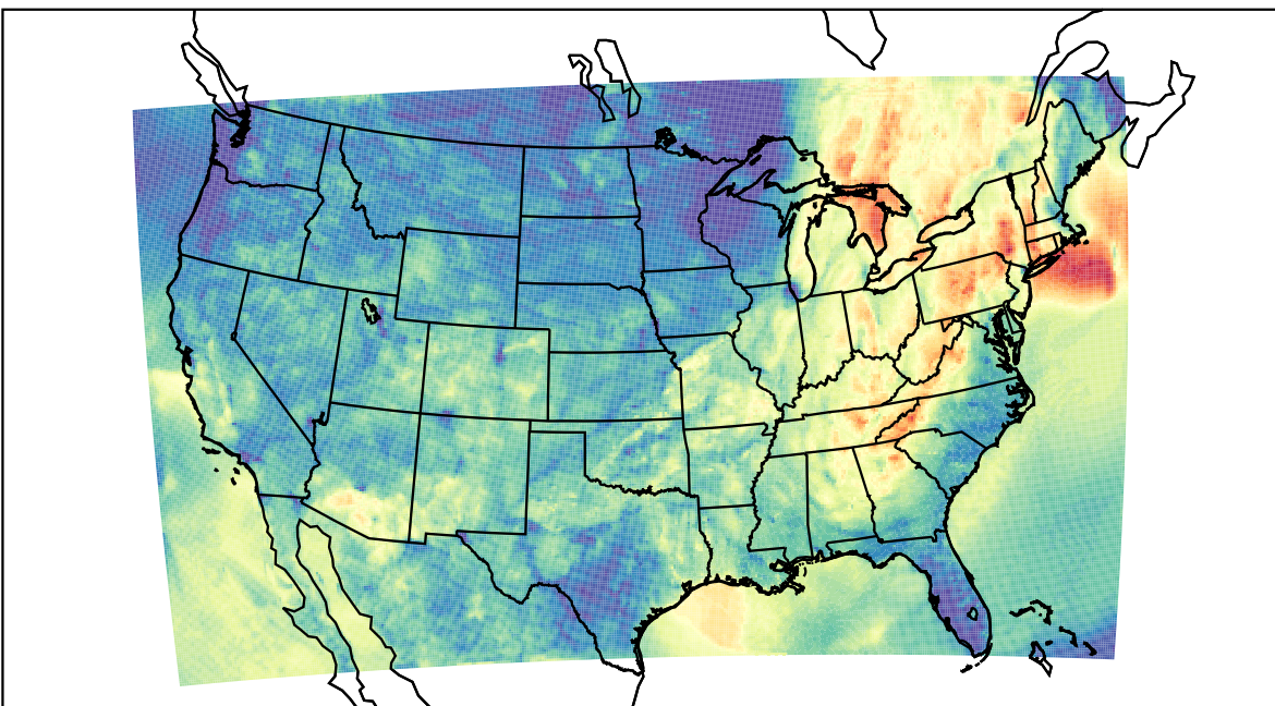
WRF (2023-10-05_04:00:00)
