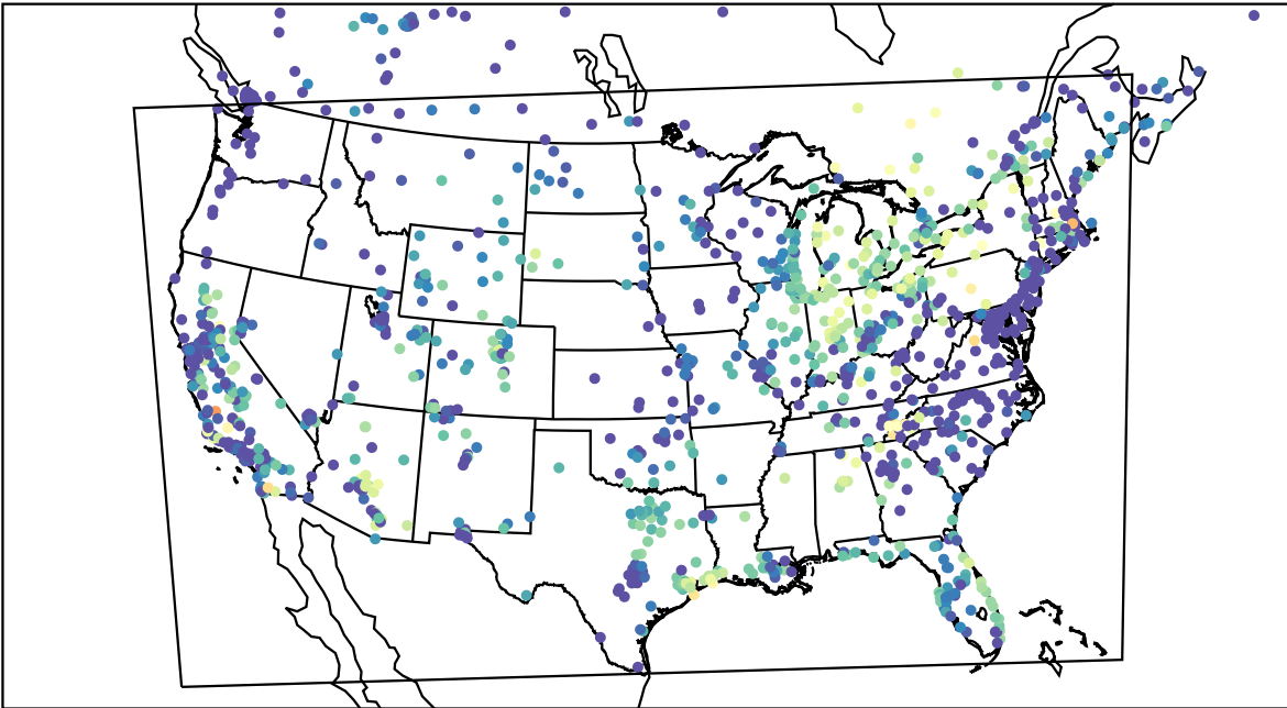
AirNOW (2023-10-05_06:00:00)
