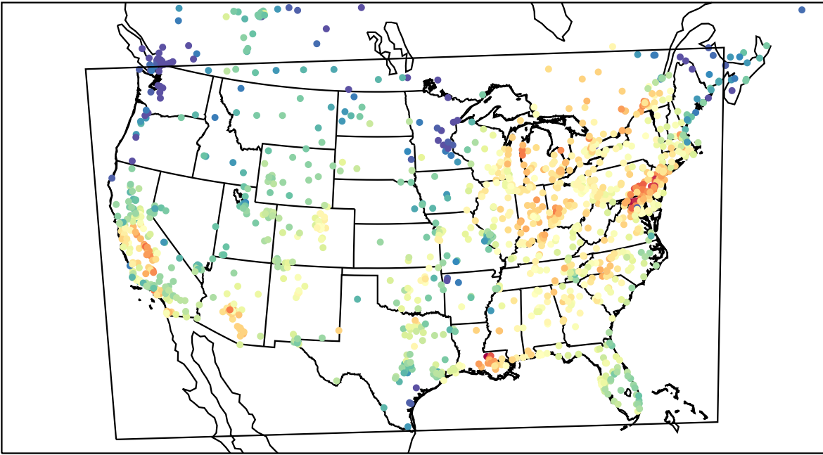
AirNOW (2023-10-04_20:00:00)
