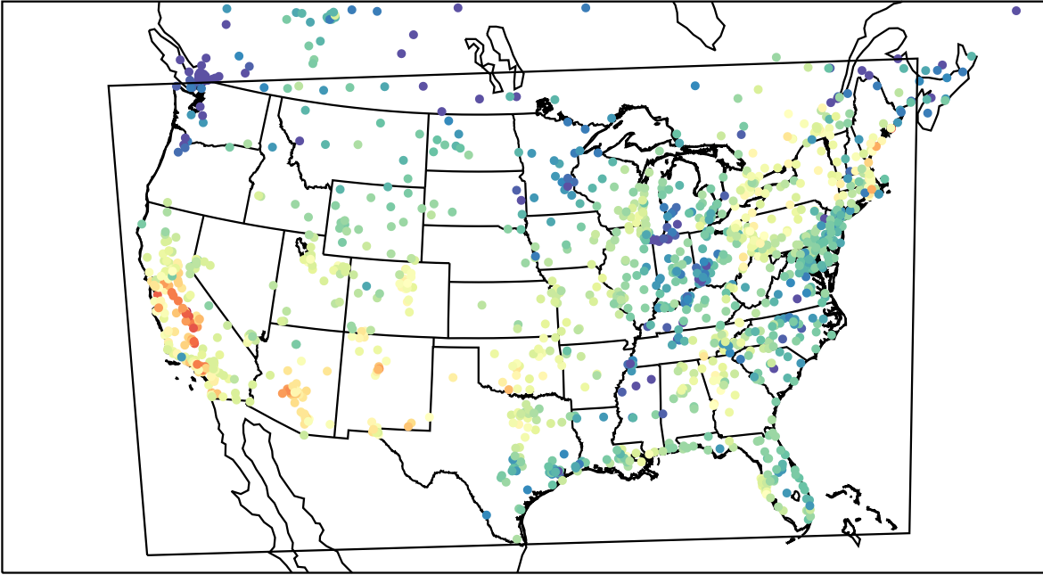
AirNOW (2023-10-05_22:00:00)
