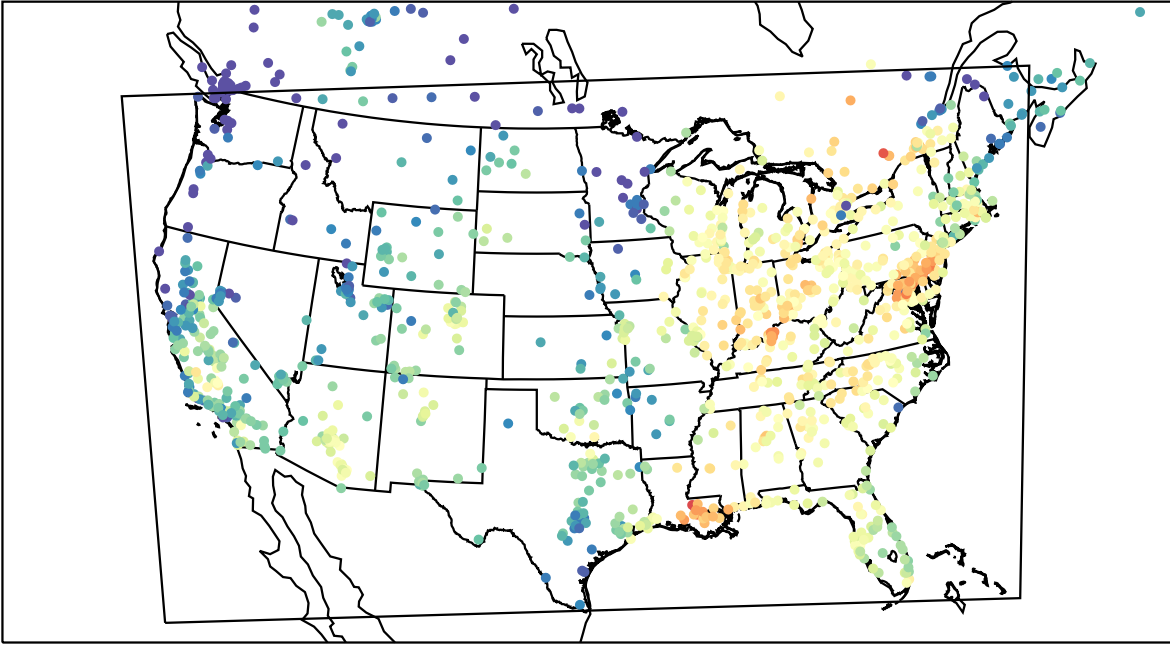
AirNOW (2023-10-04_17:00:00)
