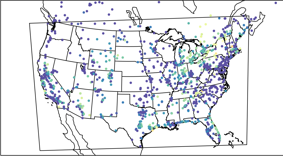
AirNOW (2023-10-05_10:00:00)
