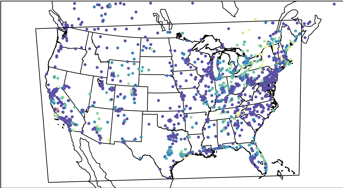
AirNOW (2023-10-05_12:00:00)
