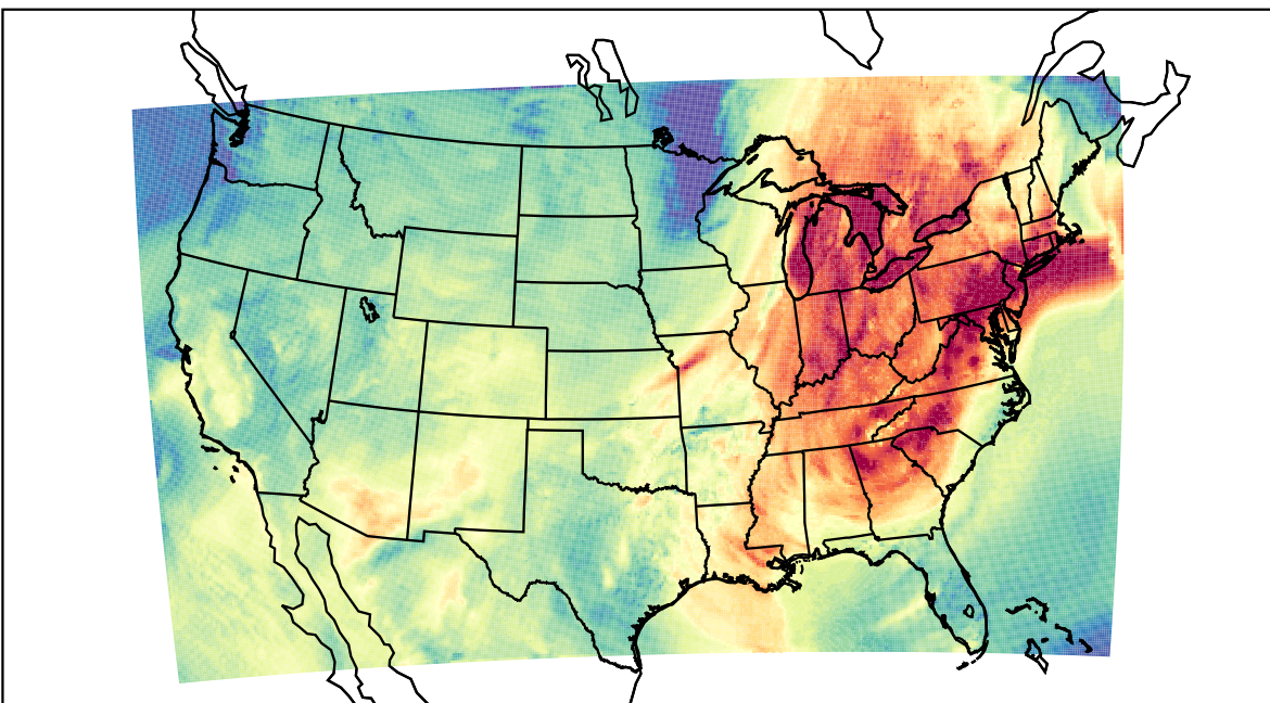
WRF (2023-10-04_21:00:00)
