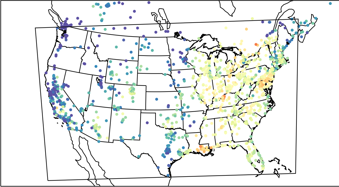
AirNOW (2023-10-04_16:00:00)
