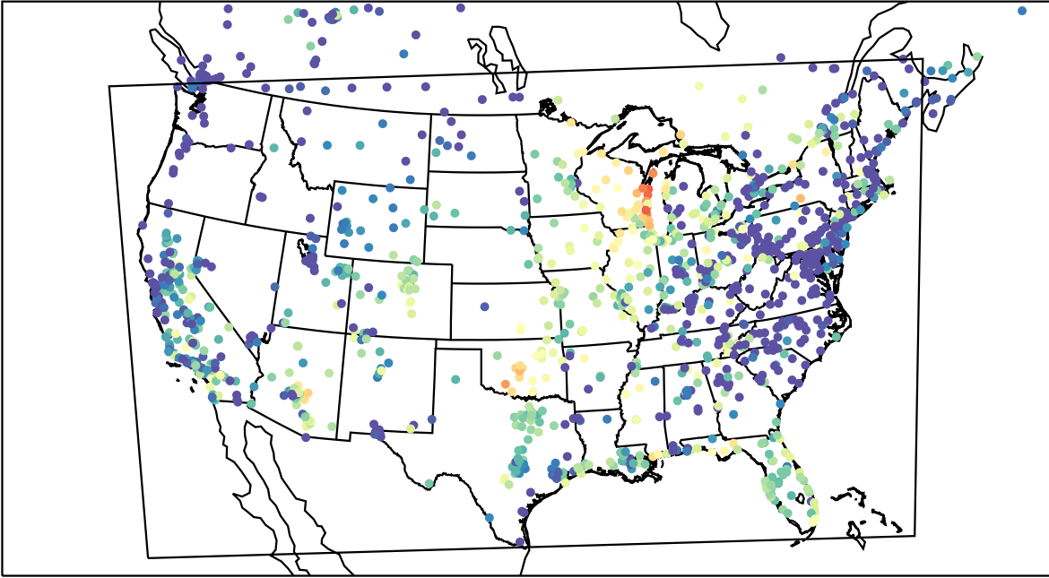
AirNOW (2023-10-04_03:00:00)
