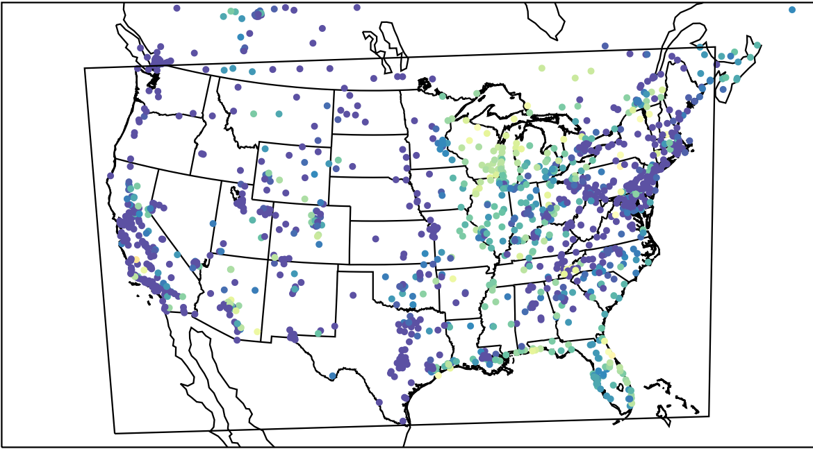
AirNOW (2023-10-04_13:00:00)
