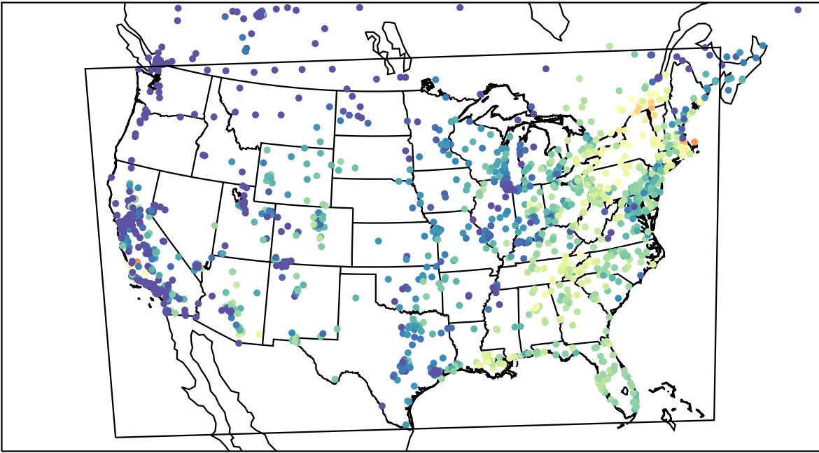
AirNOW (2023-10-05_15:00:00)
