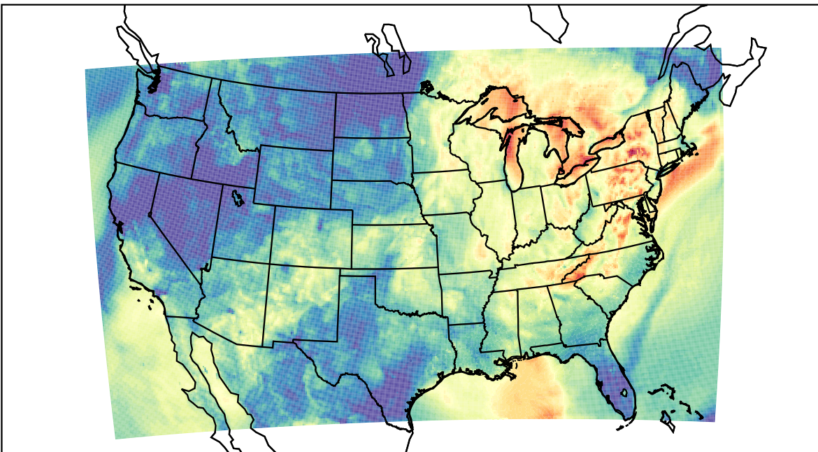
WRF (2023-10-04_06:00:00)
