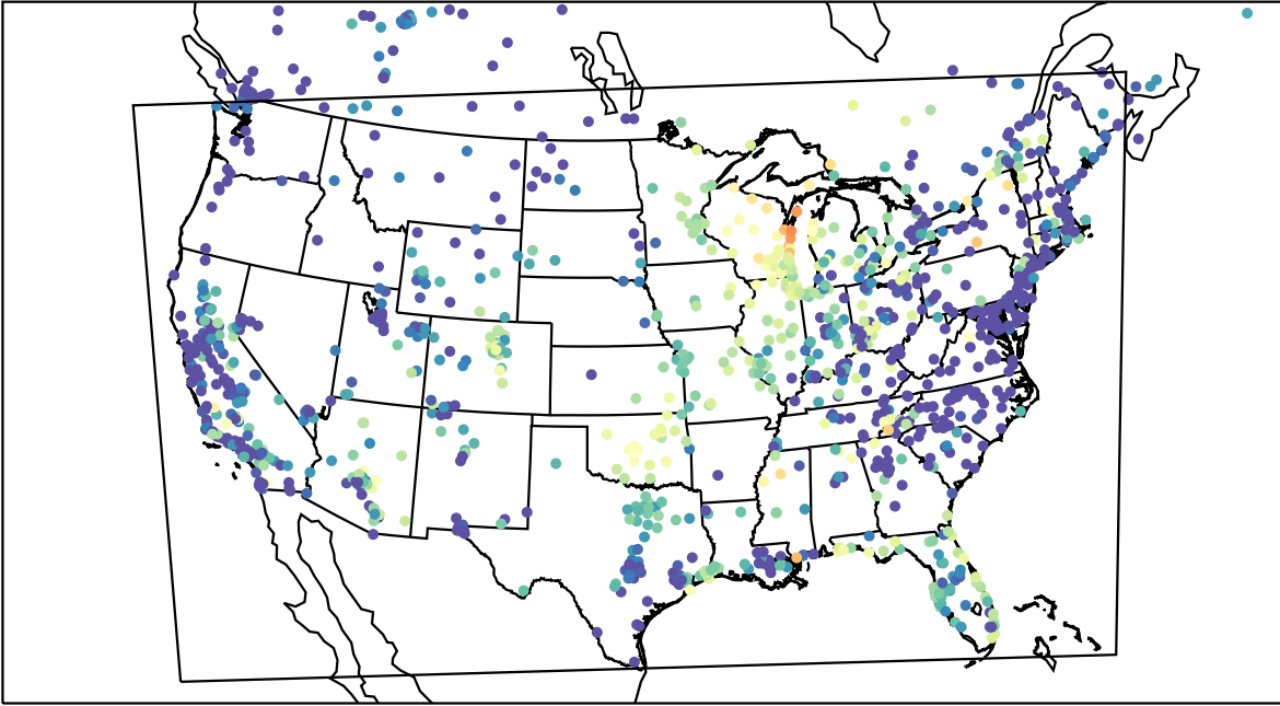
AirNOW (2023-10-04_06:00:00)
