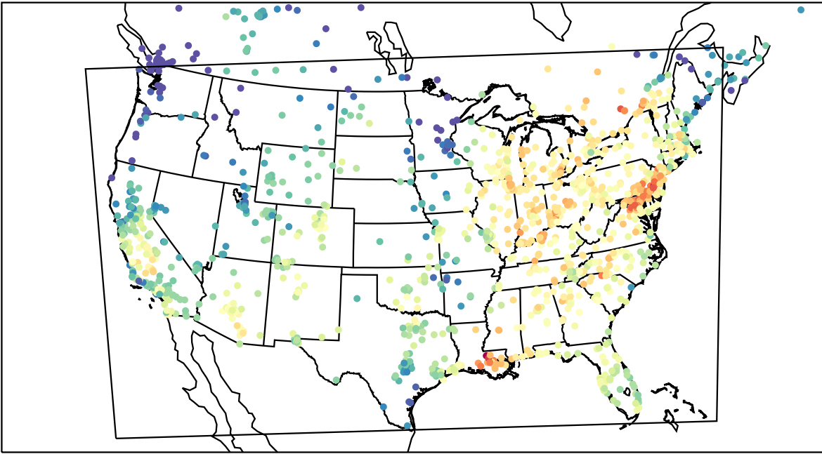
AirNOW (2023-10-04_18:00:00)
