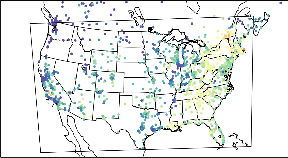
AirNOW (2023-10-05_16:00:00)
