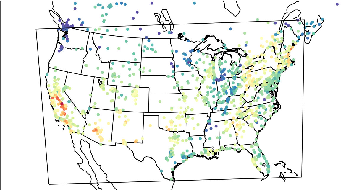
AirNOW (2023-10-05_21:00:00)
