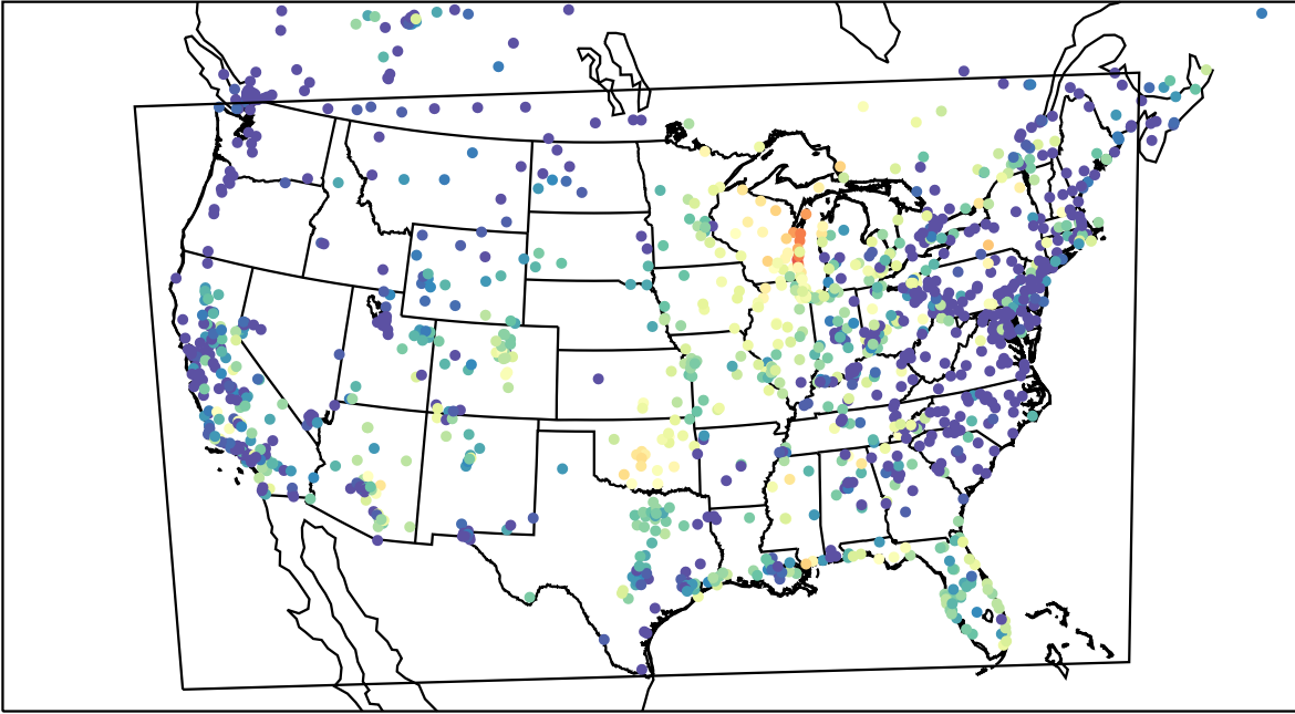
AirNOW (2023-10-04_04:00:00)
