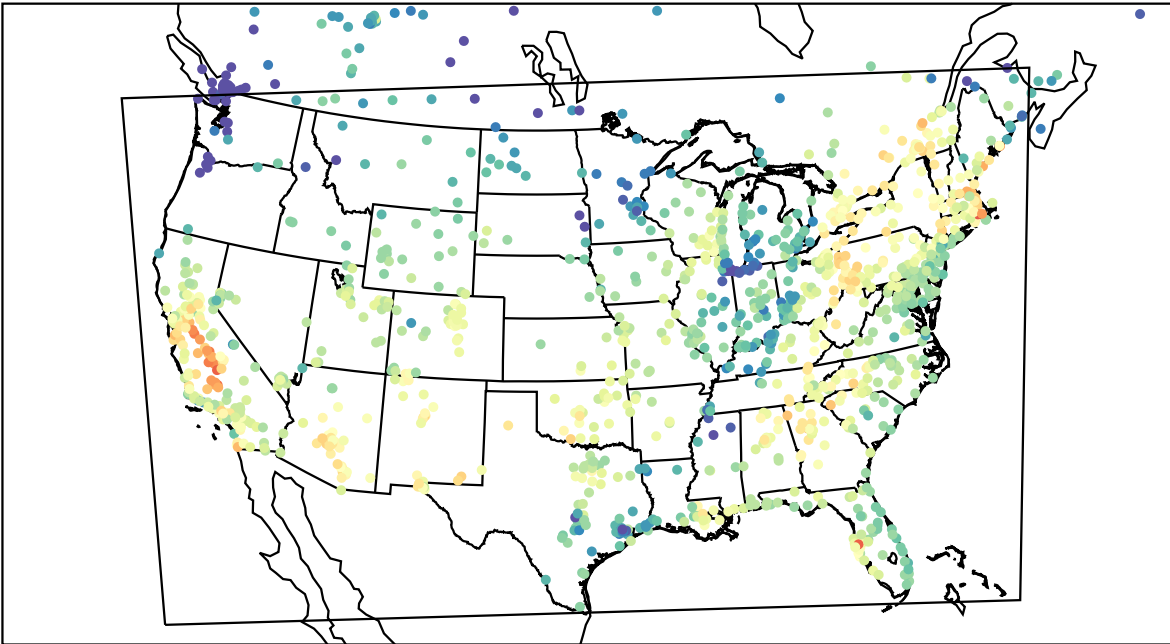
AirNOW (2023-10-05_20:00:00)
