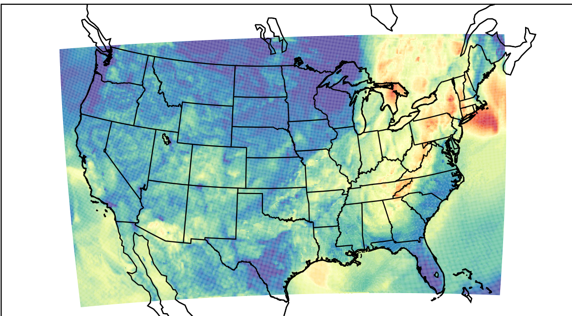
WRF (2023-10-05_06:00:00)
