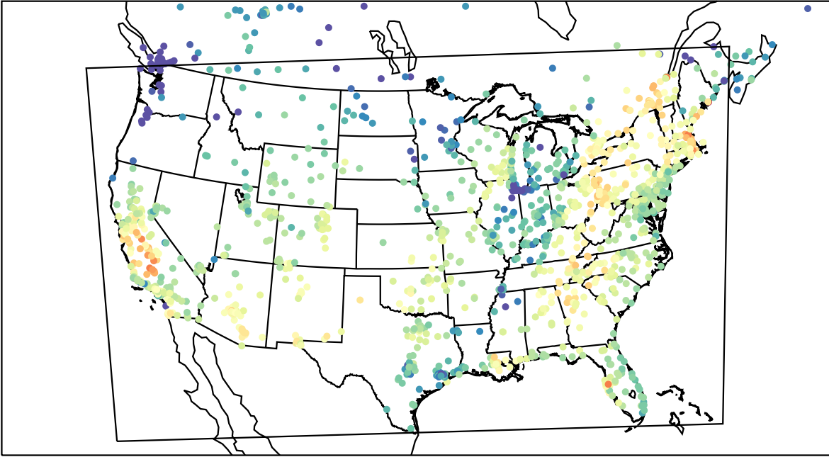
AirNOW (2023-10-05_19:00:00)
