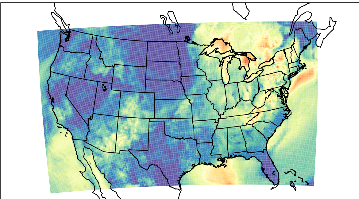
WRF (2023-10-04_12:00:00)
