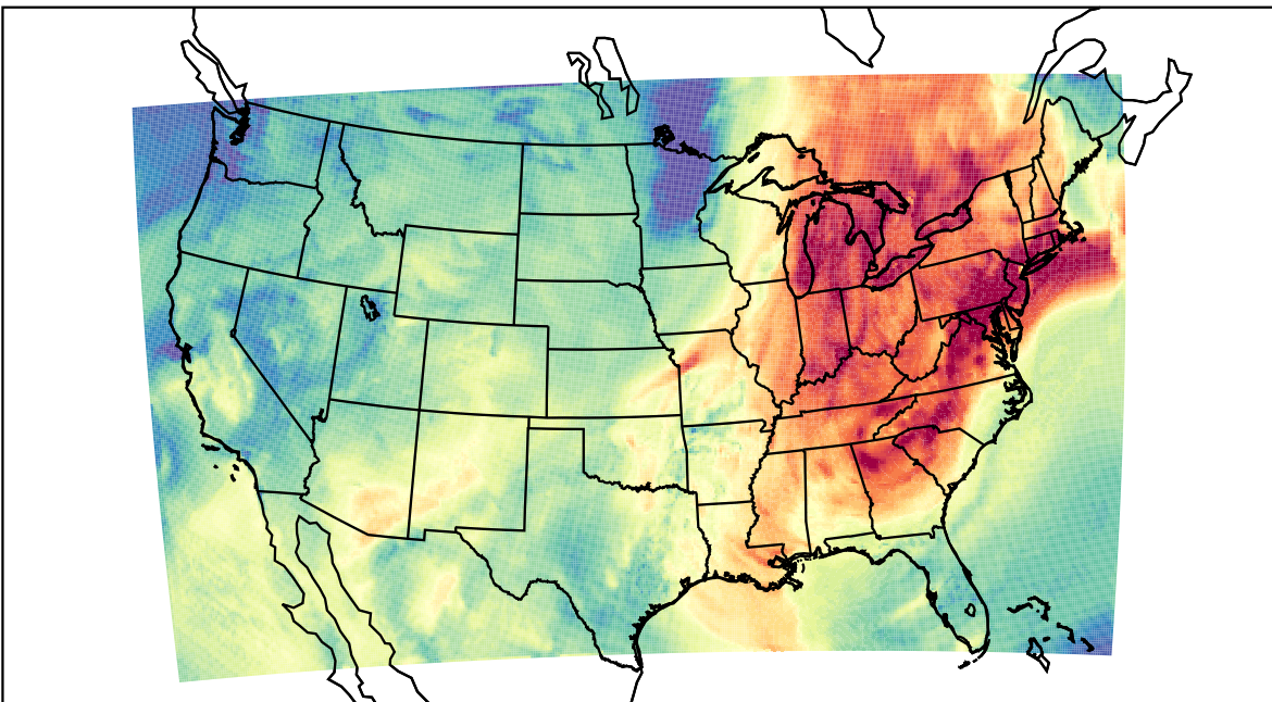
WRF (2023-10-04_19:00:00)
