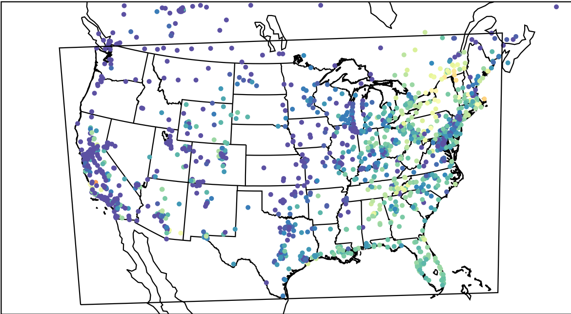
AirNOW (2023-10-05_14:00:00)
