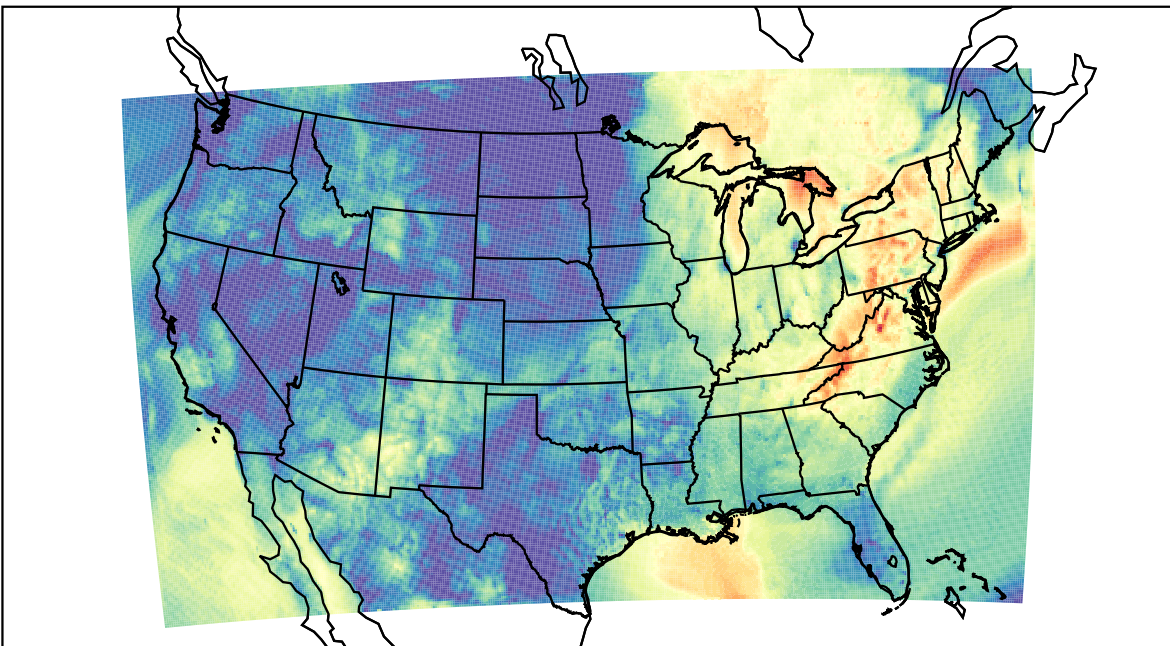
WRF (2023-10-04_14:00:00)
