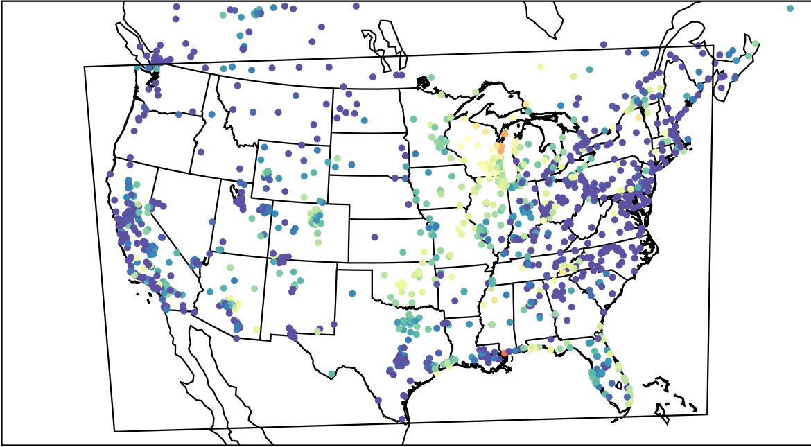
AirNOW (2023-10-04_07:00:00)
