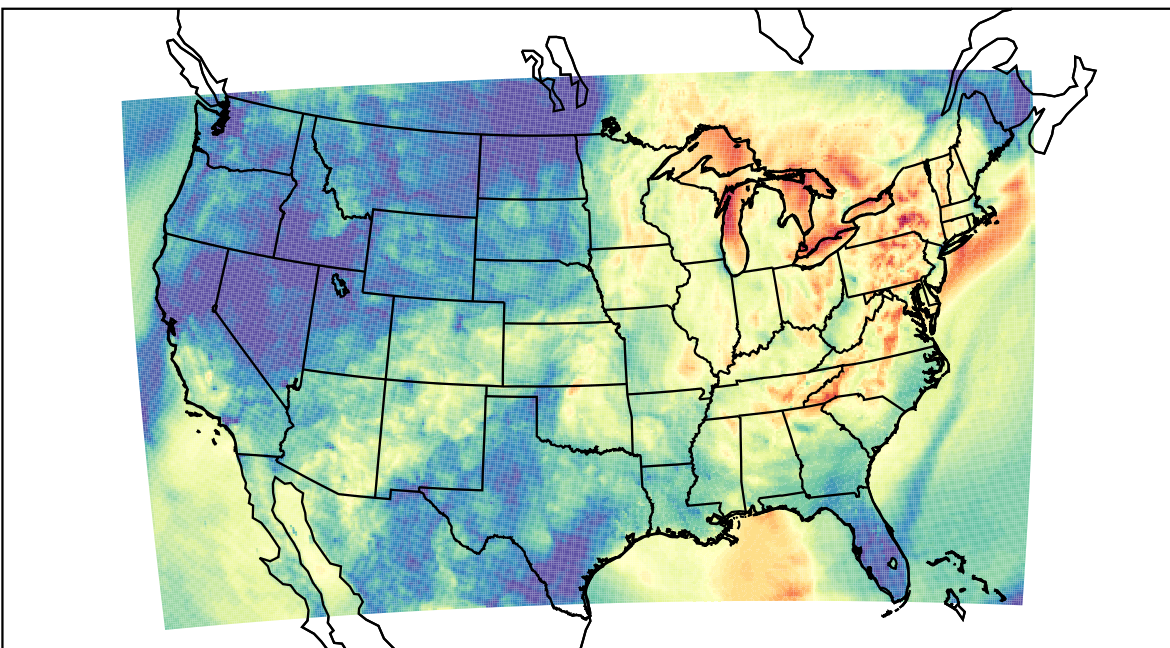
WRF (2023-10-04_05:00:00)
