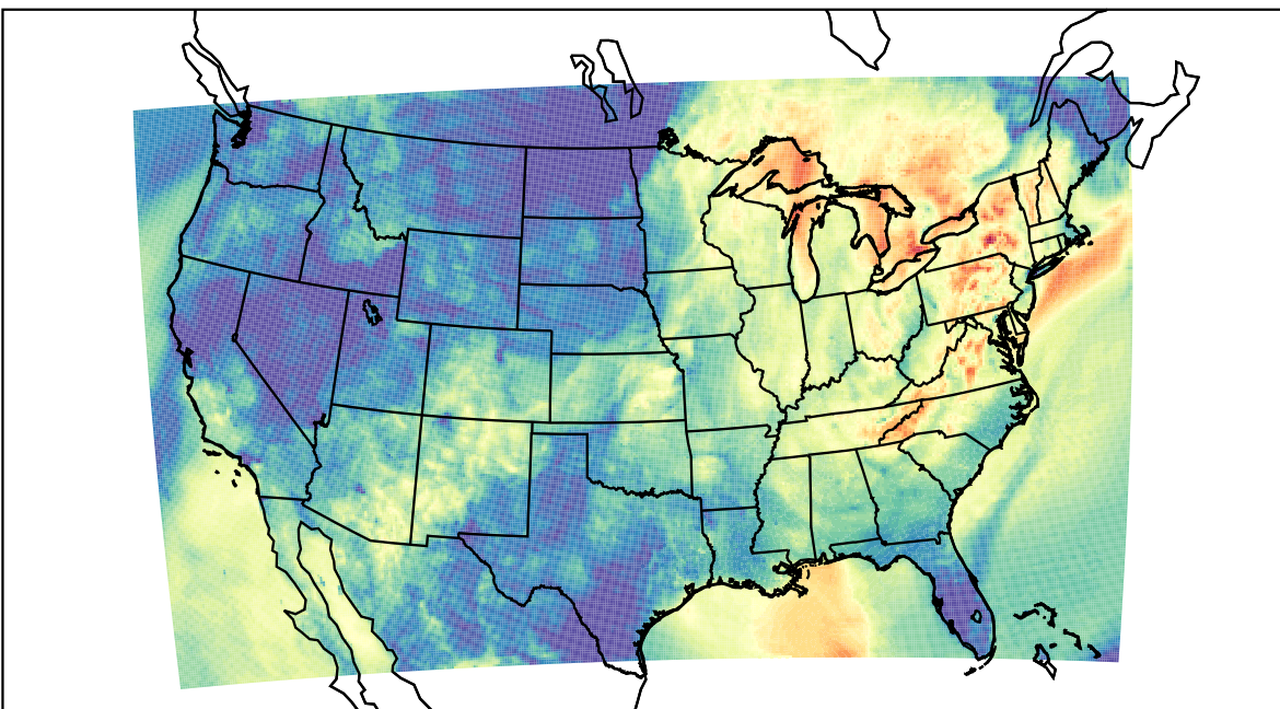
WRF (2023-10-04_08:00:00)
