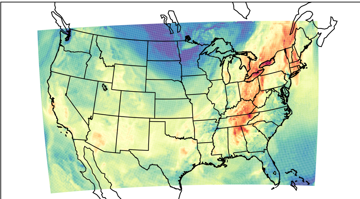
WRF (2023-10-05_22:00:00)
