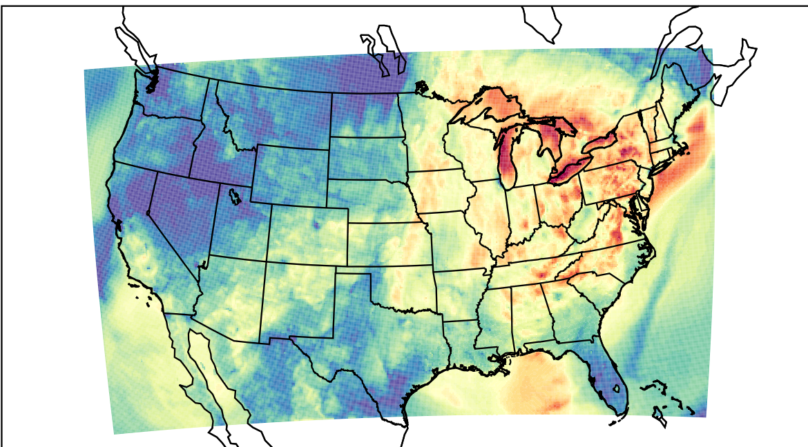
WRF (2023-10-04_03:00:00)
