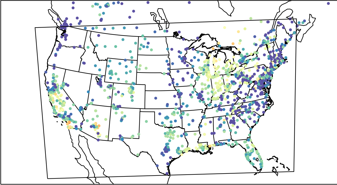
AirNOW (2023-10-05_02:00:00)
