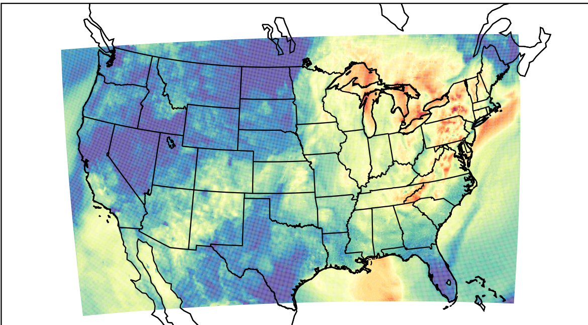
WRF (2023-10-04_07:00:00)
