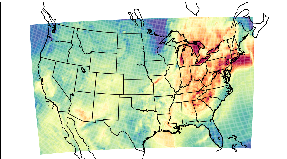
WRF (2023-10-04_23:00:00)
