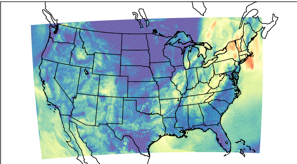
WRF (2023-10-05_13:00:00)
