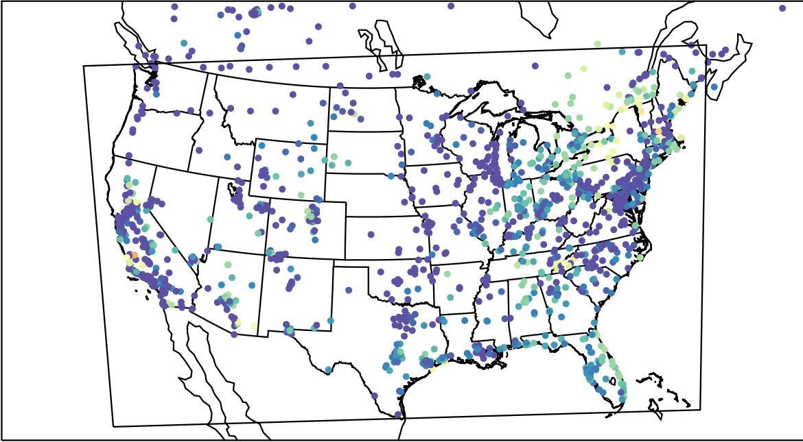
AirNOW (2023-10-05_13:00:00)
