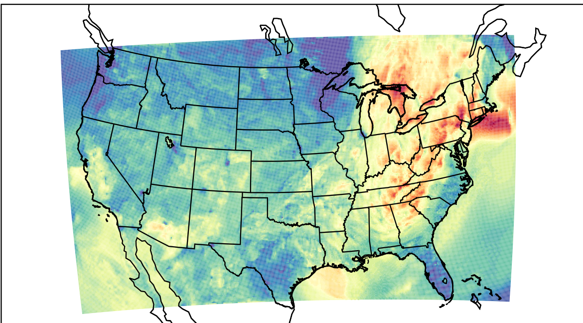
WRF (2023-10-05_02:00:00)
