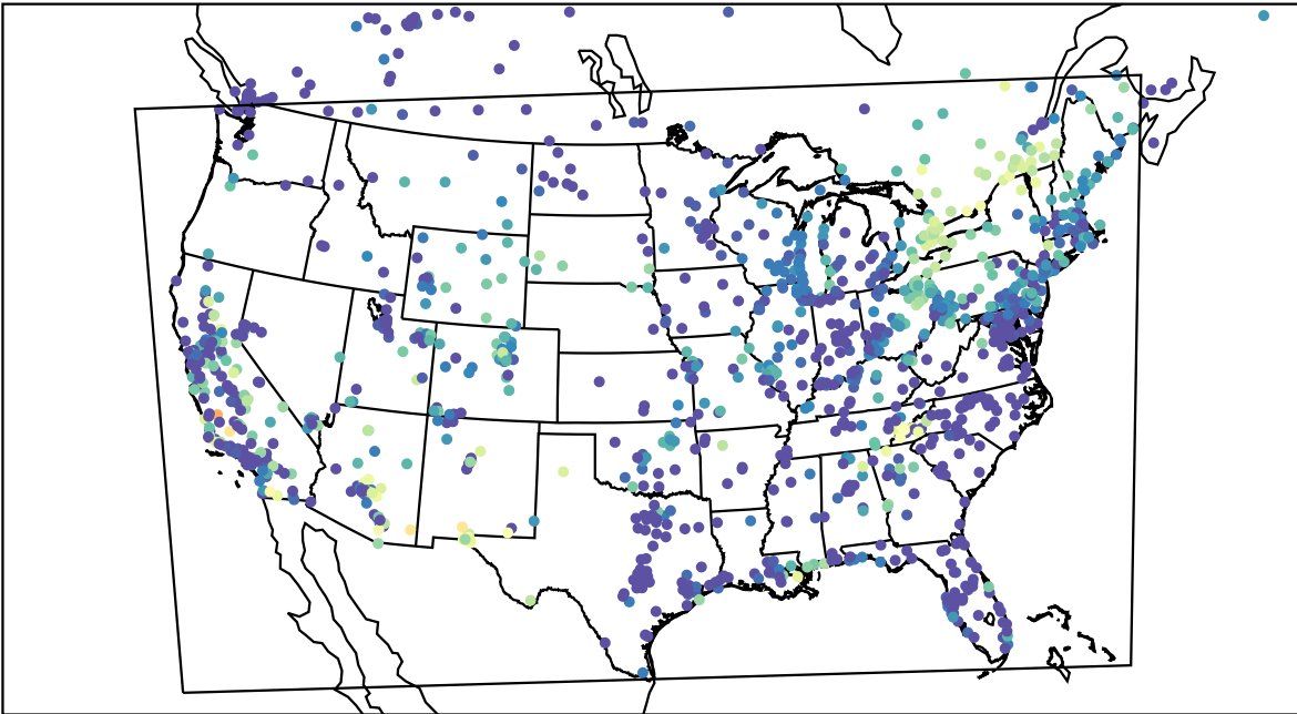
AirNOW (2023-10-06_07:00:00)
