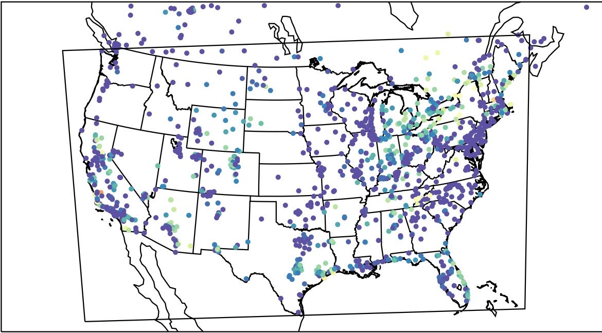
AirNOW (2023-10-05_11:00:00)
