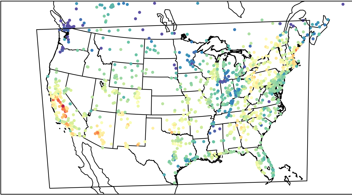
AirNOW (2023-10-05_21:00:00)
