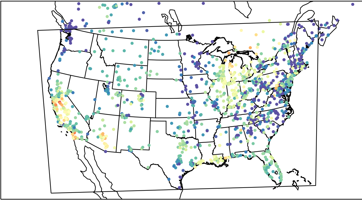
AirNOW (2023-10-05_01:00:00)
