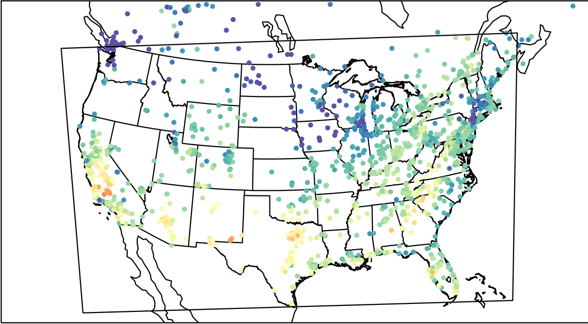
AirNOW (2023-10-06_18:00:00)
