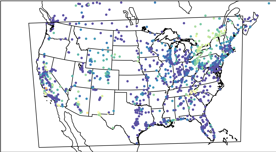
AirNOW (2023-10-06_08:00:00)
