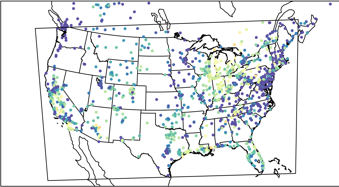
AirNOW (2023-10-05_03:00:00)
