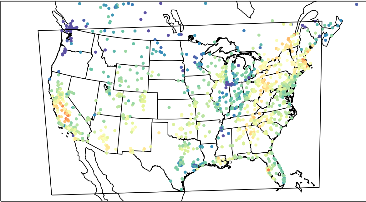
AirNOW (2023-10-05_19:00:00)
