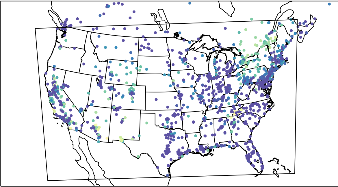
AirNOW (2023-10-06_10:00:00)
