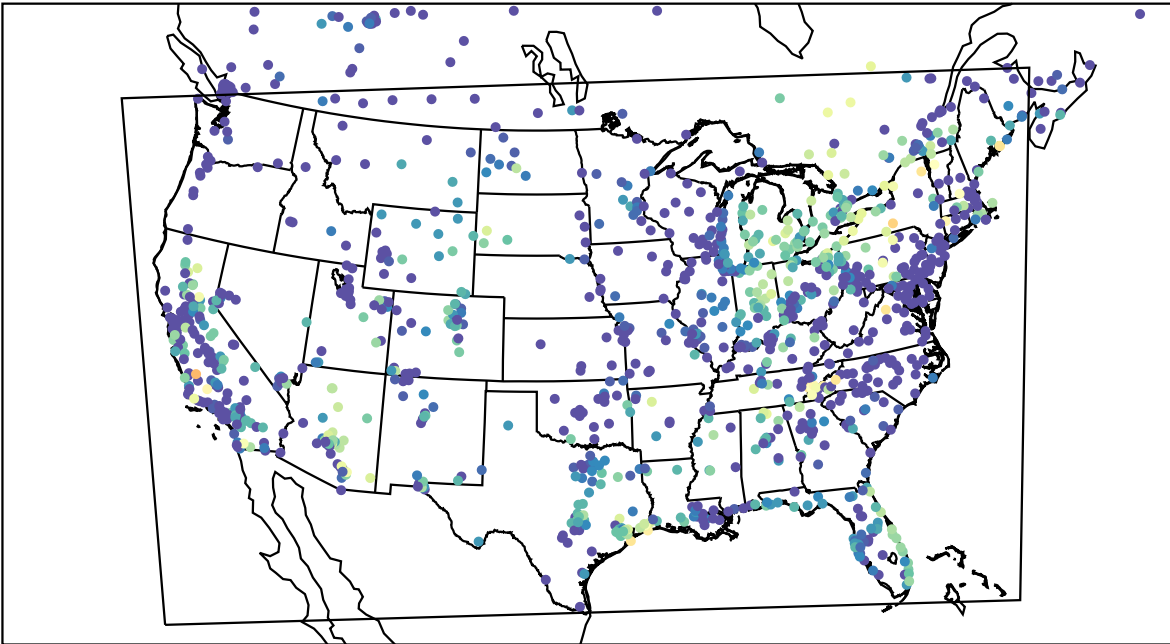
AirNOW (2023-10-05_09:00:00)
