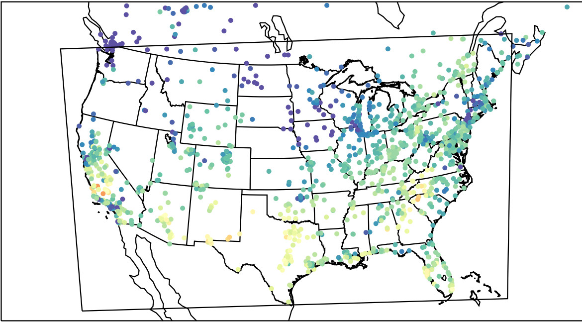
AirNOW (2023-10-06_17:00:00)
