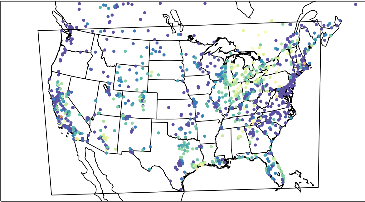
AirNOW (2023-10-05_06:00:00)
