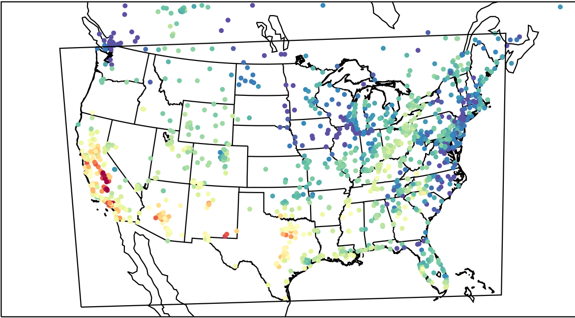
AirNOW (2023-10-06_22:00:00)
