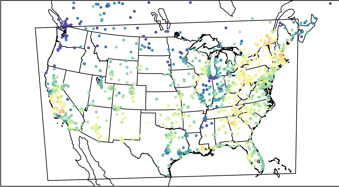
AirNOW (2023-10-05_18:00:00)
