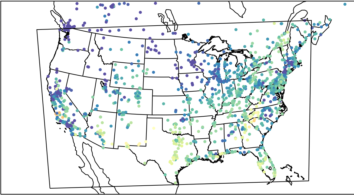
AirNOW (2023-10-06_16:00:00)
