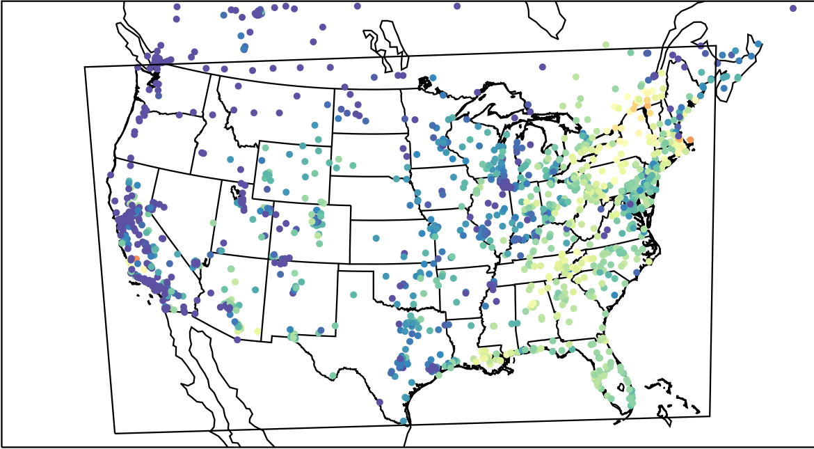
AirNOW (2023-10-05_15:00:00)
