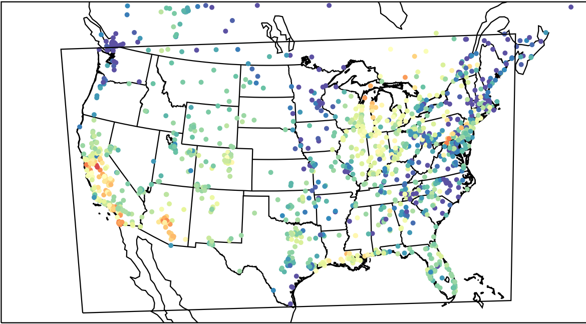
AirNOW (2023-10-05_00:00:00)
