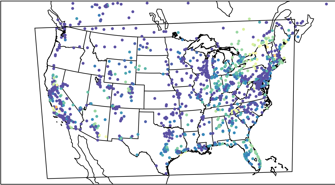
AirNOW (2023-10-05_13:00:00)
