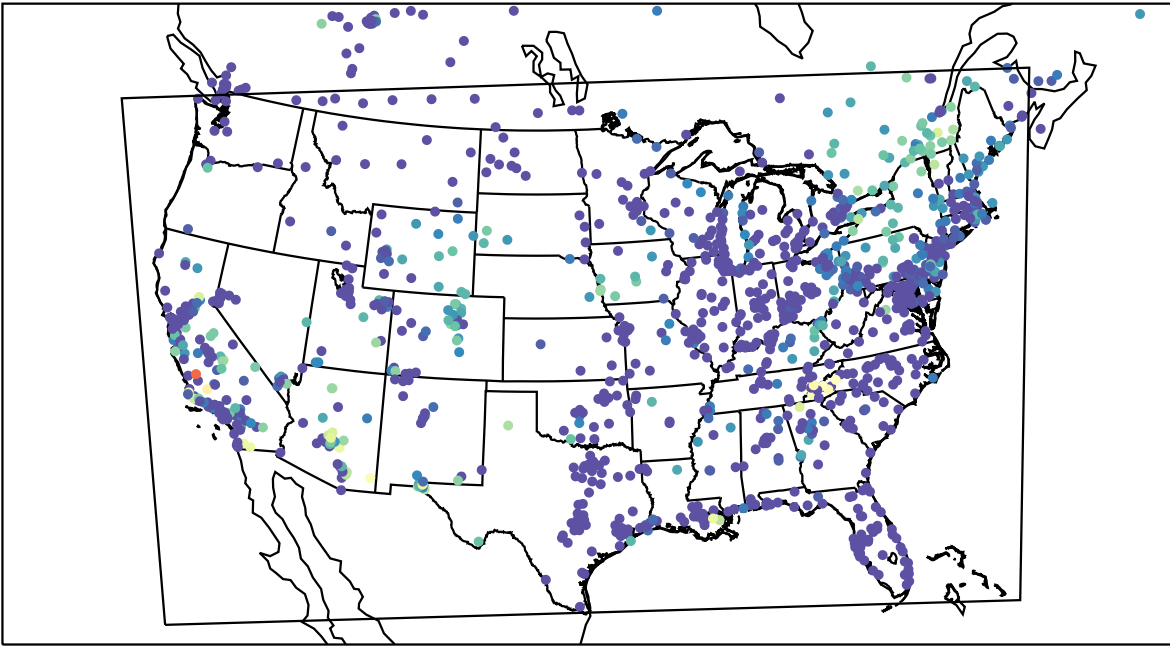
AirNOW (2023-10-06_12:00:00)
