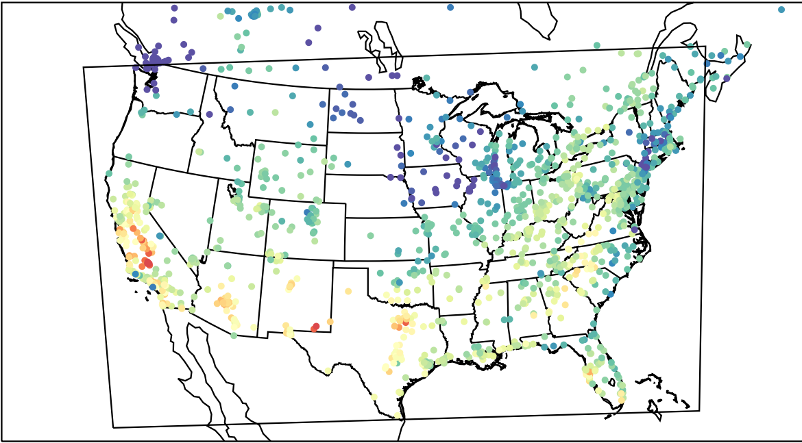
AirNOW (2023-10-06_19:00:00)
