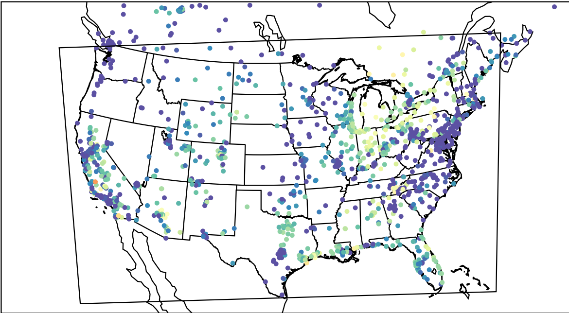
AirNOW (2023-10-05_05:00:00)
