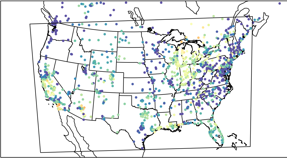
AirNOW (2023-10-05_02:00:00)
