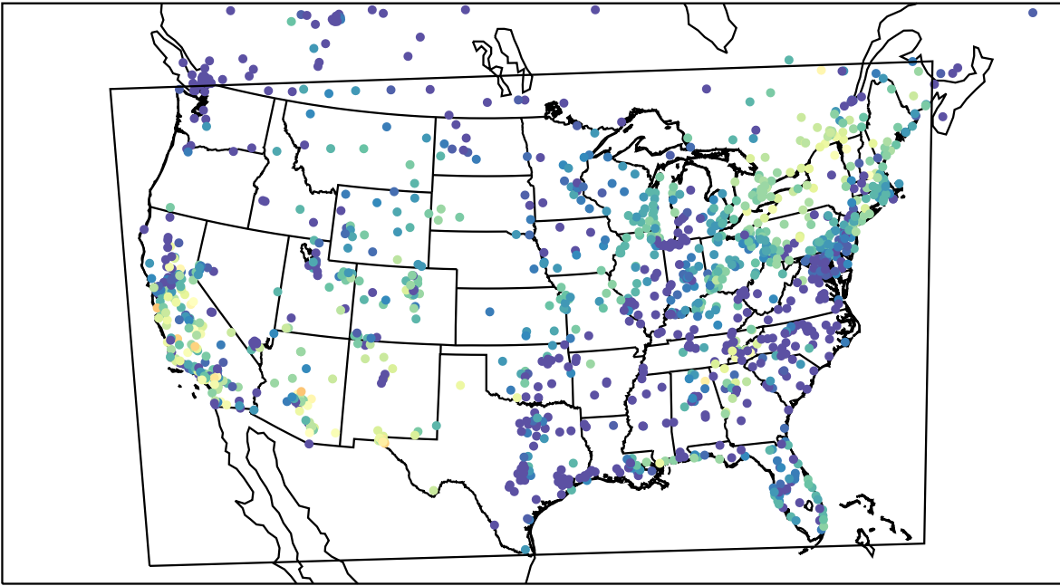
AirNOW (2023-10-06_03:00:00)
