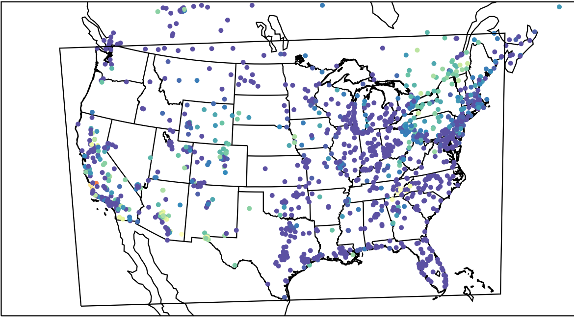
AirNOW (2023-10-06_11:00:00)
