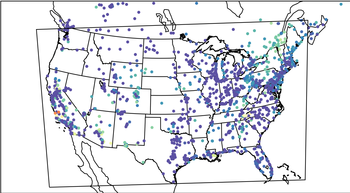
AirNOW (2023-10-06_13:00:00)
