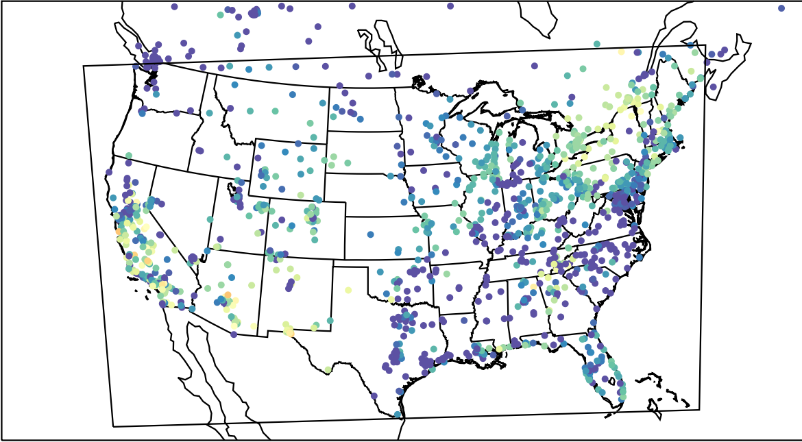
AirNOW (2023-10-06_03:00:00)
