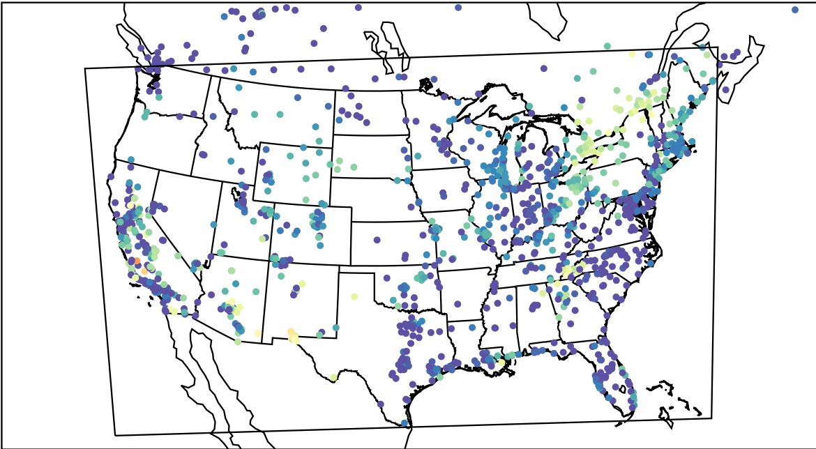
AirNOW (2023-10-06_06:00:00)
