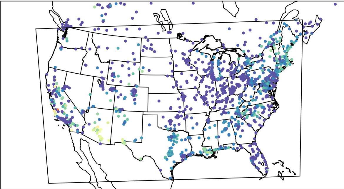
AirNOW (2023-10-07_11:00:00)
