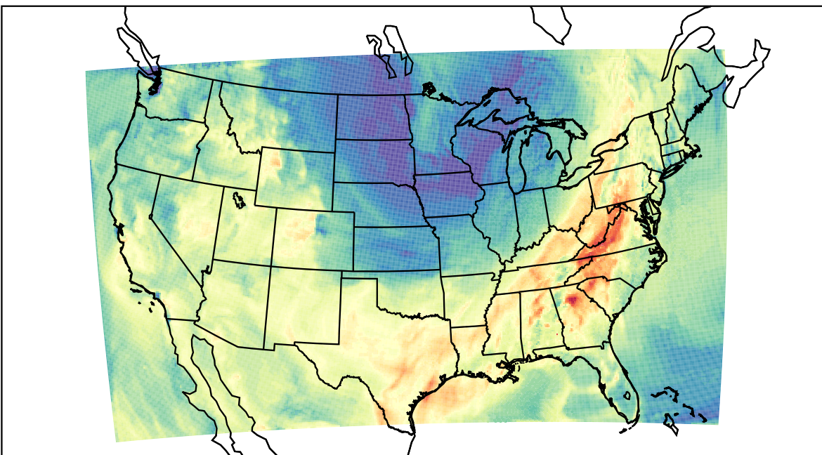
WRF (2023-10-06_19:00:00)
