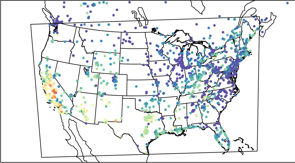
AirNOW (2023-10-07_01:00:00)
