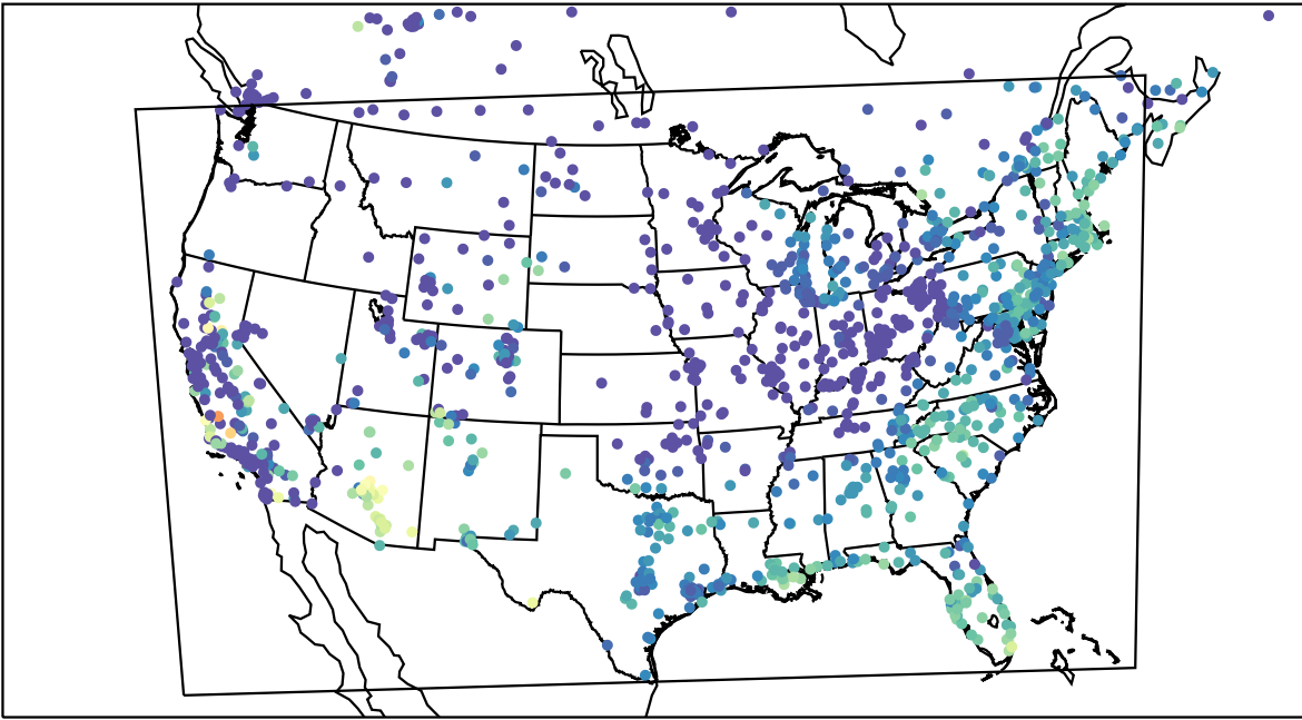
AirNOW (2023-10-07_14:00:00)
