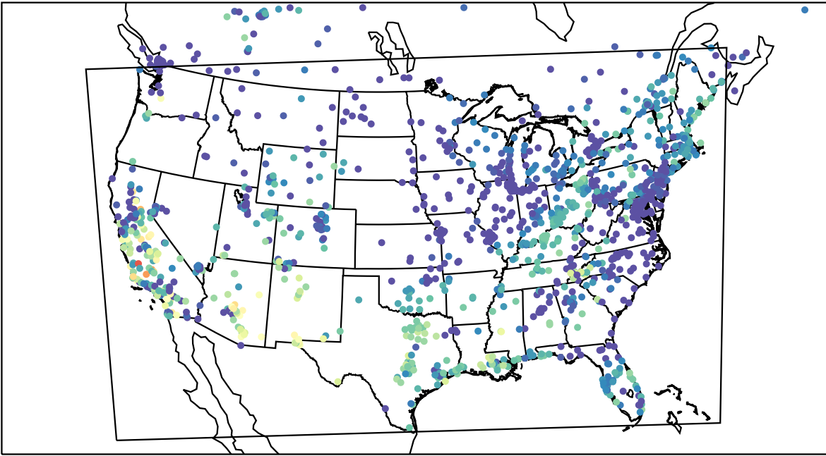
AirNOW (2023-10-07_03:00:00)
