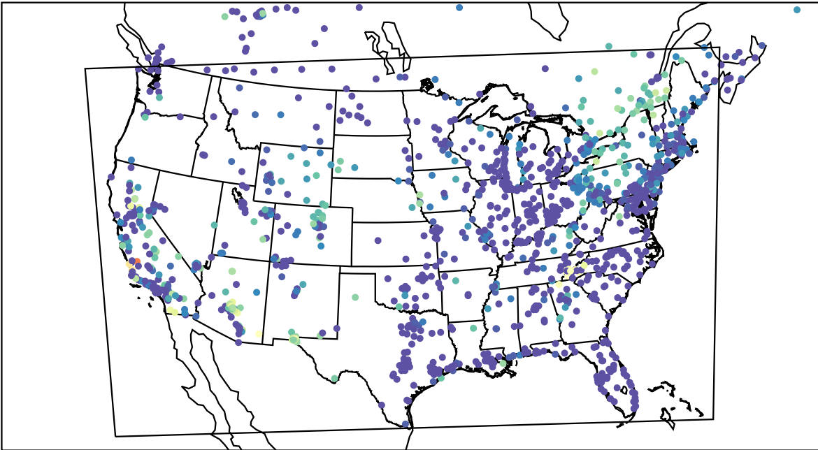
AirNOW (2023-10-06_11:00:00)
