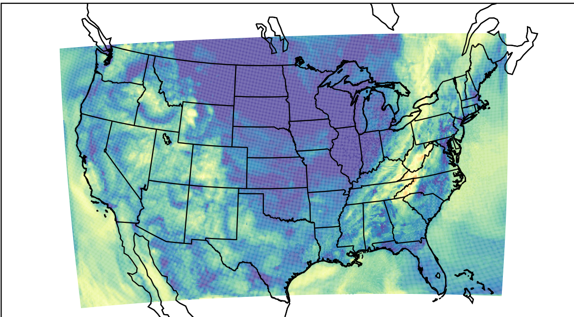
WRF (2023-10-06_14:00:00)
