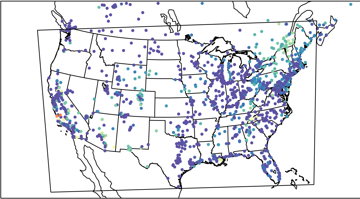
AirNOW (2023-10-06_13:00:00)
