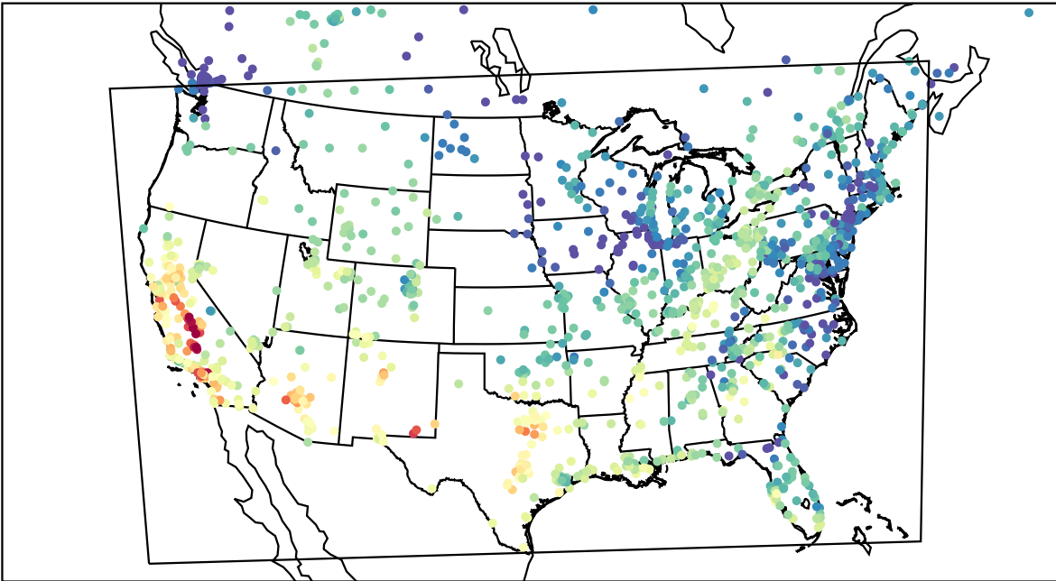
AirNOW (2023-10-06_22:00:00)
