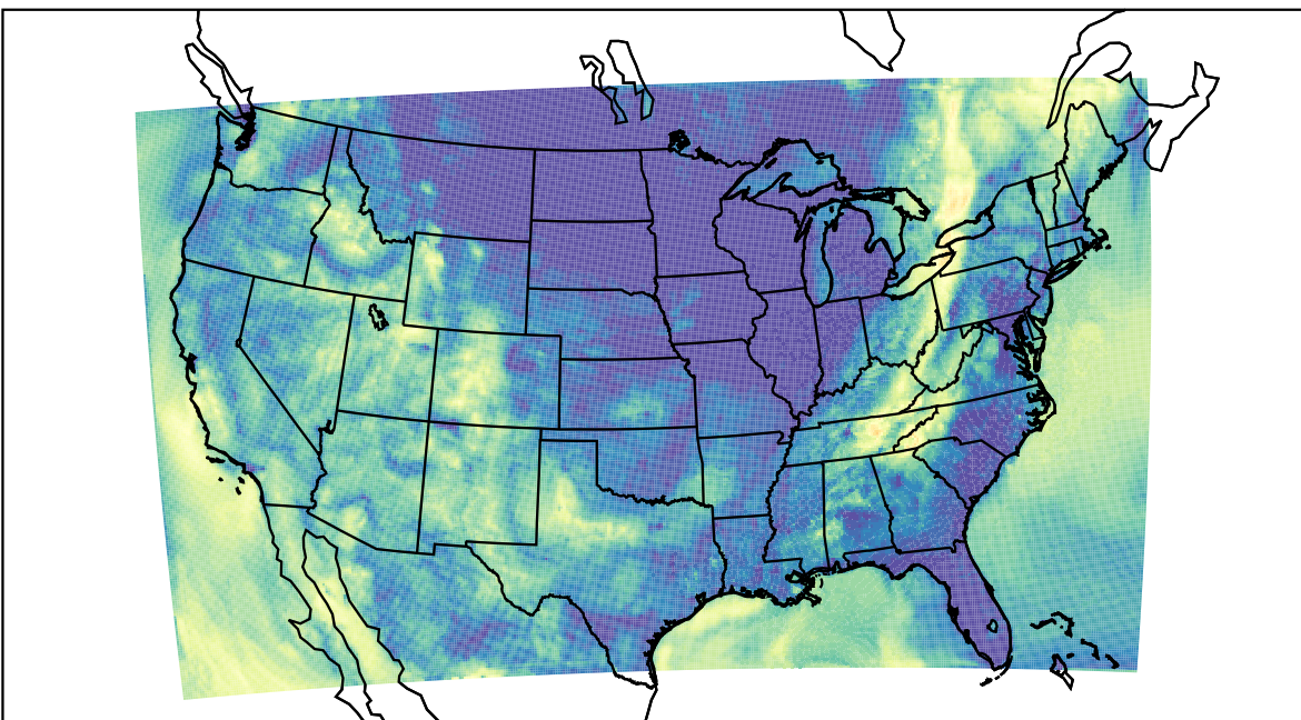
WRF (2023-10-06_11:00:00)
