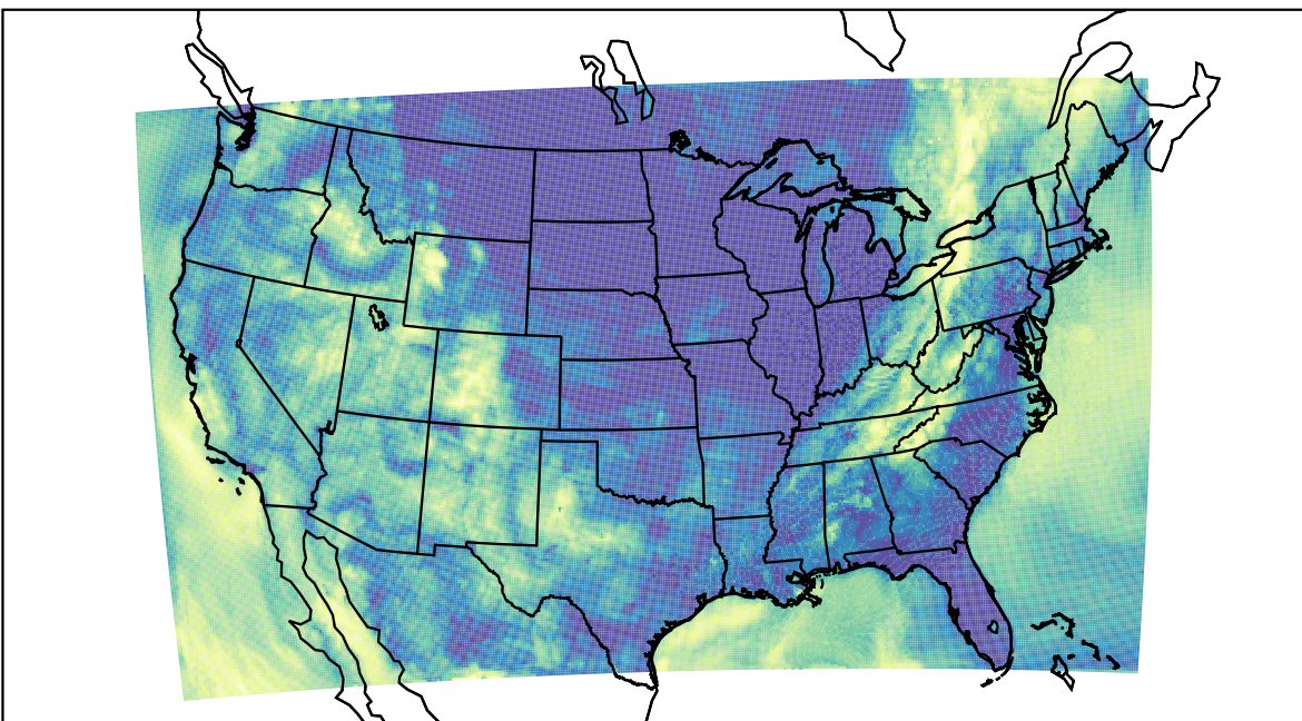
WRF (2023-10-06_13:00:00)
