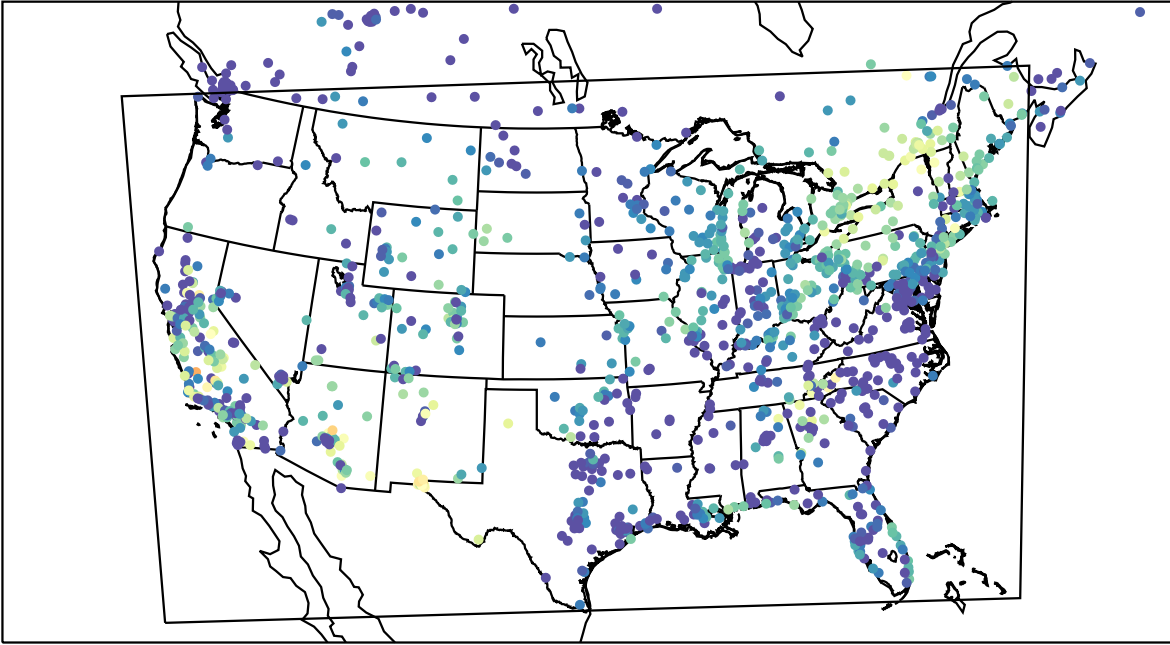
AirNOW (2023-10-06_04:00:00)
