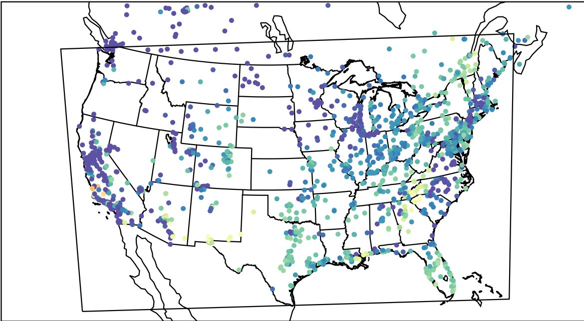
AirNOW (2023-10-06_15:00:00)
