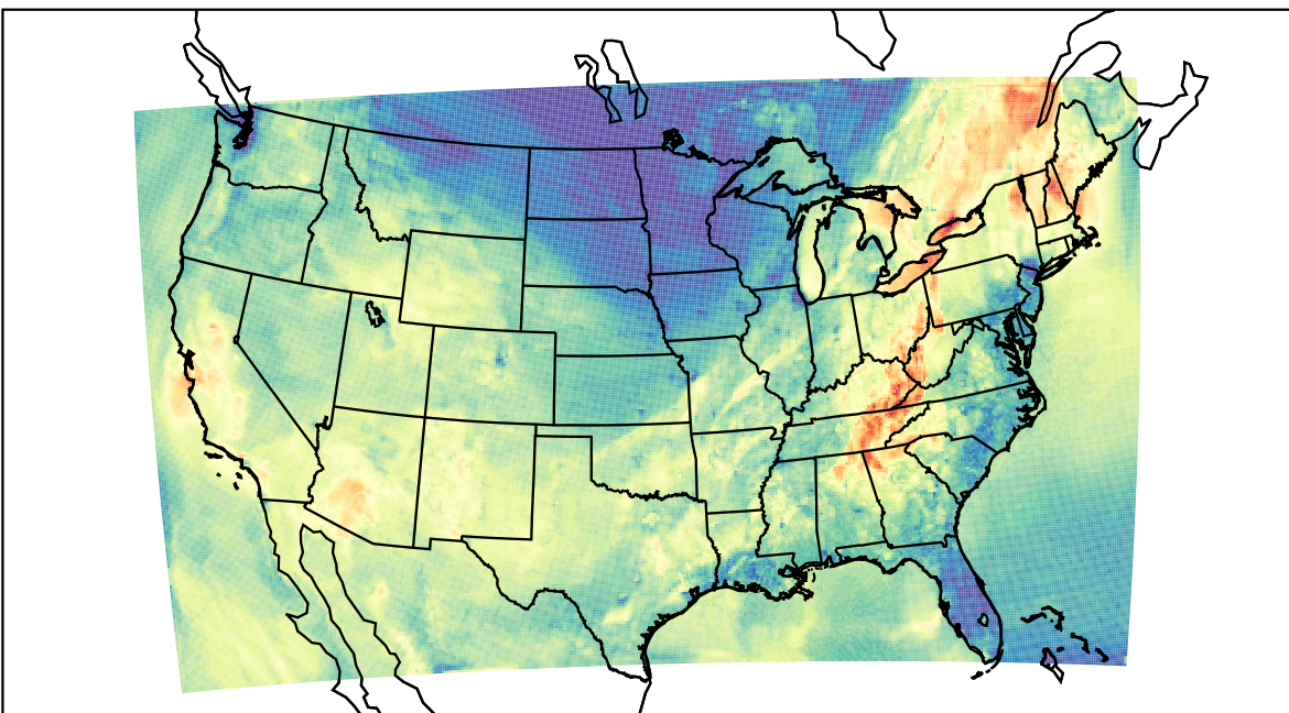
WRF (2023-10-06_00:00:00)
