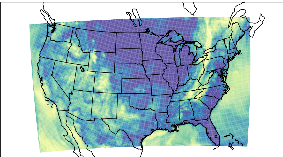
WRF (2023-10-06_12:00:00)
