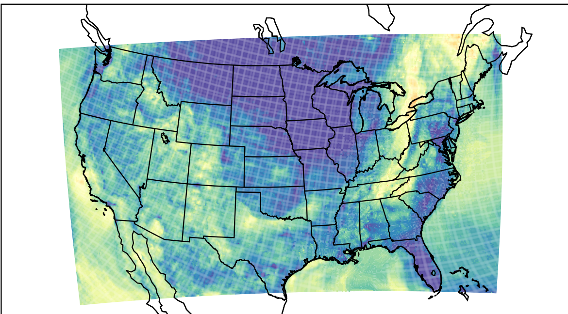
WRF (2023-10-06_08:00:00)
