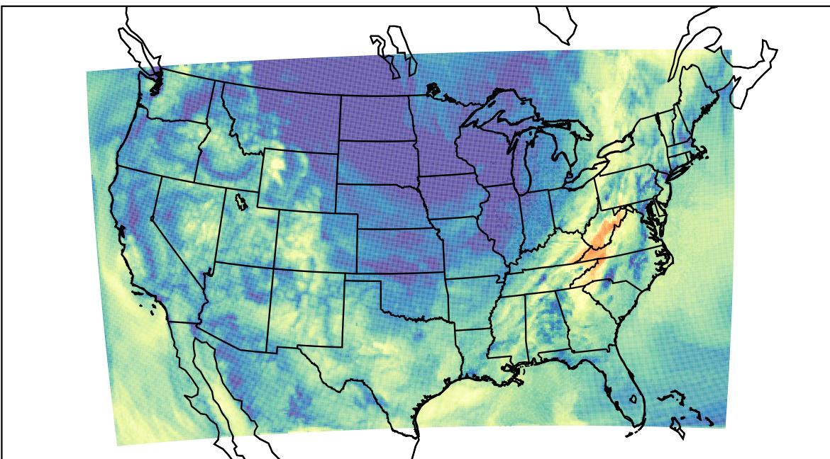
WRF (2023-10-06_15:00:00)
