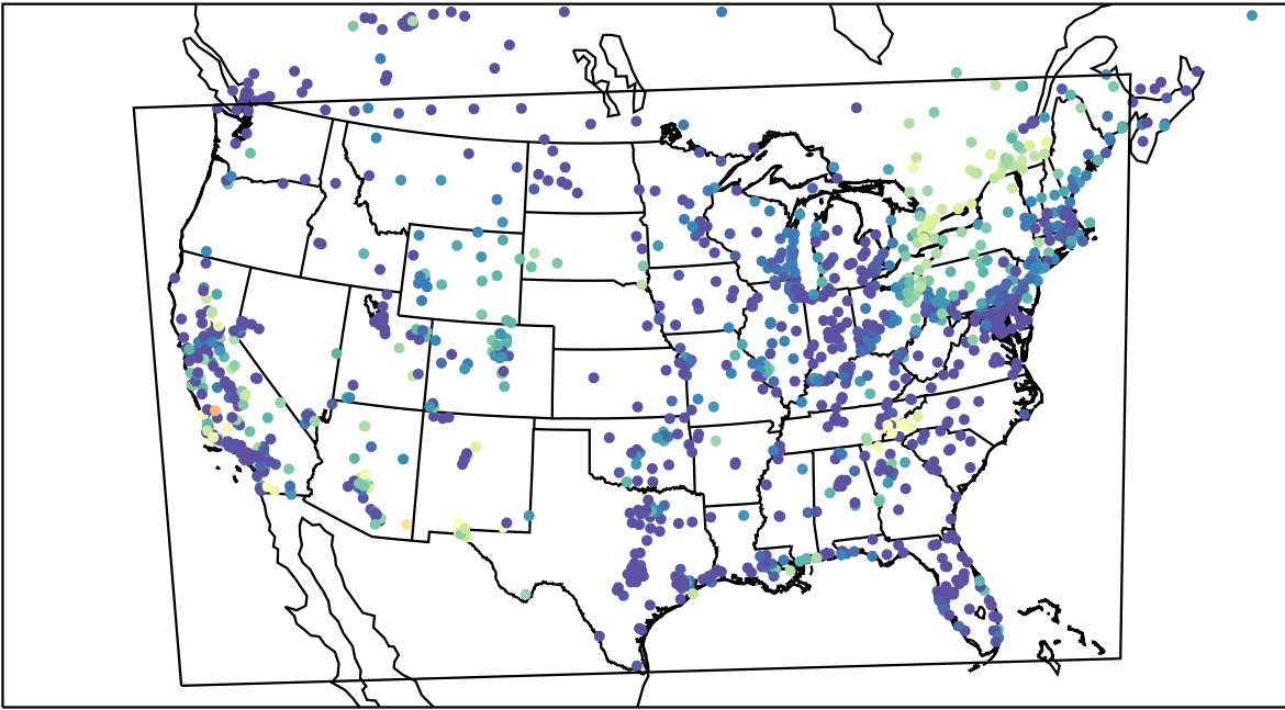
AirNOW (2023-10-06_08:00:00)
