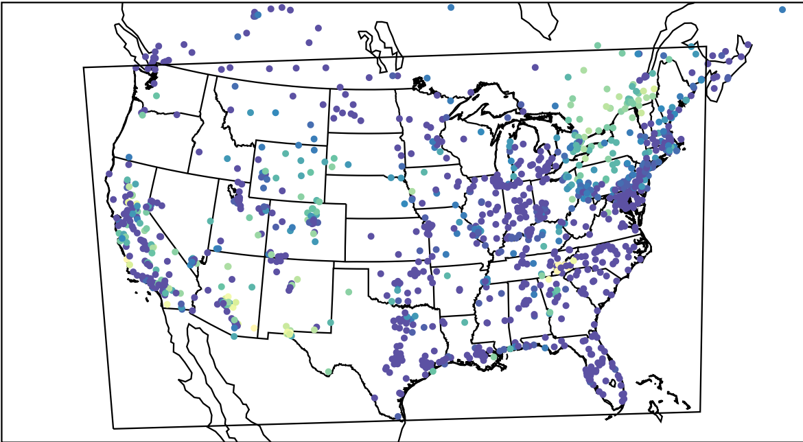
AirNOW (2023-10-06_10:00:00)
