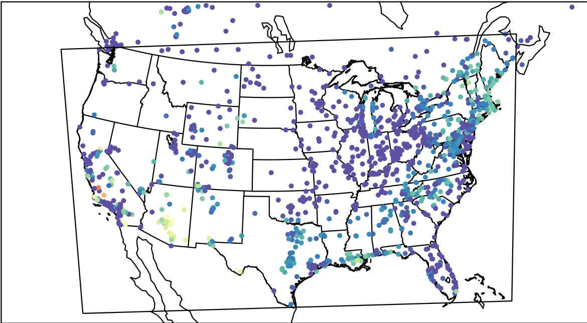
AirNOW (2023-10-07_12:00:00)
