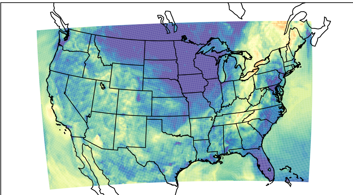
WRF (2023-10-06_06:00:00)
