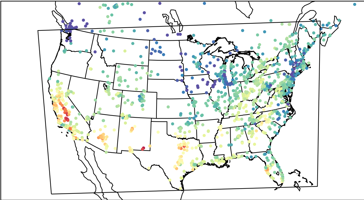
AirNOW (2023-10-06_20:00:00)
