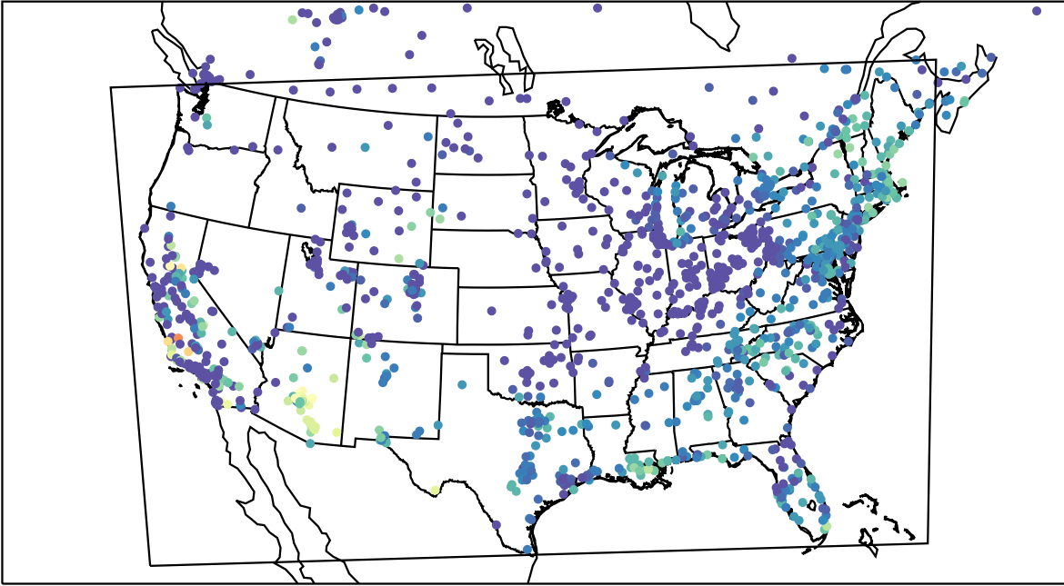
AirNOW (2023-10-07_13:00:00)
