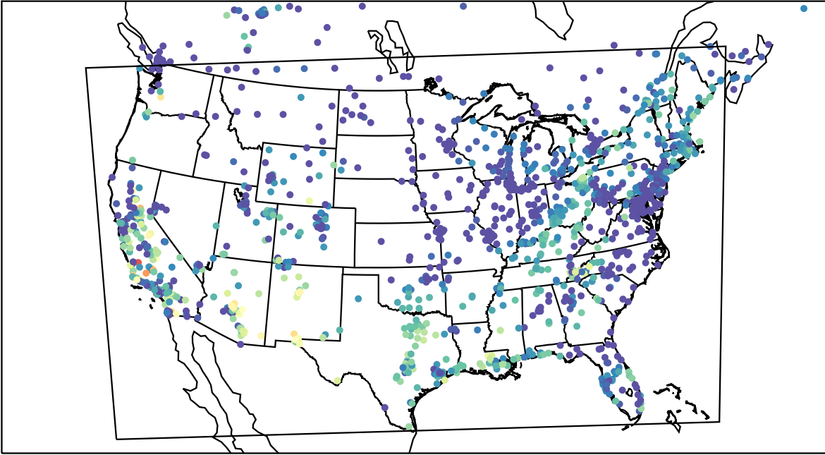
AirNOW (2023-10-07_04:00:00)
