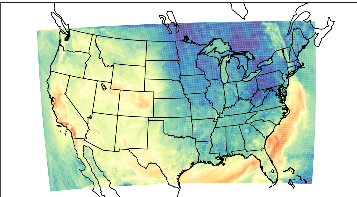
WRF (2023-10-07_23:00:00)
