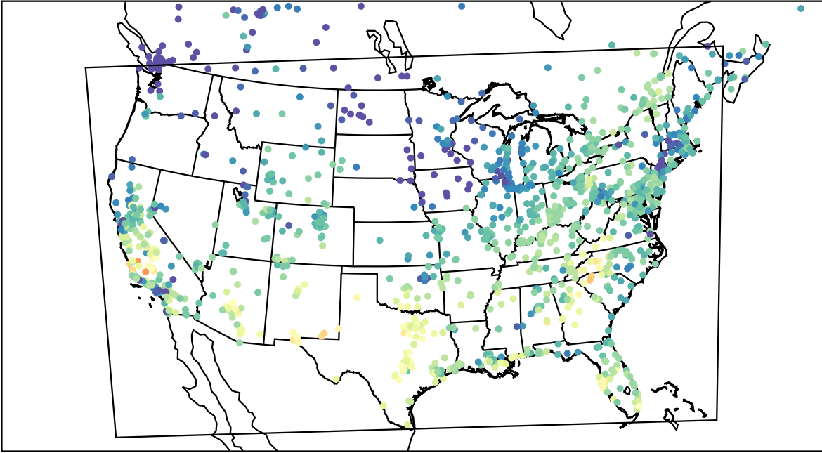
AirNOW (2023-10-06_17:00:00)
