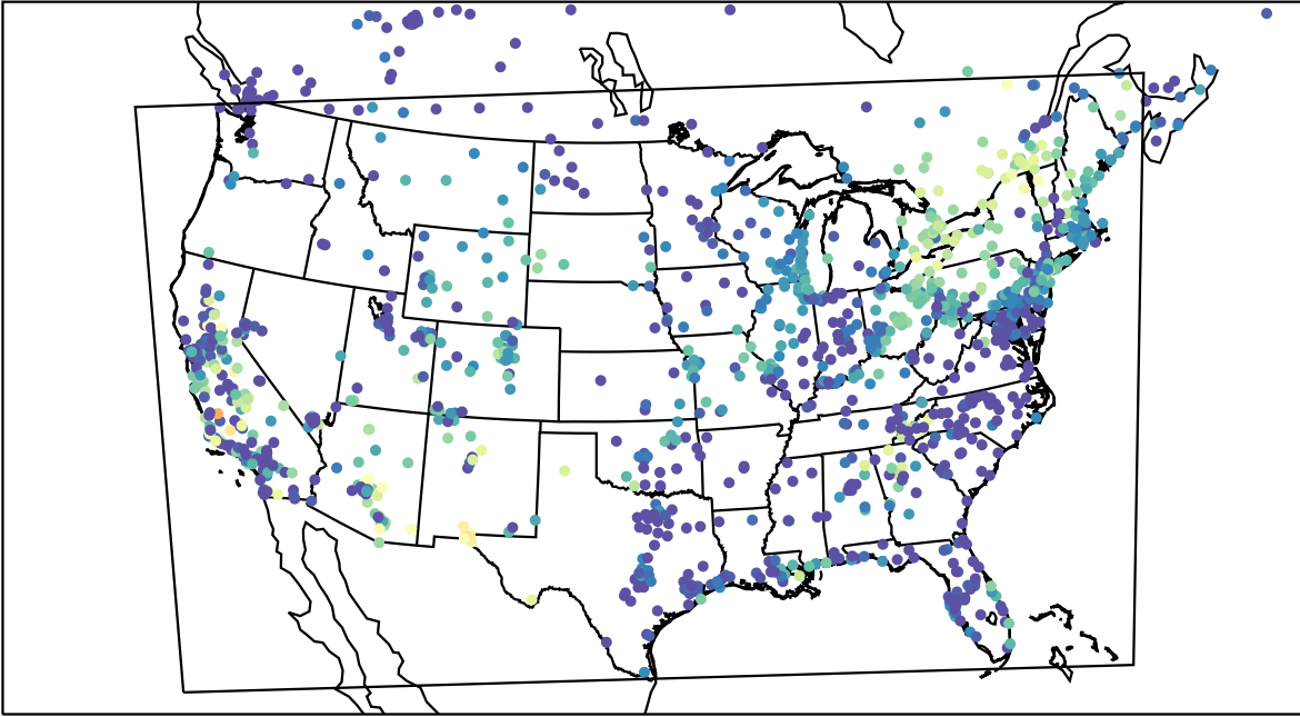
AirNOW (2023-10-06_05:00:00)
