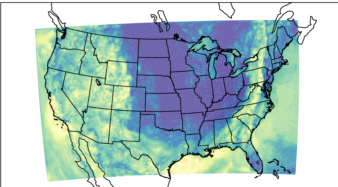
WRF (2023-10-07_06:00:00)
