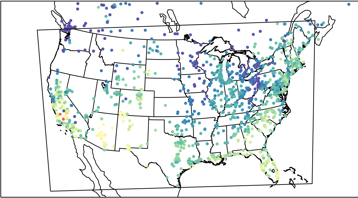
AirNOW (2023-10-07_17:00:00)
