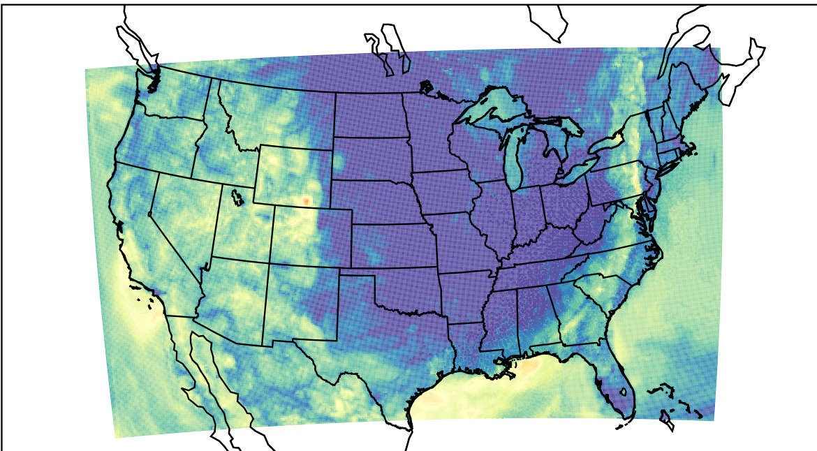
WRF (2023-10-07_09:00:00)
