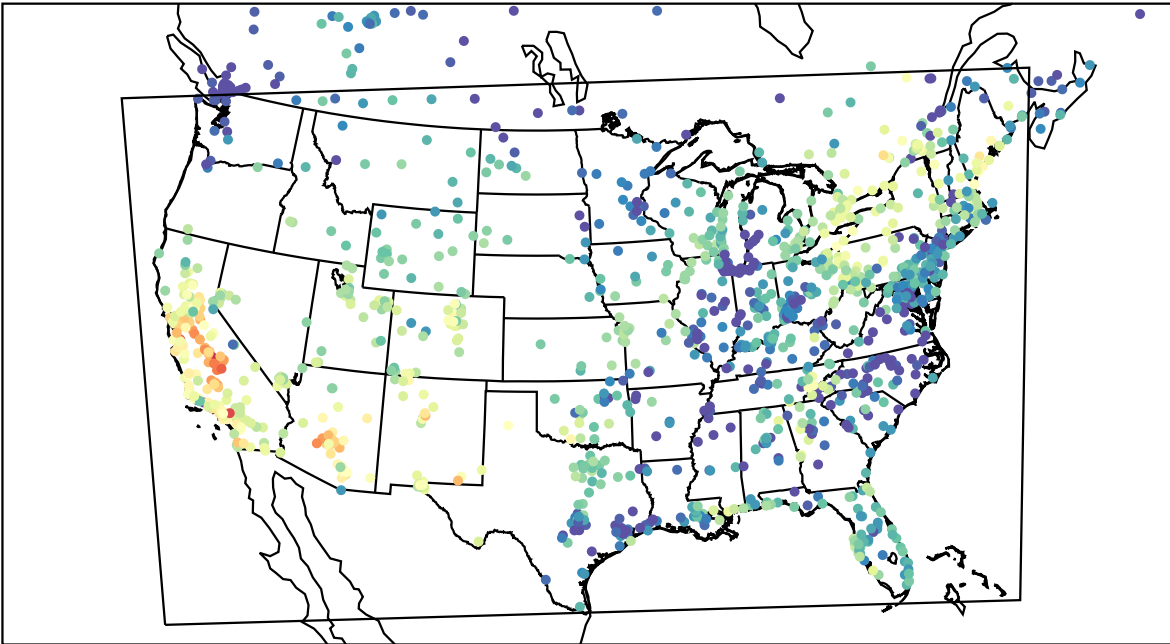
AirNOW (2023-10-06_00:00:00)
