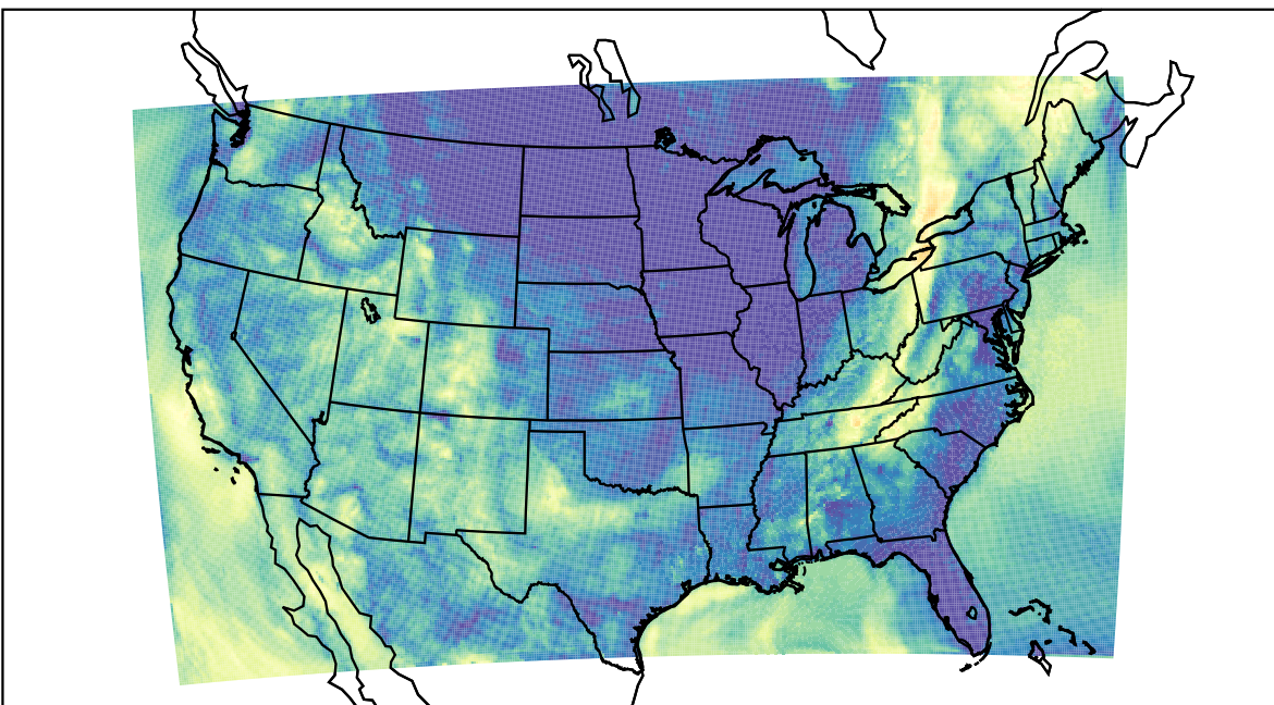
WRF (2023-10-06_10:00:00)
