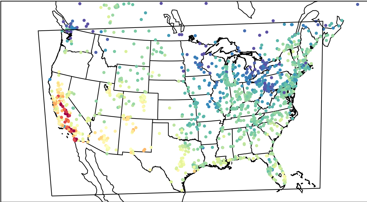
AirNOW (2023-10-07_21:00:00)
