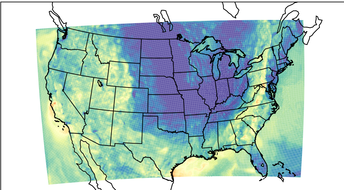
WRF (2023-10-07_04:00:00)
