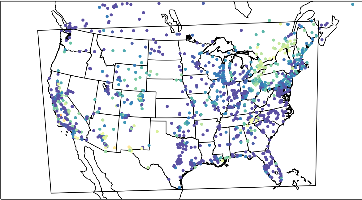
AirNOW (2023-10-06_07:00:00)
