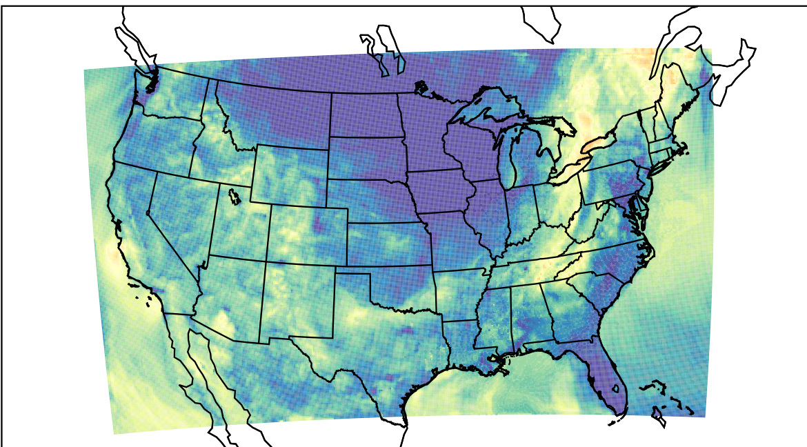
WRF (2023-10-06_07:00:00)
