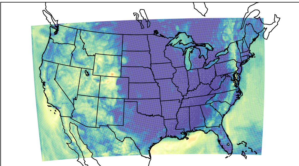
WRF (2023-10-07_12:00:00)
