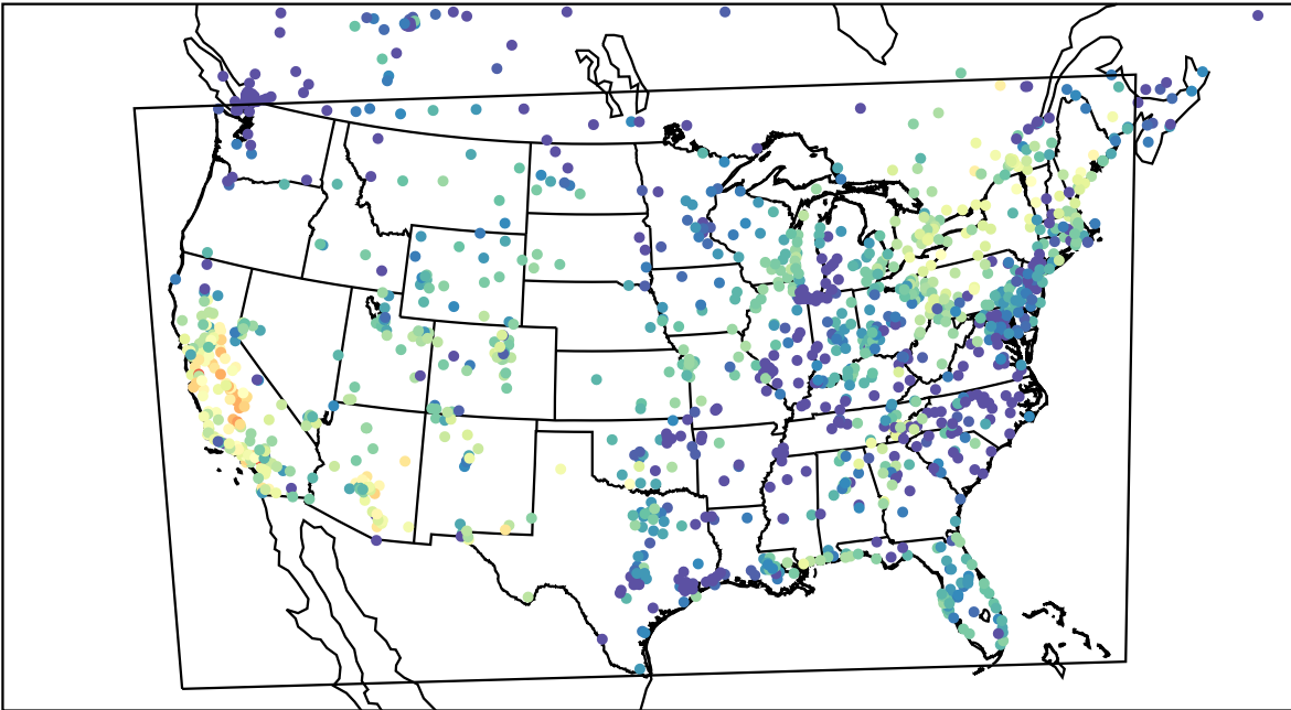
AirNOW (2023-10-06_01:00:00)
