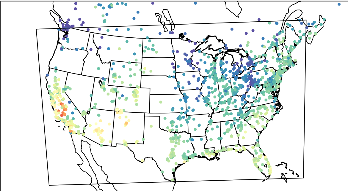
AirNOW (2023-10-07_18:00:00)
