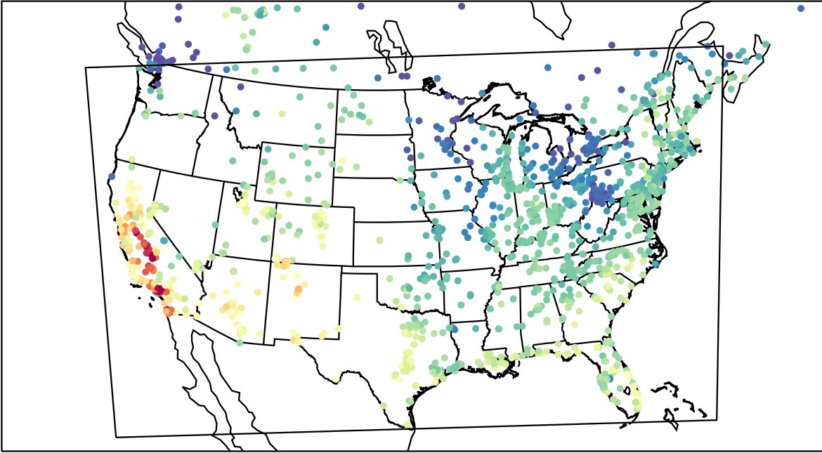
AirNOW (2023-10-07_20:00:00)
