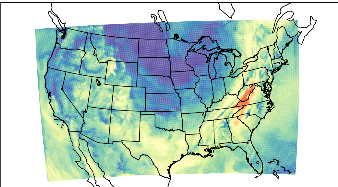
WRF (2023-10-06_16:00:00)
