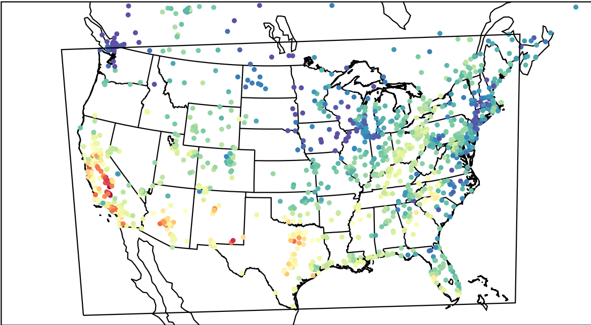
AirNOW (2023-10-06_21:00:00)
