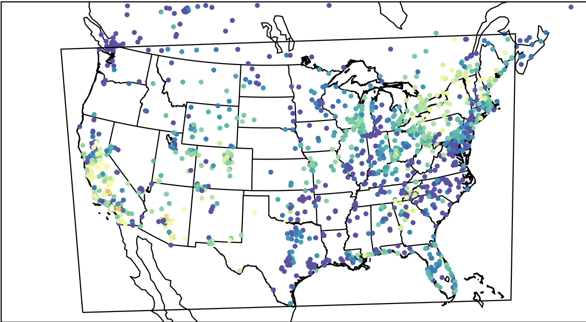
AirNOW (2023-10-06_02:00:00)
