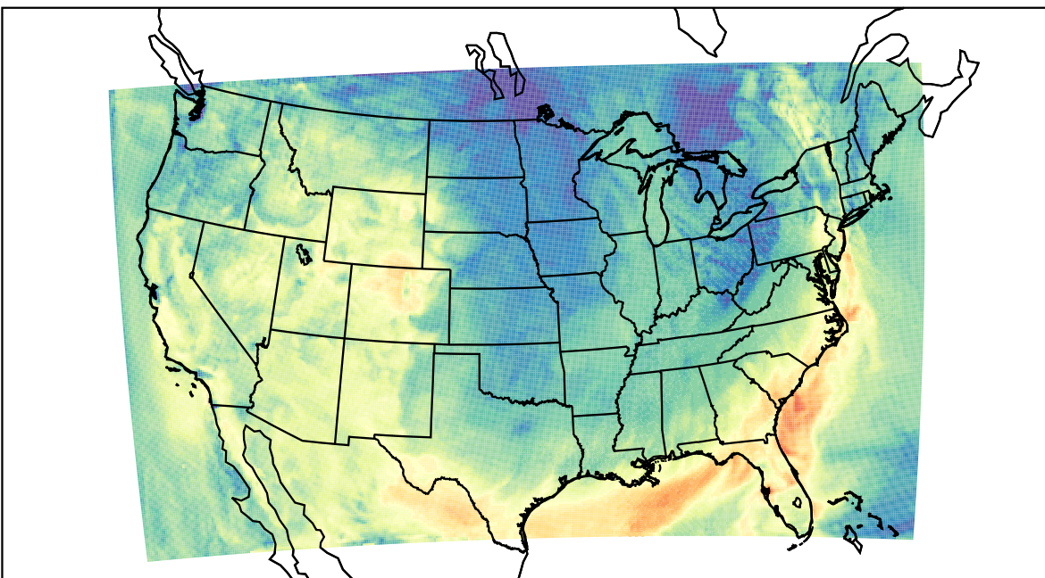
WRF (2023-10-07_18:00:00)
