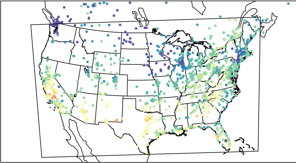
AirNOW (2023-10-06_18:00:00)
