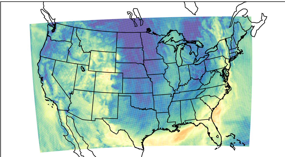
WRF (2023-10-07_16:00:00)
