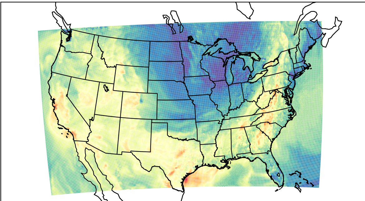
WRF (2023-10-06_23:00:00)
