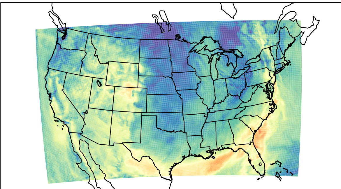
WRF (2023-10-07_17:00:00)
