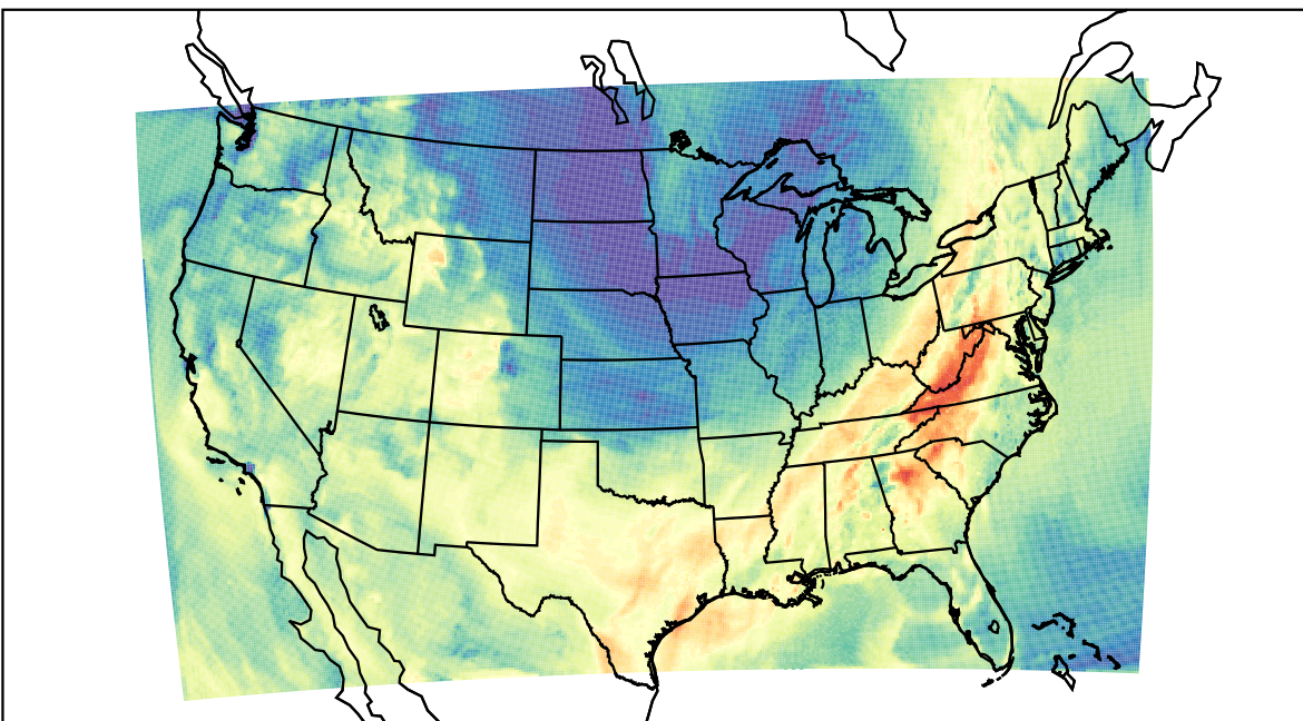
WRF (2023-10-06_18:00:00)
