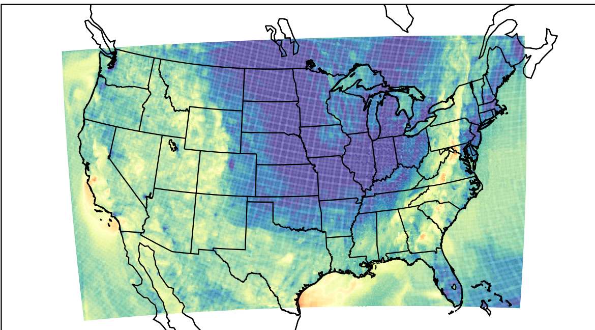
WRF (2023-10-07_03:00:00)
