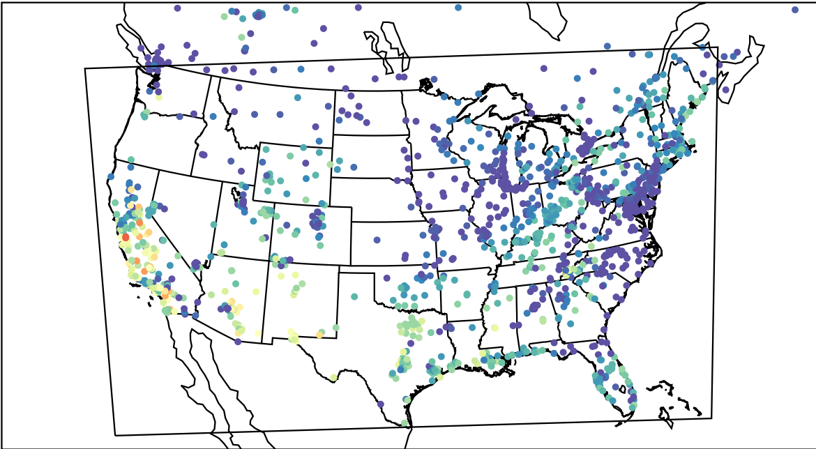
AirNOW (2023-10-07_02:00:00)
