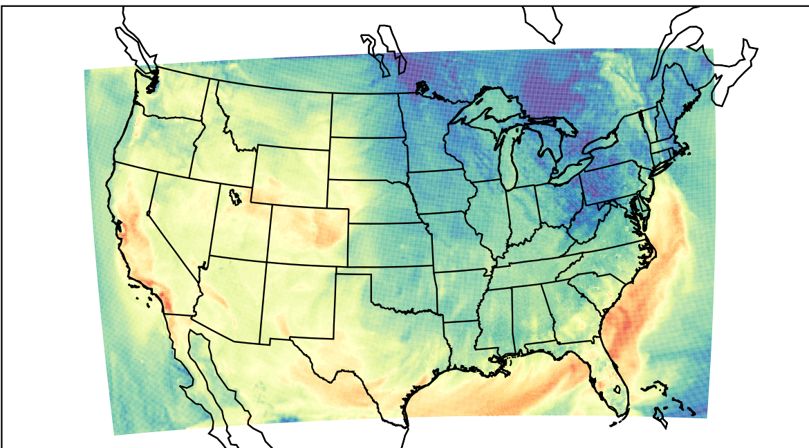
WRF (2023-10-07_22:00:00)
