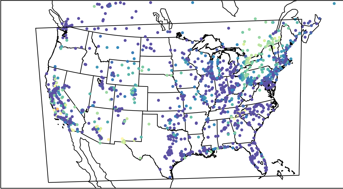
AirNOW (2023-10-06_09:00:00)
