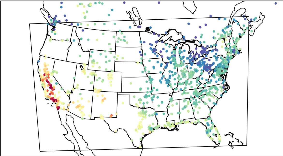
AirNOW (2023-10-07_22:00:00)
