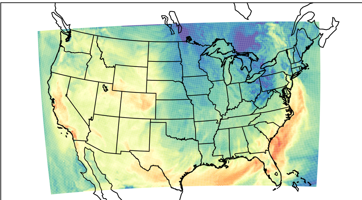
WRF (2023-10-07_21:00:00)
