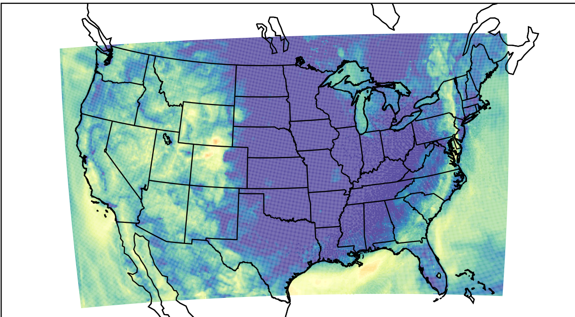
WRF (2023-10-07_13:00:00)
