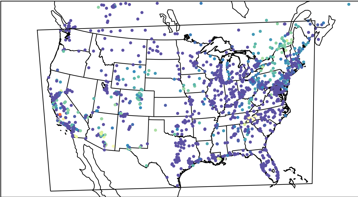
AirNOW (2023-10-06_12:00:00)
