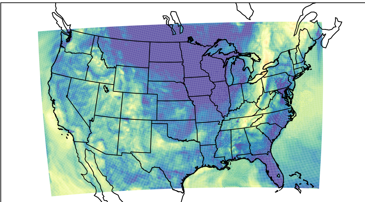
WRF (2023-10-06_09:00:00)
