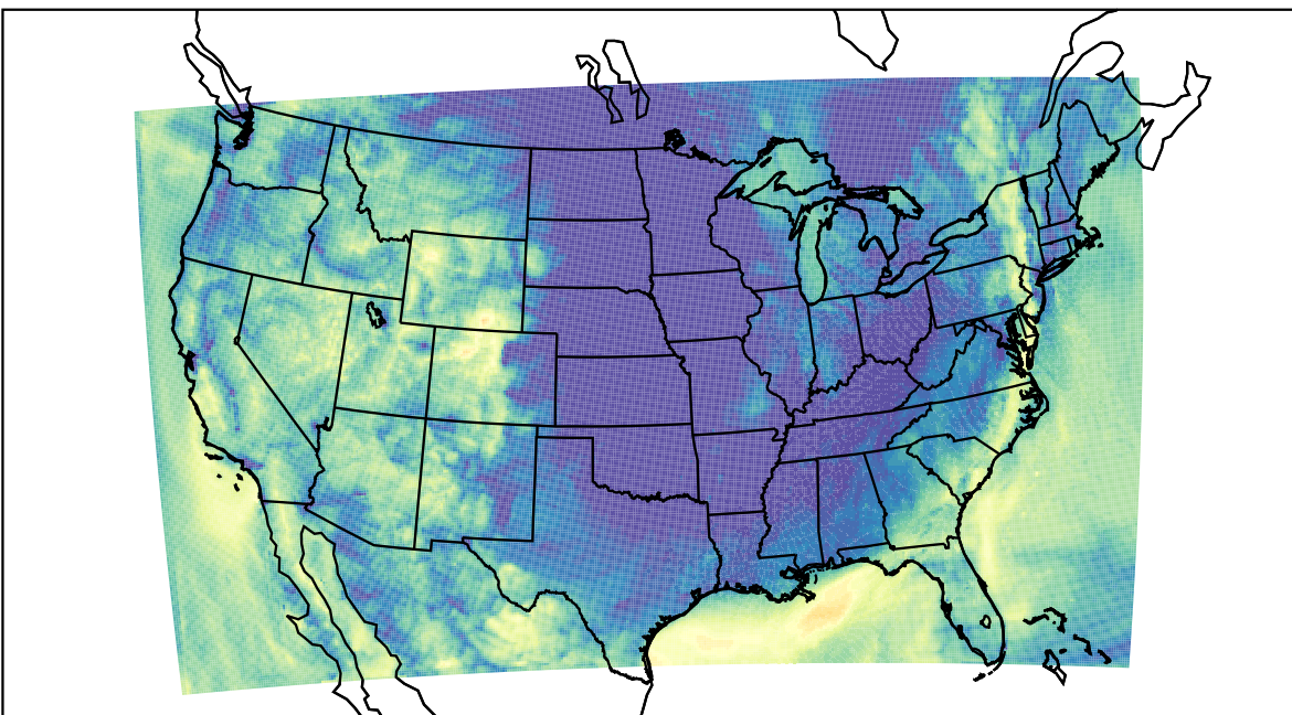
WRF (2023-10-07_14:00:00)
