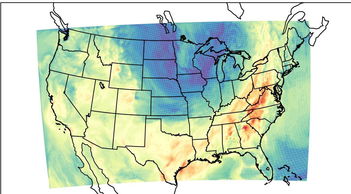
WRF (2023-10-06_20:00:00)
