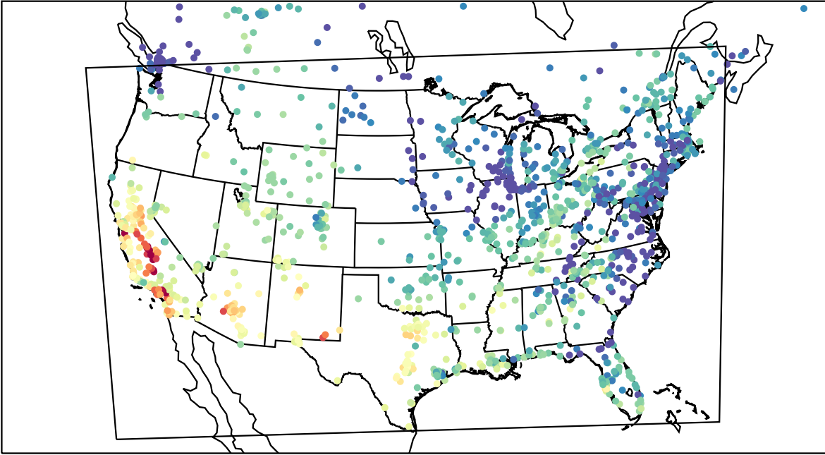
AirNOW (2023-10-06_23:00:00)
