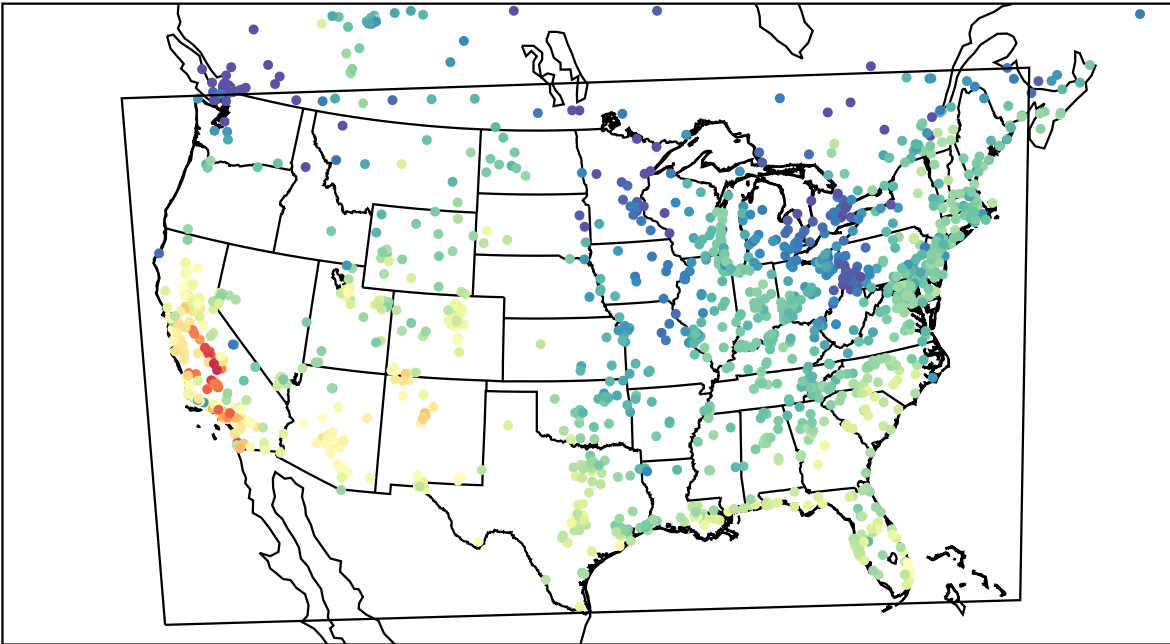
AirNOW (2023-10-07_19:00:00)
