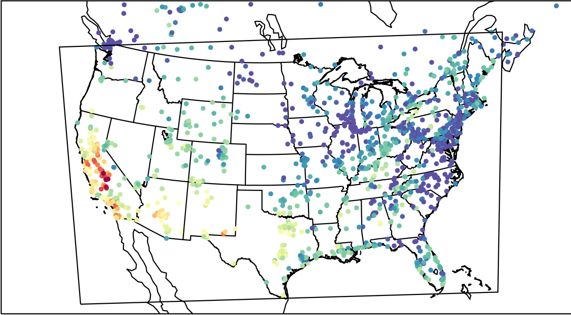
AirNOW (2023-10-07_00:00:00)
