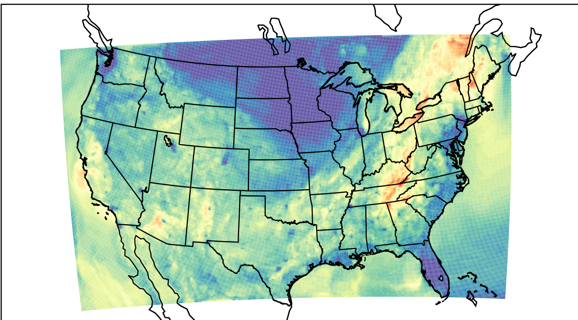
WRF (2023-10-06_02:00:00)
