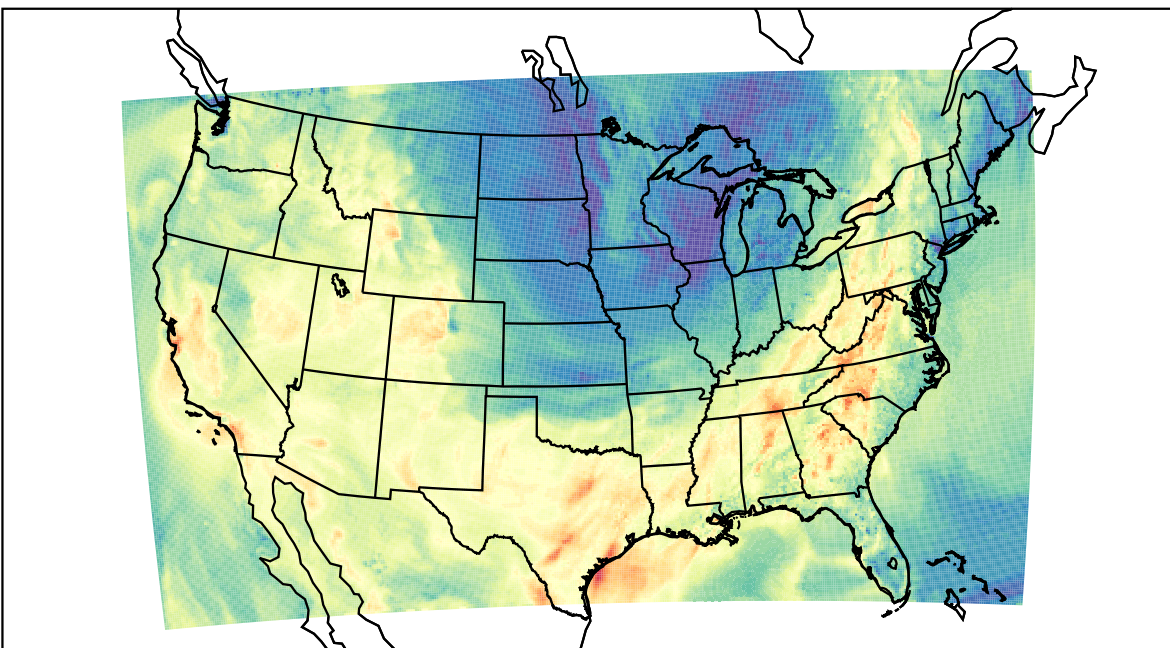
WRF (2023-10-06_22:00:00)
