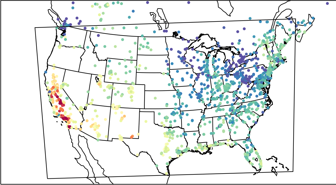
AirNOW (2023-10-07_23:00:00)
