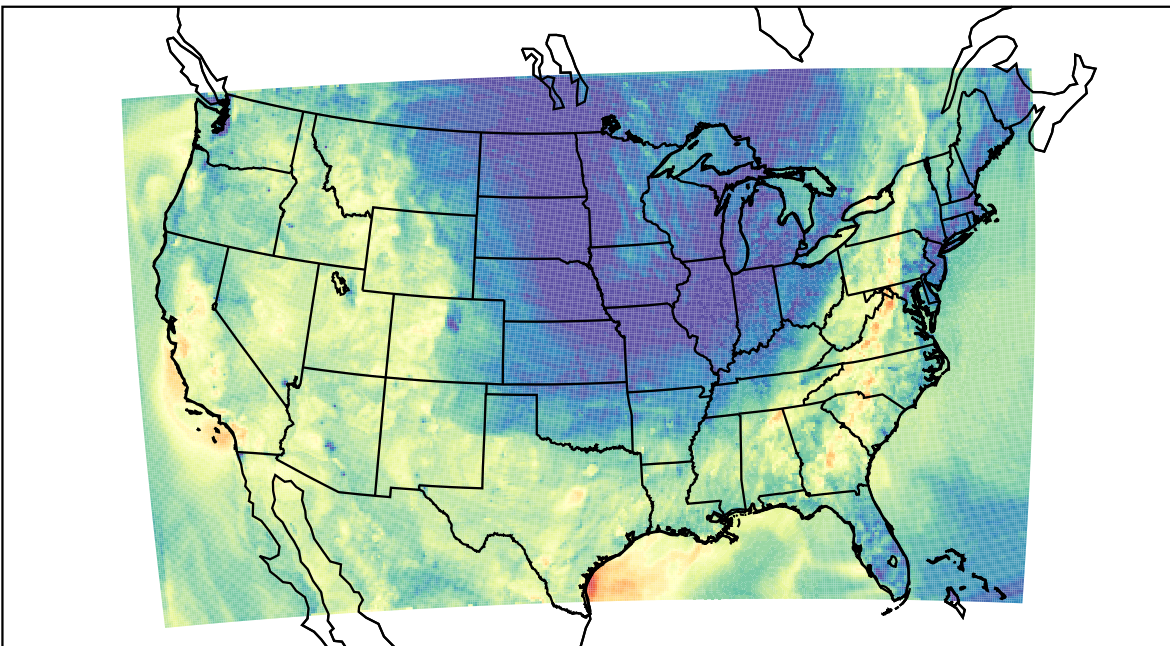
WRF (2023-10-07_01:00:00)
