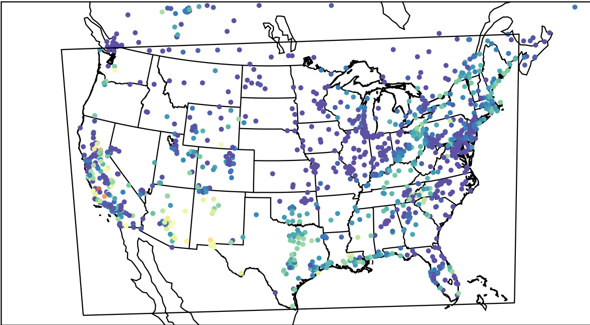
AirNOW (2023-10-07_05:00:00)
