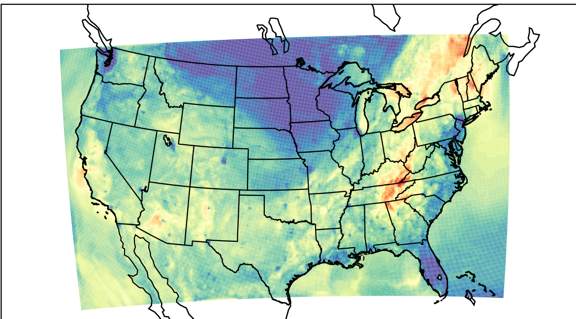
WRF (2023-10-06_01:00:00)
