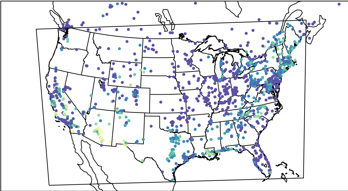
AirNOW (2023-10-07_10:00:00)
