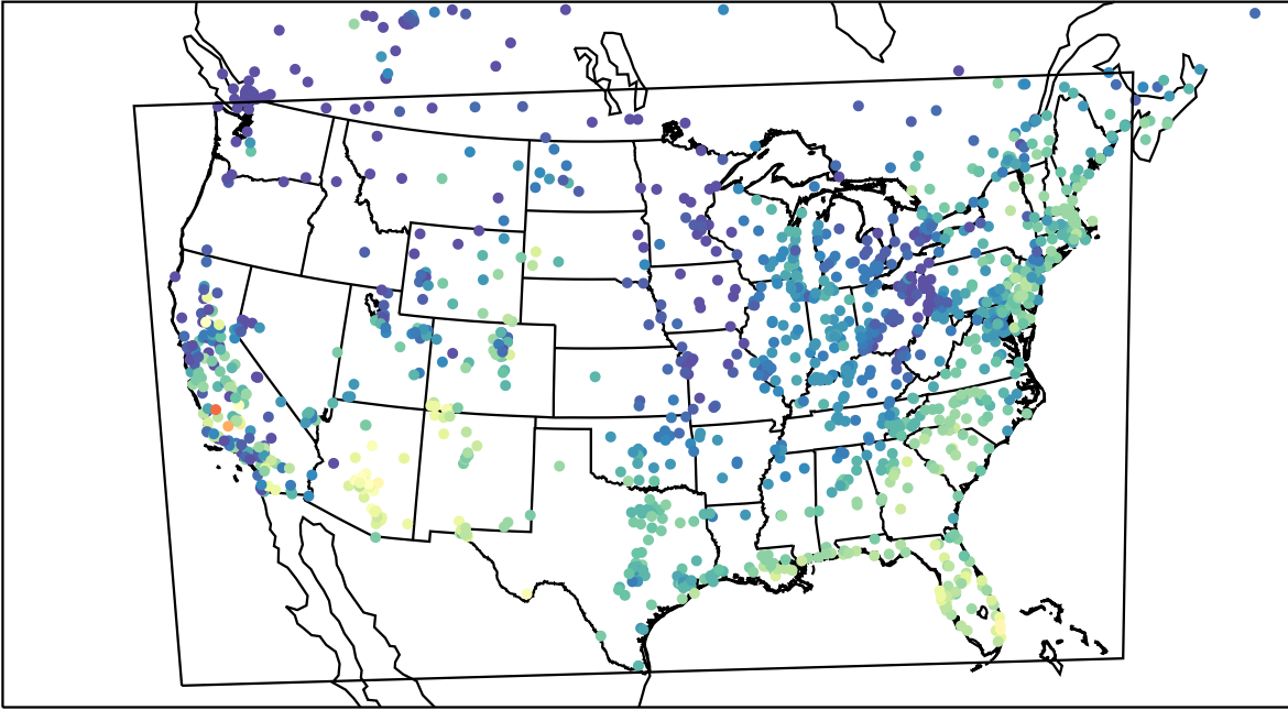
AirNOW (2023-10-07_16:00:00)
