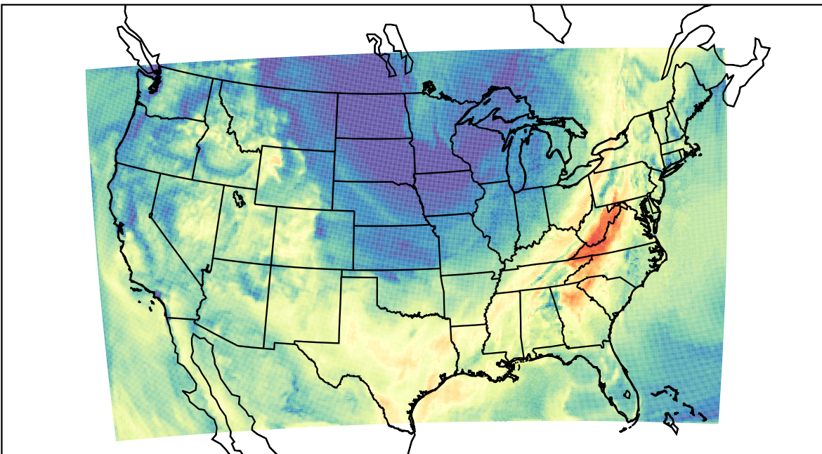
WRF (2023-10-06_17:00:00)
