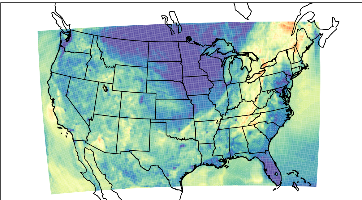
WRF (2023-10-06_04:00:00)
