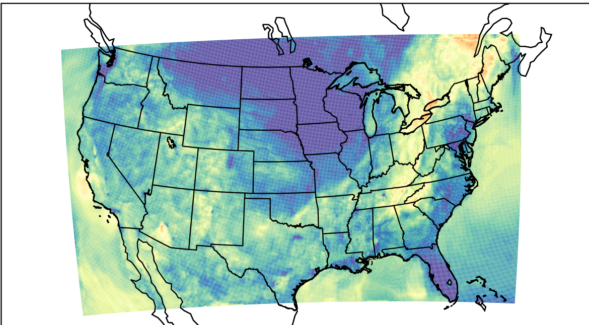
WRF (2023-10-06_05:00:00)
