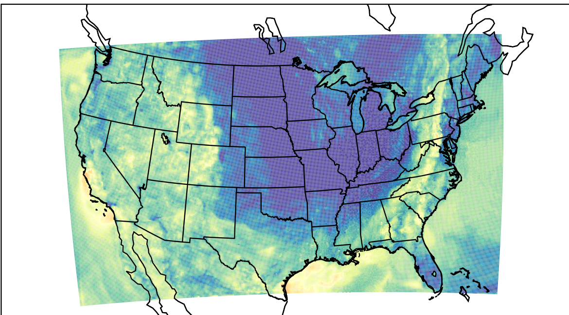
WRF (2023-10-07_05:00:00)
