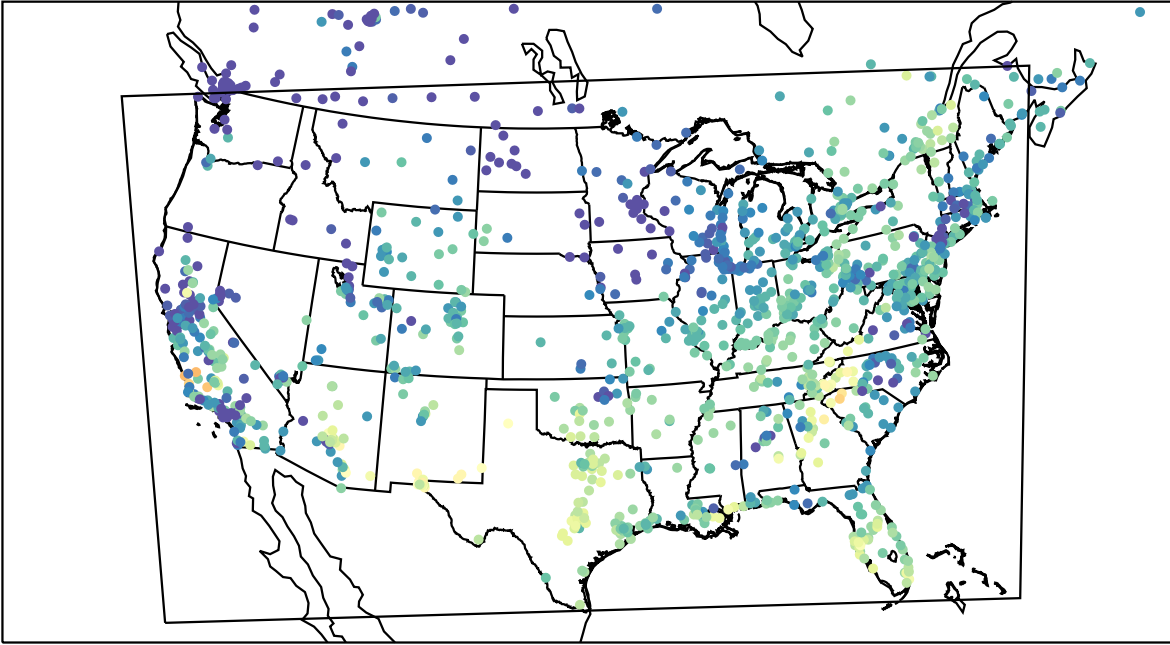
AirNOW (2023-10-06_16:00:00)
