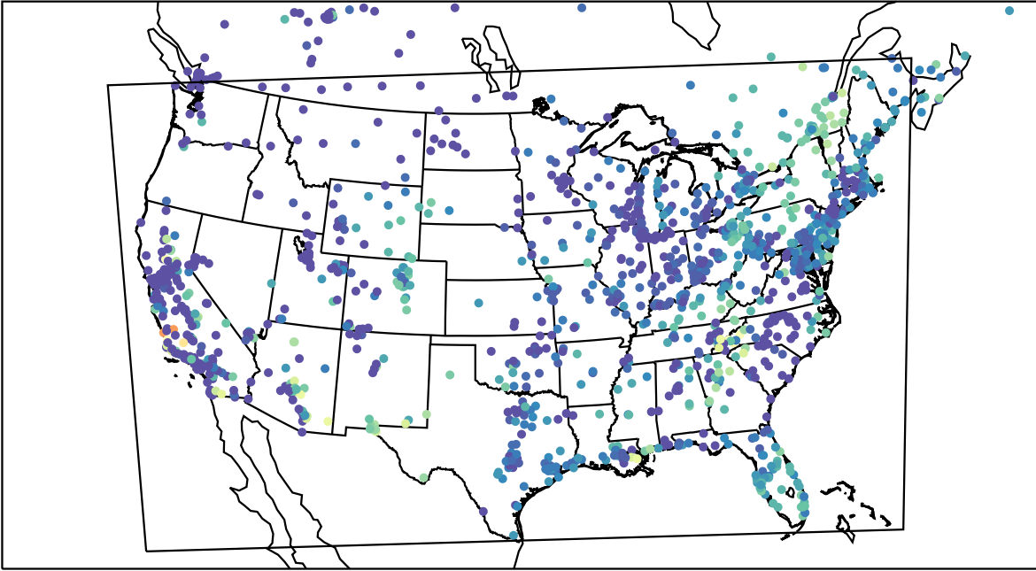
AirNOW (2023-10-06_14:00:00)
