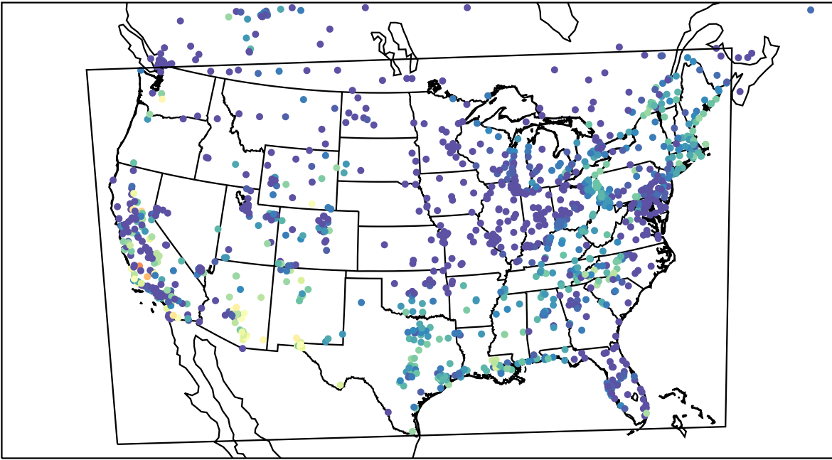
AirNOW (2023-10-07_07:00:00)
