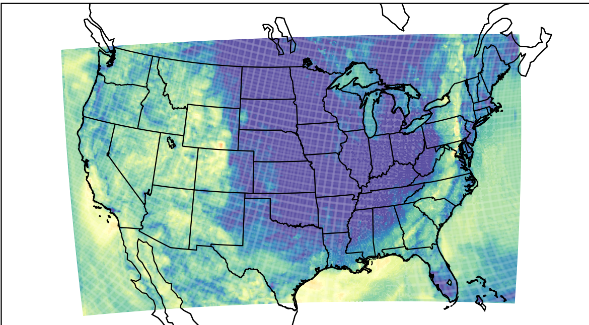
WRF (2023-10-07_08:00:00)
