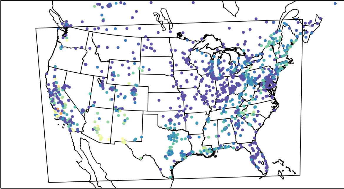
AirNOW (2023-10-07_08:00:00)
