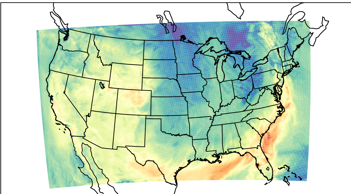
WRF (2023-10-07_19:00:00)
