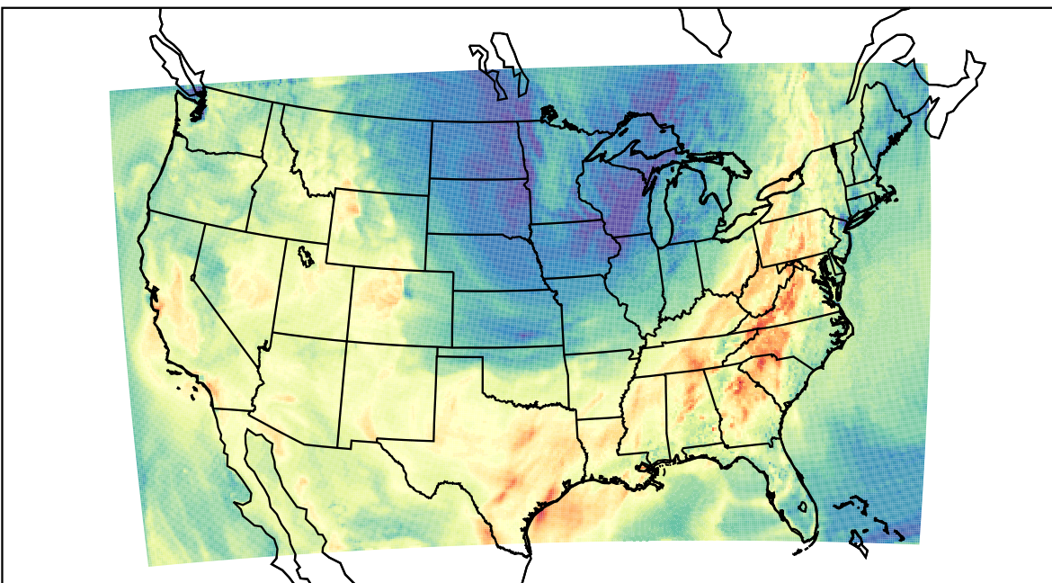
WRF (2023-10-06_21:00:00)
