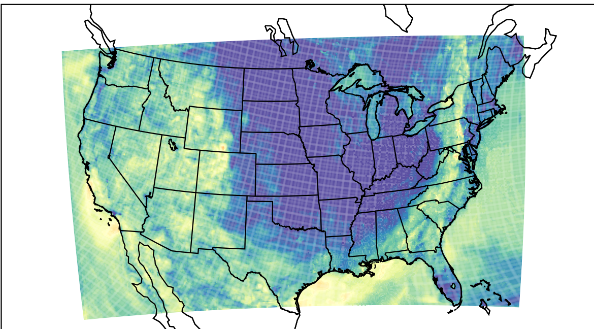
WRF (2023-10-07_07:00:00)
