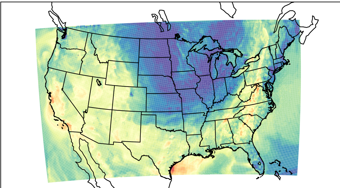
WRF (2023-10-07_00:00:00)
