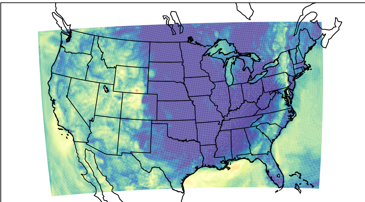
WRF (2023-10-07_11:00:00)
