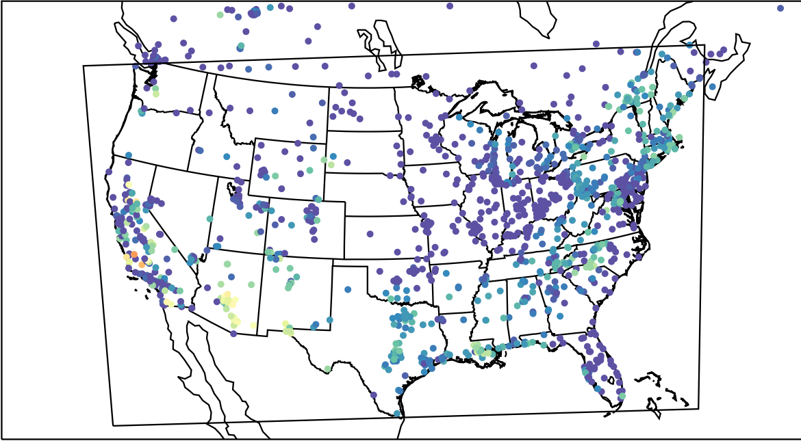
AirNOW (2023-10-07_09:00:00)
