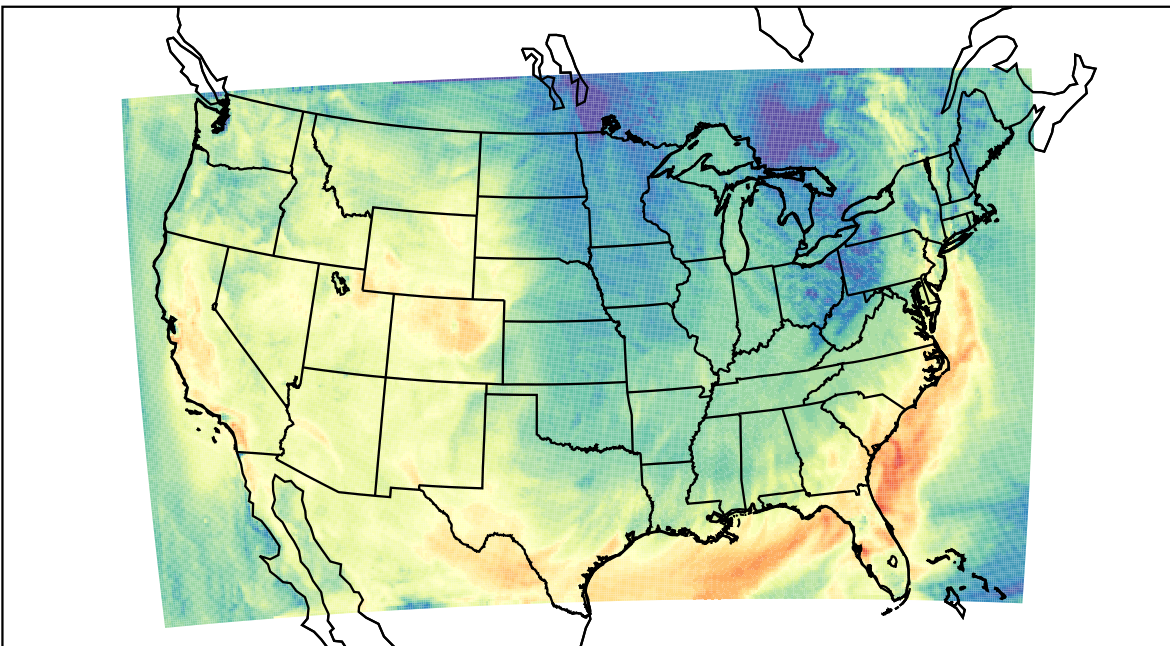
WRF (2023-10-07_20:00:00)
