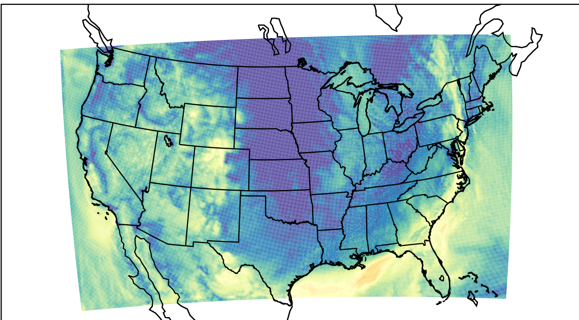
WRF (2023-10-07_15:00:00)
