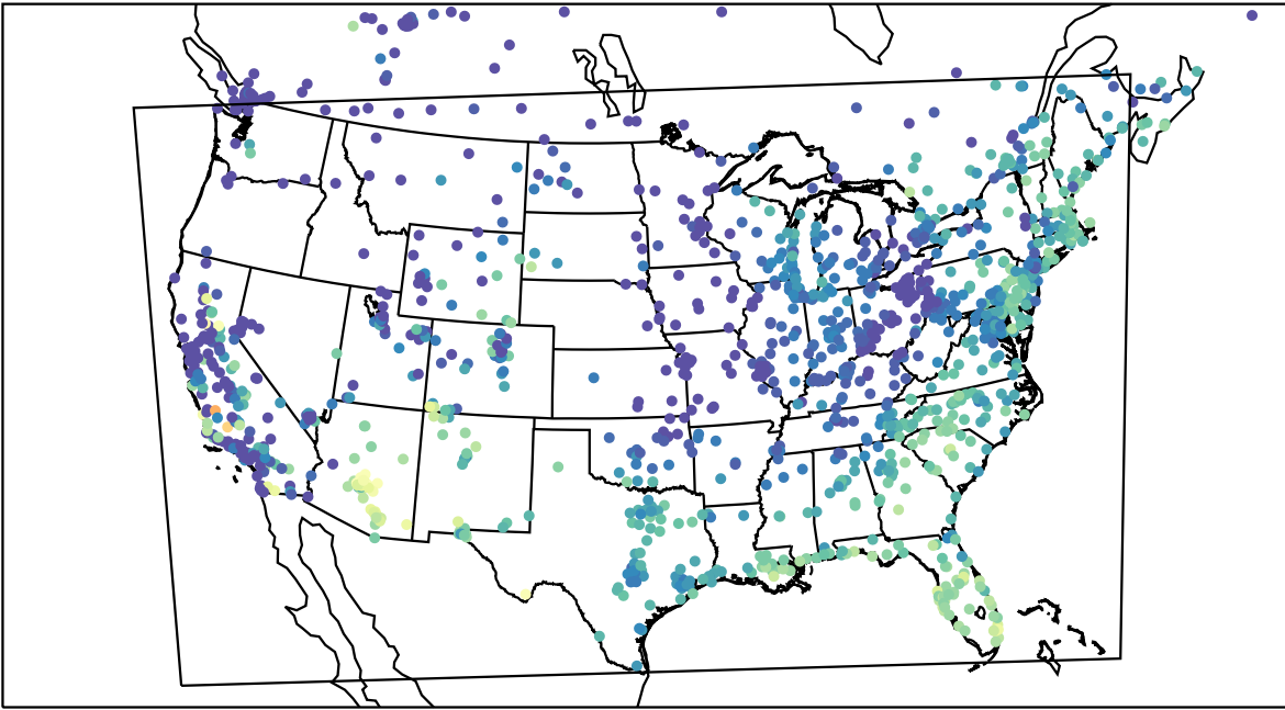
AirNOW (2023-10-07_15:00:00)
