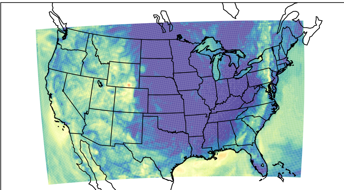
WRF (2023-10-07_10:00:00)
