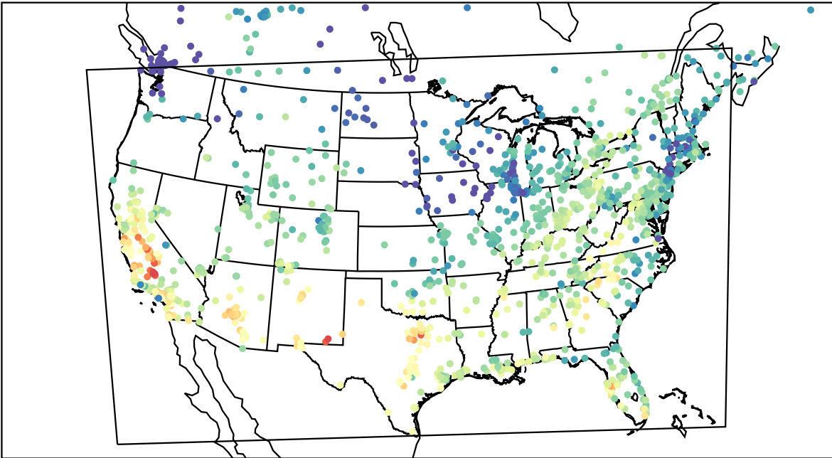
AirNOW (2023-10-06_19:00:00)
