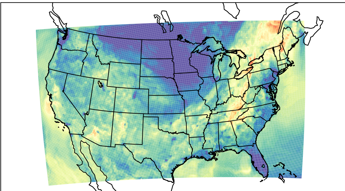
WRF (2023-10-06_03:00:00)
