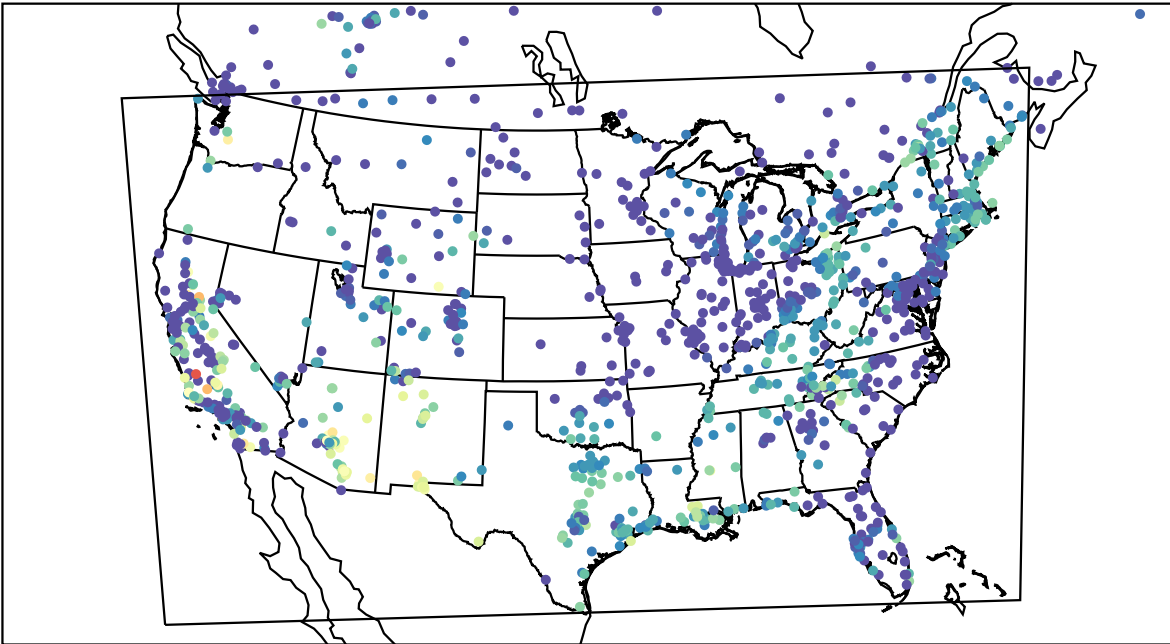
AirNOW (2023-10-07_06:00:00)
