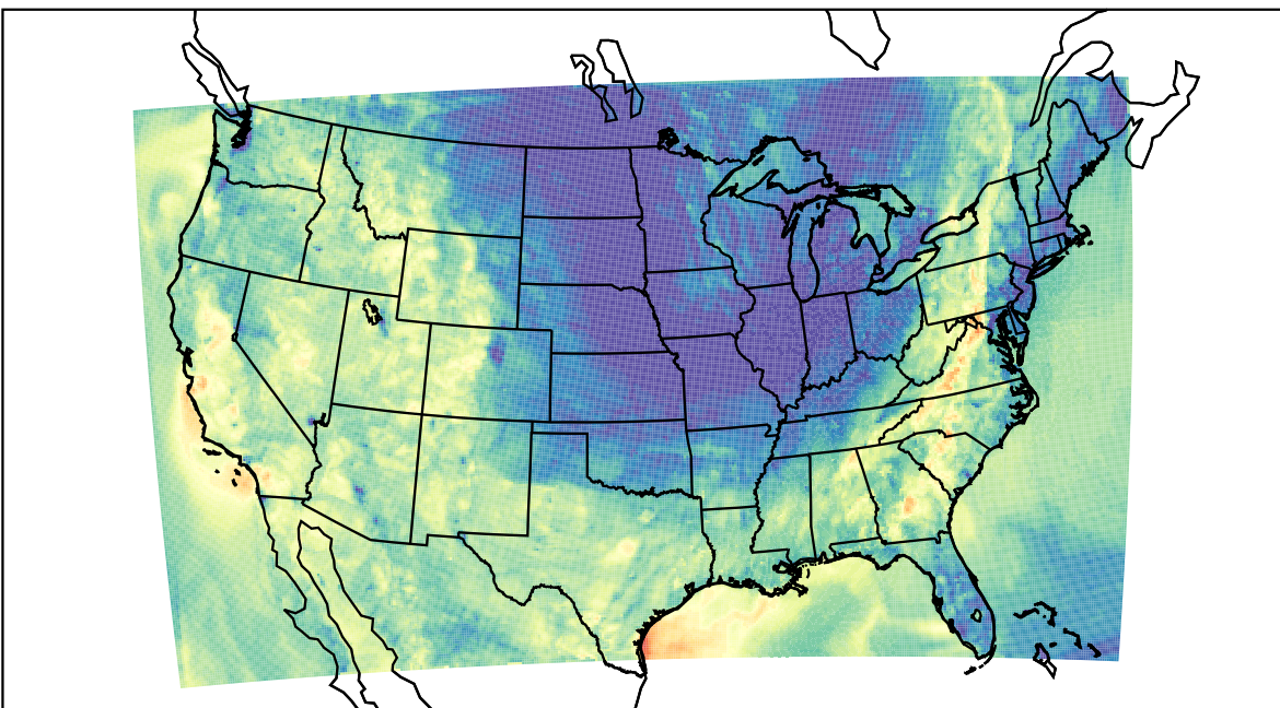
WRF (2023-10-07_02:00:00)
