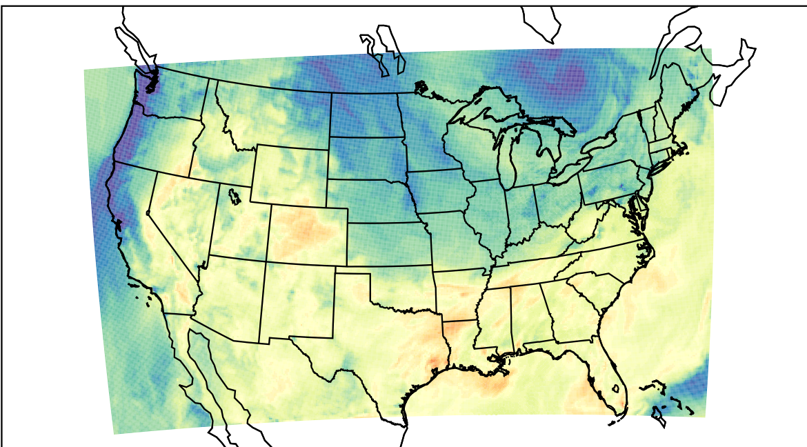
WRF (2023-10-09_18:00:00)
