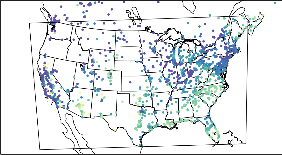
AirNOW (2023-10-08_15:00:00)
