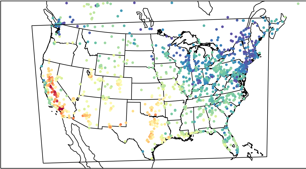
AirNOW (2023-10-08_22:00:00)
