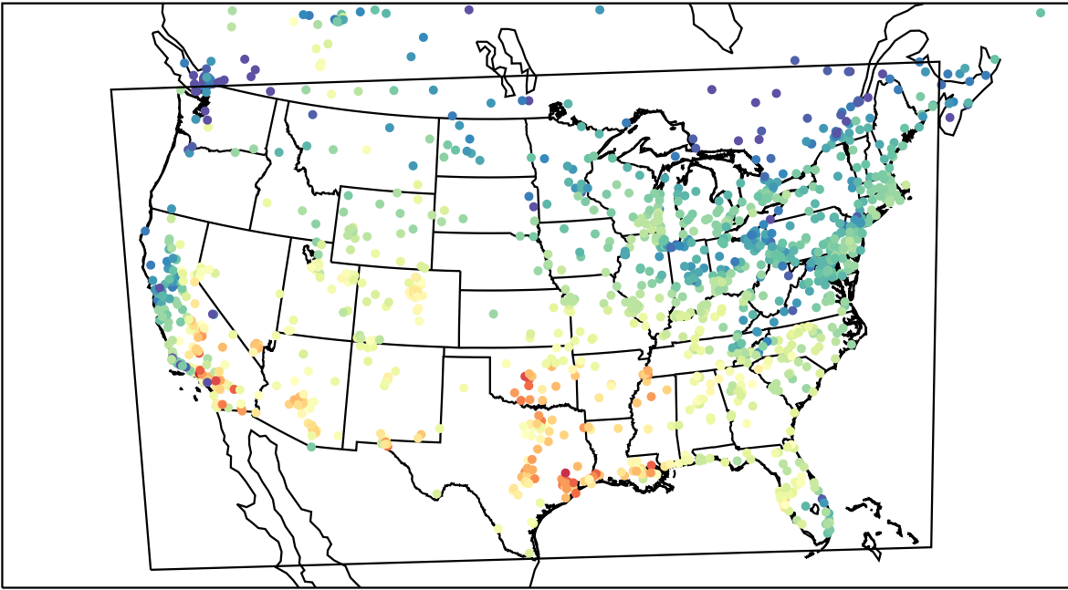
AirNOW (2023-10-09_20:00:00)
