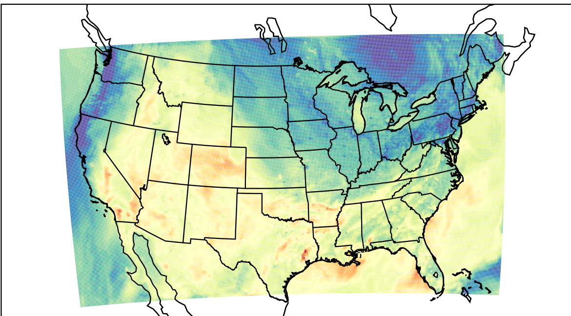
WRF (2023-10-09_23:00:00)
