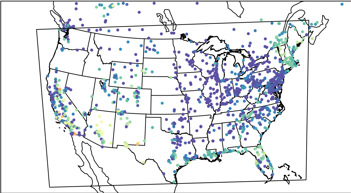
AirNOW (2023-10-08_05:00:00)
