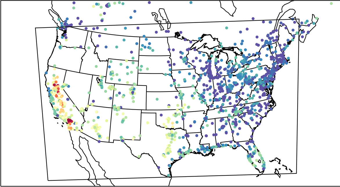
AirNOW (2023-10-09_01:00:00)
