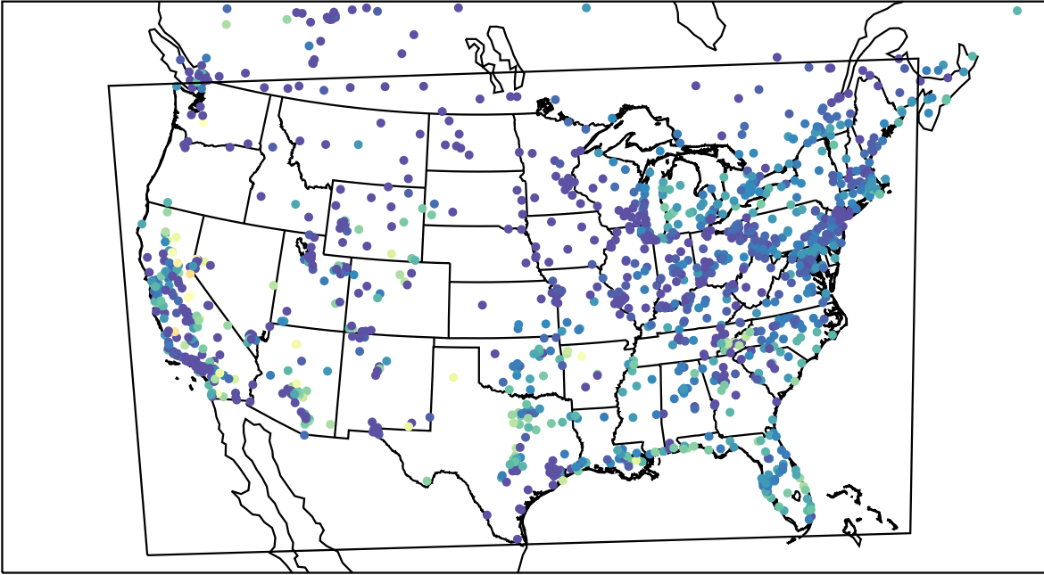
AirNOW (2023-10-09_14:00:00)
