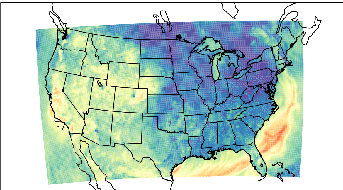
WRF (2023-10-08_02:00:00)
