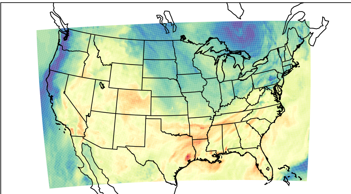
WRF (2023-10-09_20:00:00)
