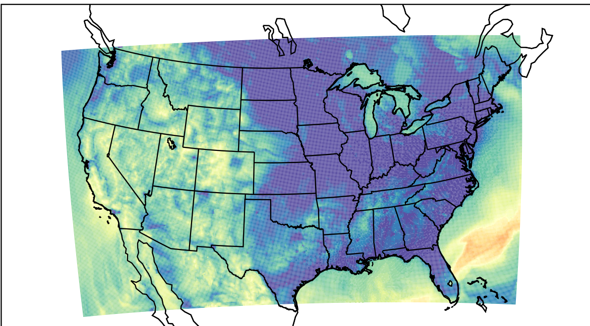
WRF (2023-10-08_12:00:00)
