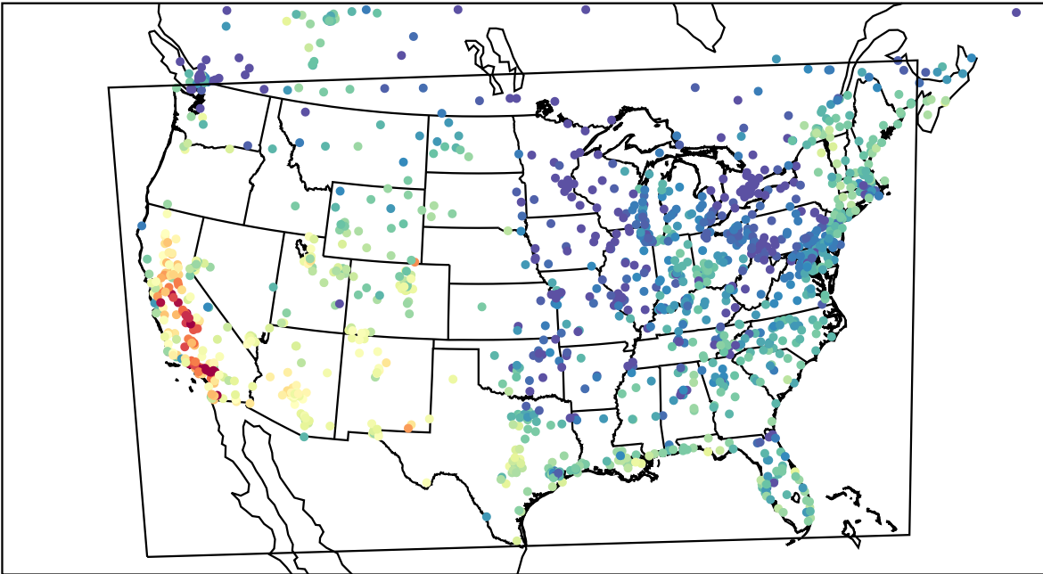
AirNOW (2023-10-08_00:00:00)
