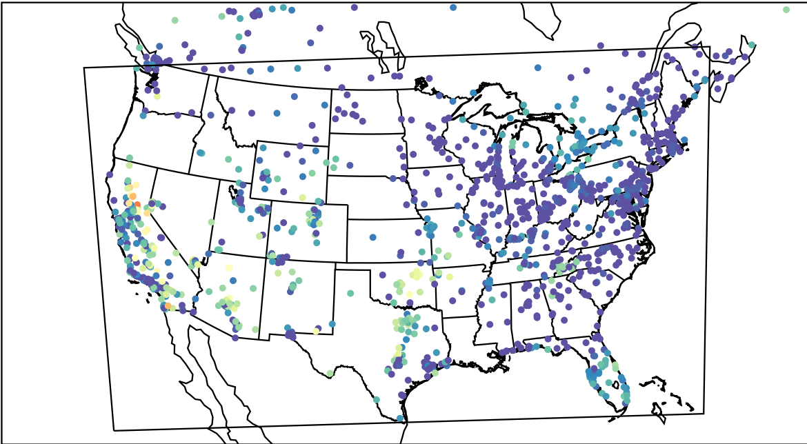
AirNOW (2023-10-09_07:00:00)
