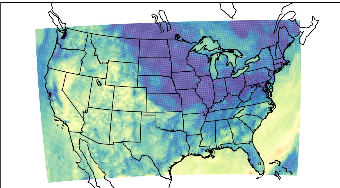
WRF (2023-10-09_08:00:00)
