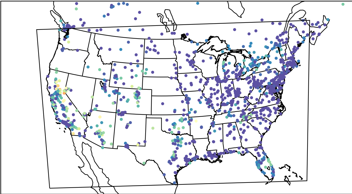
AirNOW (2023-10-09_10:00:00)
