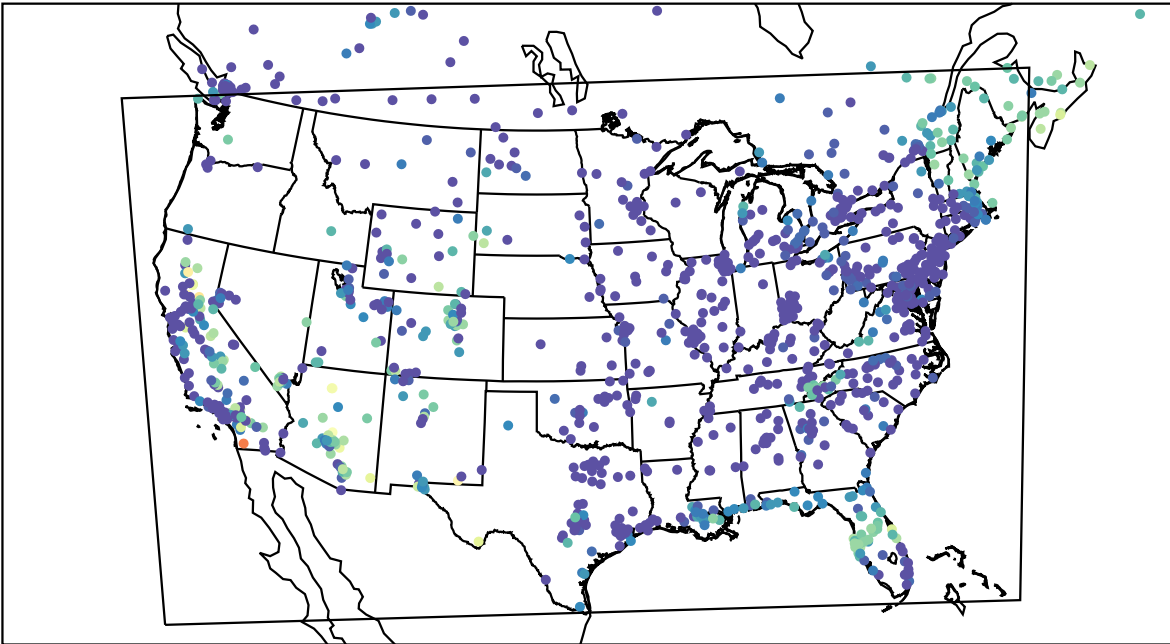
AirNOW (2023-10-08_10:00:00)
