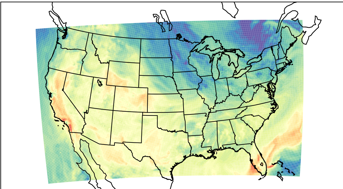
WRF (2023-10-08_20:00:00)
