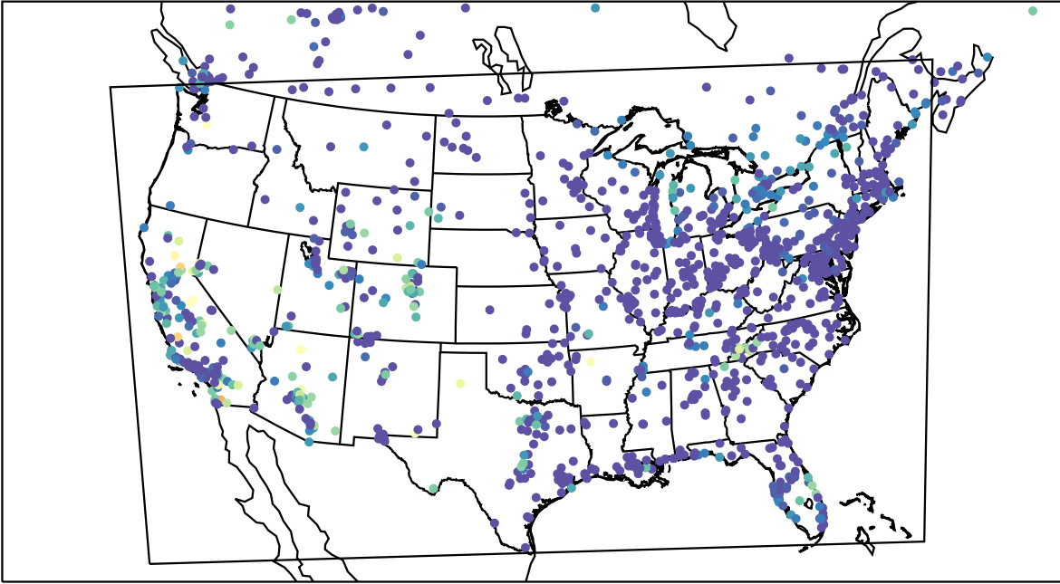
AirNOW (2023-10-09_12:00:00)
