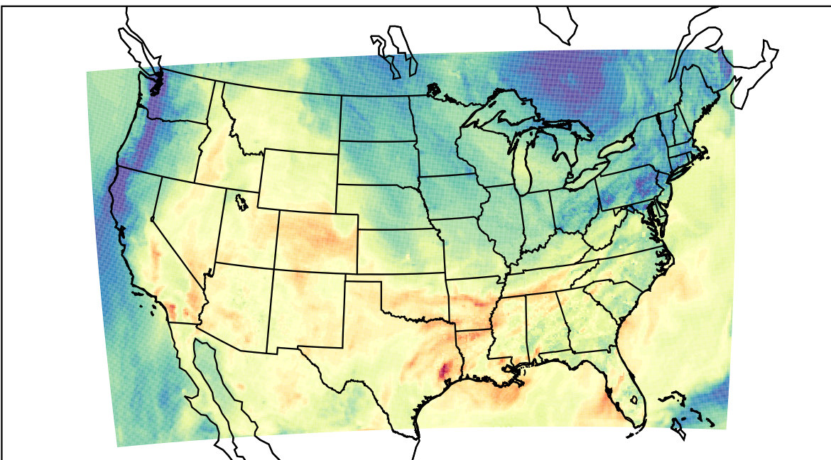
WRF (2023-10-09_22:00:00)
