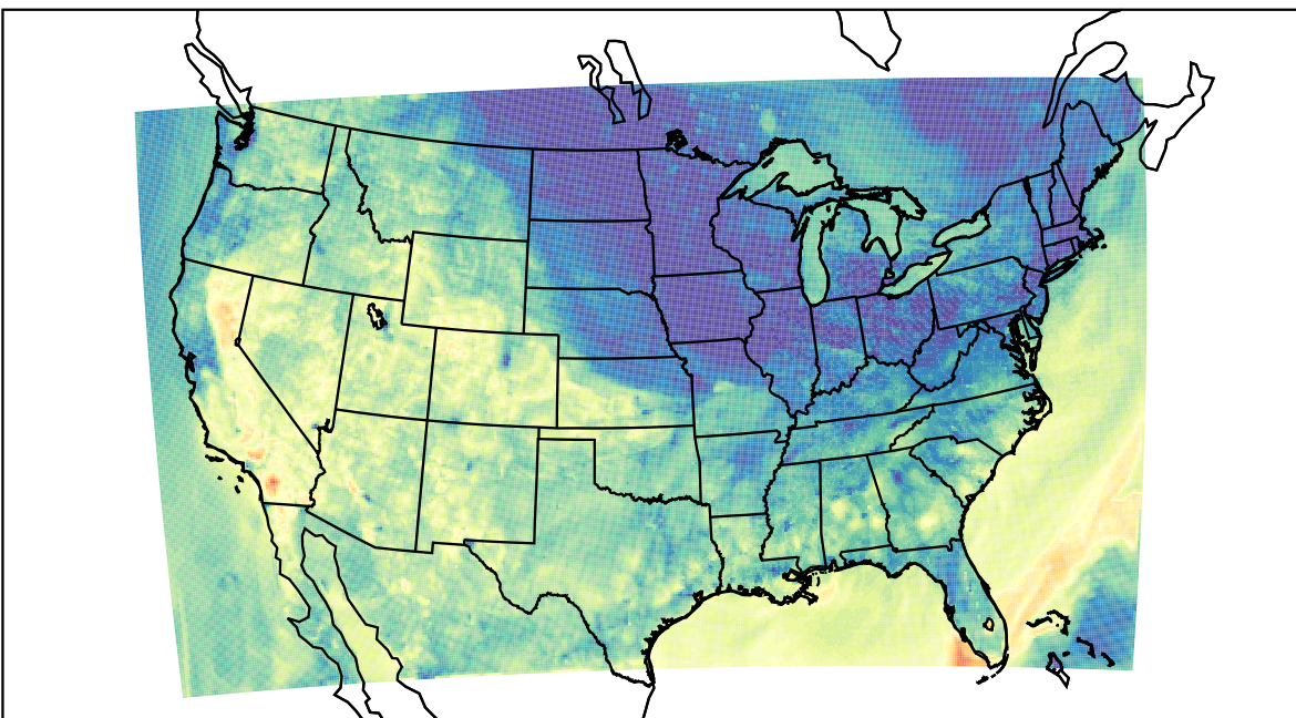
WRF (2023-10-09_03:00:00)
