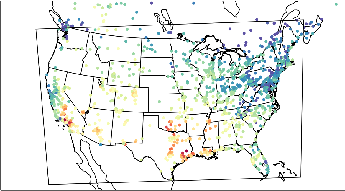
AirNOW (2023-10-09_22:00:00)
