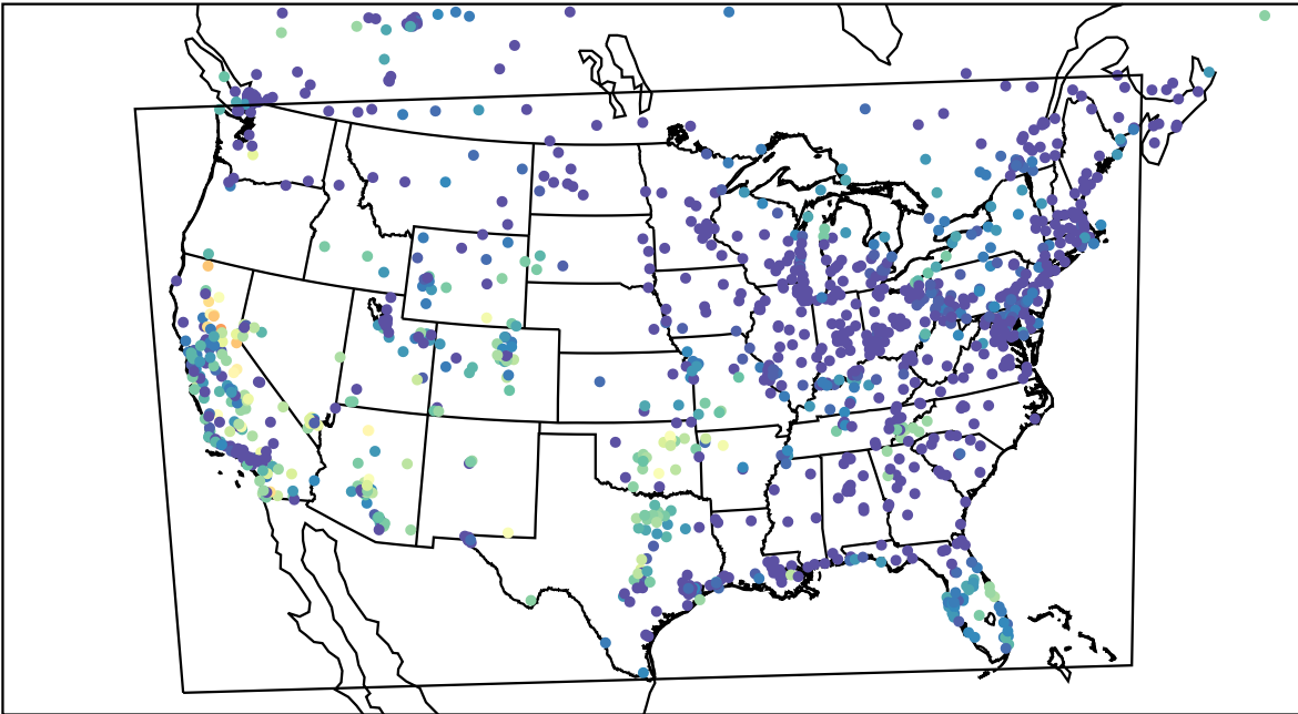
AirNOW (2023-10-09_08:00:00)
