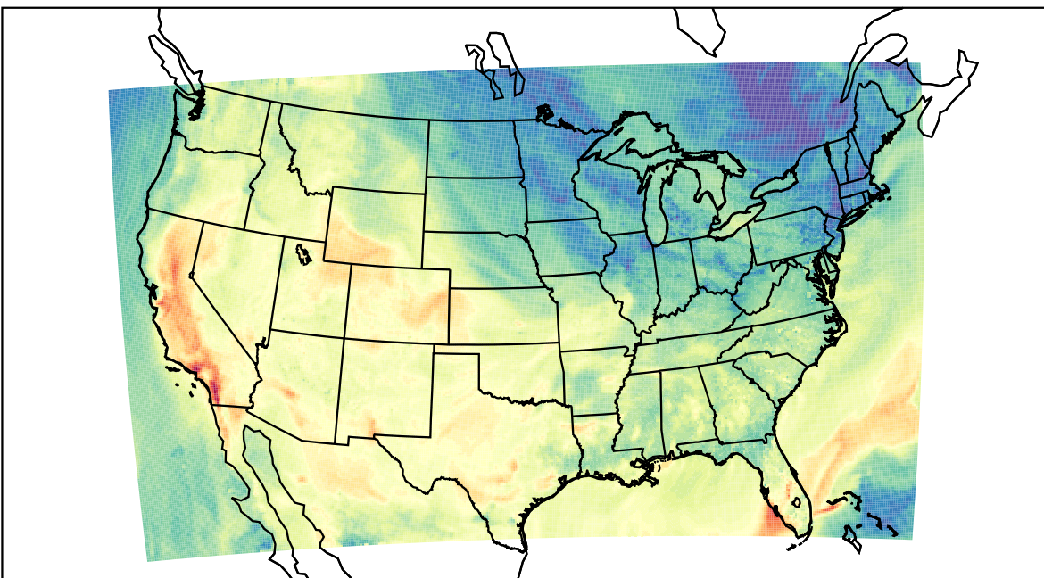
WRF (2023-10-08_22:00:00)
