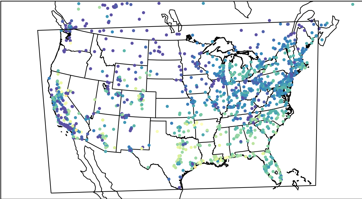
AirNOW (2023-10-09_15:00:00)
