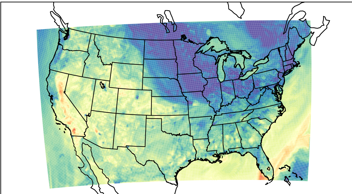
WRF (2023-10-09_02:00:00)
