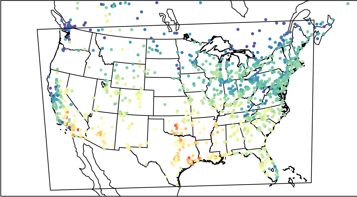
AirNOW (2023-10-09_19:00:00)
