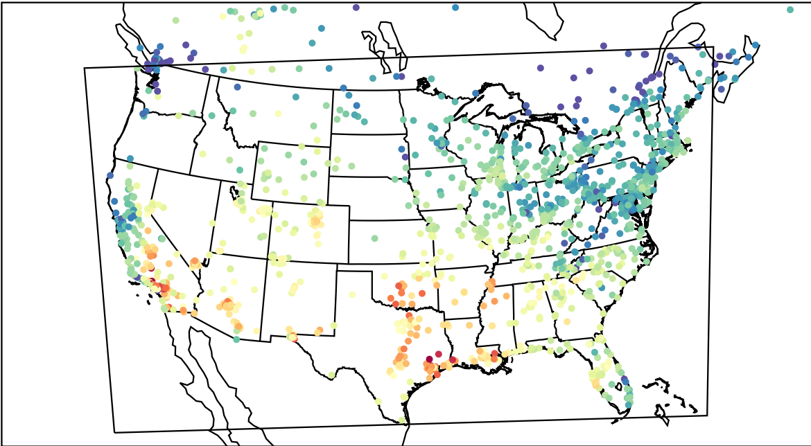
AirNOW (2023-10-09_21:00:00)
