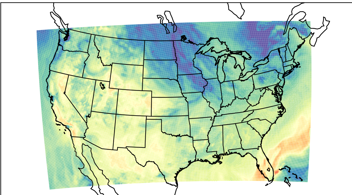
WRF (2023-10-08_18:00:00)
