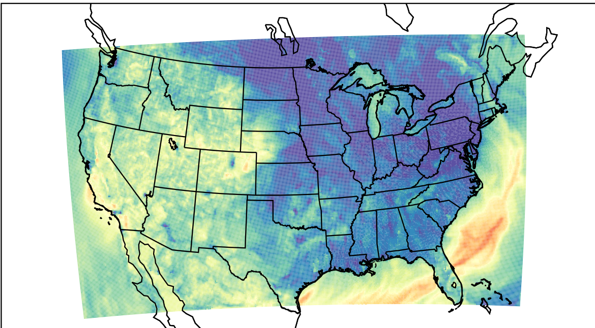
WRF (2023-10-08_04:00:00)
