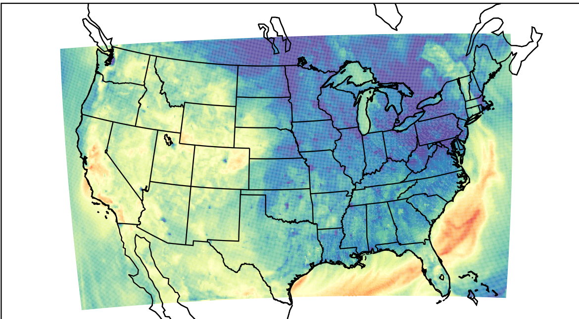
WRF (2023-10-08_01:00:00)
