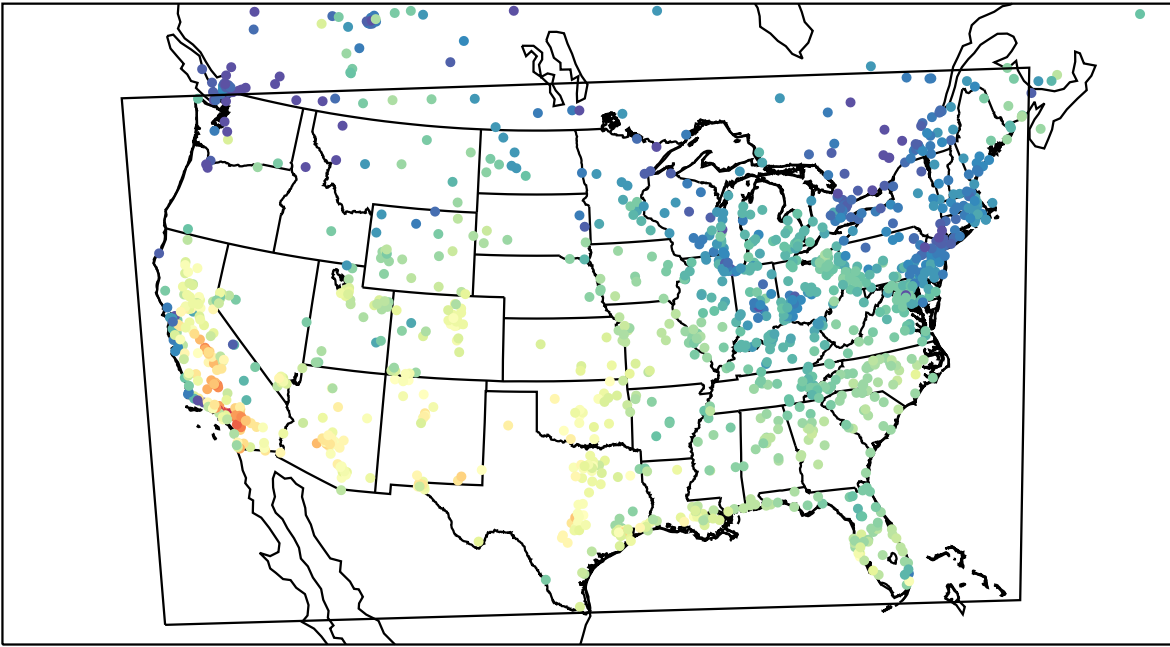
AirNOW (2023-10-08_18:00:00)
