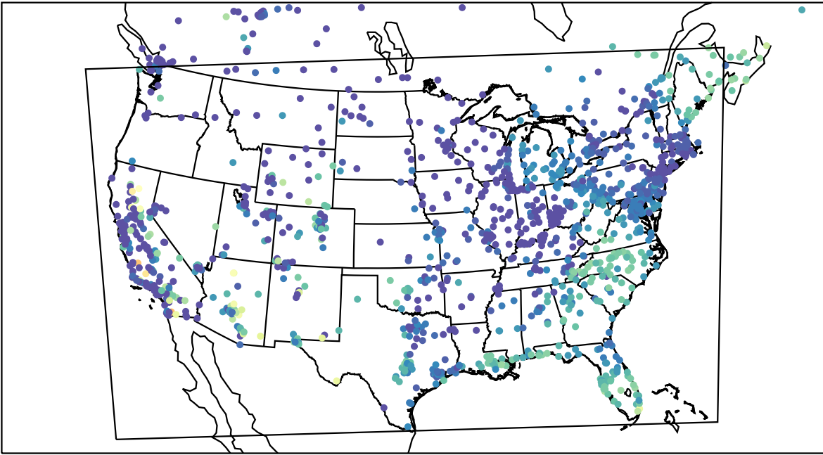
AirNOW (2023-10-08_14:00:00)
