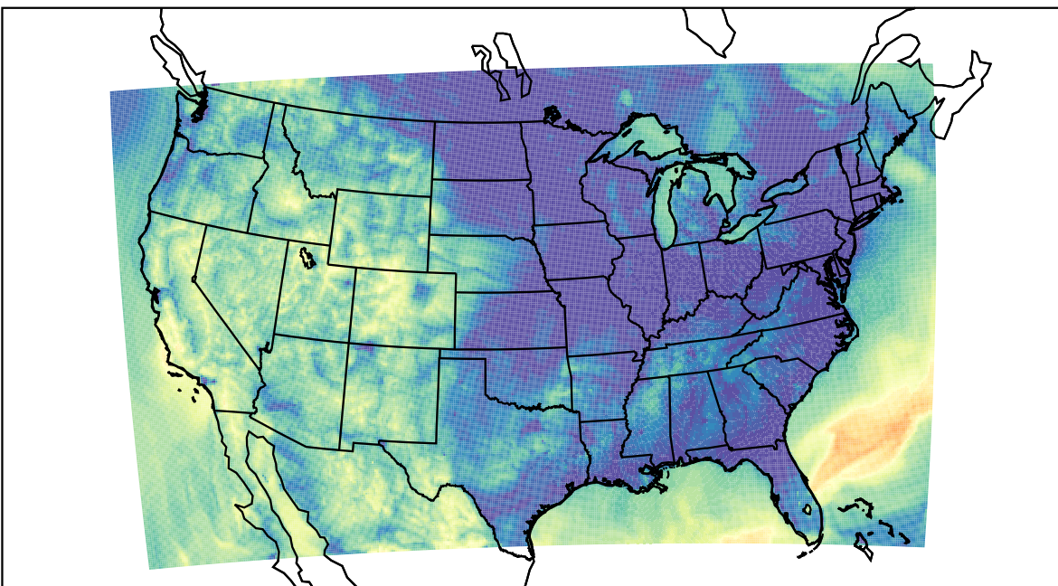
WRF (2023-10-08_11:00:00)
