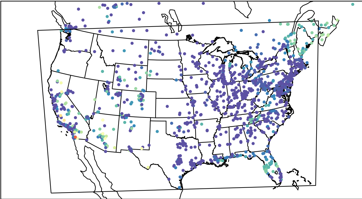
AirNOW (2023-10-08_12:00:00)
