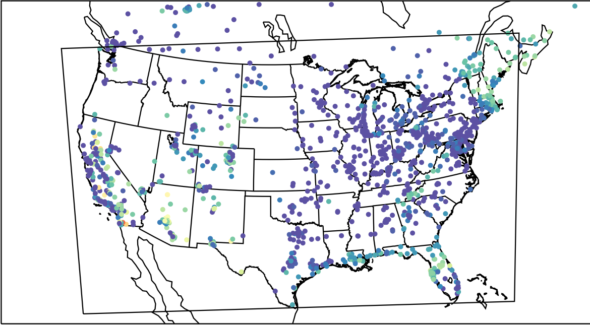
AirNOW (2023-10-08_08:00:00)
