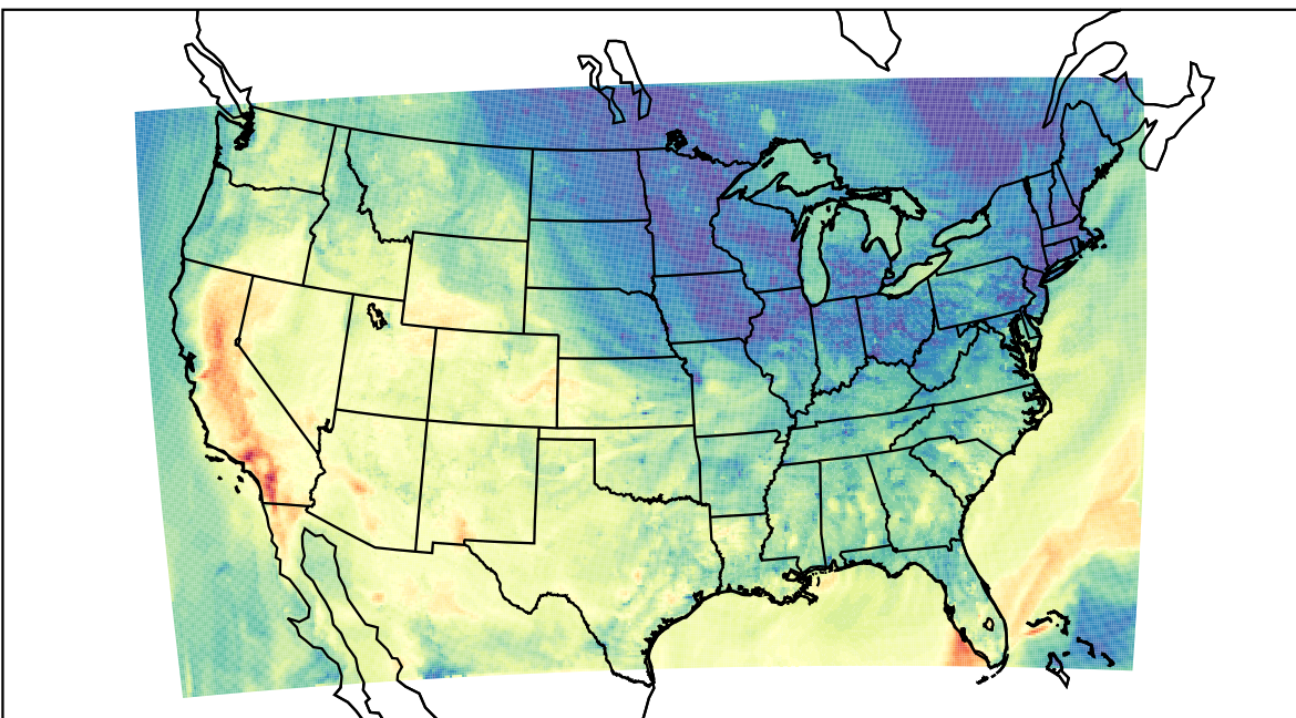
WRF (2023-10-09_00:00:00)
