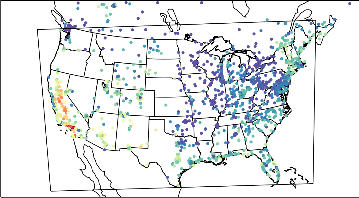
AirNOW (2023-10-08_01:00:00)
