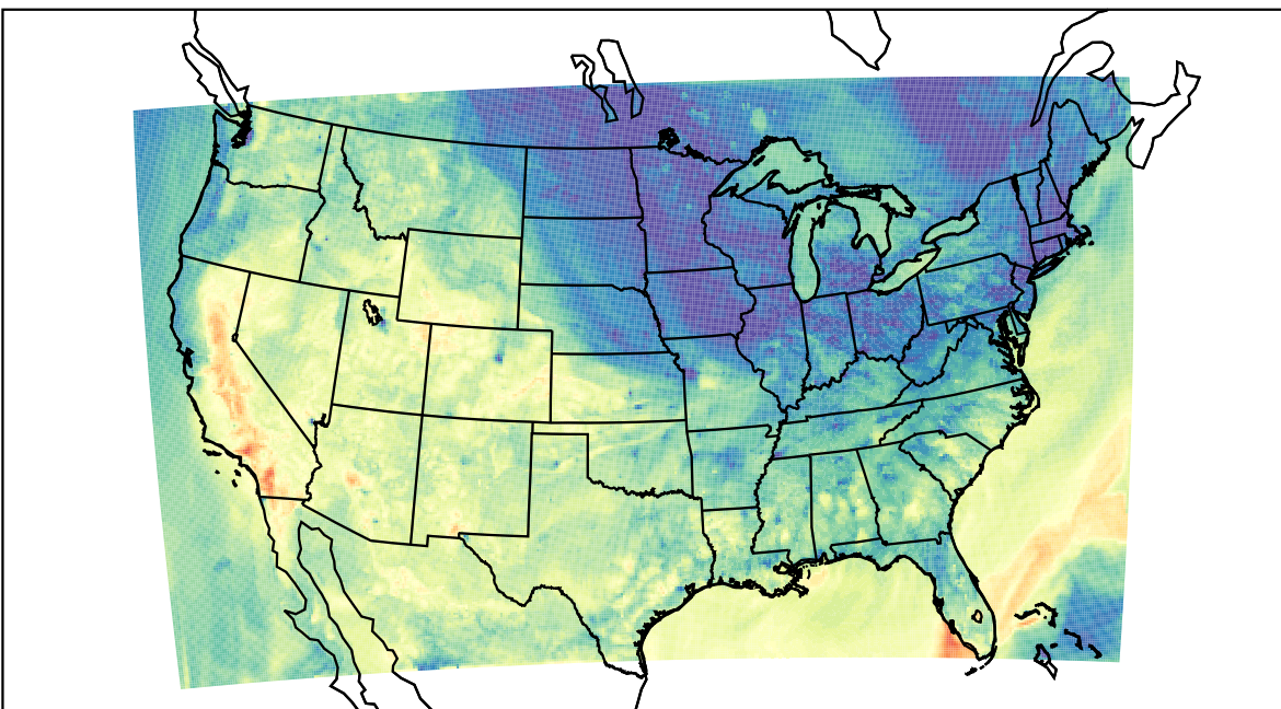
WRF (2023-10-09_01:00:00)
