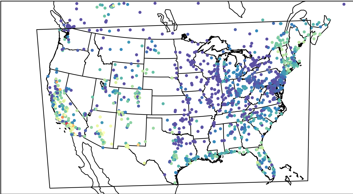
AirNOW (2023-10-08_03:00:00)
