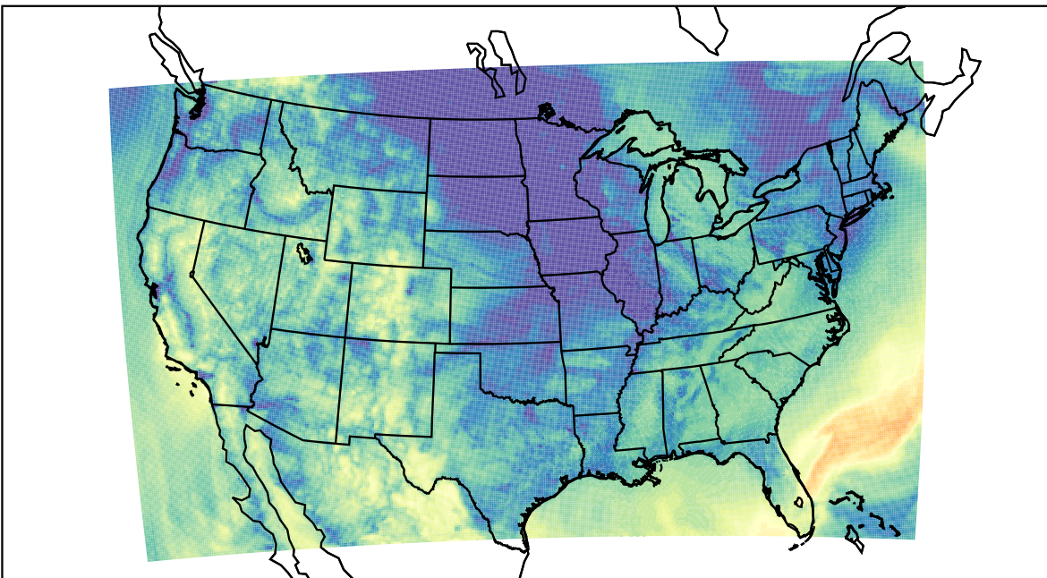
WRF (2023-10-08_15:00:00)
