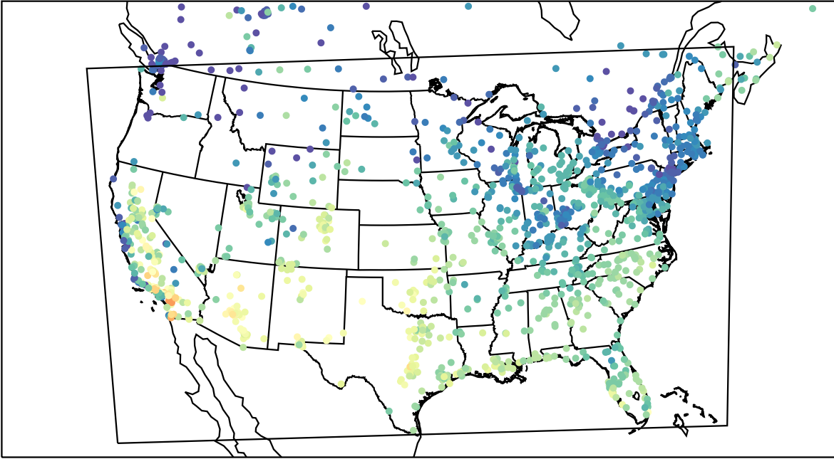
AirNOW (2023-10-08_17:00:00)
