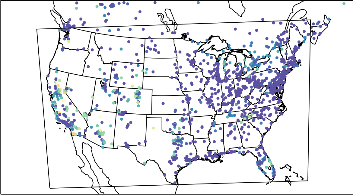
AirNOW (2023-10-09_11:00:00)
