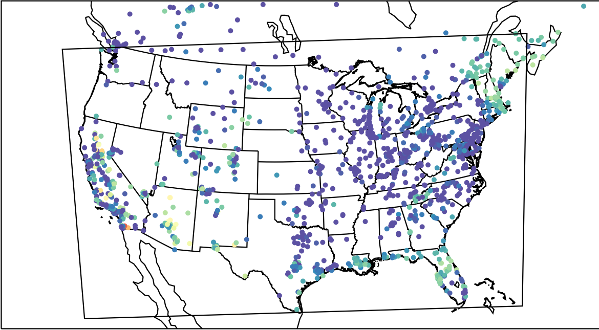
AirNOW (2023-10-08_07:00:00)
