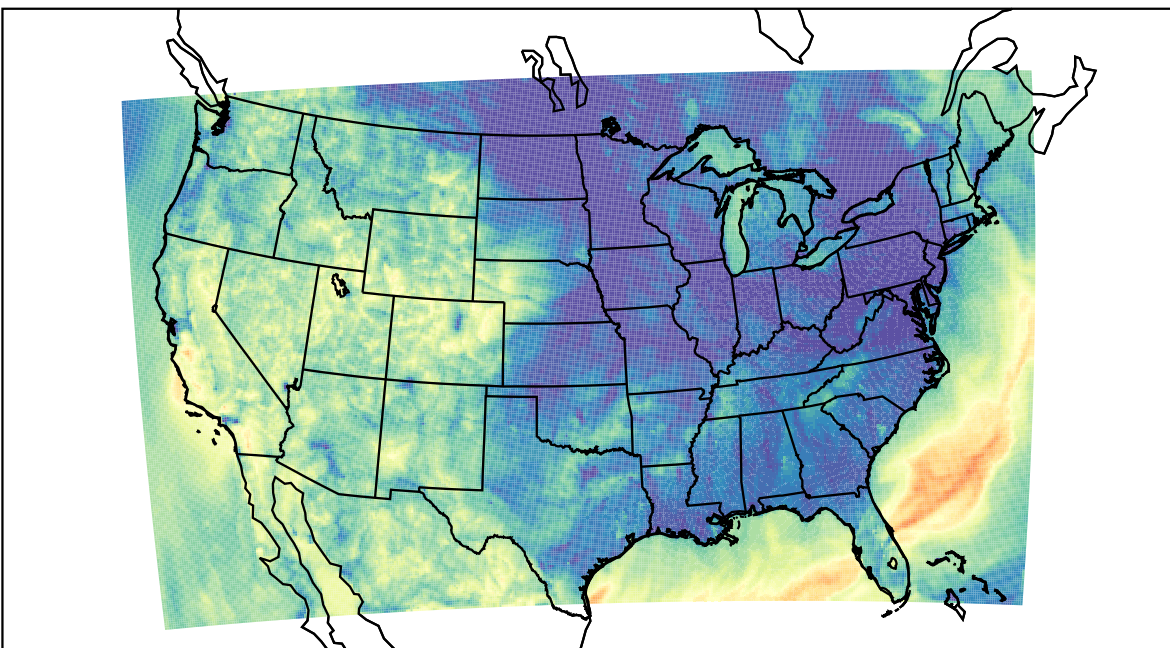
WRF (2023-10-08_06:00:00)
