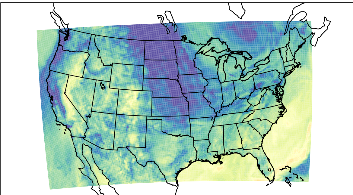
WRF (2023-10-09_15:00:00)
