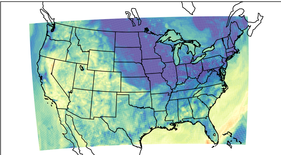
WRF (2023-10-09_06:00:00)
