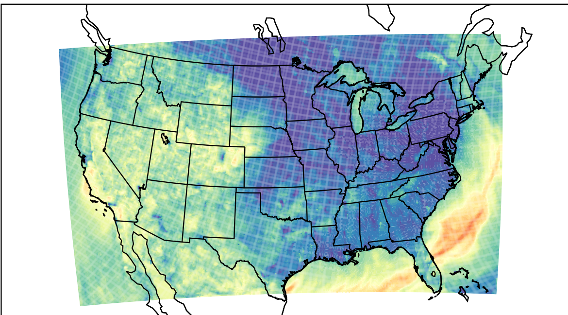
WRF (2023-10-08_05:00:00)
