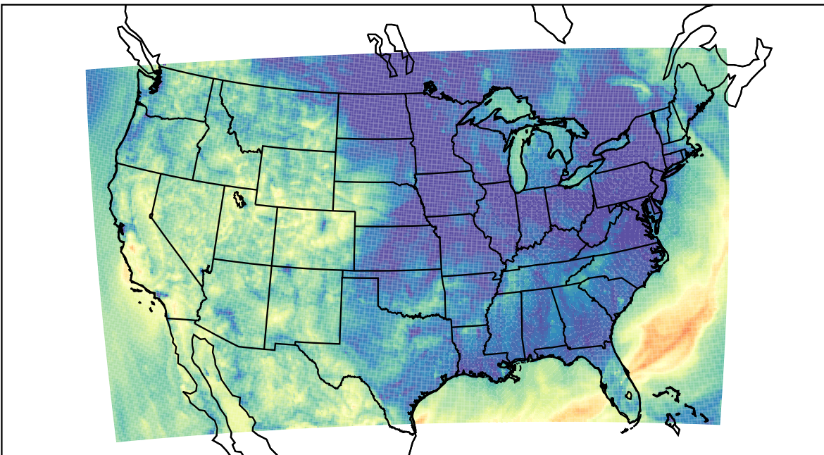
WRF (2023-10-08_07:00:00)
