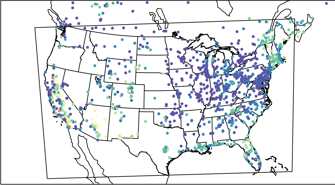
AirNOW (2023-10-08_04:00:00)
