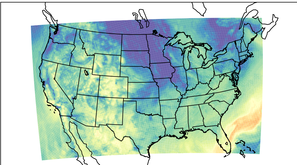
WRF (2023-10-08_16:00:00)
