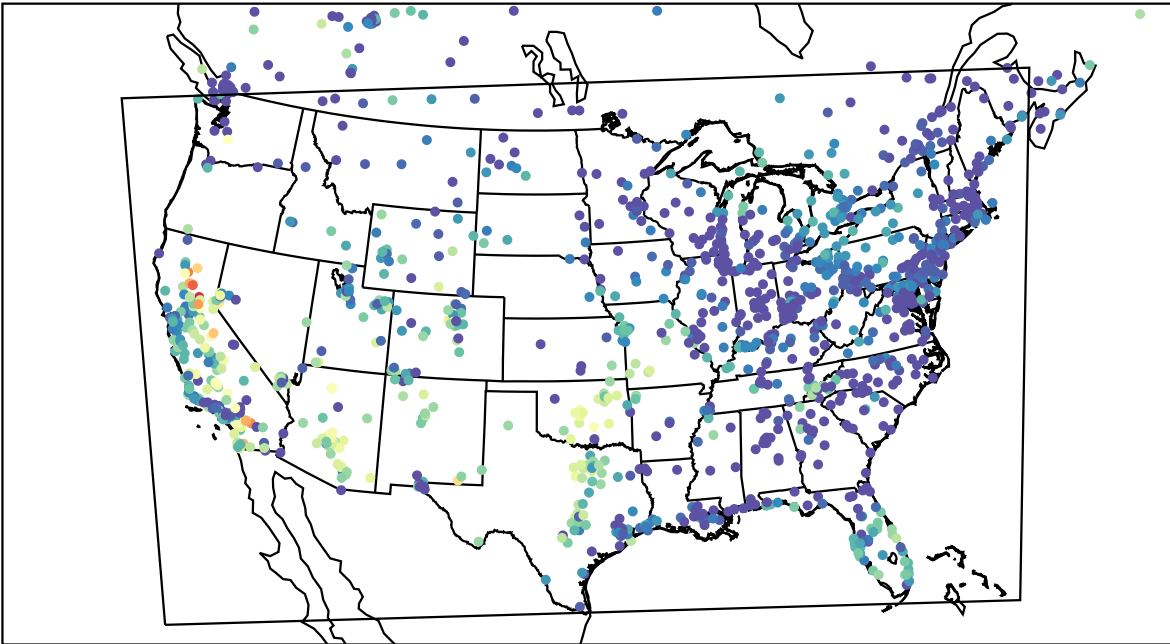
AirNOW (2023-10-09_04:00:00)
