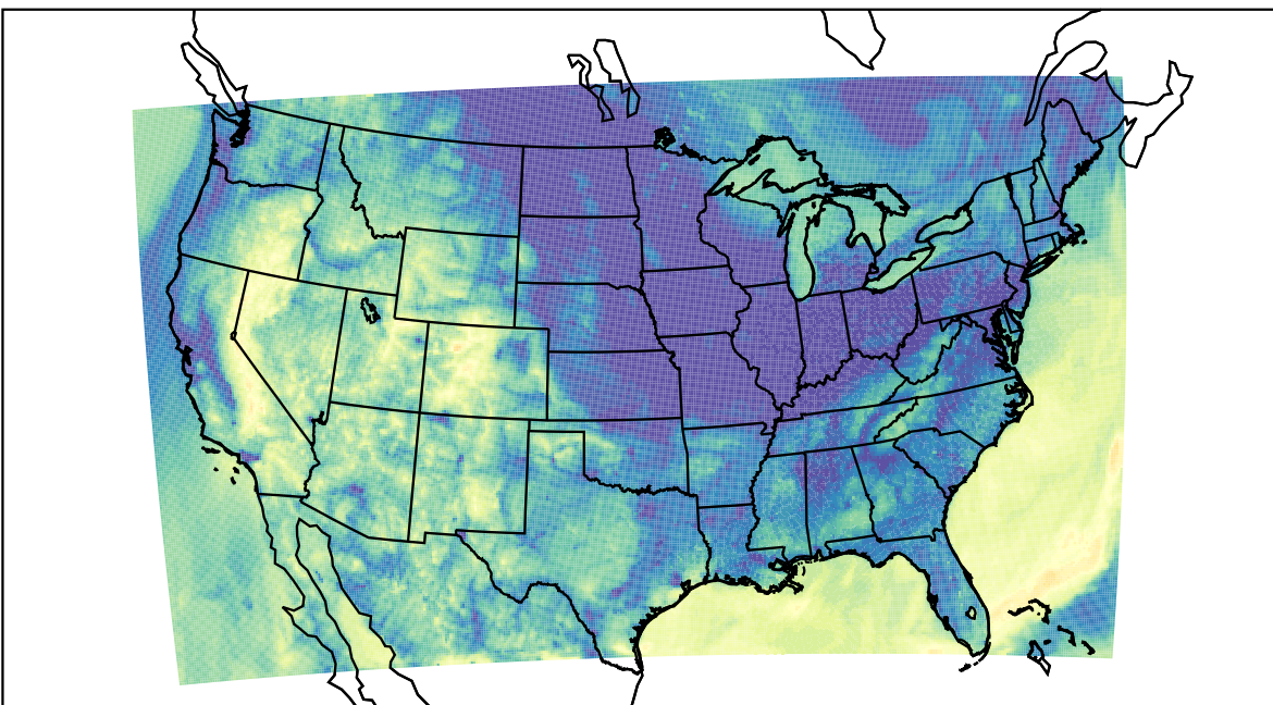
WRF (2023-10-09_13:00:00)
