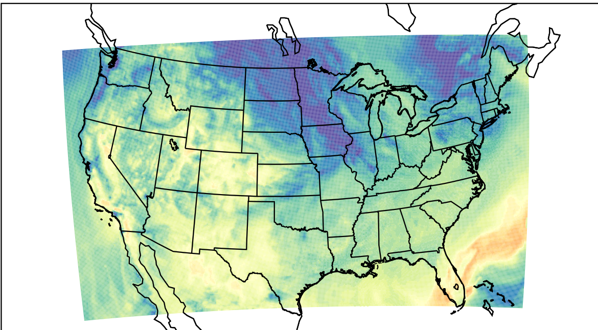
WRF (2023-10-08_17:00:00)
