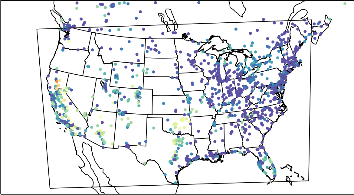
AirNOW (2023-10-09_06:00:00)
