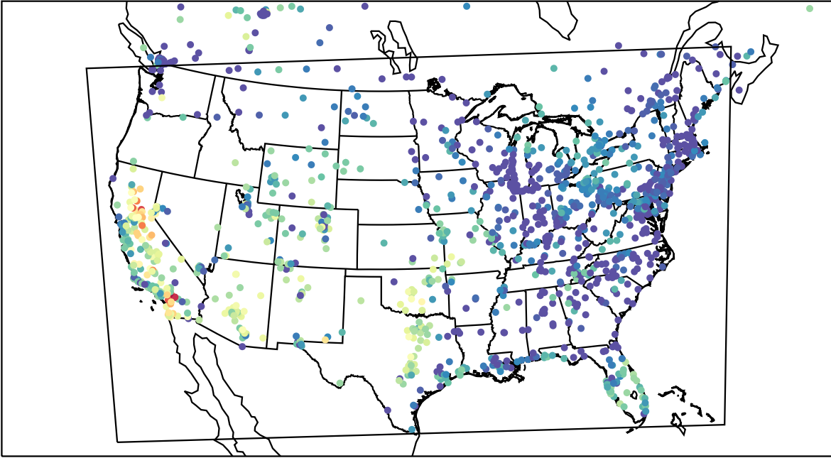
AirNOW (2023-10-09_02:00:00)
