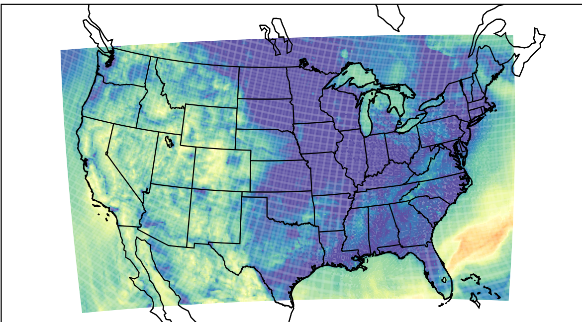
WRF (2023-10-08_13:00:00)
