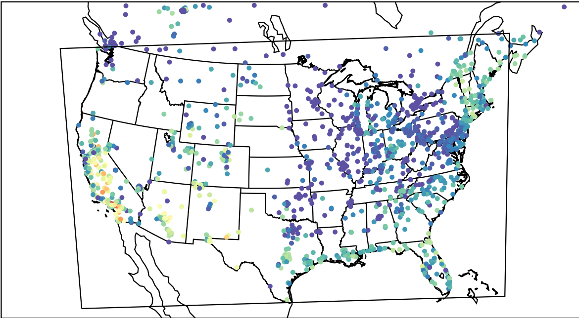
AirNOW (2023-10-08_02:00:00)
