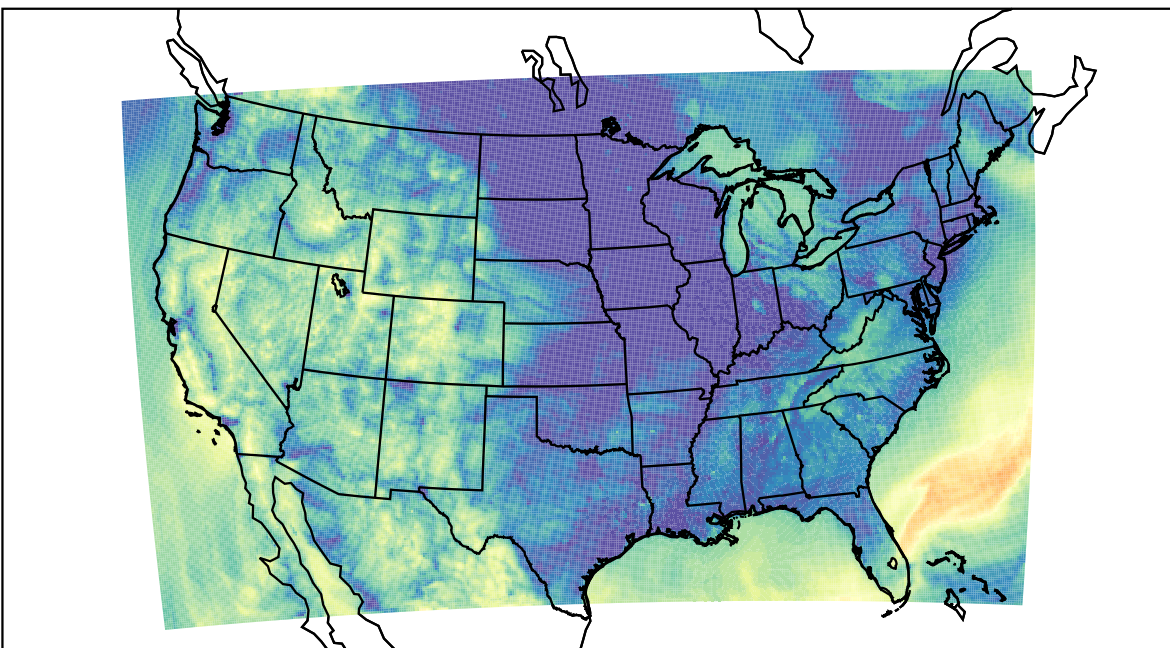
WRF (2023-10-08_14:00:00)
