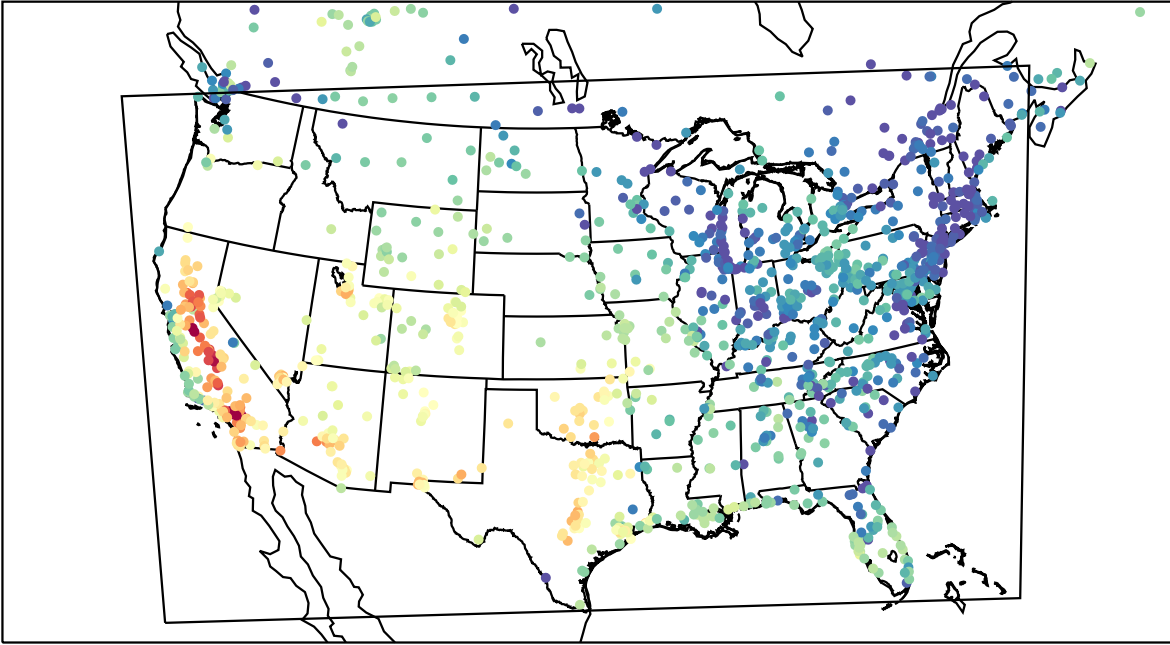
AirNOW (2023-10-08_23:00:00)
