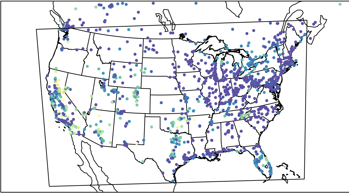
AirNOW (2023-10-09_09:00:00)
