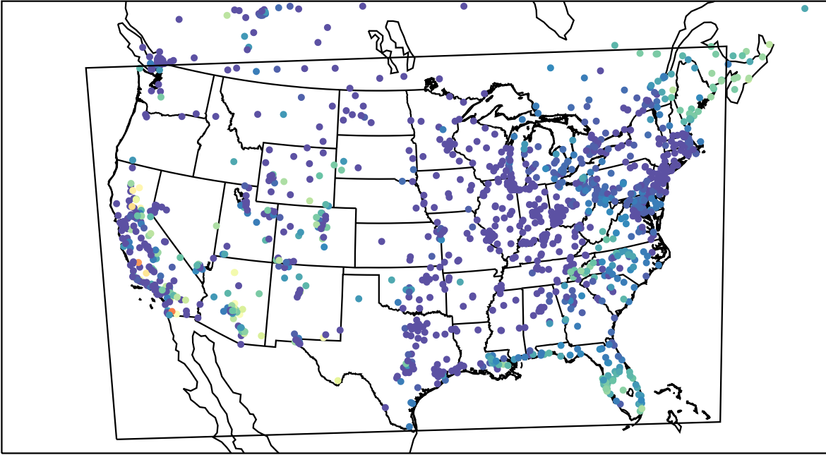
AirNOW (2023-10-08_13:00:00)
