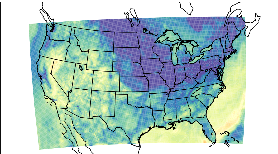
WRF (2023-10-09_09:00:00)
