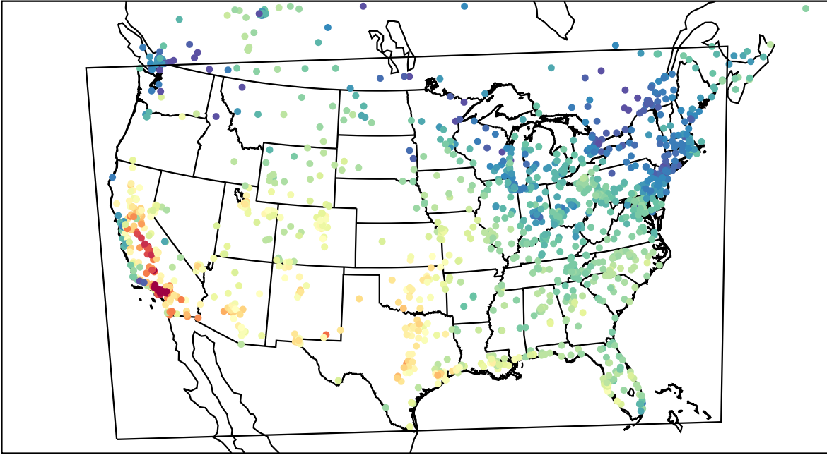
AirNOW (2023-10-08_20:00:00)
