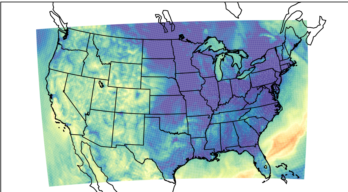
WRF (2023-10-08_09:00:00)
