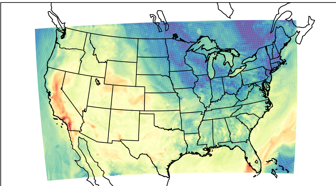
WRF (2023-10-08_23:00:00)
