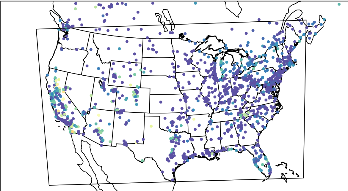
AirNOW (2023-10-09_13:00:00)
