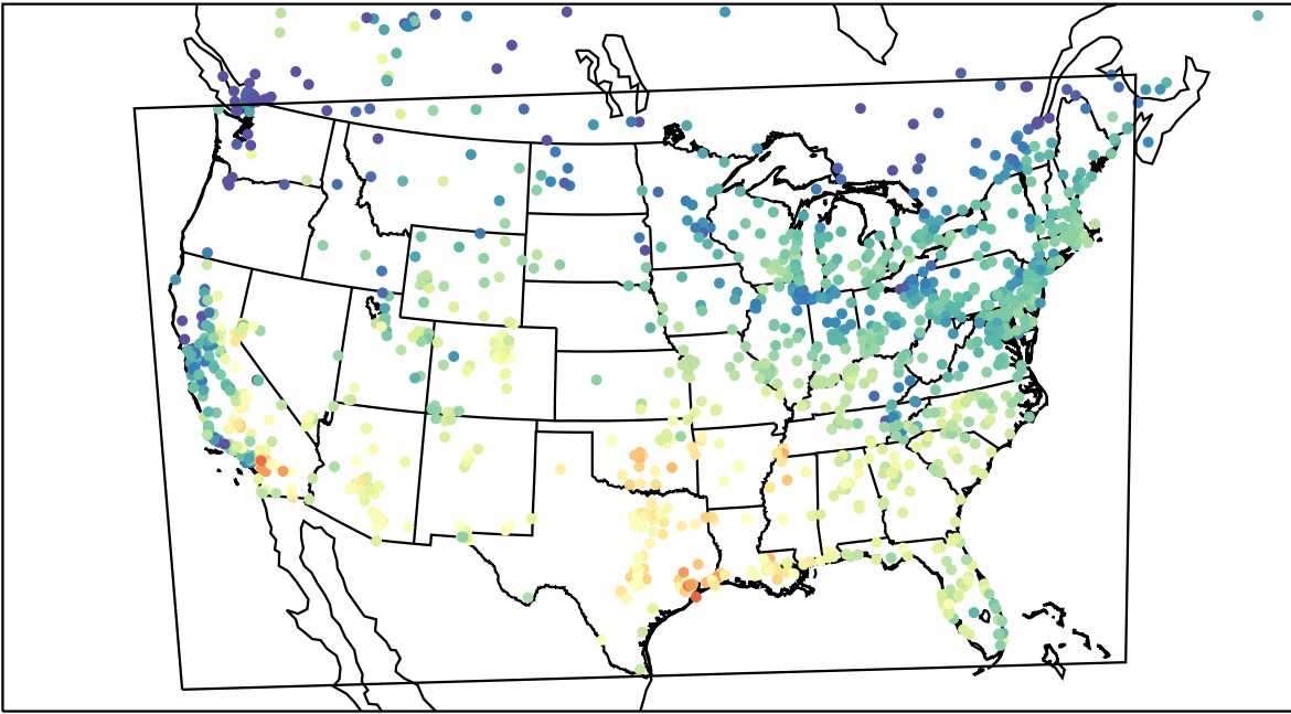
AirNOW (2023-10-09_18:00:00)
