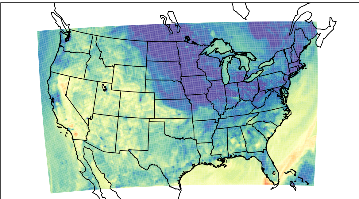
WRF (2023-10-09_04:00:00)
