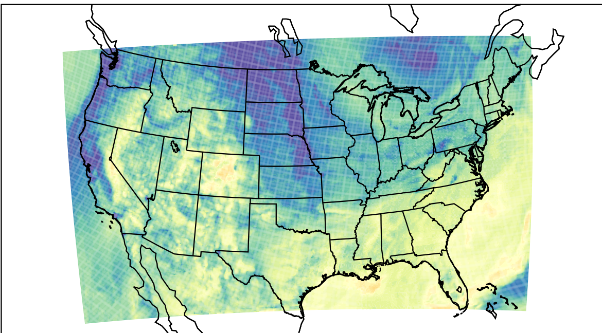
WRF (2023-10-09_16:00:00)
