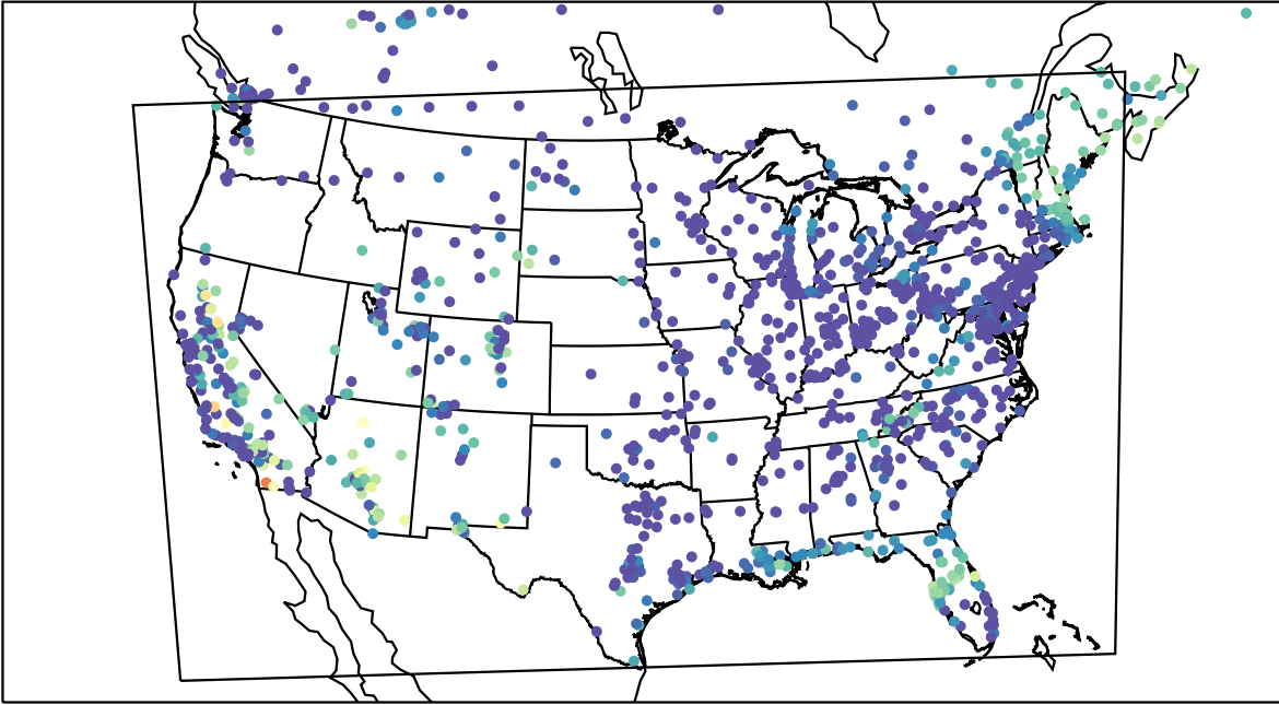
AirNOW (2023-10-08_09:00:00)
