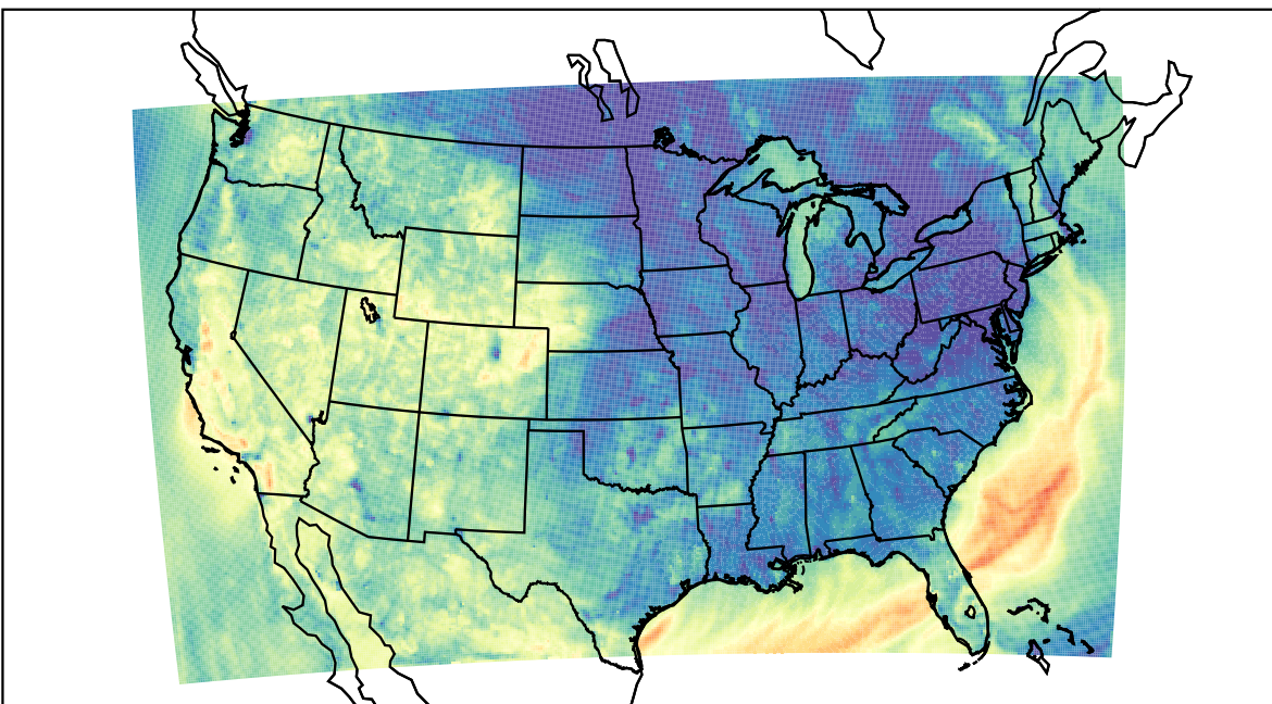
WRF (2023-10-08_03:00:00)
