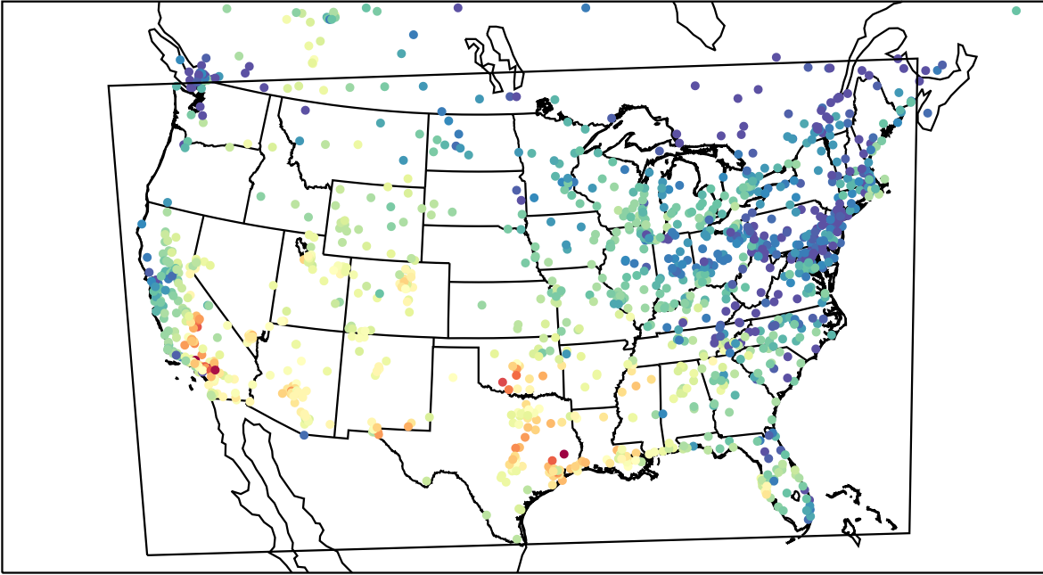
AirNOW (2023-10-09_23:00:00)
