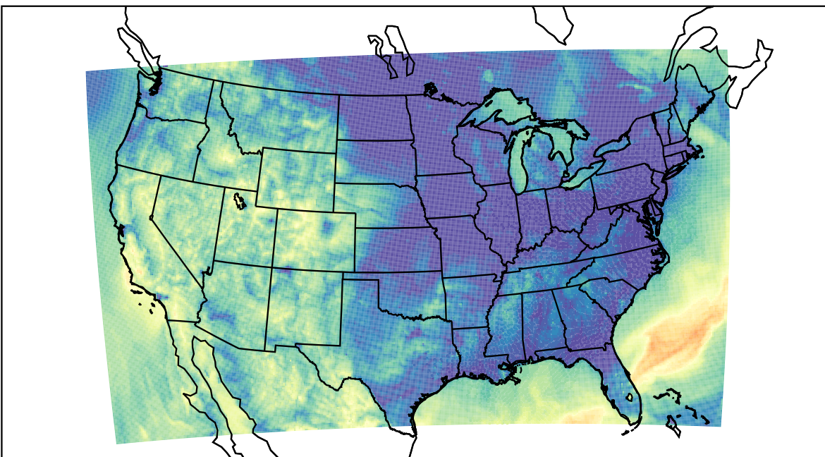
WRF (2023-10-08_10:00:00)
