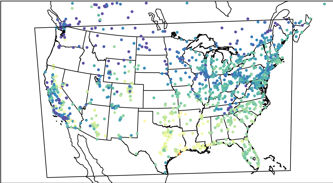
AirNOW (2023-10-09_16:00:00)
