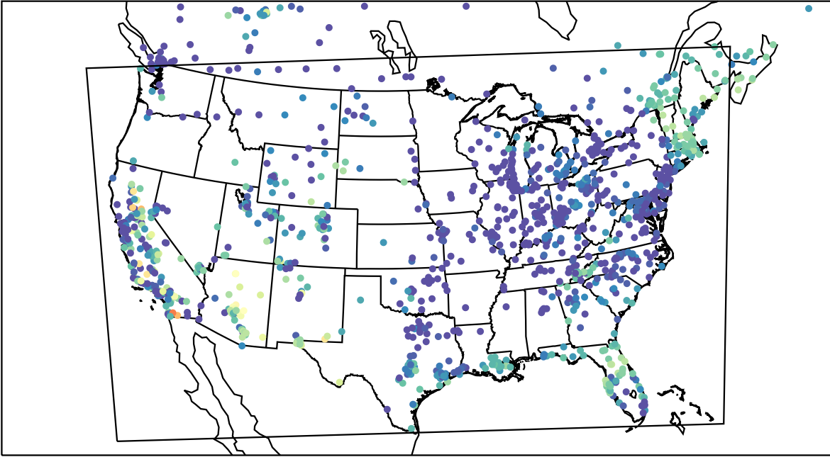
AirNOW (2023-10-08_06:00:00)
