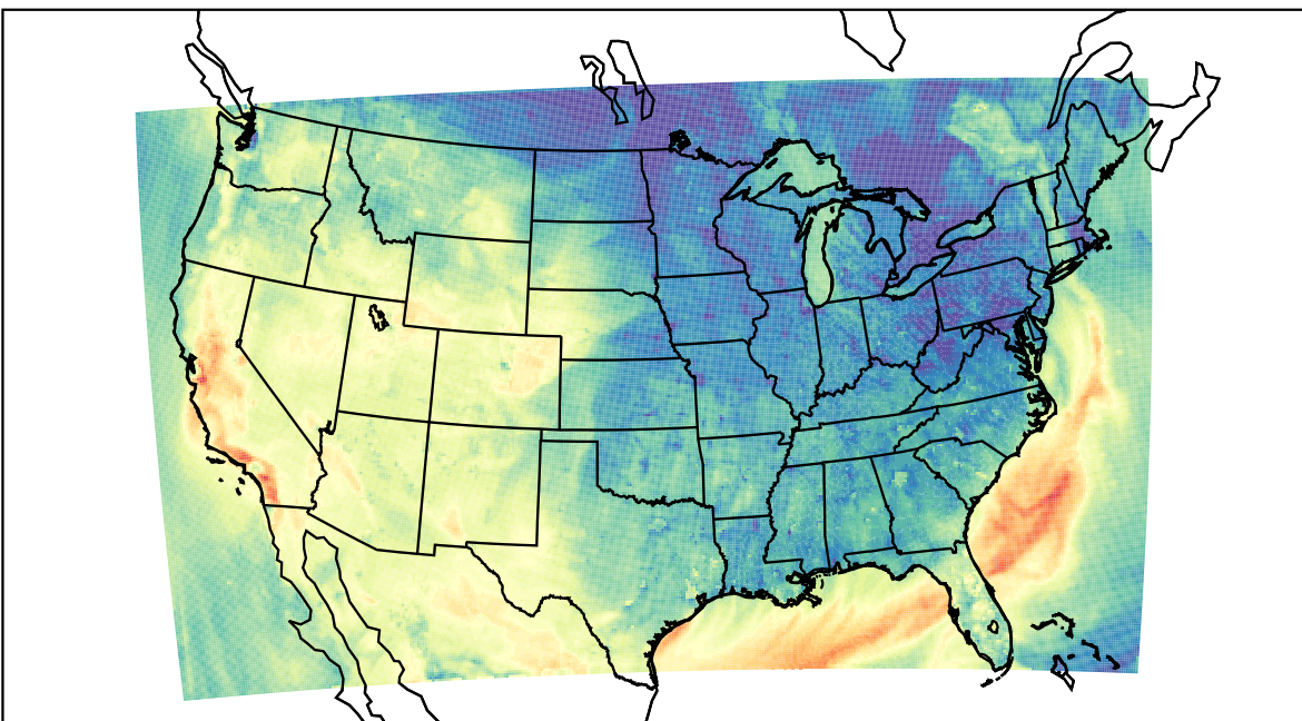
WRF (2023-10-08_00:00:00)
