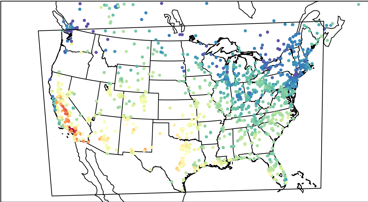
AirNOW (2023-10-08_19:00:00)
