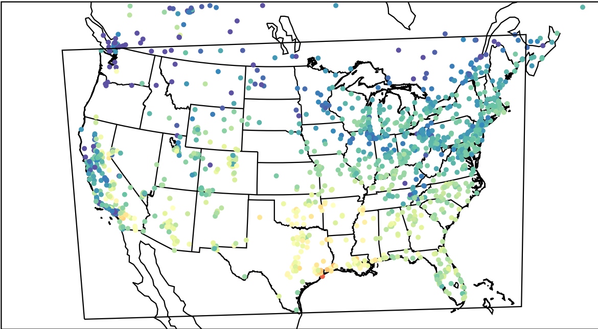
AirNOW (2023-10-09_17:00:00)
