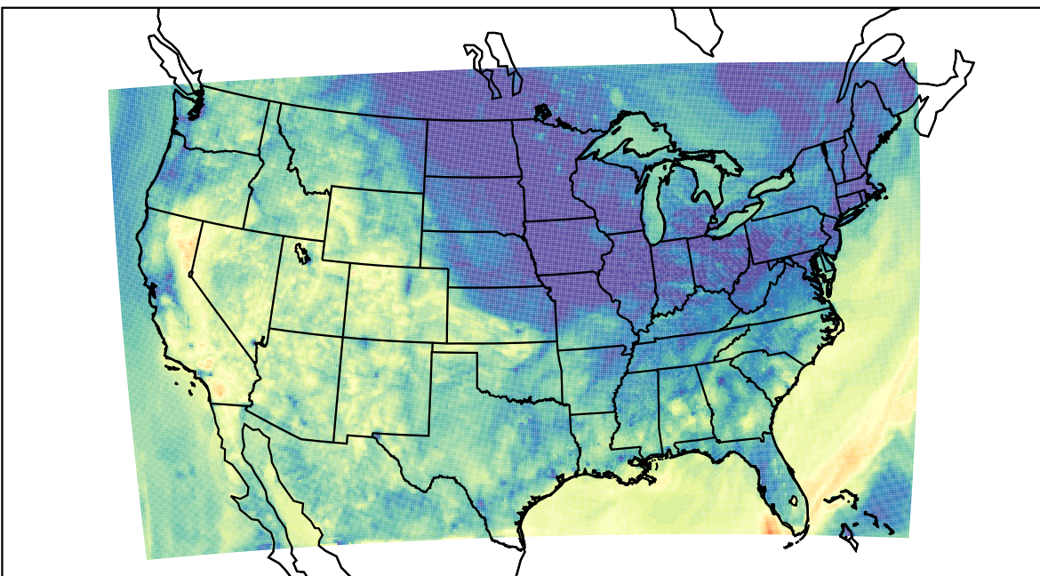
WRF (2023-10-09_05:00:00)
