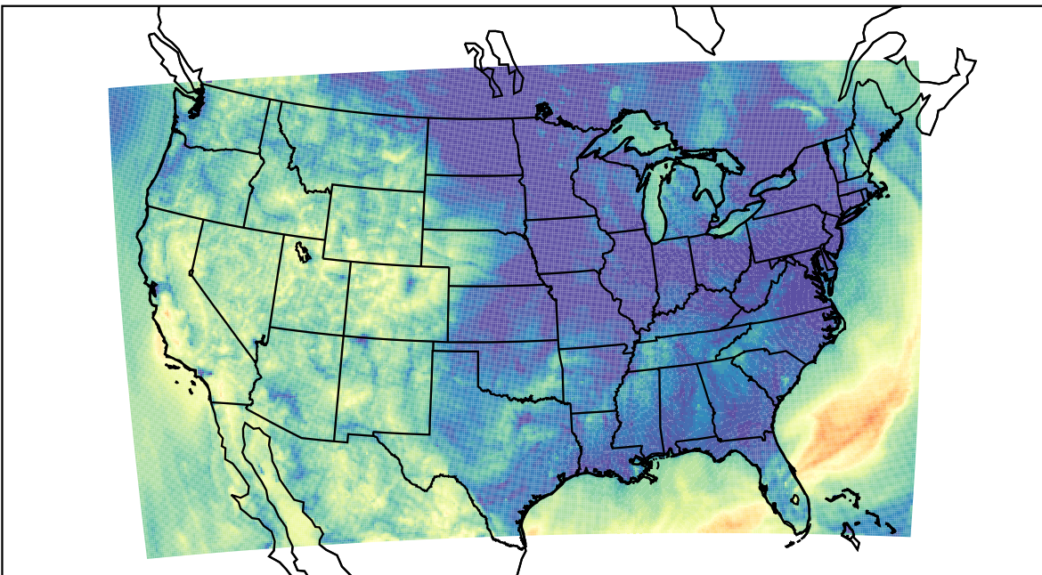
WRF (2023-10-08_08:00:00)
