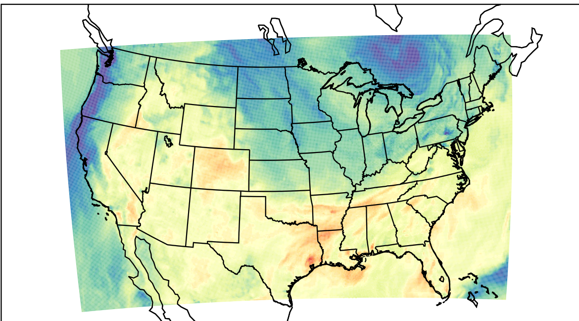
WRF (2023-10-09_19:00:00)
