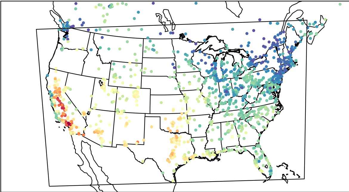
AirNOW (2023-10-08_21:00:00)
