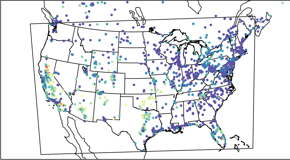
AirNOW (2023-10-09_05:00:00)
