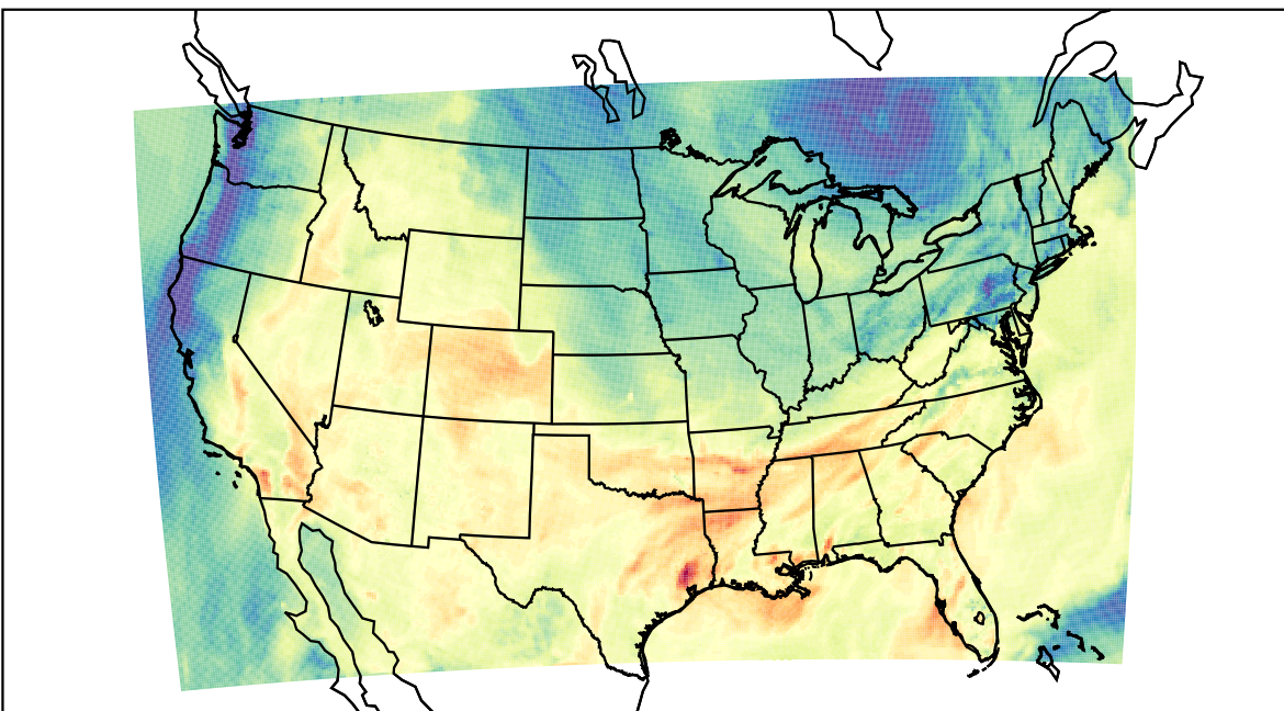
WRF (2023-10-09_21:00:00)
