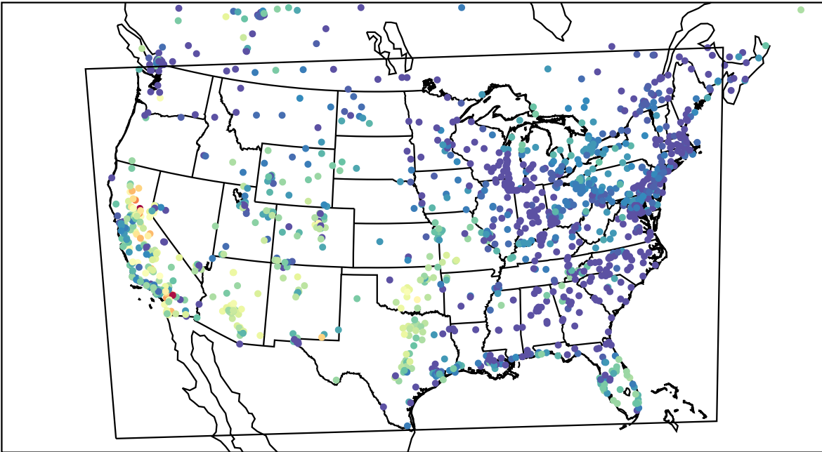
AirNOW (2023-10-09_03:00:00)
