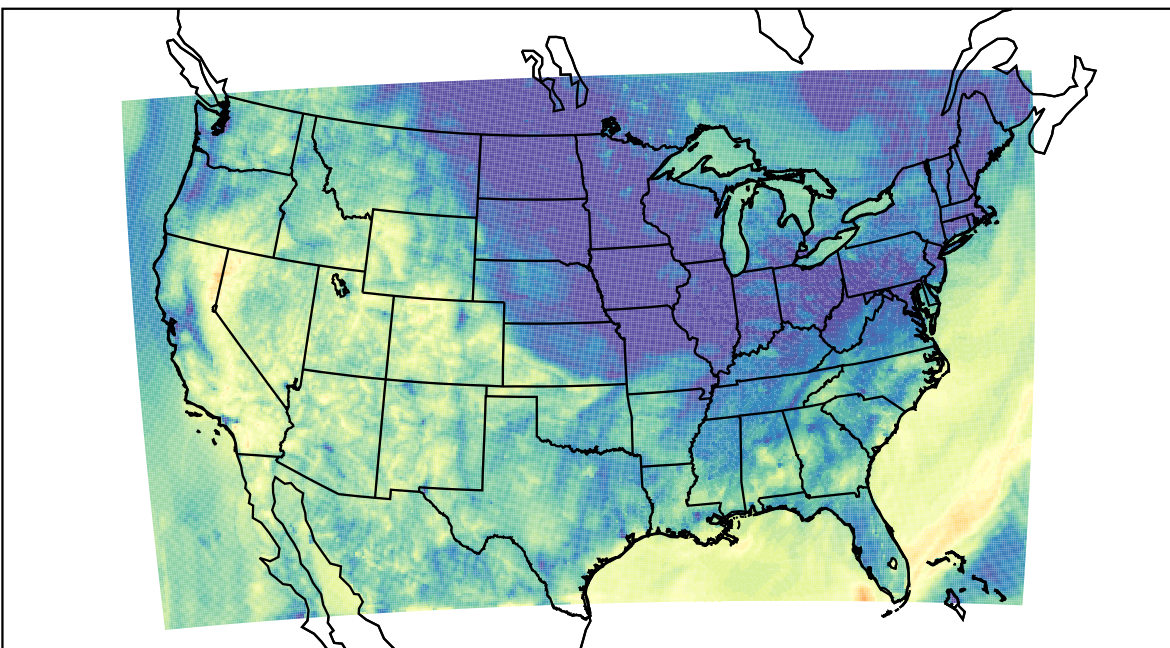
WRF (2023-10-09_07:00:00)
