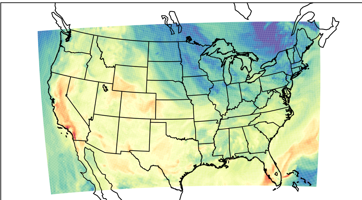
WRF (2023-10-08_21:00:00)
