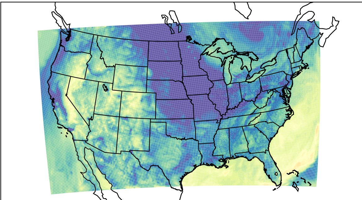
WRF (2023-10-09_14:00:00)
