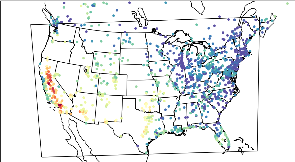
AirNOW (2023-10-09_00:00:00)
