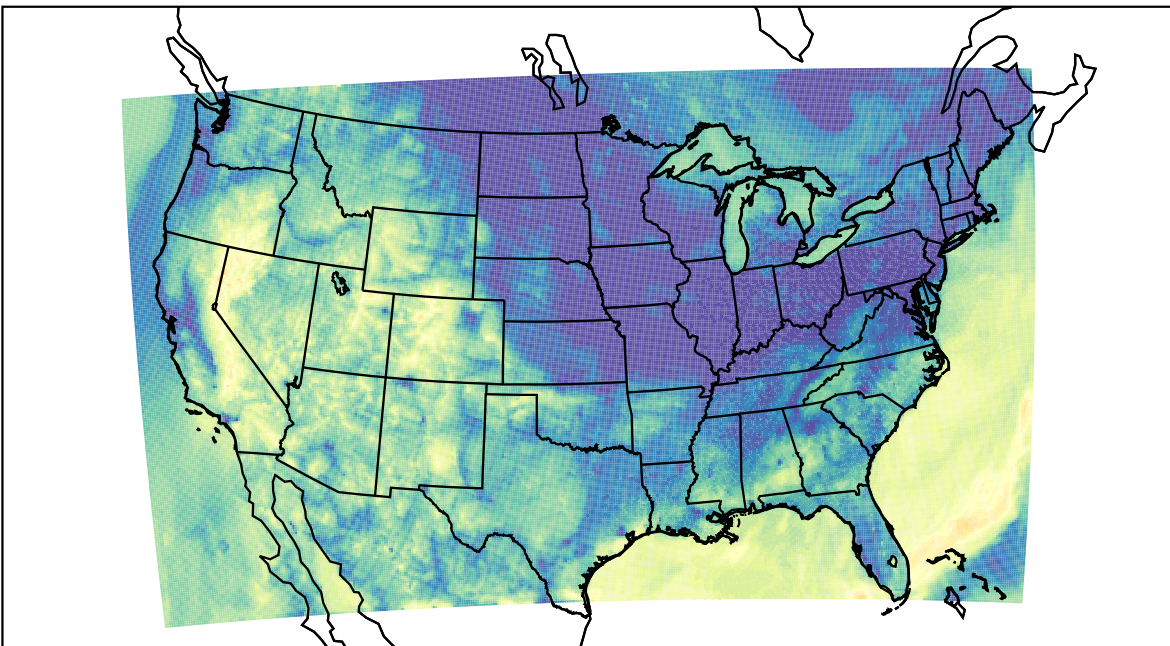
WRF (2023-10-09_11:00:00)
