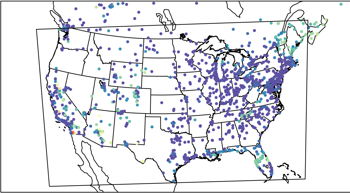
AirNOW (2023-10-08_11:00:00)
