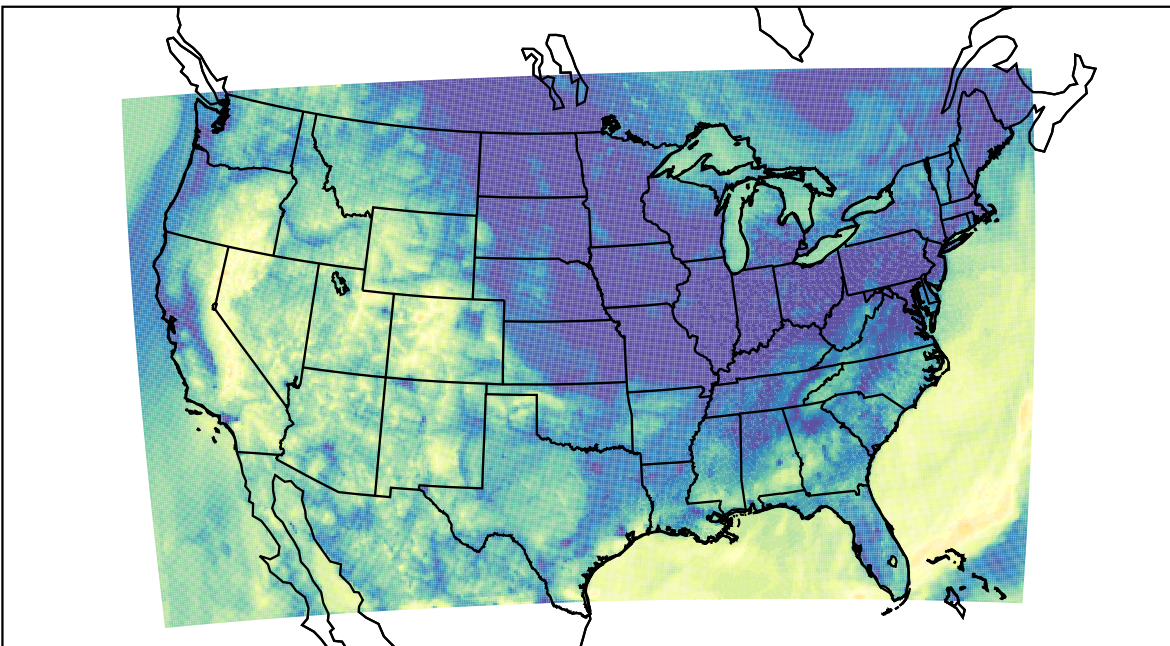
WRF (2023-10-09_12:00:00)
