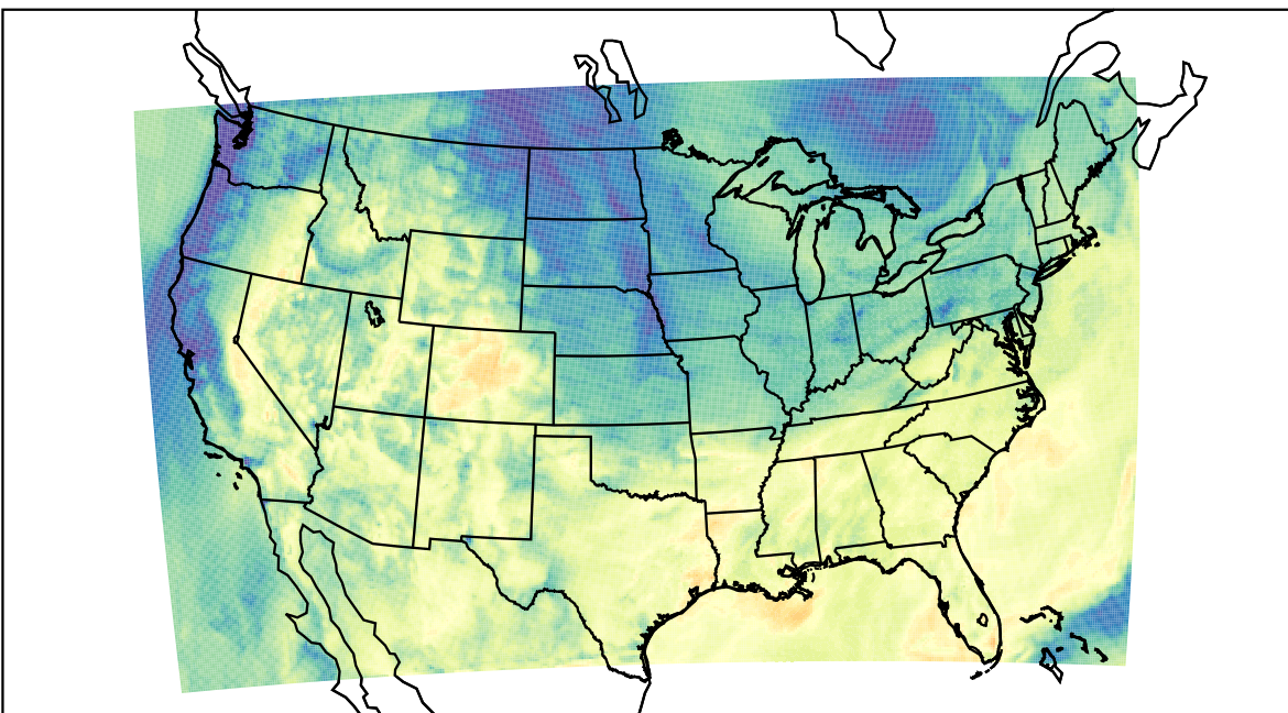
WRF (2023-10-09_17:00:00)
