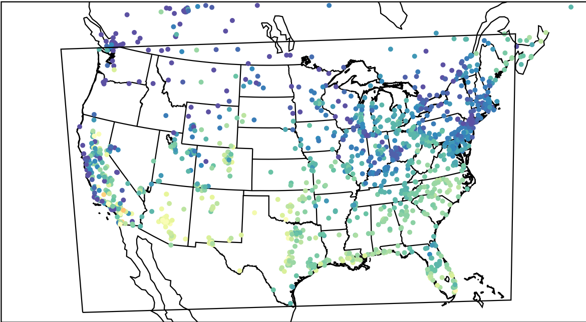
AirNOW (2023-10-08_16:00:00)
