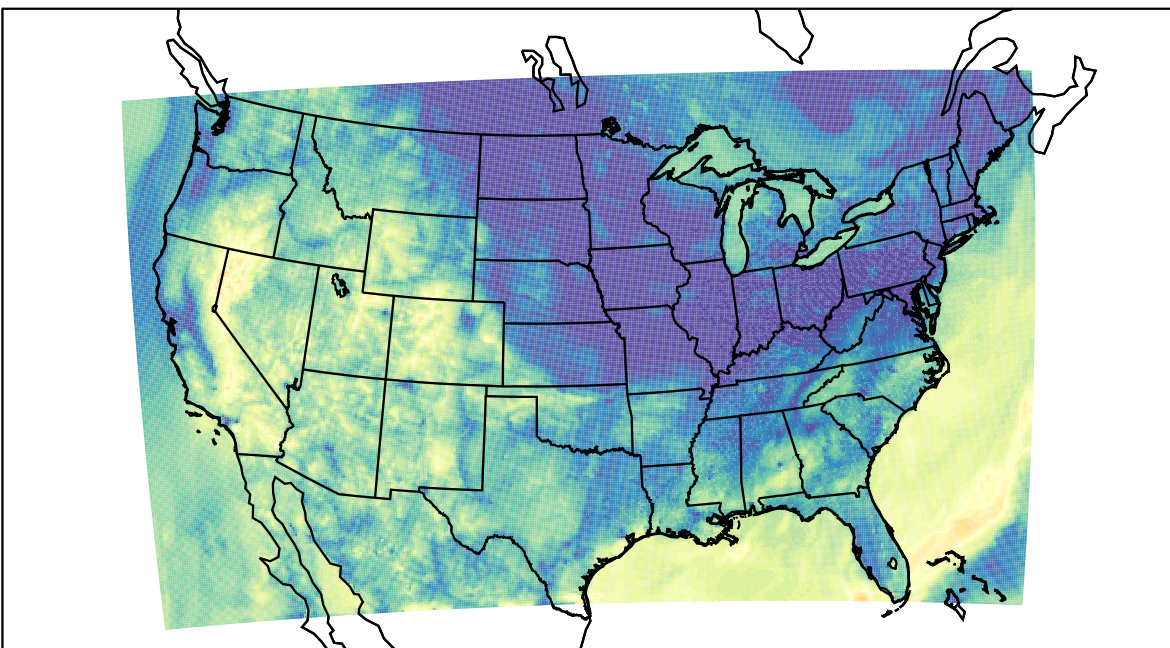
WRF (2023-10-09_10:00:00)
