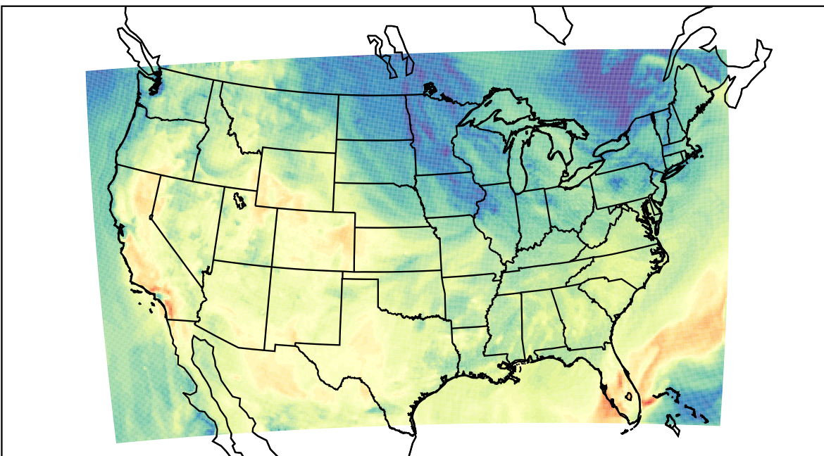
WRF (2023-10-08_19:00:00)
