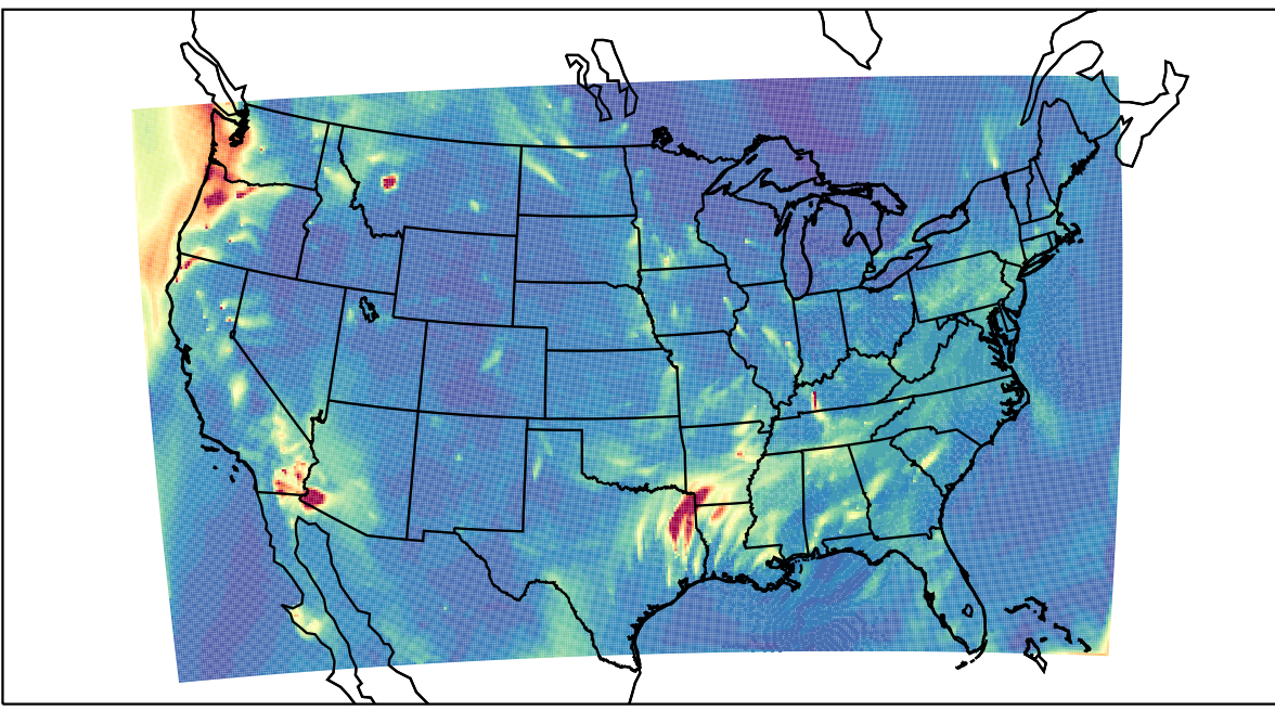
WRF 2023-10-10_05:00:00
