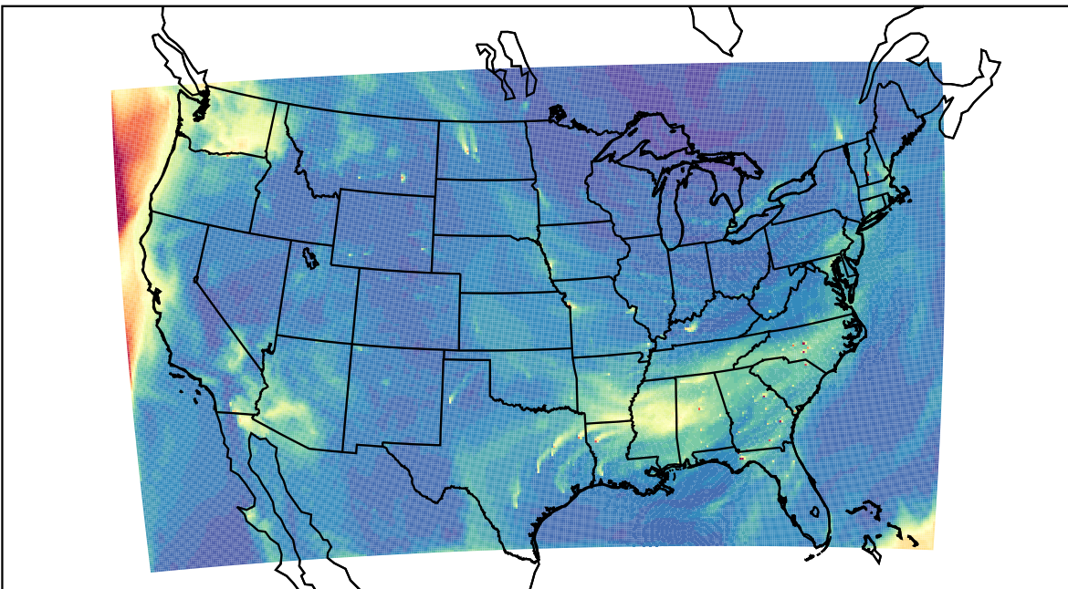
WRF 2023-10-10_17:00:00
