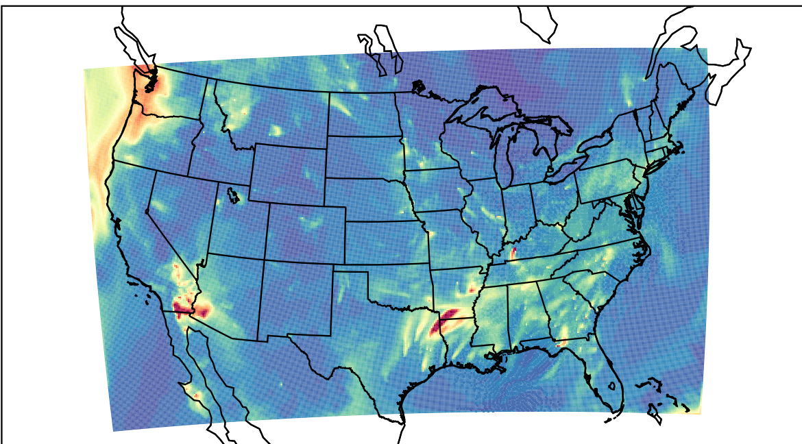
WRF 2023-10-10_07:00:00
