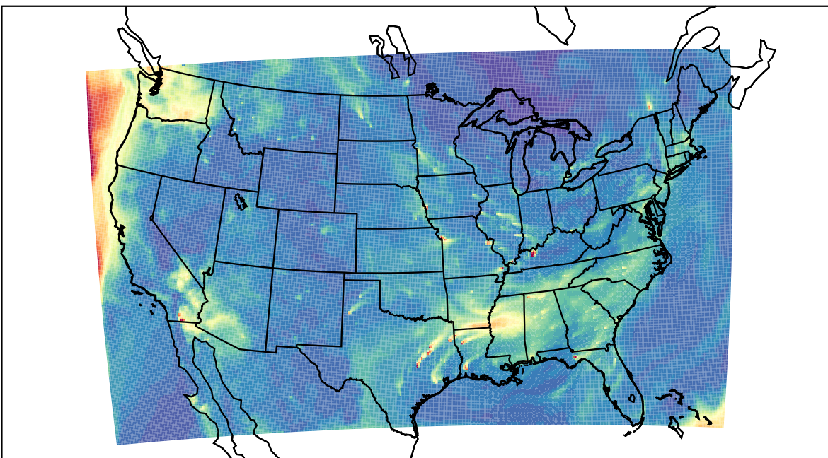
WRF 2023-10-10_15:00:00
