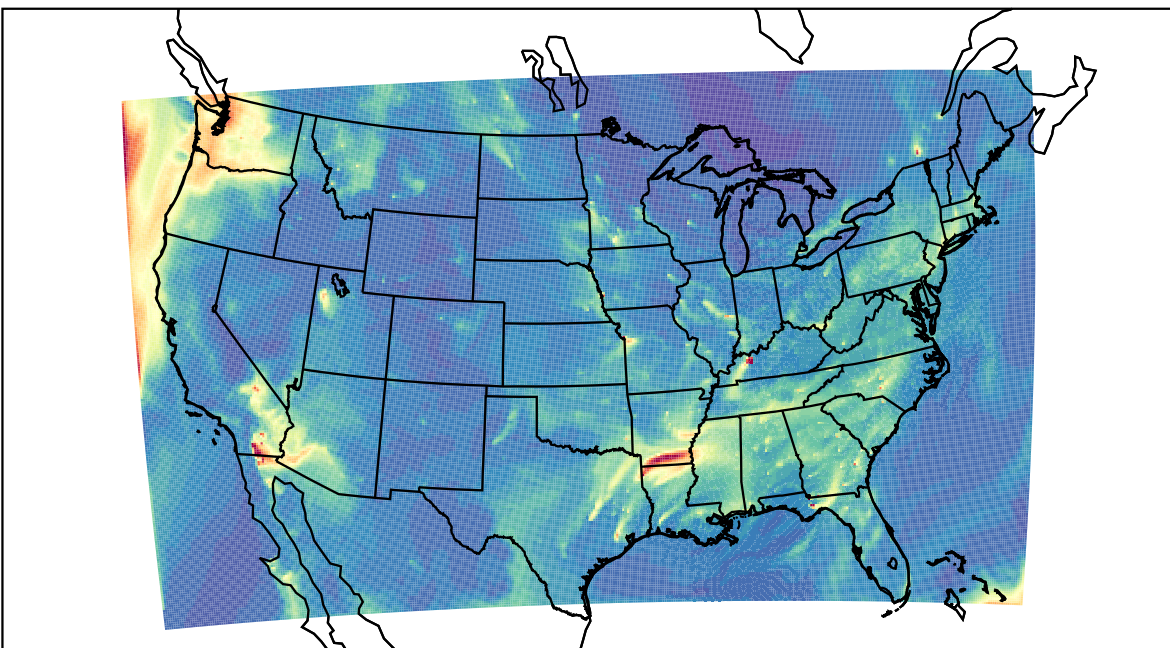
WRF 2023-10-10_11:00:00
