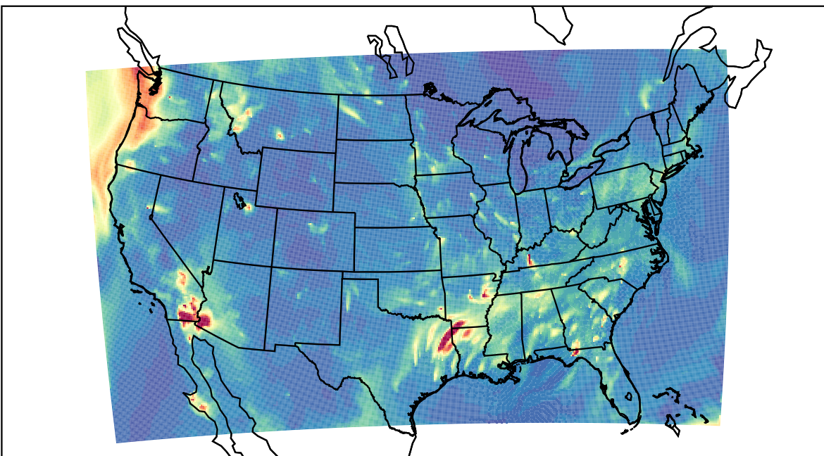
WRF 2023-10-10_05:00:00
