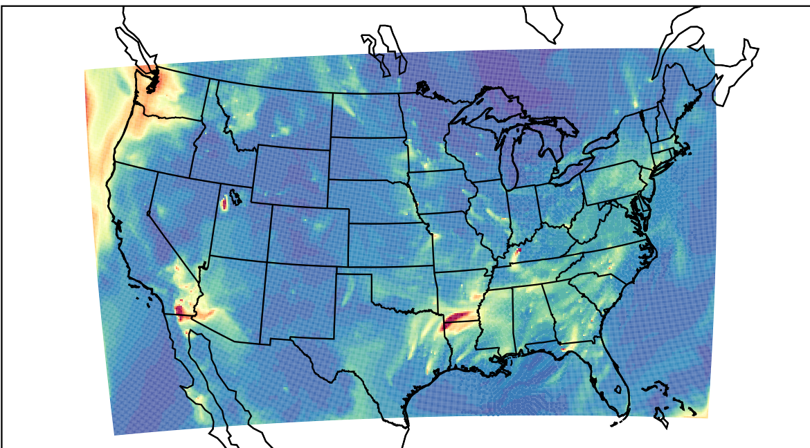
WRF 2023-10-10_09:00:00
