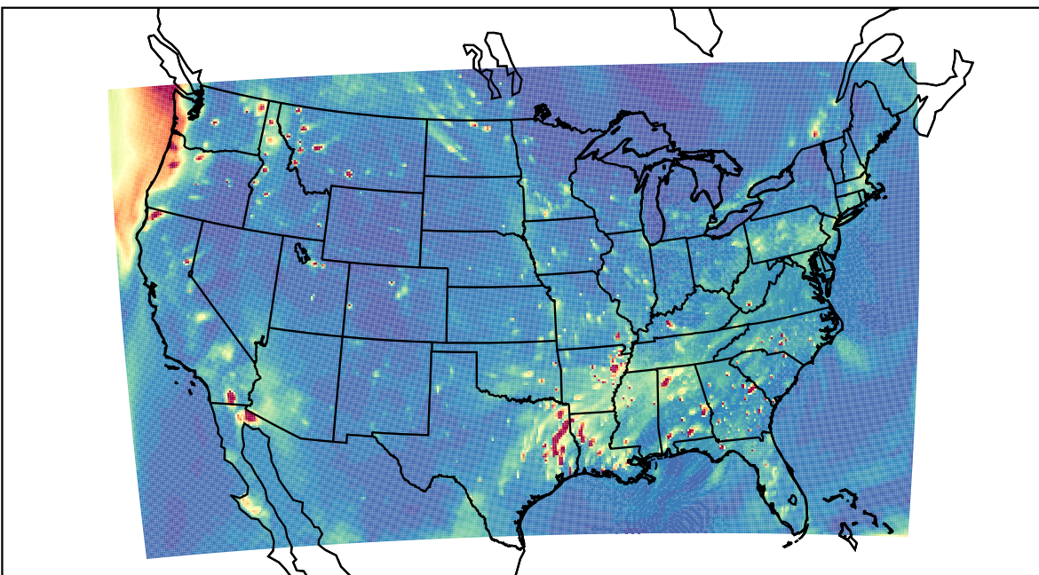
WRF 2023-10-10_01:00:00
