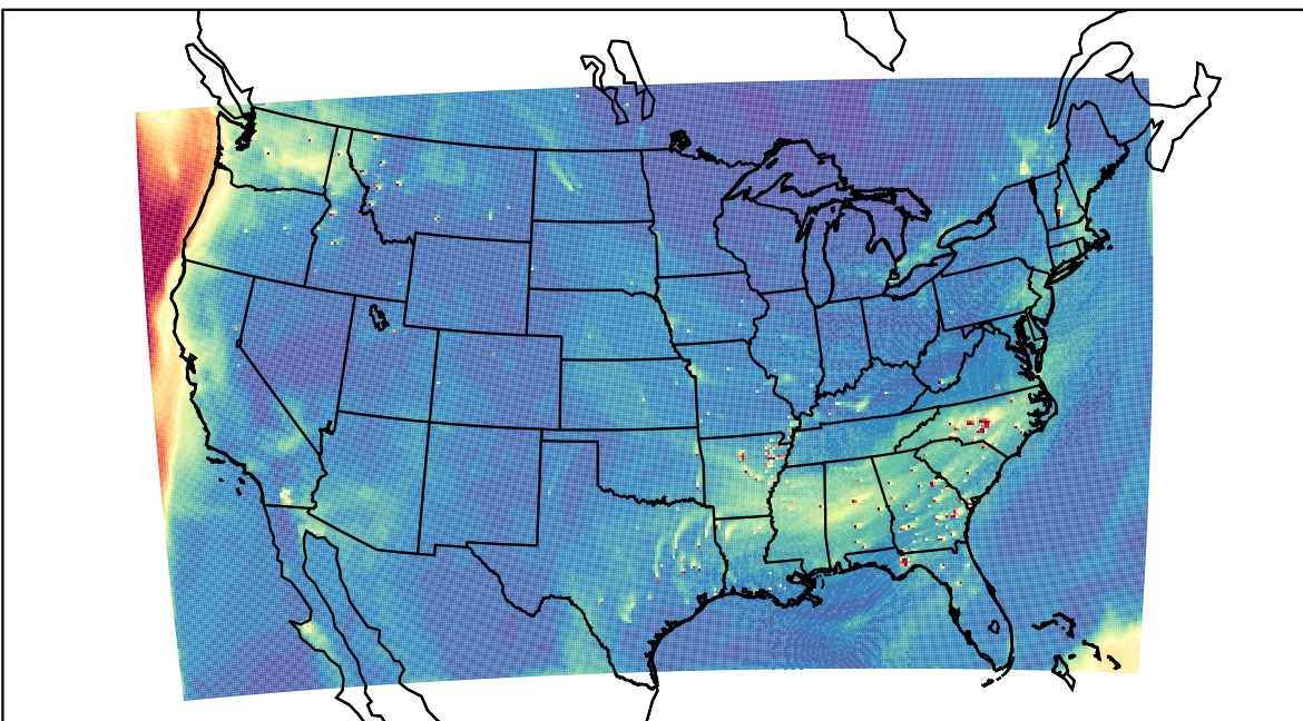
WRF 2023-10-10_21:00:00
