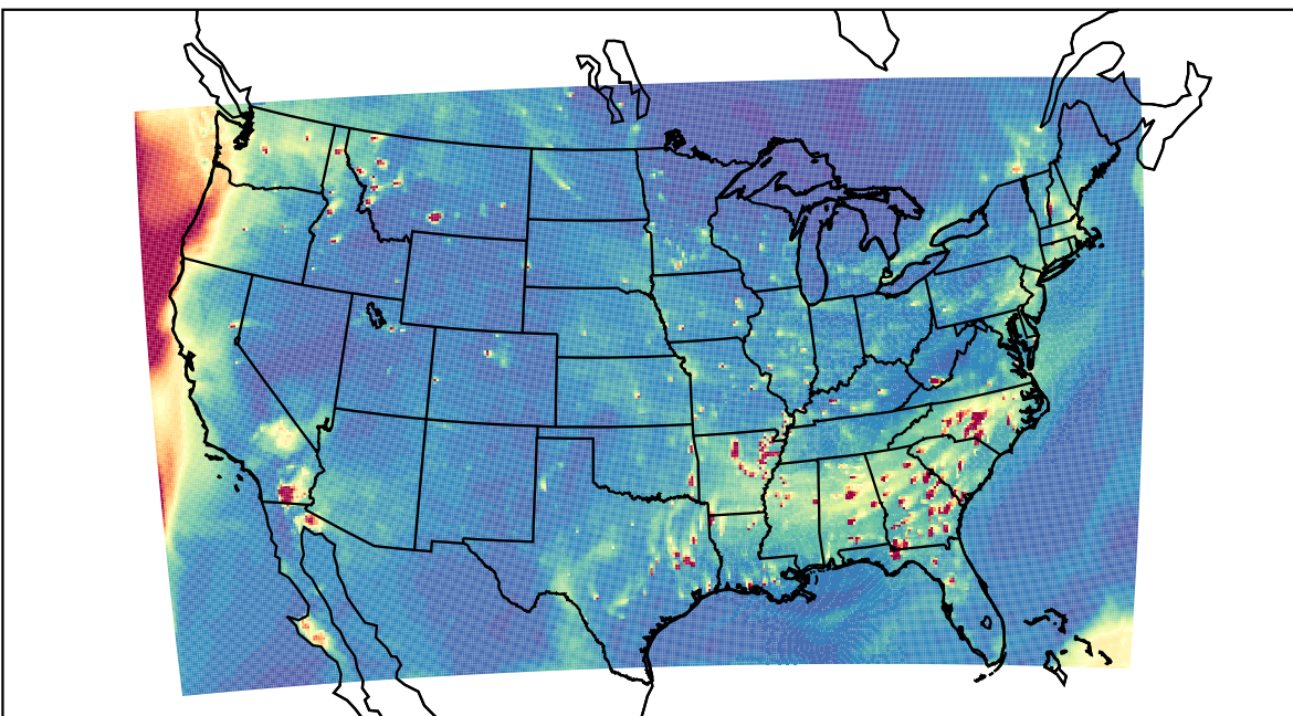
WRF 2023-10-11_00:00:00
