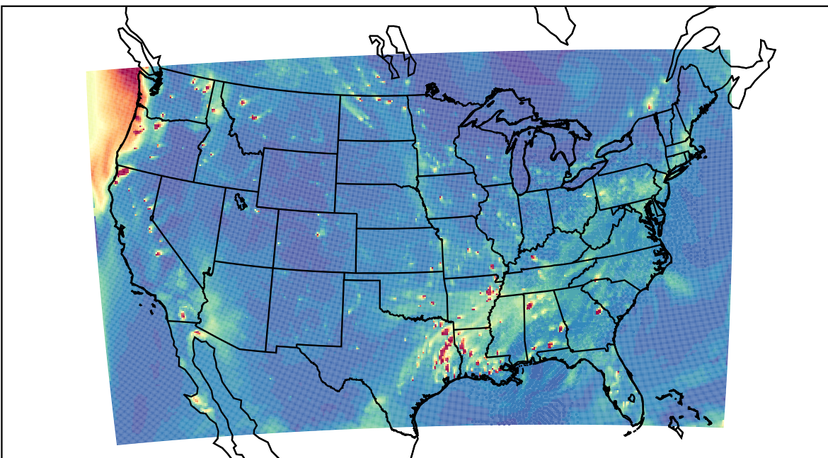
WRF 2023-10-10_00:00:00
