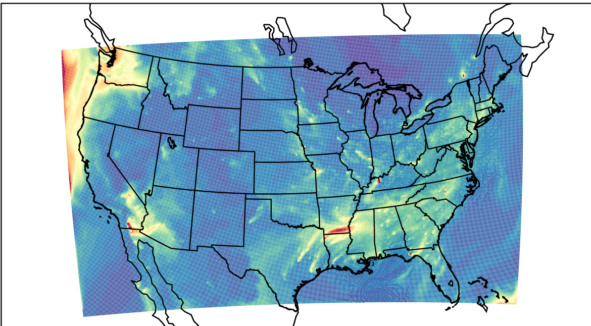
WRF 2023-10-10_12:00:00
