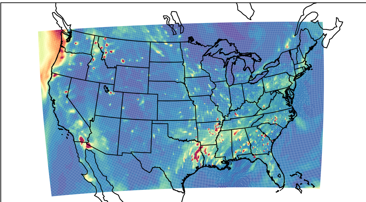
WRF 2023-10-10_02:00:00
