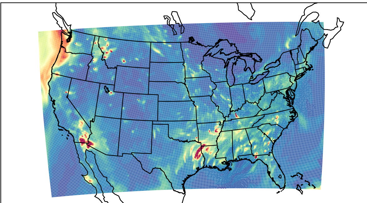
WRF 2023-10-10_04:00:00
