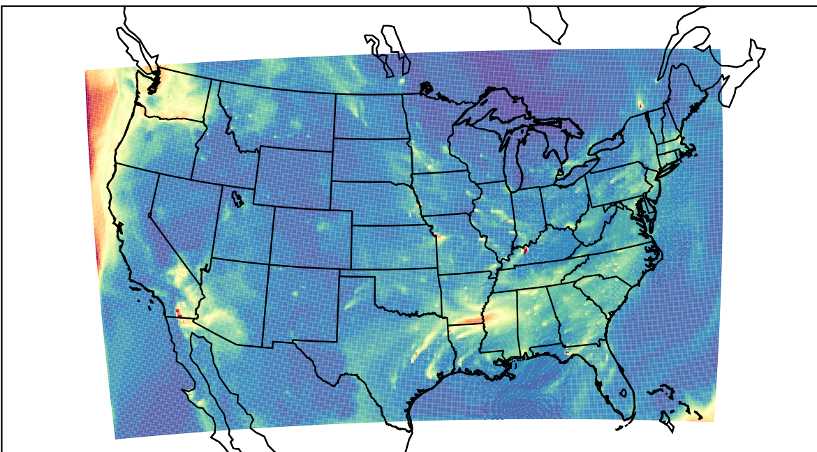
WRF 2023-10-10_14:00:00
