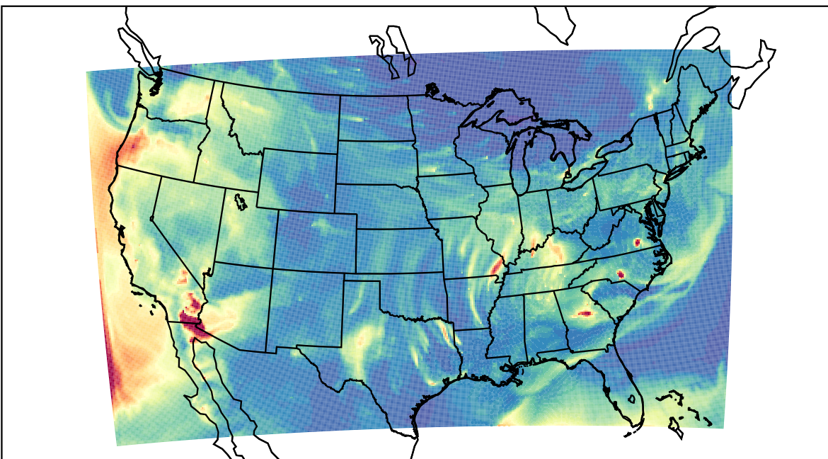
WRF 2023-10-12_05:00:00
