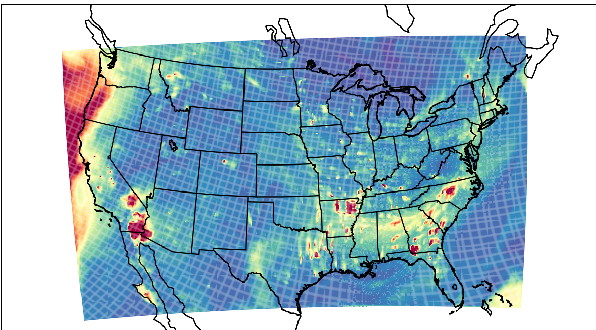
WRF 2023-10-11_03:00:00
