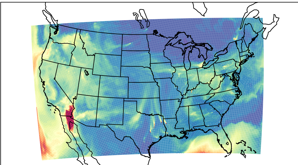
WRF 2023-10-12_16:00:00
