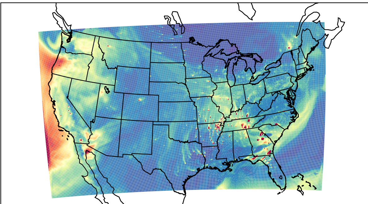
WRF 2023-10-11_23:00:00
