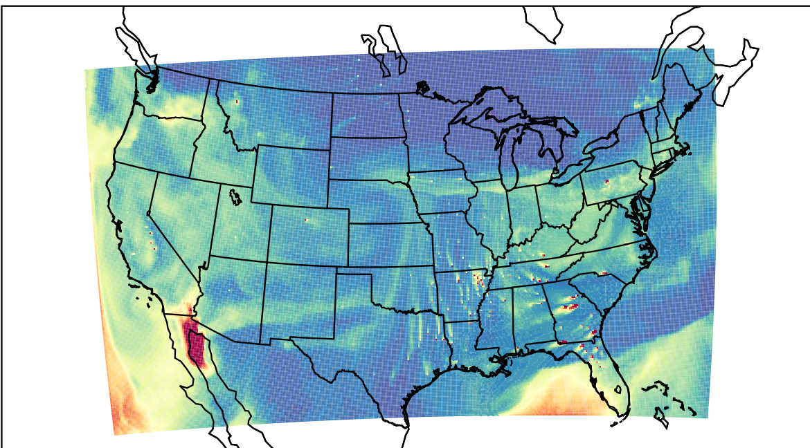
WRF 2023-10-12_21:00:00
