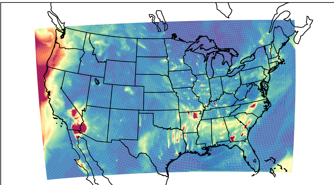
WRF 2023-10-11_05:00:00
