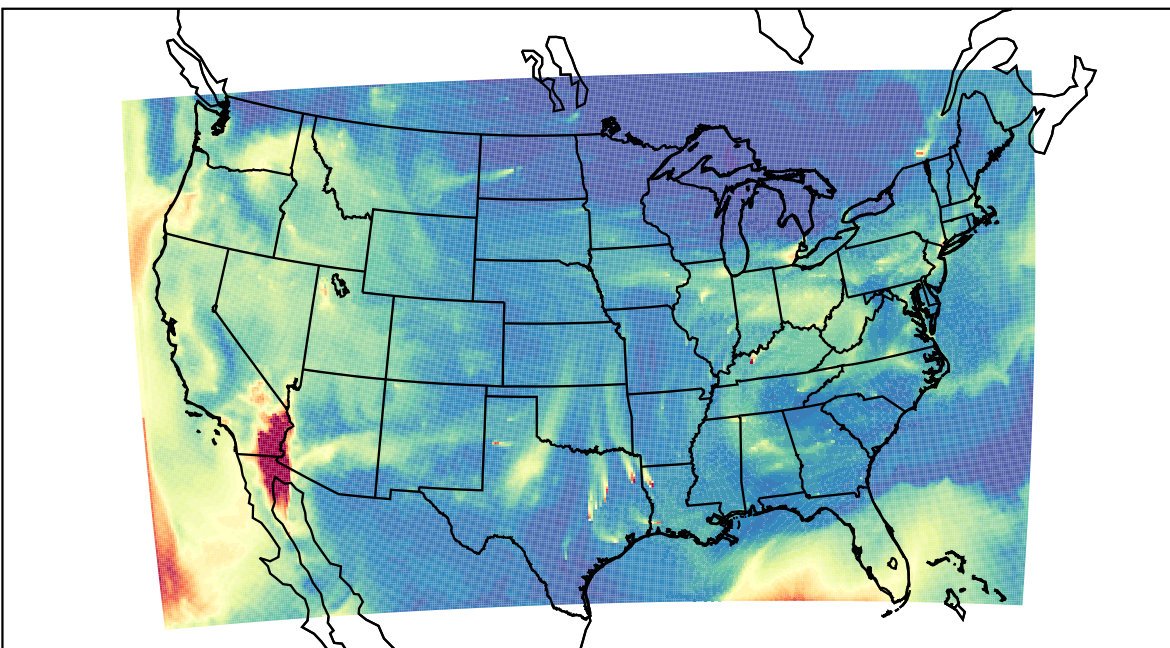
WRF 2023-10-12_15:00:00
