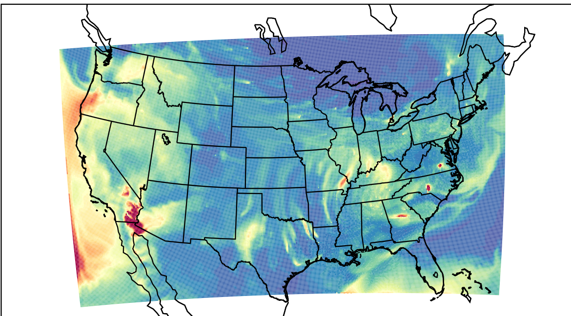
WRF 2023-10-12_06:00:00
