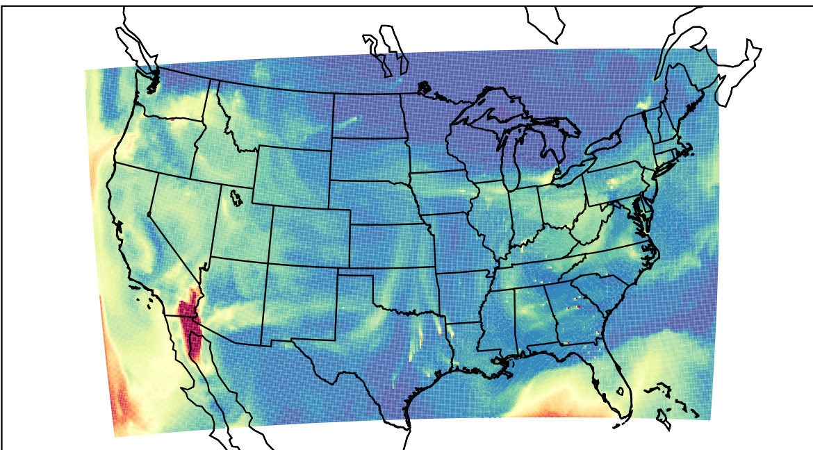
WRF 2023-10-12_17:00:00
