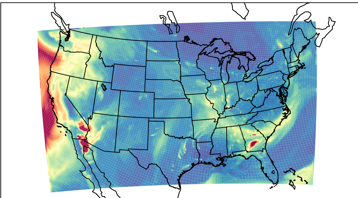
WRF 2023-10-11_17:00:00
