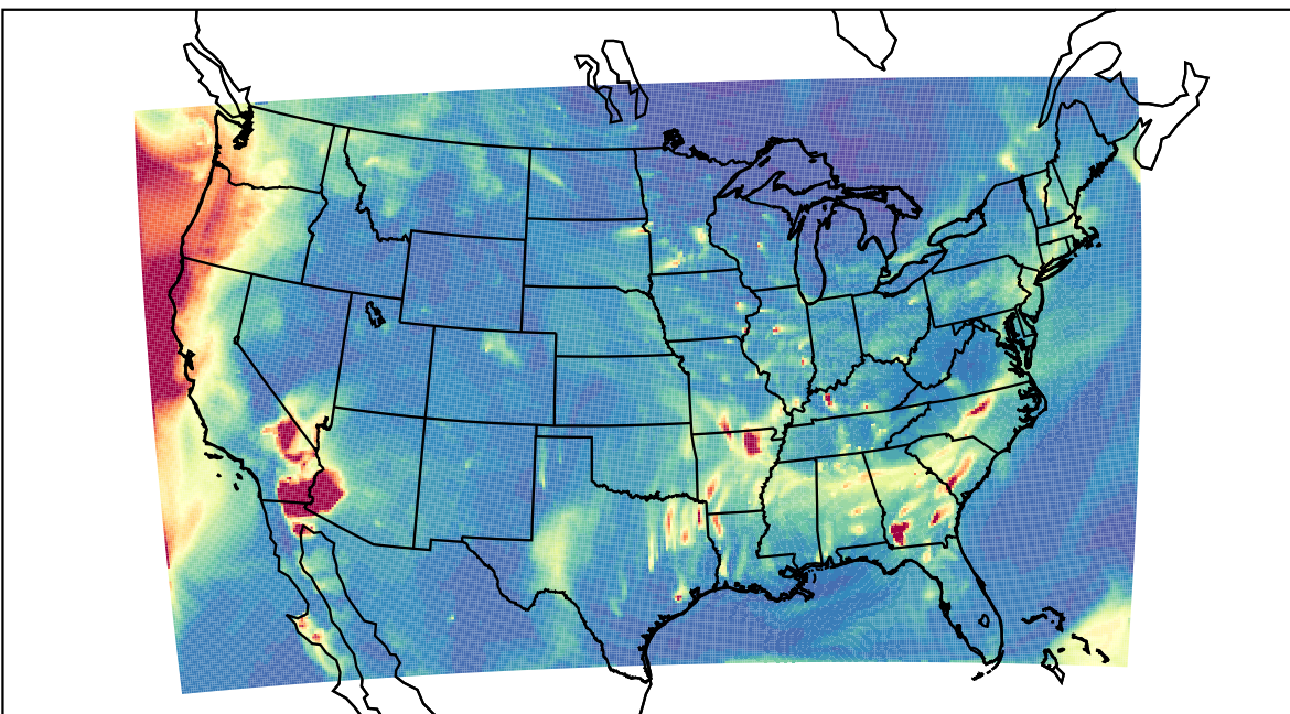
WRF 2023-10-11_06:00:00
