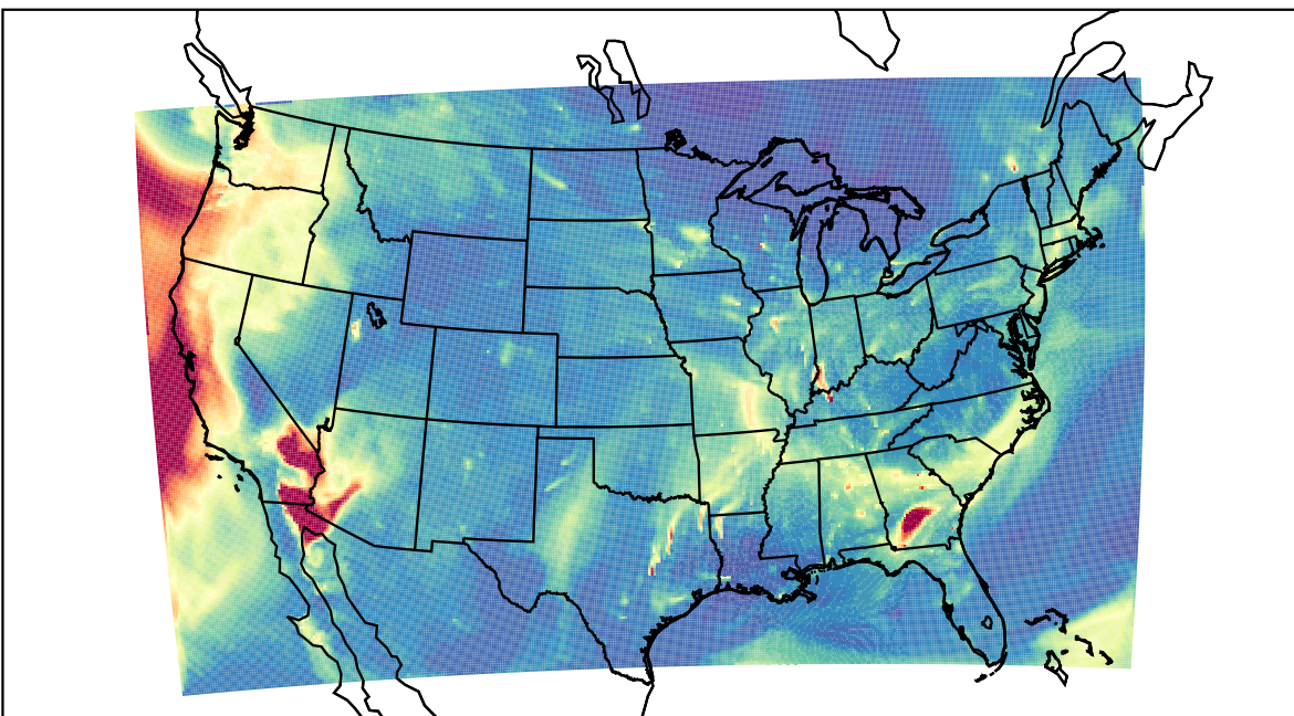
WRF 2023-10-11_14:00:00
