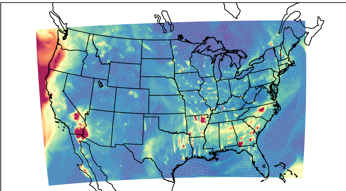
WRF 2023-10-11_04:00:00
