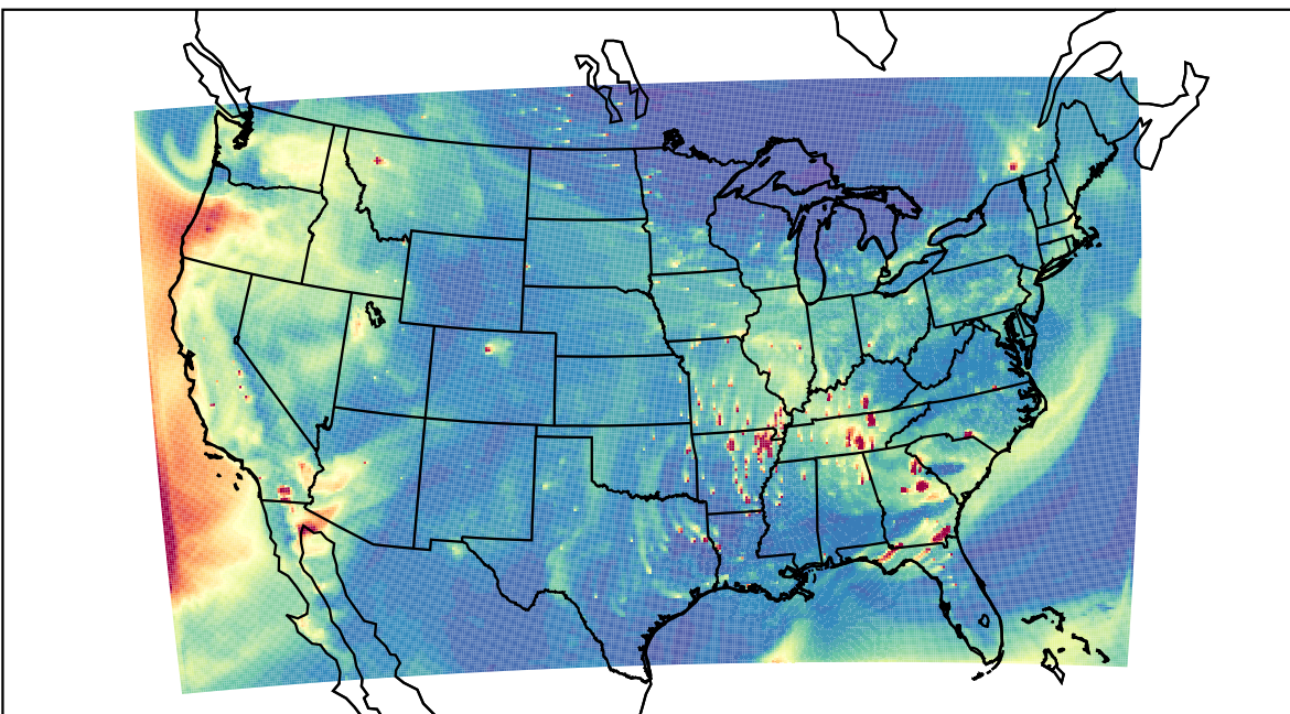
WRF 2023-10-12_00:00:00
