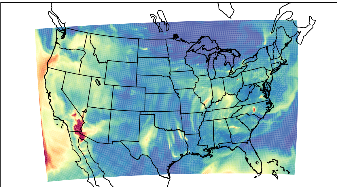
WRF 2023-10-12_08:00:00
