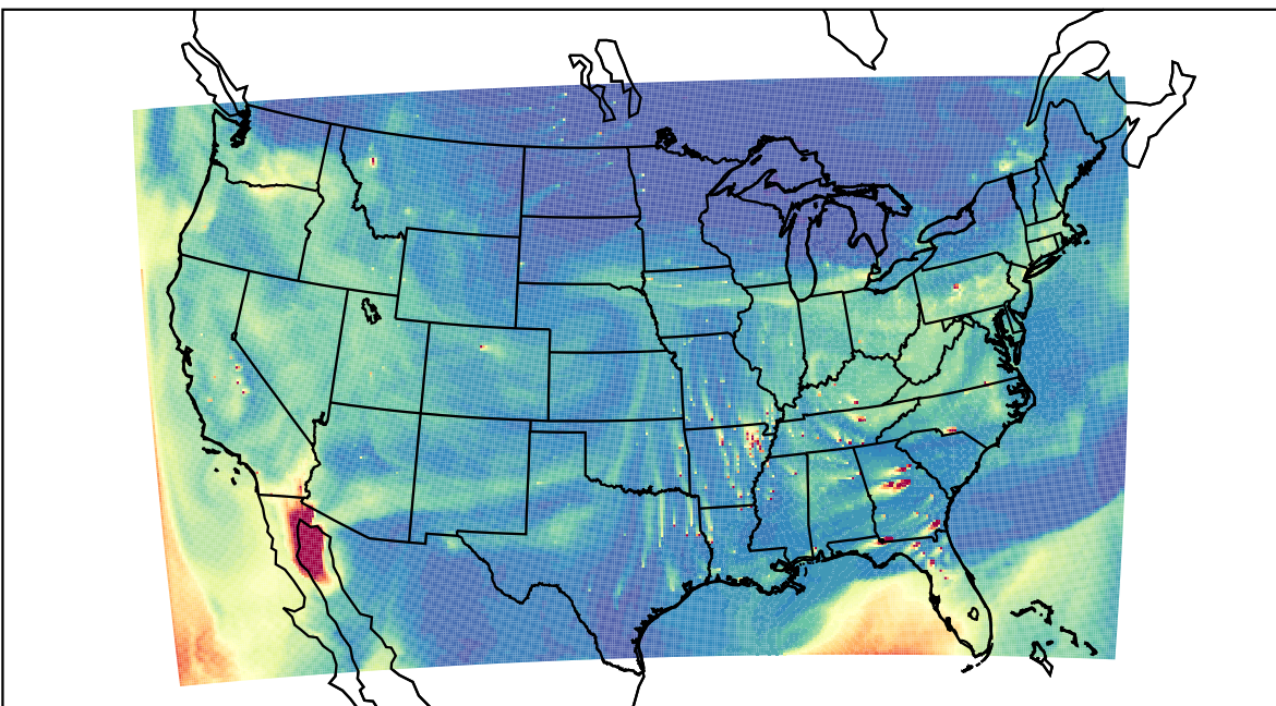
WRF 2023-10-12_22:00:00
