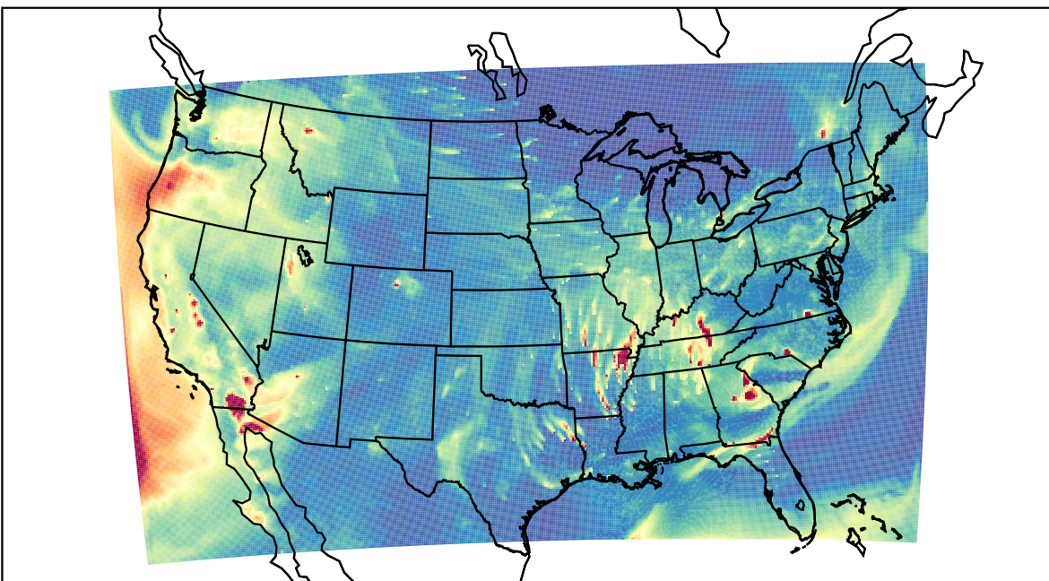
WRF 2023-10-12_02:00:00
