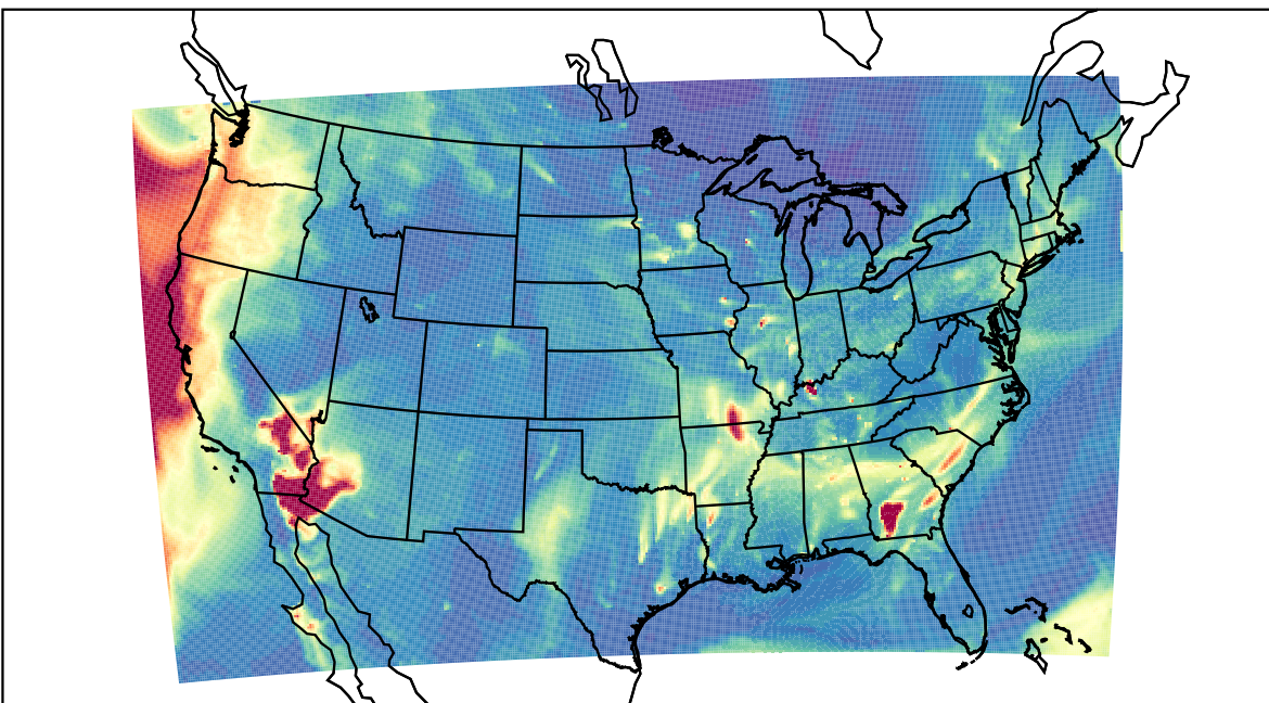
WRF 2023-10-11_09:00:00
