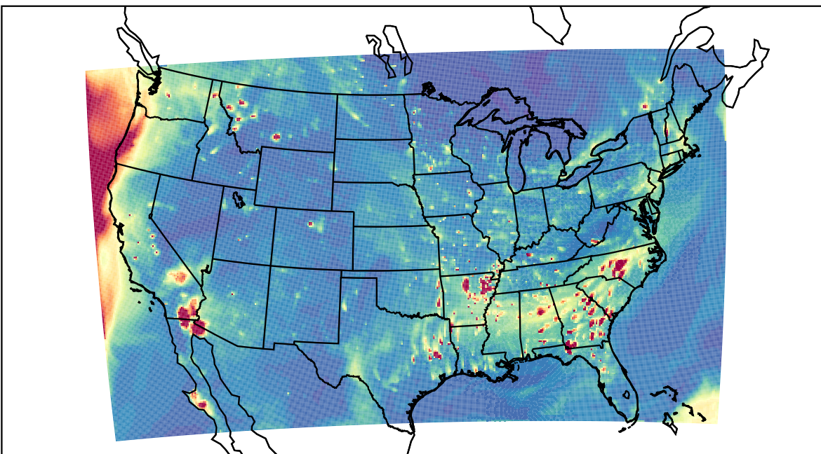
WRF 2023-10-11_01:00:00
