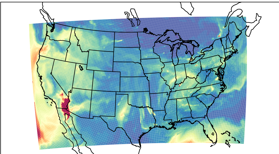
WRF 2023-10-12_11:00:00
