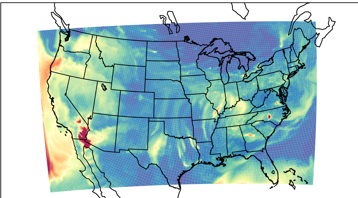
WRF 2023-10-12_07:00:00
