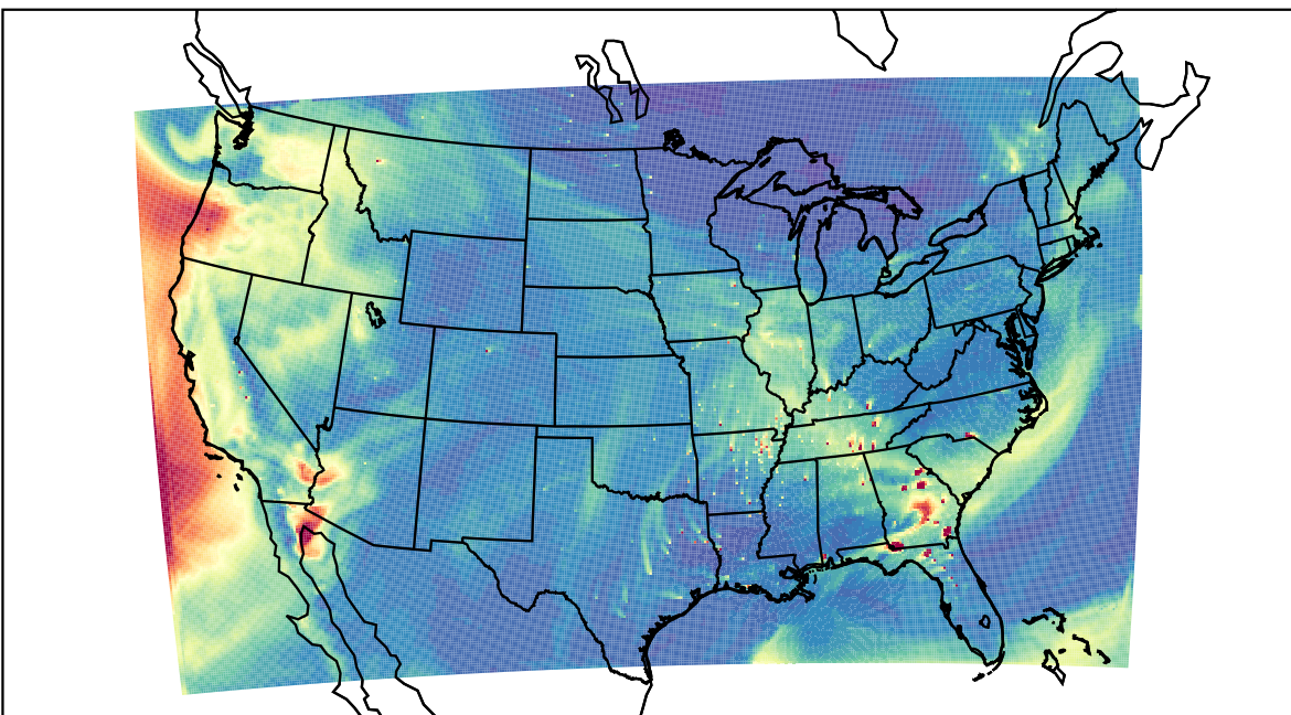
WRF 2023-10-11_21:00:00
