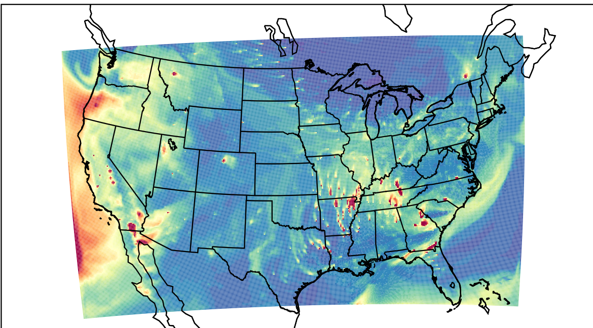
WRF 2023-10-12_01:00:00
