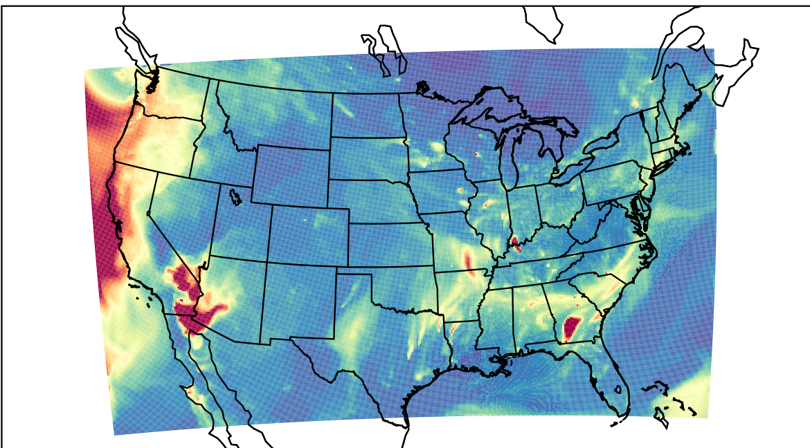
WRF 2023-10-11_11:00:00
