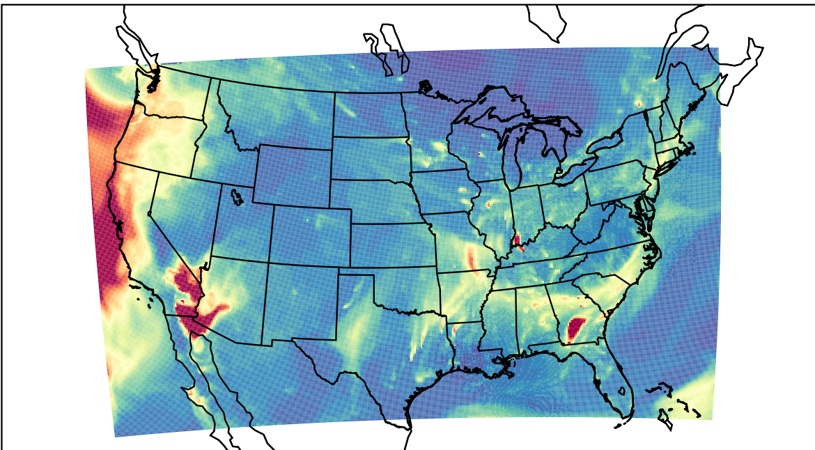
WRF 2023-10-11_12:00:00
