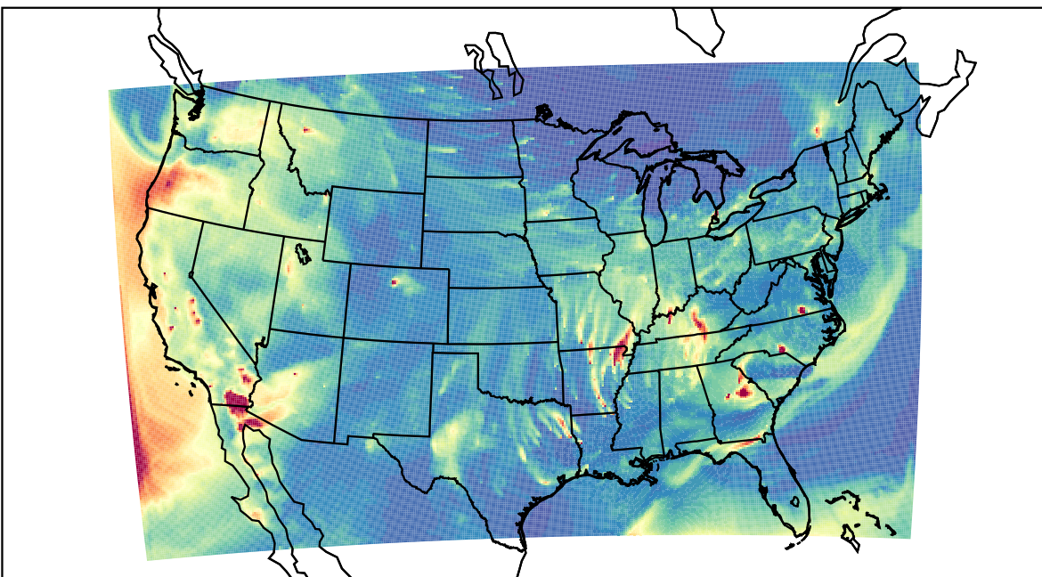
WRF 2023-10-12_03:00:00
