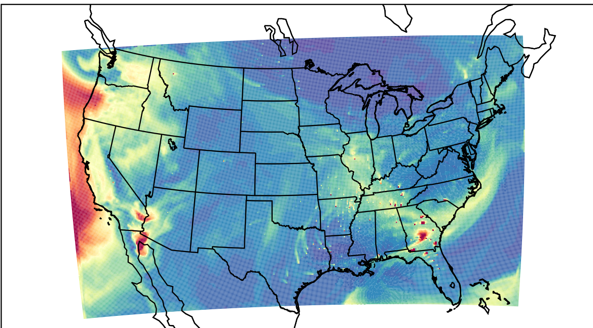
WRF 2023-10-11_20:00:00
