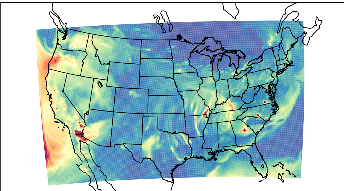
WRF 2023-10-12_04:00:00
