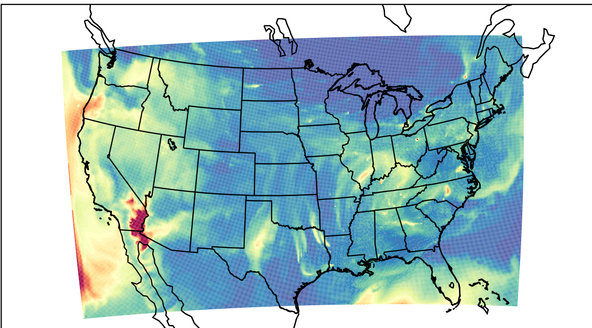
WRF 2023-10-12_09:00:00
