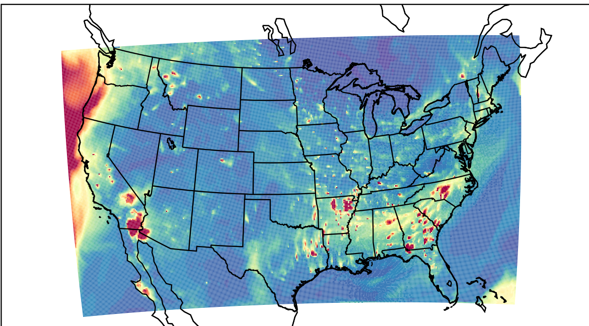
WRF 2023-10-11_02:00:00
