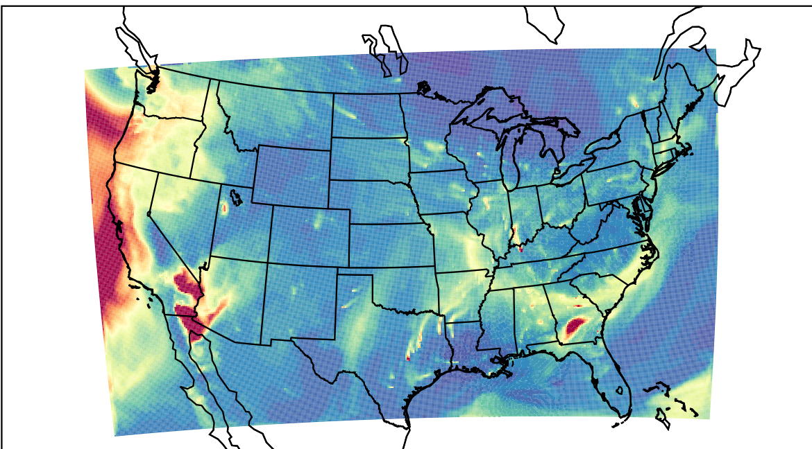
WRF 2023-10-11_15:00:00
