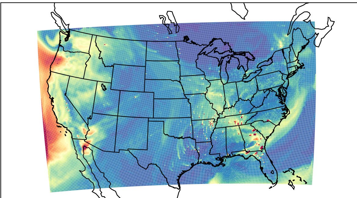
WRF 2023-10-11_22:00:00
