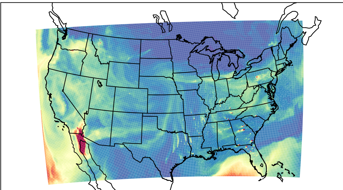
WRF 2023-10-12_19:00:00
