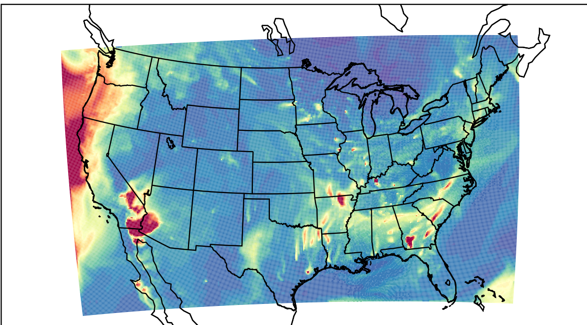
WRF 2023-10-11_07:00:00
