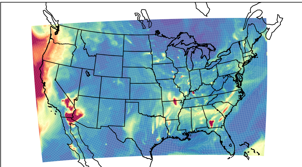
WRF 2023-10-11_08:00:00
