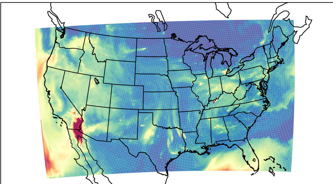
WRF 2023-10-12_14:00:00
