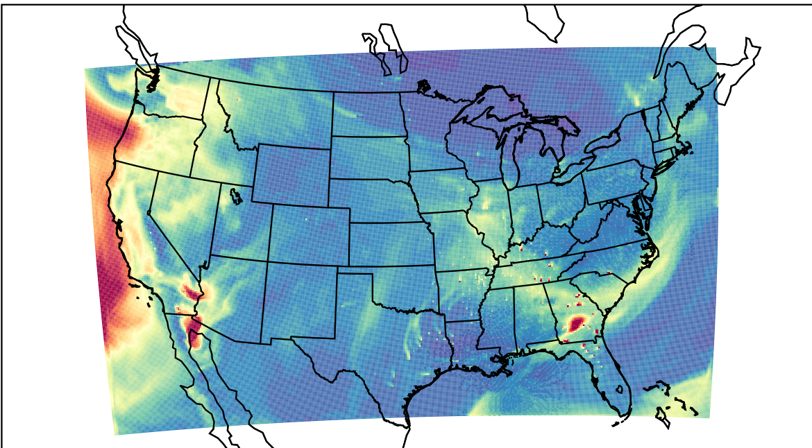
WRF 2023-10-11_19:00:00
