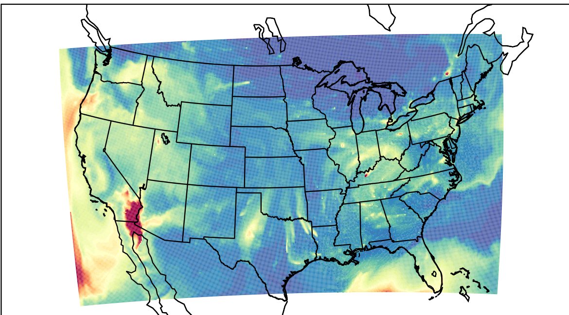
WRF 2023-10-12_12:00:00
