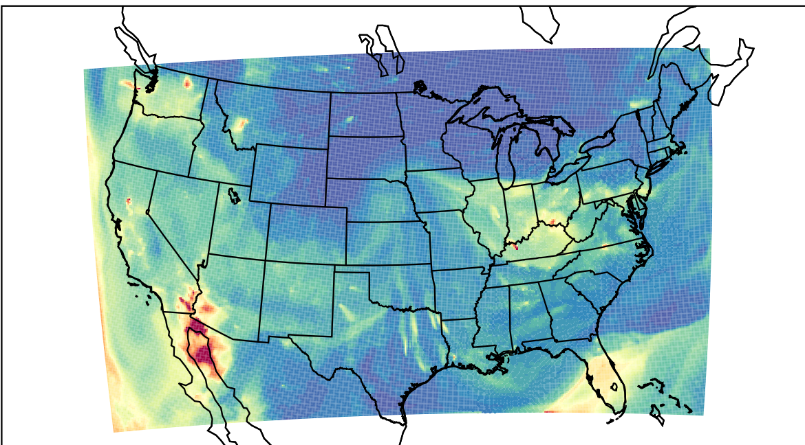
WRF 2023-10-13_05:00:00
