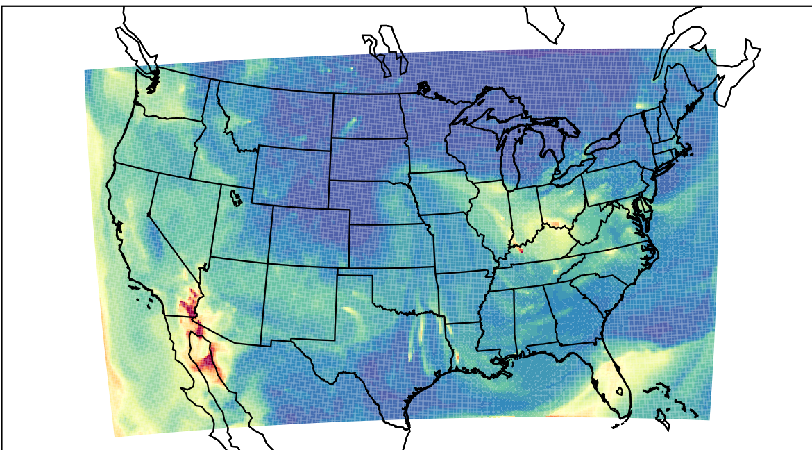
WRF 2023-10-13_09:00:00
