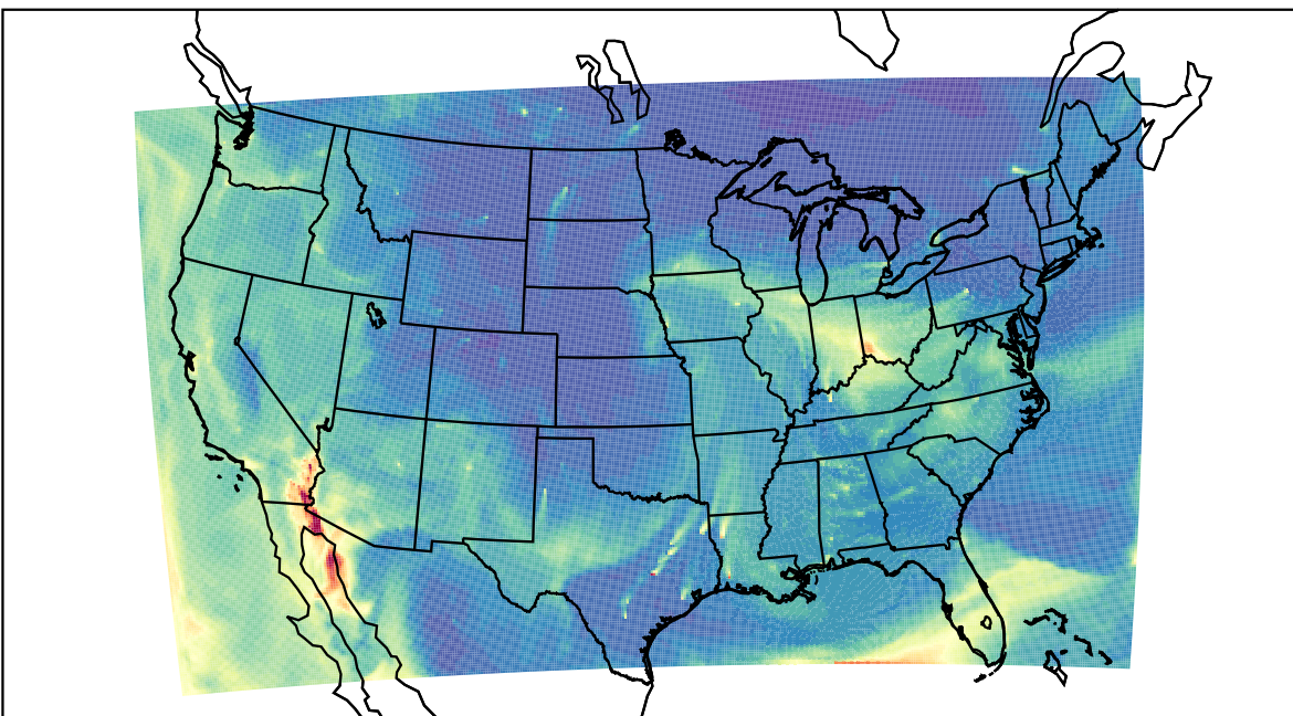
WRF 2023-10-13_16:00:00
