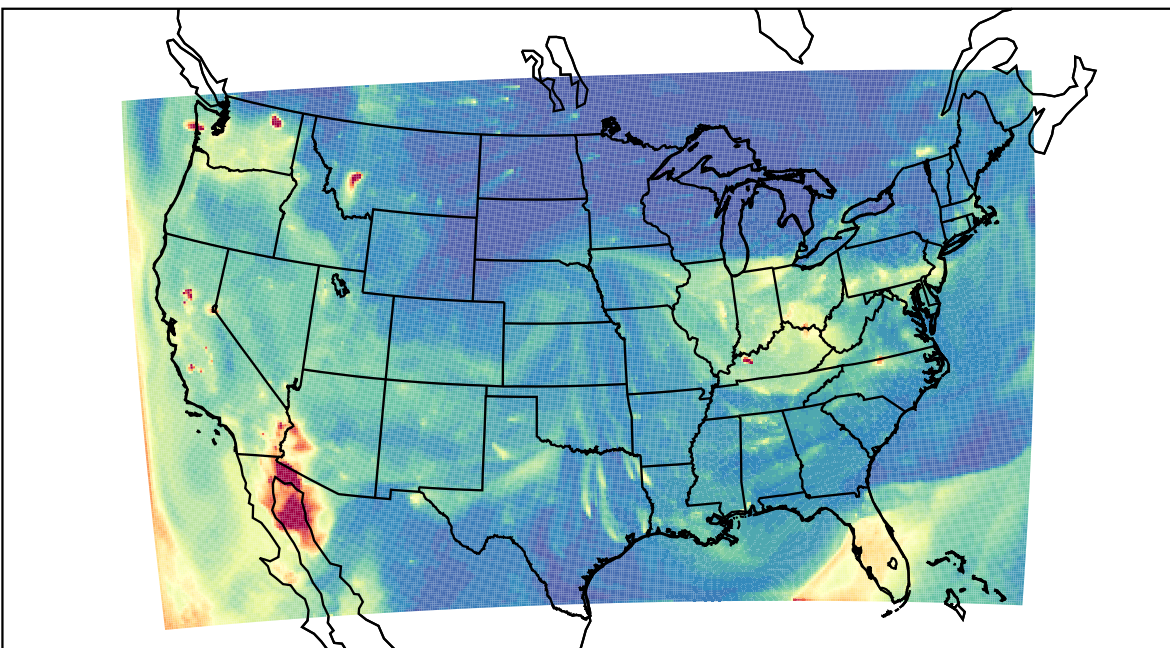
WRF 2023-10-13_03:00:00
