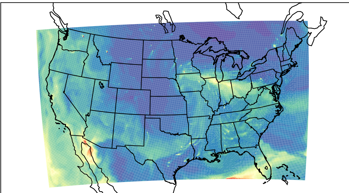
WRF 2023-10-13_21:00:00
