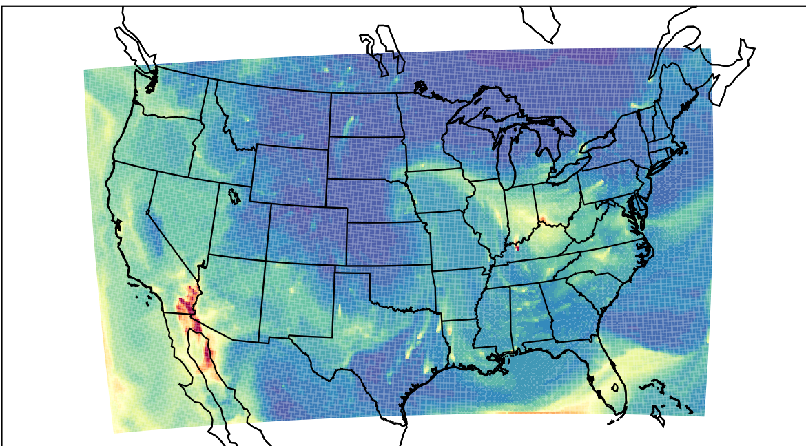
WRF 2023-10-13_14:00:00
