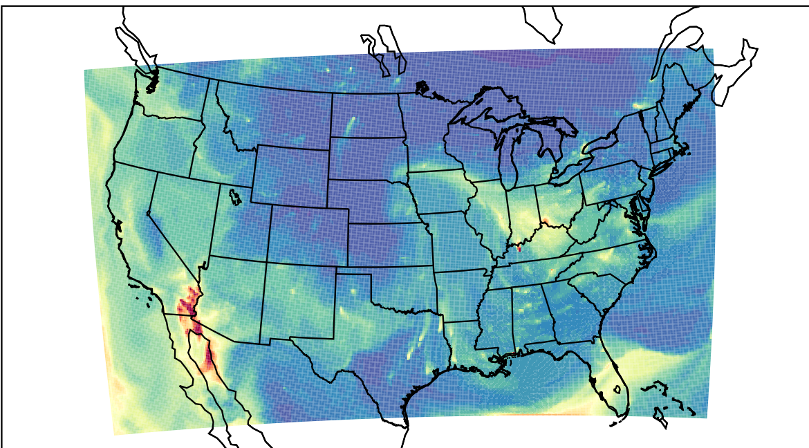
WRF 2023-10-13_13:00:00
