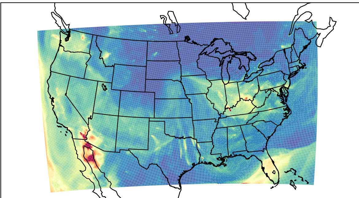
WRF 2023-10-13_06:00:00
