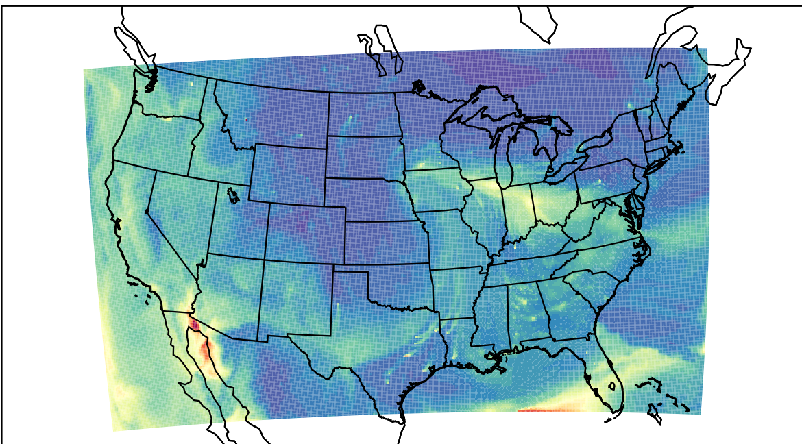
WRF 2023-10-13_19:00:00
