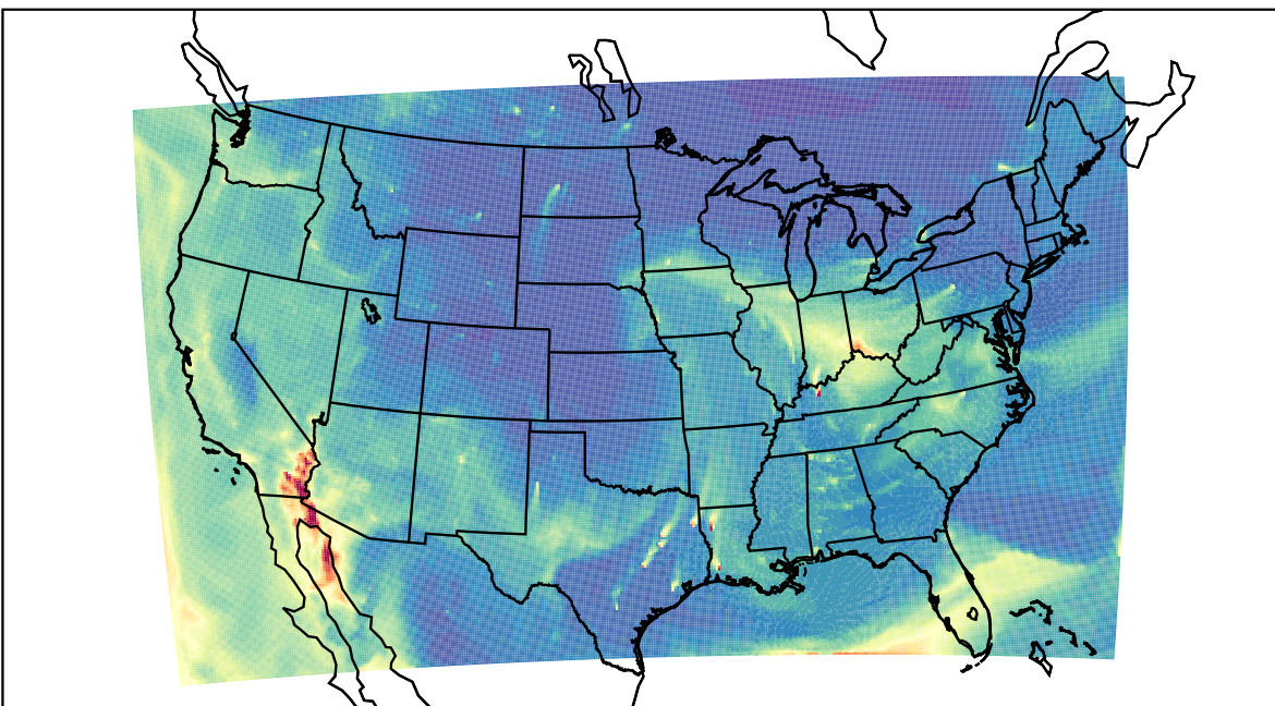
WRF 2023-10-13_15:00:00
