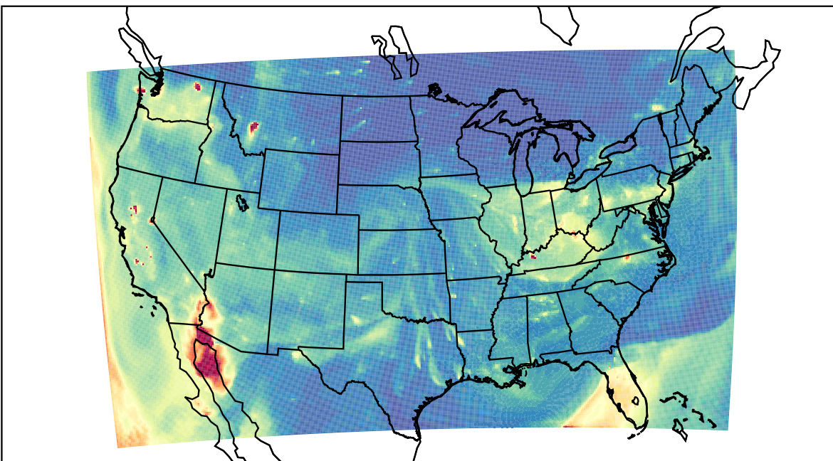
WRF 2023-10-13_02:00:00
