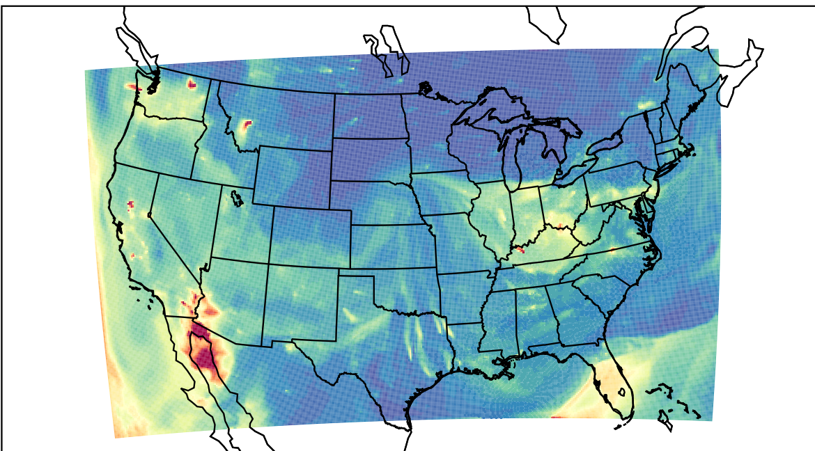
WRF 2023-10-13_04:00:00
