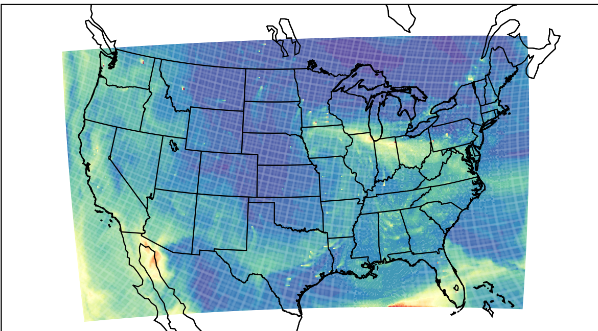
WRF 2023-10-13_22:00:00
