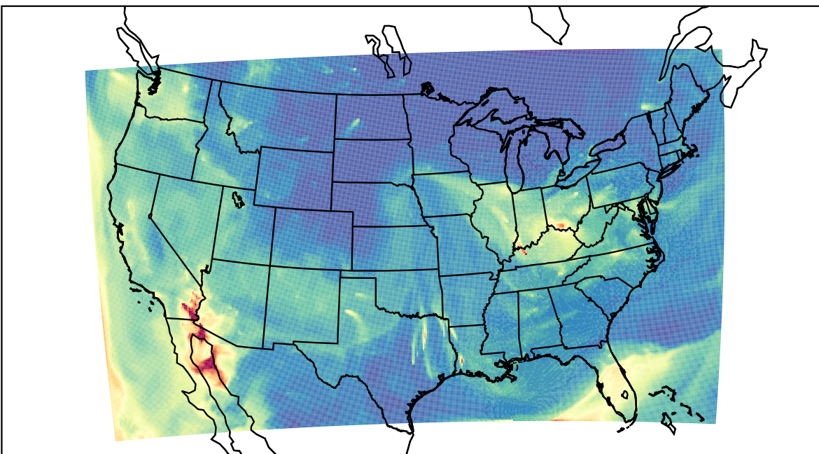
WRF 2023-10-13_08:00:00
