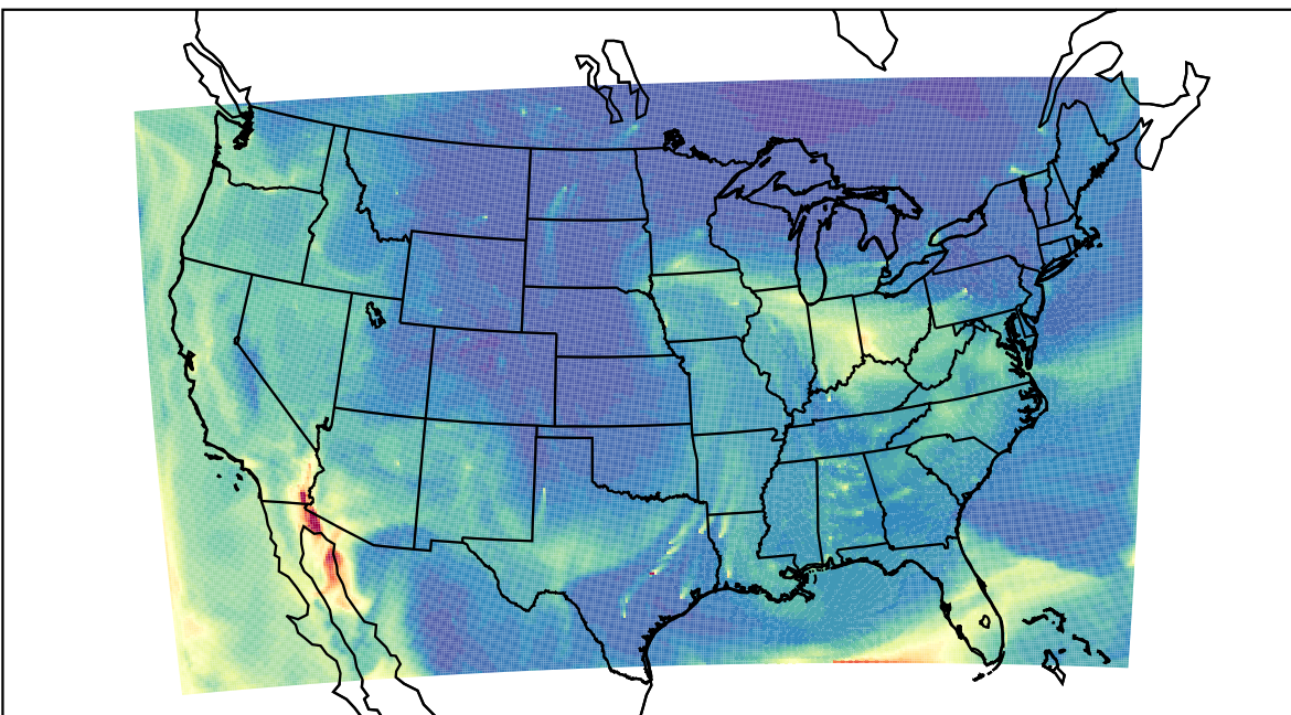
WRF 2023-10-13_17:00:00
