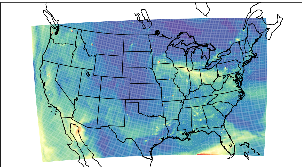
WRF 2023-10-13_23:00:00
