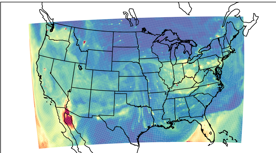
WRF 2023-10-13_00:00:00
