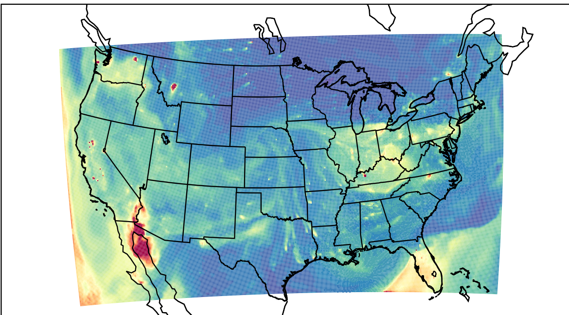
WRF 2023-10-13_01:00:00
