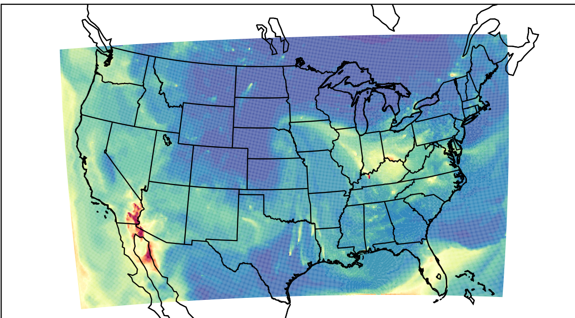
WRF 2023-10-13_11:00:00
