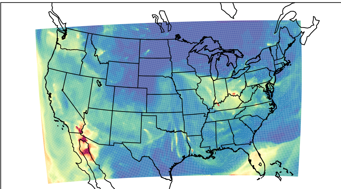
WRF 2023-10-13_07:00:00
