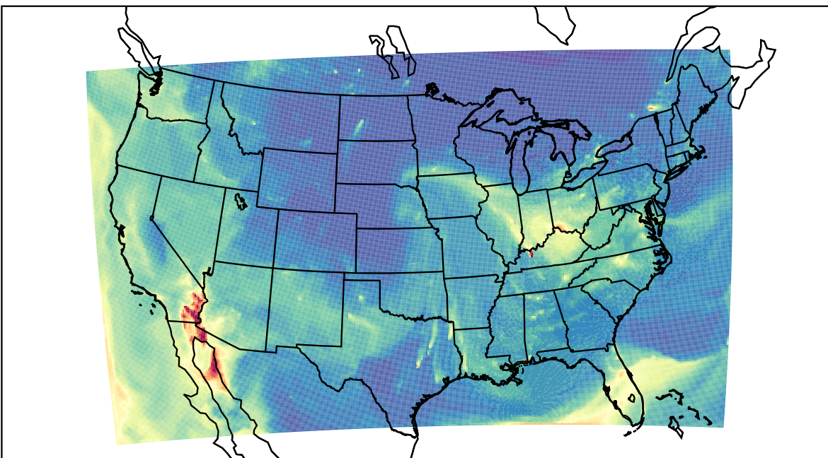
WRF 2023-10-13_12:00:00
