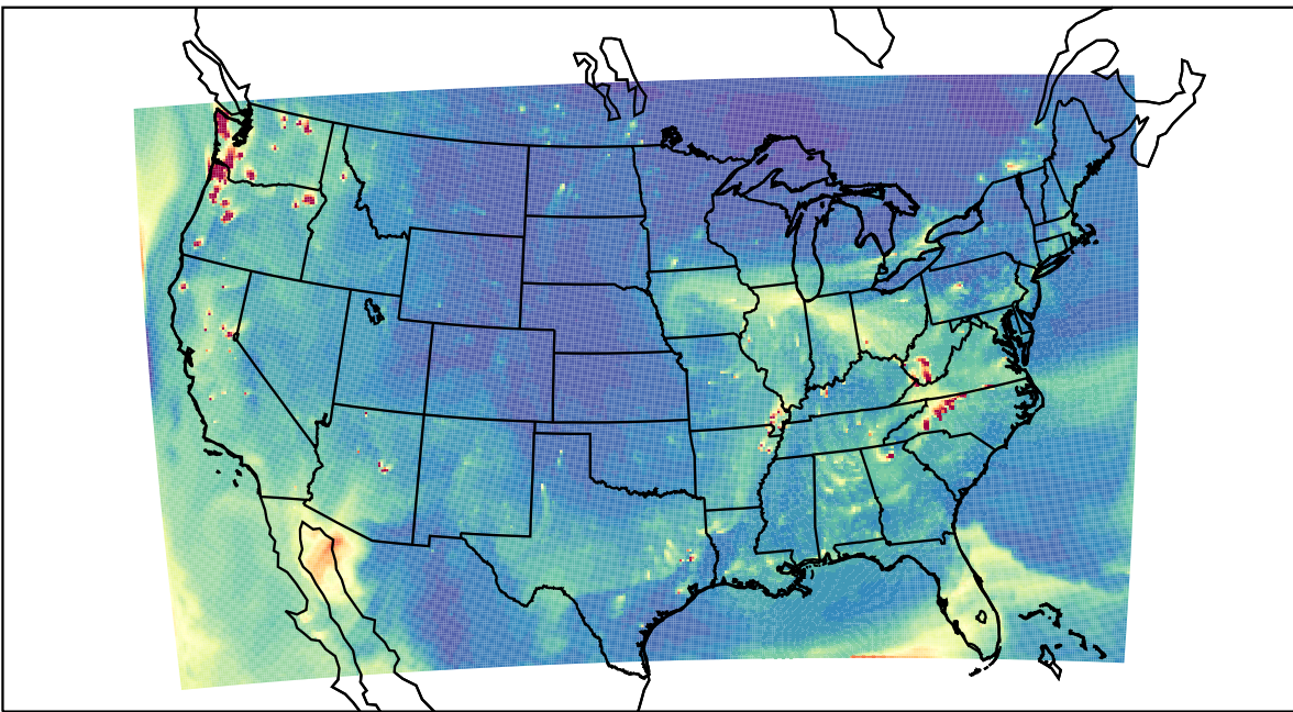
WRF 2023-10-14_00:00:00
