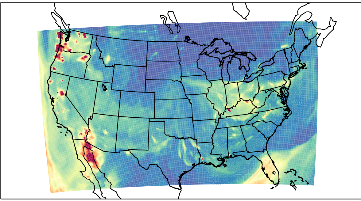
WRF 2023-10-13_04:00:00
