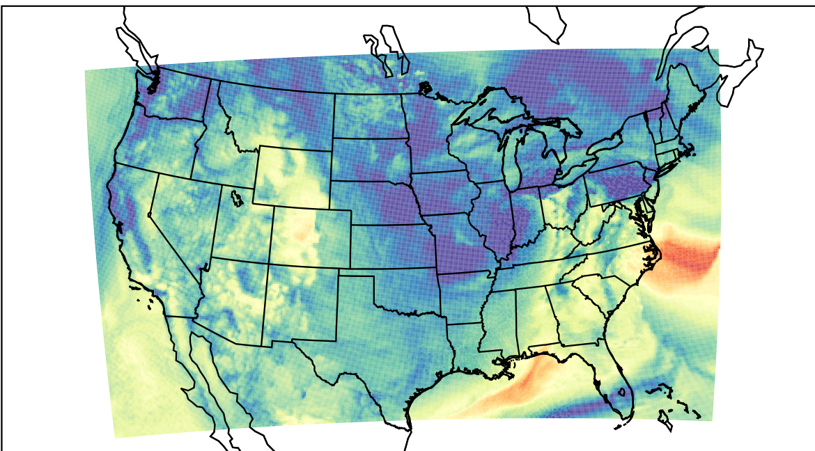
WRF (2023-10-14_16:00:00)
