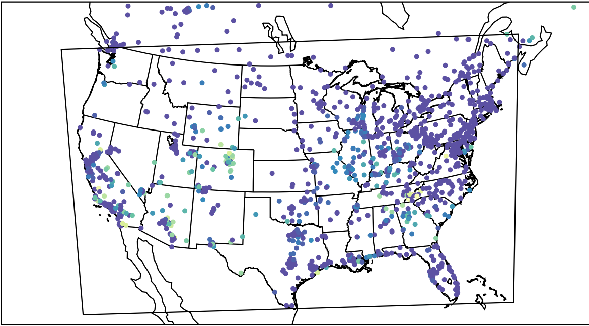
AirNOW (2023-10-13_12:00:00)
