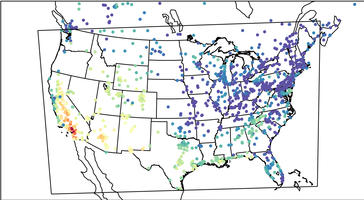
AirNOW (2023-10-14_23:00:00)
