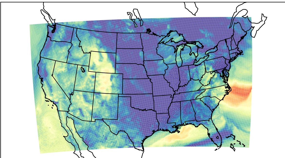
WRF (2023-10-14_13:00:00)
