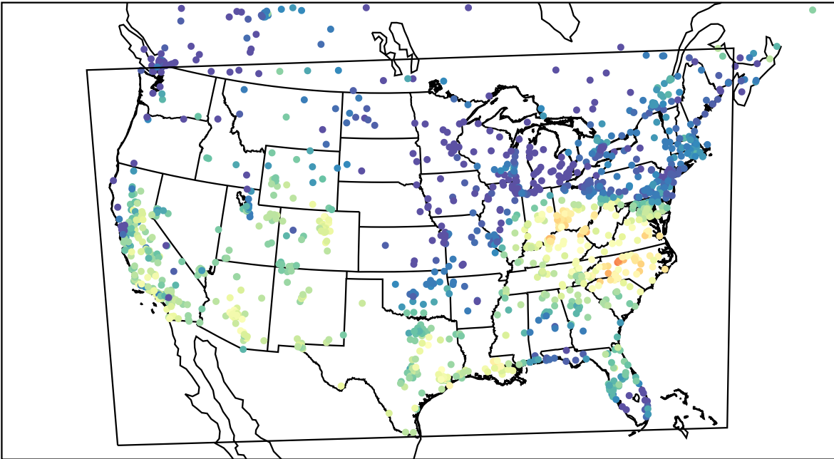
AirNOW (2023-10-13_18:00:00)
