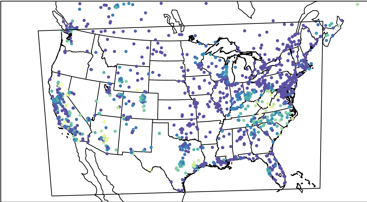
AirNOW (2023-10-14_05:00:00)
