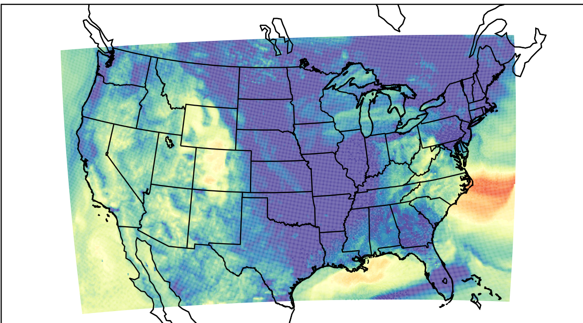
WRF (2023-10-14_11:00:00)
