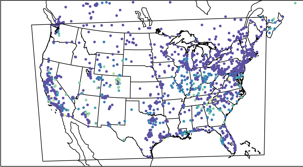
AirNOW (2023-10-13_13:00:00)
