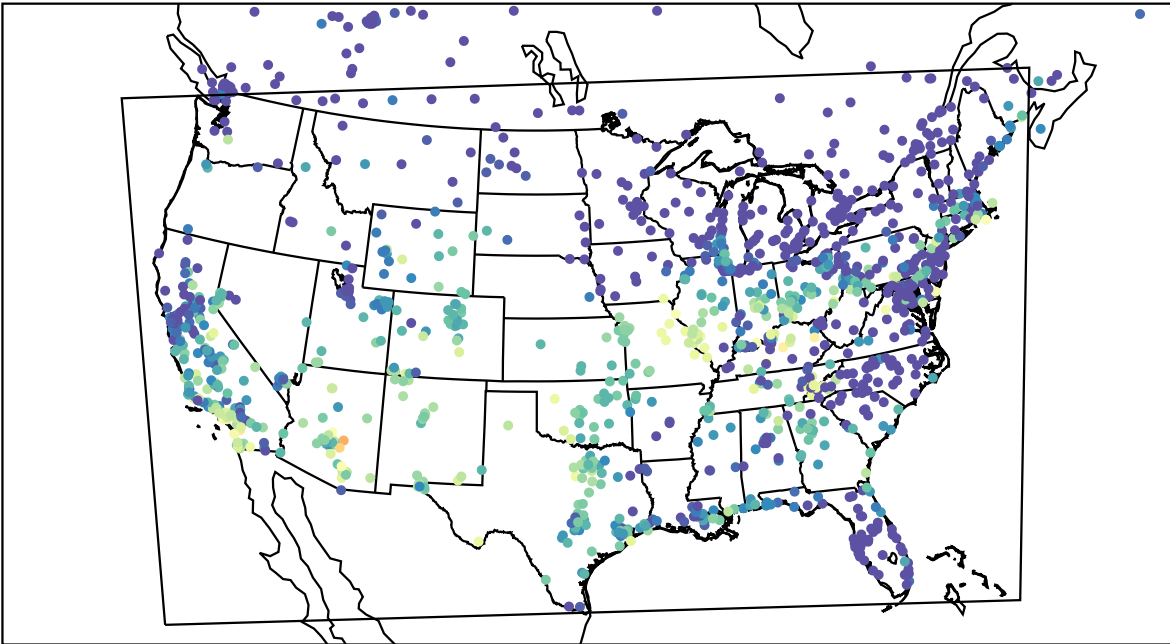
AirNOW (2023-10-13_02:00:00)
