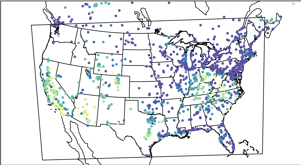
AirNOW (2023-10-14_01:00:00)
