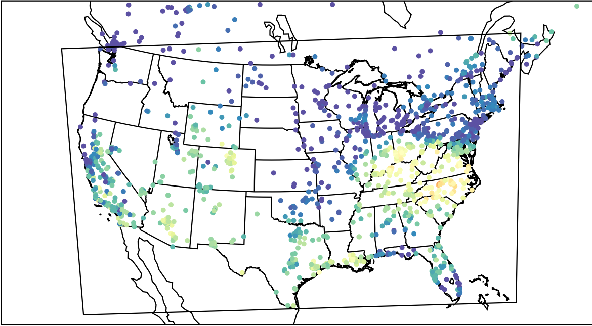
AirNOW (2023-10-13_17:00:00)
