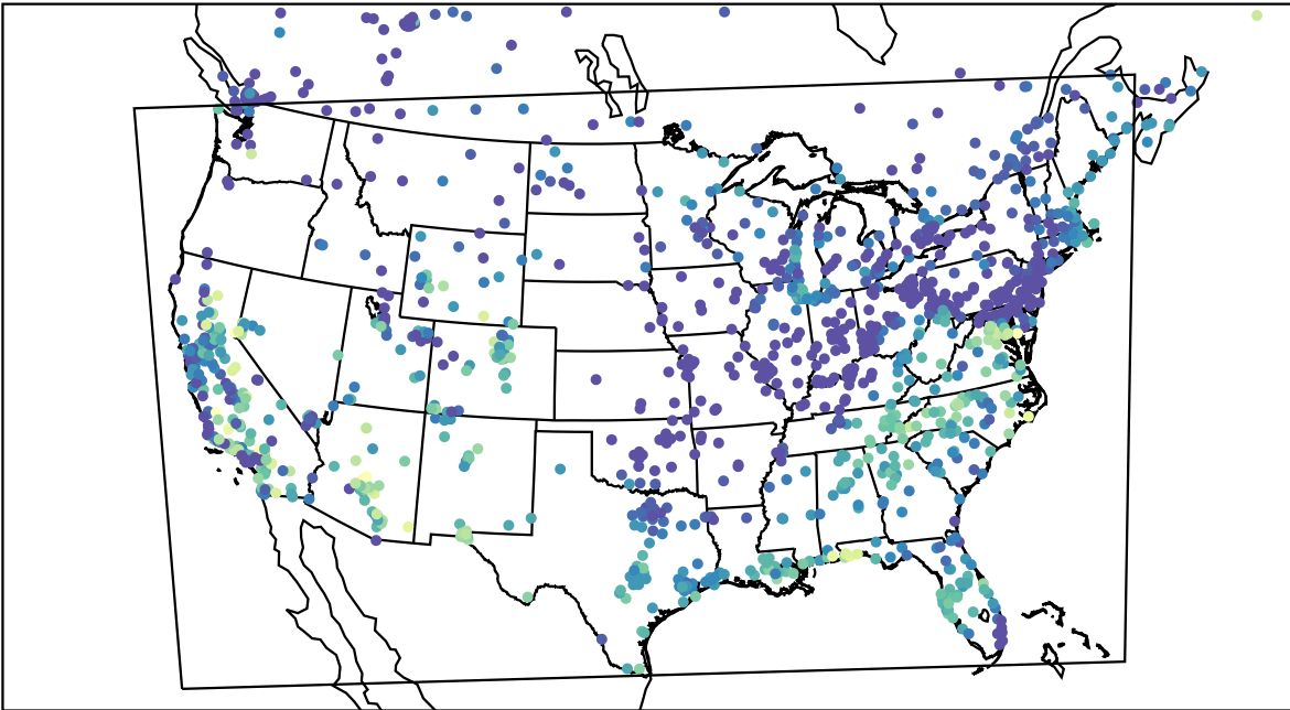
AirNOW (2023-10-14_17:00:00)
