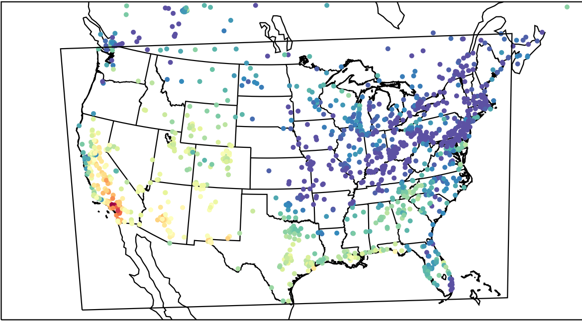
AirNOW (2023-10-14_22:00:00)
