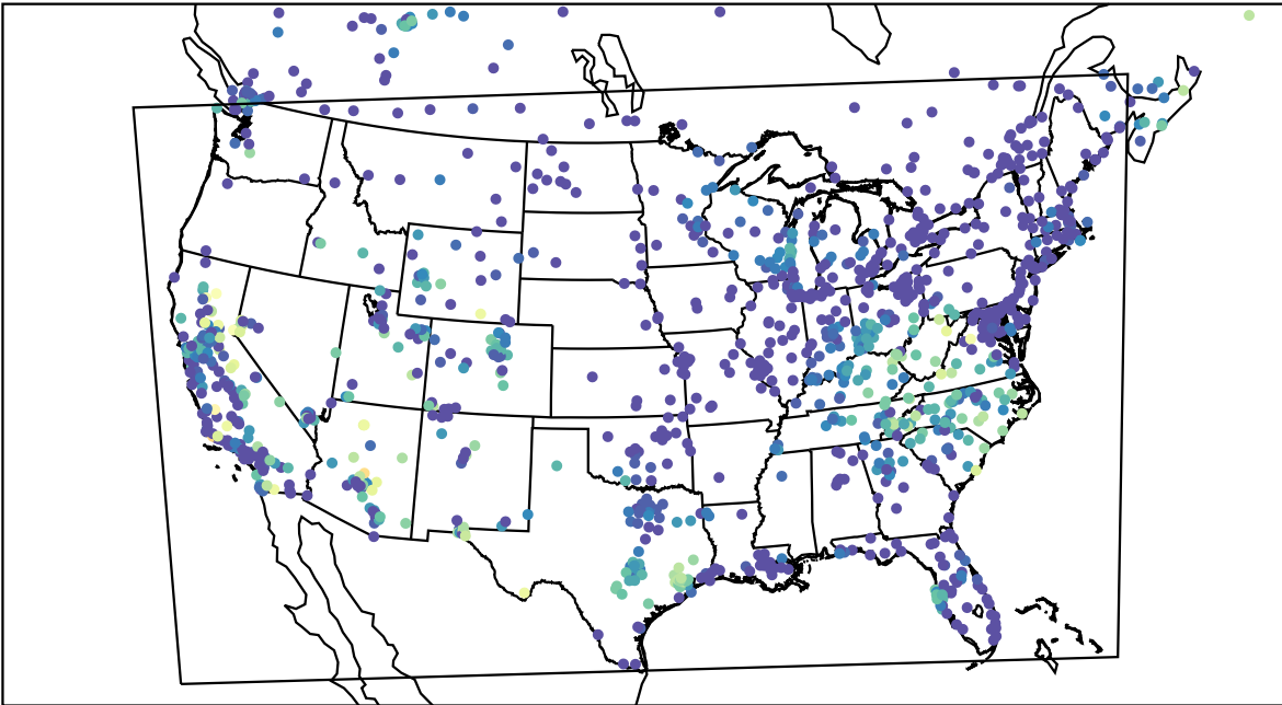
AirNOW (2023-10-14_06:00:00)
