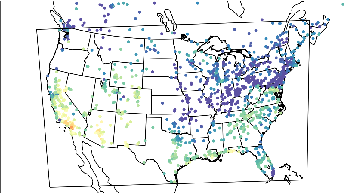
AirNOW (2023-10-14_19:00:00)
