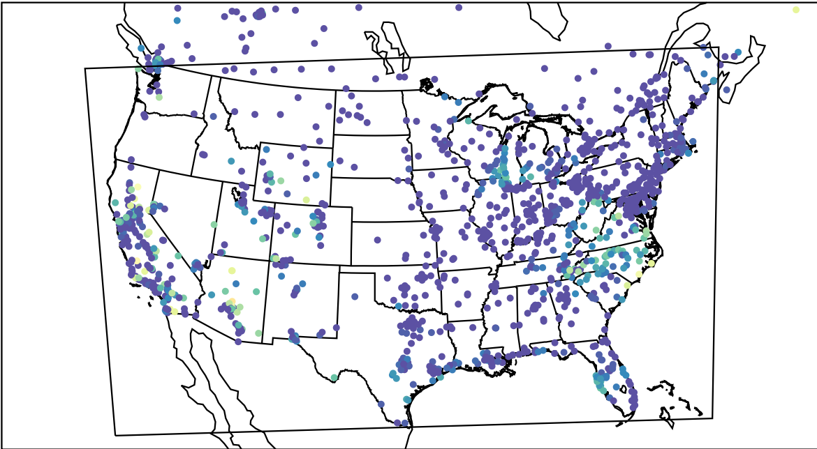
AirNOW (2023-10-14_13:00:00)
