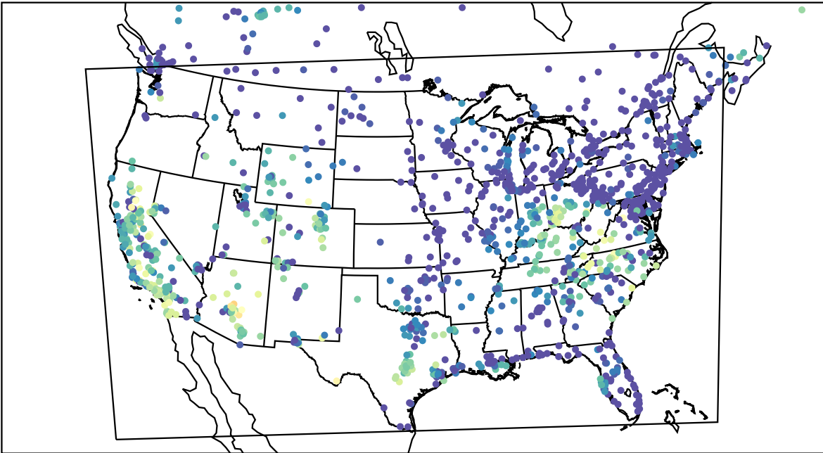
AirNOW (2023-10-14_02:00:00)
