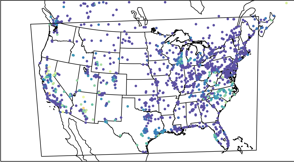
AirNOW (2023-10-14_11:00:00)
