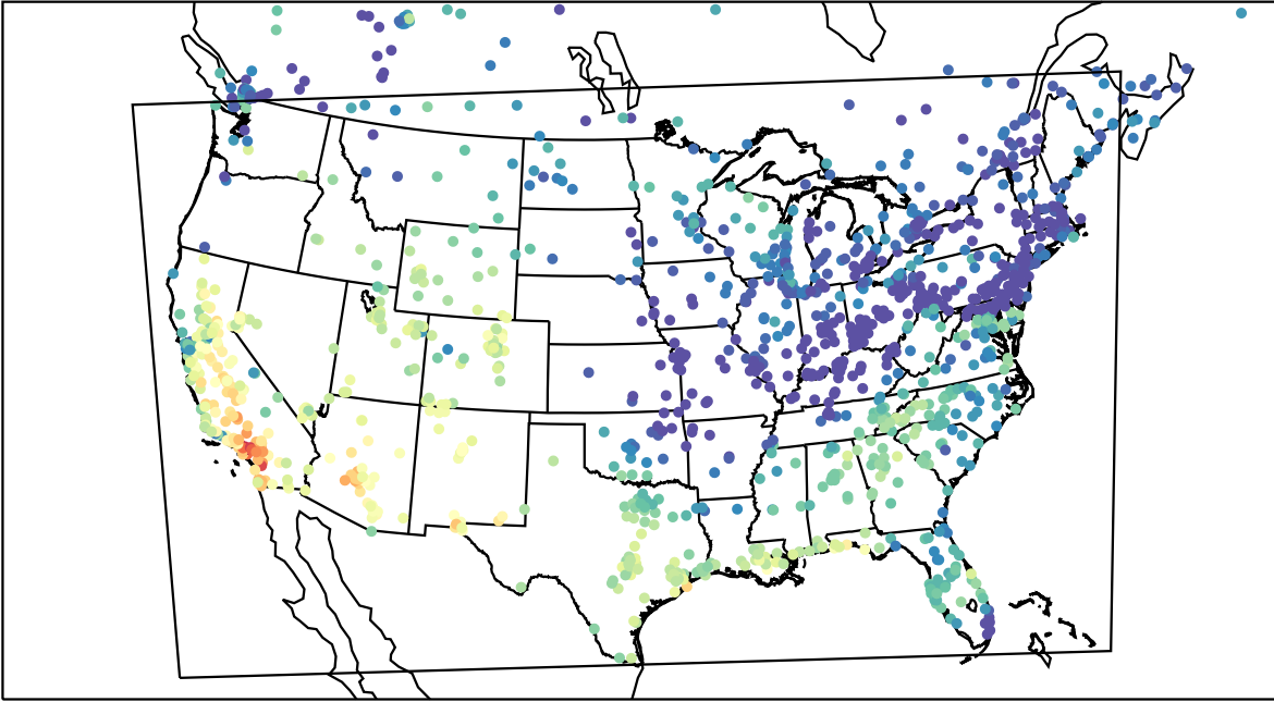
AirNOW (2023-10-14_21:00:00)
