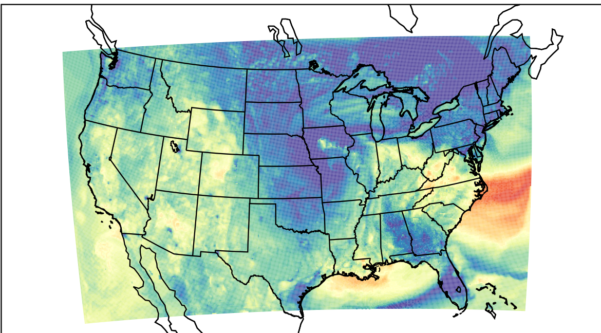
WRF (2023-10-14_02:00:00)
