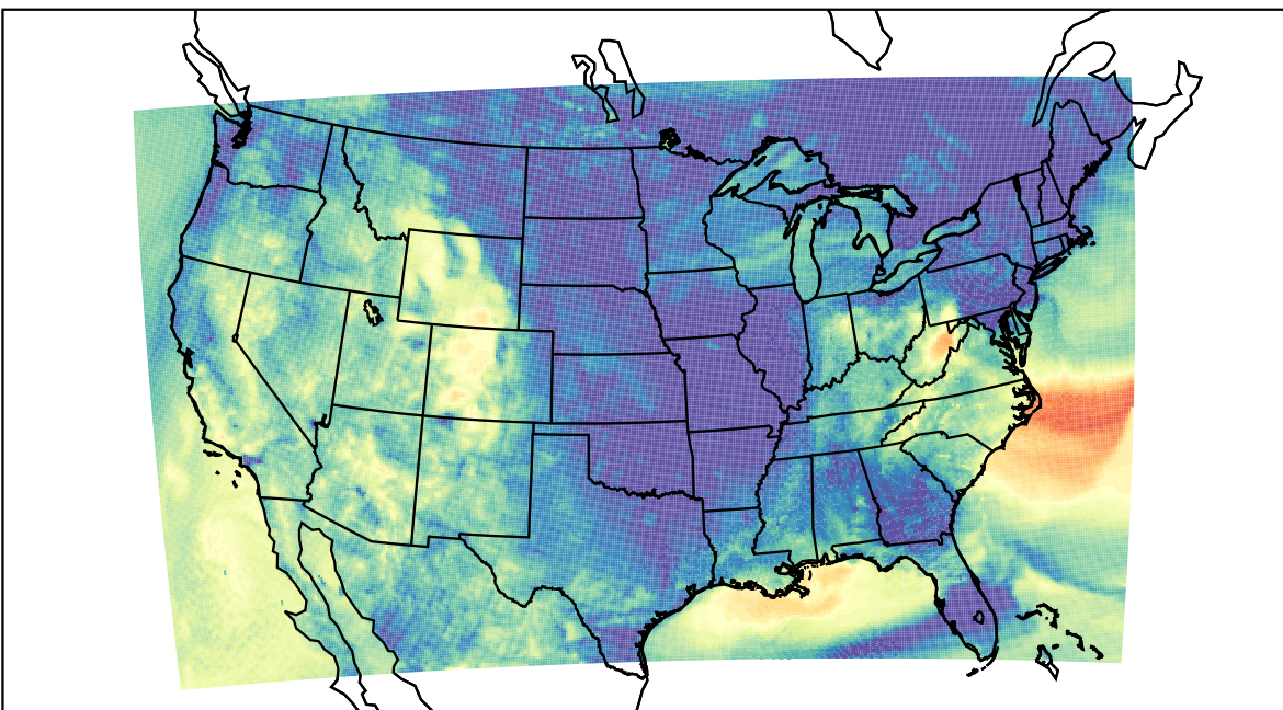
WRF (2023-10-14_08:00:00)
