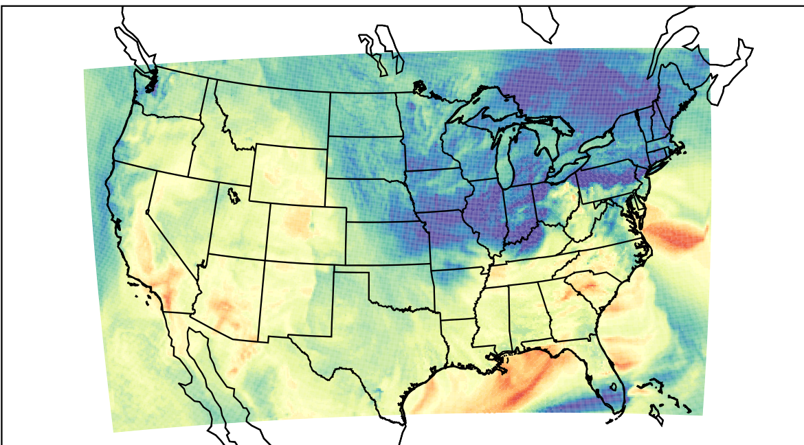
WRF (2023-10-14_22:00:00)
