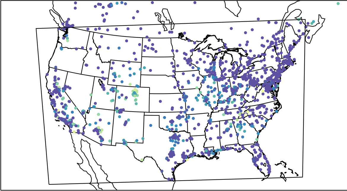
AirNOW (2023-10-13_11:00:00)
