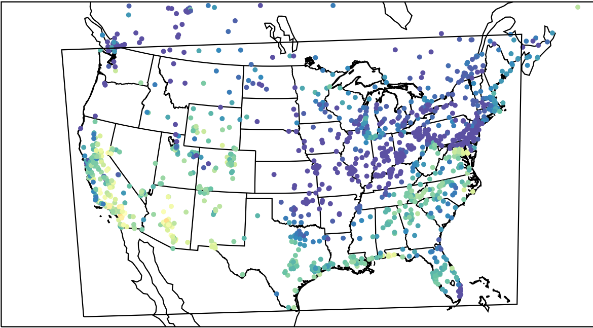
AirNOW (2023-10-14_18:00:00)
