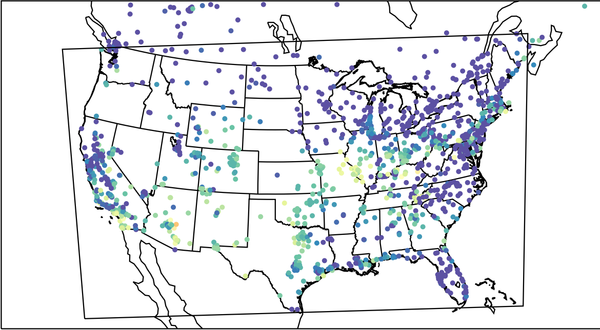
AirNOW (2023-10-13_03:00:00)
