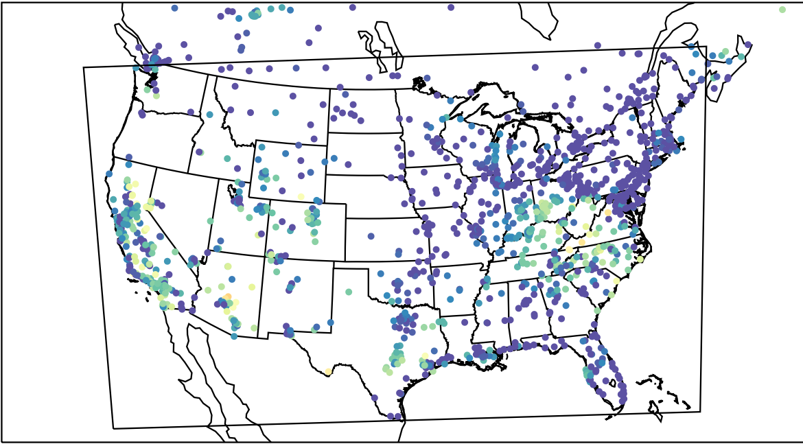
AirNOW (2023-10-14_03:00:00)
