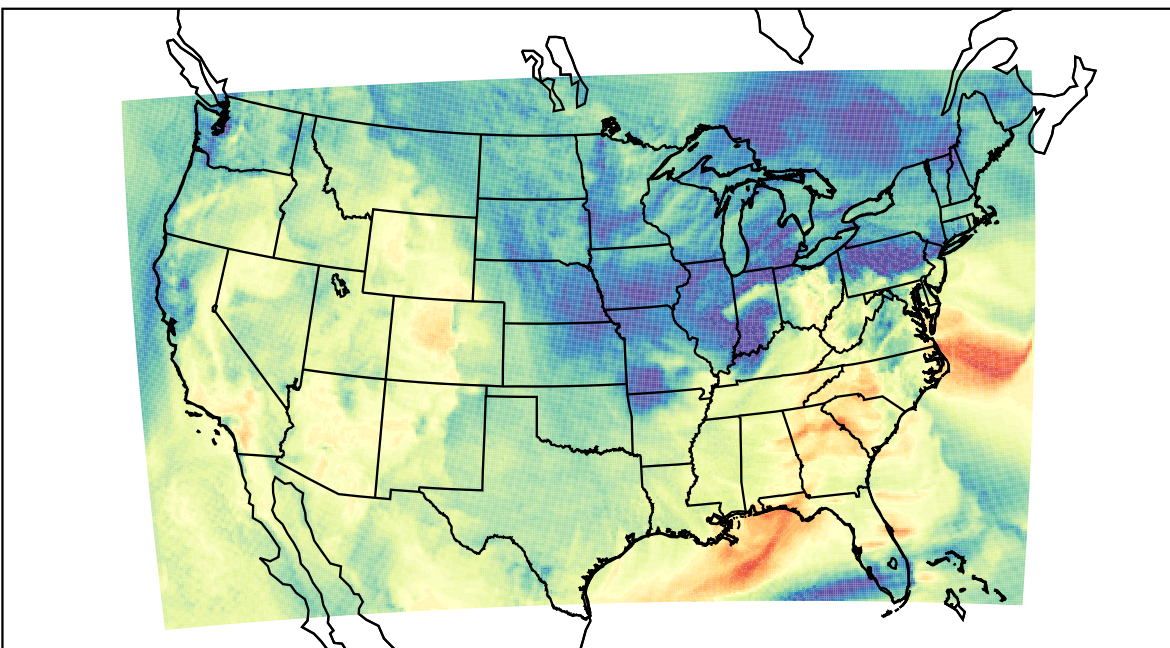
WRF (2023-10-14_19:00:00)
