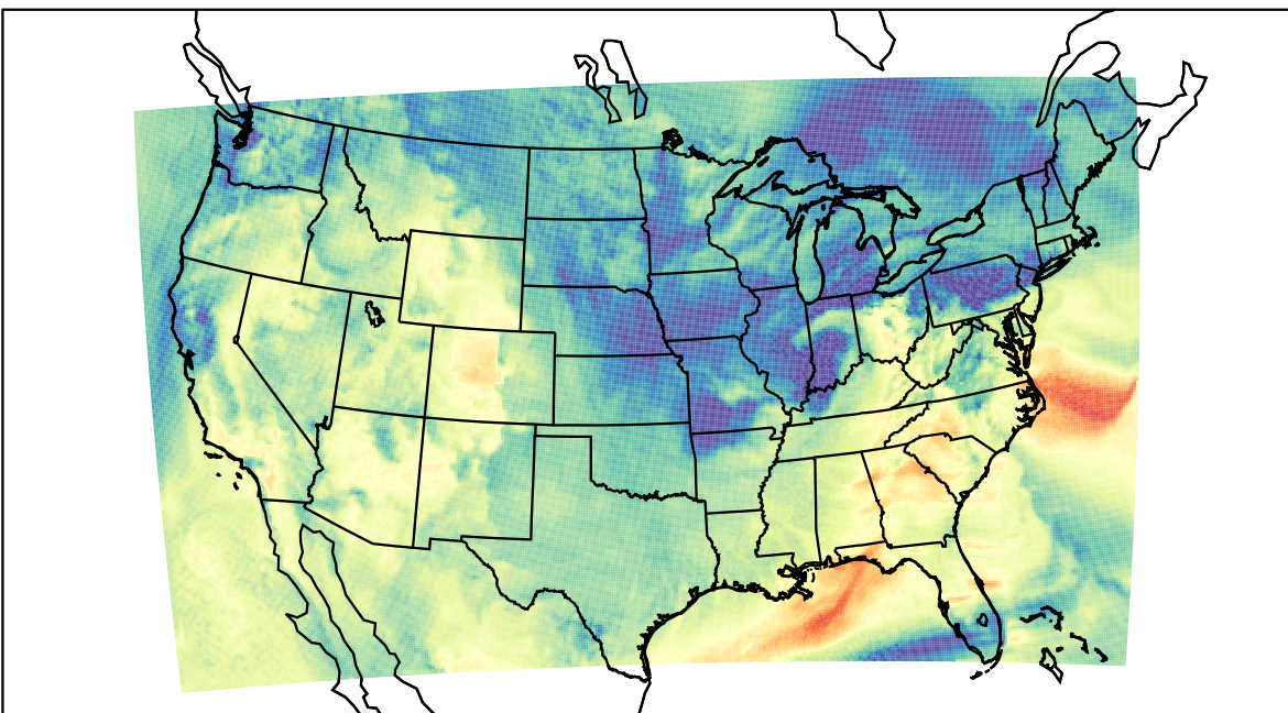
WRF (2023-10-14_18:00:00)
