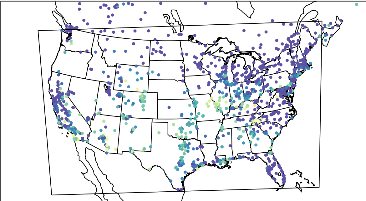
AirNOW (2023-10-13_06:00:00)
