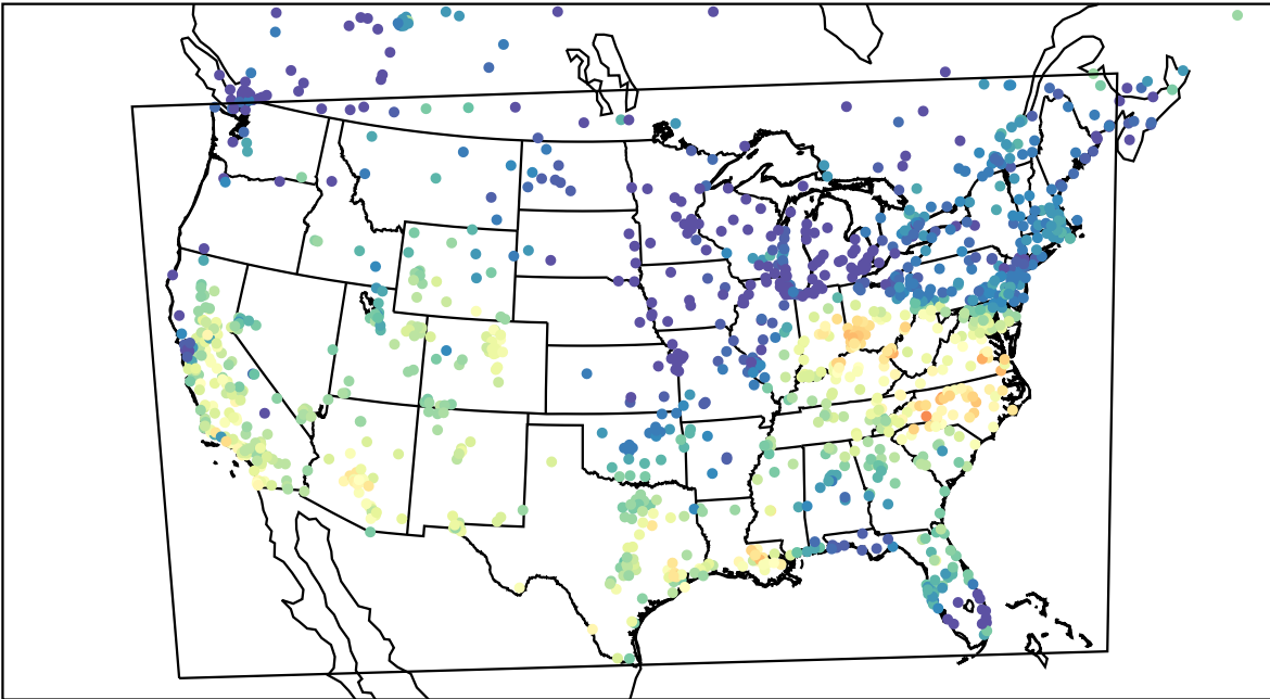
AirNOW (2023-10-13_19:00:00)
