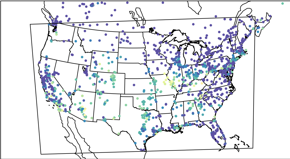
AirNOW (2023-10-13_05:00:00)
