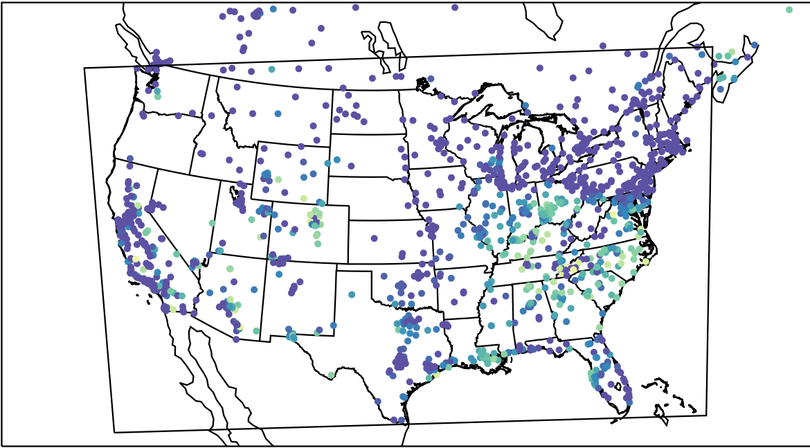
AirNOW (2023-10-13_14:00:00)
