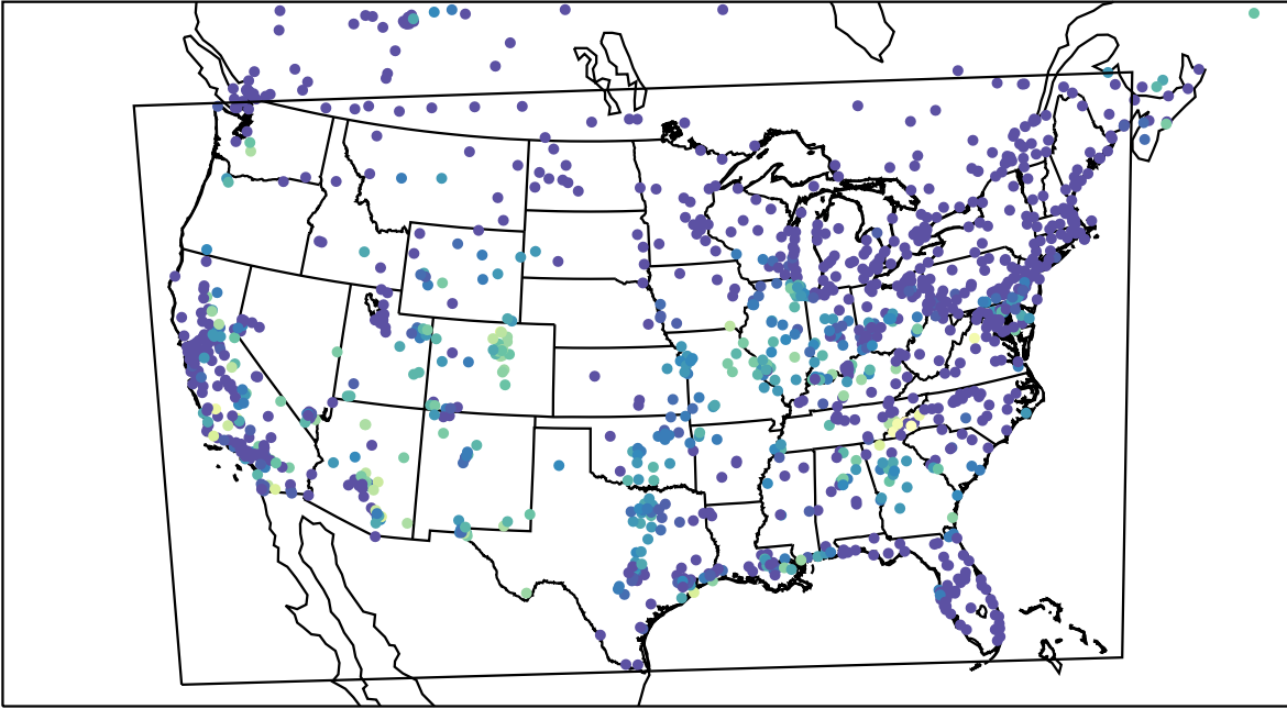
AirNOW (2023-10-13_09:00:00)
