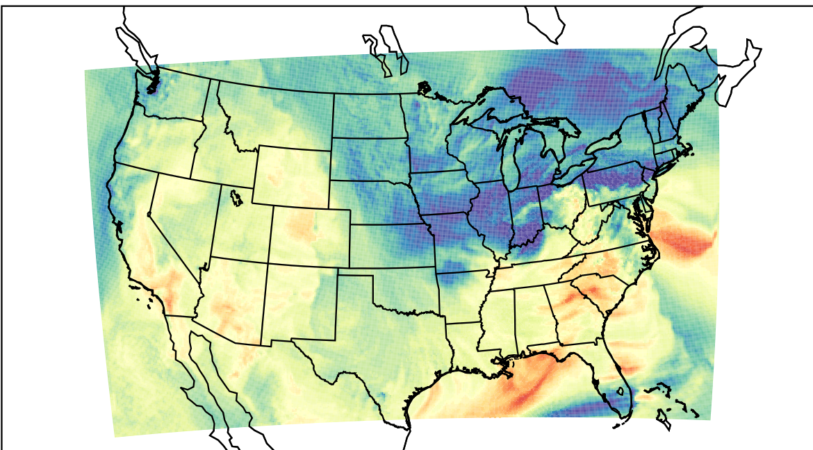
WRF (2023-10-14_21:00:00)
