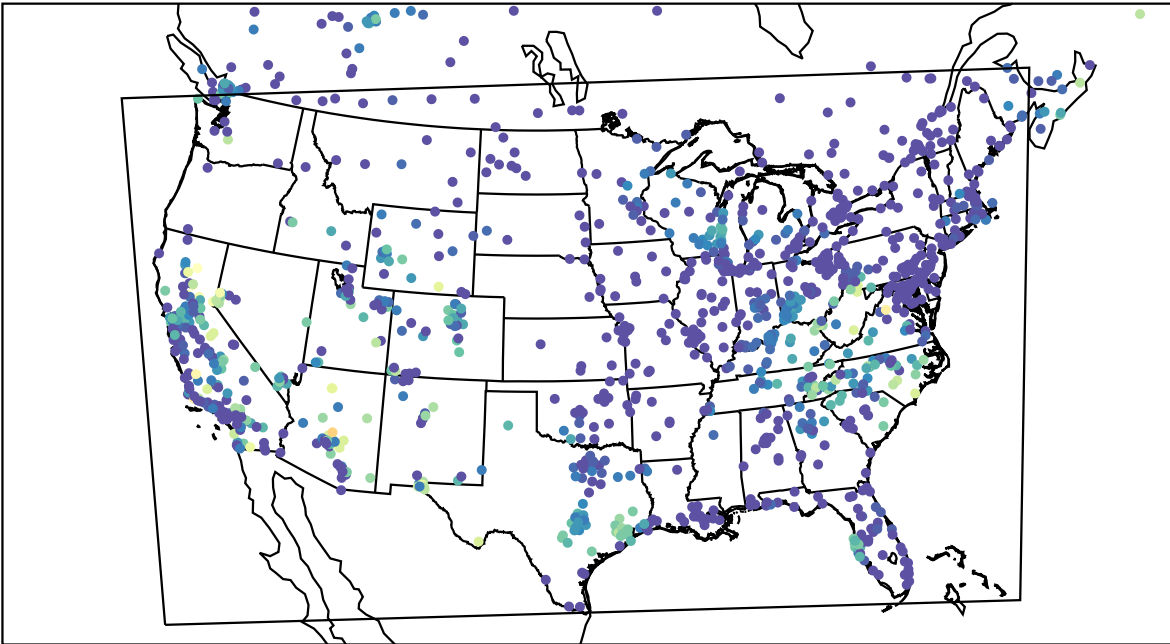
AirNOW (2023-10-14_07:00:00)
