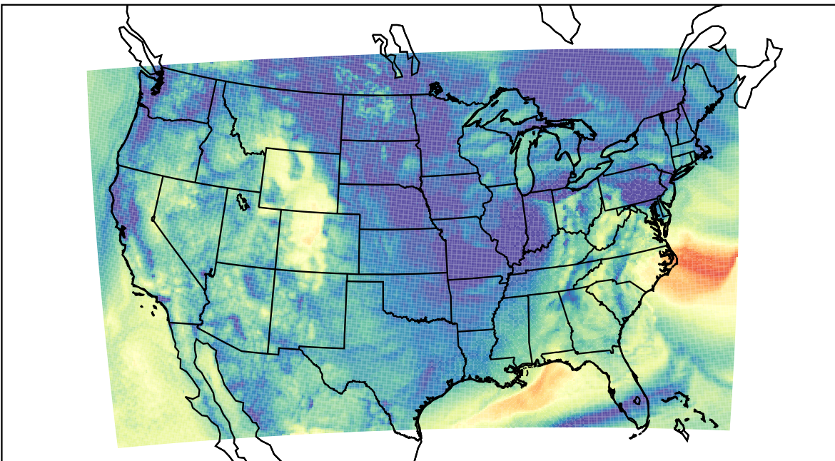
WRF (2023-10-14_15:00:00)
