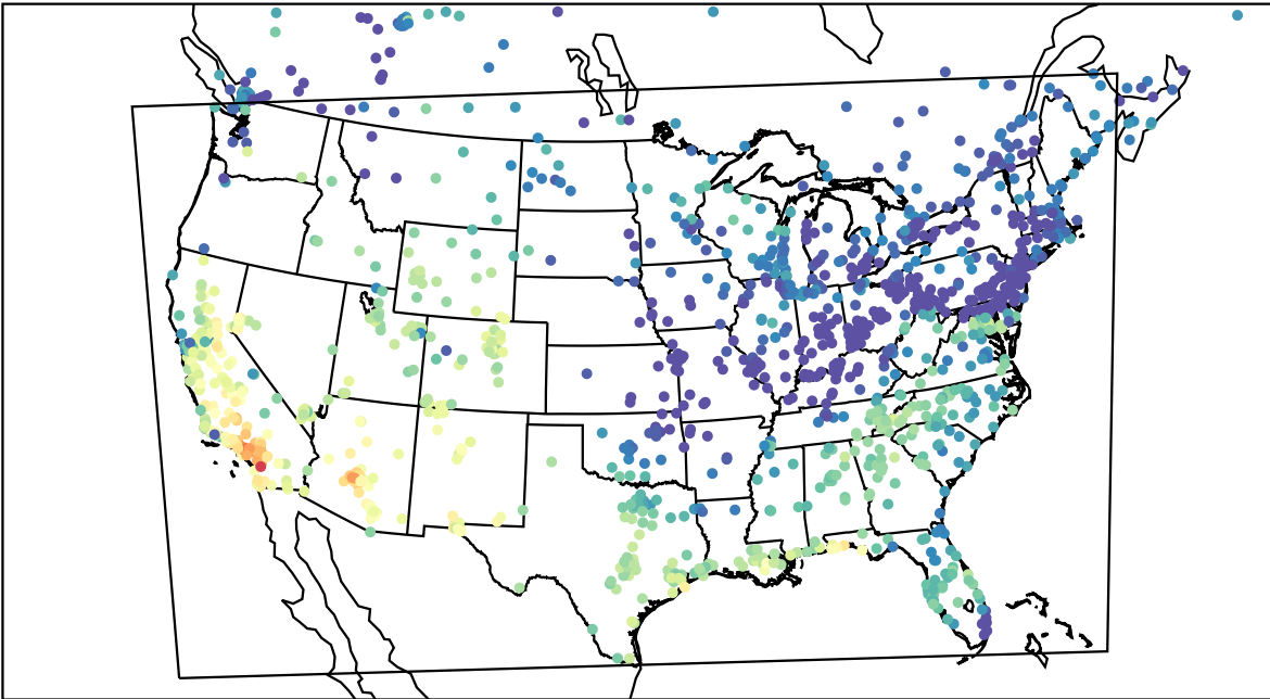
AirNOW (2023-10-14_20:00:00)
