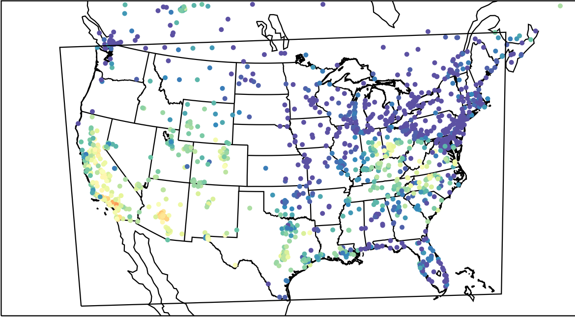
AirNOW (2023-10-14_00:00:00)
