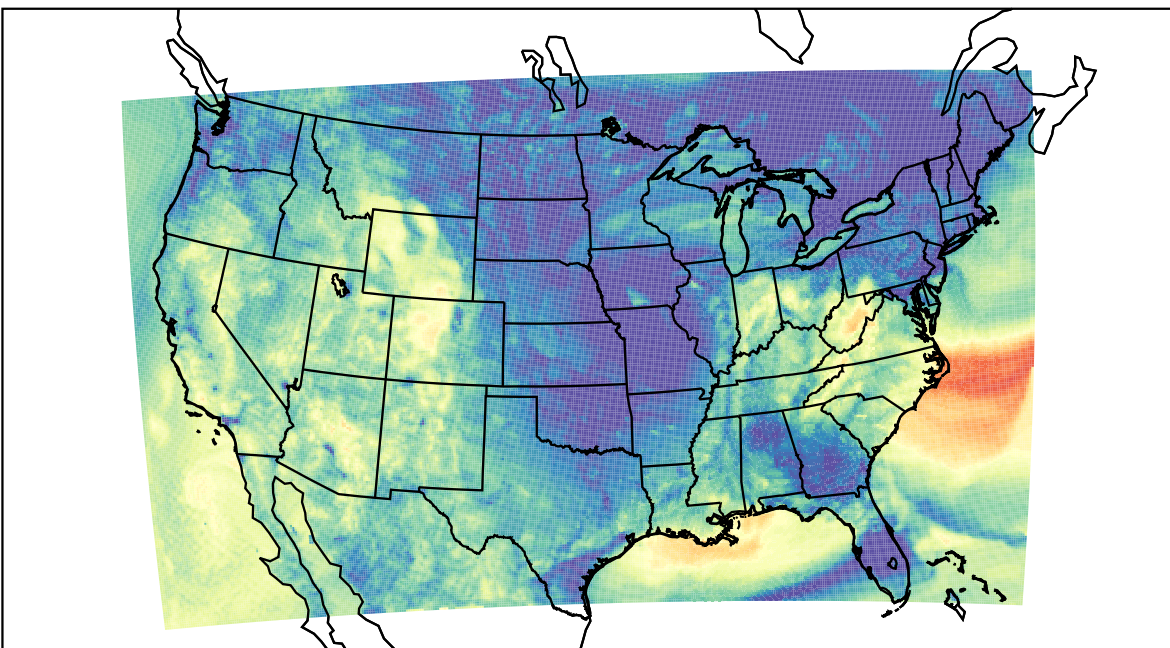
WRF (2023-10-14_05:00:00)
