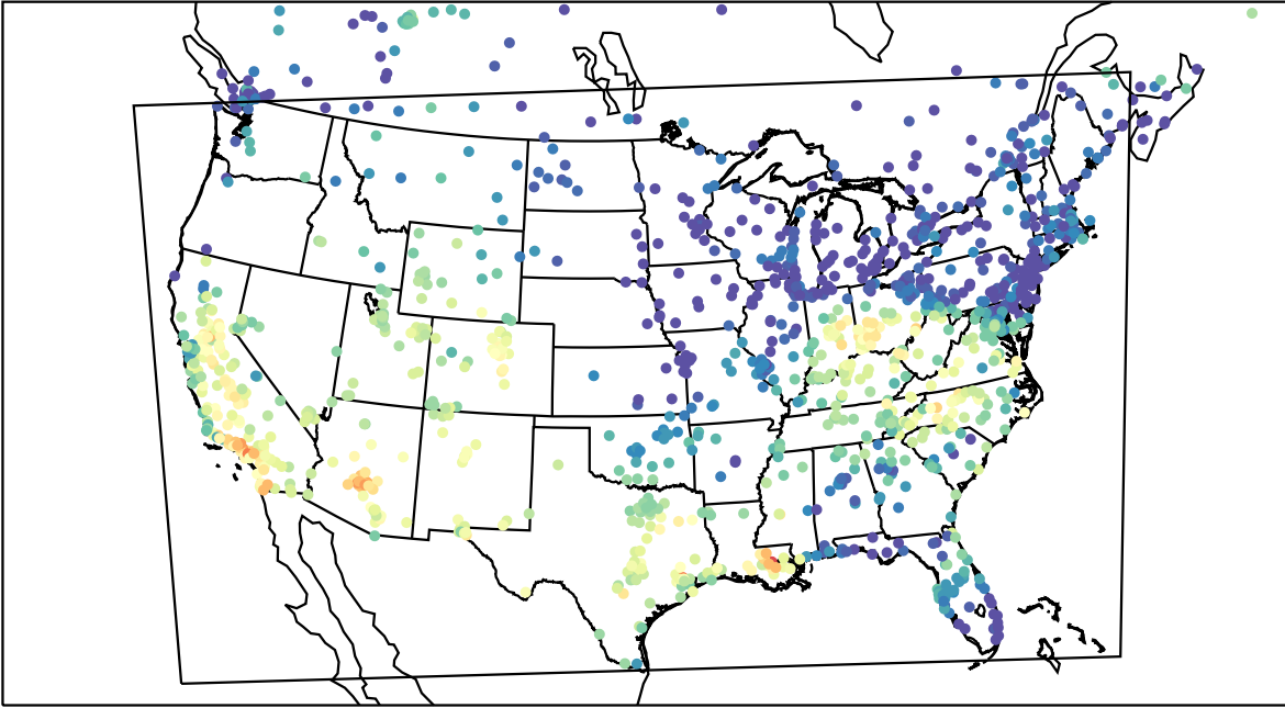
AirNOW (2023-10-13_22:00:00)
