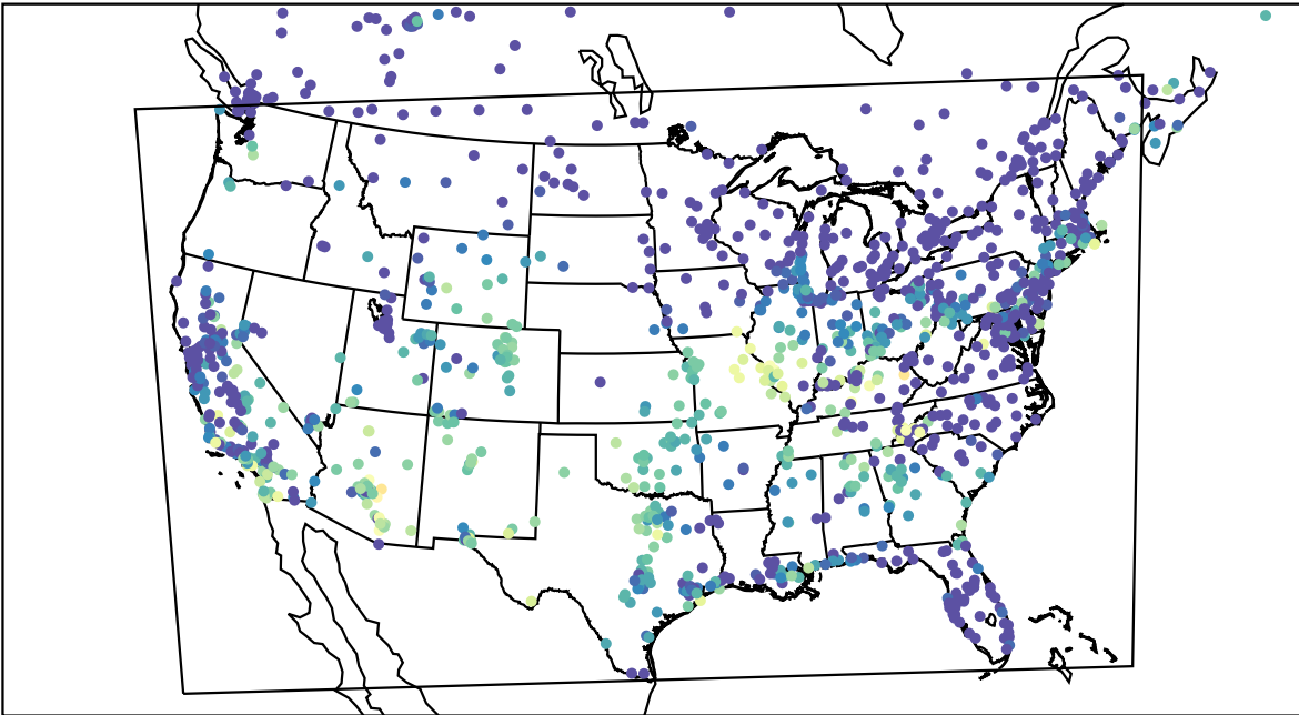
AirNOW (2023-10-13_04:00:00)
