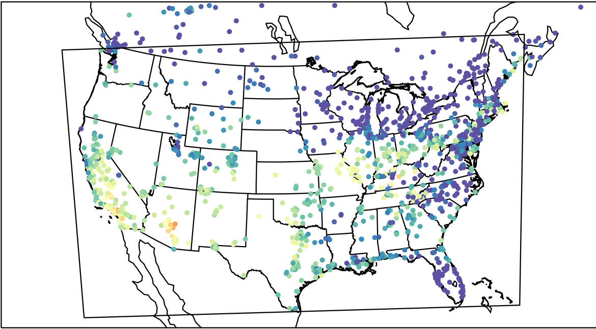
AirNOW (2023-10-13_00:00:00)
