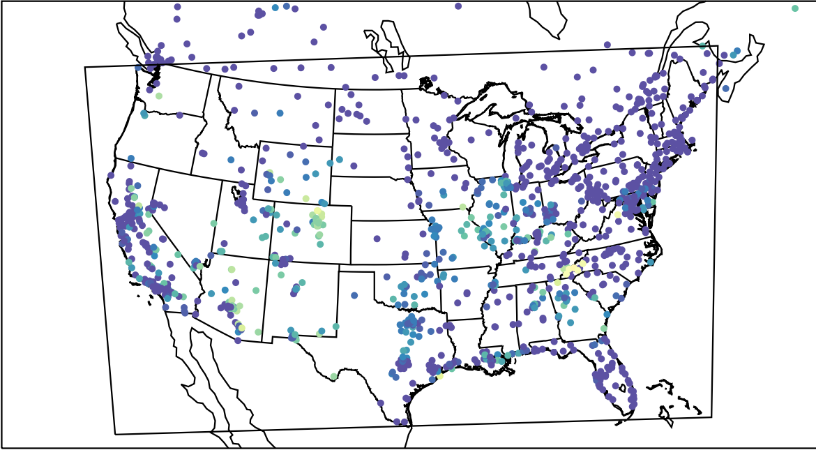
AirNOW (2023-10-13_10:00:00)
