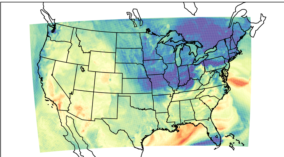
WRF (2023-10-14_23:00:00)
