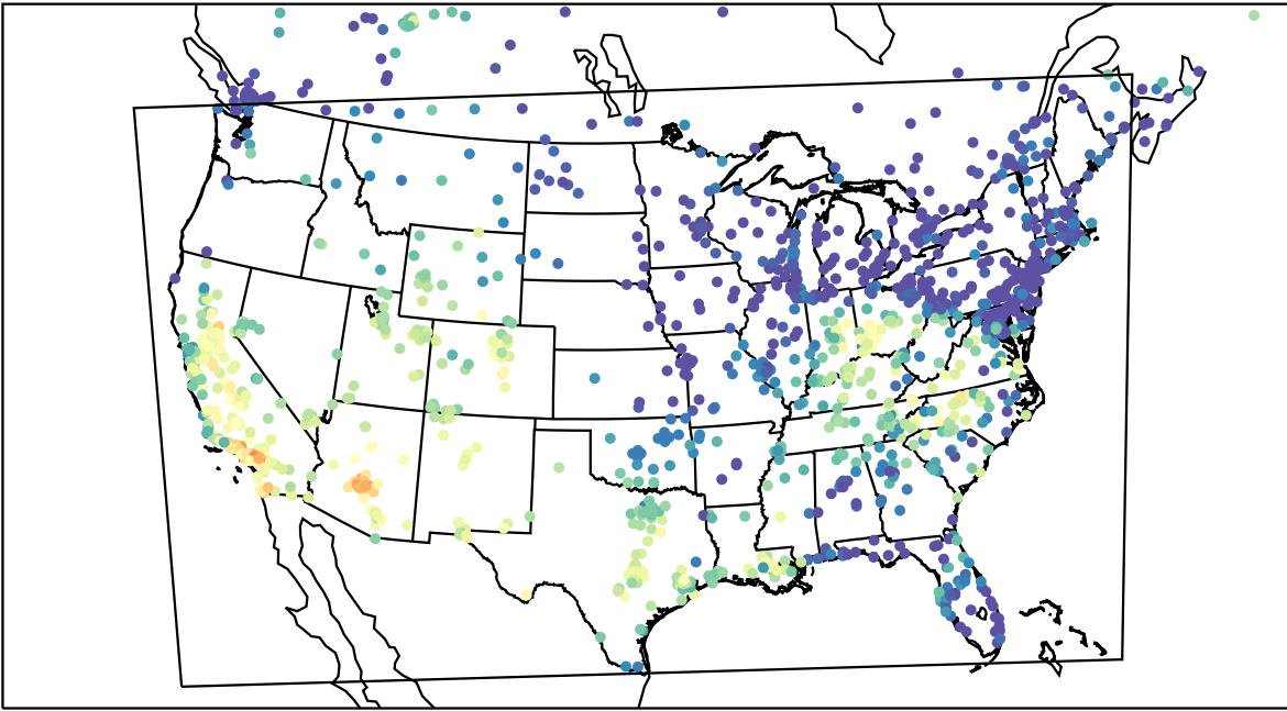
AirNOW (2023-10-13_23:00:00)
