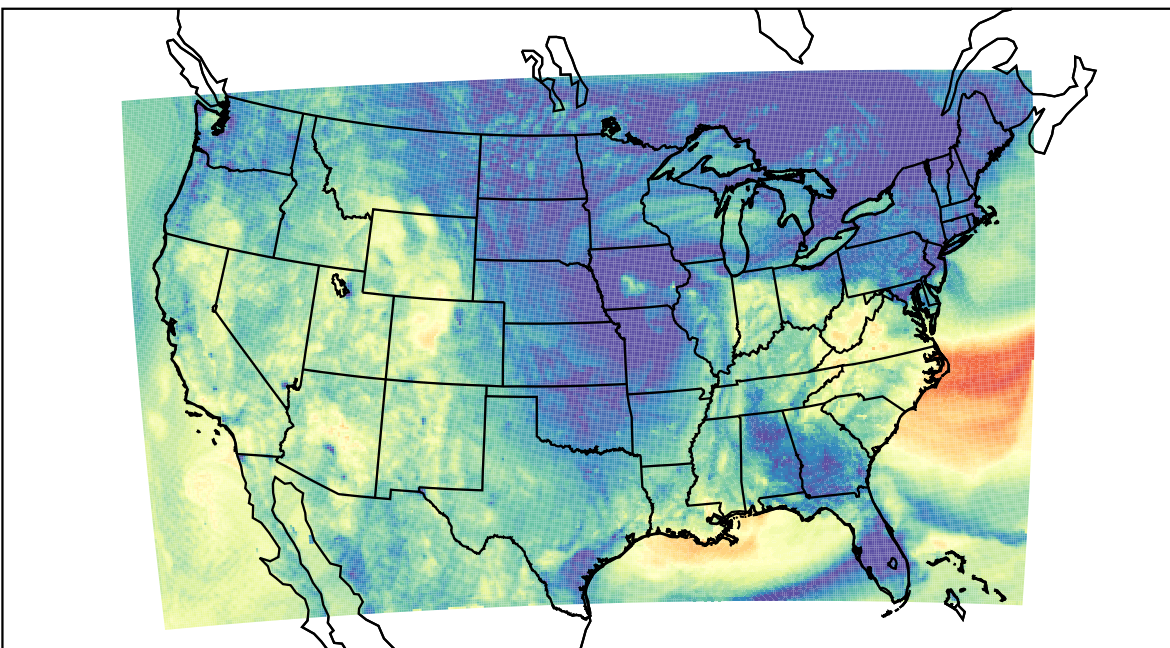
WRF (2023-10-14_03:00:00)
