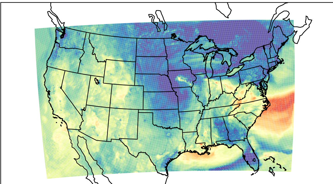
WRF (2023-10-14_01:00:00)
