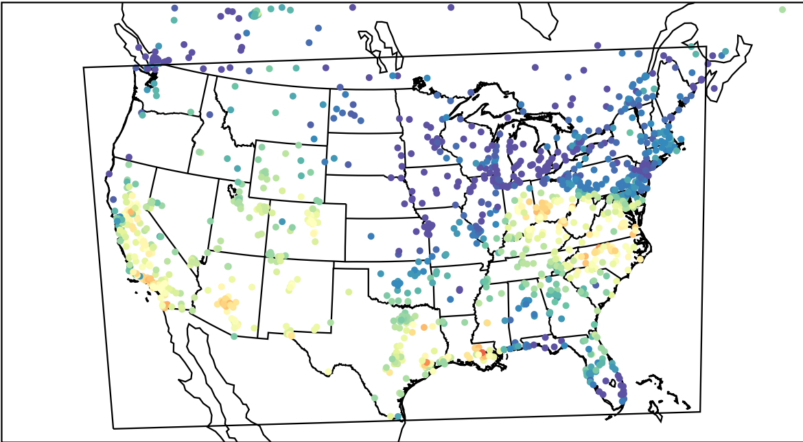
AirNOW (2023-10-13_21:00:00)
