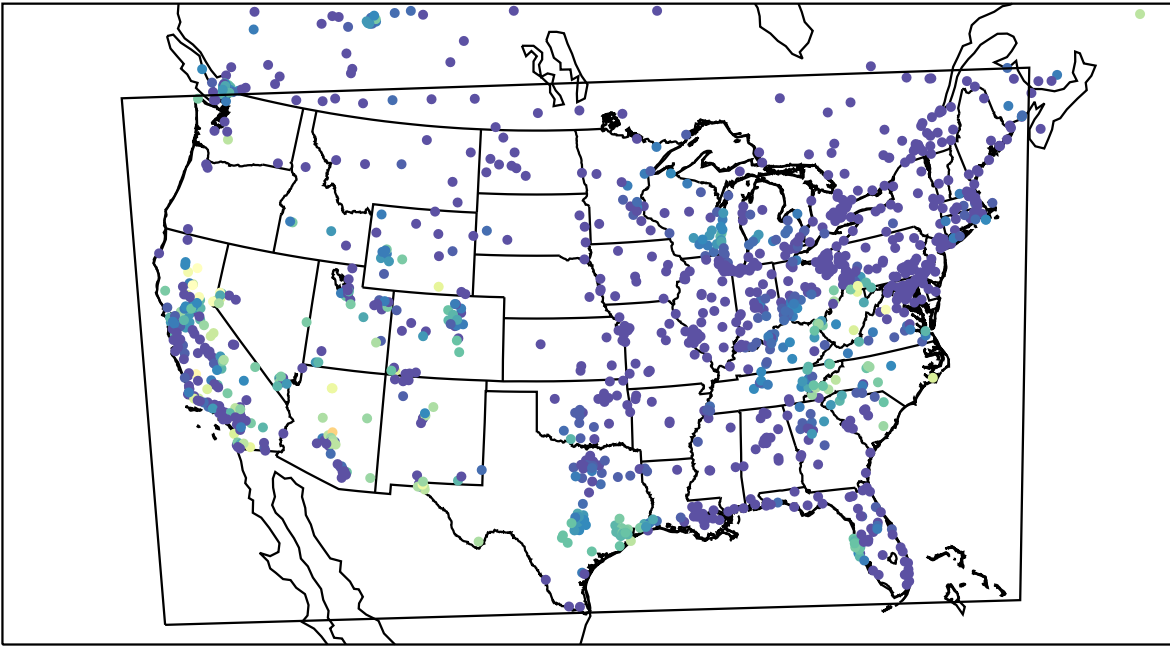
AirNOW (2023-10-14_08:00:00)
