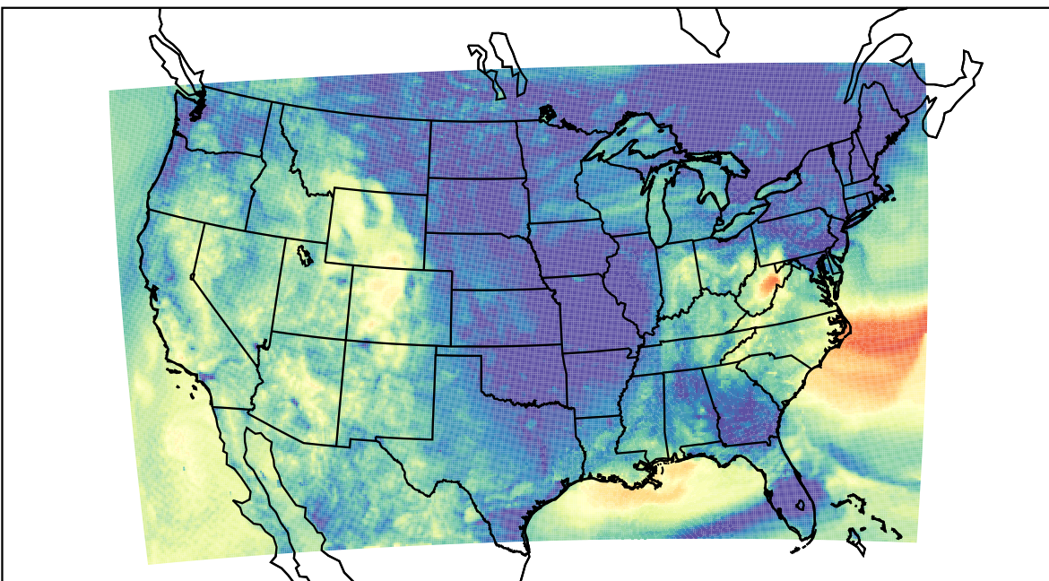
WRF (2023-10-14_07:00:00)
