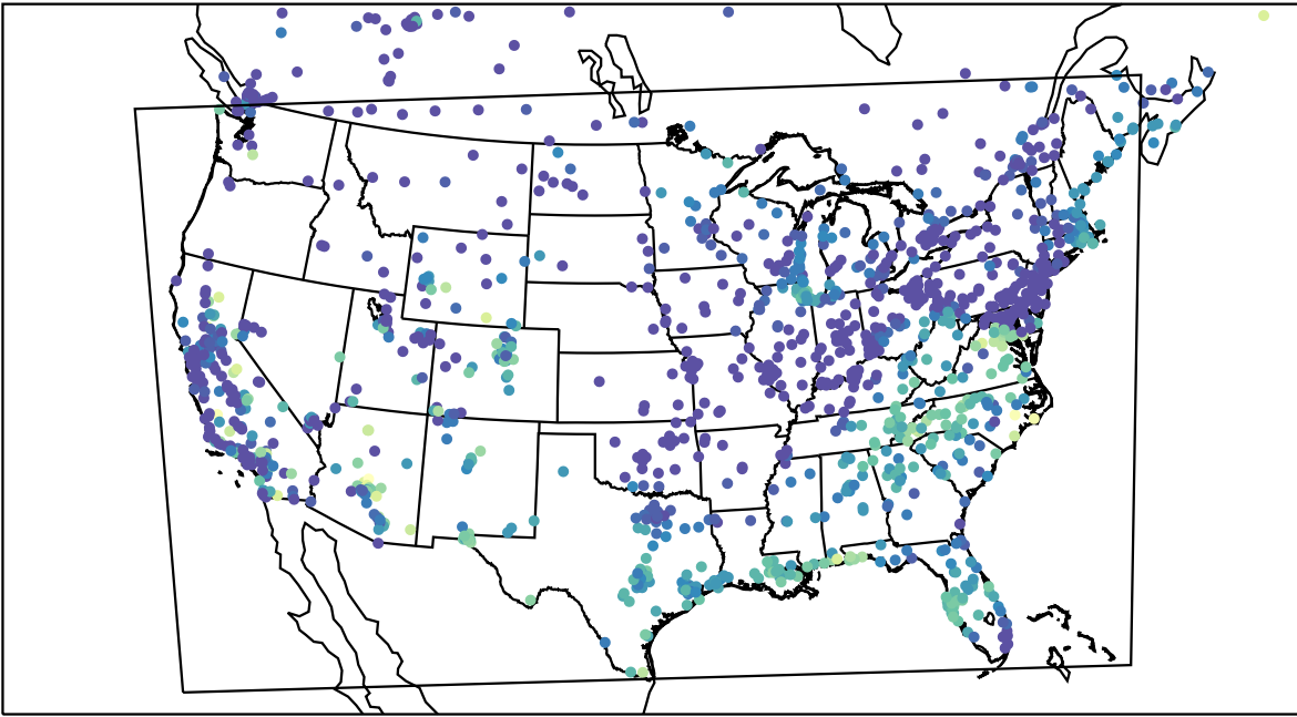
AirNOW (2023-10-14_16:00:00)
