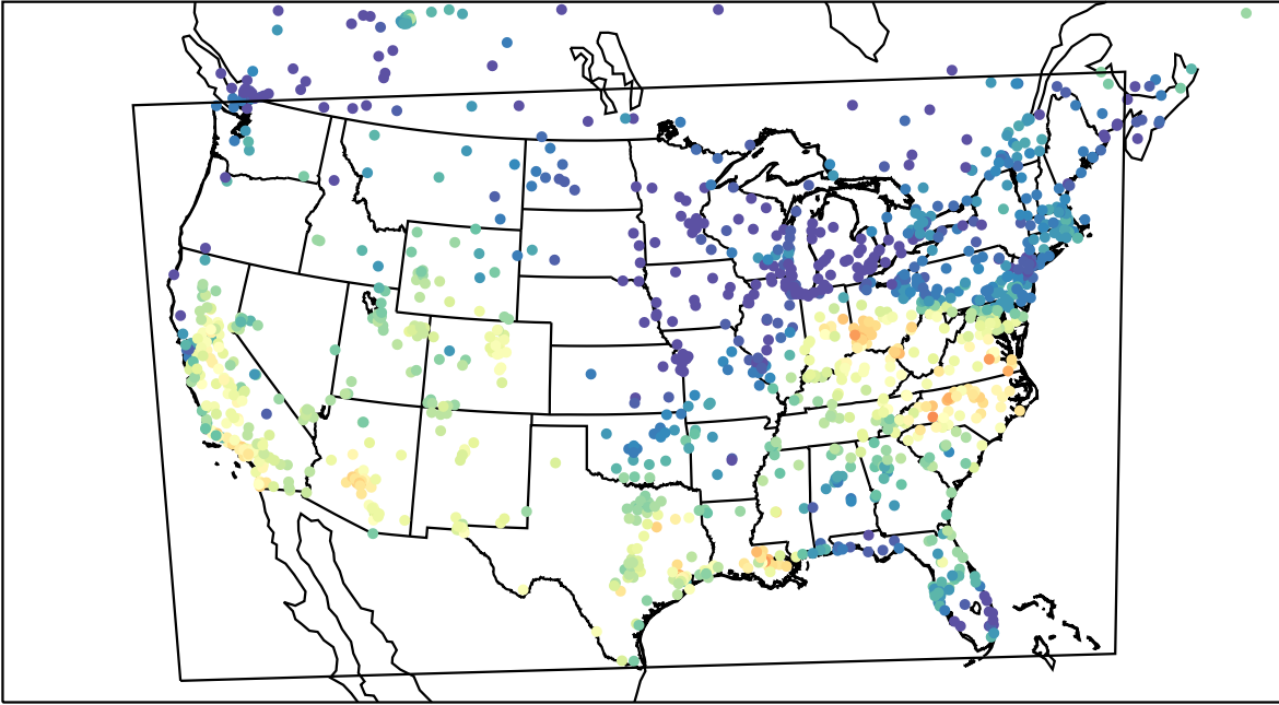
AirNOW (2023-10-13_20:00:00)
