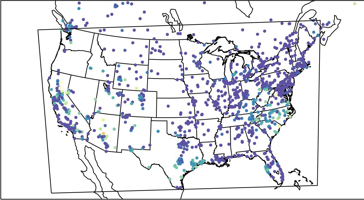
AirNOW (2023-10-14_10:00:00)
