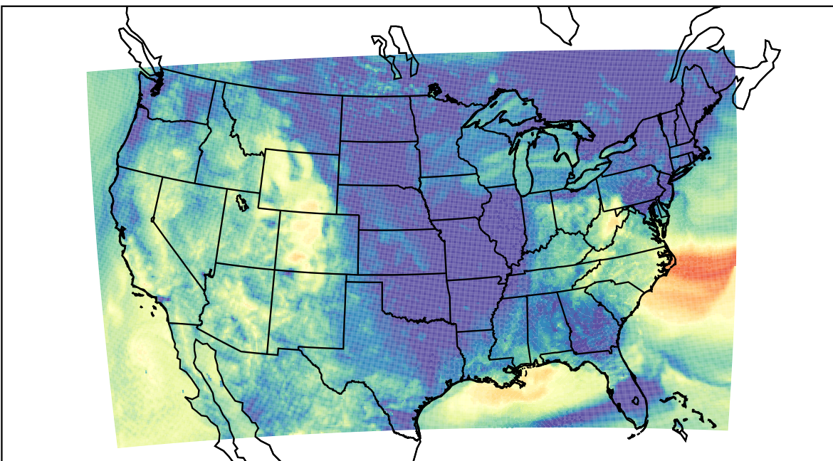
WRF (2023-10-14_09:00:00)
