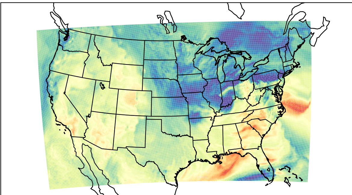
WRF (2023-10-14_20:00:00)
