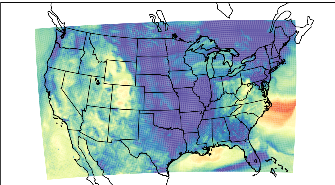
WRF (2023-10-14_10:00:00)
