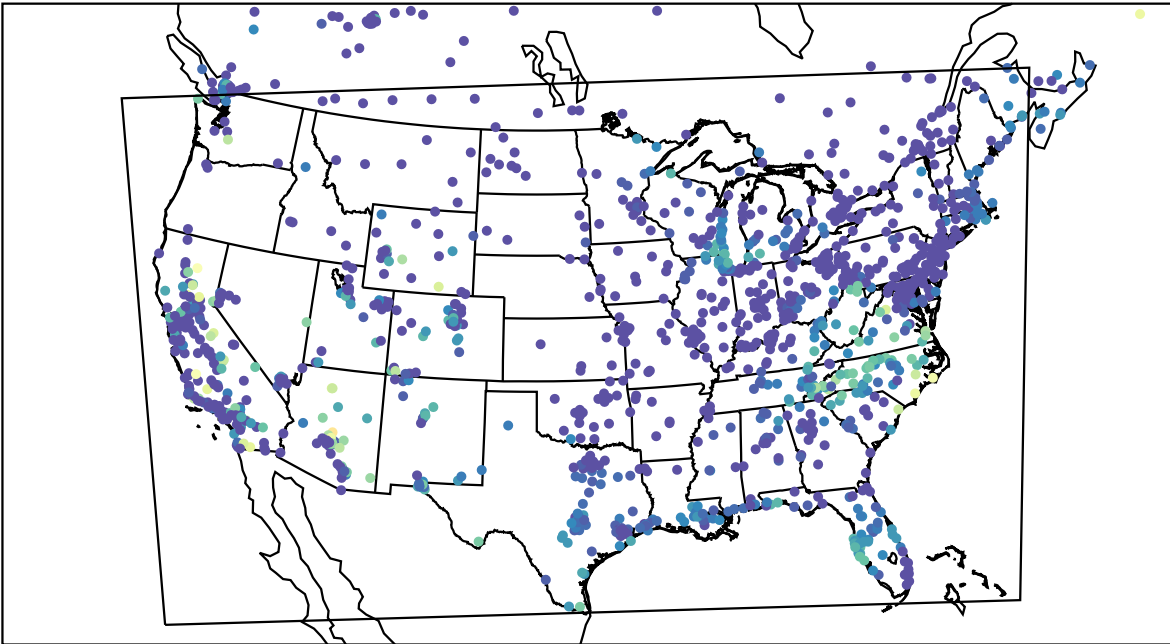
AirNOW (2023-10-14_14:00:00)
