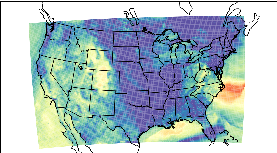
WRF (2023-10-14_12:00:00)
