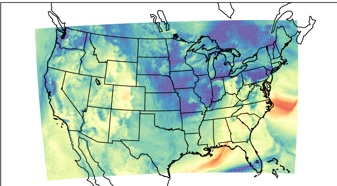
WRF (2023-10-14_17:00:00)
