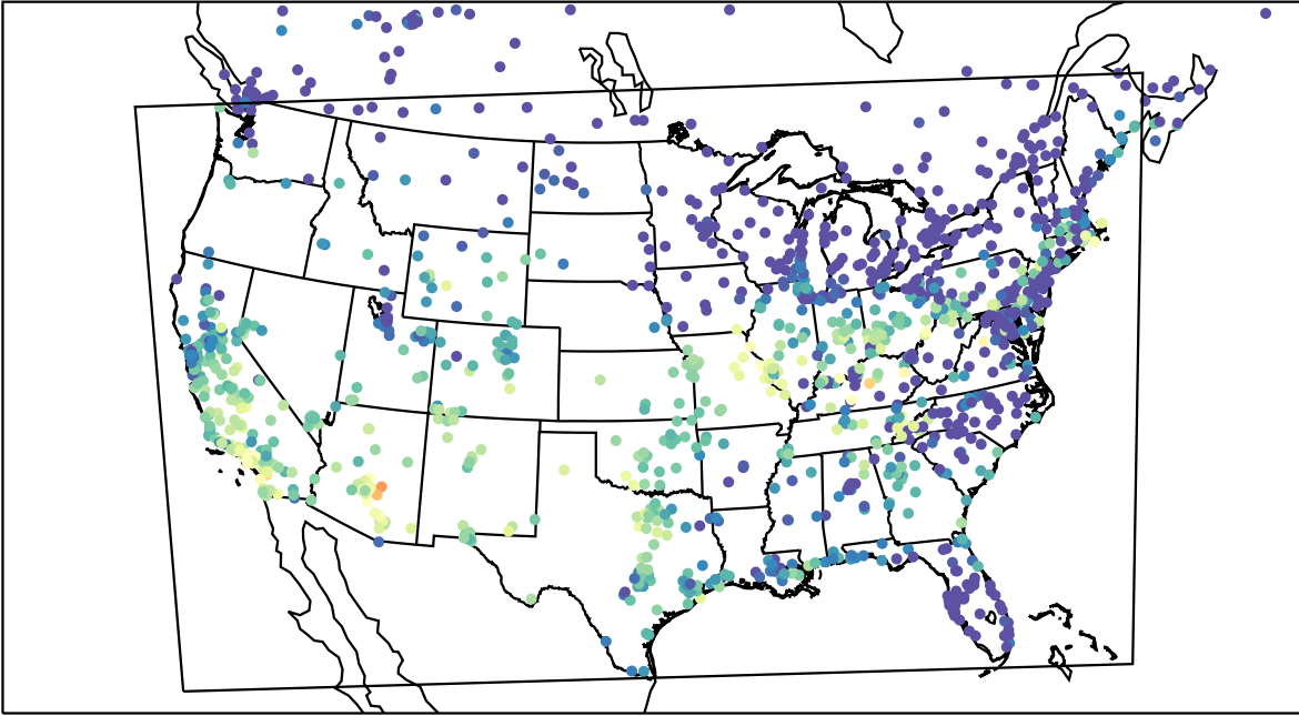
AirNOW (2023-10-13_01:00:00)
