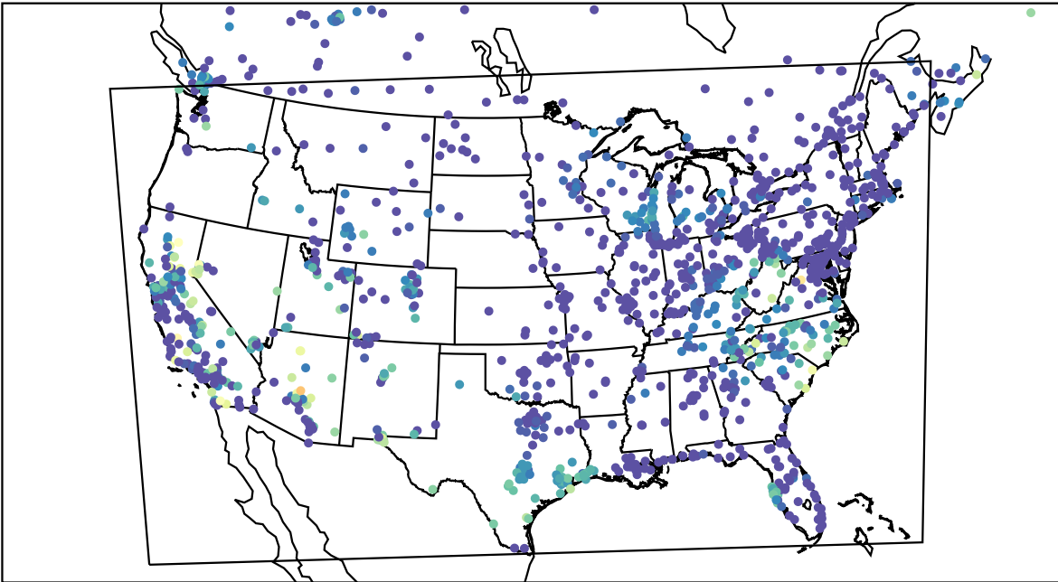
AirNOW (2023-10-14_09:00:00)
