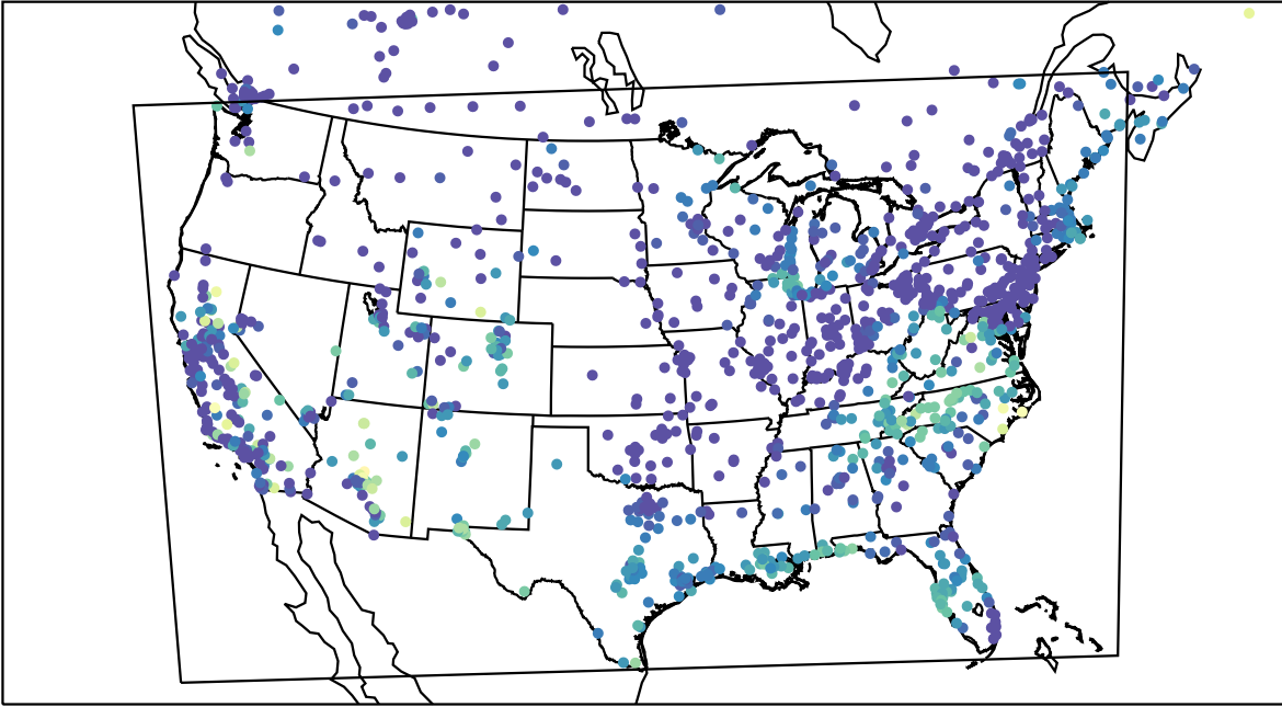
AirNOW (2023-10-14_15:00:00)
