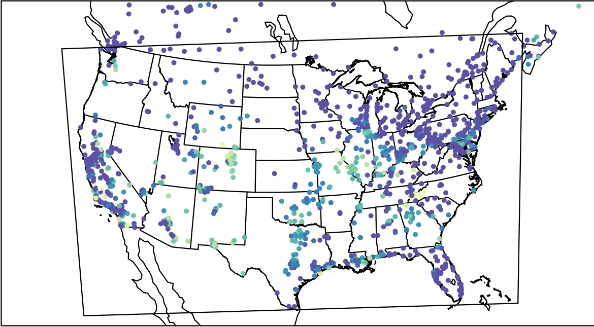
AirNOW (2023-10-13_08:00:00)
