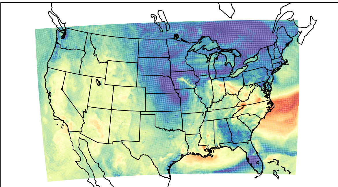
WRF (2023-10-14_00:00:00)
