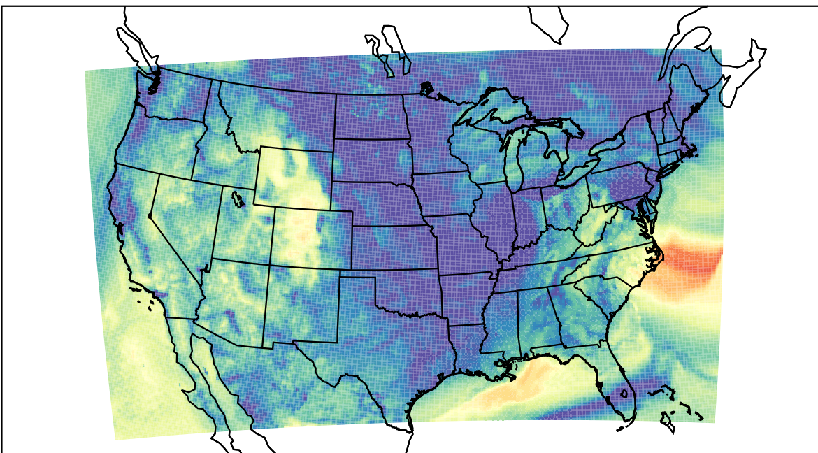
WRF (2023-10-14_14:00:00)
