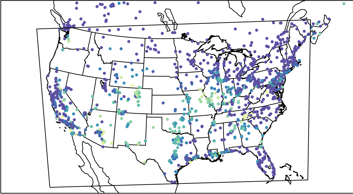
AirNOW (2023-10-13_07:00:00)
