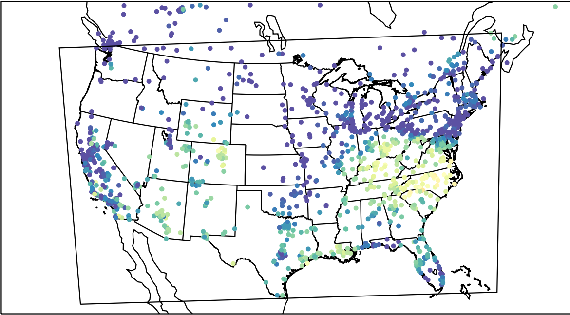
AirNOW (2023-10-13_16:00:00)
