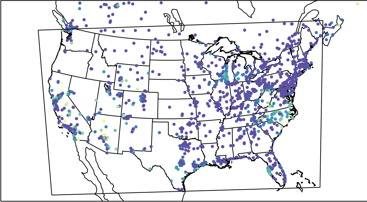
AirNOW (2023-10-14_12:00:00)
