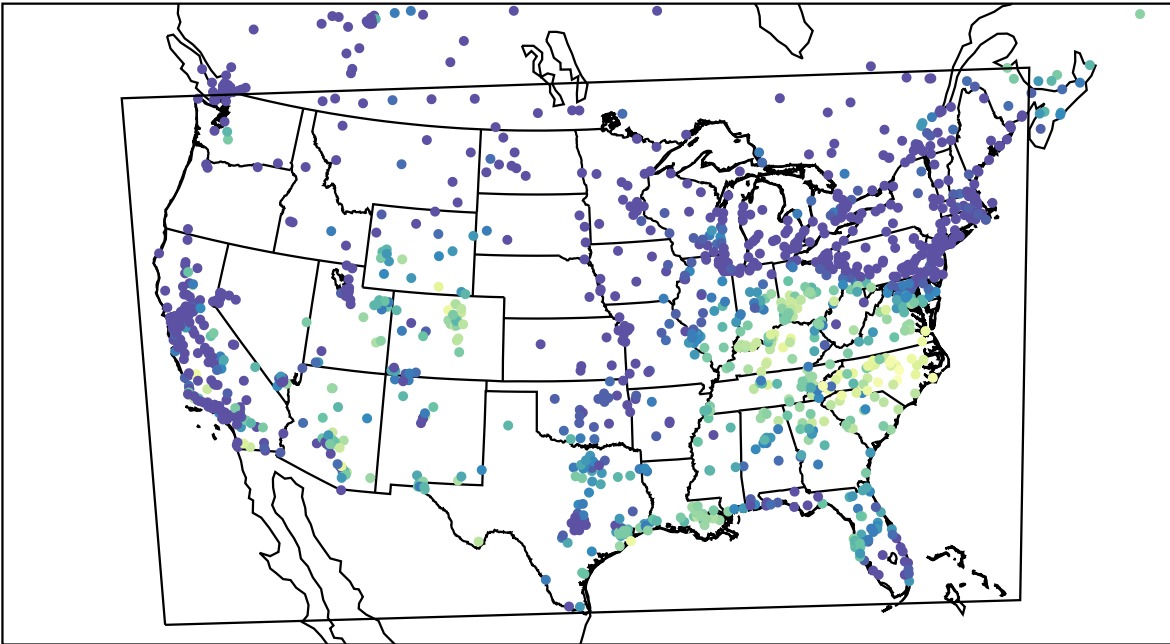
AirNOW (2023-10-13_15:00:00)
