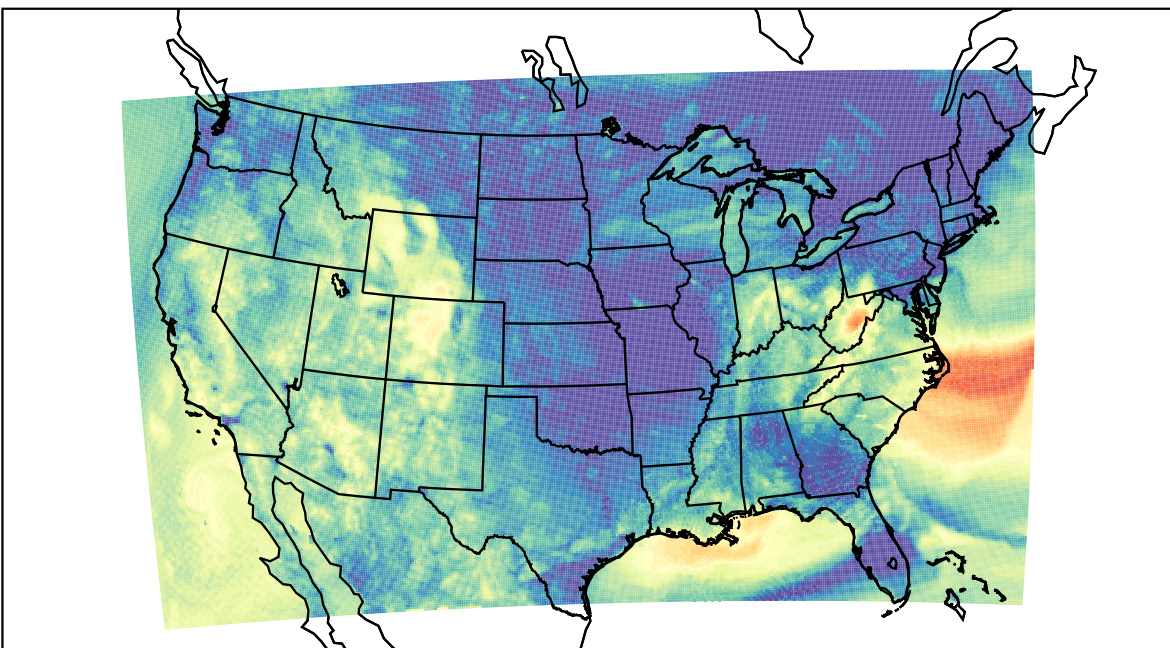
WRF (2023-10-14_06:00:00)
