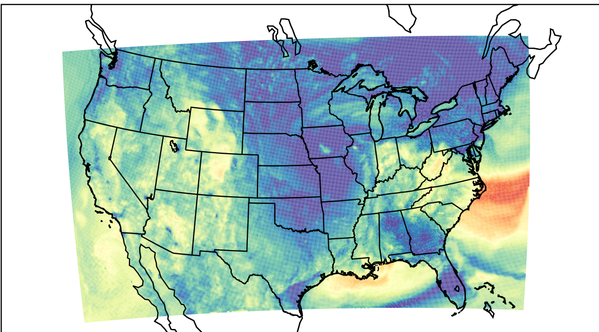
WRF (2023-10-14_04:00:00)
