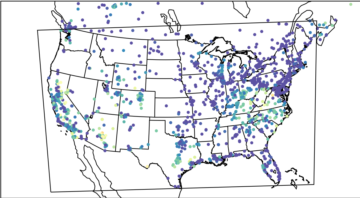
AirNOW (2023-10-14_04:00:00)
