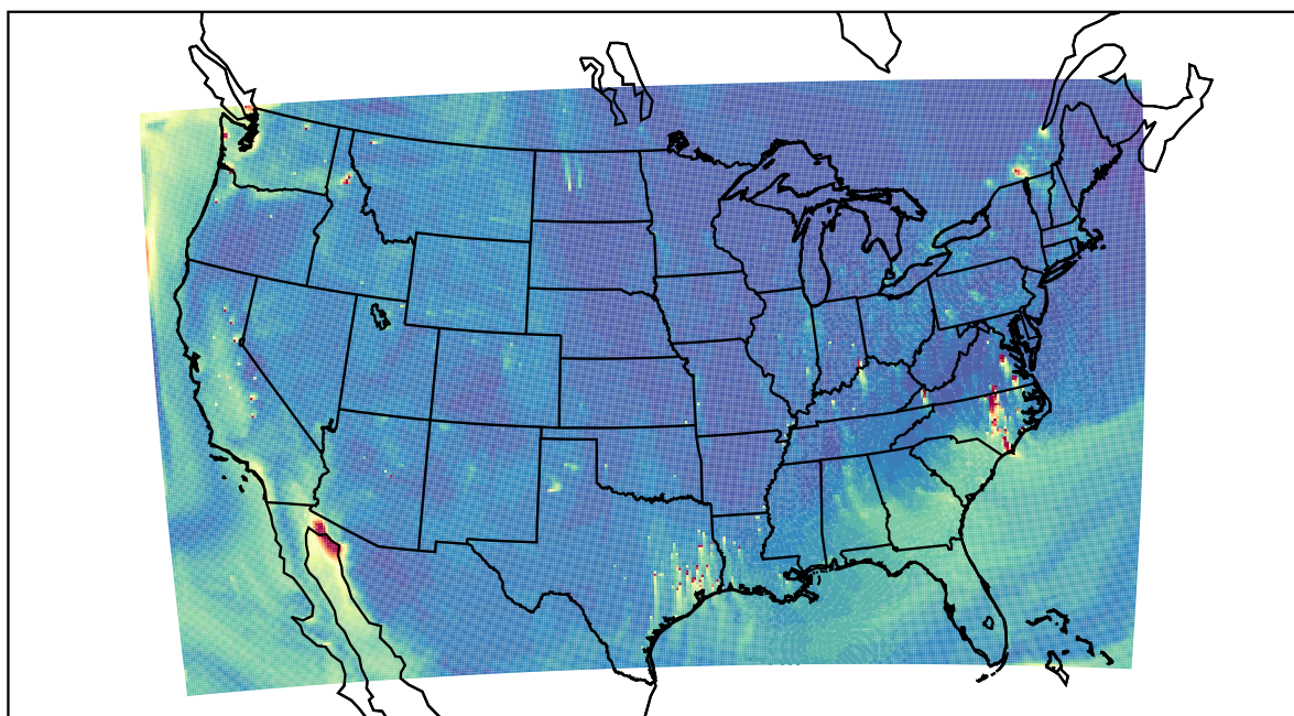
WRF 2023-10-15_22:00:00
