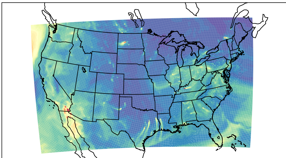
WRF 2023-10-14_14:00:00
