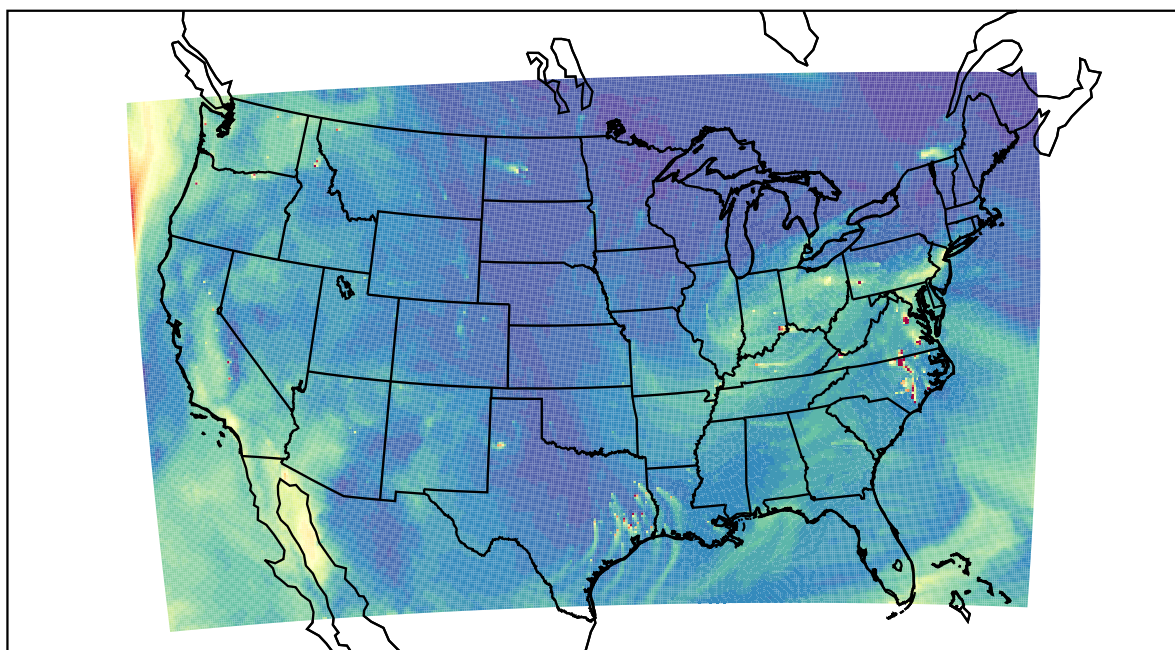
WRF 2023-10-14_20:00:00
