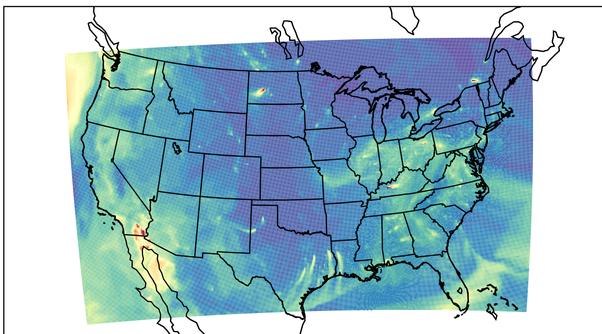
WRF 2023-10-14_13:00:00
