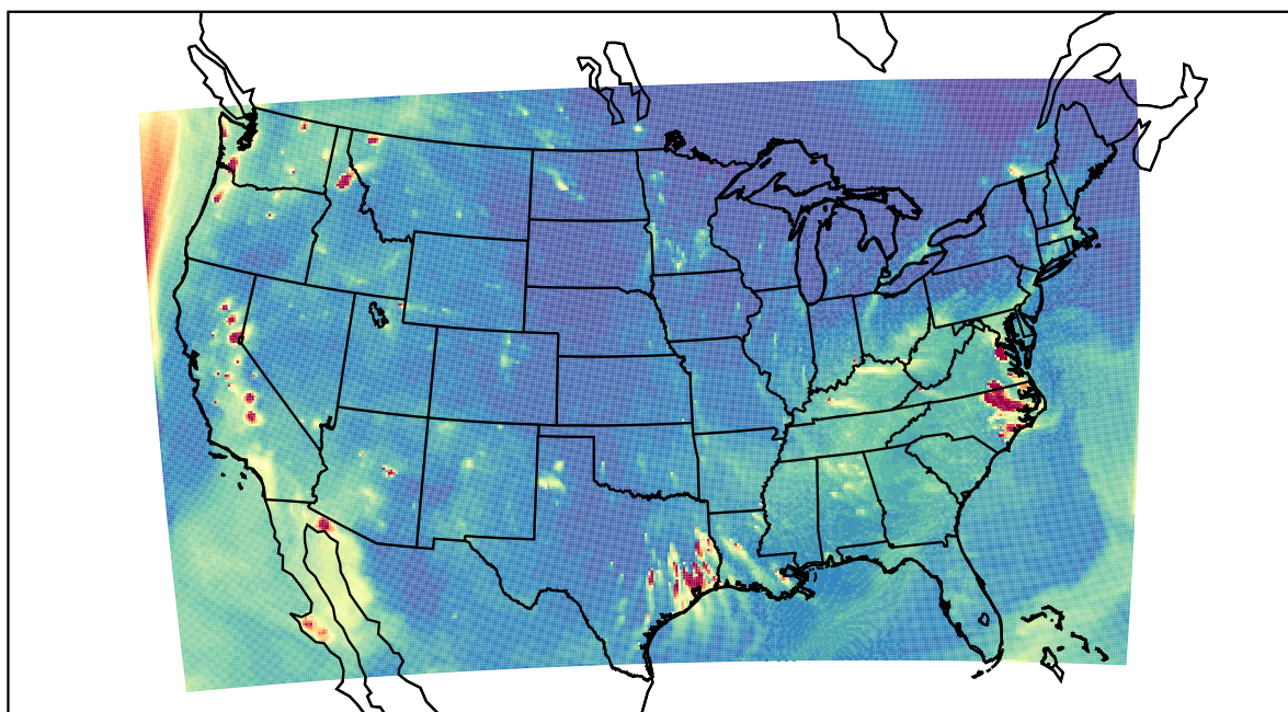
WRF 2023-10-15_02:00:00
