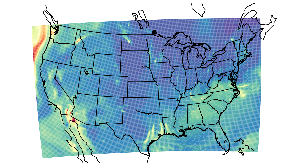
WRF 2023-10-15_09:00:00
