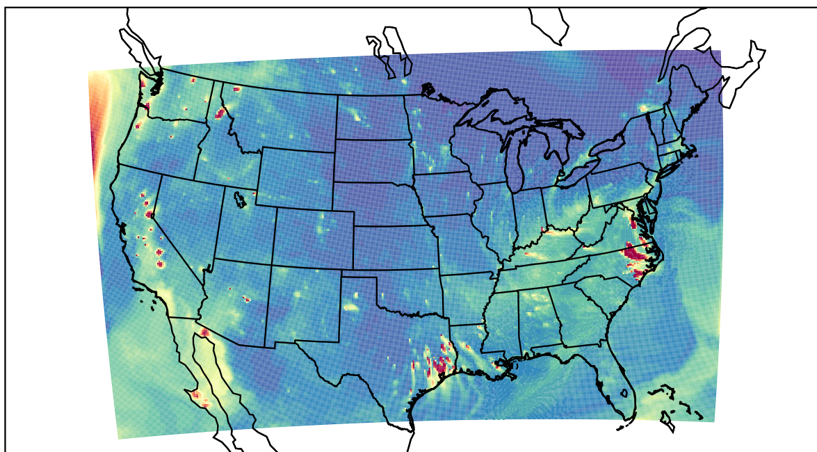
WRF 2023-10-15_01:00:00
