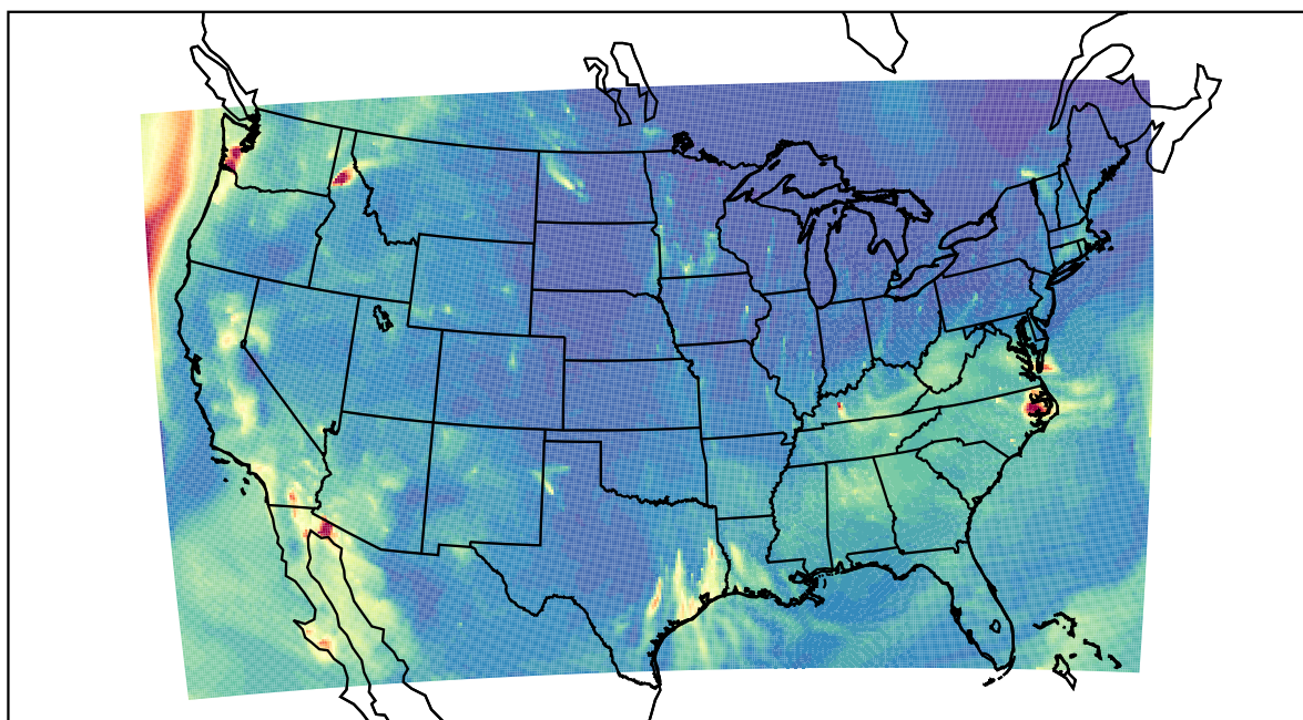
WRF 2023-10-15_06:00:00
