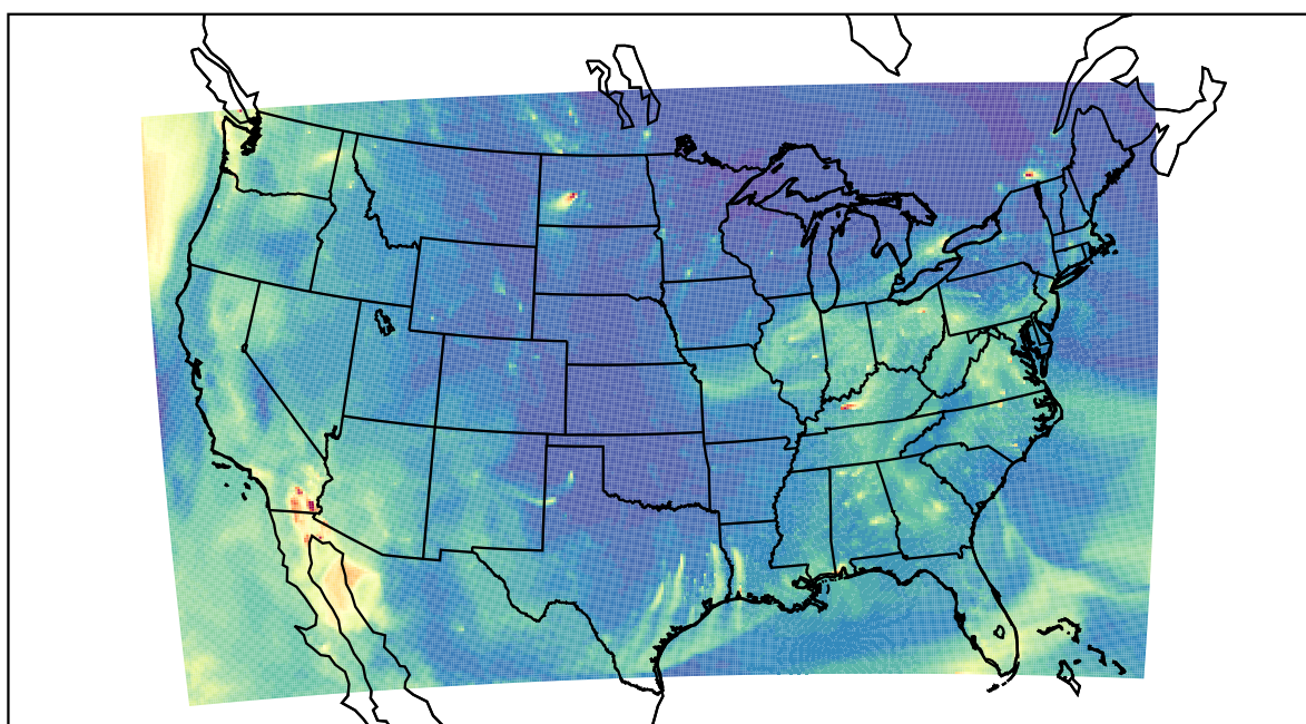
WRF 2023-10-14_12:00:00
