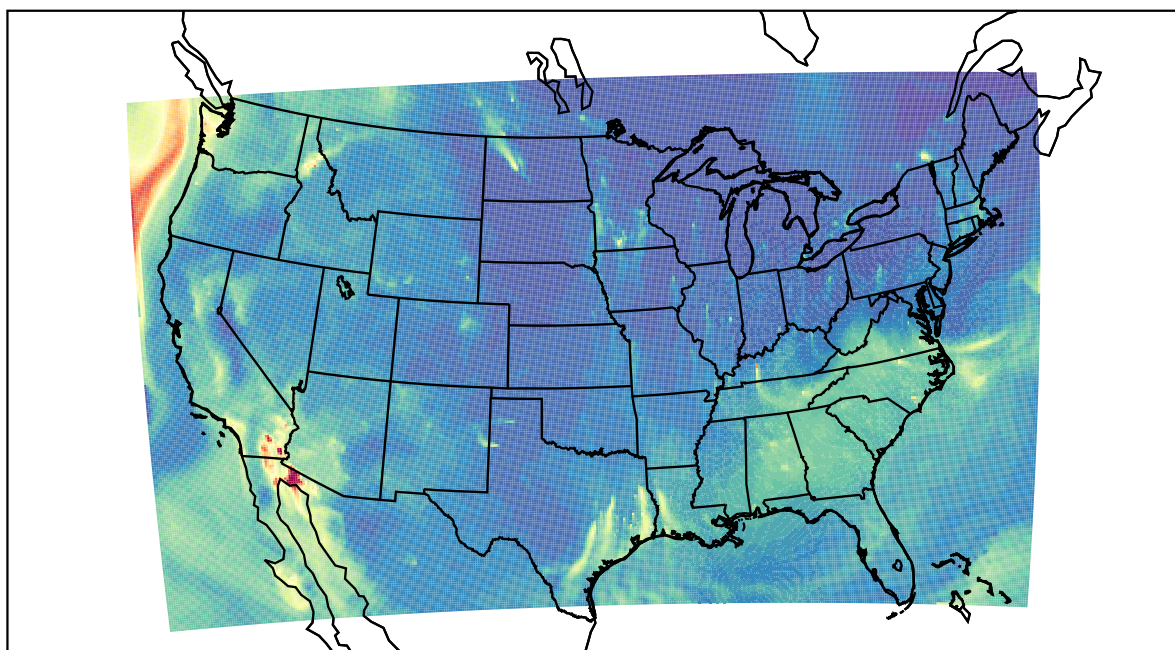
WRF 2023-10-15_10:00:00
