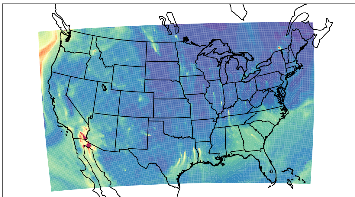
WRF 2023-10-15_14:00:00
