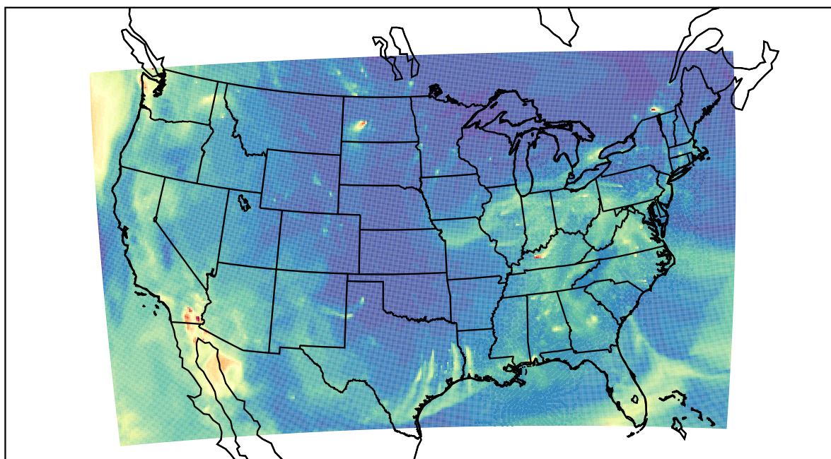
WRF 2023-10-14_11:00:00
