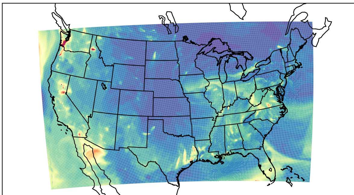
WRF 2023-10-14_05:00:00
