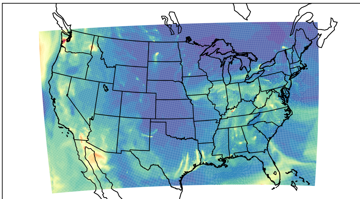
WRF 2023-10-14_08:00:00
