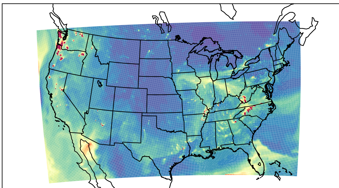
WRF 2023-10-14_00:00:00
