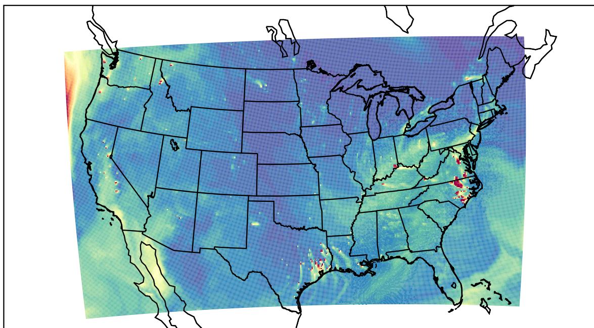
WRF 2023-10-14_23:00:00
