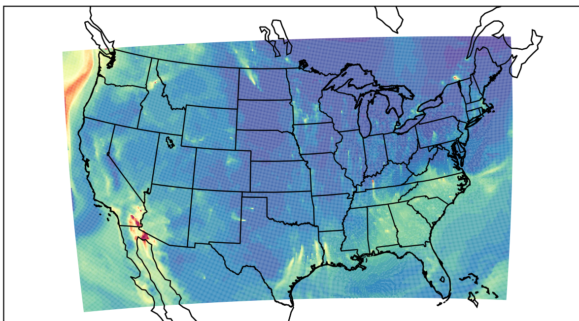
WRF 2023-10-15_12:00:00
