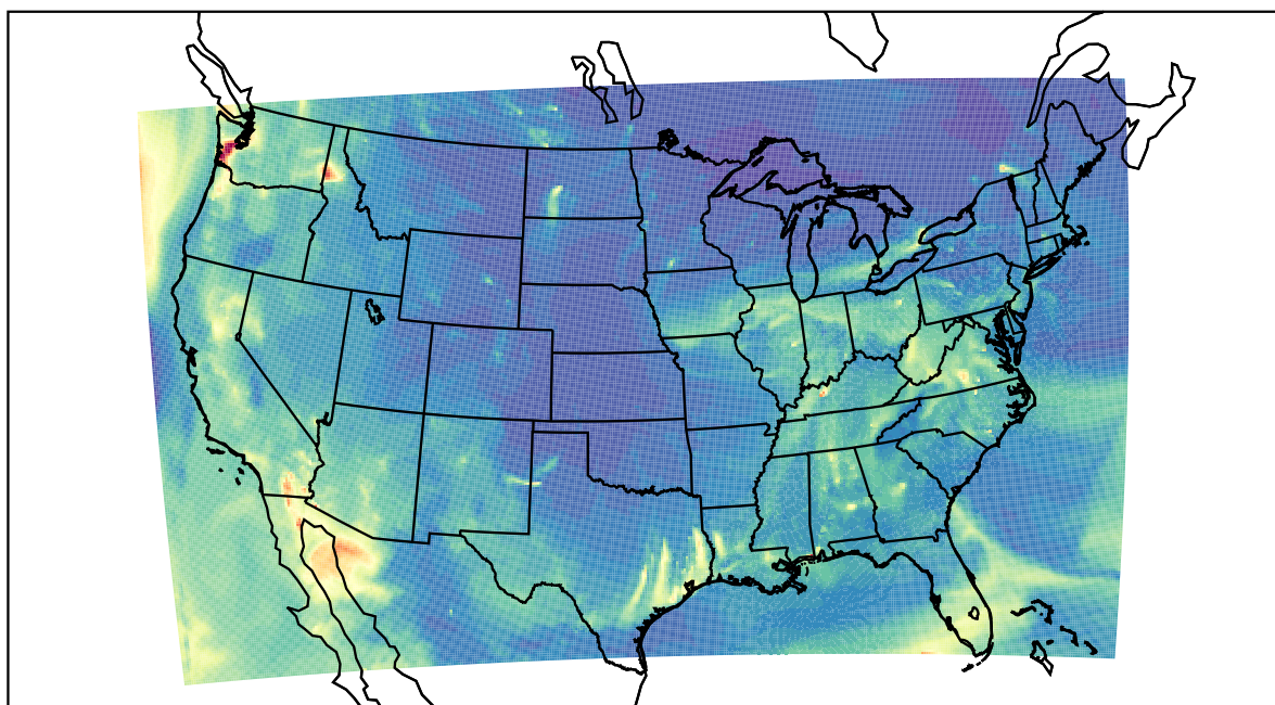
WRF 2023-10-14_07:00:00
