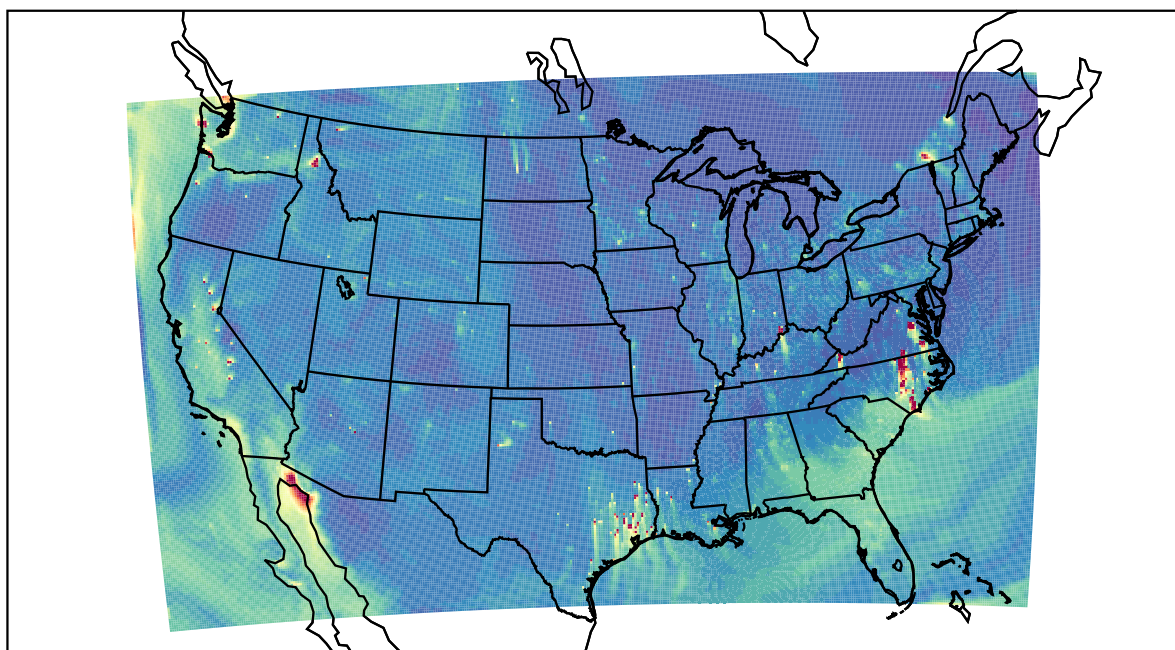
WRF 2023-10-15_23:00:00
