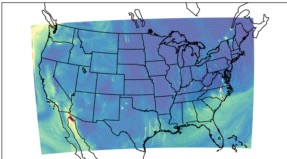
WRF 2023-10-15_20:00:00
