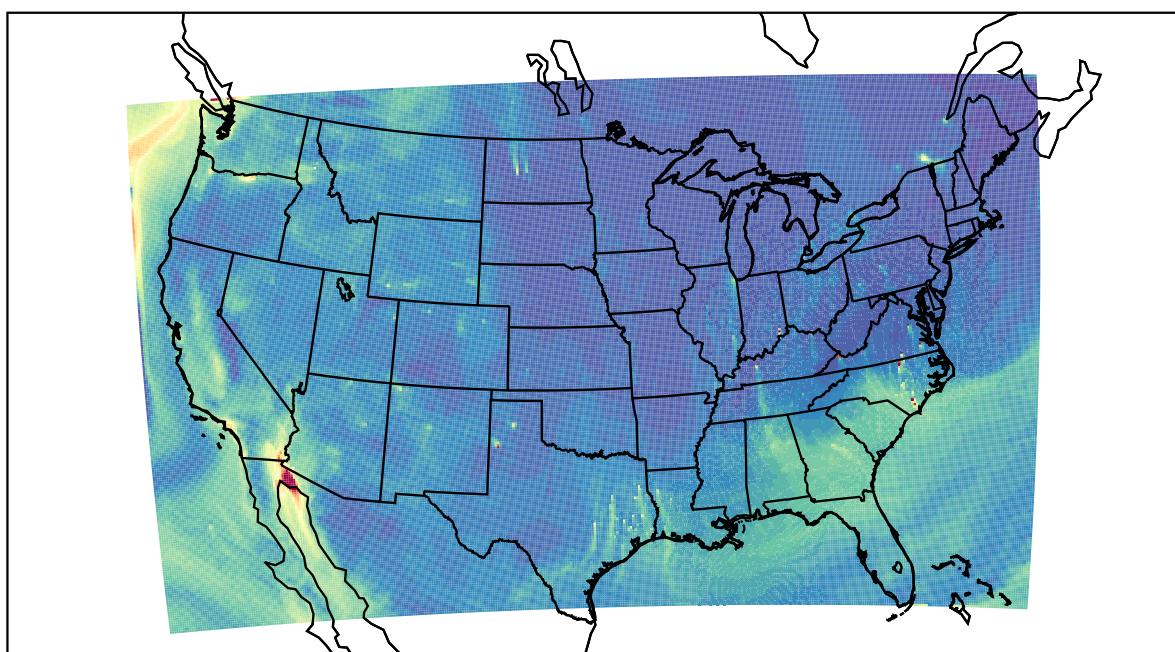
WRF 2023-10-15_18:00:00
