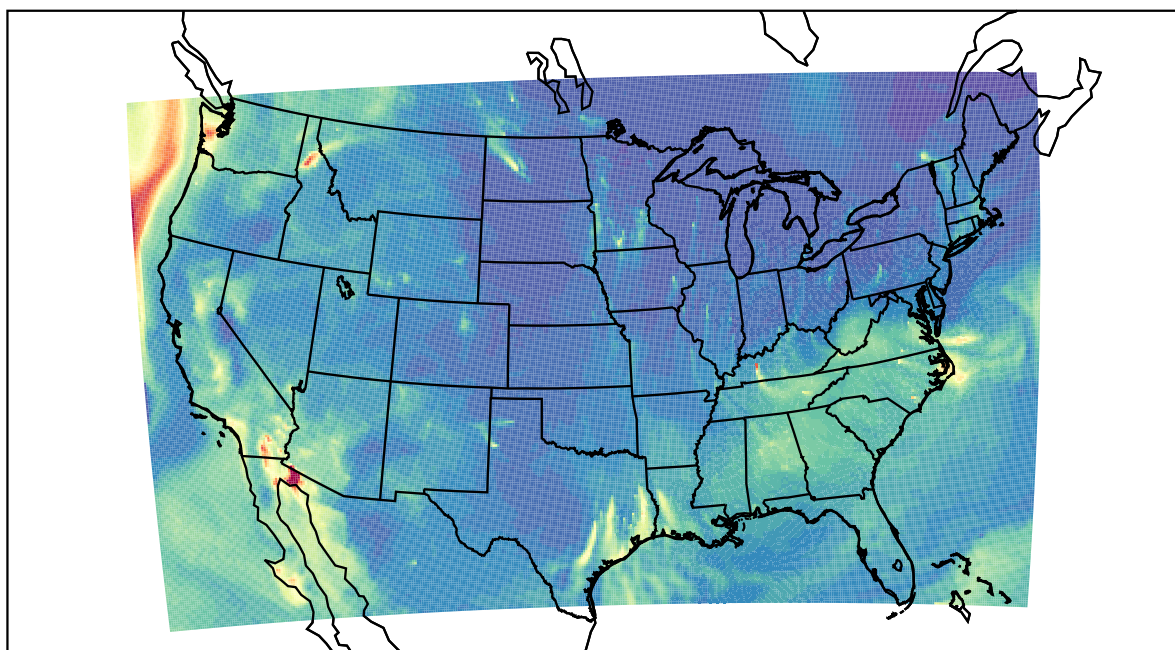
WRF 2023-10-15_08:00:00
