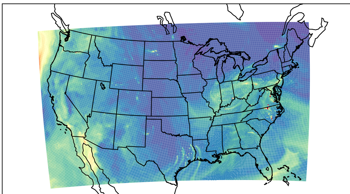
WRF 2023-10-14_18:00:00
