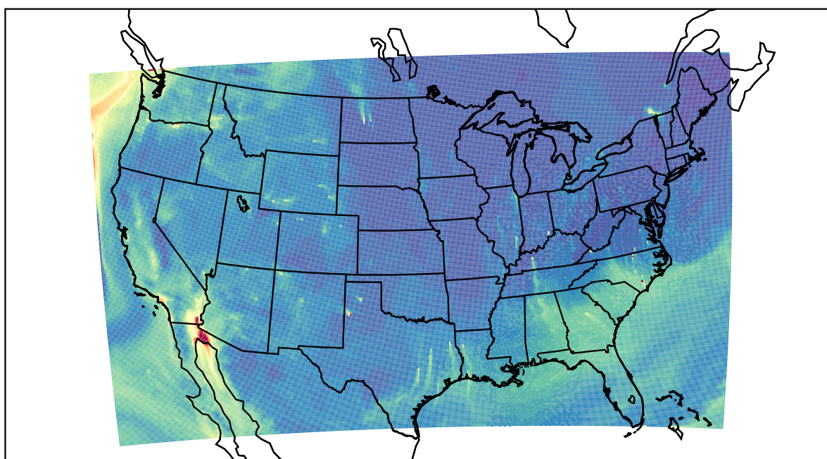
WRF 2023-10-15_17:00:00
