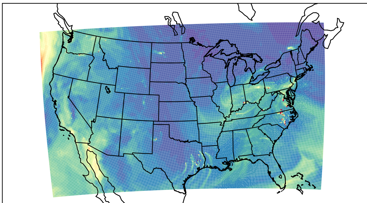
WRF 2023-10-14_19:00:00
