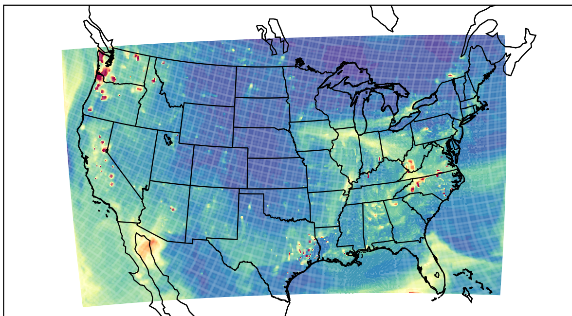
WRF 2023-10-14_01:00:00
