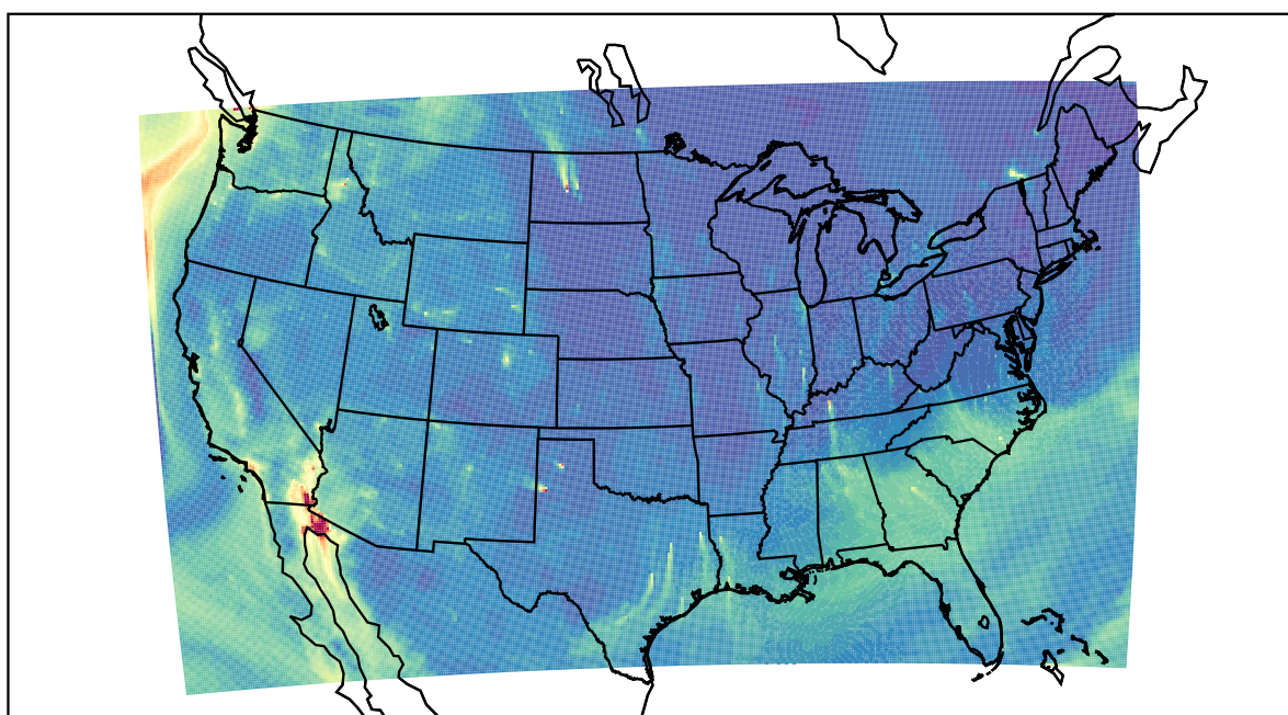
WRF 2023-10-15_16:00:00
