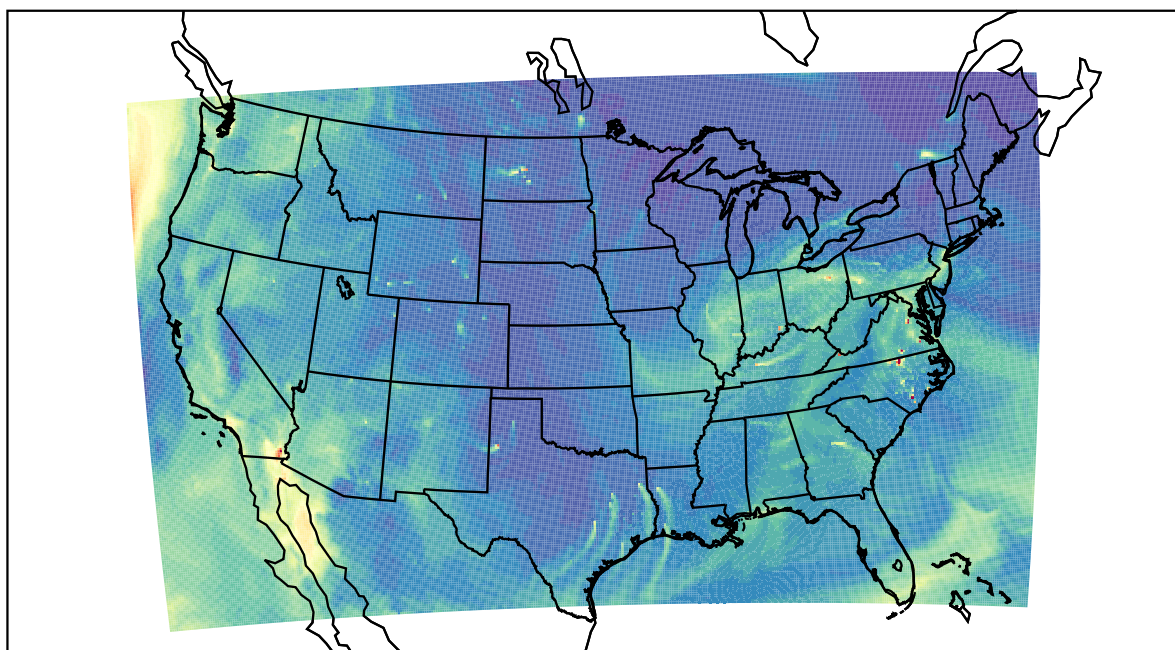
WRF 2023-10-14_17:00:00
