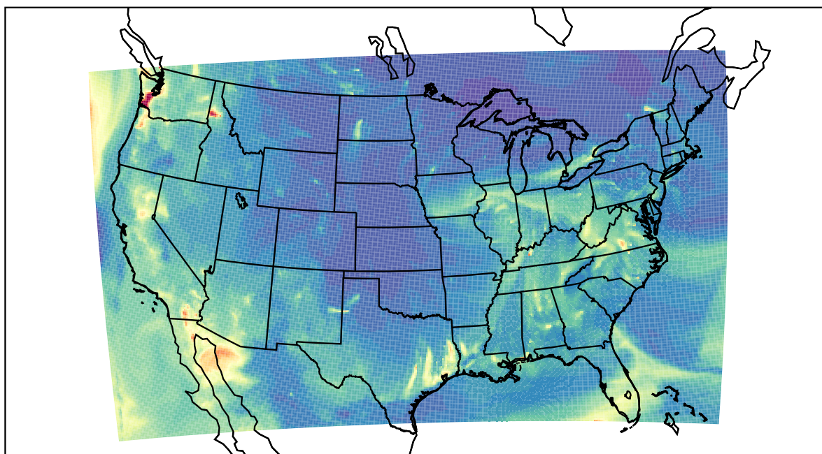
WRF 2023-10-14_06:00:00
