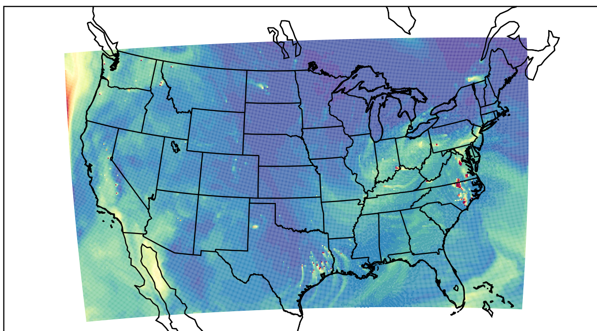
WRF 2023-10-14_21:00:00
