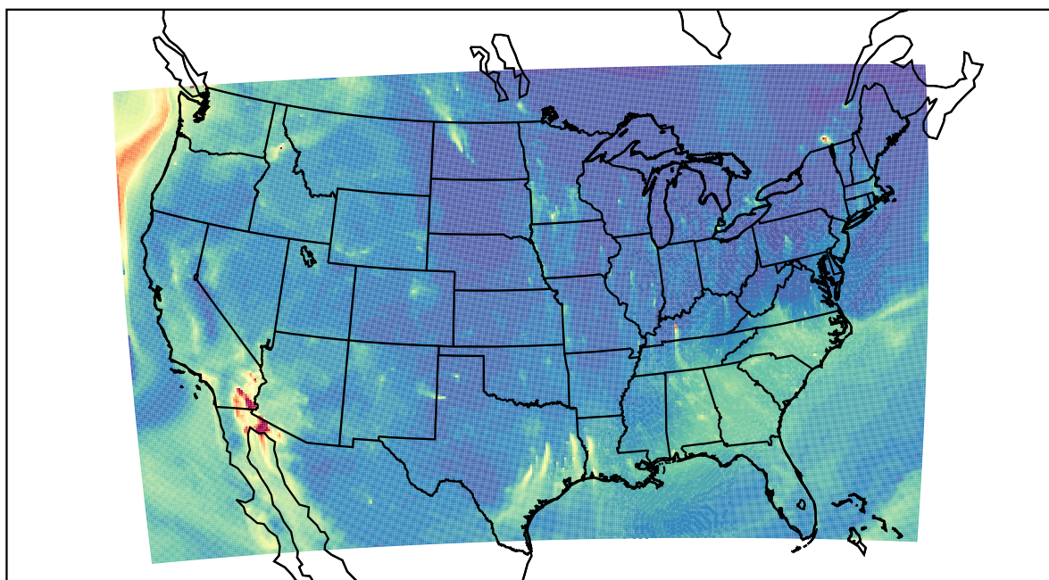
WRF 2023-10-15_13:00:00
