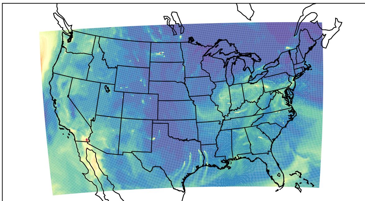
WRF 2023-10-14_16:00:00
