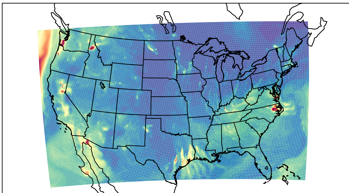
WRF 2023-10-15_05:00:00
