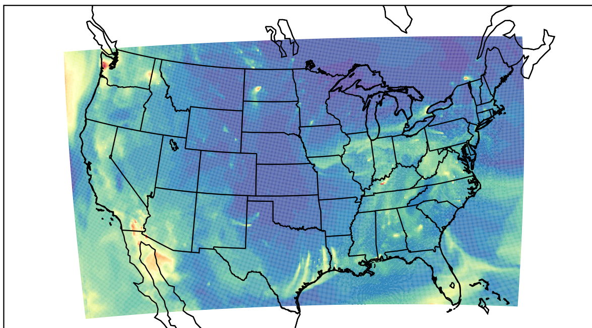
WRF 2023-10-14_09:00:00
