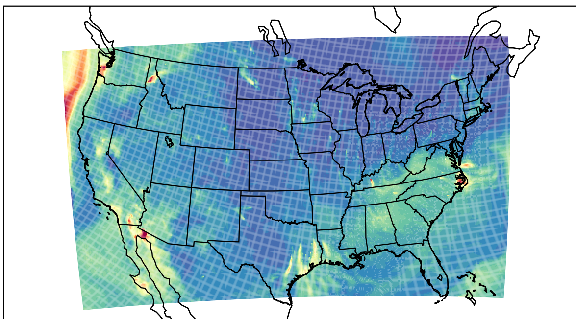
WRF 2023-10-15_07:00:00
