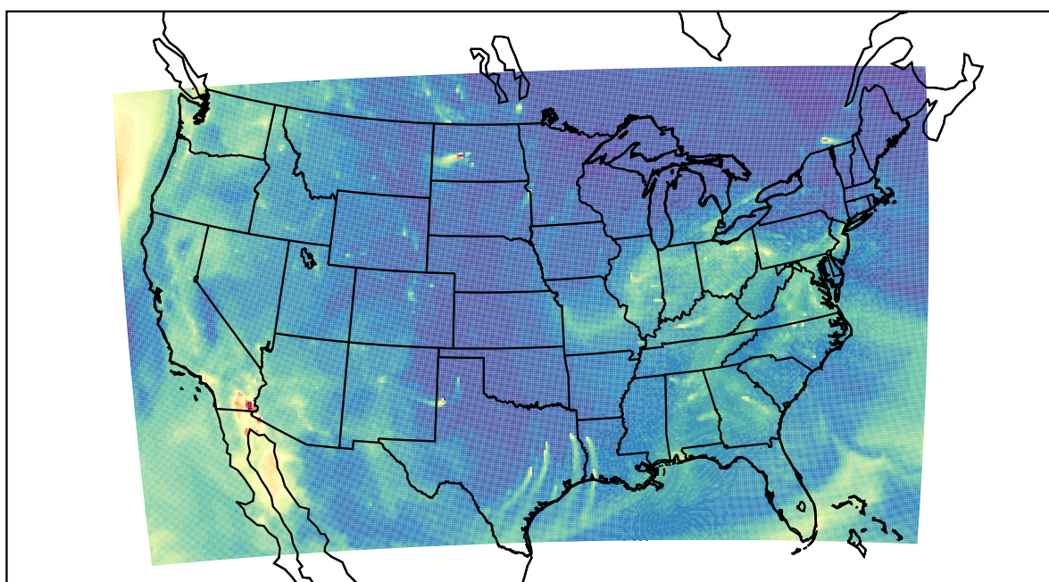
WRF 2023-10-14_15:00:00
