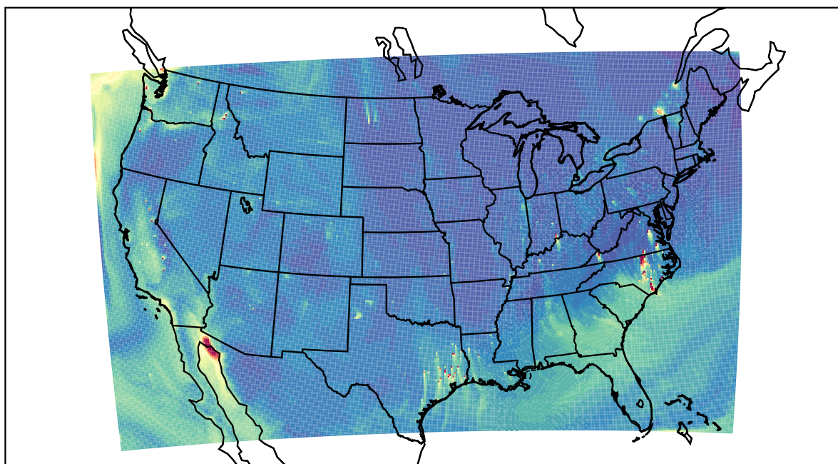
WRF 2023-10-15_21:00:00
