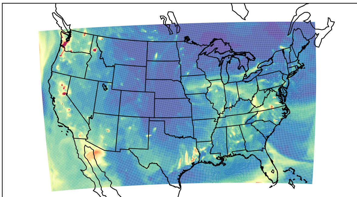
WRF 2023-10-14_04:00:00
