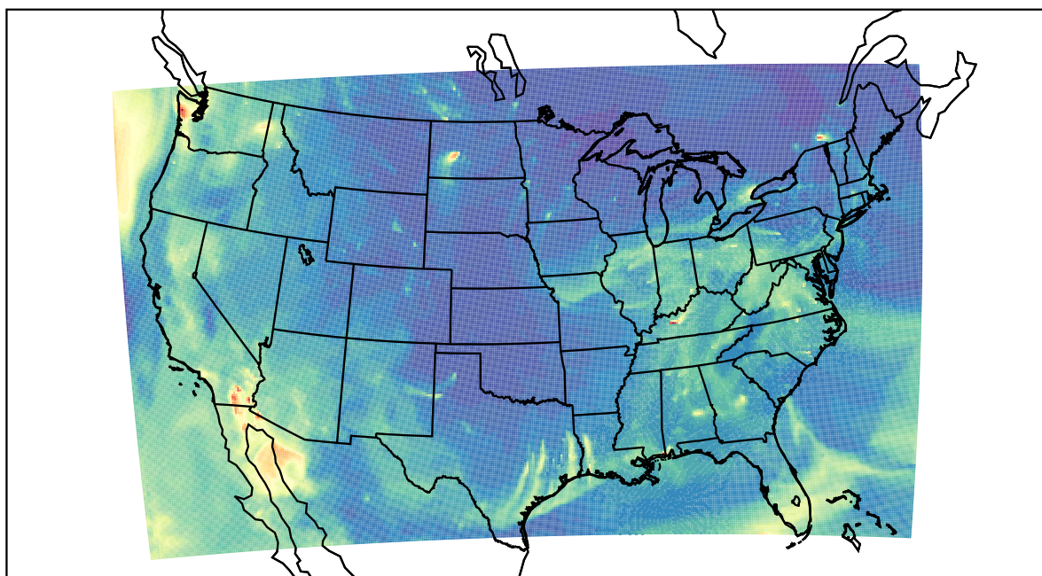
WRF 2023-10-14_10:00:00
