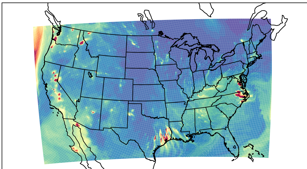
WRF 2023-10-15_03:00:00
