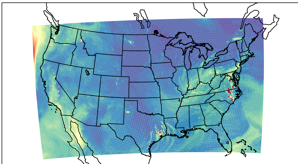
WRF 2023-10-14_22:00:00
