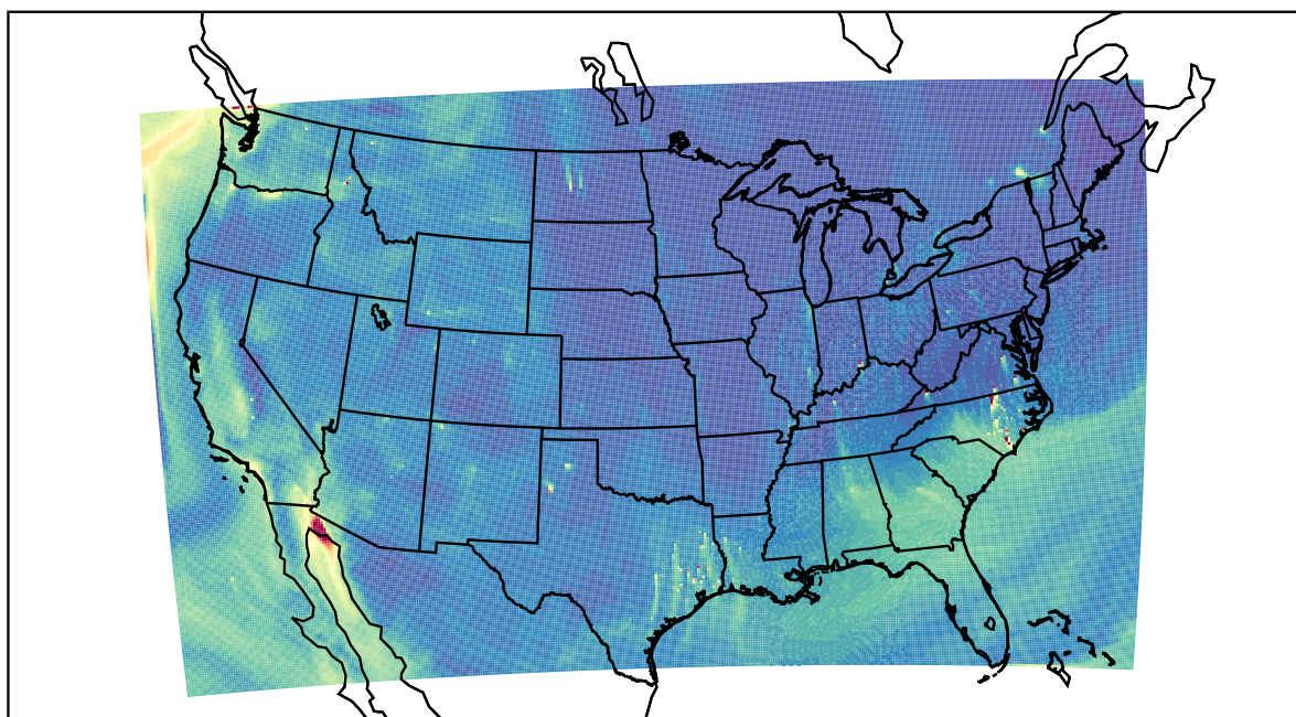
WRF 2023-10-15_19:00:00
