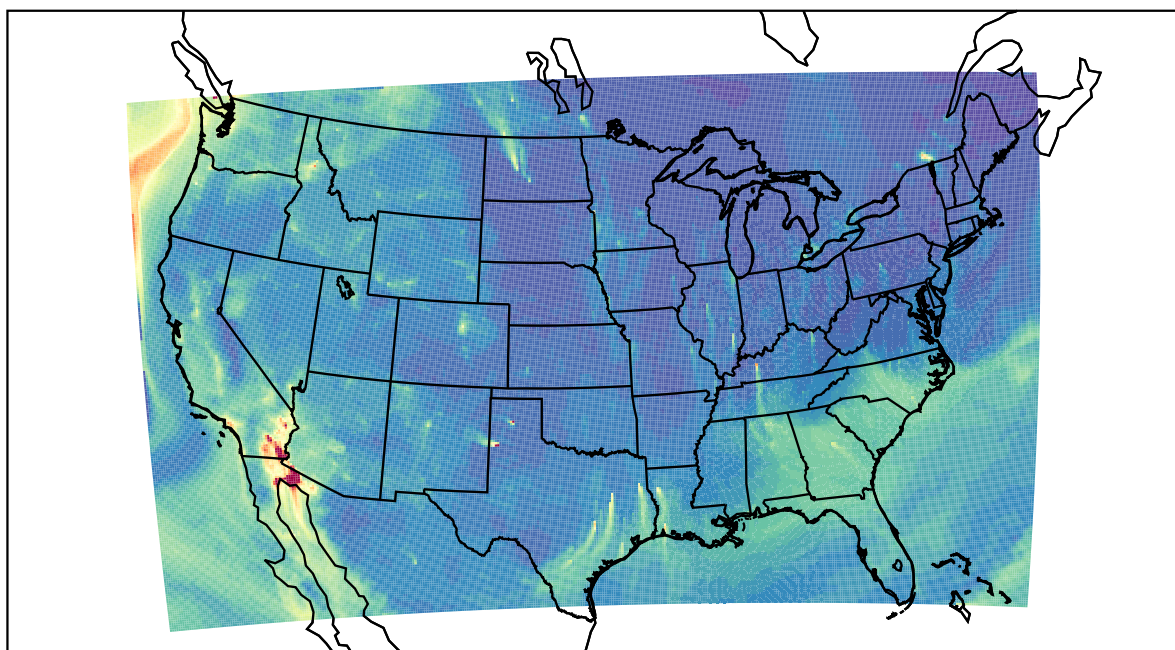
WRF 2023-10-15_15:00:00
