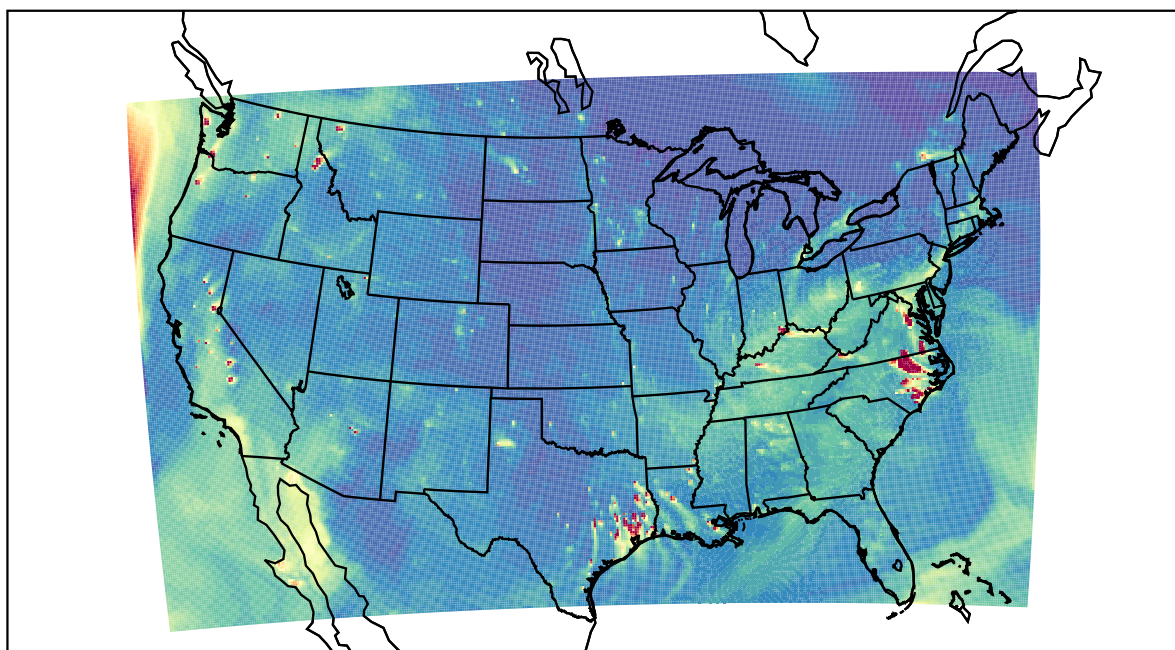
WRF 2023-10-15_00:00:00
