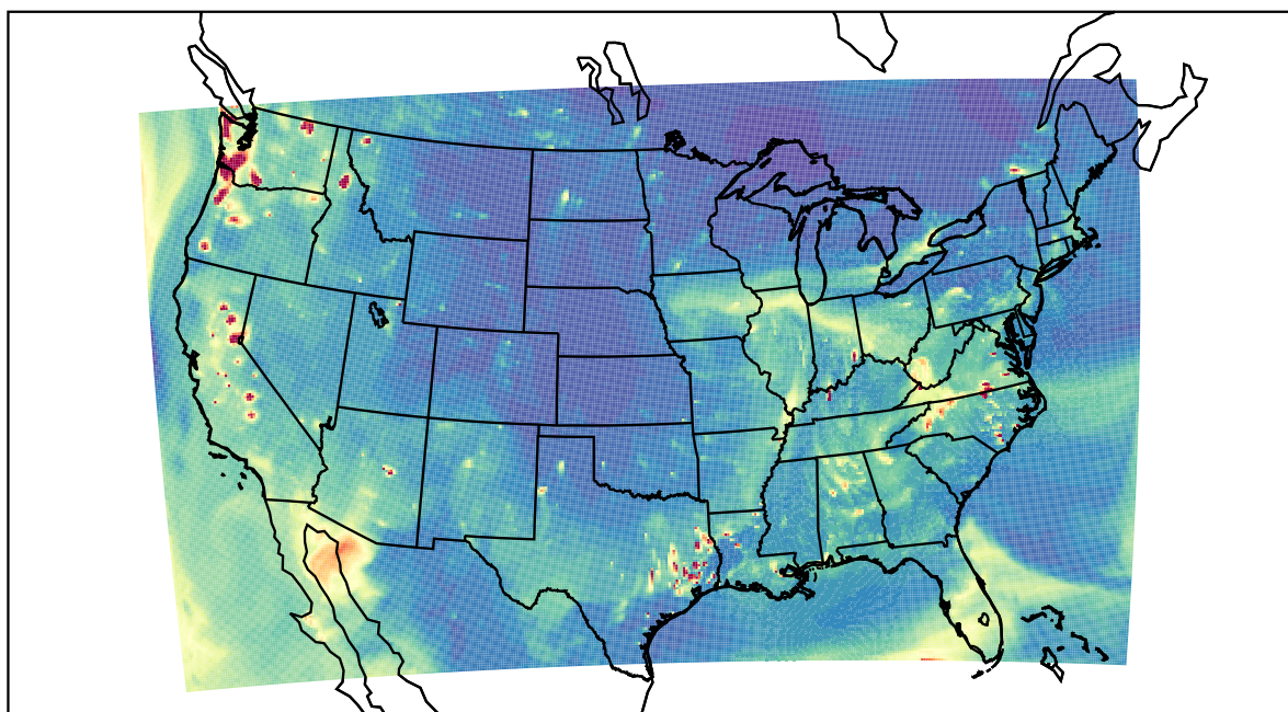
WRF 2023-10-14_02:00:00
