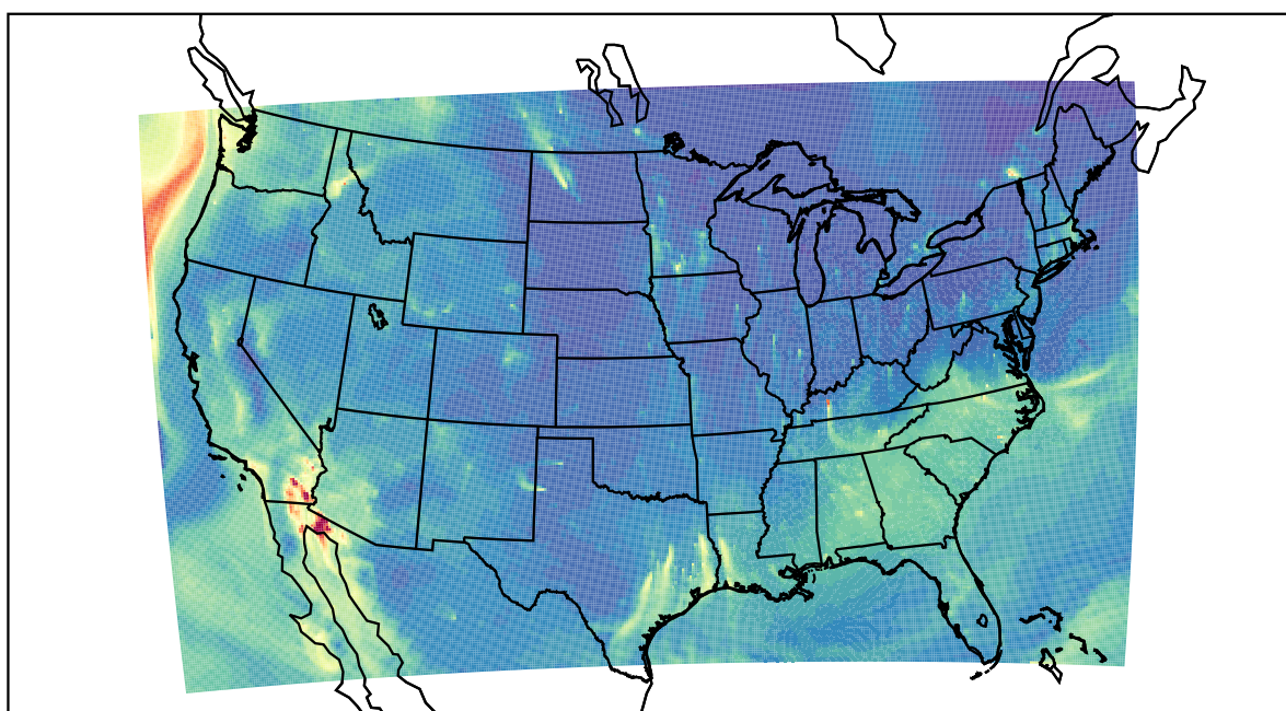
WRF 2023-10-15_11:00:00
