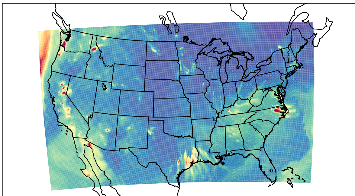
WRF 2023-10-15_04:00:00
