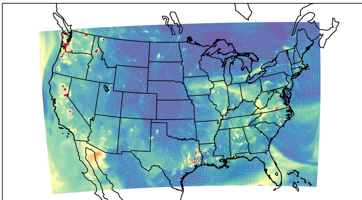
WRF 2023-10-14_03:00:00
