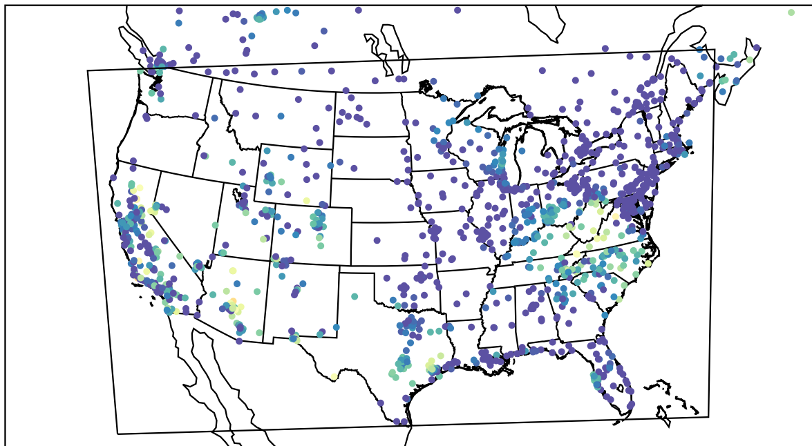
AirNOW (2023-10-14_05:00:00)
