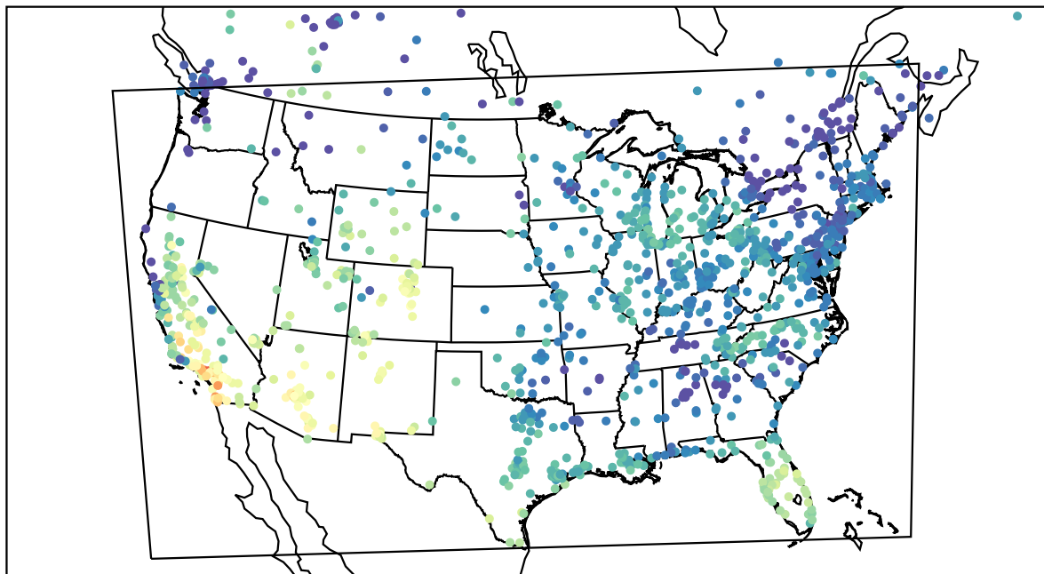
AirNOW (2023-10-15_18:00:00)
