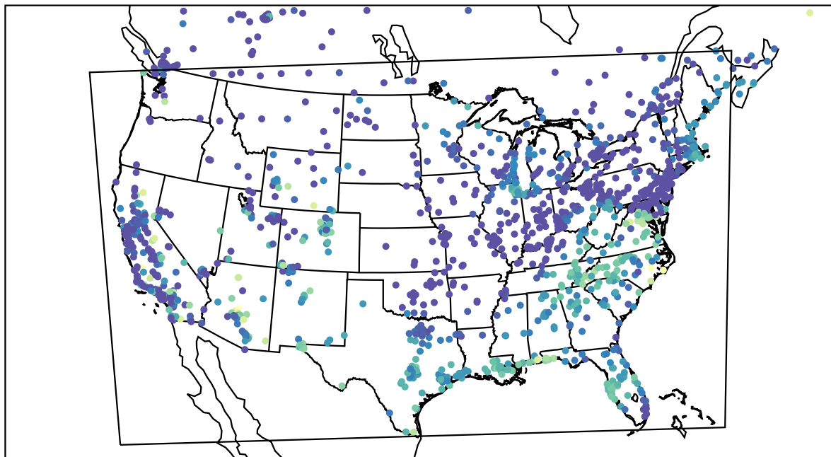
AirNOW (2023-10-14_16:00:00)
