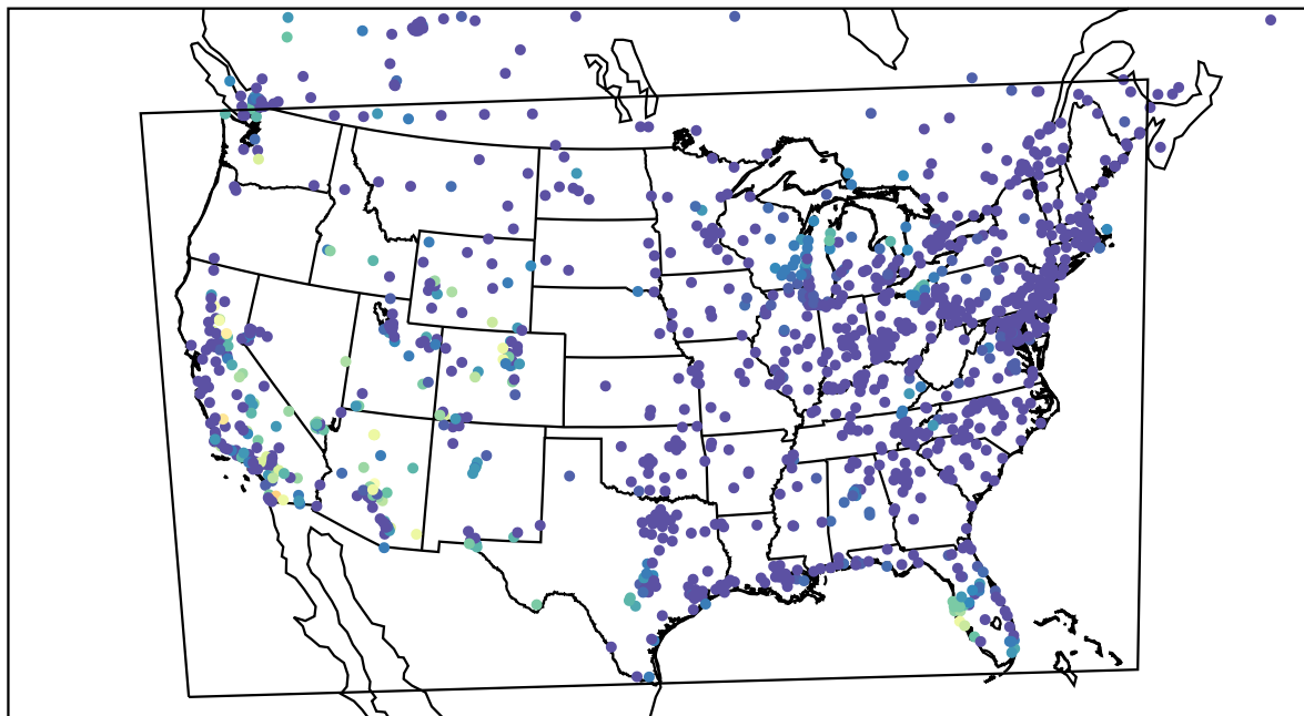
AirNOW (2023-10-15_11:00:00)
