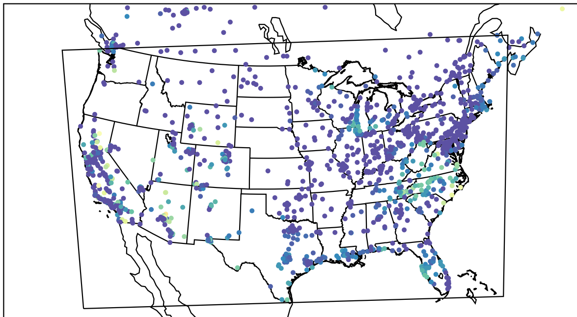
AirNOW (2023-10-14_14:00:00)
