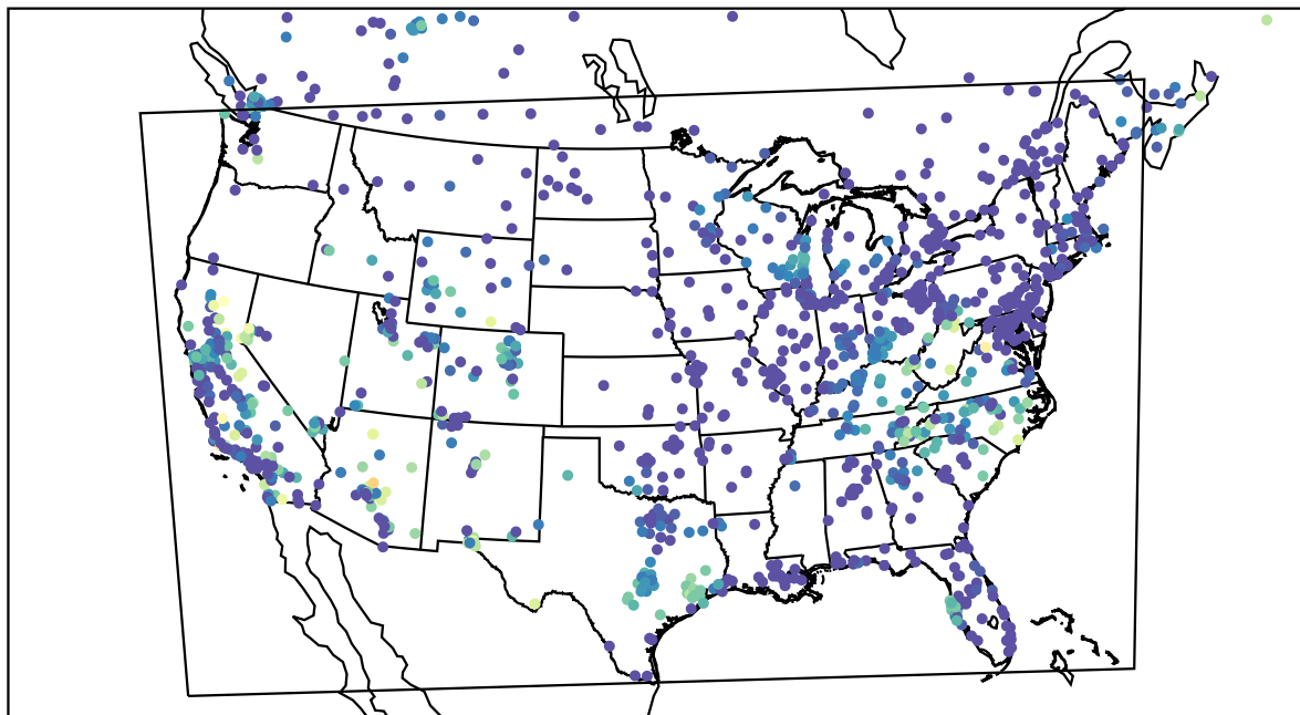
AirNOW (2023-10-14_07:00:00)
