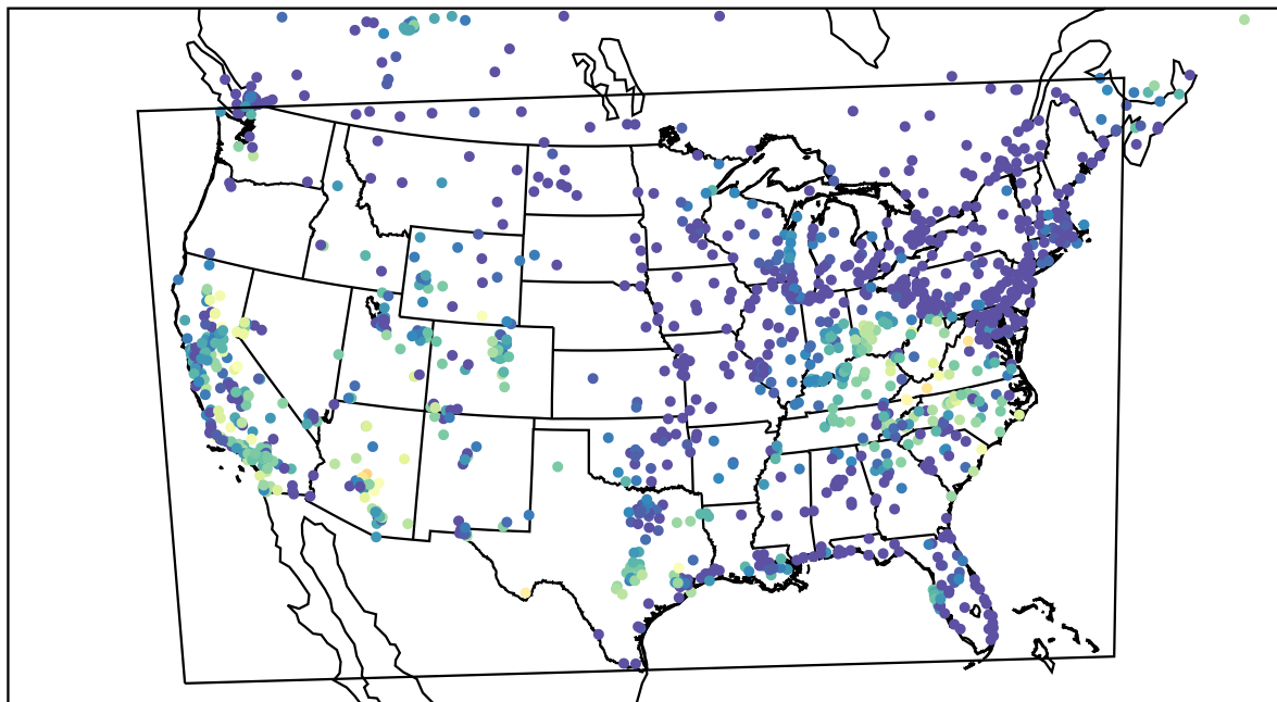
AirNOW (2023-10-14_03:00:00)
