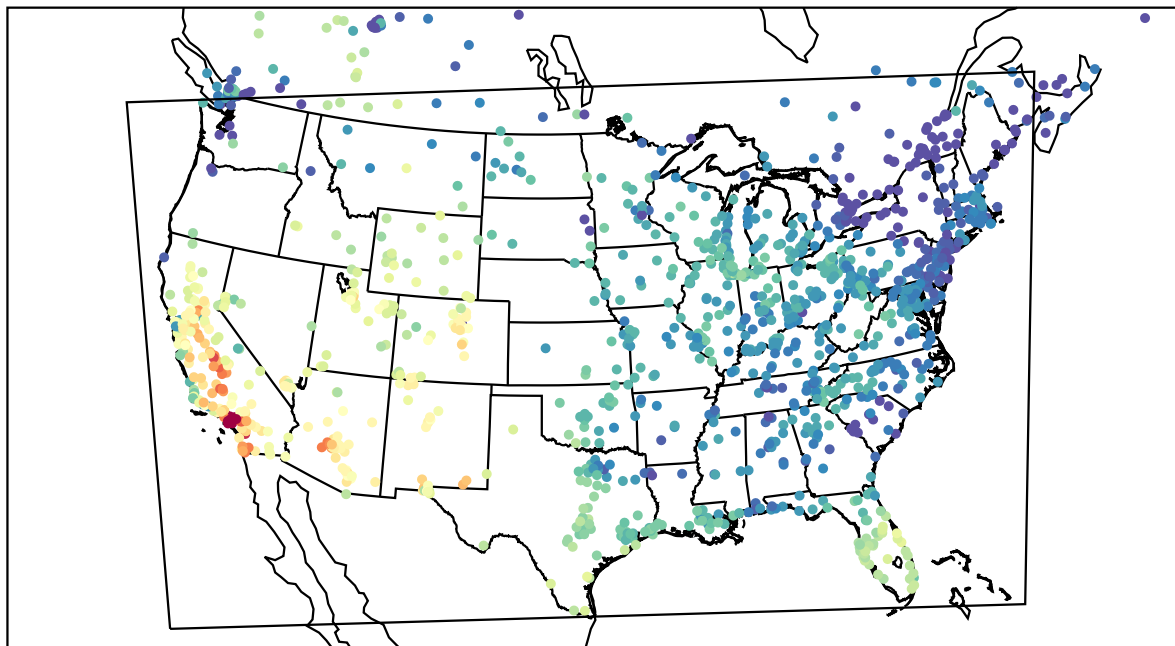
AirNOW (2023-10-15_21:00:00)
