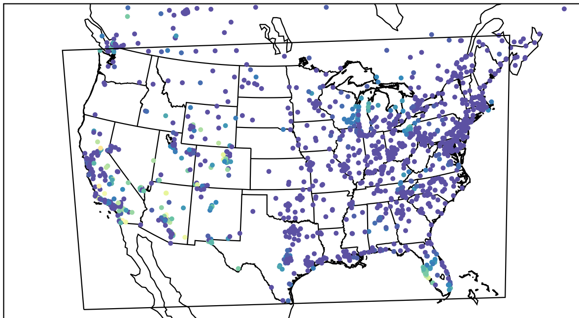
AirNOW (2023-10-15_12:00:00)
