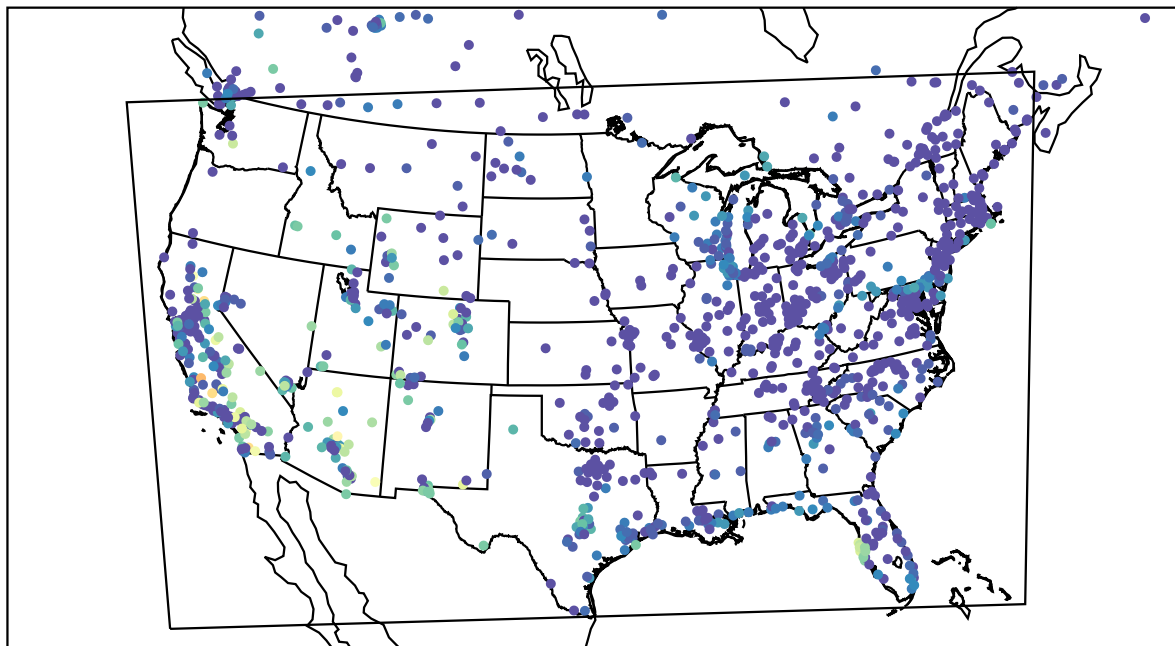
AirNOW (2023-10-15_06:00:00)
