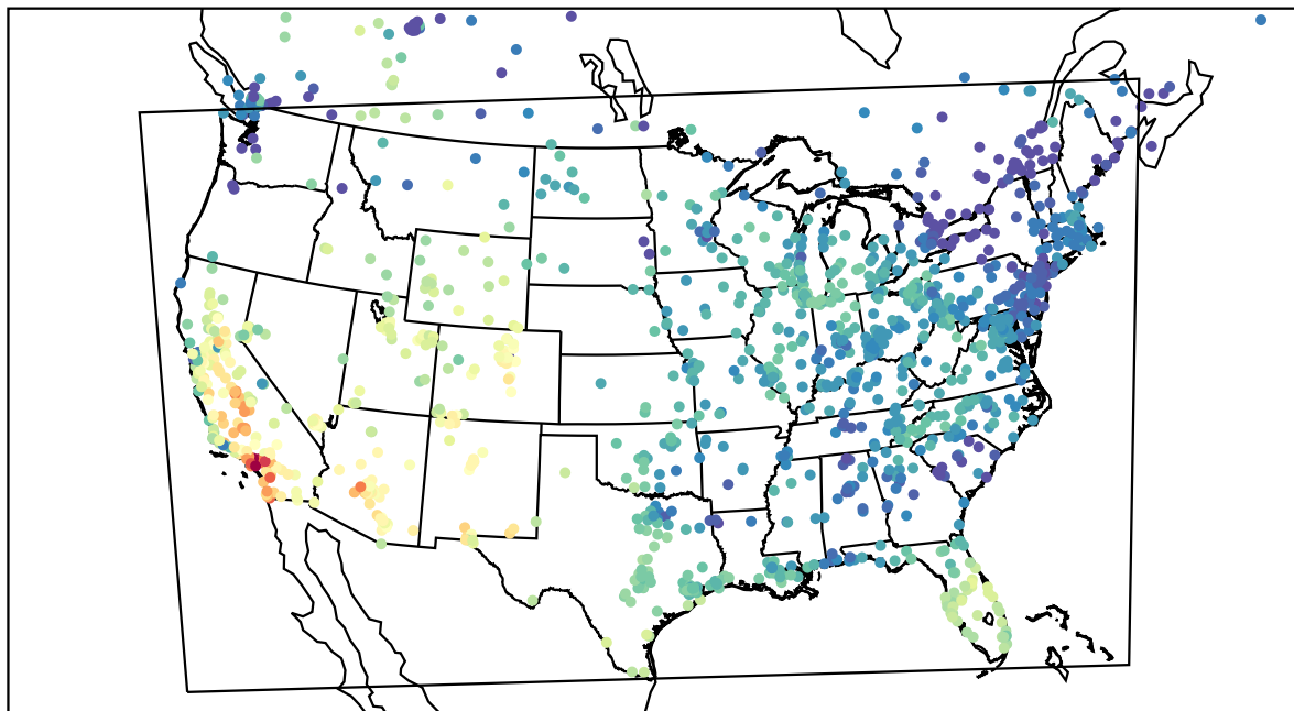
AirNOW (2023-10-15_20:00:00)
