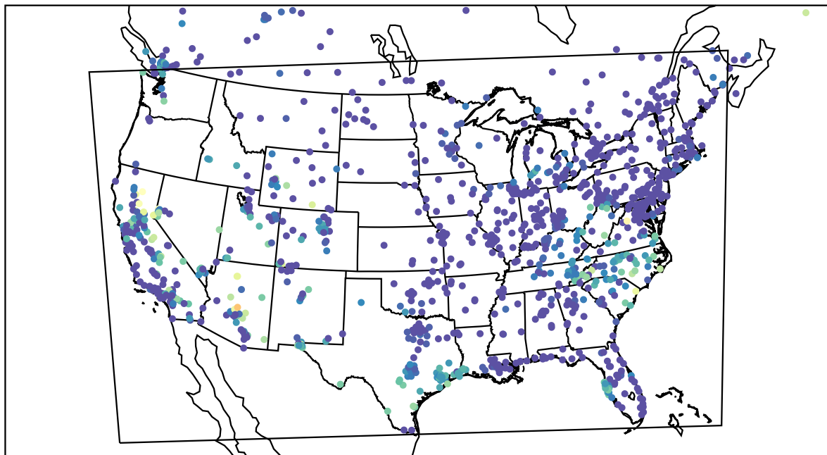
AirNOW (2023-10-14_10:00:00)
