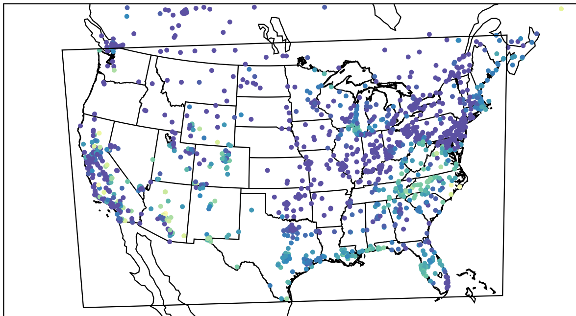
AirNOW (2023-10-14_15:00:00)
