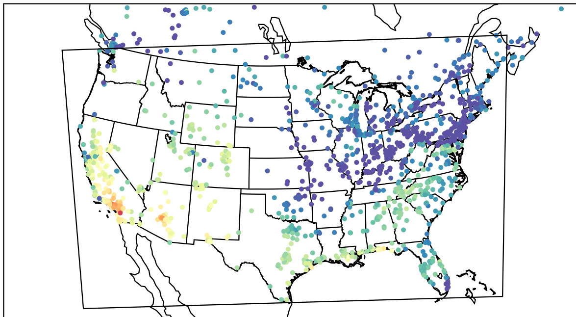
AirNOW (2023-10-14_20:00:00)
