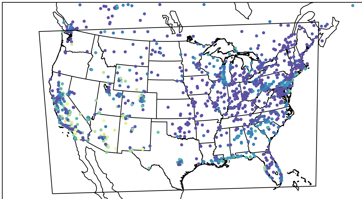
AirNOW (2023-10-15_04:00:00)
