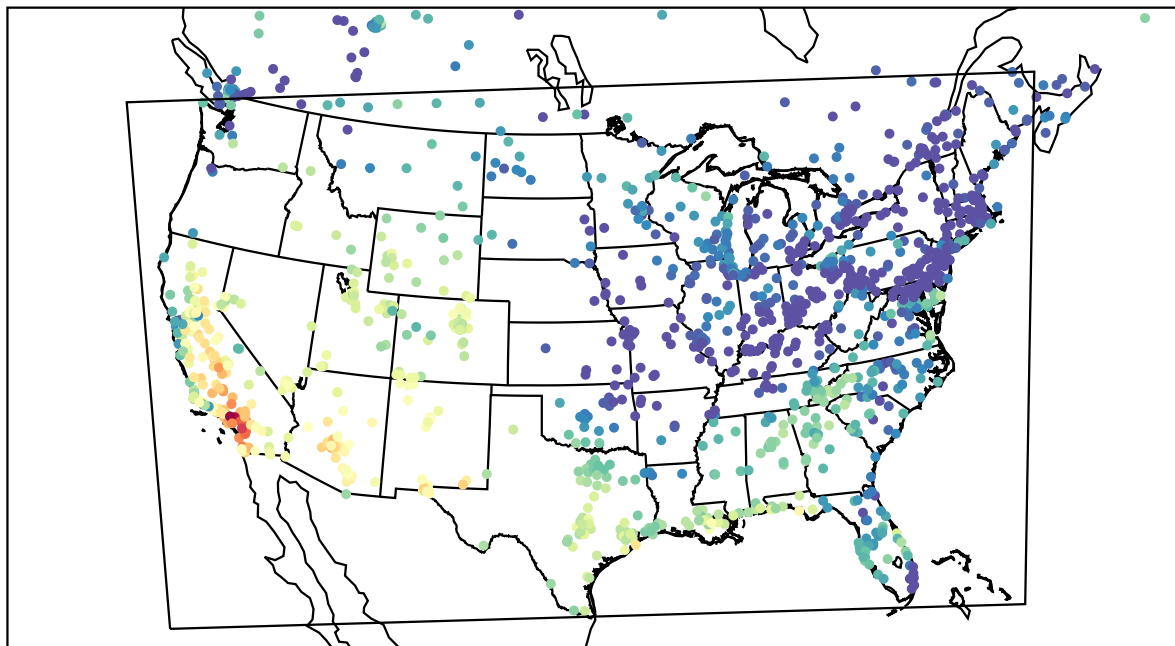
AirNOW (2023-10-14_22:00:00)
