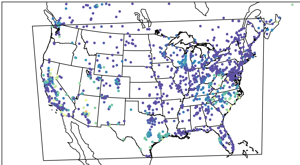
AirNOW (2023-10-14_09:00:00)
