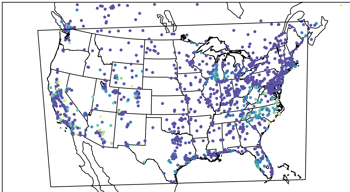
AirNOW (2023-10-14_13:00:00)
