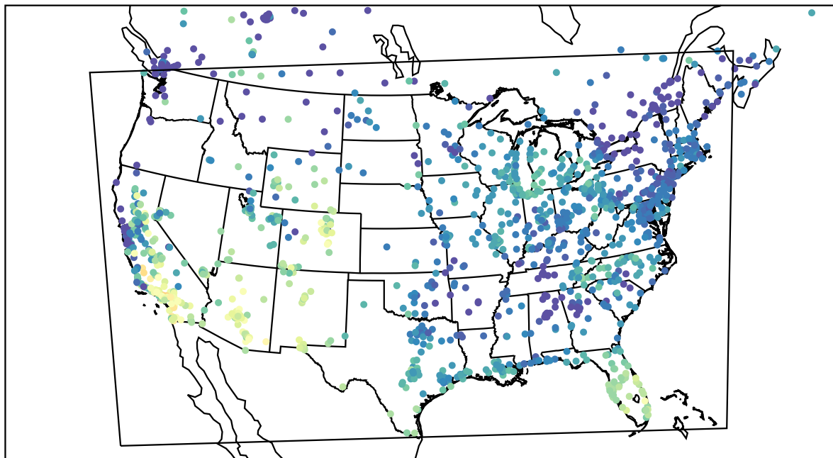
AirNOW (2023-10-15_17:00:00)
