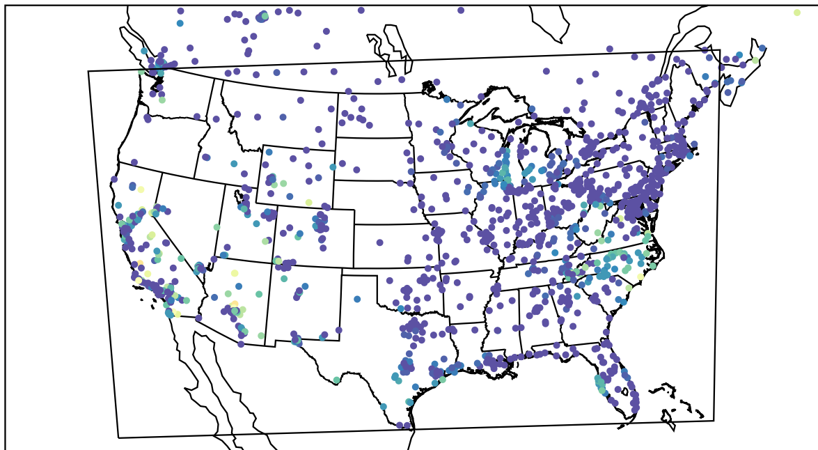
AirNOW (2023-10-14_12:00:00)
