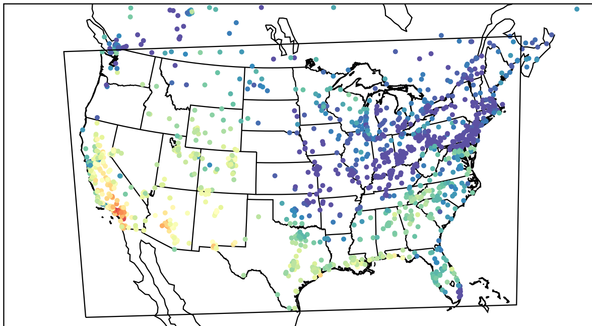
AirNOW (2023-10-14_21:00:00)
