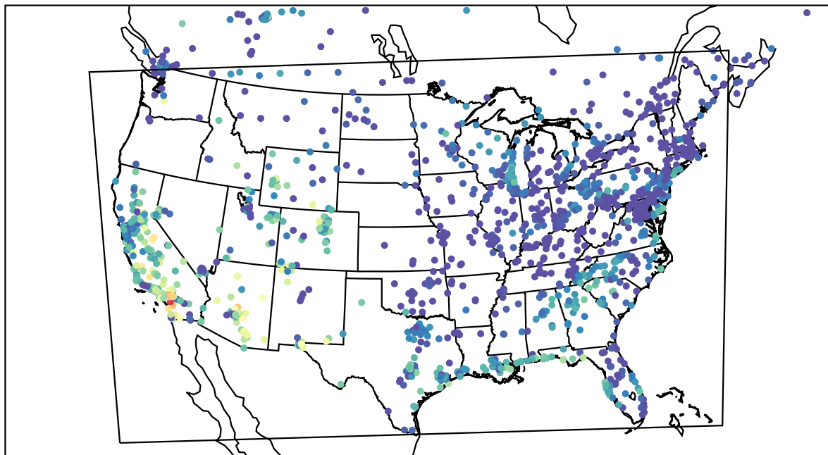
AirNOW (2023-10-15_02:00:00)
