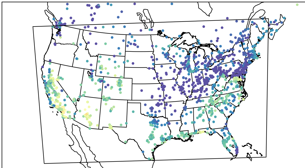
AirNOW (2023-10-14_18:00:00)
