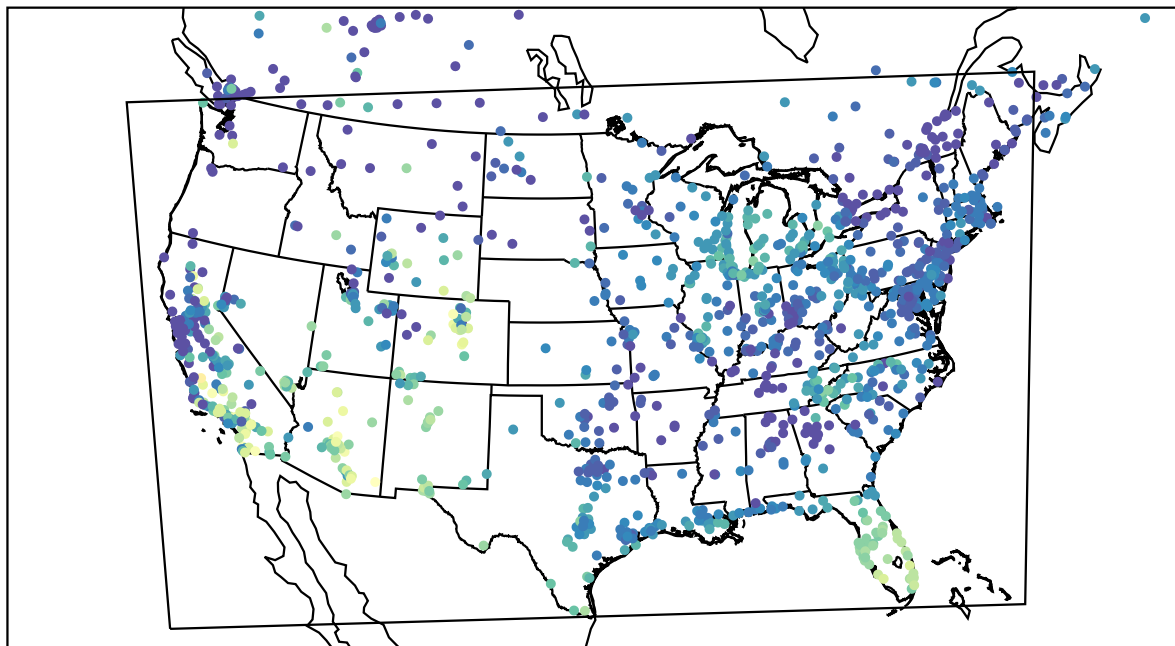
AirNOW (2023-10-15_16:00:00)
