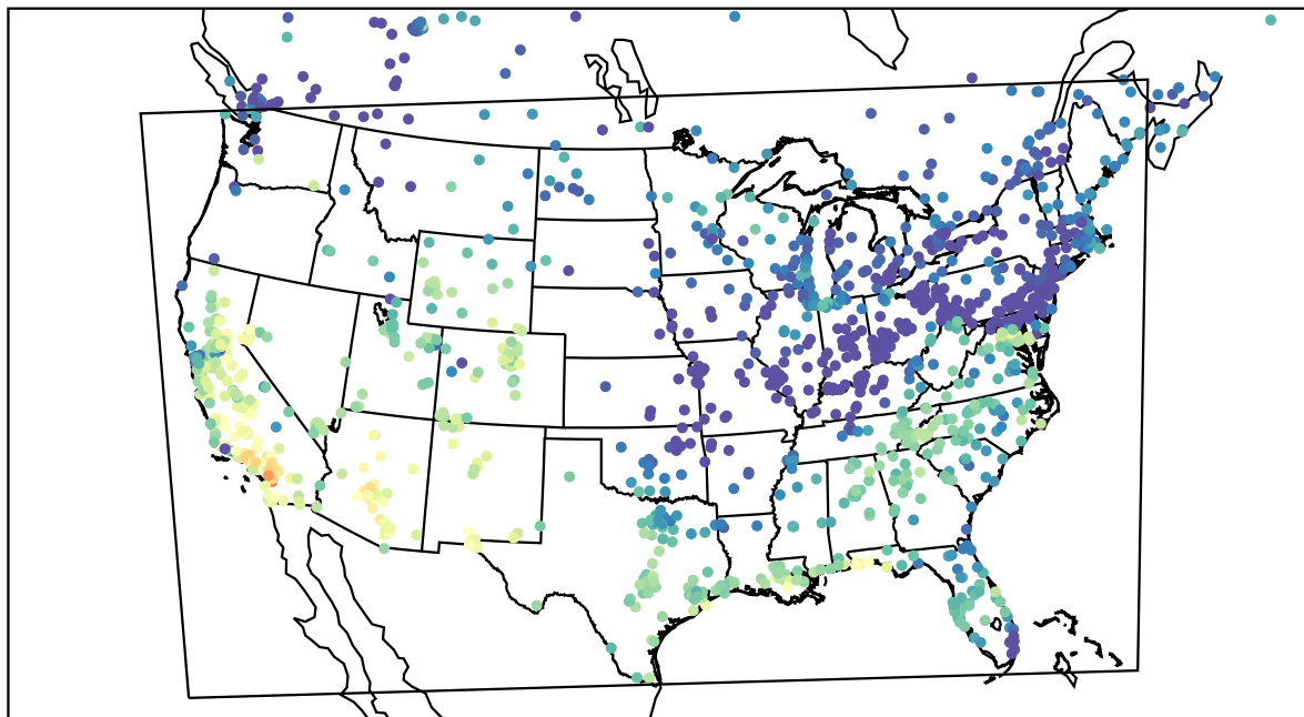
AirNOW (2023-10-14_19:00:00)
