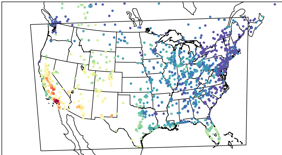
AirNOW (2023-10-15_23:00:00)
