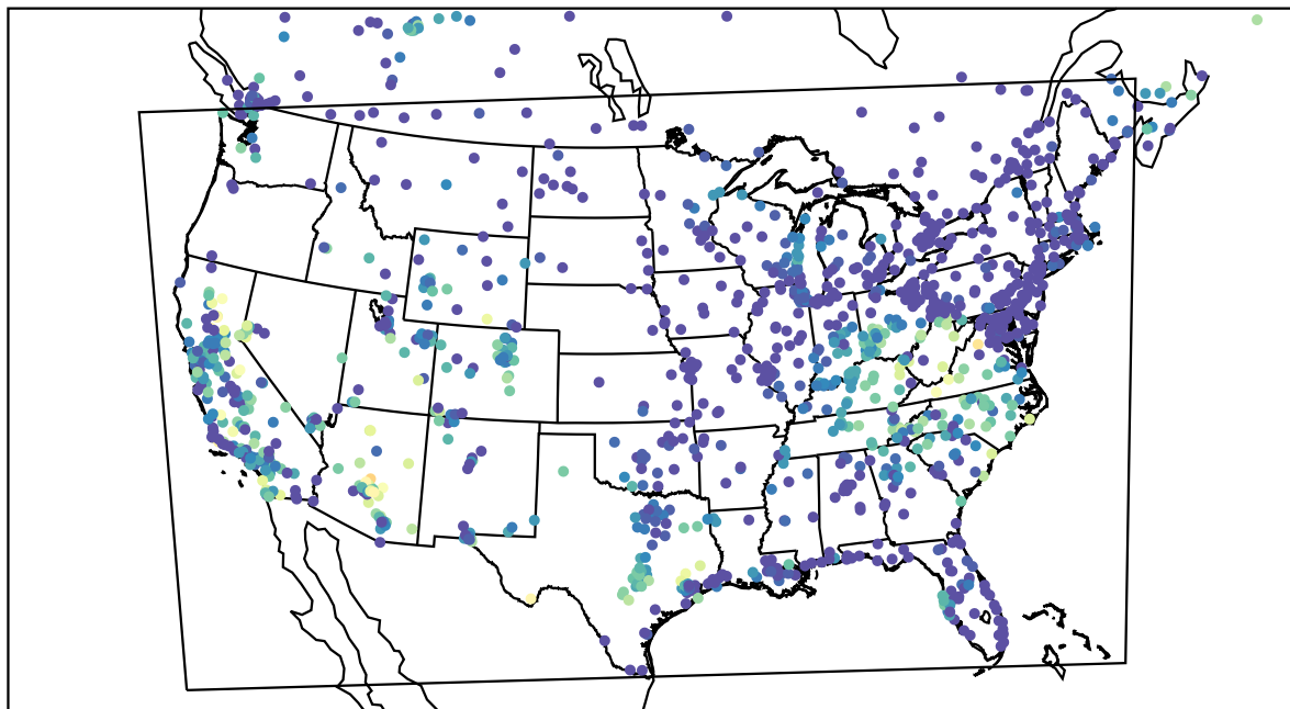
AirNOW (2023-10-14_04:00:00)
