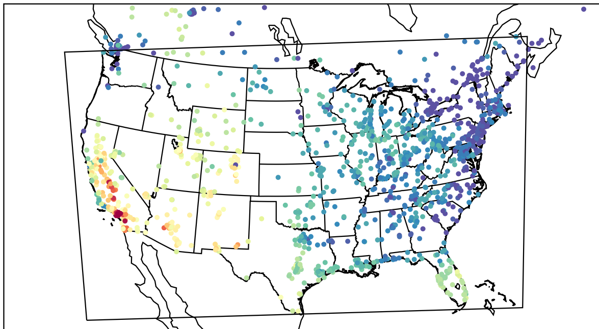
AirNOW (2023-10-15_22:00:00)
