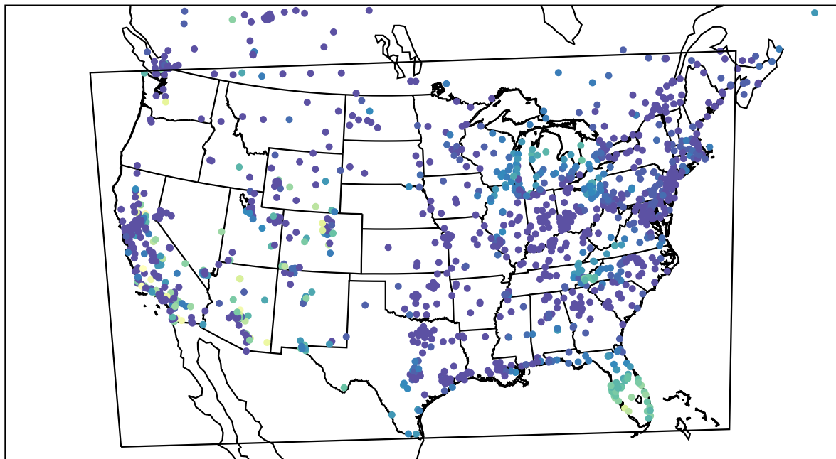
AirNOW (2023-10-15_14:00:00)
