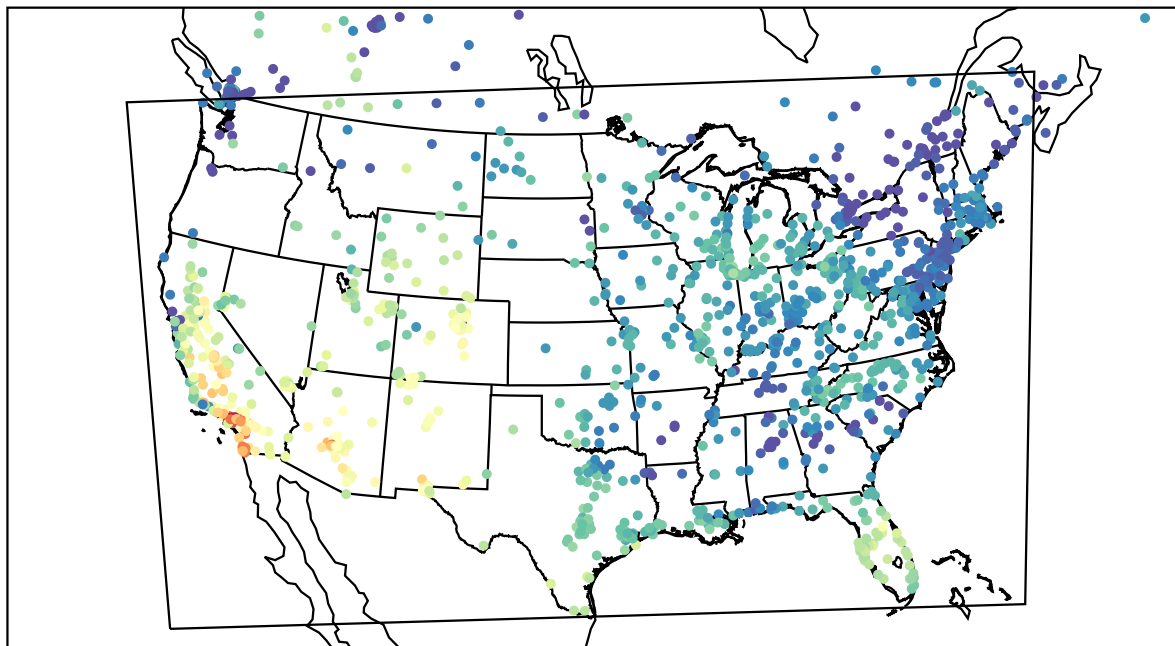
AirNOW (2023-10-15_19:00:00)
