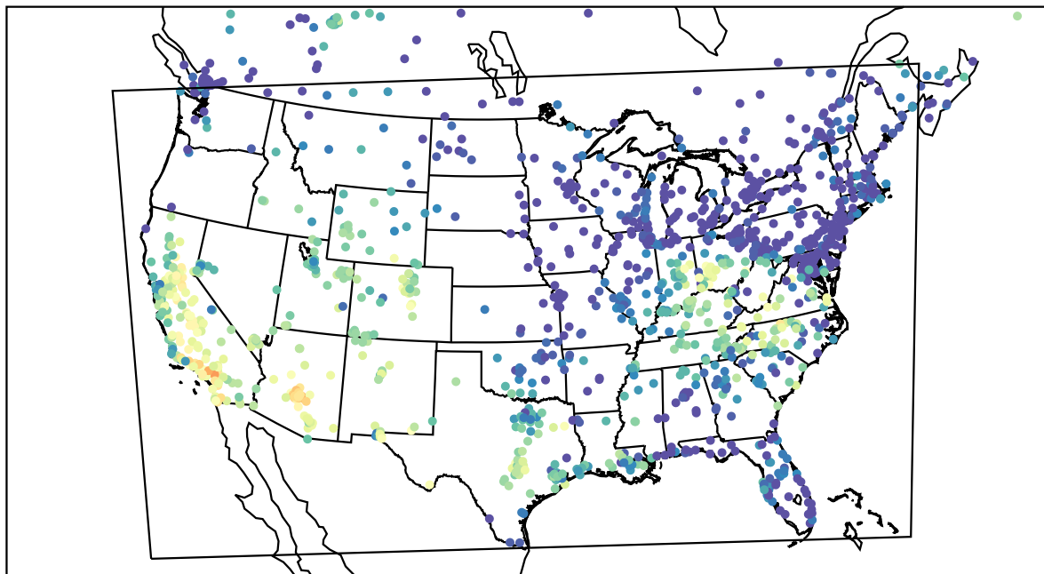
AirNOW (2023-10-14_00:00:00)
