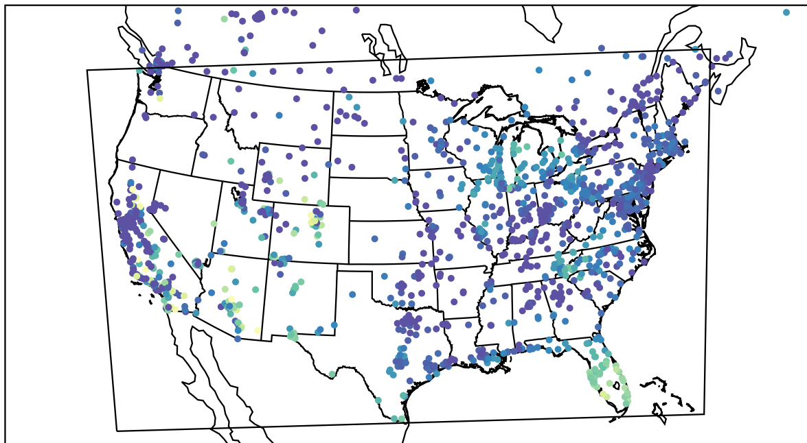
AirNOW (2023-10-15_15:00:00)
