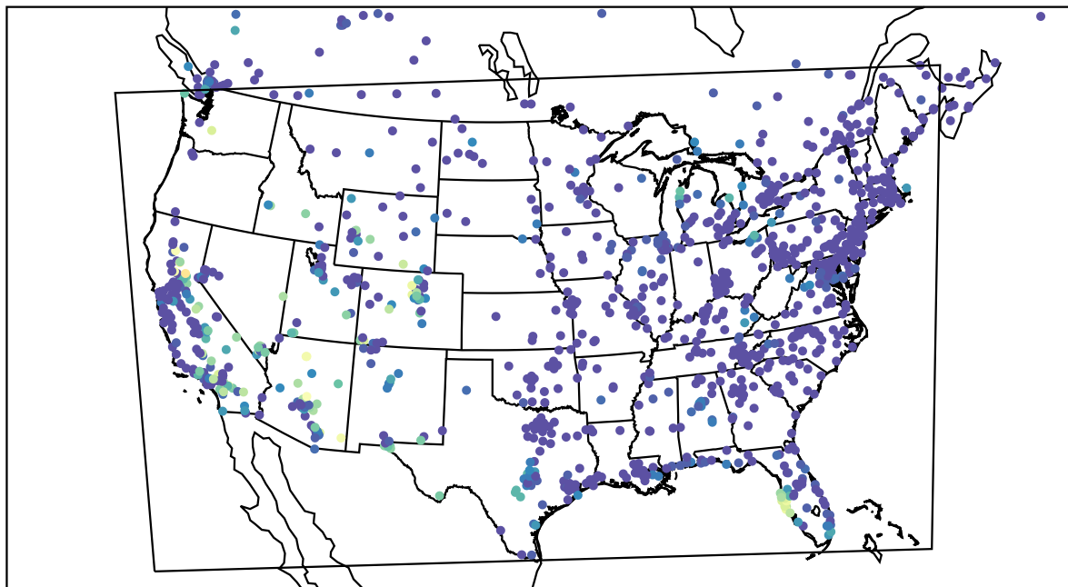
AirNOW (2023-10-15_10:00:00)
