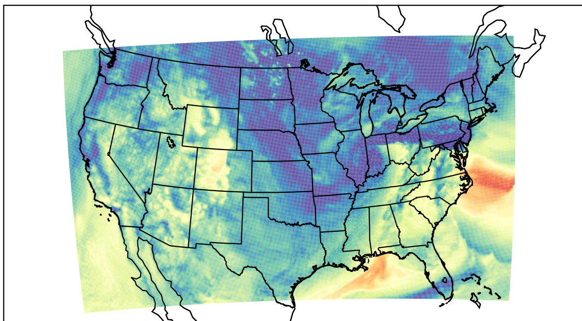
WRF (2023-10-14_16:00:00)
