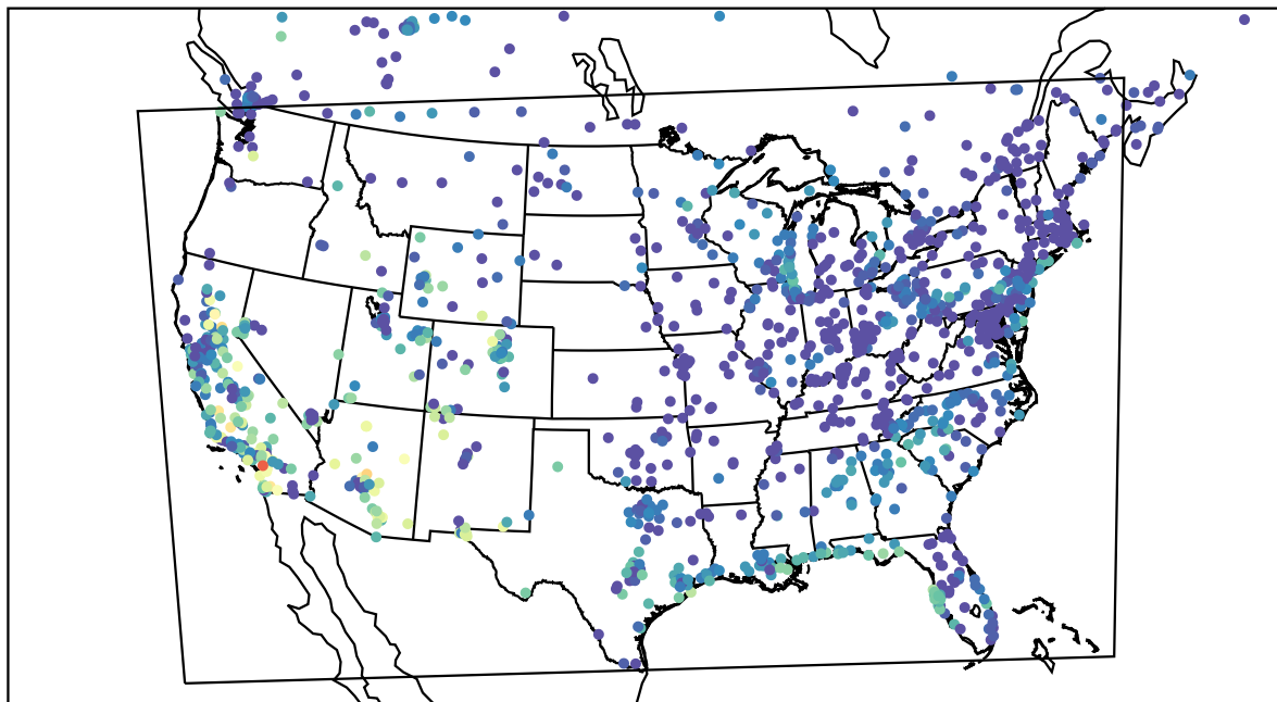
AirNOW (2023-10-15_03:00:00)
