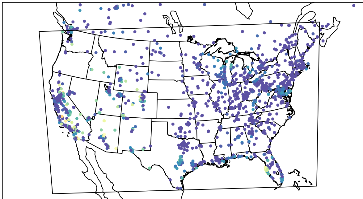
AirNOW (2023-10-15_08:00:00)
