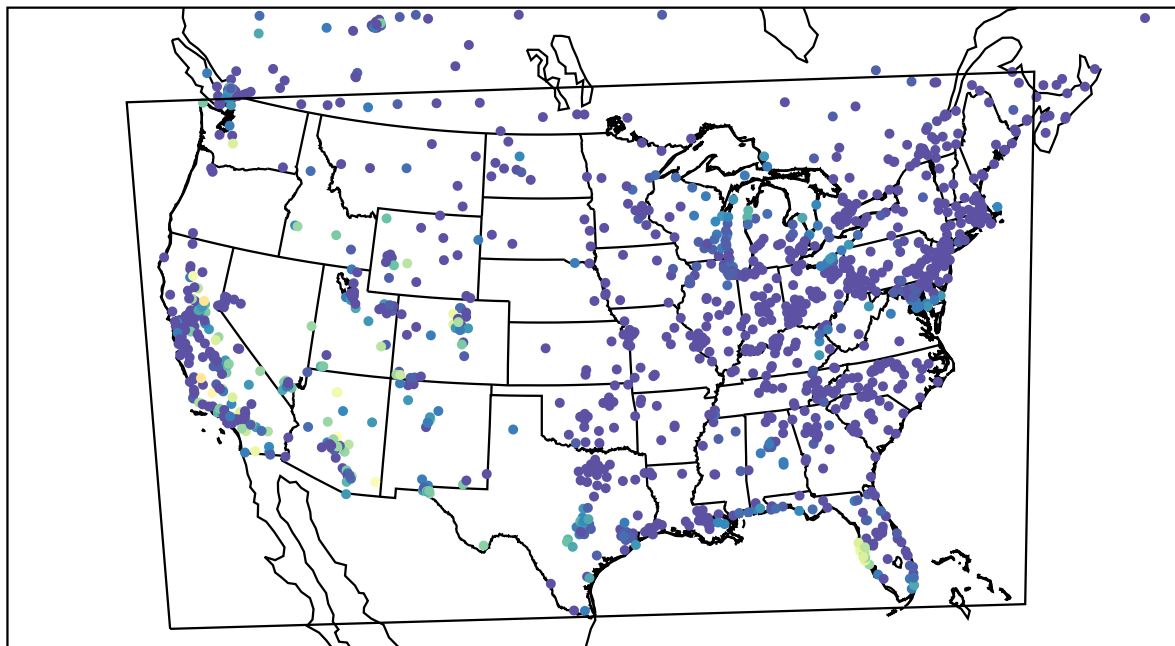
AirNOW (2023-10-15_09:00:00)
