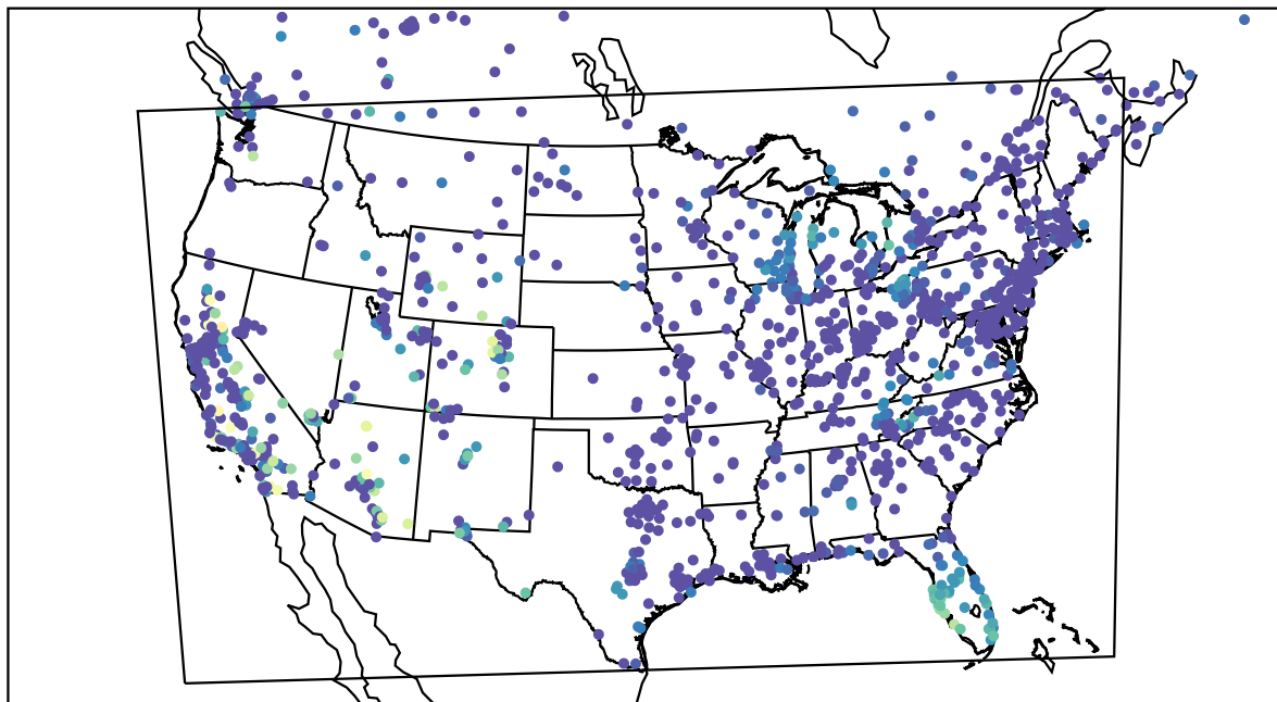
AirNOW (2023-10-15_13:00:00)
