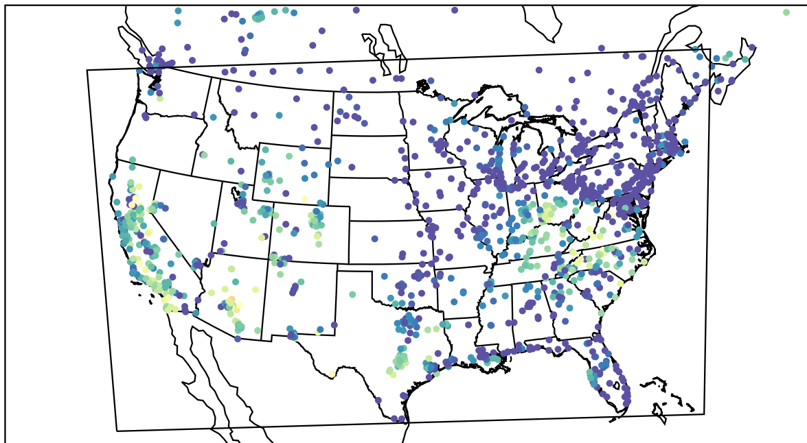
AirNOW (2023-10-14_02:00:00)
