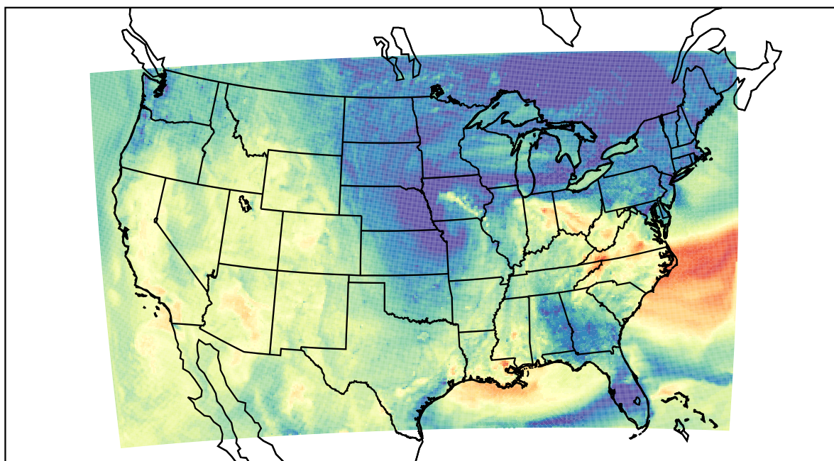
WRF (2023-10-14_00:00:00)
