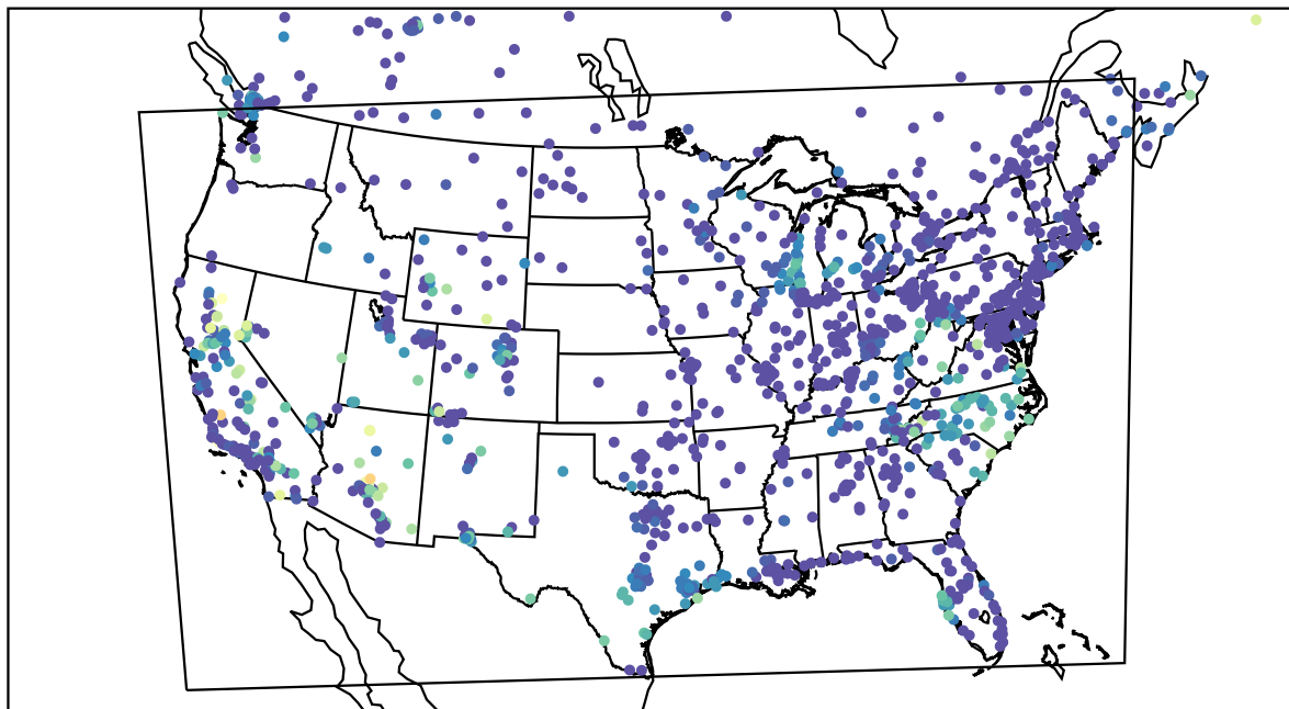
AirNOW (2023-10-14_11:00:00)
