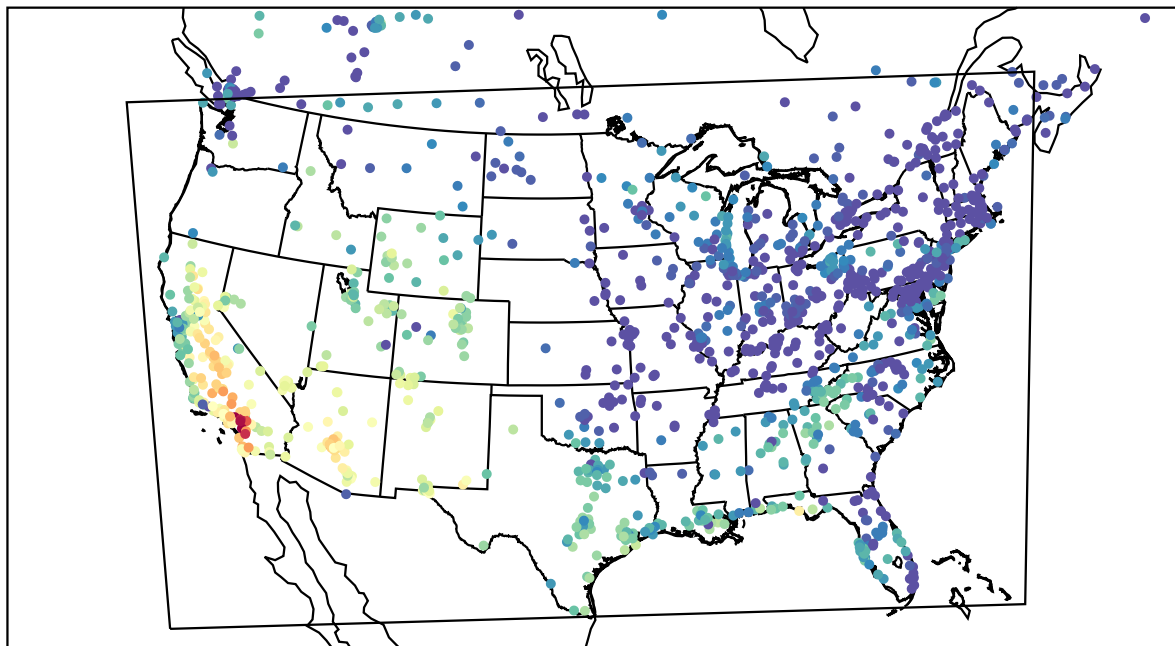
AirNOW (2023-10-15_00:00:00)
