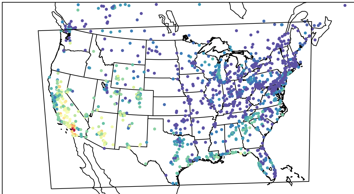
AirNOW (2023-10-15_01:00:00)
