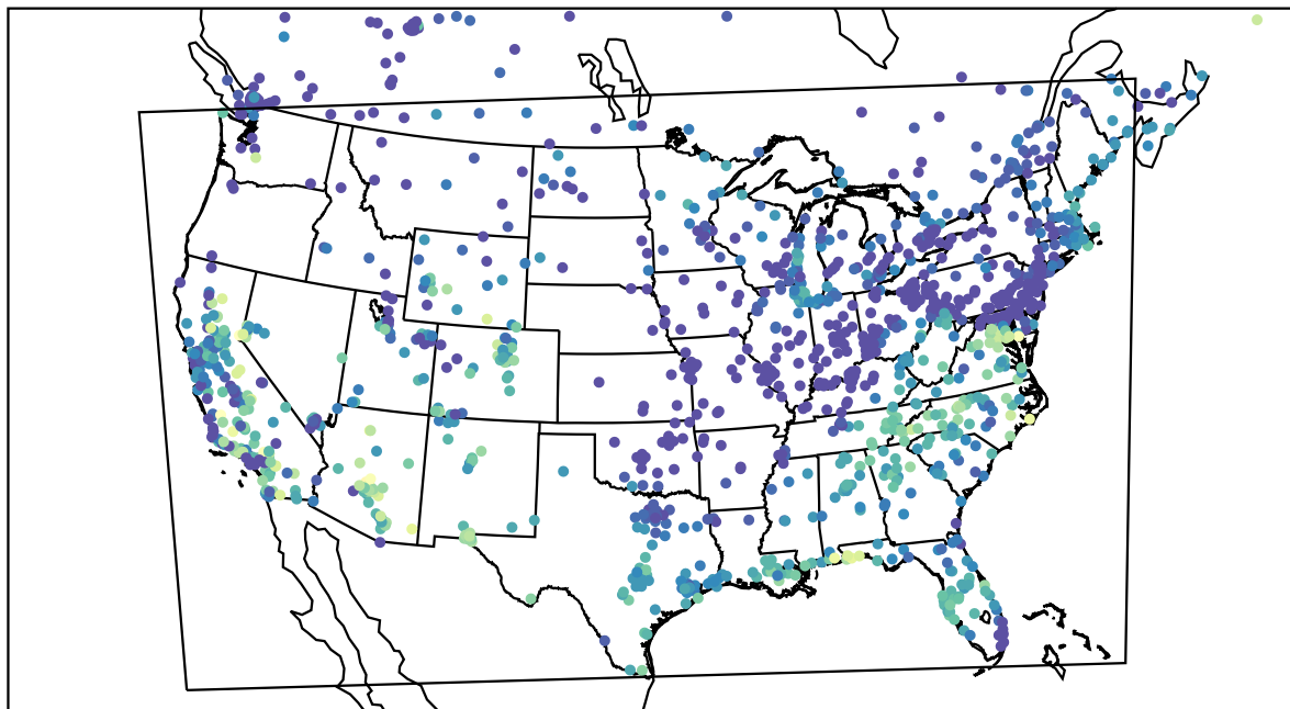
AirNOW (2023-10-14_17:00:00)
