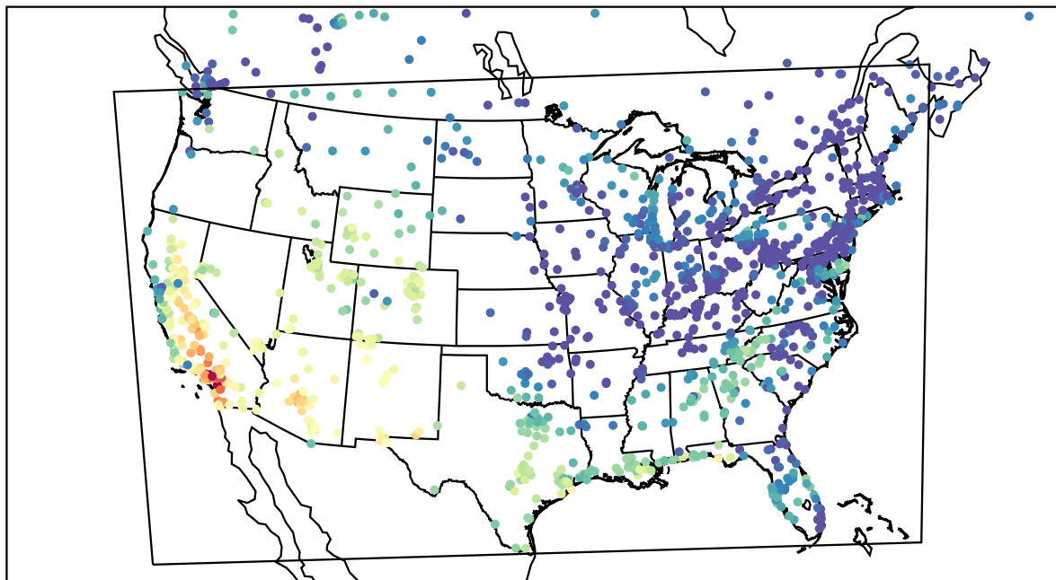
AirNOW (2023-10-14_23:00:00)
