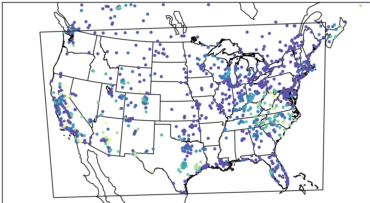
AirNOW (2023-10-14_06:00:00)
