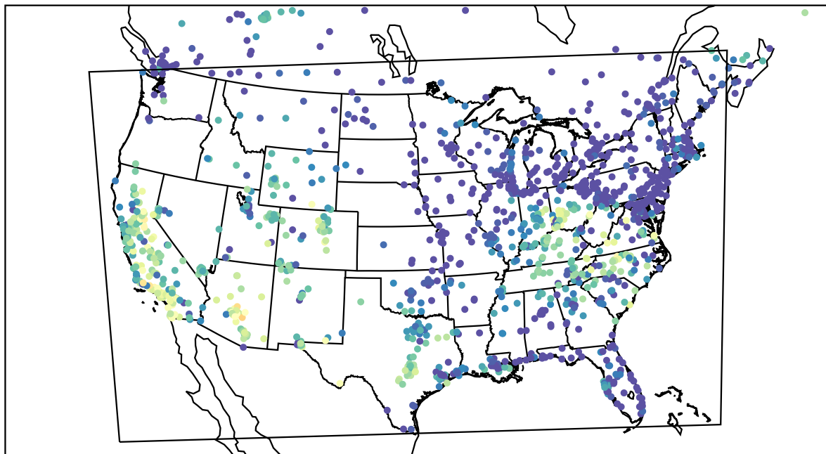
AirNOW (2023-10-14_01:00:00)
