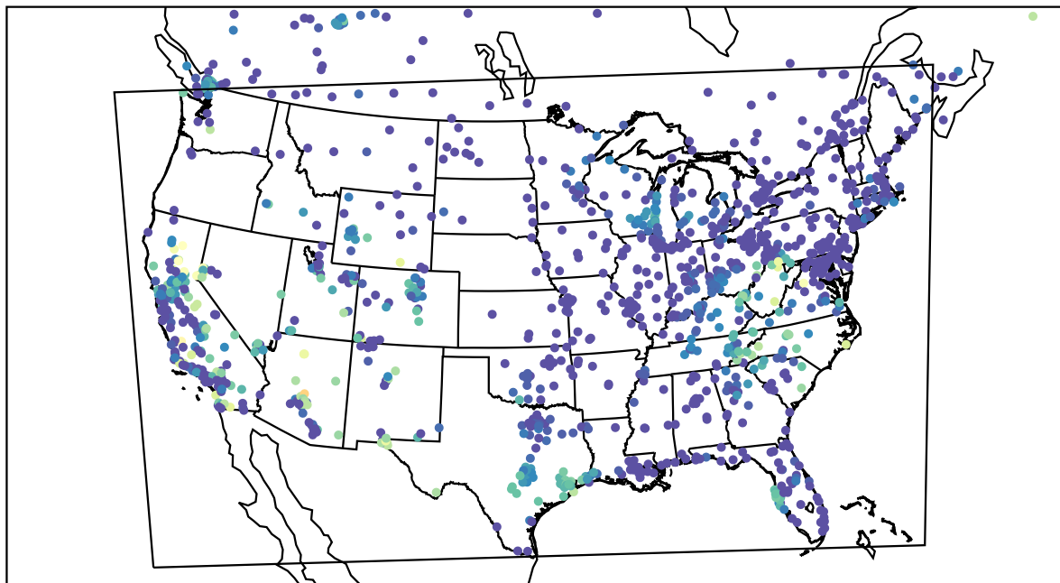
AirNOW (2023-10-14_08:00:00)
