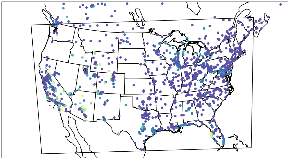
AirNOW (2023-10-15_07:00:00)
