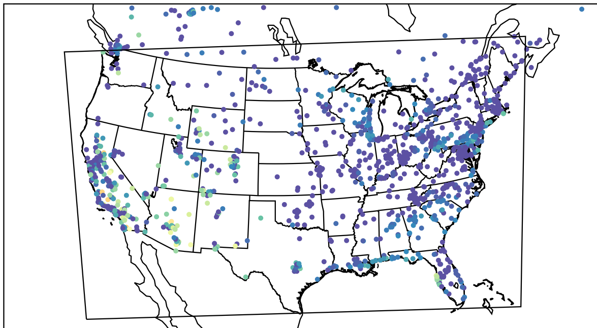
AirNOW (2023-10-15_05:00:00)
