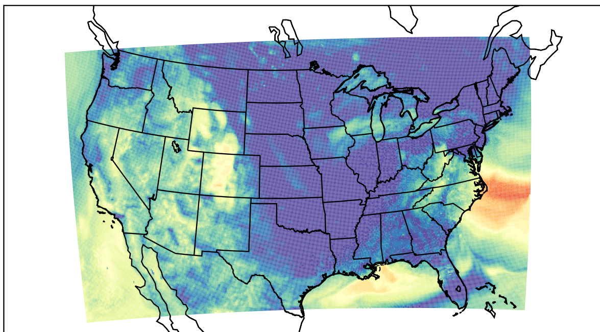
WRF (2023-10-14_12:00:00)
