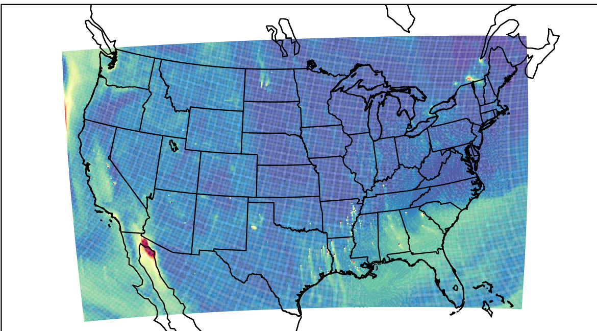
WRF 2023-10-15_21:00:00
