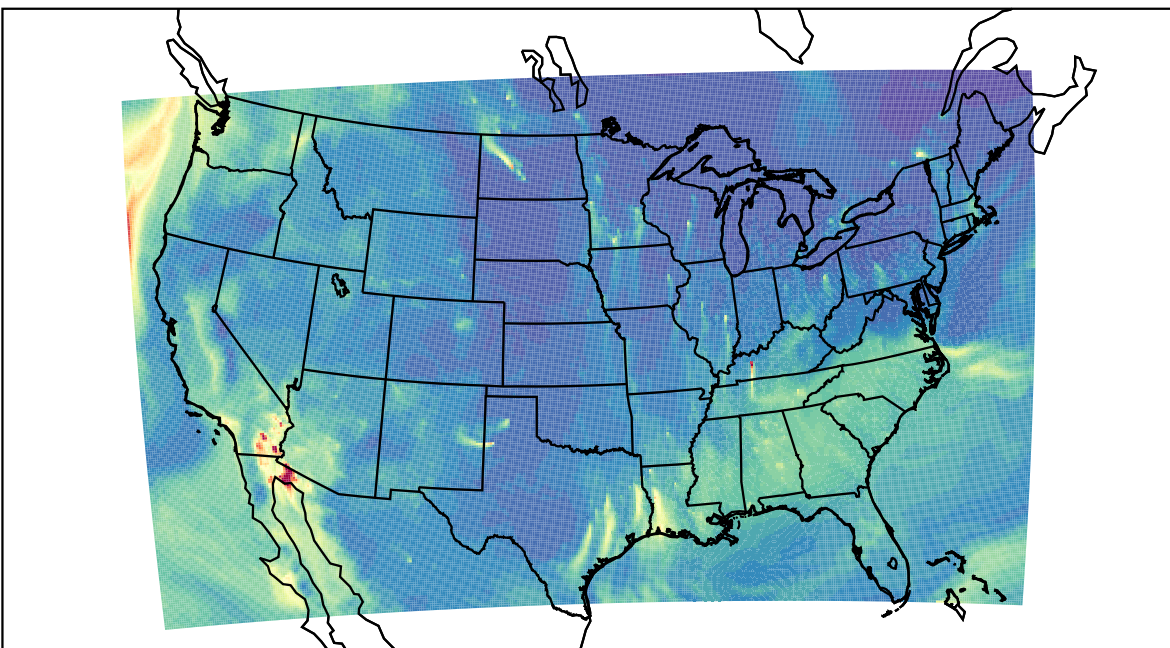
WRF 2023-10-15_10:00:00
