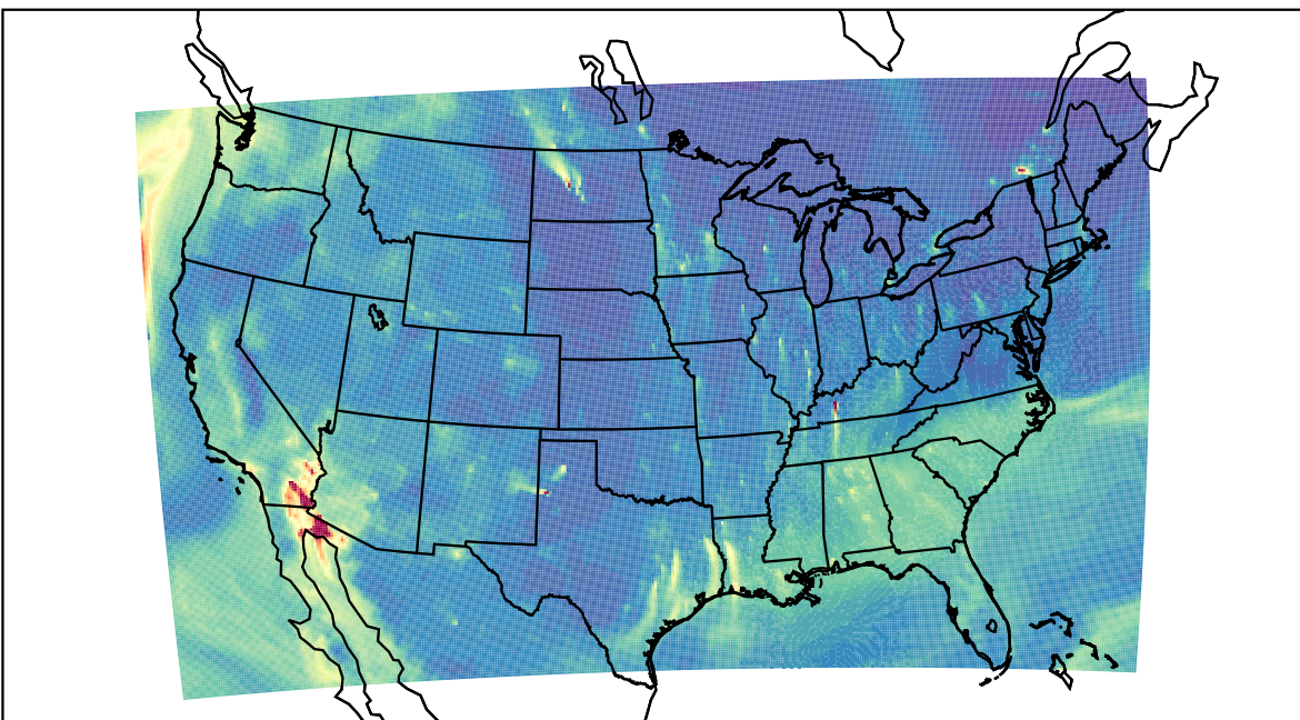
WRF 2023-10-15_13:00:00
