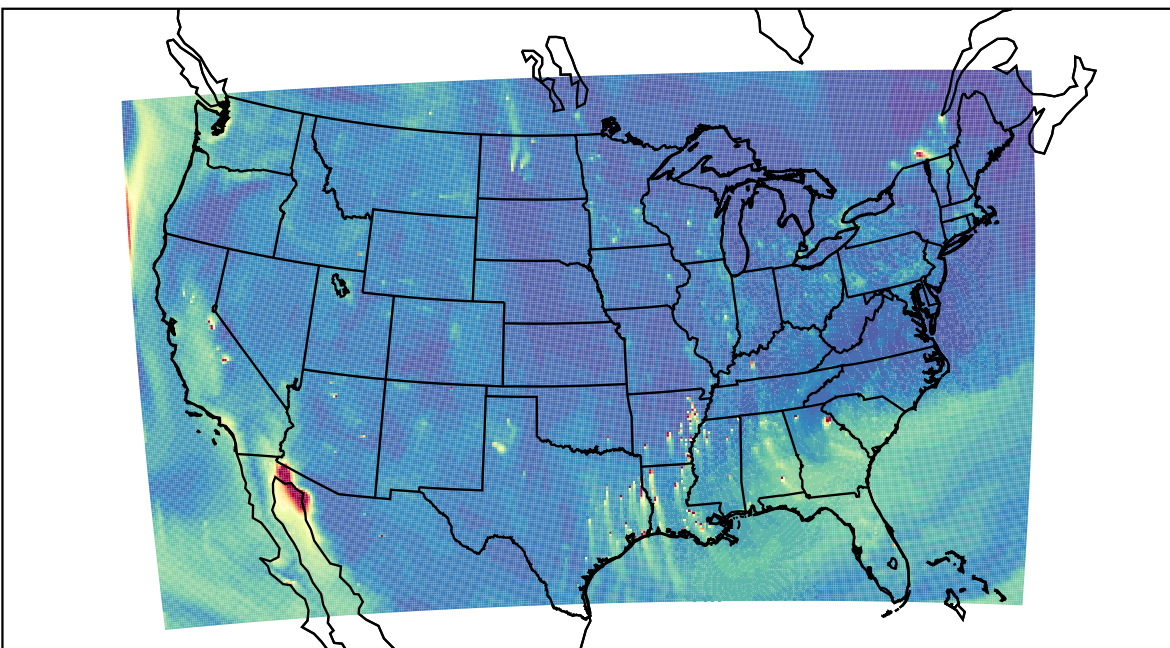
WRF 2023-10-15_23:00:00
