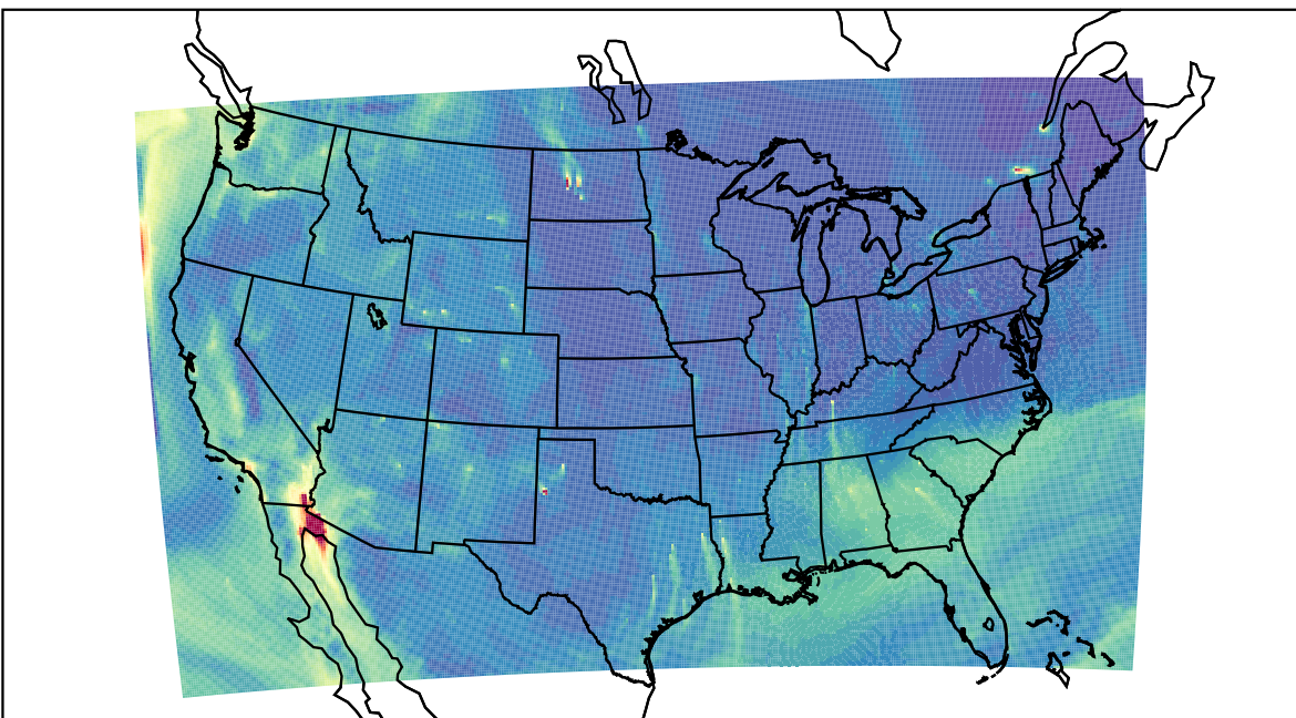
WRF 2023-10-15_17:00:00
