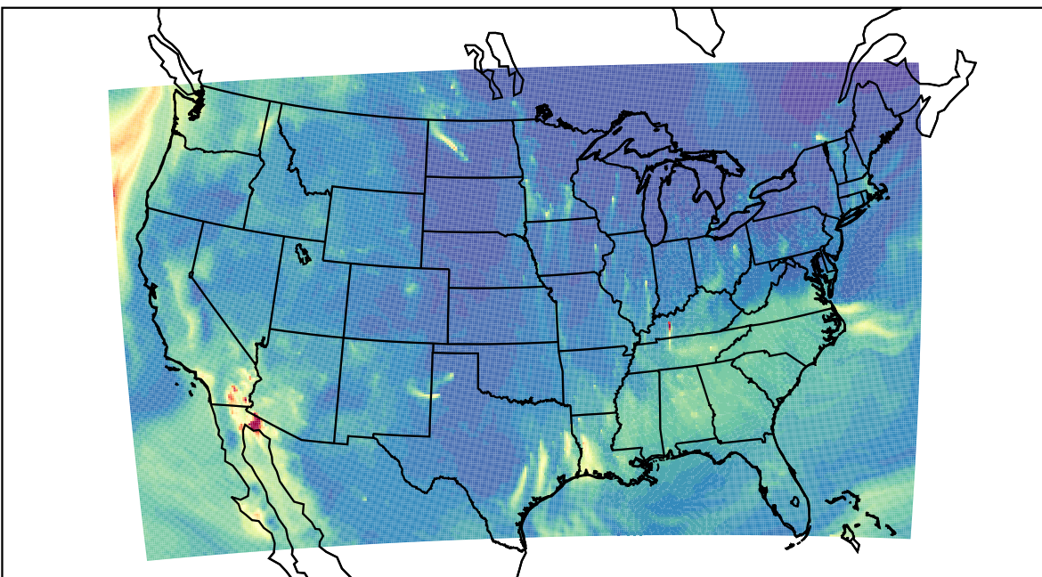
WRF 2023-10-15_09:00:00
