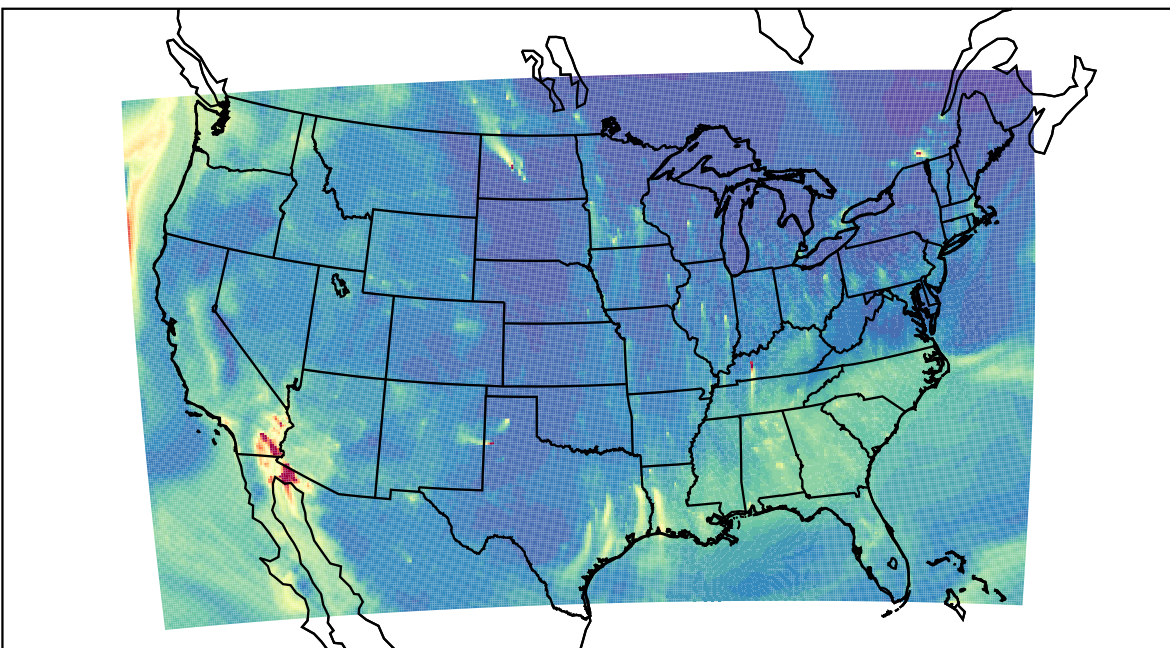
WRF 2023-10-15_12:00:00
