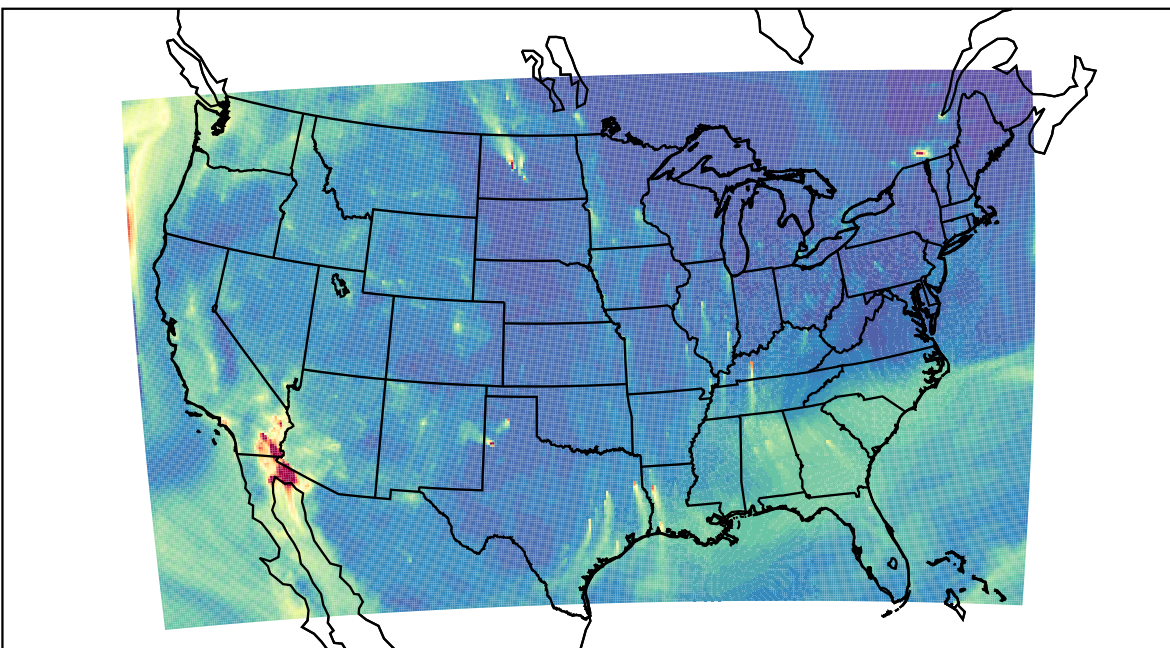
WRF 2023-10-15_15:00:00
