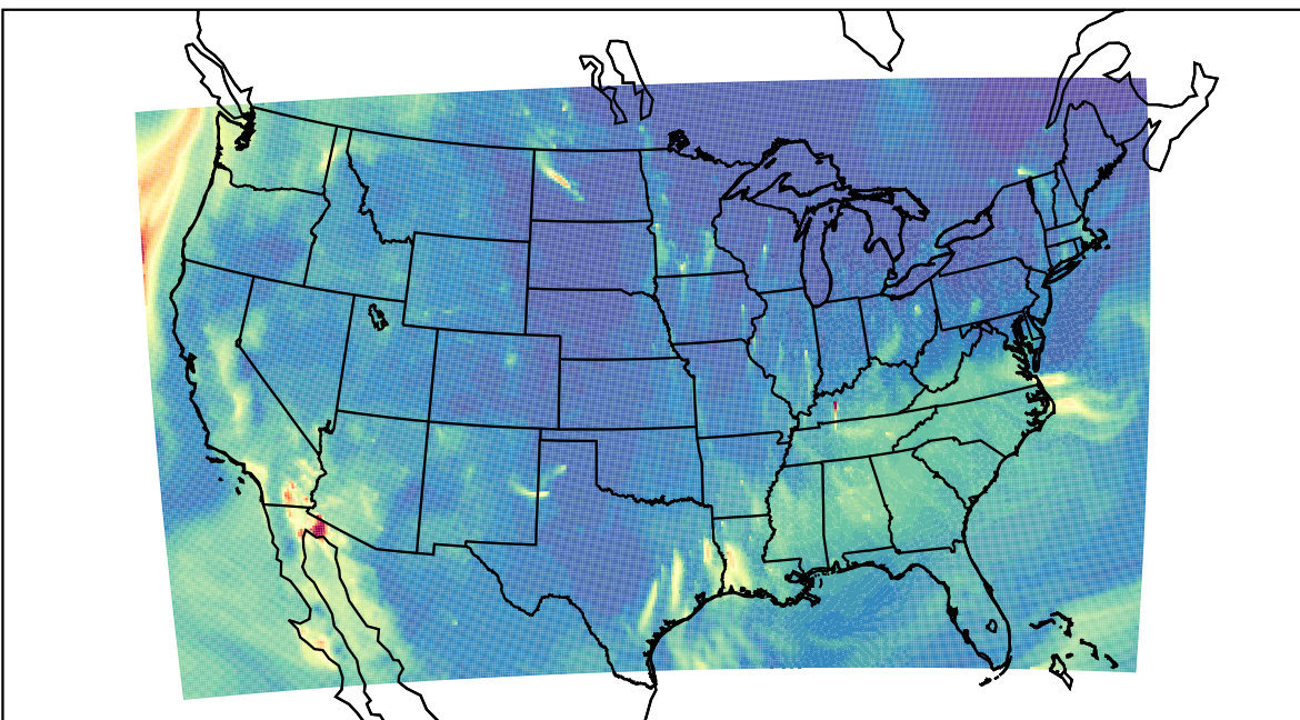
WRF 2023-10-15_08:00:00
