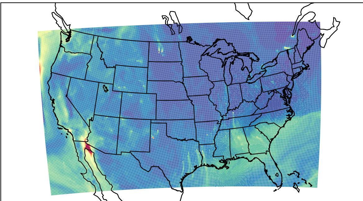
WRF 2023-10-15_18:00:00
