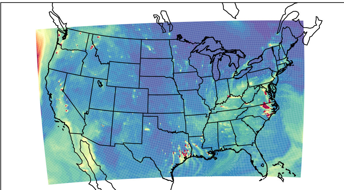
WRF 2023-10-15_00:00:00
