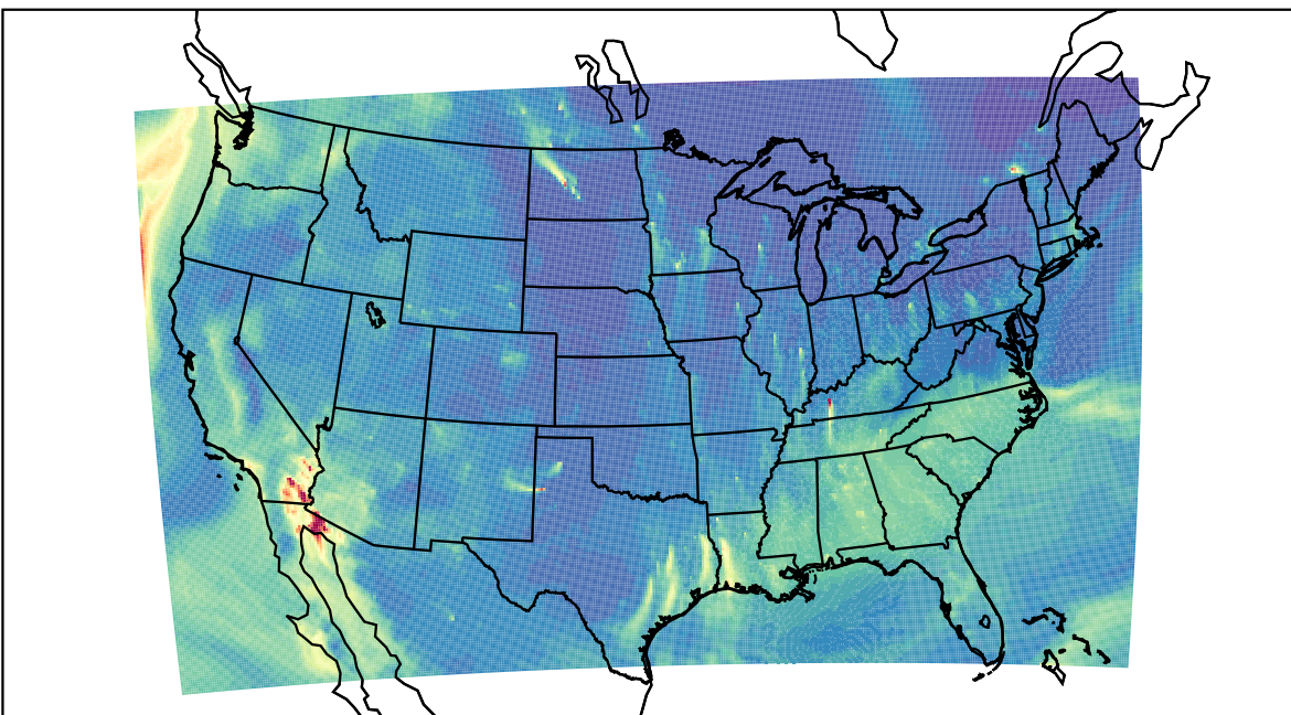
WRF 2023-10-15_11:00:00
