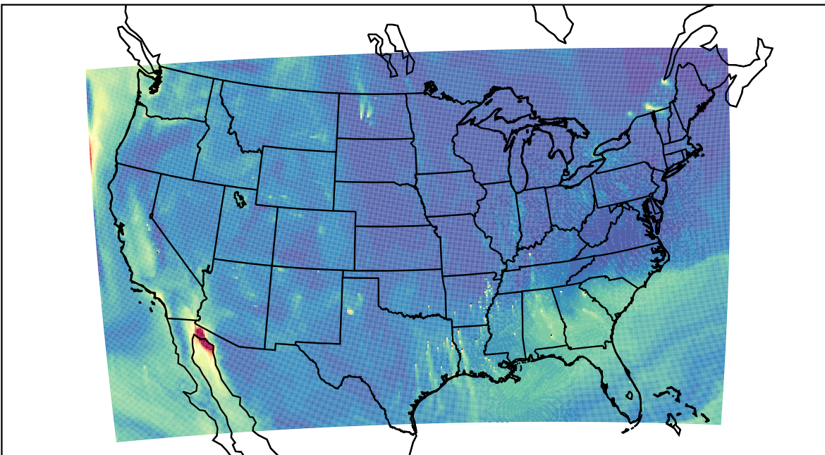
WRF 2023-10-15_20:00:00
