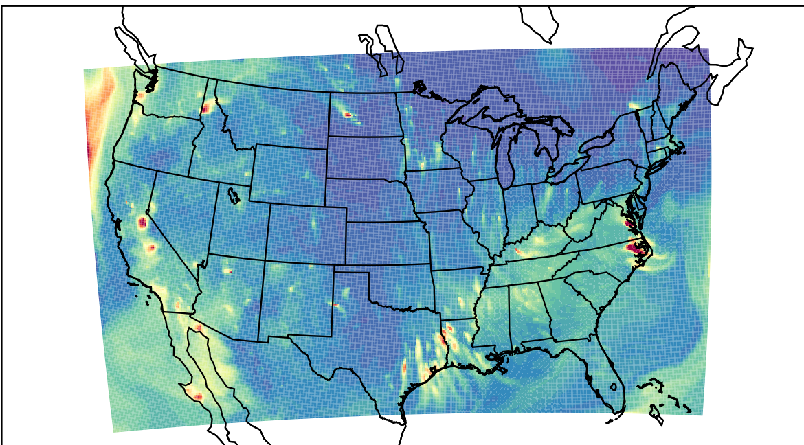
WRF 2023-10-15_04:00:00
