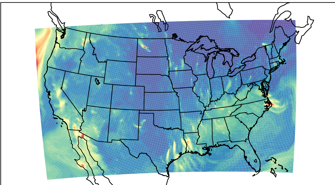
WRF 2023-10-15_06:00:00
