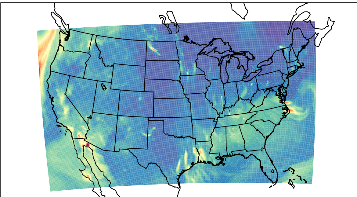
WRF 2023-10-15_07:00:00
