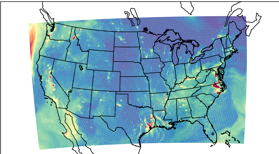
WRF 2023-10-15_01:00:00
