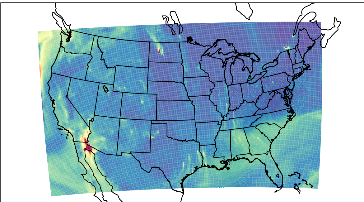
WRF 2023-10-15_16:00:00
