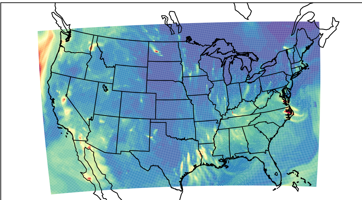
WRF 2023-10-15_05:00:00
