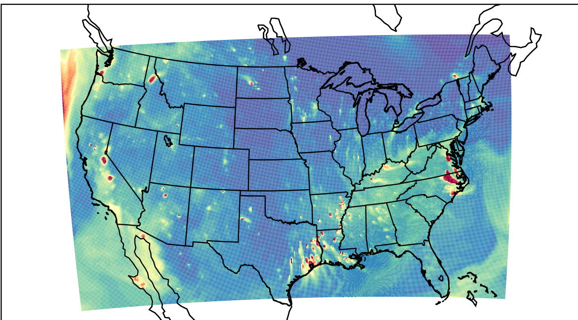
WRF 2023-10-15_02:00:00
