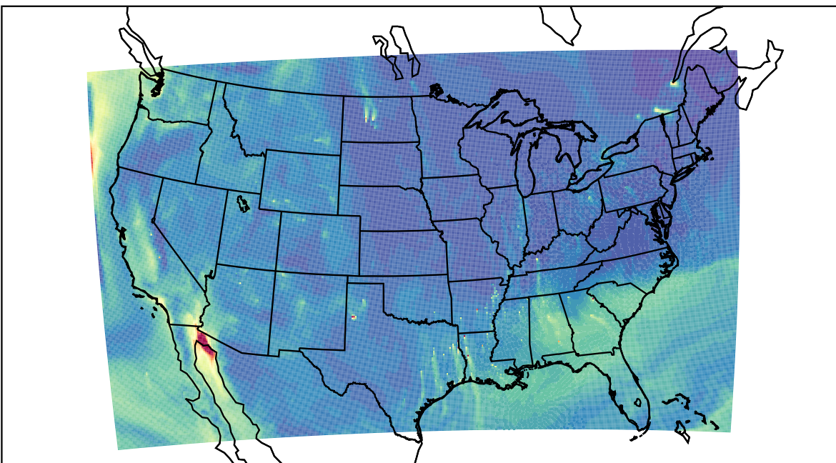
WRF 2023-10-15_19:00:00
