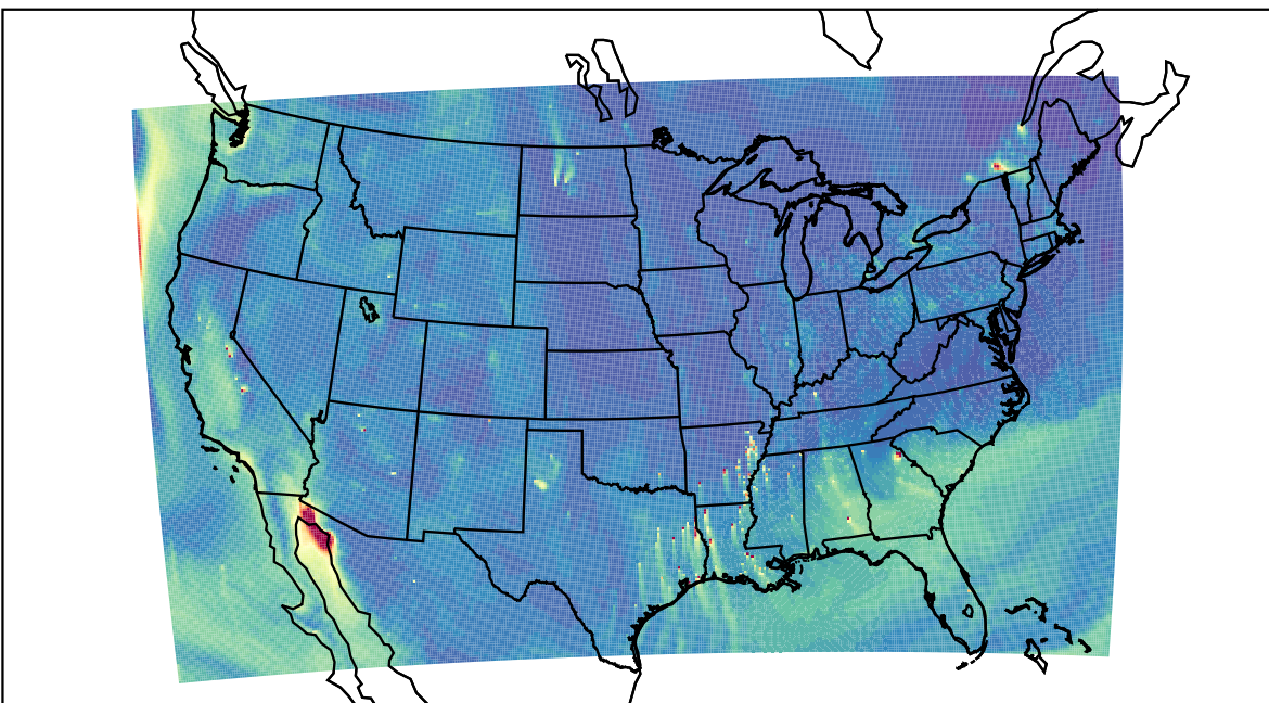
WRF 2023-10-15_22:00:00
