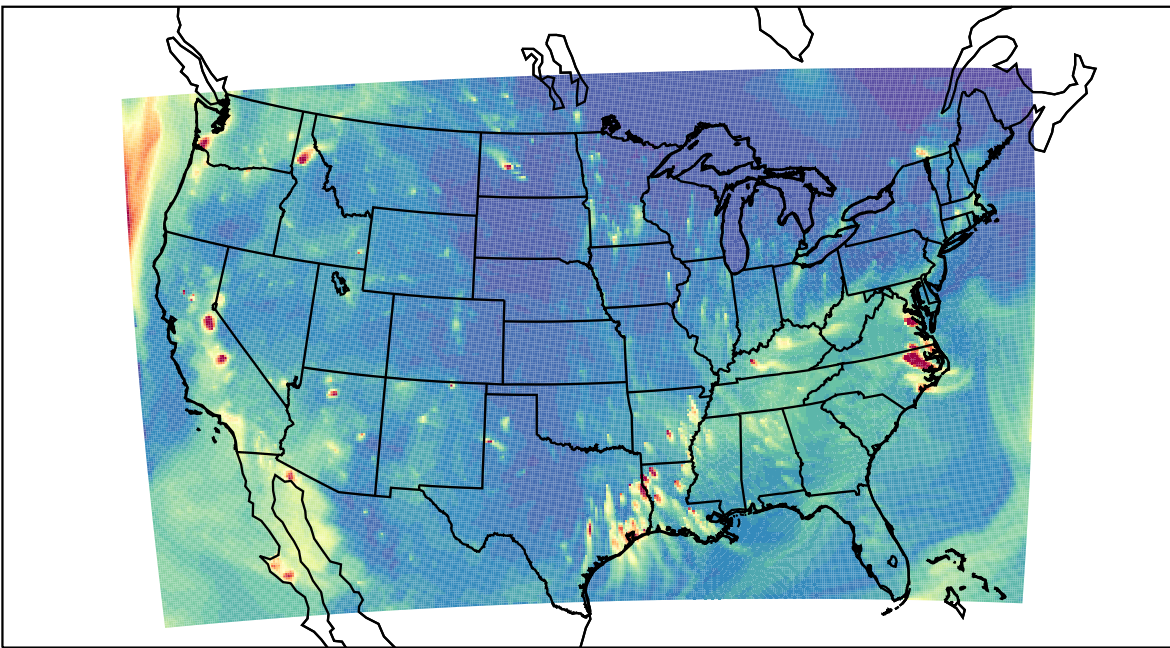
WRF 2023-10-15_03:00:00
