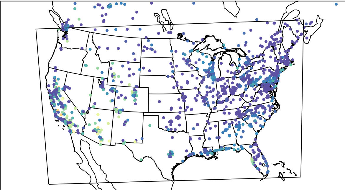
AirNOW (2023-10-15_05:00:00)
