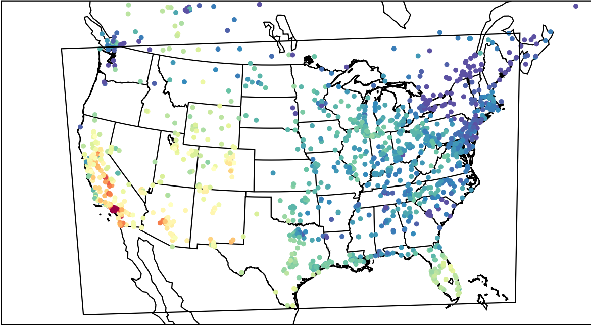
AirNOW (2023-10-15_21:00:00)
