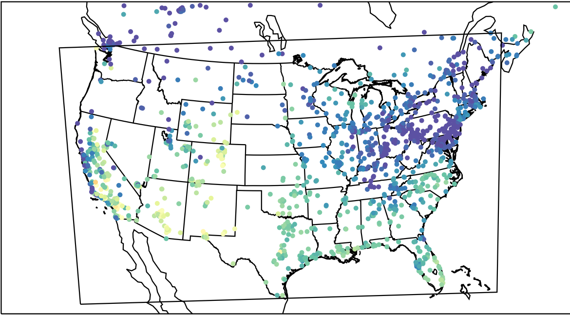
AirNOW (2023-10-16_17:00:00)
