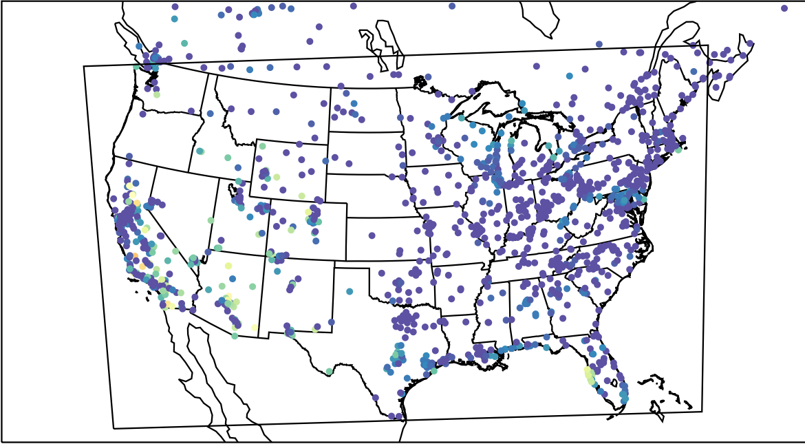
AirNOW (2023-10-15_07:00:00)
