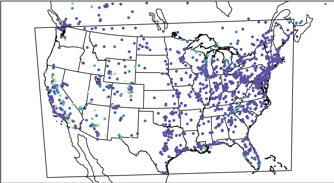
AirNOW (2023-10-16_11:00:00)
