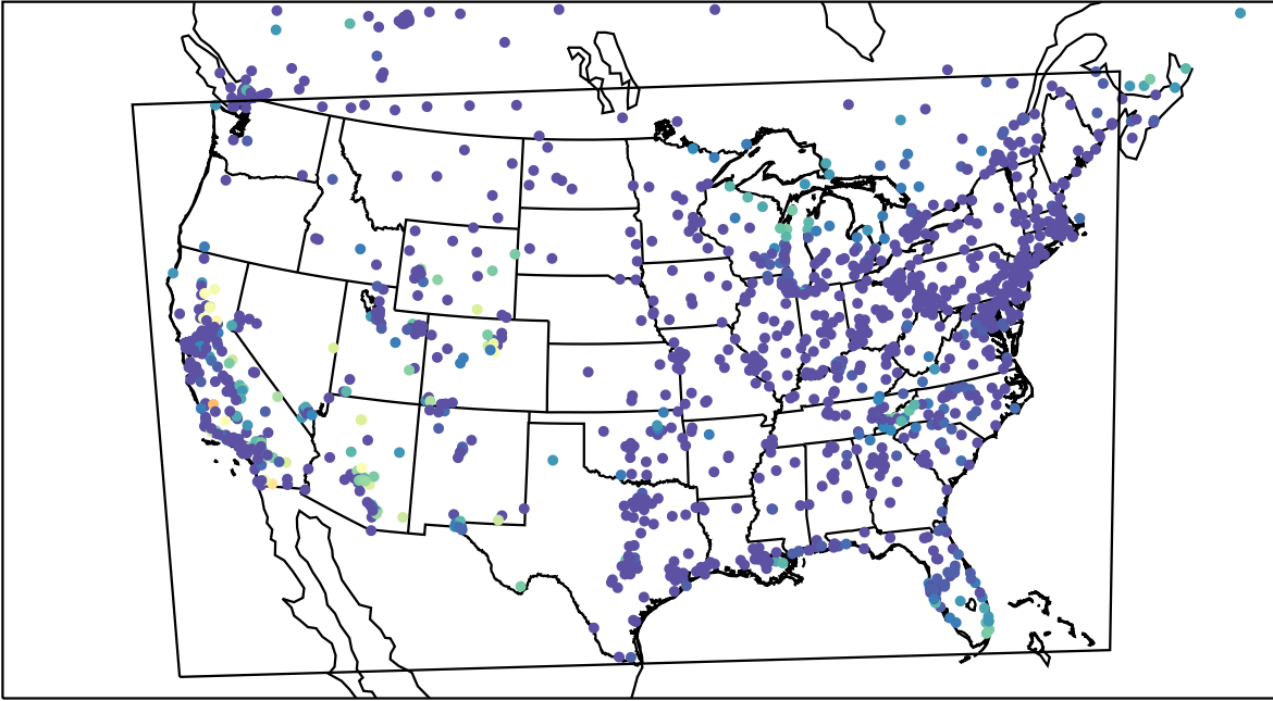
AirNOW (2023-10-16_13:00:00)
