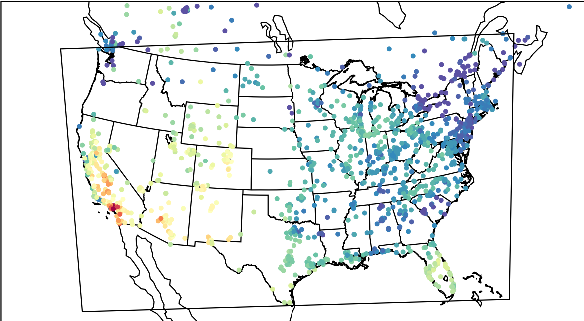
AirNOW (2023-10-15_20:00:00)
