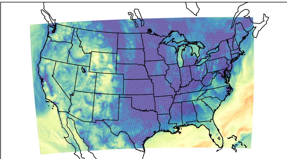
WRF (2023-10-15_14:00:00)
