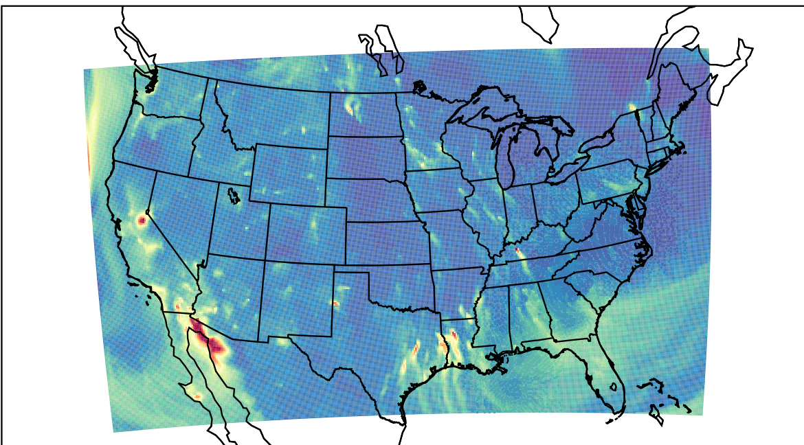
WRF 2023-10-16_04:00:00
