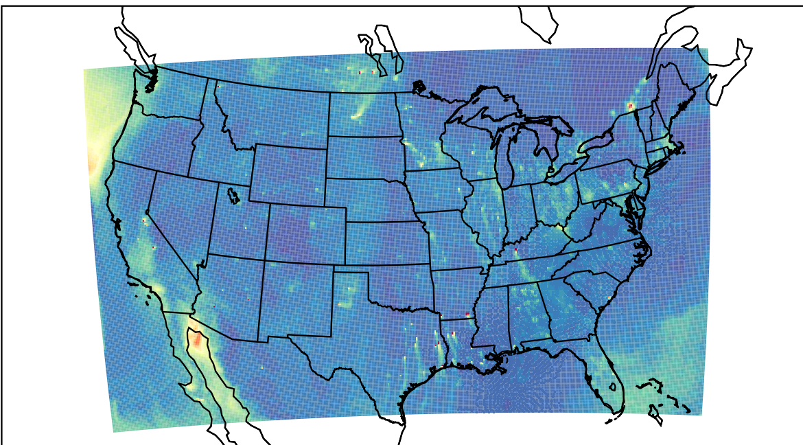
WRF 2023-10-16_23:00:00
