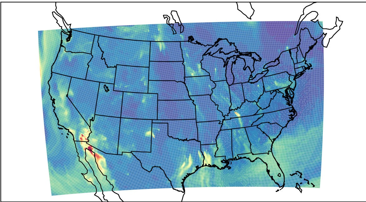
WRF 2023-10-16_08:00:00
