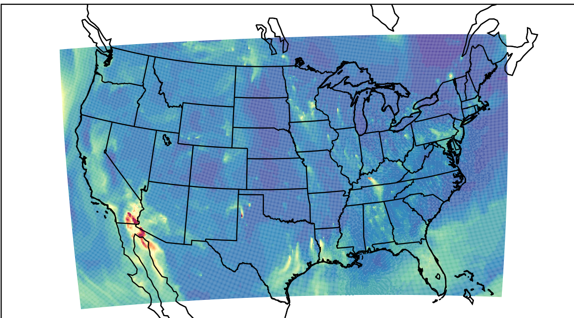
WRF 2023-10-16_11:00:00
