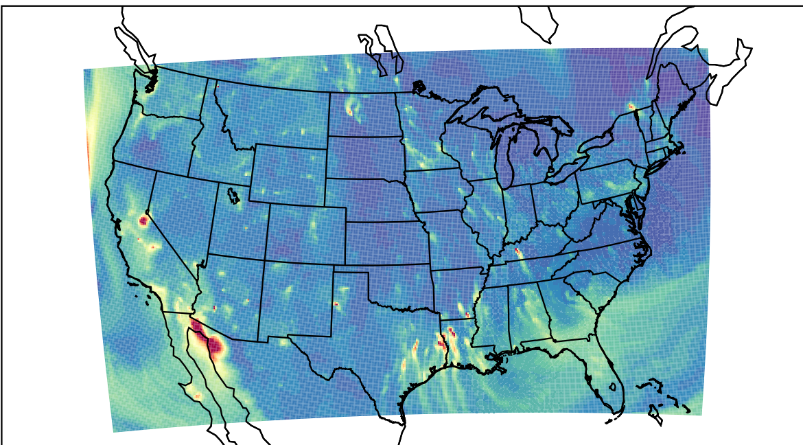
WRF 2023-10-16_03:00:00
