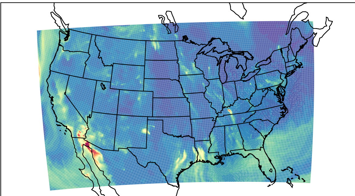
WRF 2023-10-16_07:00:00
