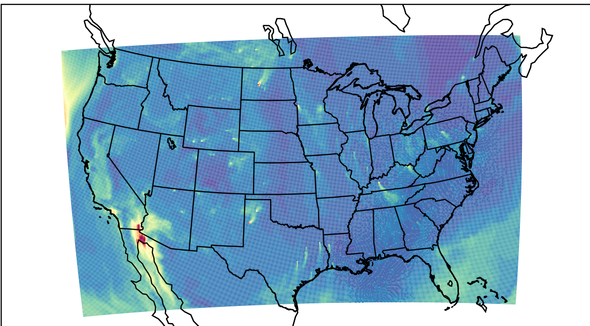
WRF 2023-10-16_17:00:00
