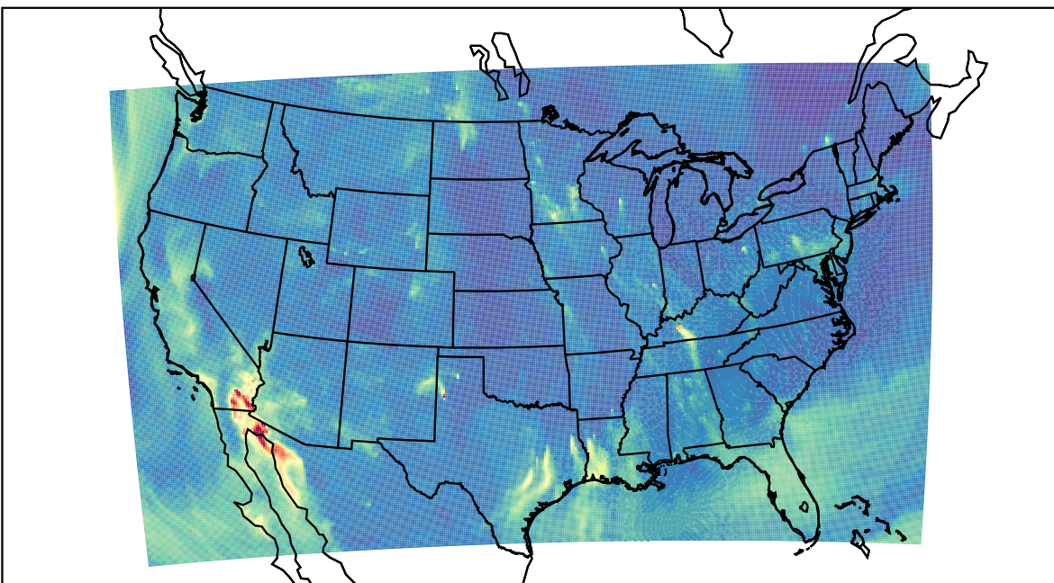
WRF 2023-10-16_09:00:00
