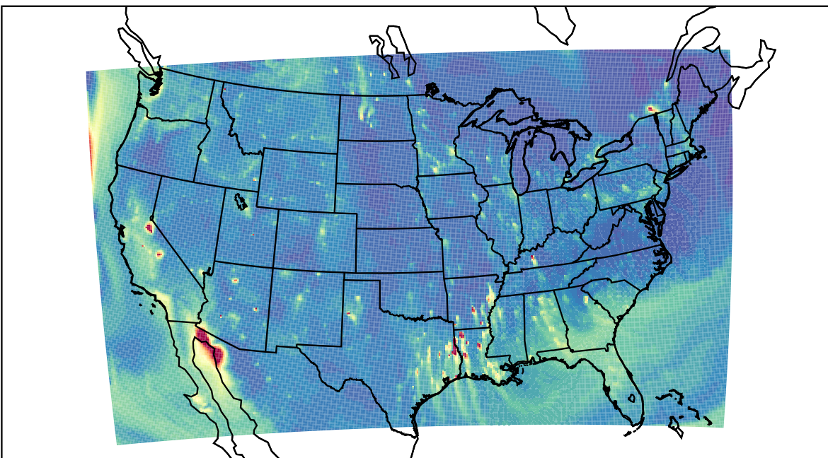
WRF 2023-10-16_01:00:00
