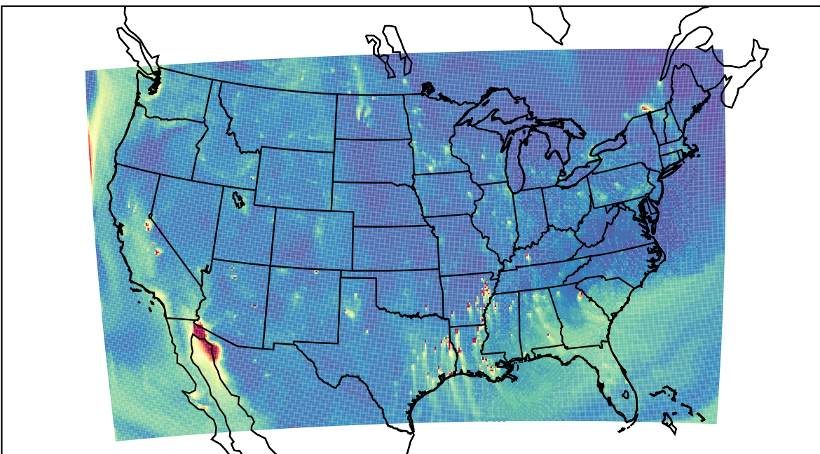
WRF 2023-10-16_00:00:00
