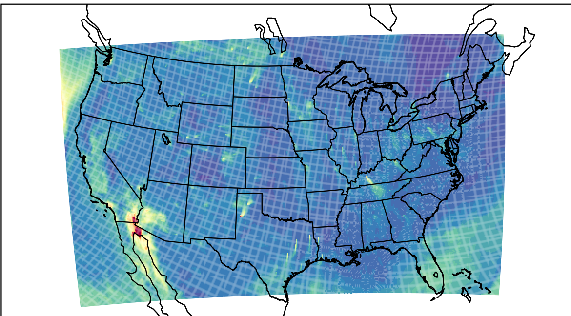
WRF 2023-10-16_16:00:00
