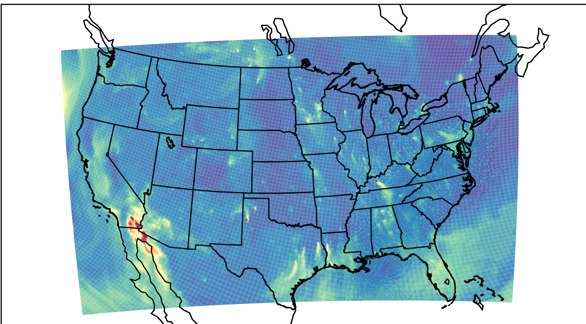
WRF 2023-10-16_12:00:00
