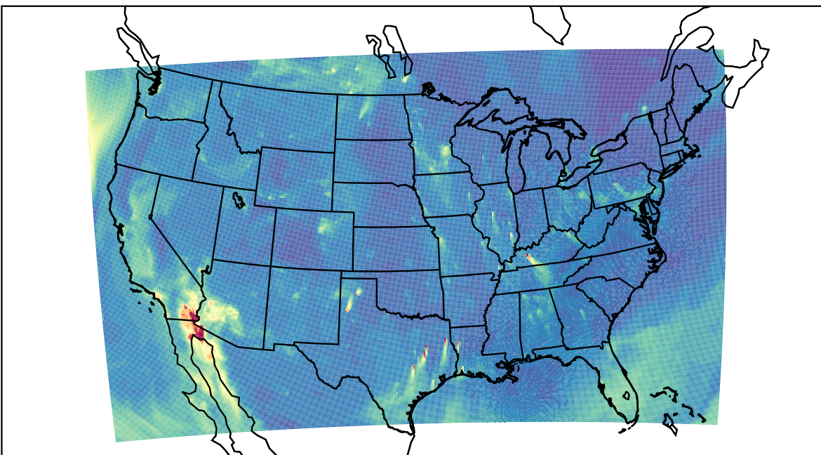
WRF 2023-10-16_15:00:00
