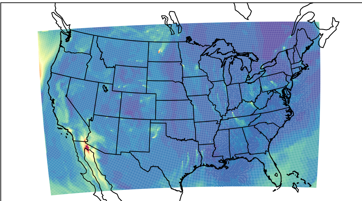
WRF 2023-10-16_18:00:00
