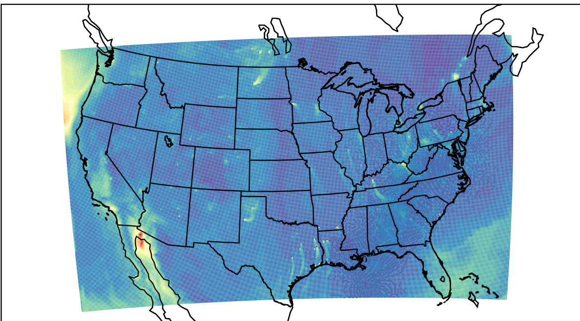
WRF 2023-10-16_21:00:00
