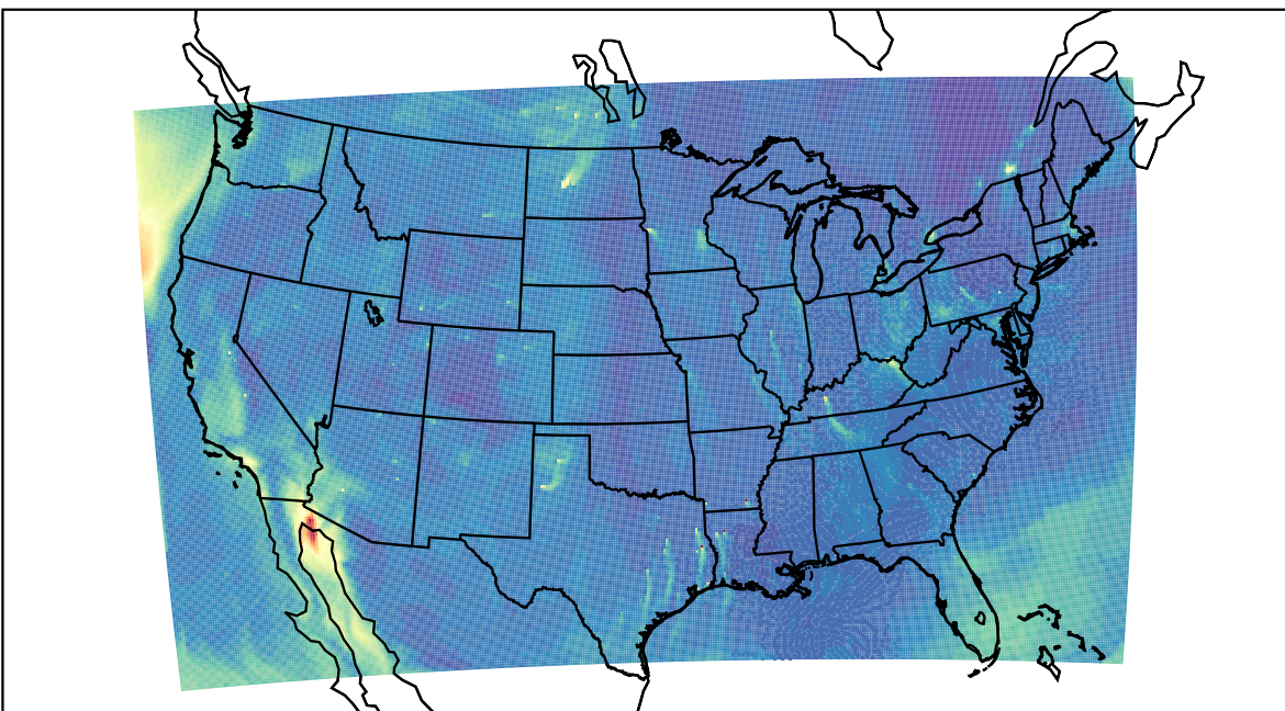
WRF 2023-10-16_20:00:00
