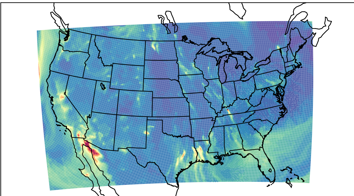
WRF 2023-10-16_05:00:00
