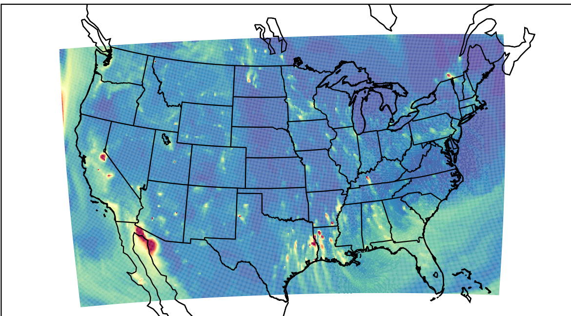
WRF 2023-10-16_02:00:00
