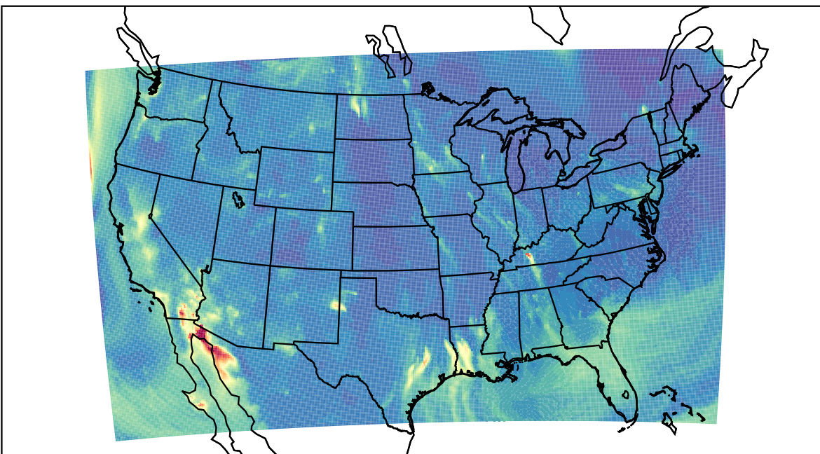
WRF 2023-10-16_06:00:00
