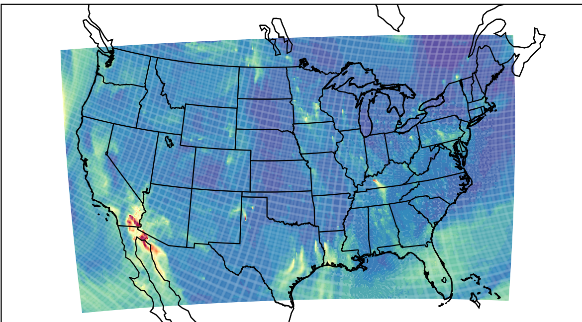
WRF 2023-10-16_10:00:00
