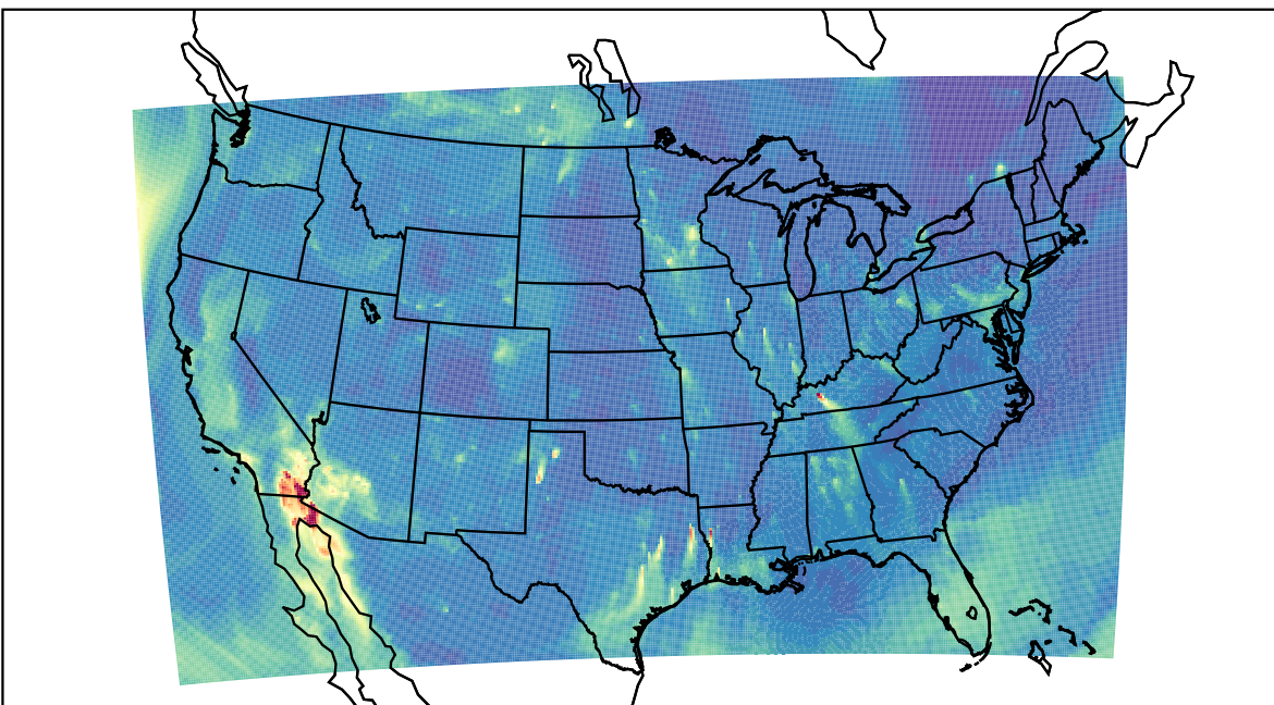
WRF 2023-10-16_14:00:00
