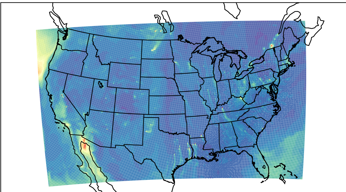
WRF 2023-10-16_22:00:00
