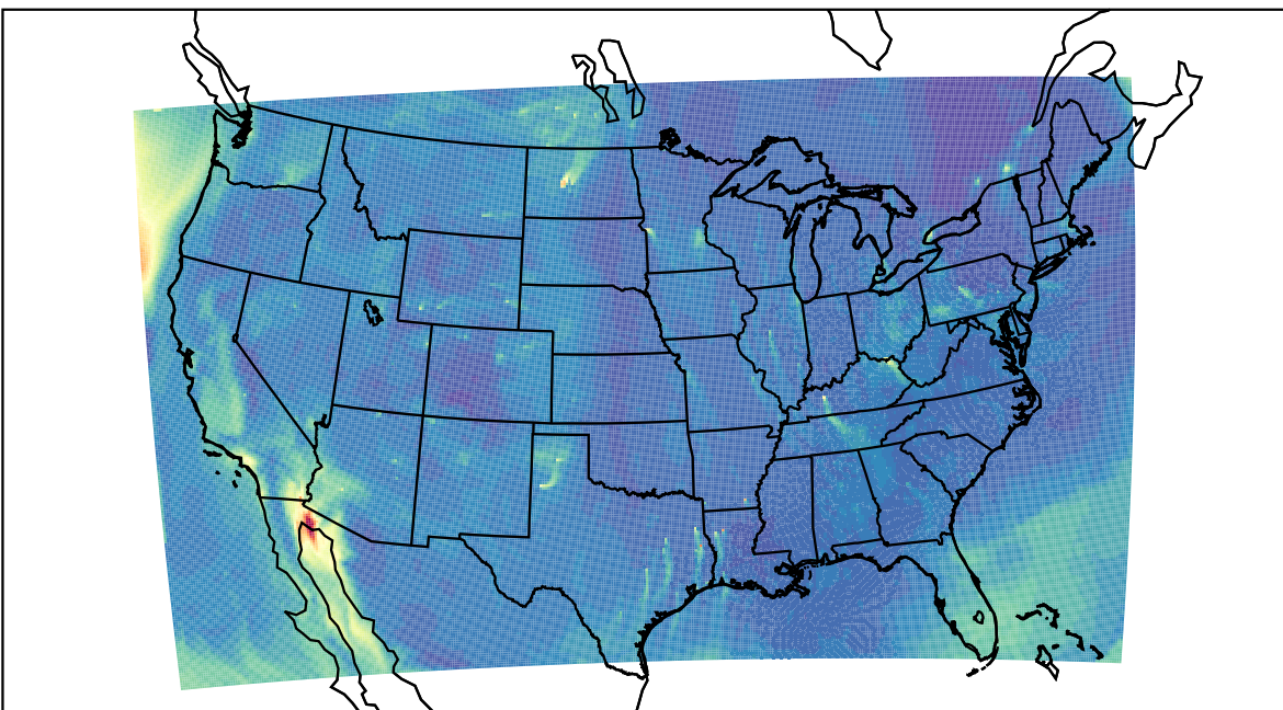
WRF 2023-10-16_19:00:00
