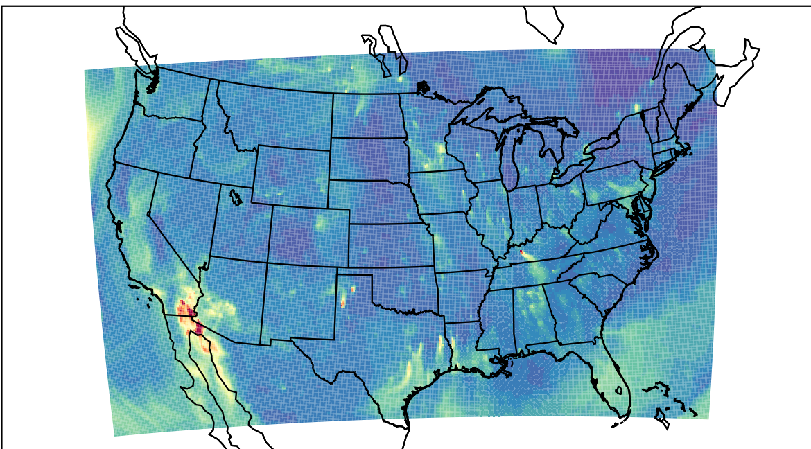
WRF 2023-10-16_13:00:00
