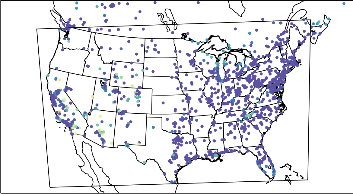
AirNOW (2023-10-16_12:00:00)
