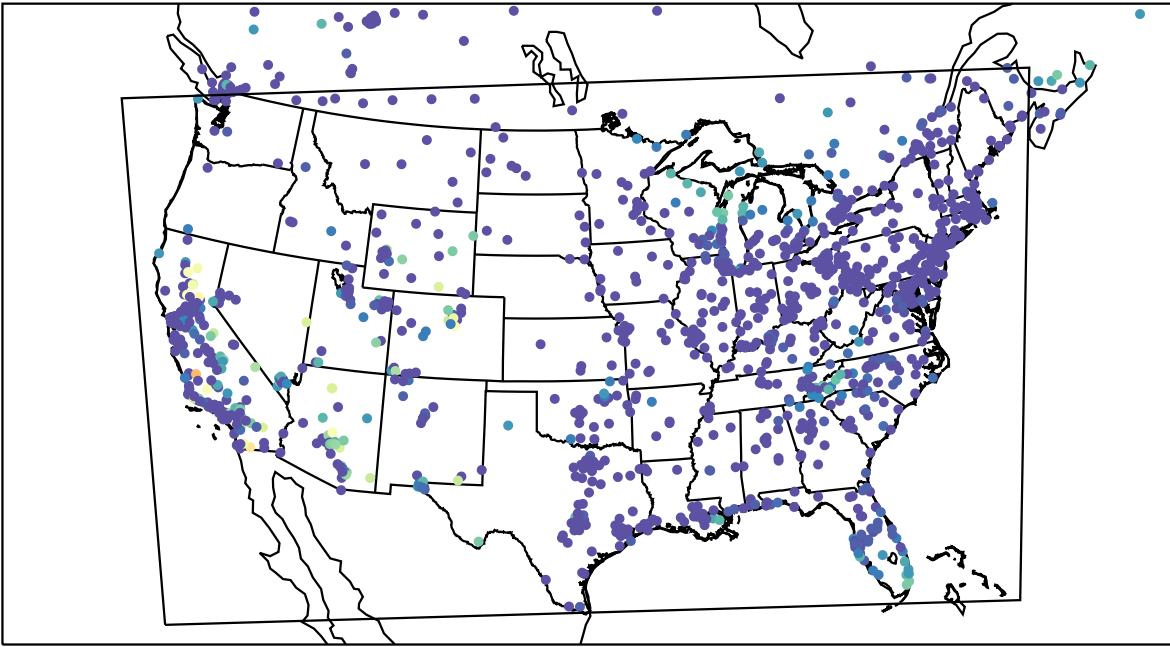
AirNOW (2023-10-16_13:00:00)
