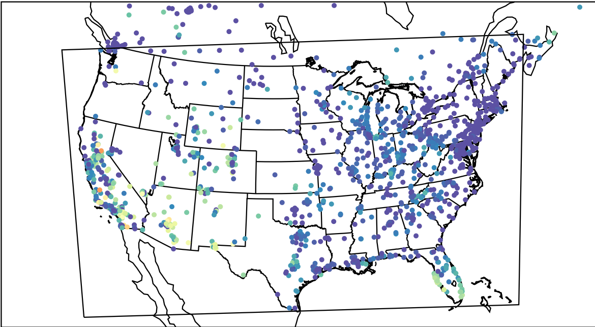
AirNOW (2023-10-16_04:00:00)
