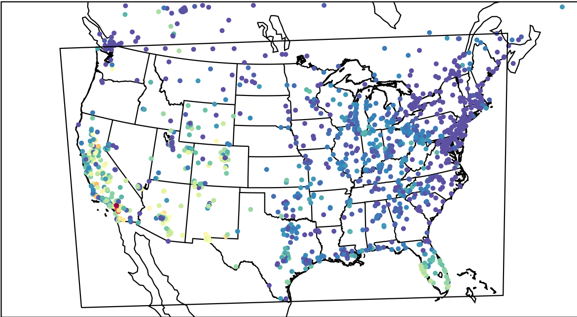
AirNOW (2023-10-16_02:00:00)
