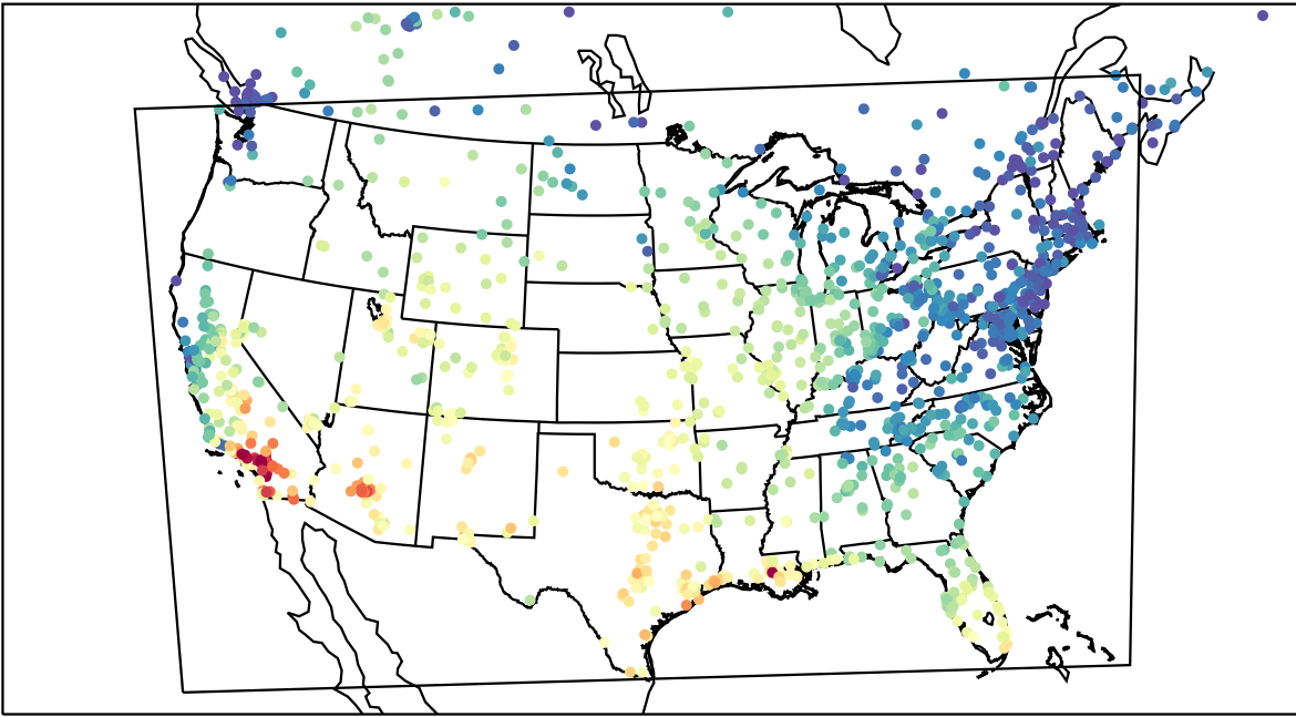
AirNOW (2023-10-17_20:00:00)
