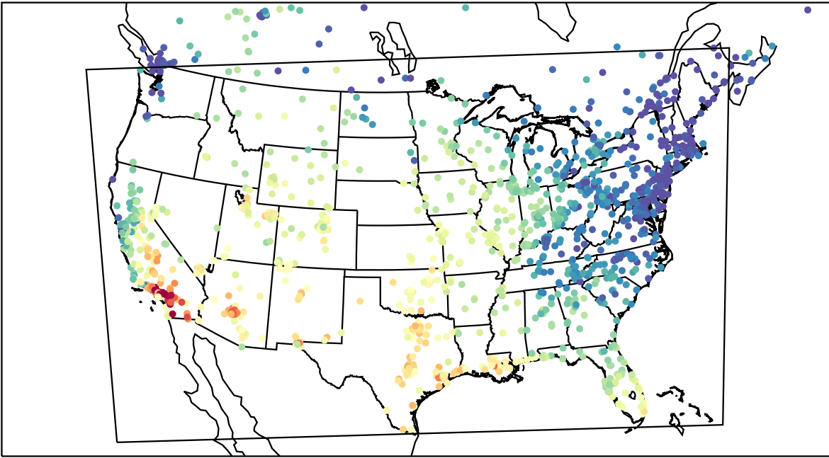
AirNOW (2023-10-17_21:00:00)
