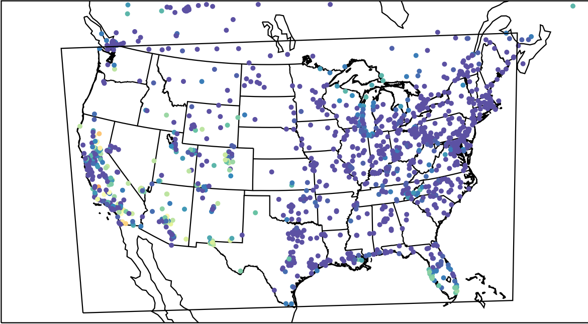
AirNOW (2023-10-16_09:00:00)
