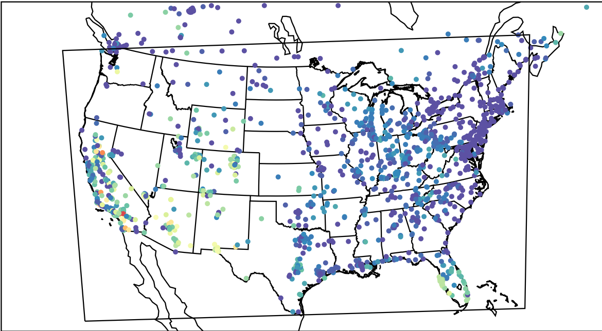
AirNOW (2023-10-16_03:00:00)
