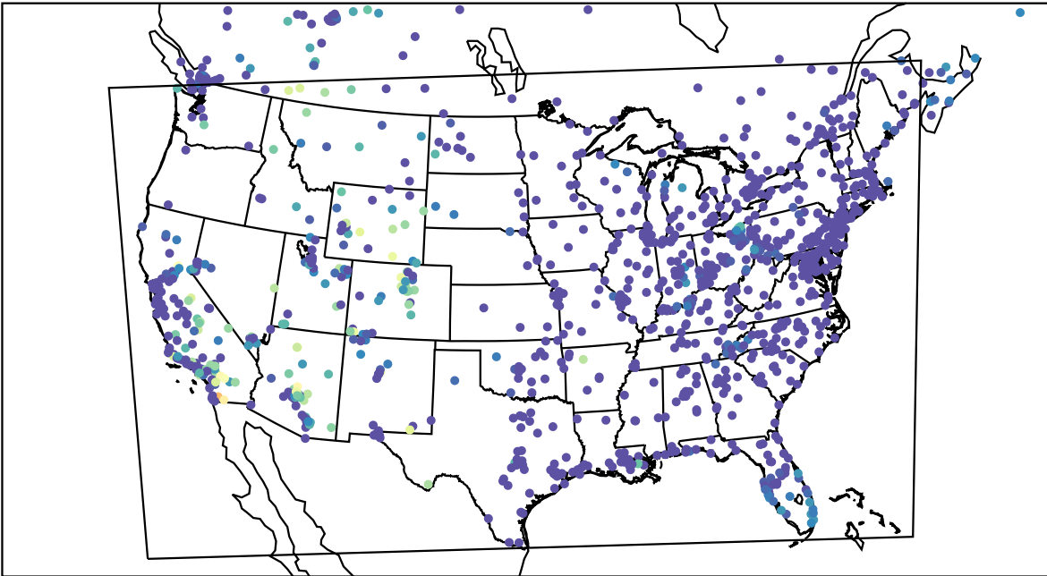
AirNOW (2023-10-17_12:00:00)
