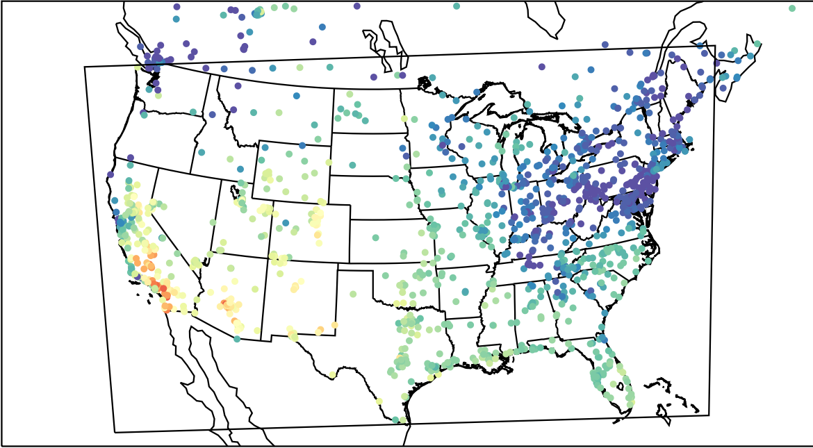
AirNOW (2023-10-16_19:00:00)
