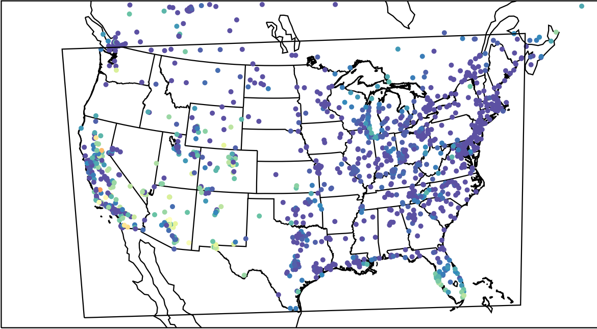
AirNOW (2023-10-16_06:00:00)
