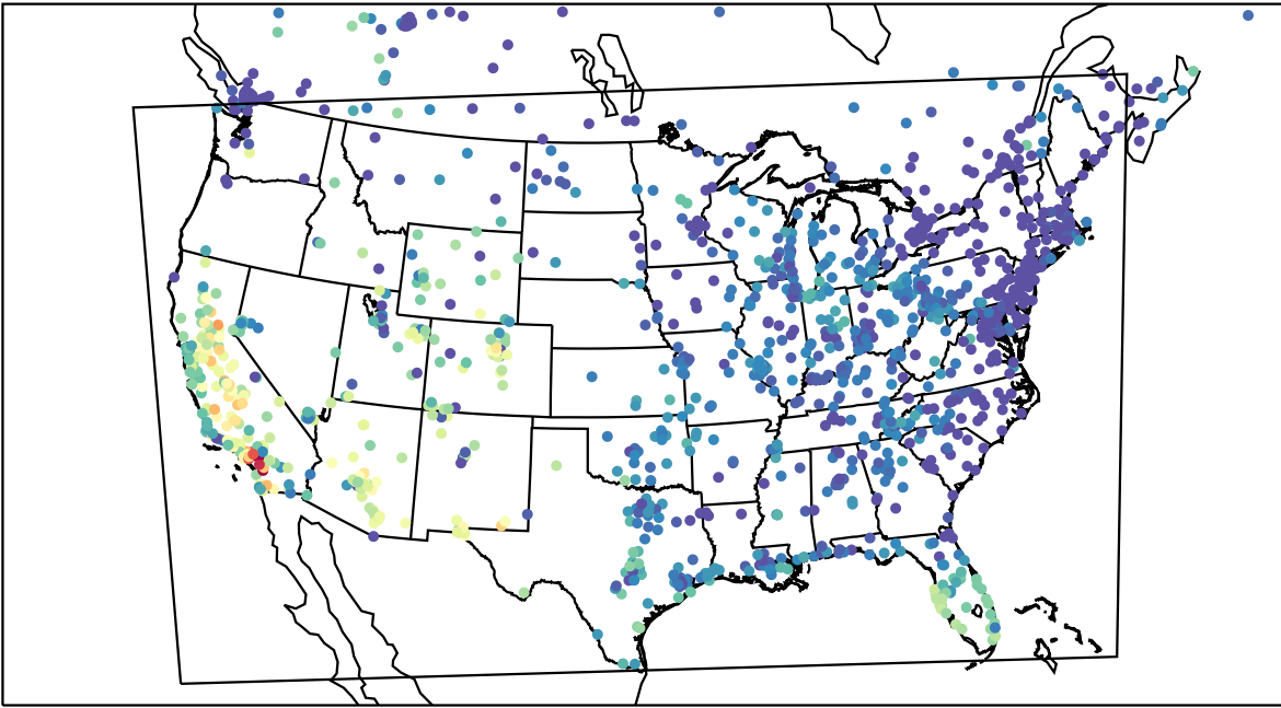
AirNOW (2023-10-16_01:00:00)
