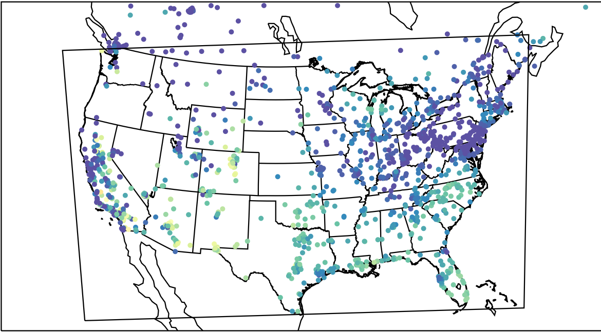
AirNOW (2023-10-16_16:00:00)
