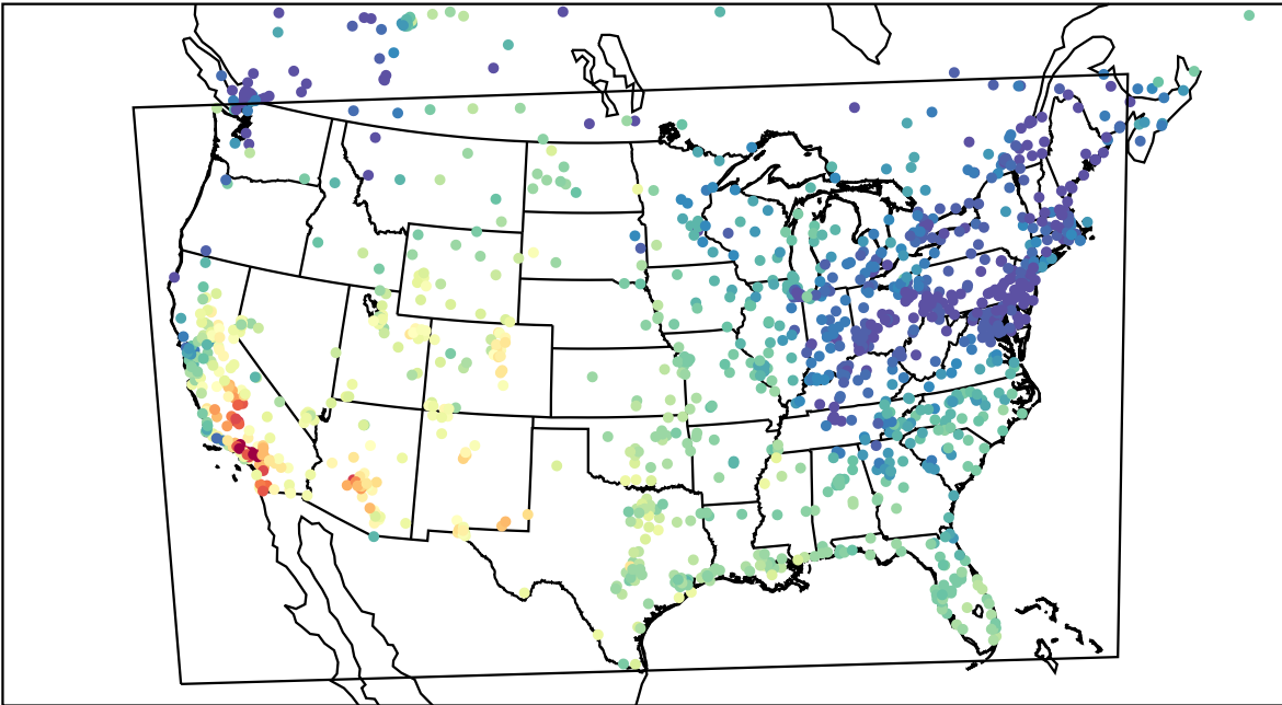
AirNOW (2023-10-16_20:00:00)
