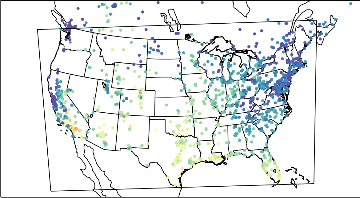
AirNOW (2023-10-17_17:00:00)
