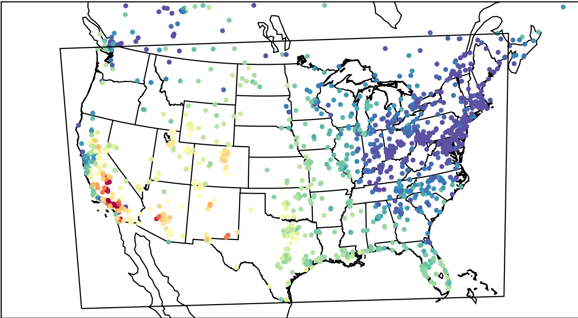
AirNOW (2023-10-16_22:00:00)
