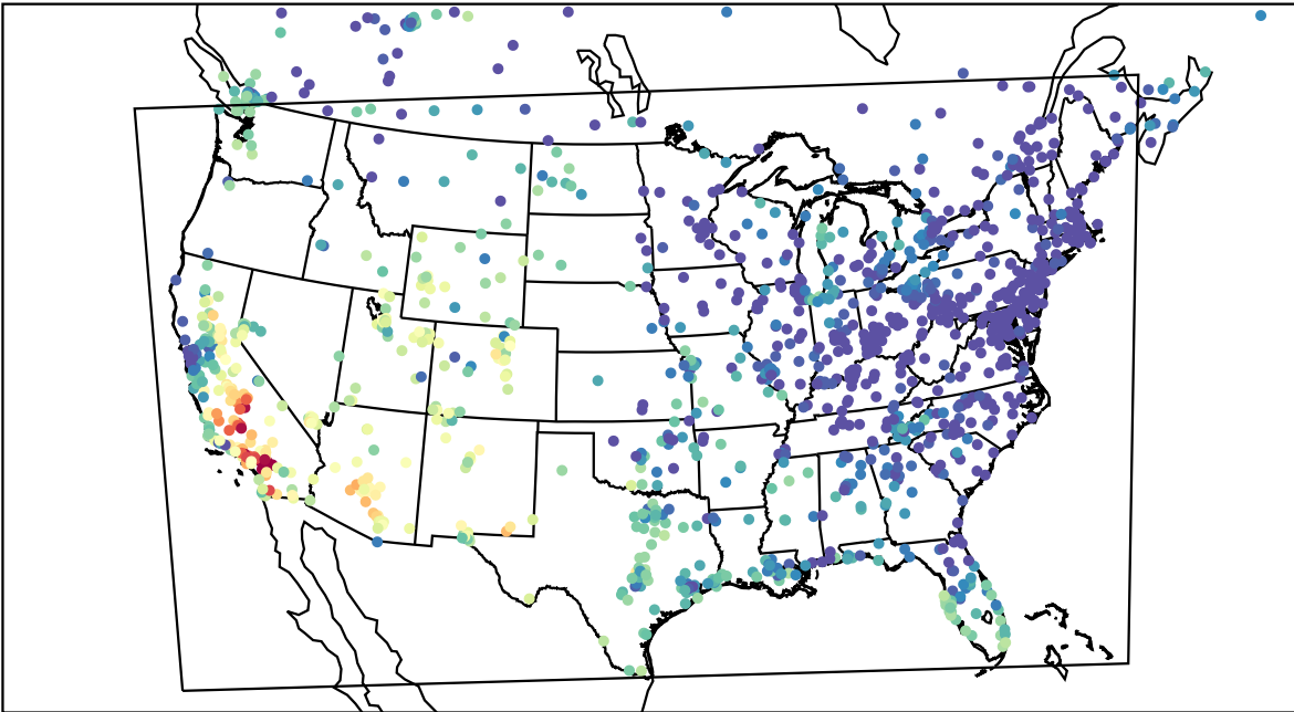
AirNOW (2023-10-17_00:00:00)
