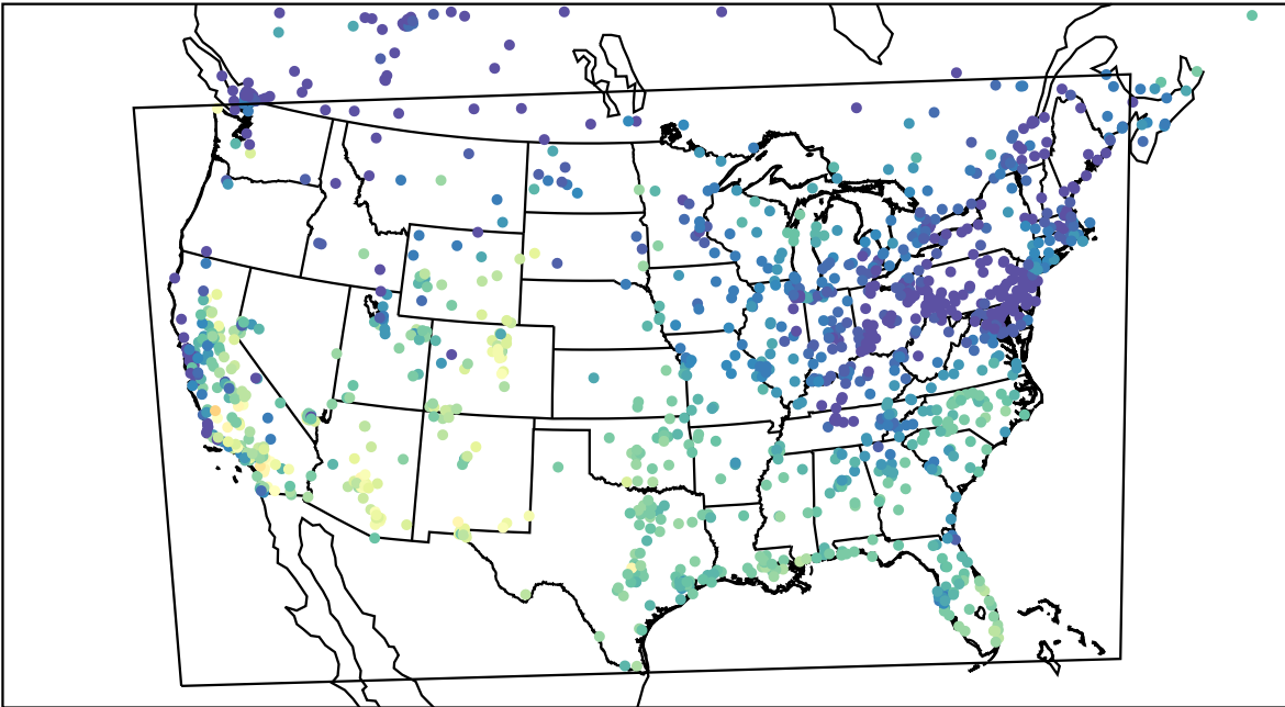
AirNOW (2023-10-16_17:00:00)
