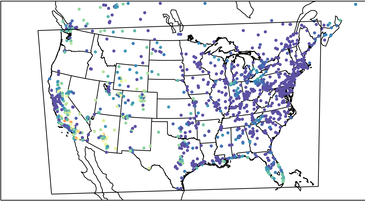
AirNOW (2023-10-17_04:00:00)
