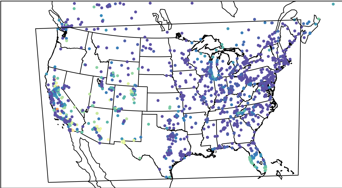
AirNOW (2023-10-16_07:00:00)
