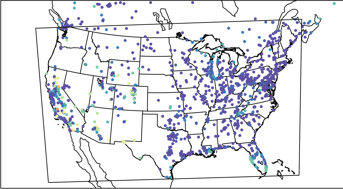
AirNOW (2023-10-16_08:00:00)
