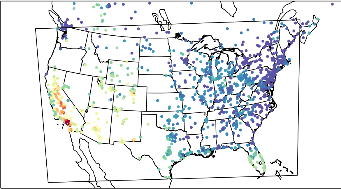
AirNOW (2023-10-16_00:00:00)
