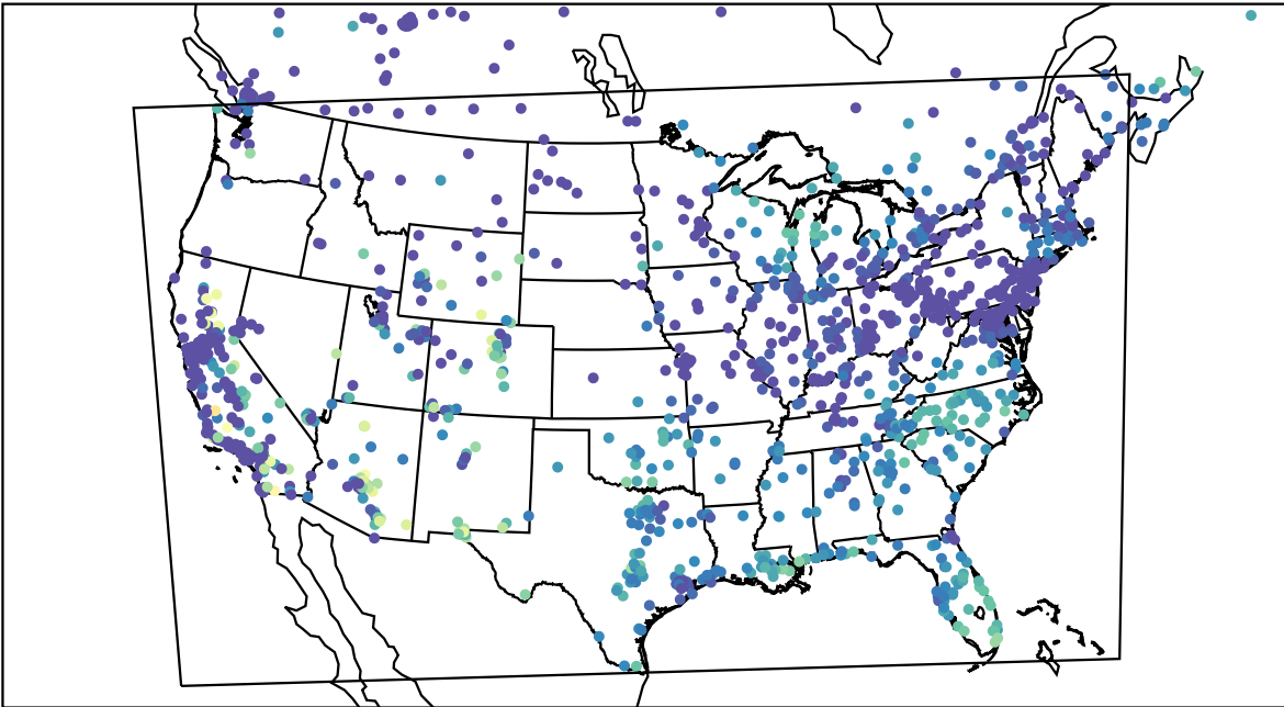
AirNOW (2023-10-16_15:00:00)
