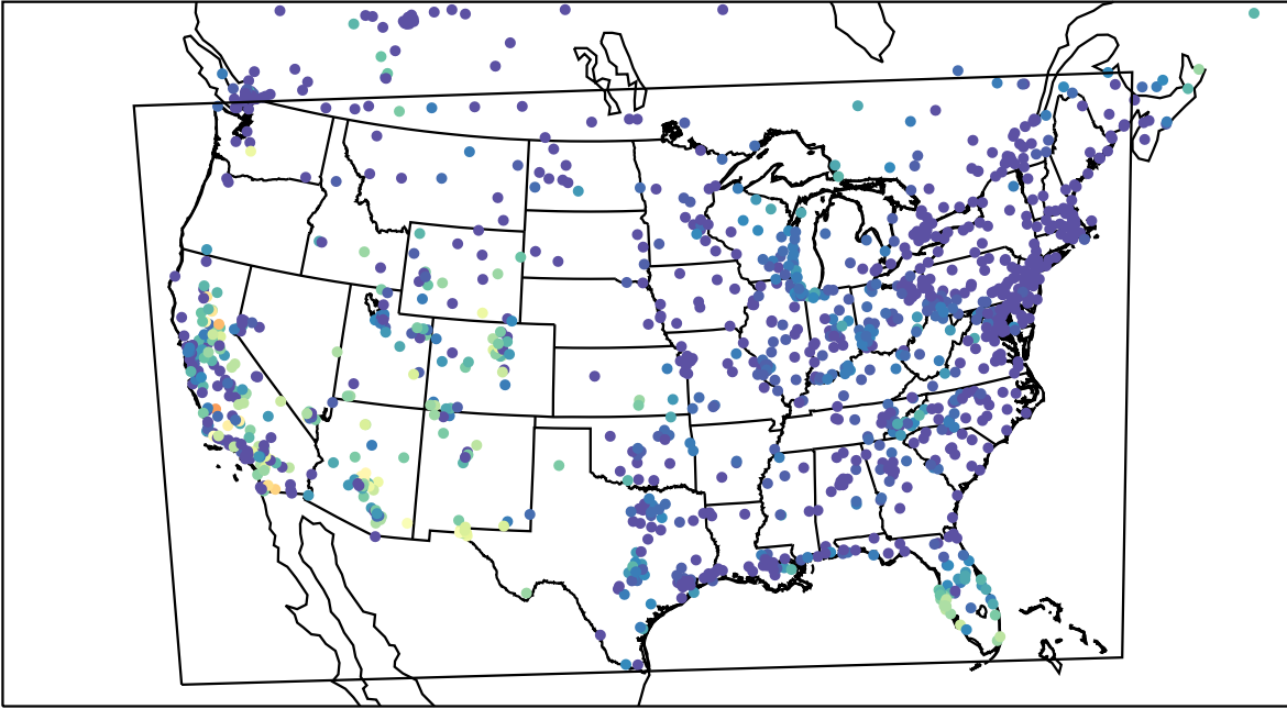
AirNOW (2023-10-16_05:00:00)
