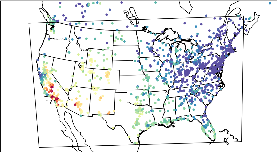
AirNOW (2023-10-16_23:00:00)
