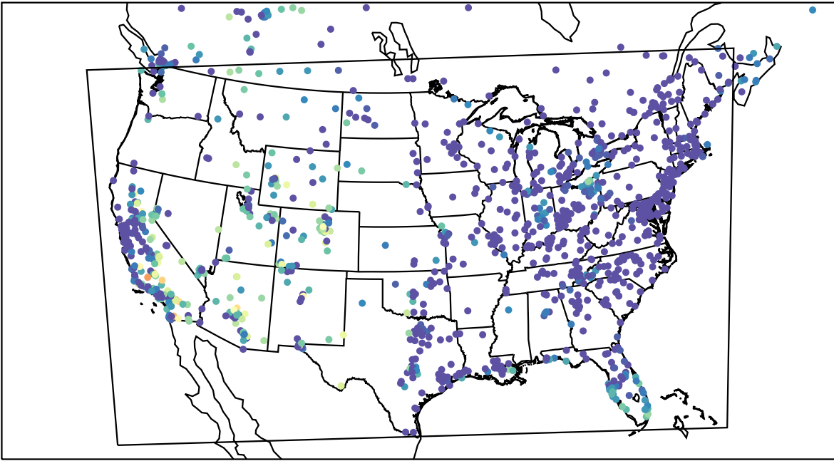
AirNOW (2023-10-17_06:00:00)
