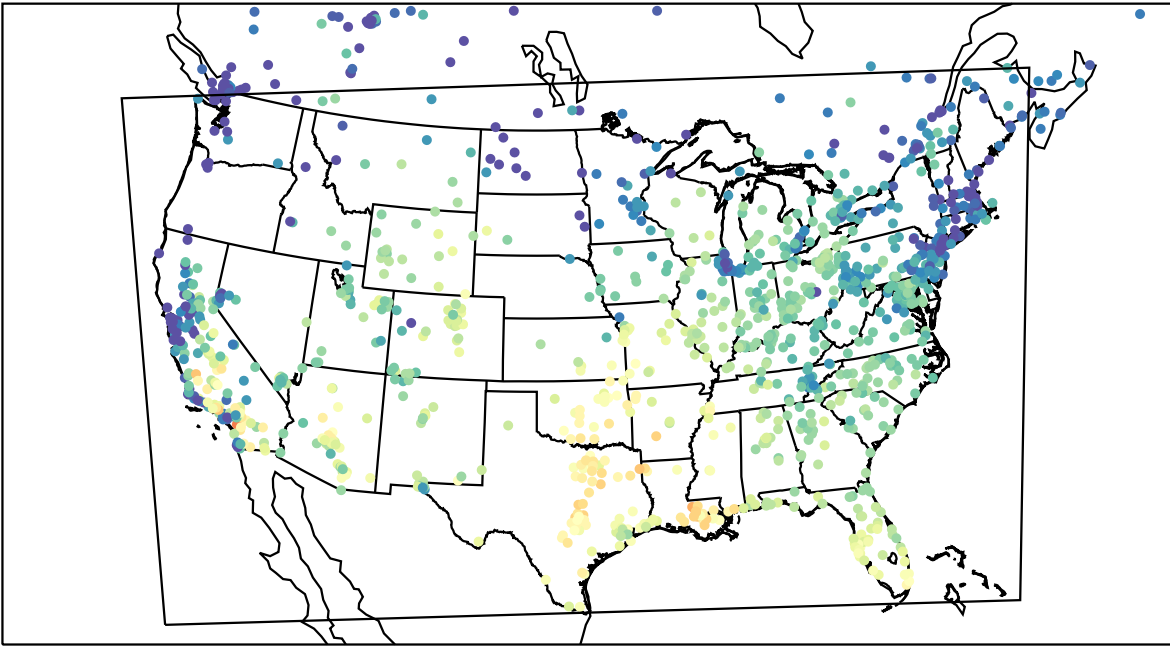
AirNOW (2023-10-18_17:00:00)
