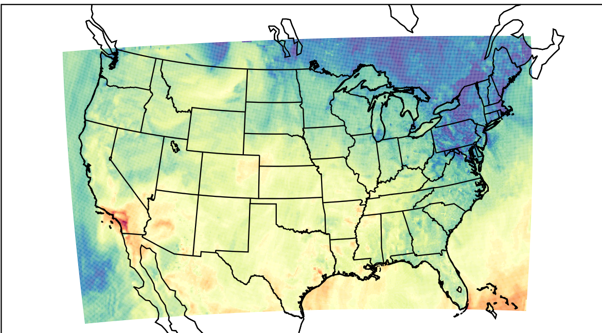
WRF (2023-10-17_22:00:00)
