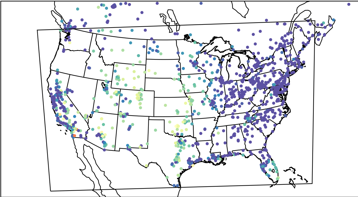
AirNOW (2023-10-18_05:00:00)
