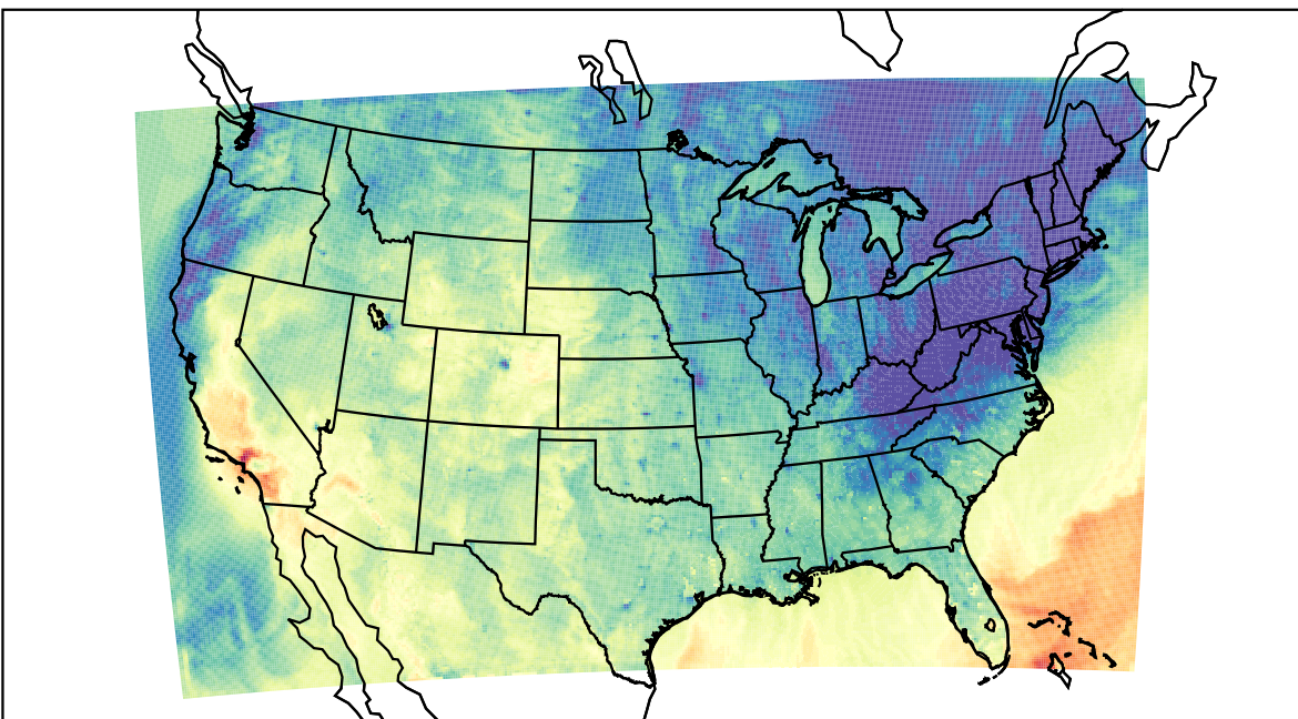
WRF (2023-10-17_00:00:00)
