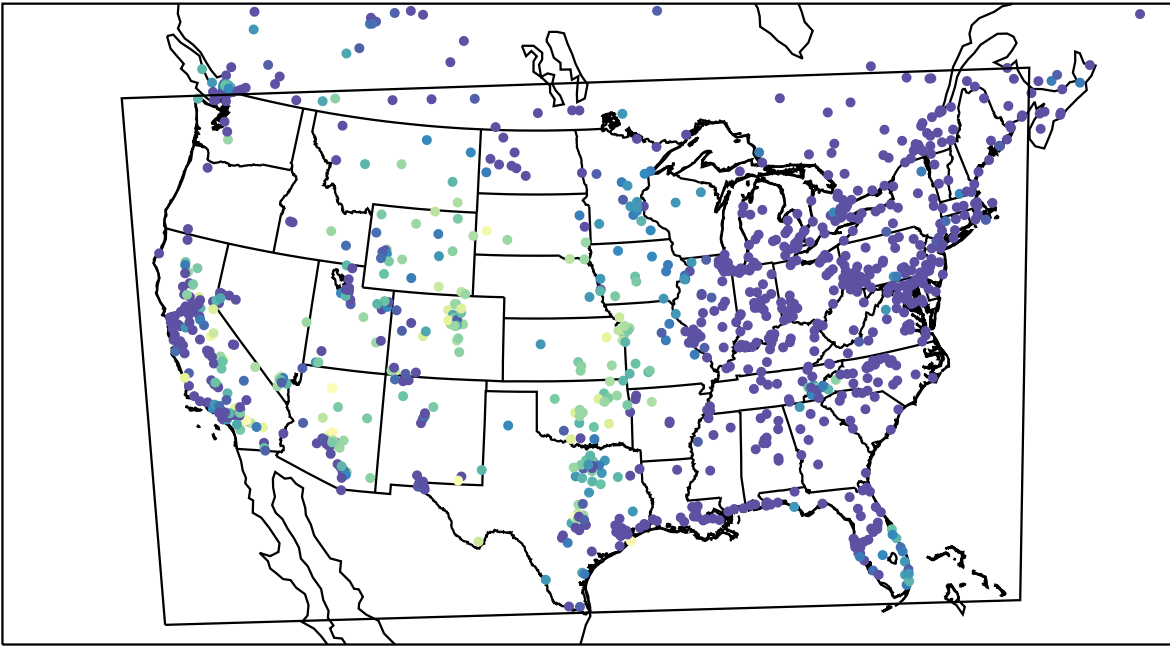
AirNOW (2023-10-18_10:00:00)
