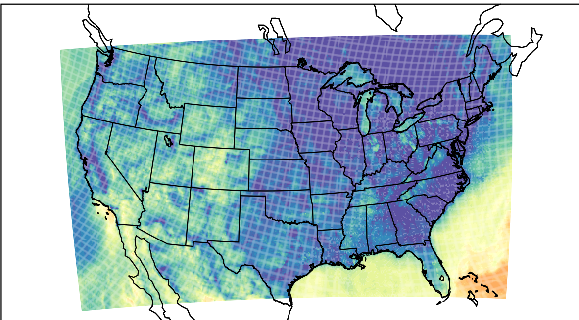
WRF (2023-10-17_14:00:00)
