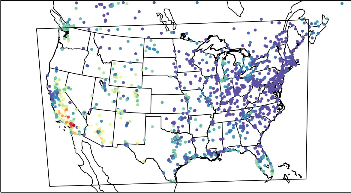
AirNOW (2023-10-17_01:00:00)
