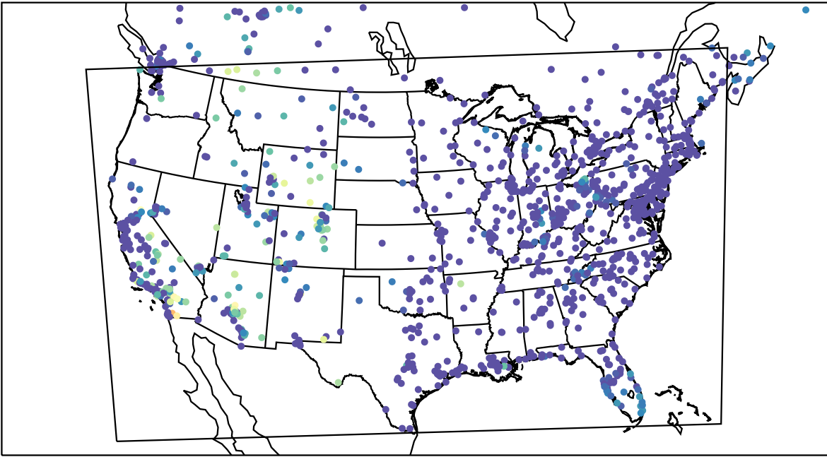
AirNOW (2023-10-17_12:00:00)
