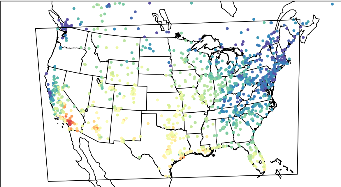
AirNOW (2023-10-17_19:00:00)
