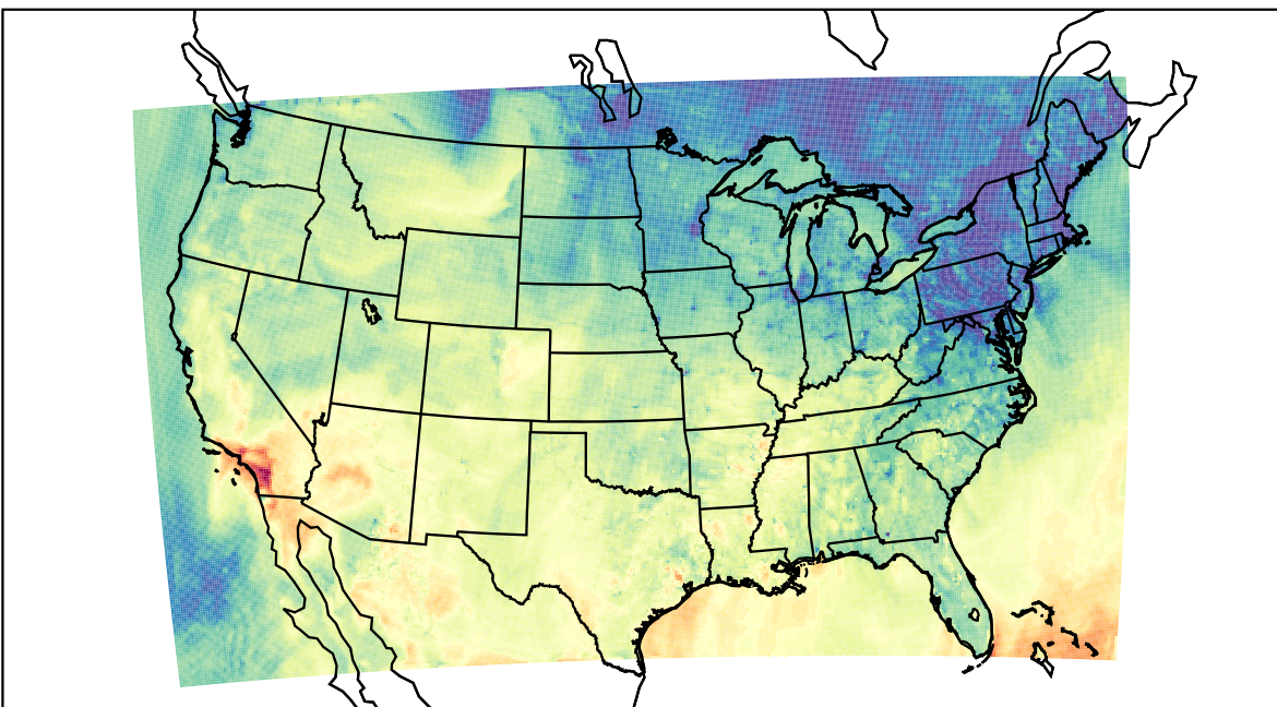
WRF (2023-10-17_23:00:00)
