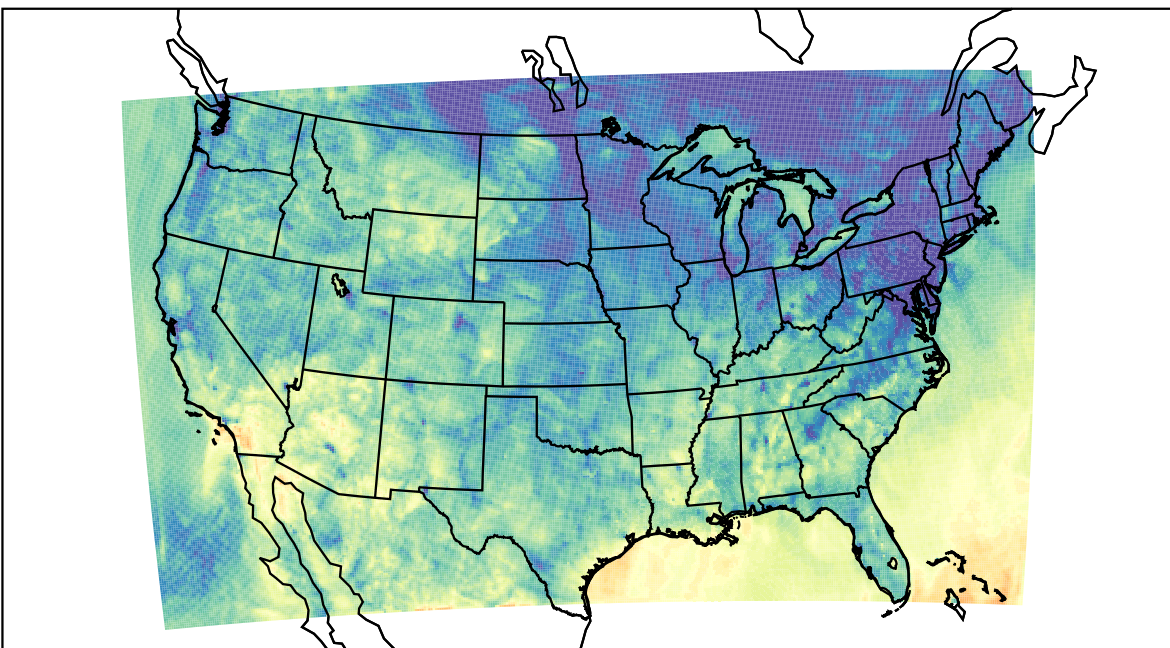
WRF (2023-10-18_05:00:00)
