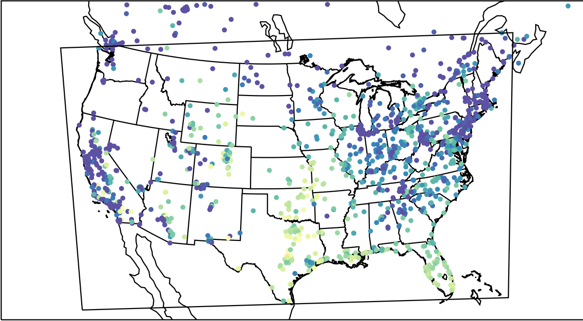
AirNOW (2023-10-18_15:00:00)
