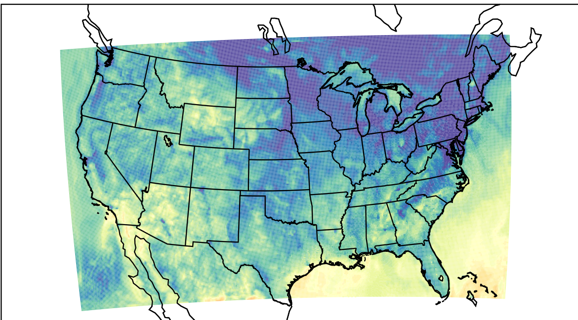
WRF (2023-10-18_08:00:00)
