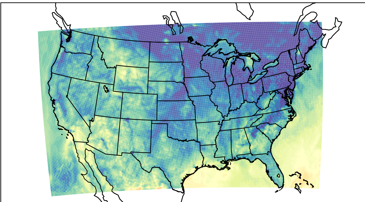
WRF (2023-10-18_10:00:00)
