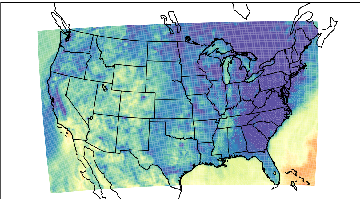
WRF (2023-10-17_09:00:00)
