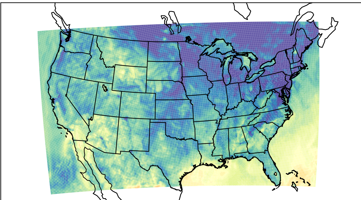
WRF (2023-10-18_09:00:00)
