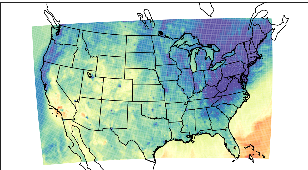
WRF (2023-10-17_01:00:00)
