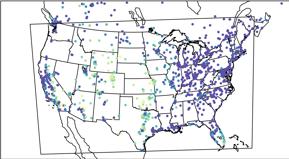
AirNOW (2023-10-18_06:00:00)
