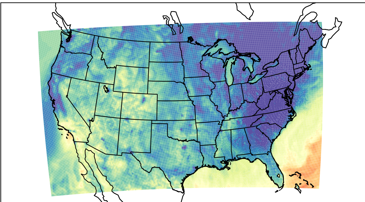
WRF (2023-10-17_06:00:00)
