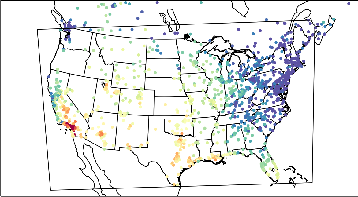
AirNOW (2023-10-17_22:00:00)
