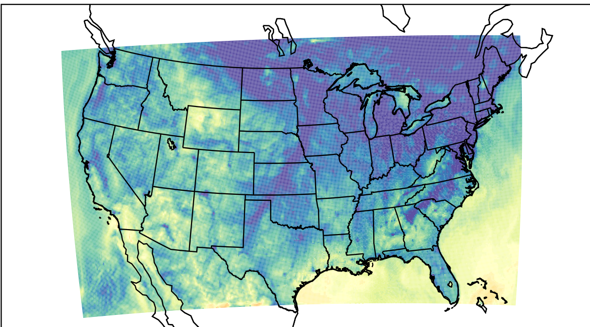
WRF (2023-10-18_12:00:00)
