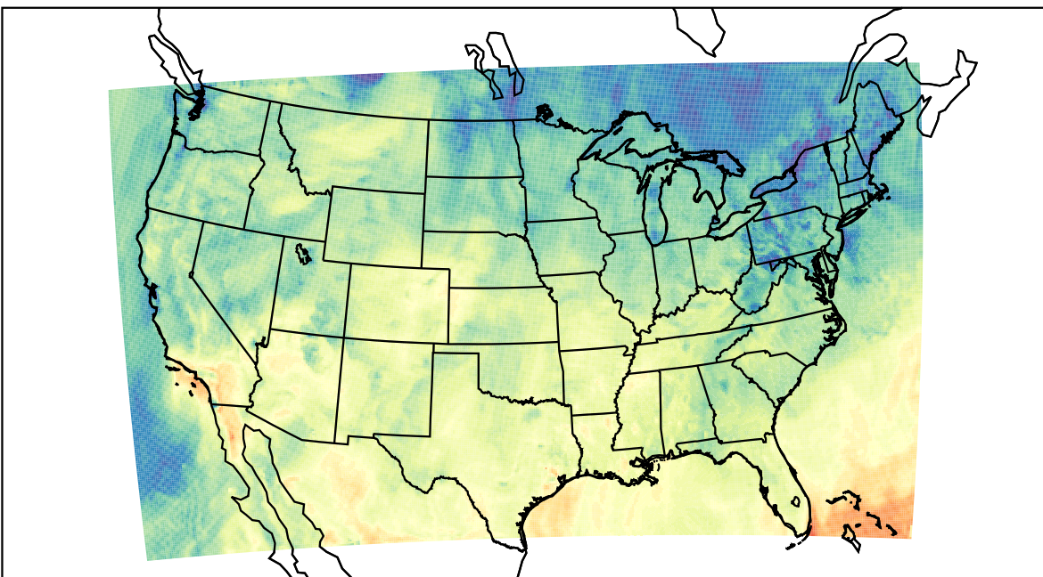
WRF (2023-10-17_19:00:00)
