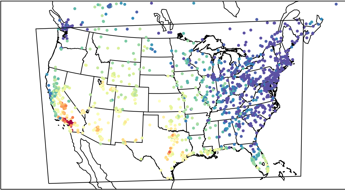
AirNOW (2023-10-17_23:00:00)
