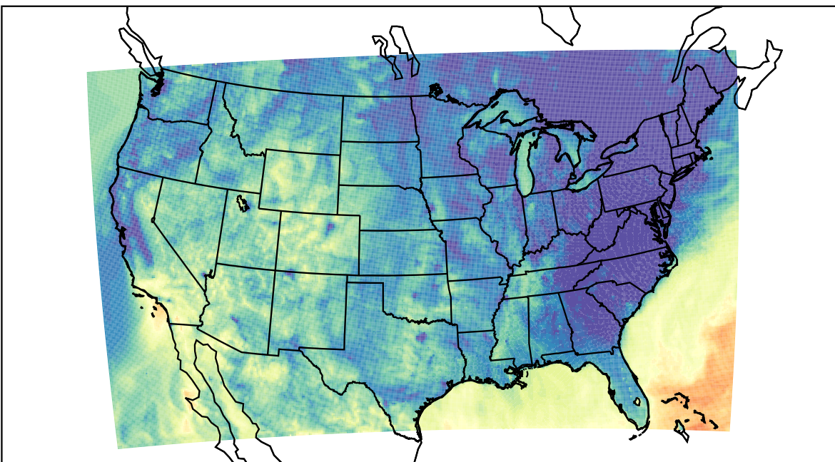
WRF (2023-10-17_07:00:00)
