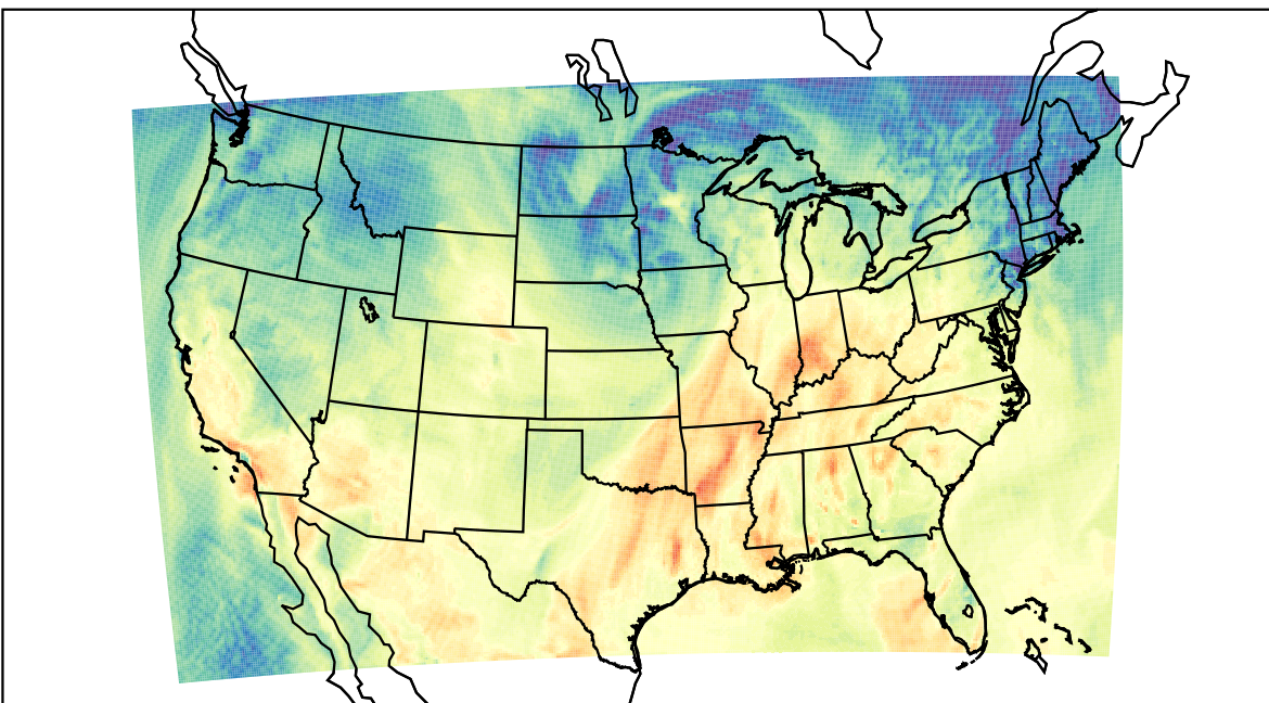
WRF (2023-10-18_21:00:00)
