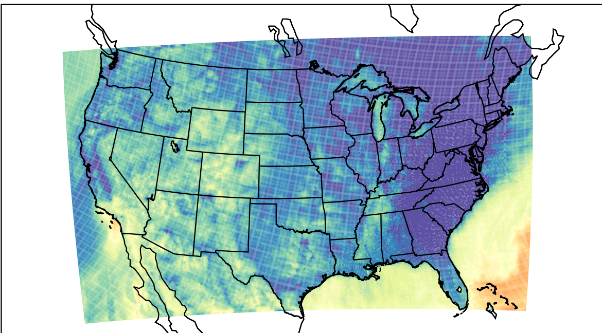
WRF (2023-10-17_10:00:00)
