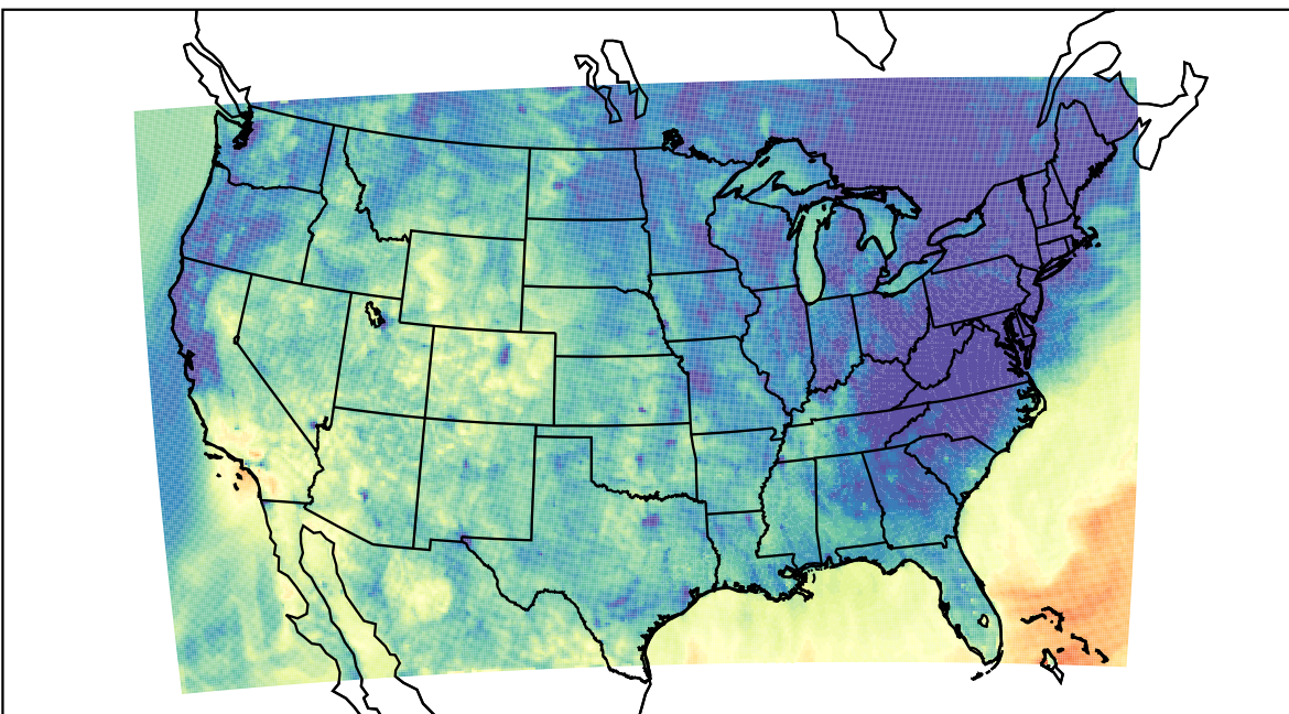
WRF (2023-10-17_04:00:00)
