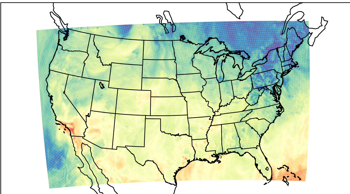
WRF (2023-10-17_21:00:00)
