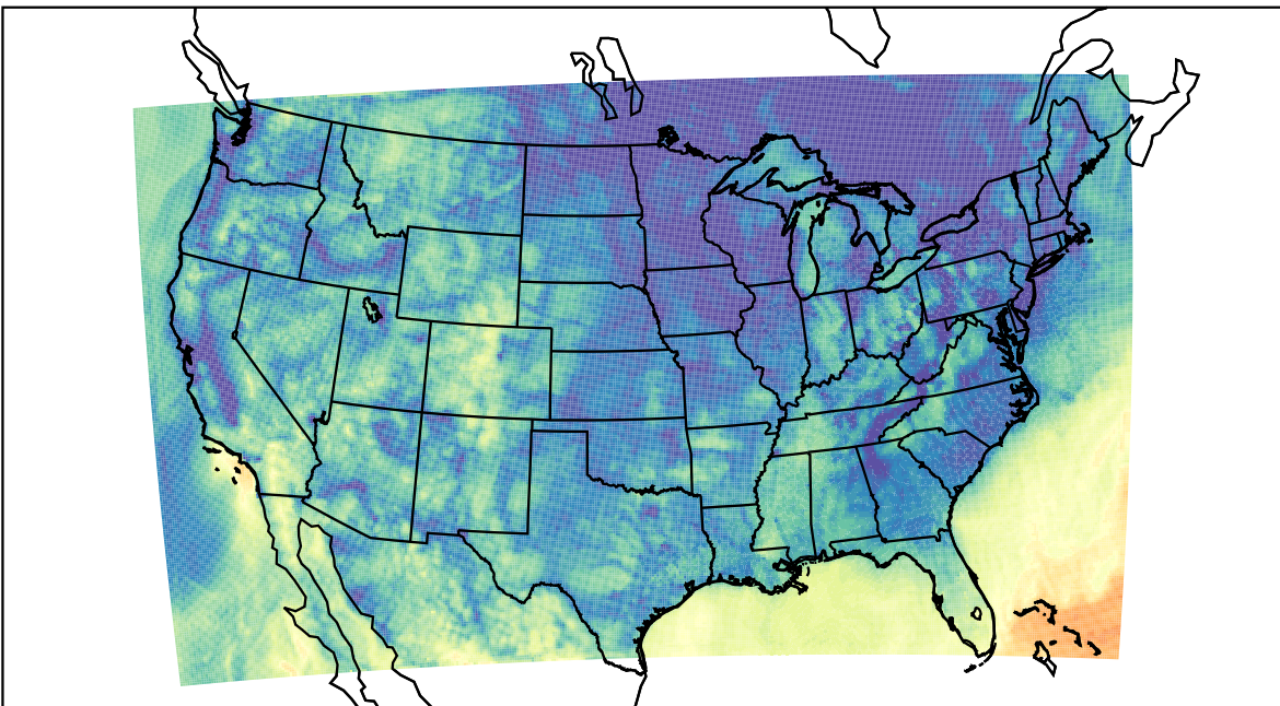
WRF (2023-10-17_15:00:00)
