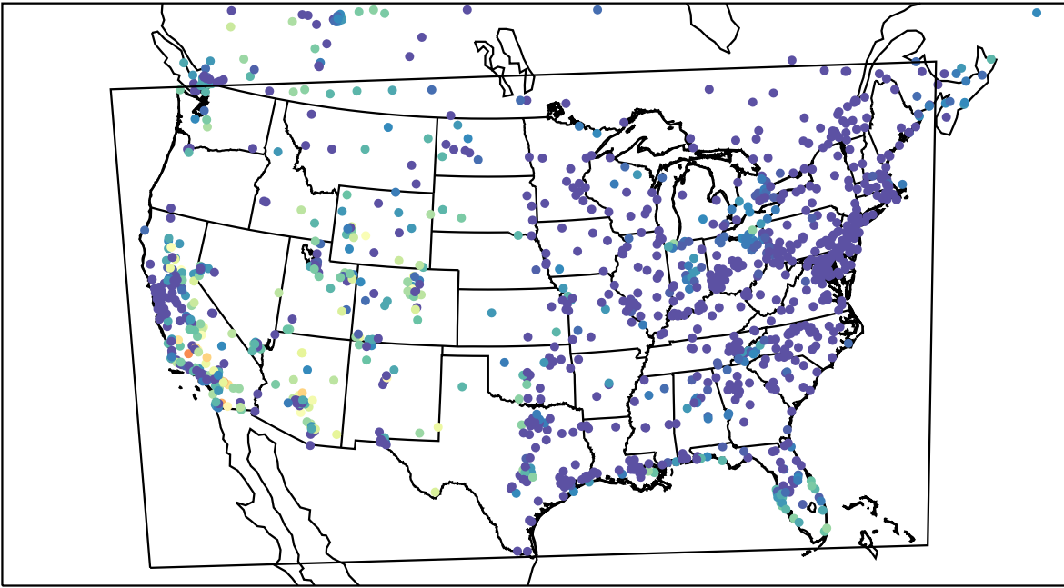
AirNOW (2023-10-17_05:00:00)
