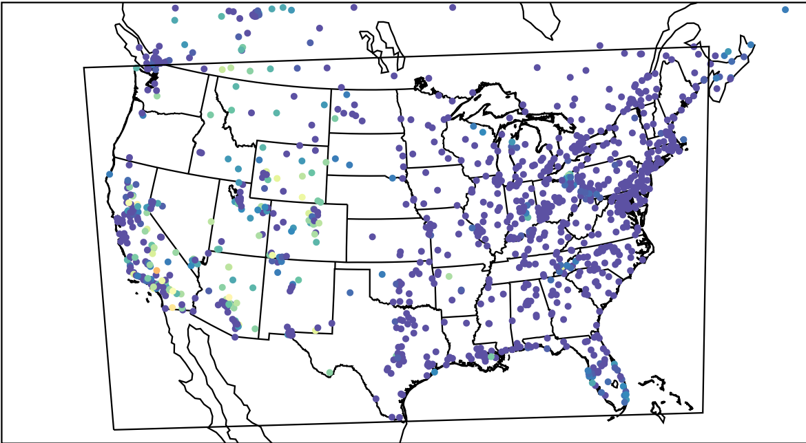
AirNOW (2023-10-17_11:00:00)
