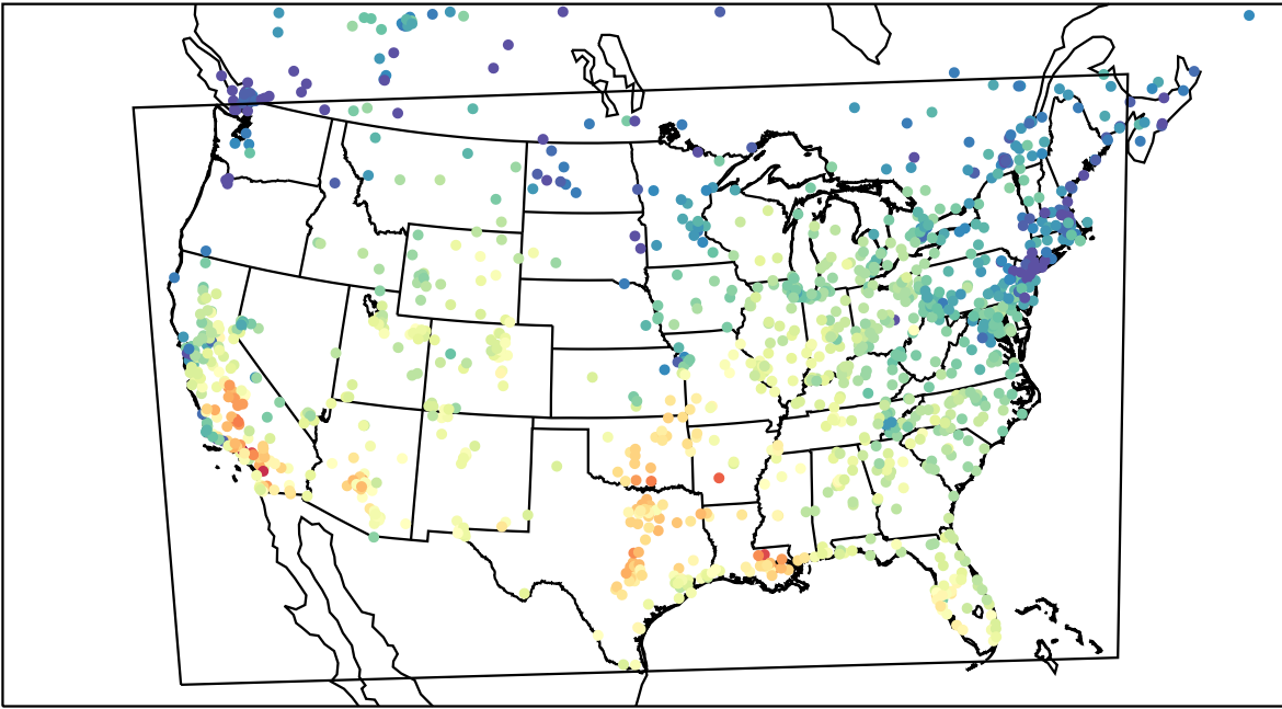
AirNOW (2023-10-18_19:00:00)
