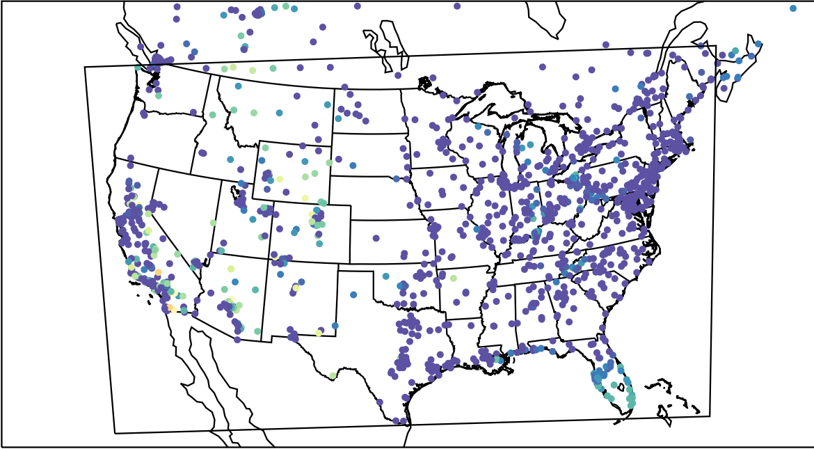
AirNOW (2023-10-17_13:00:00)
