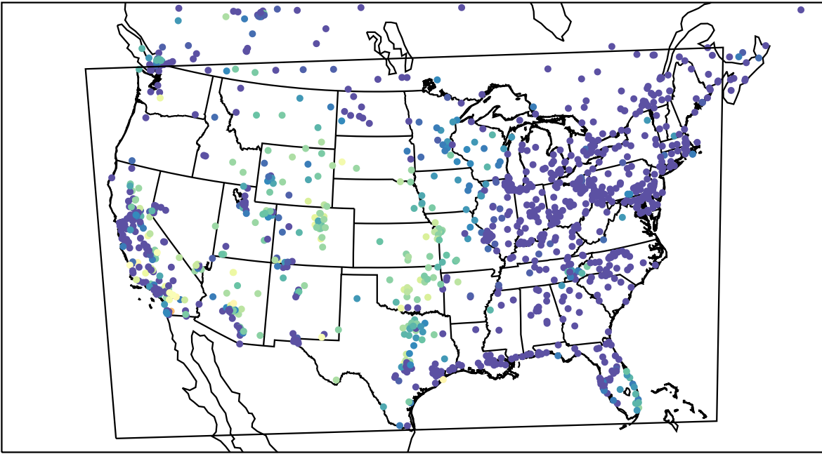
AirNOW (2023-10-18_09:00:00)
