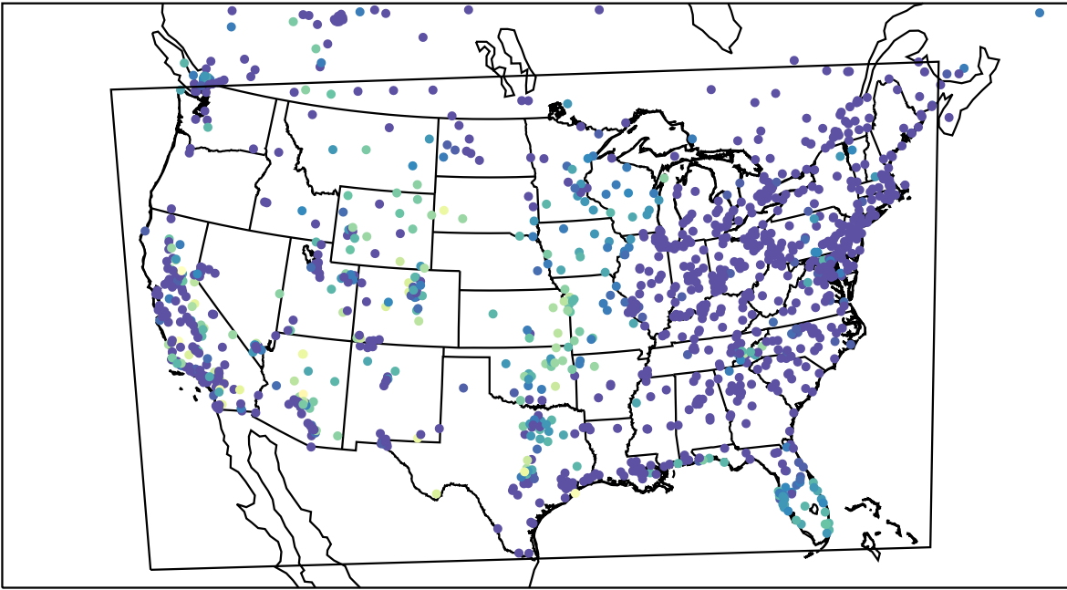
AirNOW (2023-10-18_13:00:00)
