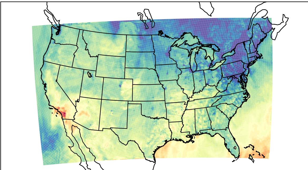
WRF (2023-10-18_00:00:00)
