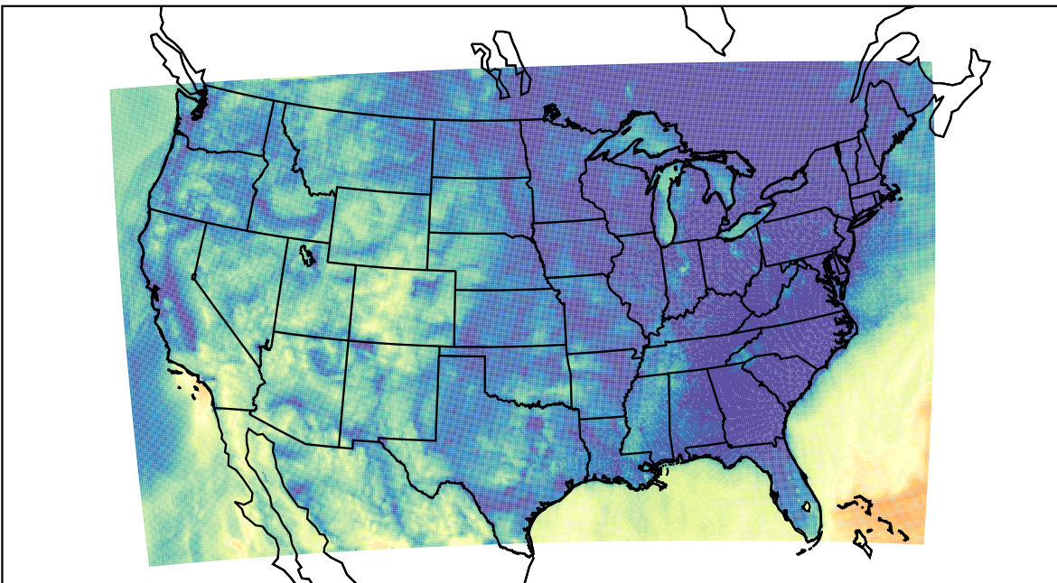
WRF (2023-10-17_13:00:00)
