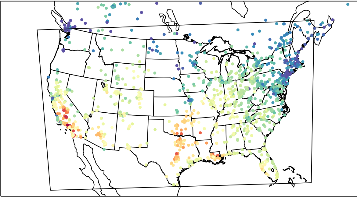
AirNOW (2023-10-18_20:00:00)
