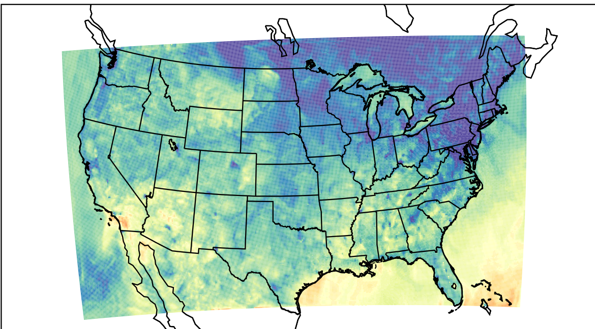
WRF (2023-10-18_04:00:00)
