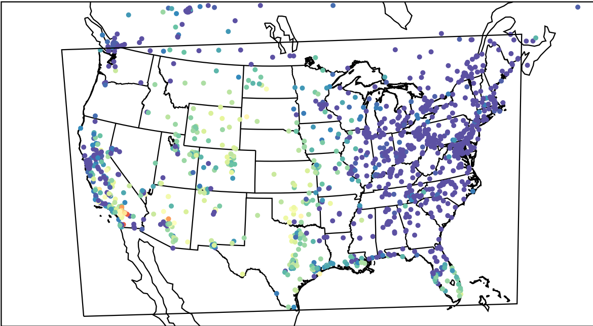
AirNOW (2023-10-18_03:00:00)
