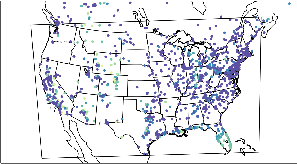
AirNOW (2023-10-17_14:00:00)
