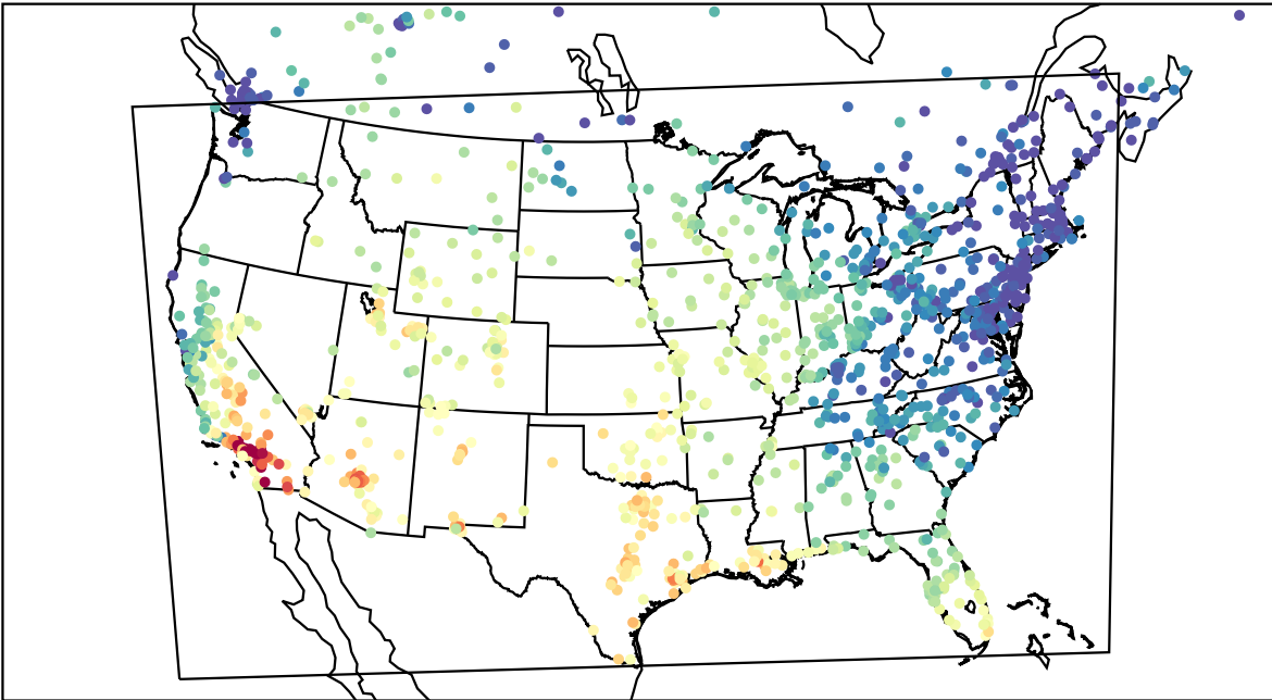
AirNOW (2023-10-17_21:00:00)
