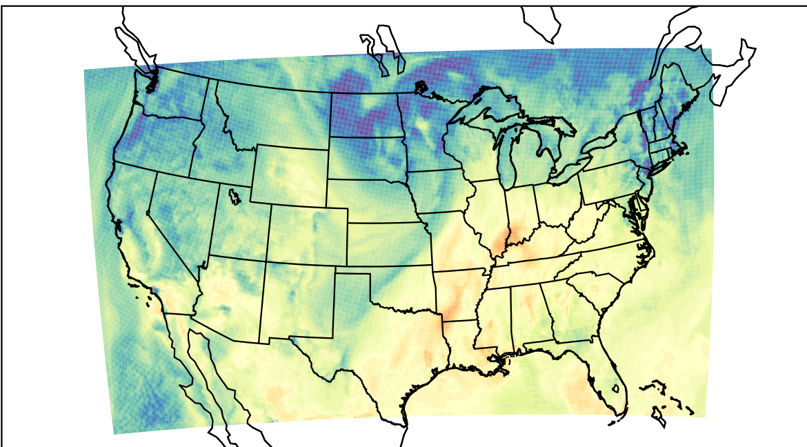
WRF (2023-10-18_18:00:00)
