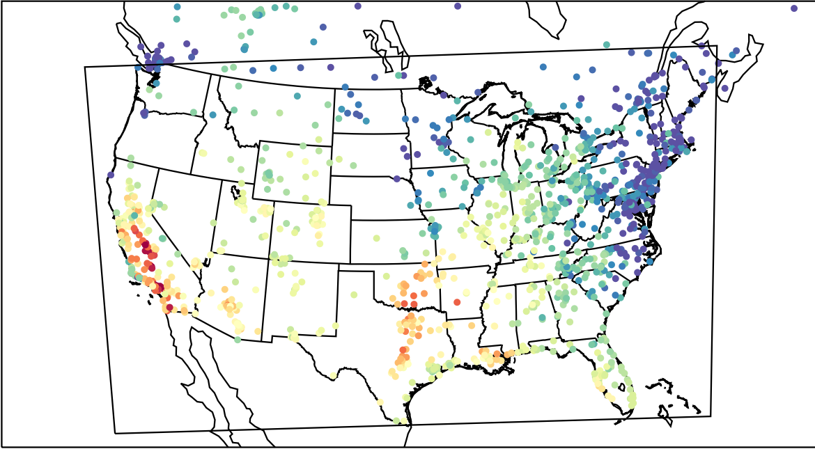
AirNOW (2023-10-18_22:00:00)
