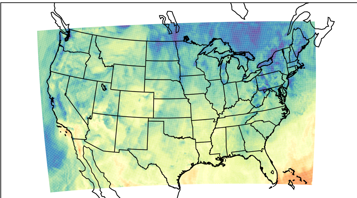
WRF (2023-10-17_18:00:00)
