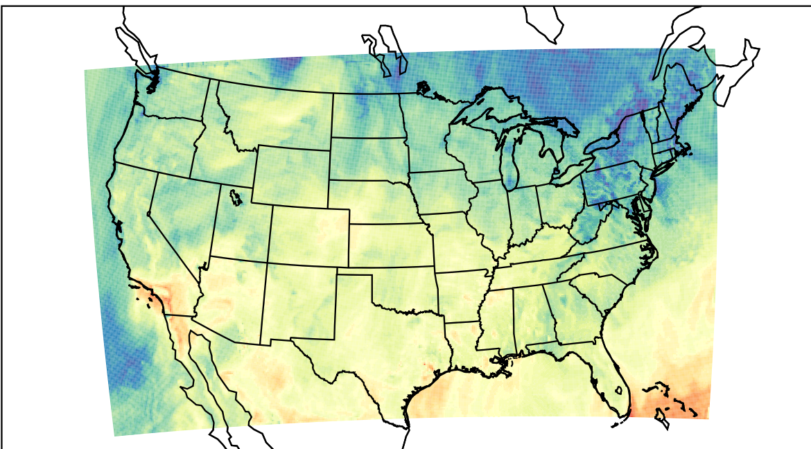
WRF (2023-10-17_20:00:00)
