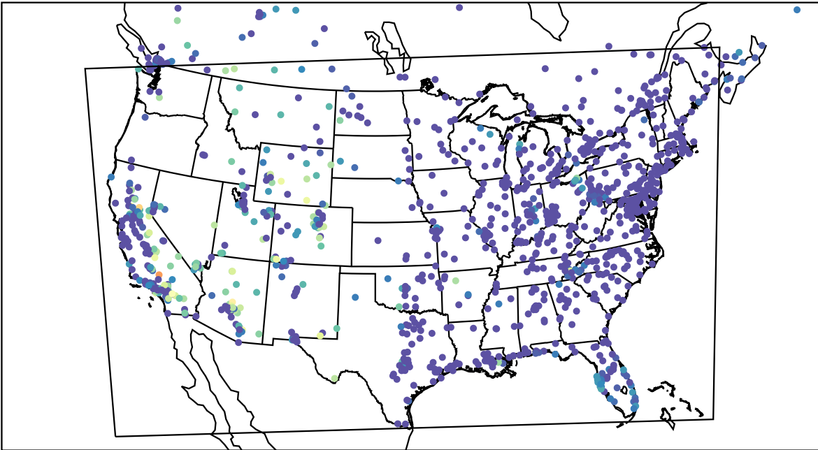
AirNOW (2023-10-17_10:00:00)
