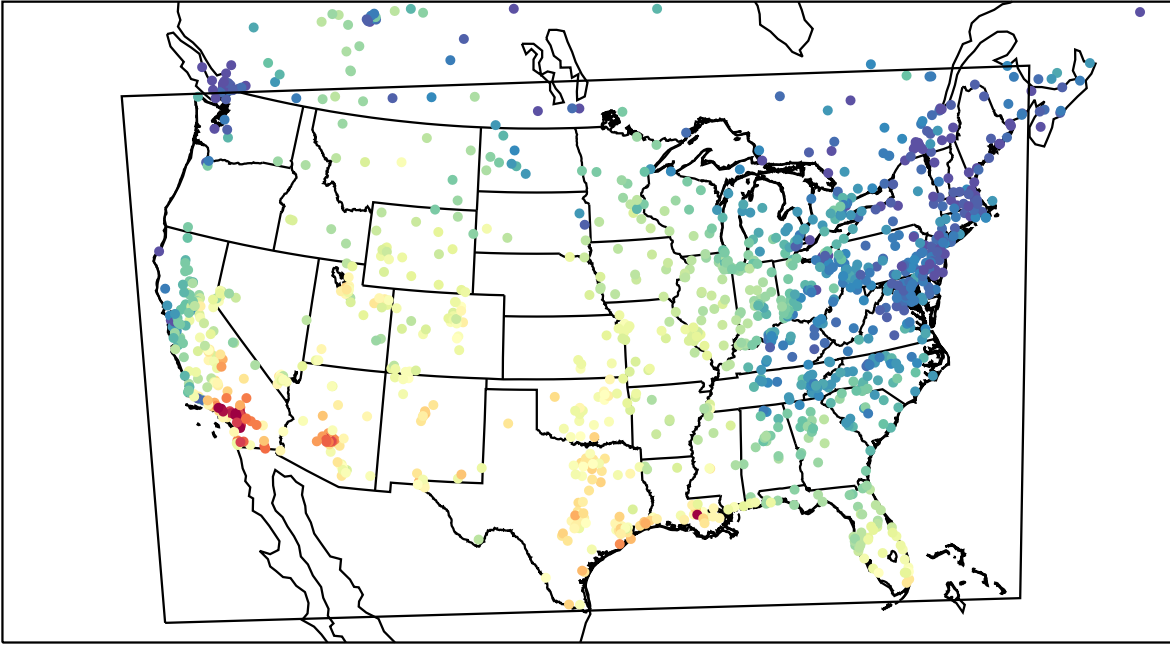
AirNOW (2023-10-17_20:00:00)
