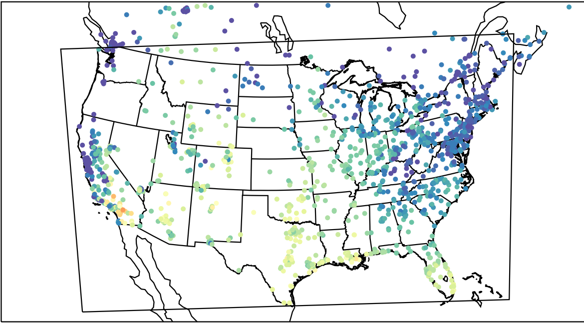
AirNOW (2023-10-17_17:00:00)
