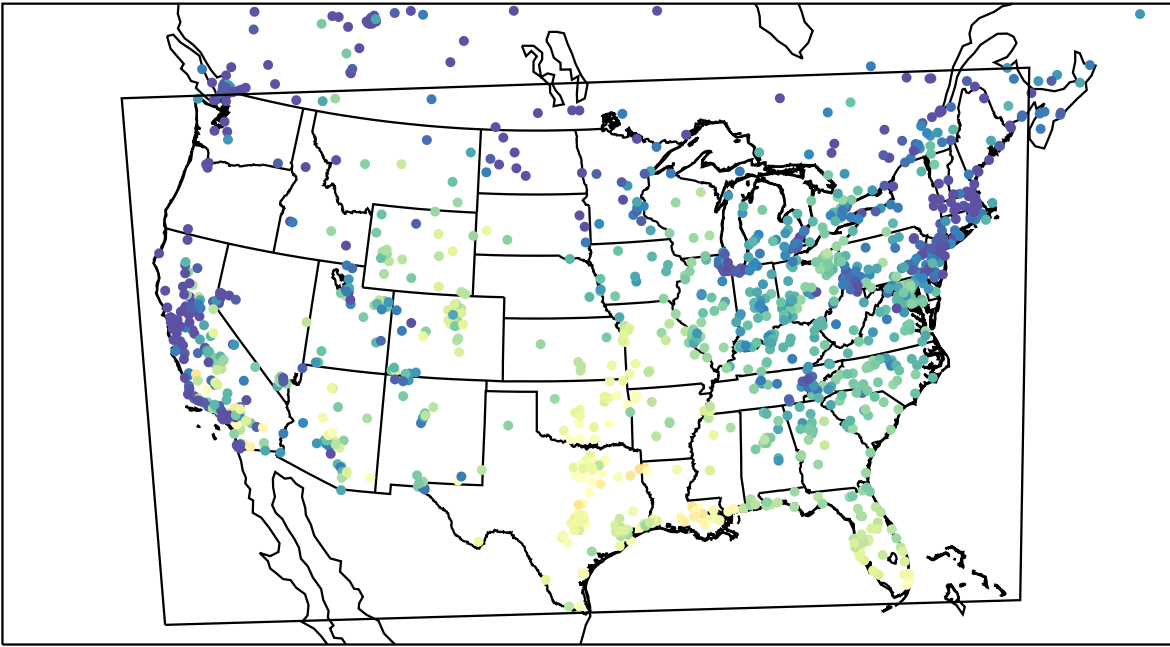
AirNOW (2023-10-18_16:00:00)
