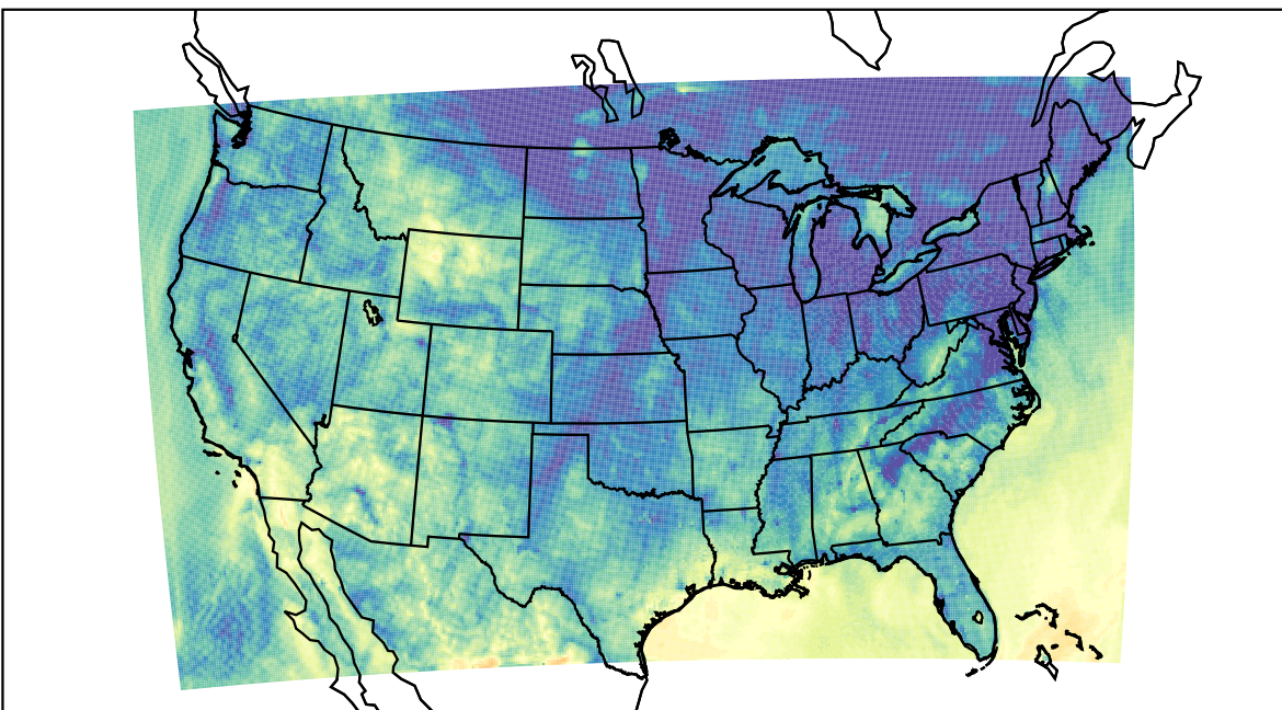
WRF (2023-10-18_11:00:00)
