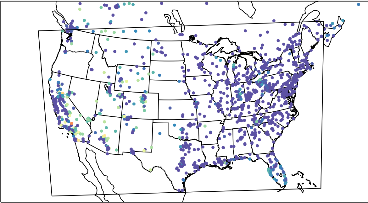
AirNOW (2023-10-17_09:00:00)
