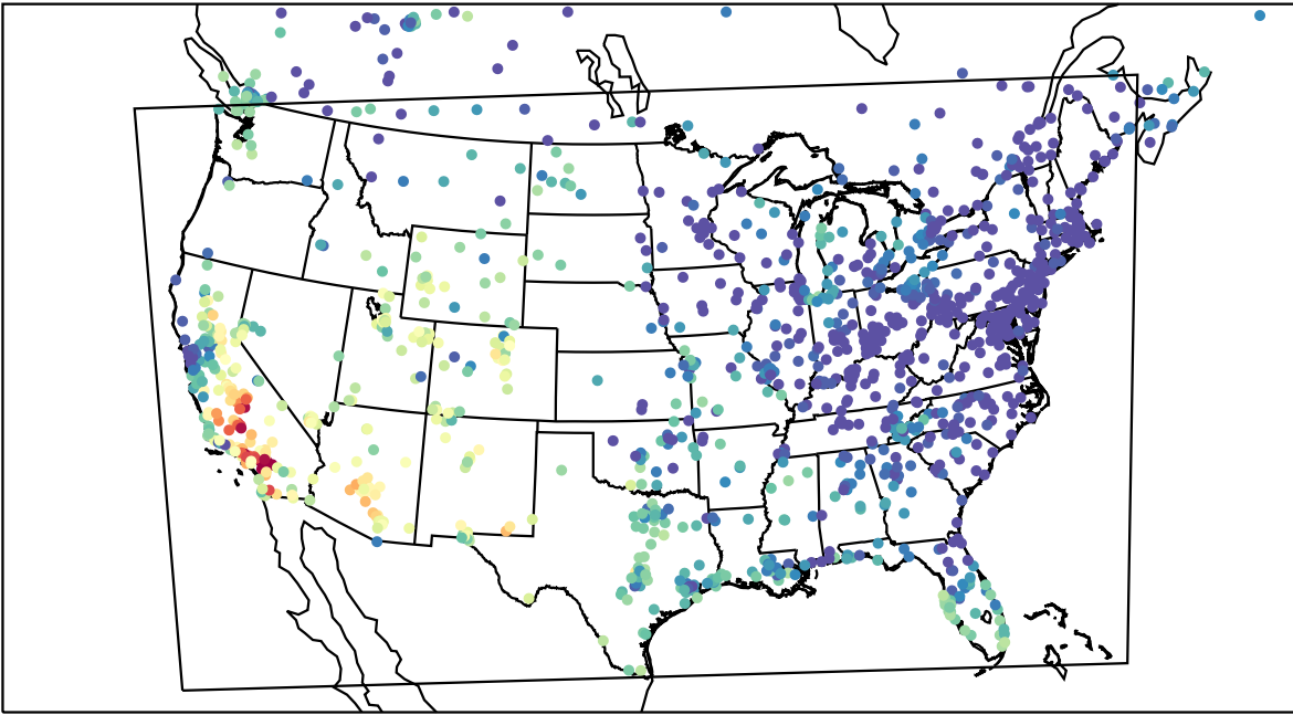
AirNOW (2023-10-17_00:00:00)
