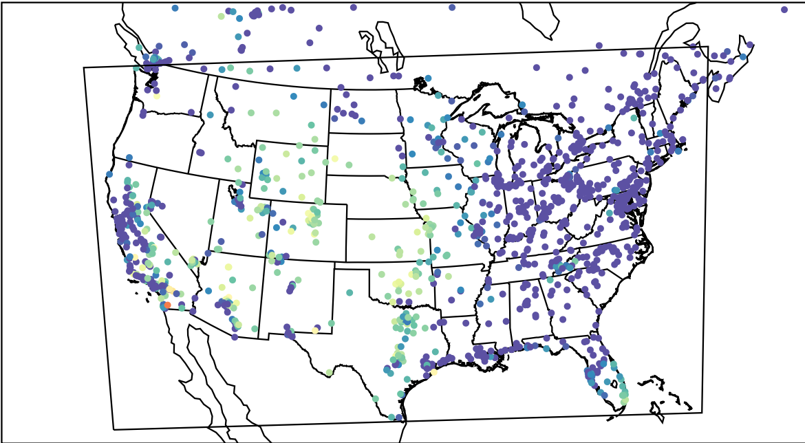
AirNOW (2023-10-18_07:00:00)
