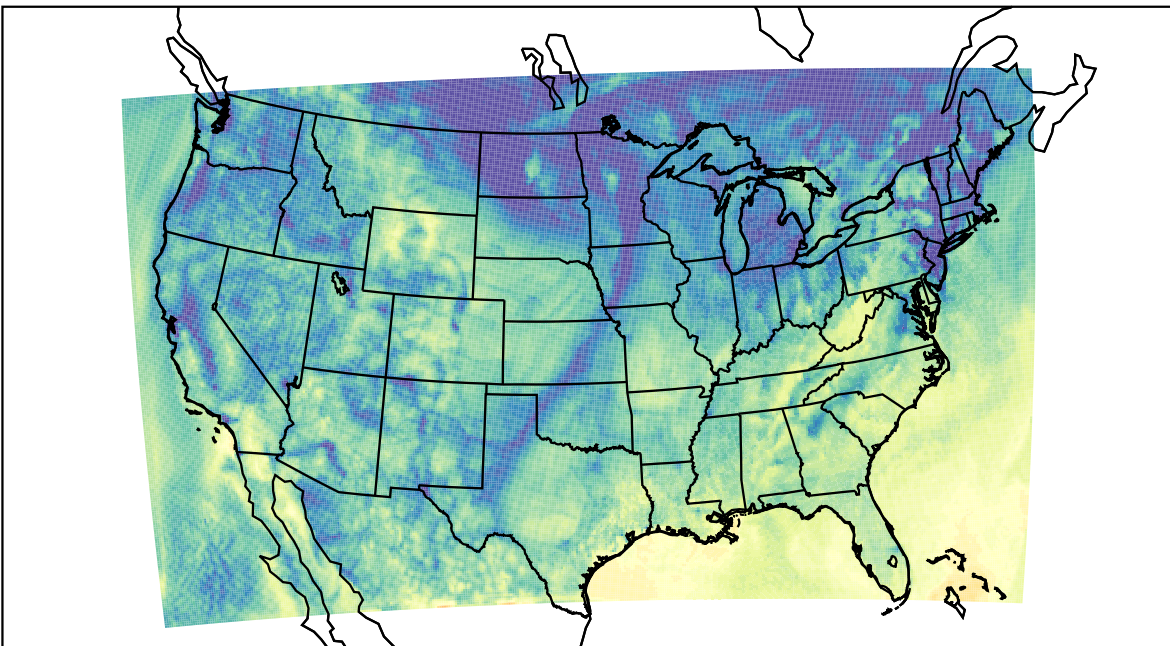
WRF (2023-10-18_15:00:00)
