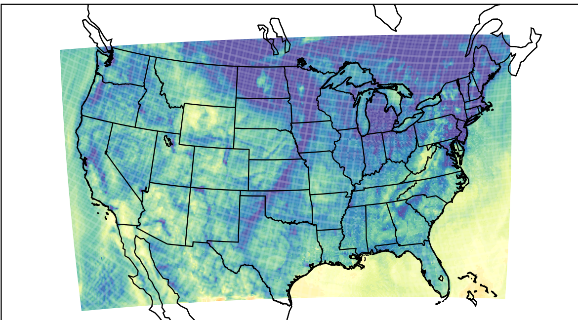
WRF (2023-10-18_14:00:00)
