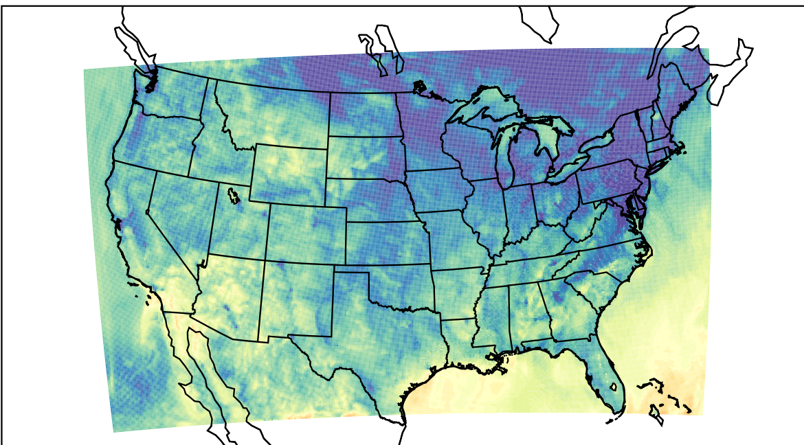
WRF (2023-10-18_07:00:00)
