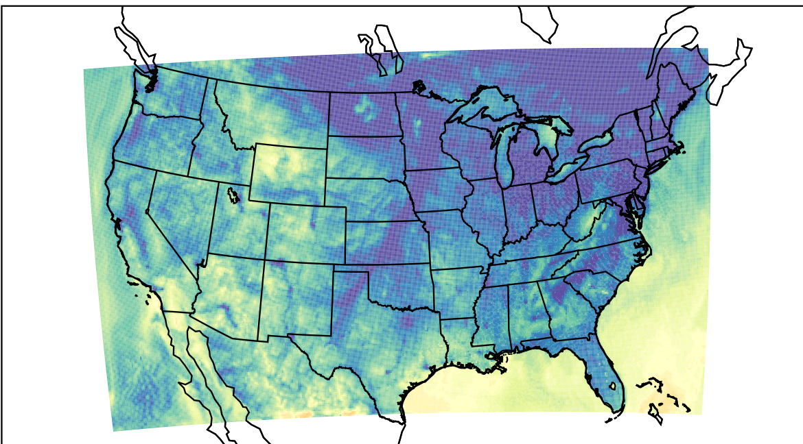
WRF (2023-10-18_13:00:00)
