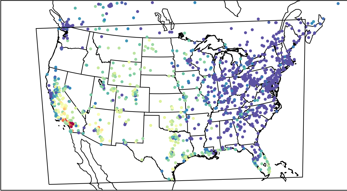
AirNOW (2023-10-18_01:00:00)
