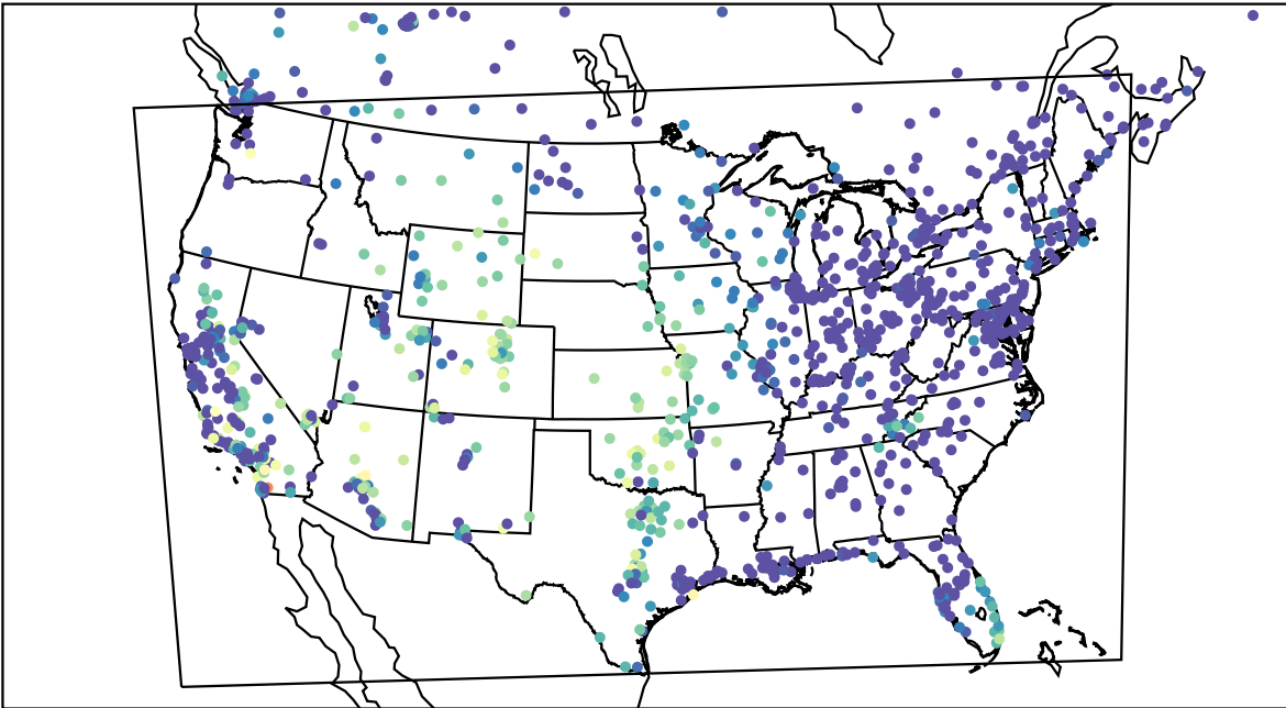
AirNOW (2023-10-18_08:00:00)
