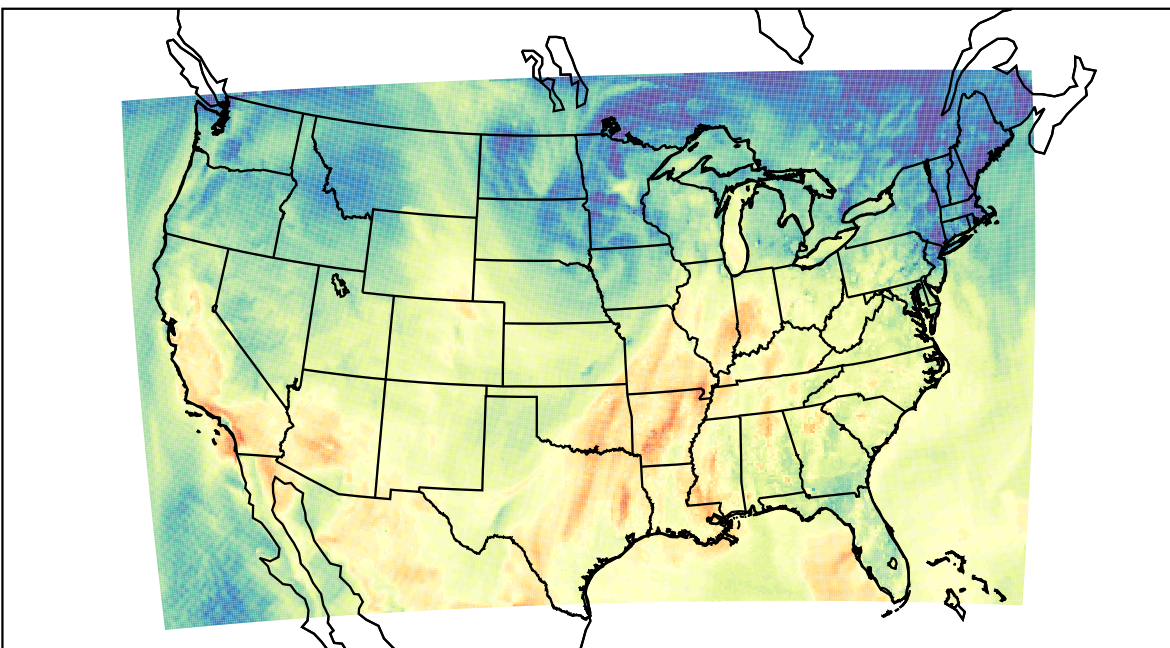
WRF (2023-10-18_22:00:00)
