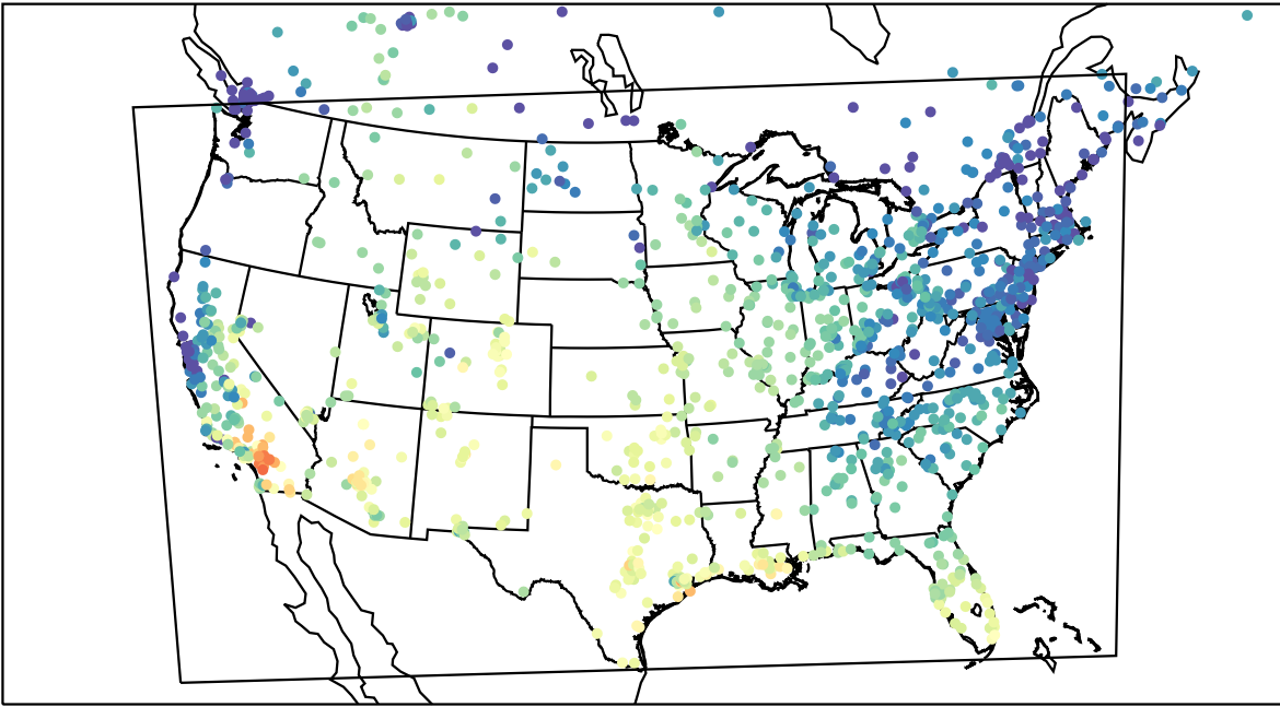
AirNOW (2023-10-17_18:00:00)
