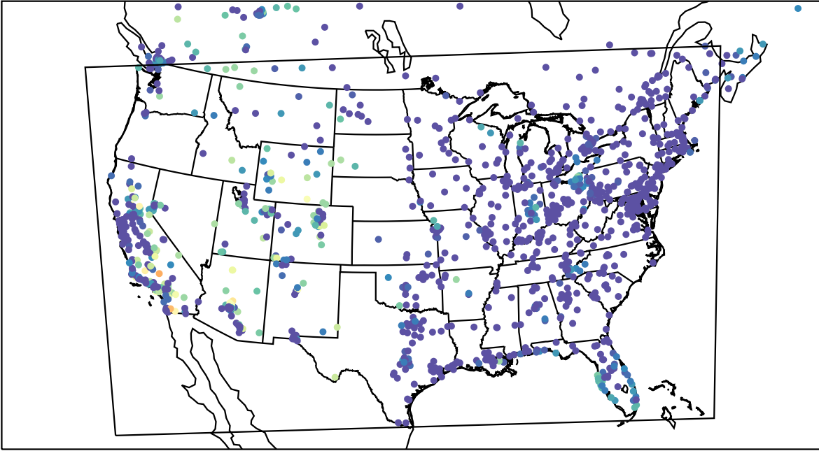
AirNOW (2023-10-17_08:00:00)
