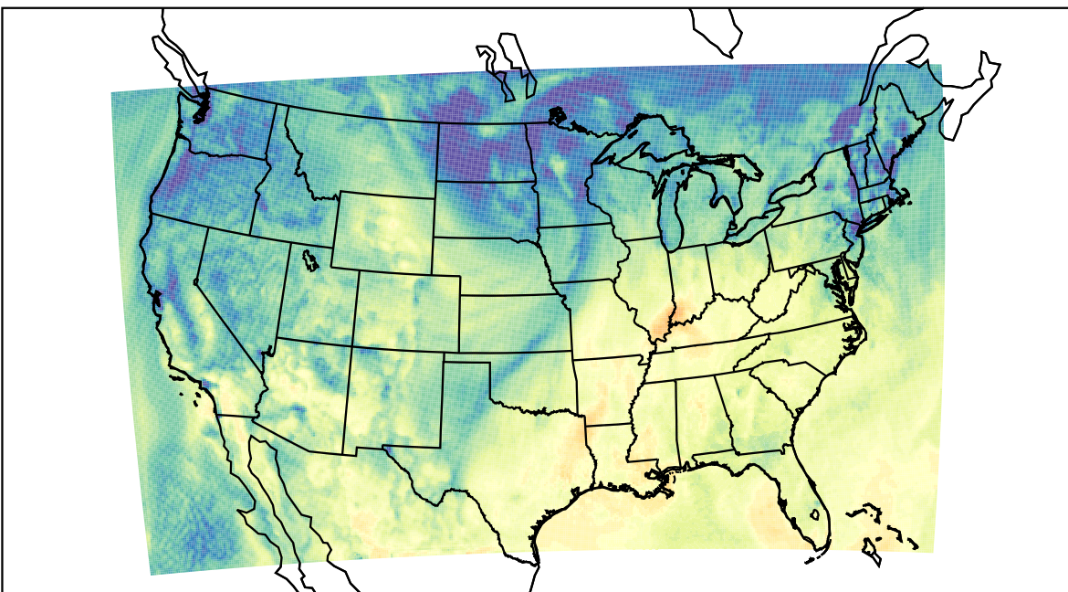
WRF (2023-10-18_17:00:00)
