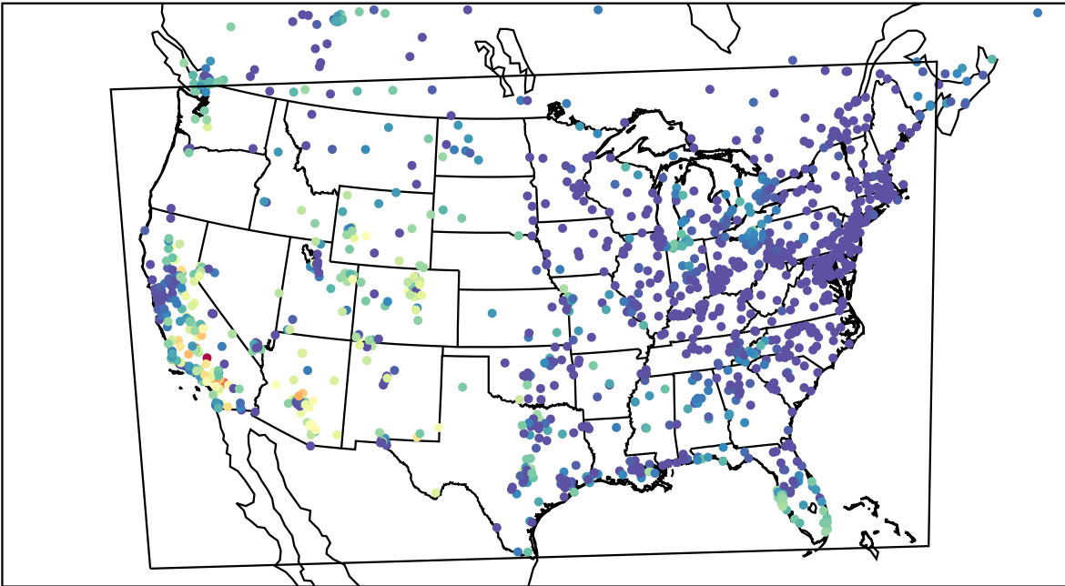
AirNOW (2023-10-17_02:00:00)
