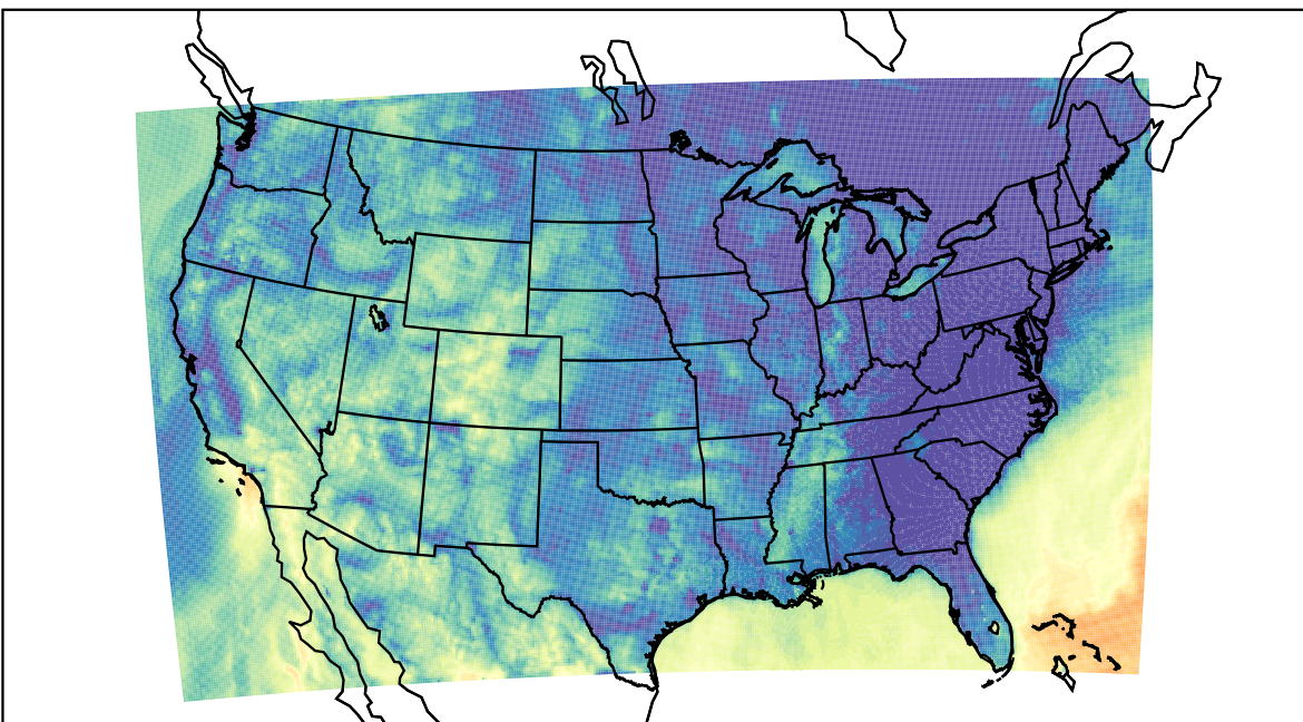
WRF (2023-10-17_12:00:00)
