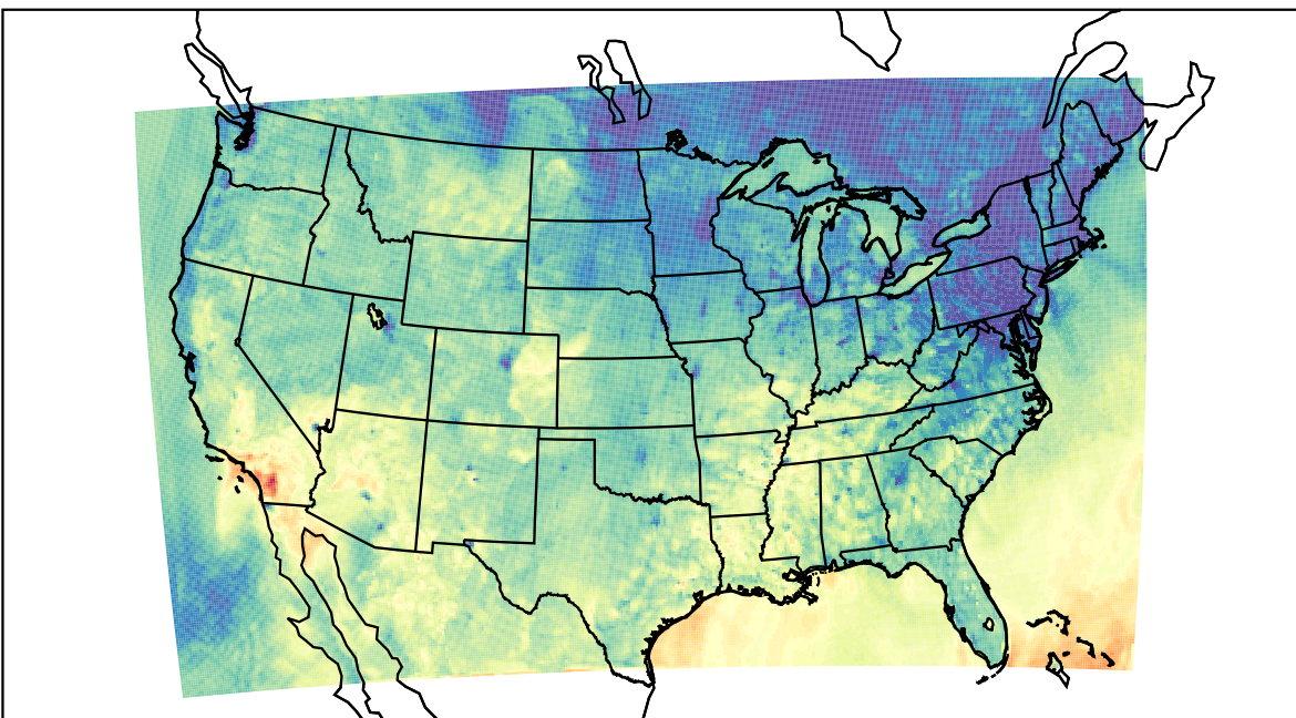
WRF (2023-10-18_01:00:00)
