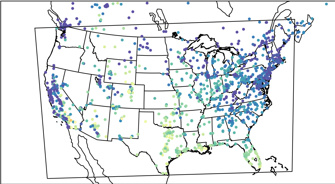
AirNOW (2023-10-17_16:00:00)
