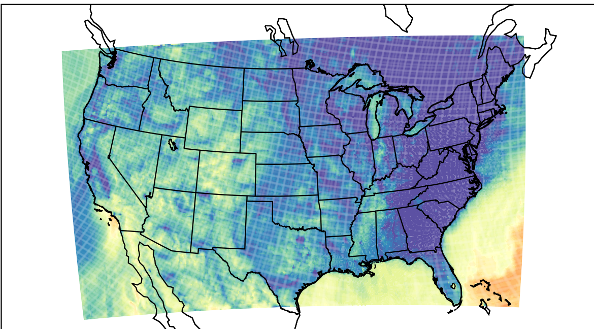
WRF (2023-10-17_11:00:00)
