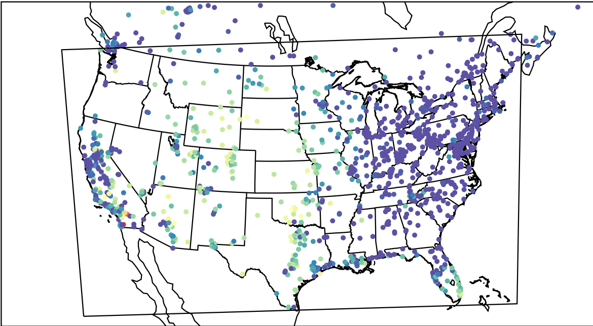
AirNOW (2023-10-18_04:00:00)
