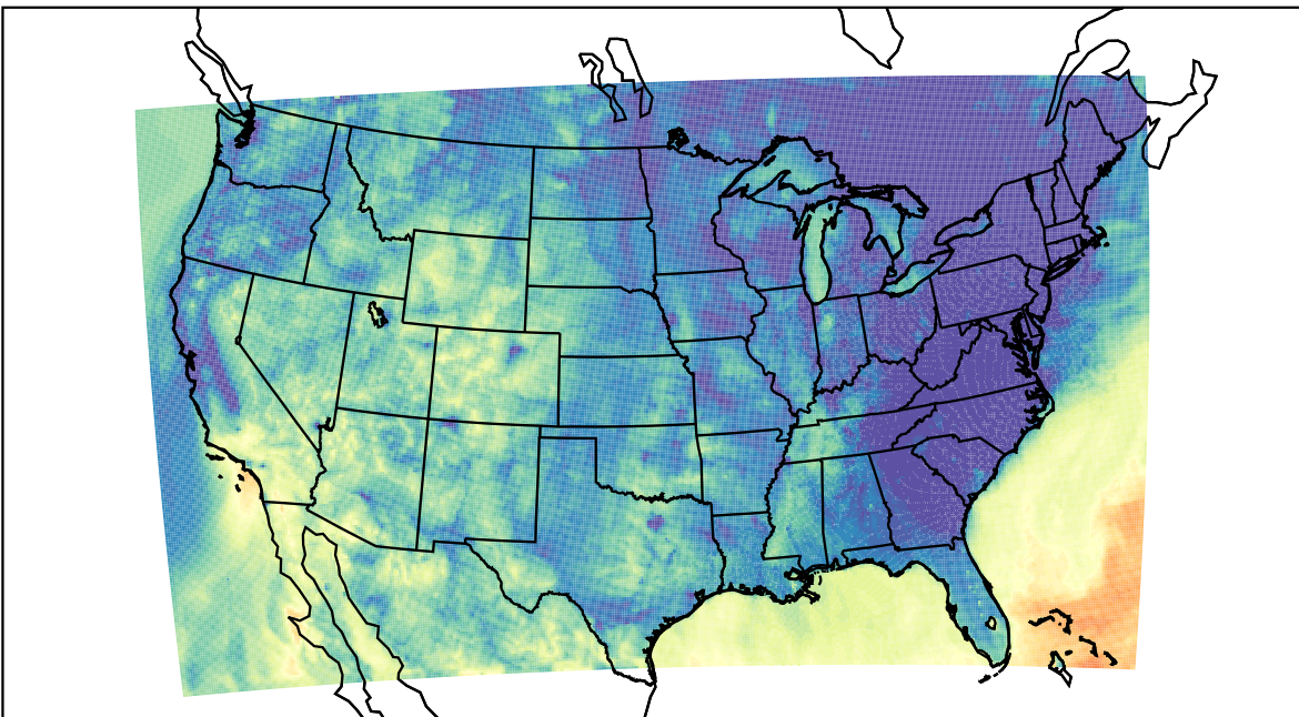
WRF (2023-10-17_08:00:00)
