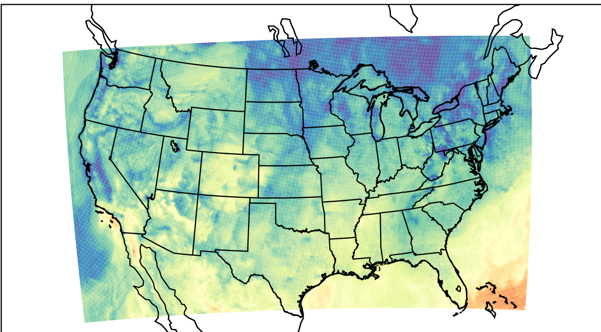
WRF (2023-10-17_17:00:00)
