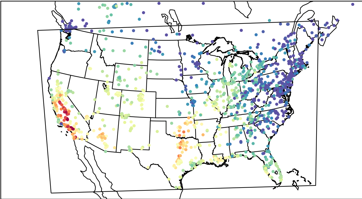
AirNOW (2023-10-18_23:00:00)
