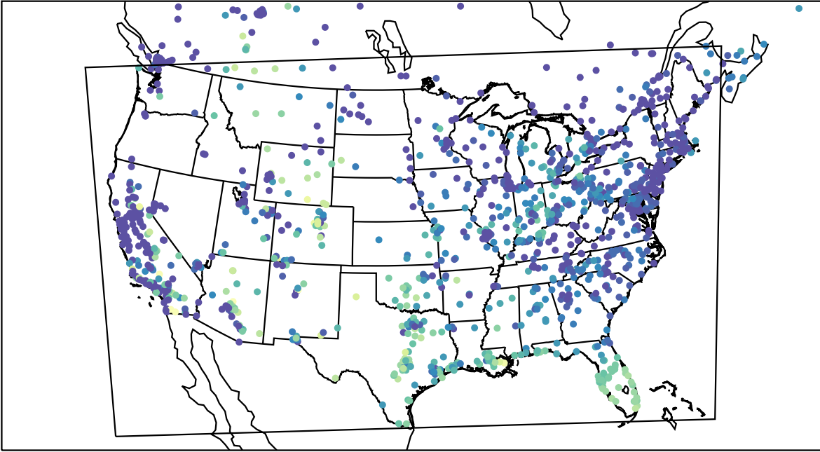
AirNOW (2023-10-17_15:00:00)
