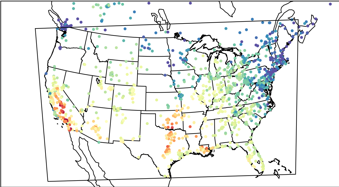
AirNOW (2023-10-18_21:00:00)
