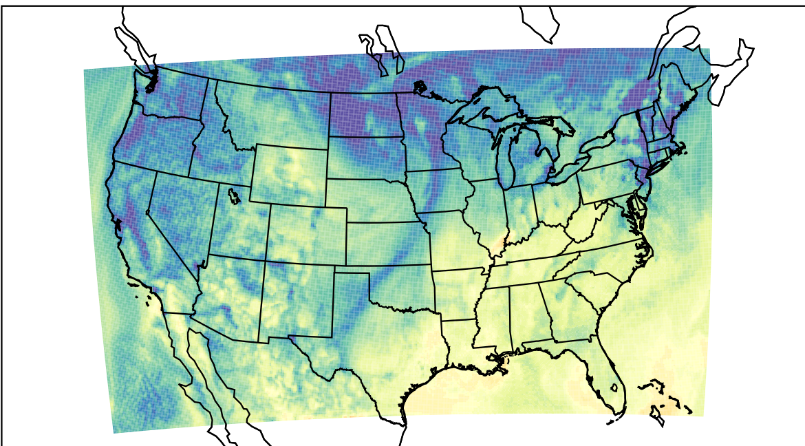
WRF (2023-10-18_16:00:00)
