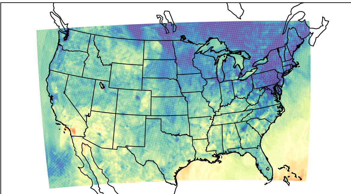
WRF (2023-10-18_03:00:00)
