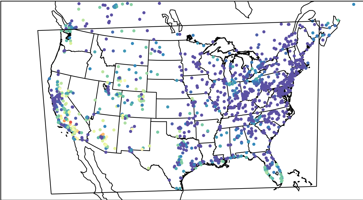
AirNOW (2023-10-17_03:00:00)
