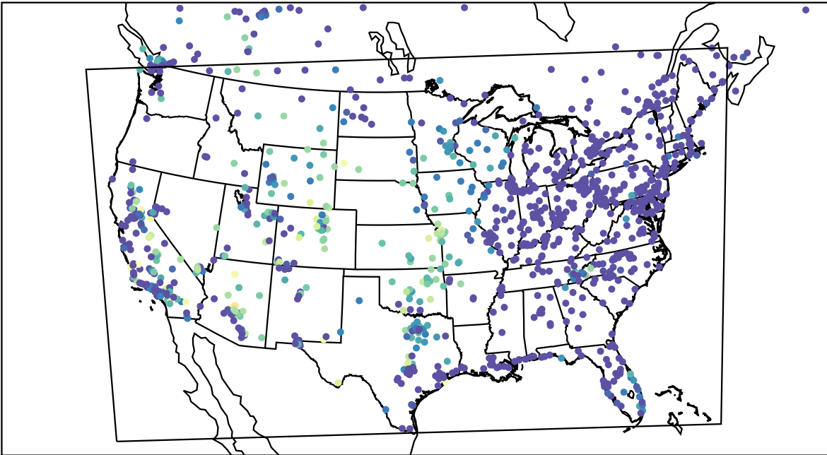
AirNOW (2023-10-18_11:00:00)
