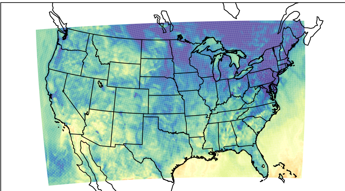
WRF (2023-10-18_06:00:00)
