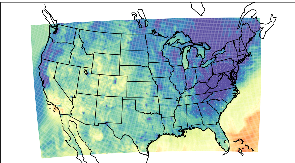
WRF (2023-10-17_03:00:00)
