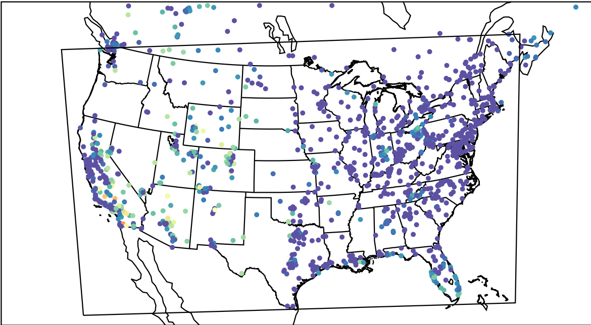
AirNOW (2023-10-17_07:00:00)
