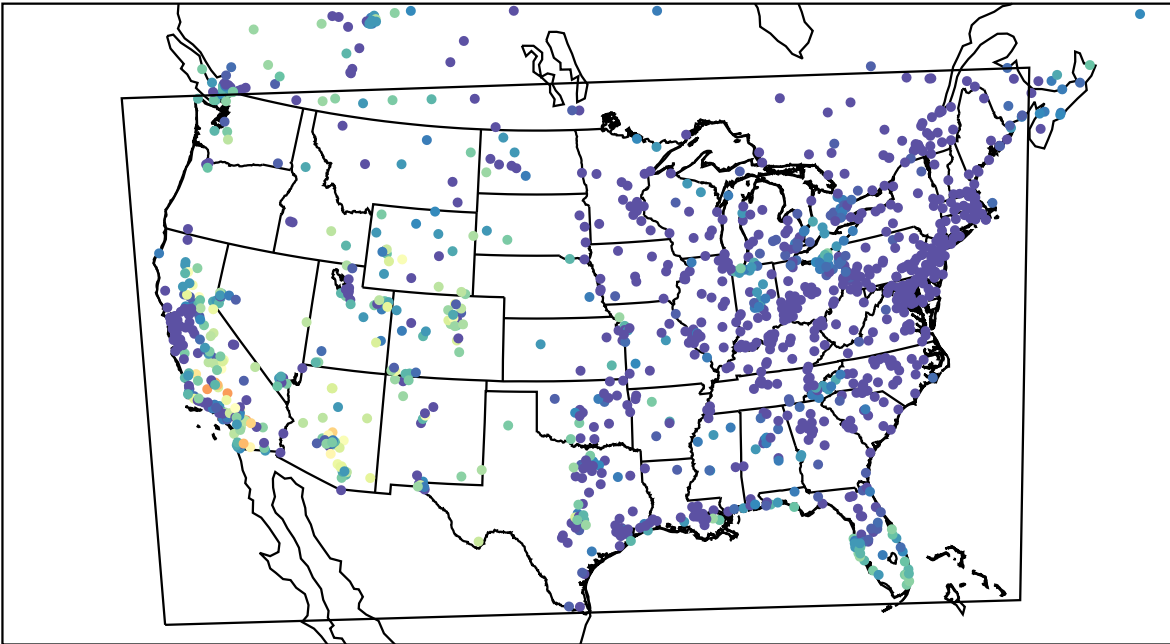
AirNOW (2023-10-17_04:00:00)
