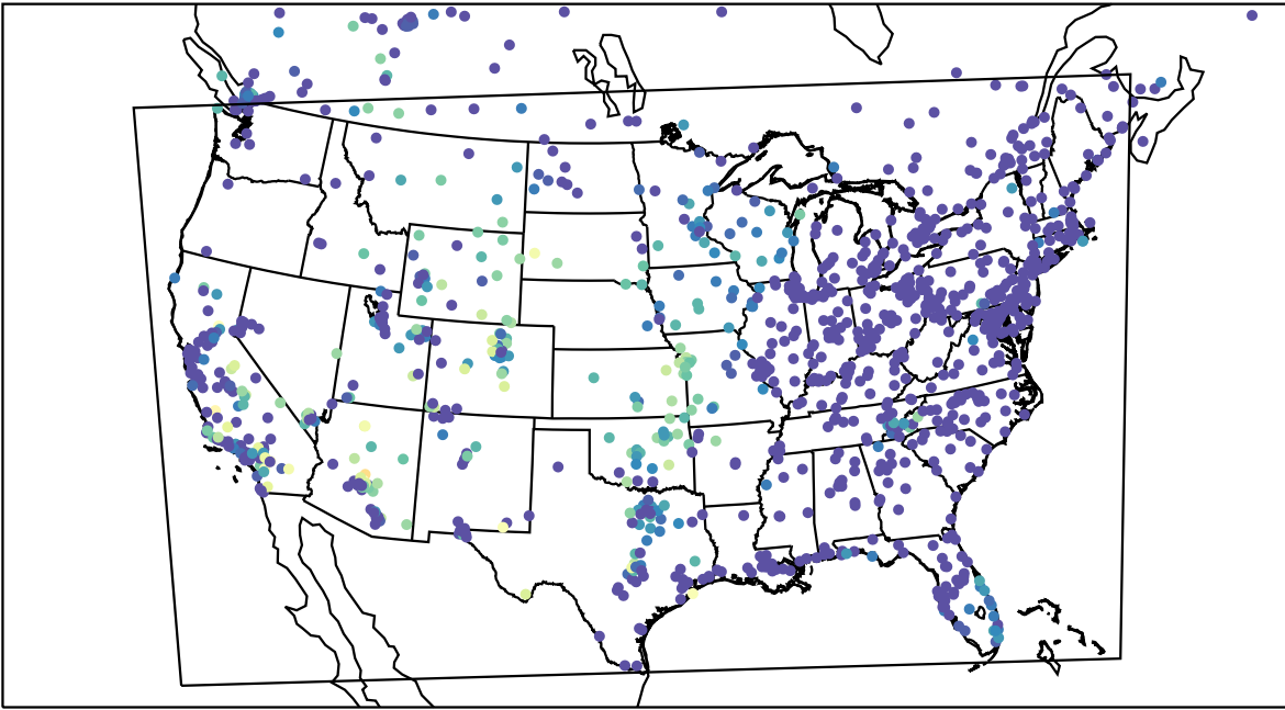
AirNOW (2023-10-18_12:00:00)
