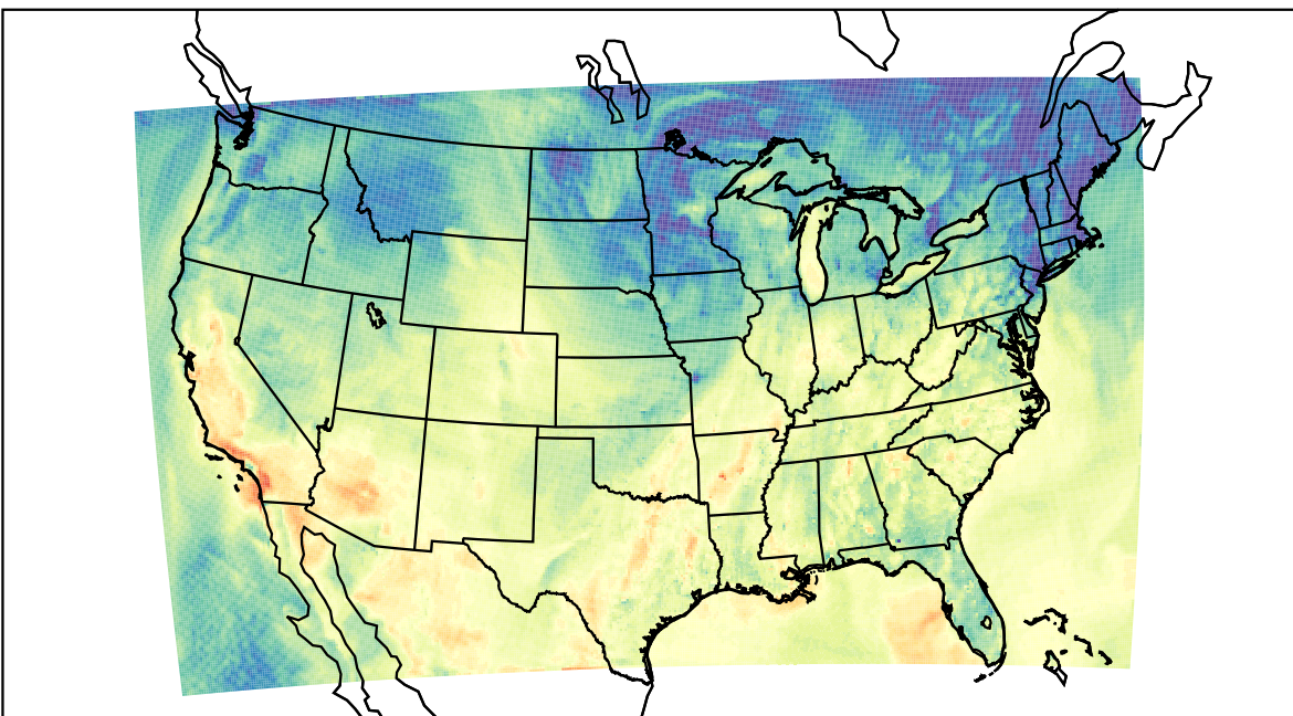
WRF (2023-10-18_23:00:00)
