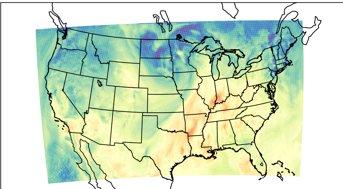
WRF (2023-10-18_19:00:00)
