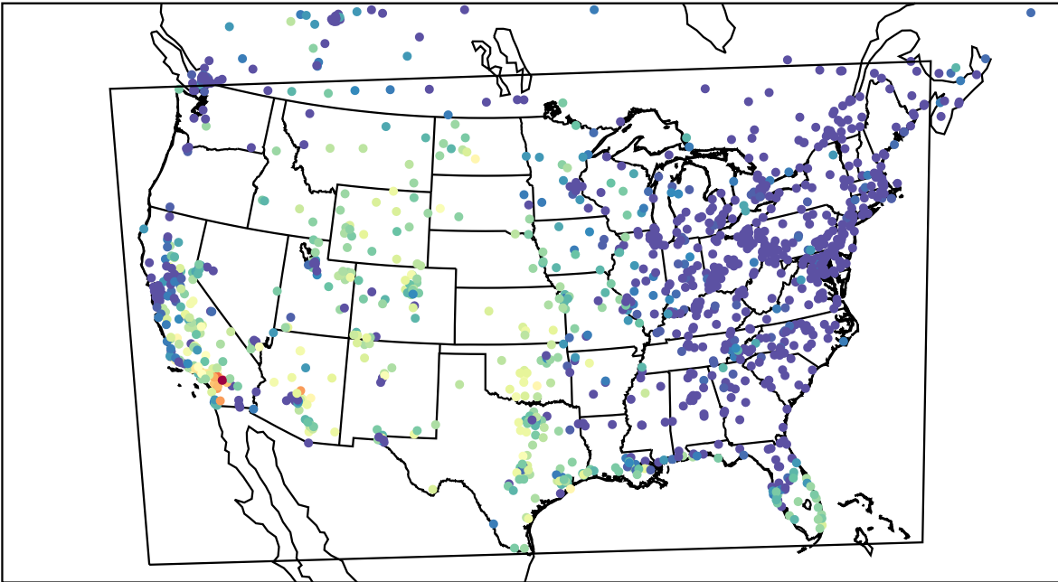
AirNOW (2023-10-18_02:00:00)
