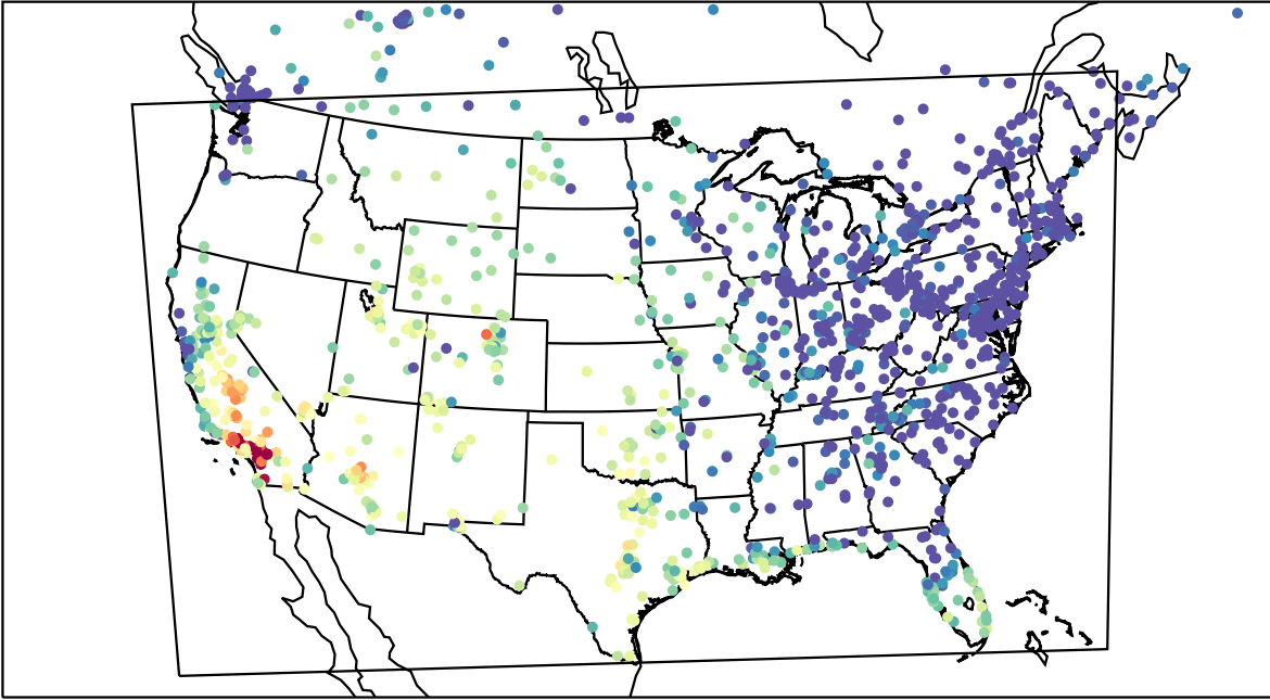
AirNOW (2023-10-18_00:00:00)
