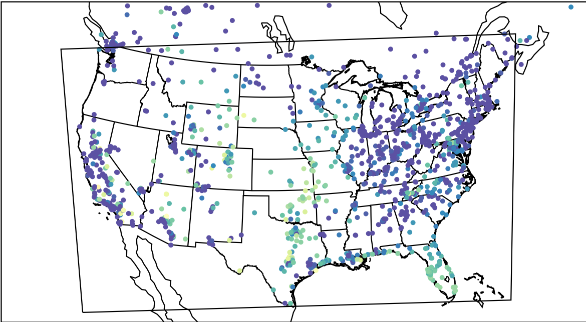
AirNOW (2023-10-18_14:00:00)
