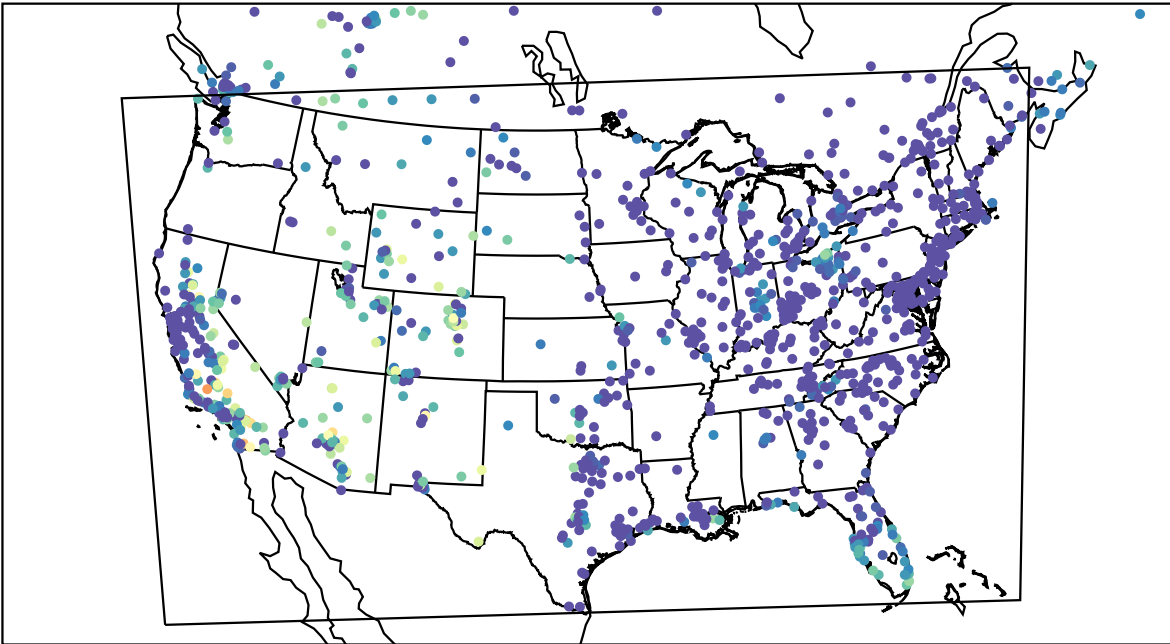
AirNOW (2023-10-17_06:00:00)
