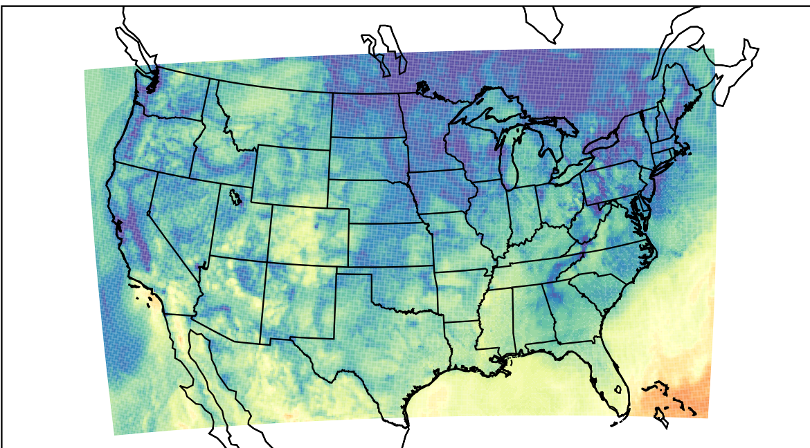
WRF (2023-10-17_16:00:00)
