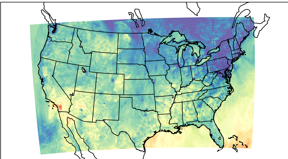
WRF (2023-10-18_02:00:00)
