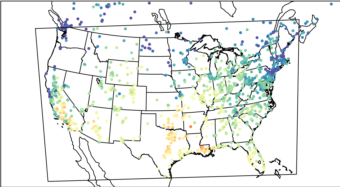
AirNOW (2023-10-18_18:00:00)
