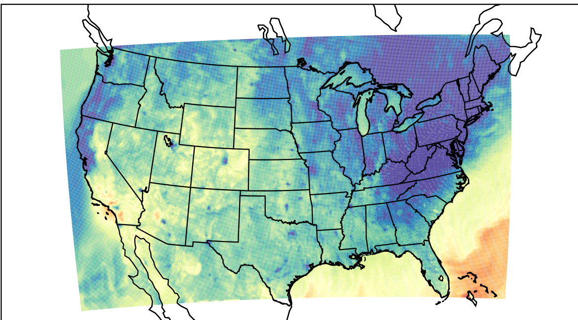
WRF (2023-10-17_02:00:00)
