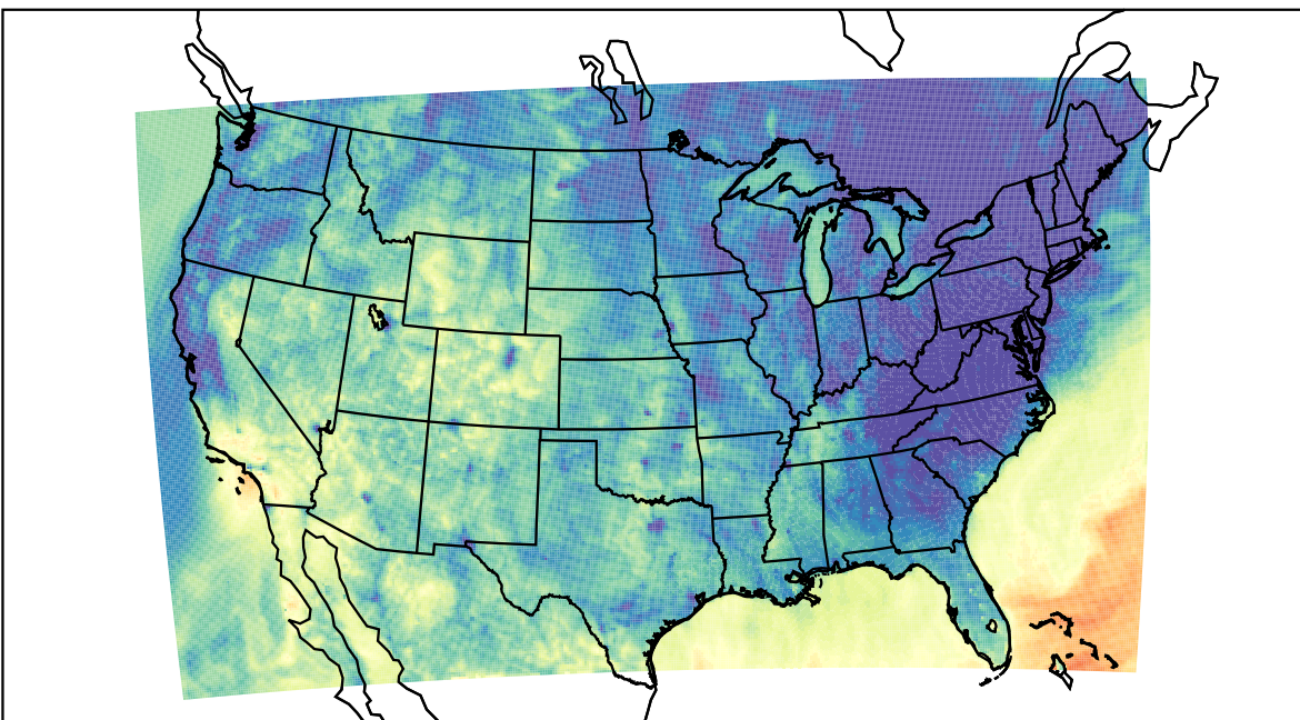
WRF (2023-10-17_05:00:00)
