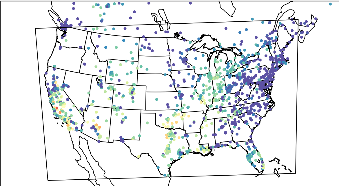
AirNOW (2023-10-19_02:00:00)
