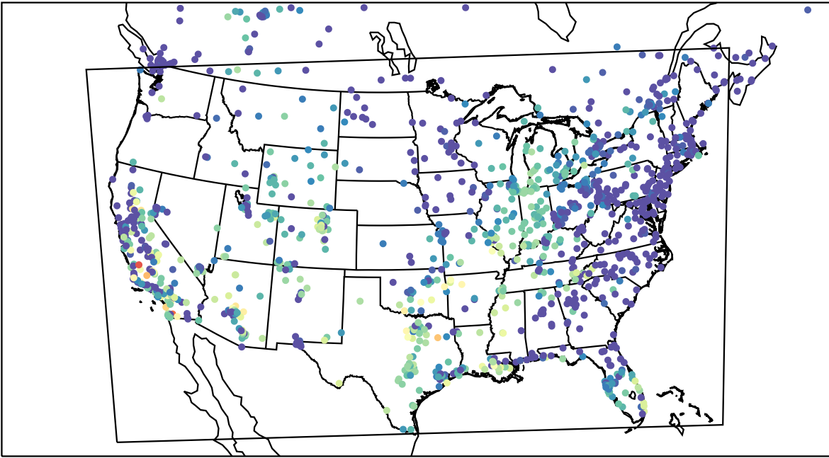
AirNOW (2023-10-19_04:00:00)
