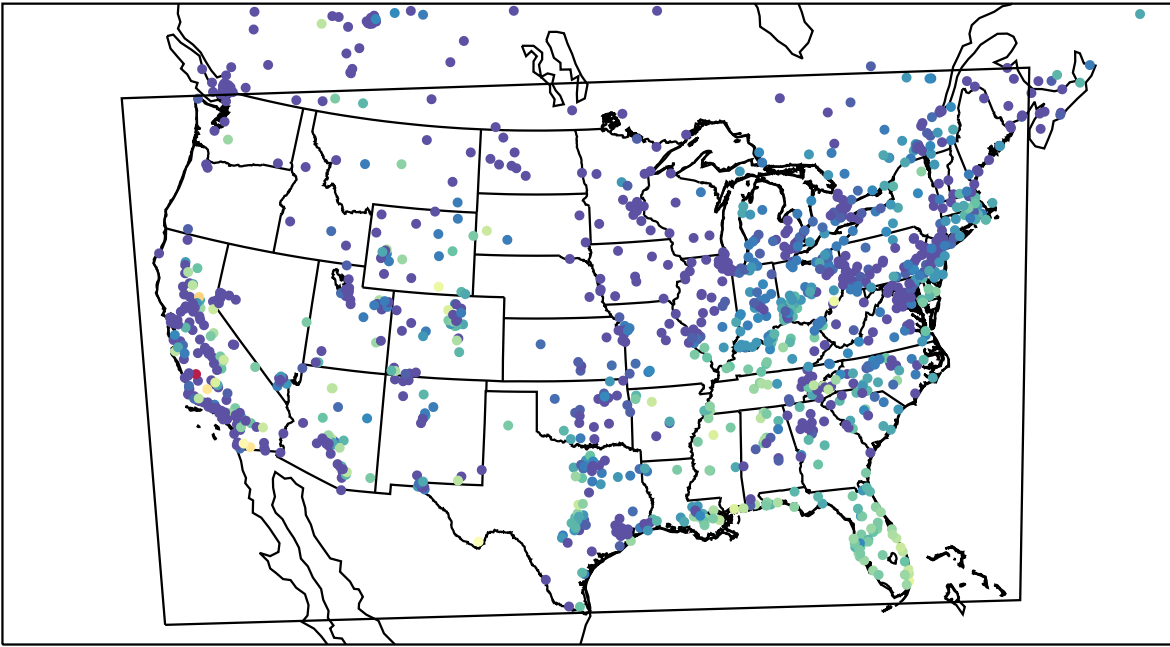
AirNOW (2023-10-19_14:00:00)
