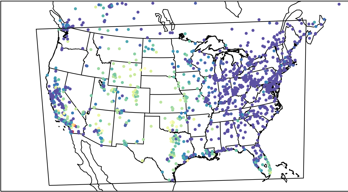
AirNOW (2023-10-18_04:00:00)
