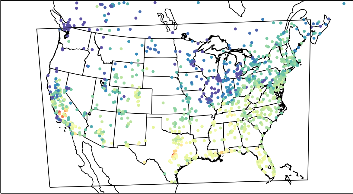
AirNOW (2023-10-19_17:00:00)
