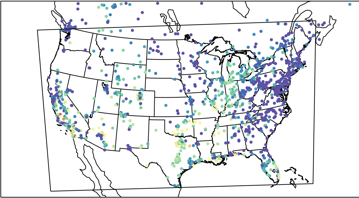
AirNOW (2023-10-19_03:00:00)
