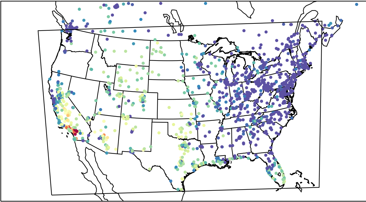
AirNOW (2023-10-18_01:00:00)
