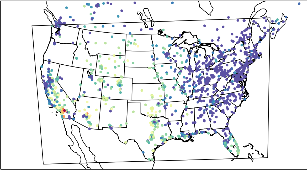
AirNOW (2023-10-18_02:00:00)
