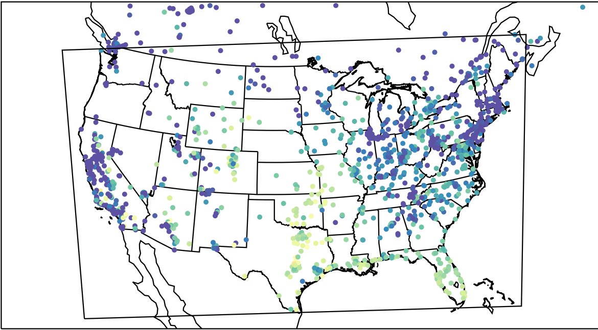
AirNOW (2023-10-18_15:00:00)
