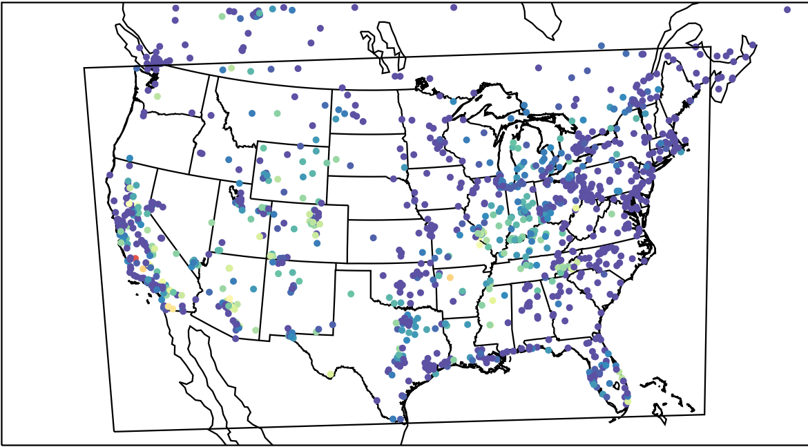
AirNOW (2023-10-19_09:00:00)
