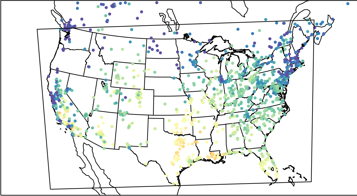
AirNOW (2023-10-18_17:00:00)
