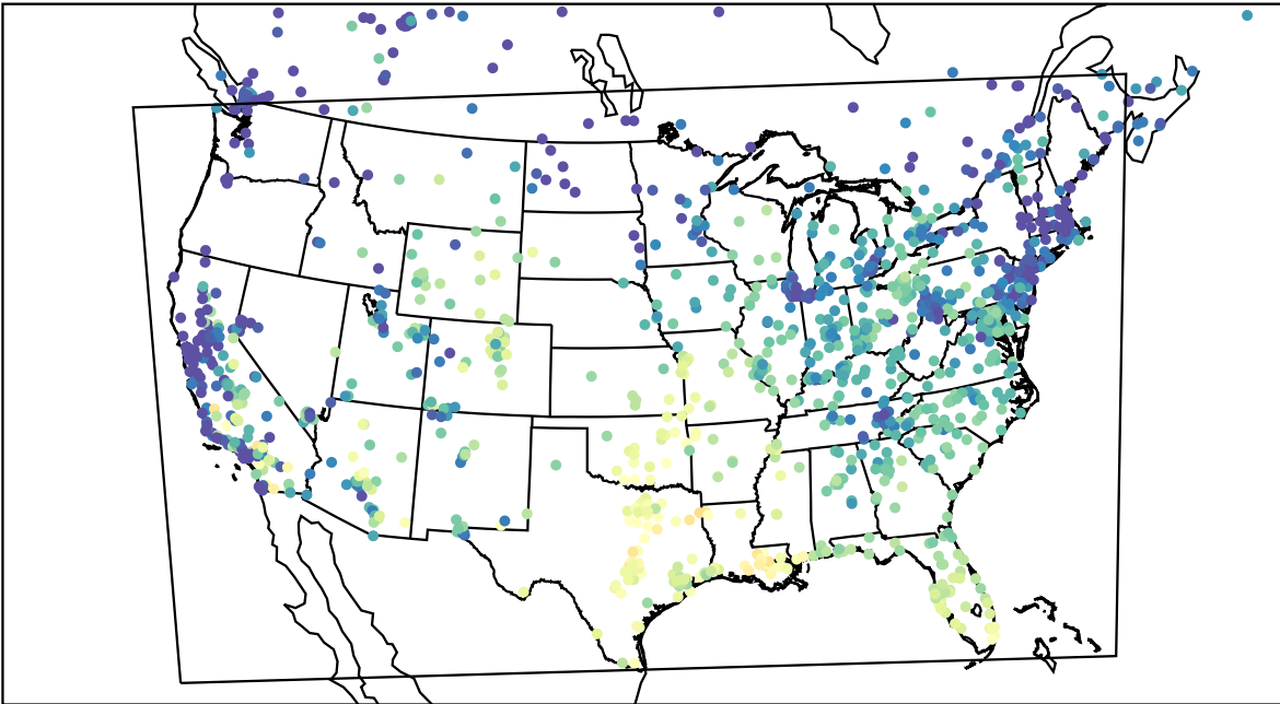
AirNOW (2023-10-18_16:00:00)
