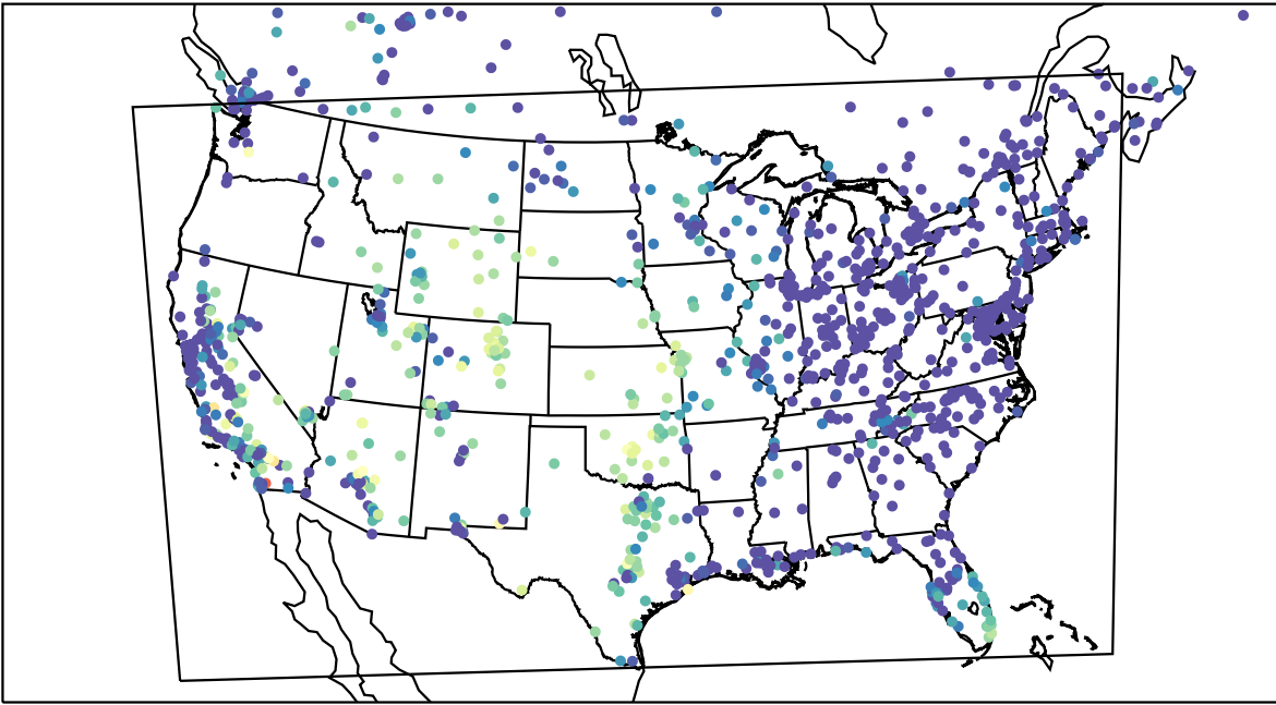
AirNOW (2023-10-18_06:00:00)
