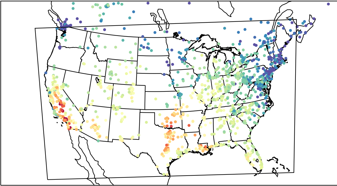
AirNOW (2023-10-18_21:00:00)
