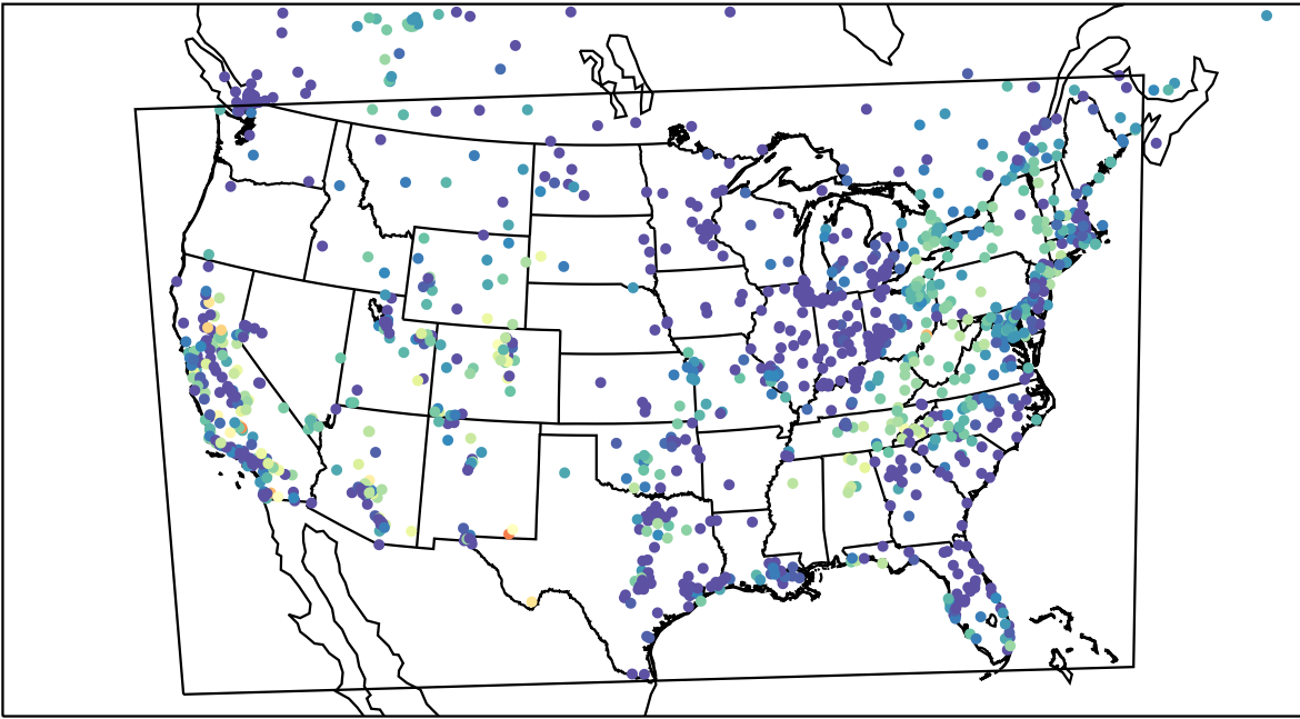
AirNOW (2023-10-20_06:00:00)
