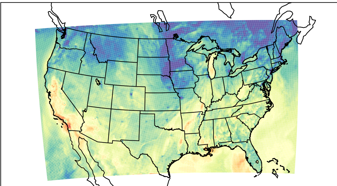
WRF (2023-10-19_00:00:00)
