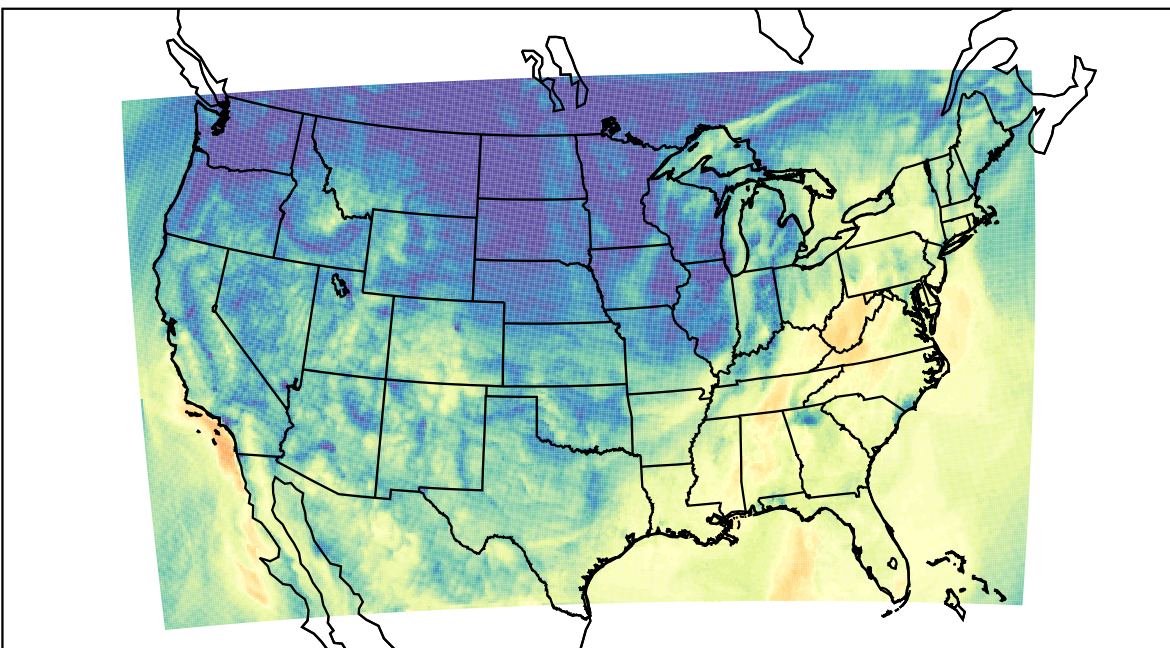
WRF (2023-10-19_16:00:00)
