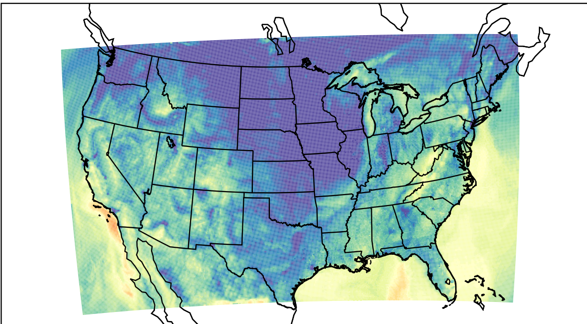
WRF (2023-10-19_14:00:00)
