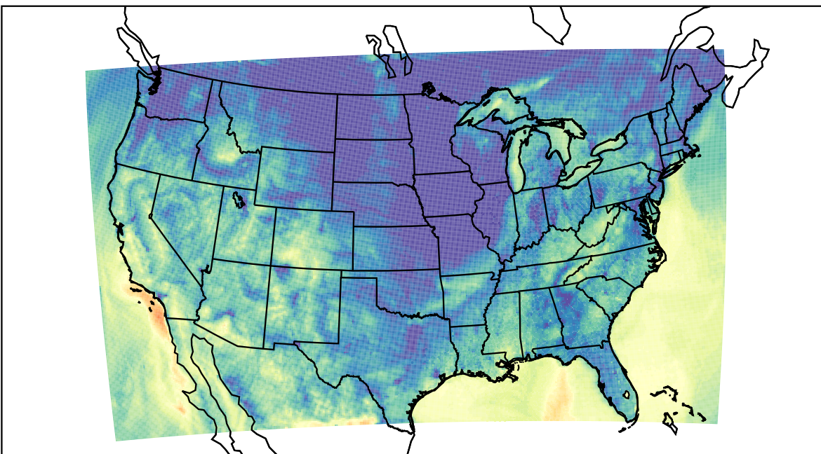
WRF (2023-10-19_13:00:00)
