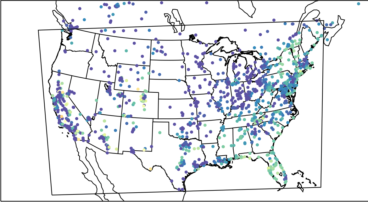
AirNOW (2023-10-20_14:00:00)
