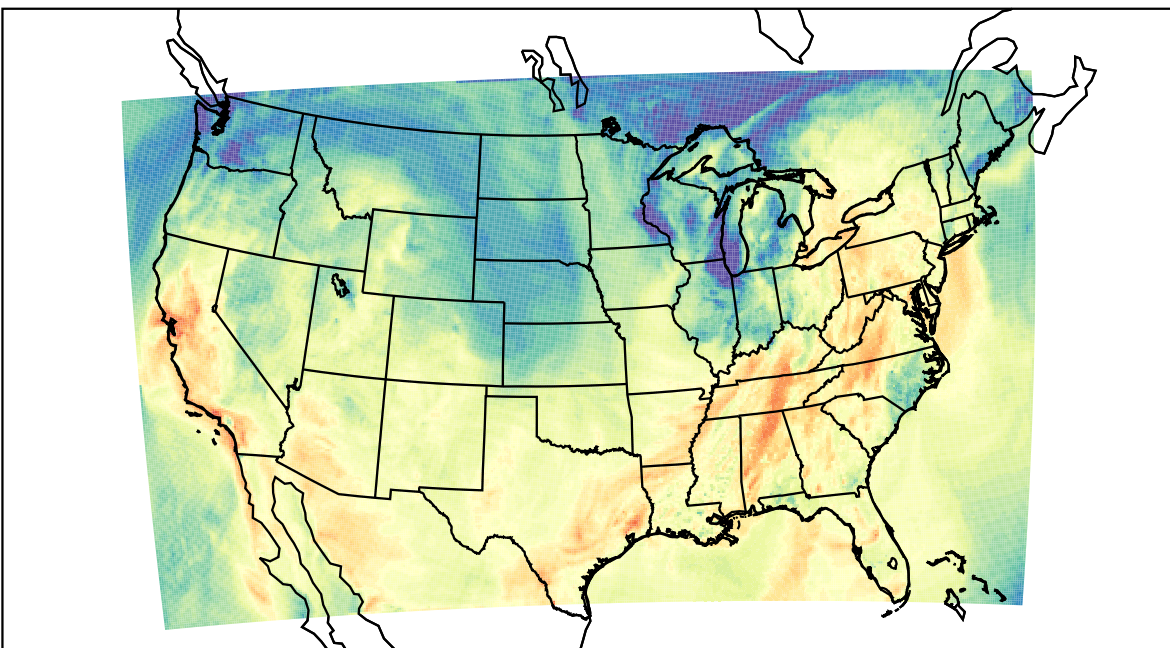
WRF (2023-10-19_21:00:00)
