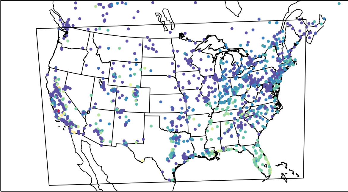
AirNOW (2023-10-19_14:00:00)
