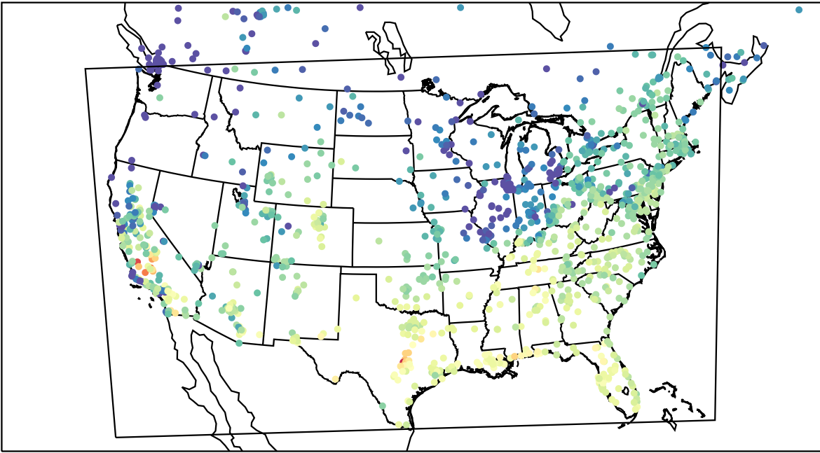
AirNOW (2023-10-19_17:00:00)
