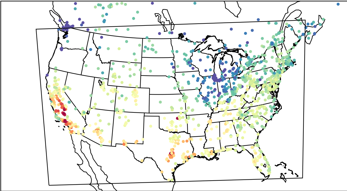
AirNOW (2023-10-19_20:00:00)
