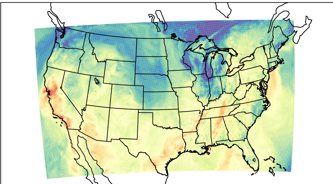
WRF (2023-10-19_22:00:00)
