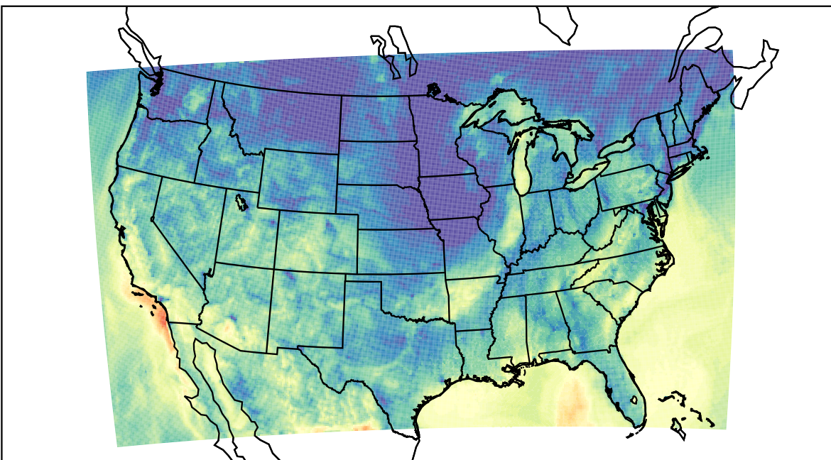
WRF (2023-10-19_08:00:00)
