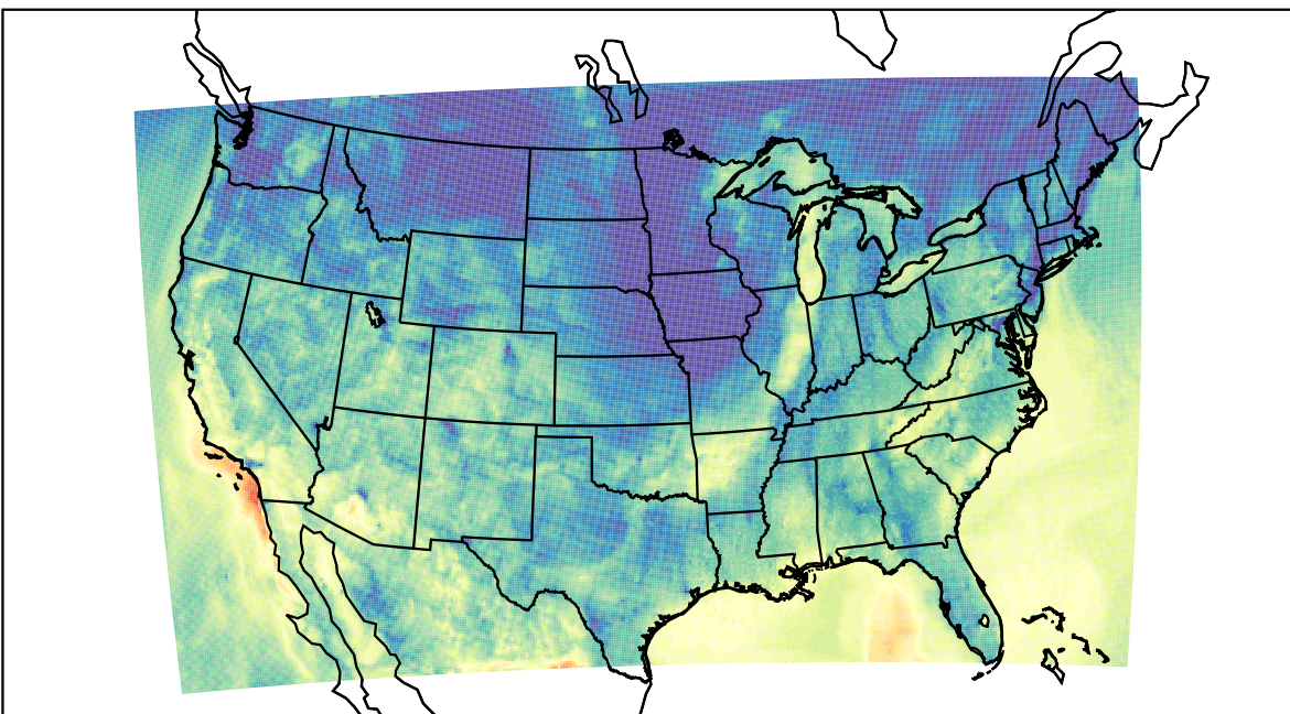
WRF (2023-10-19_07:00:00)
