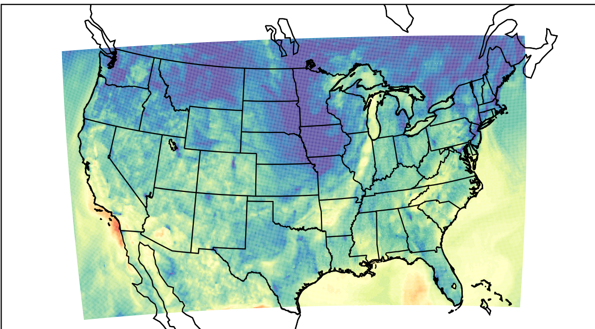
WRF (2023-10-19_05:00:00)
