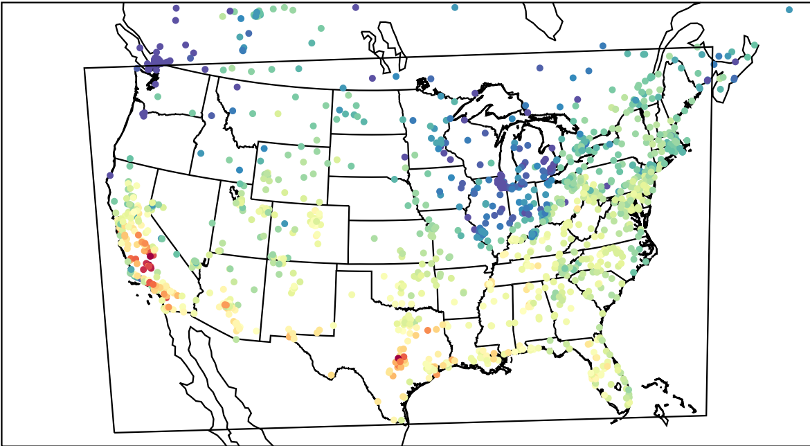
AirNOW (2023-10-19_19:00:00)
