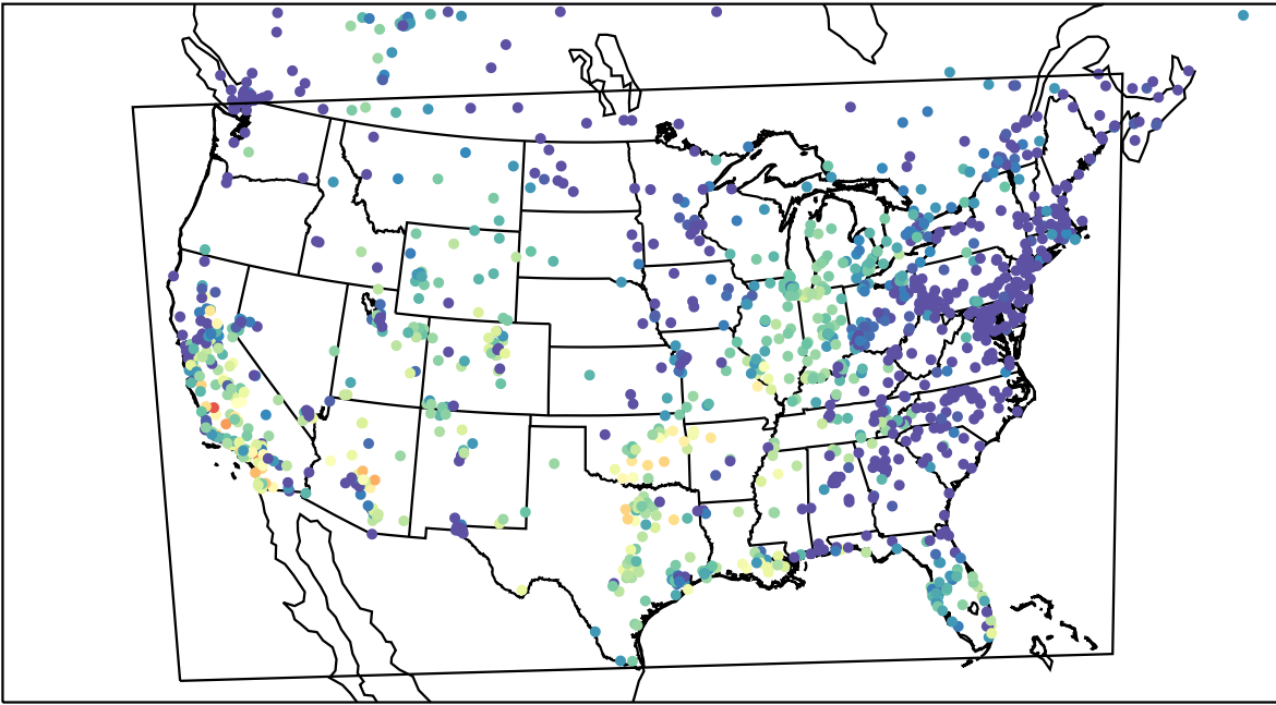
AirNOW (2023-10-19_02:00:00)
