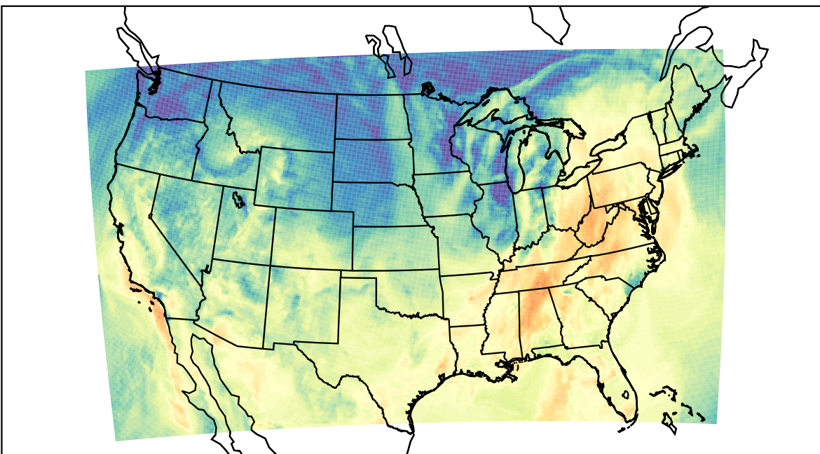
WRF (2023-10-19_18:00:00)
