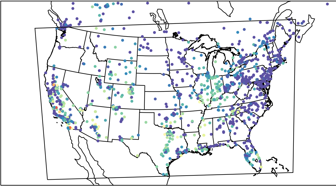
AirNOW (2023-10-19_05:00:00)
