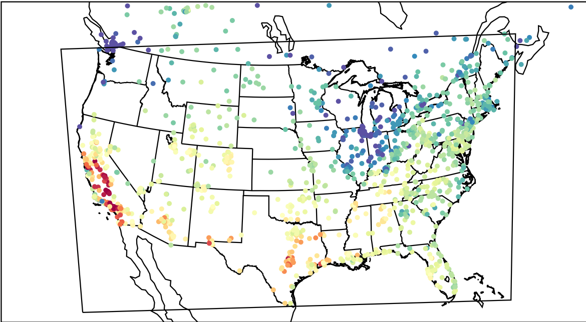
AirNOW (2023-10-19_21:00:00)
