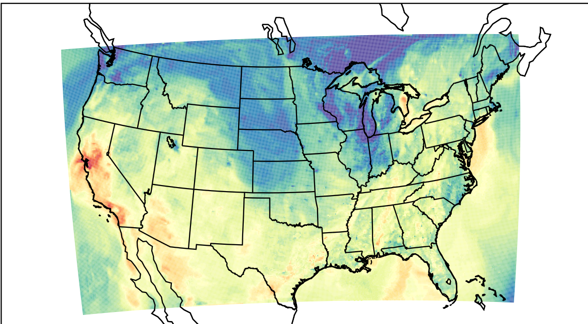
WRF (2023-10-19_23:00:00)
