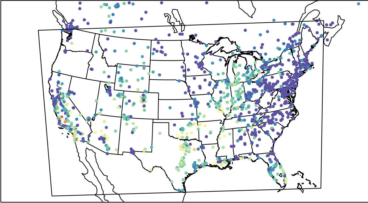
AirNOW (2023-10-19_03:00:00)
