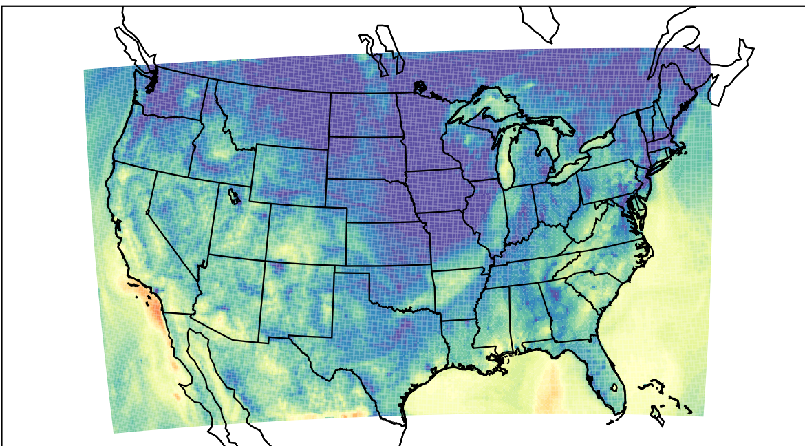
WRF (2023-10-19_11:00:00)
