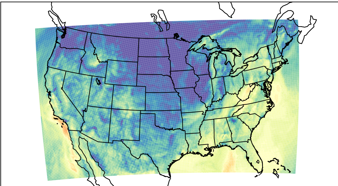
WRF (2023-10-19_15:00:00)
