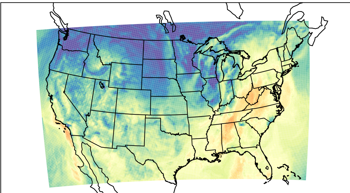
WRF (2023-10-19_17:00:00)
