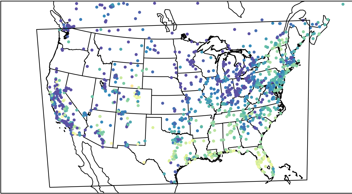
AirNOW (2023-10-20_15:00:00)
