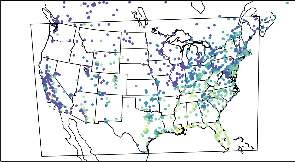
AirNOW (2023-10-19_15:00:00)
