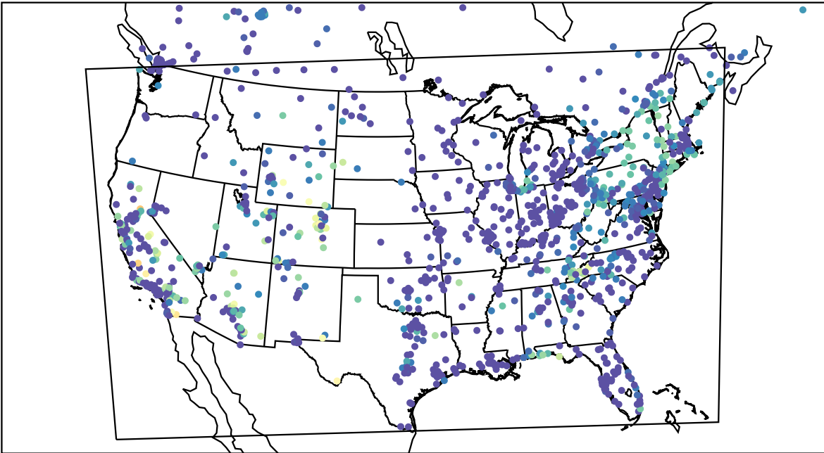
AirNOW (2023-10-20_12:00:00)
