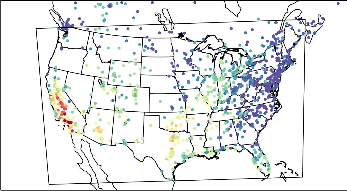
AirNOW (2023-10-19_00:00:00)
