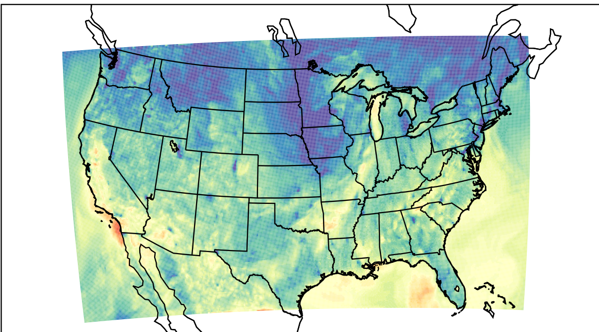
WRF (2023-10-19_03:00:00)
