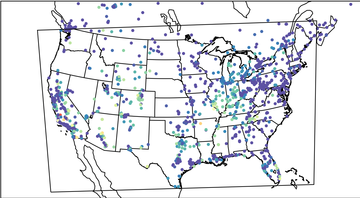
AirNOW (2023-10-19_08:00:00)
