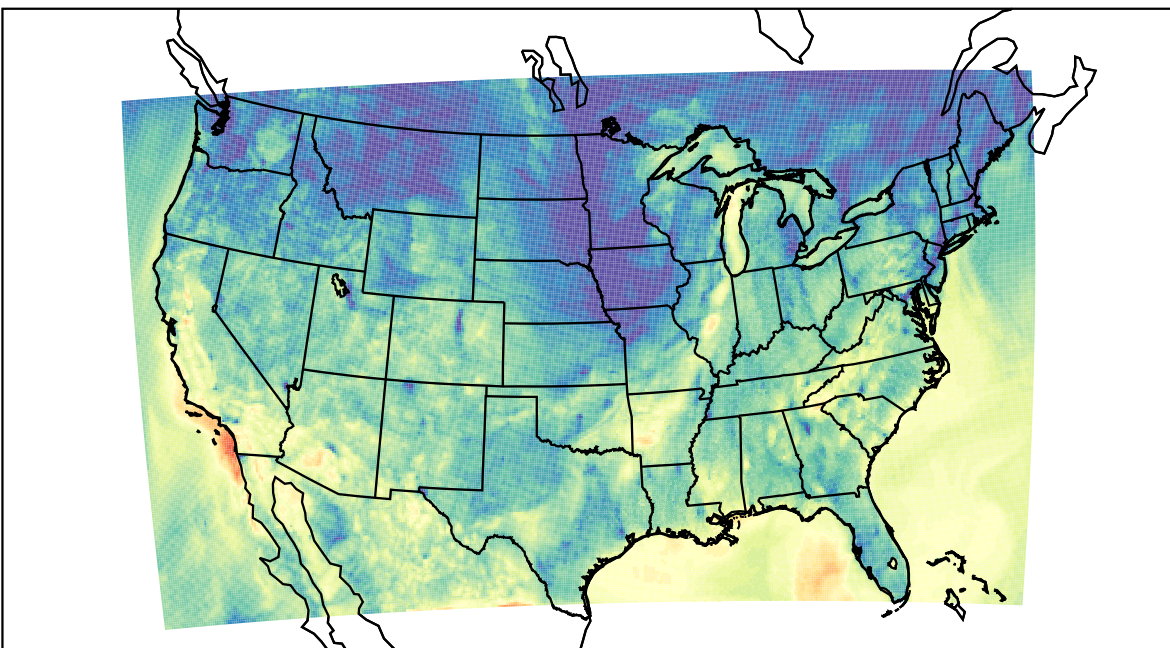
WRF (2023-10-19_04:00:00)
