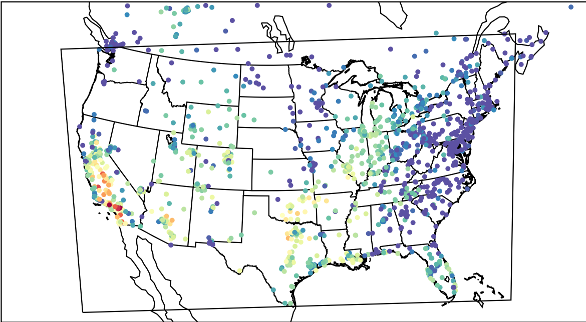
AirNOW (2023-10-19_01:00:00)
