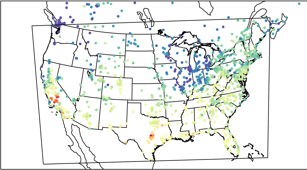
AirNOW (2023-10-19_18:00:00)
