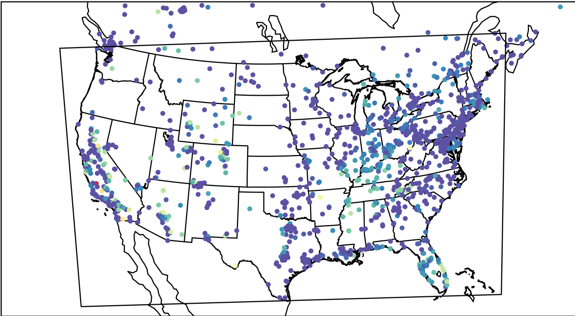
AirNOW (2023-10-19_13:00:00)
