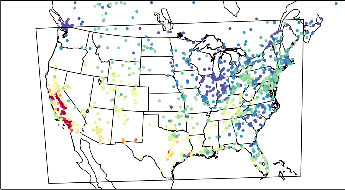
AirNOW (2023-10-19_23:00:00)
