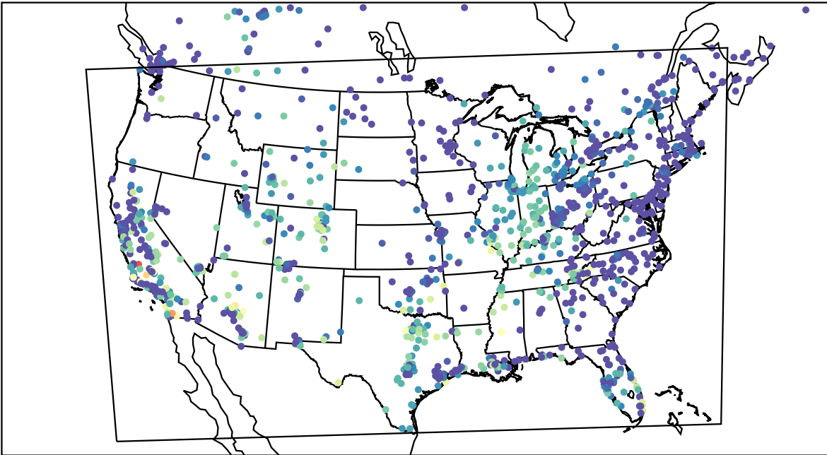
AirNOW (2023-10-19_06:00:00)
