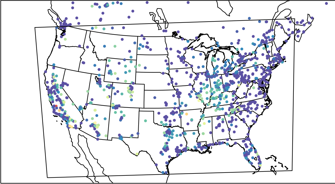
AirNOW (2023-10-19_09:00:00)
