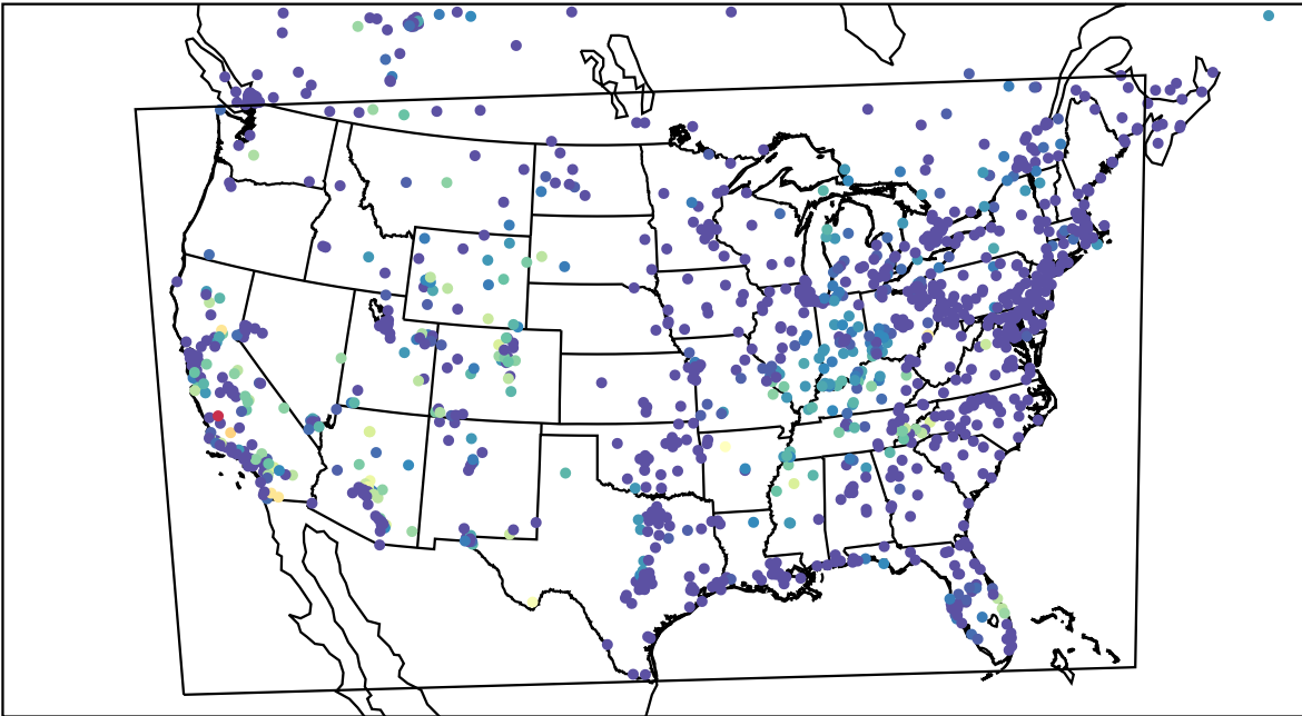
AirNOW (2023-10-19_12:00:00)
