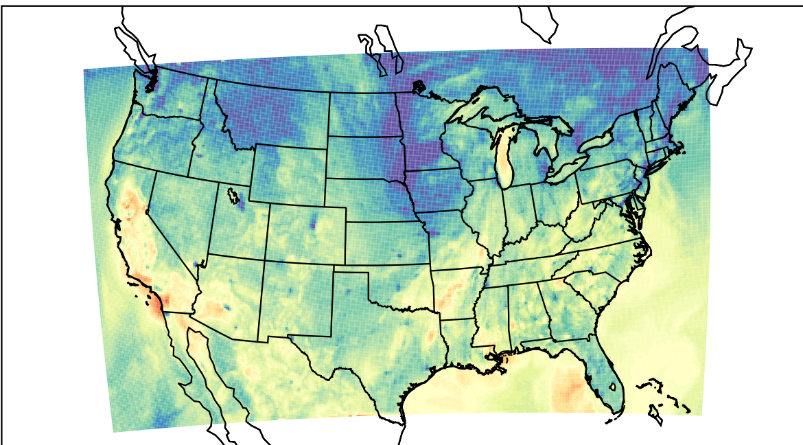
WRF (2023-10-19_01:00:00)
