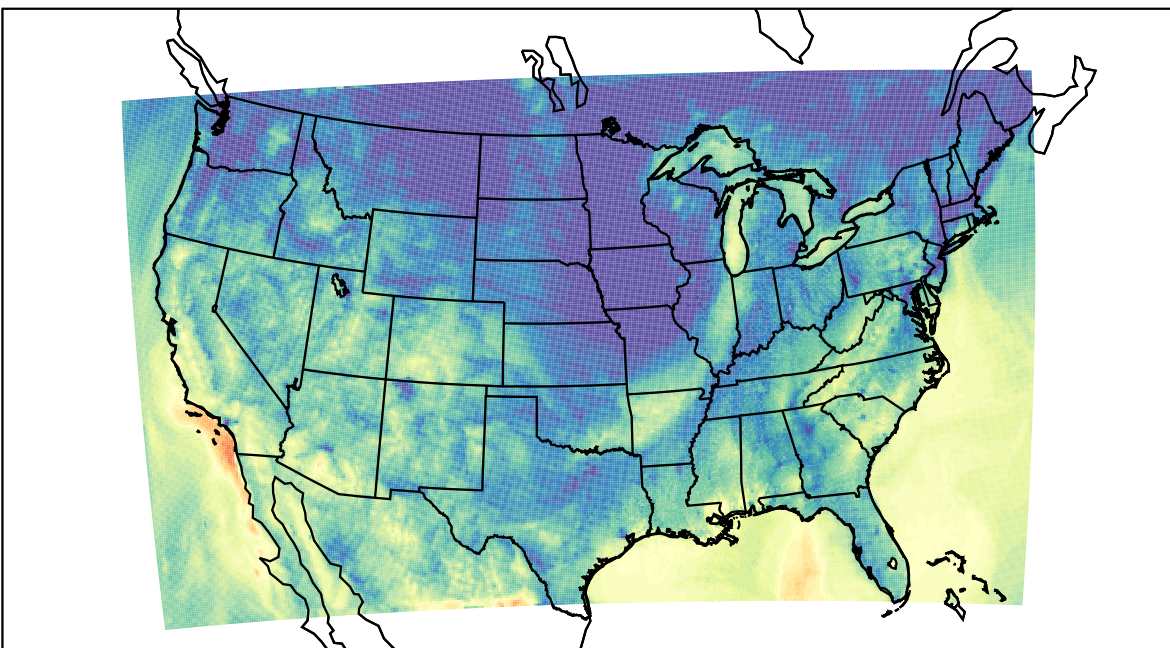
WRF (2023-10-19_10:00:00)
