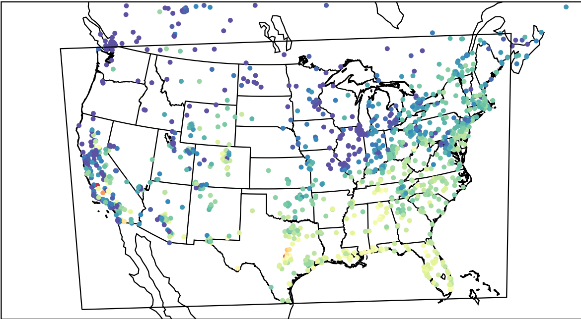
AirNOW (2023-10-19_16:00:00)
