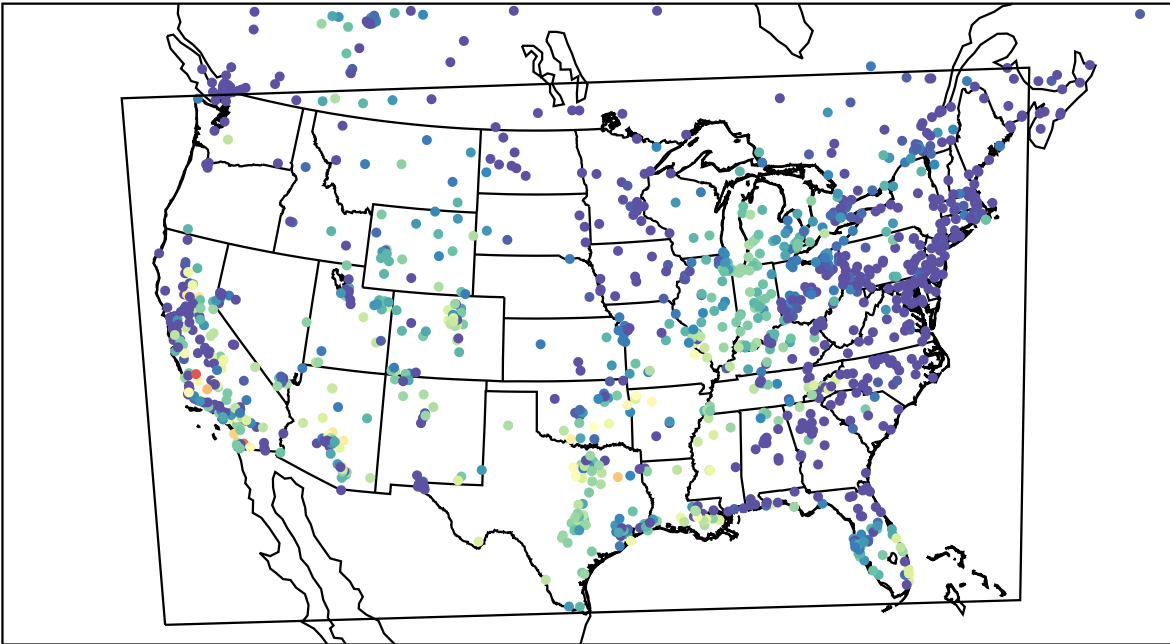
AirNOW (2023-10-19_04:00:00)
