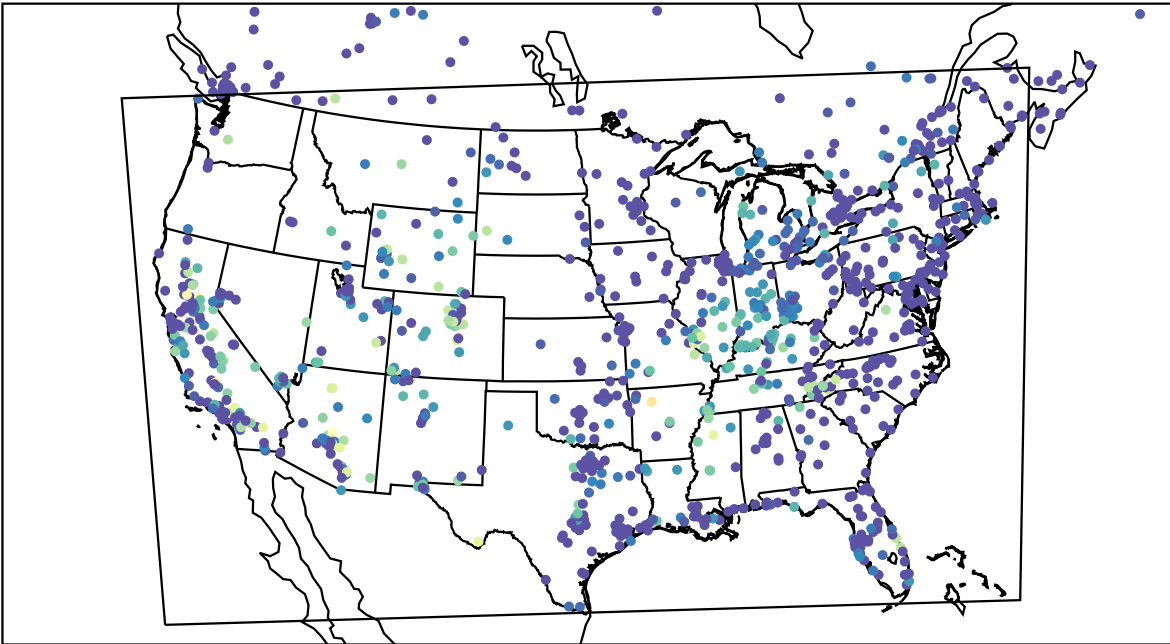
AirNOW (2023-10-19_10:00:00)
