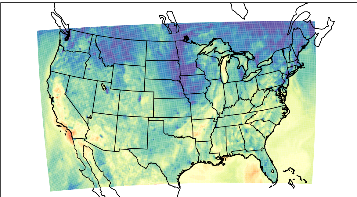
WRF (2023-10-19_02:00:00)
