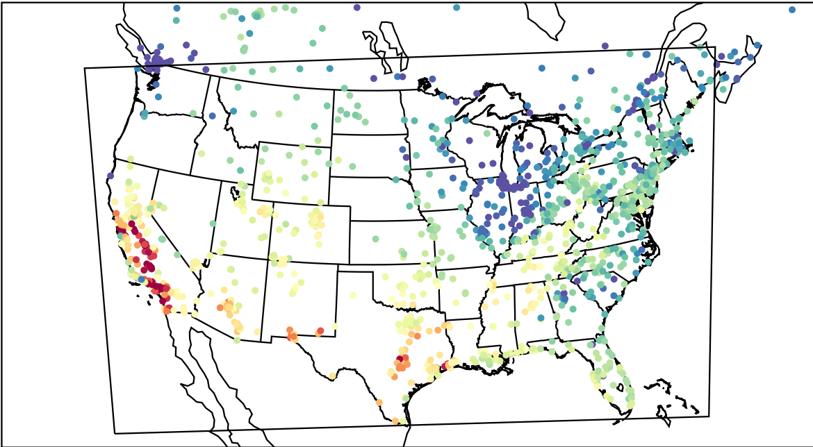
AirNOW (2023-10-19_22:00:00)
