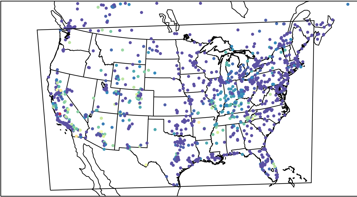
AirNOW (2023-10-19_11:00:00)
