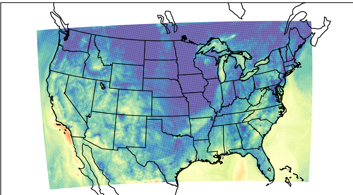
WRF (2023-10-19_12:00:00)
