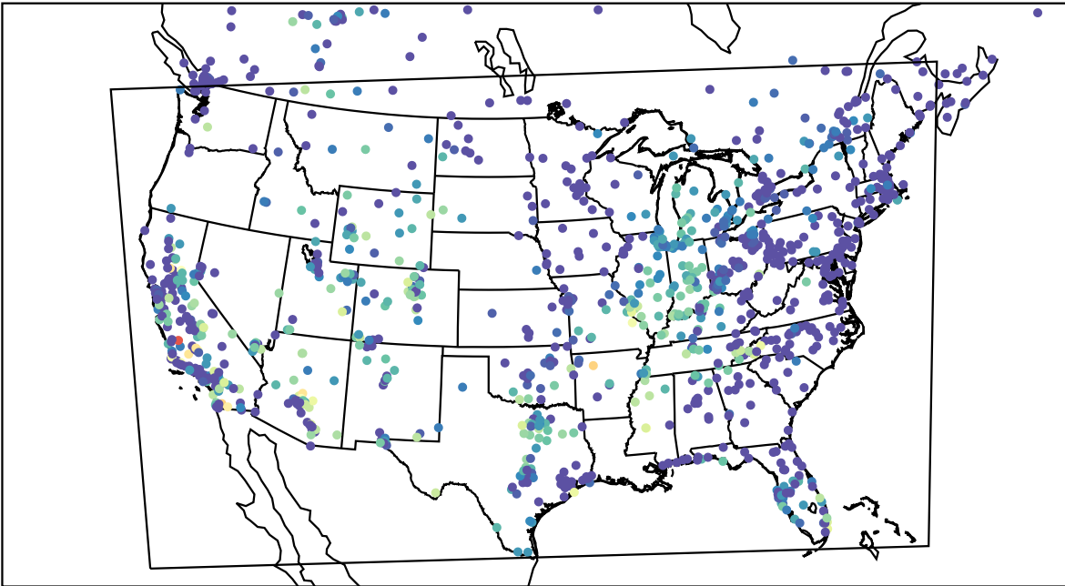
AirNOW (2023-10-19_07:00:00)
