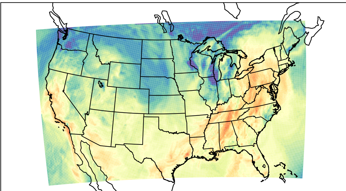
WRF (2023-10-19_20:00:00)
