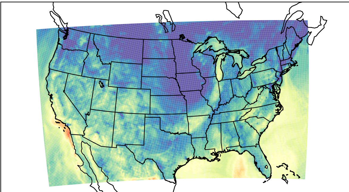
WRF (2023-10-19_09:00:00)
