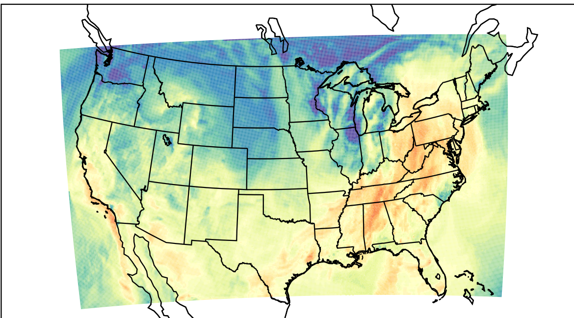
WRF (2023-10-19_19:00:00)
