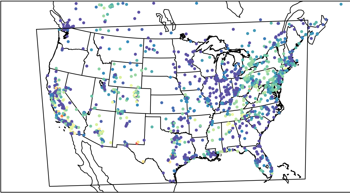
AirNOW (2023-10-20_04:00:00)
