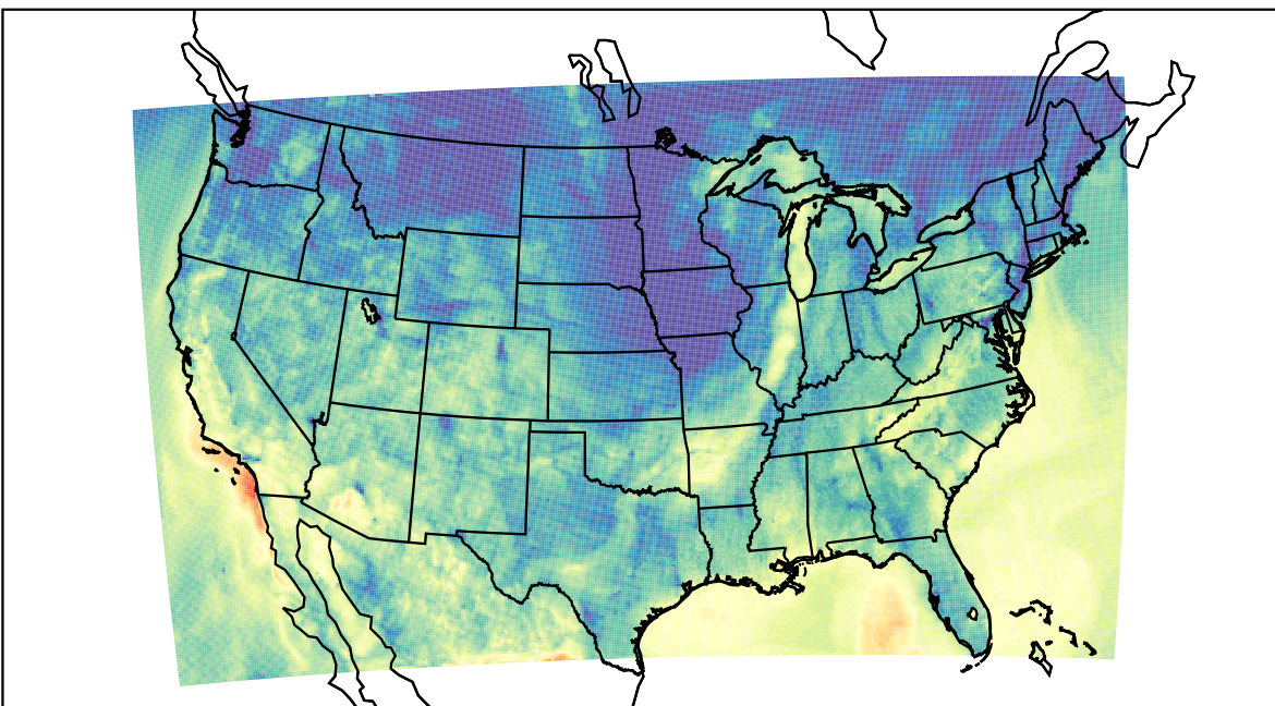
WRF (2023-10-19_06:00:00)
