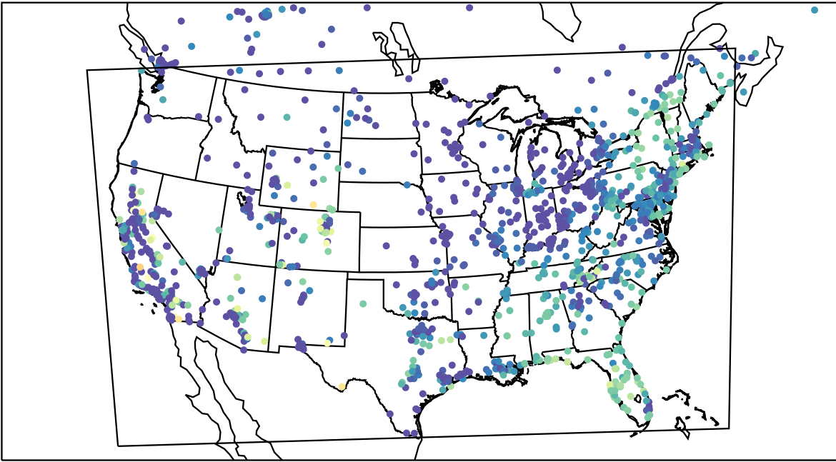
AirNOW (2023-10-20_14:00:00)
