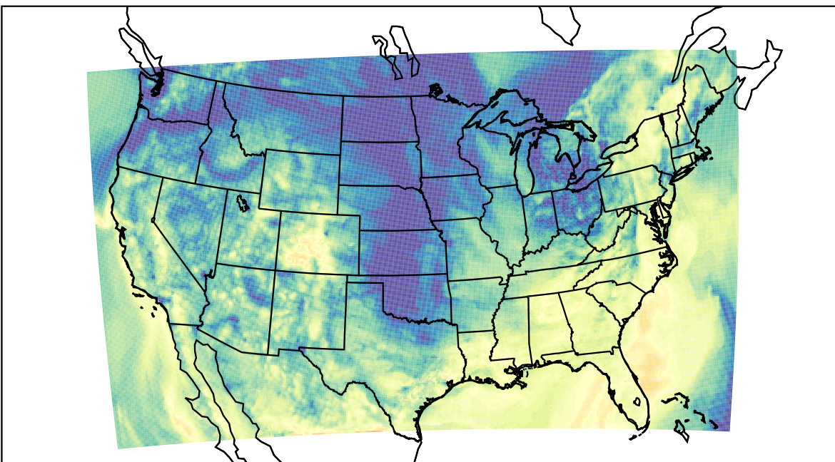
WRF (2023-10-20_16:00:00)
