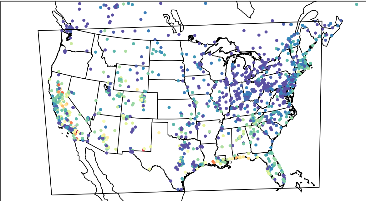
AirNOW (2023-10-21_03:00:00)
