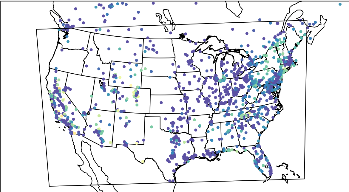
AirNOW (2023-10-20_13:00:00)
