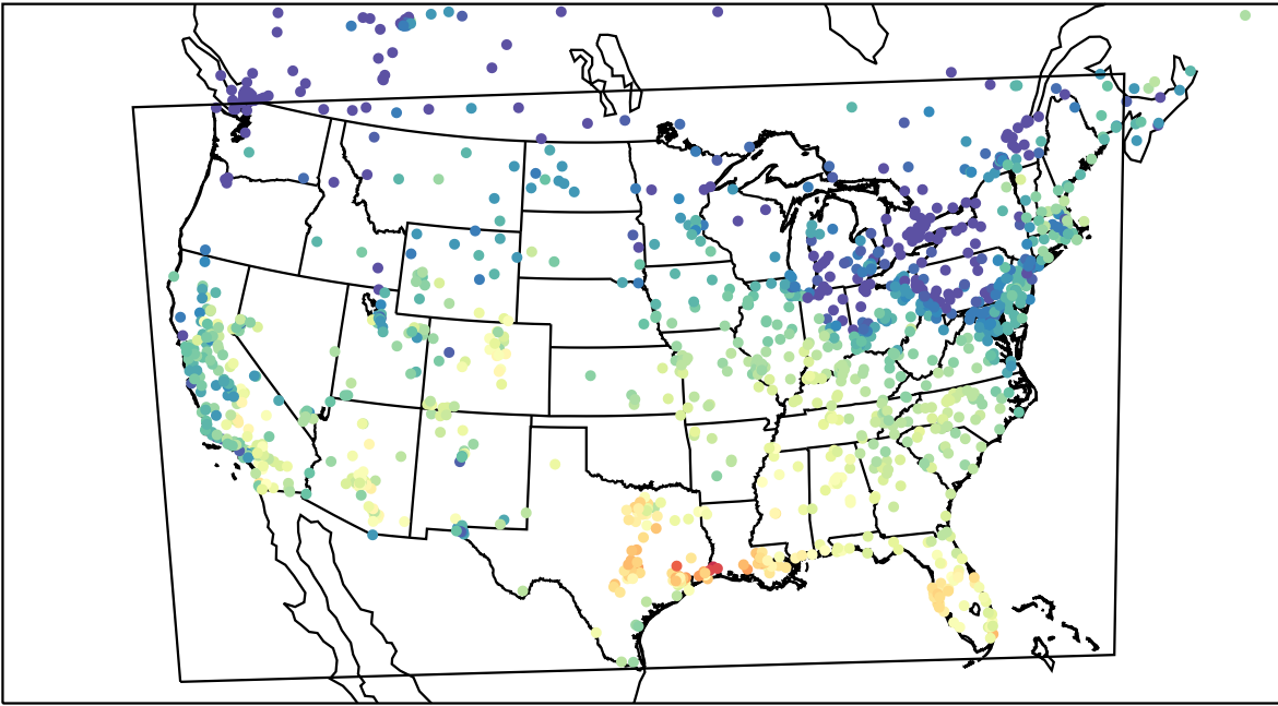
AirNOW (2023-10-21_17:00:00)
