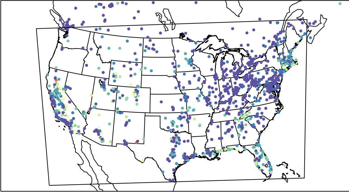
AirNOW (2023-10-21_08:00:00)
