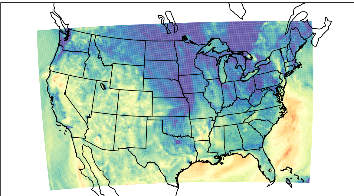
WRF (2023-10-21_05:00:00)
