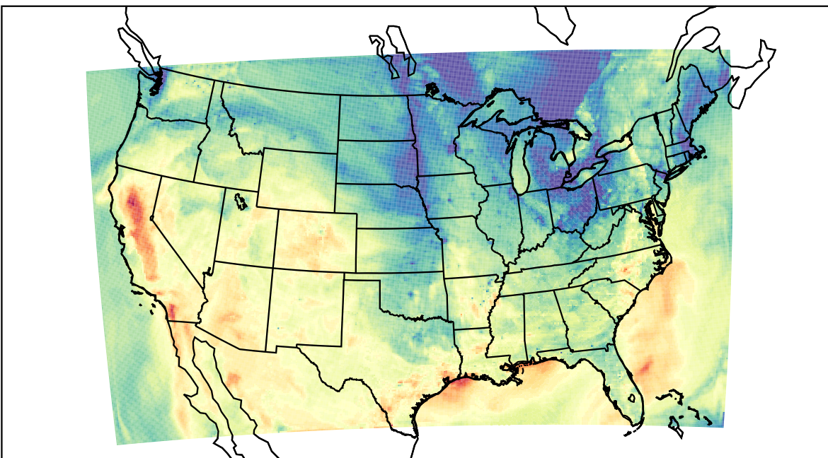
WRF (2023-10-20_23:00:00)
