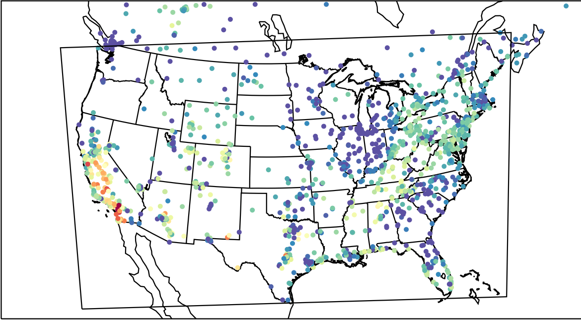
AirNOW (2023-10-20_01:00:00)
