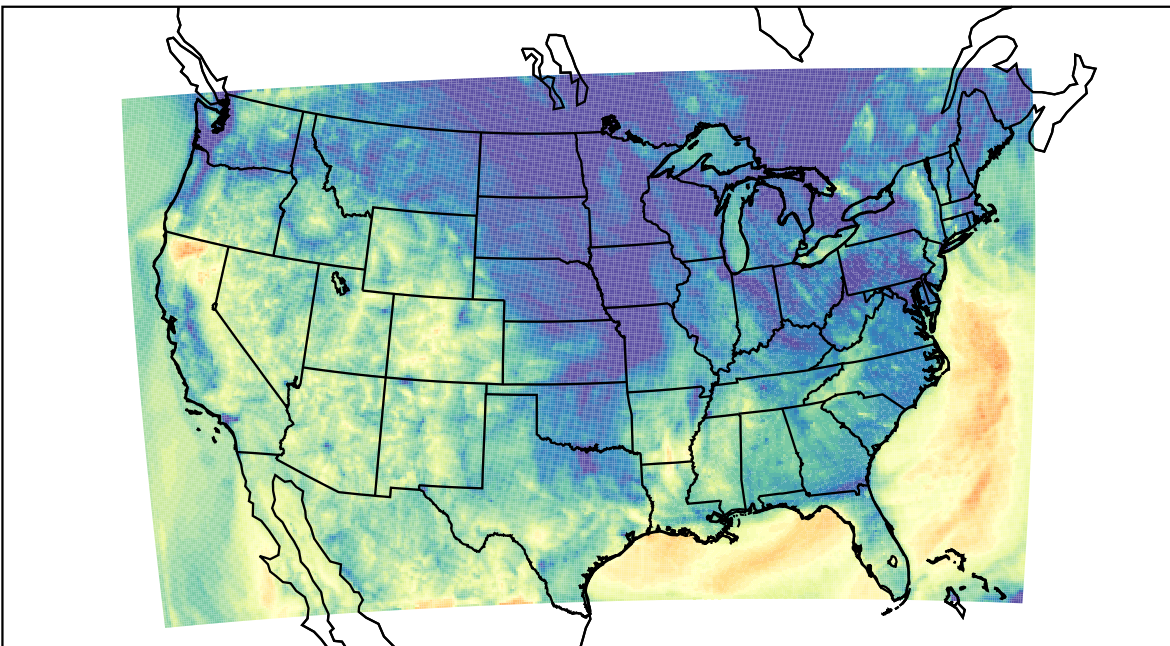
WRF (2023-10-21_08:00:00)
