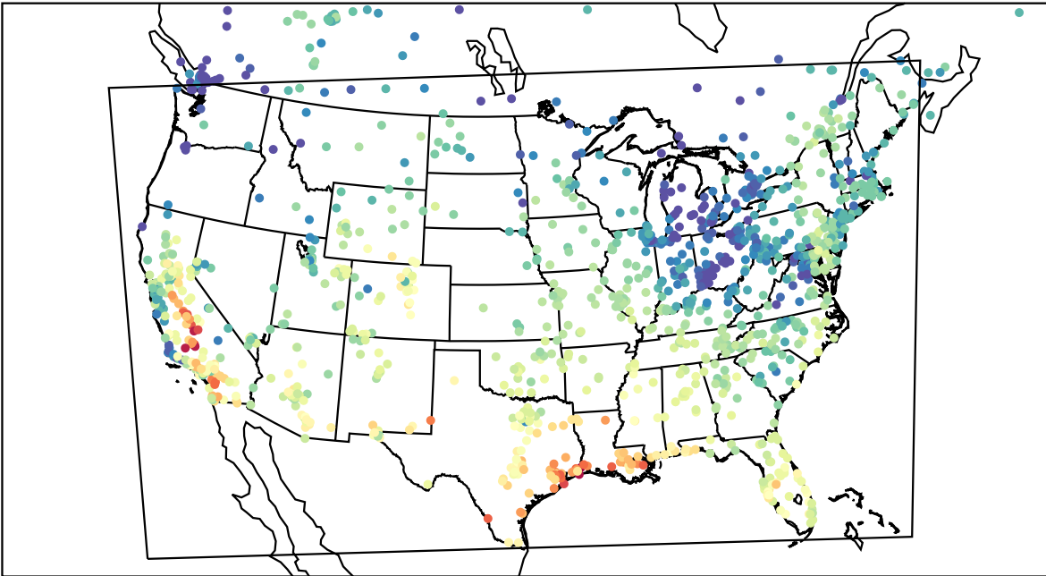
AirNOW (2023-10-20_18:00:00)
