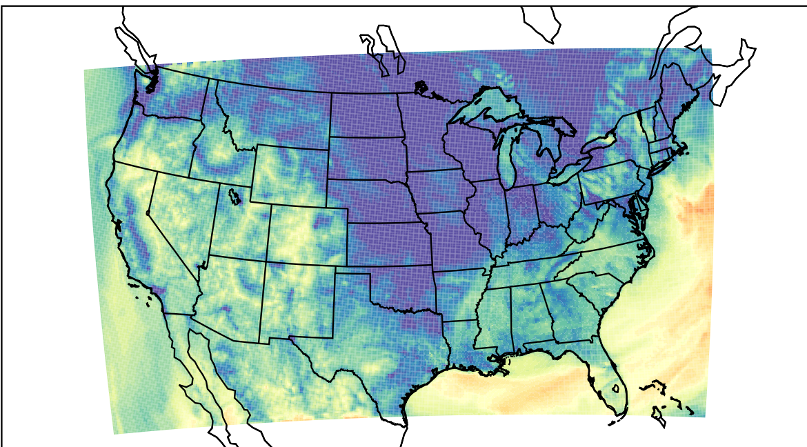
WRF (2023-10-21_14:00:00)
