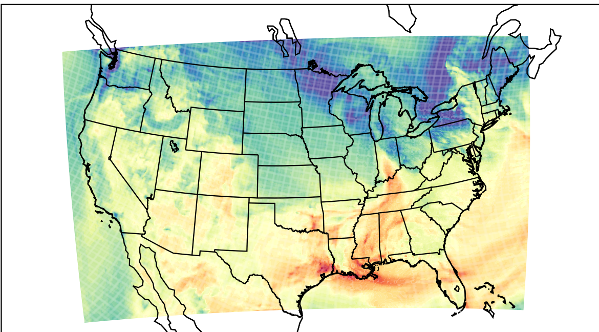
WRF (2023-10-21_19:00:00)
