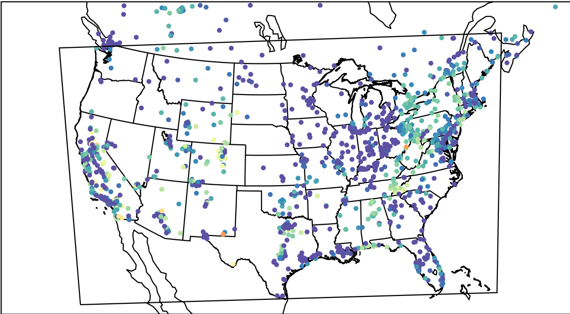
AirNOW (2023-10-20_08:00:00)
