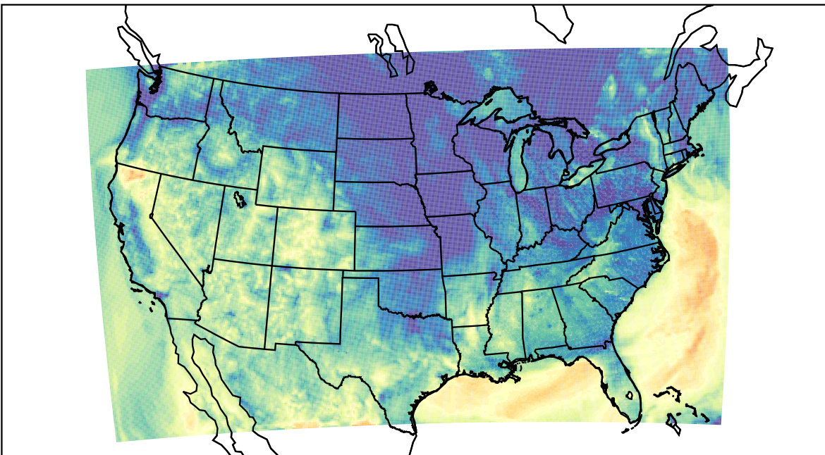
WRF (2023-10-21_09:00:00)
