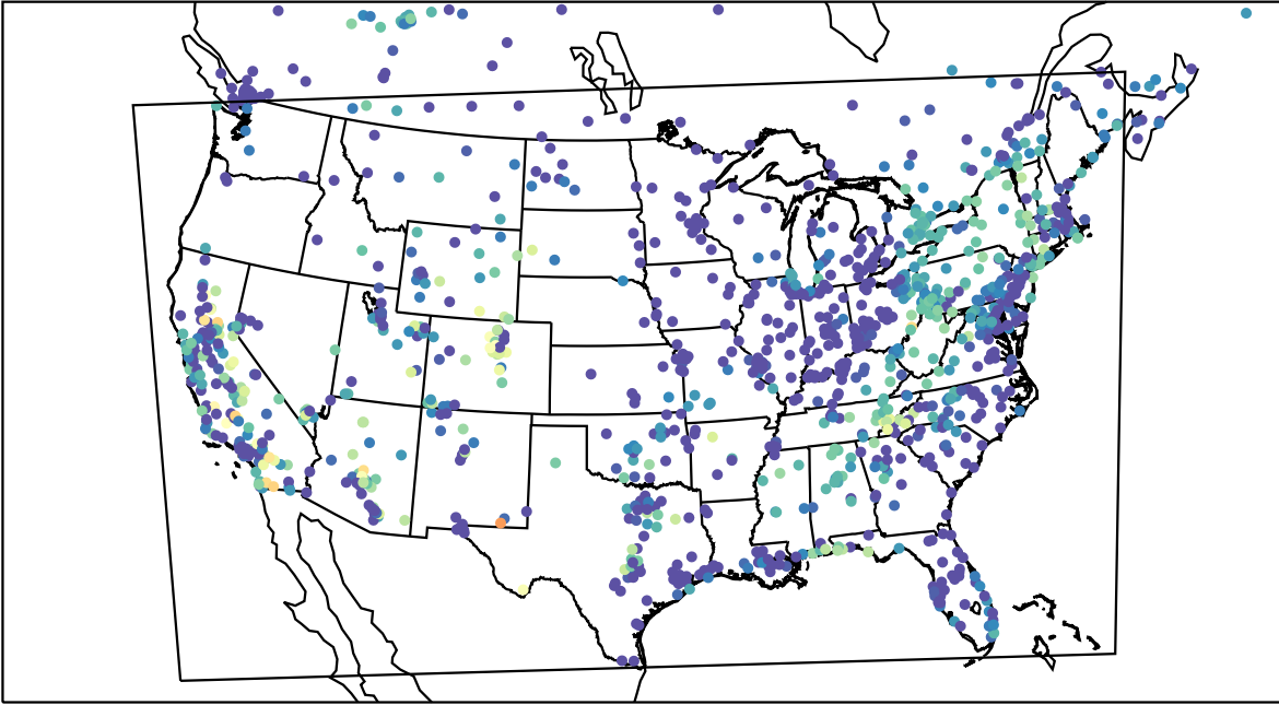
AirNOW (2023-10-20_09:00:00)
