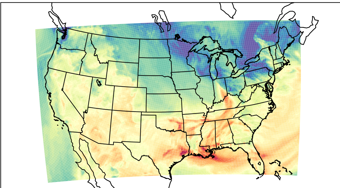
WRF (2023-10-21_21:00:00)
