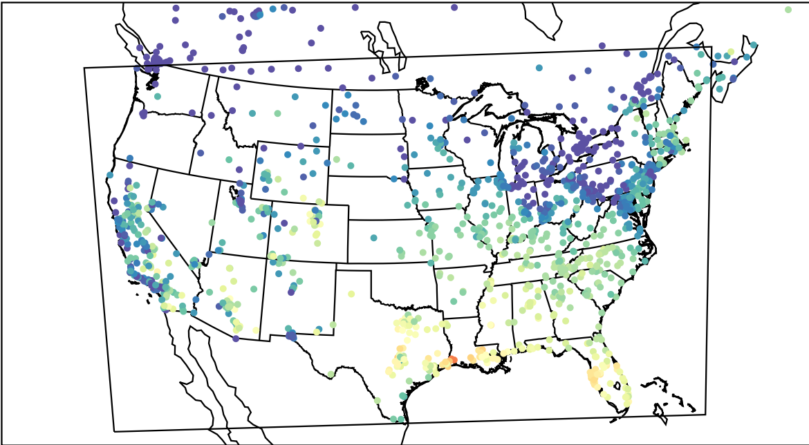
AirNOW (2023-10-21_16:00:00)
