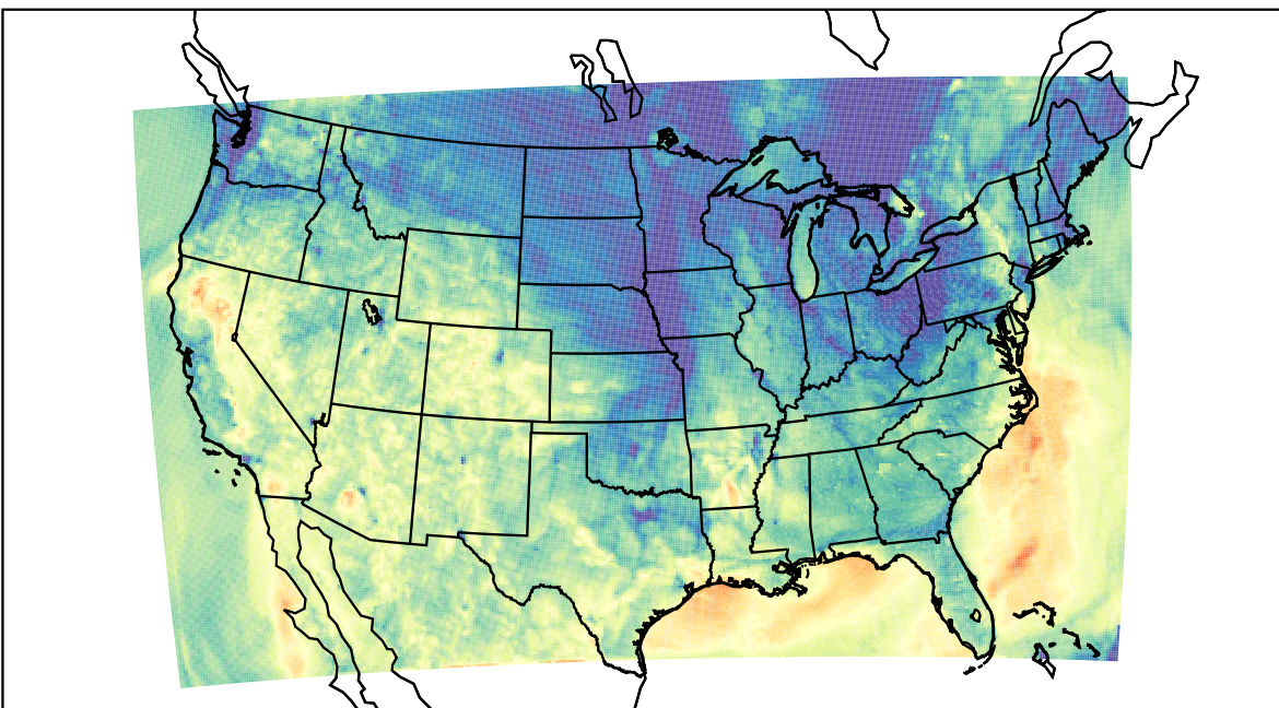
WRF (2023-10-21_03:00:00)
