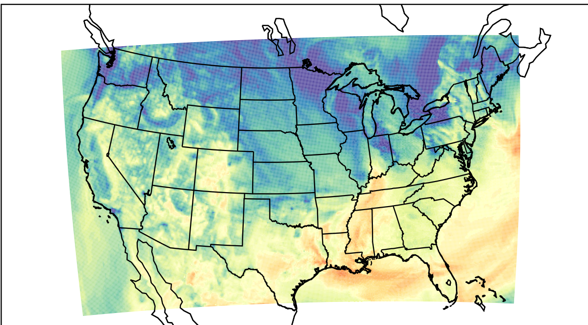
WRF (2023-10-21_17:00:00)
