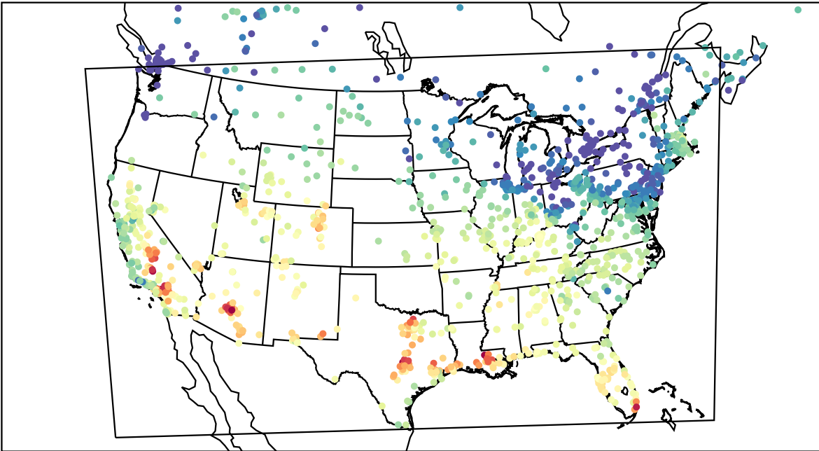
AirNOW (2023-10-21_21:00:00)
