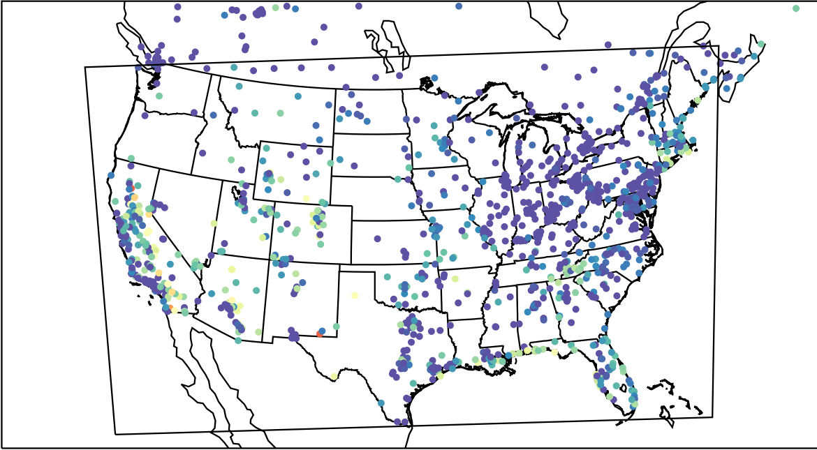
AirNOW (2023-10-21_07:00:00)
