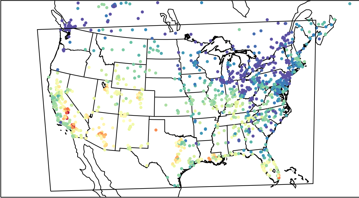
AirNOW (2023-10-21_23:00:00)
