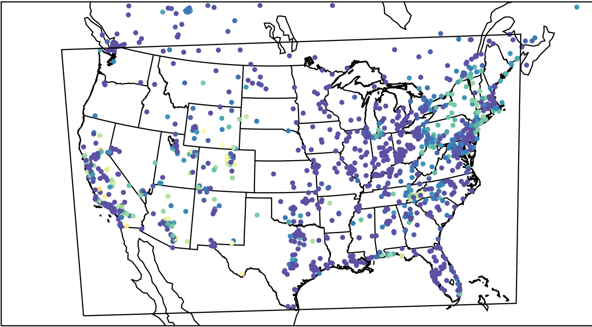
AirNOW (2023-10-20_12:00:00)
