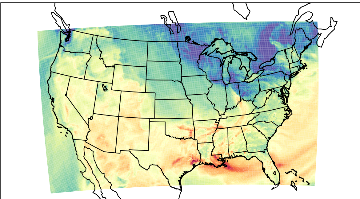
WRF (2023-10-21_22:00:00)
