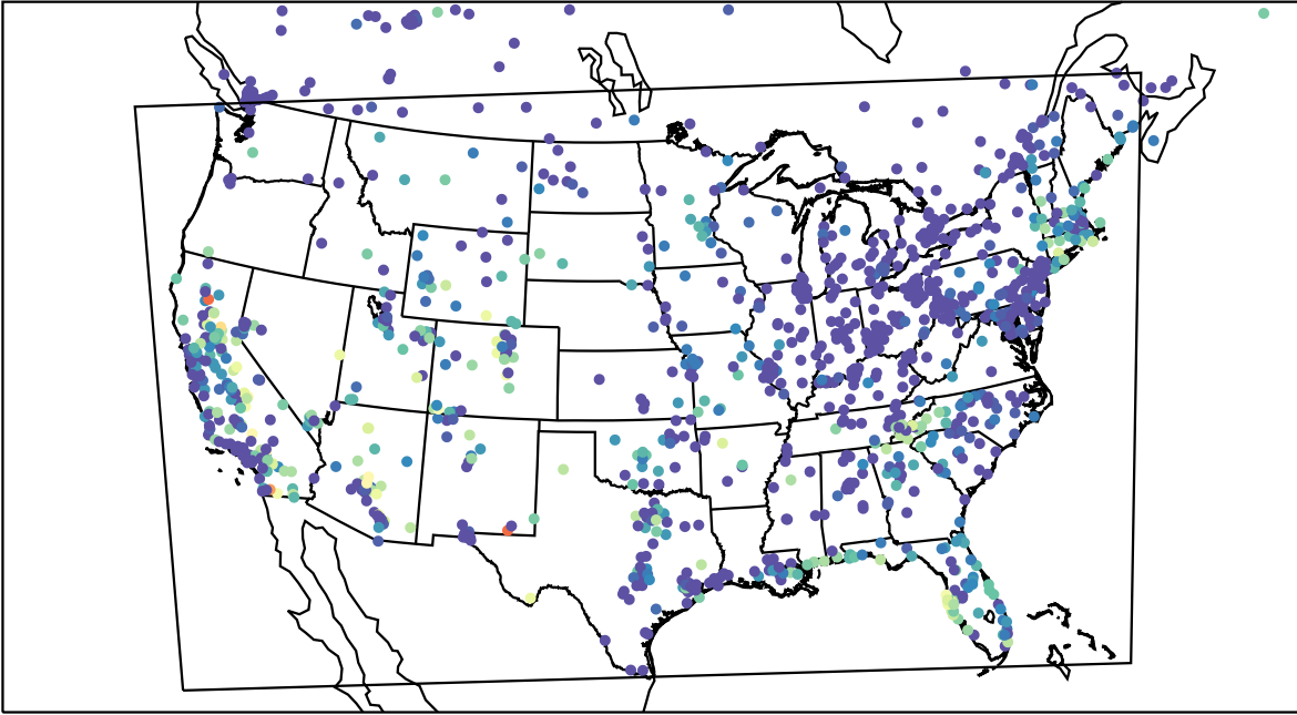
AirNOW (2023-10-21_09:00:00)
