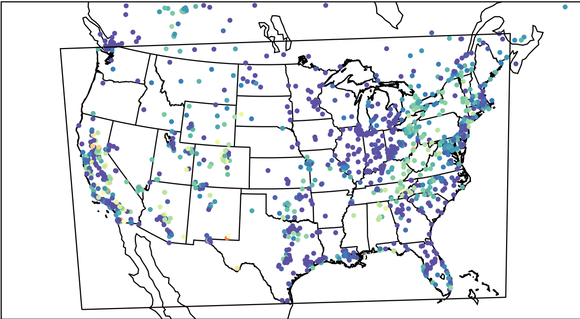
AirNOW (2023-10-20_06:00:00)
