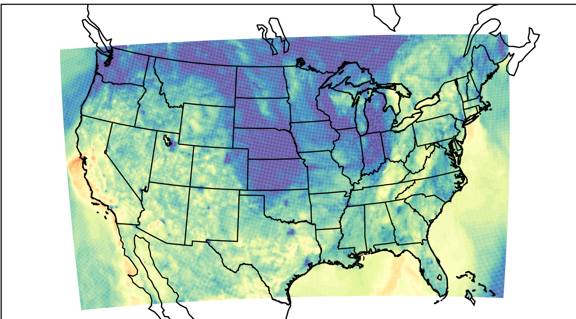
WRF (2023-10-20_04:00:00)
