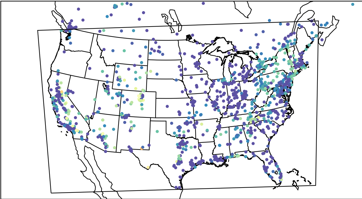
AirNOW (2023-10-20_10:00:00)
