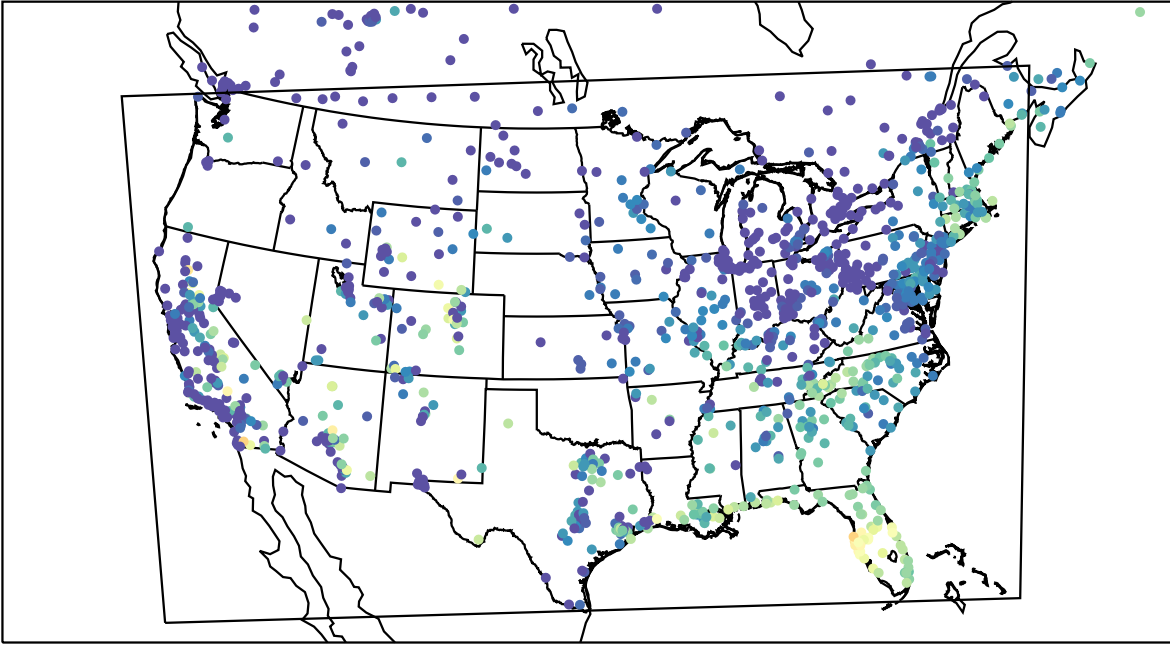
AirNOW (2023-10-21_14:00:00)
