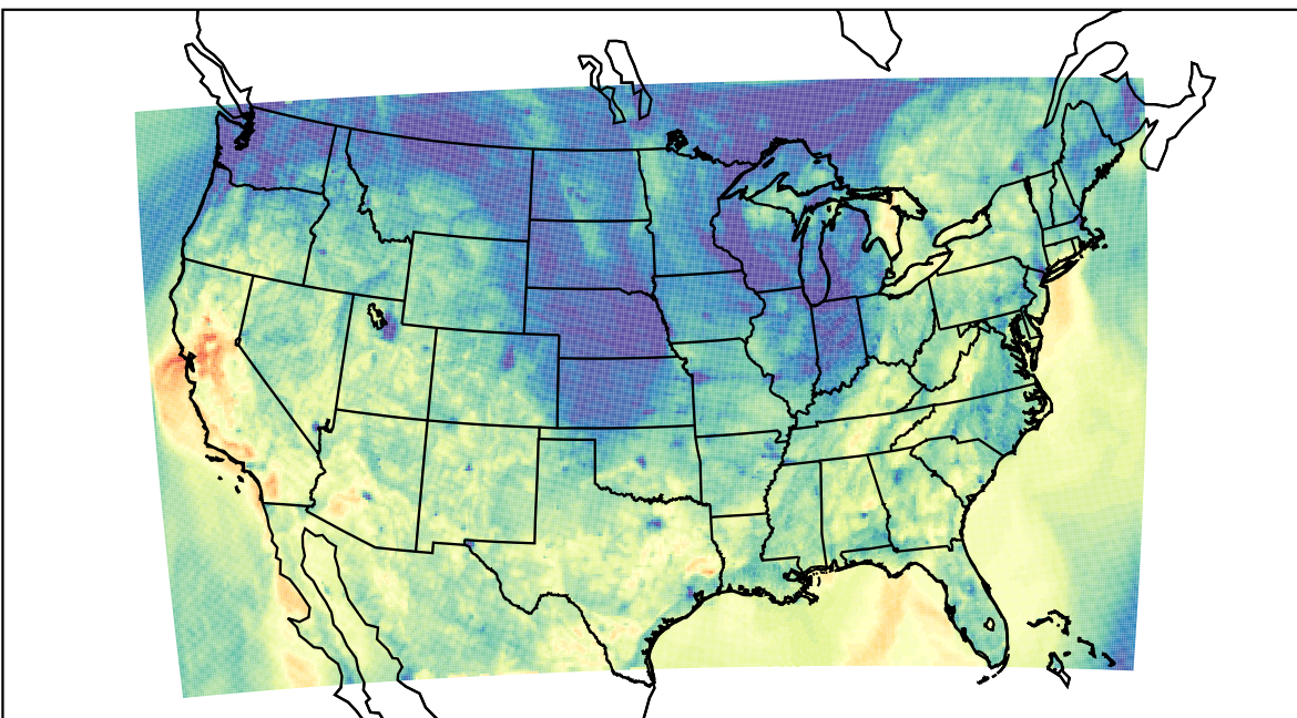
WRF (2023-10-20_02:00:00)
