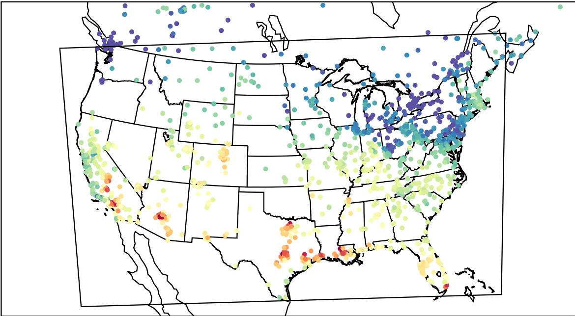
AirNOW (2023-10-21_20:00:00)
