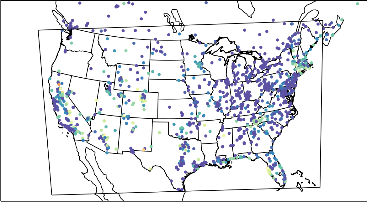
AirNOW (2023-10-21_10:00:00)
