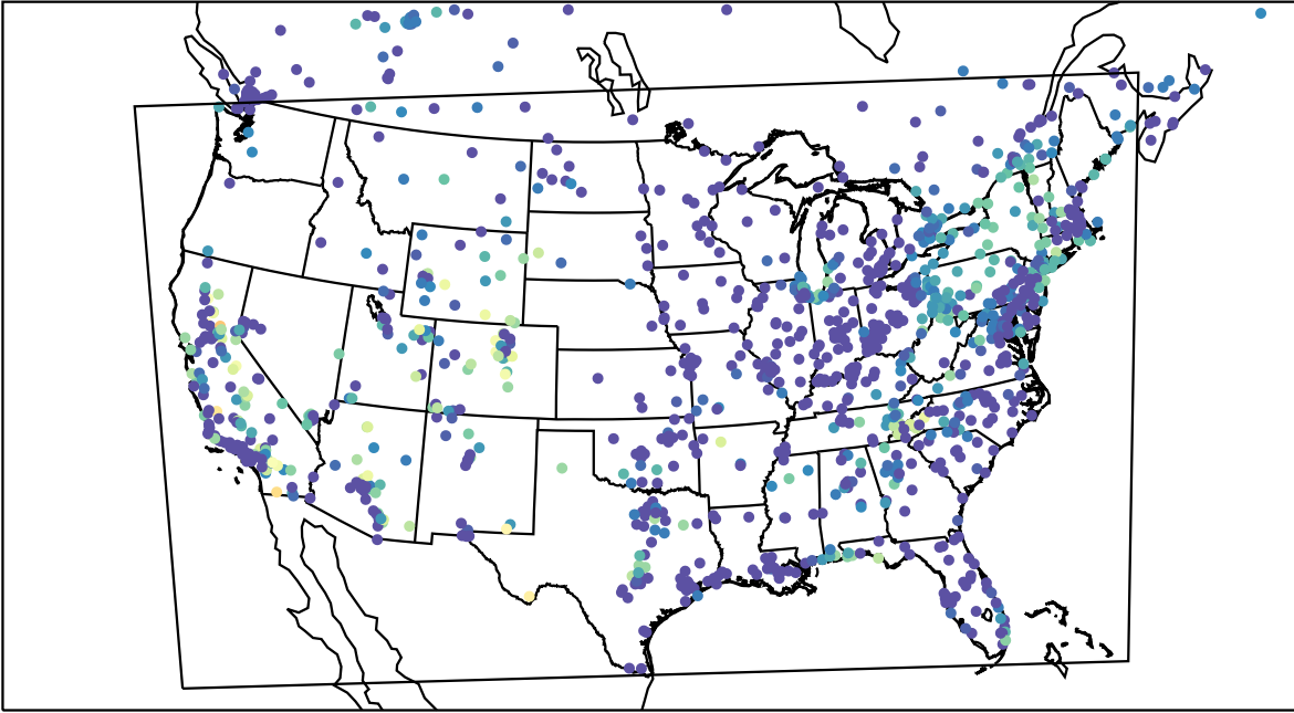
AirNOW (2023-10-20_11:00:00)
