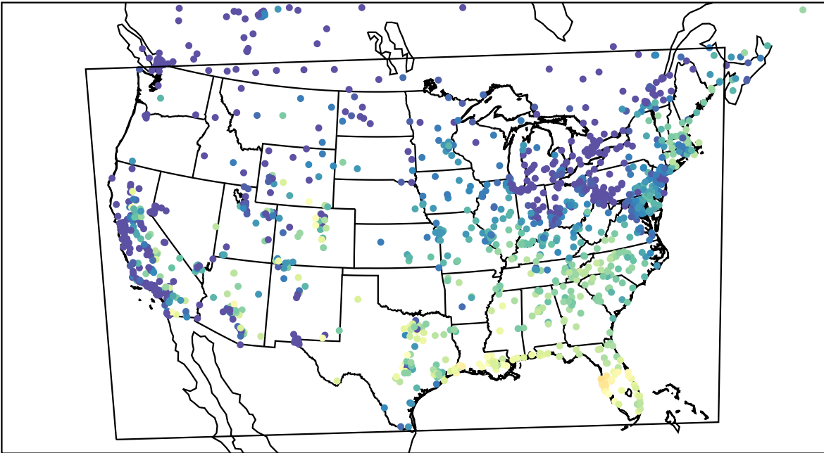
AirNOW (2023-10-21_15:00:00)
