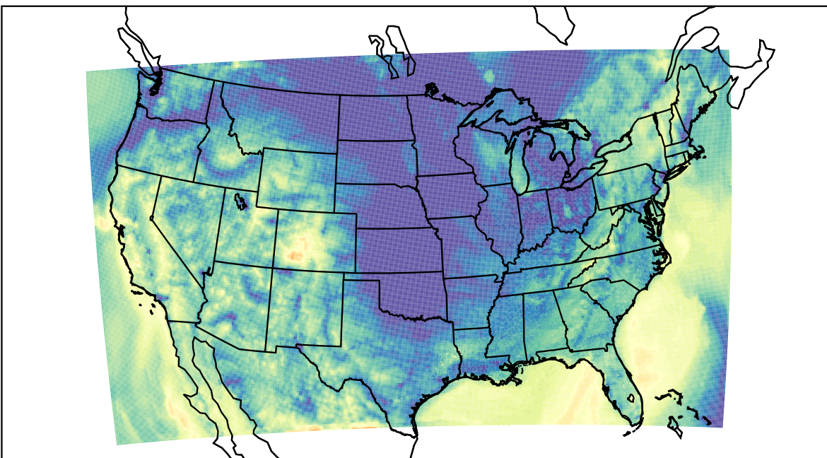
WRF (2023-10-20_14:00:00)
