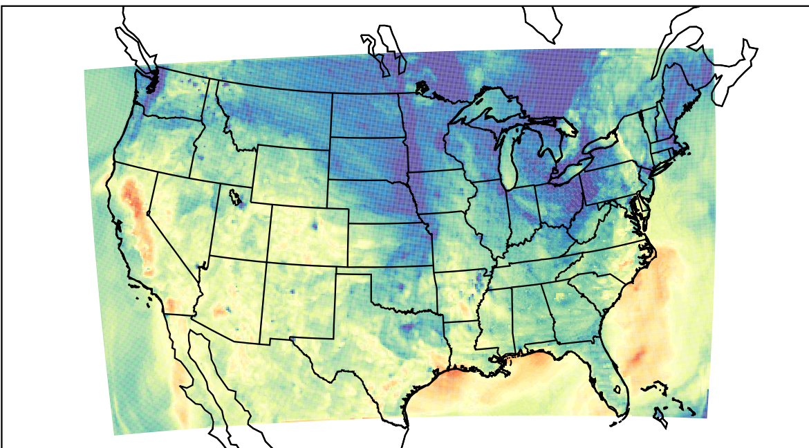
WRF (2023-10-21_01:00:00)
