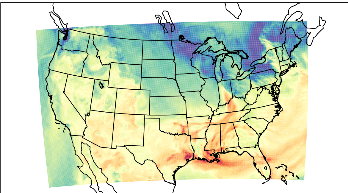
WRF (2023-10-21_20:00:00)
