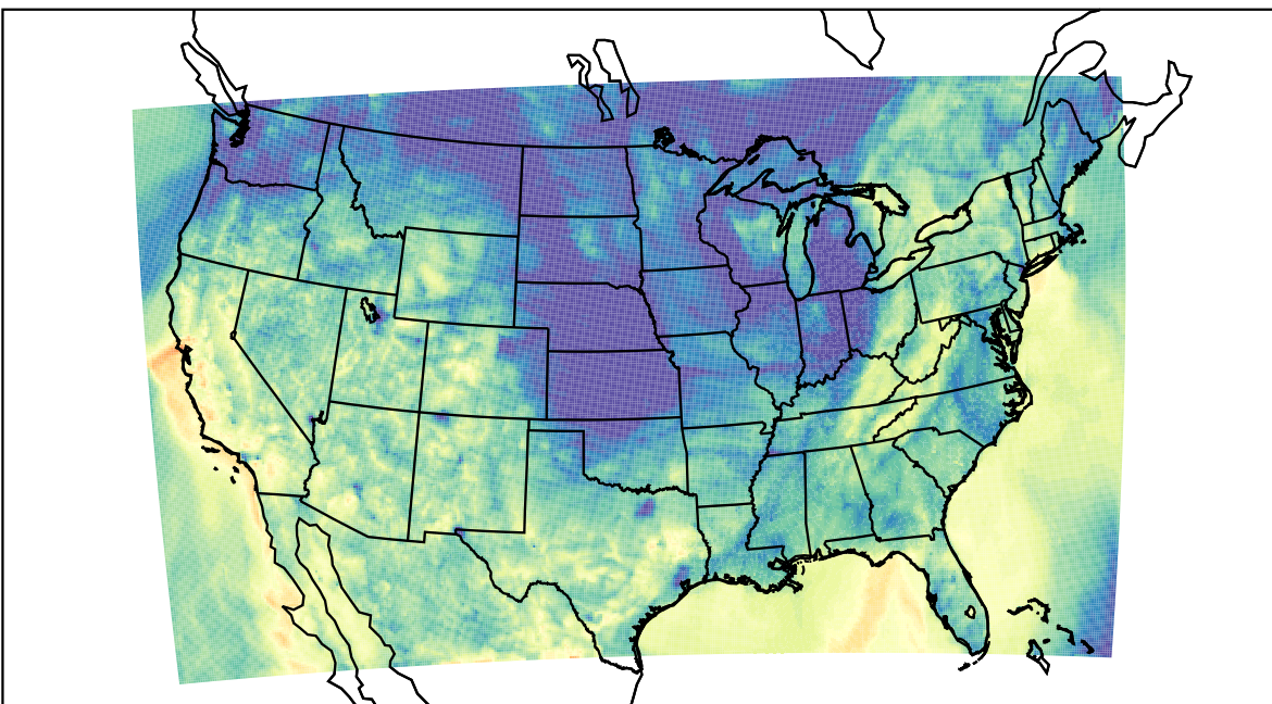
WRF (2023-10-20_06:00:00)
