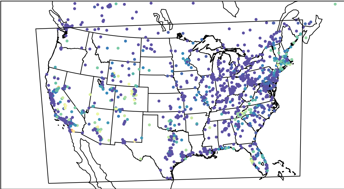
AirNOW (2023-10-21_12:00:00)
