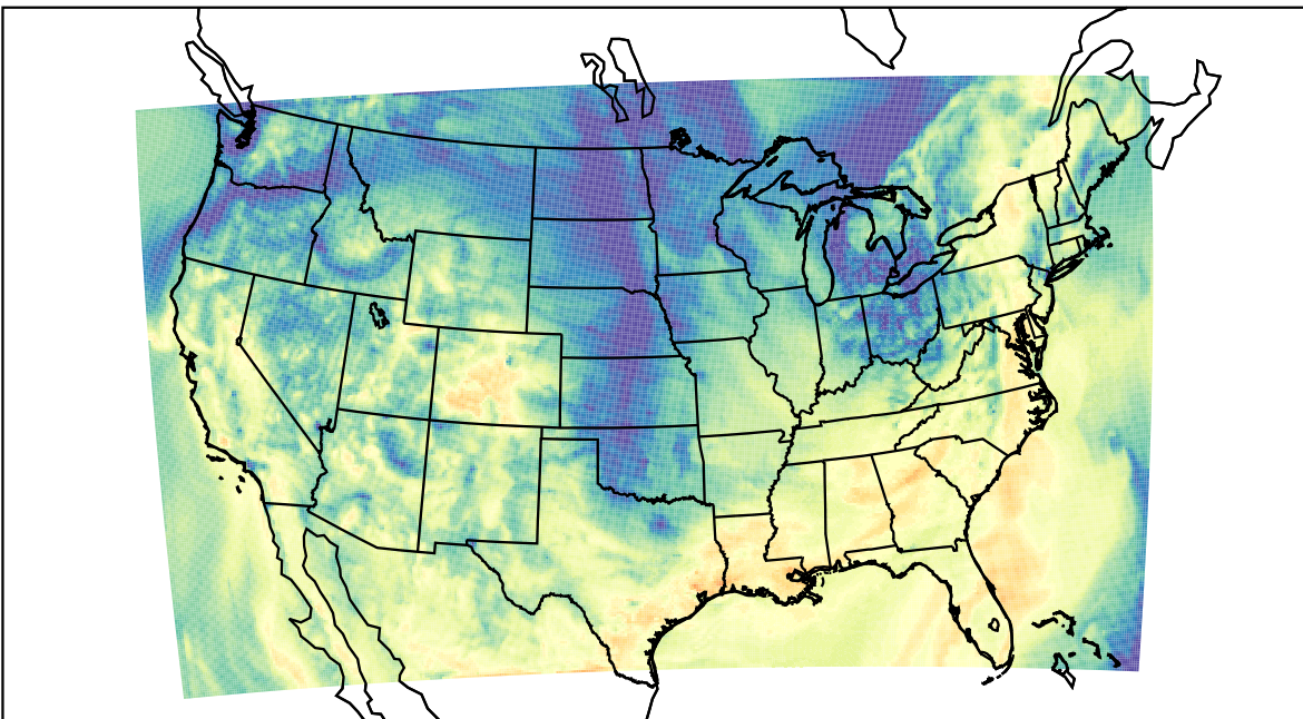
WRF (2023-10-20_17:00:00)
