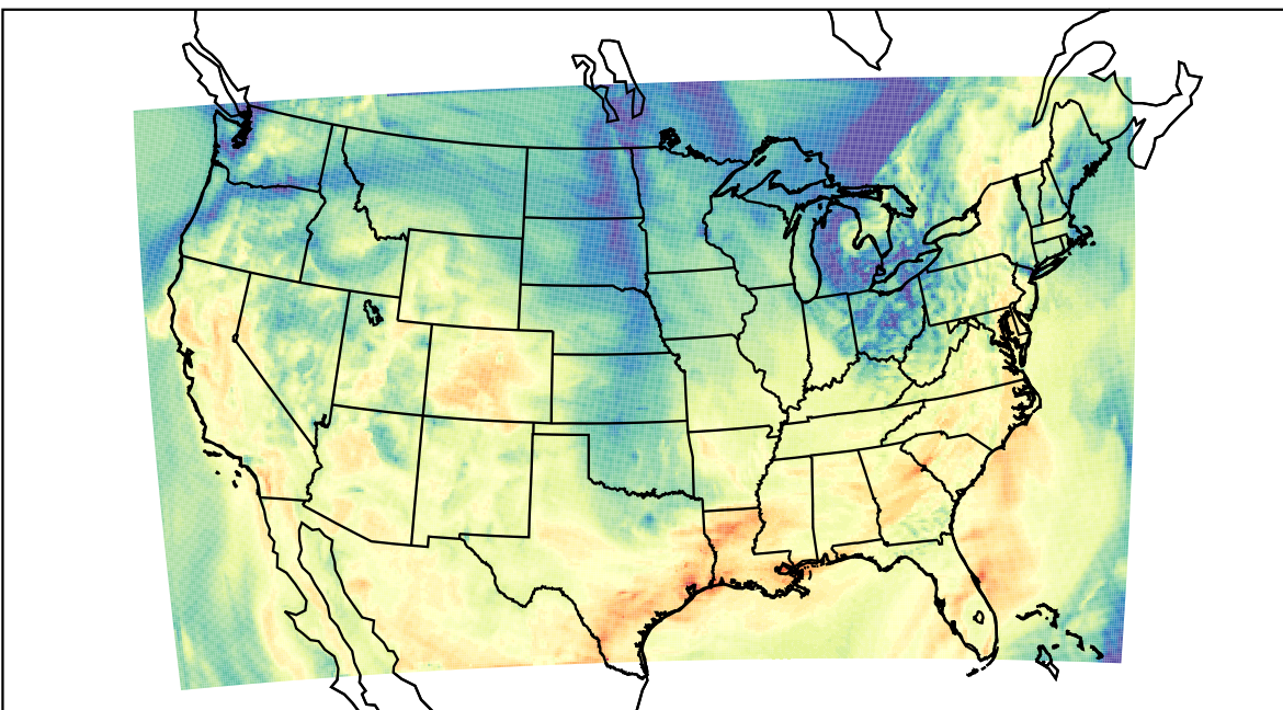
WRF (2023-10-20_19:00:00)
