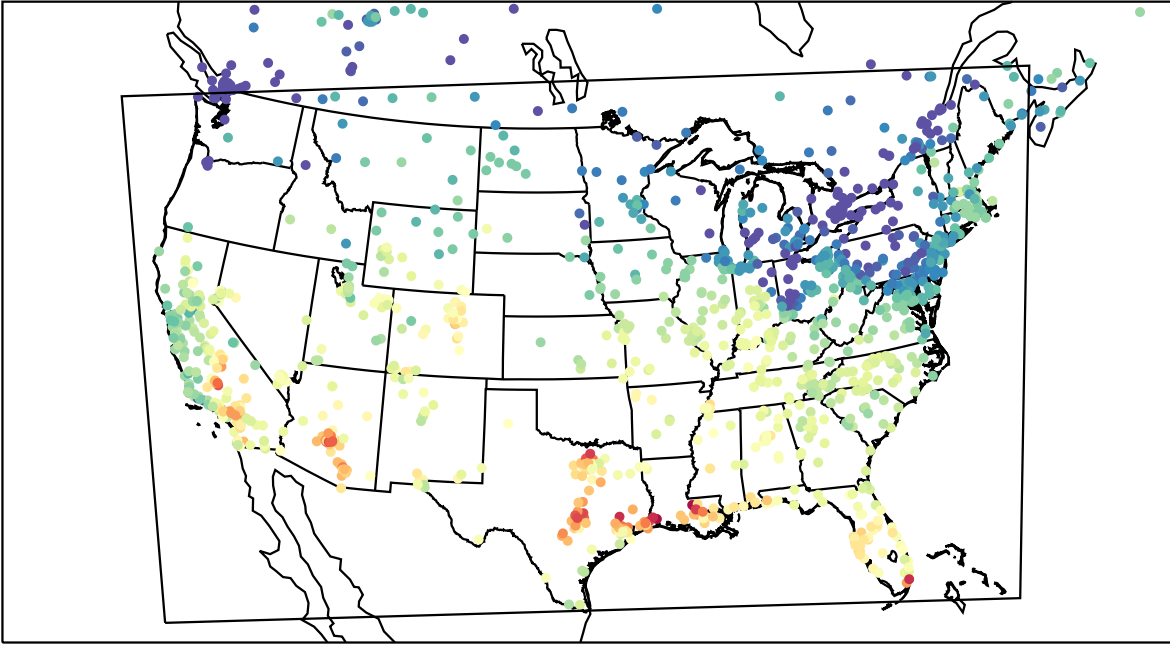
AirNOW (2023-10-21_19:00:00)
