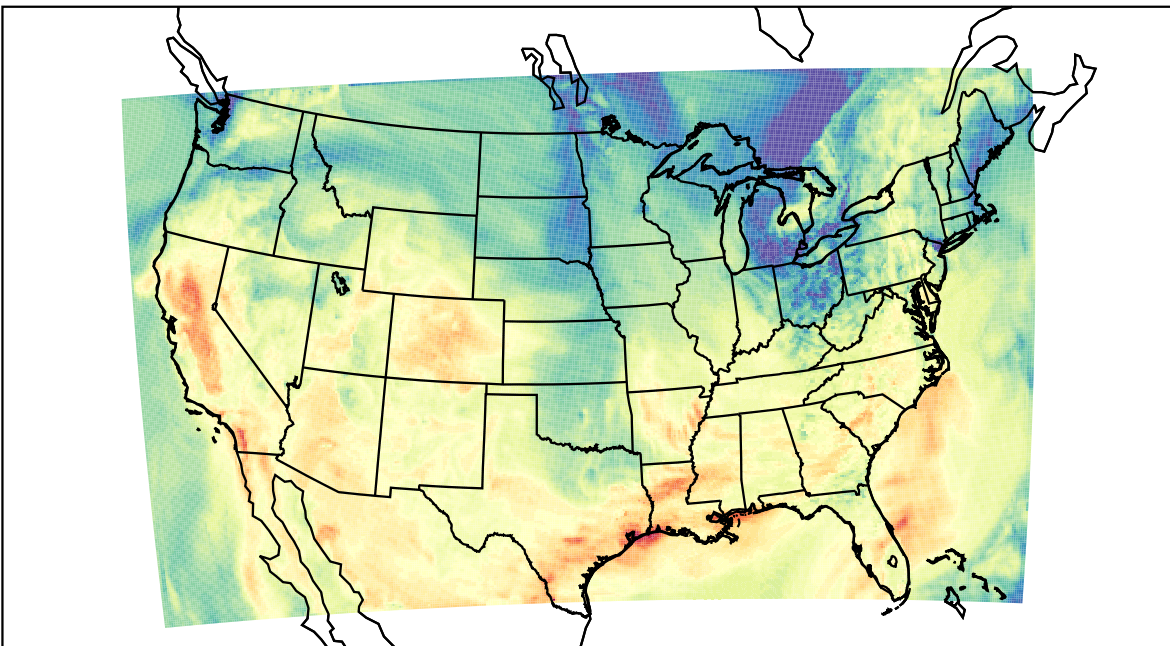
WRF (2023-10-20_21:00:00)
