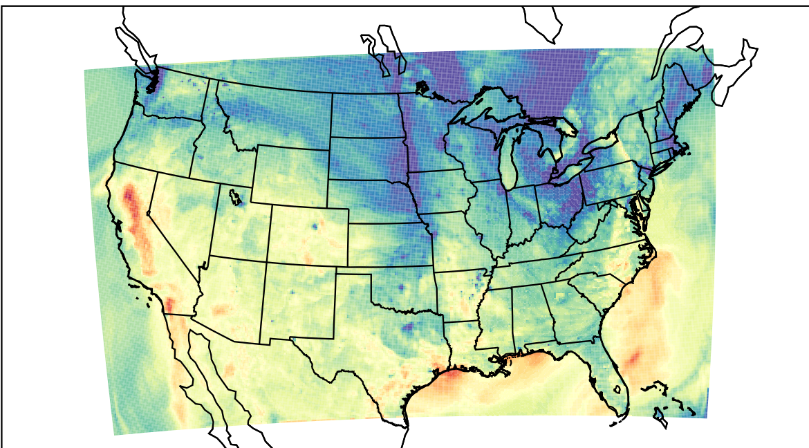
WRF (2023-10-21_00:00:00)
