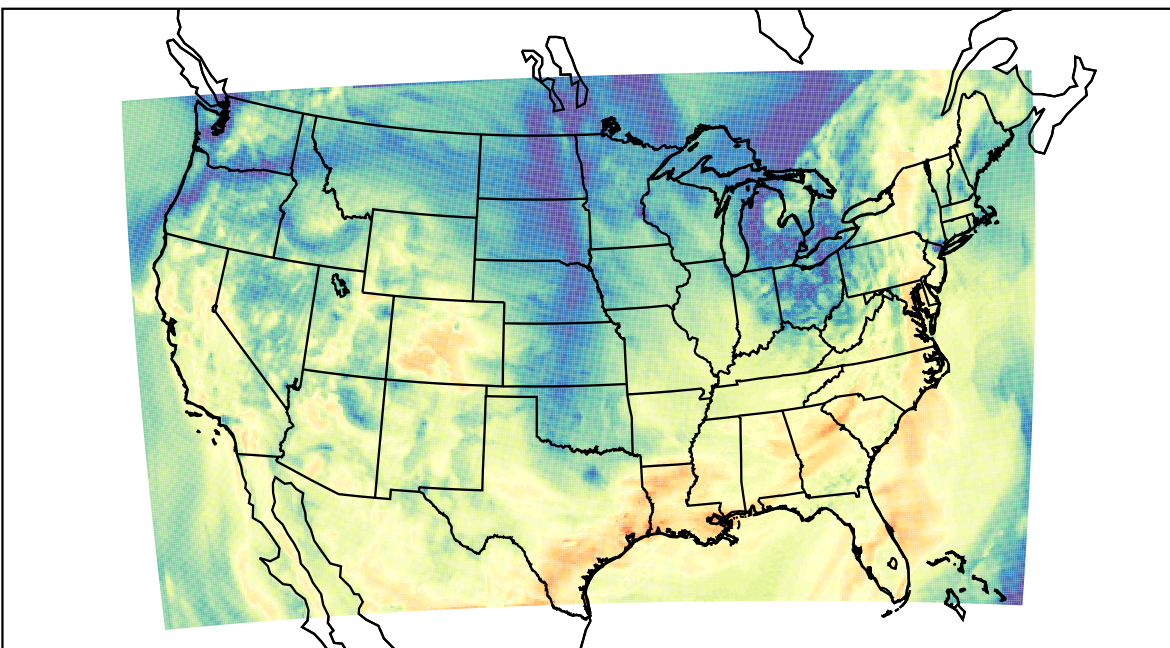
WRF (2023-10-20_18:00:00)
