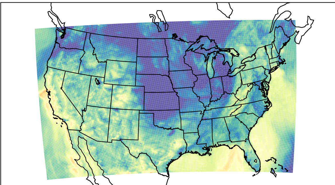
WRF (2023-10-20_08:00:00)
