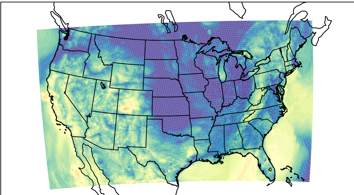
WRF (2023-10-20_11:00:00)
