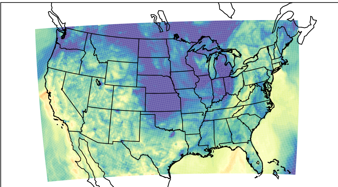
WRF (2023-10-20_07:00:00)
