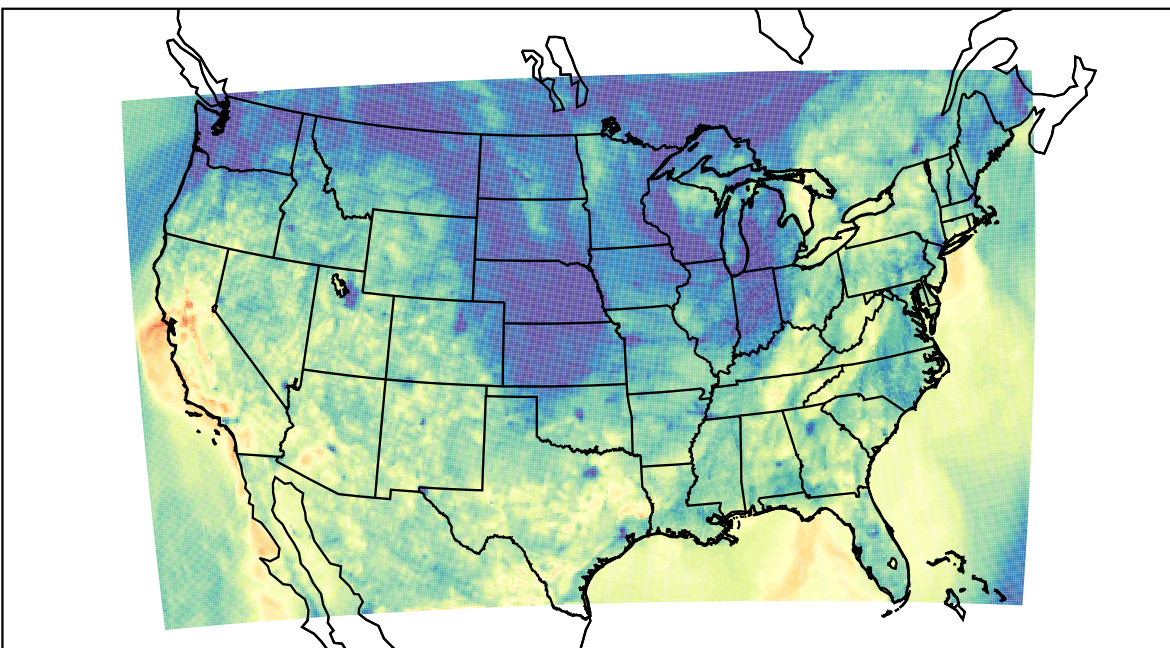
WRF (2023-10-20_03:00:00)
