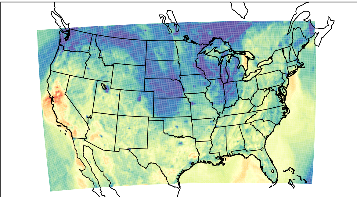
WRF (2023-10-20_01:00:00)
