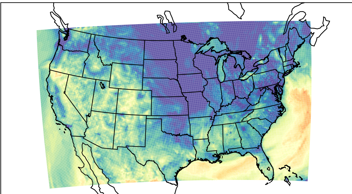
WRF (2023-10-21_11:00:00)
