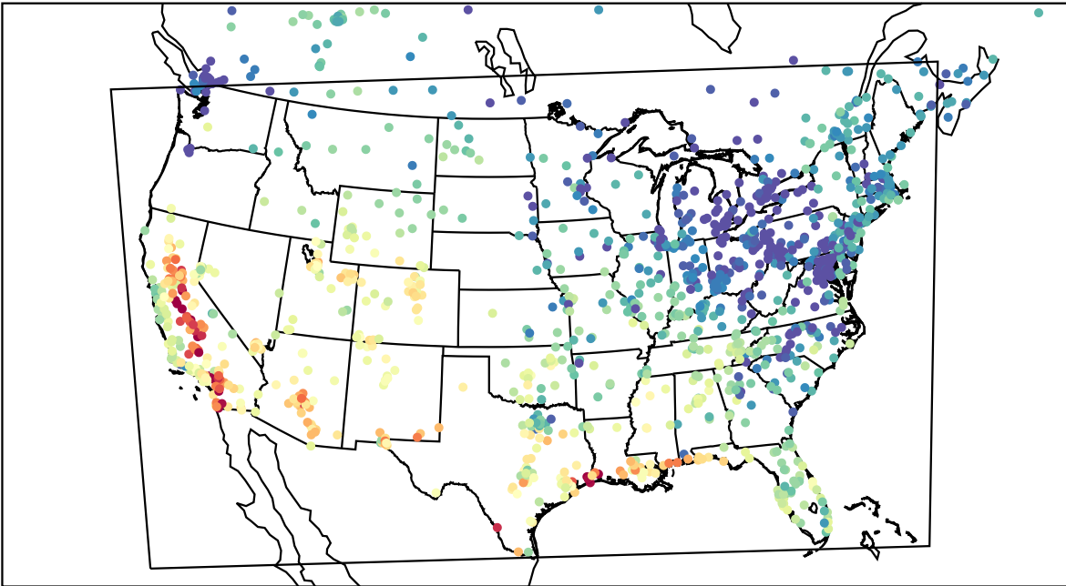
AirNOW (2023-10-20_23:00:00)
