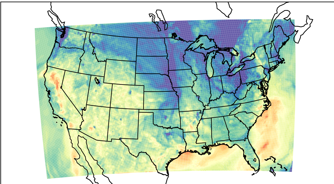
WRF (2023-10-21_02:00:00)
