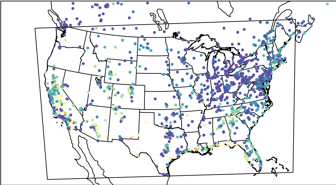
AirNOW (2023-10-21_04:00:00)
