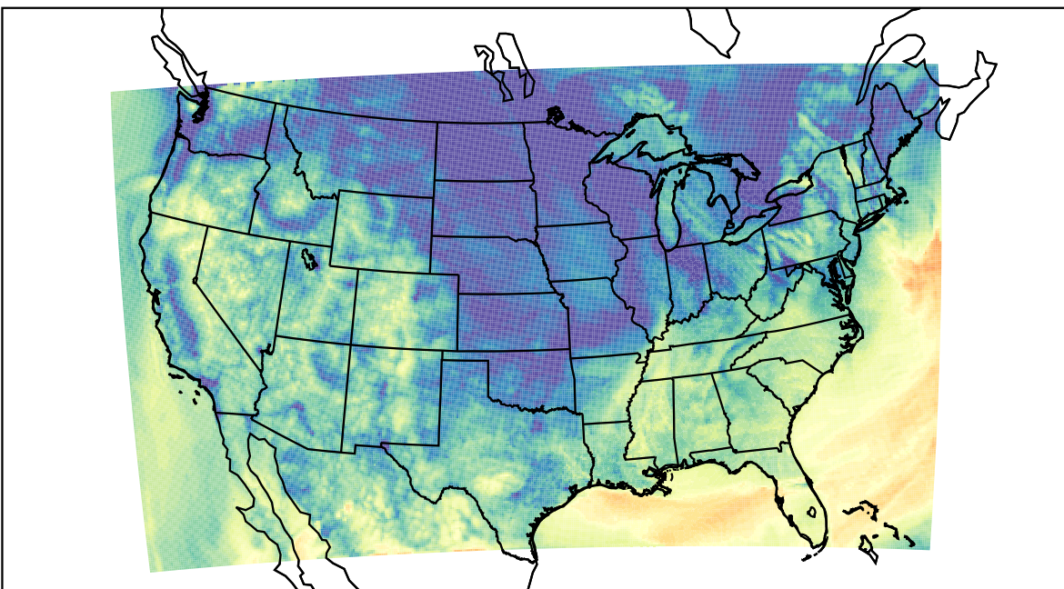
WRF (2023-10-21_15:00:00)
