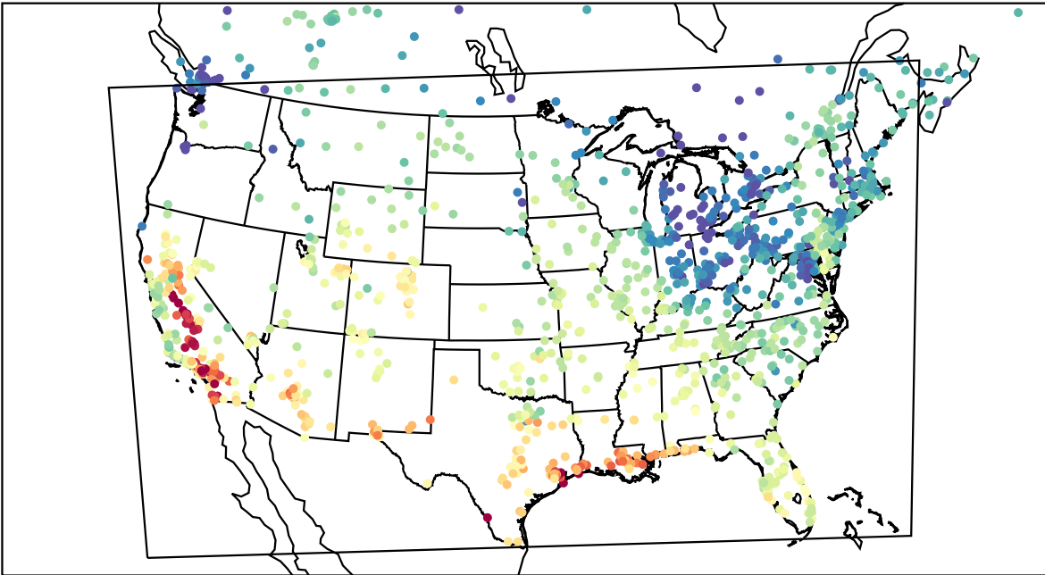
AirNOW (2023-10-20_20:00:00)
