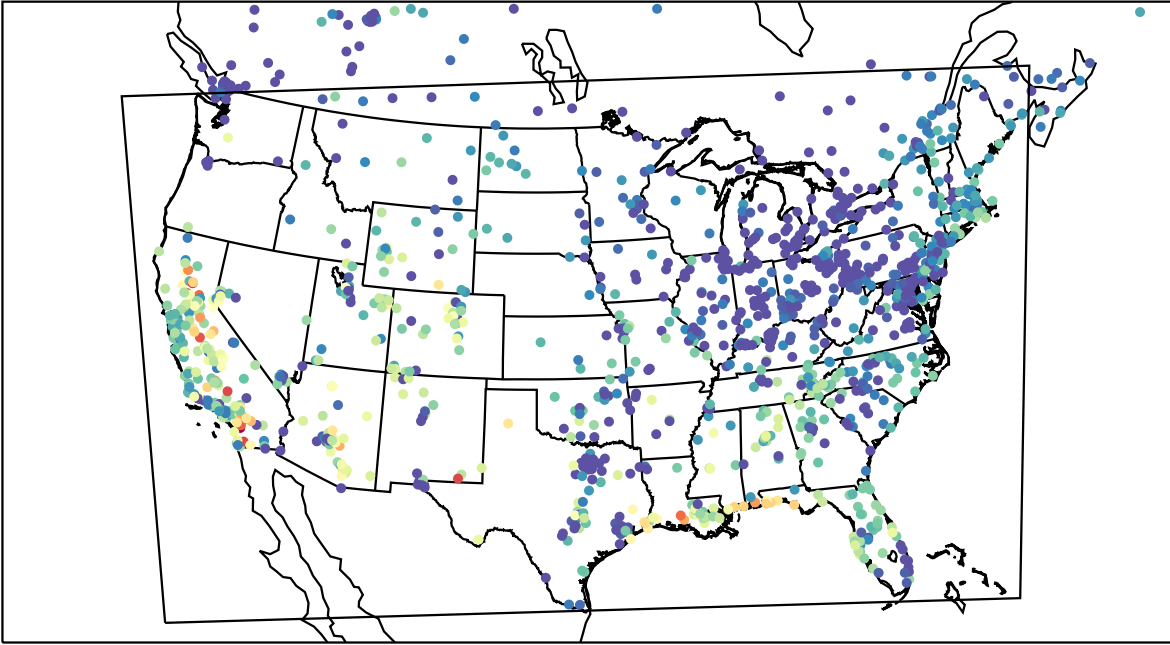
AirNOW (2023-10-21_02:00:00)
