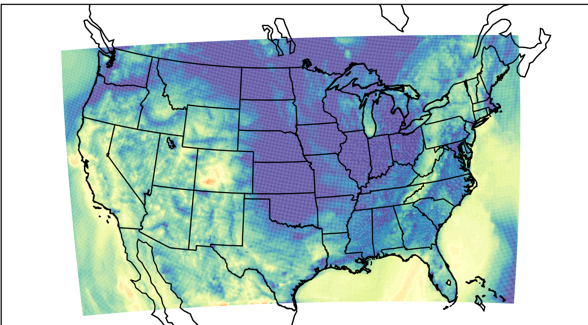
WRF (2023-10-20_12:00:00)
