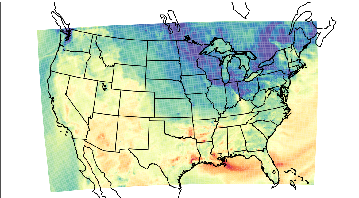
WRF (2023-10-21_23:00:00)
