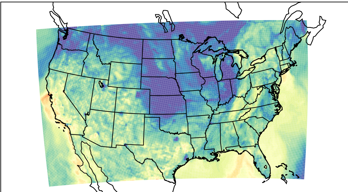
WRF (2023-10-20_05:00:00)
