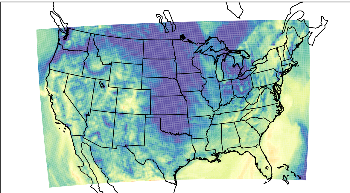
WRF (2023-10-20_15:00:00)
