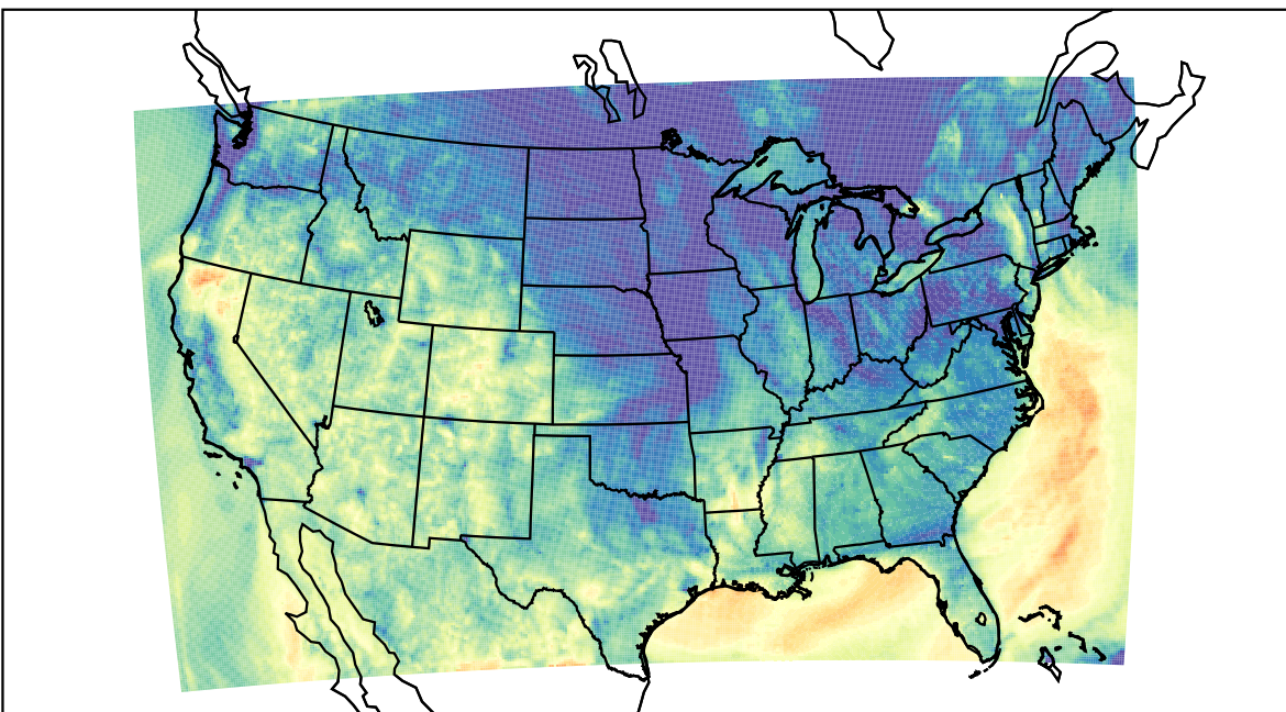
WRF (2023-10-21_07:00:00)
