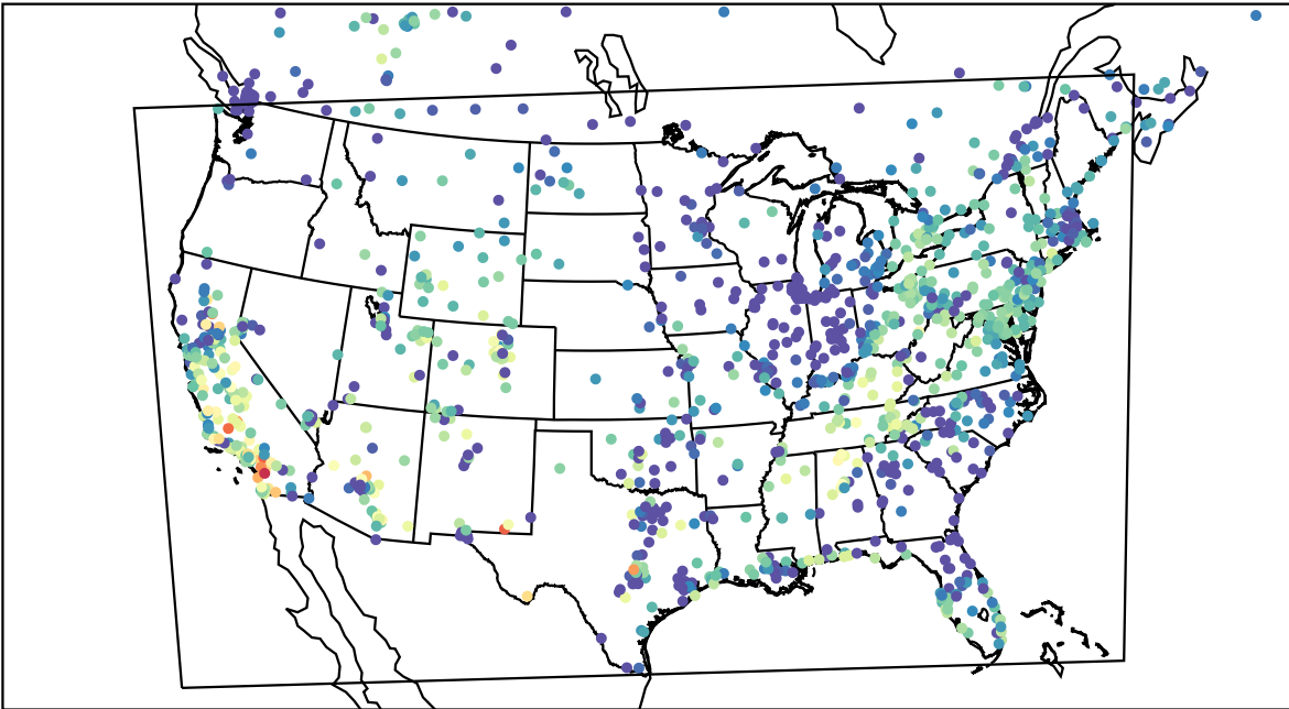
AirNOW (2023-10-20_02:00:00)
