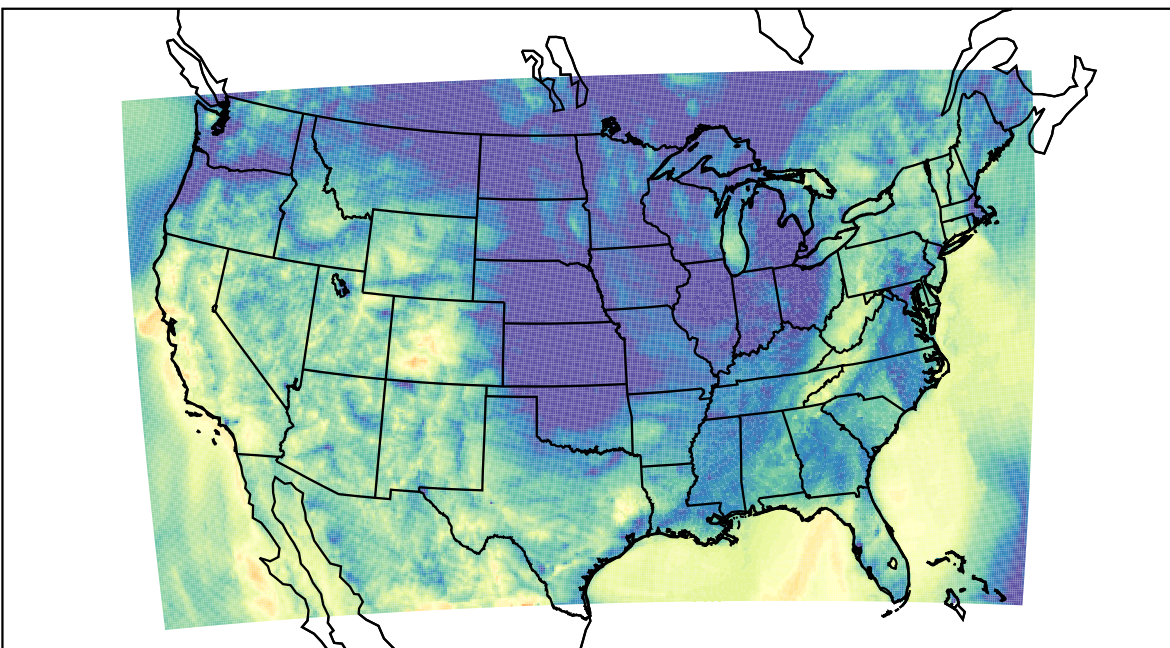
WRF (2023-10-20_10:00:00)
