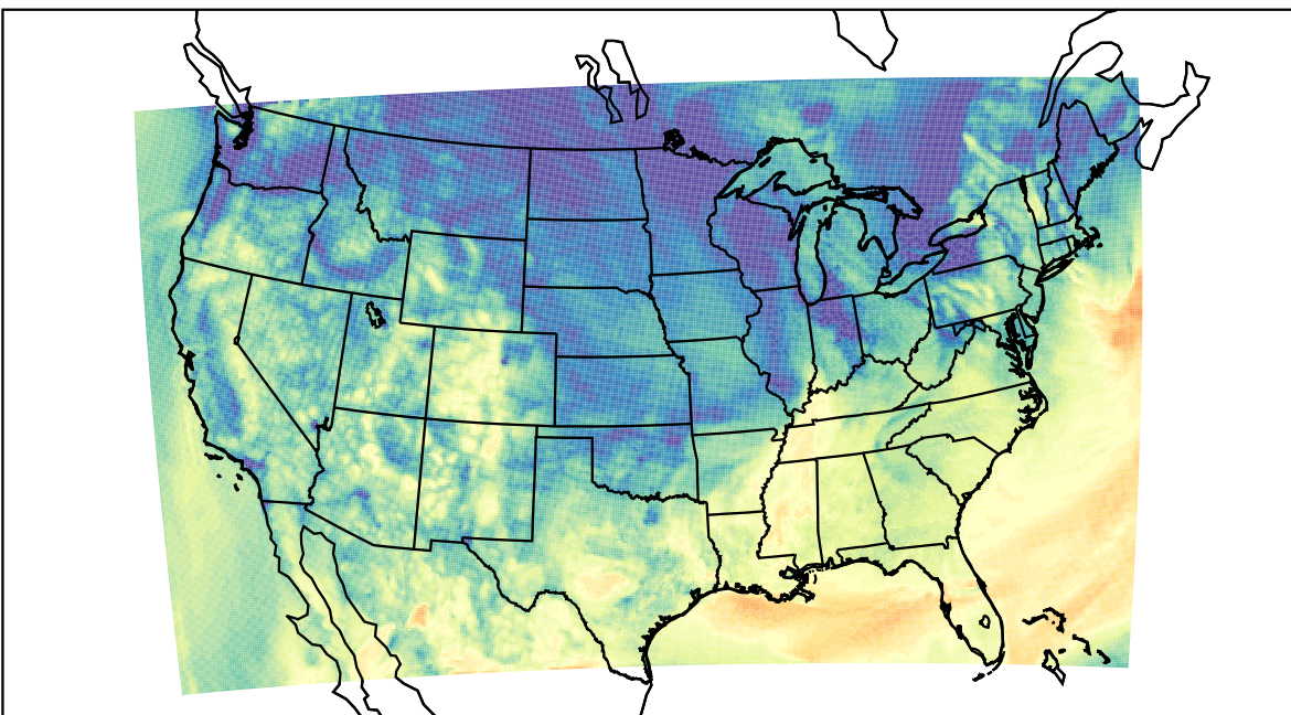
WRF (2023-10-21_16:00:00)
