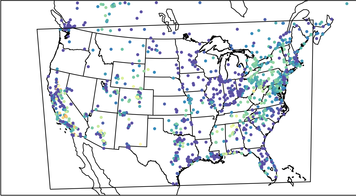
AirNOW (2023-10-20_05:00:00)
