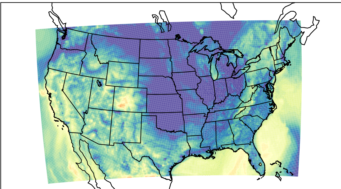
WRF (2023-10-20_13:00:00)
