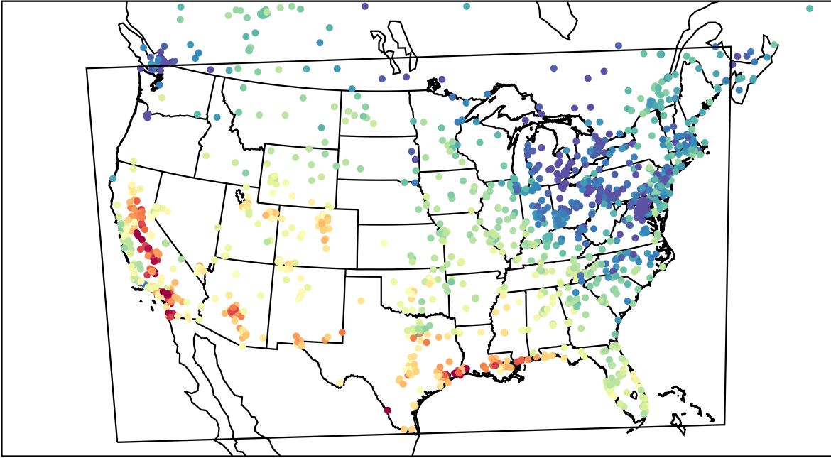
AirNOW (2023-10-20_22:00:00)
