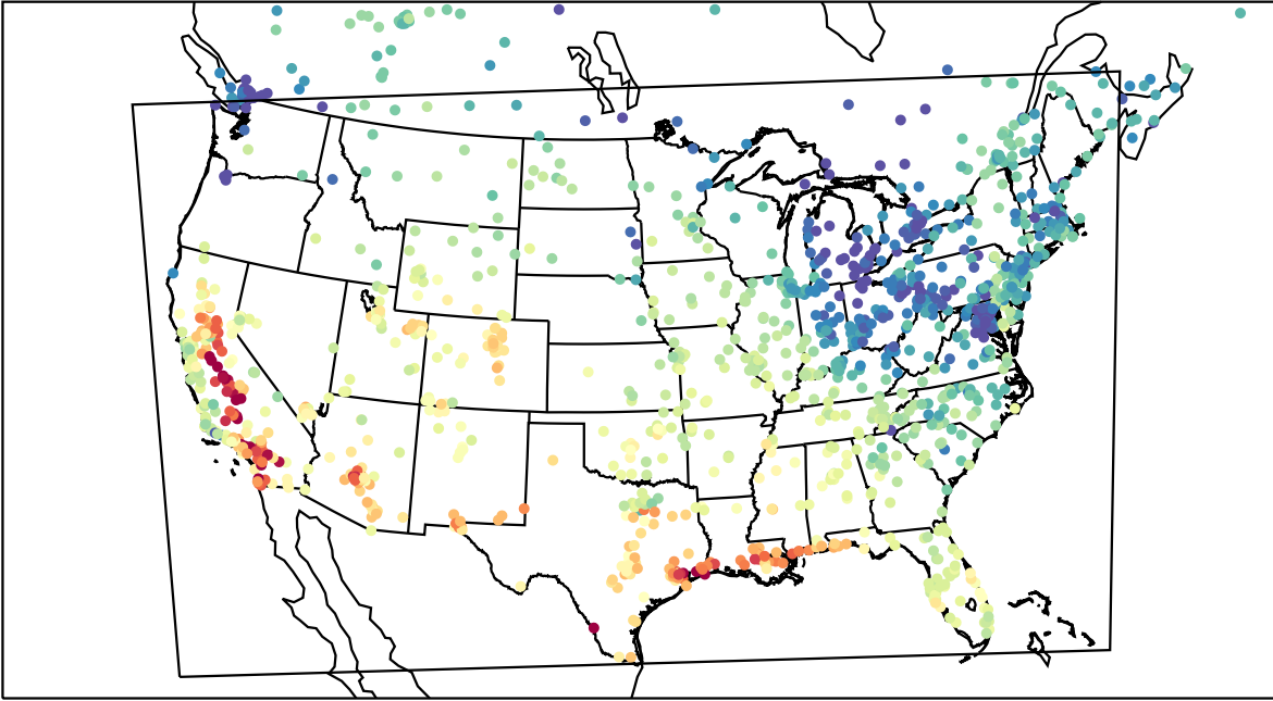
AirNOW (2023-10-20_21:00:00)
