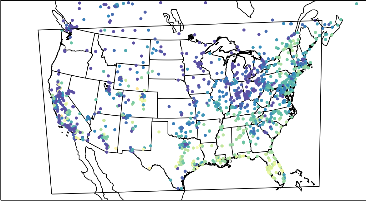
AirNOW (2023-10-20_15:00:00)
