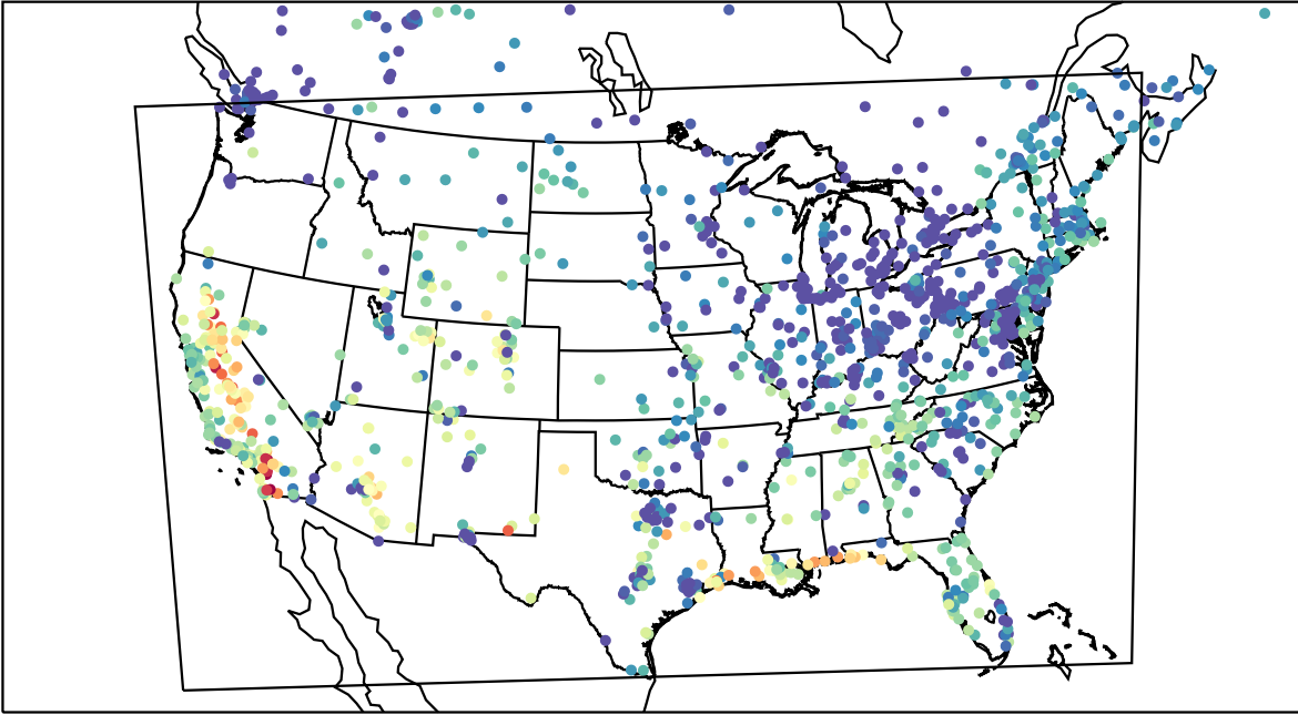
AirNOW (2023-10-21_01:00:00)
