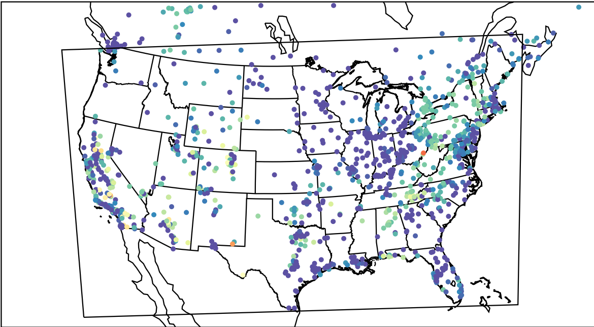
AirNOW (2023-10-20_07:00:00)
