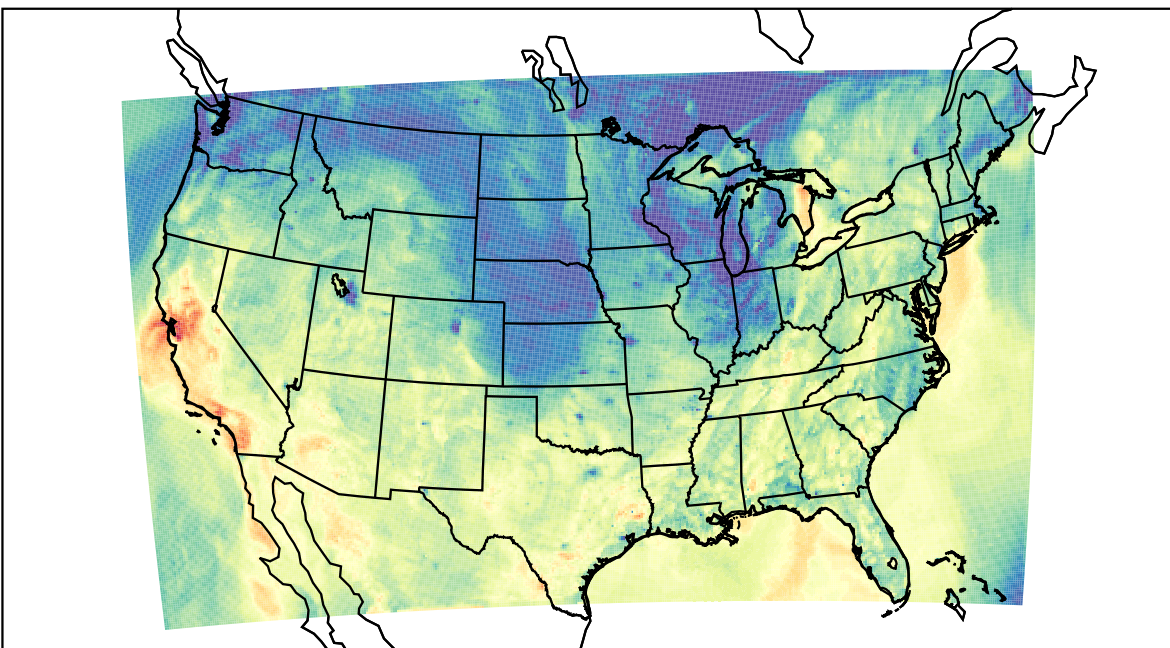
WRF (2023-10-20_00:00:00)
