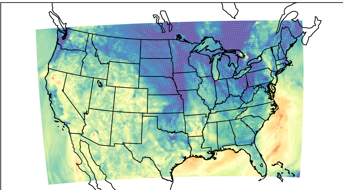
WRF (2023-10-21_04:00:00)
