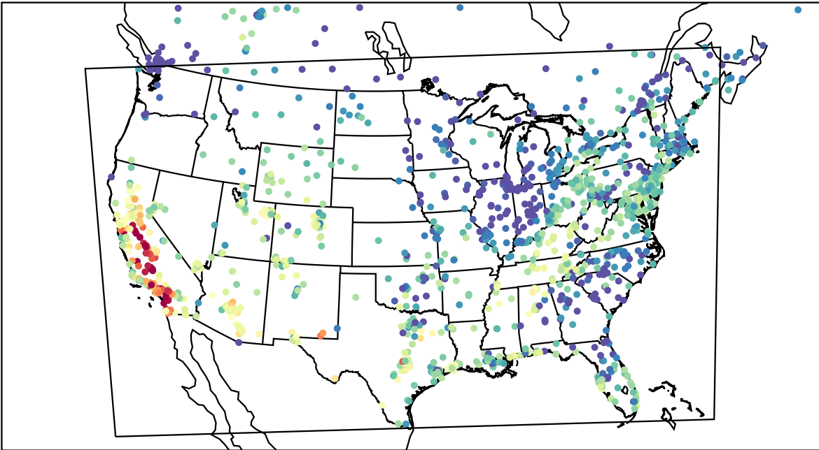
AirNOW (2023-10-20_00:00:00)
