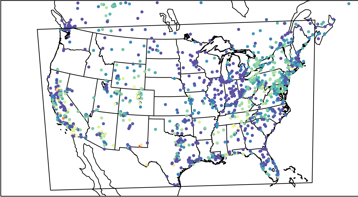
AirNOW (2023-10-20_04:00:00)
