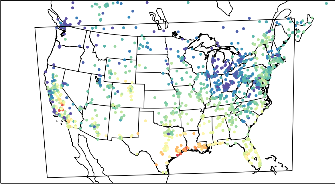
AirNOW (2023-10-20_17:00:00)
