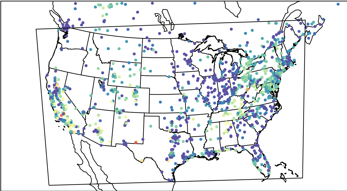
AirNOW (2023-10-20_03:00:00)
