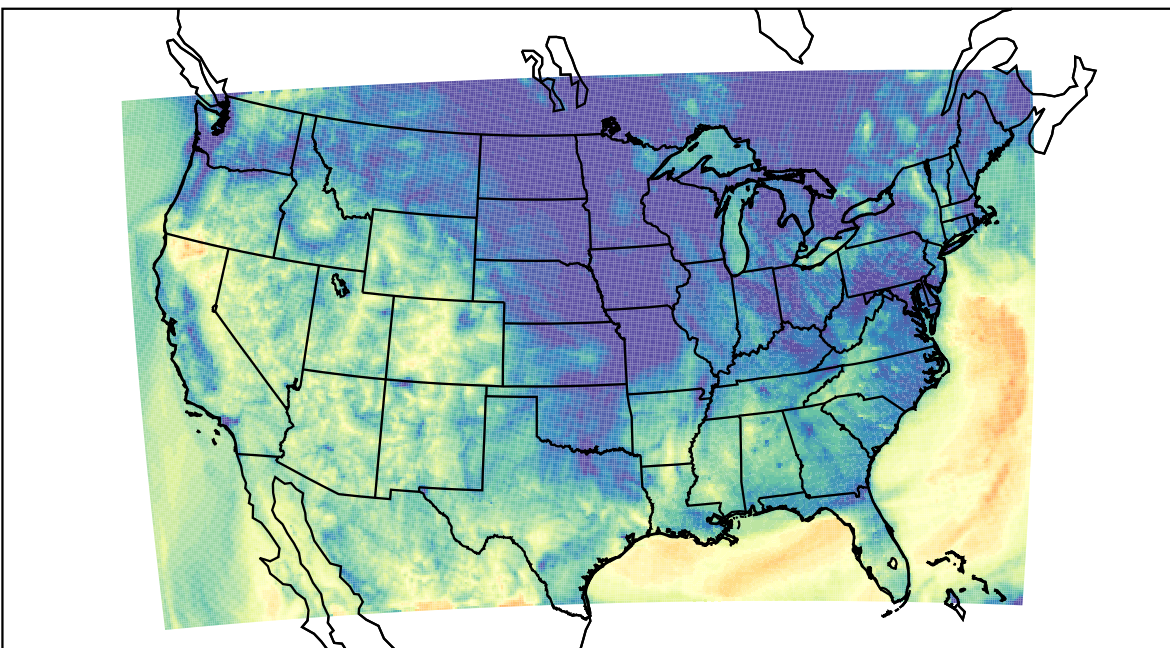
WRF (2023-10-21_10:00:00)
