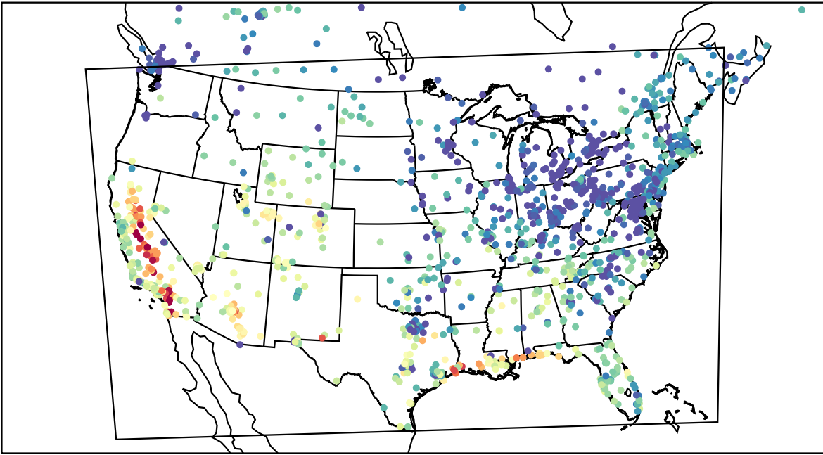
AirNOW (2023-10-21_00:00:00)
