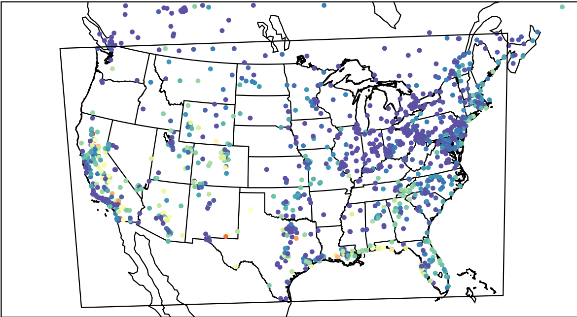
AirNOW (2023-10-21_05:00:00)
