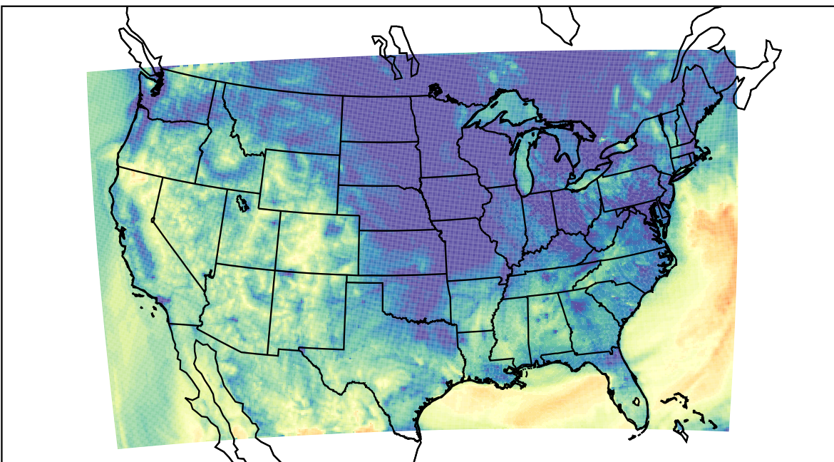
WRF (2023-10-21_12:00:00)
