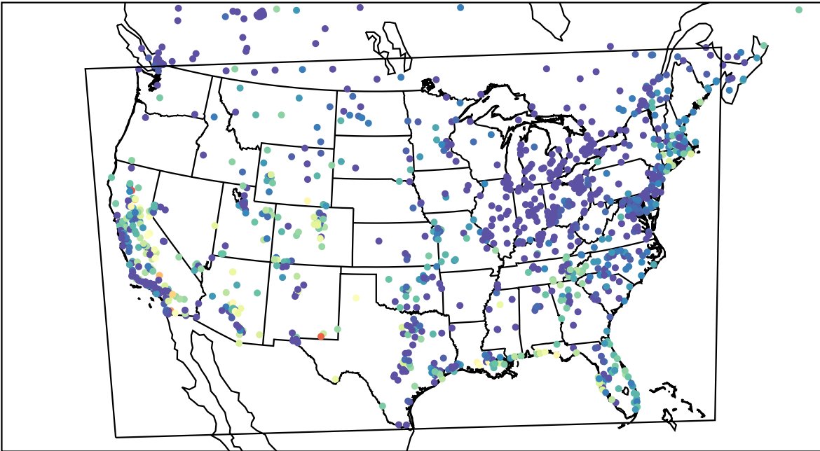
AirNOW (2023-10-21_06:00:00)
