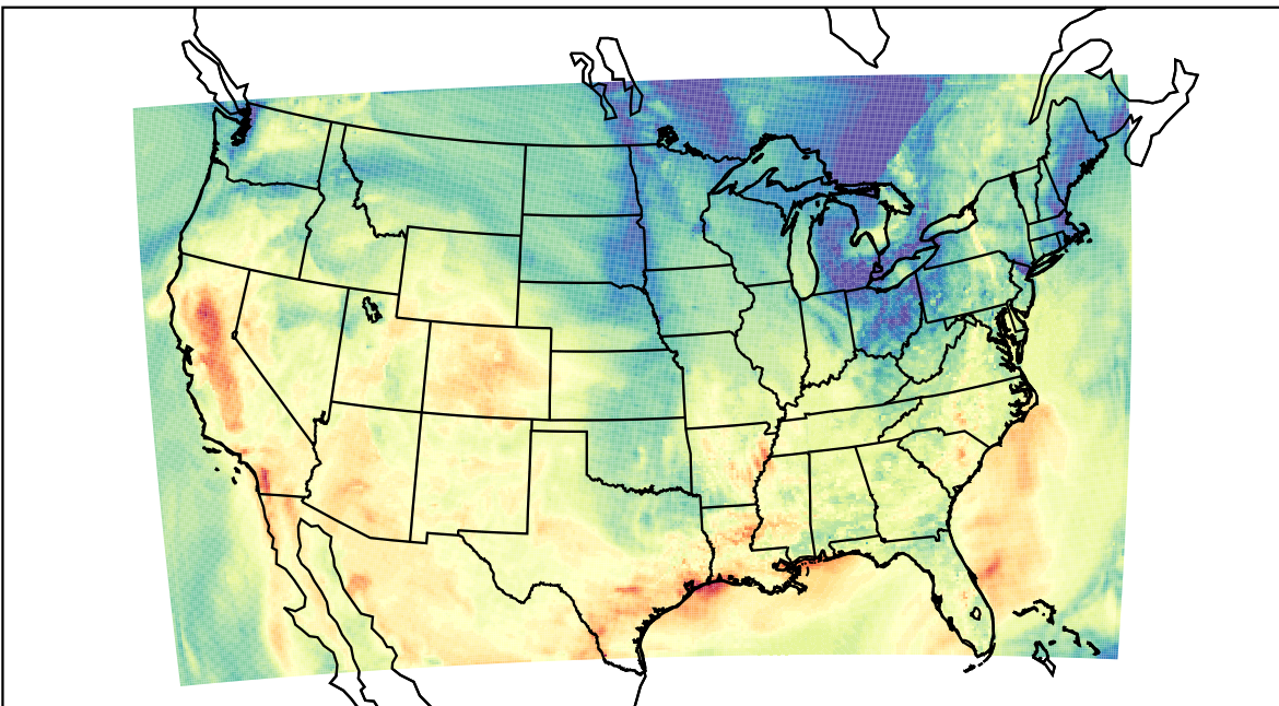
WRF (2023-10-20_22:00:00)
