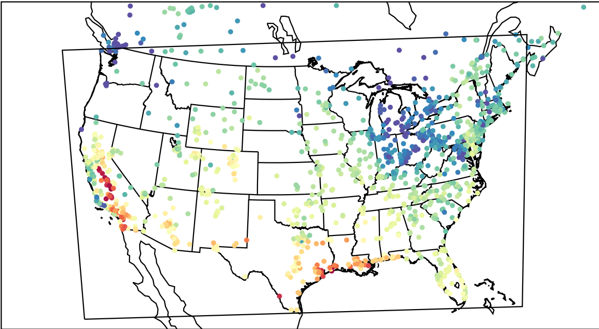
AirNOW (2023-10-20_19:00:00)
