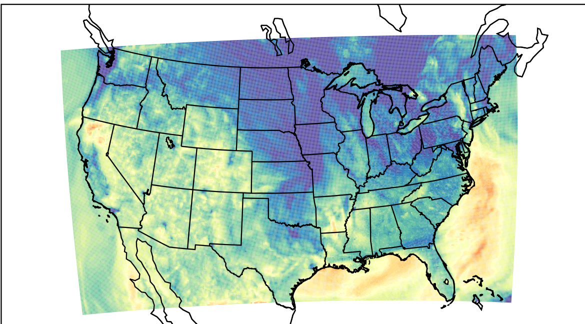
WRF (2023-10-21_06:00:00)
