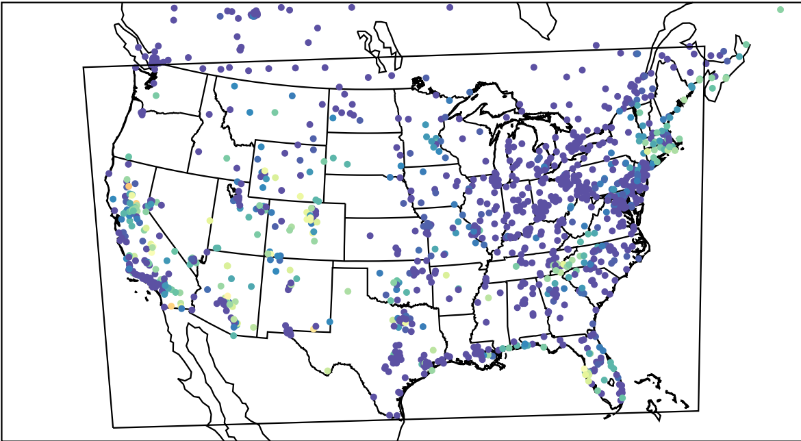
AirNOW (2023-10-21_11:00:00)
