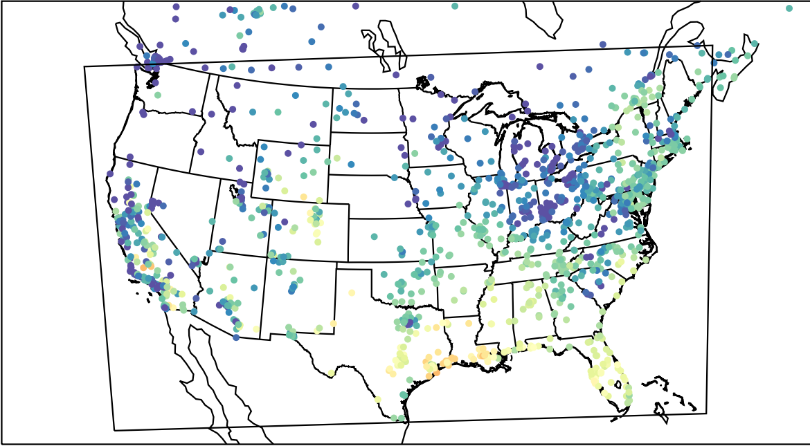
AirNOW (2023-10-20_16:00:00)
