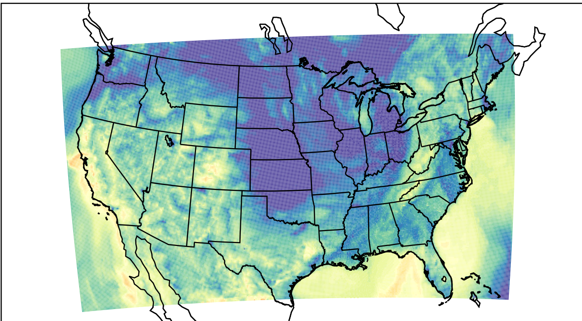
WRF (2023-10-20_09:00:00)
