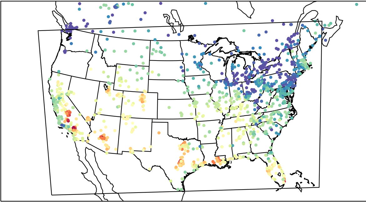
AirNOW (2023-10-21_22:00:00)
