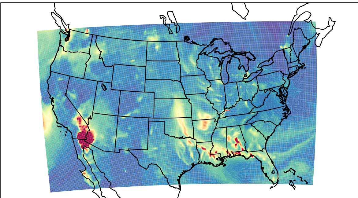
WRF 2023-10-23_06:00:00
