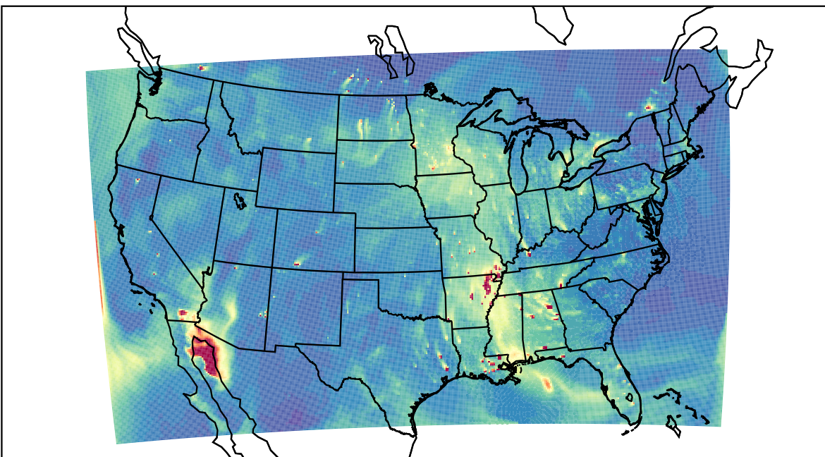
WRF 2023-10-23_23:00:00
