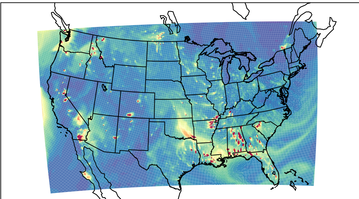
WRF 2023-10-23_00:00:00
