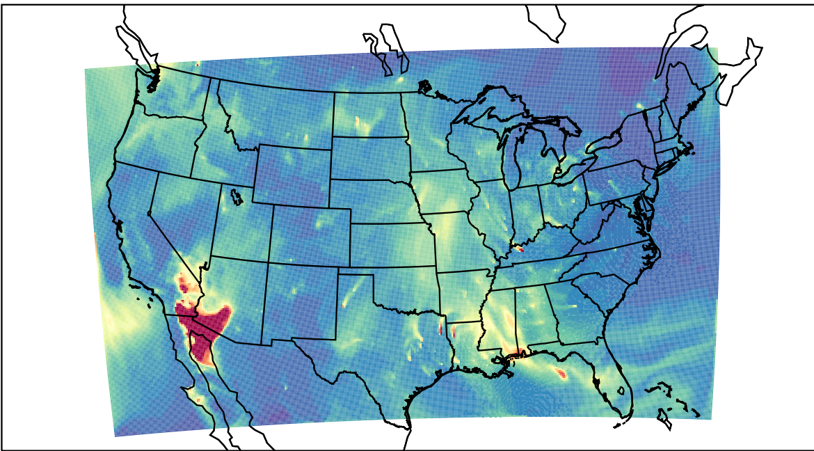
WRF 2023-10-23_15:00:00
