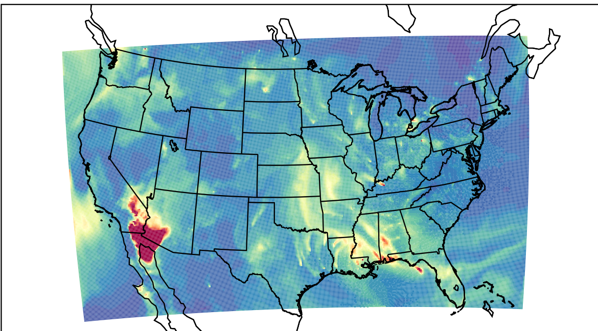
WRF 2023-10-23_11:00:00
