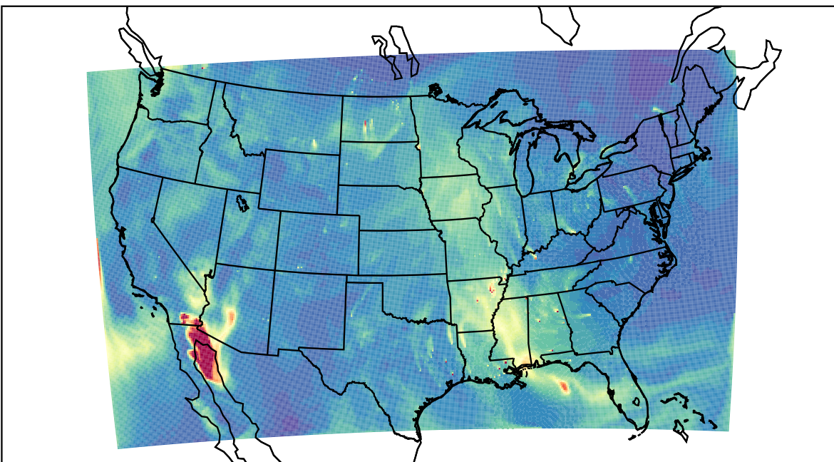
WRF 2023-10-23_19:00:00
