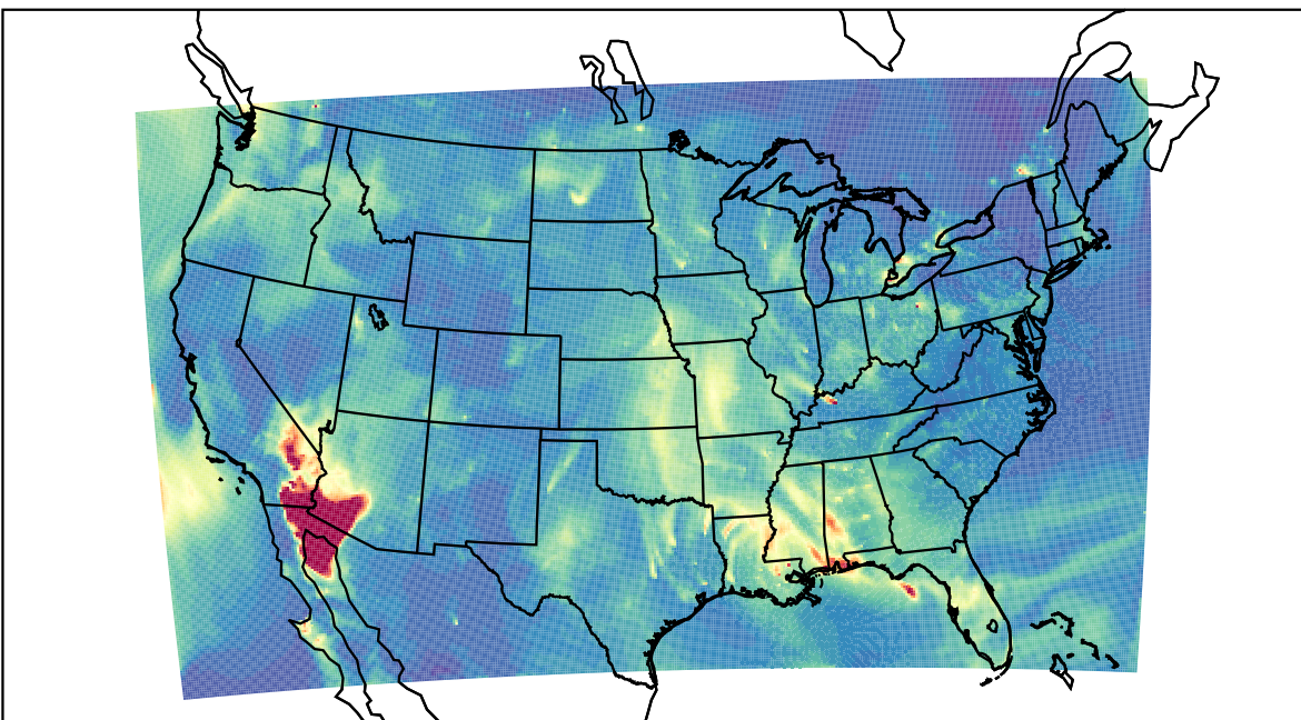
WRF 2023-10-23_12:00:00
