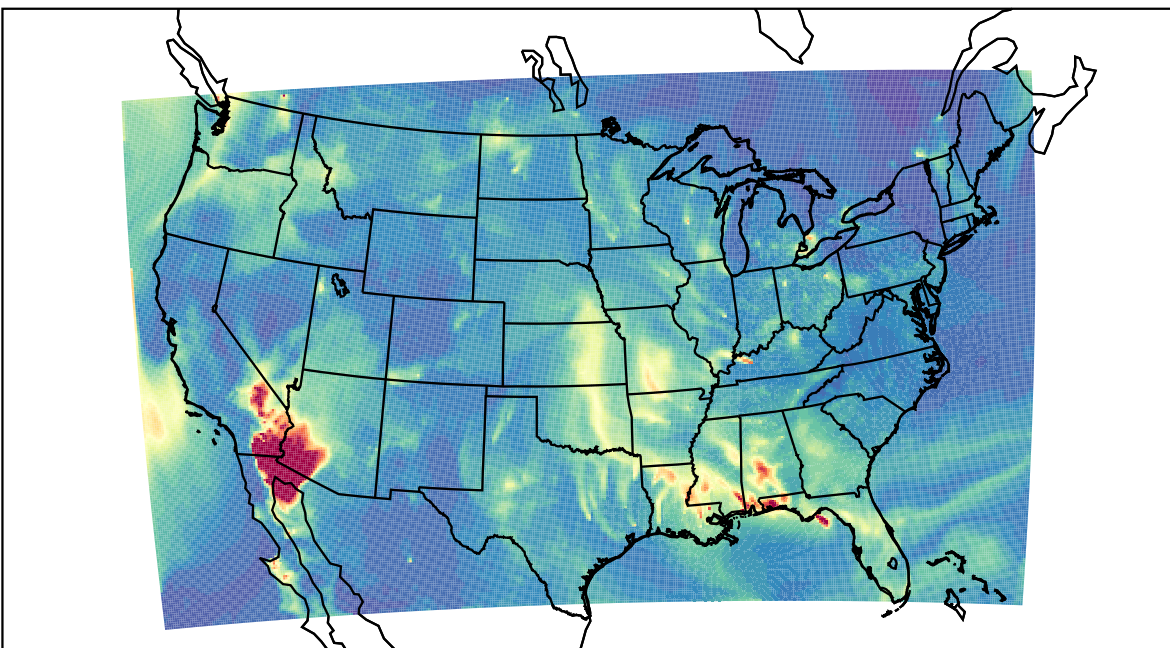
WRF 2023-10-23_09:00:00
