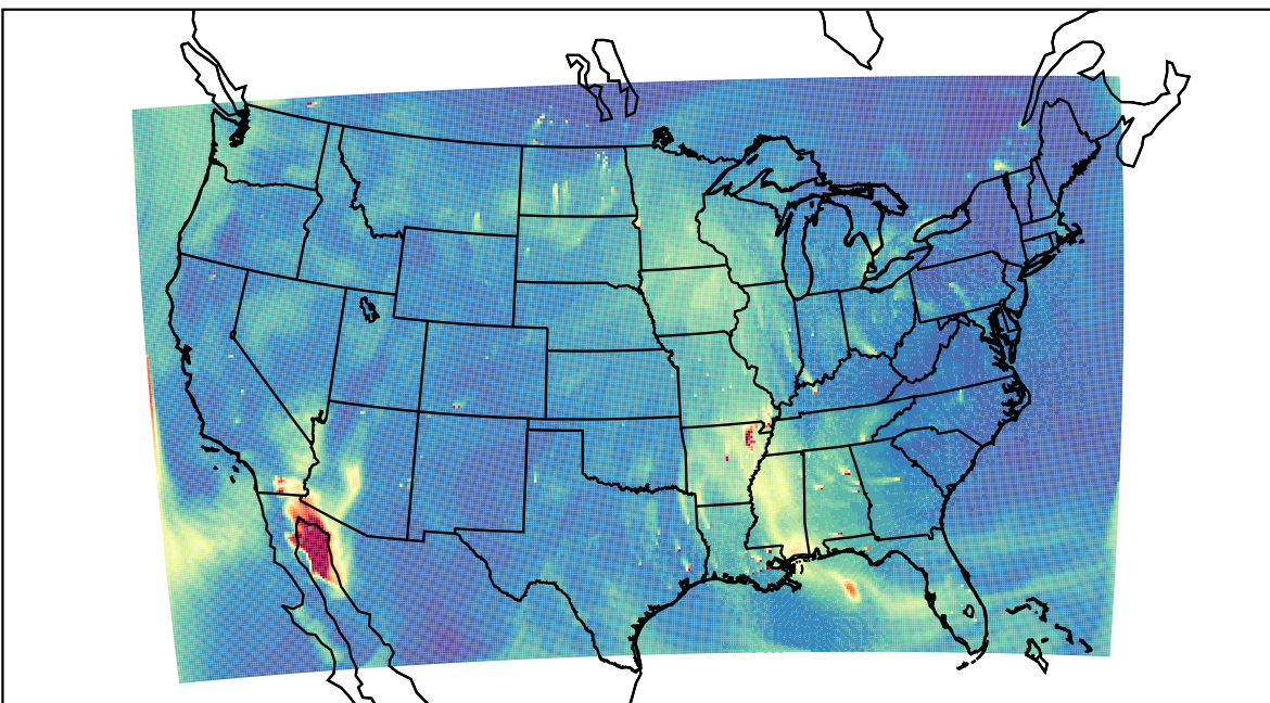
WRF 2023-10-23_21:00:00
