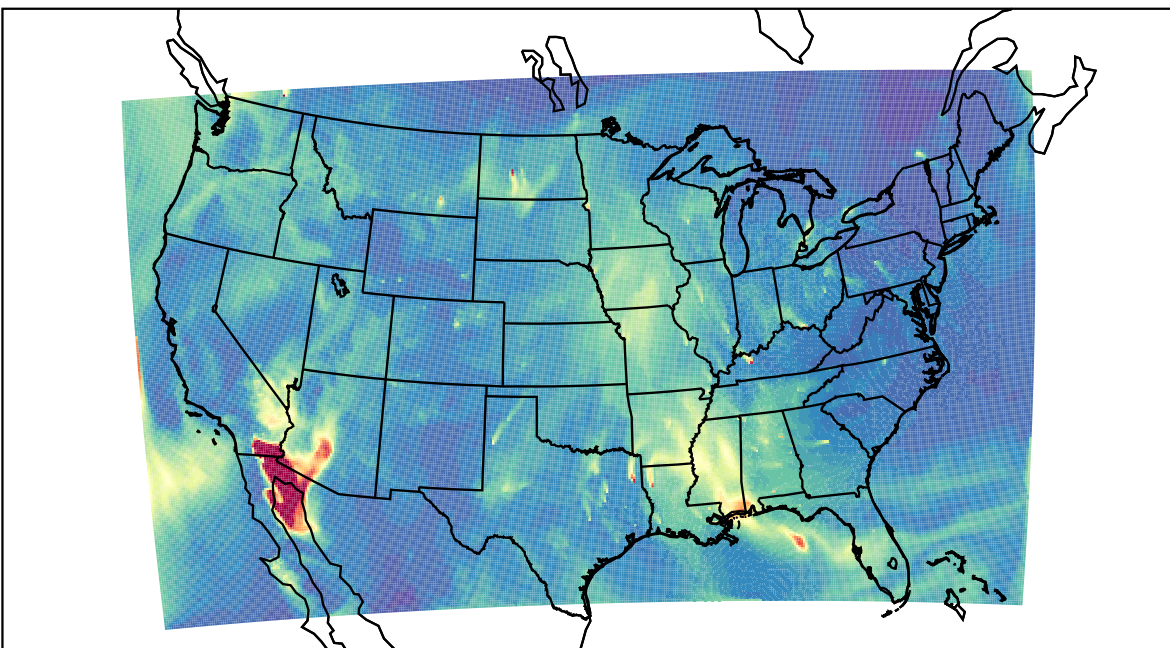
WRF 2023-10-23_17:00:00
