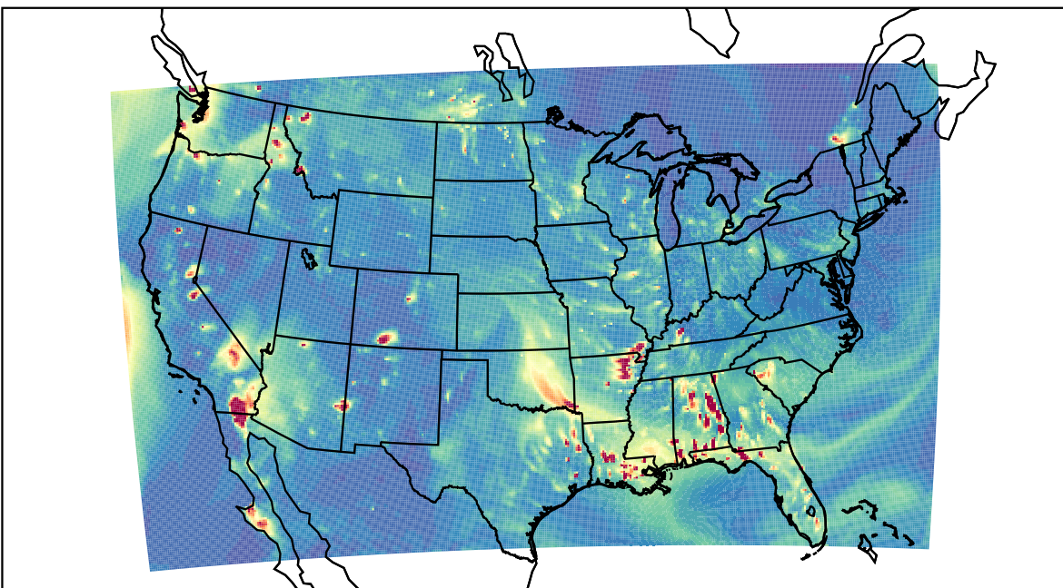
WRF 2023-10-23_01:00:00
