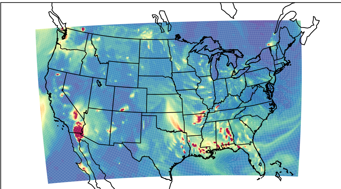
WRF 2023-10-23_03:00:00
