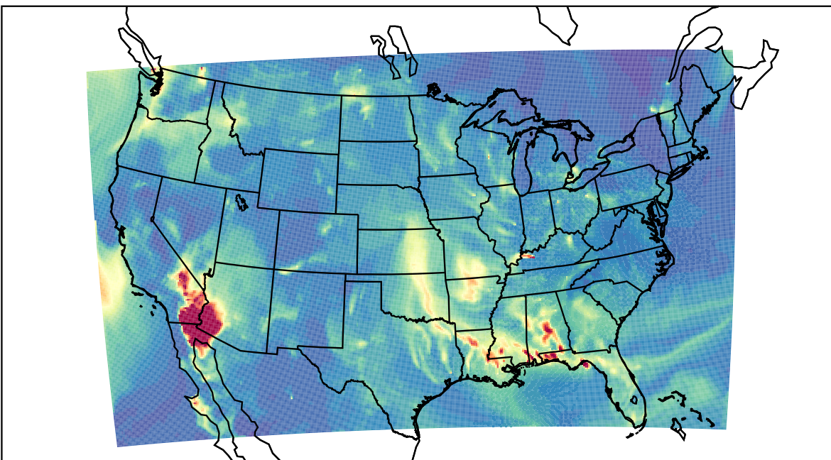
WRF 2023-10-23_07:00:00
