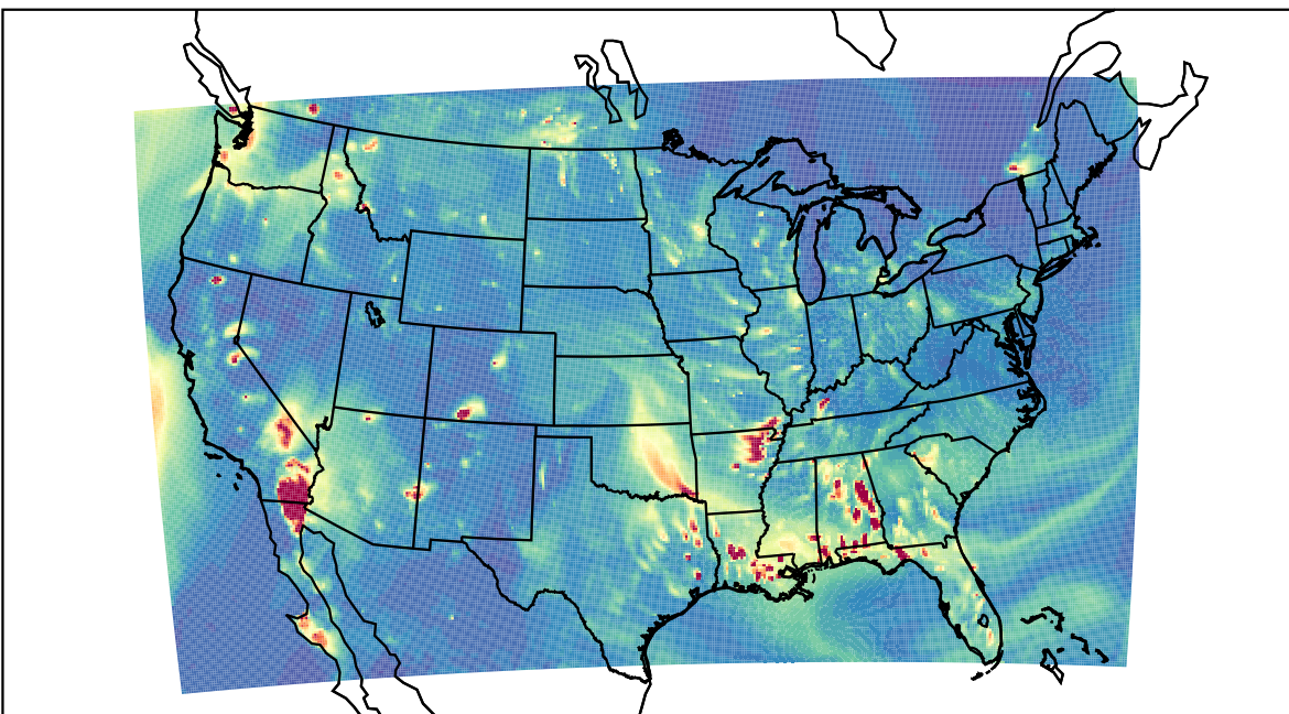
WRF 2023-10-23_02:00:00
