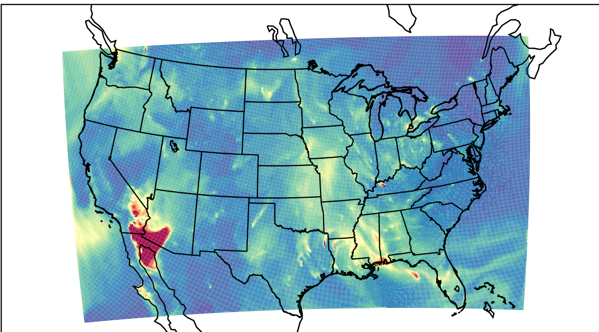
WRF 2023-10-23_14:00:00
