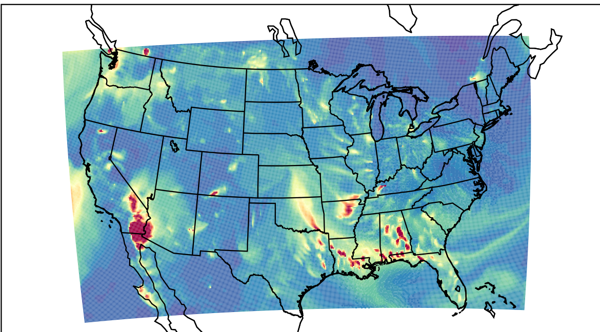
WRF 2023-10-23_04:00:00
