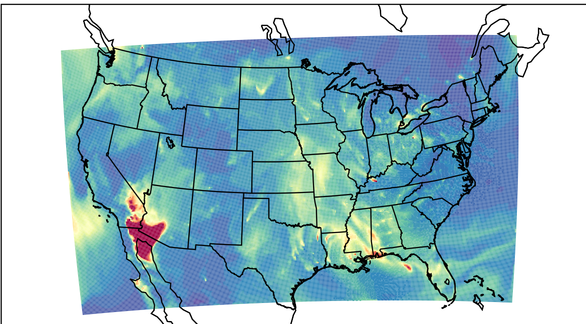
WRF 2023-10-23_13:00:00
