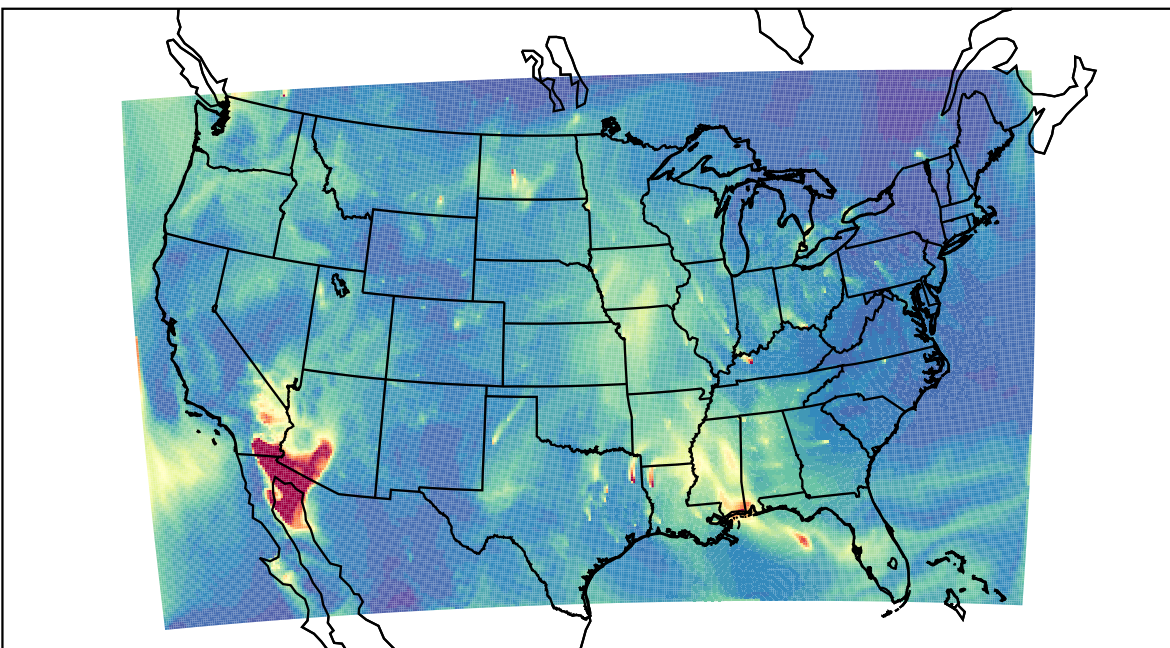
WRF 2023-10-23_16:00:00
