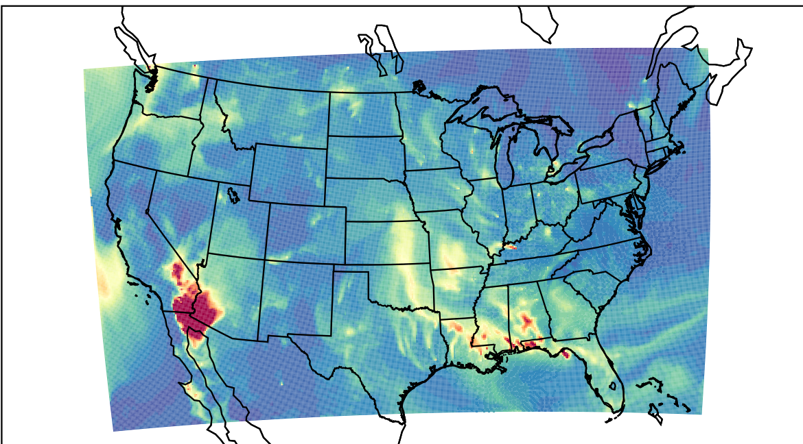
WRF 2023-10-23_08:00:00
