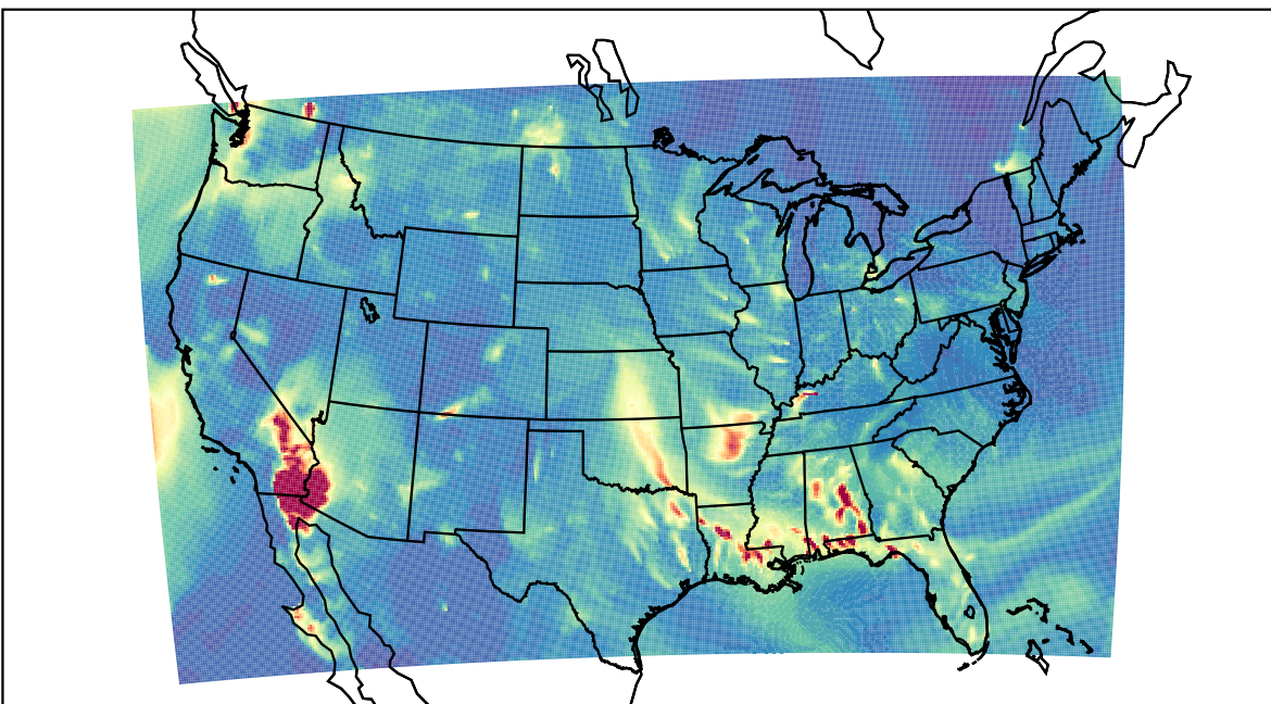
WRF 2023-10-23_05:00:00
