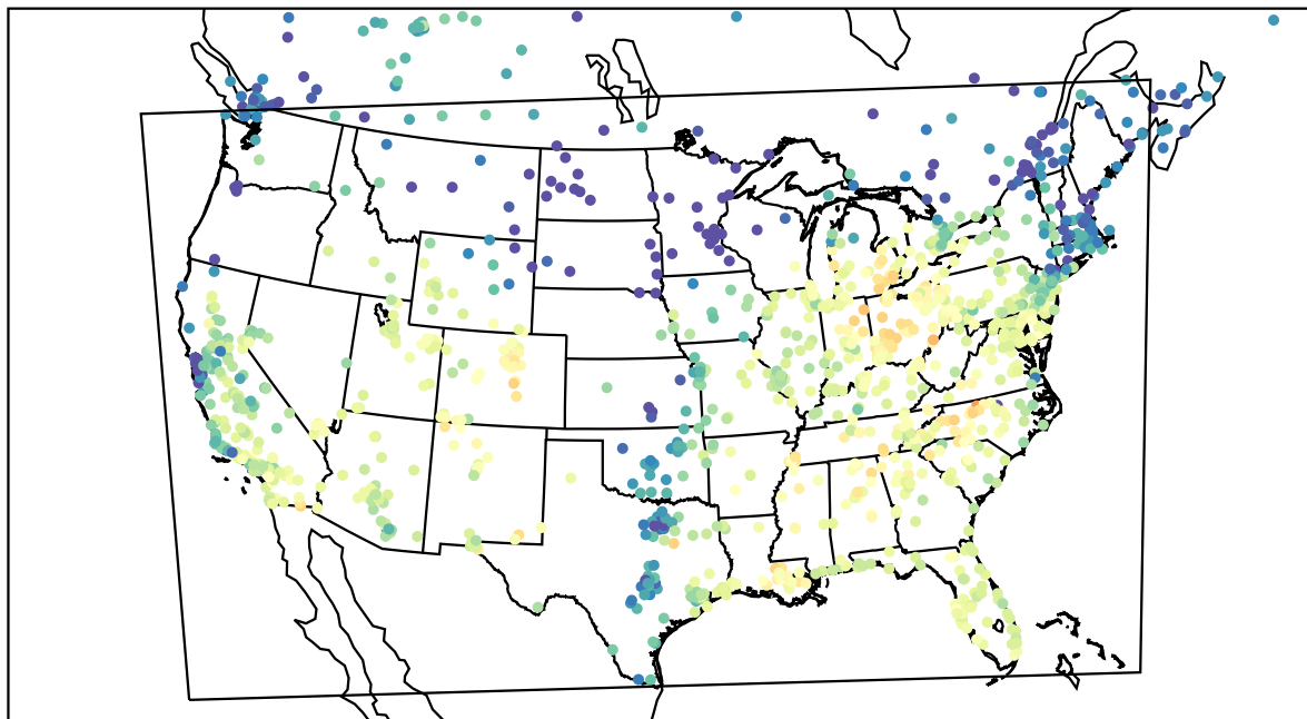
AirNOW (2023-10-24_20:00:00)
