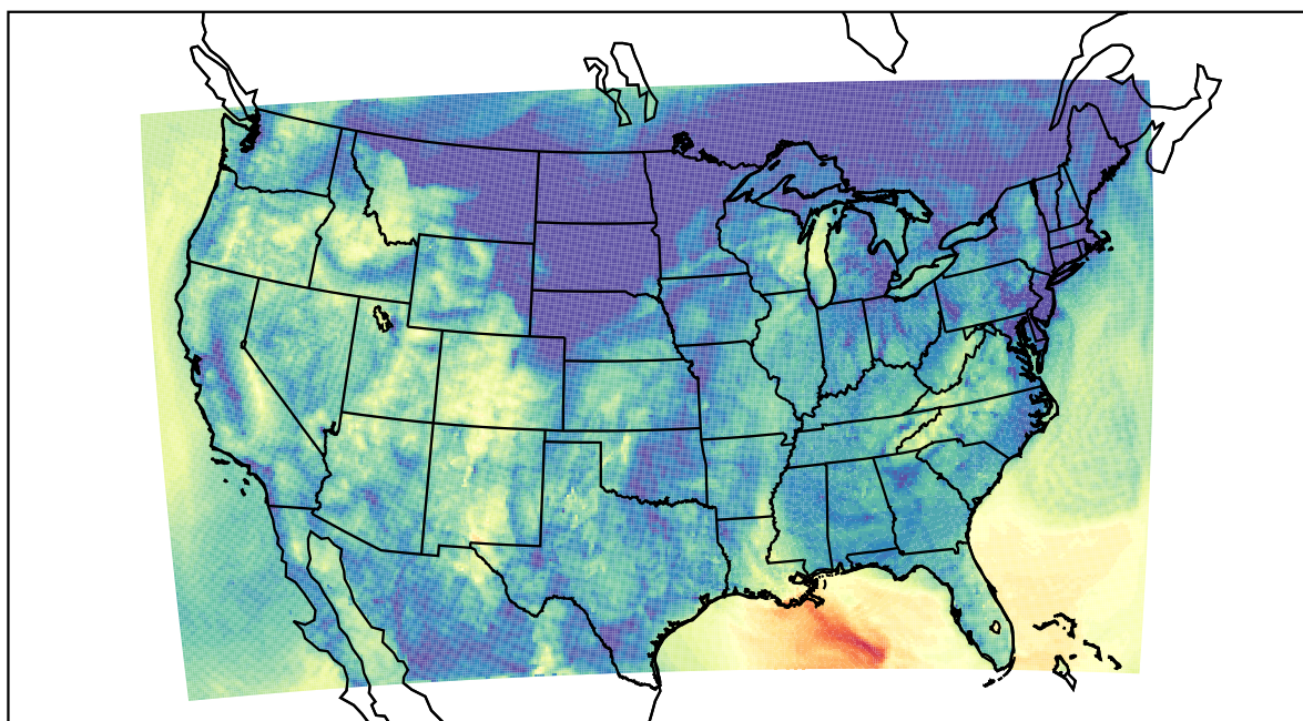
WRF (2023-10-24_12:00:00)
