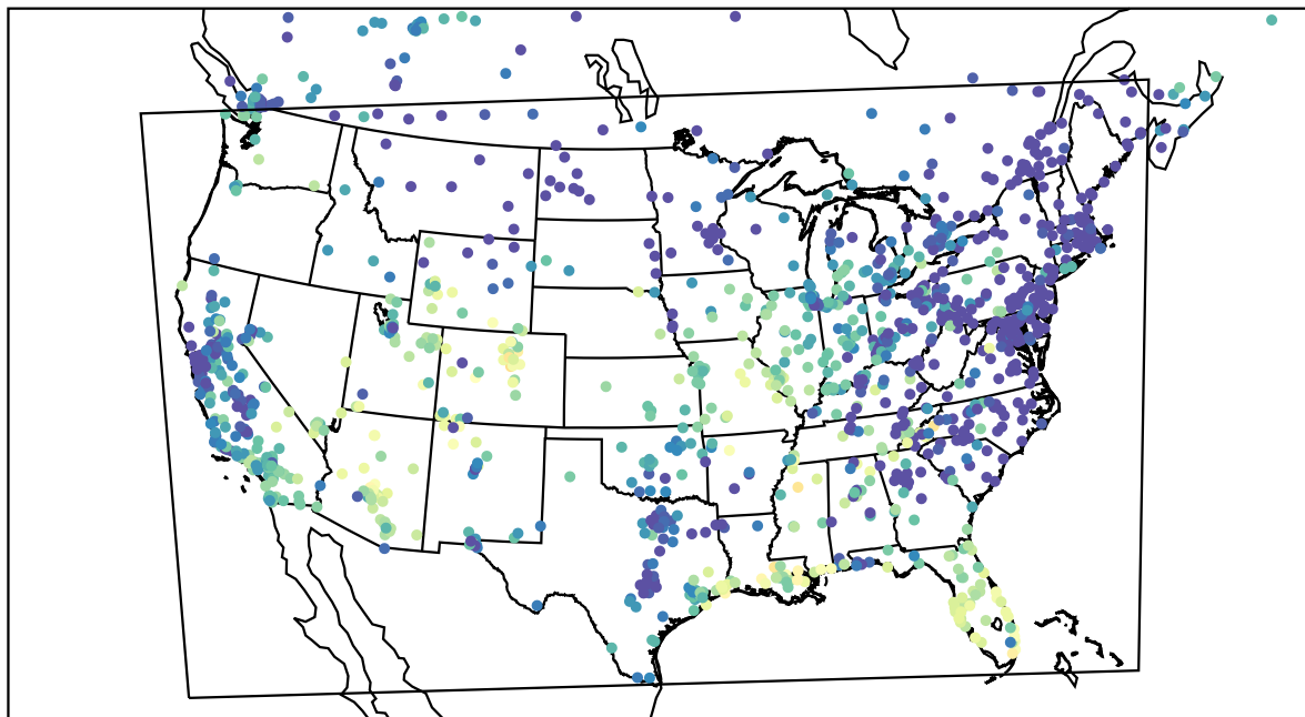
AirNOW (2023-10-24_01:00:00)
