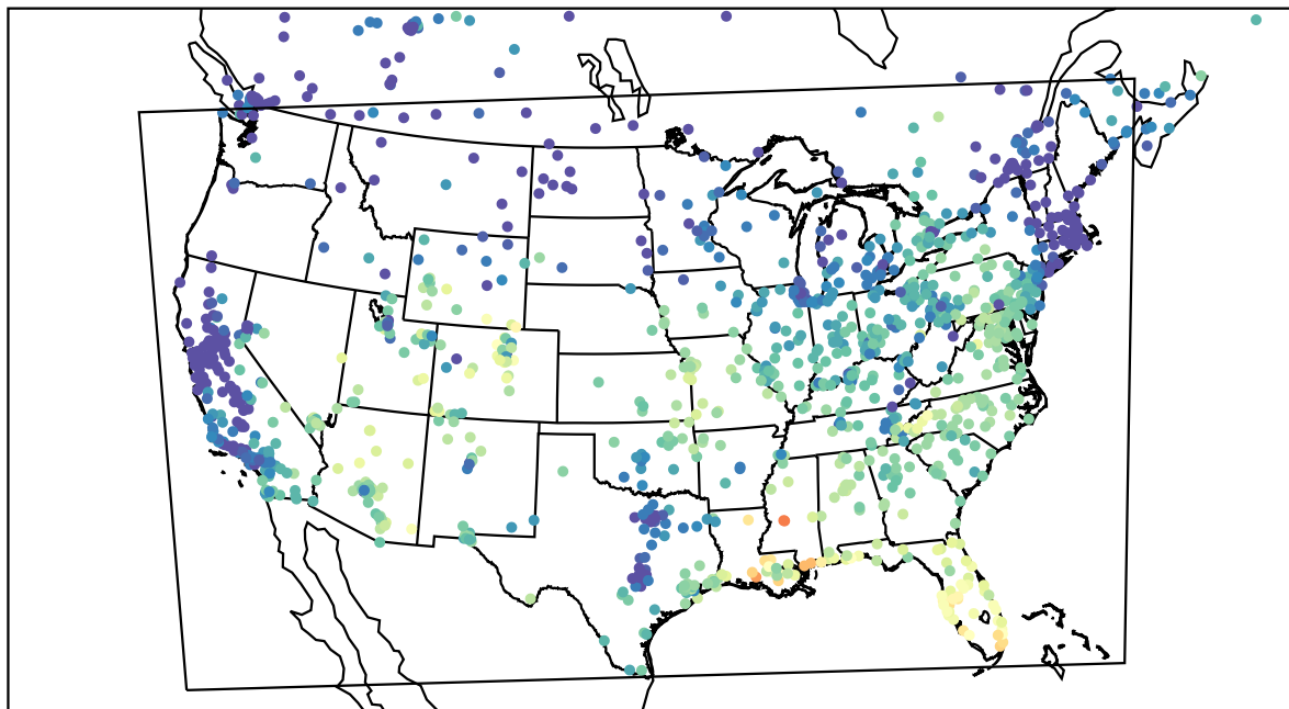
AirNOW (2023-10-23_16:00:00)
