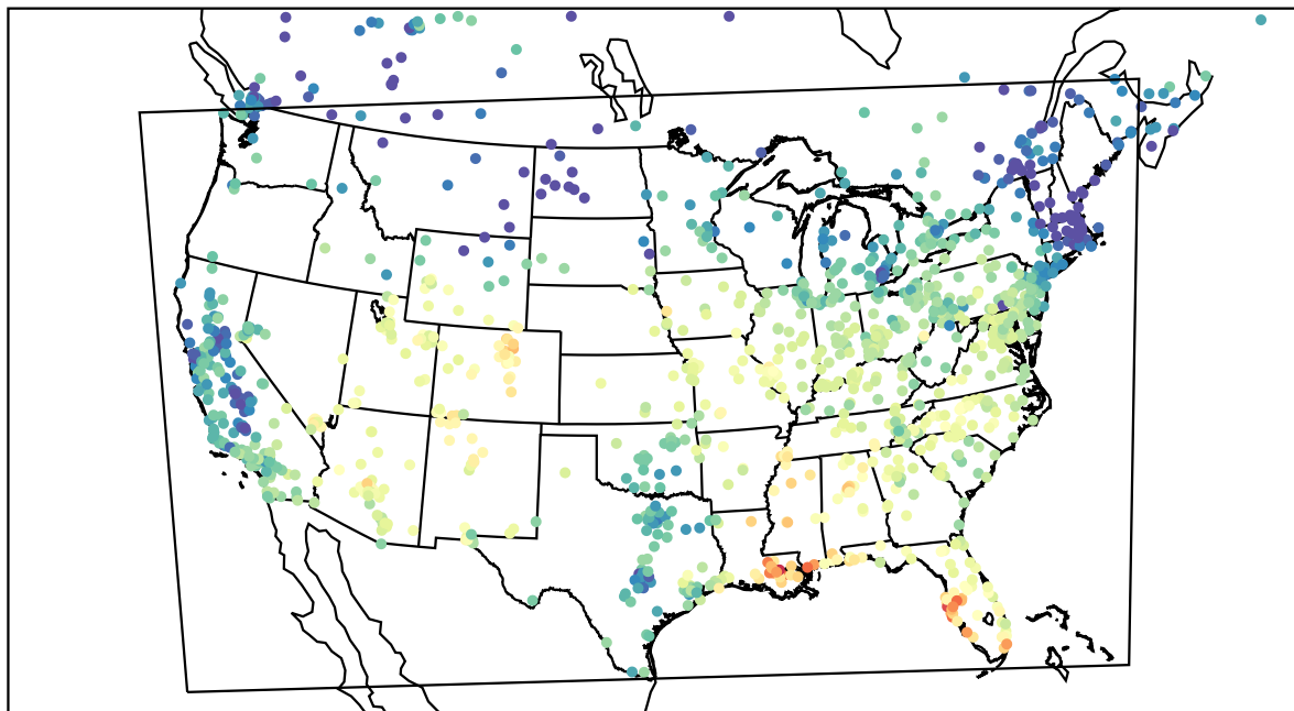
AirNOW (2023-10-23_20:00:00)
