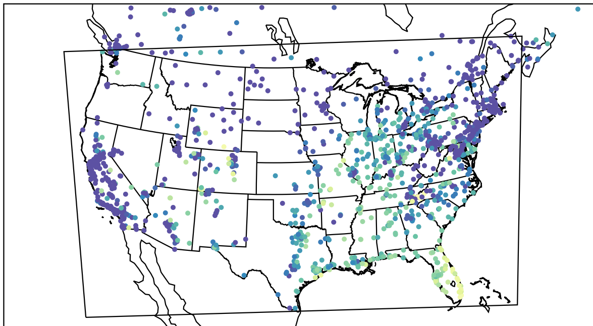
AirNOW (2023-10-24_14:00:00)
