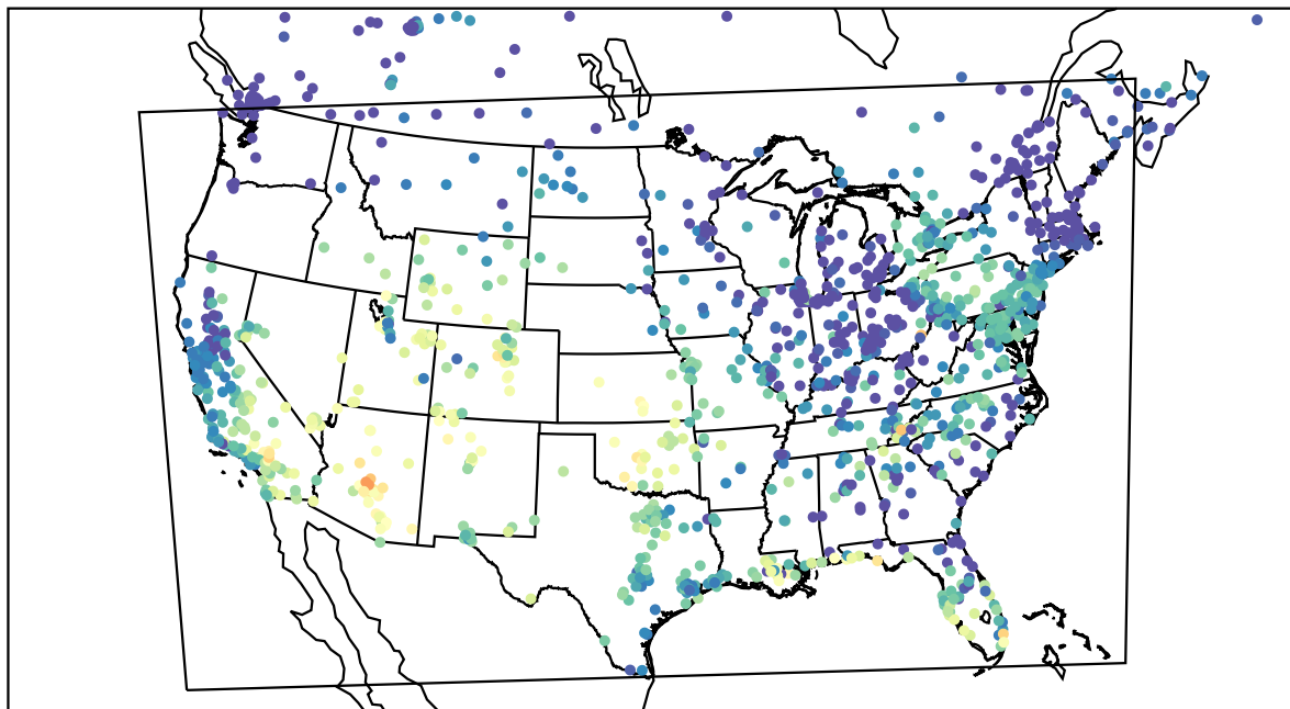
AirNOW (2023-10-23_00:00:00)
