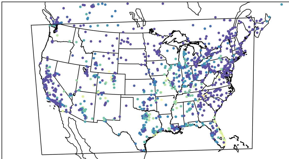
AirNOW (2023-10-24_11:00:00)
