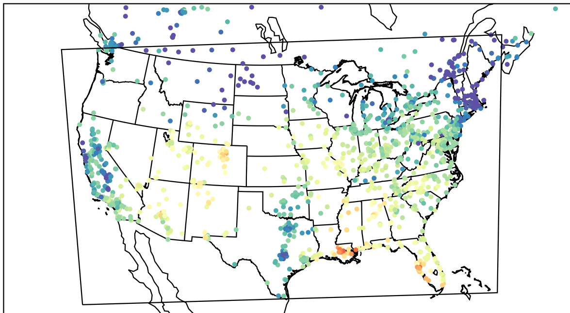
AirNOW (2023-10-23_21:00:00)
