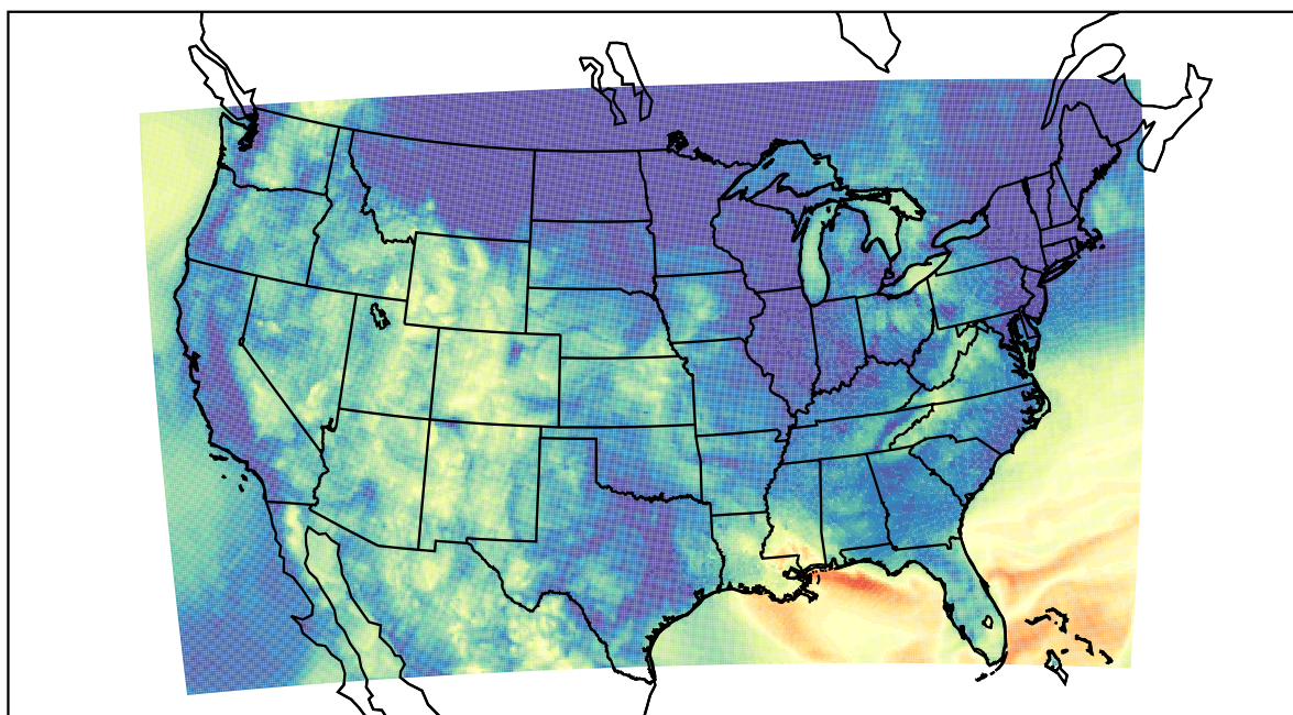
WRF (2023-10-23_11:00:00)
