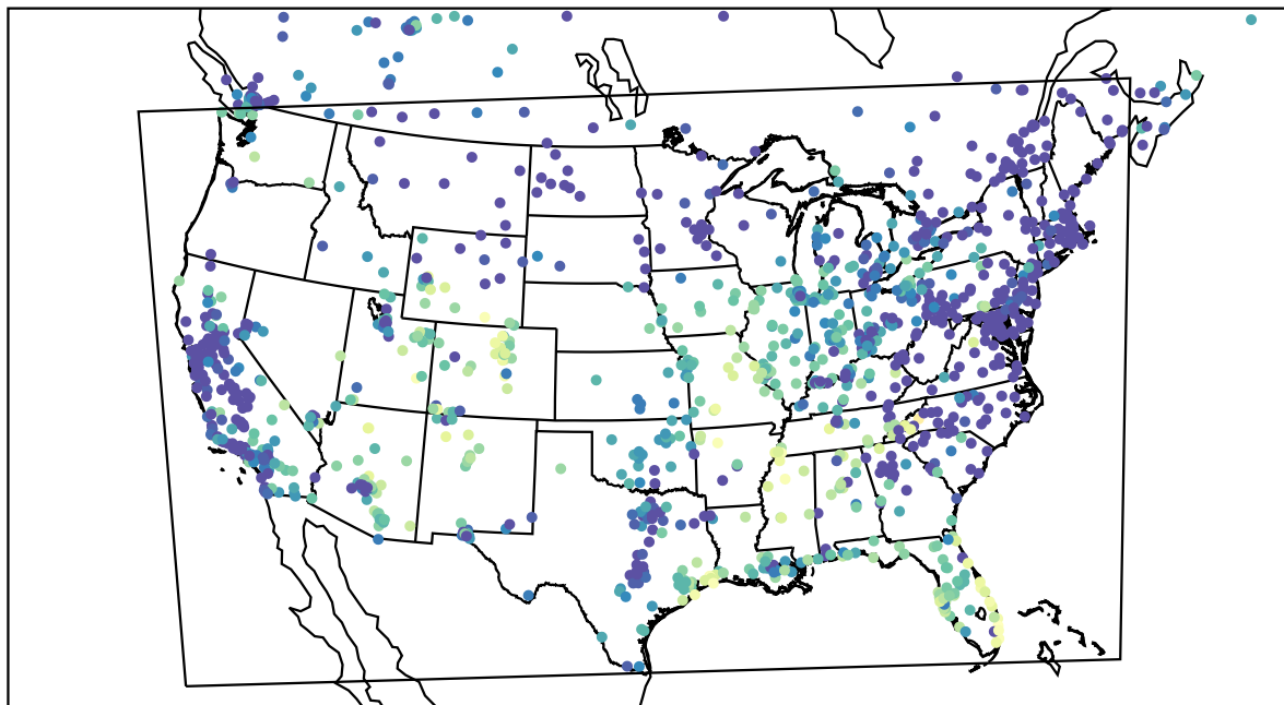
AirNOW (2023-10-24_04:00:00)
