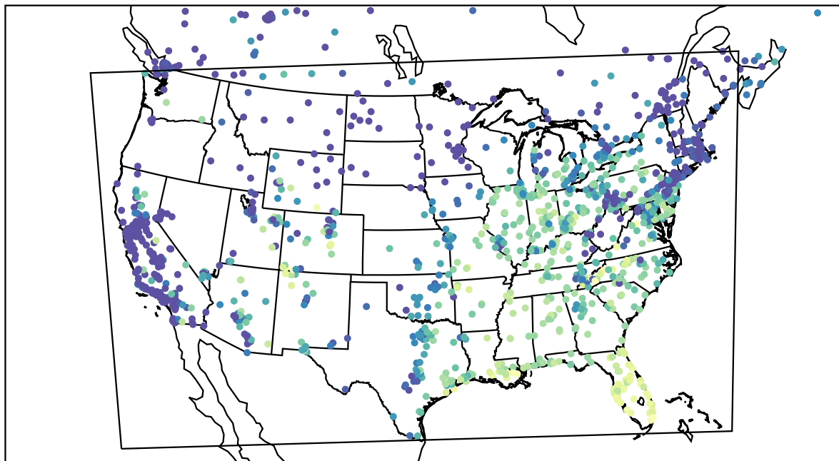
AirNOW (2023-10-24_15:00:00)
