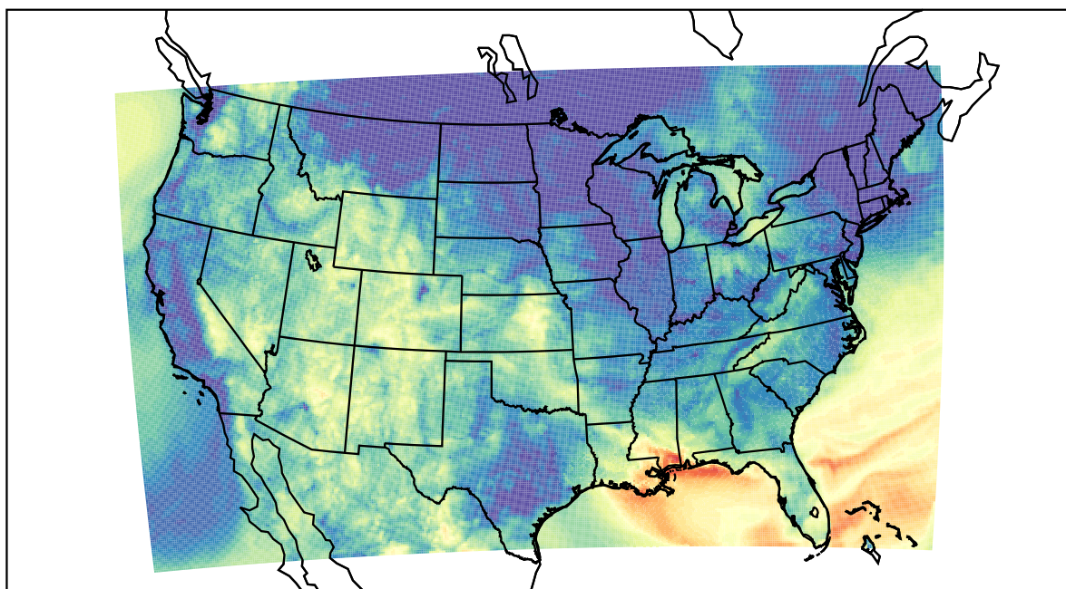
WRF (2023-10-23_07:00:00)
