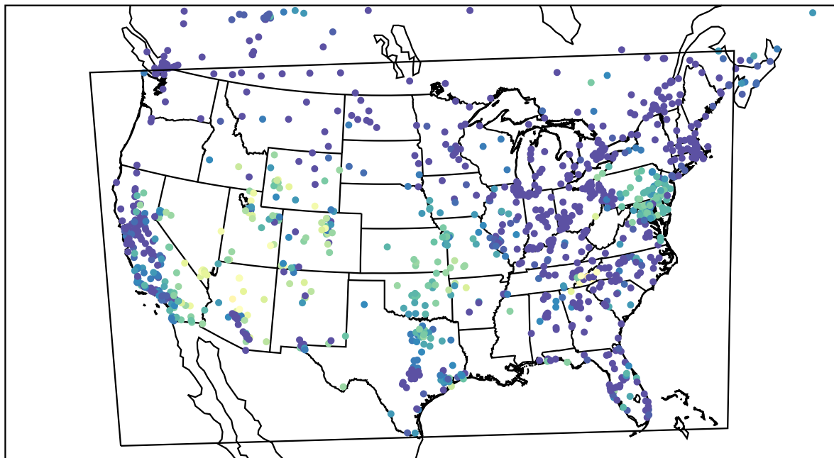
AirNOW (2023-10-23_07:00:00)
