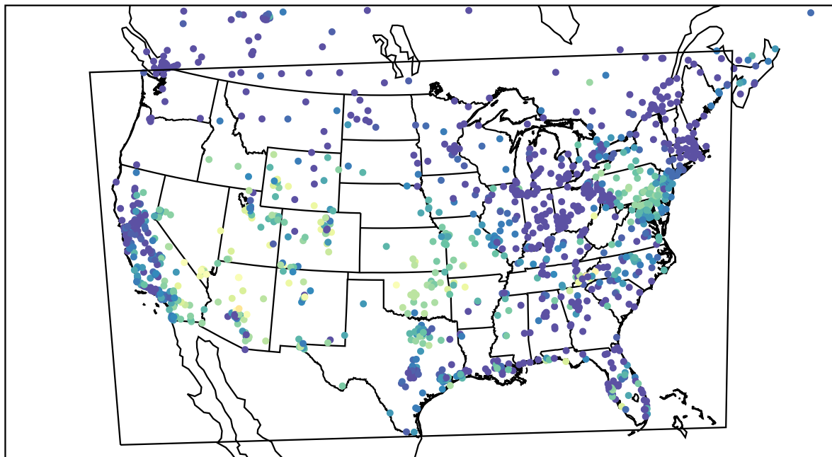
AirNOW (2023-10-23_04:00:00)
