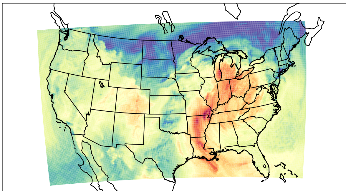
WRF (2023-10-24_21:00:00)
