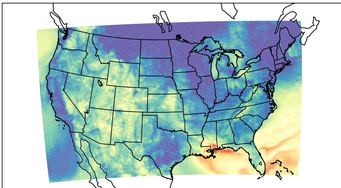
WRF (2023-10-23_08:00:00)
