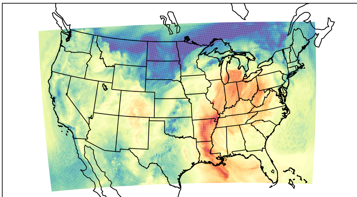
WRF (2023-10-24_19:00:00)
