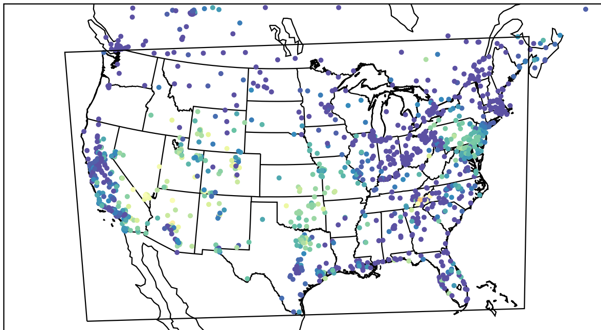
AirNOW (2023-10-23_05:00:00)
