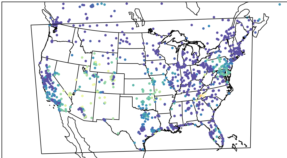
AirNOW (2023-10-23_08:00:00)
