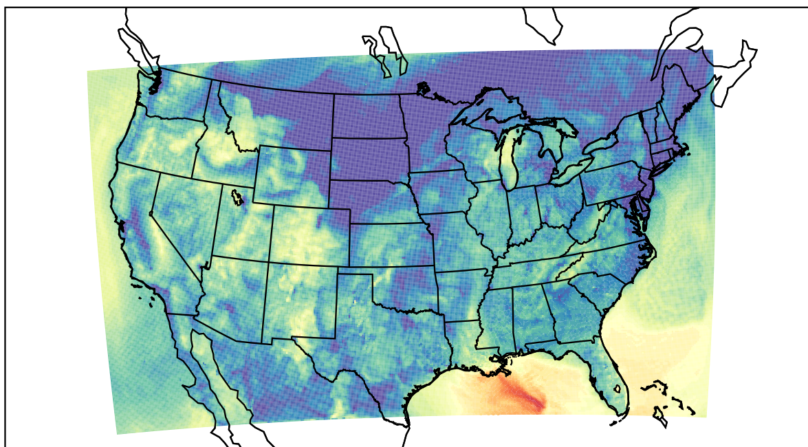
WRF (2023-10-24_13:00:00)
