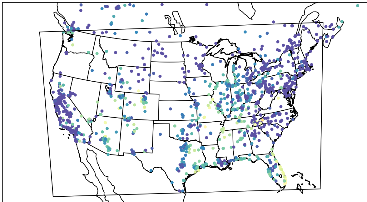
AirNOW (2023-10-24_09:00:00)
