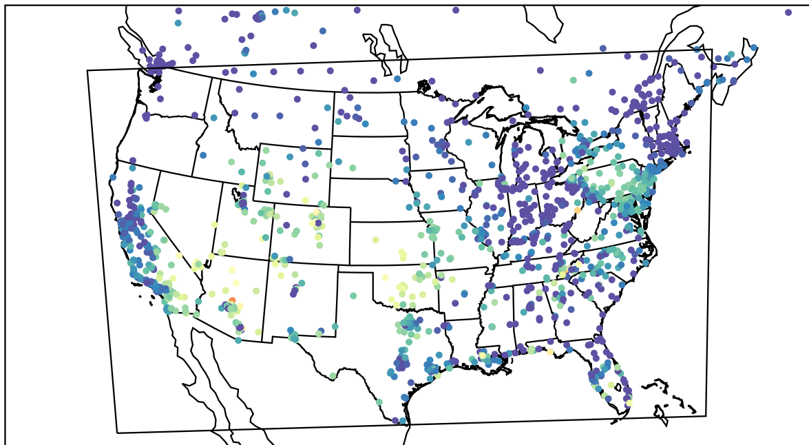
AirNOW (2023-10-23_02:00:00)
