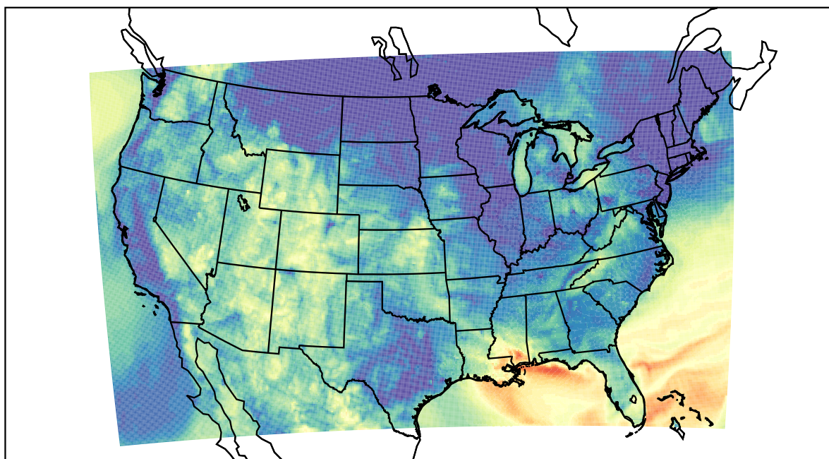
WRF (2023-10-23_09:00:00)
