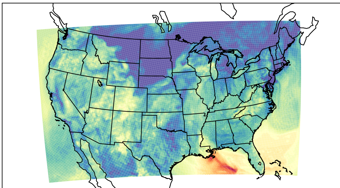
WRF (2023-10-24_09:00:00)
