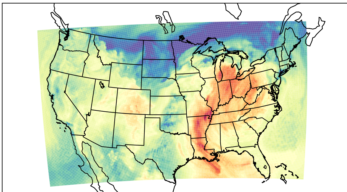
WRF (2023-10-24_20:00:00)
