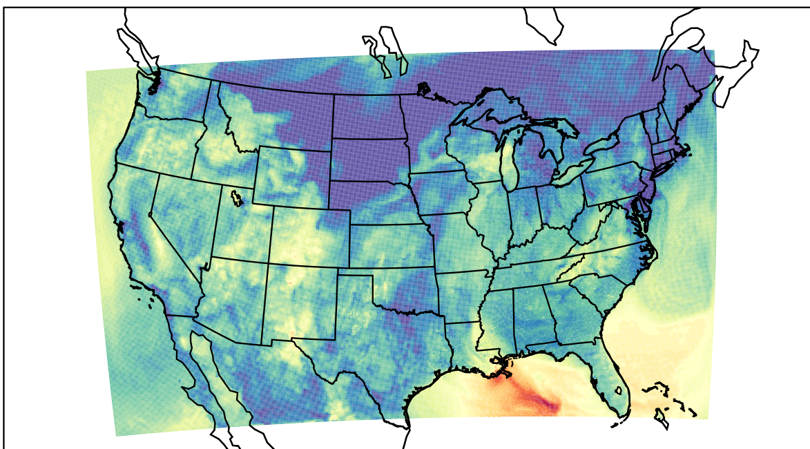
WRF (2023-10-24_10:00:00)
