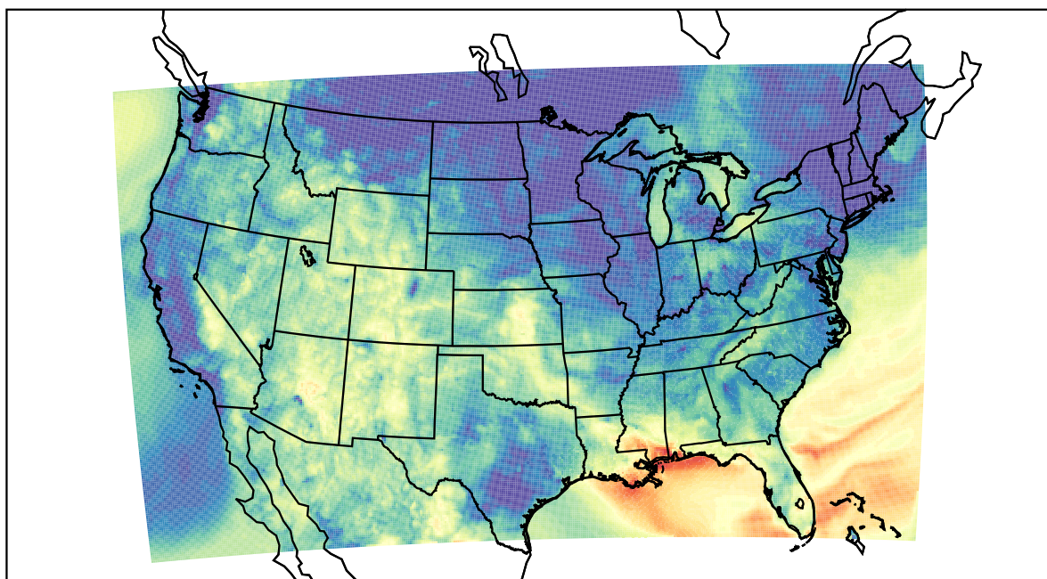
WRF (2023-10-23_05:00:00)
