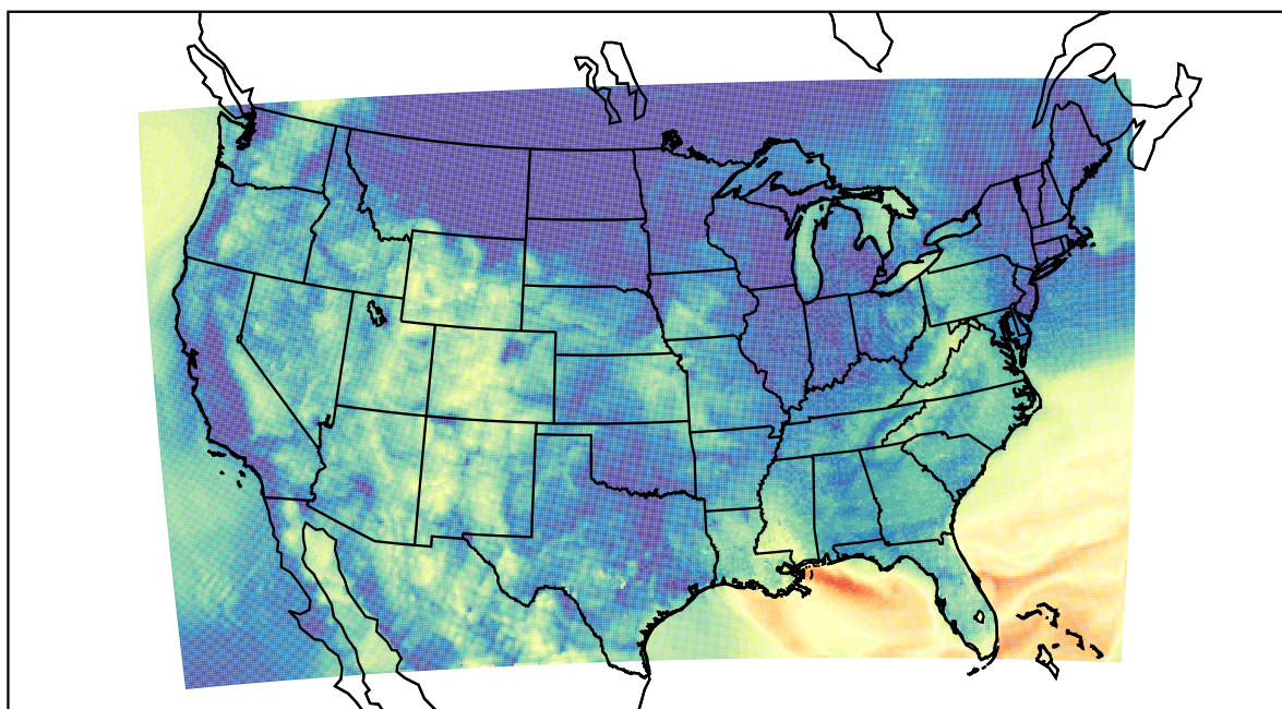
WRF (2023-10-23_14:00:00)
