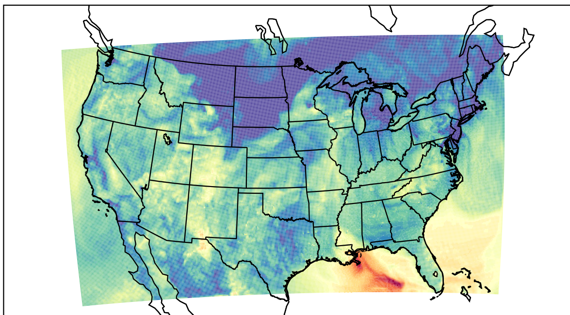
WRF (2023-10-24_07:00:00)
