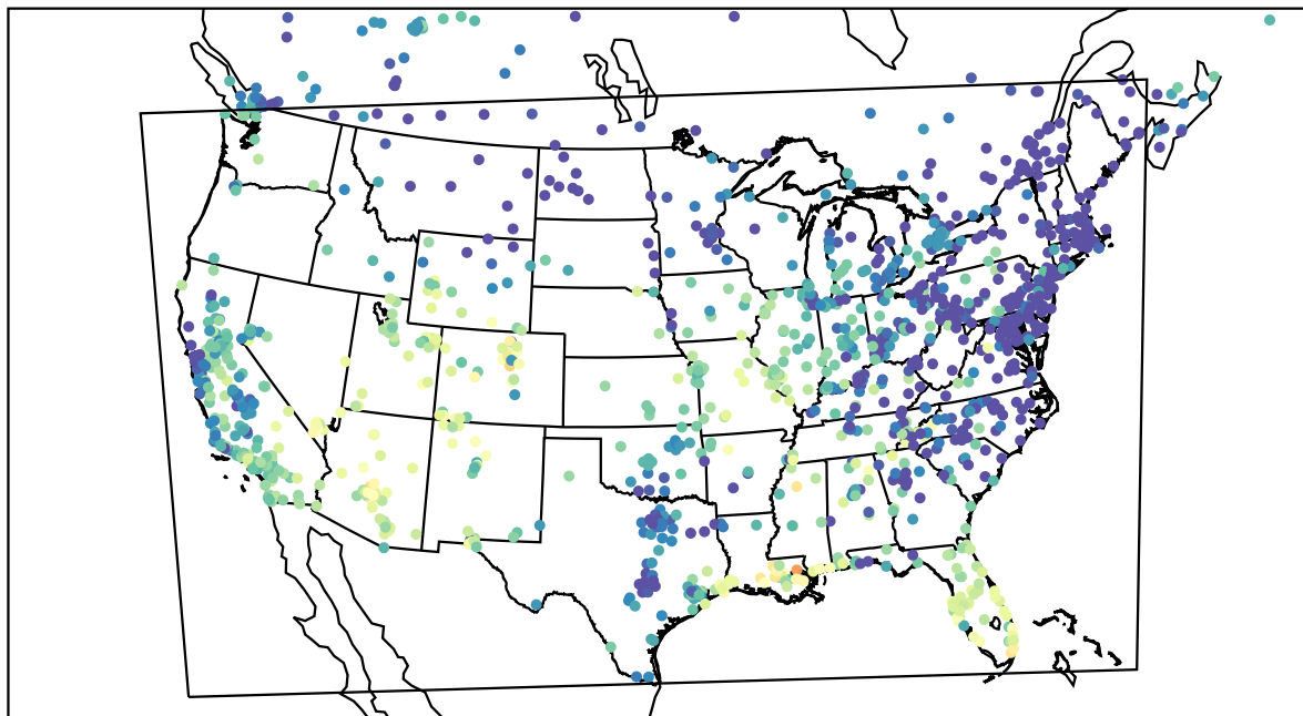
AirNOW (2023-10-24_00:00:00)
