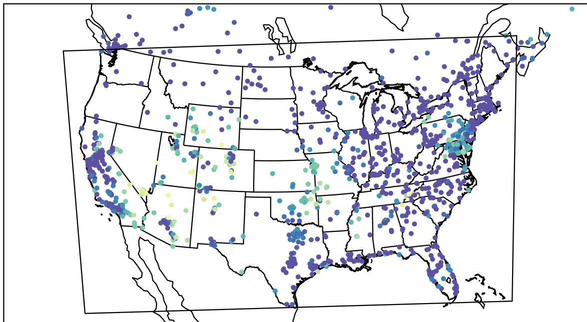
AirNOW (2023-10-23_10:00:00)
