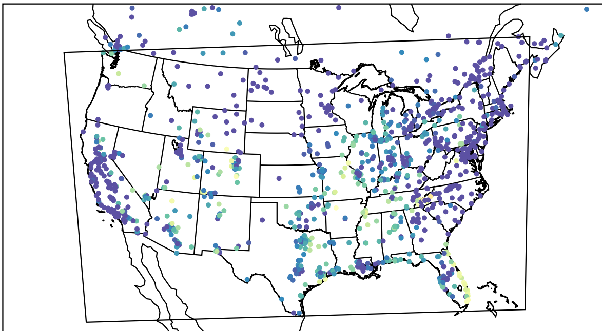
AirNOW (2023-10-24_10:00:00)
