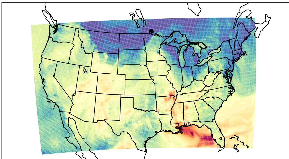
WRF (2023-10-23_23:00:00)
