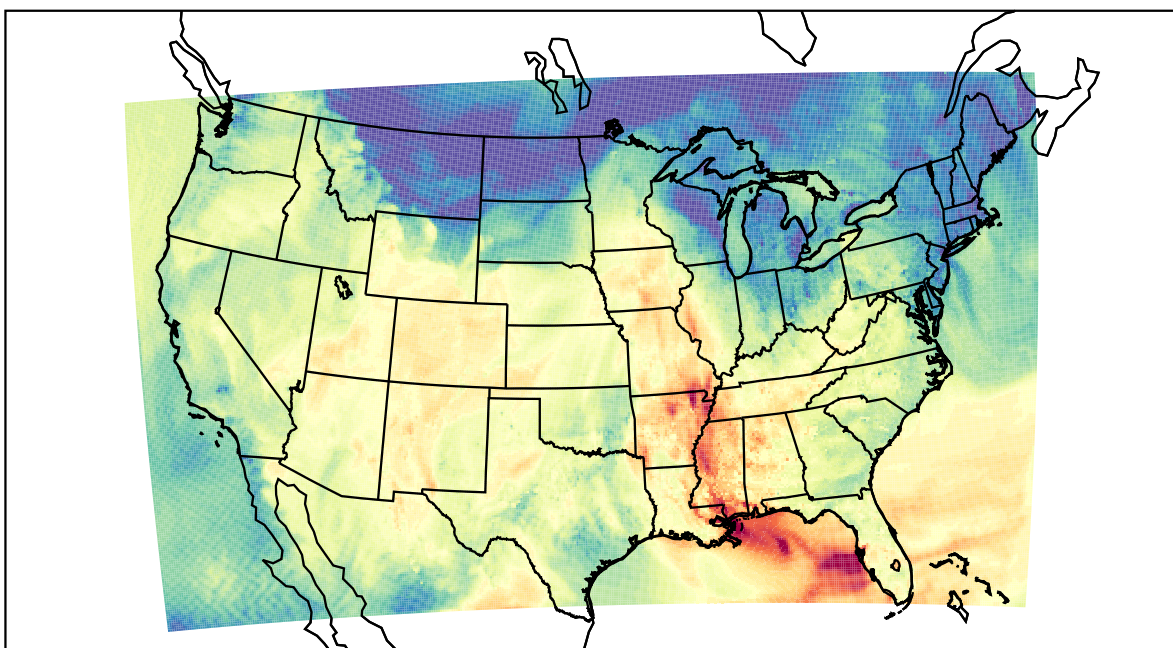
WRF (2023-10-23_22:00:00)
