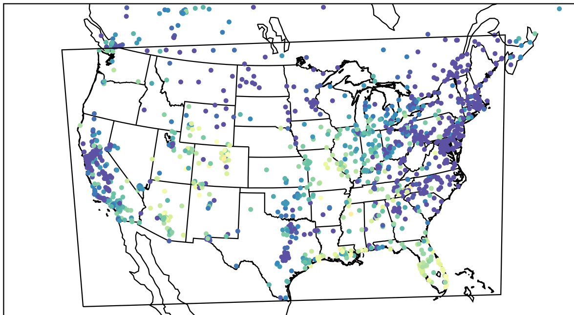
AirNOW (2023-10-24_02:00:00)
