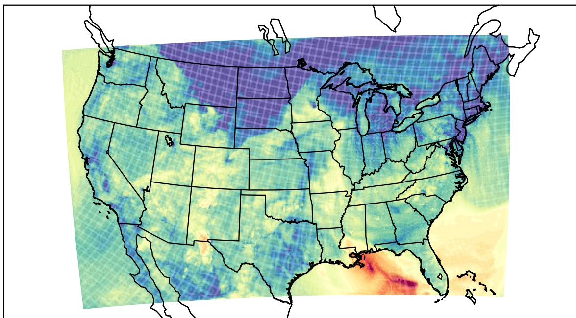
WRF (2023-10-24_04:00:00)
