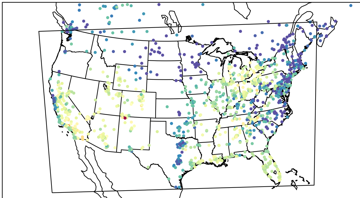
AirNOW (2023-10-24_23:00:00)
