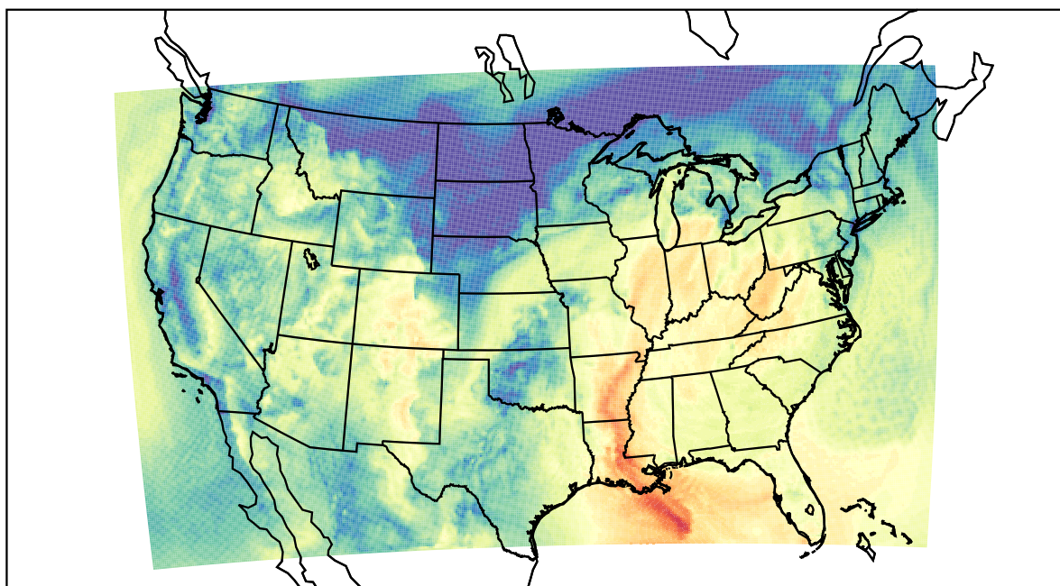
WRF (2023-10-24_17:00:00)
