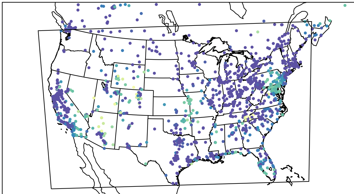
AirNOW (2023-10-23_13:00:00)
