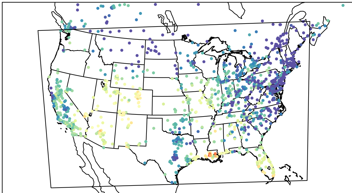
AirNOW (2023-10-23_23:00:00)
