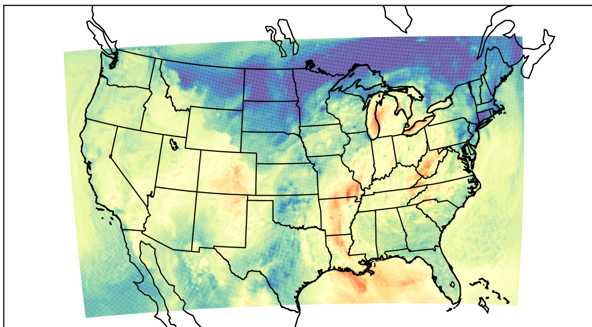
WRF (2023-10-24_23:00:00)
