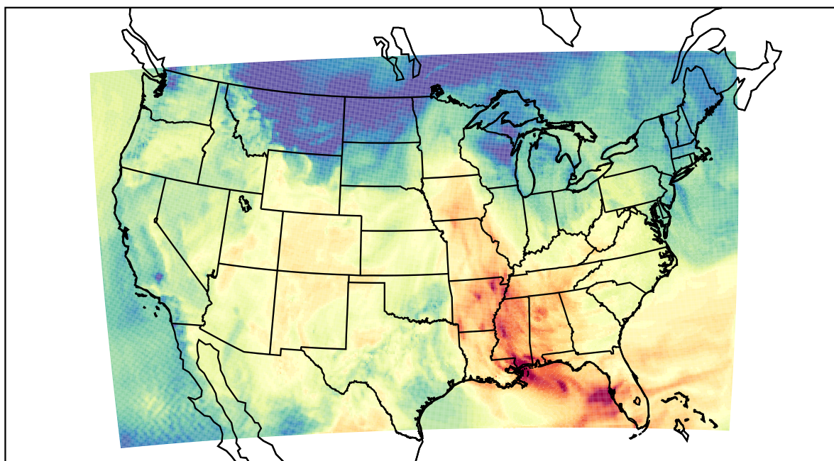
WRF (2023-10-23_20:00:00)
