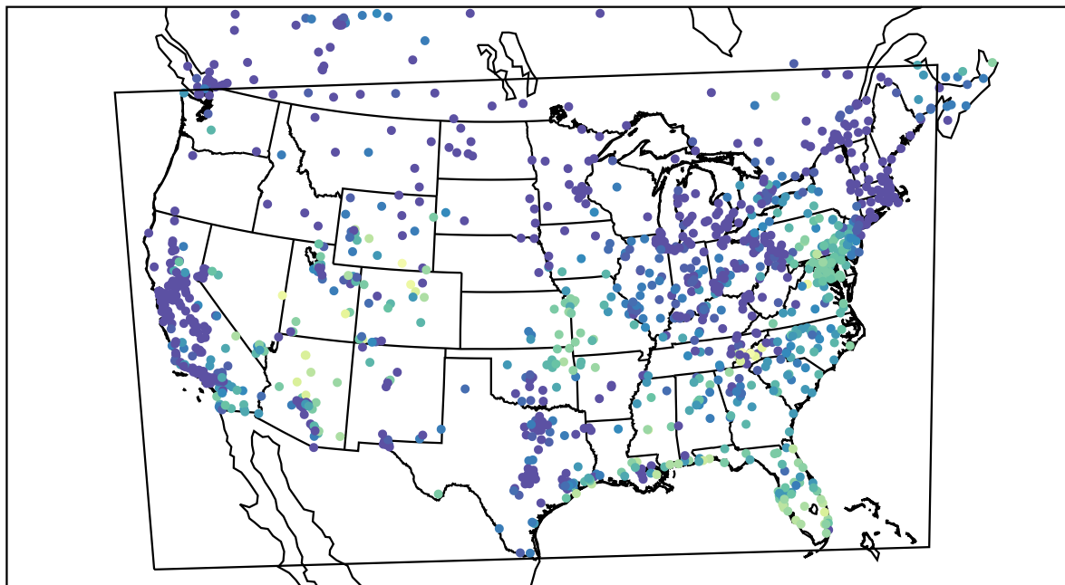
AirNOW (2023-10-23_14:00:00)
