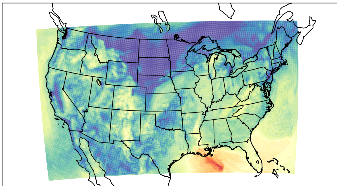
WRF (2023-10-24_15:00:00)
