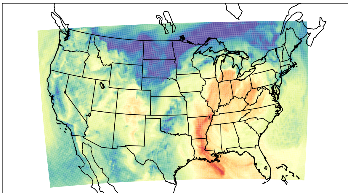
WRF (2023-10-24_18:00:00)
