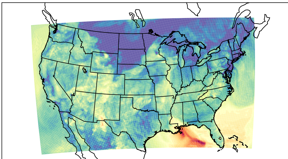
WRF (2023-10-24_06:00:00)
