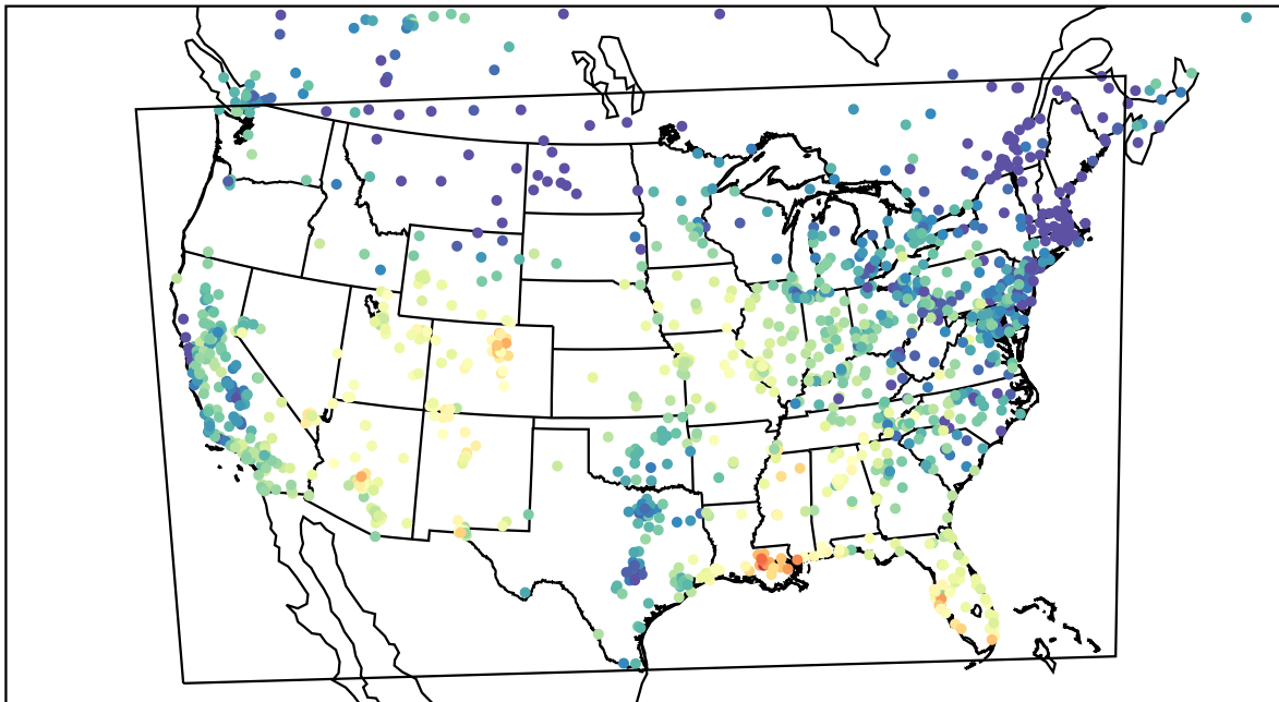
AirNOW (2023-10-23_22:00:00)
