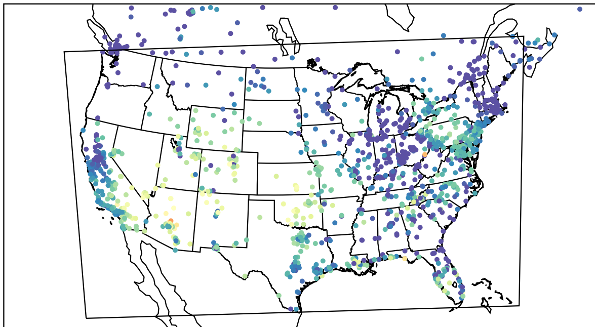
AirNOW (2023-10-23_01:00:00)
