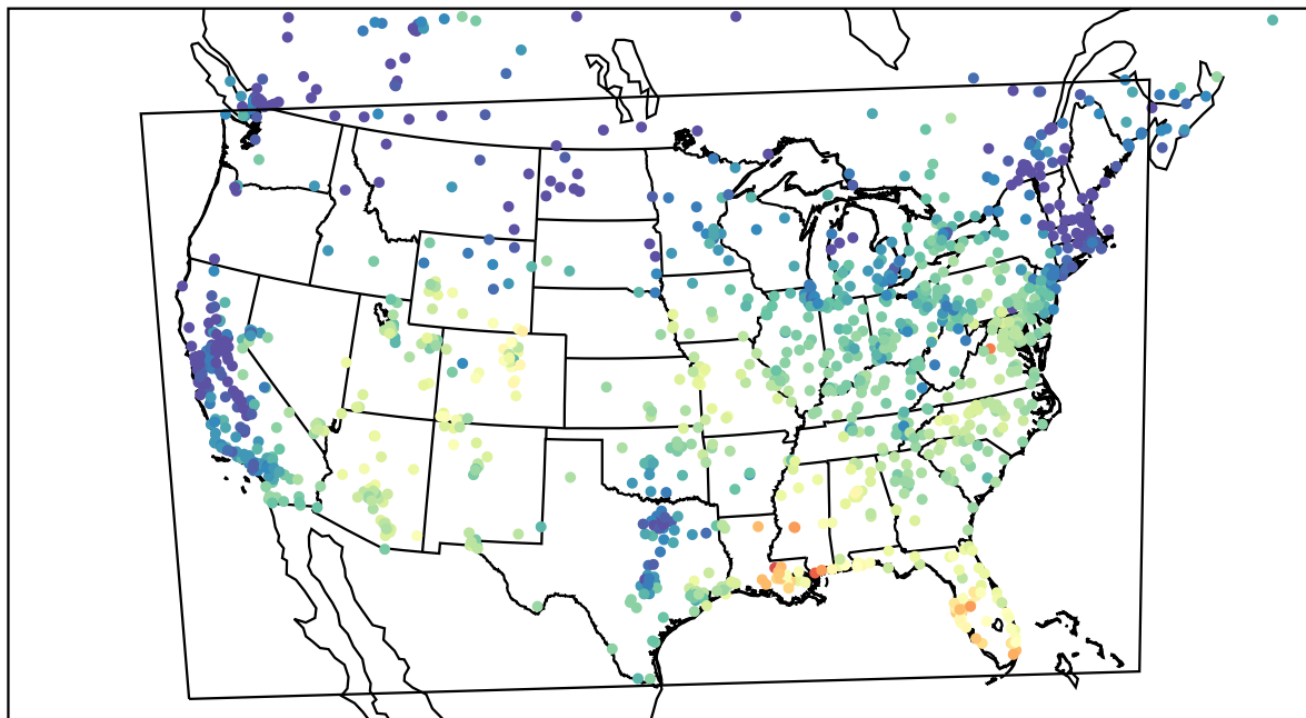
AirNOW (2023-10-23_17:00:00)
