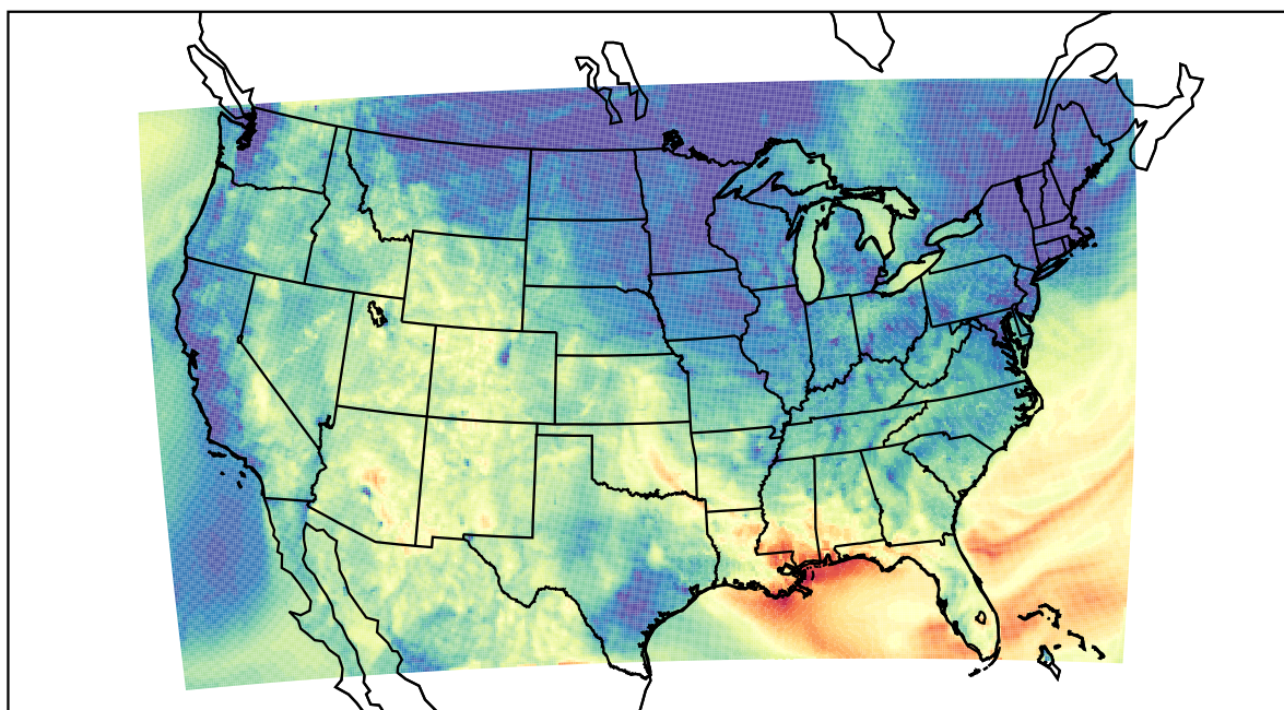
WRF (2023-10-23_02:00:00)
