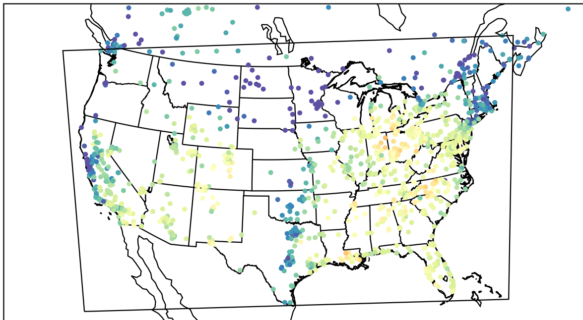
AirNOW (2023-10-24_19:00:00)
