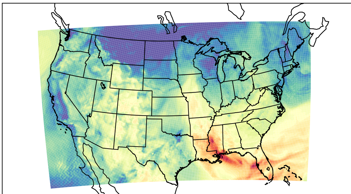
WRF (2023-10-23_17:00:00)
