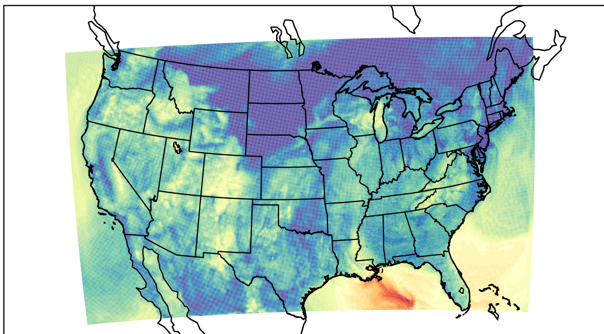
WRF (2023-10-24_11:00:00)
