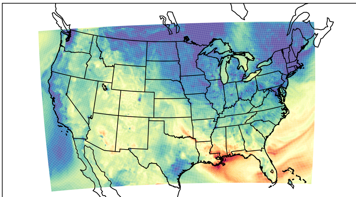
WRF (2023-10-23_01:00:00)
