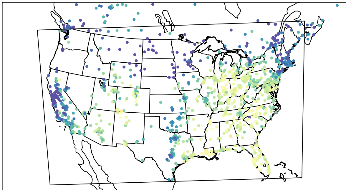
AirNOW (2023-10-24_17:00:00)
