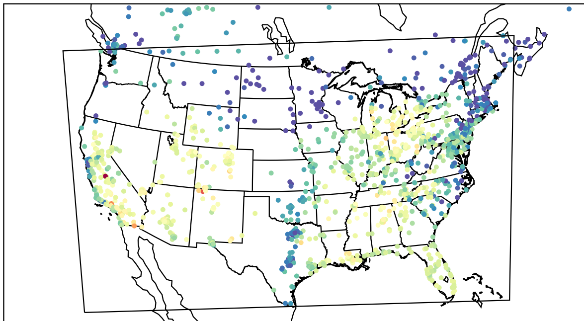
AirNOW (2023-10-24_22:00:00)
