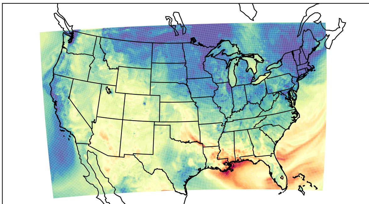
WRF (2023-10-23_00:00:00)
