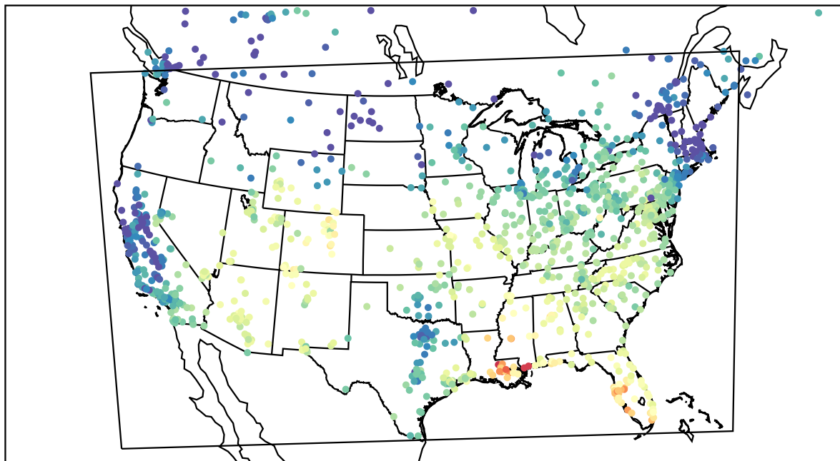
AirNOW (2023-10-23_18:00:00)
