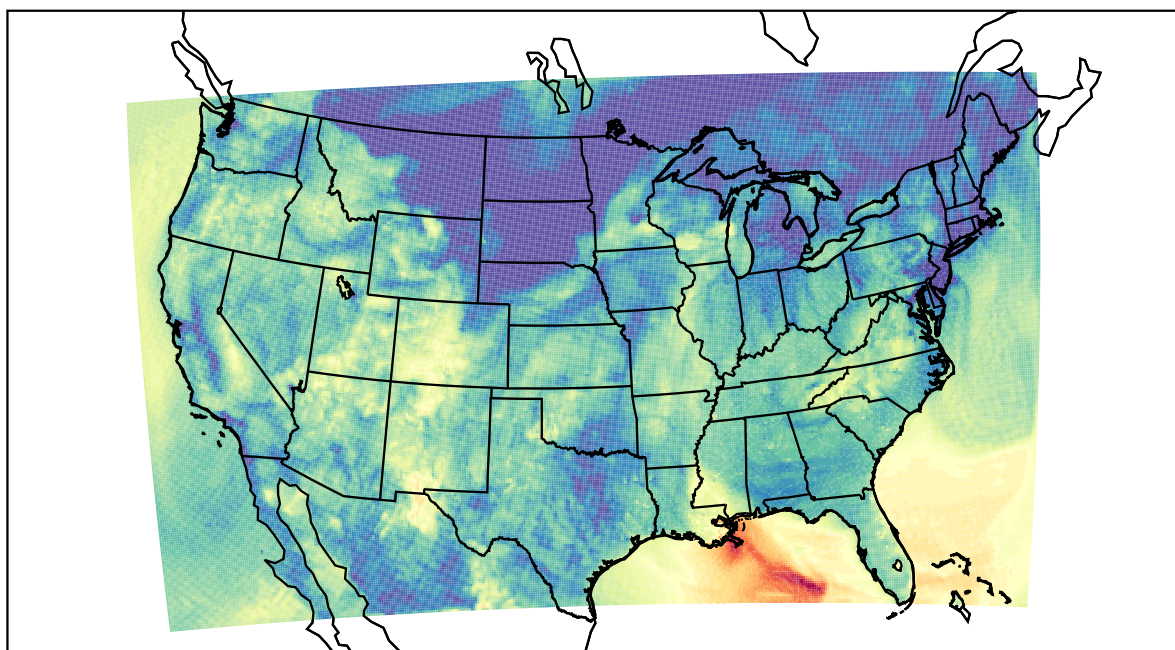
WRF (2023-10-24_08:00:00)
