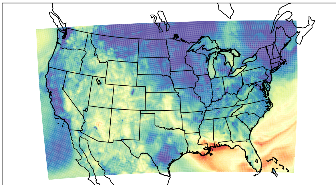
WRF (2023-10-23_04:00:00)
