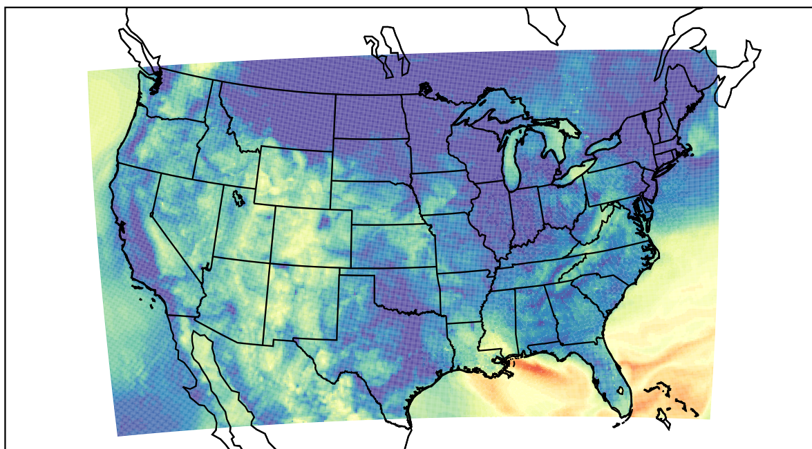
WRF (2023-10-23_13:00:00)
