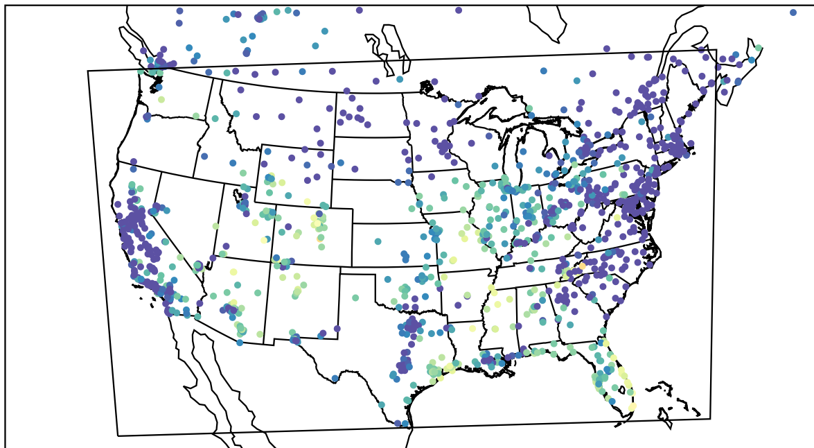
AirNOW (2023-10-24_05:00:00)
