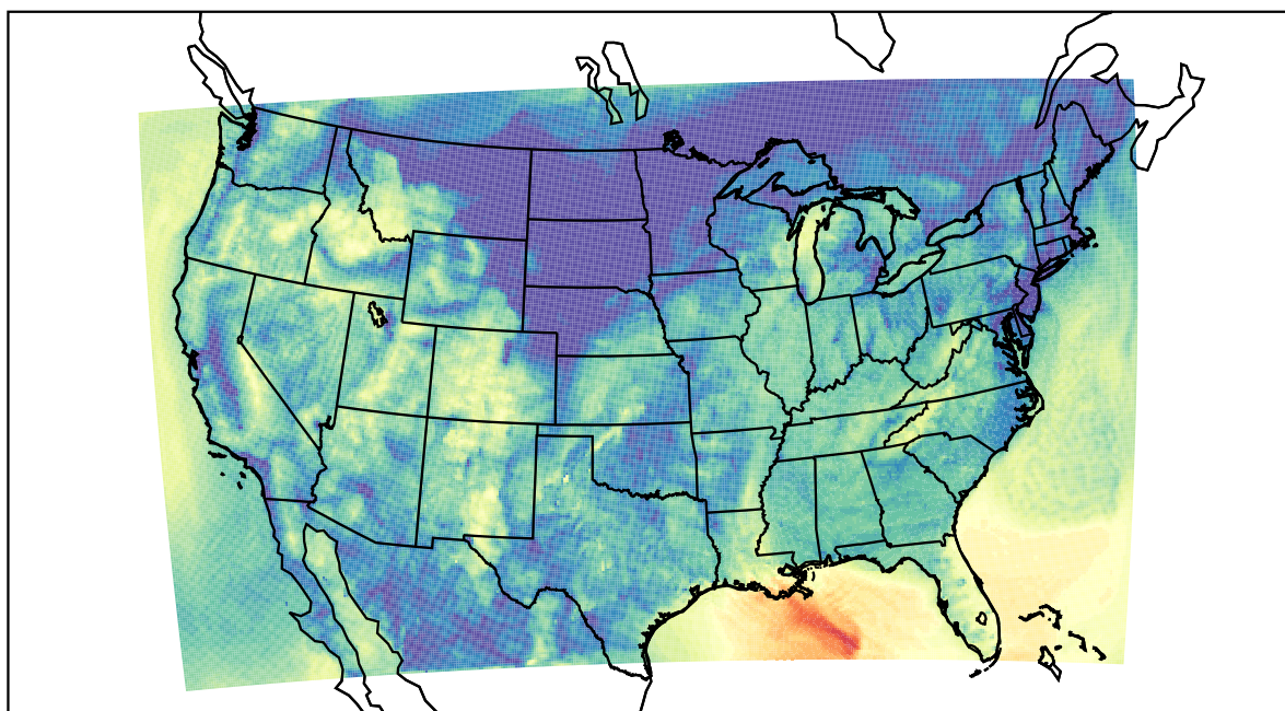
WRF (2023-10-24_14:00:00)
