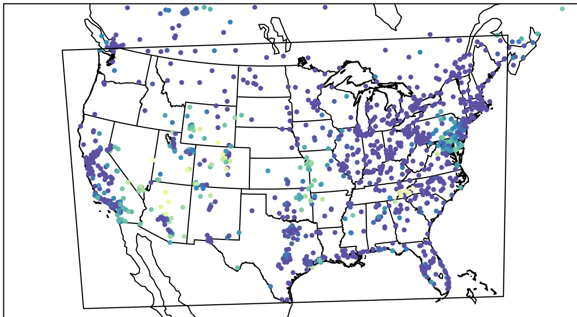
AirNOW (2023-10-23_12:00:00)
