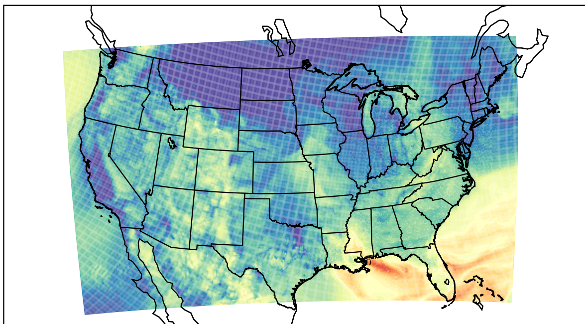
WRF (2023-10-23_15:00:00)
