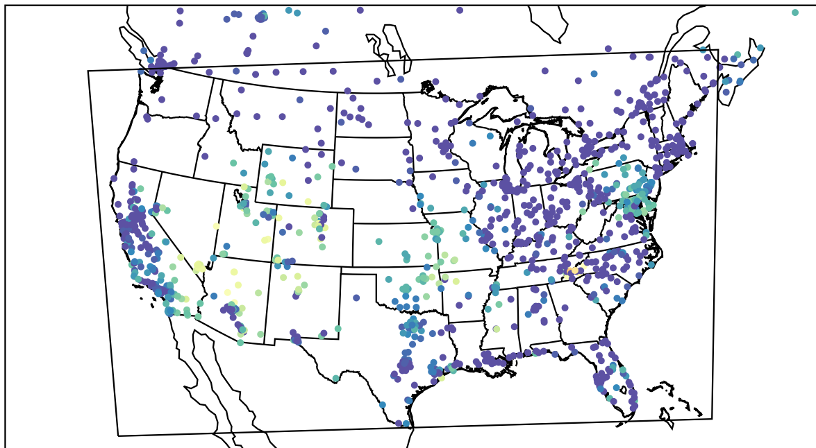
AirNOW (2023-10-23_09:00:00)
