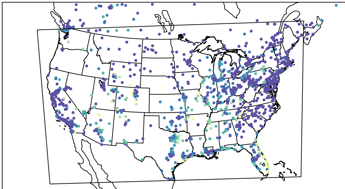
AirNOW (2023-10-24_12:00:00)
