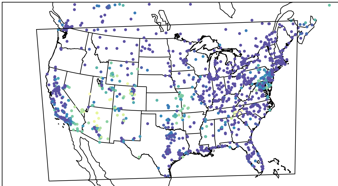
AirNOW (2023-10-23_11:00:00)
