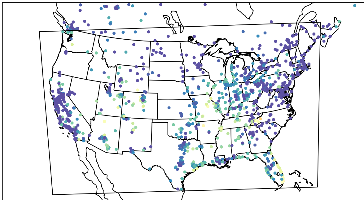
AirNOW (2023-10-24_08:00:00)
