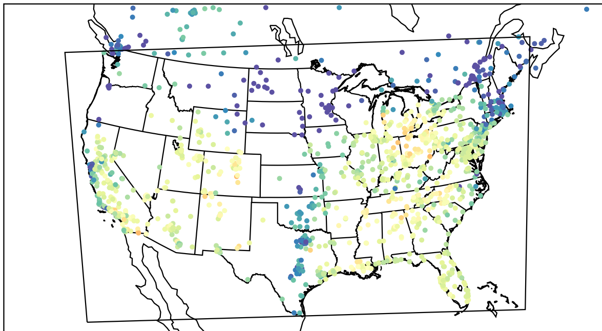
AirNOW (2023-10-24_21:00:00)
