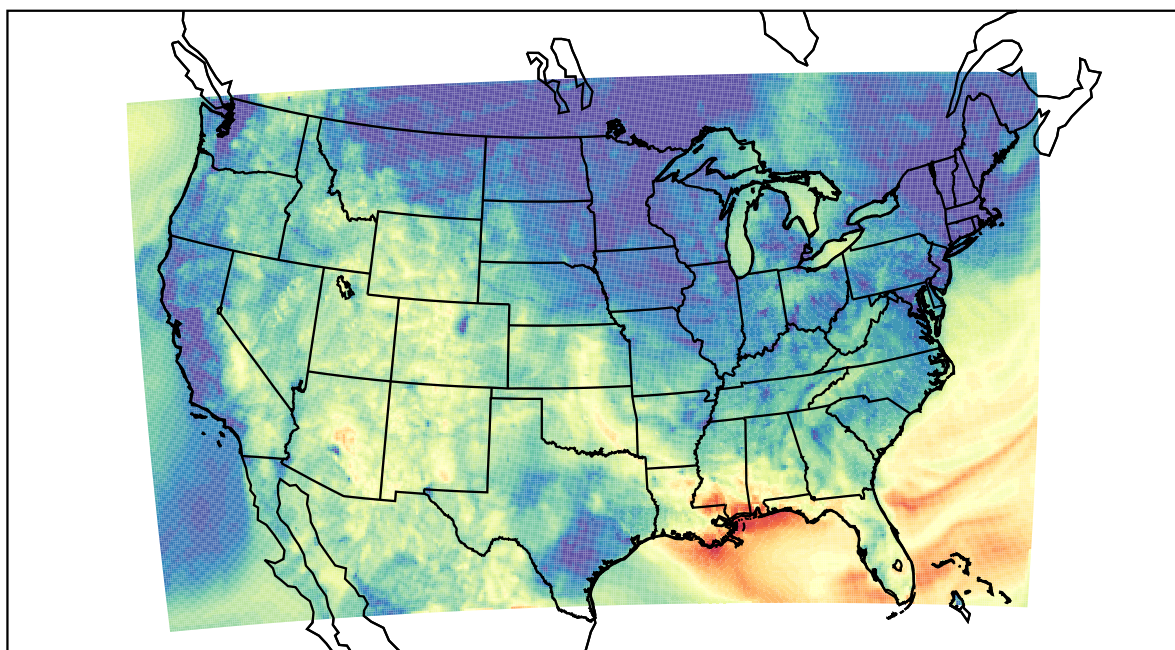
WRF (2023-10-23_03:00:00)
