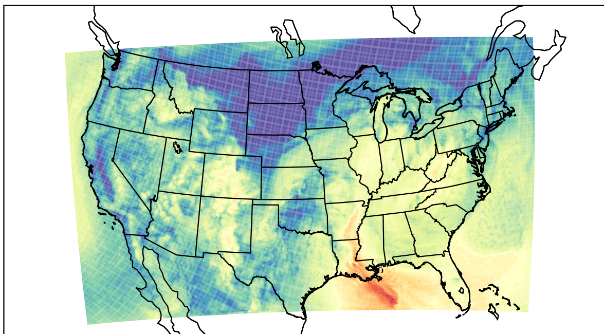
WRF (2023-10-24_16:00:00)
