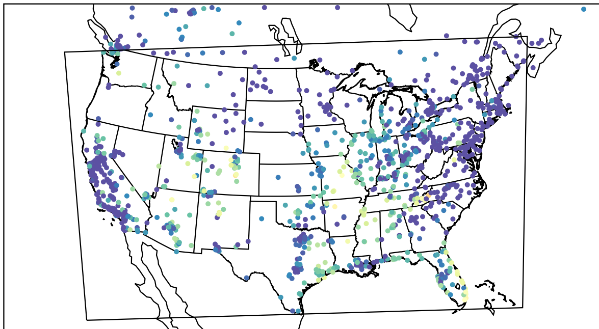
AirNOW (2023-10-24_07:00:00)
