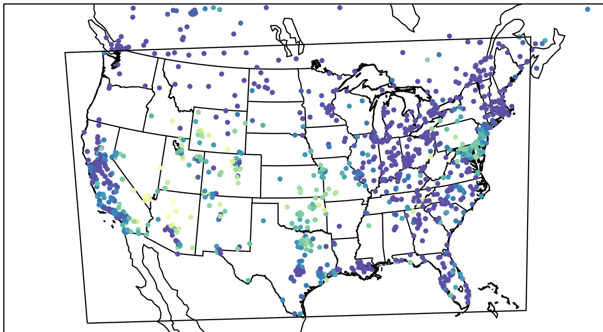
AirNOW (2023-10-23_06:00:00)
