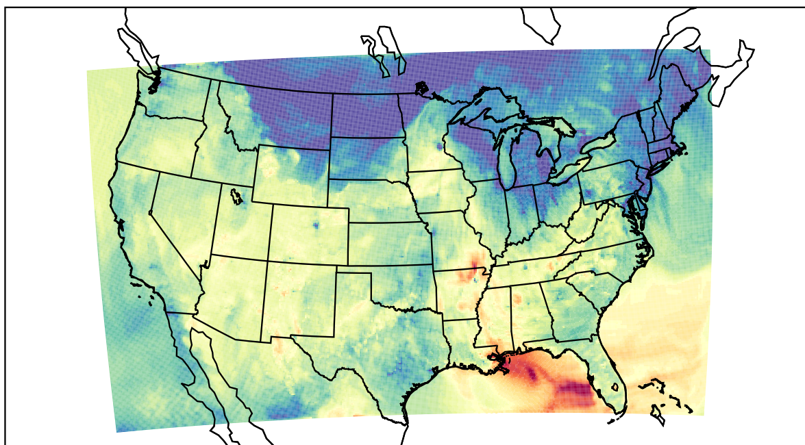
WRF (2023-10-24_00:00:00)
