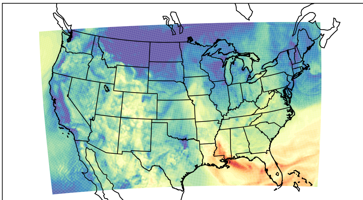
WRF (2023-10-23_16:00:00)
