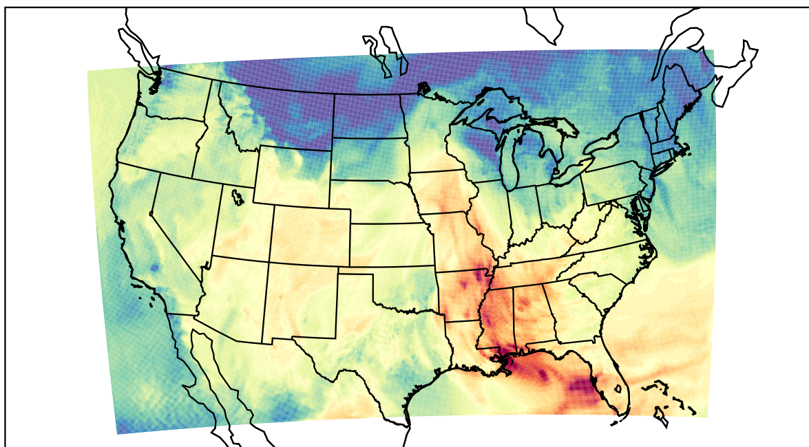
WRF (2023-10-23_21:00:00)
