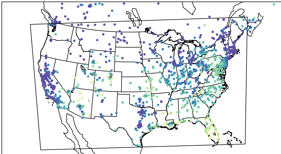
AirNOW (2023-10-23_15:00:00)
