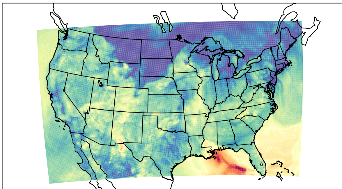
WRF (2023-10-24_05:00:00)
