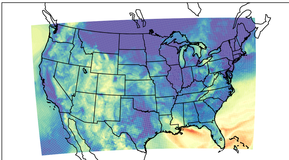
WRF (2023-10-23_12:00:00)
