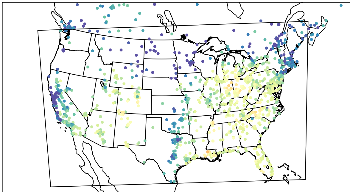
AirNOW (2023-10-24_18:00:00)
