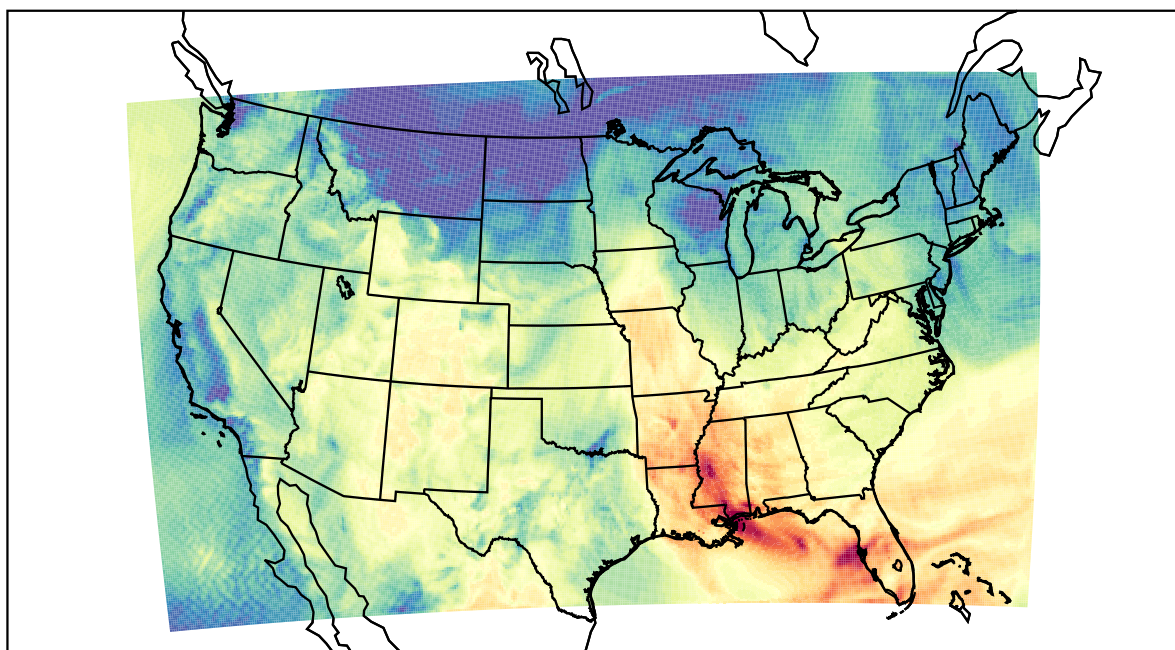
WRF (2023-10-23_18:00:00)
