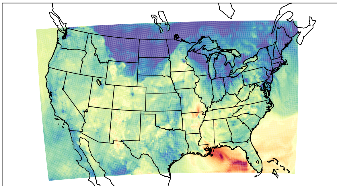
WRF (2023-10-24_01:00:00)
