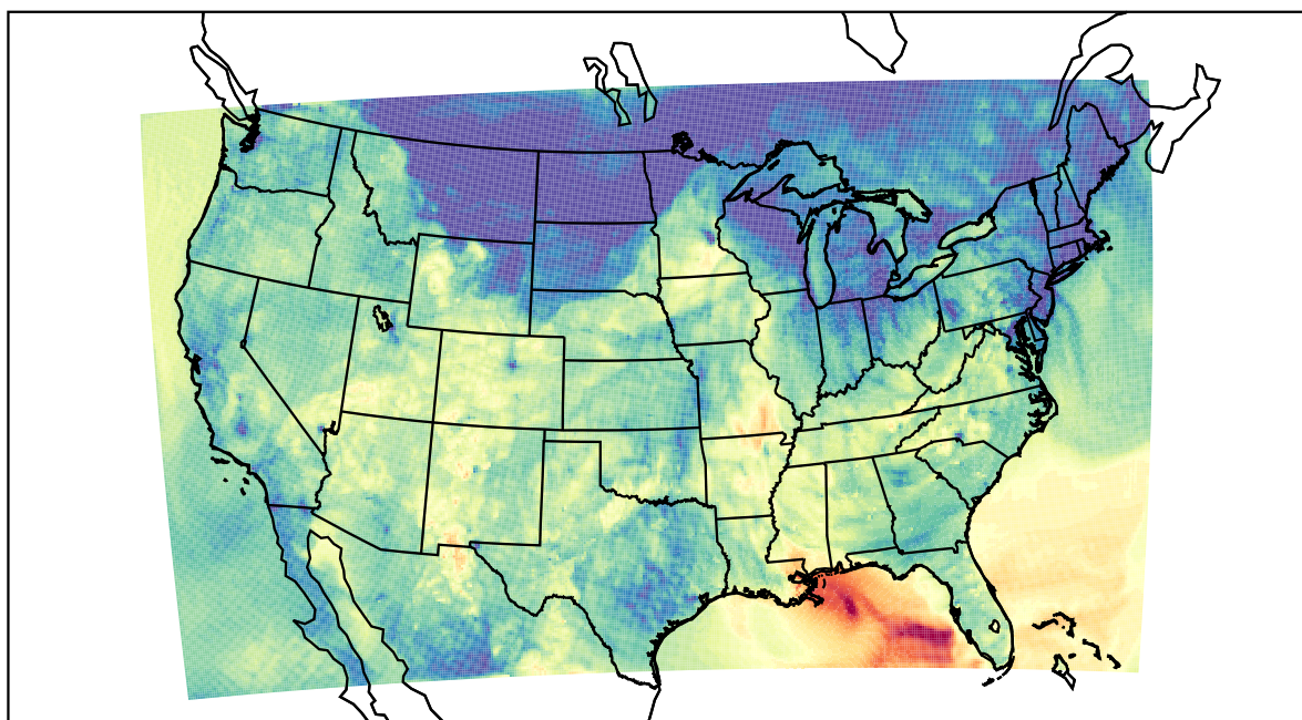
WRF (2023-10-24_02:00:00)
