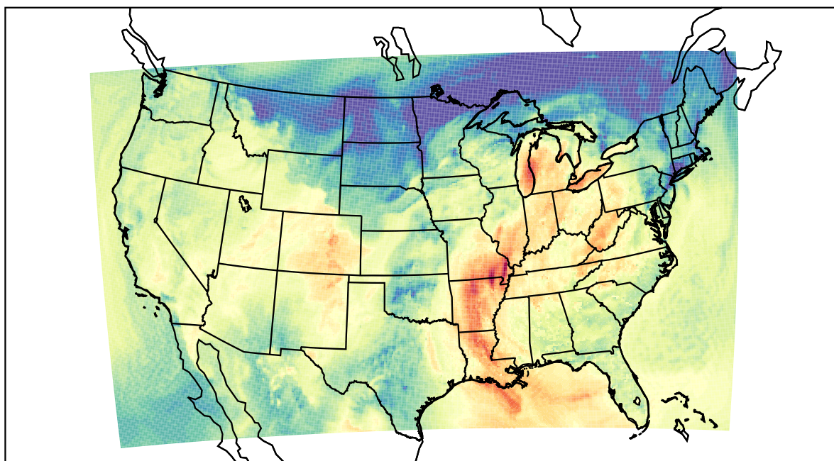
WRF (2023-10-24_22:00:00)
