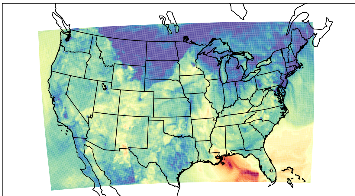
WRF (2023-10-24_03:00:00)
