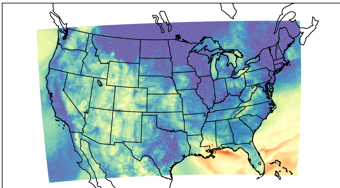
WRF (2023-10-23_10:00:00)
