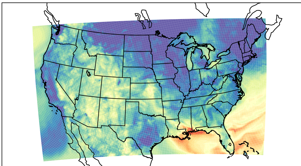
WRF (2023-10-23_06:00:00)
