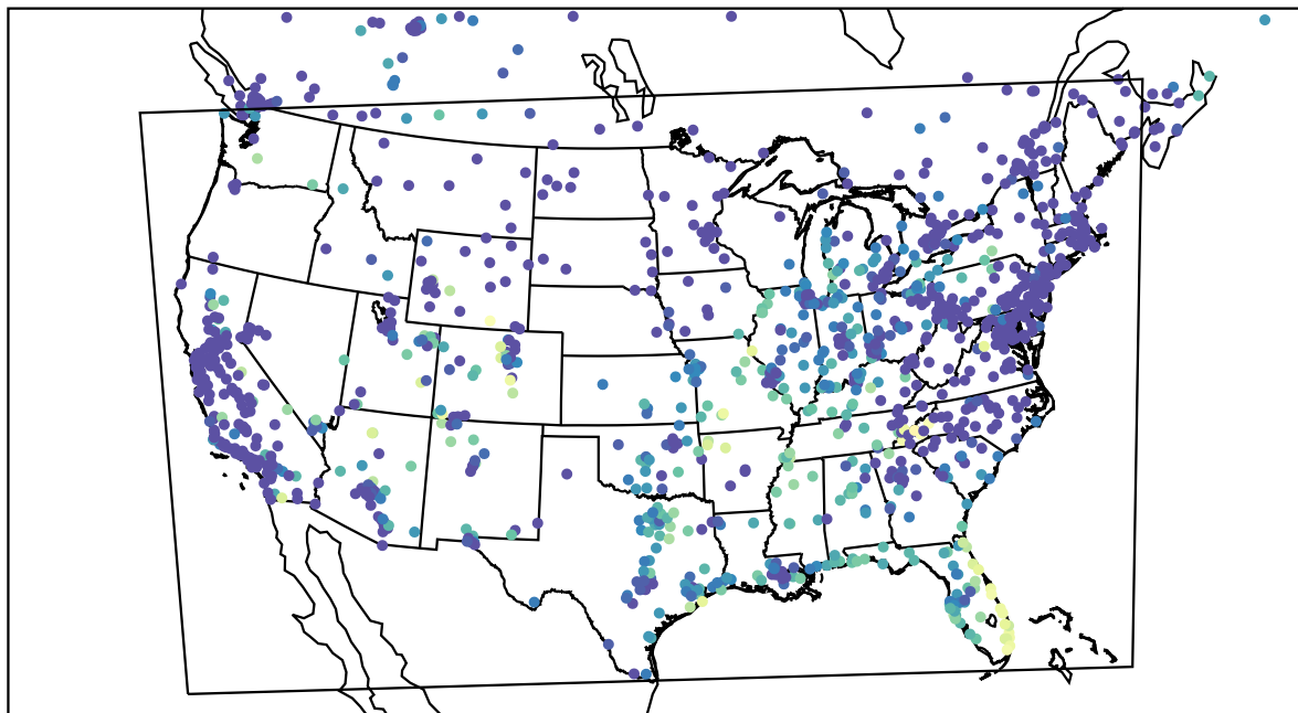
AirNOW (2023-10-24_13:00:00)
