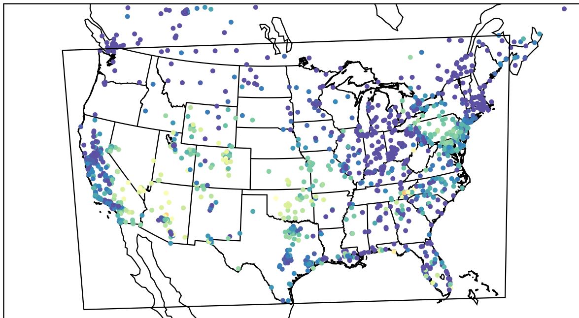
AirNOW (2023-10-23_03:00:00)
