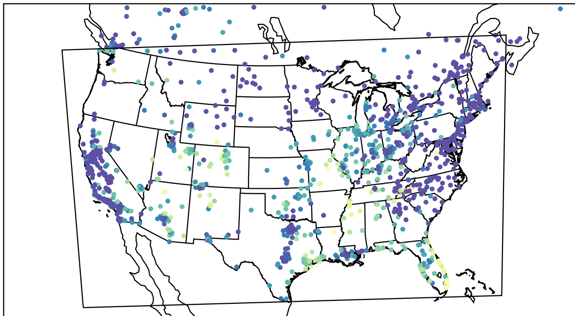
AirNOW (2023-10-24_06:00:00)
