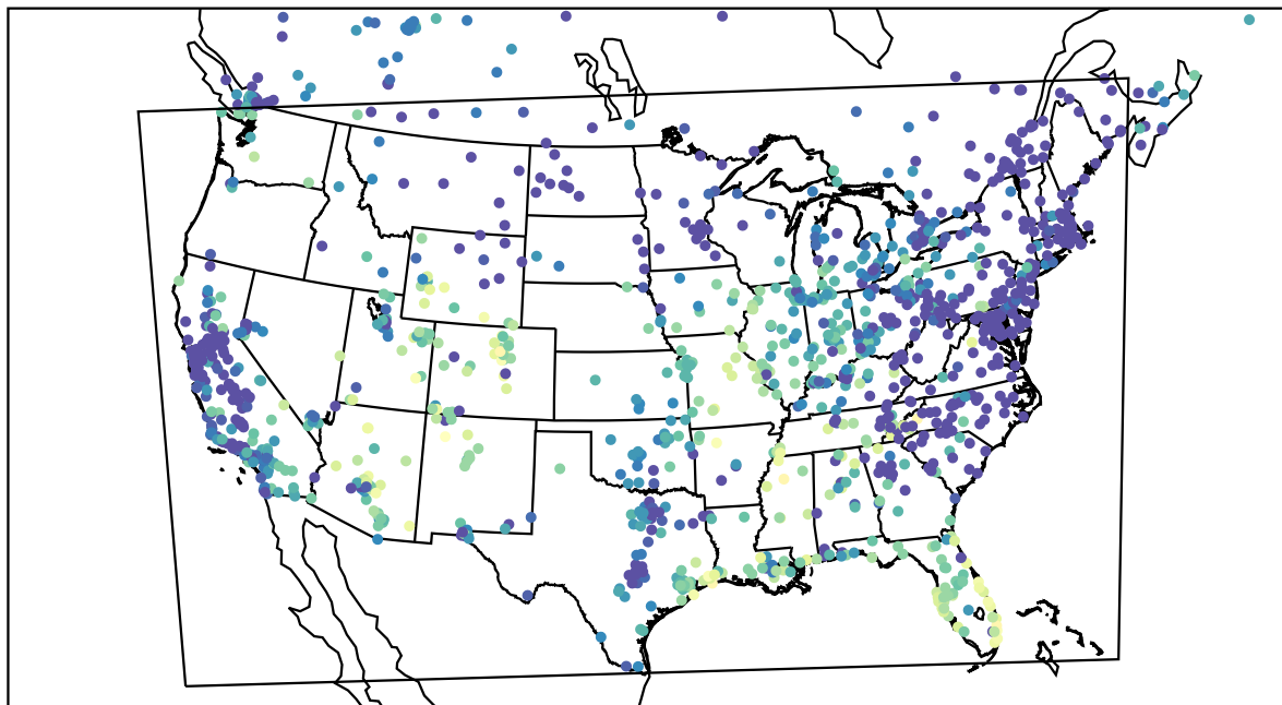
AirNOW (2023-10-24_03:00:00)
