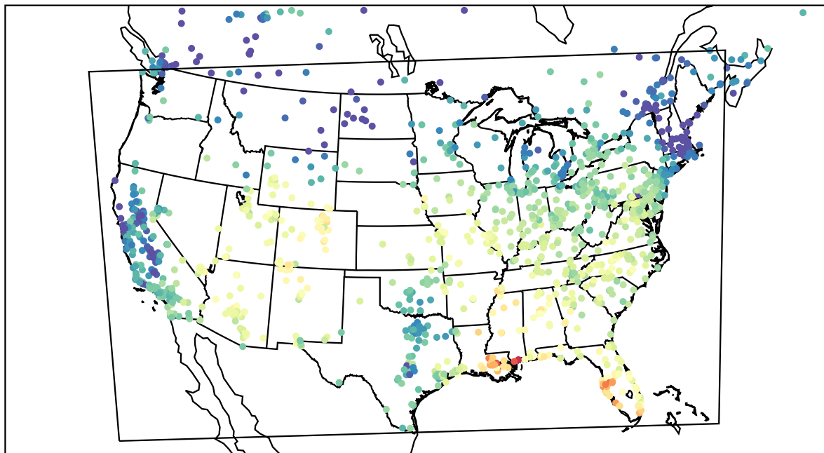
AirNOW (2023-10-23_19:00:00)
