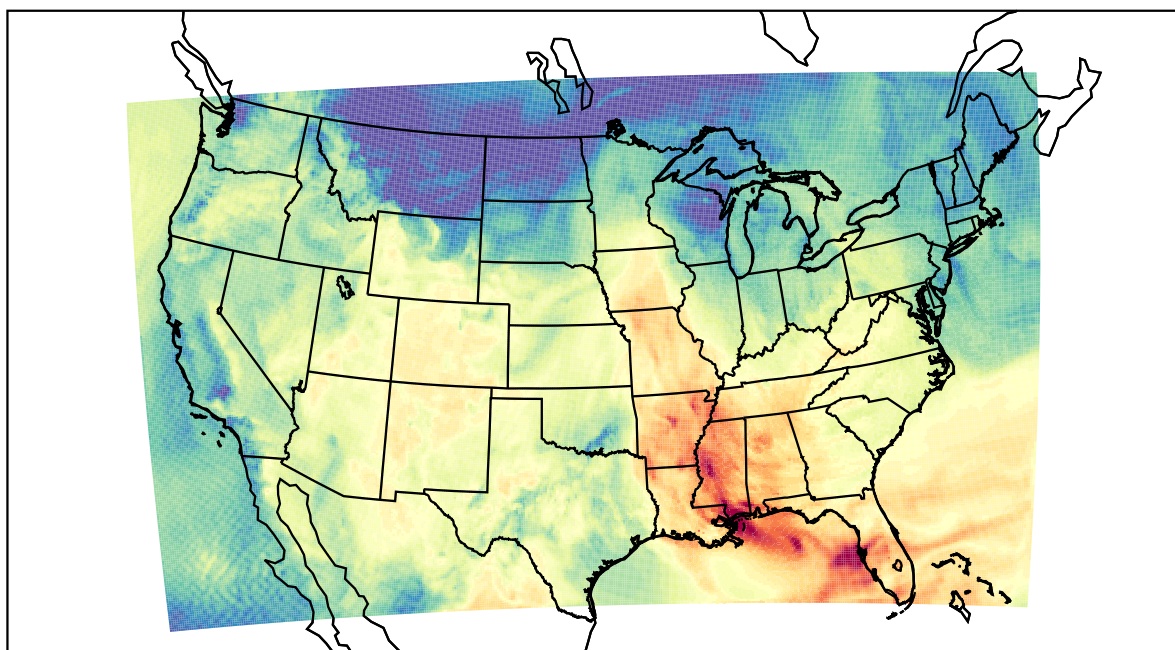
WRF (2023-10-23_19:00:00)
