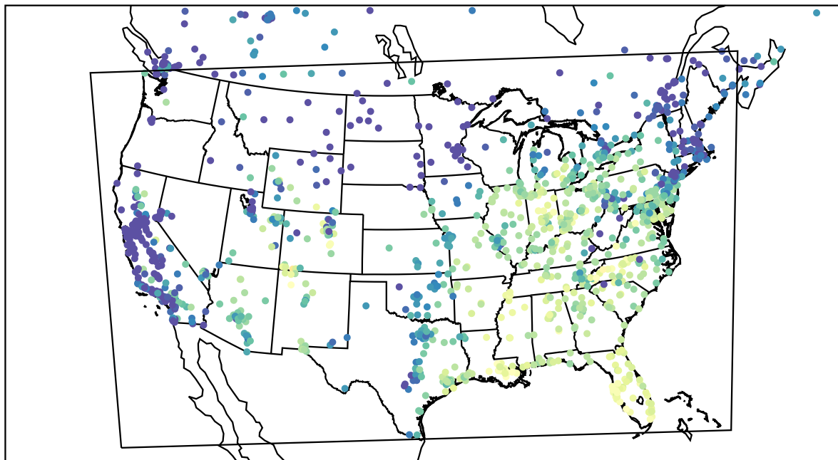
AirNOW (2023-10-24_16:00:00)
