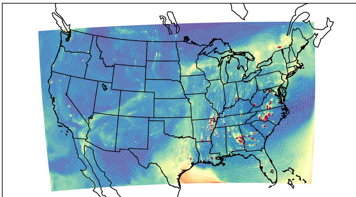
WRF 2023-10-26_23:00:00
