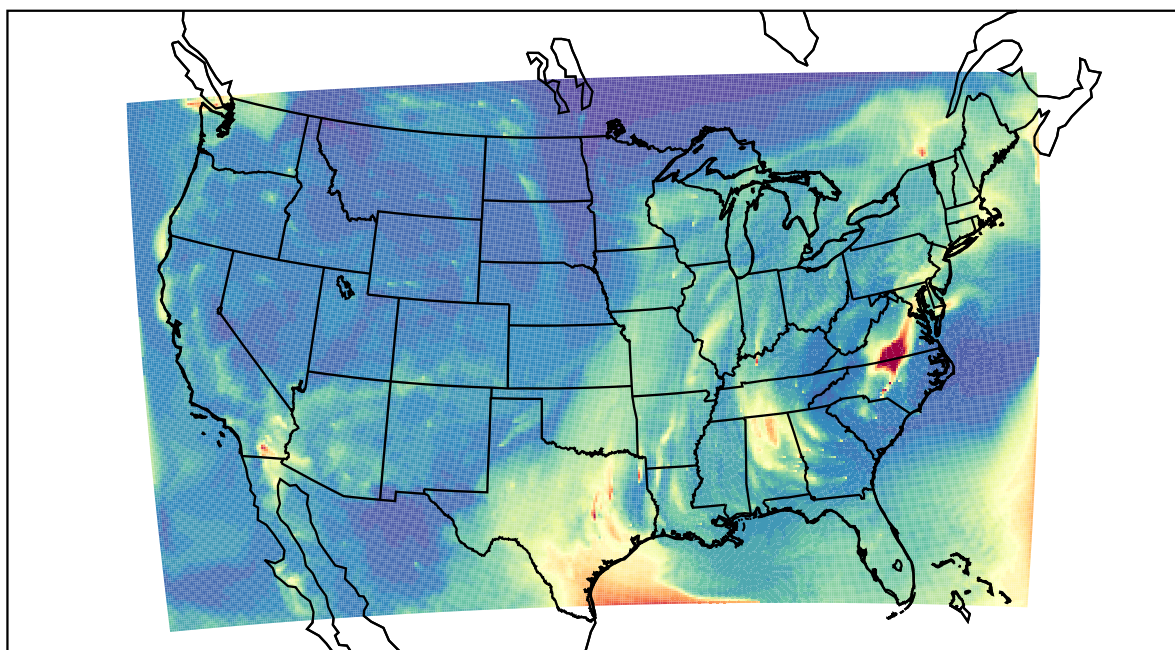
WRF 2023-10-27_08:00:00
