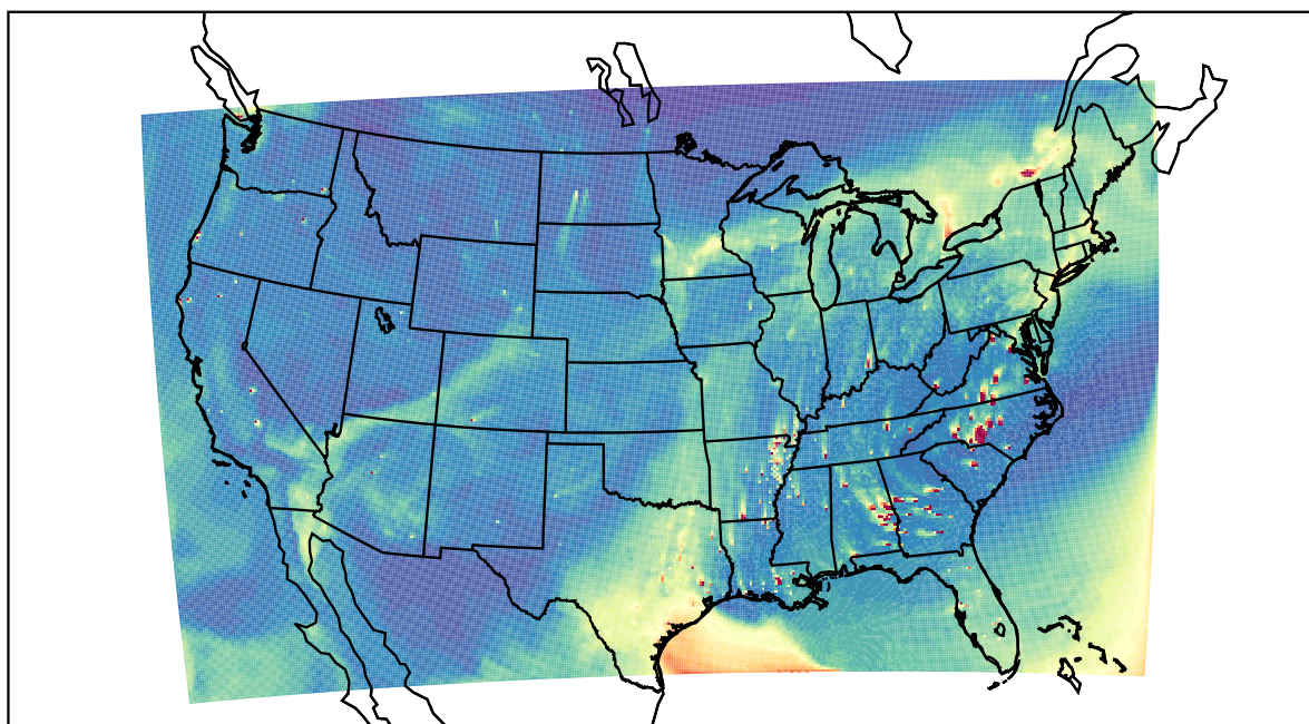
WRF 2023-10-26_22:00:00
