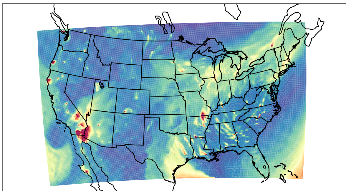
WRF 2023-10-26_03:00:00
