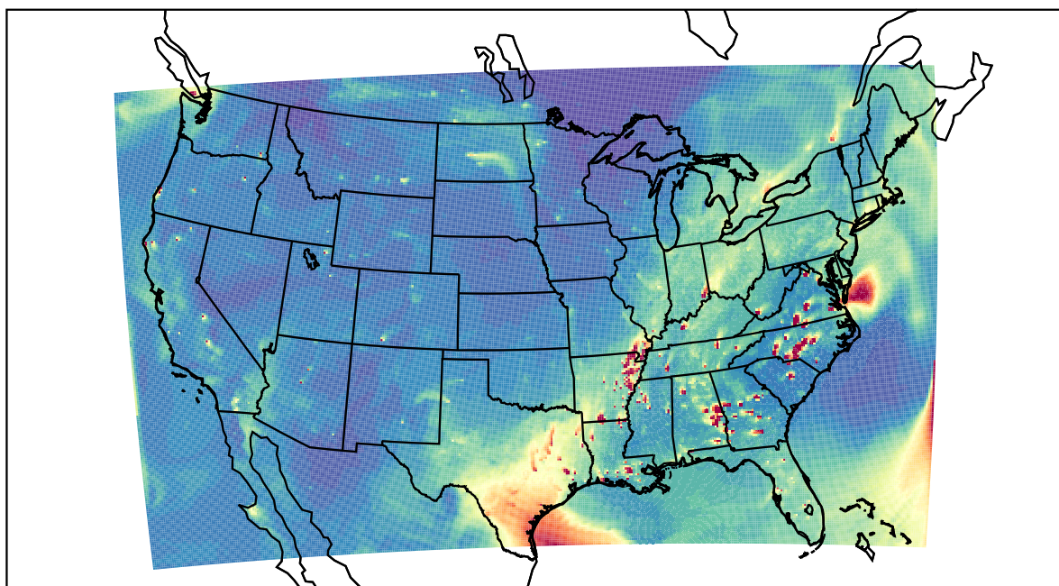
WRF 2023-10-27_23:00:00
