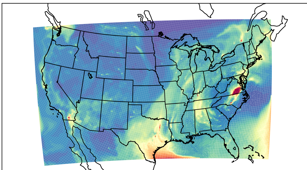
WRF 2023-10-27_11:00:00
