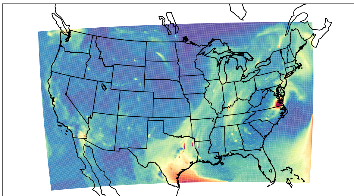
WRF 2023-10-27_15:00:00
