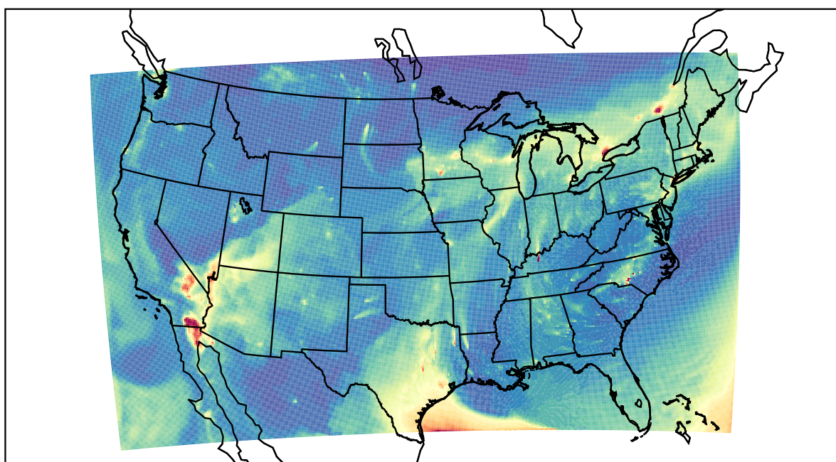
WRF 2023-10-26_14:00:00
