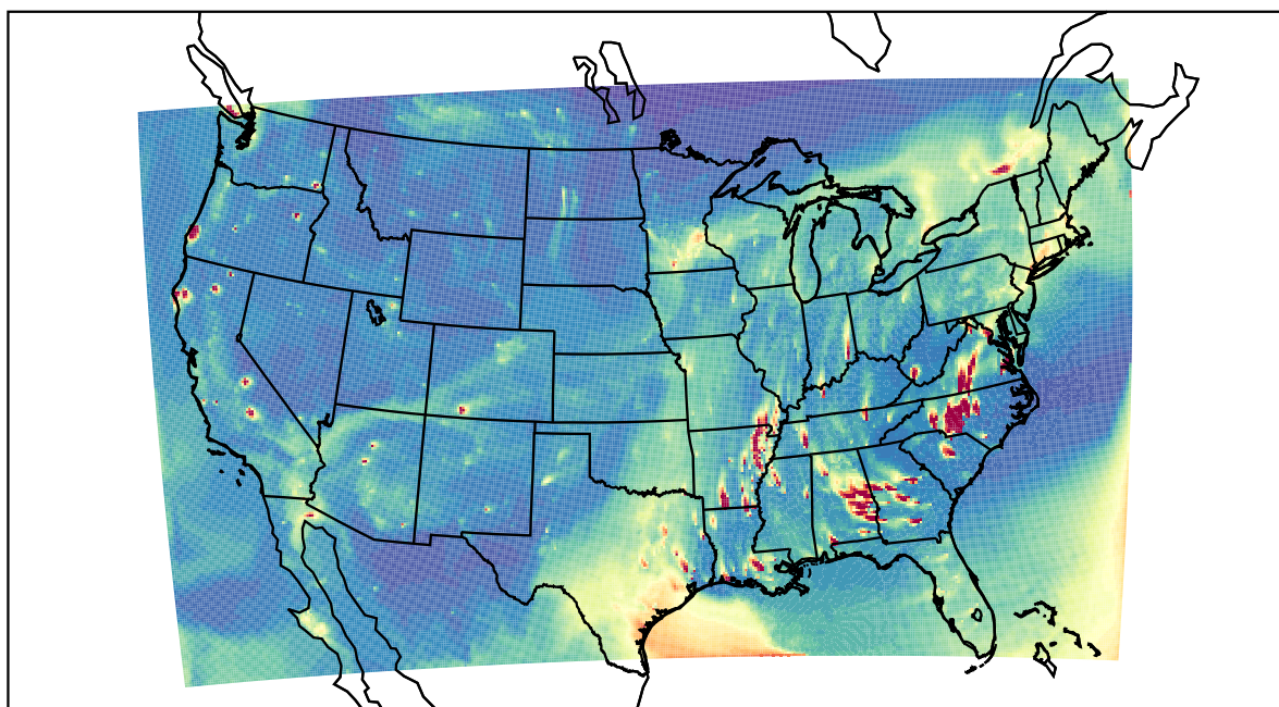
WRF 2023-10-27_01:00:00
