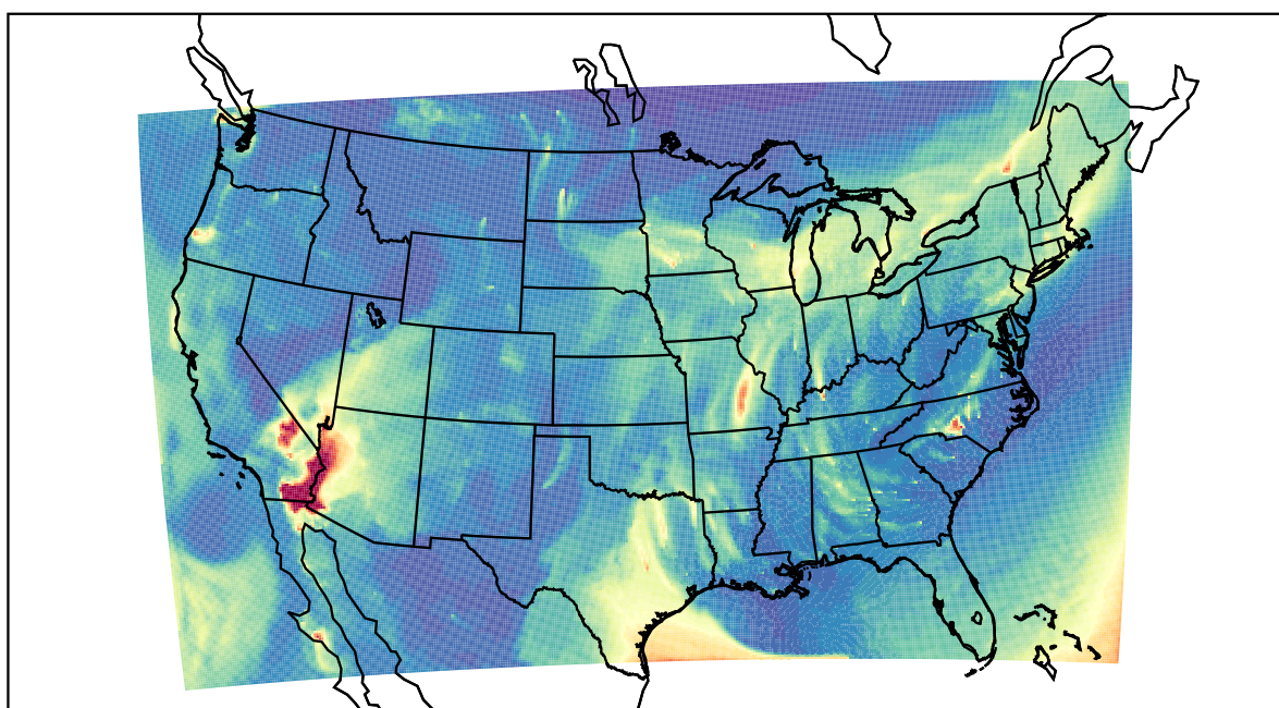
WRF 2023-10-26_07:00:00
