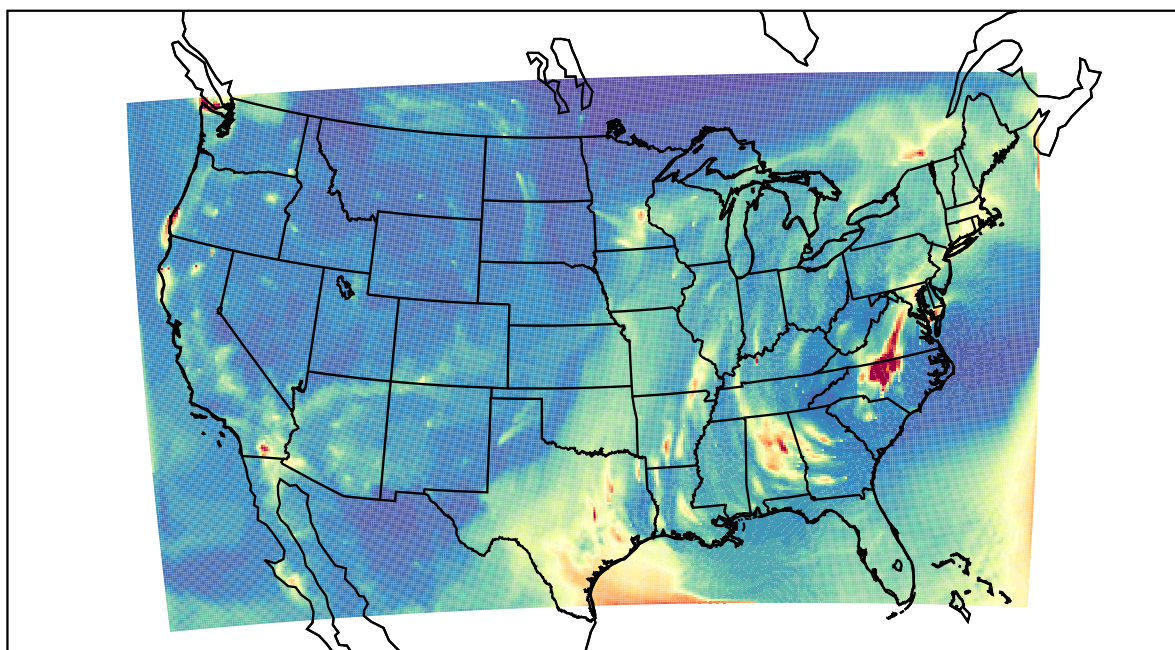
WRF 2023-10-27_05:00:00
