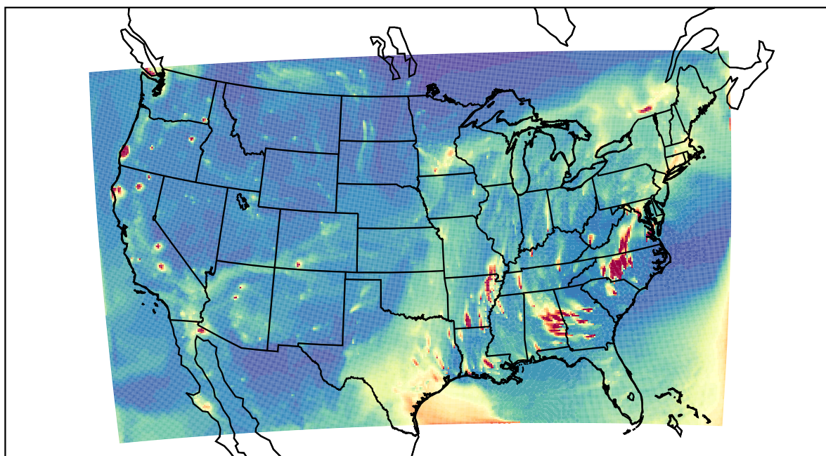
WRF 2023-10-27_02:00:00
