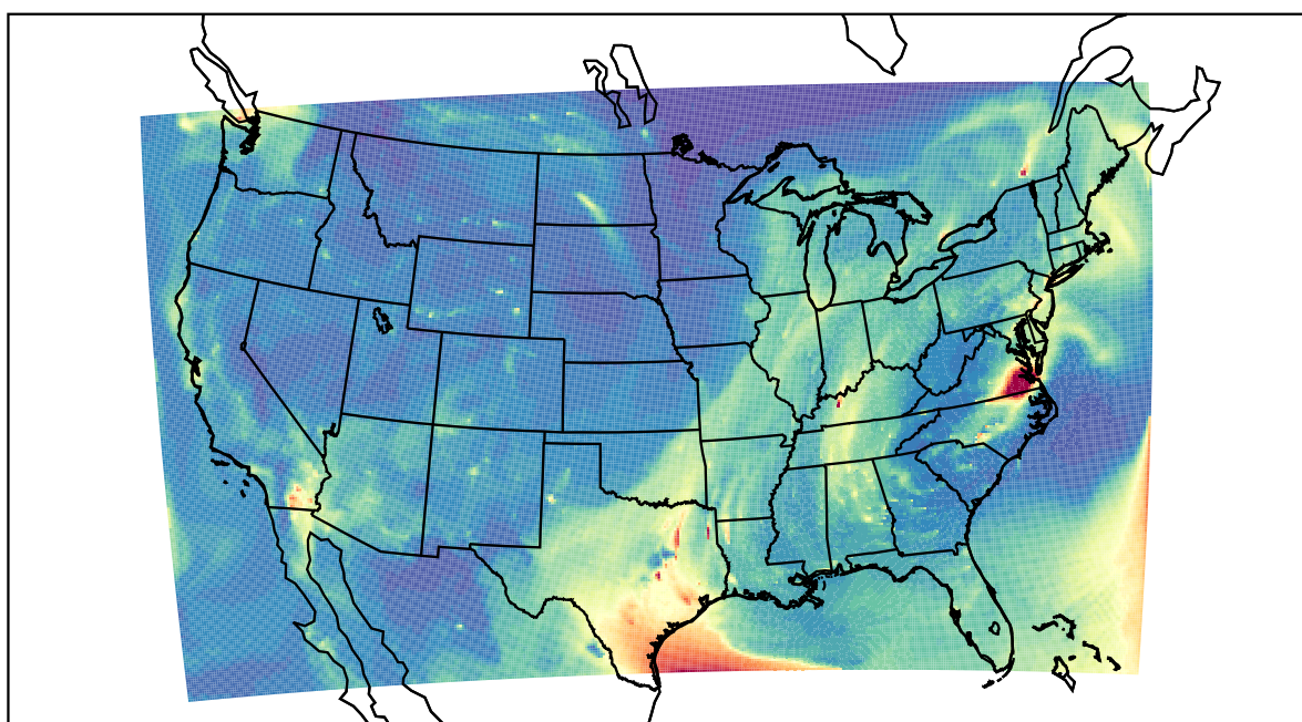
WRF 2023-10-27_14:00:00
