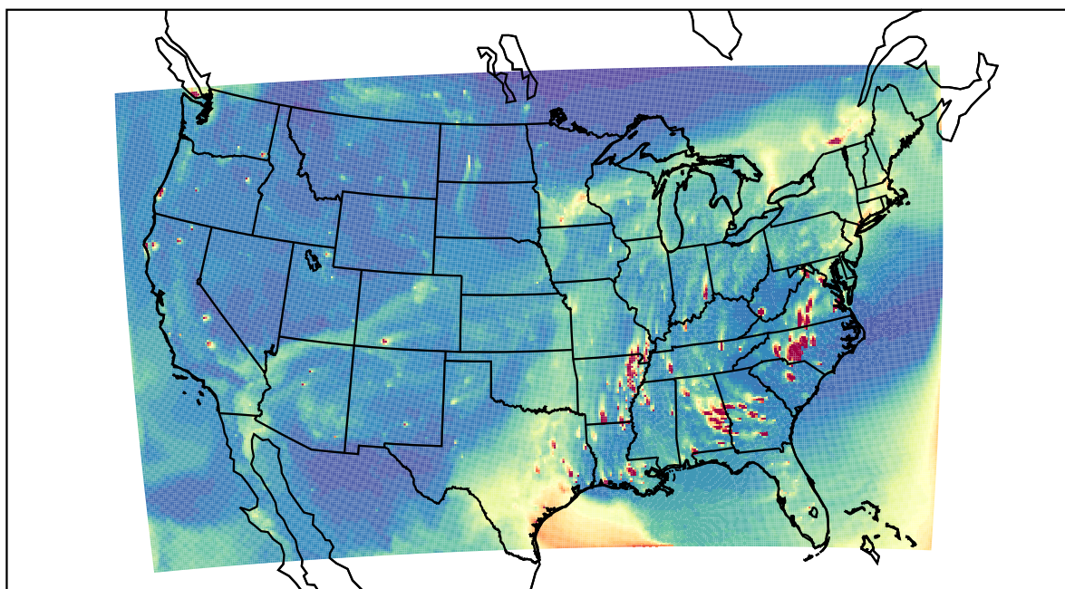
WRF 2023-10-27_00:00:00
