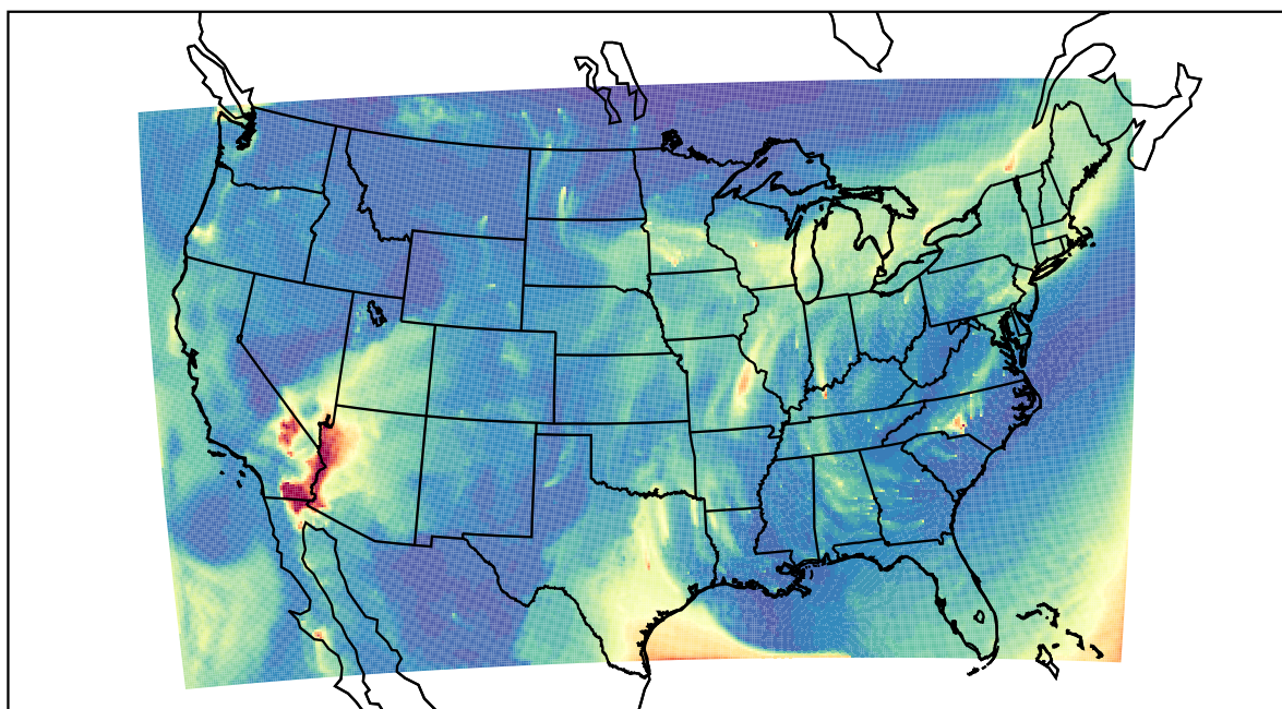
WRF 2023-10-26_08:00:00
