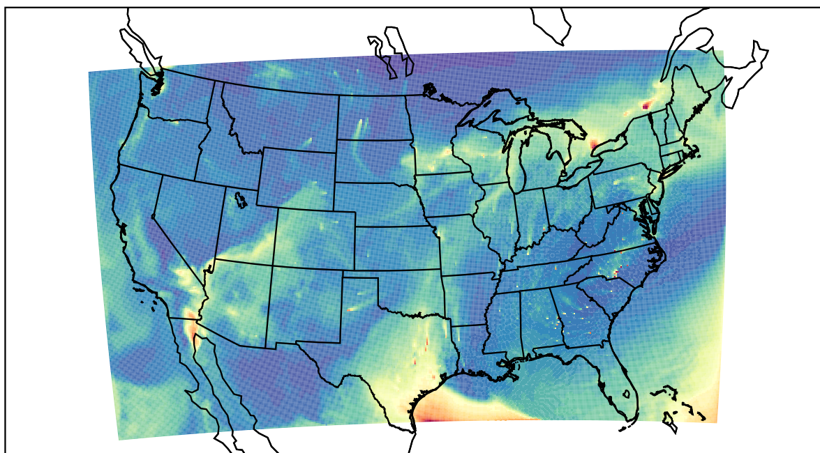
WRF 2023-10-26_17:00:00
