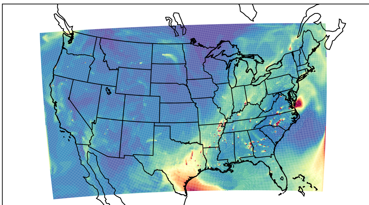
WRF 2023-10-27_21:00:00
