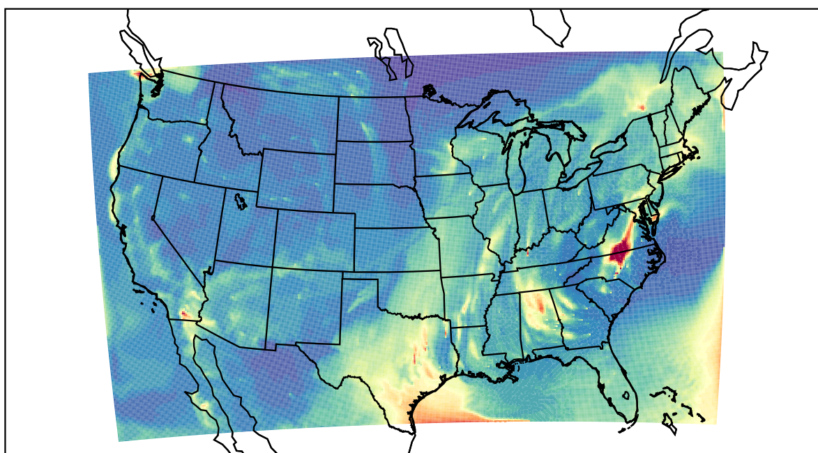
WRF 2023-10-27_07:00:00
