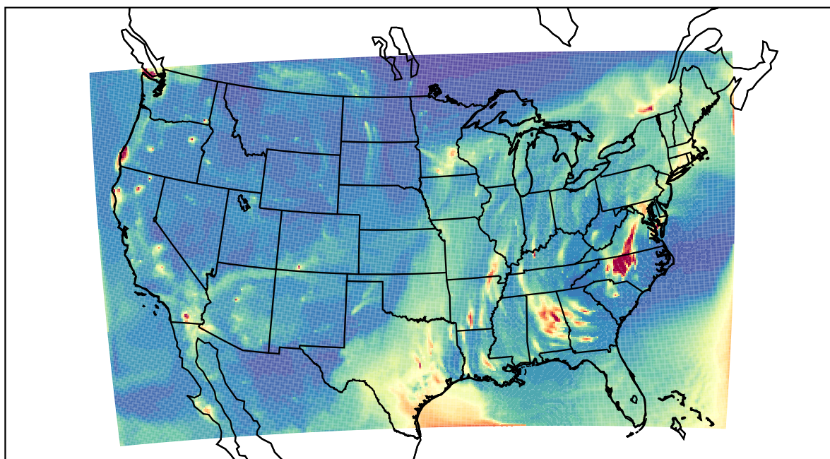
WRF 2023-10-27_04:00:00
