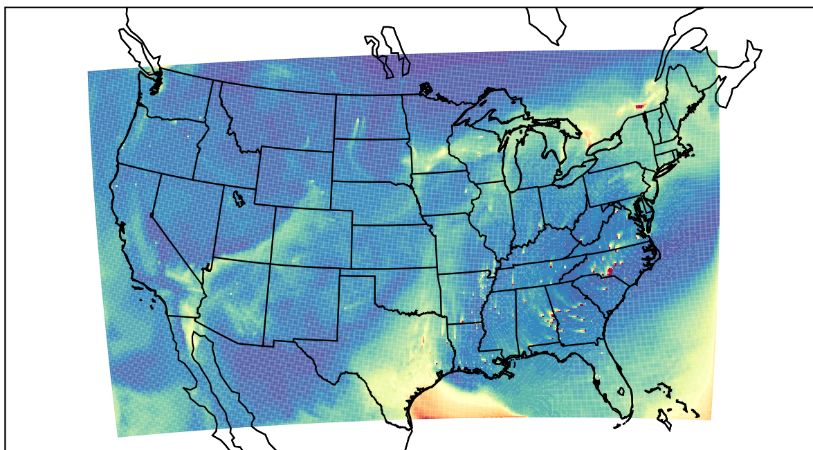
WRF 2023-10-26_20:00:00
