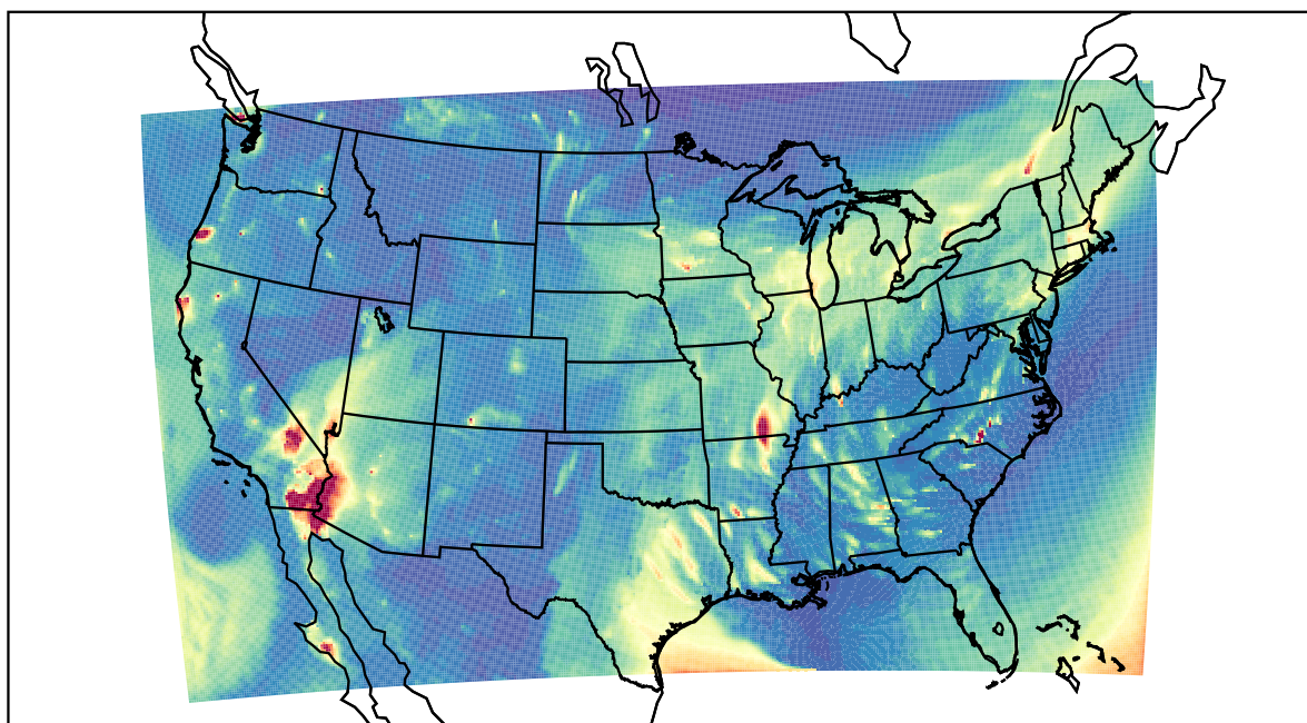
WRF 2023-10-26_04:00:00
