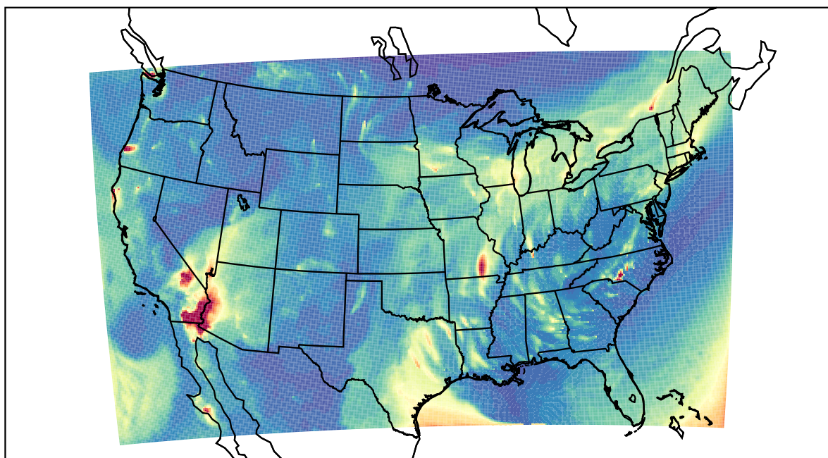
WRF 2023-10-26_05:00:00
