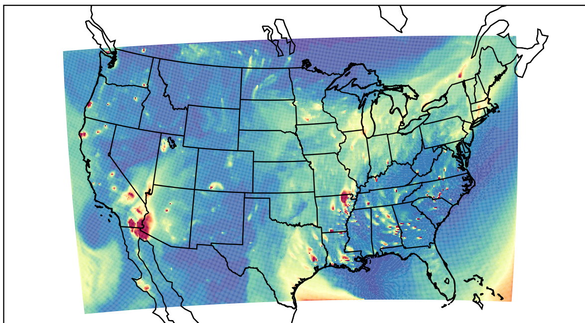
WRF 2023-10-26_02:00:00
