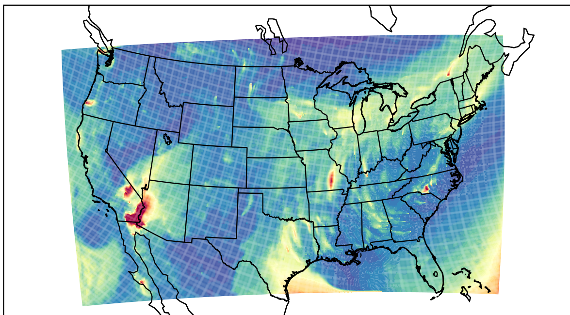
WRF 2023-10-26_06:00:00
