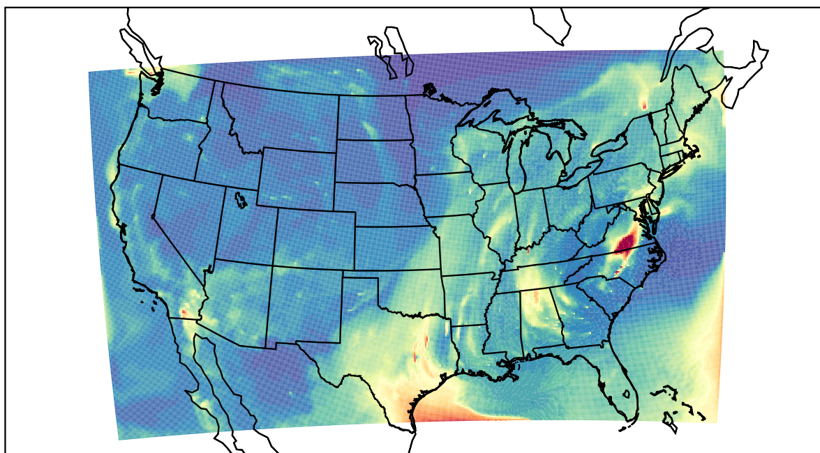
WRF 2023-10-27_09:00:00
