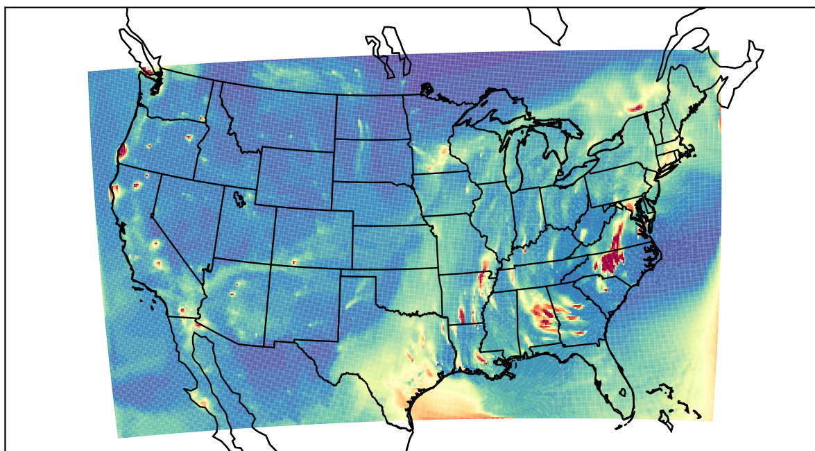
WRF 2023-10-27_03:00:00
