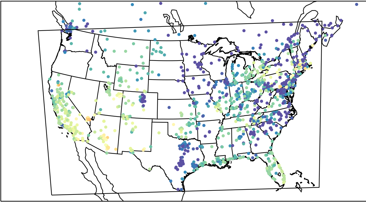
AirNOW (2023-10-27_00:00:00)
