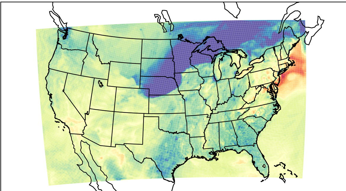
WRF (2023-10-26_23:00:00)
