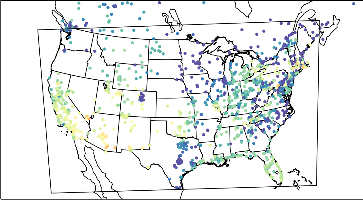
AirNOW (2023-10-26_23:00:00)
