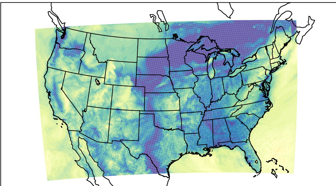
WRF (2023-10-26_10:00:00)
