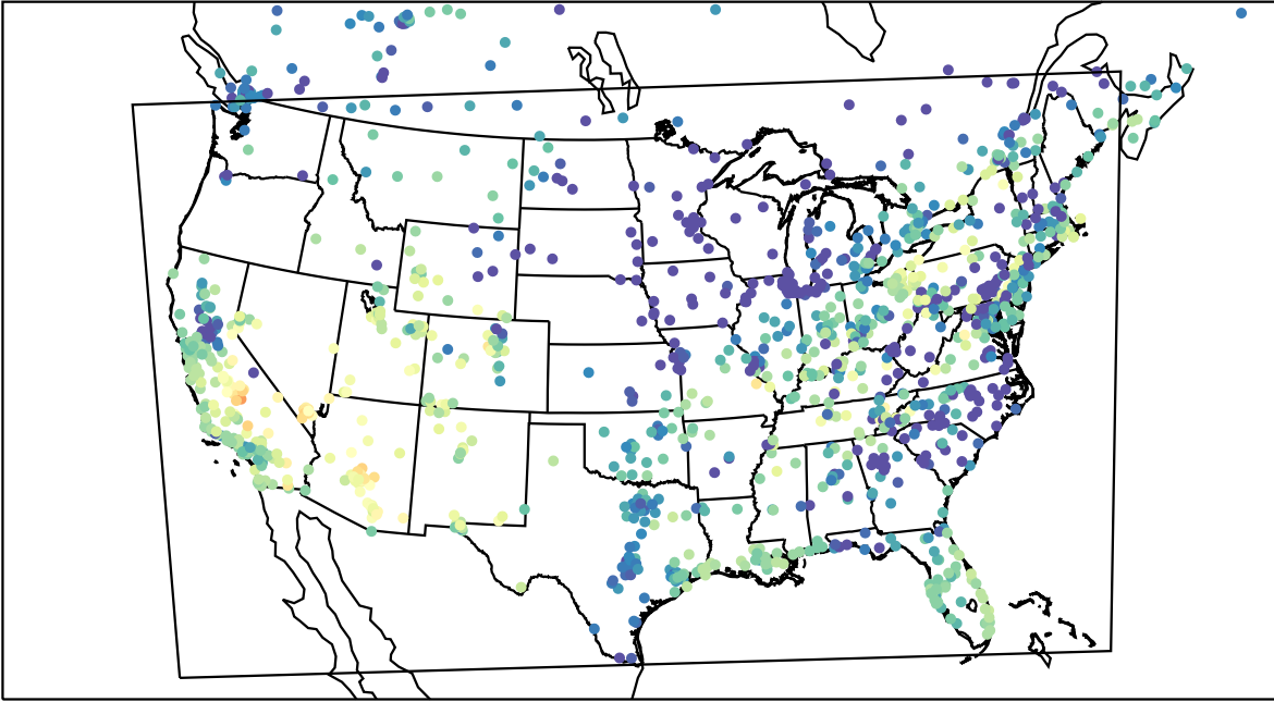
AirNOW (2023-10-26_00:00:00)
