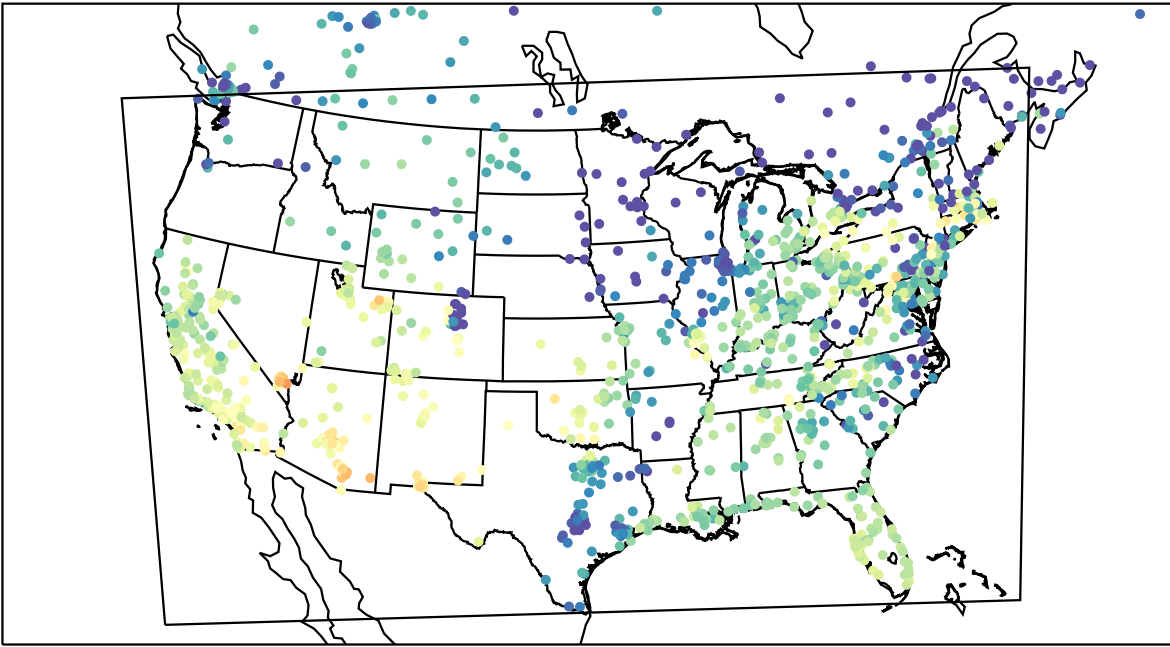
AirNOW (2023-10-26_22:00:00)
