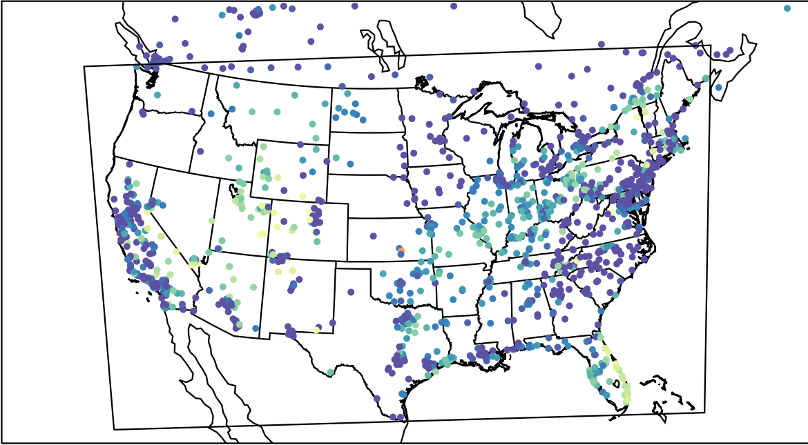
AirNOW (2023-10-26_13:00:00)
