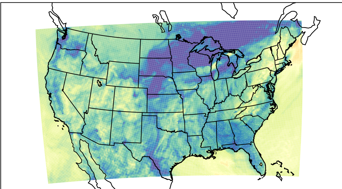
WRF (2023-10-26_05:00:00)
