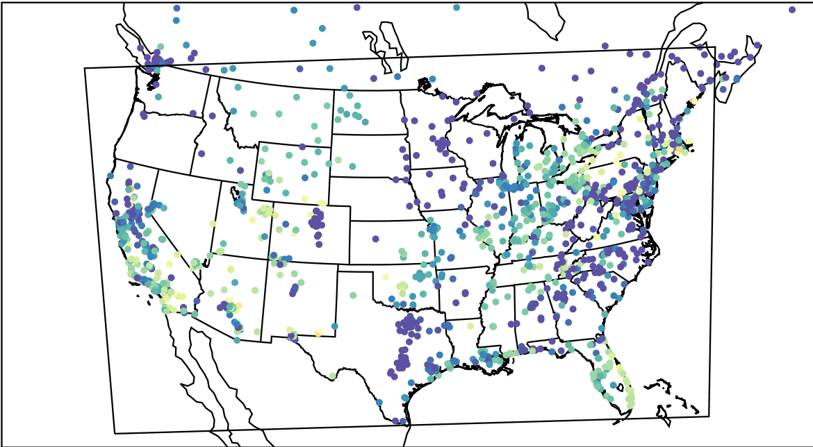
AirNOW (2023-10-27_02:00:00)
