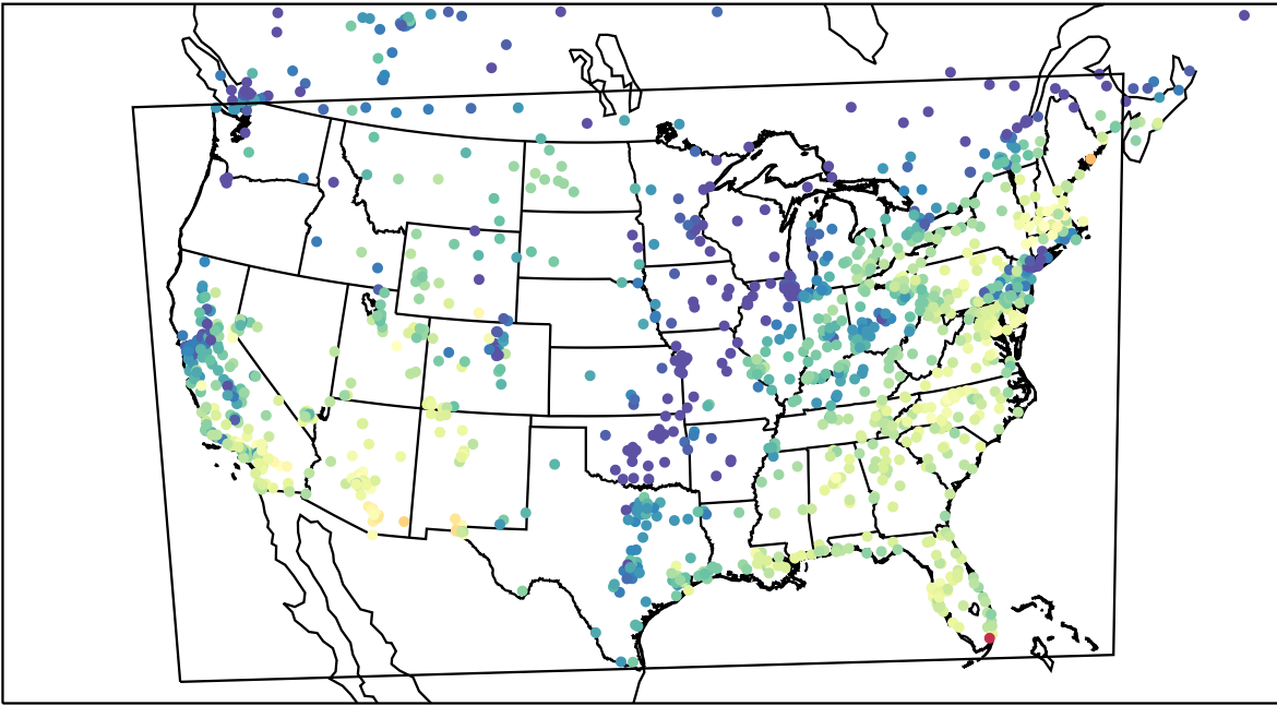
AirNOW (2023-10-27_18:00:00)
