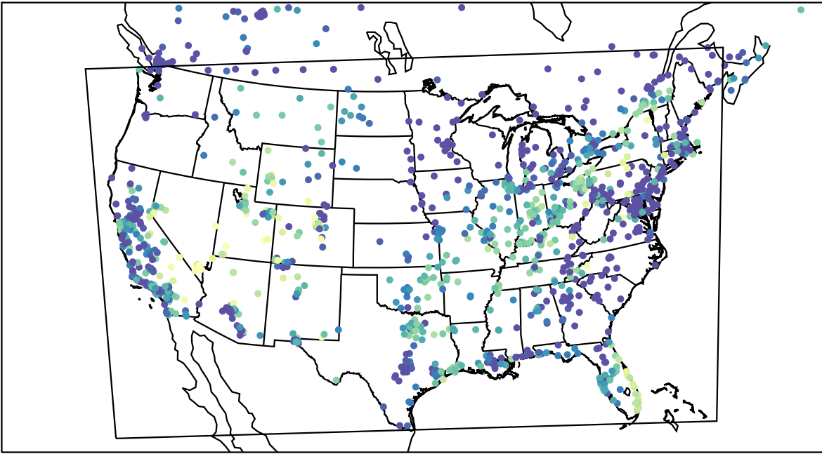
AirNOW (2023-10-26_08:00:00)
