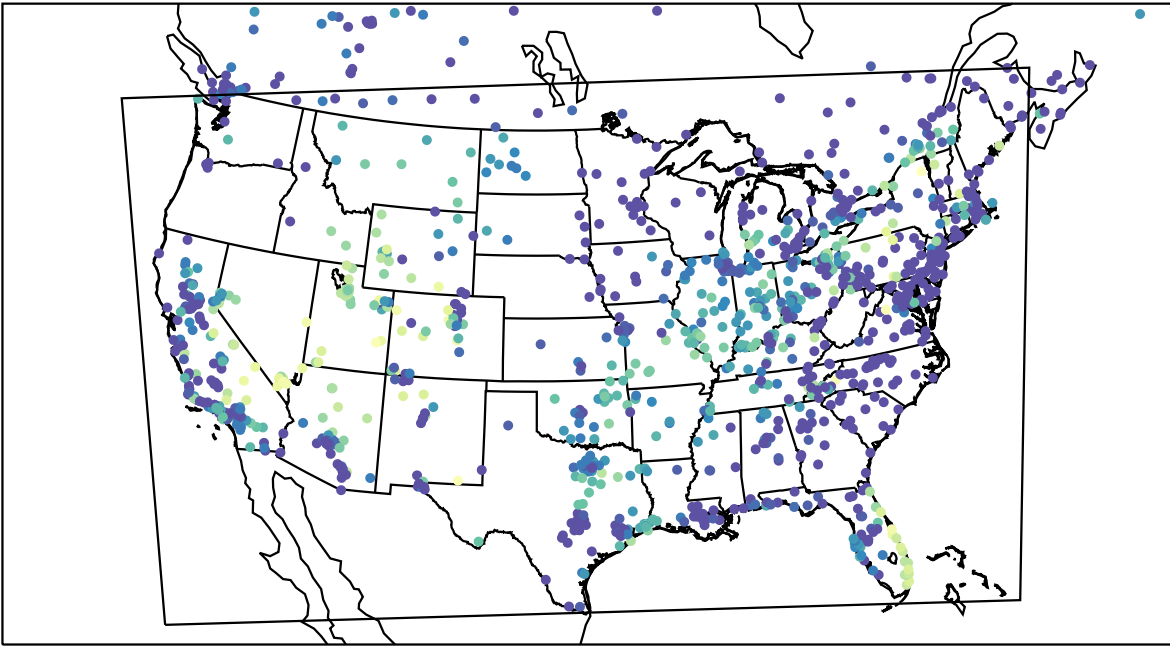
AirNOW (2023-10-26_11:00:00)
