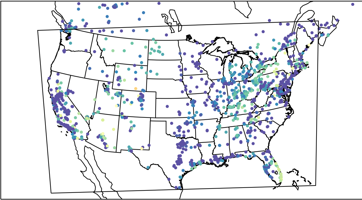
AirNOW (2023-10-27_08:00:00)
