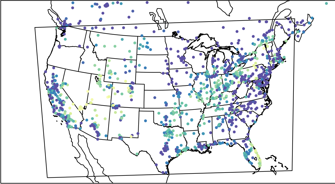
AirNOW (2023-10-26_09:00:00)
