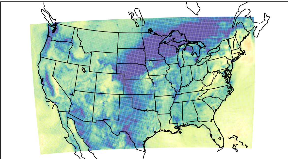
WRF (2023-10-26_15:00:00)
