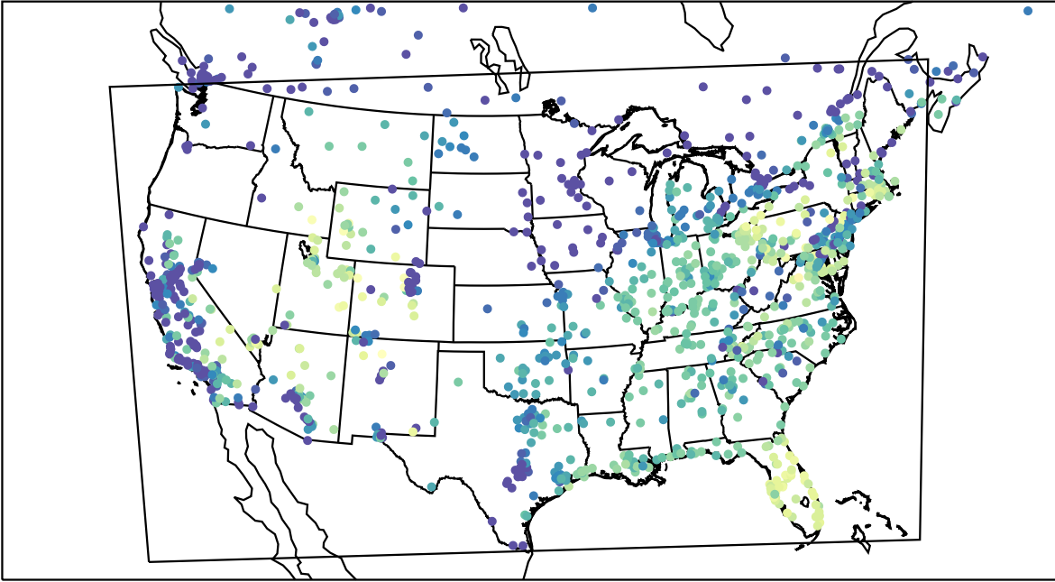
AirNOW (2023-10-26_15:00:00)
