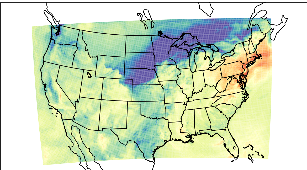
WRF (2023-10-26_18:00:00)
