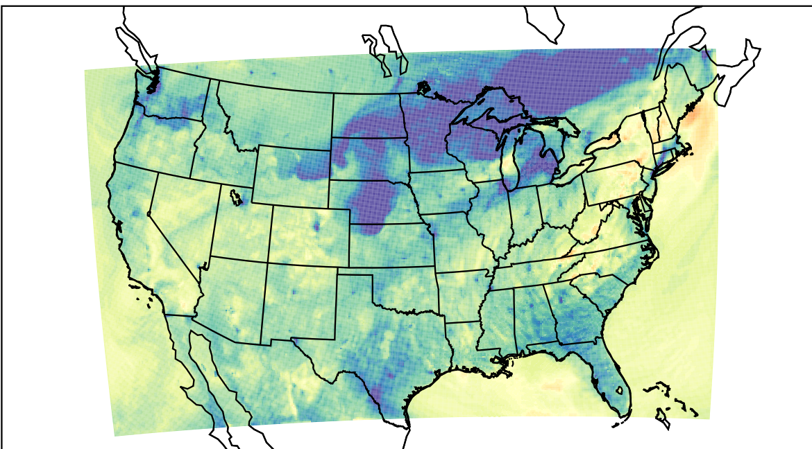
WRF (2023-10-26_01:00:00)
