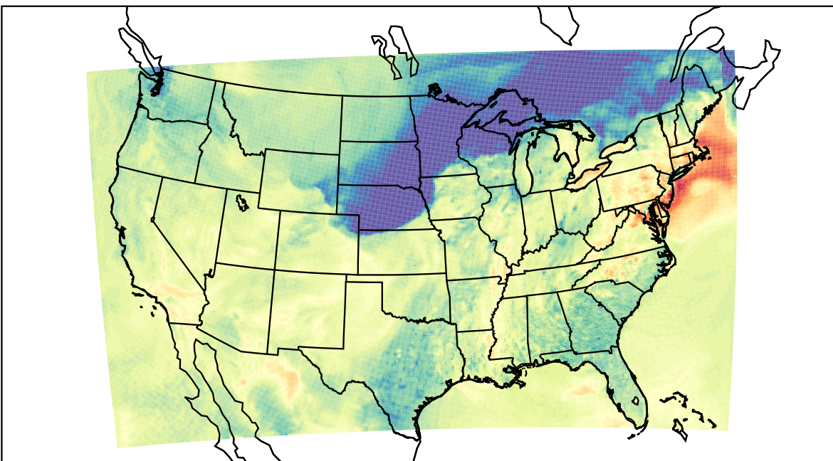
WRF (2023-10-26_22:00:00)
