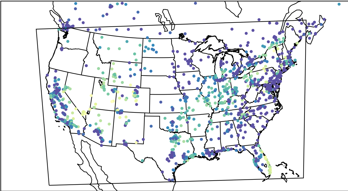
AirNOW (2023-10-26_10:00:00)
