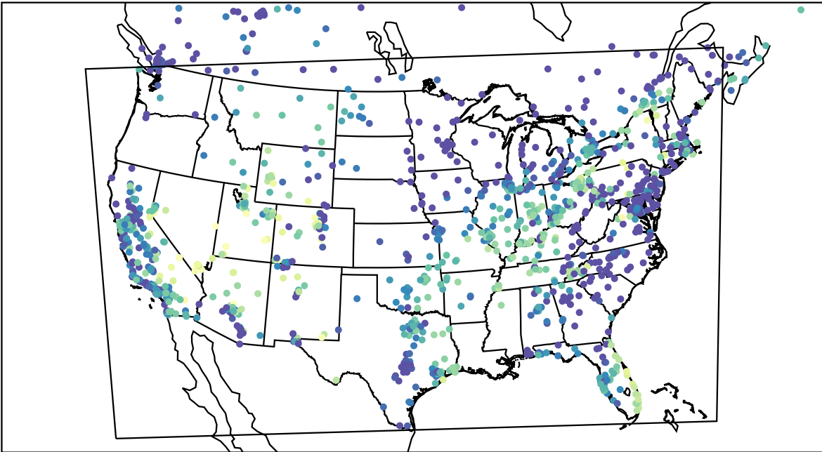
AirNOW (2023-10-26_07:00:00)
