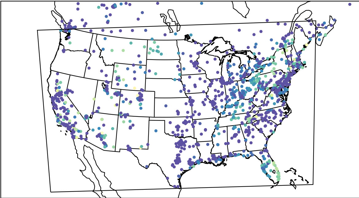
AirNOW (2023-10-27_13:00:00)
