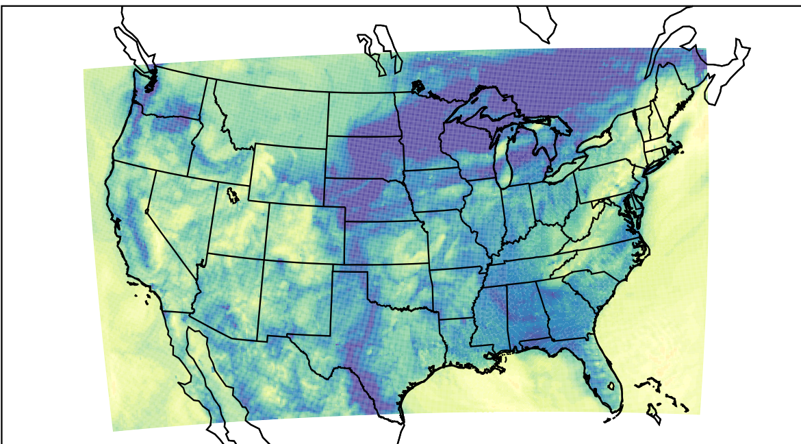
WRF (2023-10-26_08:00:00)
