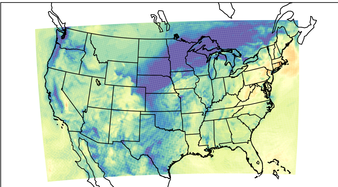
WRF (2023-10-26_16:00:00)
