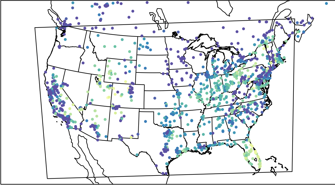
AirNOW (2023-10-26_14:00:00)
