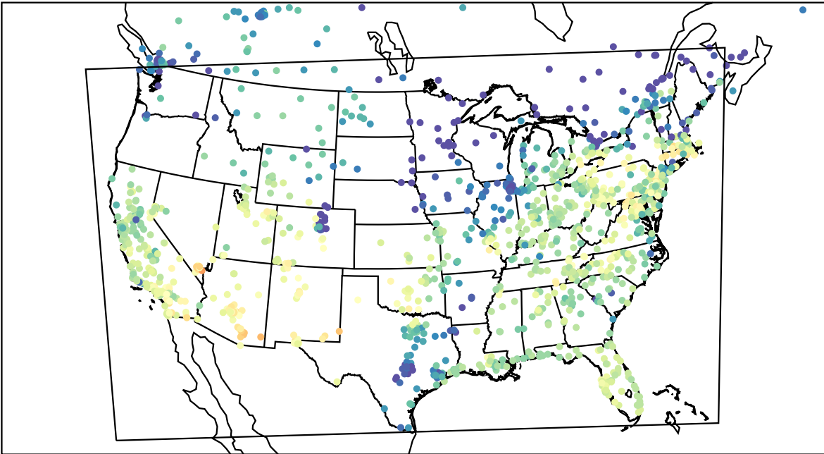
AirNOW (2023-10-26_21:00:00)
