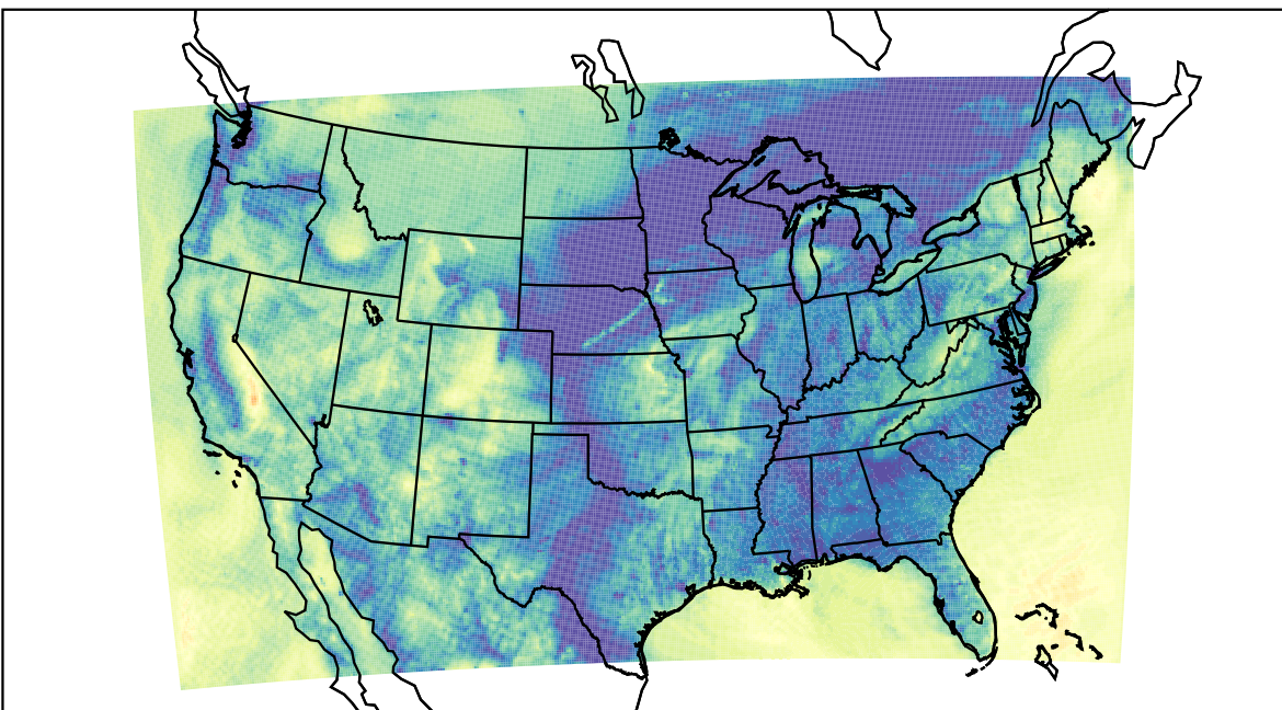
WRF (2023-10-26_13:00:00)
