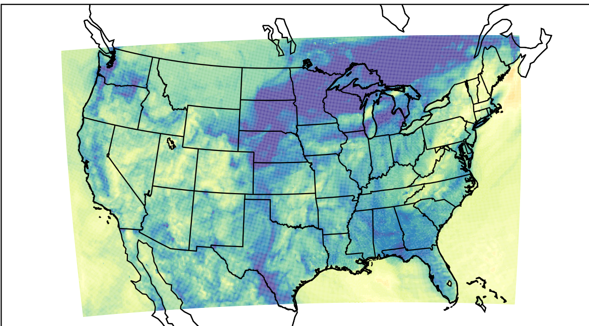
WRF (2023-10-26_06:00:00)
