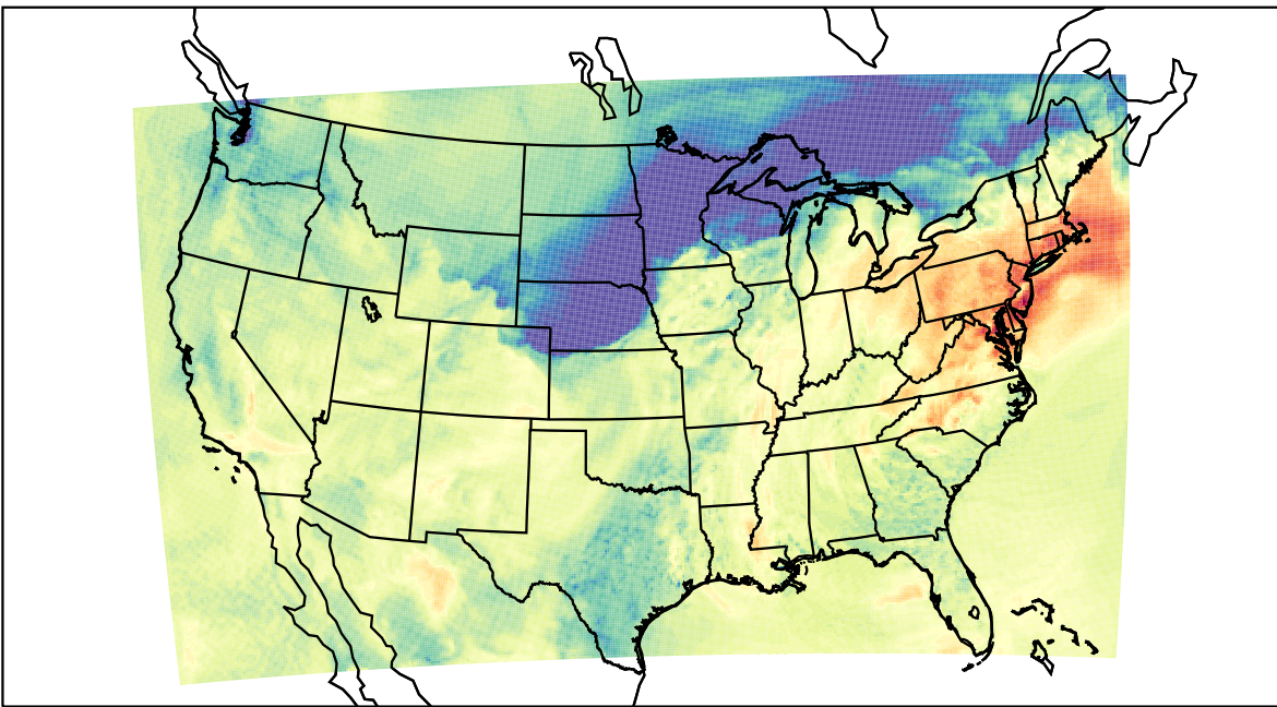
WRF (2023-10-26_20:00:00)
