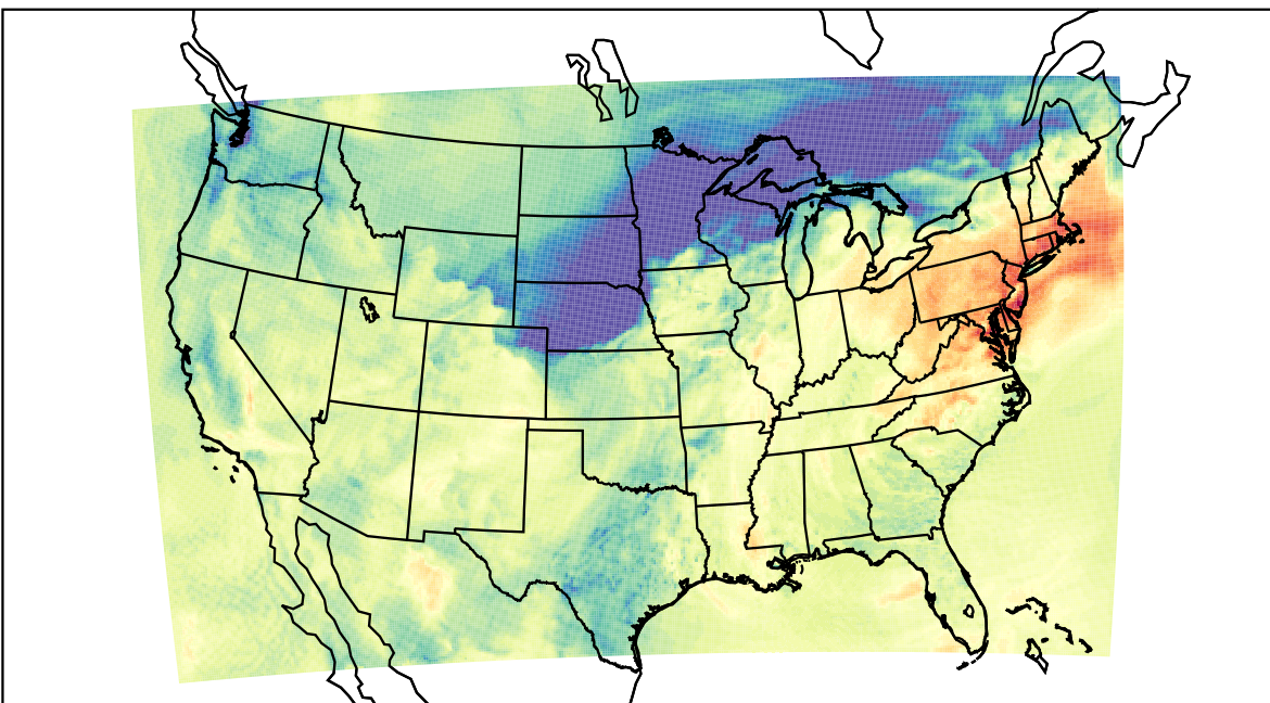
WRF (2023-10-26_19:00:00)
