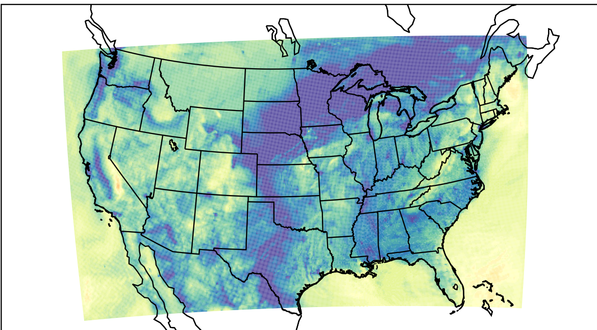
WRF (2023-10-26_14:00:00)
