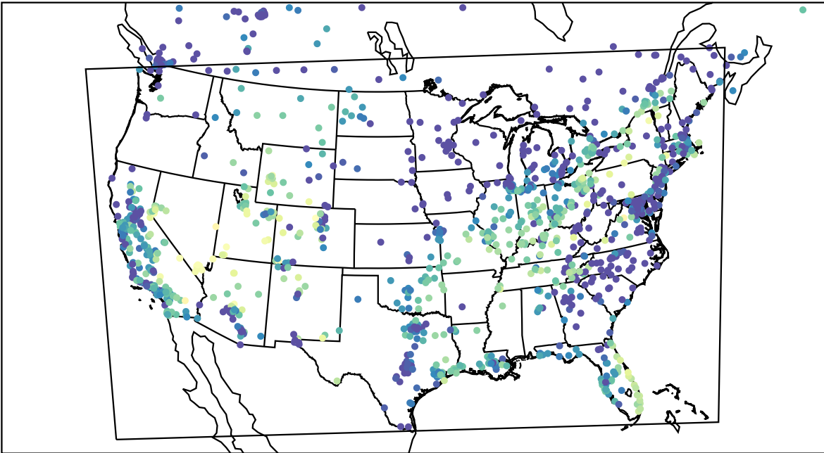
AirNOW (2023-10-26_06:00:00)
