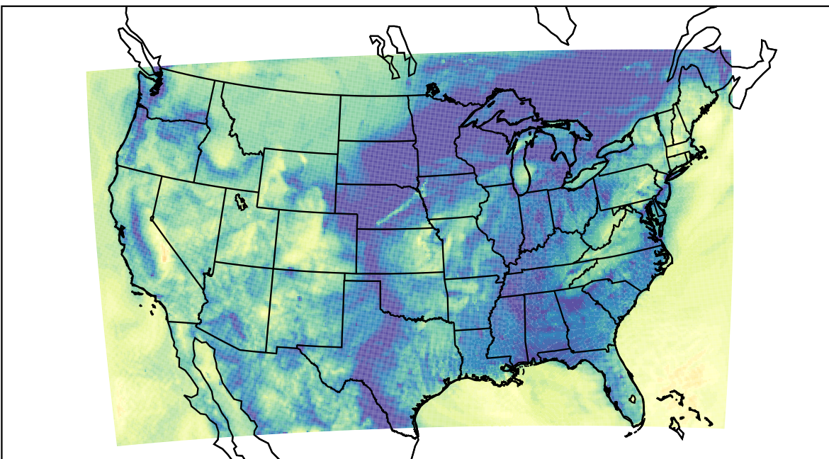
WRF (2023-10-26_12:00:00)
