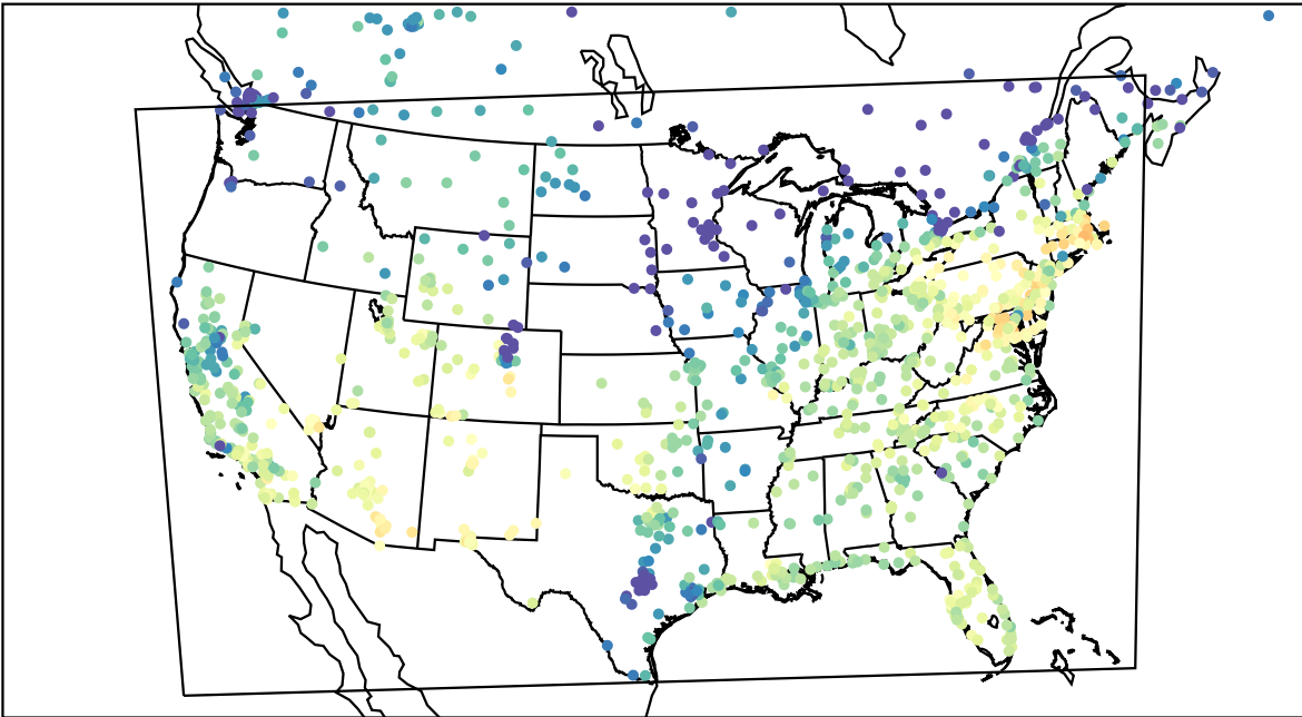
AirNOW (2023-10-26_19:00:00)
