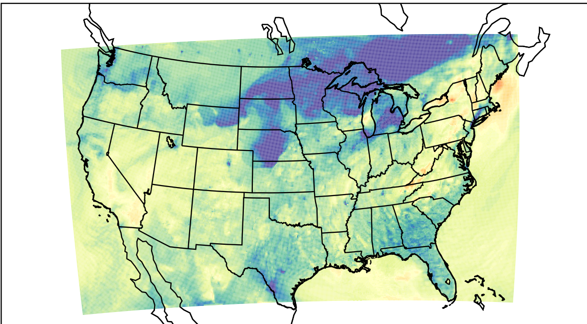
WRF (2023-10-26_00:00:00)
