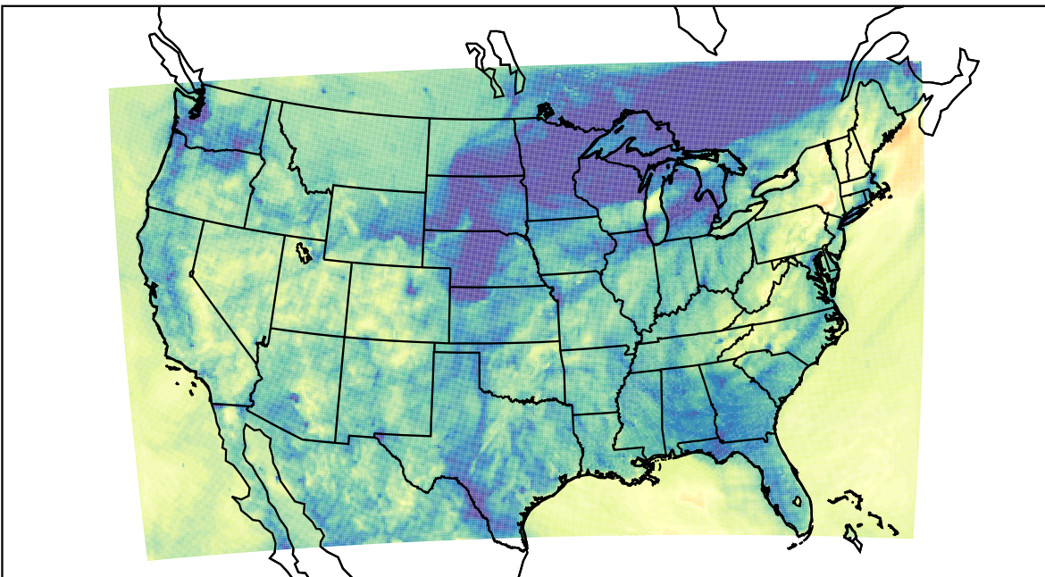
WRF (2023-10-26_04:00:00)
