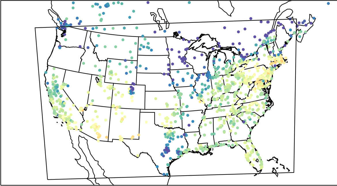
AirNOW (2023-10-26_20:00:00)
