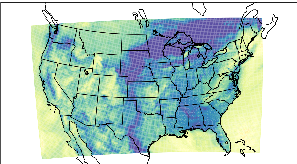
WRF (2023-10-26_09:00:00)
