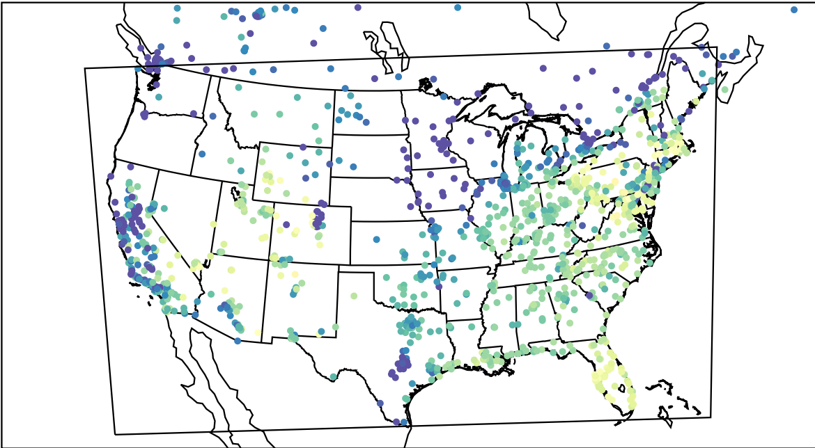
AirNOW (2023-10-26_16:00:00)
