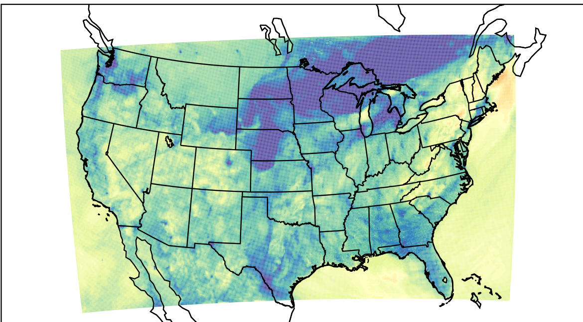
WRF (2023-10-26_03:00:00)
