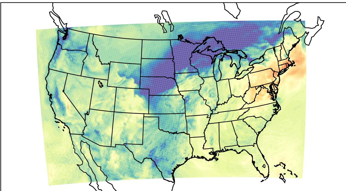
WRF (2023-10-26_17:00:00)
