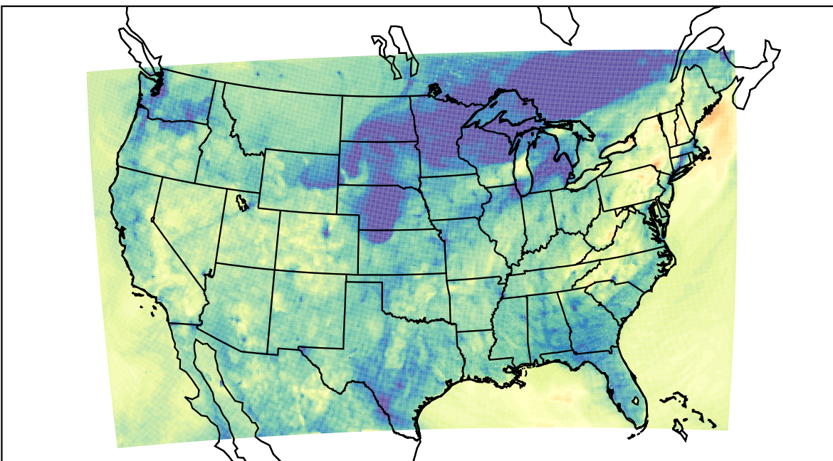
WRF (2023-10-26_02:00:00)
