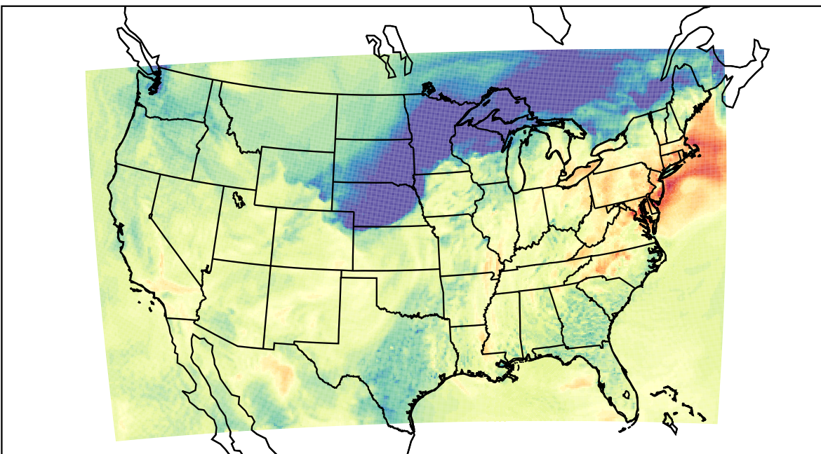
WRF (2023-10-26_21:00:00)
