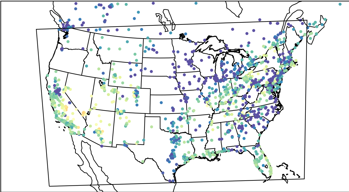
AirNOW (2023-10-26_01:00:00)
