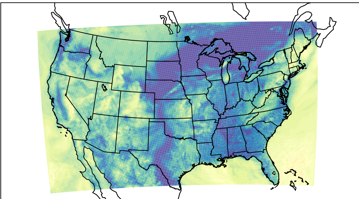
WRF (2023-10-26_11:00:00)
