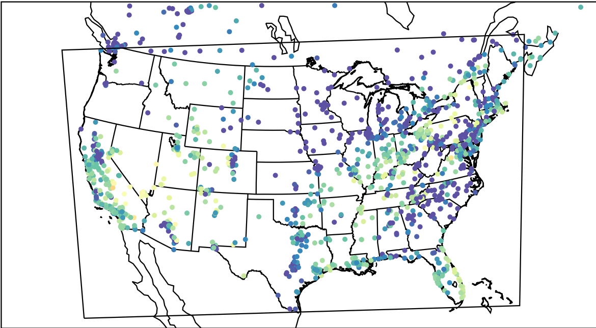
AirNOW (2023-10-26_03:00:00)
