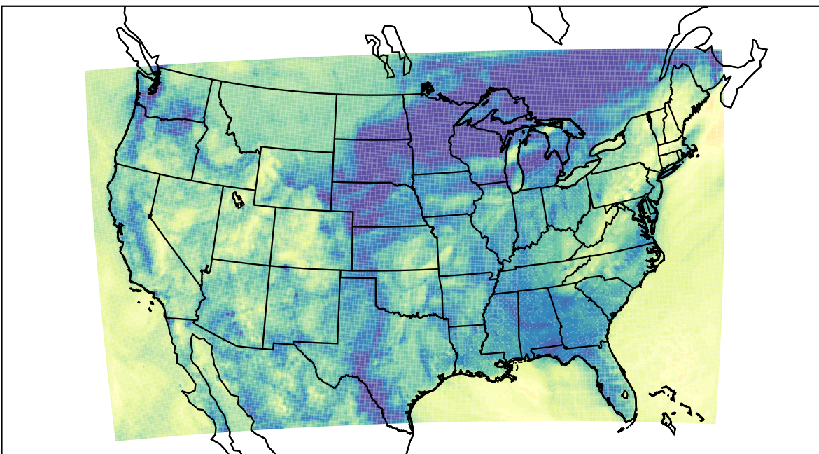
WRF (2023-10-26_07:00:00)
