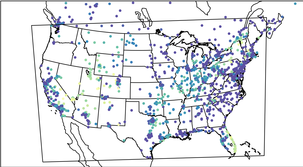
AirNOW (2023-10-26_12:00:00)
