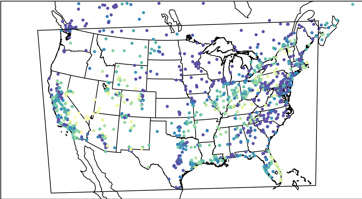
AirNOW (2023-10-26_05:00:00)
