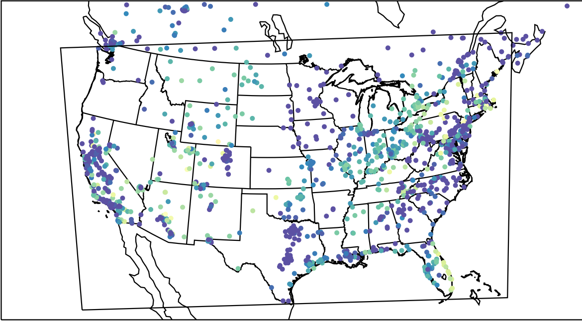
AirNOW (2023-10-27_05:00:00)
