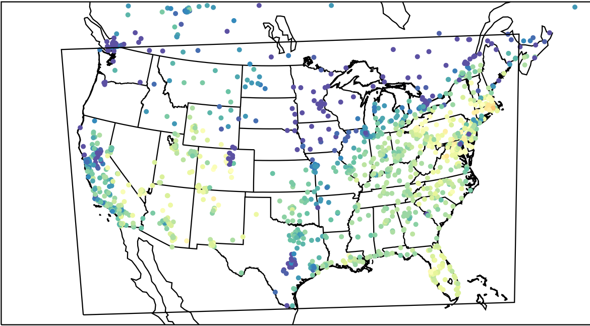
AirNOW (2023-10-26_17:00:00)
