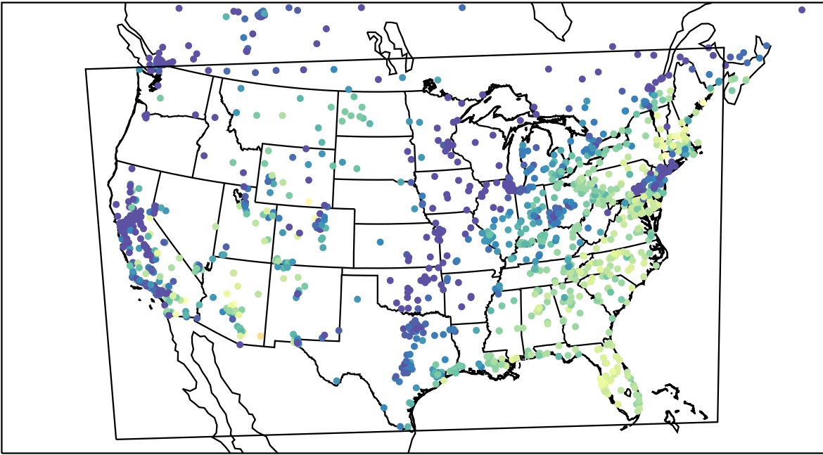
AirNOW (2023-10-27_16:00:00)
