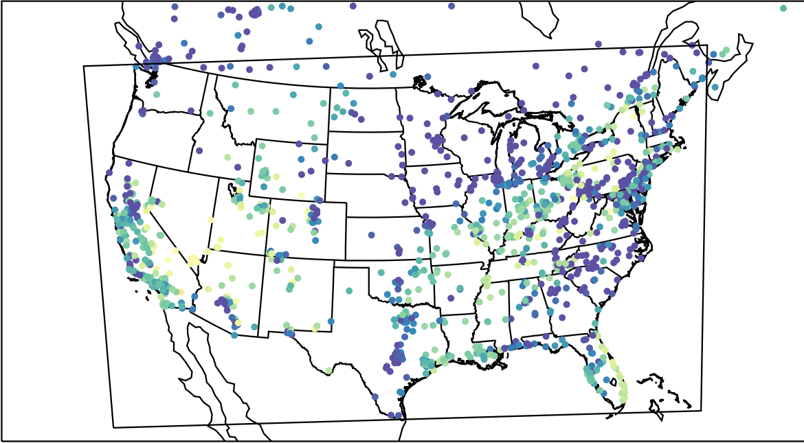
AirNOW (2023-10-26_04:00:00)
