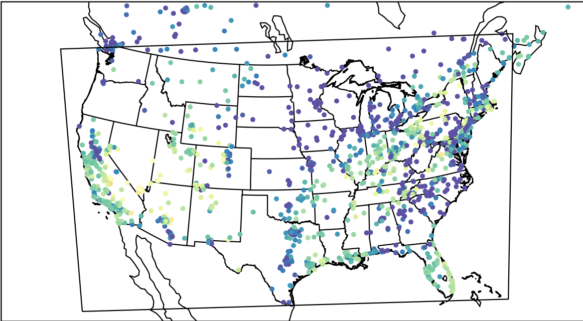
AirNOW (2023-10-26_02:00:00)
