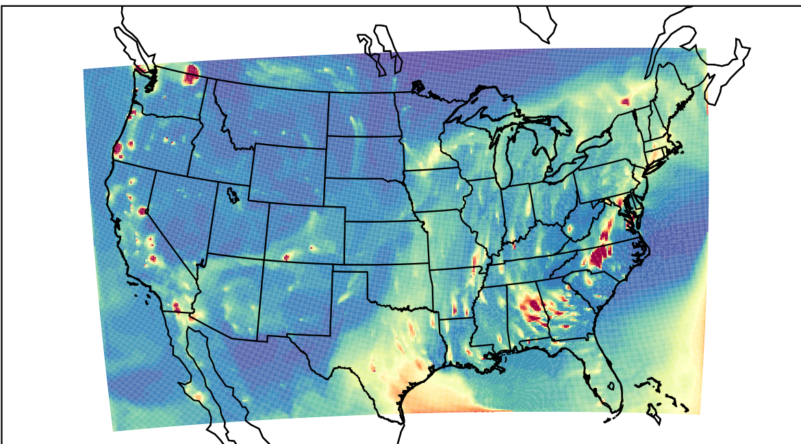
WRF 2023-10-27_03:00:00
