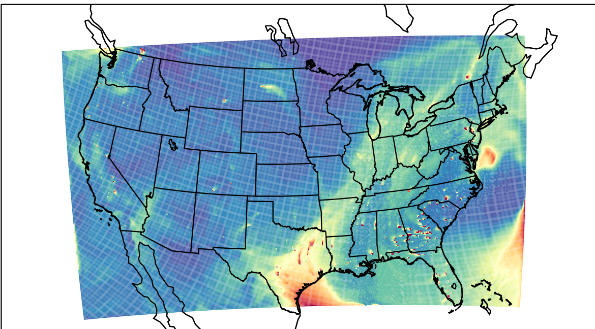
WRF 2023-10-27_21:00:00
