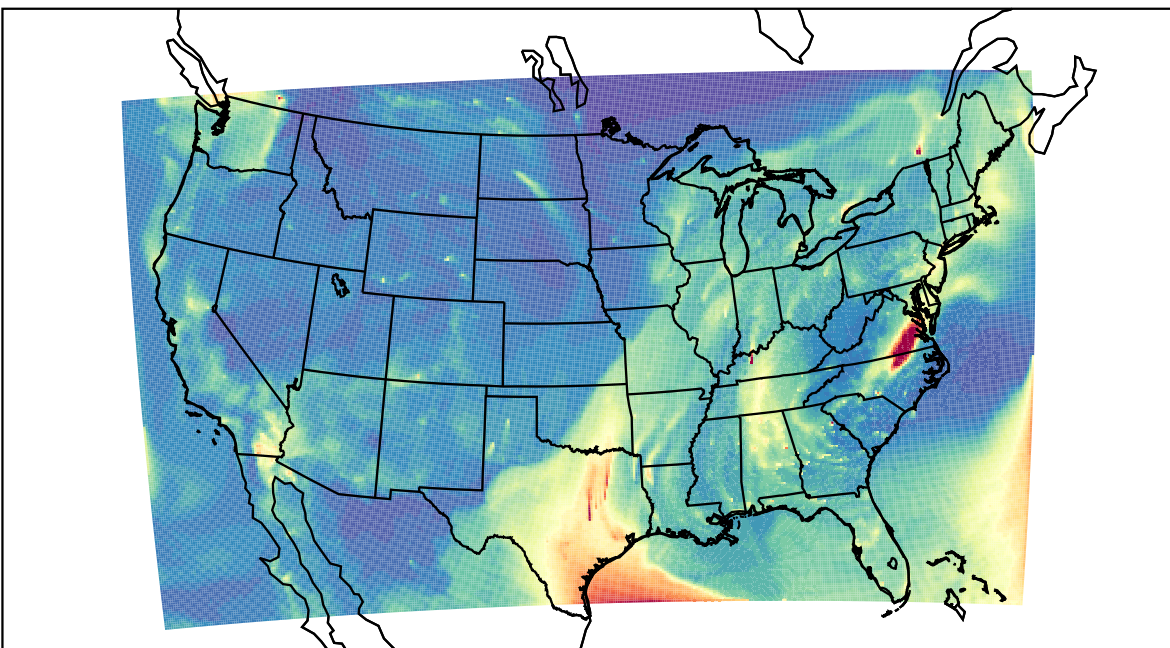
WRF 2023-10-27_12:00:00
