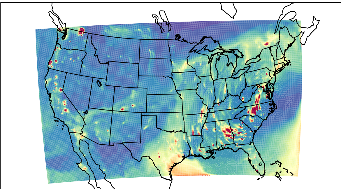
WRF 2023-10-27_02:00:00
