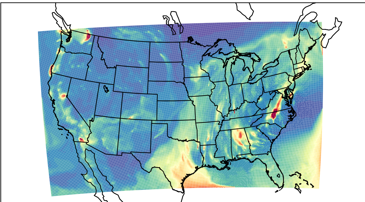
WRF 2023-10-27_06:00:00
