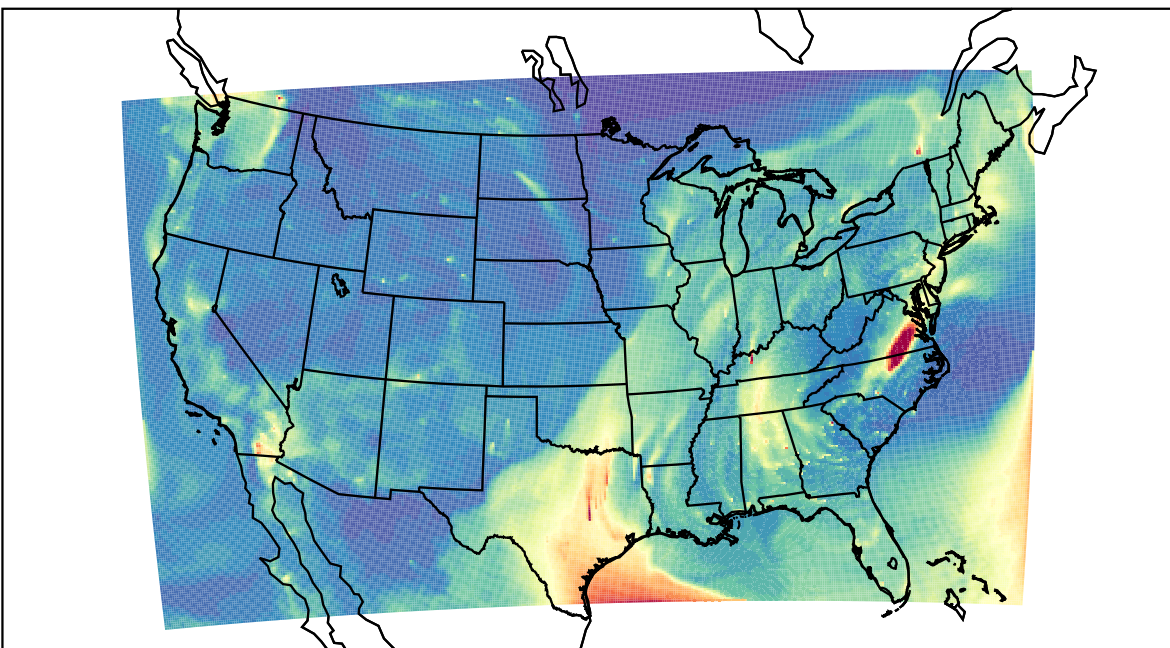
WRF 2023-10-27_11:00:00
