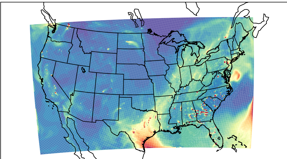
WRF 2023-10-27_22:00:00
