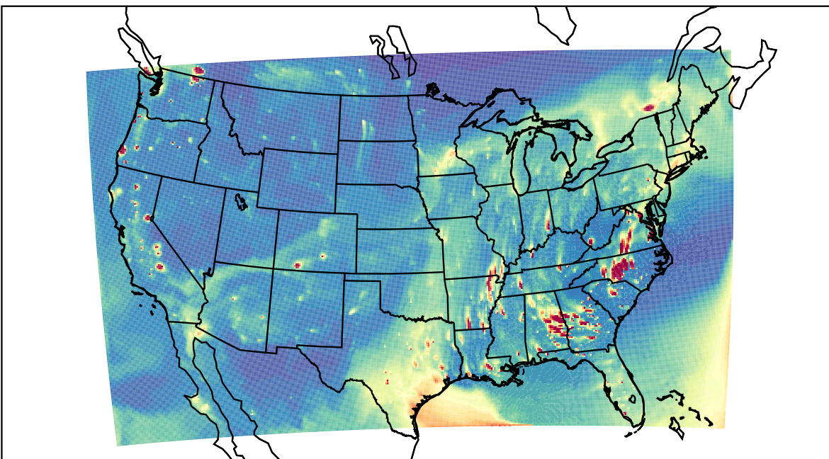
WRF 2023-10-27_01:00:00
