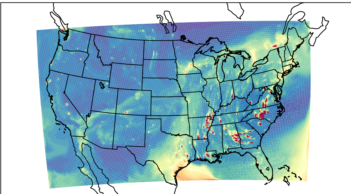
WRF 2023-10-27_00:00:00
