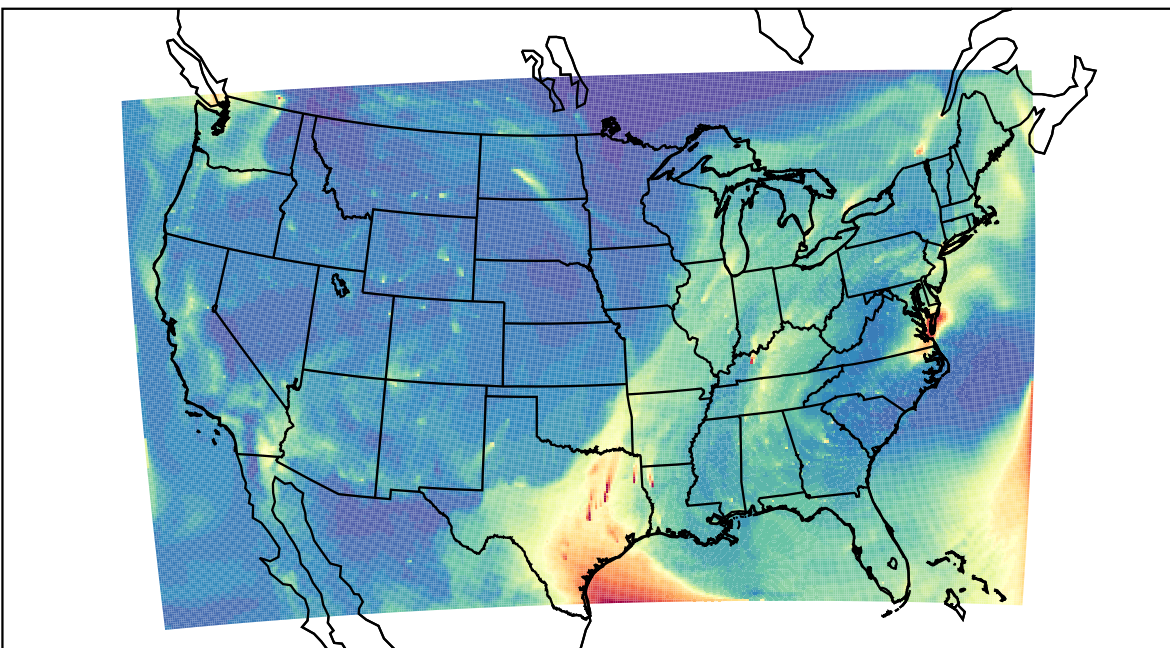
WRF 2023-10-27_16:00:00
