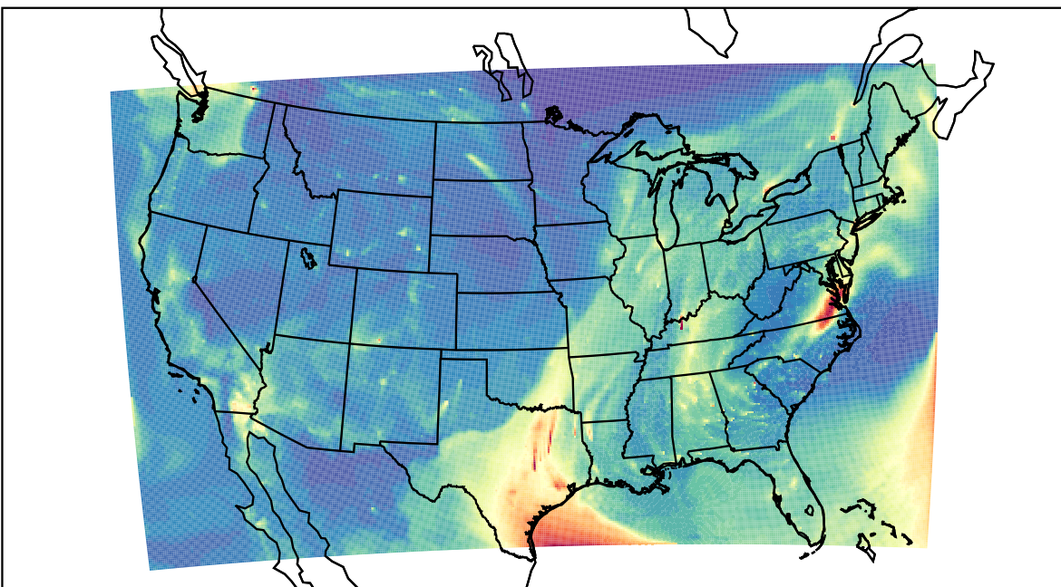
WRF 2023-10-27_14:00:00
