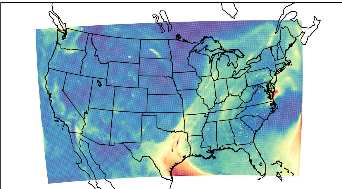
WRF 2023-10-27_17:00:00
