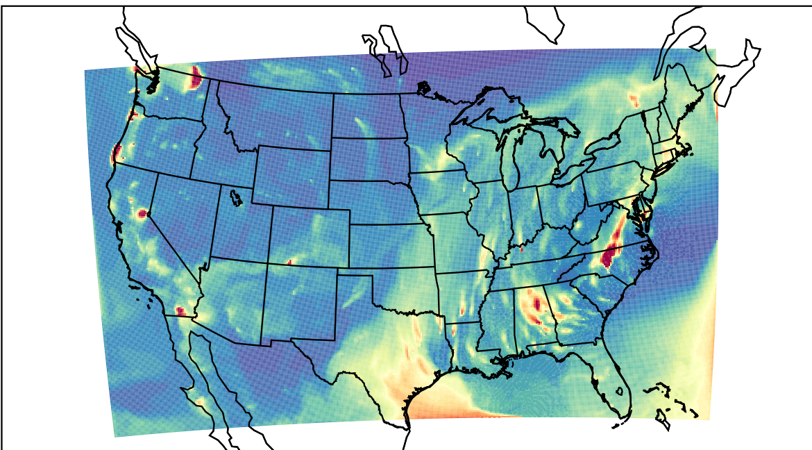
WRF 2023-10-27_05:00:00
