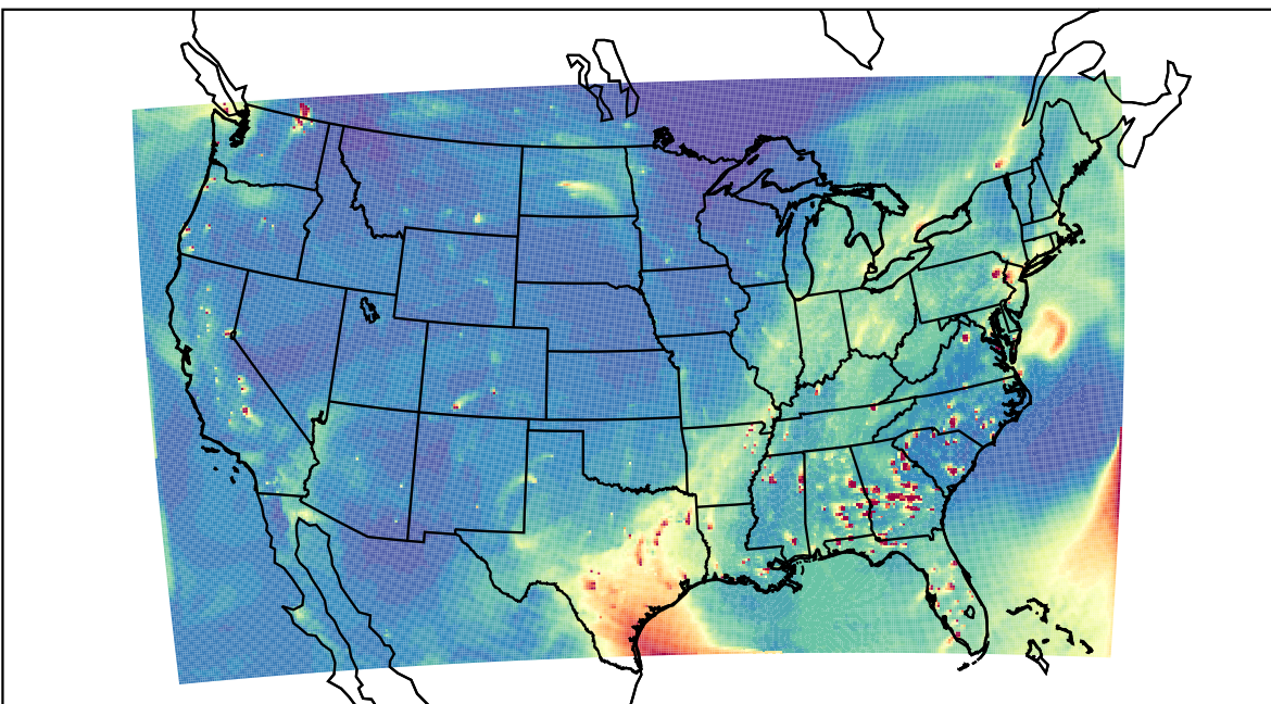
WRF 2023-10-27_23:00:00
