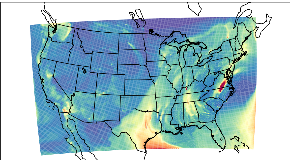
WRF 2023-10-27_10:00:00
