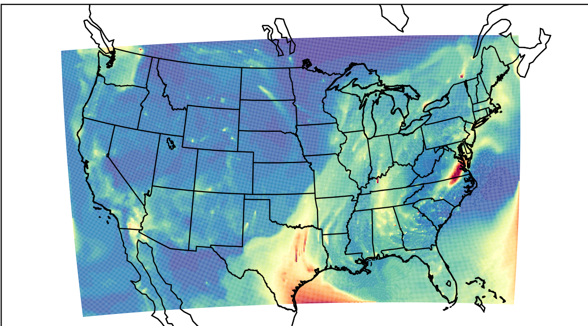
WRF 2023-10-27_13:00:00
