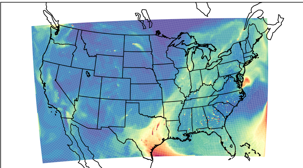
WRF 2023-10-27_19:00:00
