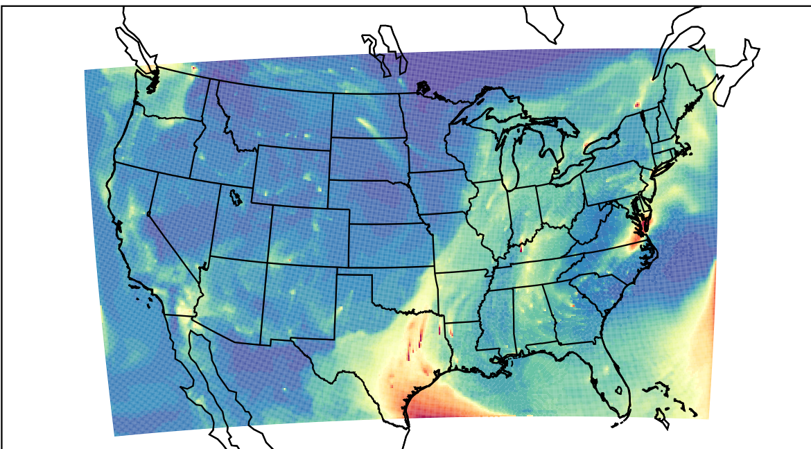
WRF 2023-10-27_15:00:00
