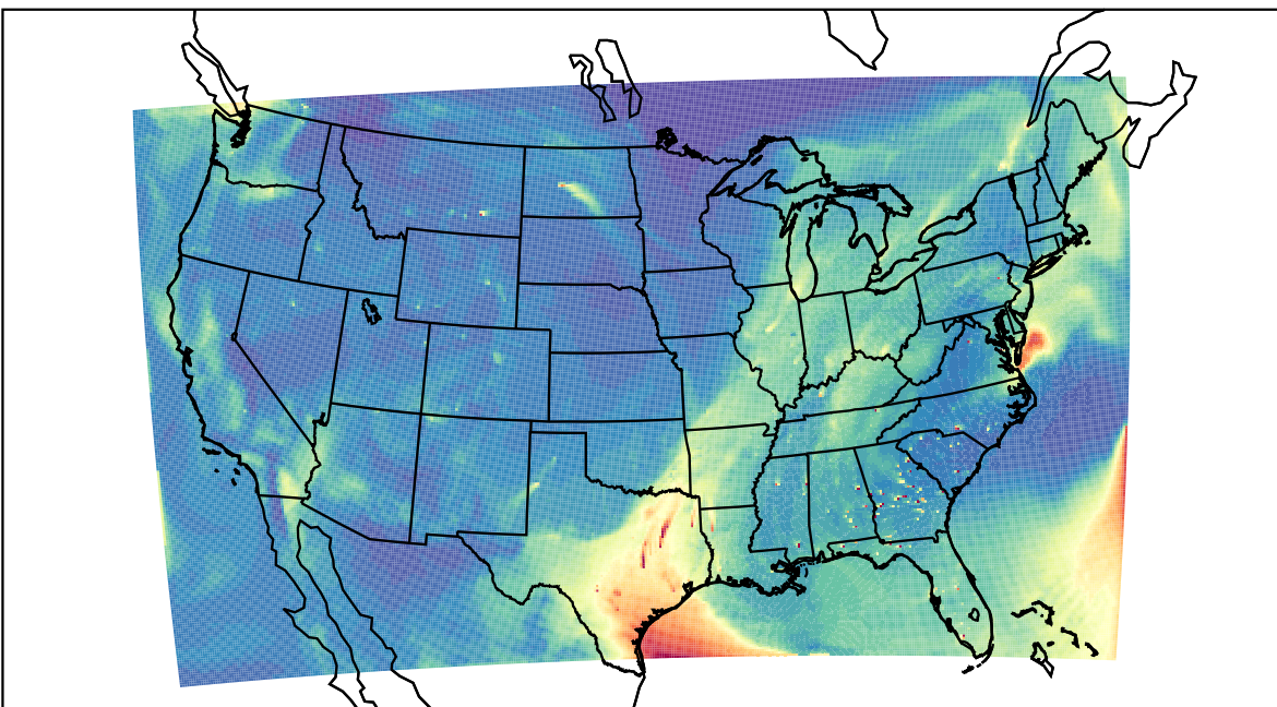
WRF 2023-10-27_18:00:00
