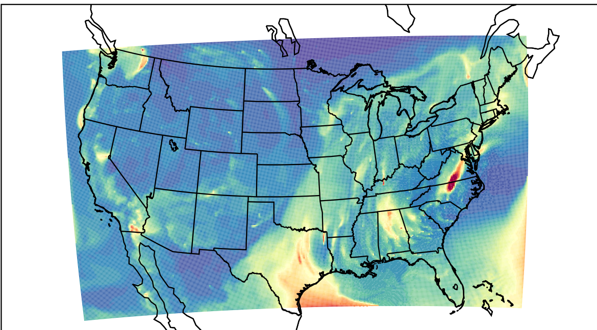
WRF 2023-10-27_08:00:00
