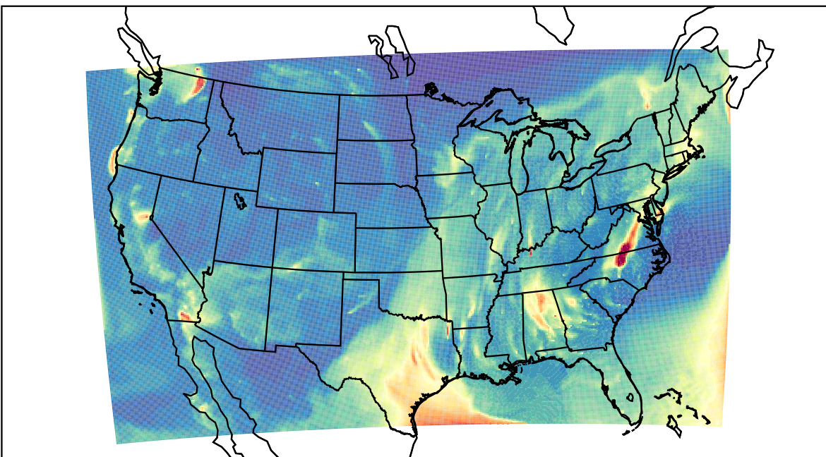
WRF 2023-10-27_07:00:00
