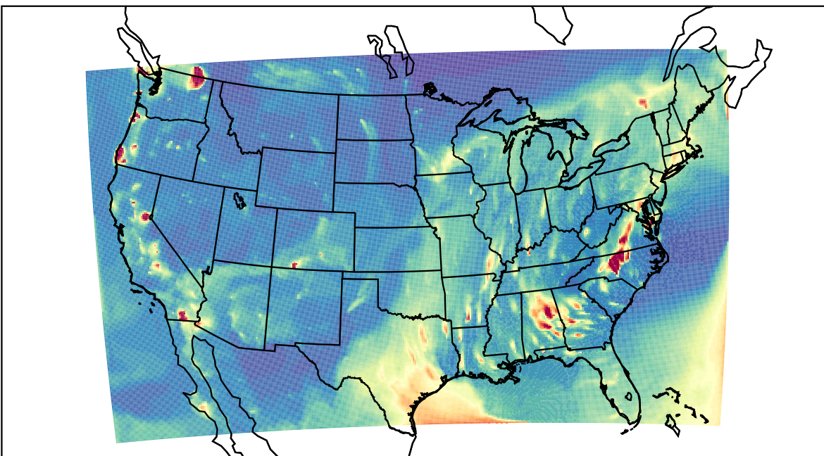
WRF 2023-10-27_04:00:00
