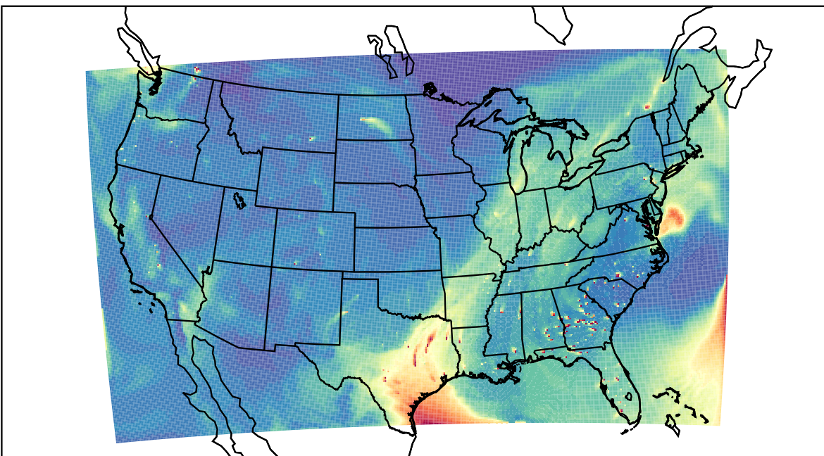
WRF 2023-10-27_20:00:00
