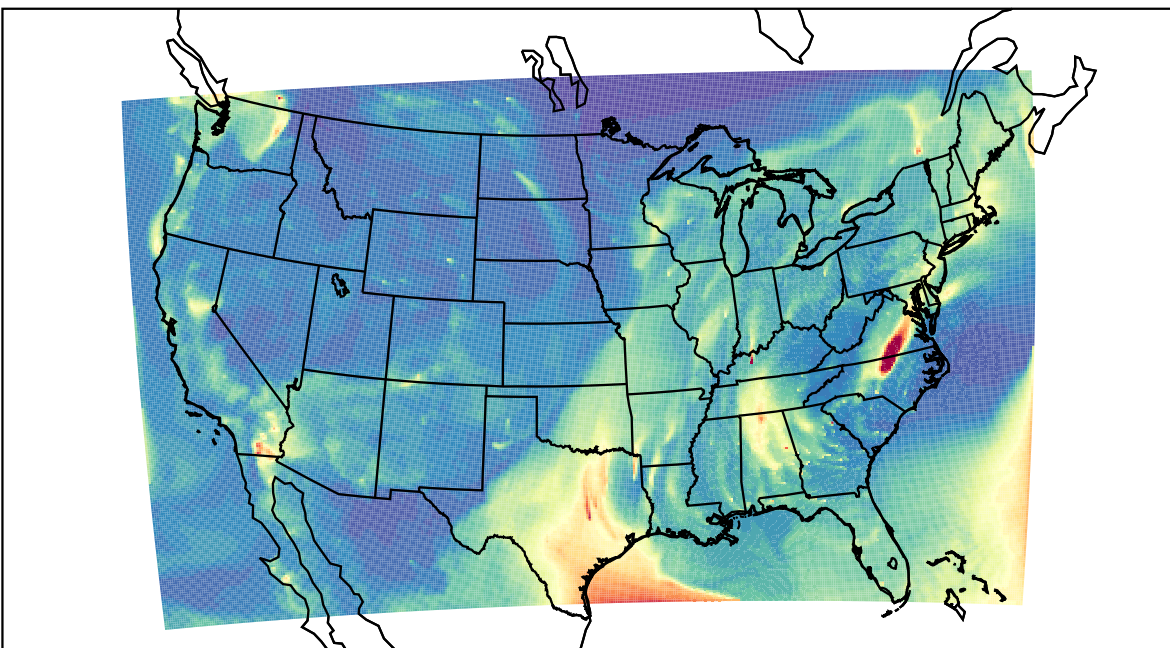
WRF 2023-10-27_09:00:00
