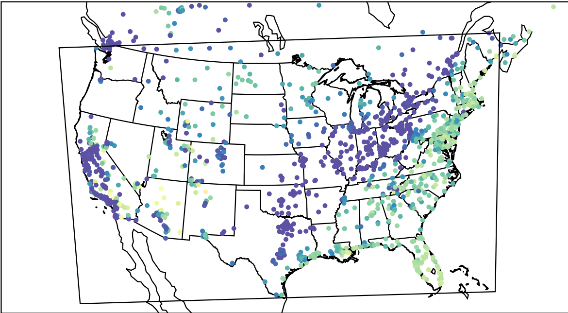
AirNOW (2023-10-28_15:00:00)
