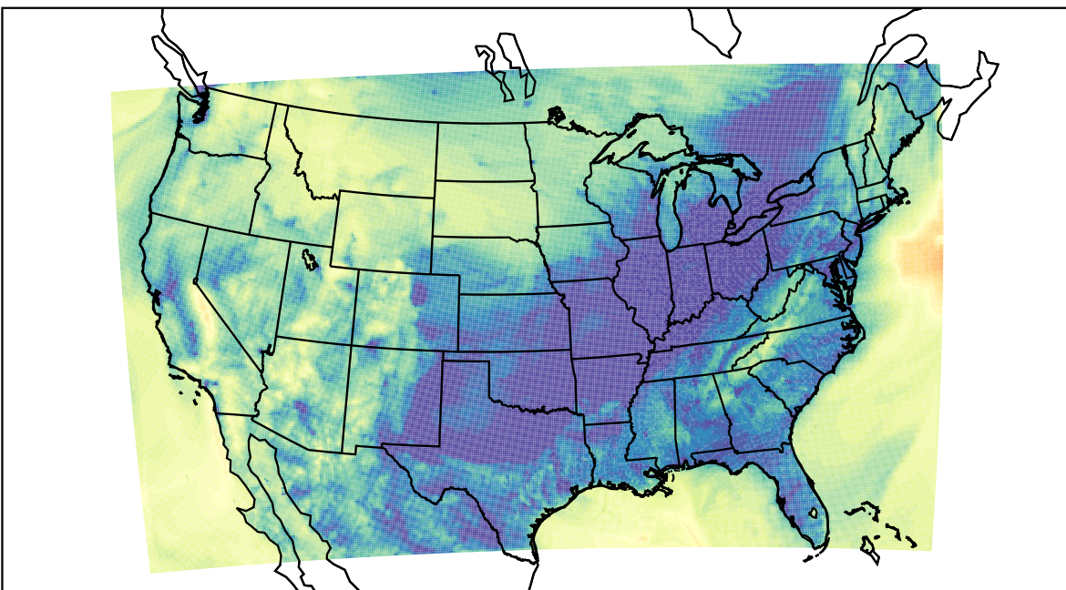
WRF (2023-10-28_13:00:00)
