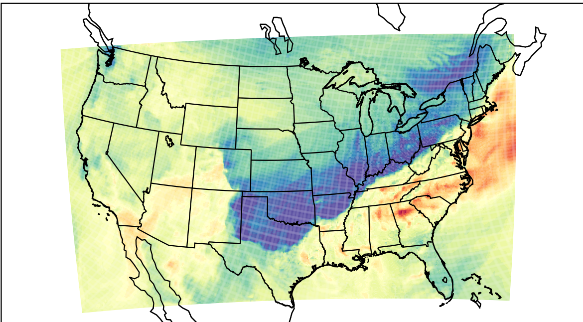
WRF (2023-10-28_21:00:00)
