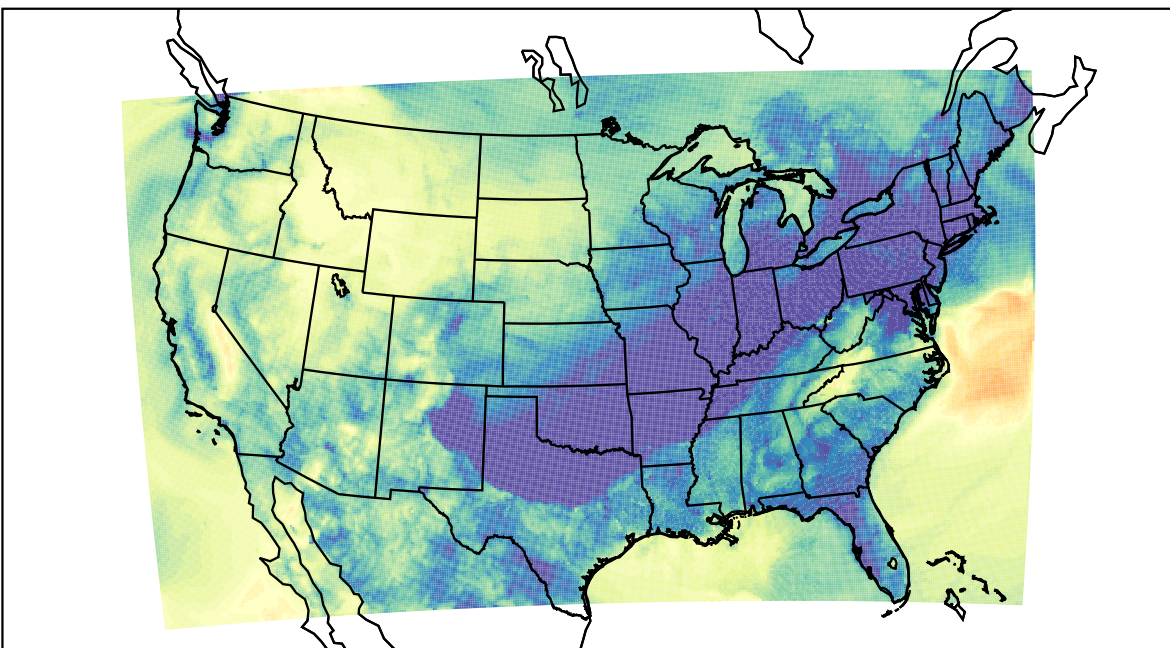
WRF (2023-10-29_11:00:00)
