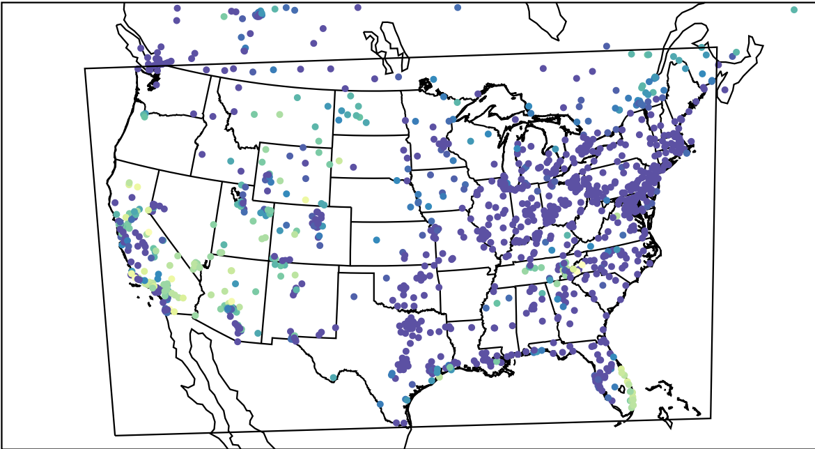
AirNOW (2023-10-29_12:00:00)
