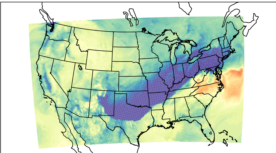
WRF (2023-10-29_16:00:00)
