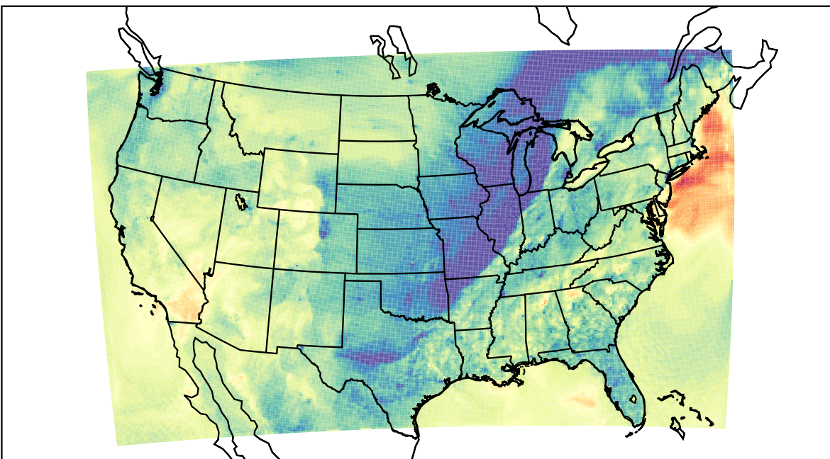
WRF (2023-10-28_00:00:00)
