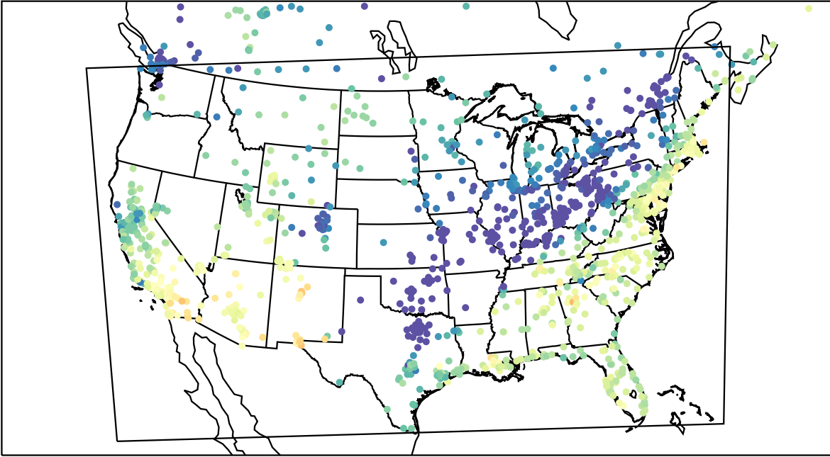
AirNOW (2023-10-28_19:00:00)
