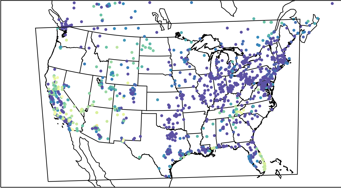
AirNOW (2023-10-29_08:00:00)
