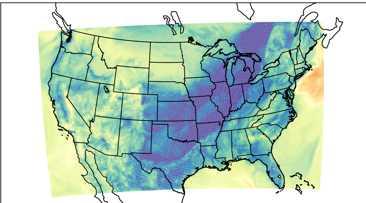
WRF (2023-10-28_07:00:00)
