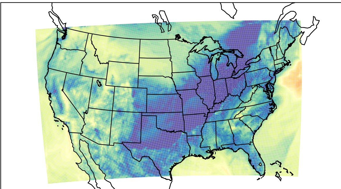
WRF (2023-10-28_10:00:00)
