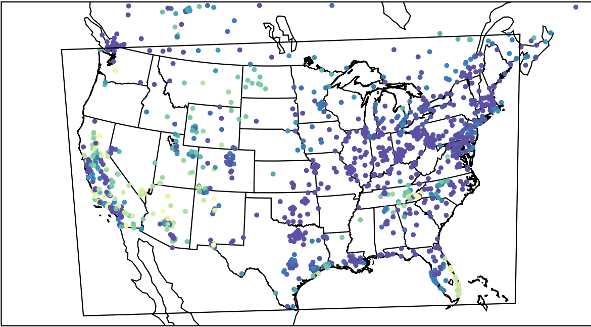
AirNOW (2023-10-29_07:00:00)
