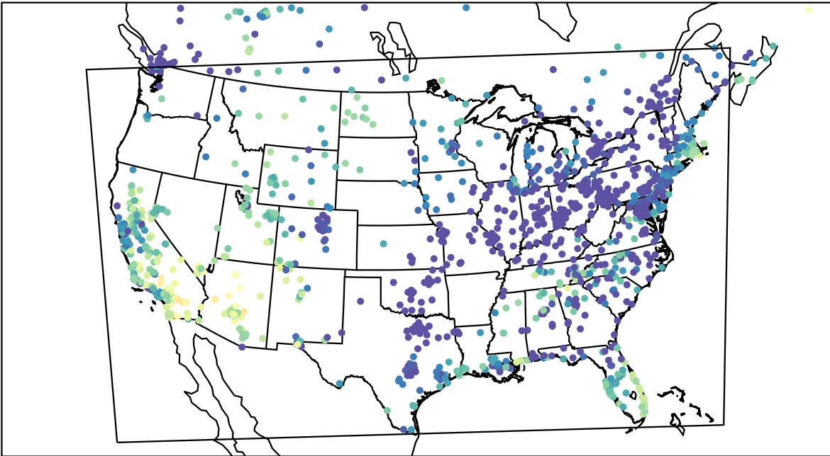
AirNOW (2023-10-29_02:00:00)
