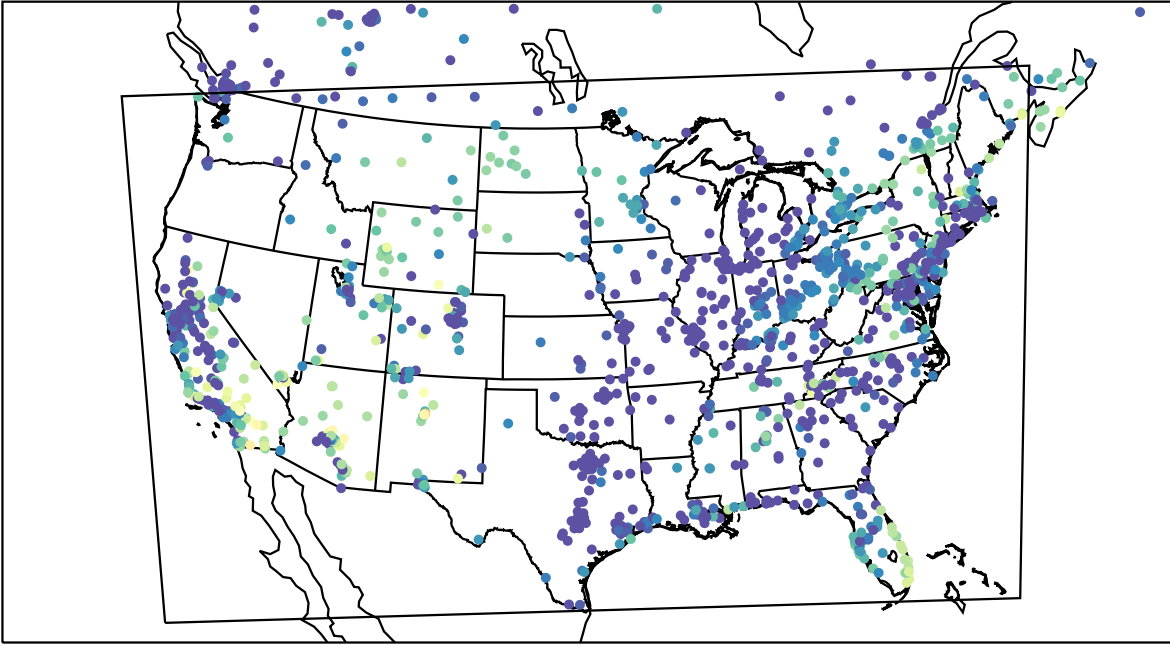
AirNOW (2023-10-28_04:00:00)
