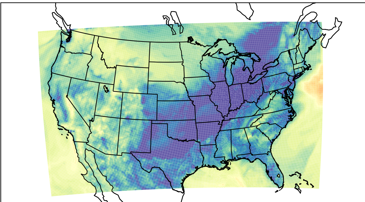
WRF (2023-10-28_11:00:00)
