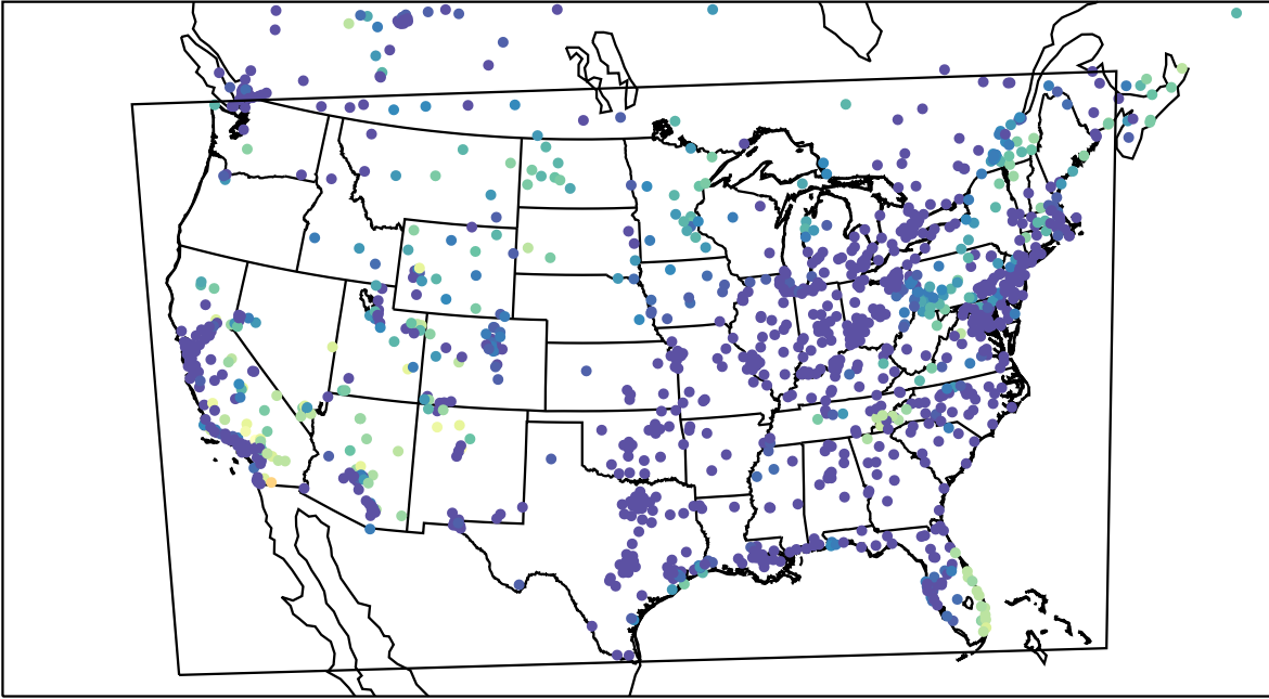
AirNOW (2023-10-28_12:00:00)
