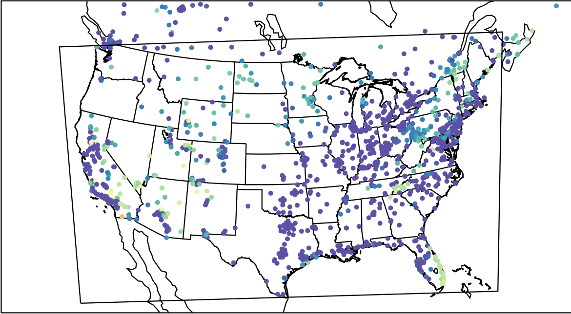
AirNOW (2023-10-28_11:00:00)
