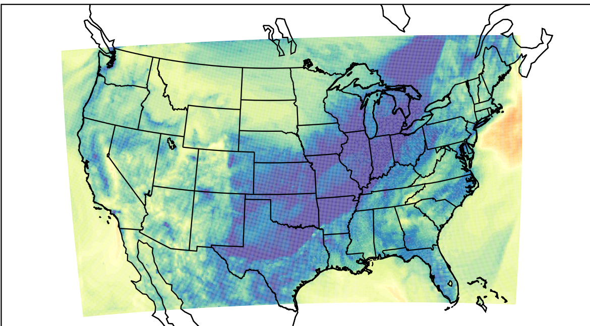
WRF (2023-10-28_08:00:00)
