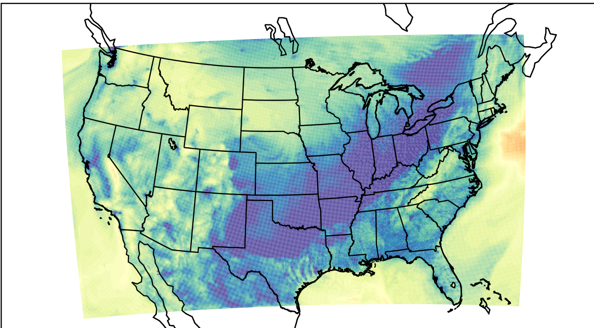
WRF (2023-10-28_14:00:00)
