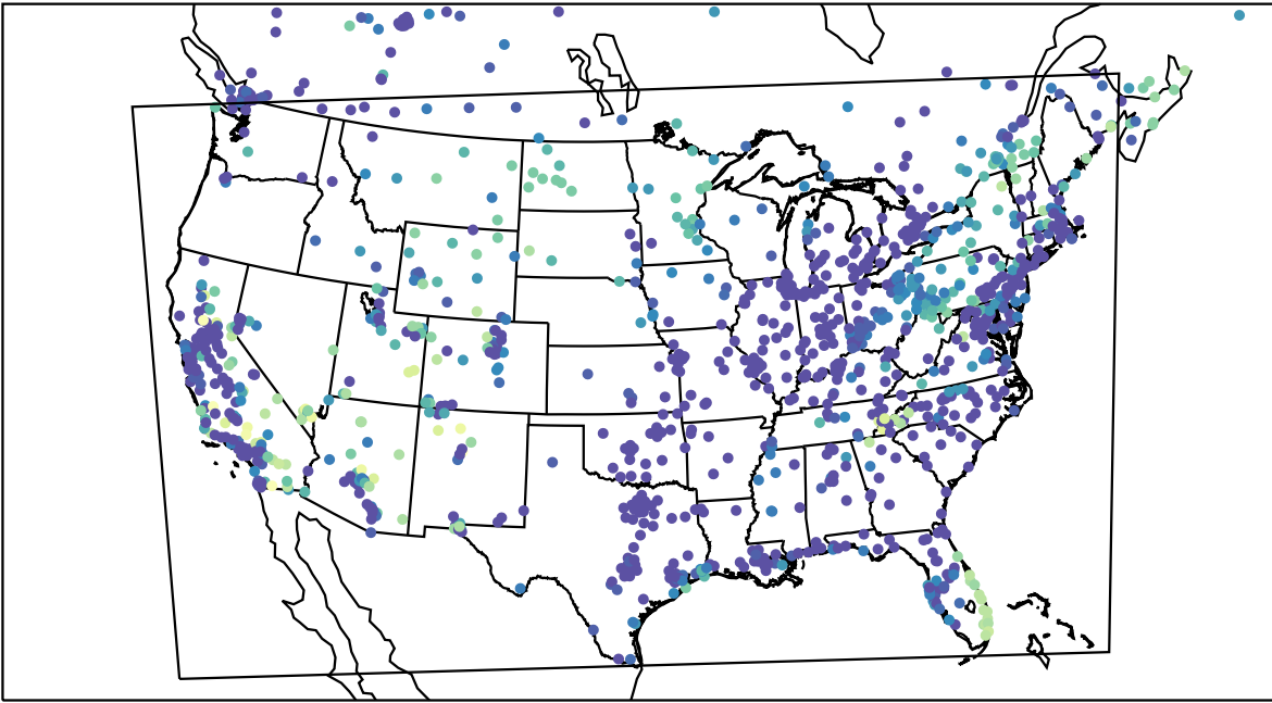
AirNOW (2023-10-28_09:00:00)
