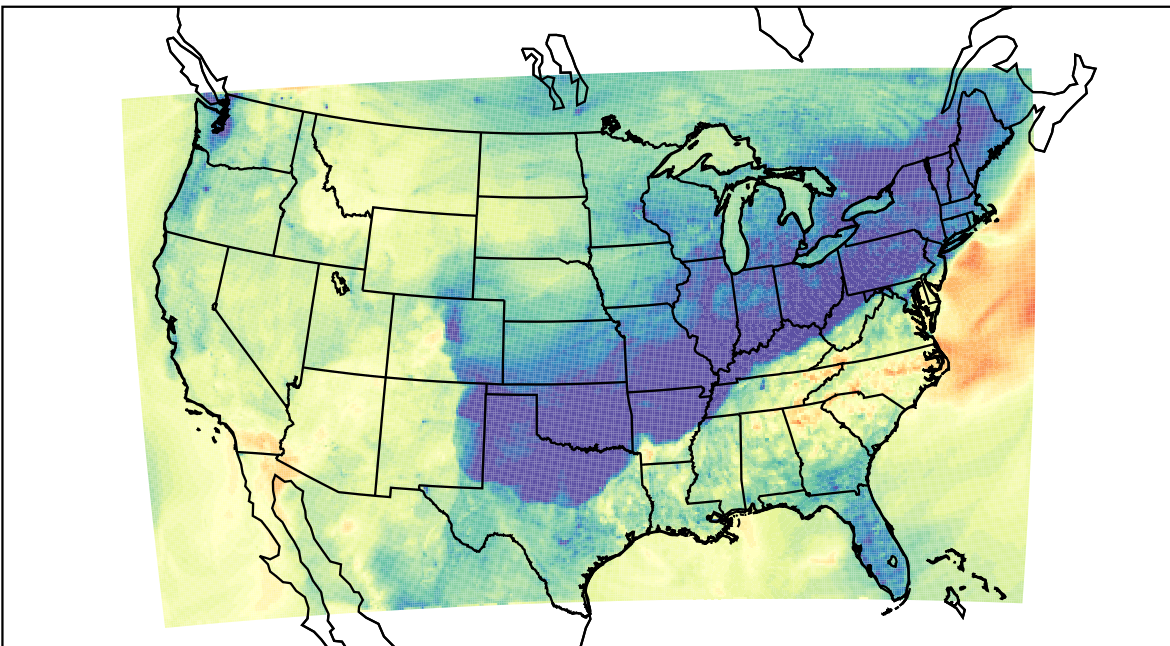
WRF (2023-10-29_00:00:00)
