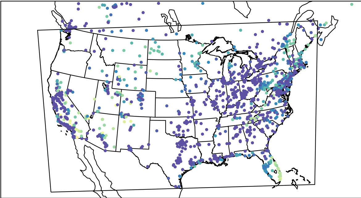
AirNOW (2023-10-28_13:00:00)
