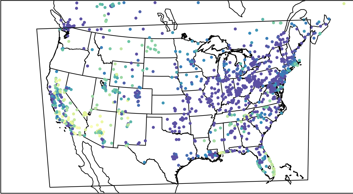
AirNOW (2023-10-29_04:00:00)
