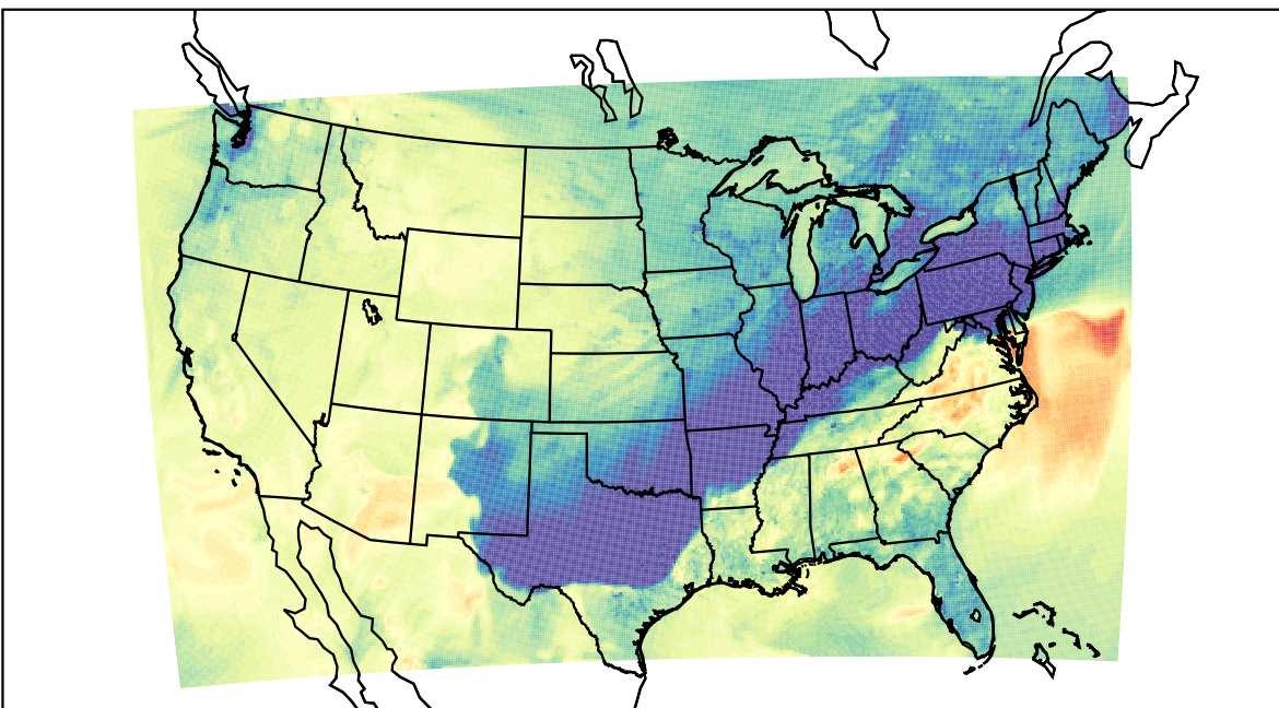
WRF (2023-10-29_23:00:00)
