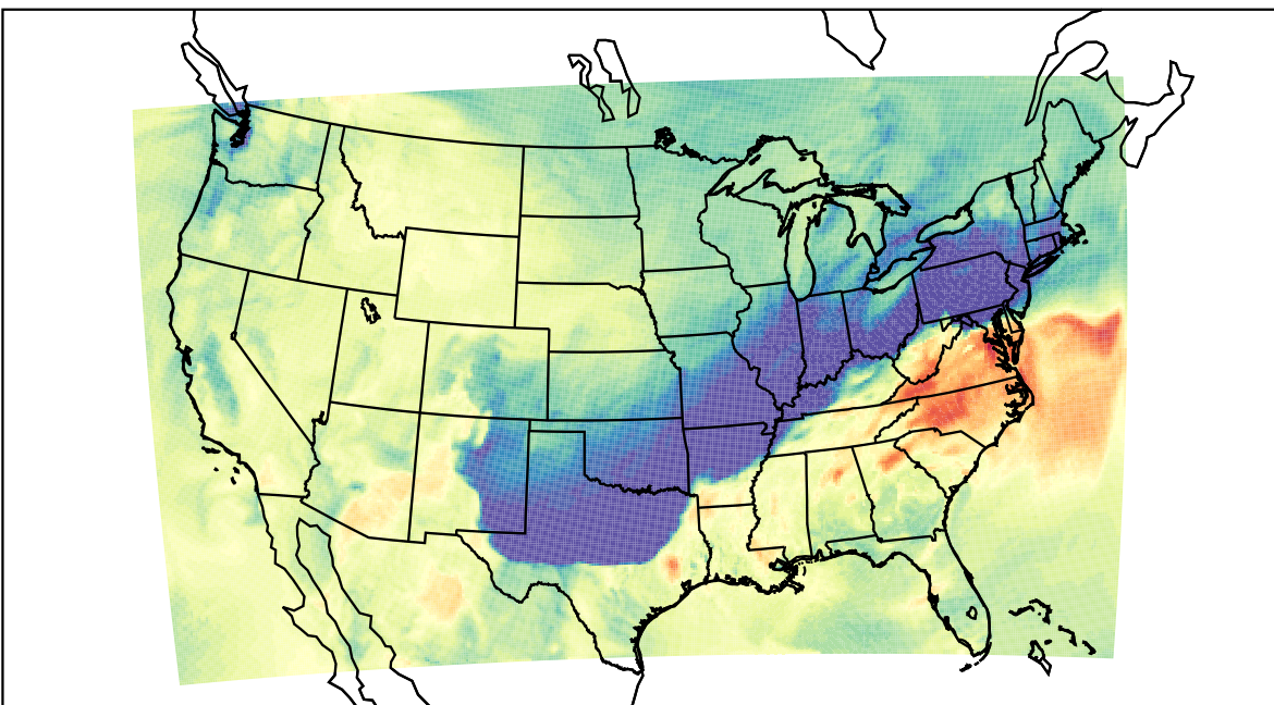
WRF (2023-10-29_19:00:00)
