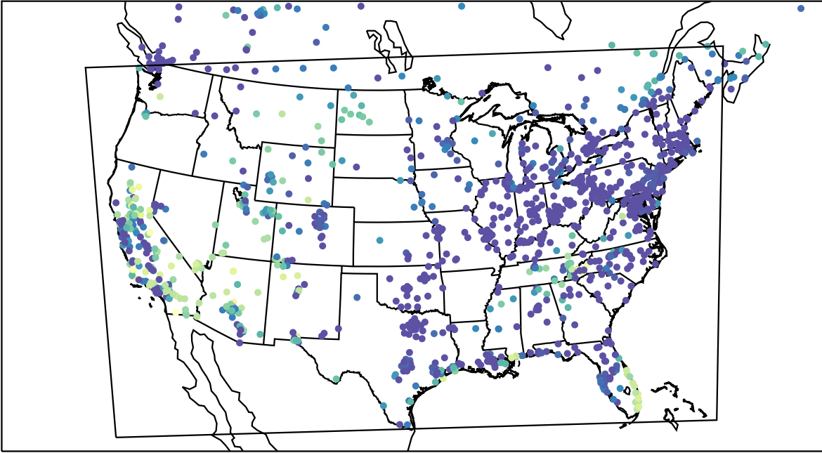
AirNOW (2023-10-29_09:00:00)
