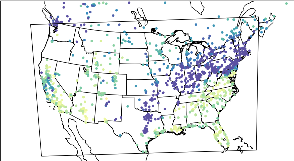
AirNOW (2023-10-29_17:00:00)
