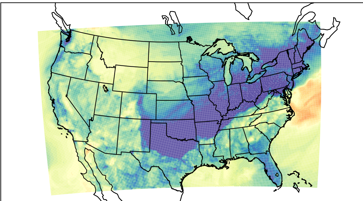
WRF (2023-10-29_04:00:00)
