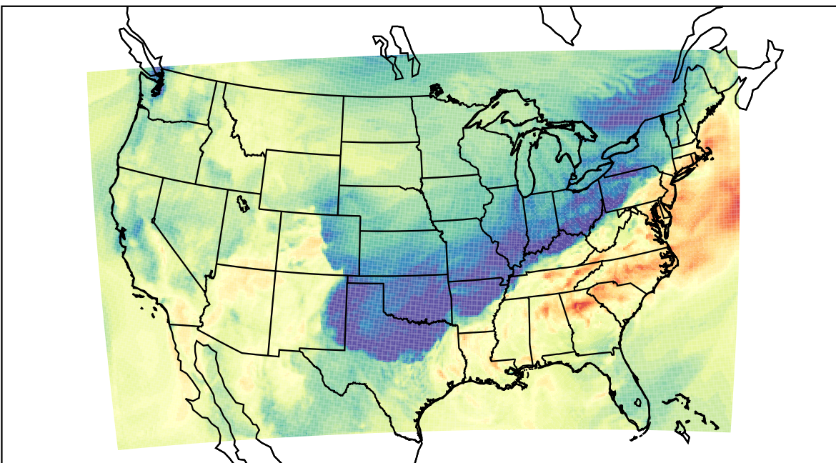
WRF (2023-10-28_19:00:00)
