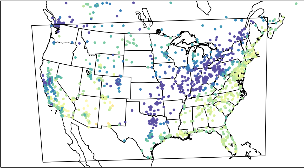
AirNOW (2023-10-28_17:00:00)
