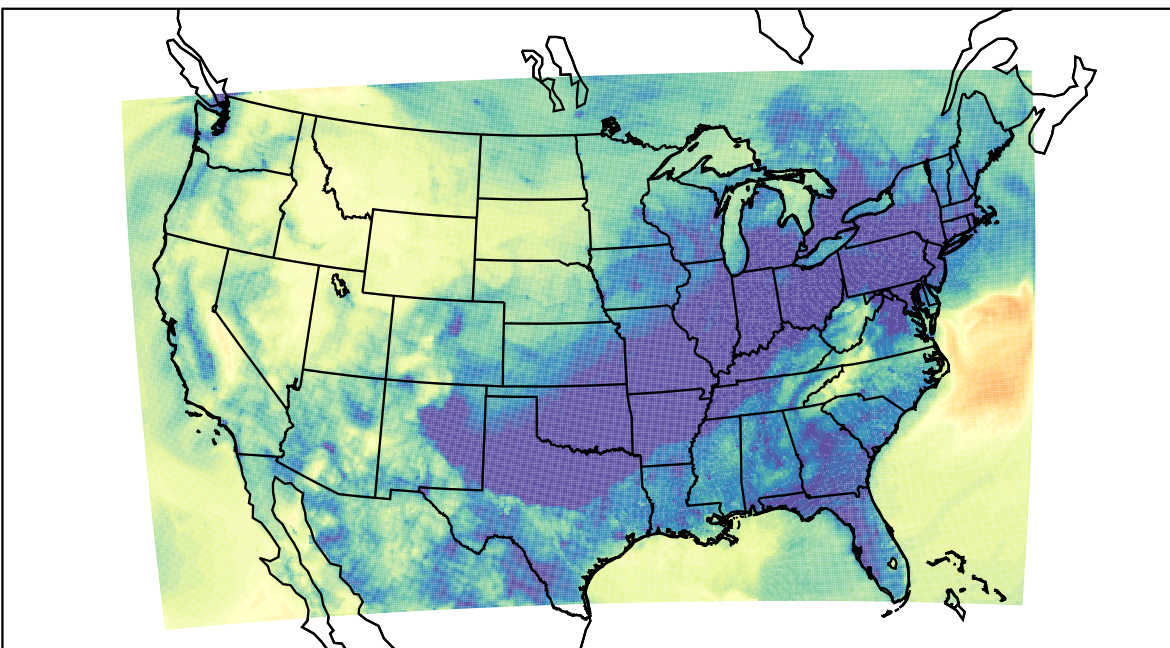
WRF (2023-10-29_13:00:00)
