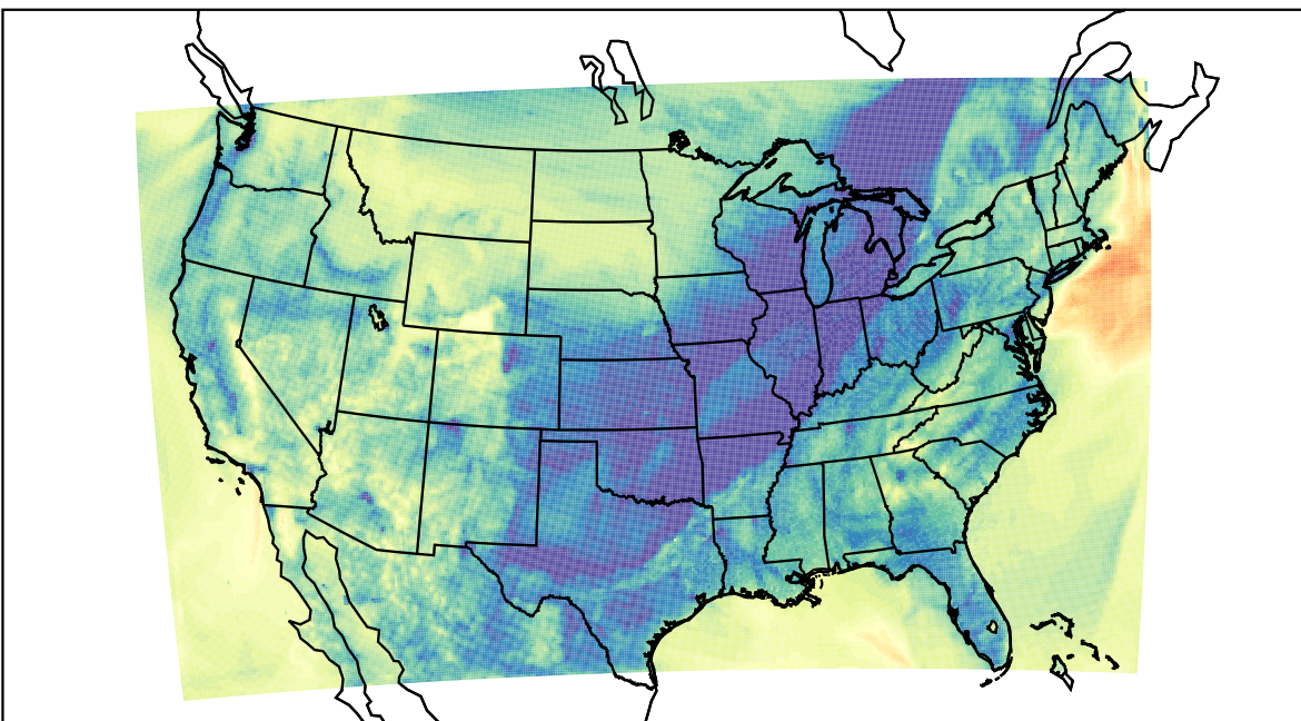
WRF (2023-10-28_06:00:00)
