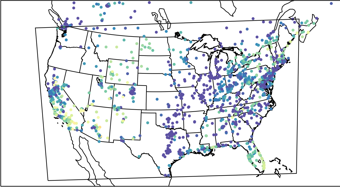
AirNOW (2023-10-28_02:00:00)
