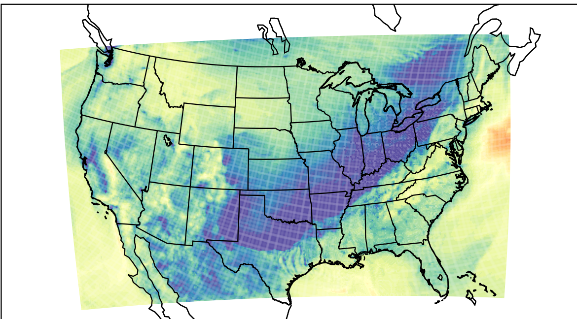
WRF (2023-10-28_15:00:00)
