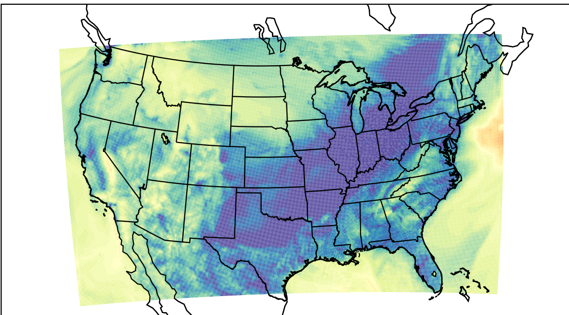
WRF (2023-10-28_12:00:00)
