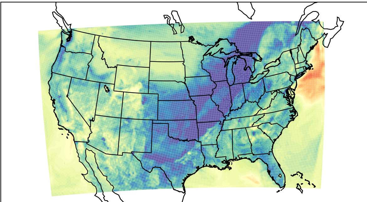
WRF (2023-10-28_04:00:00)
