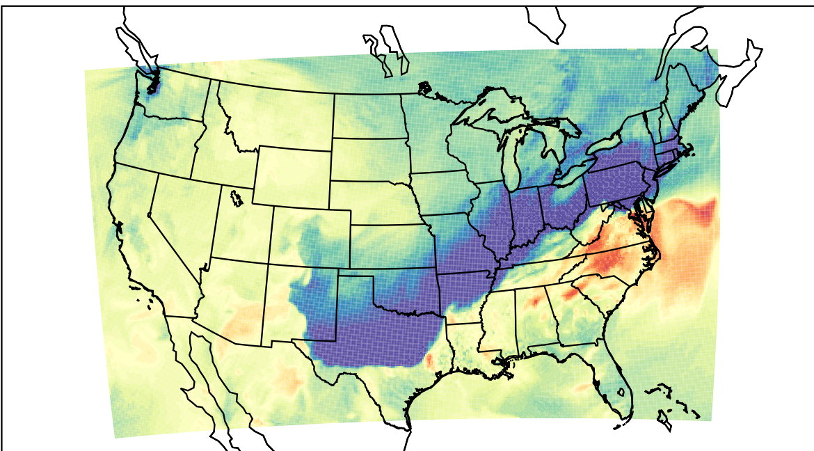
WRF (2023-10-29_21:00:00)
