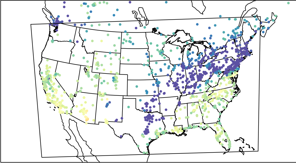
AirNOW (2023-10-29_19:00:00)
