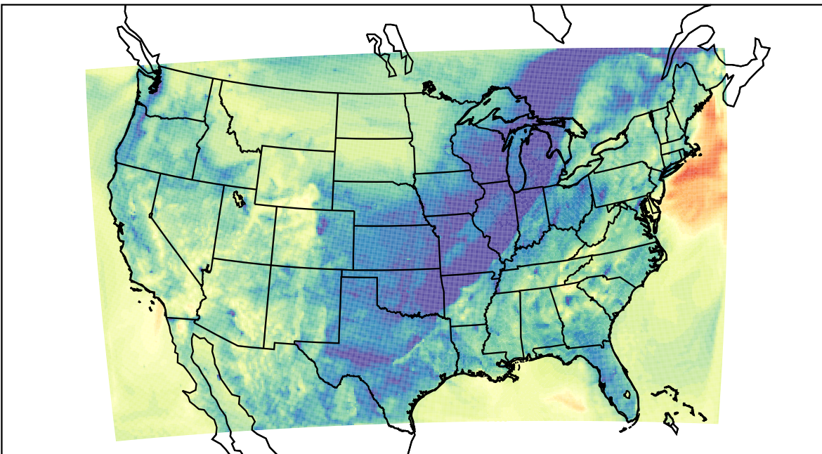
WRF (2023-10-28_03:00:00)
