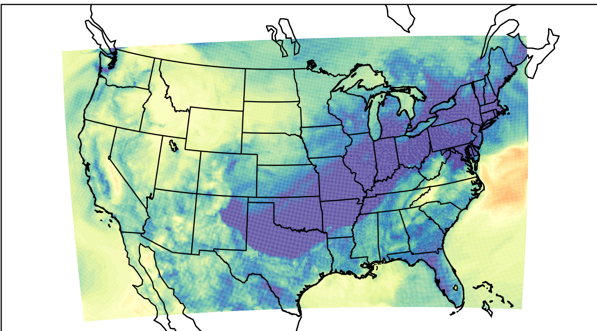
WRF (2023-10-29_10:00:00)
