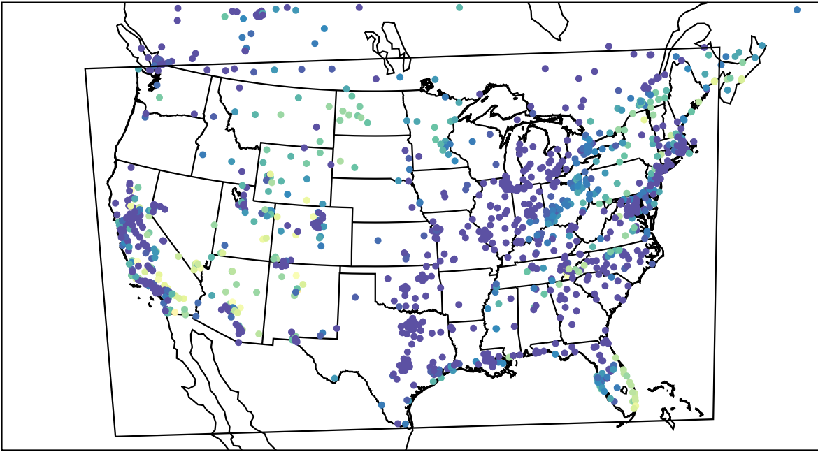
AirNOW (2023-10-28_06:00:00)
