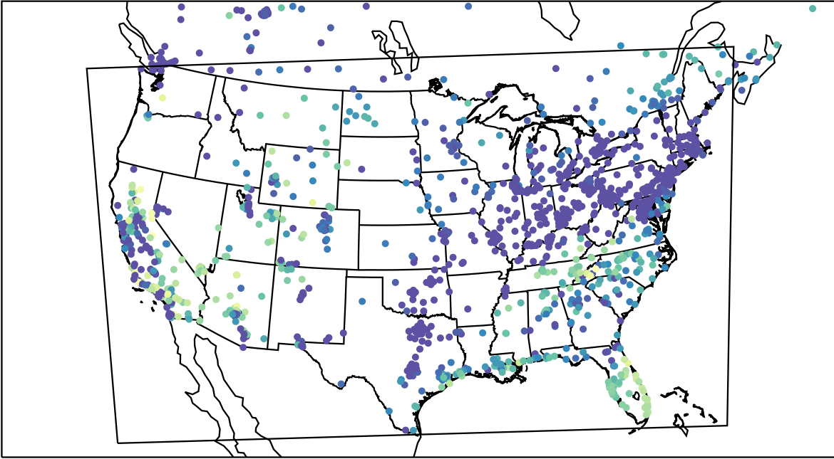
AirNOW (2023-10-29_14:00:00)
