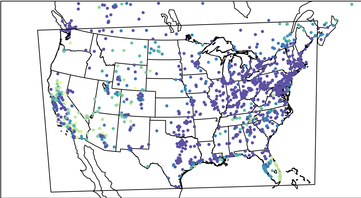
AirNOW (2023-10-29_13:00:00)
