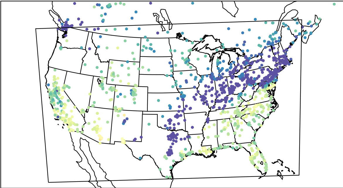
AirNOW (2023-10-29_18:00:00)
