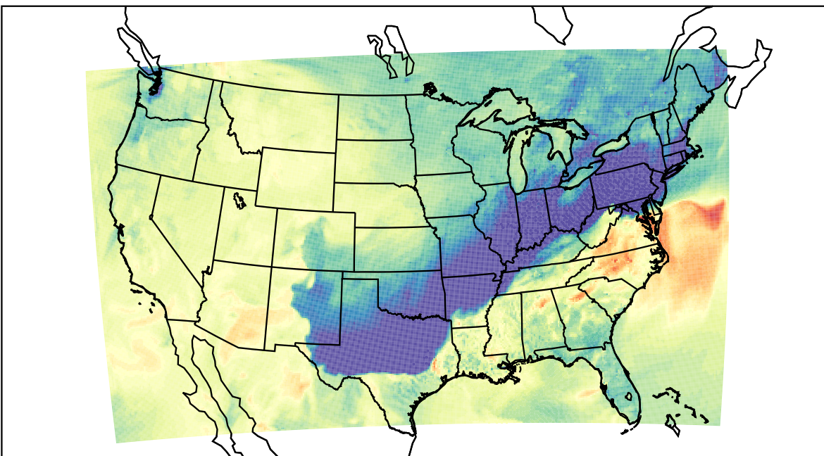
WRF (2023-10-29_22:00:00)
