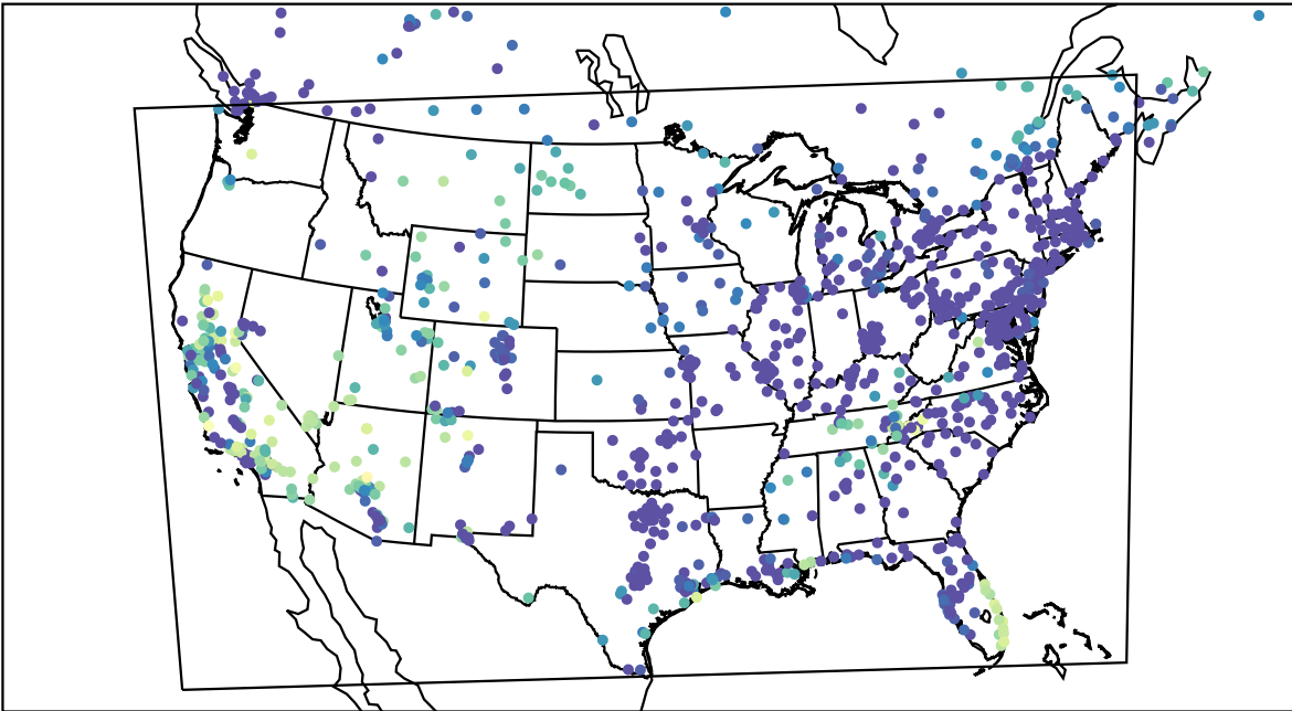
AirNOW (2023-10-29_10:00:00)
