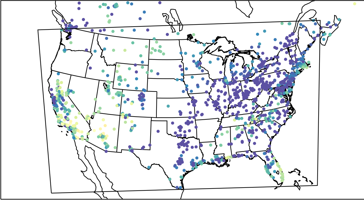
AirNOW (2023-10-29_03:00:00)
