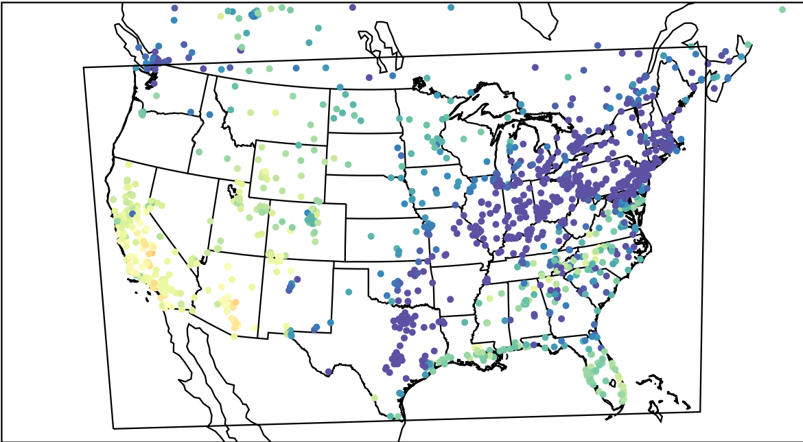
AirNOW (2023-10-29_23:00:00)
