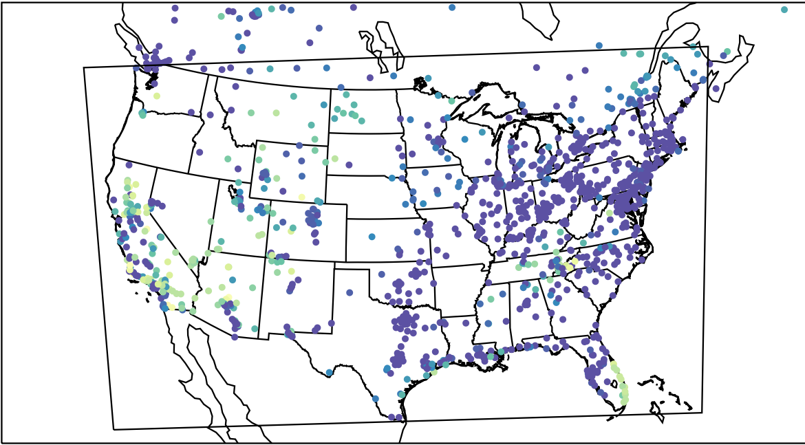
AirNOW (2023-10-29_11:00:00)
