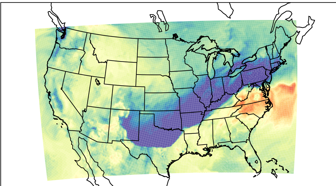
WRF (2023-10-29_17:00:00)
