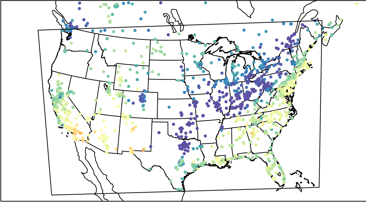
AirNOW (2023-10-28_20:00:00)
