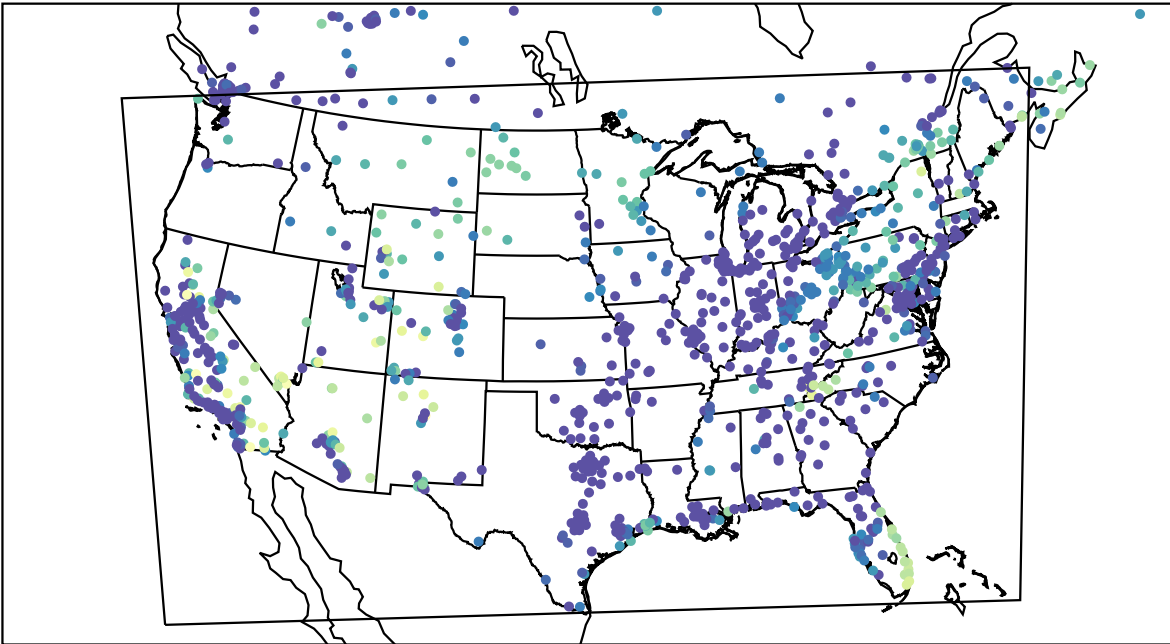
AirNOW (2023-10-28_08:00:00)
