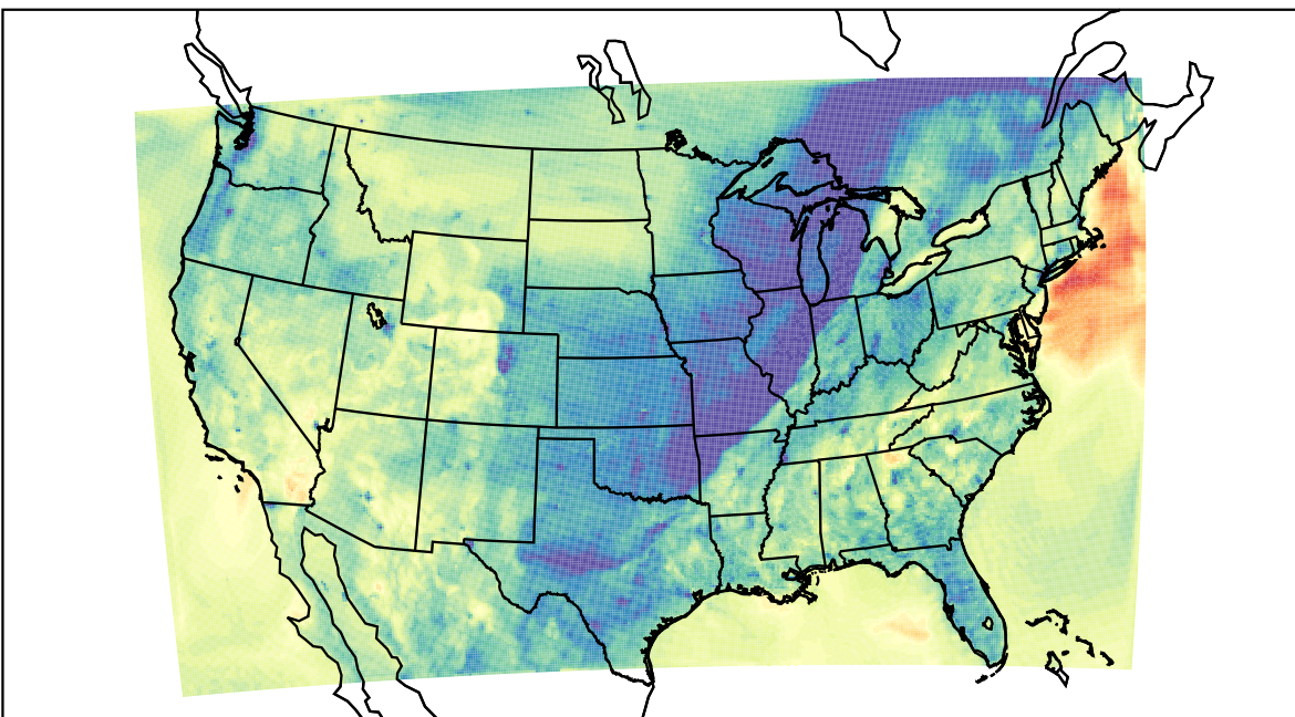
WRF (2023-10-28_01:00:00)
