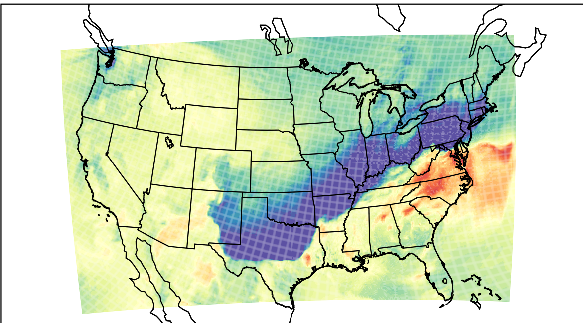
WRF (2023-10-29_20:00:00)
