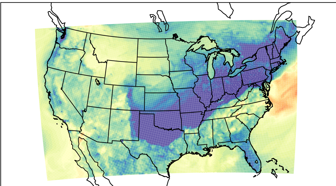
WRF (2023-10-29_03:00:00)
