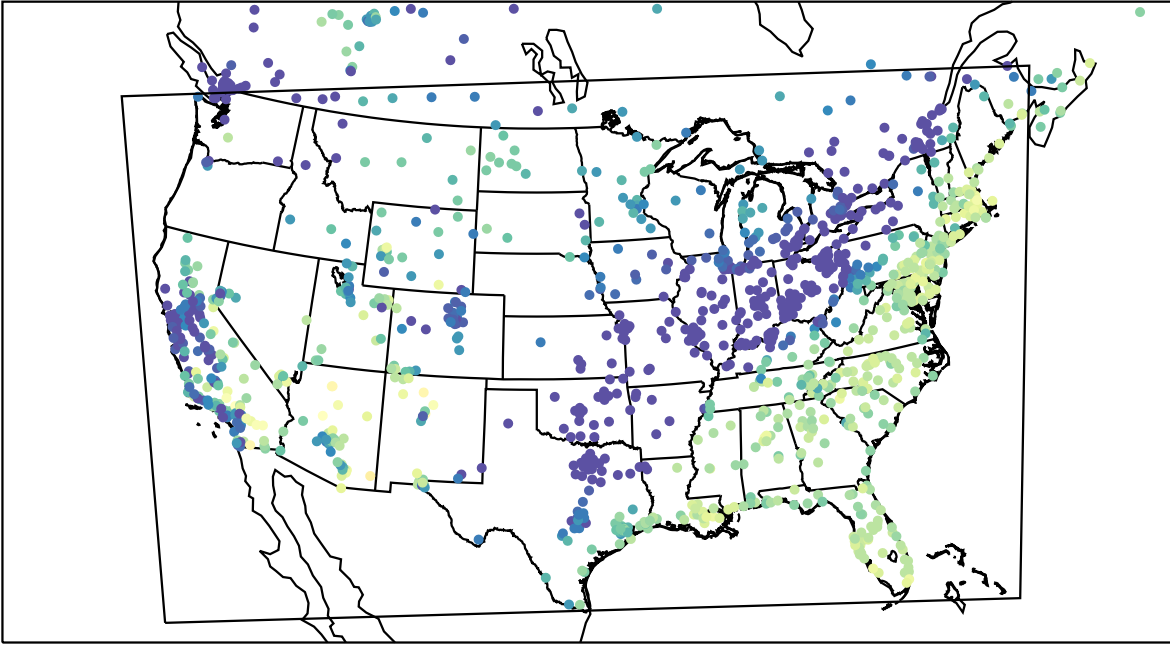
AirNOW (2023-10-28_16:00:00)
