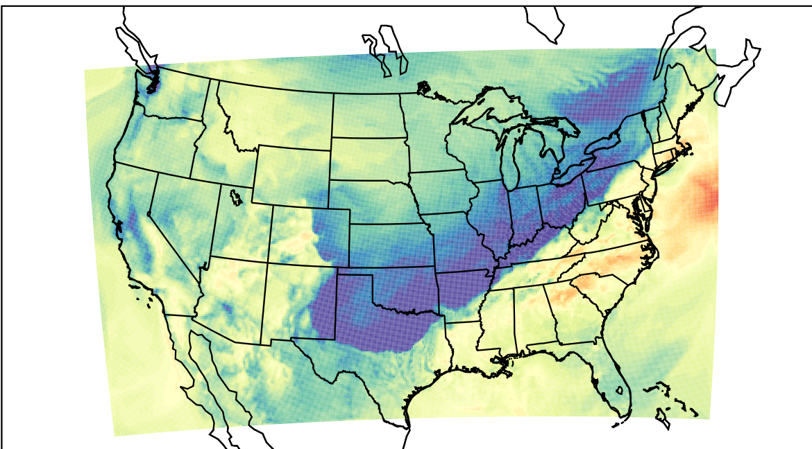
WRF (2023-10-28_17:00:00)
