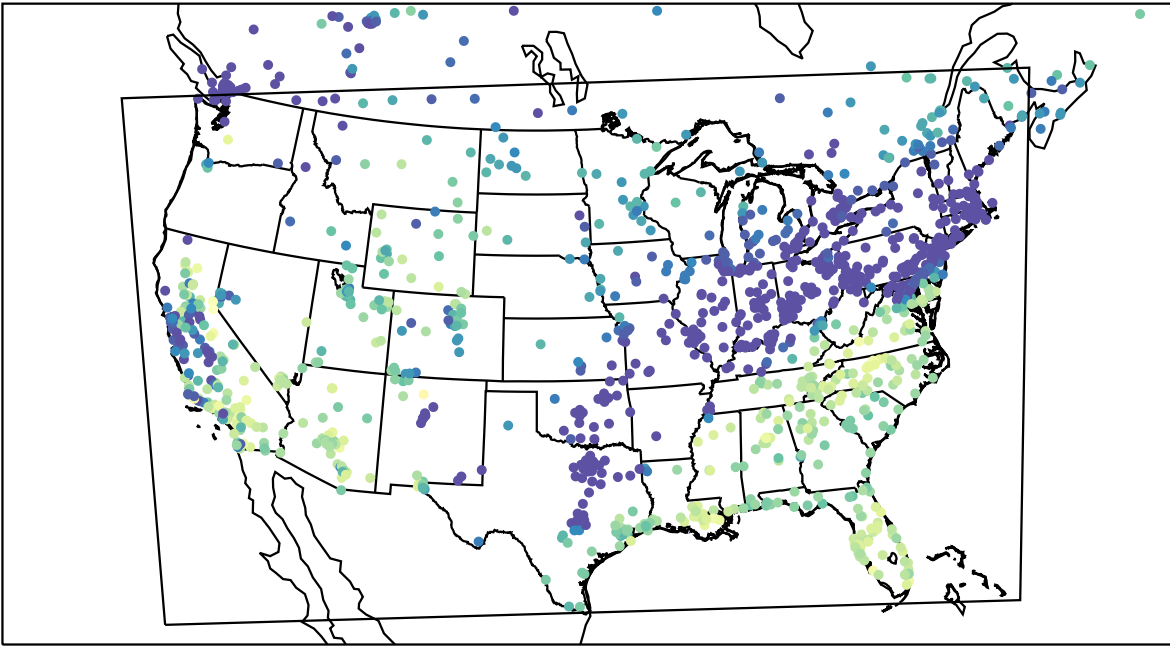
AirNOW (2023-10-29_16:00:00)
