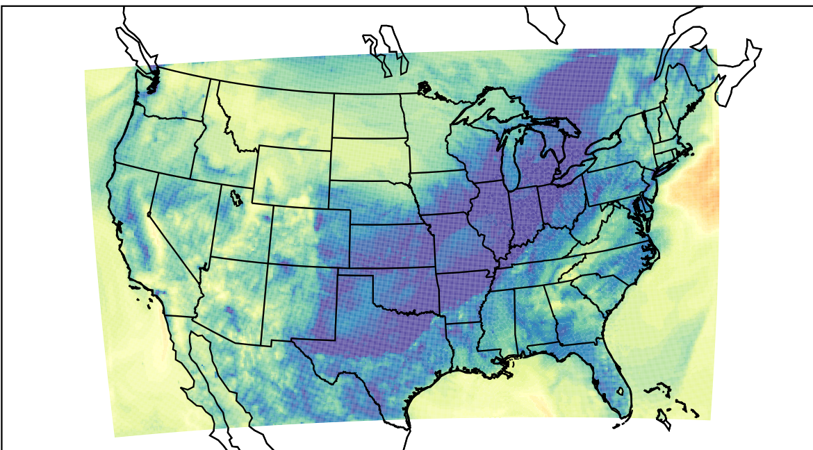
WRF (2023-10-28_09:00:00)
