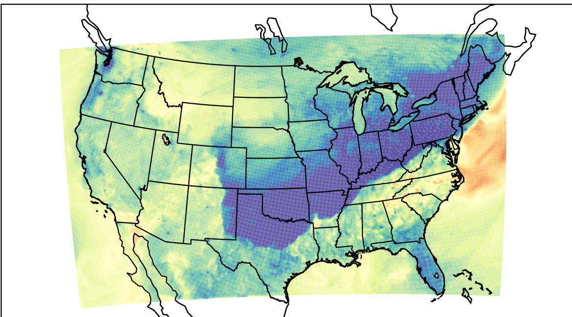
WRF (2023-10-29_01:00:00)
