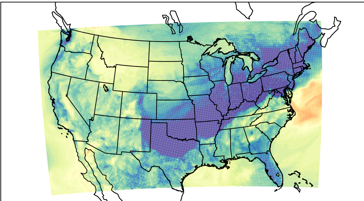
WRF (2023-10-29_05:00:00)
