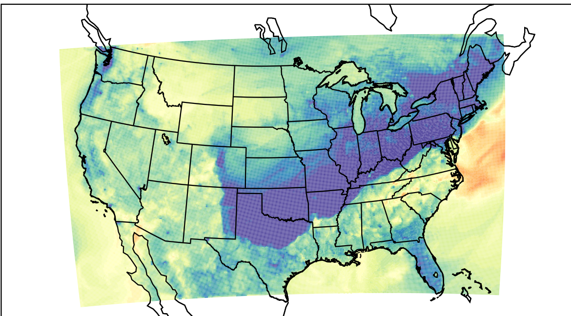
WRF (2023-10-29_02:00:00)
