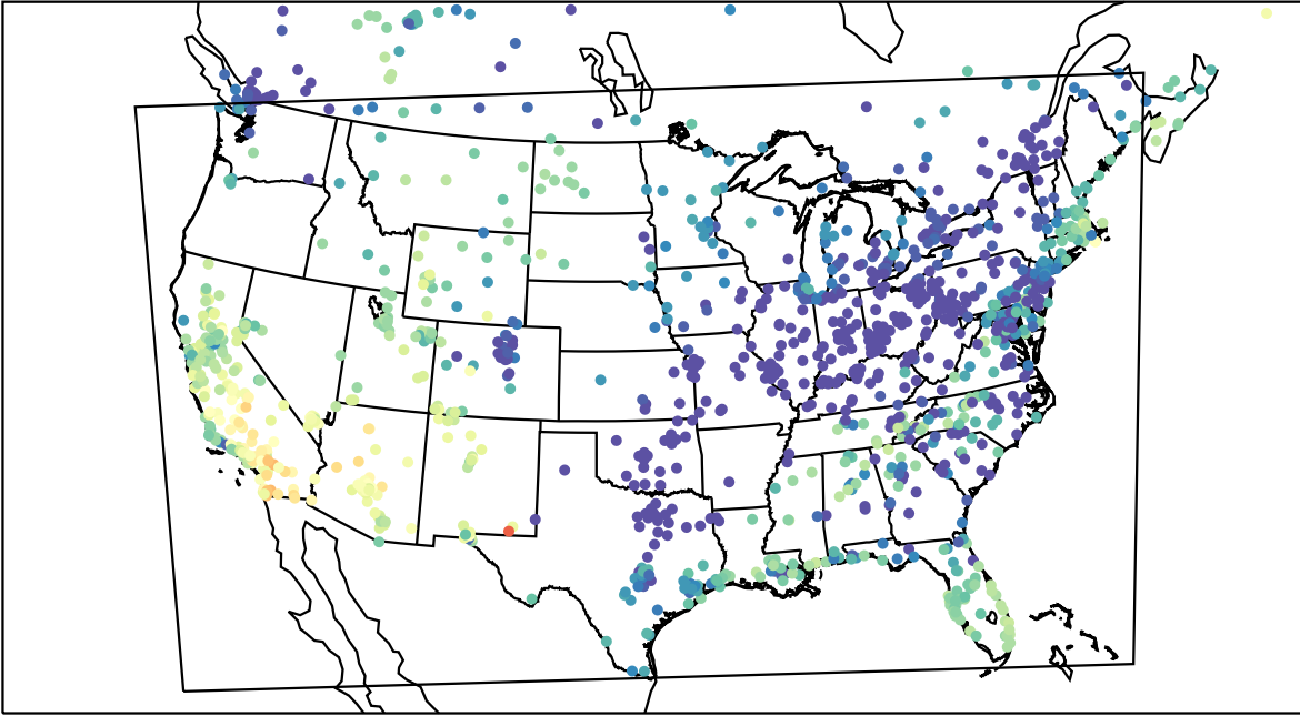
AirNOW (2023-10-29_00:00:00)
