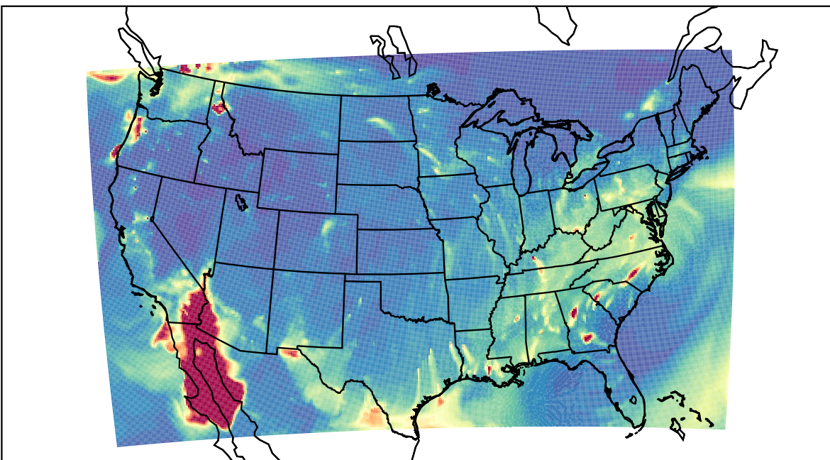
WRF 2023-10-30_04:00:00
