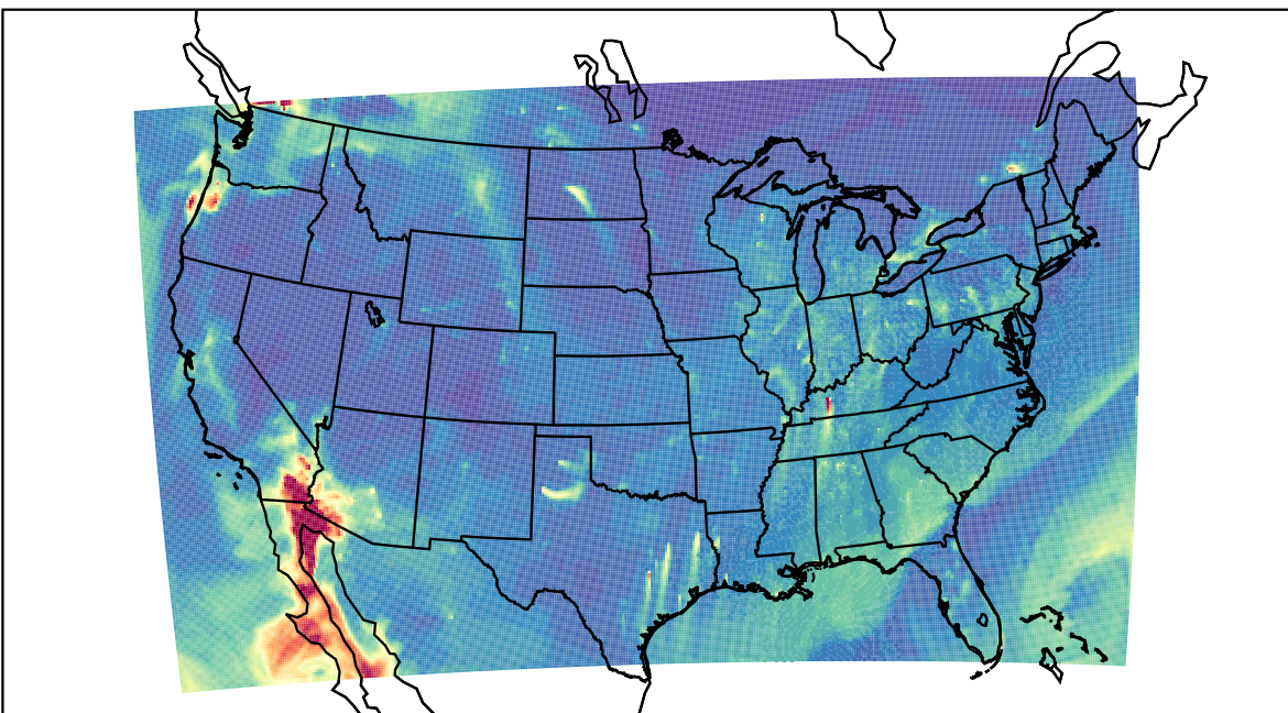
WRF 2023-10-31_12:00:00
