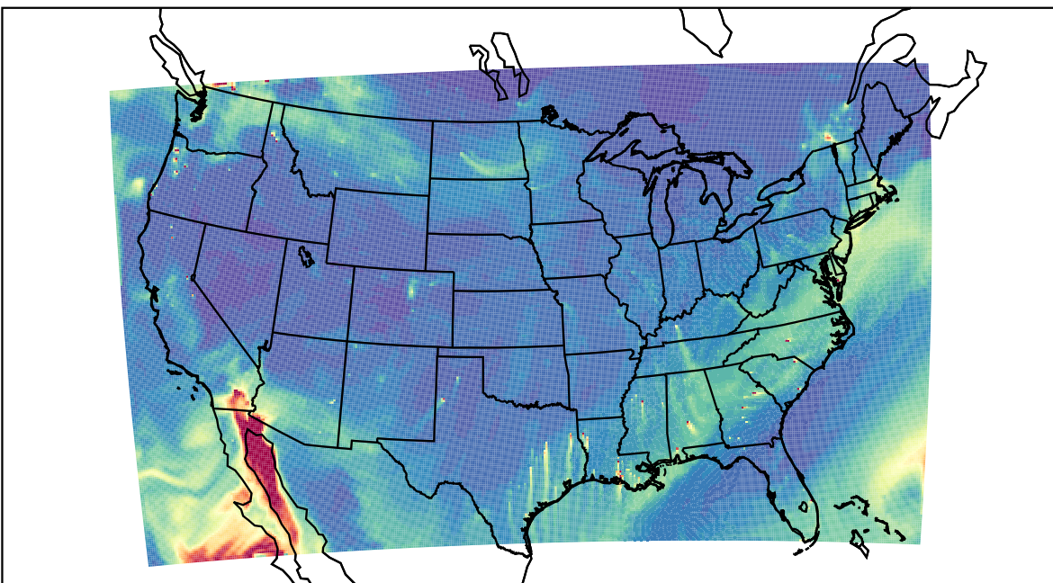
WRF 2023-10-30_21:00:00
