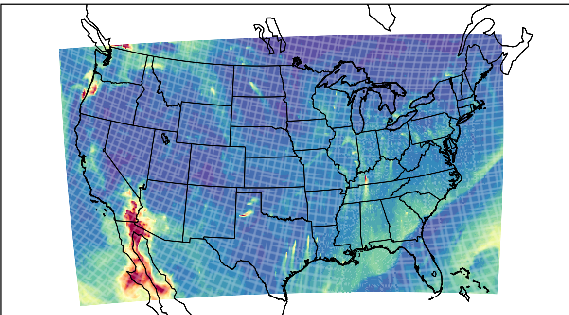
WRF 2023-10-31_09:00:00
