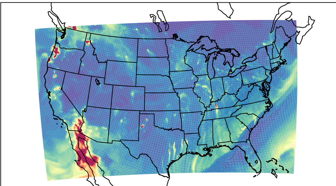
WRF 2023-10-31_04:00:00
