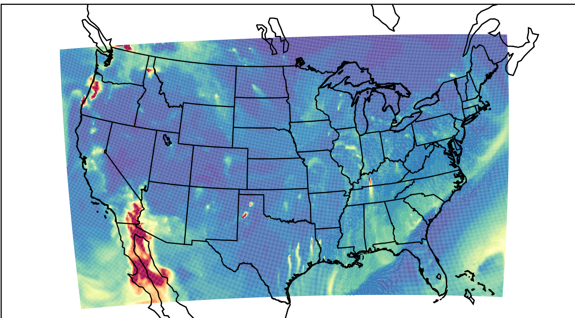
WRF 2023-10-31_05:00:00
