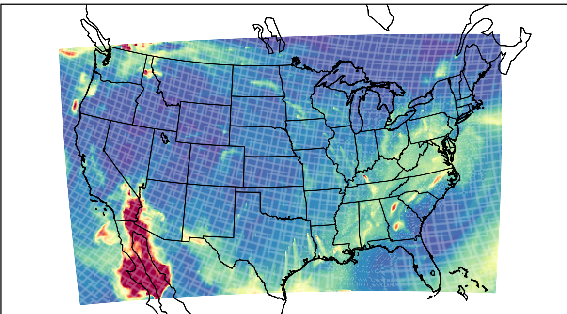
WRF 2023-10-30_07:00:00
