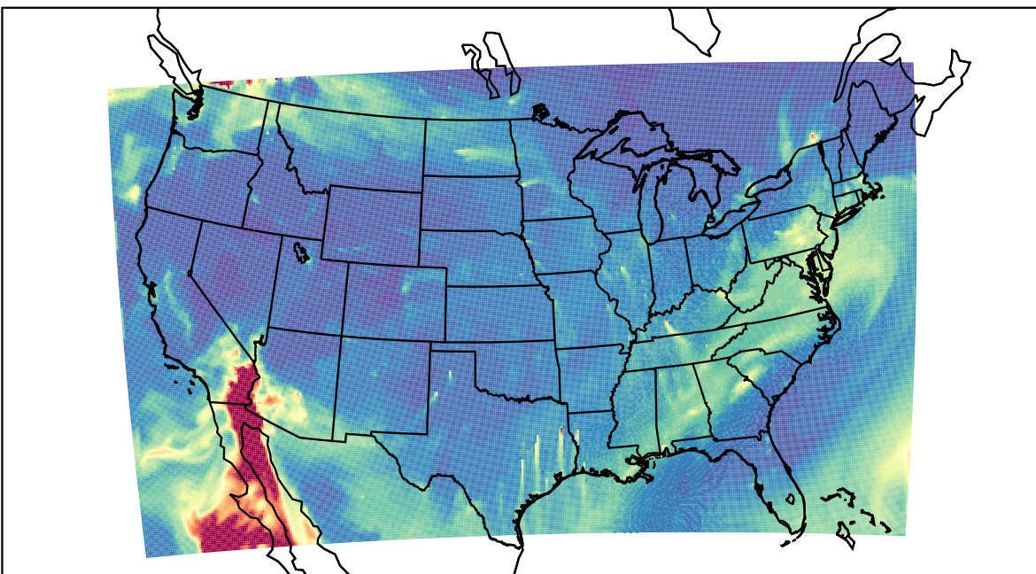
WRF 2023-10-30_15:00:00
