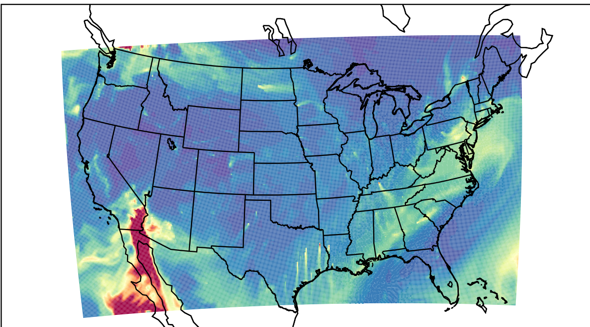
WRF 2023-10-30_16:00:00
