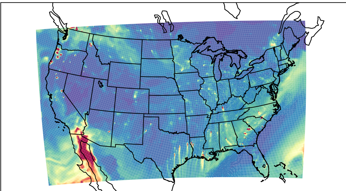
WRF 2023-10-31_00:00:00
