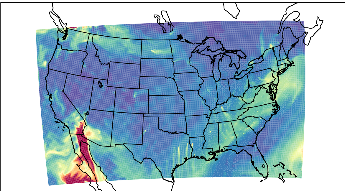
WRF 2023-10-30_17:00:00
