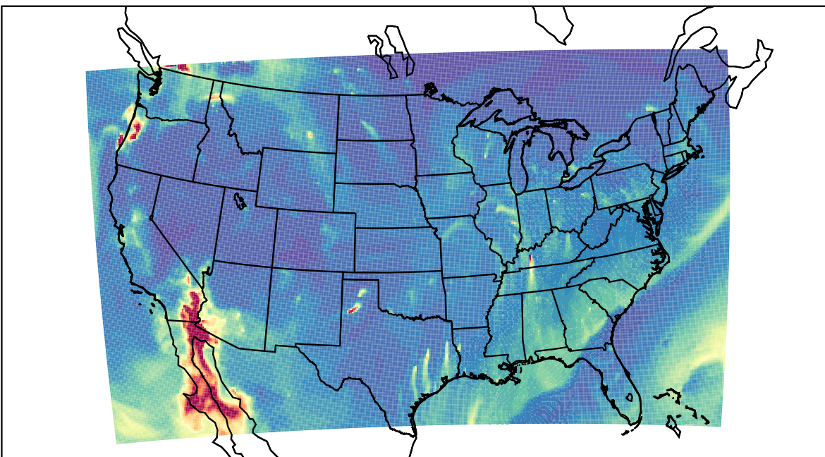
WRF 2023-10-31_07:00:00
