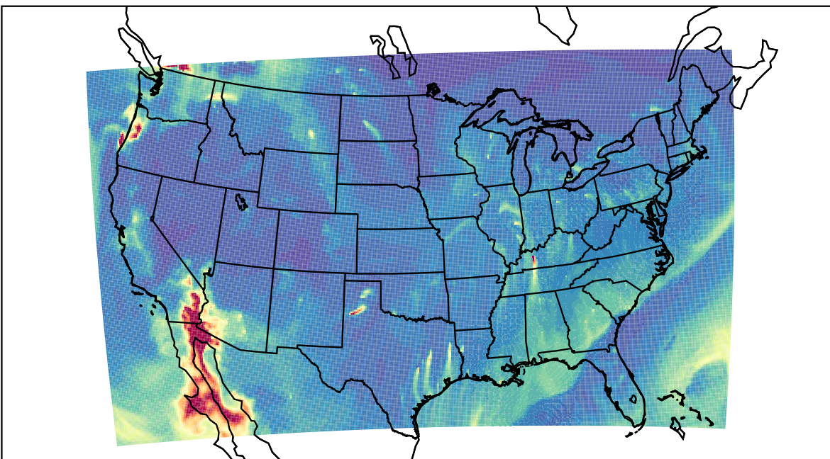
WRF 2023-10-31_08:00:00
