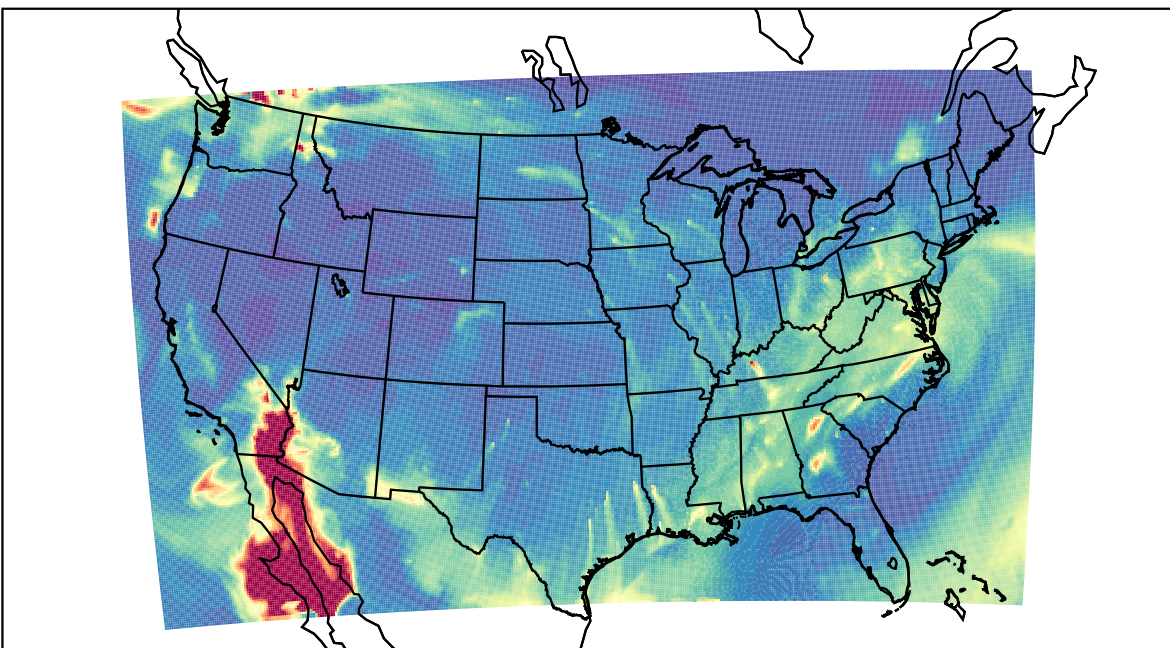
WRF 2023-10-30_08:00:00
