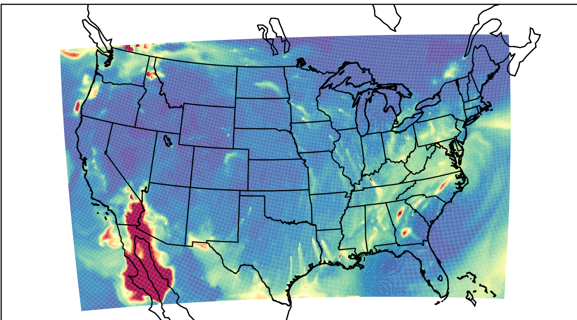
WRF 2023-10-30_06:00:00
