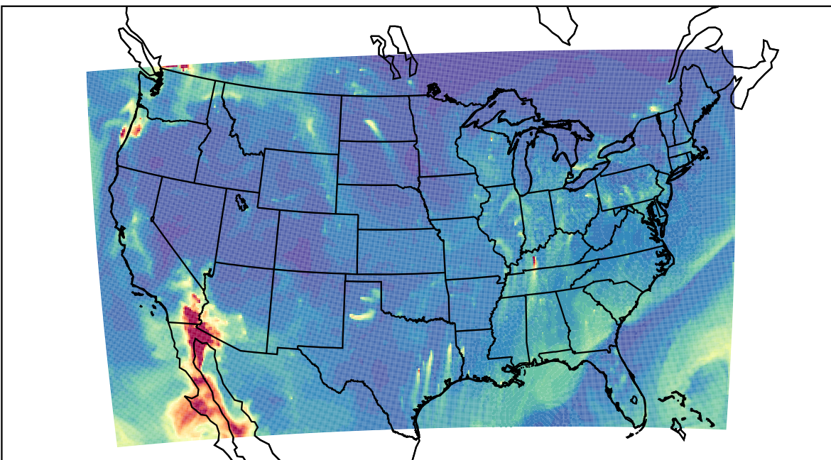
WRF 2023-10-31_11:00:00
