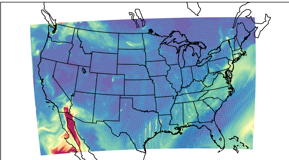
WRF 2023-10-30_19:00:00
