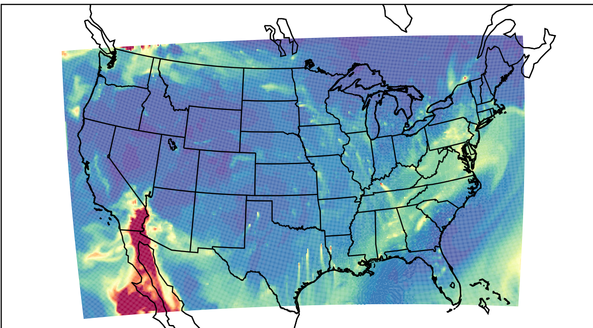
WRF 2023-10-30_13:00:00
