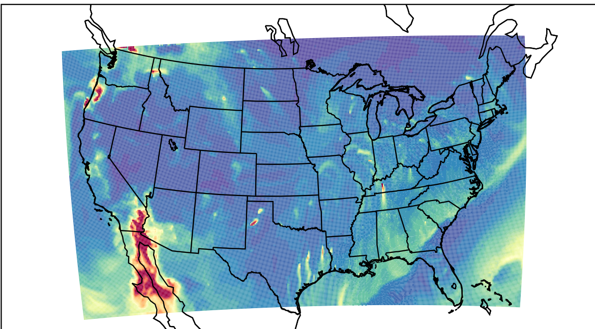
WRF 2023-10-31_06:00:00
