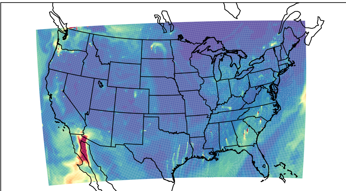
WRF 2023-10-31_21:00:00
