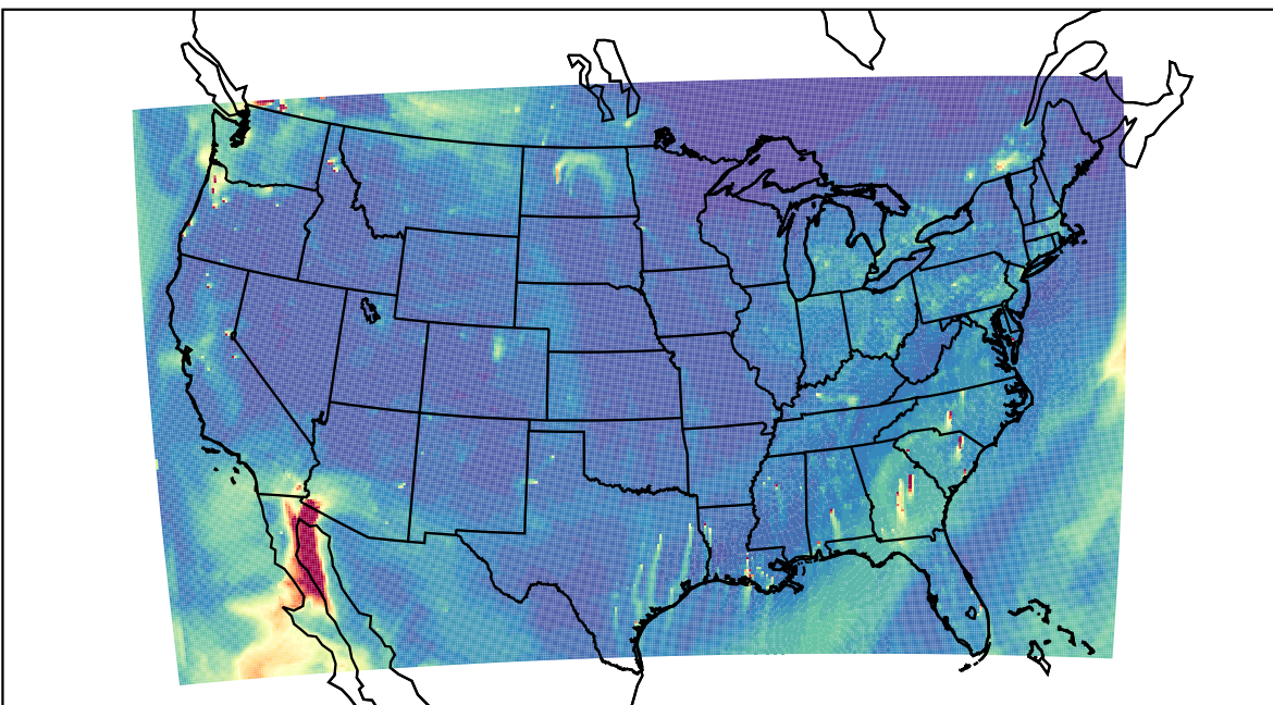
WRF 2023-10-31_22:00:00
