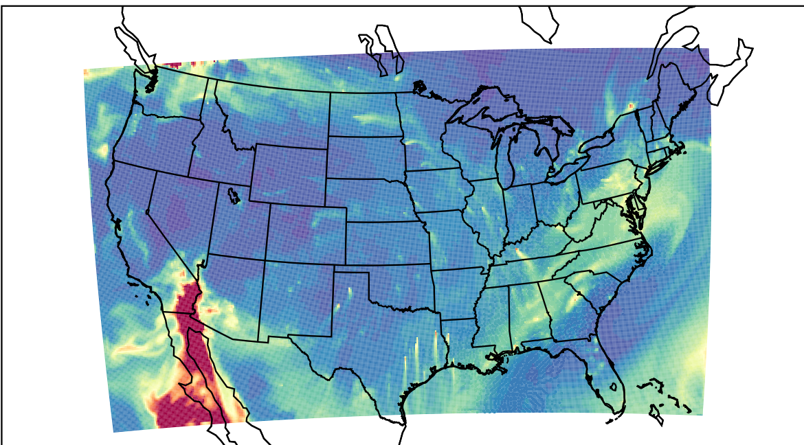
WRF 2023-10-30_14:00:00
