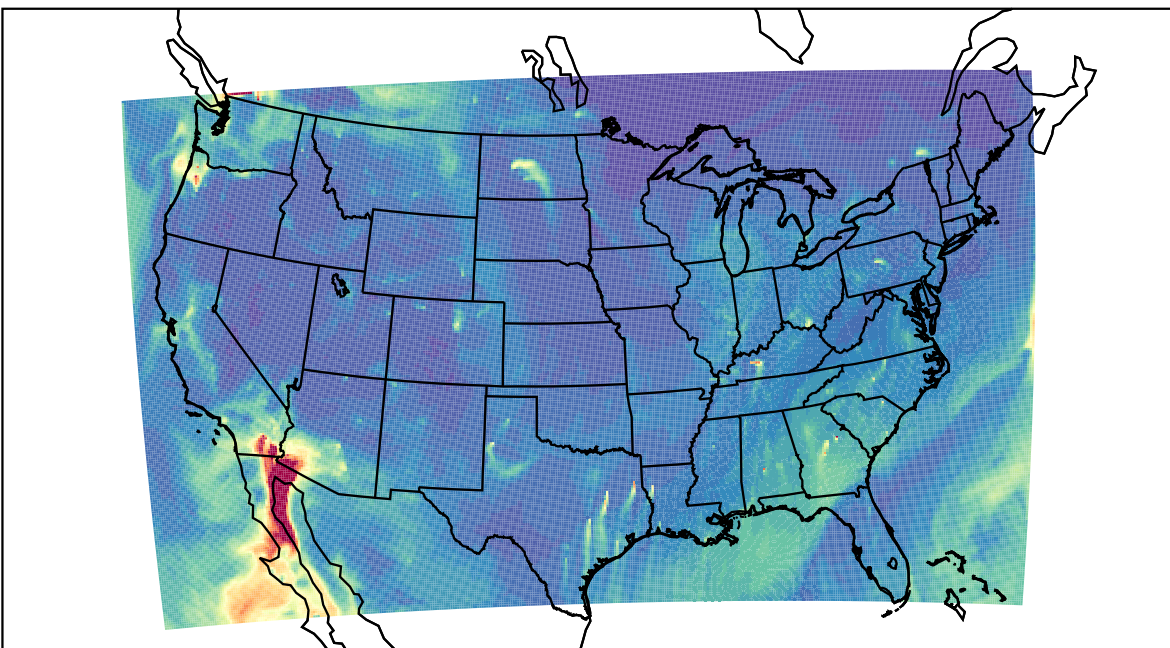
WRF 2023-10-31_17:00:00
