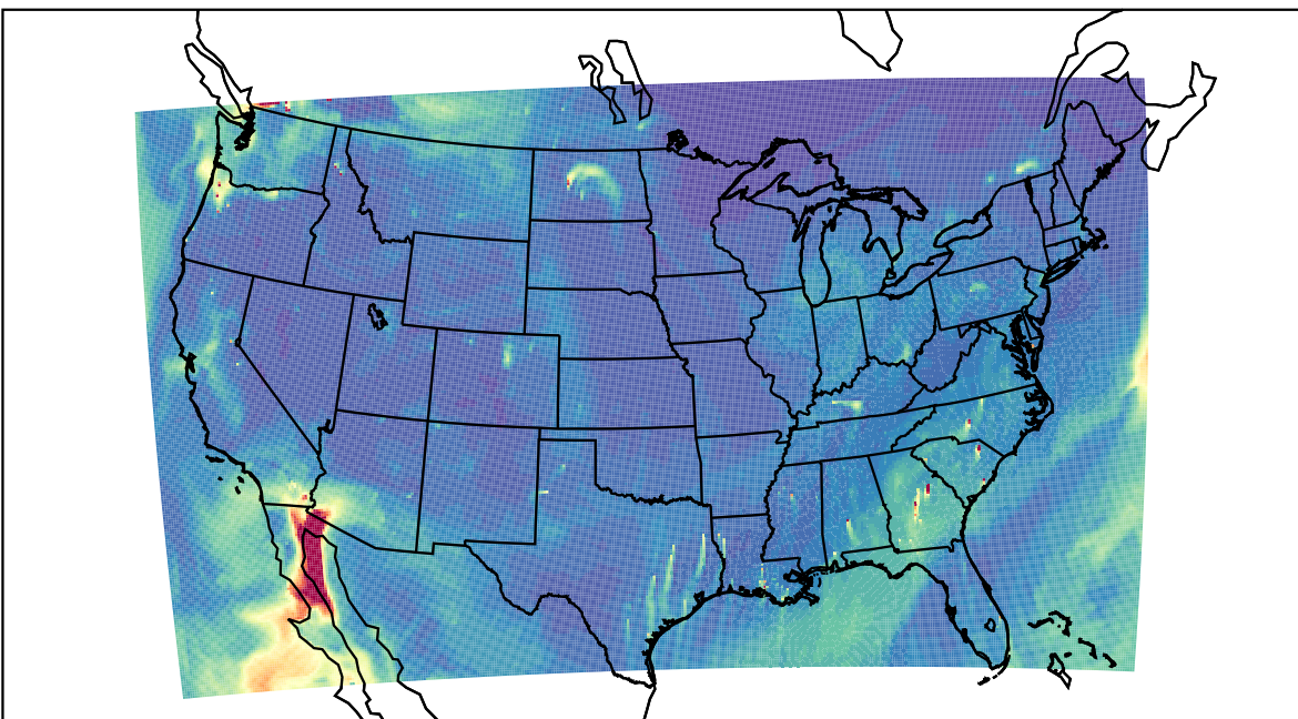
WRF 2023-10-31_20:00:00
