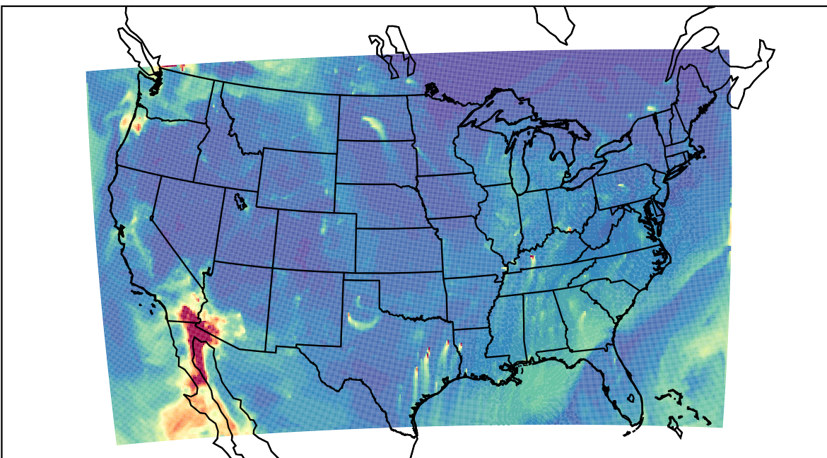
WRF 2023-10-31_15:00:00
