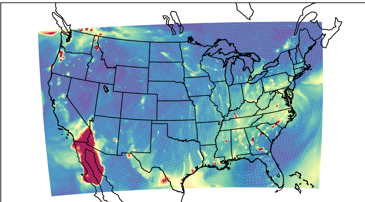
WRF 2023-10-30_02:00:00
