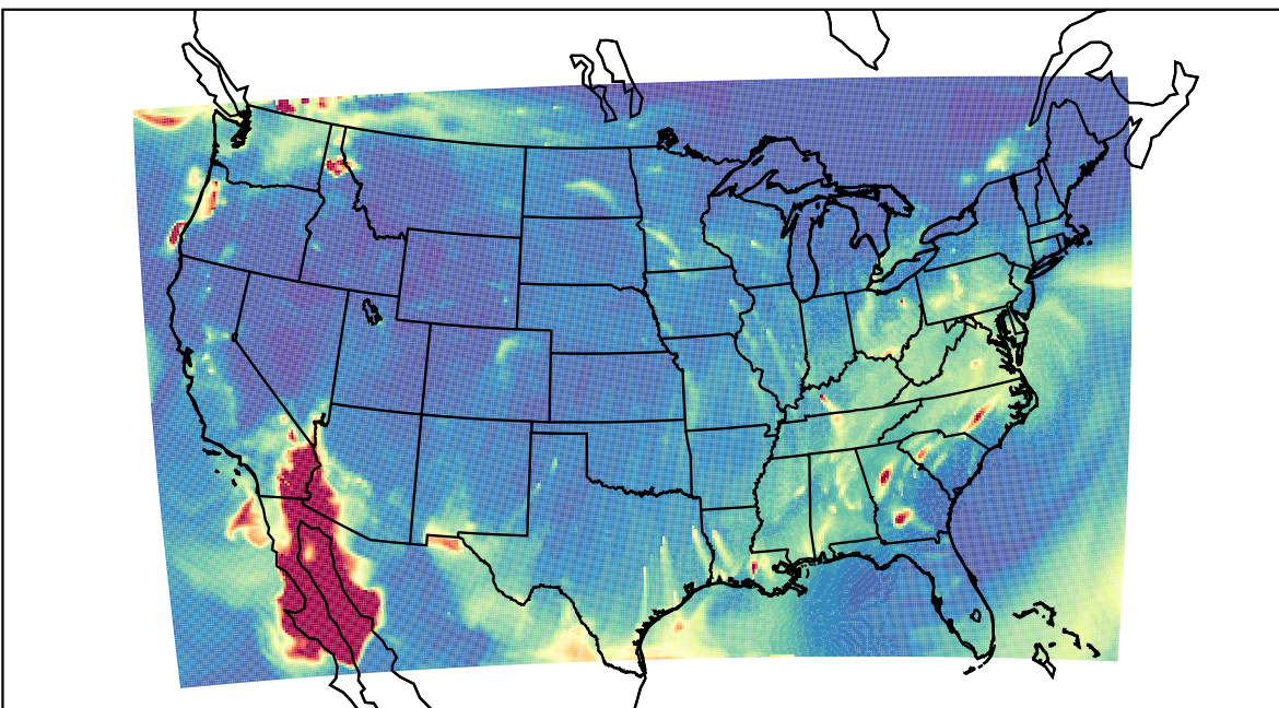
WRF 2023-10-30_05:00:00
