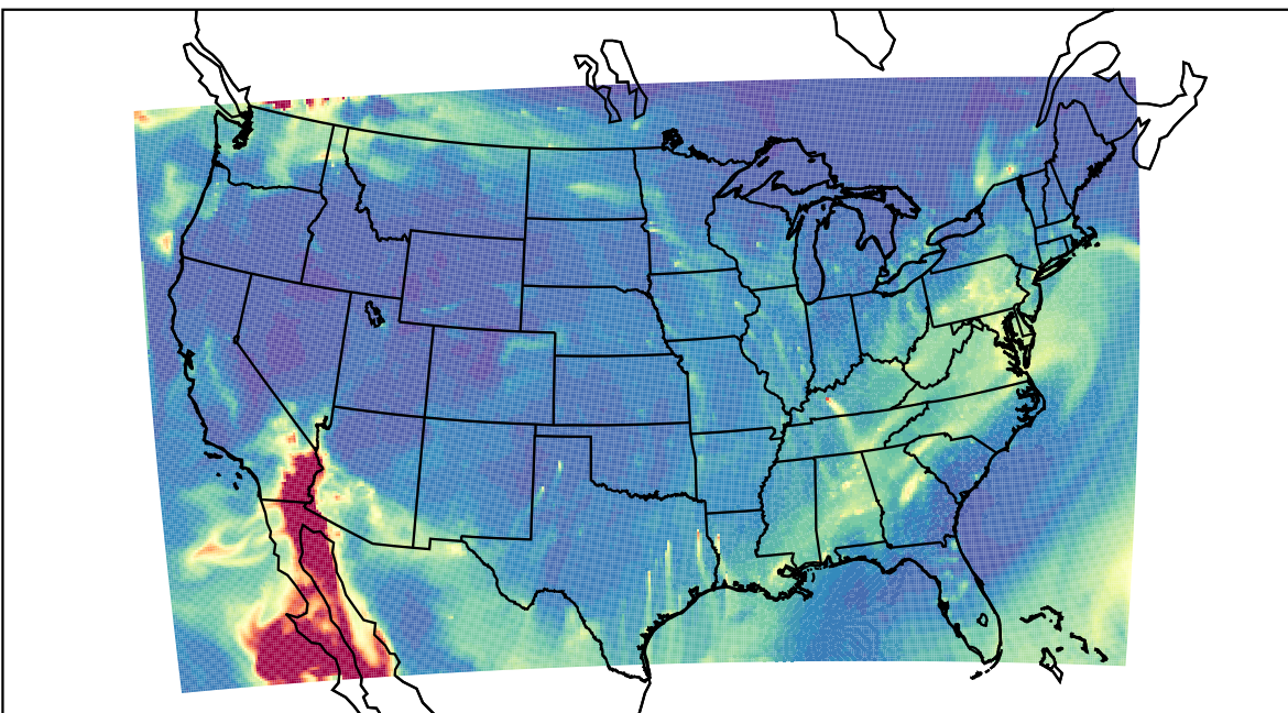
WRF 2023-10-30_12:00:00
