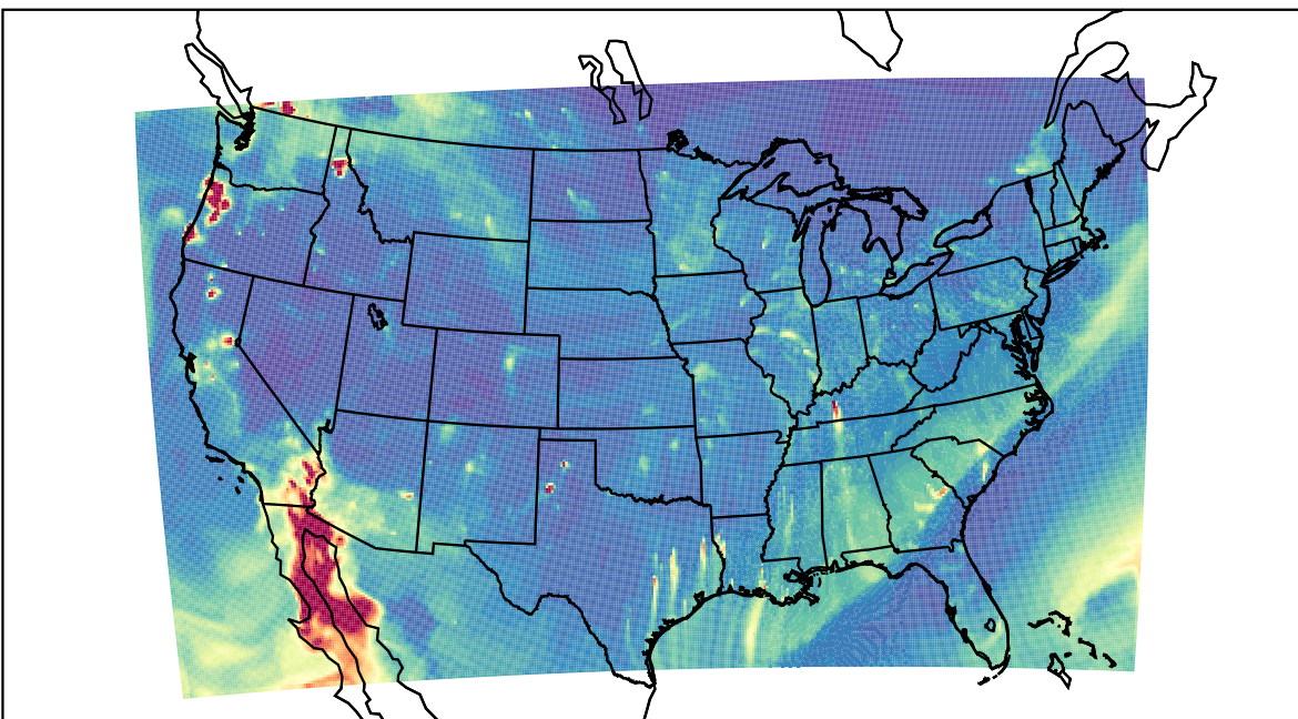
WRF 2023-10-31_03:00:00
