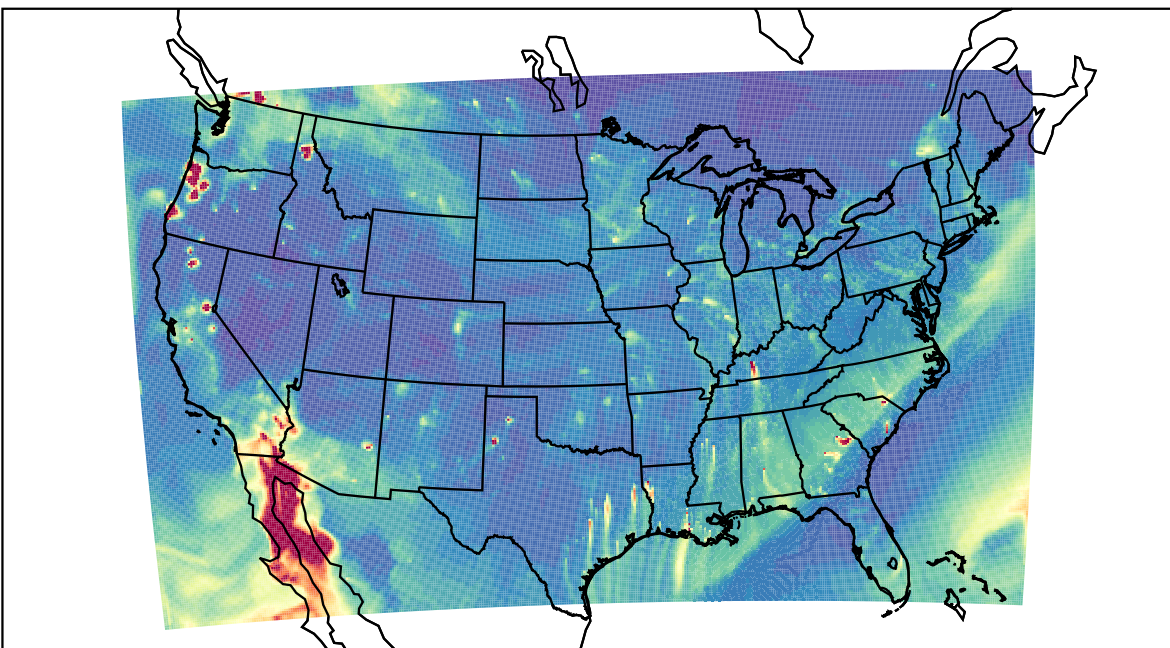
WRF 2023-10-31_02:00:00
