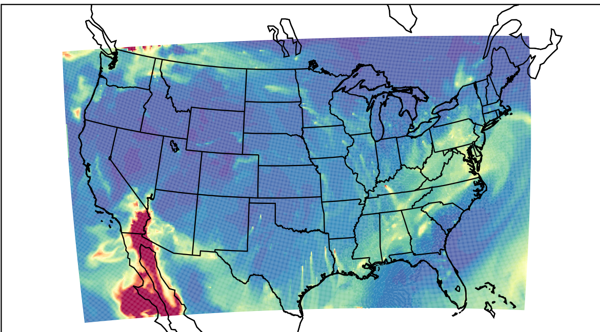
WRF 2023-10-30_11:00:00
