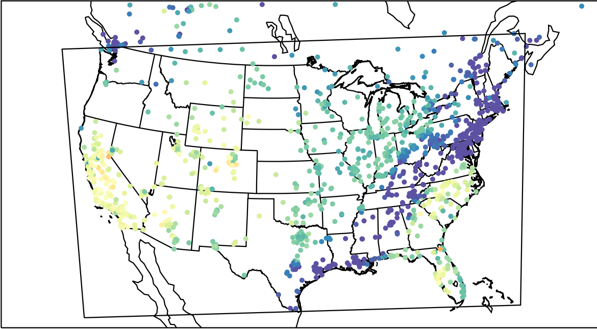
AirNOW (2023-10-30_21:00:00)
