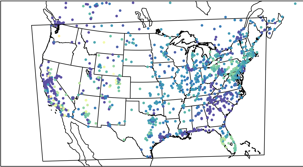
AirNOW (2023-10-31_15:00:00)
