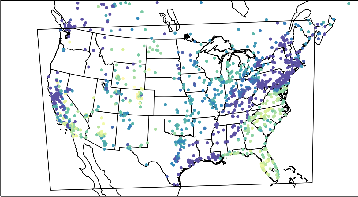
AirNOW (2023-10-30_16:00:00)
