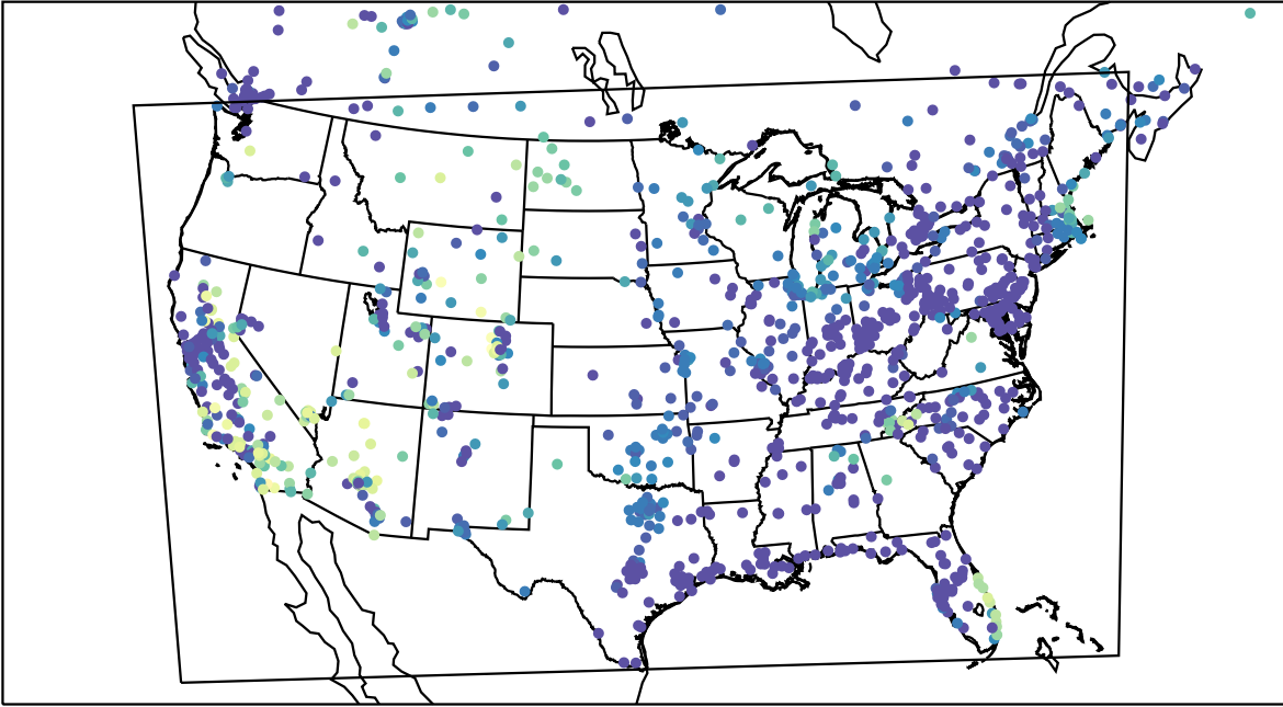
AirNOW (2023-10-30_09:00:00)
