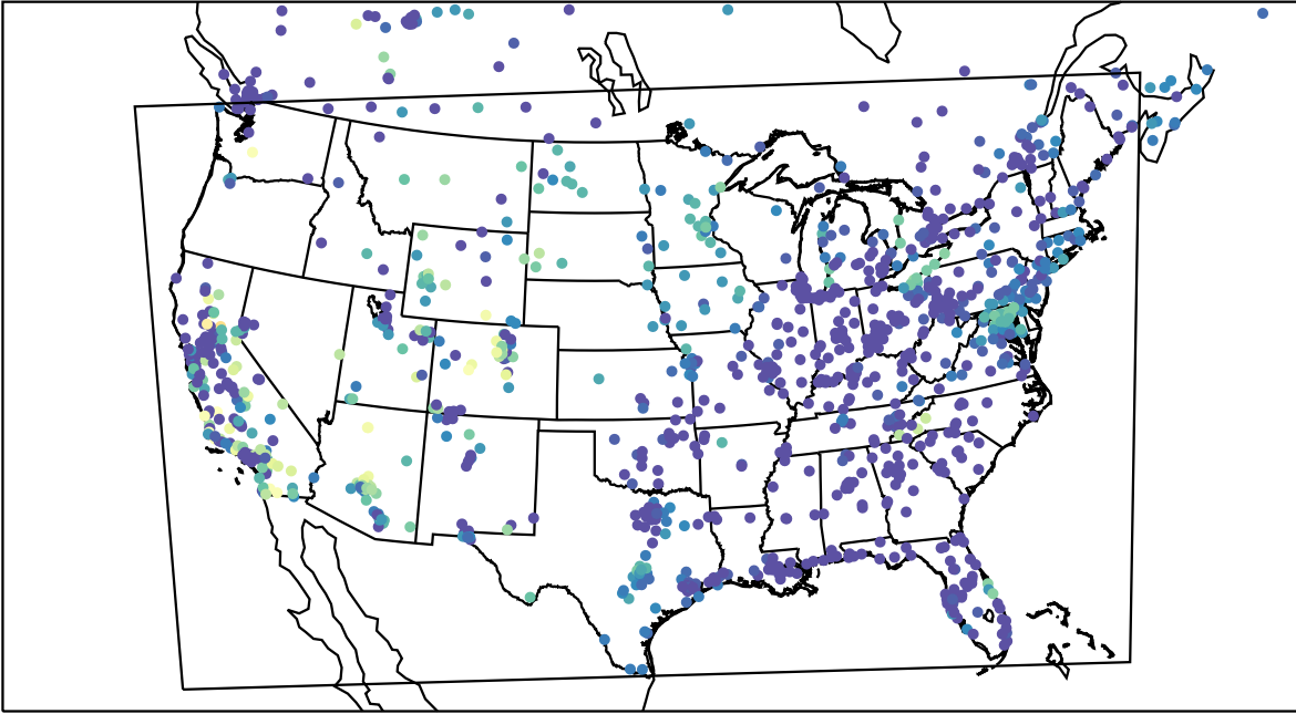
AirNOW (2023-10-31_08:00:00)
