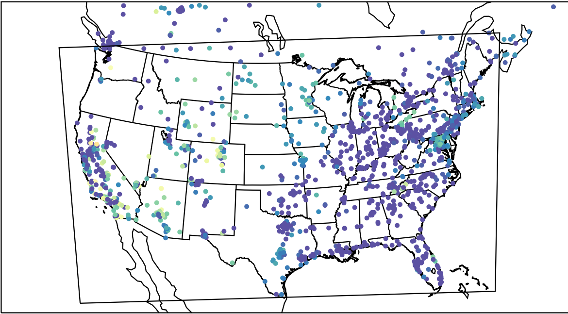
AirNOW (2023-10-31_09:00:00)
