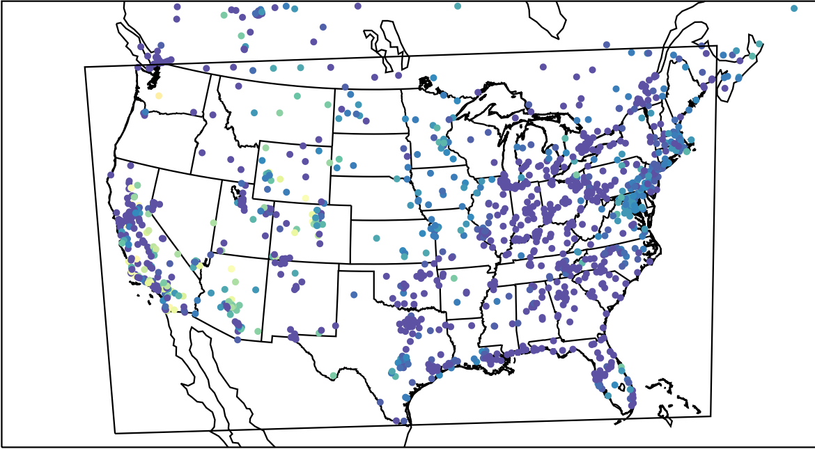
AirNOW (2023-10-31_13:00:00)
