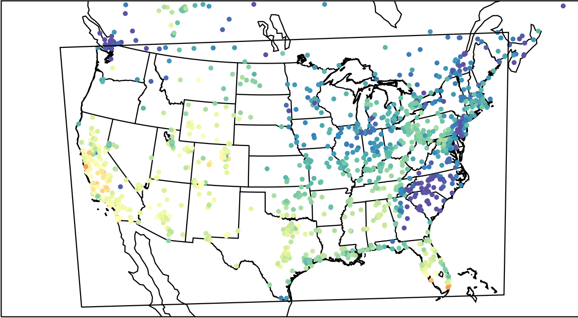
AirNOW (2023-10-31_21:00:00)
