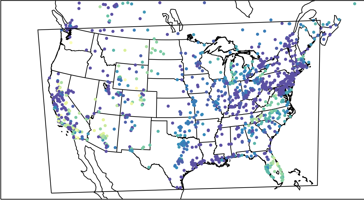
AirNOW (2023-10-30_14:00:00)
