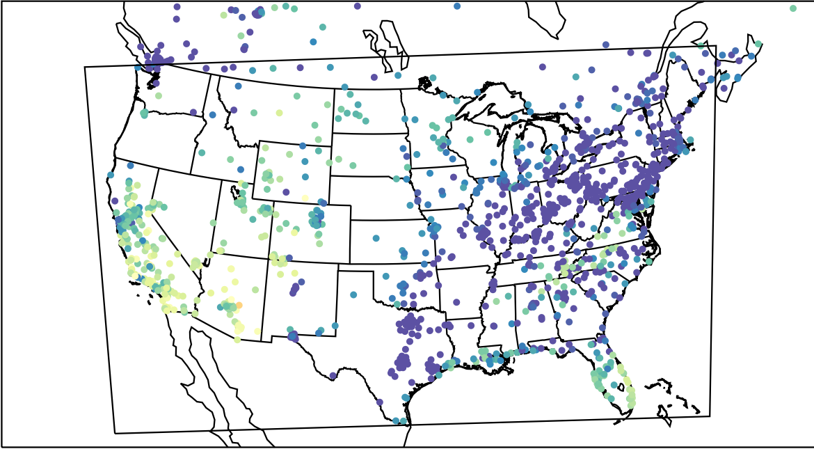
AirNOW (2023-10-30_01:00:00)
