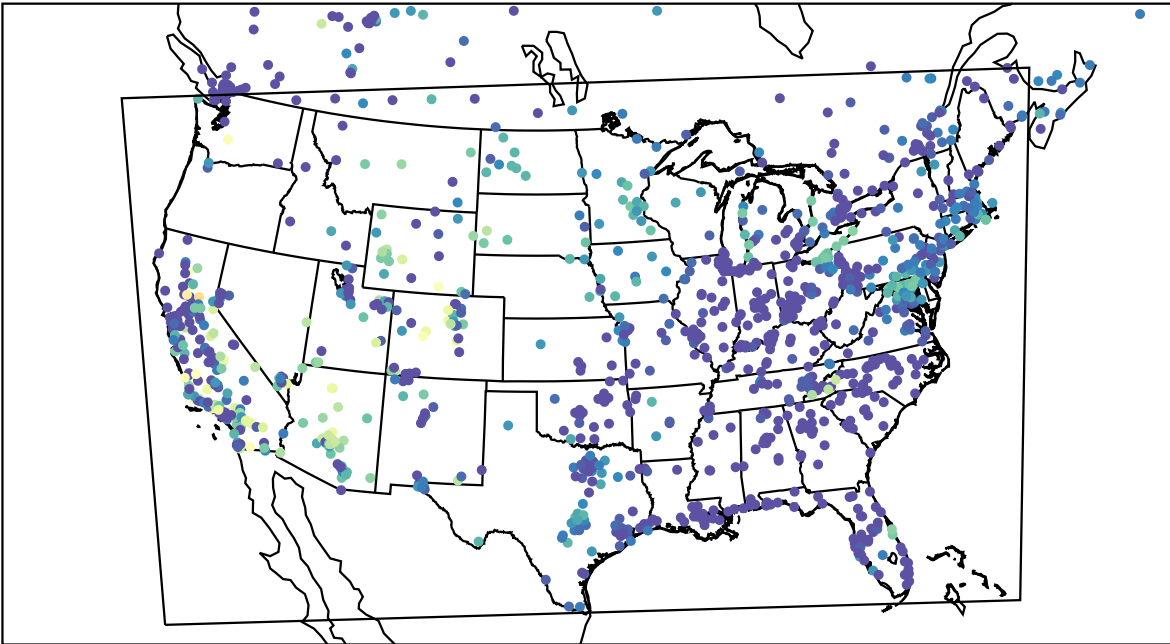
AirNOW (2023-10-31_07:00:00)
