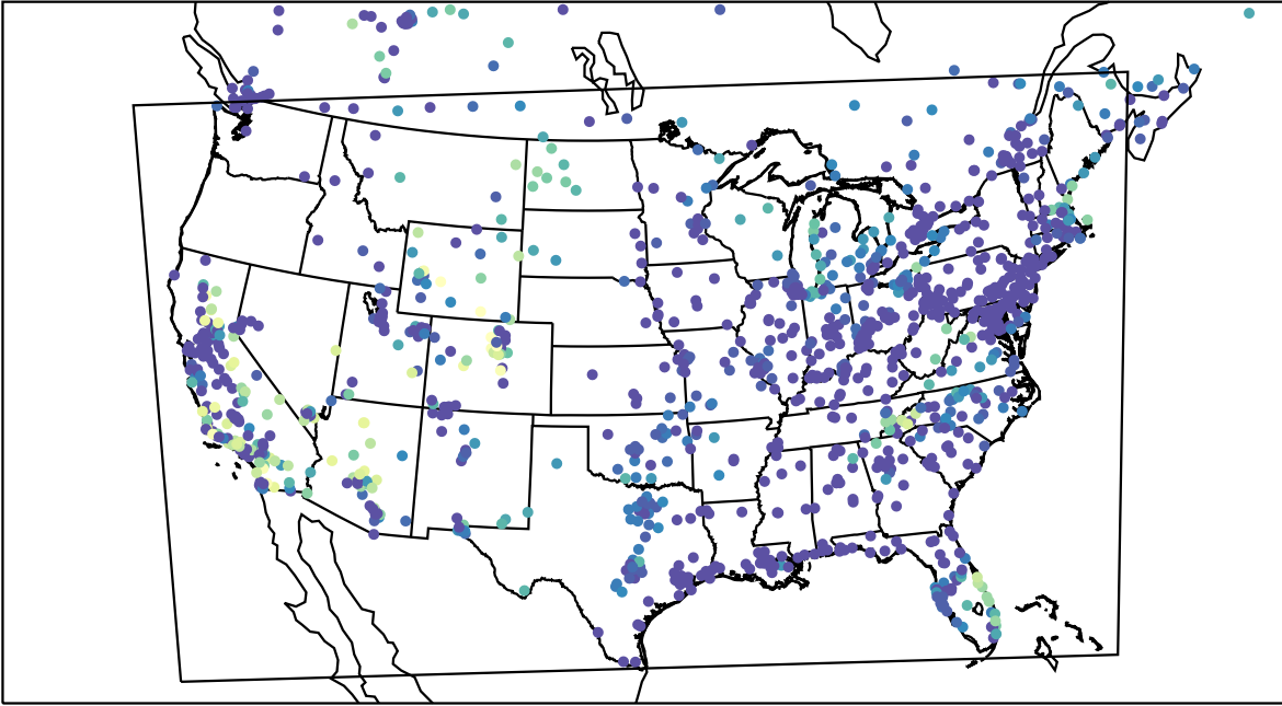
AirNOW (2023-10-30_13:00:00)
