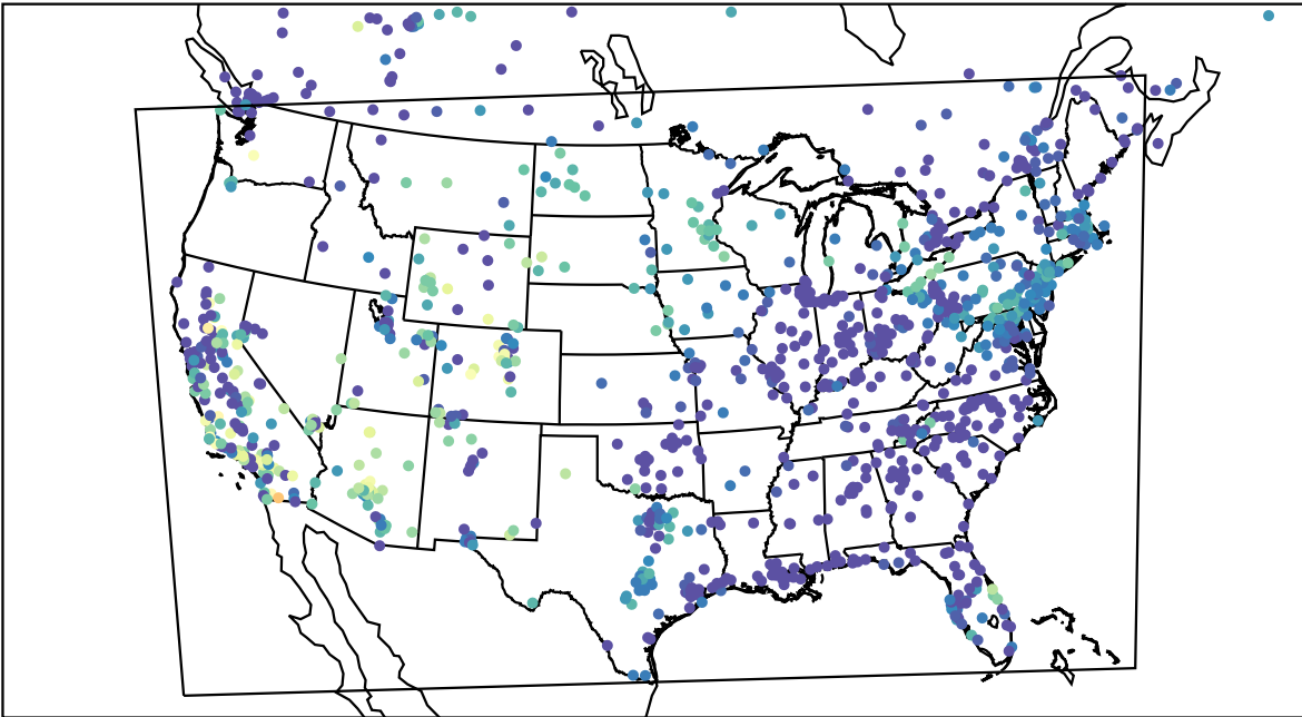
AirNOW (2023-10-31_05:00:00)
