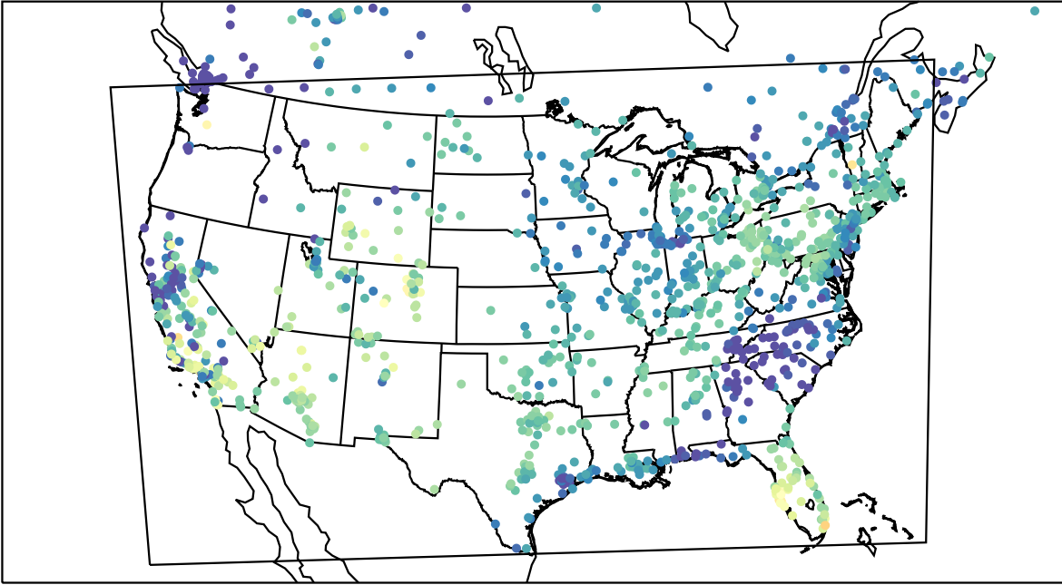
AirNOW (2023-10-31_17:00:00)
