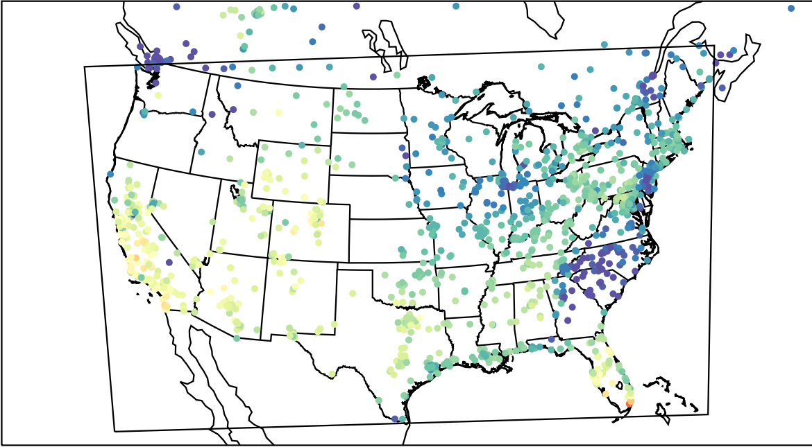
AirNOW (2023-10-31_20:00:00)
