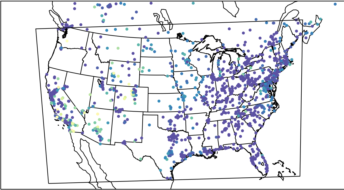
AirNOW (2023-10-31_12:00:00)
