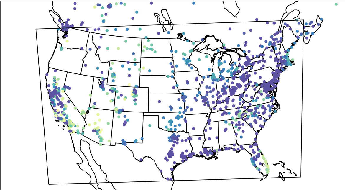
AirNOW (2023-10-30_06:00:00)
