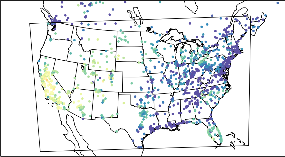
AirNOW (2023-10-31_00:00:00)
