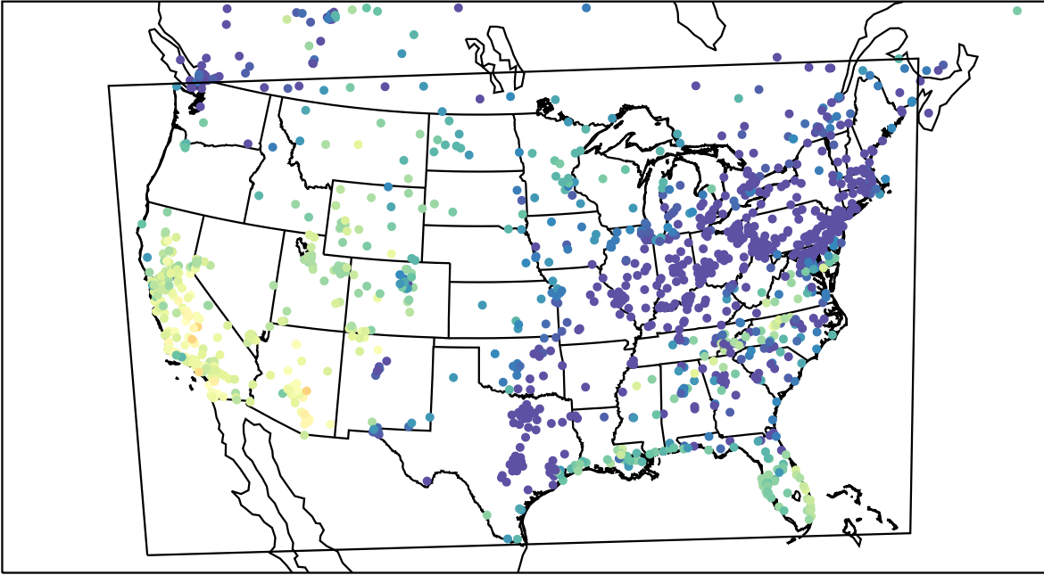
AirNOW (2023-10-30_00:00:00)
