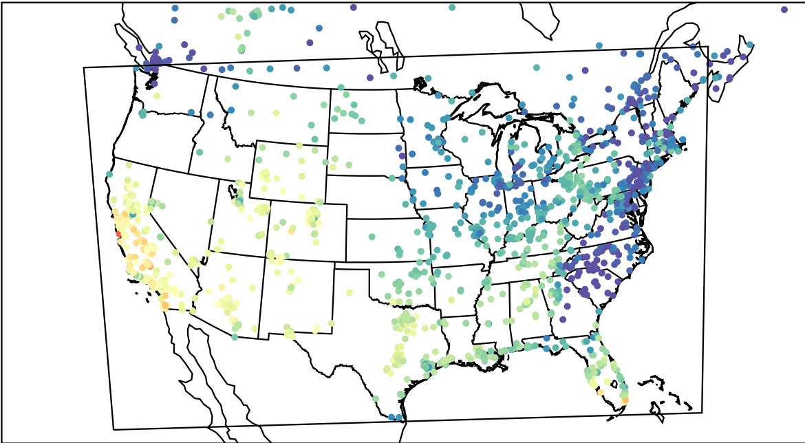
AirNOW (2023-10-31_22:00:00)
