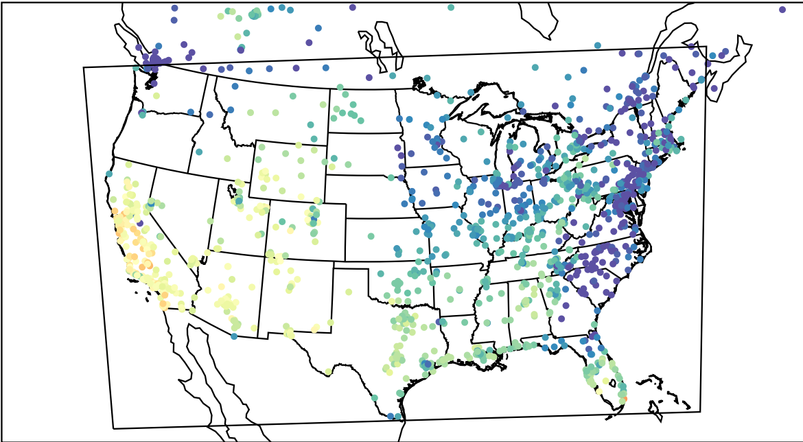
AirNOW (2023-10-31_23:00:00)
