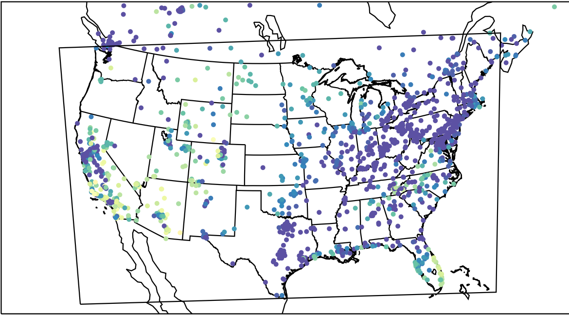
AirNOW (2023-10-30_03:00:00)
