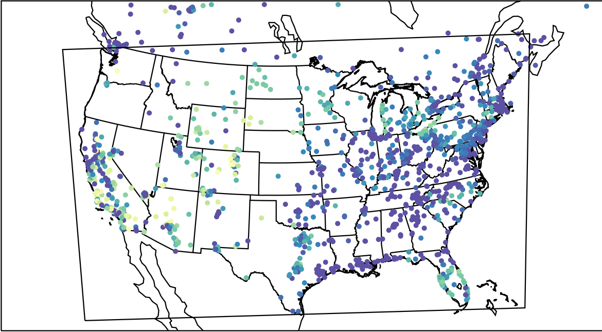
AirNOW (2023-10-31_02:00:00)
