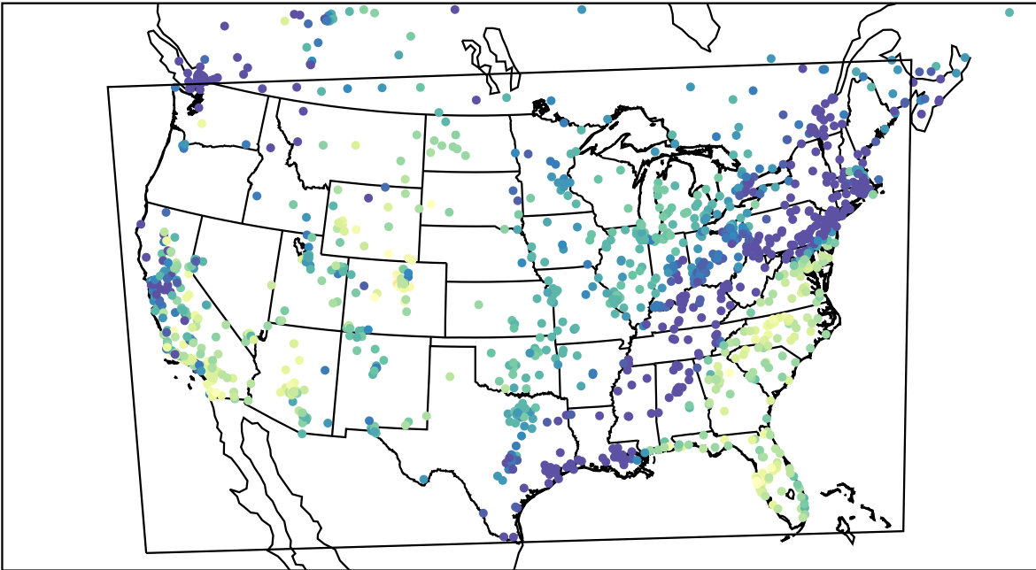
AirNOW (2023-10-30_17:00:00)
