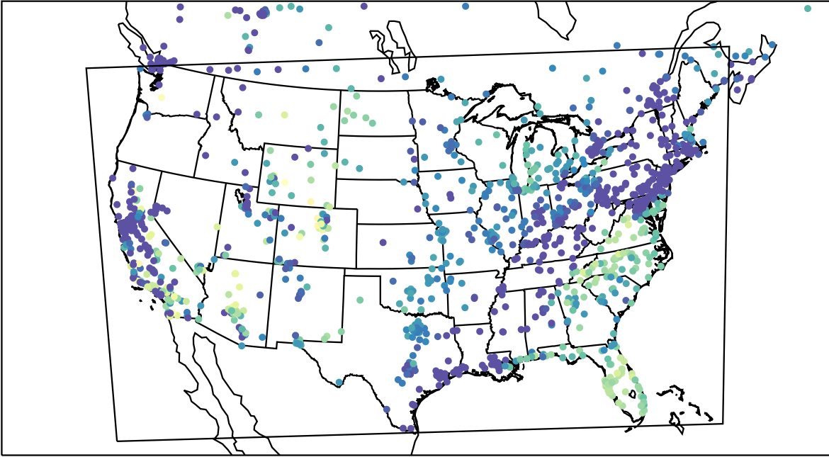
AirNOW (2023-10-30_15:00:00)
