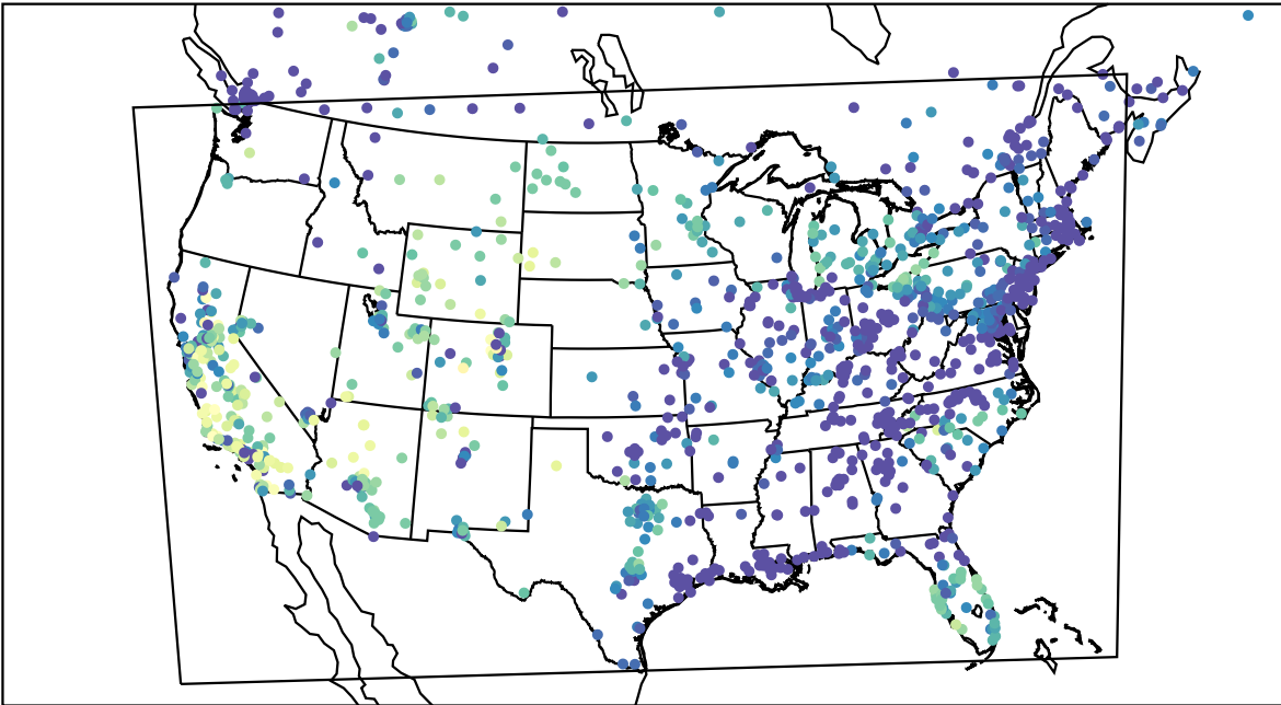
AirNOW (2023-10-31_01:00:00)
