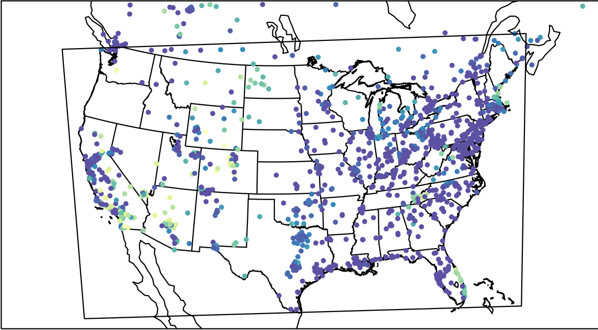
AirNOW (2023-10-30_12:00:00)
