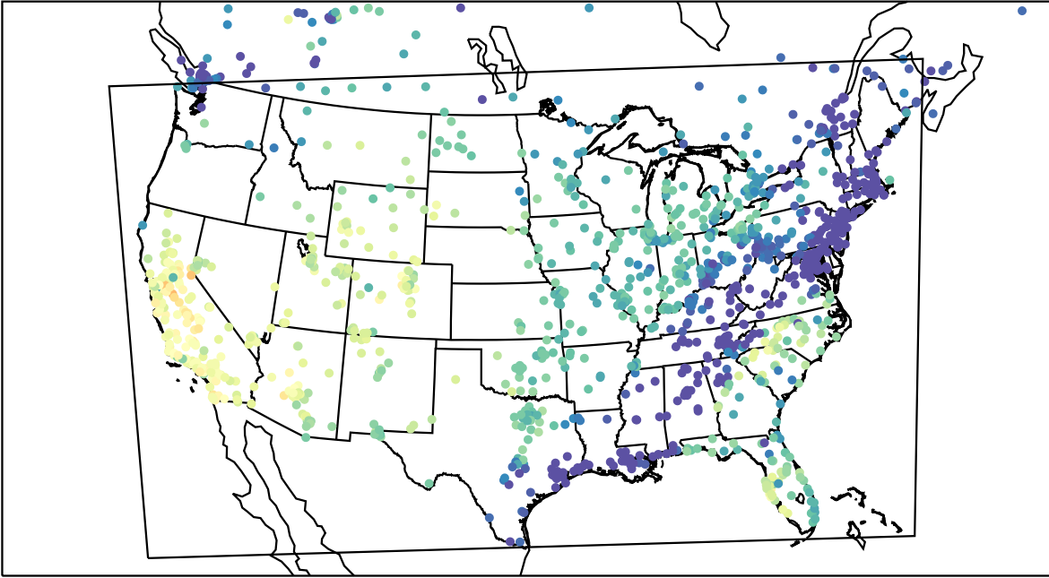
AirNOW (2023-10-30_22:00:00)
