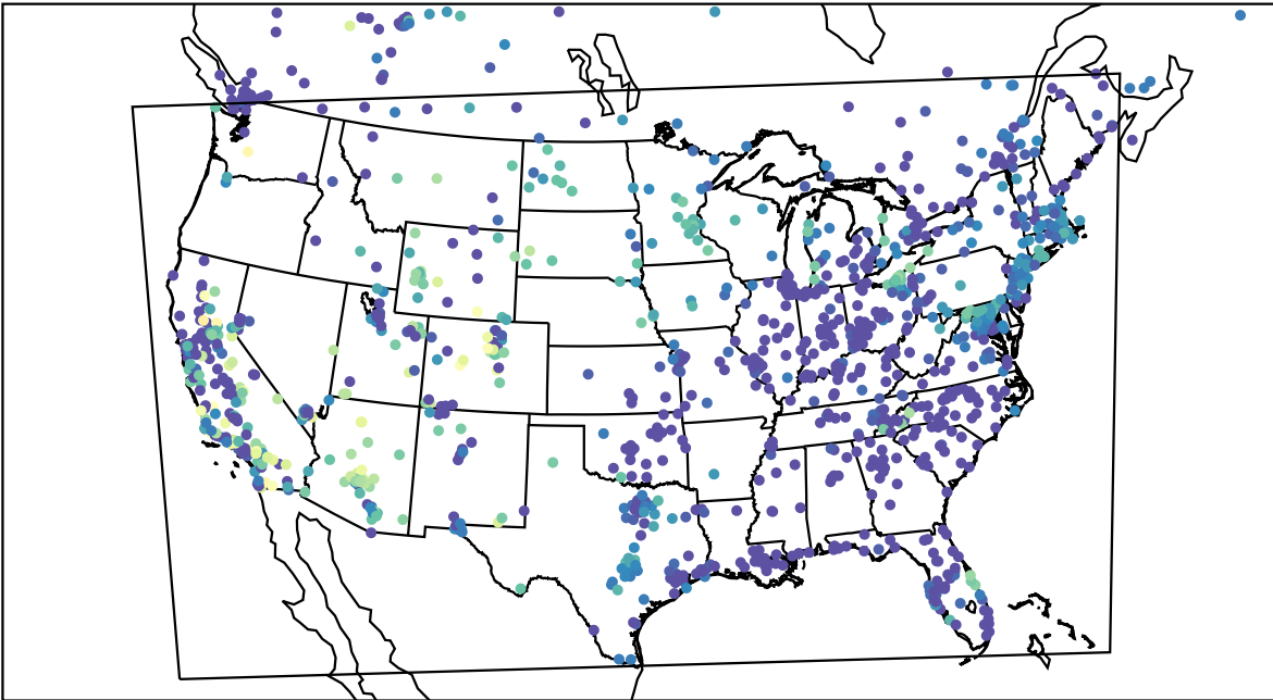
AirNOW (2023-10-31_06:00:00)
