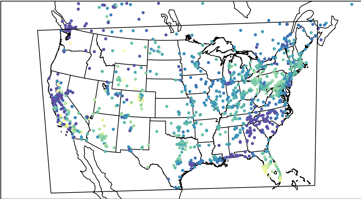
AirNOW (2023-10-31_16:00:00)
