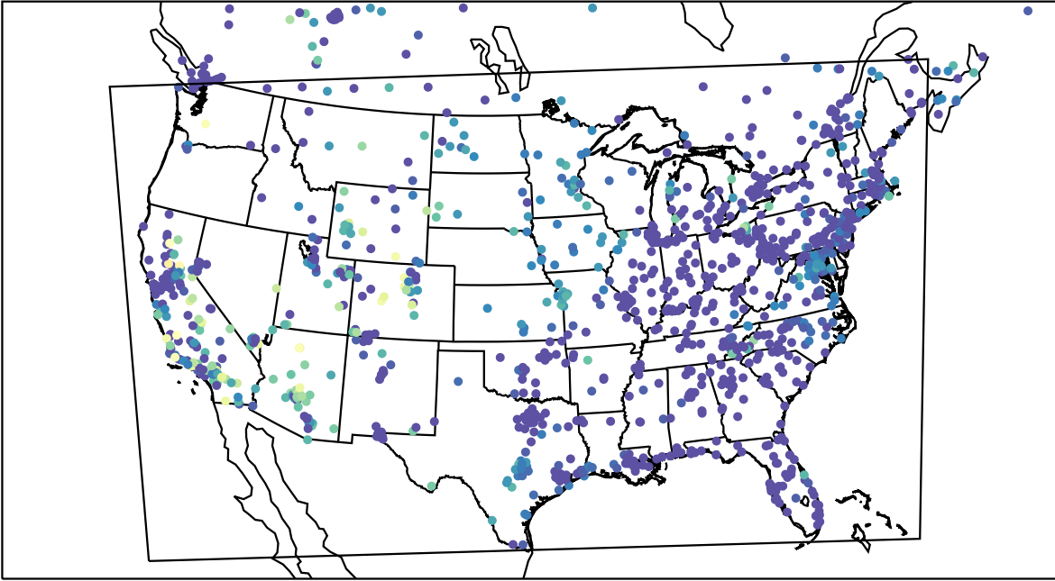
AirNOW (2023-10-31_11:00:00)
