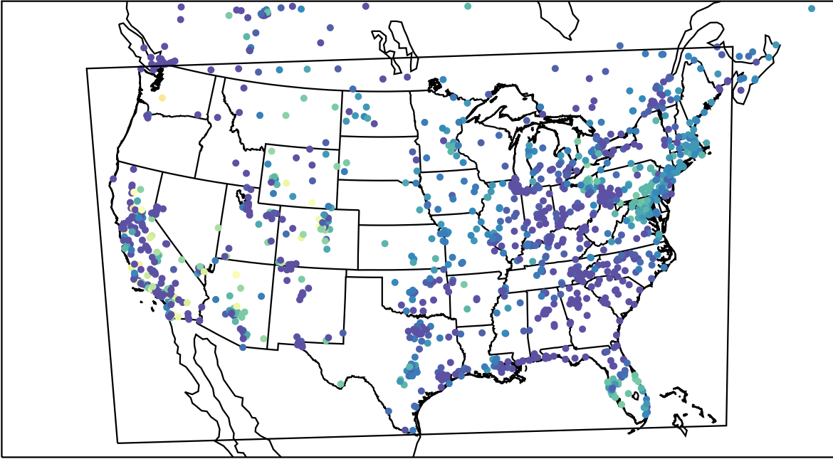
AirNOW (2023-10-31_14:00:00)
