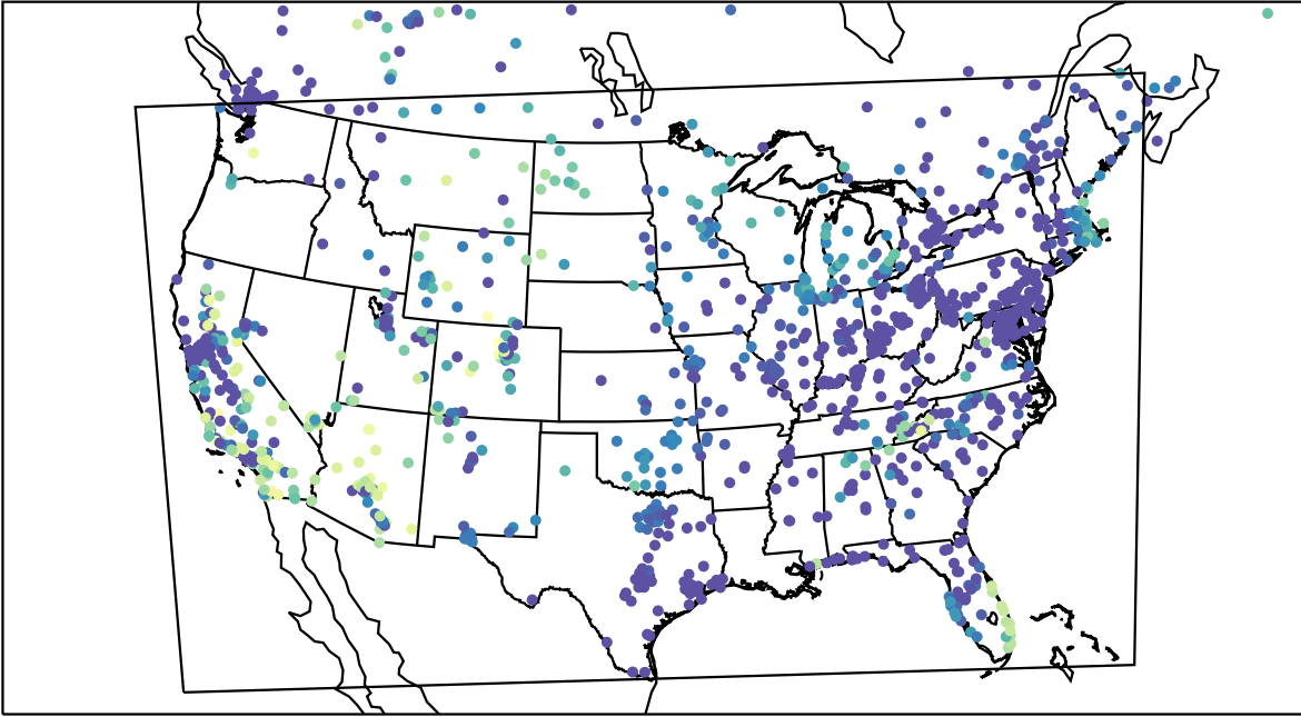
AirNOW (2023-10-30_07:00:00)
