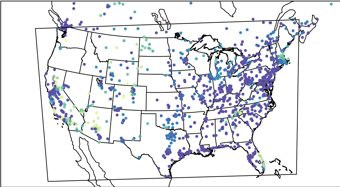
AirNOW (2023-10-30_10:00:00)
