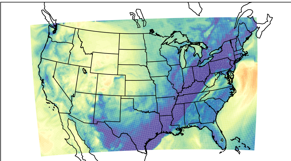
WRF (2023-10-30_09:00:00)
