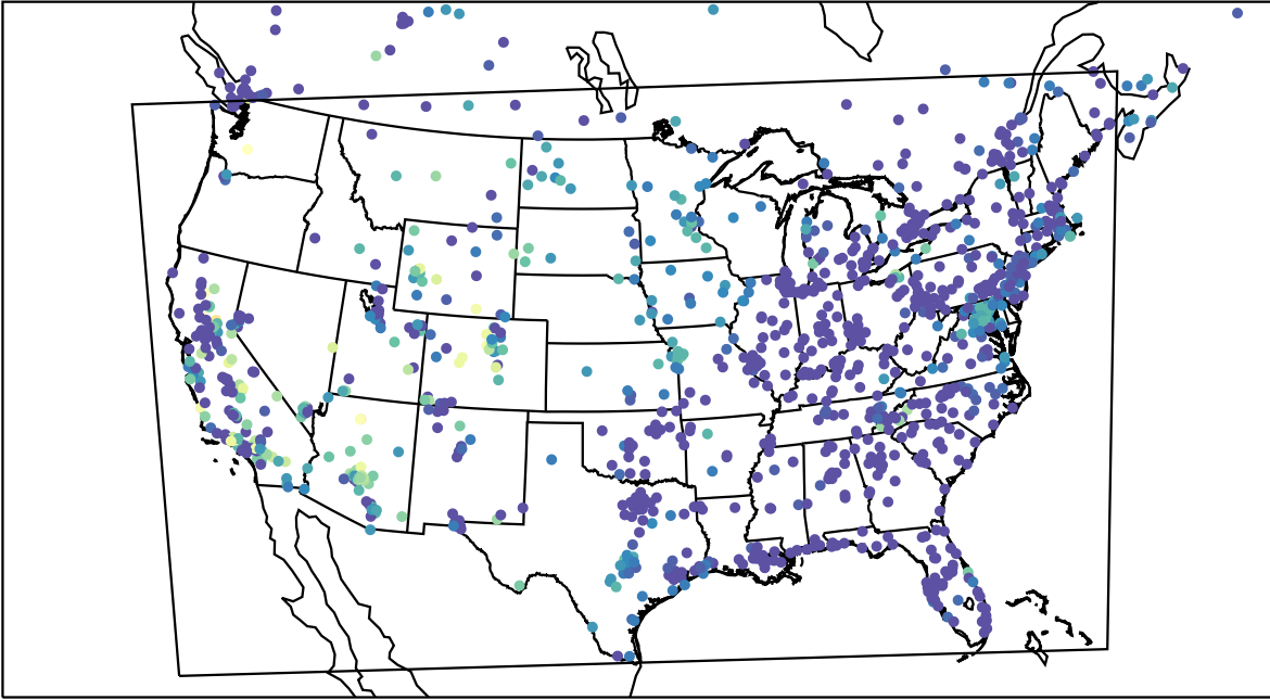
AirNOW (2023-10-31_10:00:00)
