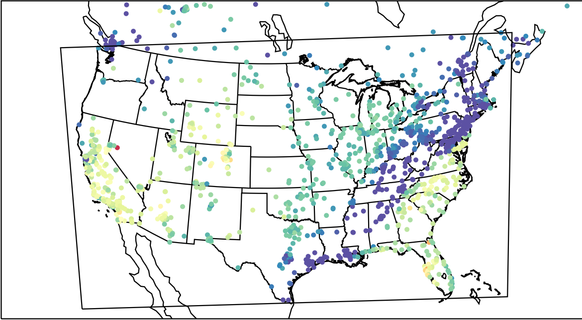
AirNOW (2023-10-30_19:00:00)
