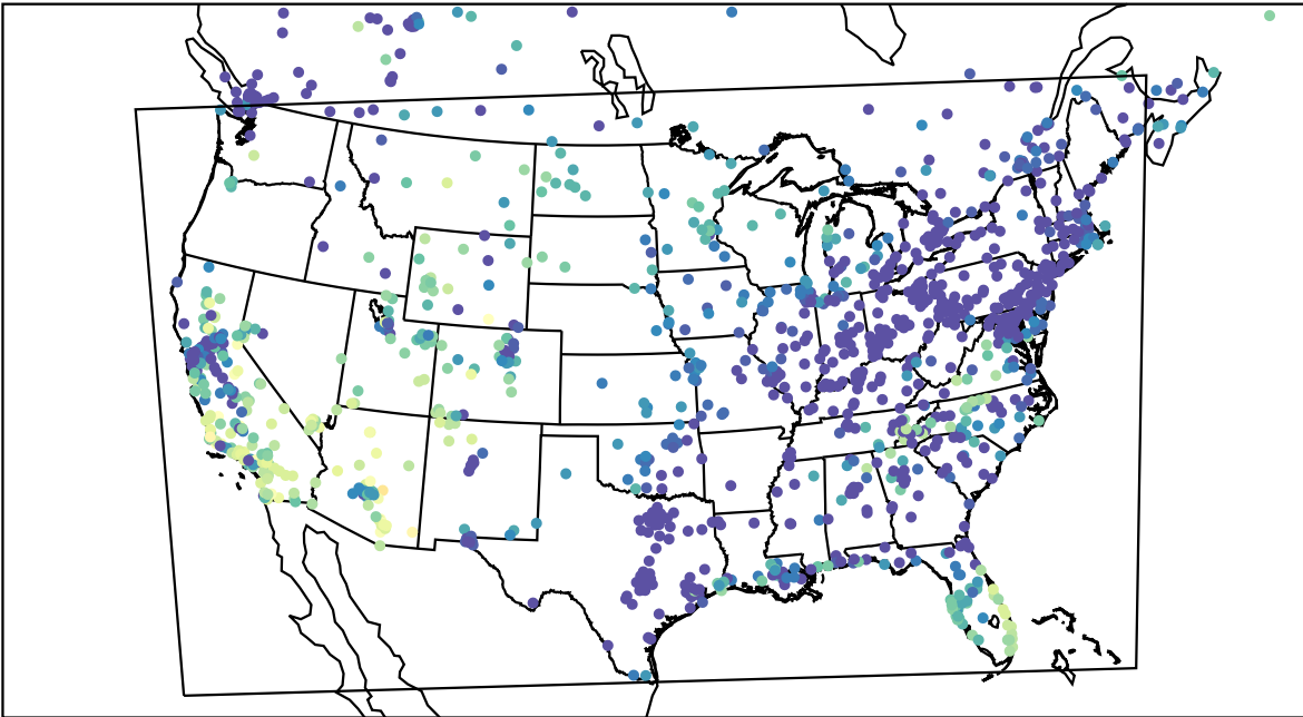
AirNOW (2023-10-30_02:00:00)
