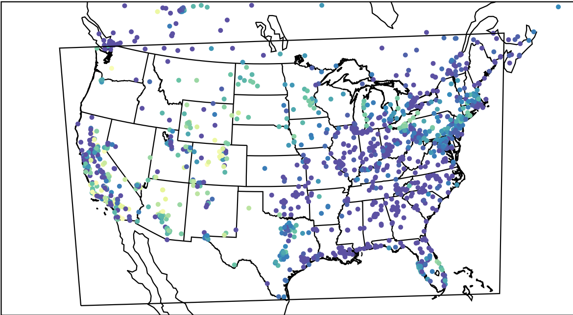
AirNOW (2023-10-31_04:00:00)
