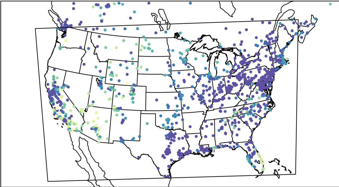
AirNOW (2023-10-30_05:00:00)
