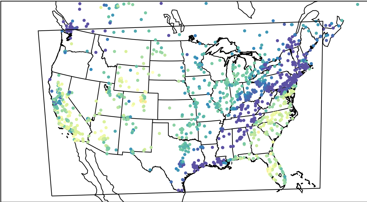
AirNOW (2023-10-30_18:00:00)
