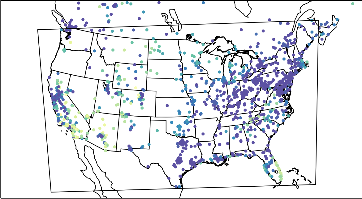
AirNOW (2023-10-30_04:00:00)
