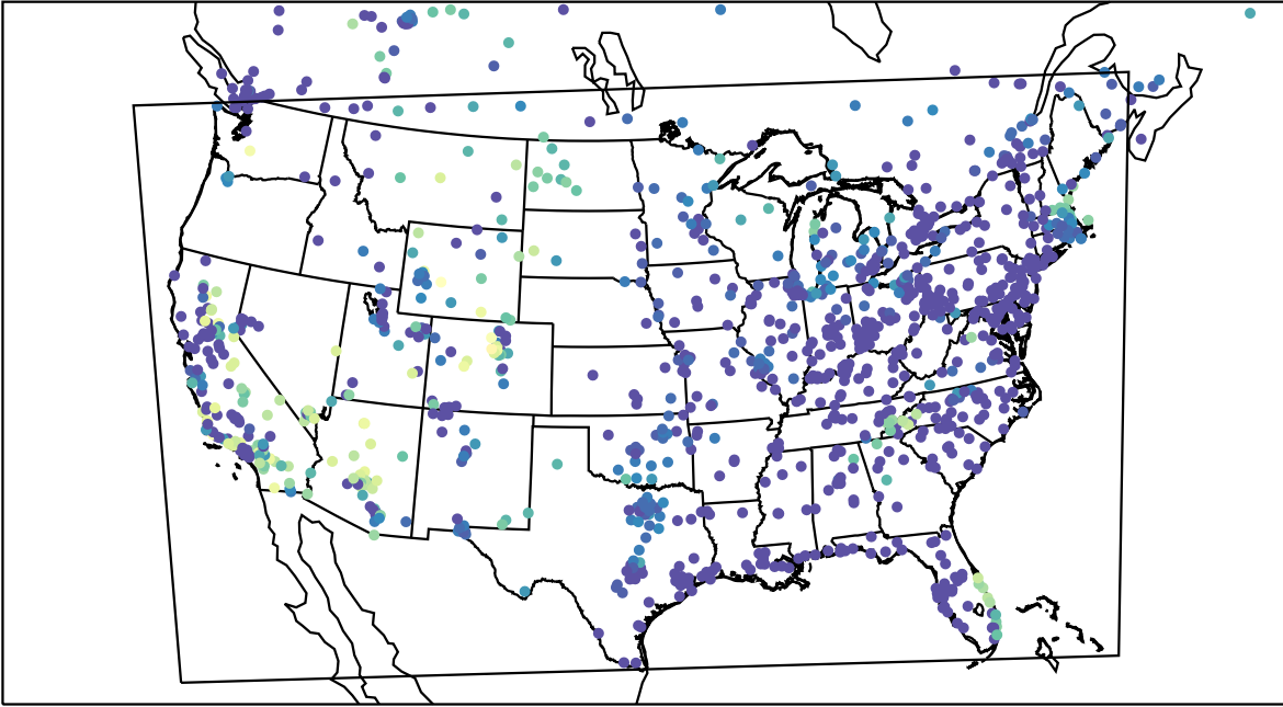
AirNOW (2023-10-30_11:00:00)
