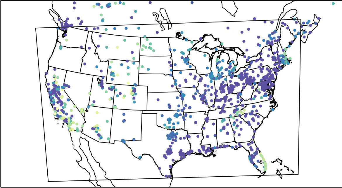
AirNOW (2023-10-30_08:00:00)
