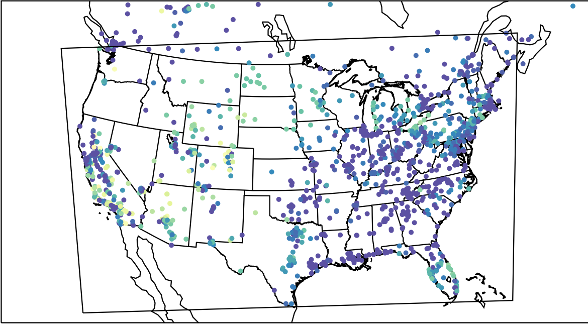
AirNOW (2023-10-31_03:00:00)
