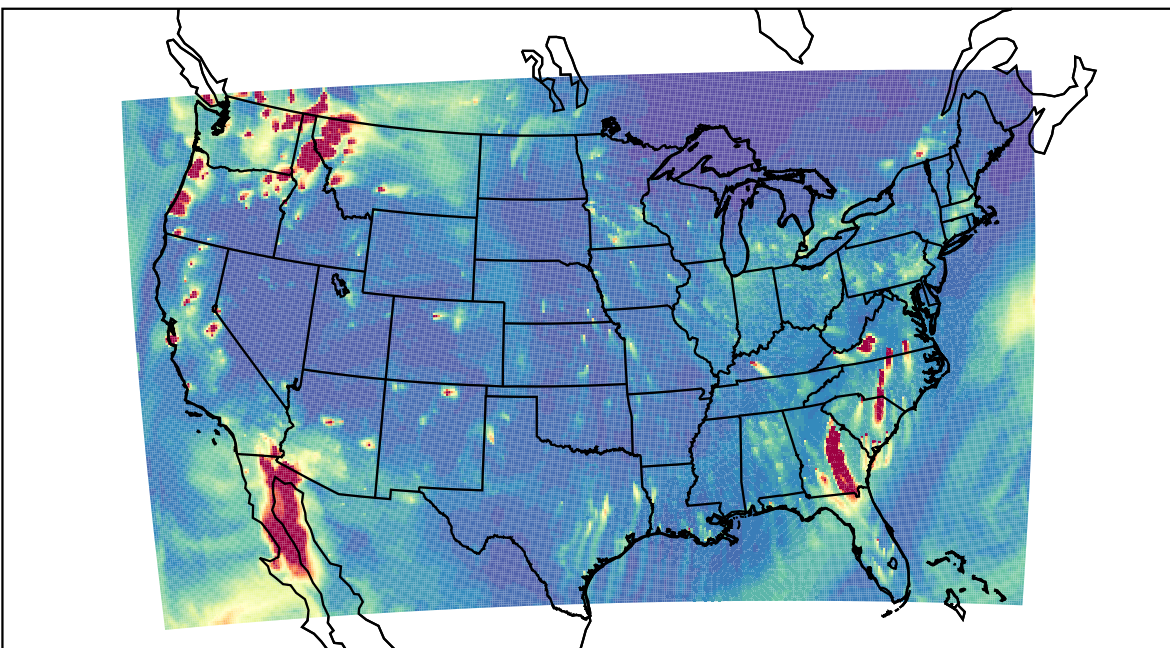
WRF 2023-11-01_02:00:00
