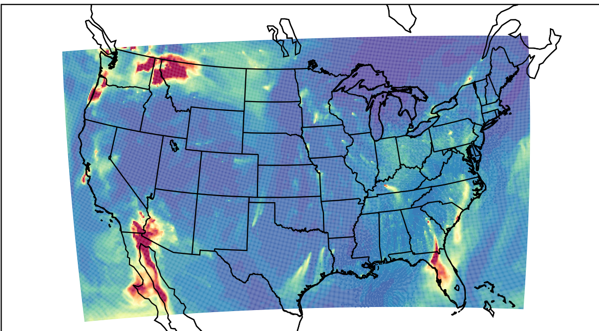
WRF 2023-11-01_09:00:00
