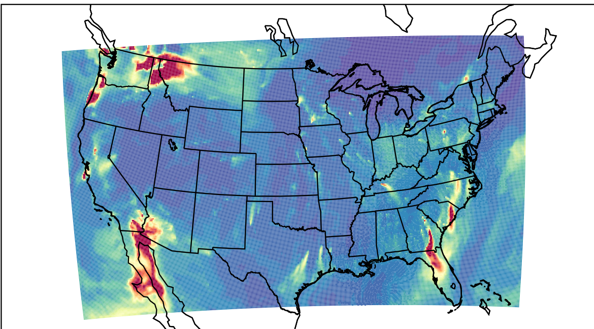
WRF 2023-11-01_07:00:00
