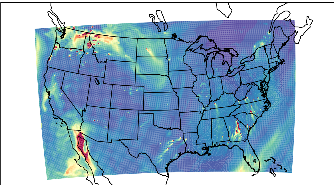
WRF 2023-11-01_21:00:00
