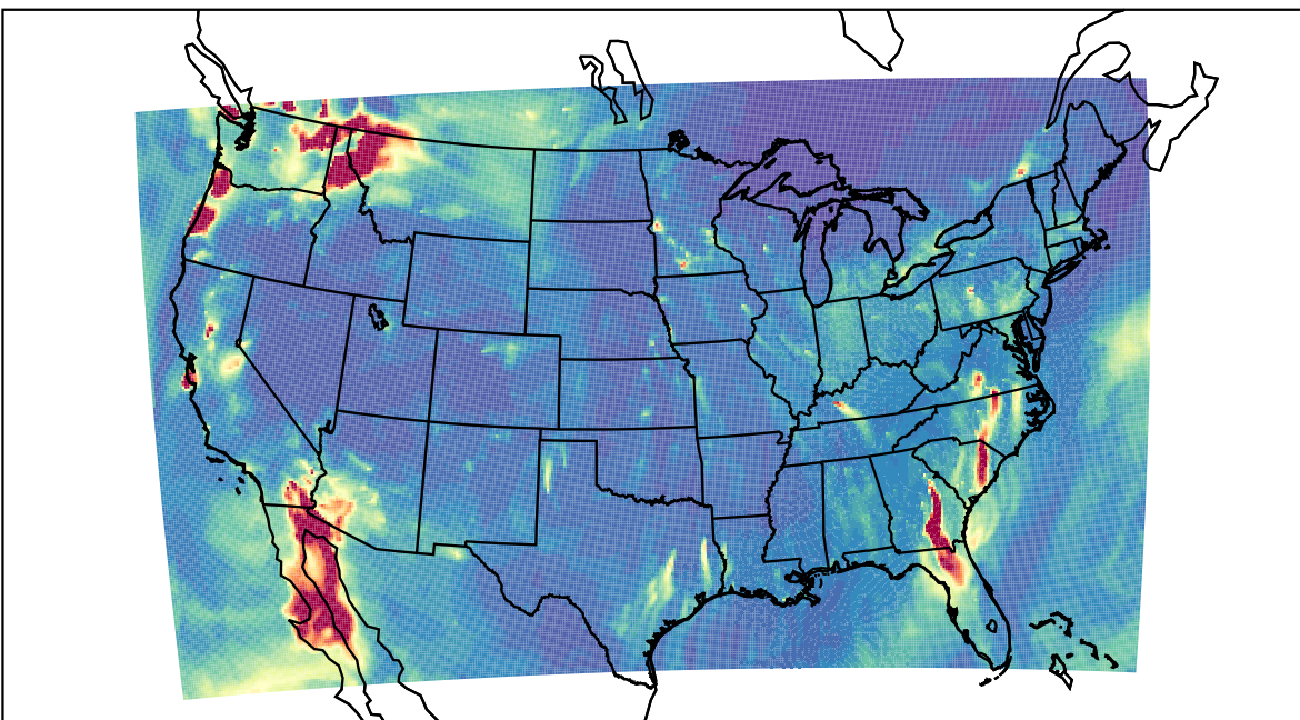
WRF 2023-11-01_05:00:00
