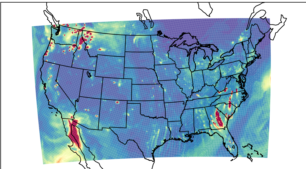
WRF 2023-11-01_00:00:00
