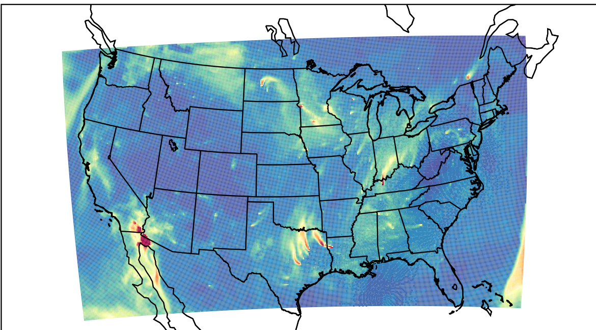
WRF 2023-11-02_15:00:00
