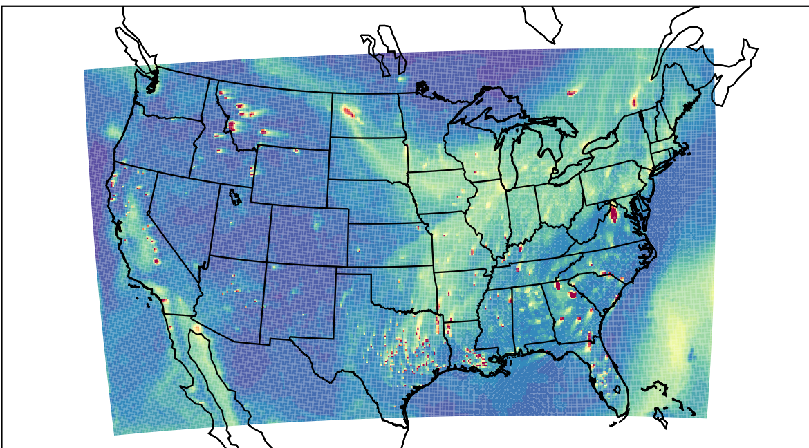
WRF 2023-11-03_23:00:00
