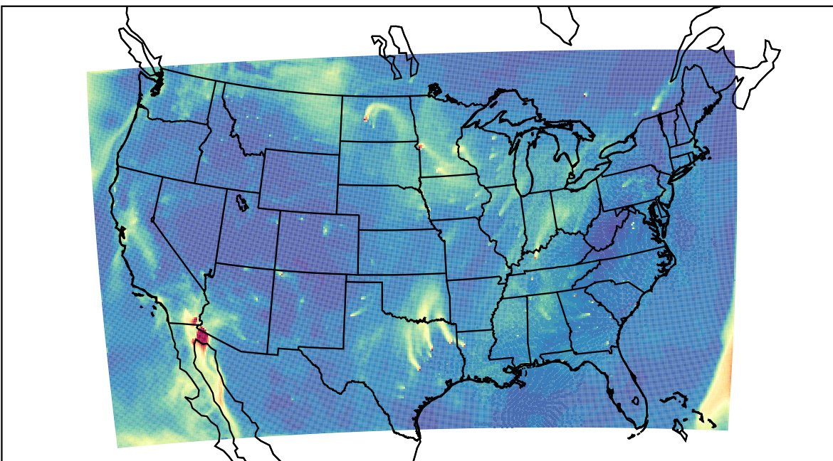
WRF 2023-11-02_17:00:00
