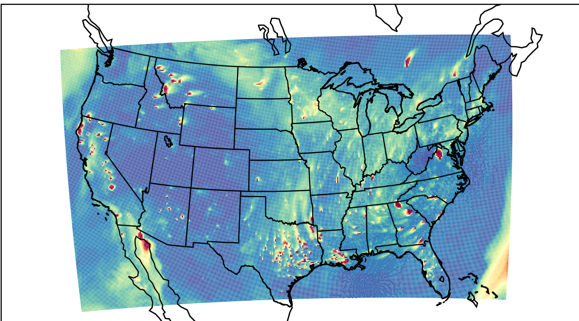
WRF 2023-11-03_00:00:00
