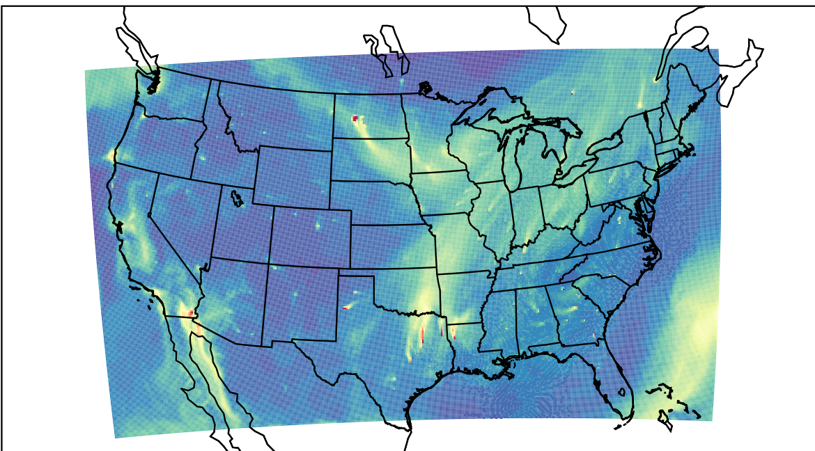
WRF 2023-11-03_17:00:00
