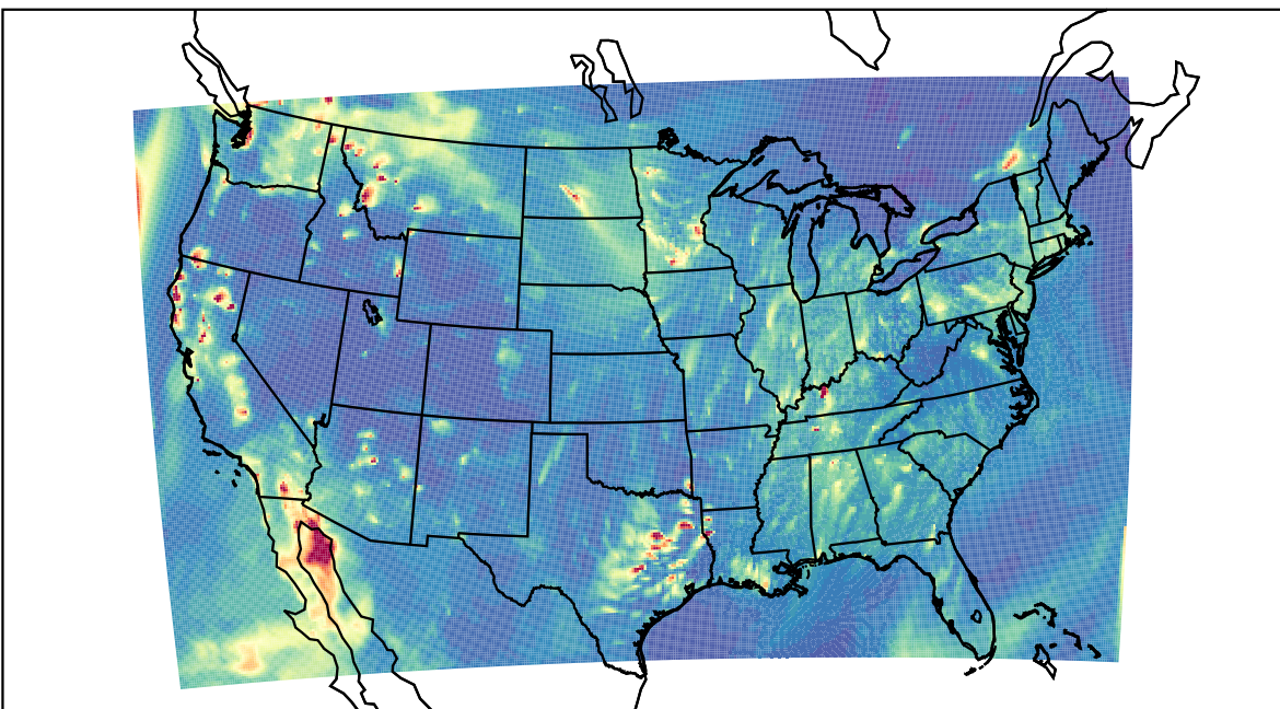
WRF 2023-11-02_04:00:00
