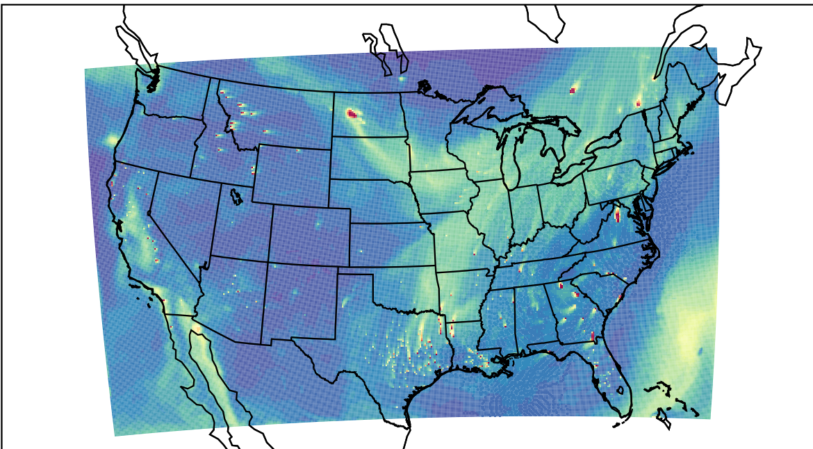
WRF 2023-11-03_21:00:00
