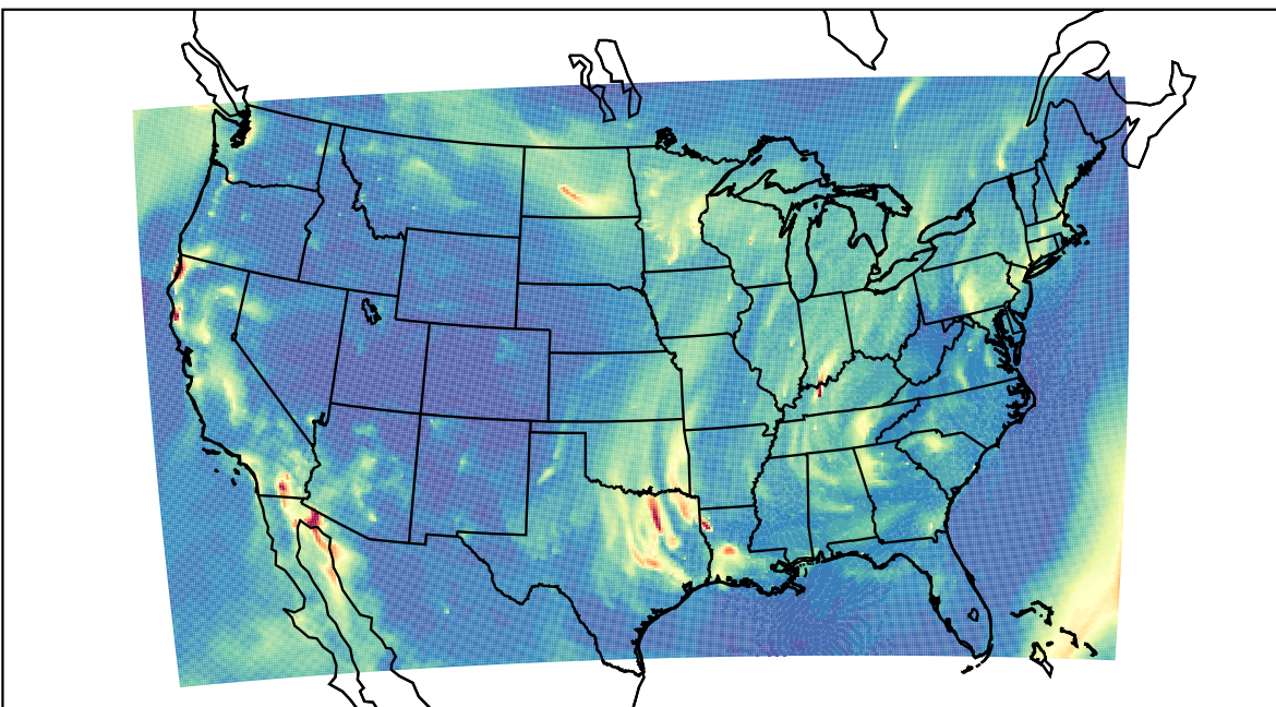
WRF 2023-11-03_07:00:00
