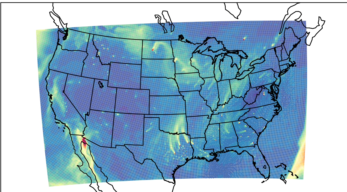
WRF 2023-11-02_19:00:00
