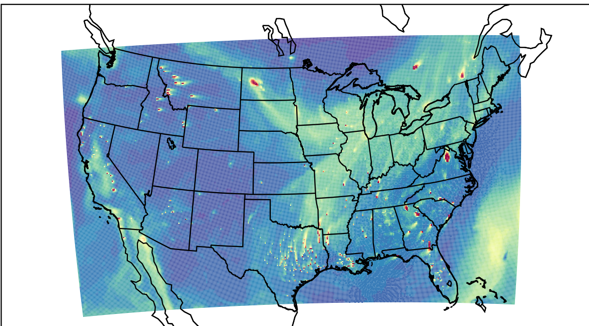
WRF 2023-11-03_22:00:00
