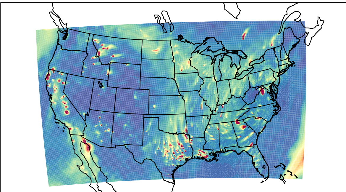
WRF 2023-11-03_01:00:00
