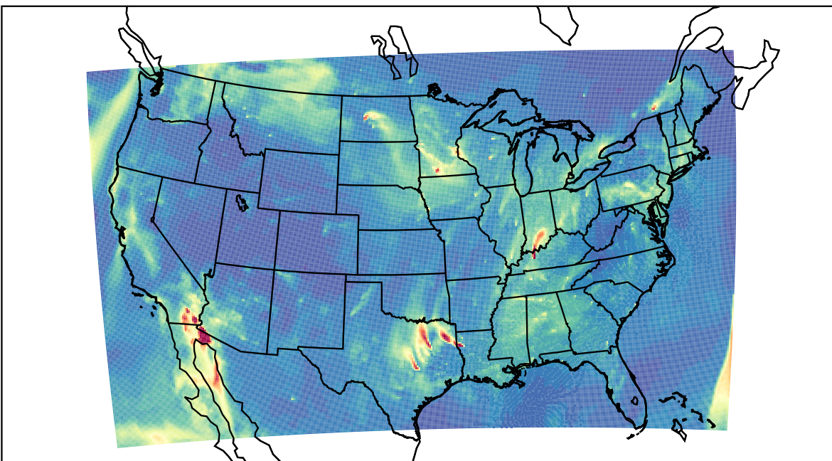
WRF 2023-11-02_12:00:00
