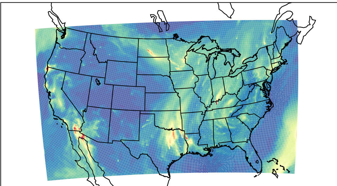
WRF 2023-11-03_11:00:00
