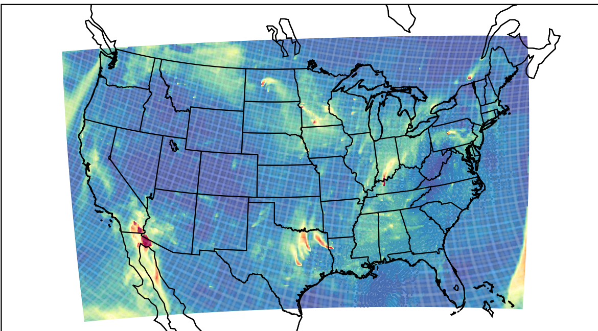
WRF 2023-11-02_14:00:00
