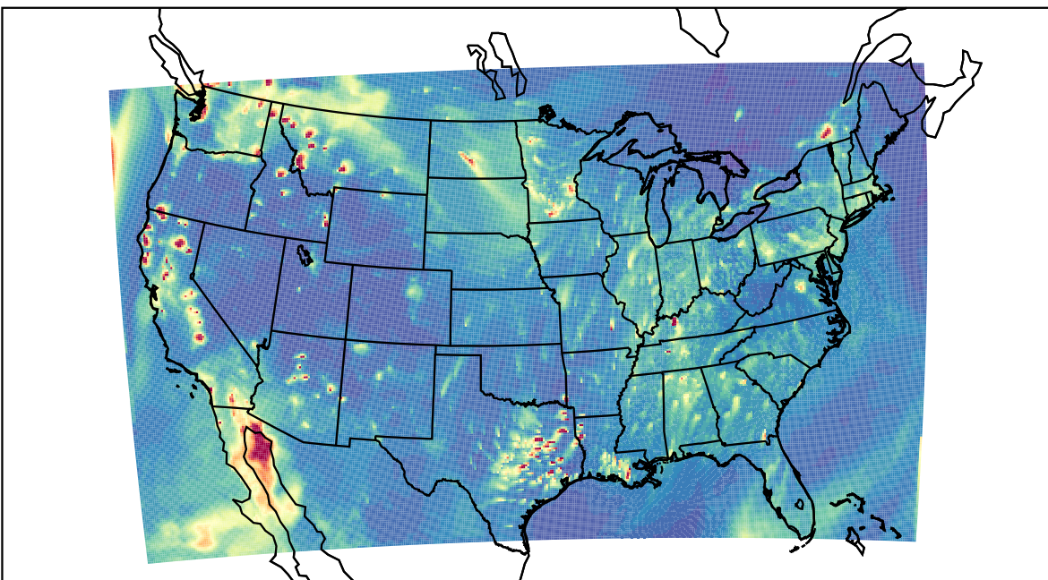
WRF 2023-11-02_03:00:00
