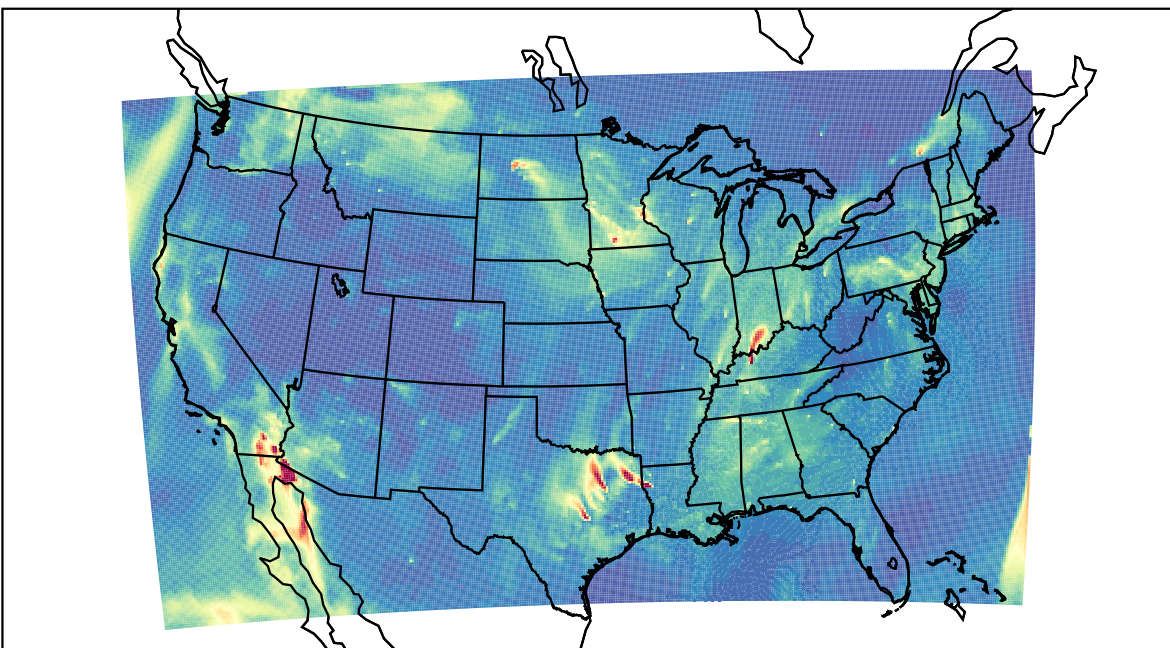
WRF 2023-11-02_11:00:00
