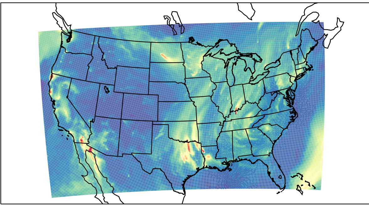
WRF 2023-11-03_09:00:00
