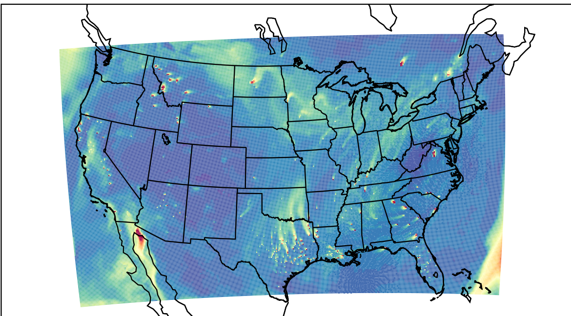
WRF 2023-11-02_21:00:00
