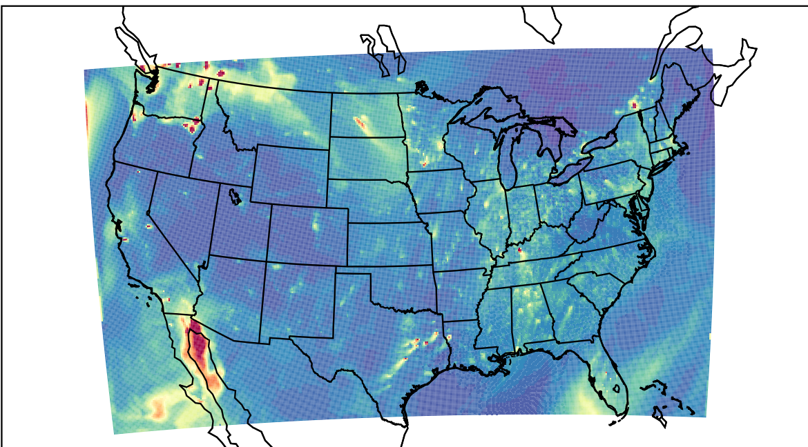
WRF 2023-11-02_00:00:00
