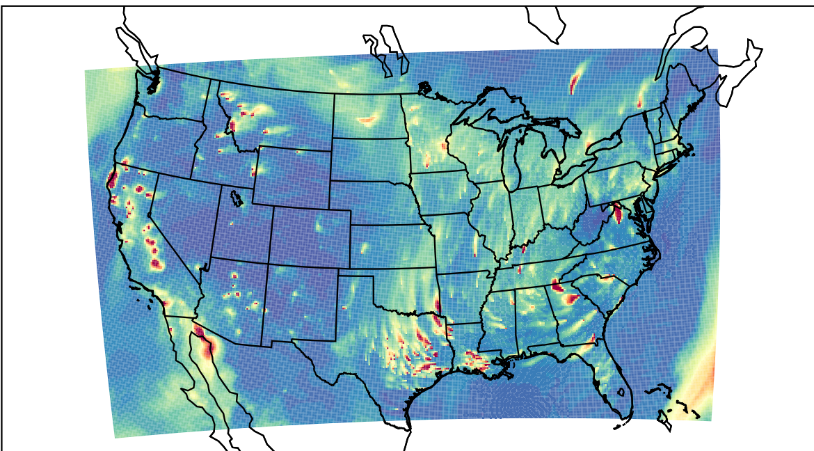
WRF 2023-11-03_02:00:00
