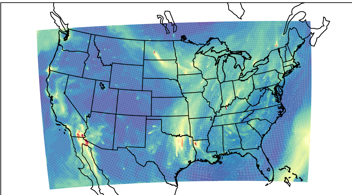
WRF 2023-11-03_14:00:00
