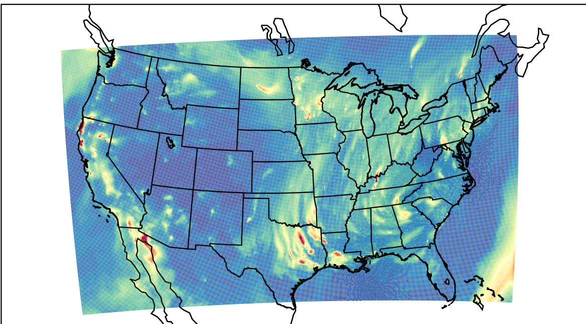
WRF 2023-11-03_05:00:00
