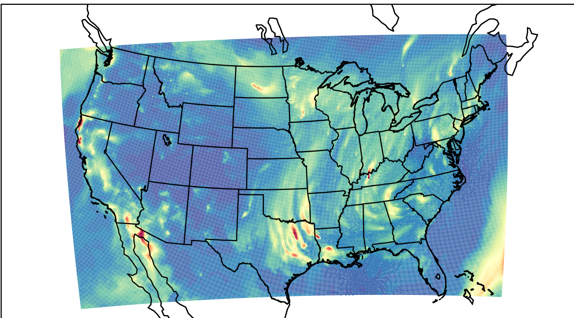
WRF 2023-11-03_06:00:00
