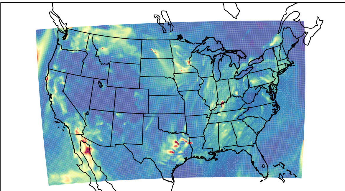
WRF 2023-11-02_07:00:00
