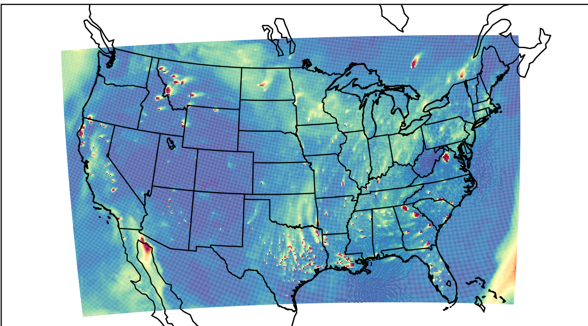
WRF 2023-11-02_23:00:00
