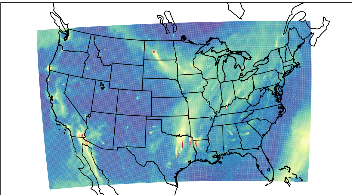
WRF 2023-11-03_16:00:00
