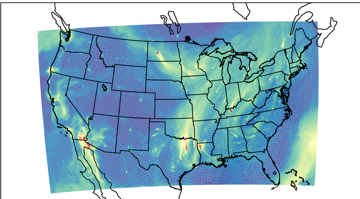
WRF 2023-11-03_15:00:00
