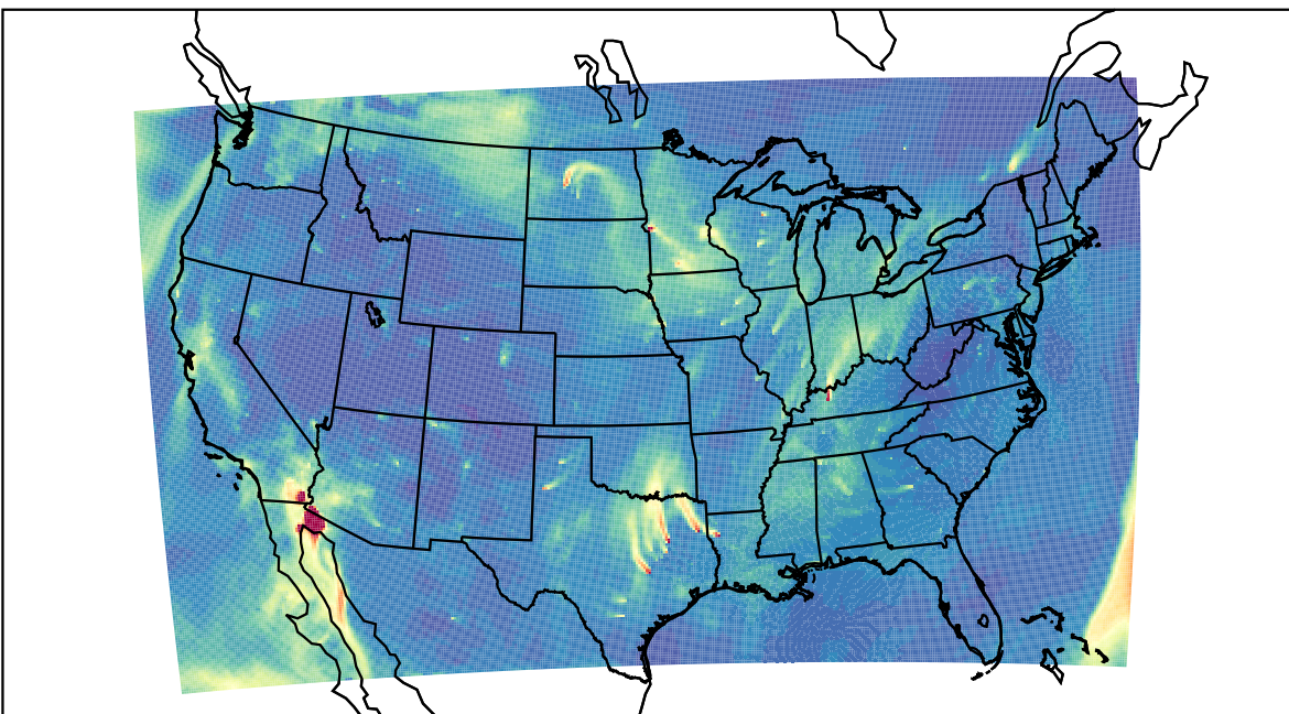
WRF 2023-11-02_16:00:00
