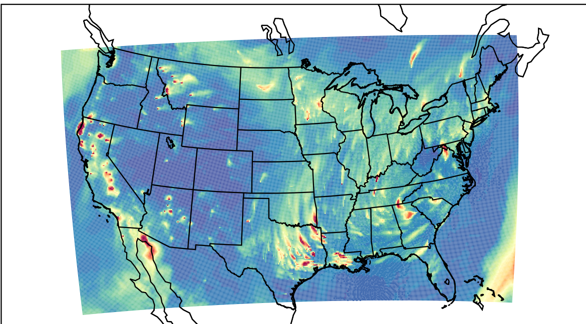
WRF 2023-11-03_03:00:00
