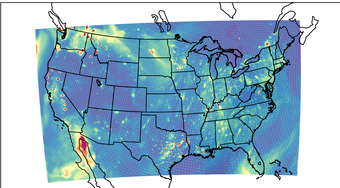
WRF 2023-11-02_01:00:00
