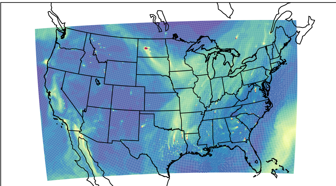
WRF 2023-11-03_19:00:00
