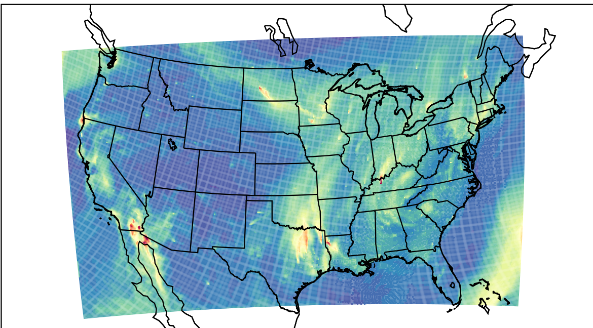
WRF 2023-11-03_12:00:00
