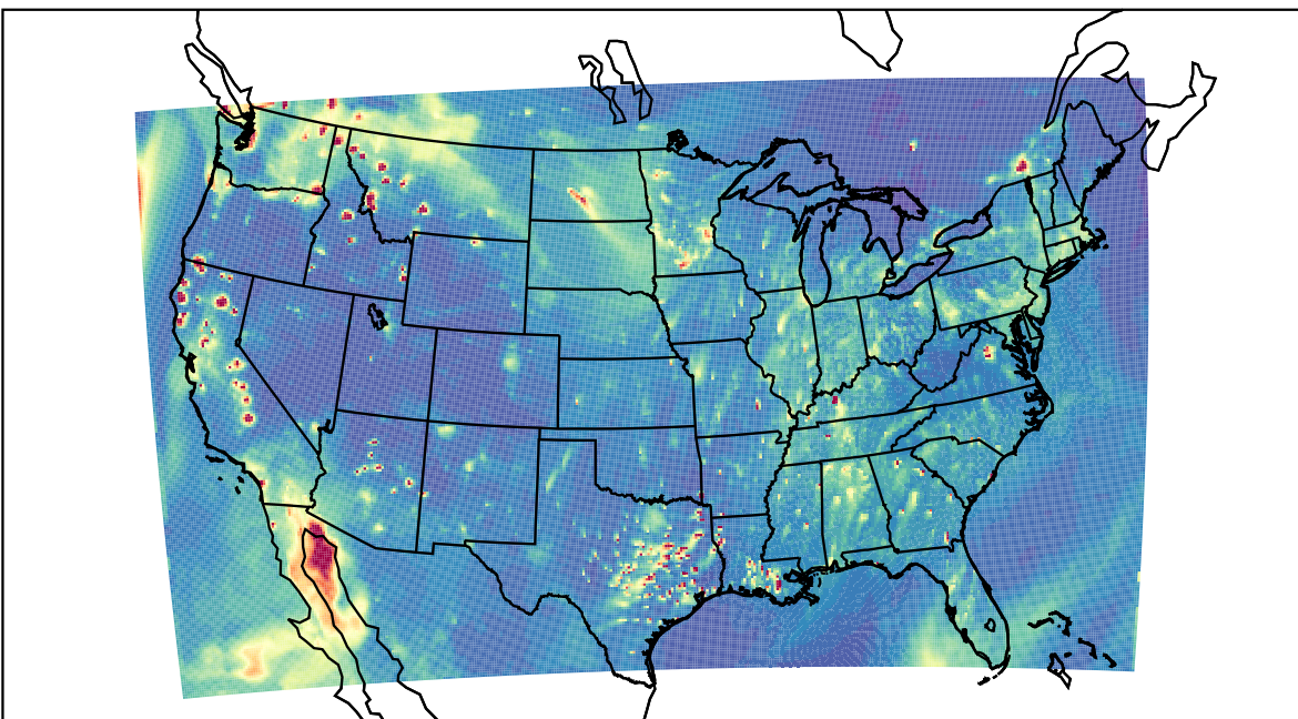
WRF 2023-11-02_02:00:00
