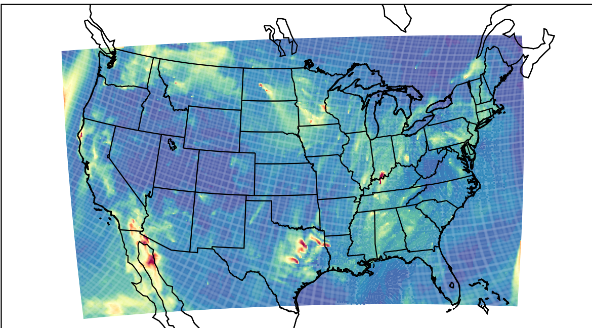
WRF 2023-11-02_08:00:00
