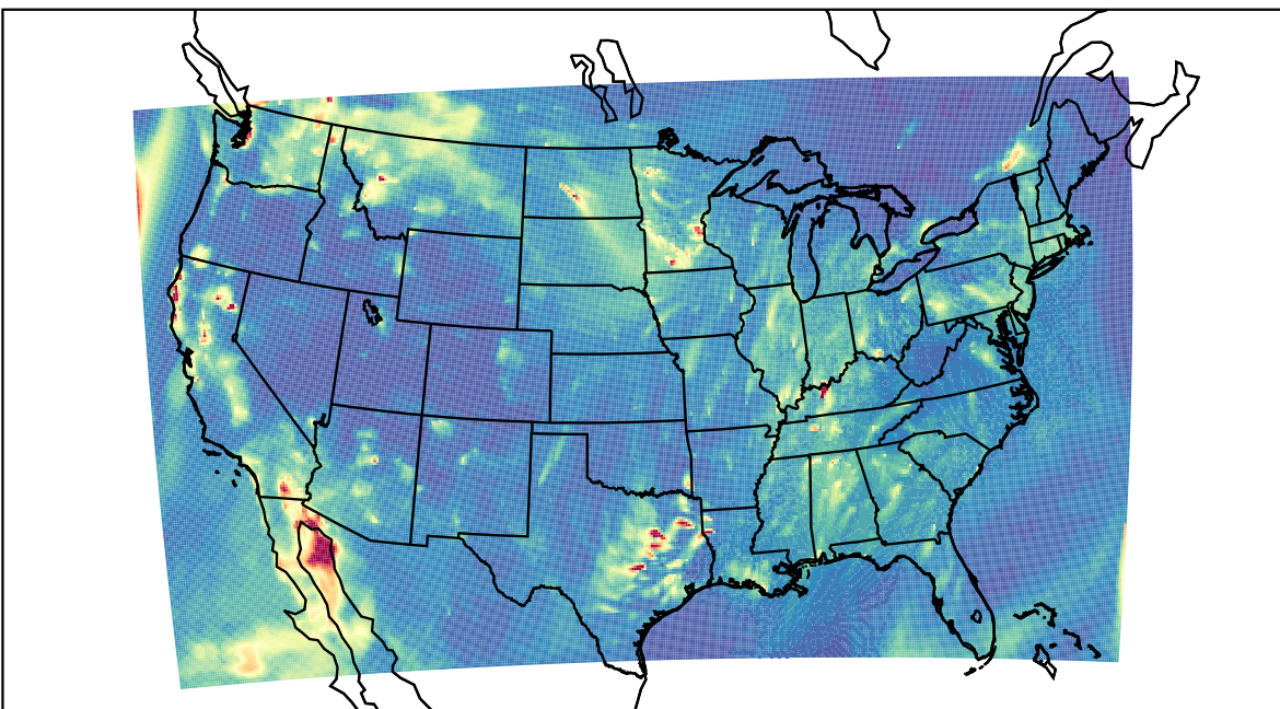
WRF 2023-11-02_05:00:00
