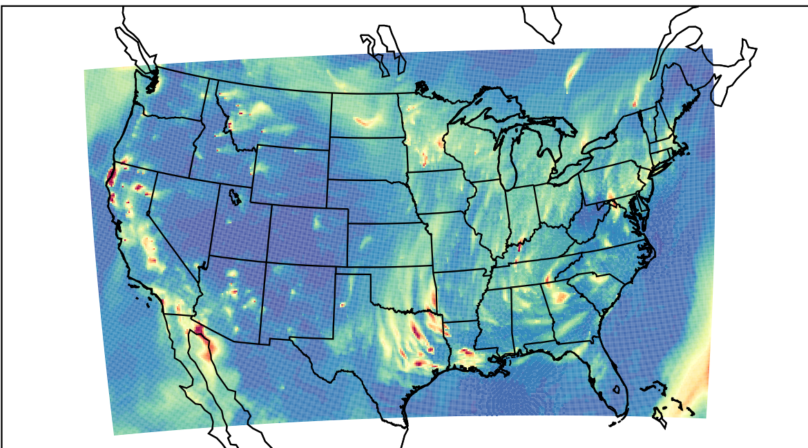
WRF 2023-11-03_04:00:00
