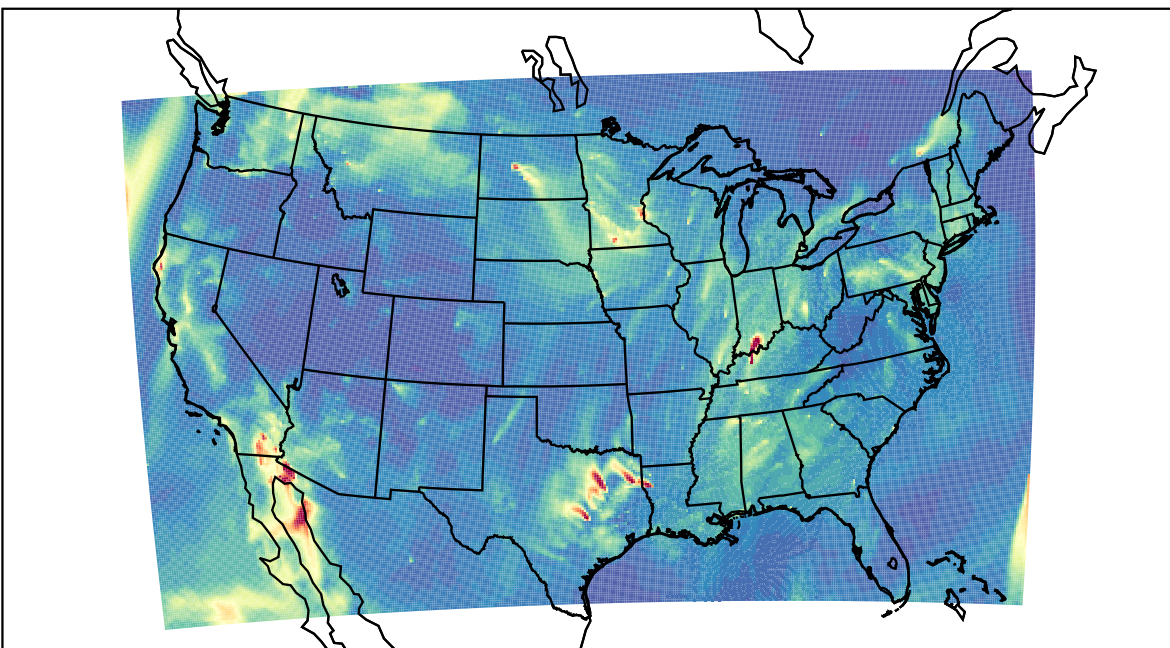
WRF 2023-11-02_09:00:00
