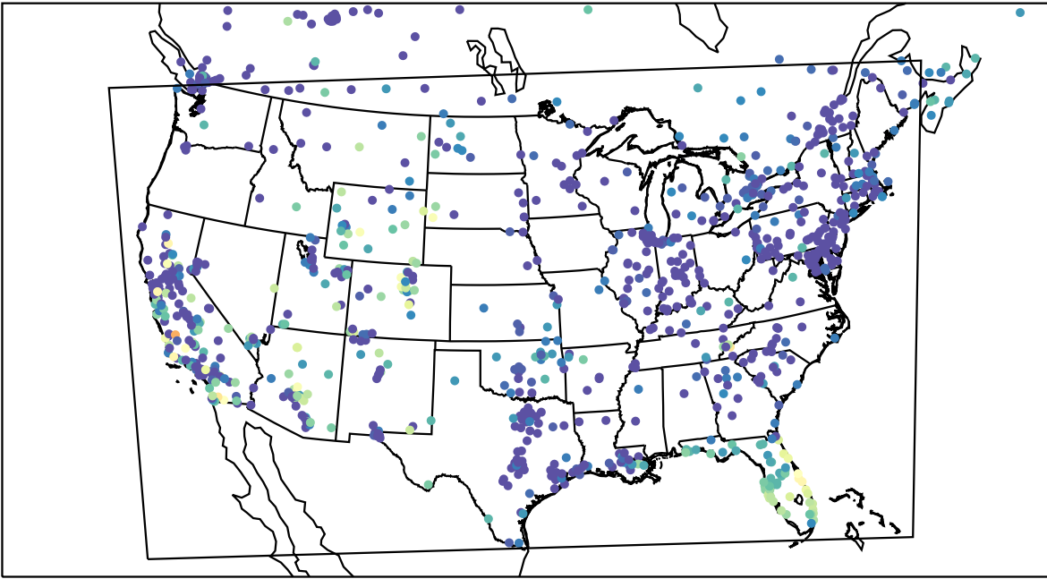
AirNOW (2023-11-02_09:00:00)
