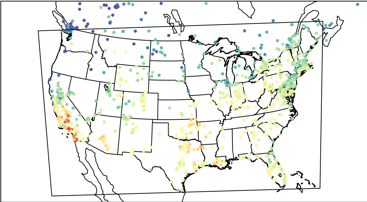
AirNOW (2023-11-03_20:00:00)
