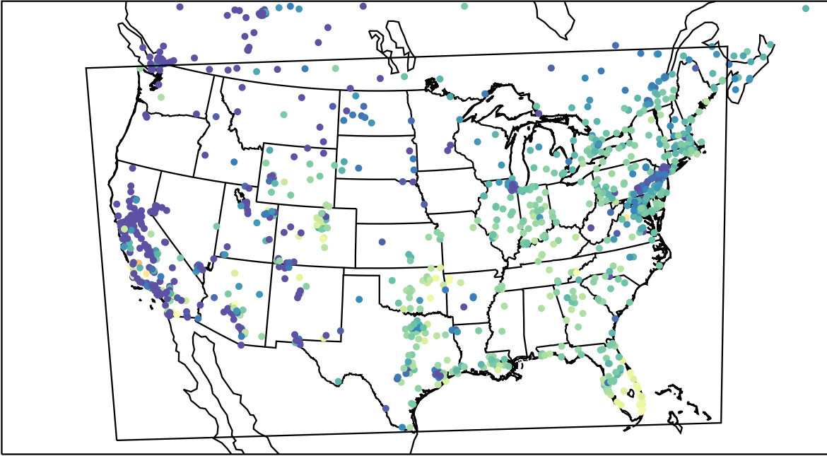
AirNOW (2023-11-03_15:00:00)
