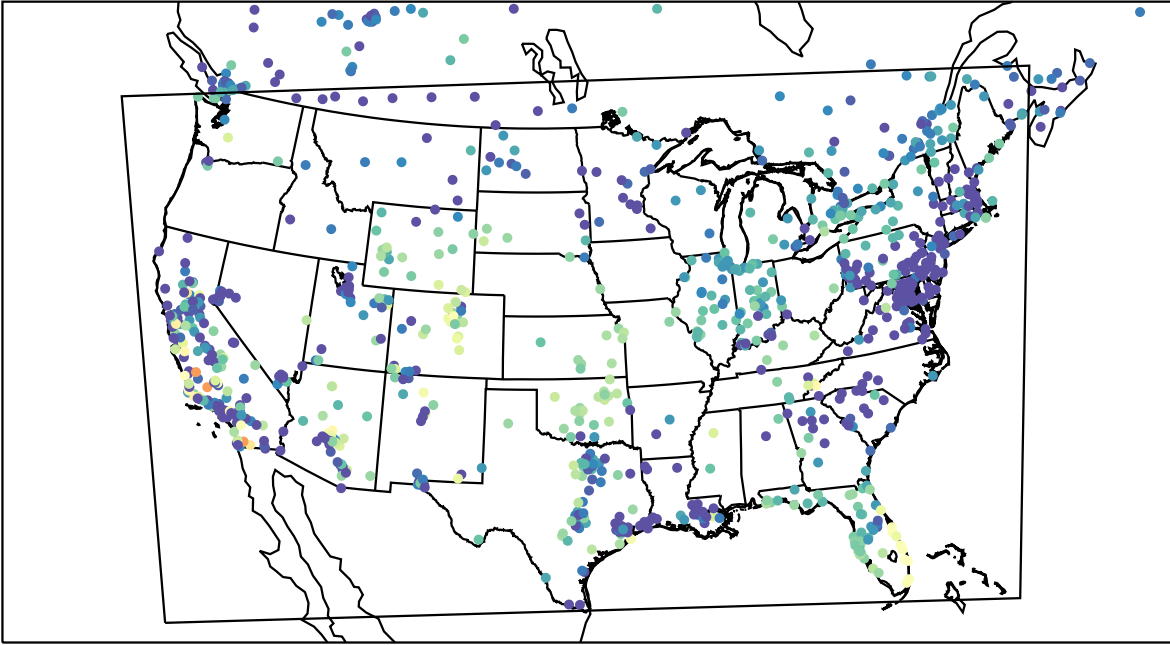
AirNOW (2023-11-03_05:00:00)
