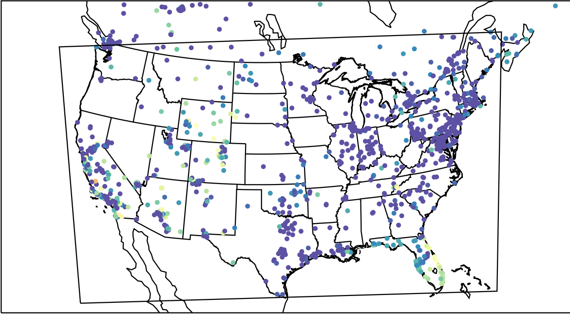
AirNOW (2023-11-02_12:00:00)
