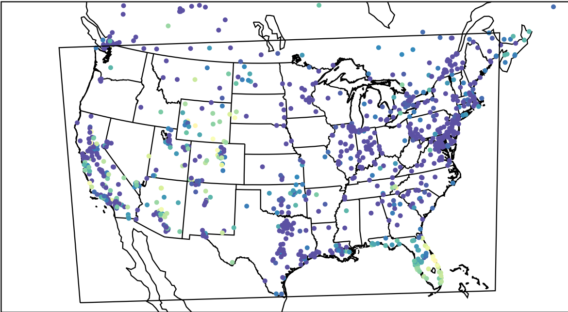
AirNOW (2023-11-02_10:00:00)
