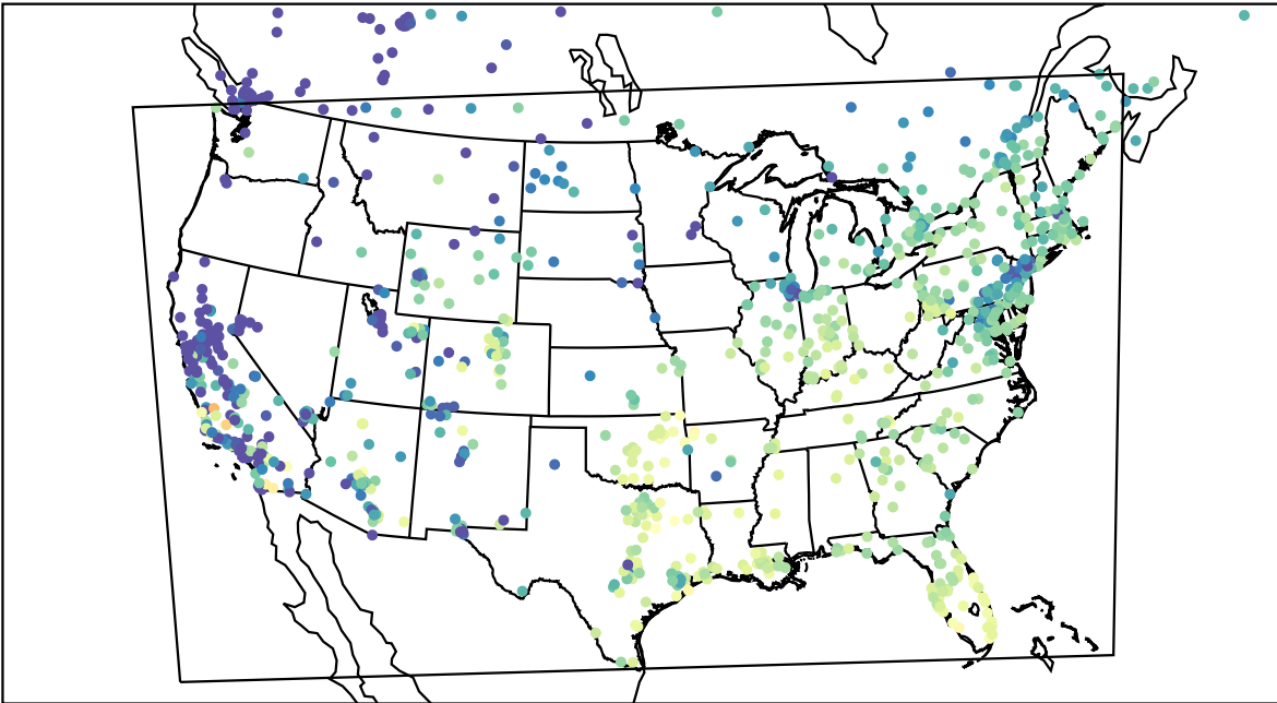
AirNOW (2023-11-03_16:00:00)
