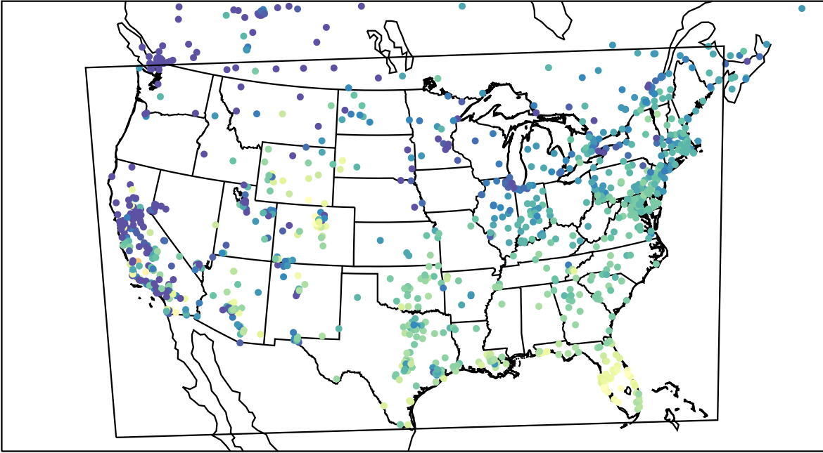
AirNOW (2023-11-02_16:00:00)
