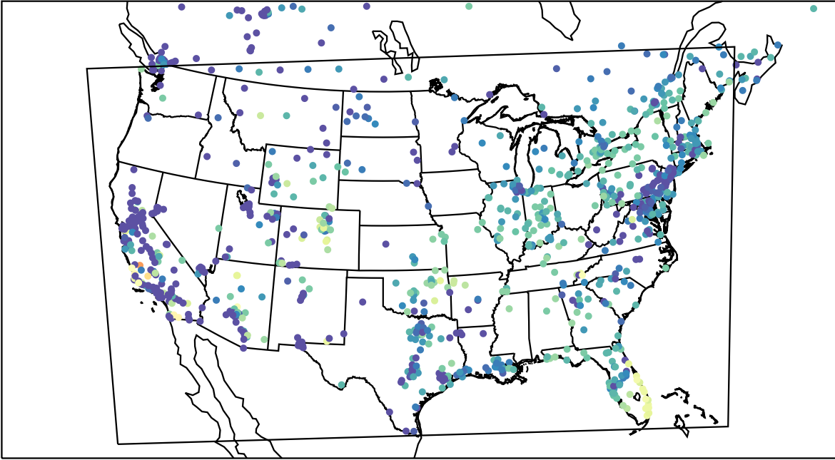
AirNOW (2023-11-03_14:00:00)
