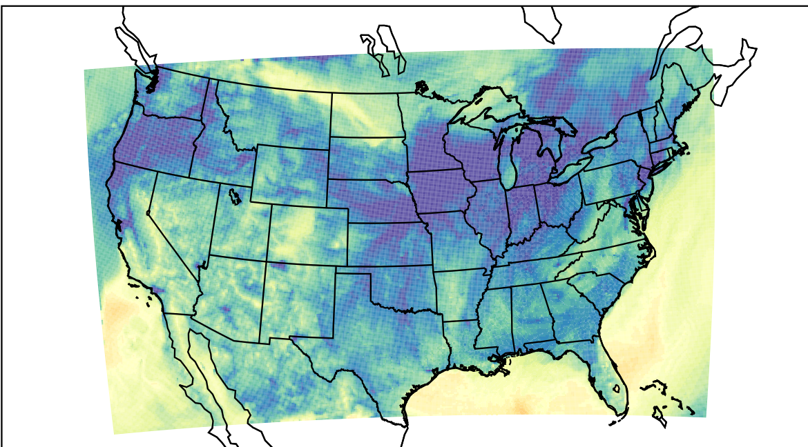
WRF (2023-11-03_09:00:00)
