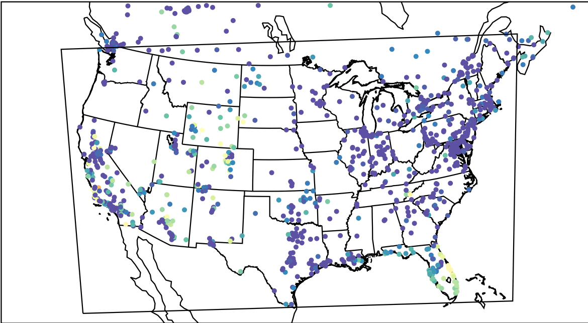
AirNOW (2023-11-02_11:00:00)
