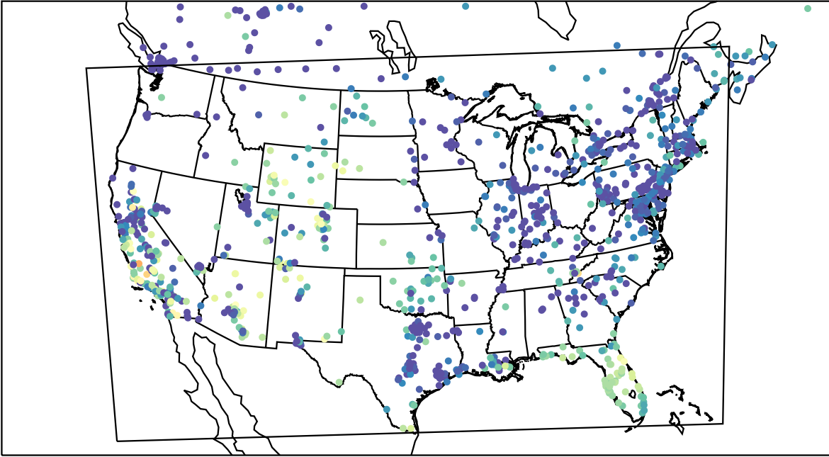
AirNOW (2023-11-02_02:00:00)
