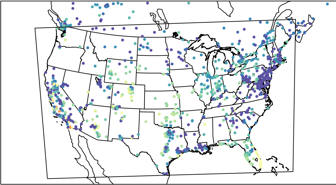
AirNOW (2023-11-03_04:00:00)
