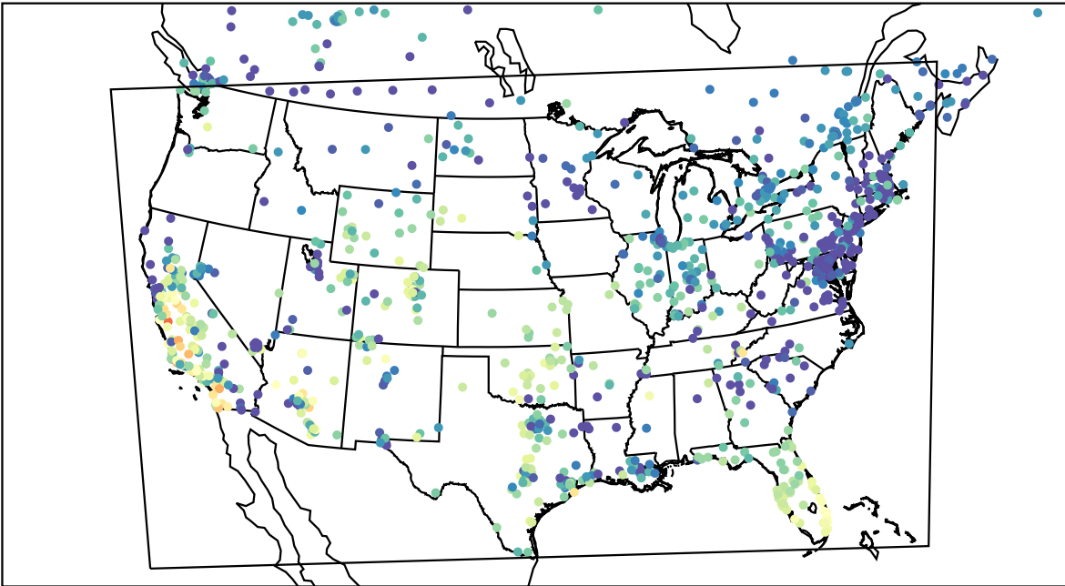
AirNOW (2023-11-03_01:00:00)
