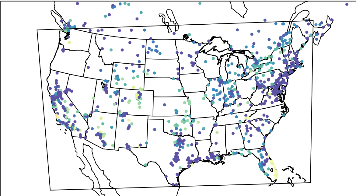
AirNOW (2023-11-03_10:00:00)
