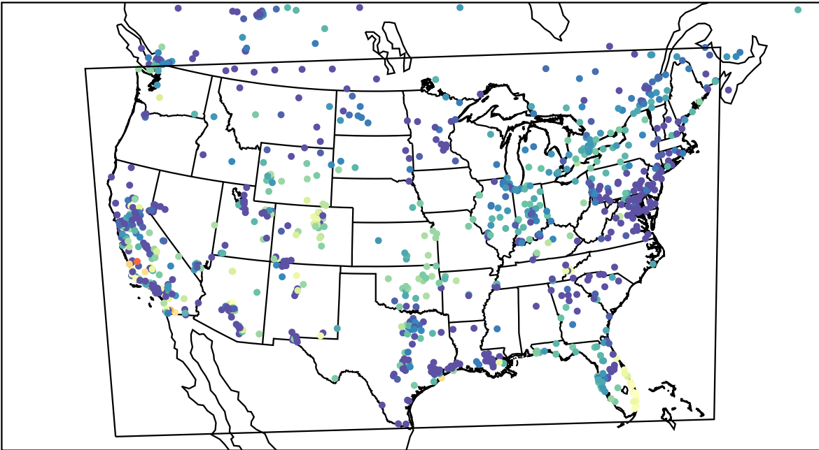
AirNOW (2023-11-03_08:00:00)
