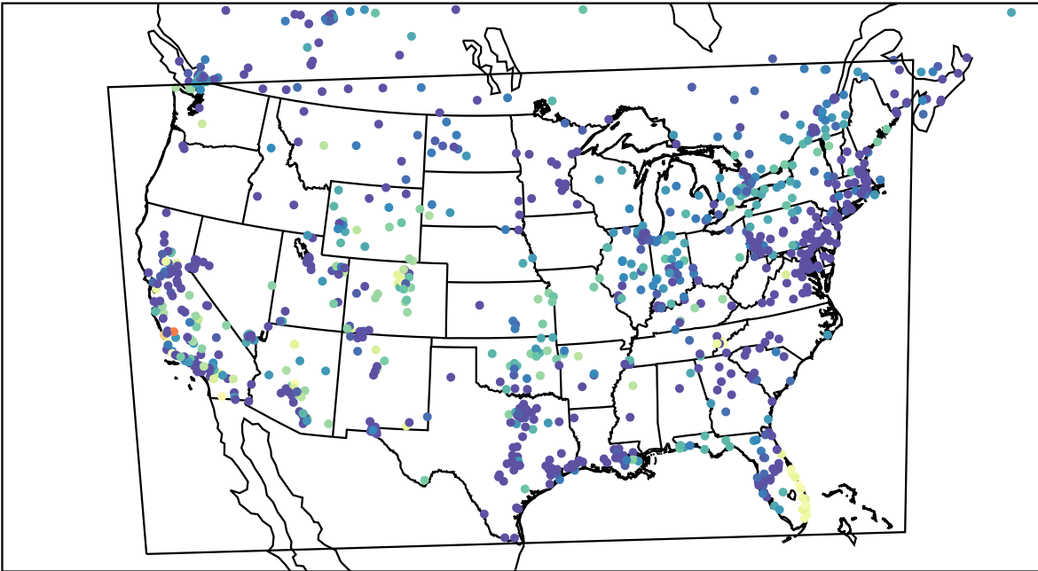
AirNOW (2023-11-03_11:00:00)
