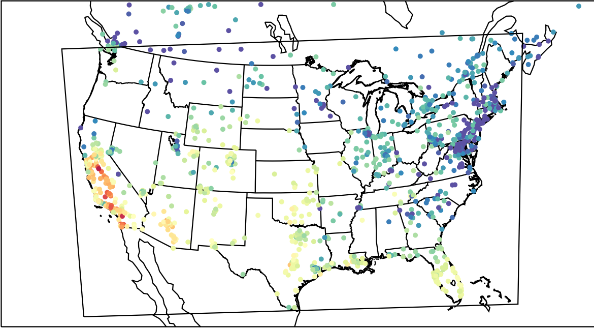
AirNOW (2023-11-02_23:00:00)
