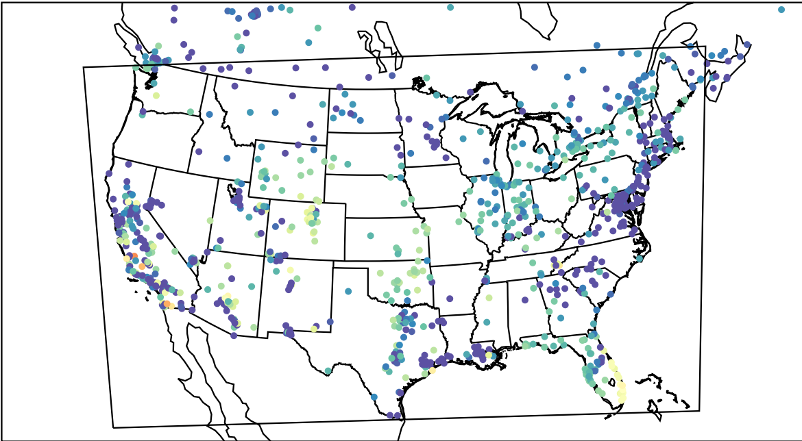
AirNOW (2023-11-03_06:00:00)
