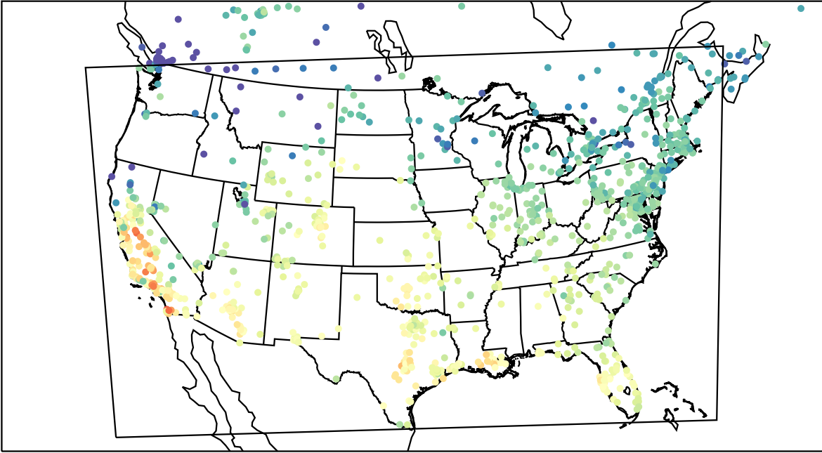
AirNOW (2023-11-02_20:00:00)
