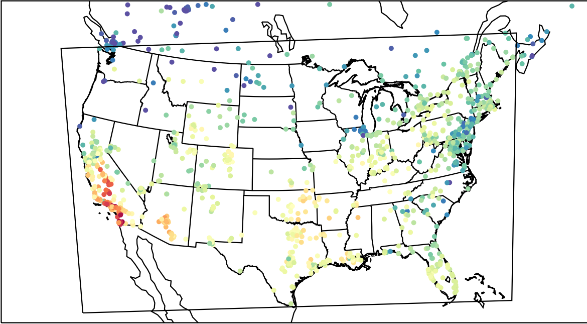
AirNOW (2023-11-03_22:00:00)
