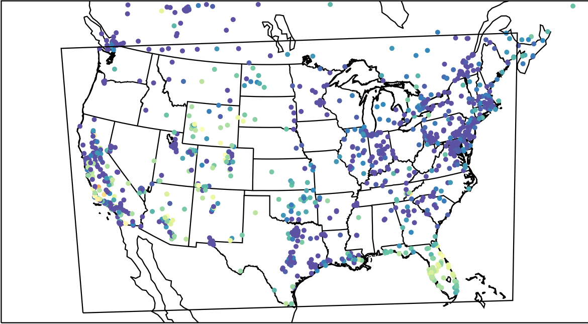
AirNOW (2023-11-02_04:00:00)
