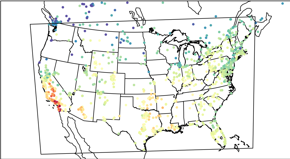
AirNOW (2023-11-03_21:00:00)
