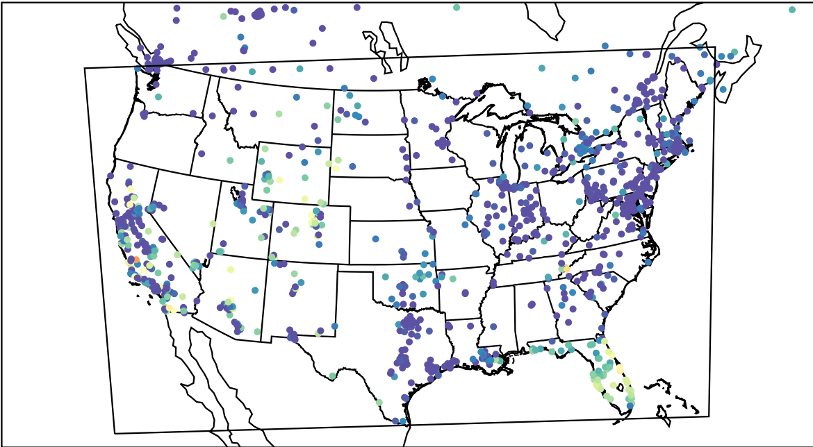
AirNOW (2023-11-02_08:00:00)
