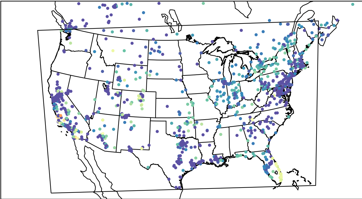
AirNOW (2023-11-03_13:00:00)
