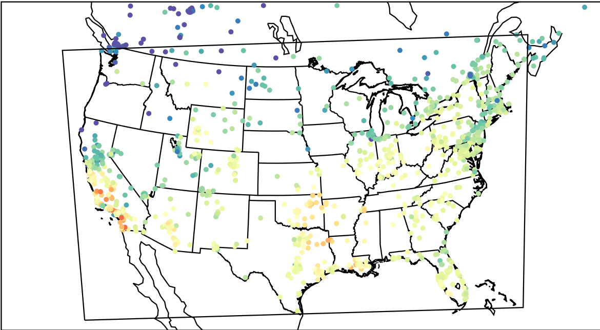
AirNOW (2023-11-03_19:00:00)
