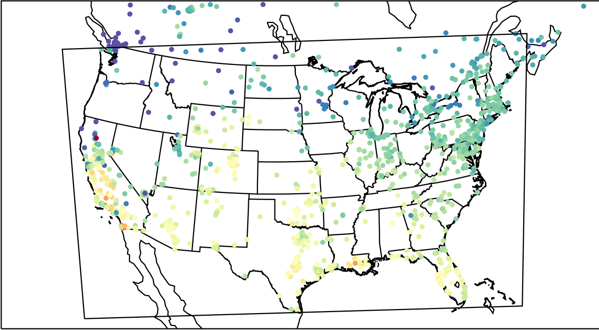
AirNOW (2023-11-02_19:00:00)
