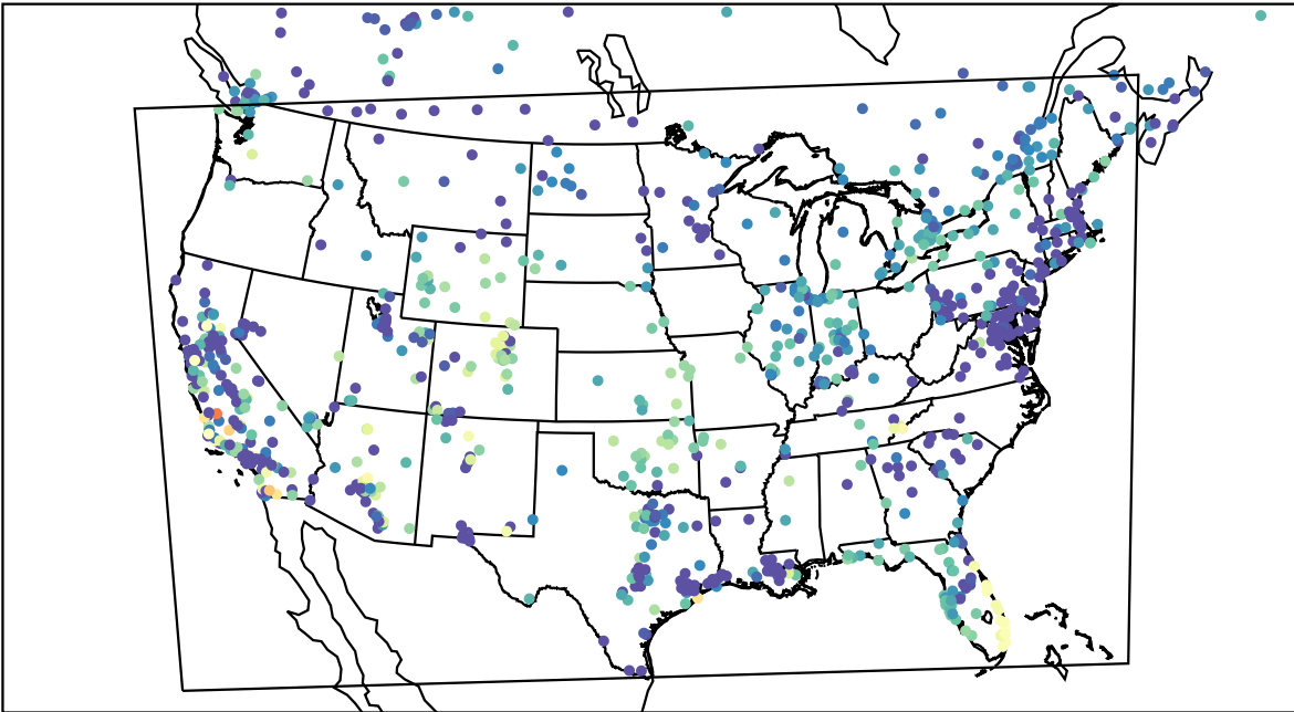
AirNOW (2023-11-03_07:00:00)
