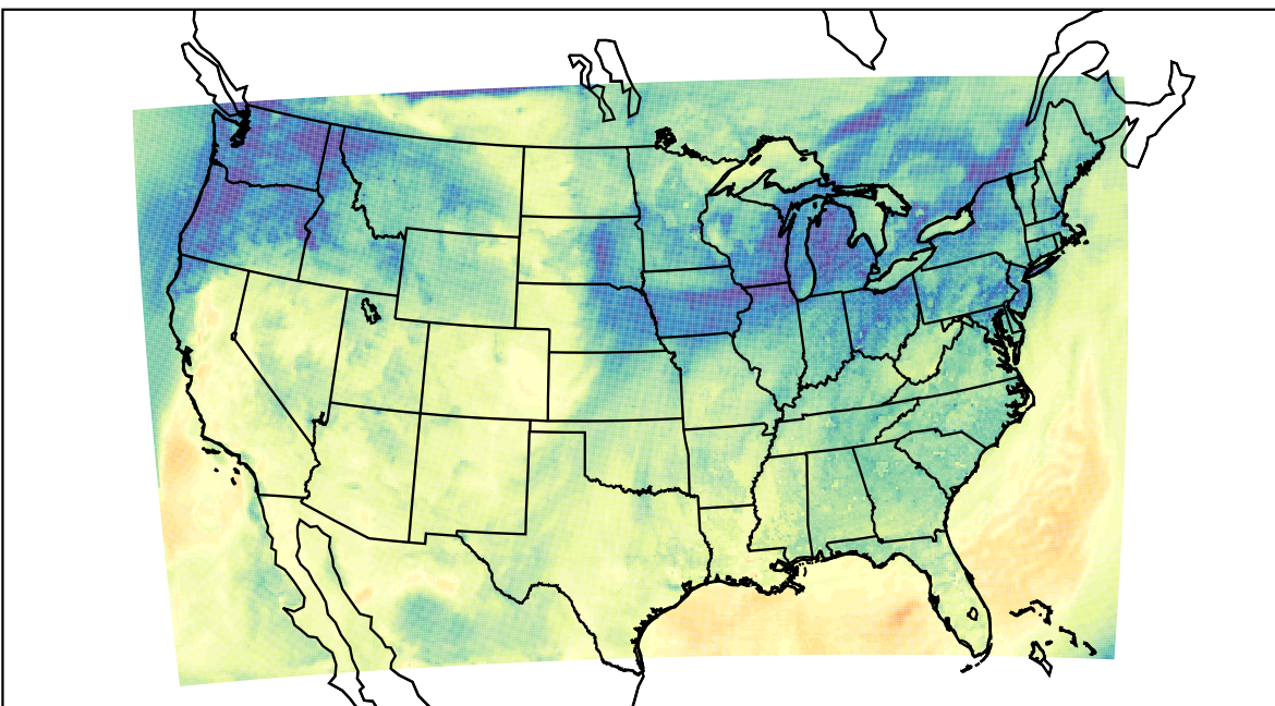
WRF (2023-11-02_22:00:00)
