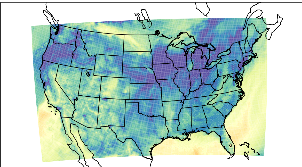
WRF (2023-11-03_08:00:00)
