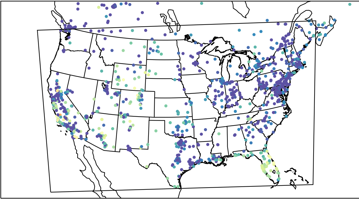
AirNOW (2023-11-02_05:00:00)
