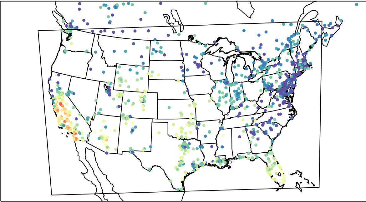
AirNOW (2023-11-03_00:00:00)
