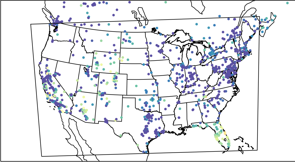
AirNOW (2023-11-02_07:00:00)
