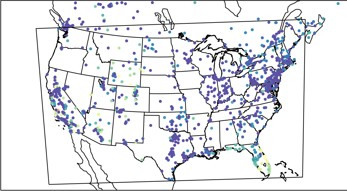
AirNOW (2023-11-02_13:00:00)
