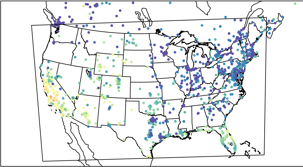
AirNOW (2023-11-02_00:00:00)
