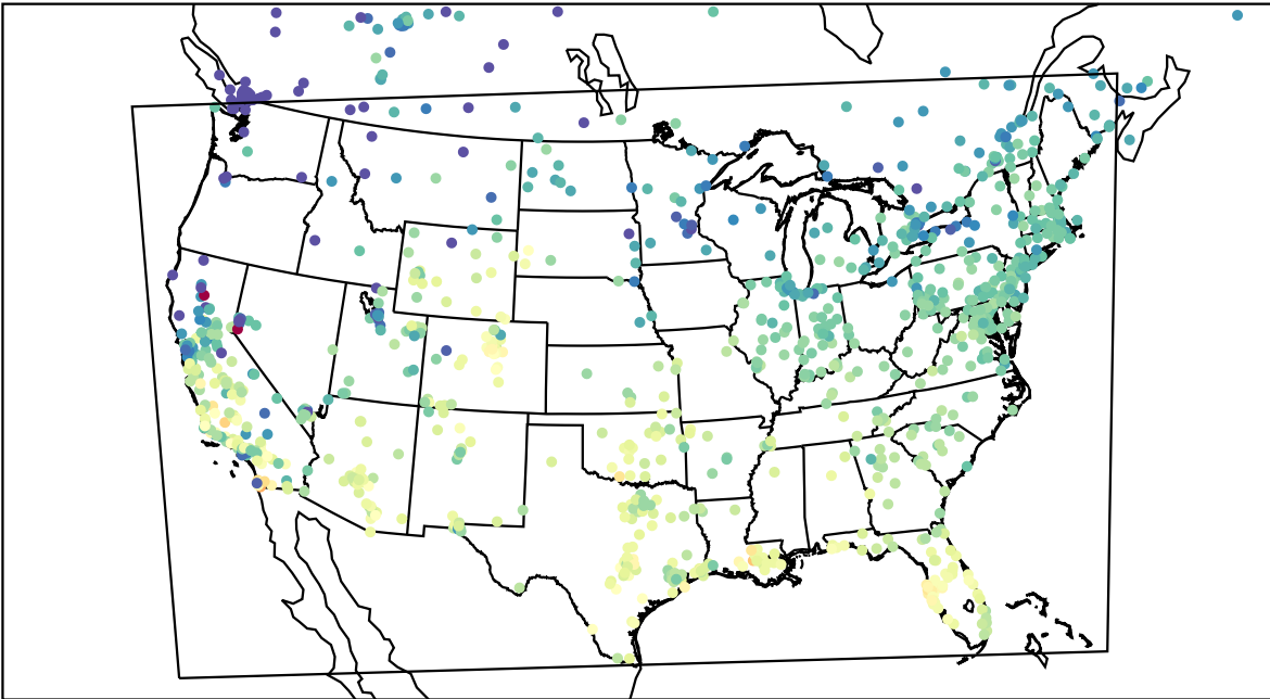
AirNOW (2023-11-02_18:00:00)
