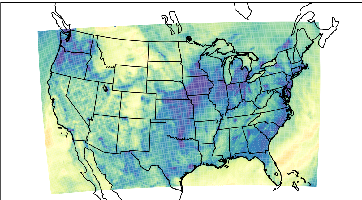
WRF (2023-11-02_06:00:00)
