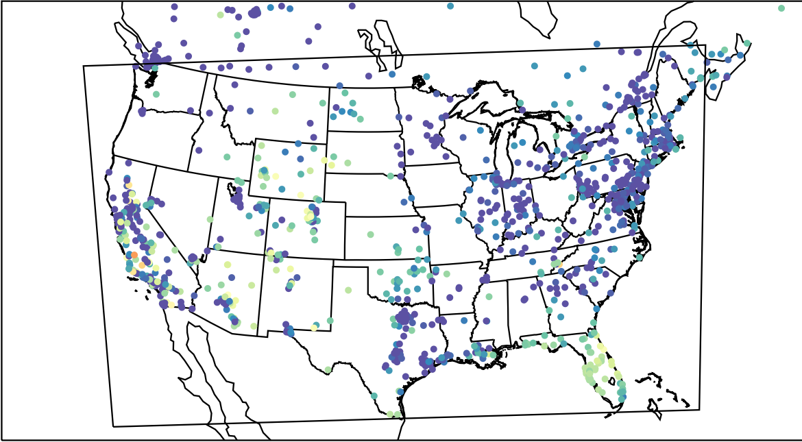
AirNOW (2023-11-02_03:00:00)
