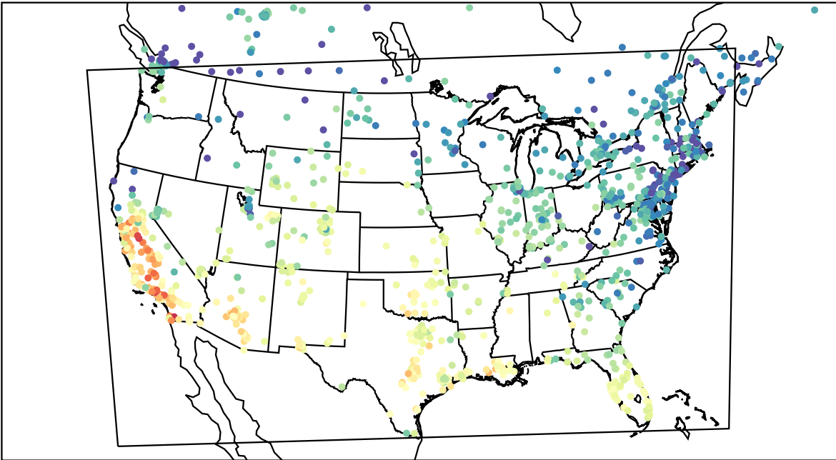
AirNOW (2023-11-02_22:00:00)
