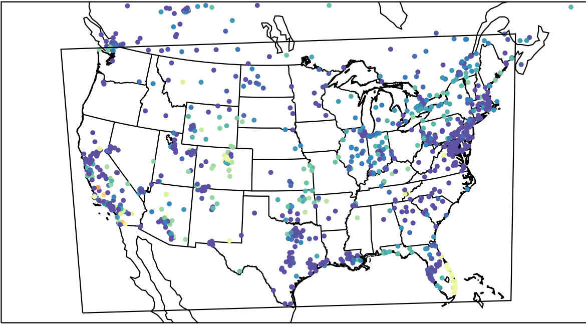
AirNOW (2023-11-03_12:00:00)
