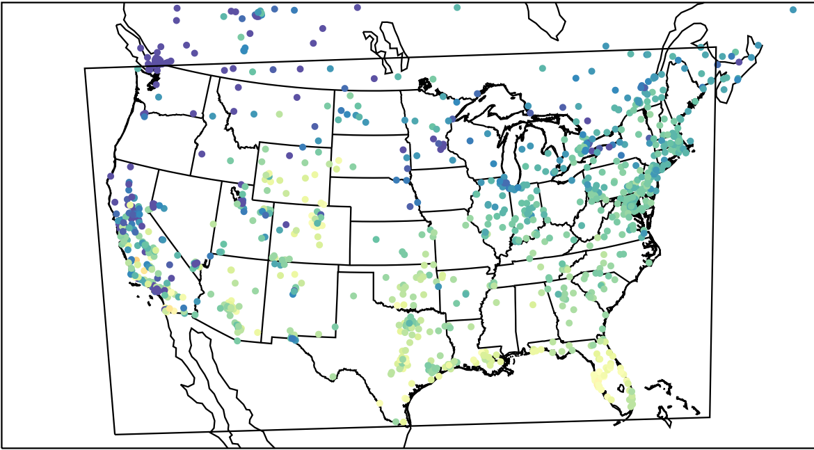
AirNOW (2023-11-02_17:00:00)
