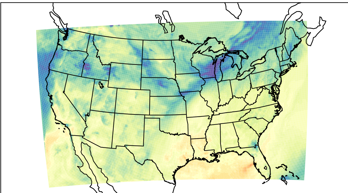
WRF (2023-11-03_20:00:00)
