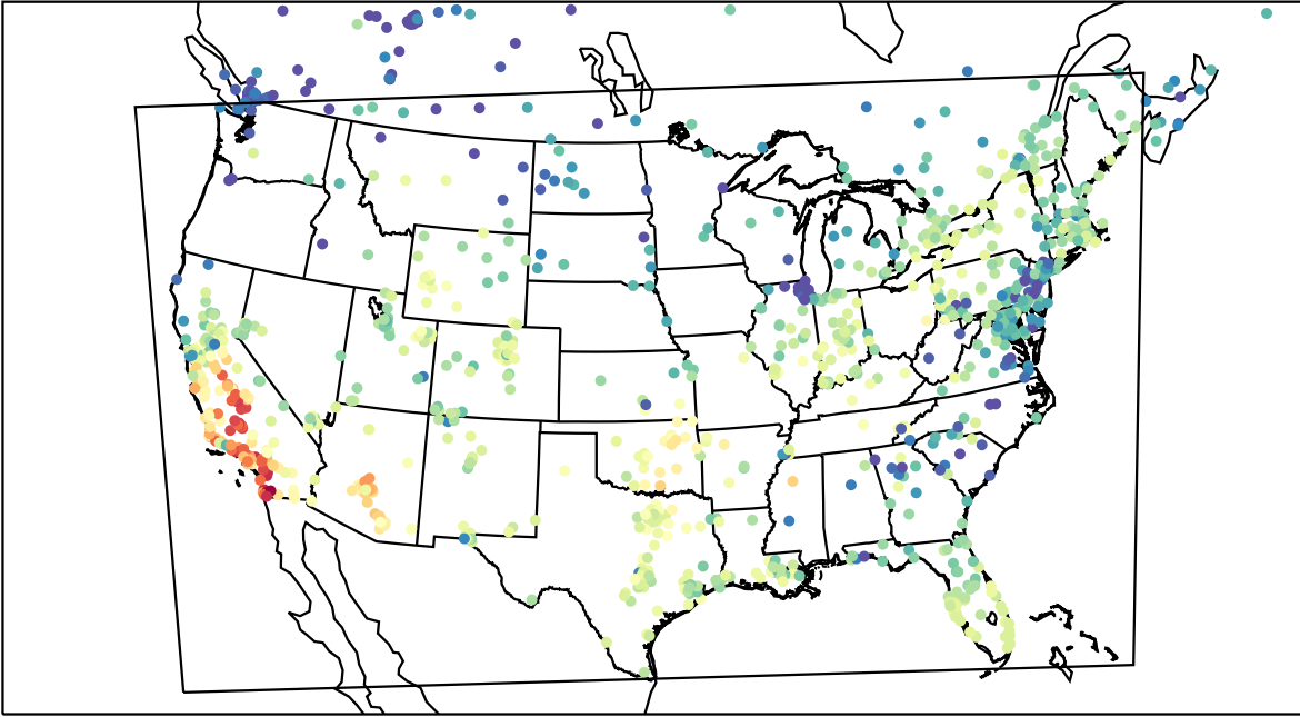
AirNOW (2023-11-03_23:00:00)
