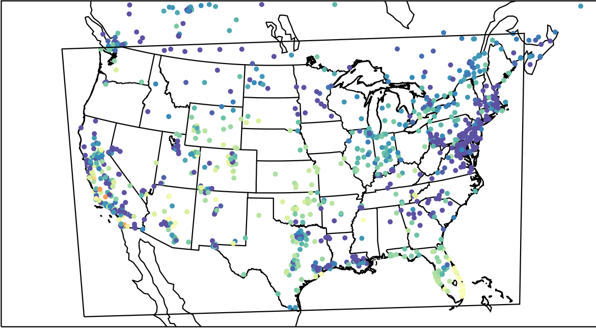
AirNOW (2023-11-03_03:00:00)
