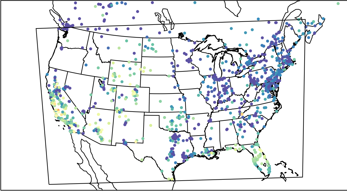
AirNOW (2023-11-02_01:00:00)
