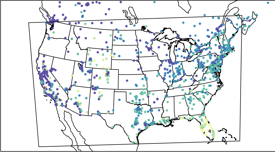
AirNOW (2023-11-02_15:00:00)
