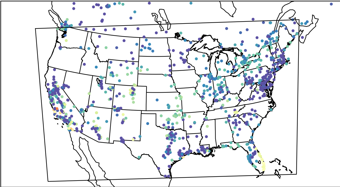
AirNOW (2023-11-03_09:00:00)
