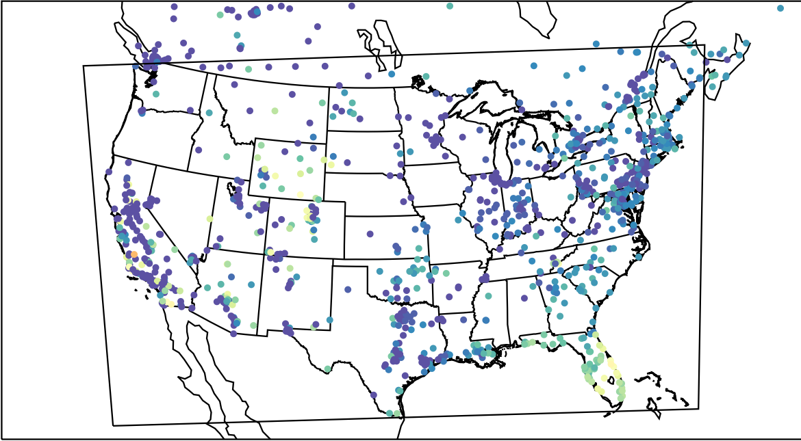
AirNOW (2023-11-02_14:00:00)
