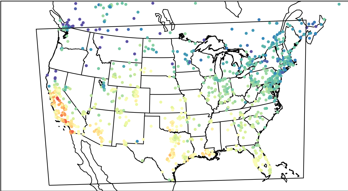
AirNOW (2023-11-02_21:00:00)
