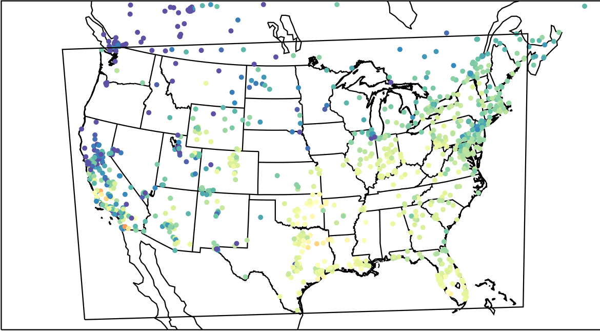
AirNOW (2023-11-03_17:00:00)
