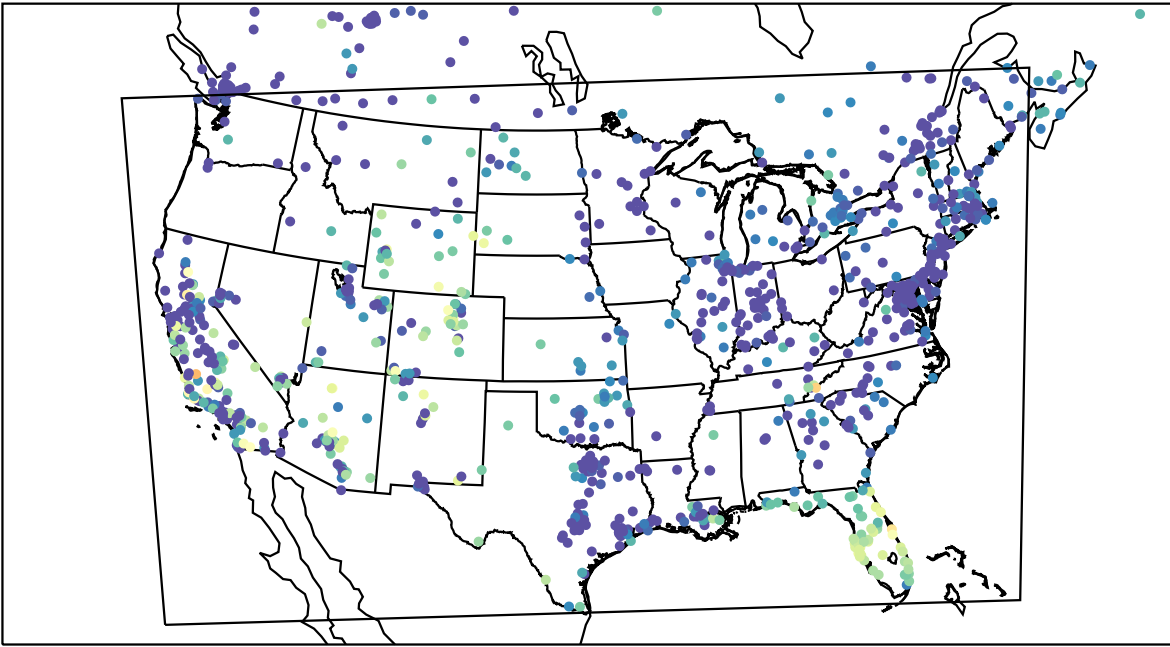
AirNOW (2023-11-02_06:00:00)
