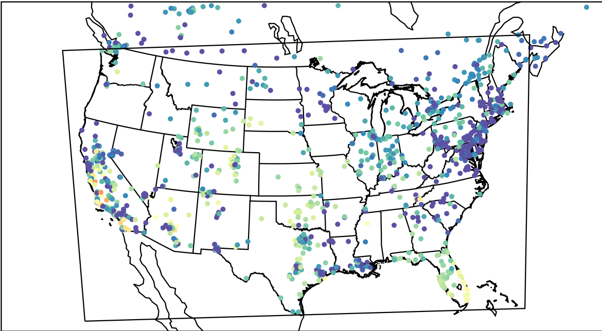
AirNOW (2023-11-03_02:00:00)
