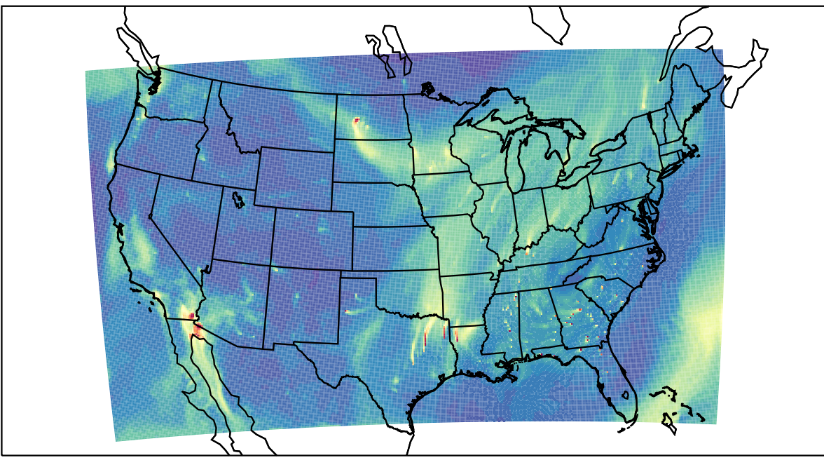
WRF 2023-11-03_17:00:00
