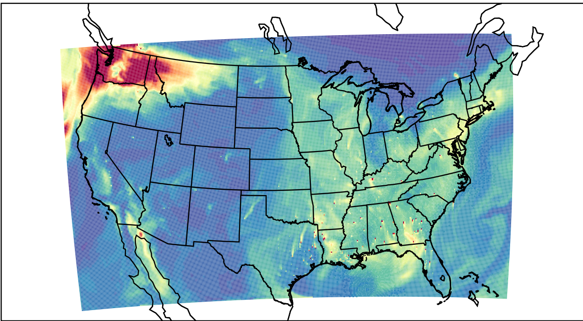
WRF 2023-11-05_19:00:00
