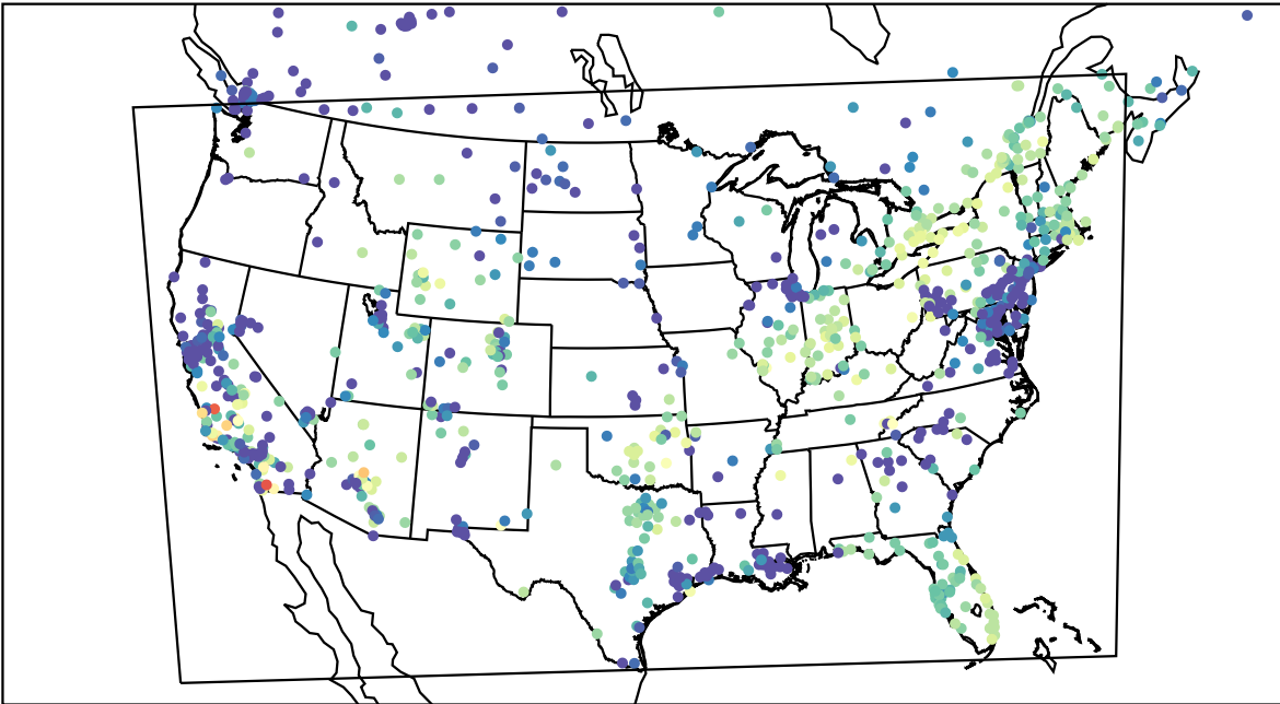
AirNOW (2023-11-04_04:00:00)
