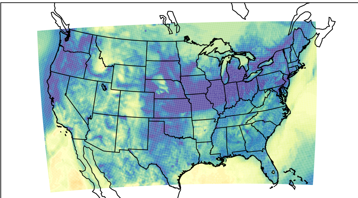
WRF (2023-11-04_13:00:00)
