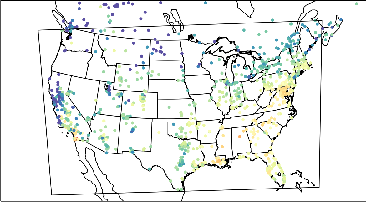
AirNOW (2023-11-05_17:00:00)
