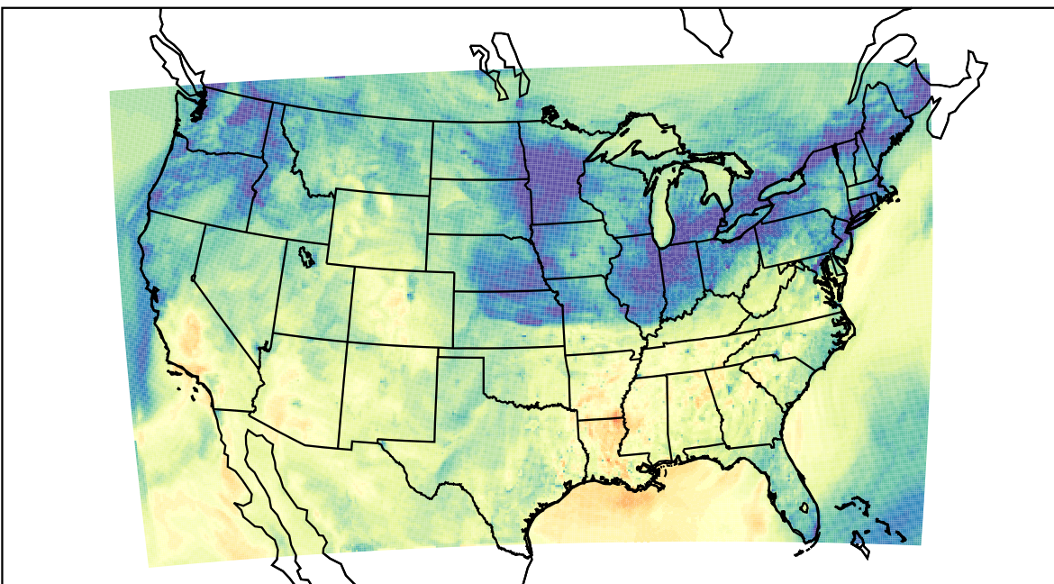
WRF (2023-11-04_23:00:00)
