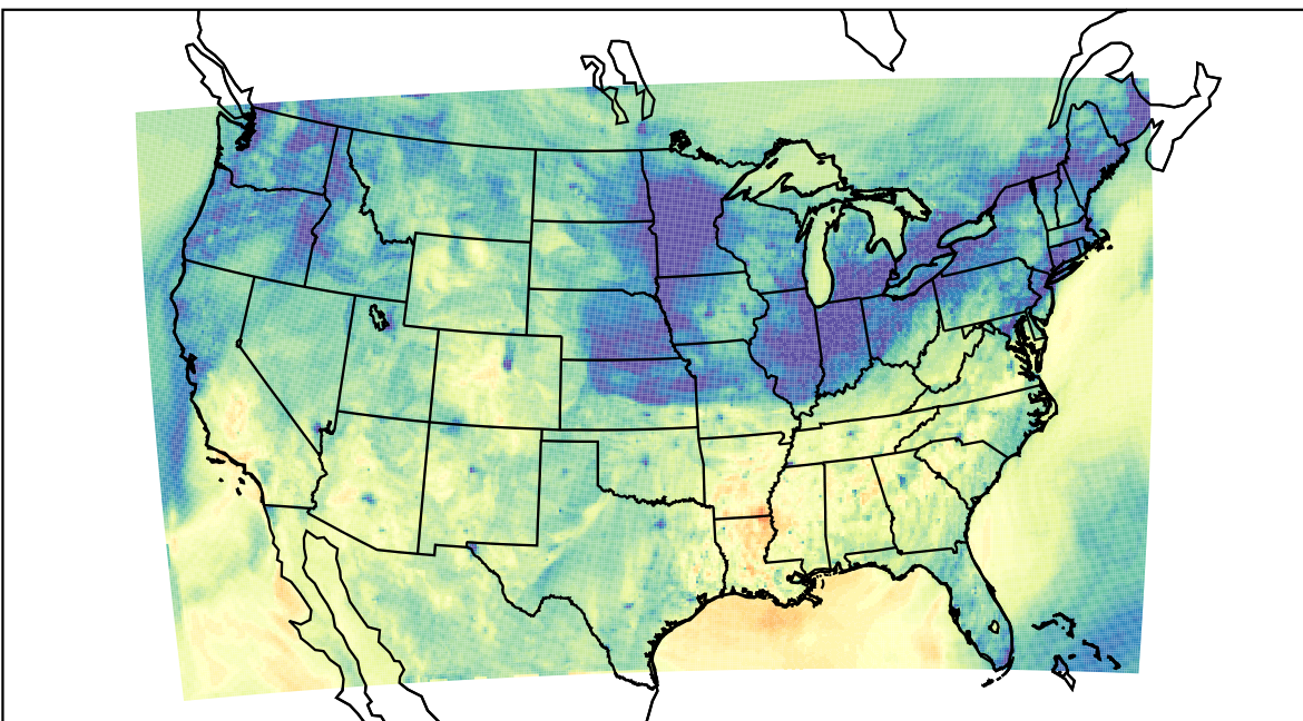
WRF (2023-11-05_00:00:00)
