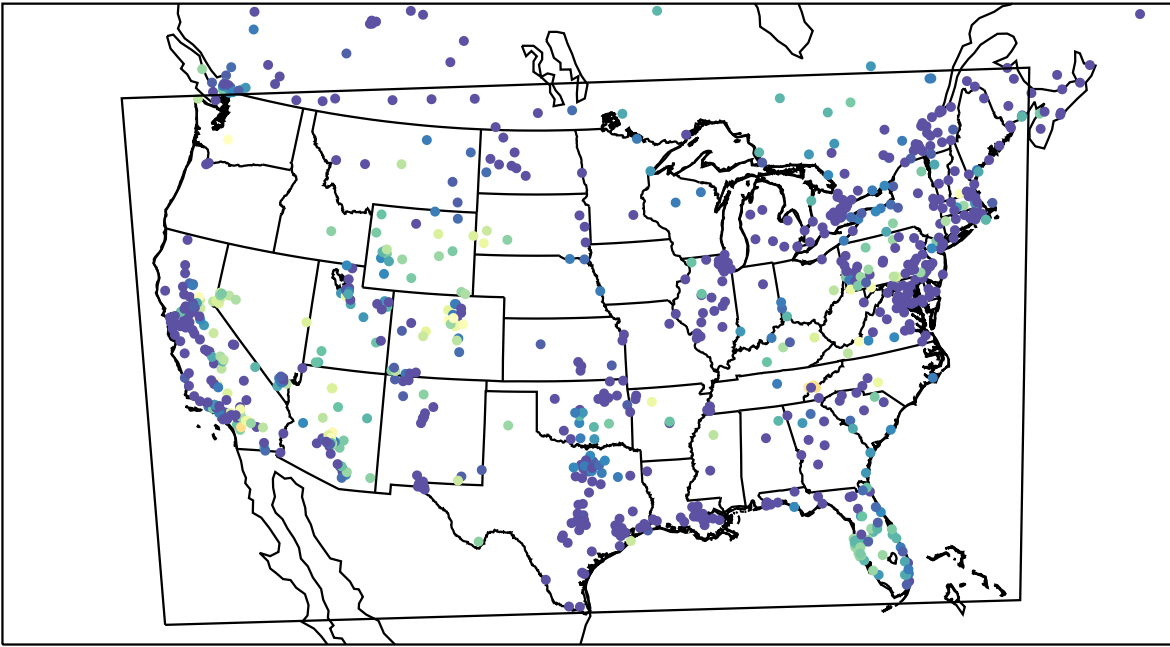
AirNOW (2023-11-05_10:00:00)
