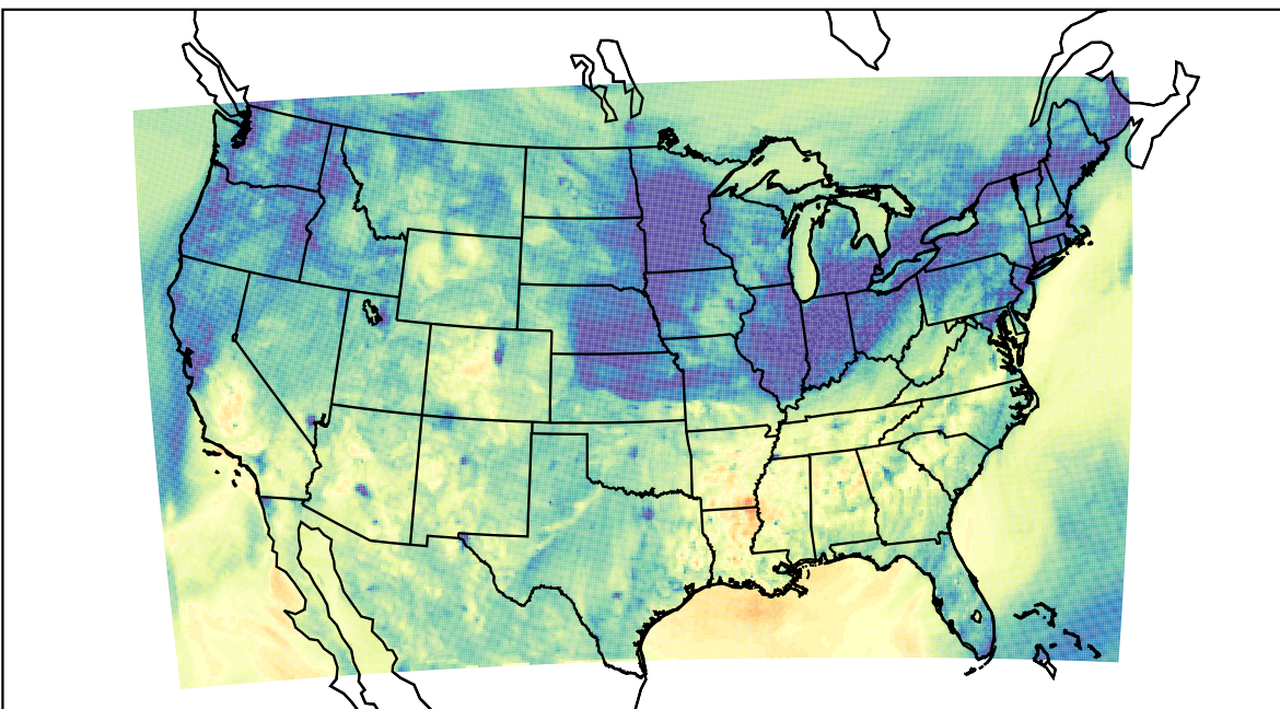
WRF (2023-11-05_01:00:00)
