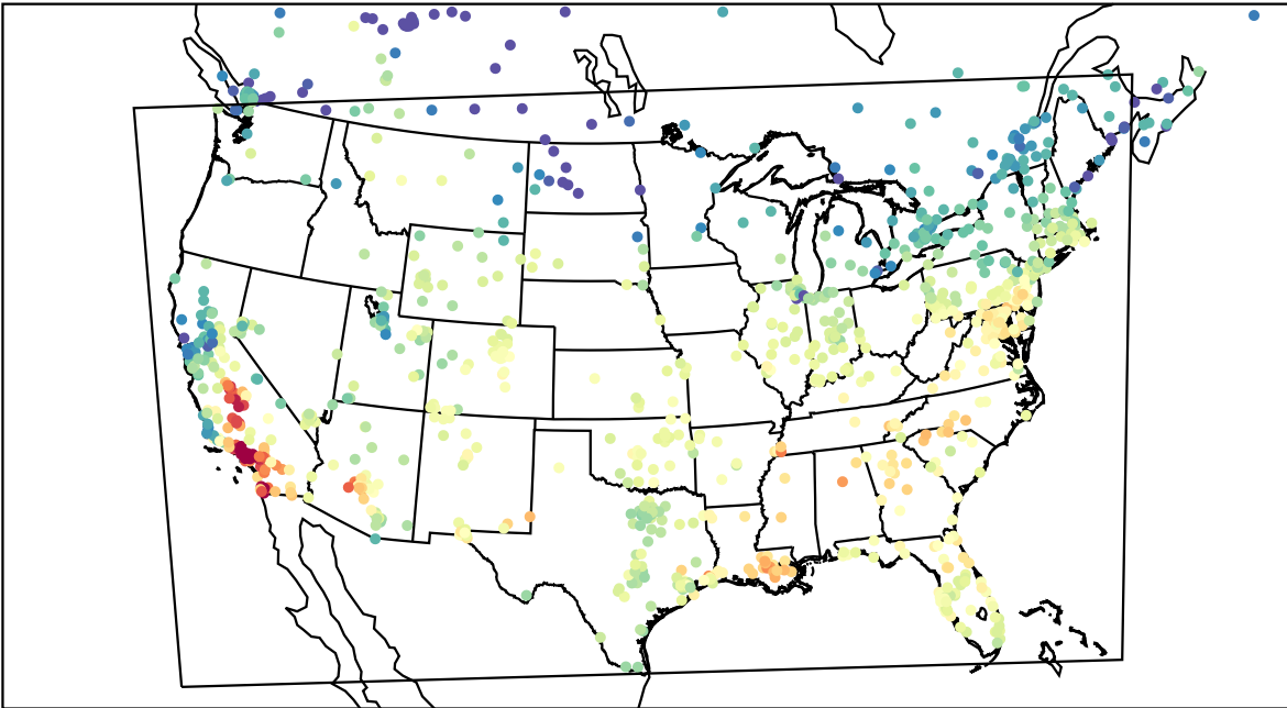
AirNOW (2023-11-05_21:00:00)
