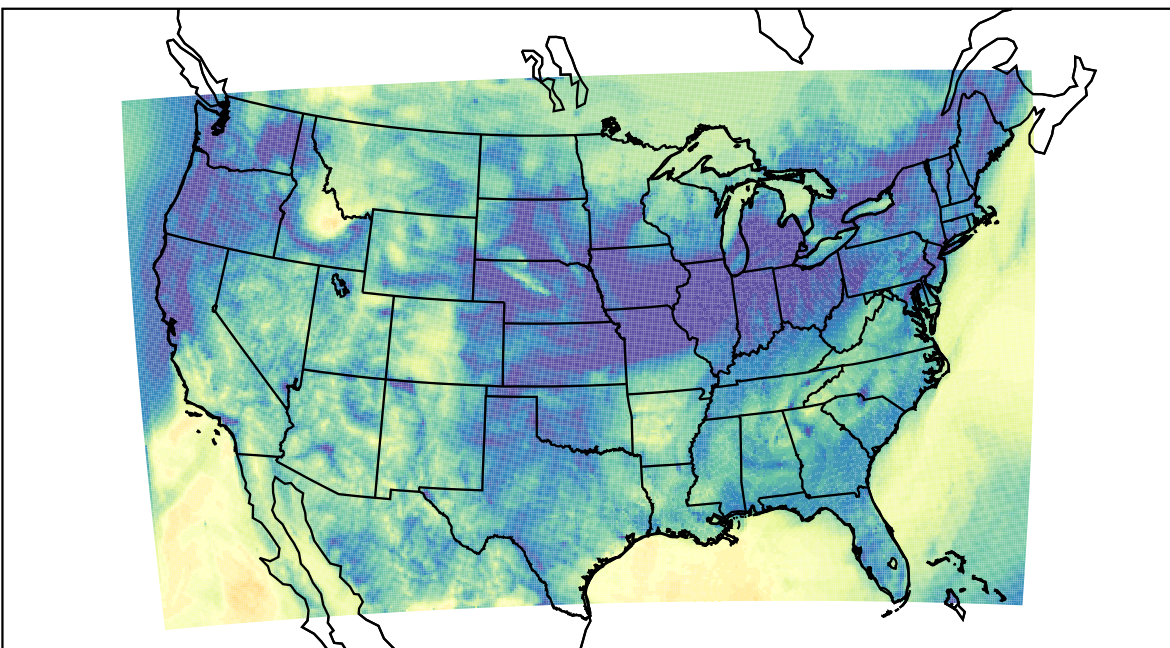
WRF (2023-11-04_11:00:00)
