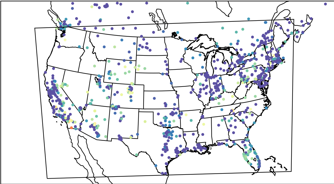
AirNOW (2023-11-05_09:00:00)
