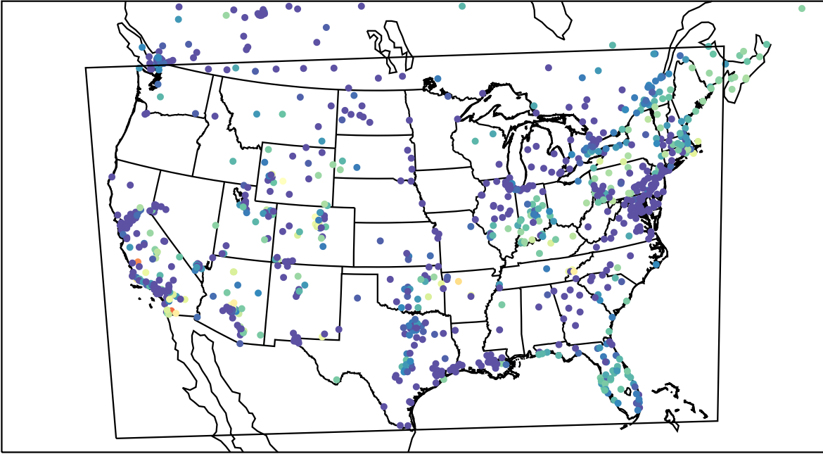
AirNOW (2023-11-04_12:00:00)
