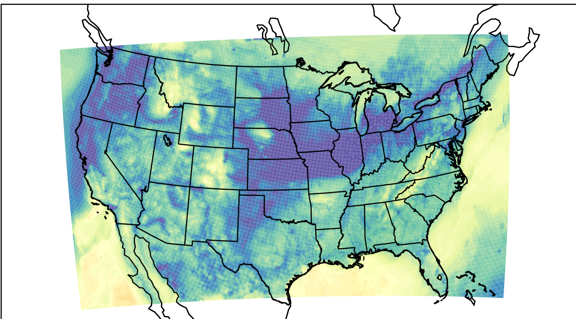
WRF (2023-11-04_15:00:00)
