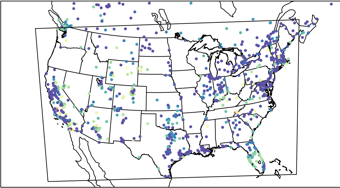
AirNOW (2023-11-05_06:00:00)
