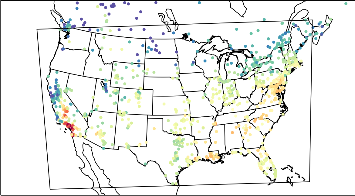
AirNOW (2023-11-05_19:00:00)
