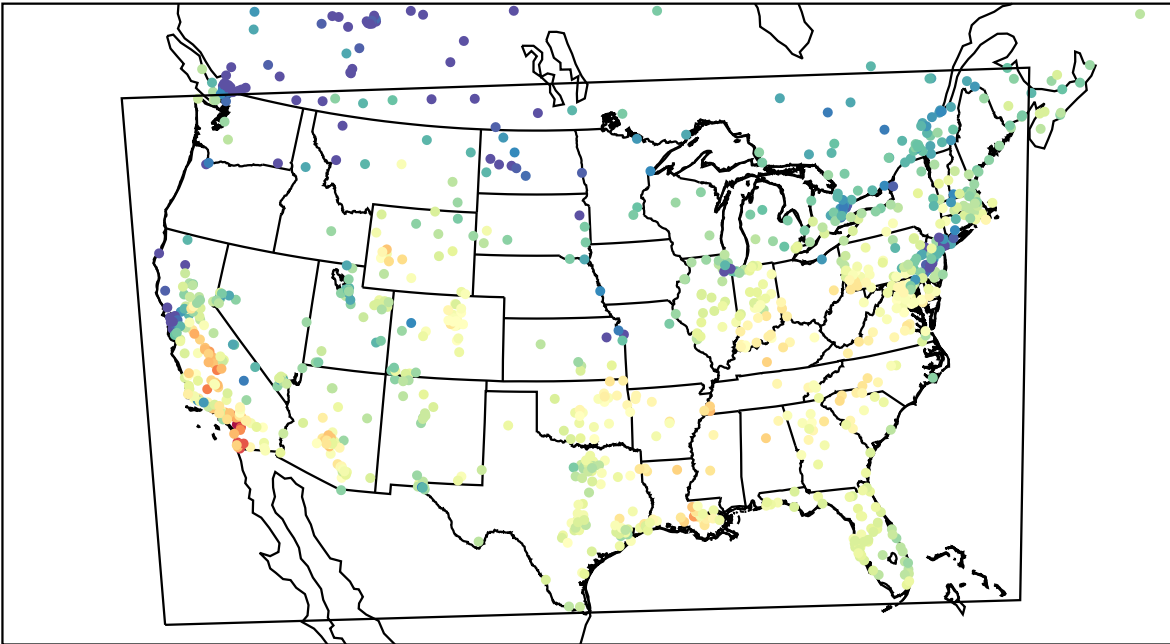
AirNOW (2023-11-04_19:00:00)
