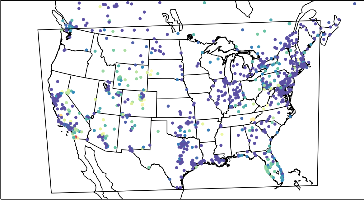
AirNOW (2023-11-05_12:00:00)
