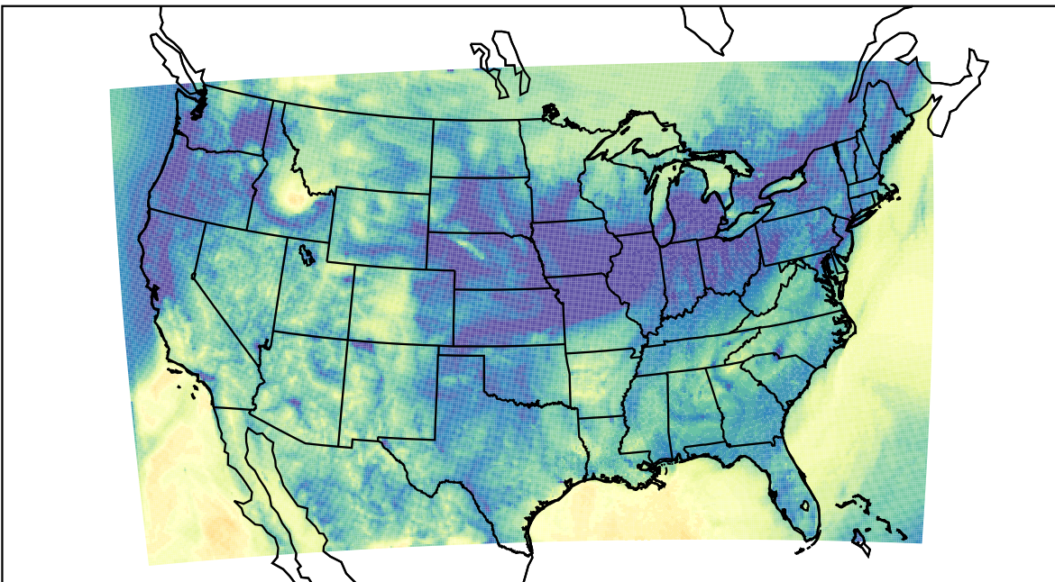
WRF (2023-11-04_10:00:00)
