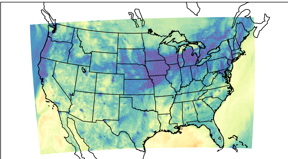
WRF (2023-11-04_03:00:00)
