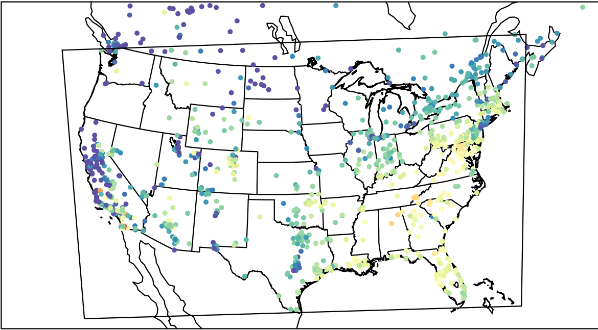
AirNOW (2023-11-05_16:00:00)
