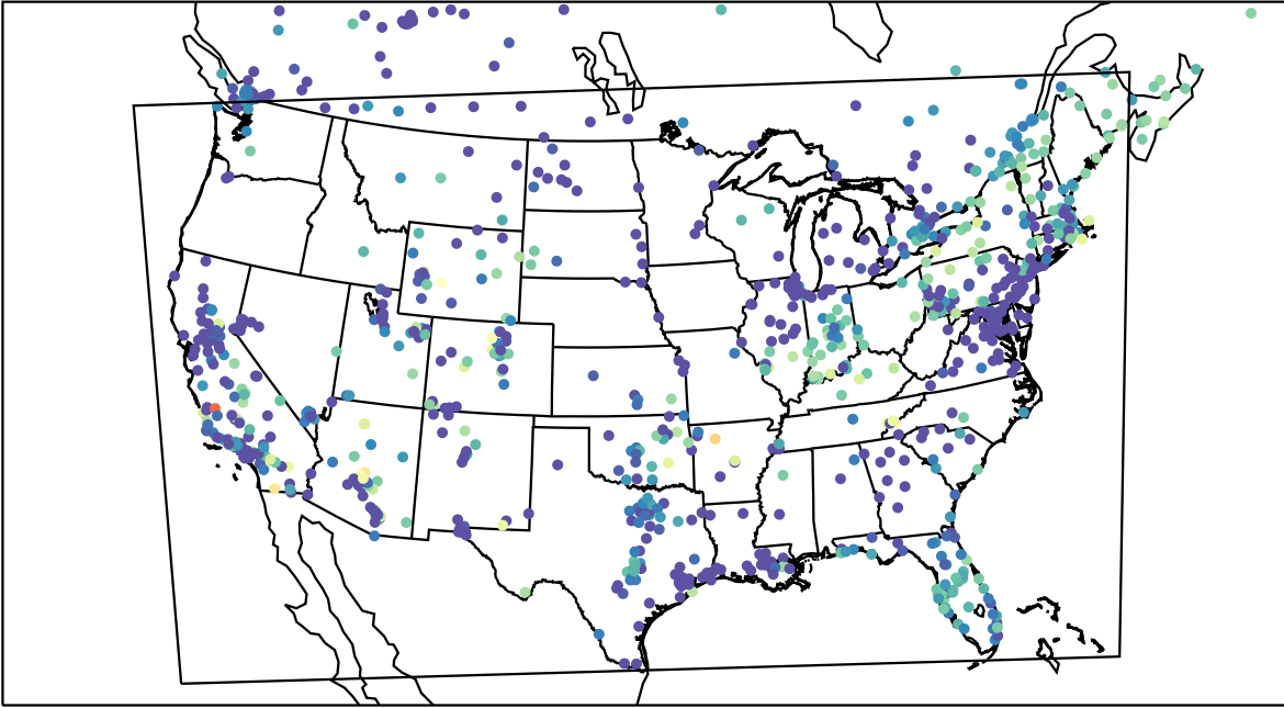
AirNOW (2023-11-04_11:00:00)
