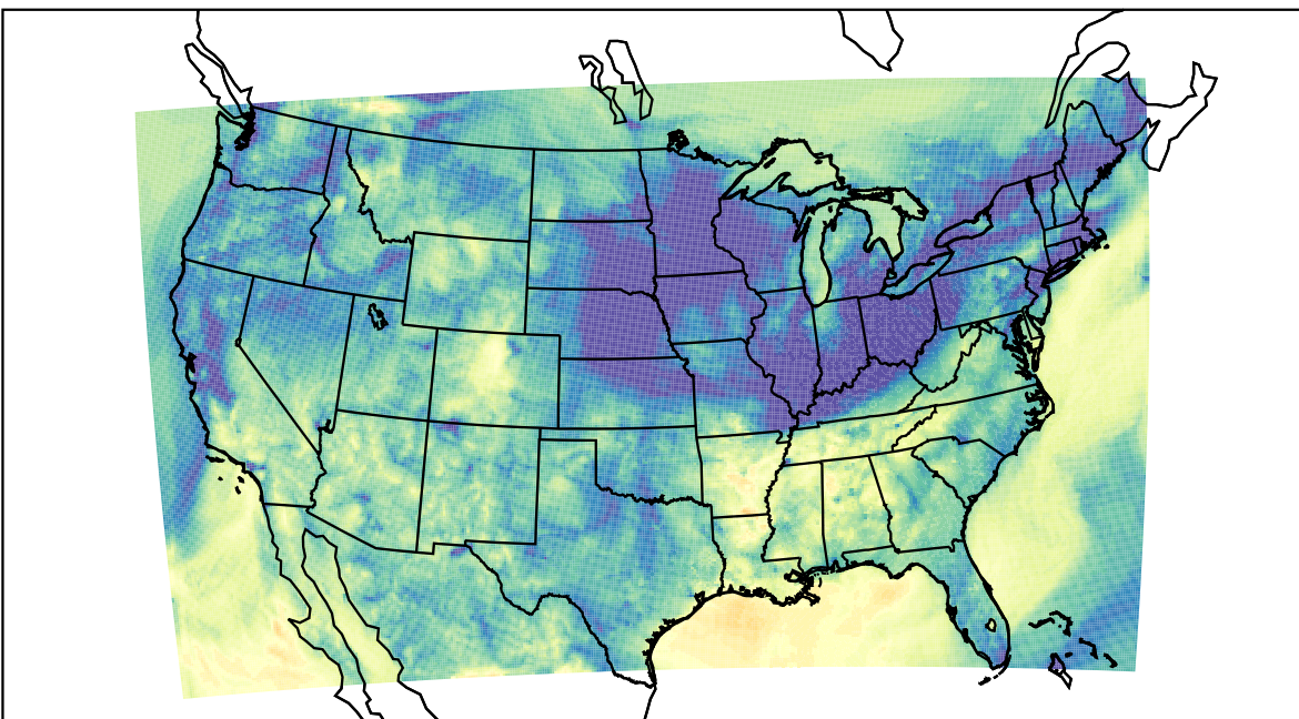
WRF (2023-11-05_08:00:00)
