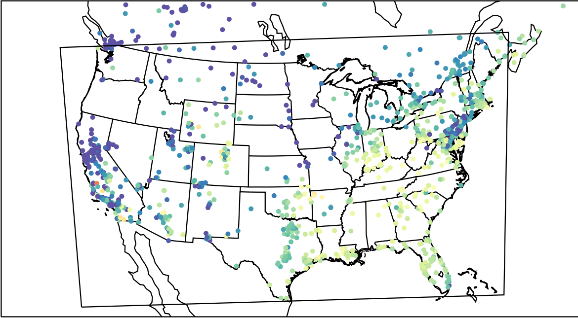
AirNOW (2023-11-04_16:00:00)
