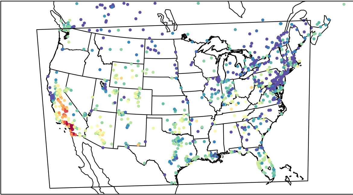
AirNOW (2023-11-05_00:00:00)
