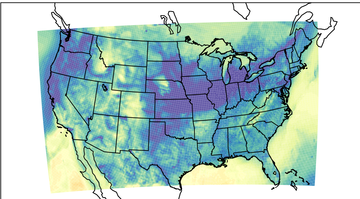
WRF (2023-11-04_14:00:00)
