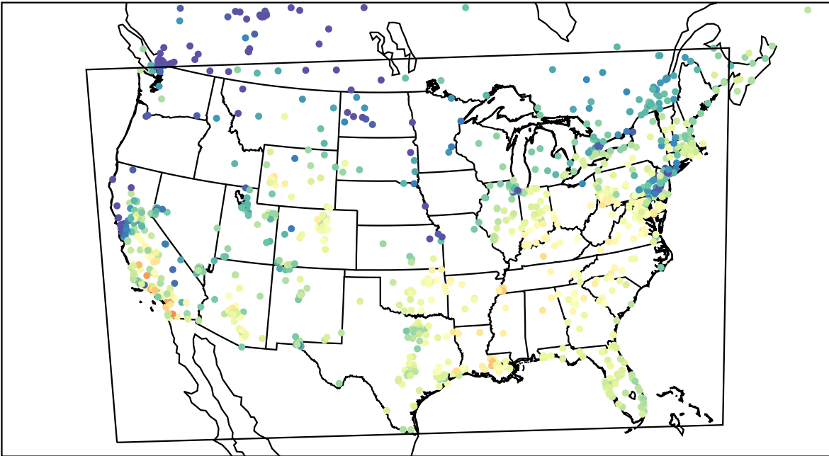
AirNOW (2023-11-04_18:00:00)
