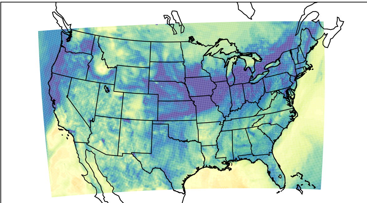
WRF (2023-11-04_08:00:00)
