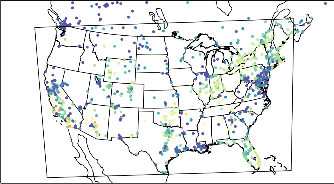
AirNOW (2023-11-04_02:00:00)
