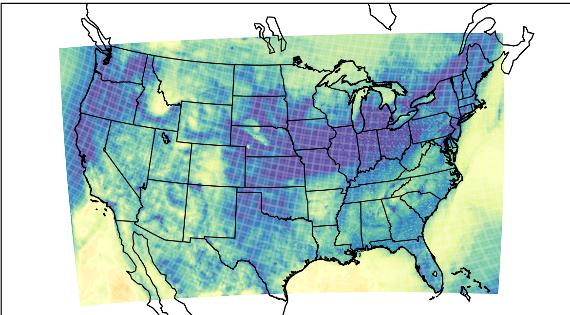
WRF (2023-11-04_12:00:00)
