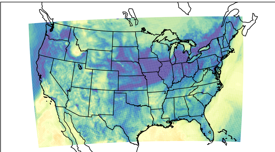
WRF (2023-11-04_09:00:00)
