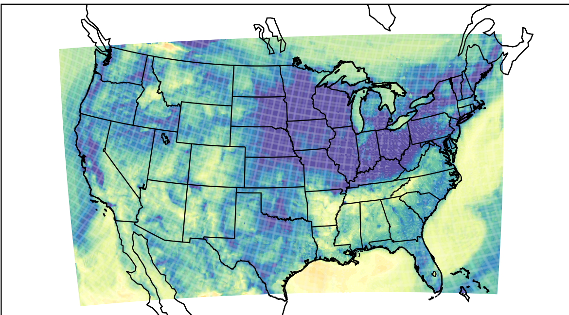
WRF (2023-11-05_13:00:00)
