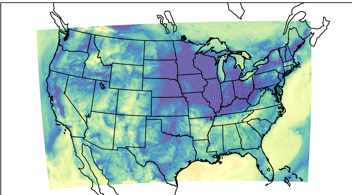
WRF (2023-11-05_14:00:00)
