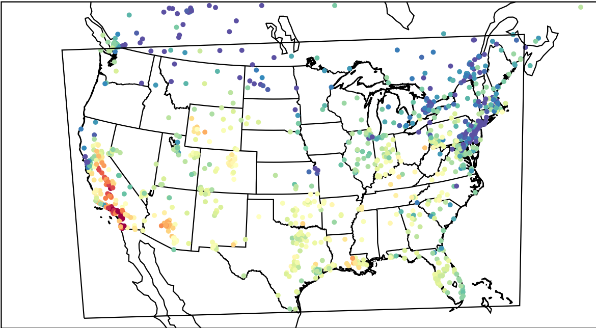
AirNOW (2023-11-04_22:00:00)
