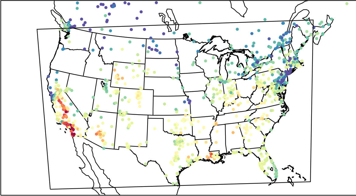
AirNOW (2023-11-04_21:00:00)
