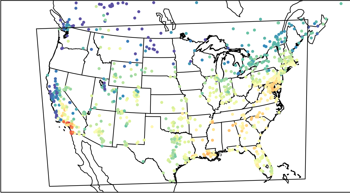
AirNOW (2023-11-05_18:00:00)
