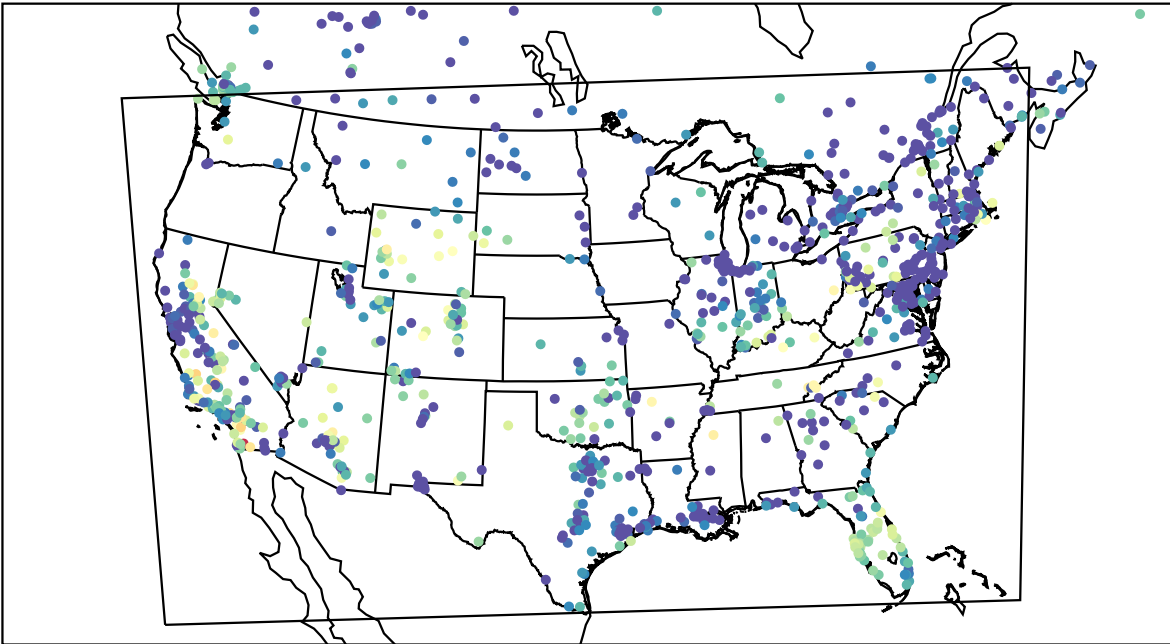
AirNOW (2023-11-05_03:00:00)
