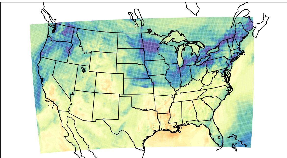
WRF (2023-11-04_22:00:00)
