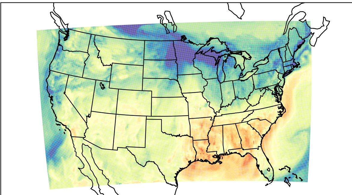
WRF (2023-11-05_21:00:00)
