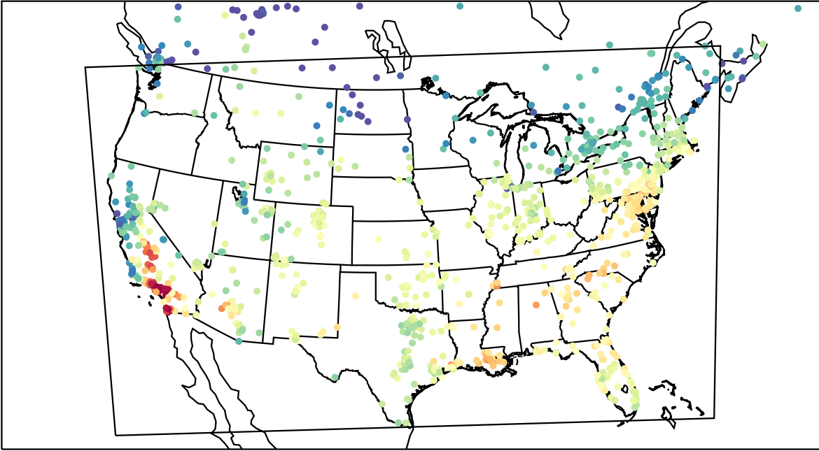
AirNOW (2023-11-05_20:00:00)
