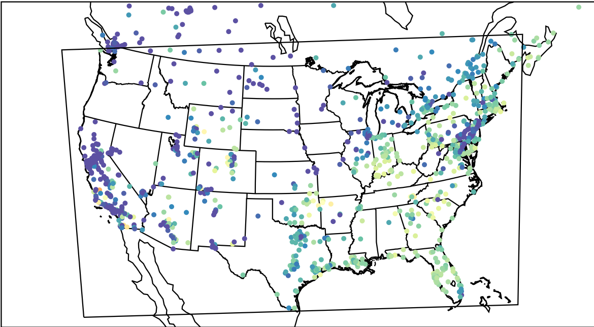
AirNOW (2023-11-04_15:00:00)
