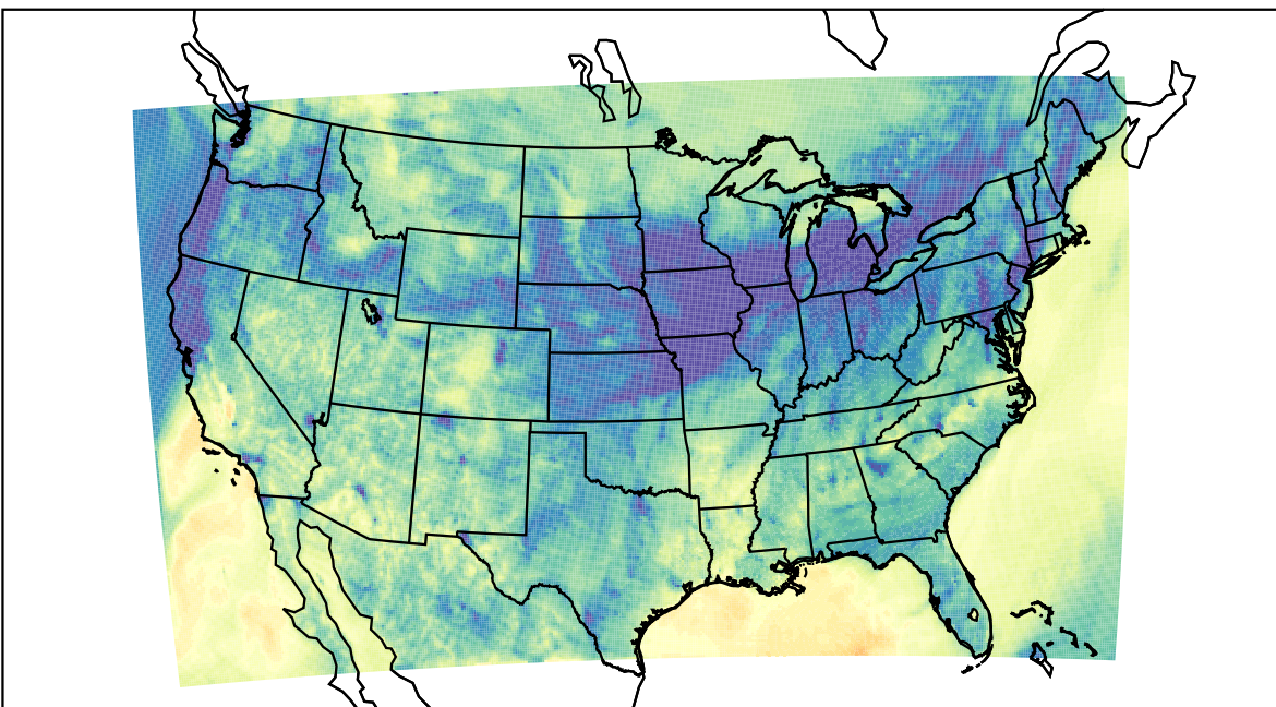
WRF (2023-11-04_04:00:00)
