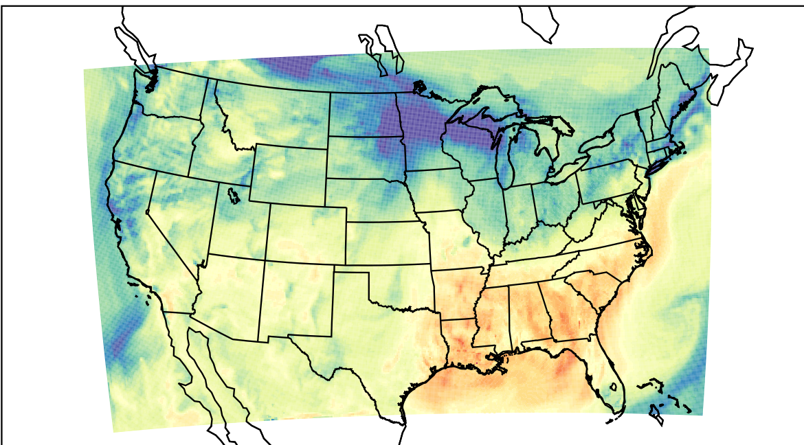
WRF (2023-11-05_20:00:00)
