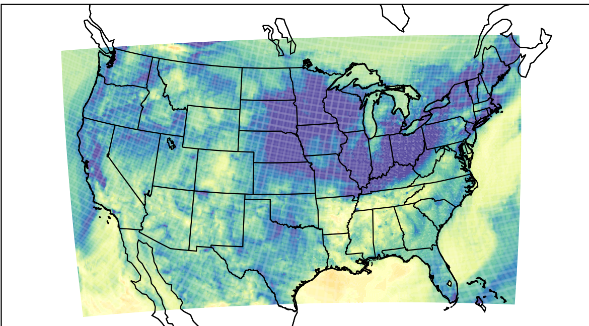
WRF (2023-11-05_10:00:00)
