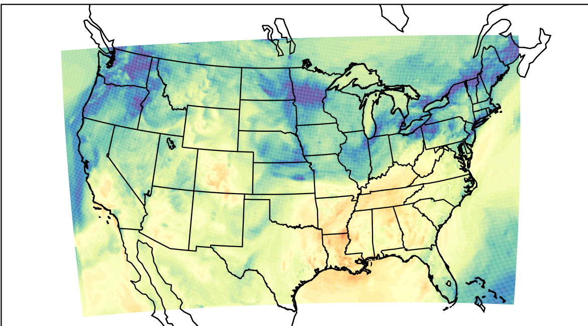
WRF (2023-11-04_21:00:00)
