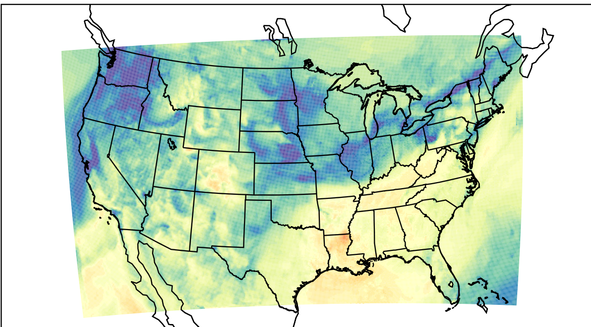
WRF (2023-11-04_18:00:00)
