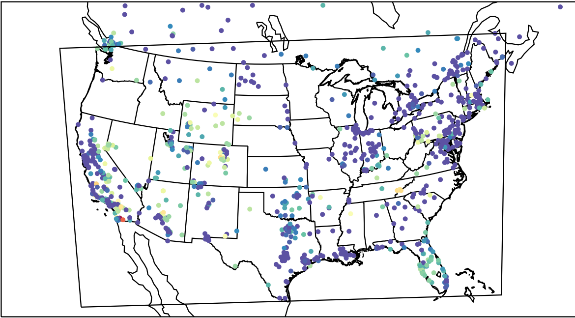
AirNOW (2023-11-05_07:00:00)
