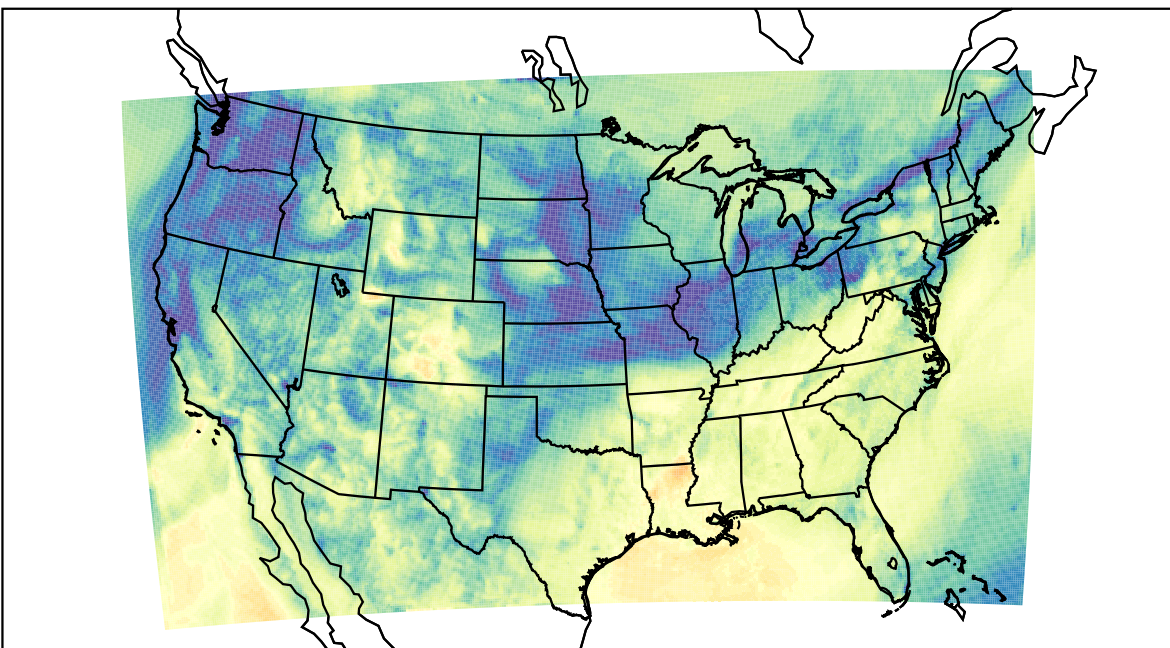
WRF (2023-11-04_17:00:00)
