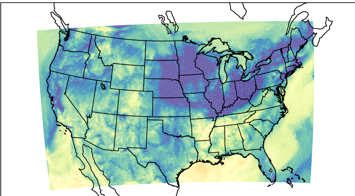
WRF (2023-11-05_09:00:00)
