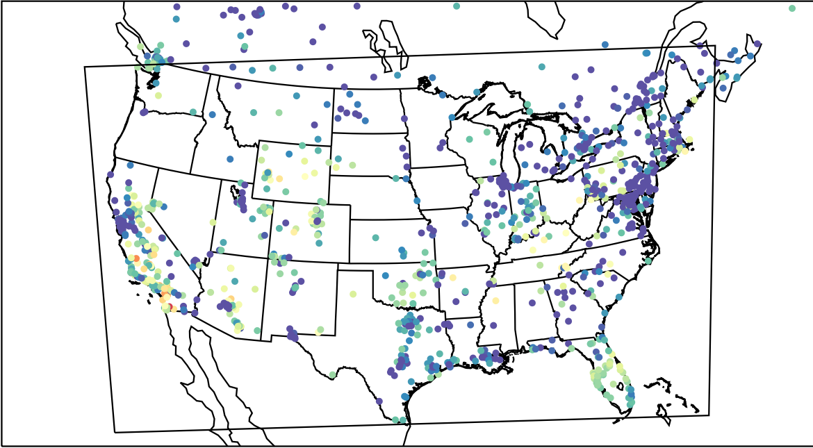
AirNOW (2023-11-05_02:00:00)
