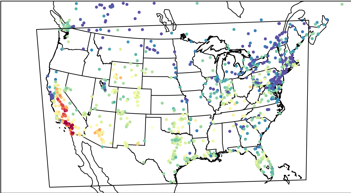
AirNOW (2023-11-04_23:00:00)
