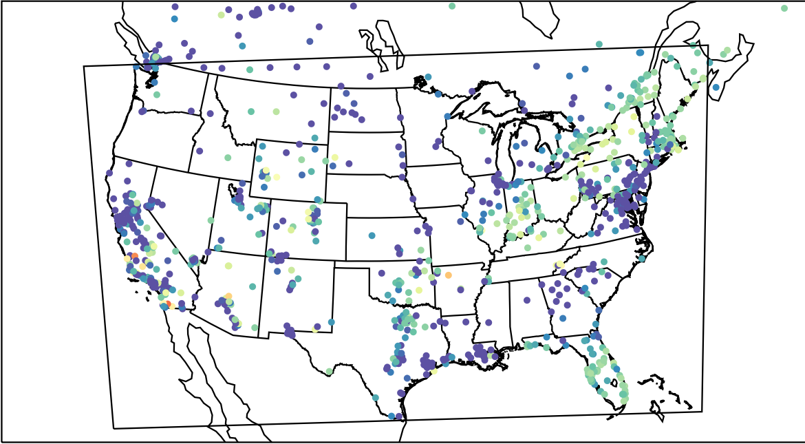
AirNOW (2023-11-04_08:00:00)
