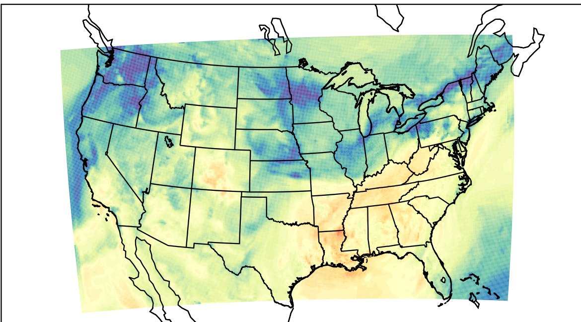
WRF (2023-11-04_20:00:00)
