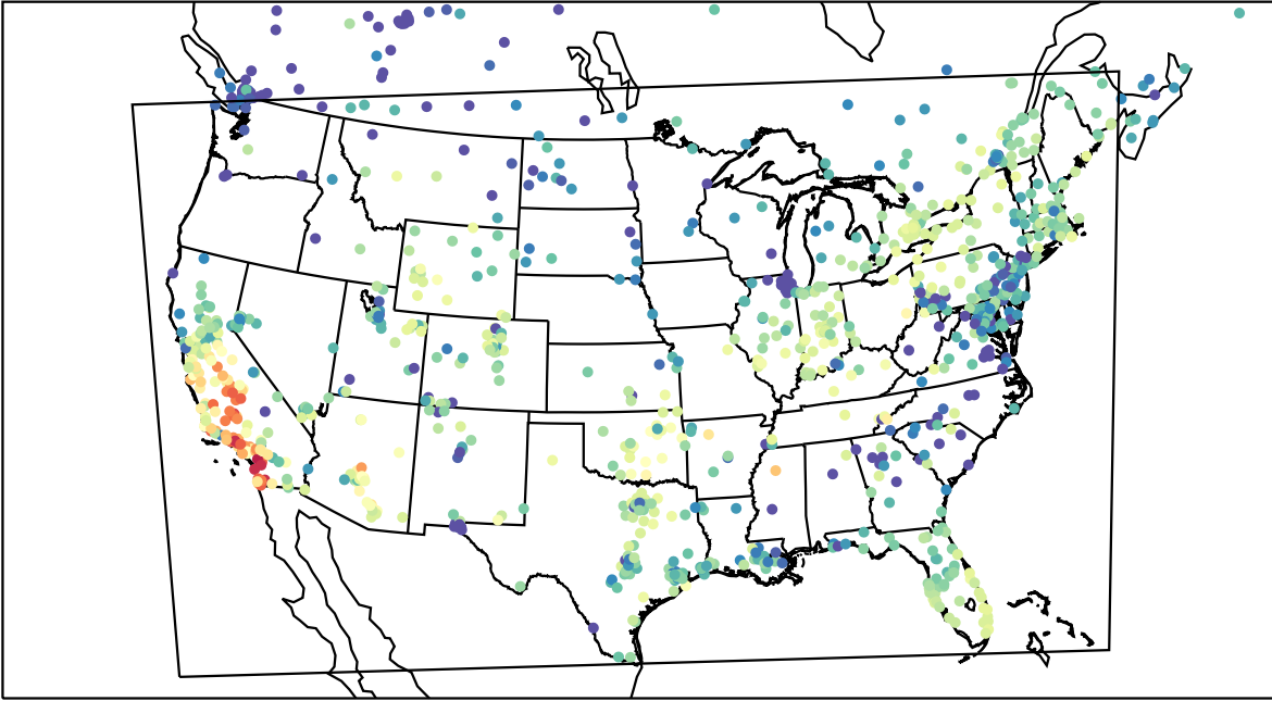
AirNOW (2023-11-04_00:00:00)
