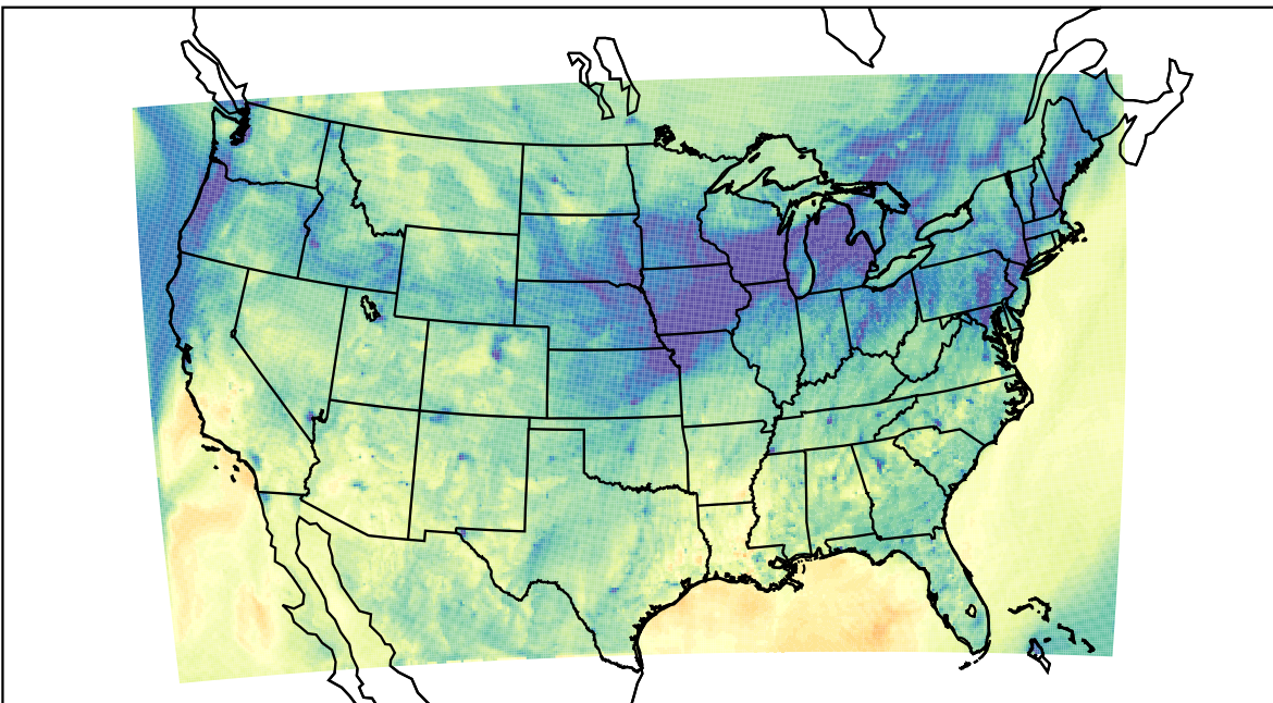
WRF (2023-11-04_00:00:00)
