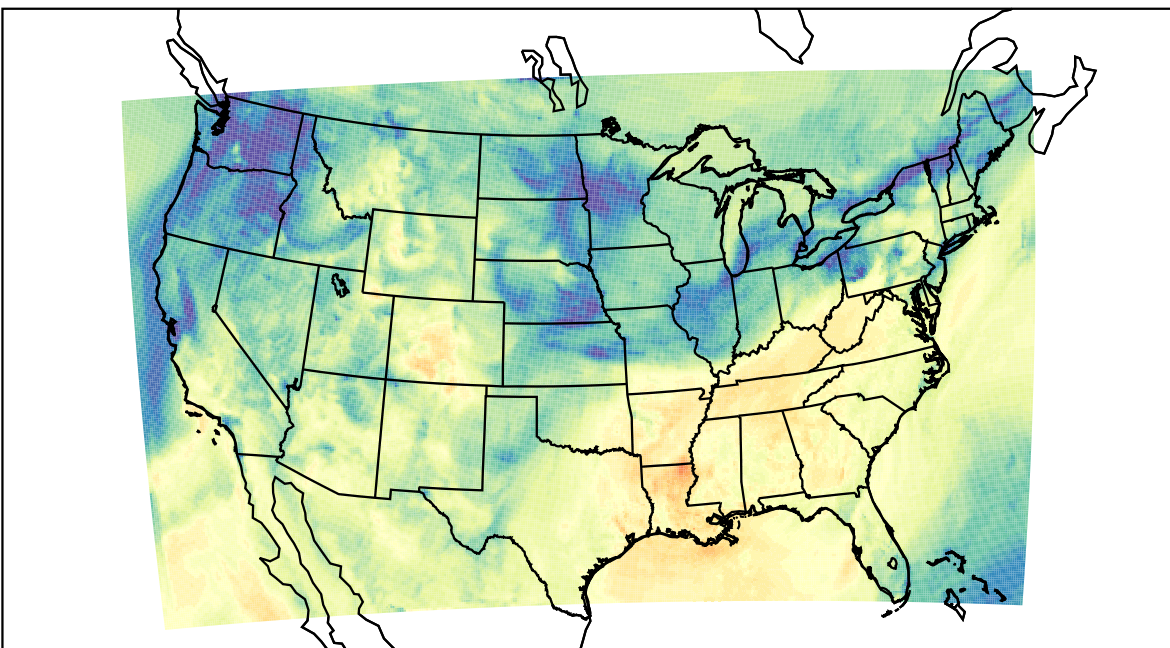
WRF (2023-11-04_19:00:00)
