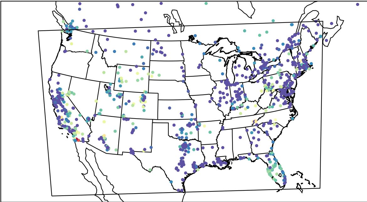
AirNOW (2023-11-05_08:00:00)
