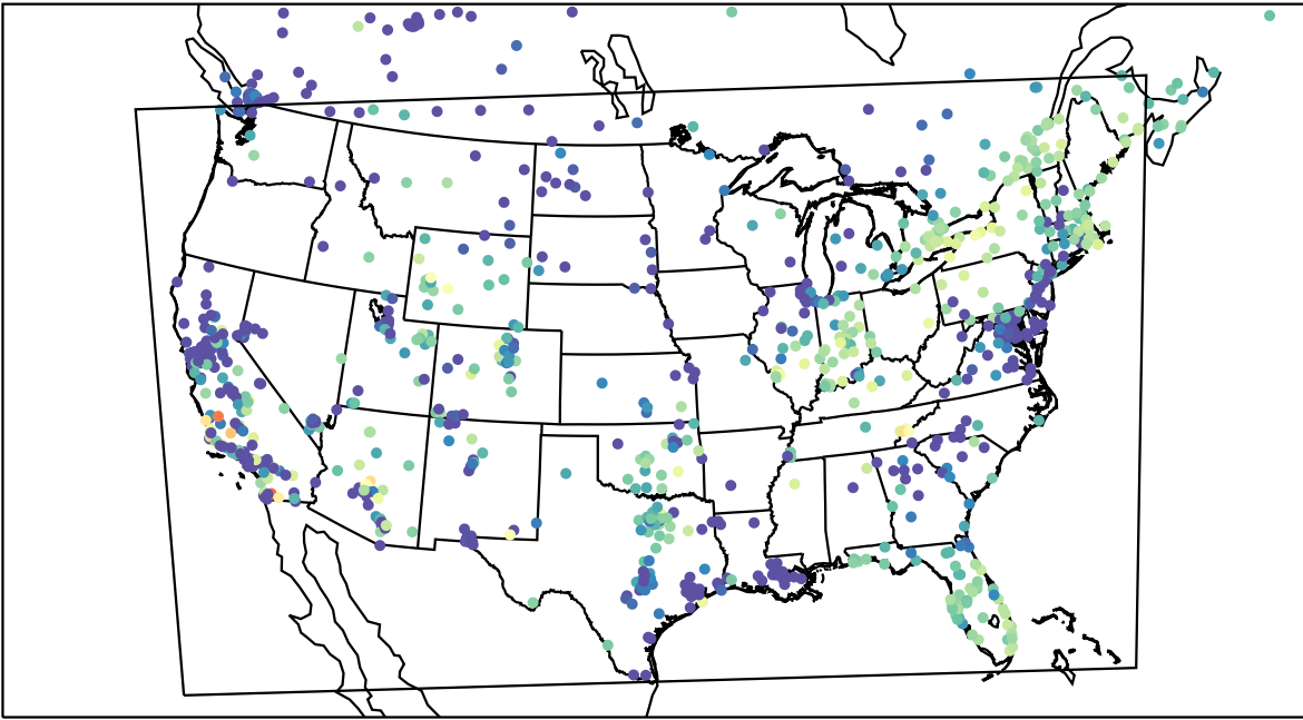
AirNOW (2023-11-04_06:00:00)
