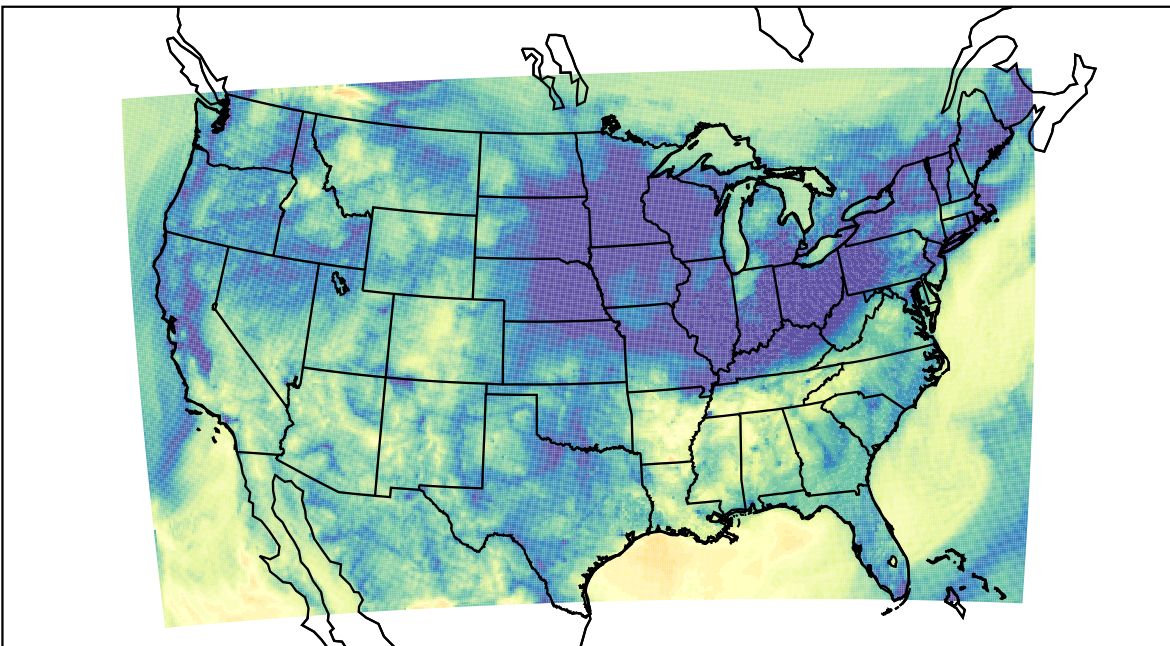
WRF (2023-11-05_11:00:00)
