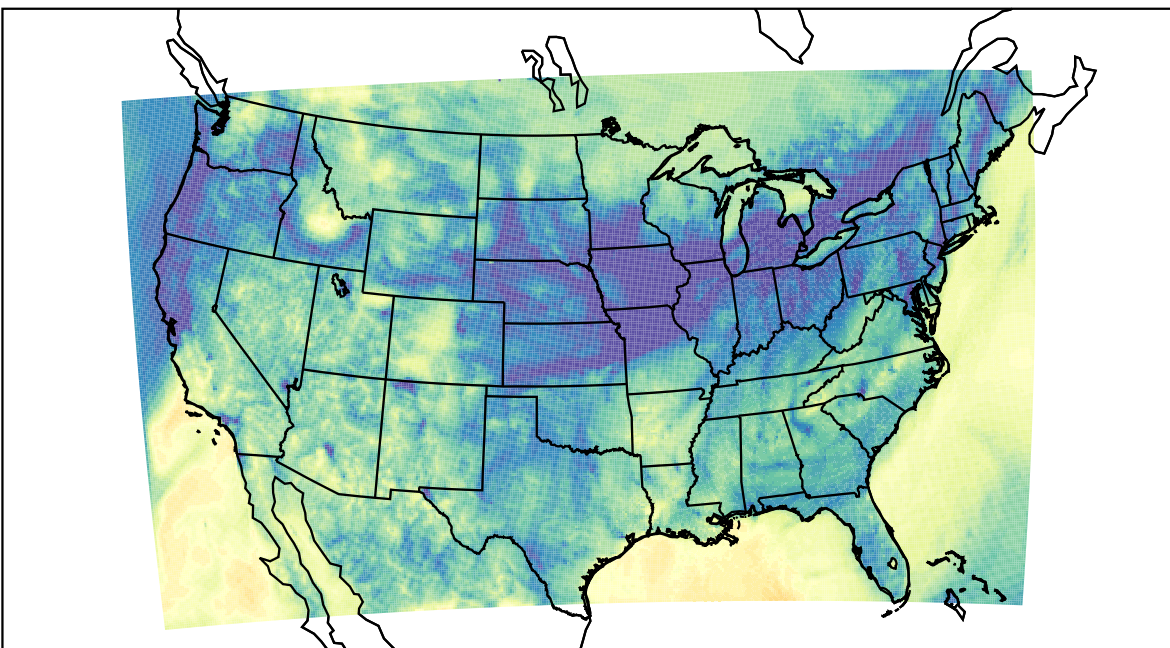
WRF (2023-11-04_07:00:00)
