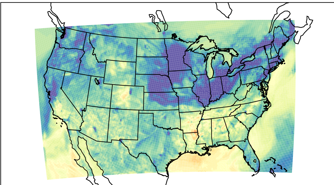
WRF (2023-11-05_03:00:00)
