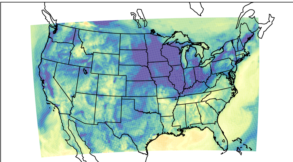
WRF (2023-11-05_15:00:00)
