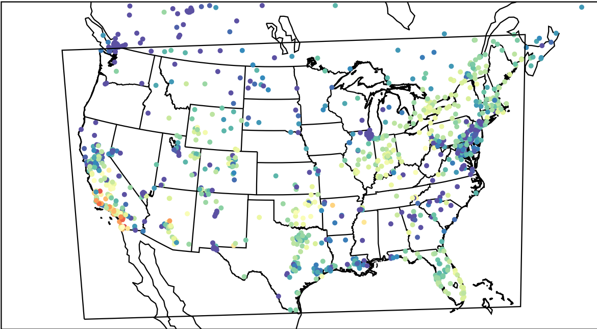
AirNOW (2023-11-04_01:00:00)
