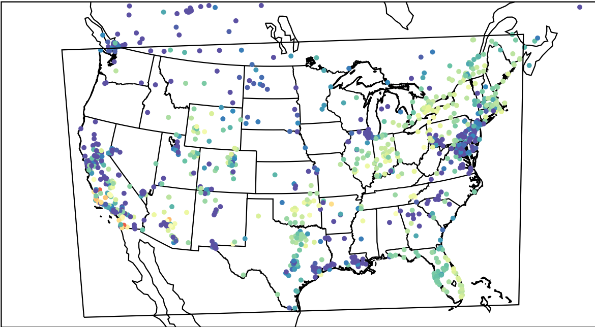
AirNOW (2023-11-04_03:00:00)
