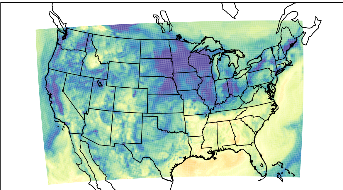
WRF (2023-11-05_16:00:00)
