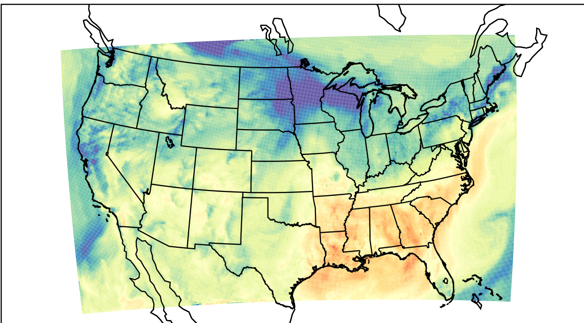
WRF (2023-11-05_19:00:00)
