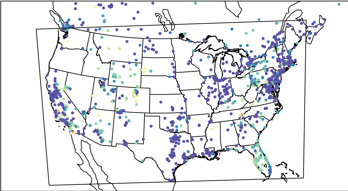
AirNOW (2023-11-05_13:00:00)
