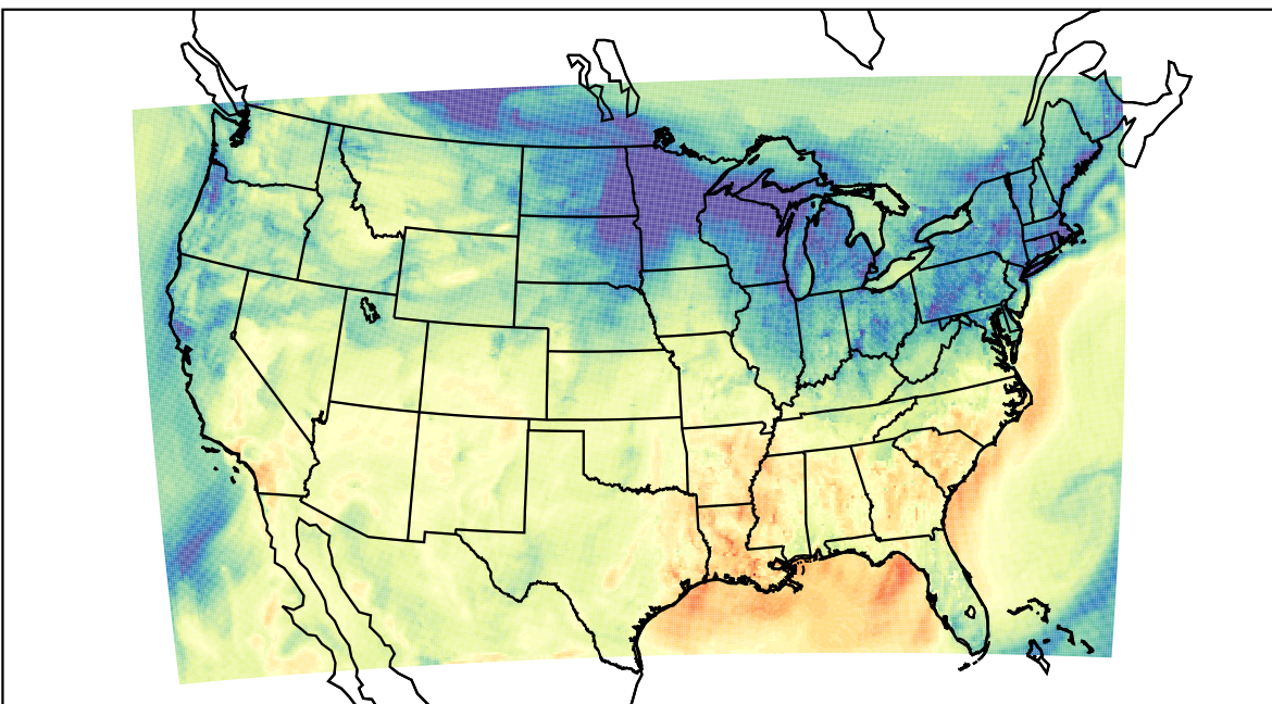
WRF (2023-11-05_22:00:00)
