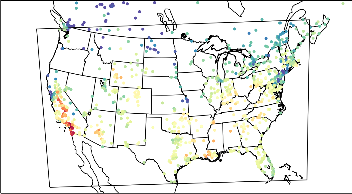
AirNOW (2023-11-04_20:00:00)
