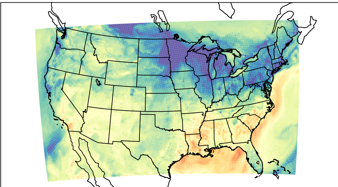
WRF (2023-11-05_23:00:00)
