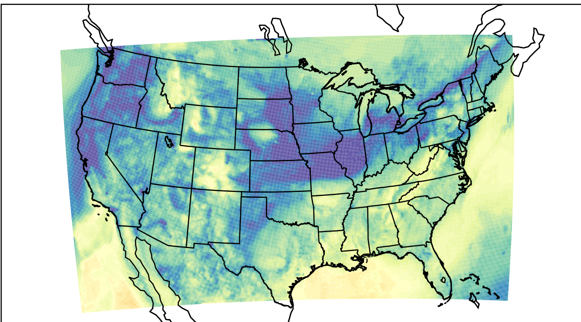
WRF (2023-11-04_16:00:00)
