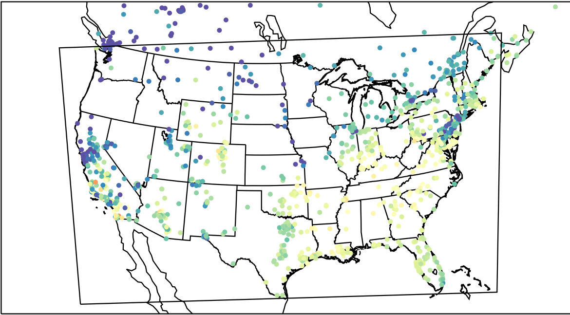
AirNOW (2023-11-04_17:00:00)
