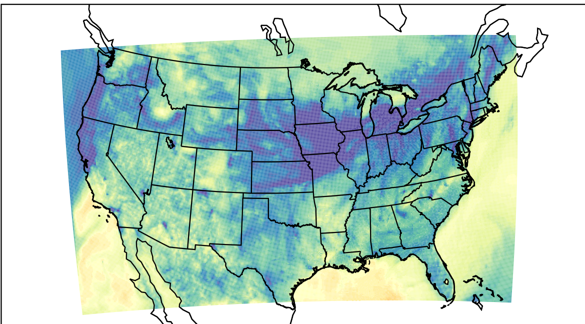
WRF (2023-11-04_06:00:00)
