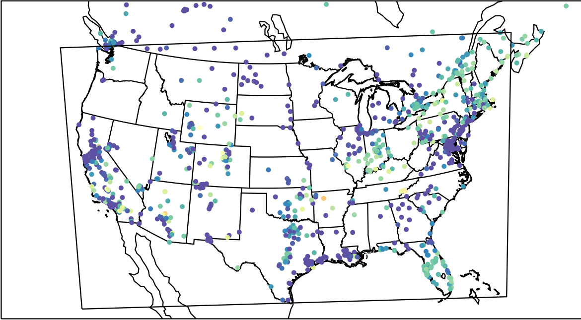
AirNOW (2023-11-04_10:00:00)
