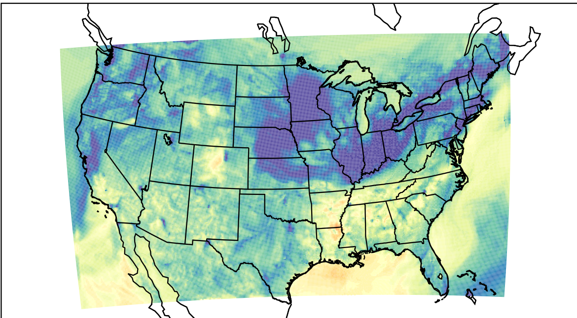
WRF (2023-11-05_04:00:00)
