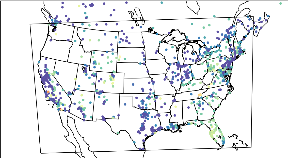
AirNOW (2023-11-05_14:00:00)
