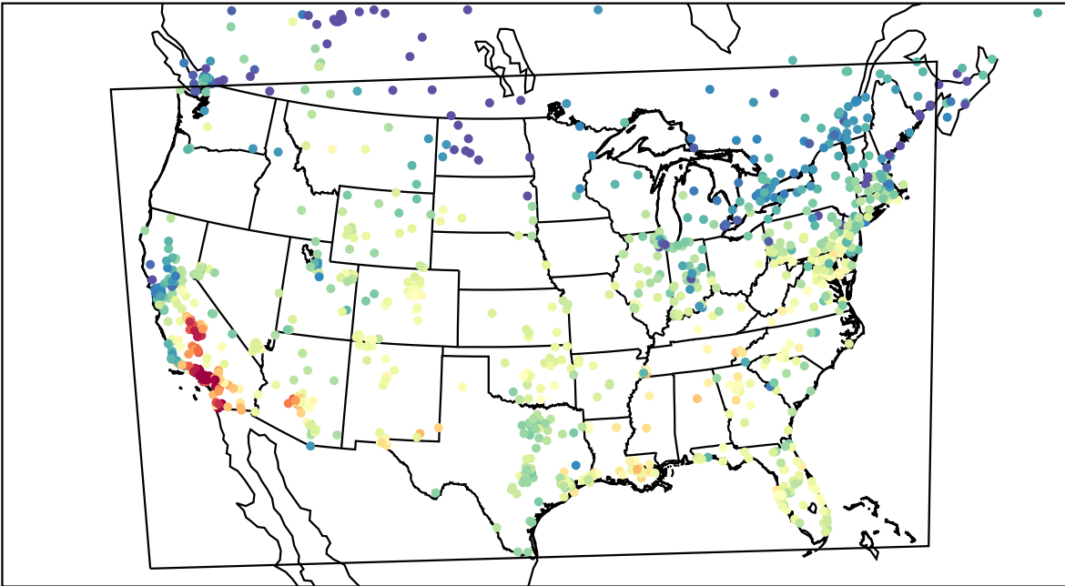
AirNOW (2023-11-05_22:00:00)
