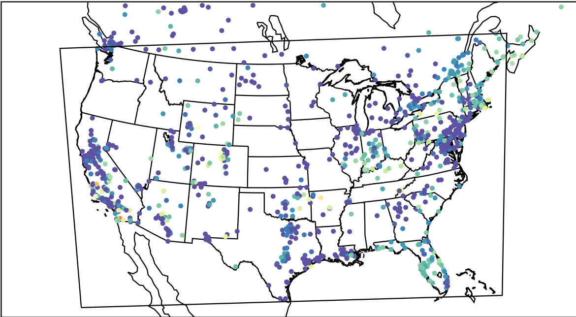
AirNOW (2023-11-04_13:00:00)
