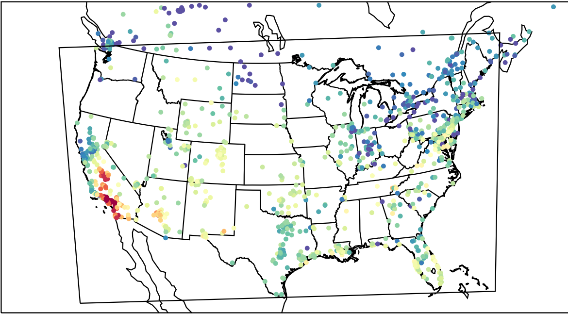
AirNOW (2023-11-05_23:00:00)
