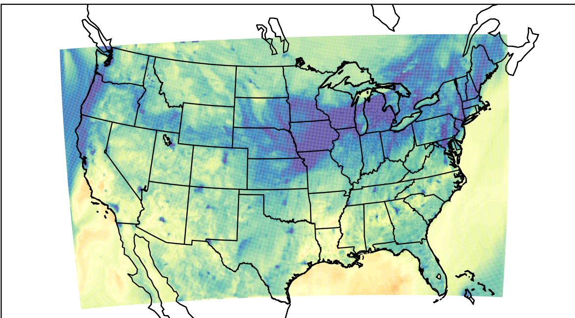
WRF (2023-11-04_01:00:00)
