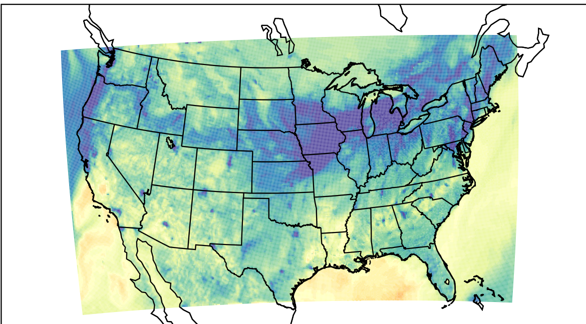
WRF (2023-11-04_02:00:00)
