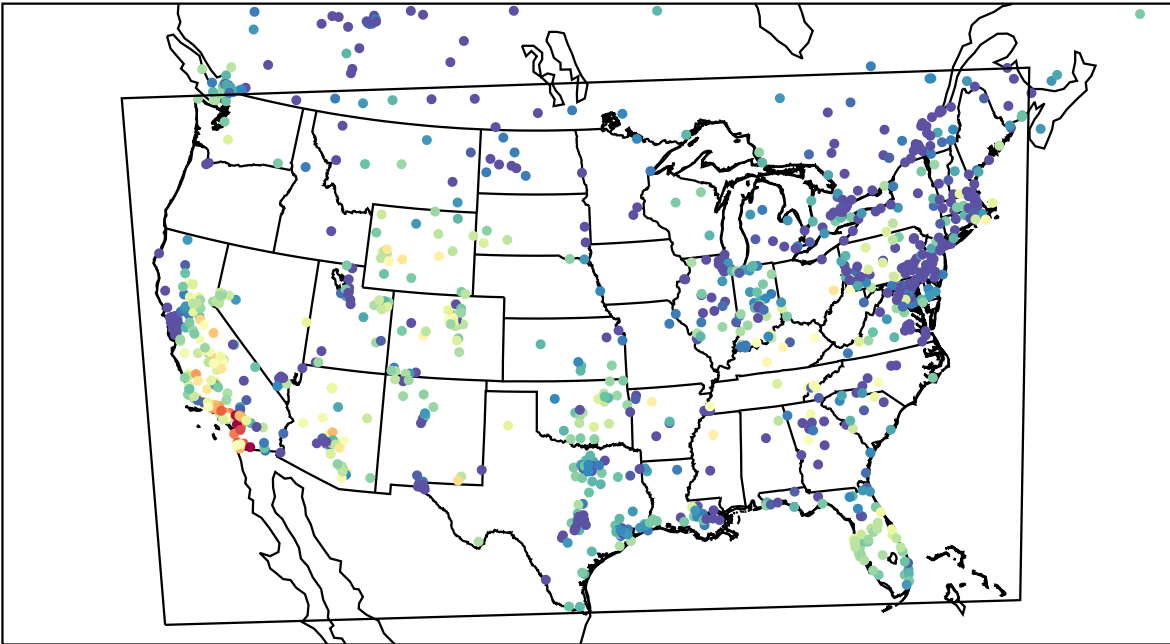
AirNOW (2023-11-05_01:00:00)
