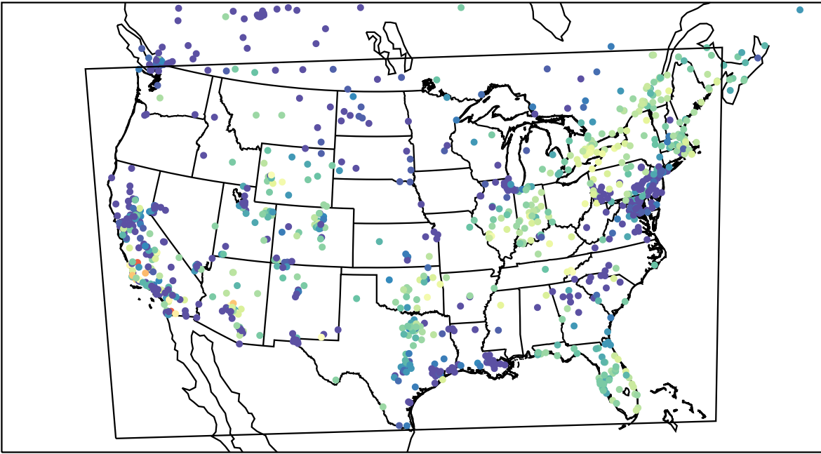
AirNOW (2023-11-04_05:00:00)
