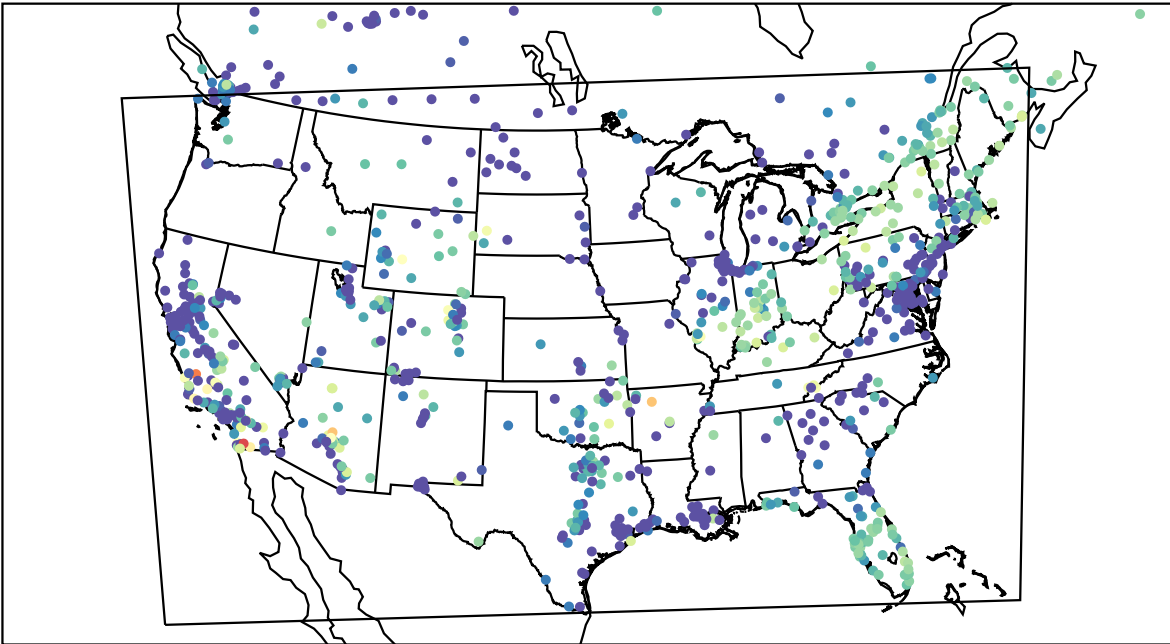
AirNOW (2023-11-04_09:00:00)
