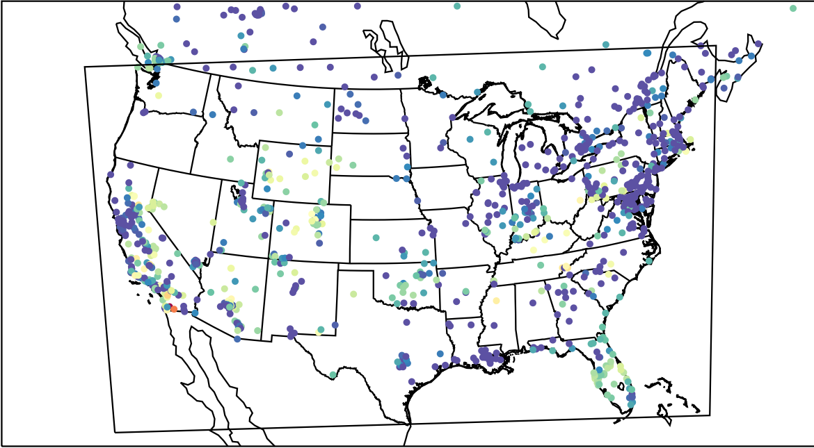
AirNOW (2023-11-05_04:00:00)
