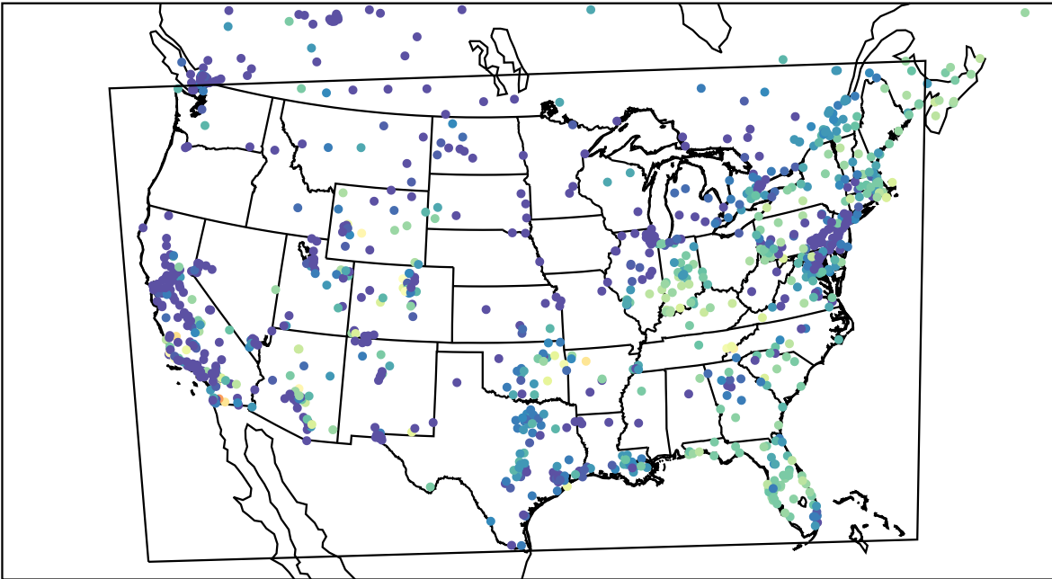
AirNOW (2023-11-04_14:00:00)
