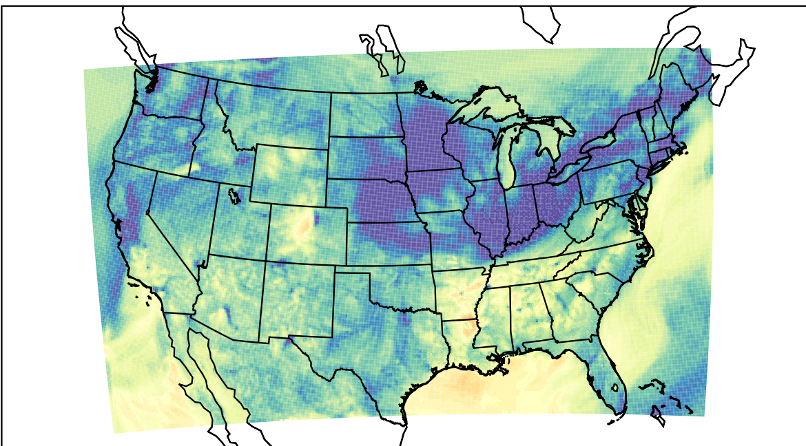
WRF (2023-11-05_05:00:00)
