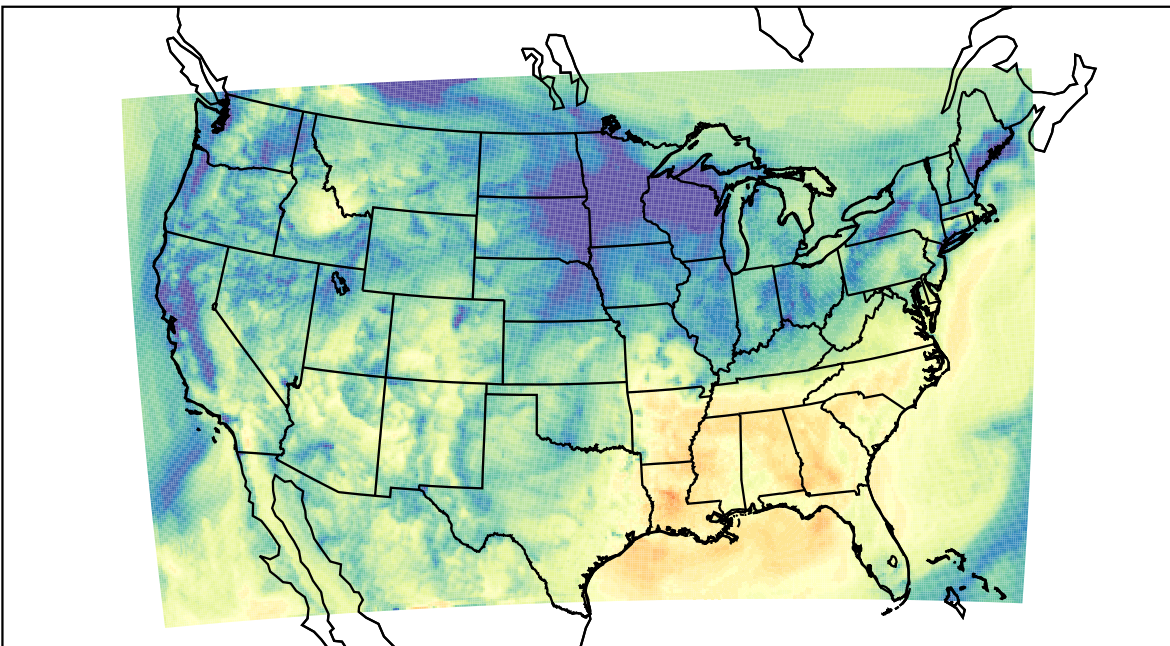
WRF (2023-11-05_17:00:00)
