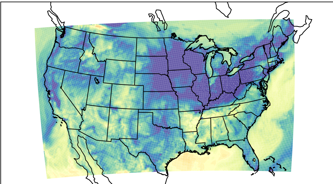
WRF (2023-11-05_12:00:00)
