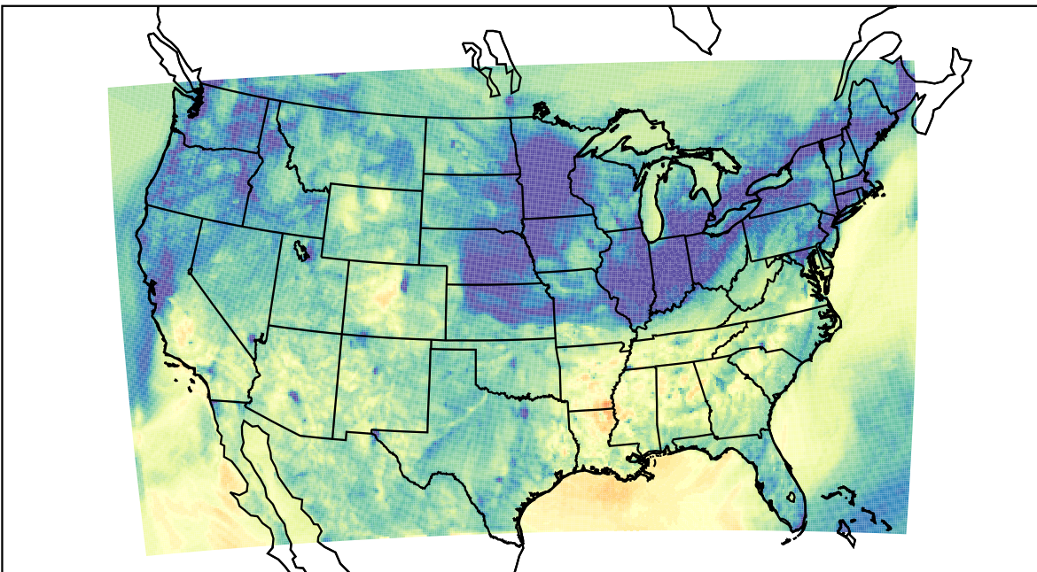
WRF (2023-11-05_02:00:00)
