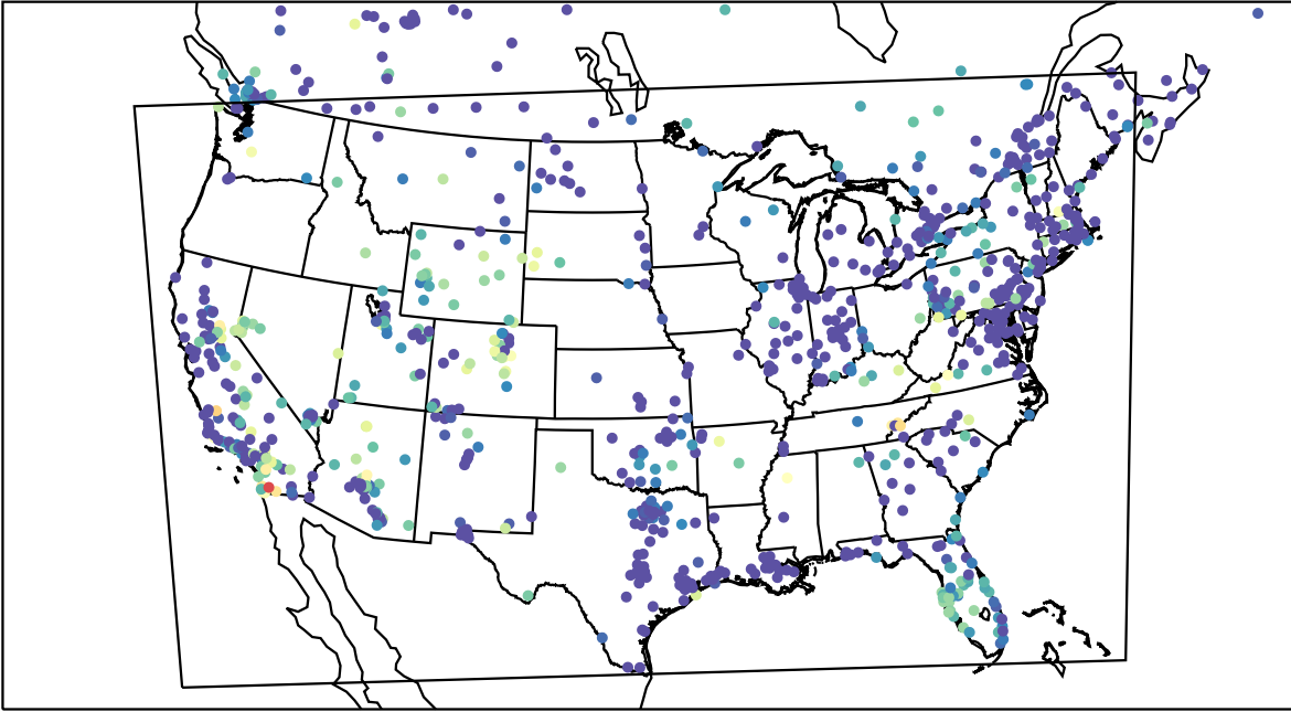
AirNOW (2023-11-05_11:00:00)
