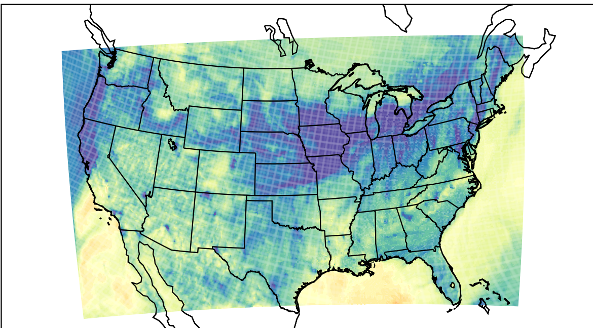
WRF (2023-11-04_05:00:00)
