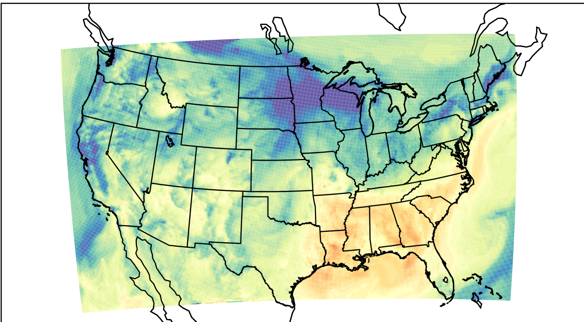
WRF (2023-11-05_18:00:00)
