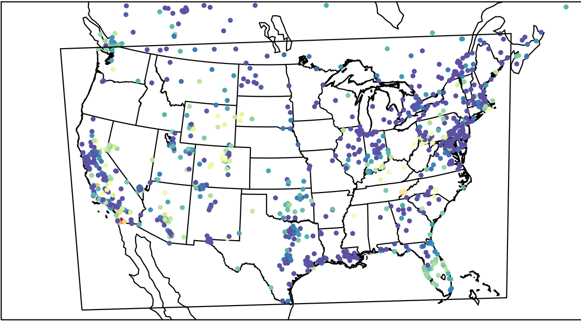
AirNOW (2023-11-05_05:00:00)
