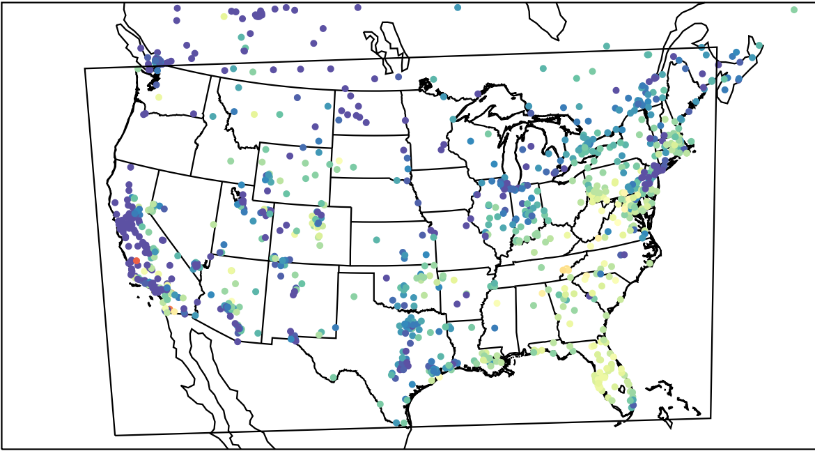
AirNOW (2023-11-05_15:00:00)
