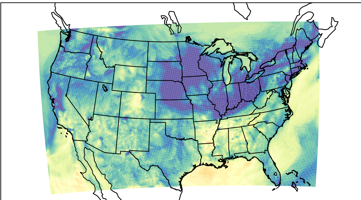
WRF (2023-11-05_07:00:00)
