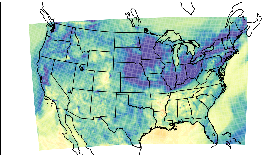
WRF (2023-11-05_06:00:00)
