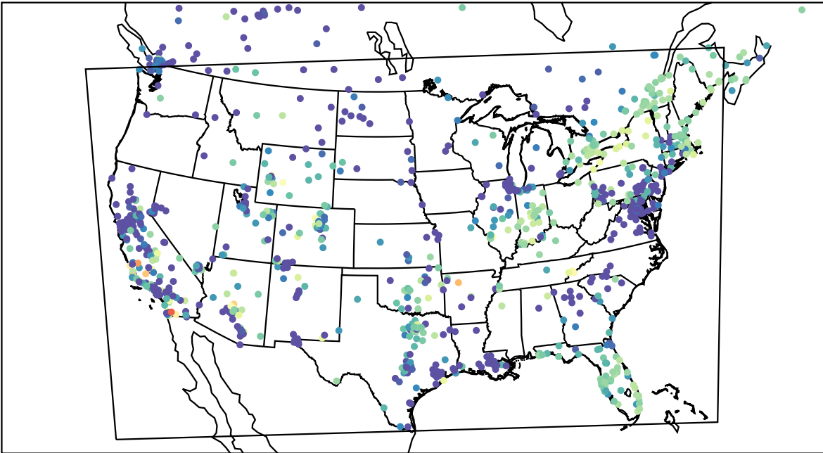
AirNOW (2023-11-04_07:00:00)
