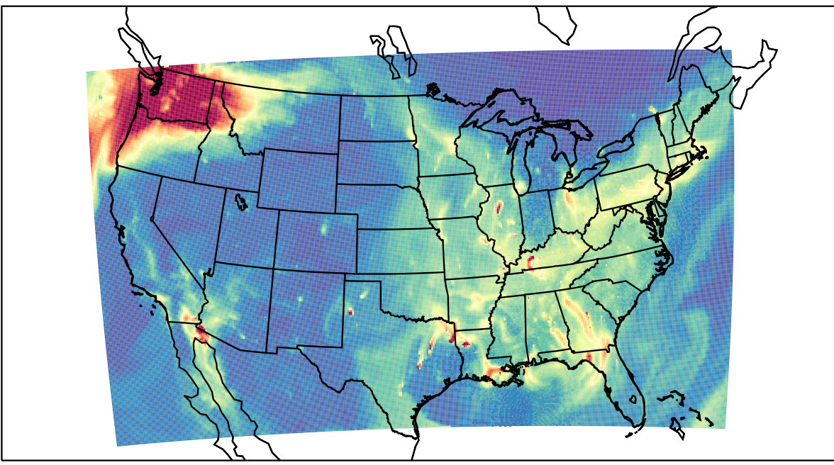
WRF 2023-11-05_16:00:00
