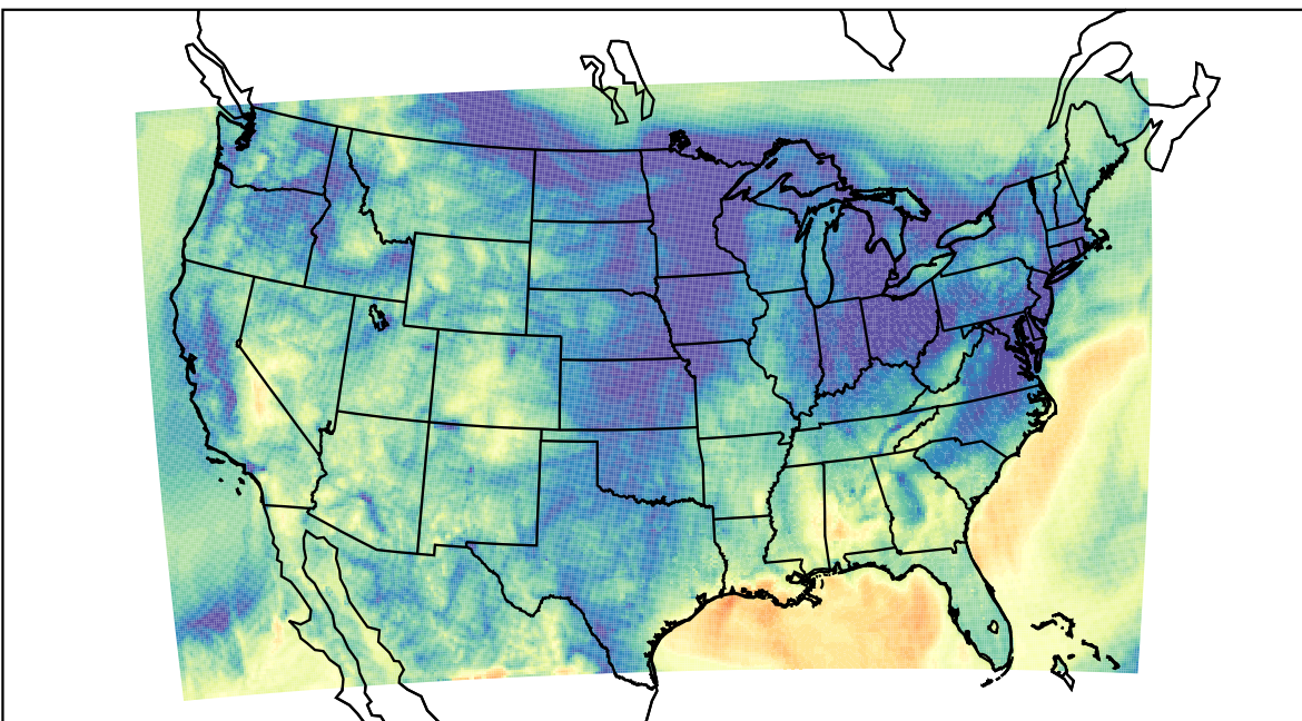
WRF (2023-11-06_10:00:00)
