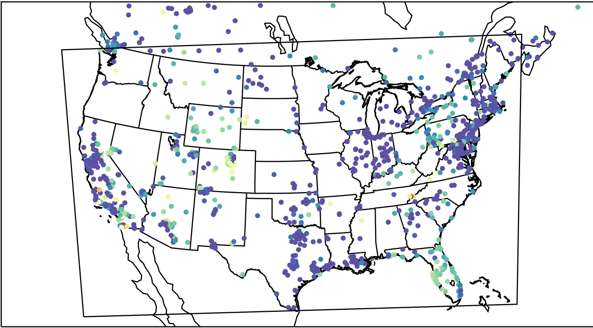
AirNOW (2023-11-05_13:00:00)
