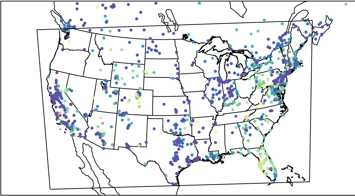
AirNOW (2023-11-05_14:00:00)
