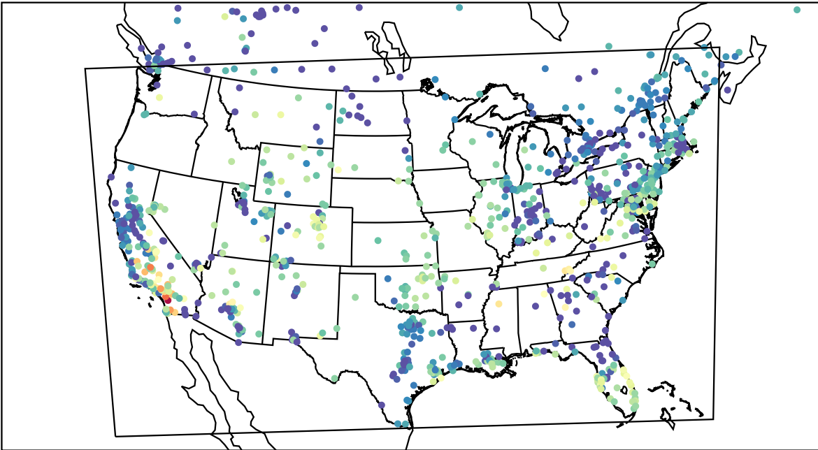
AirNOW (2023-11-06_02:00:00)
