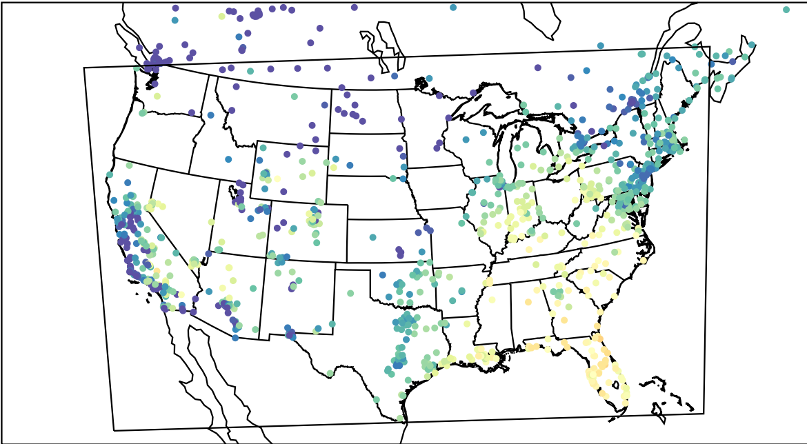
AirNOW (2023-11-06_16:00:00)
