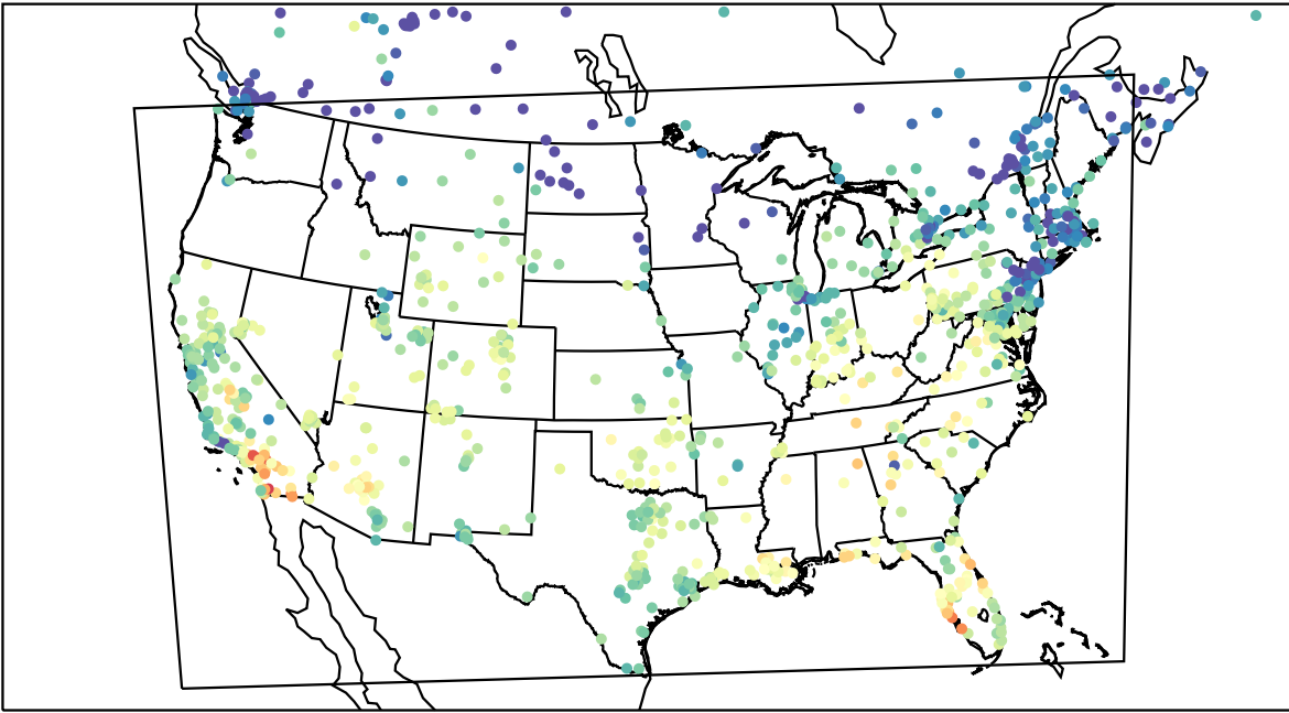
AirNOW (2023-11-06_22:00:00)
