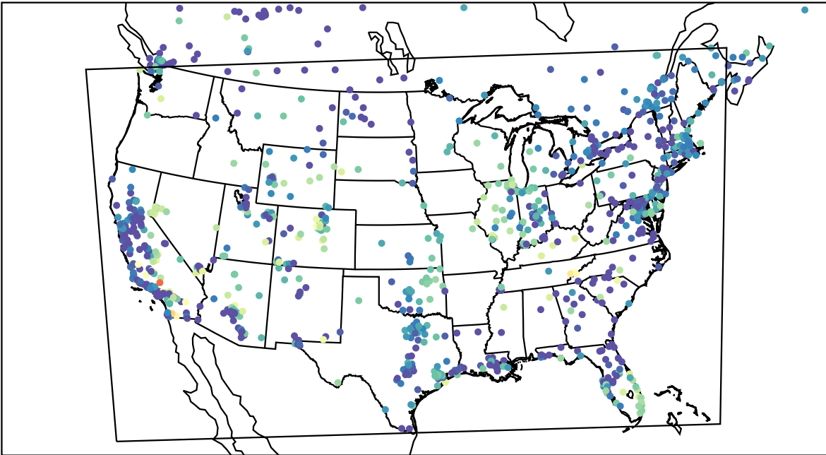
AirNOW (2023-11-06_06:00:00)
