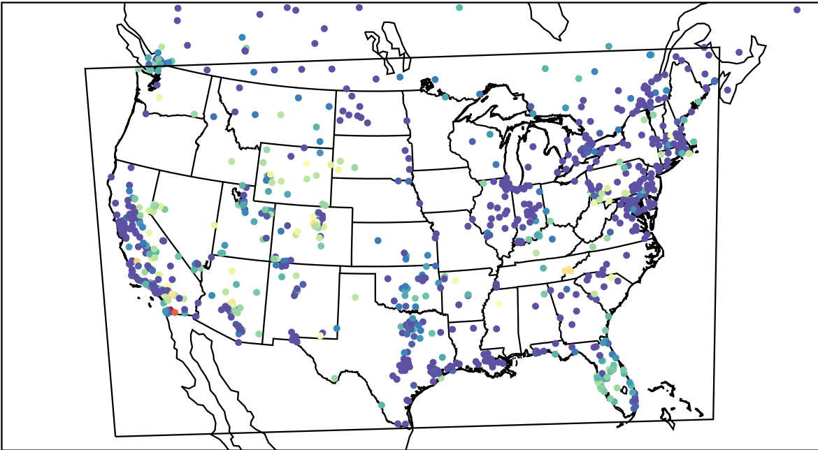
AirNOW (2023-11-05_07:00:00)
