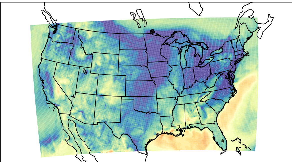
WRF (2023-11-06_12:00:00)
