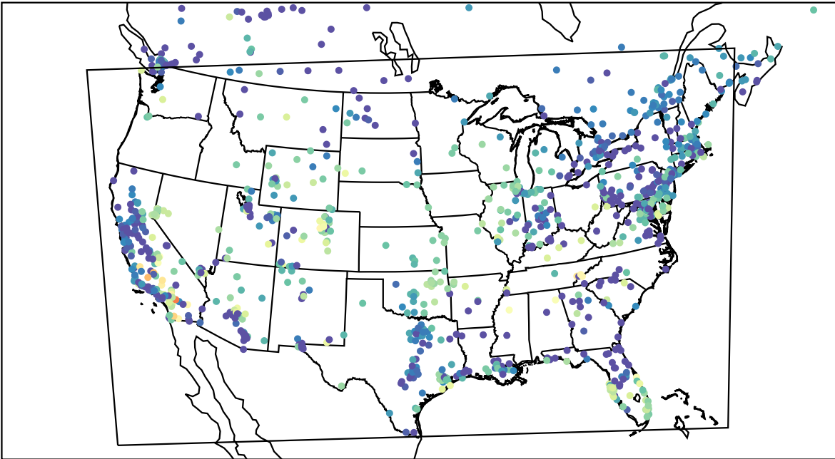
AirNOW (2023-11-06_04:00:00)
