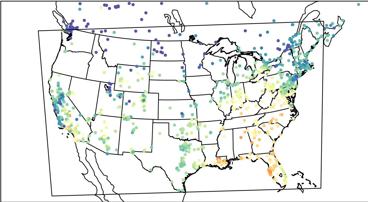
AirNOW (2023-11-06_18:00:00)
