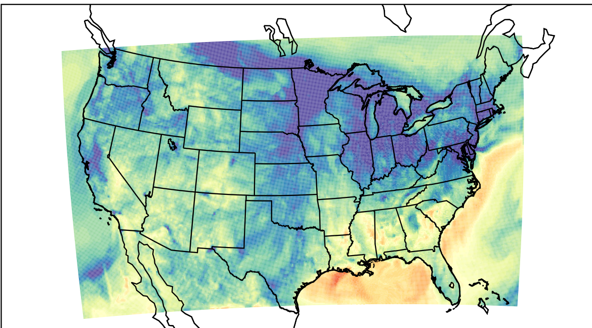
WRF (2023-11-06_05:00:00)
