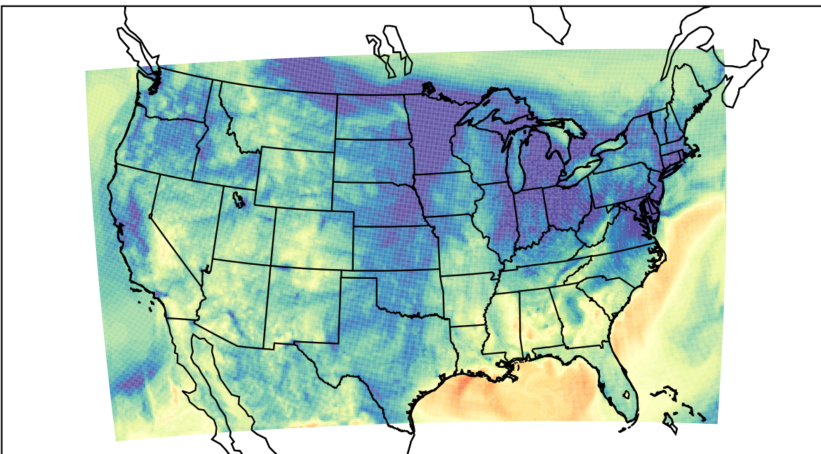
WRF (2023-11-06_07:00:00)
