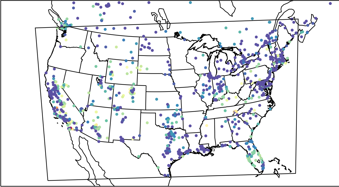
AirNOW (2023-11-05_06:00:00)
