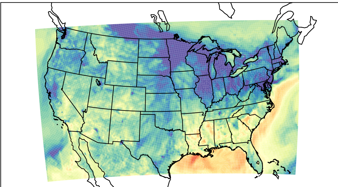
WRF (2023-11-06_03:00:00)
