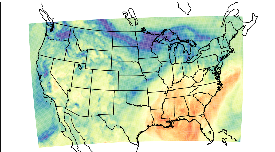
WRF (2023-11-06_18:00:00)
