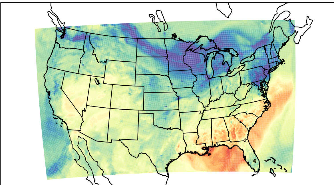
WRF (2023-11-06_23:00:00)
