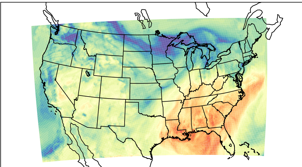
WRF (2023-11-06_19:00:00)
