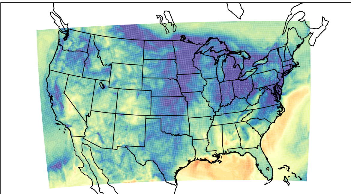
WRF (2023-11-06_09:00:00)
