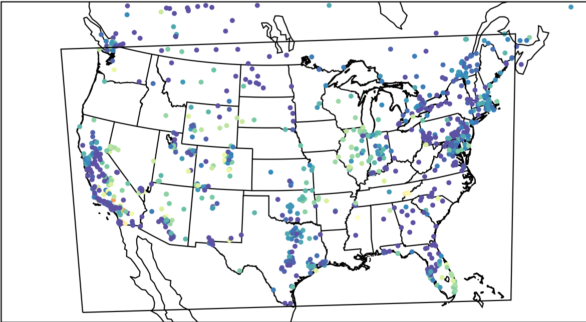
AirNOW (2023-11-06_07:00:00)
