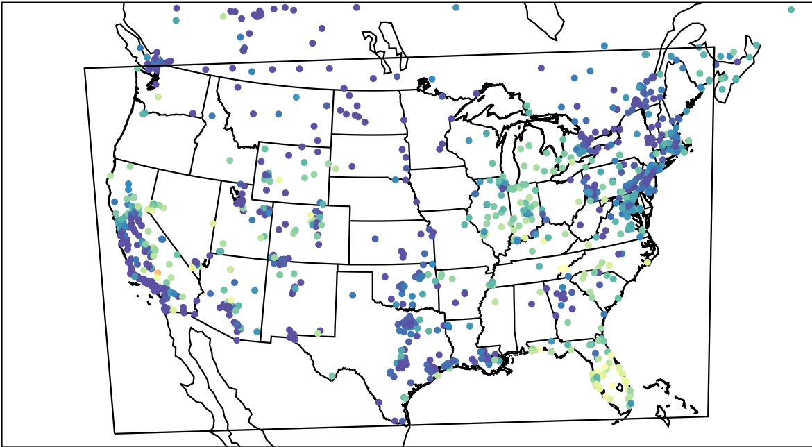
AirNOW (2023-11-06_14:00:00)
