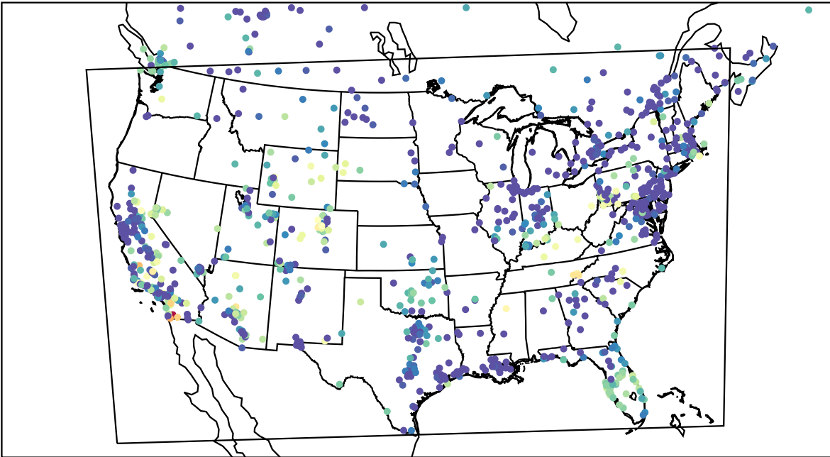
AirNOW (2023-11-05_05:00:00)
