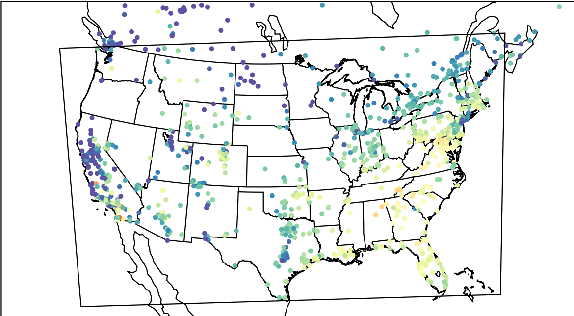
AirNOW (2023-11-05_16:00:00)
