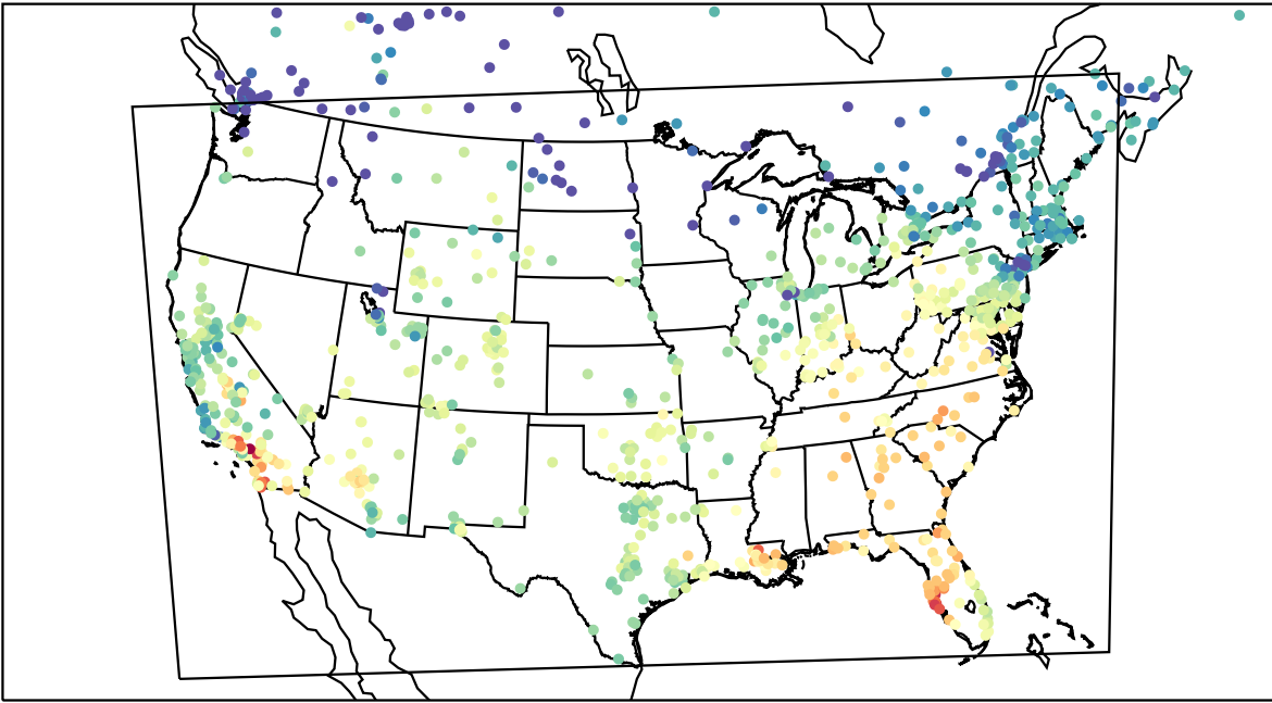
AirNOW (2023-11-06_20:00:00)
