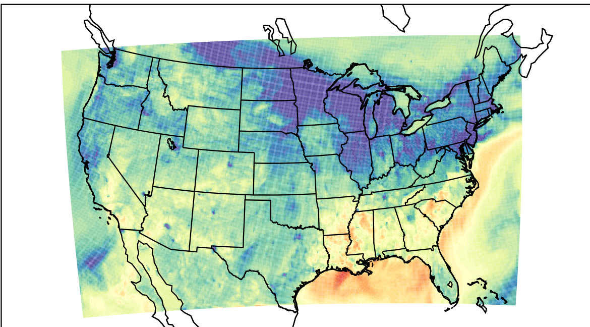
WRF (2023-11-06_01:00:00)
