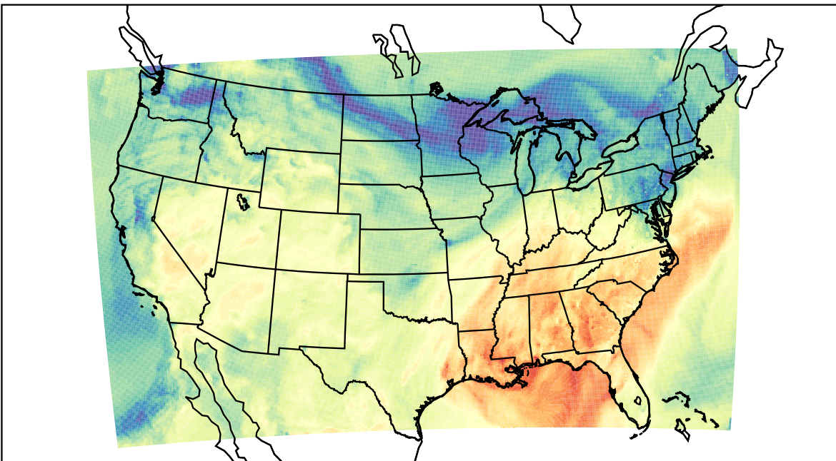
WRF (2023-11-06_21:00:00)
