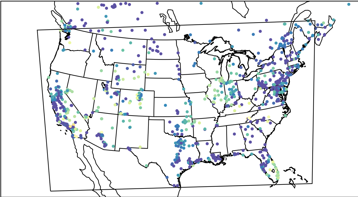
AirNOW (2023-11-06_08:00:00)
