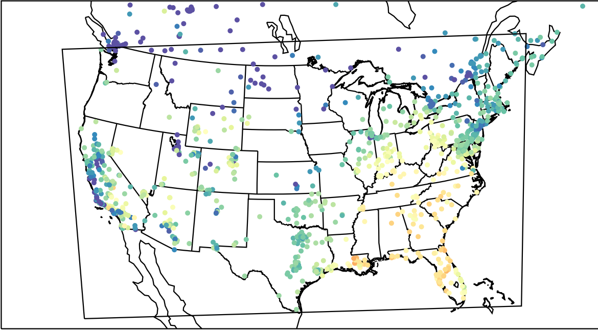
AirNOW (2023-11-06_17:00:00)
