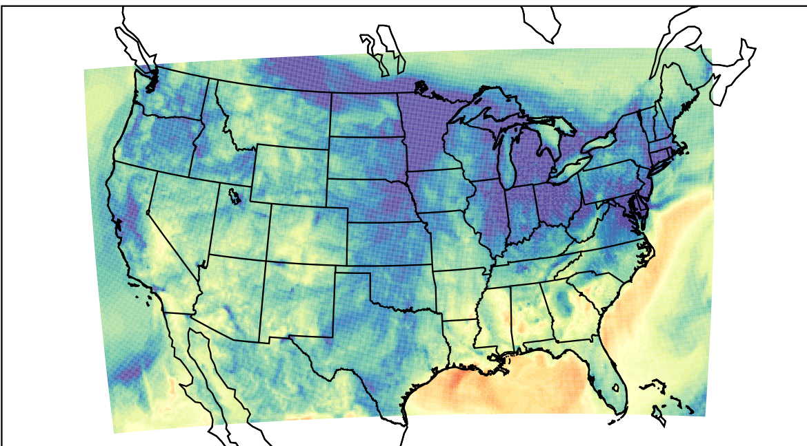
WRF (2023-11-06_06:00:00)
