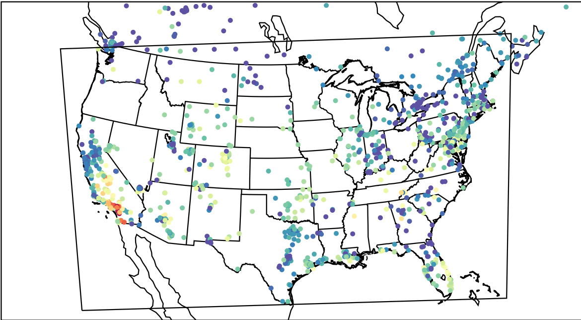
AirNOW (2023-11-06_01:00:00)
