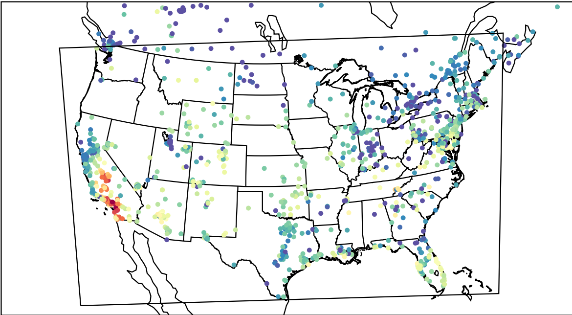
AirNOW (2023-11-06_00:00:00)
