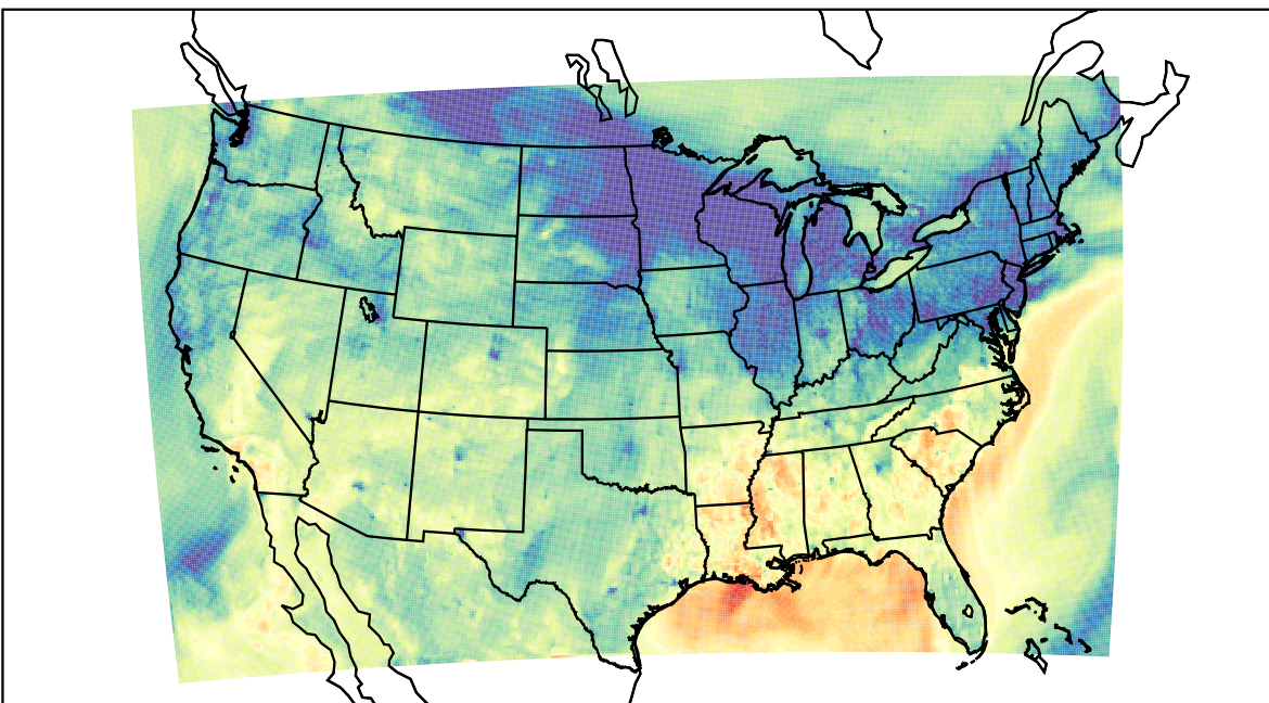
WRF (2023-11-06_00:00:00)
