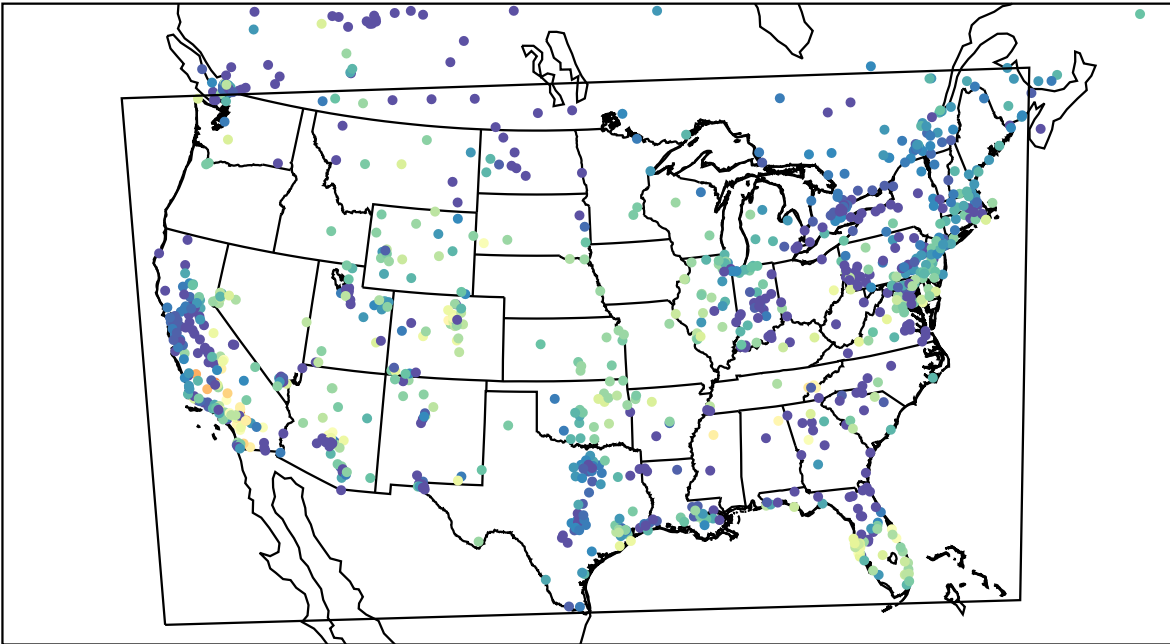
AirNOW (2023-11-06_03:00:00)
