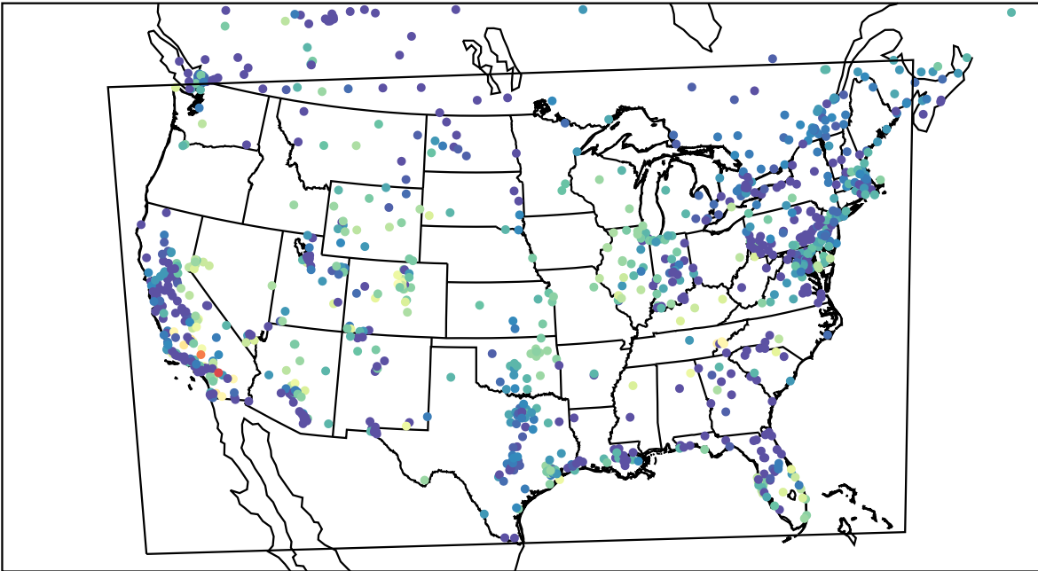
AirNOW (2023-11-06_05:00:00)
