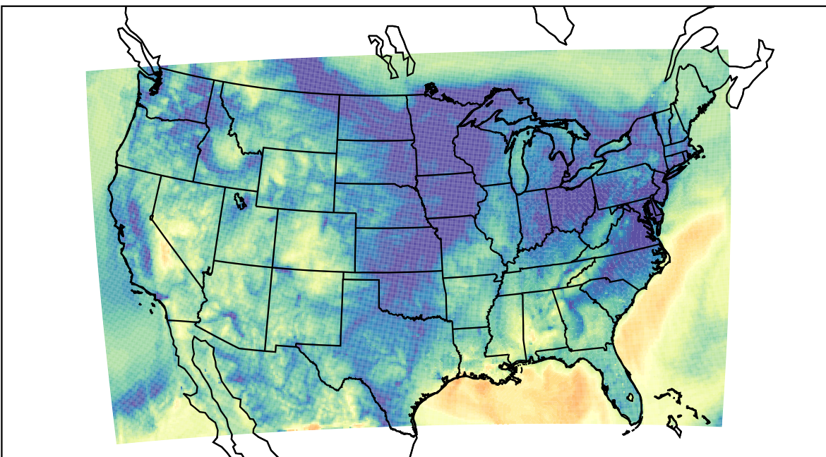
WRF (2023-11-06_13:00:00)
