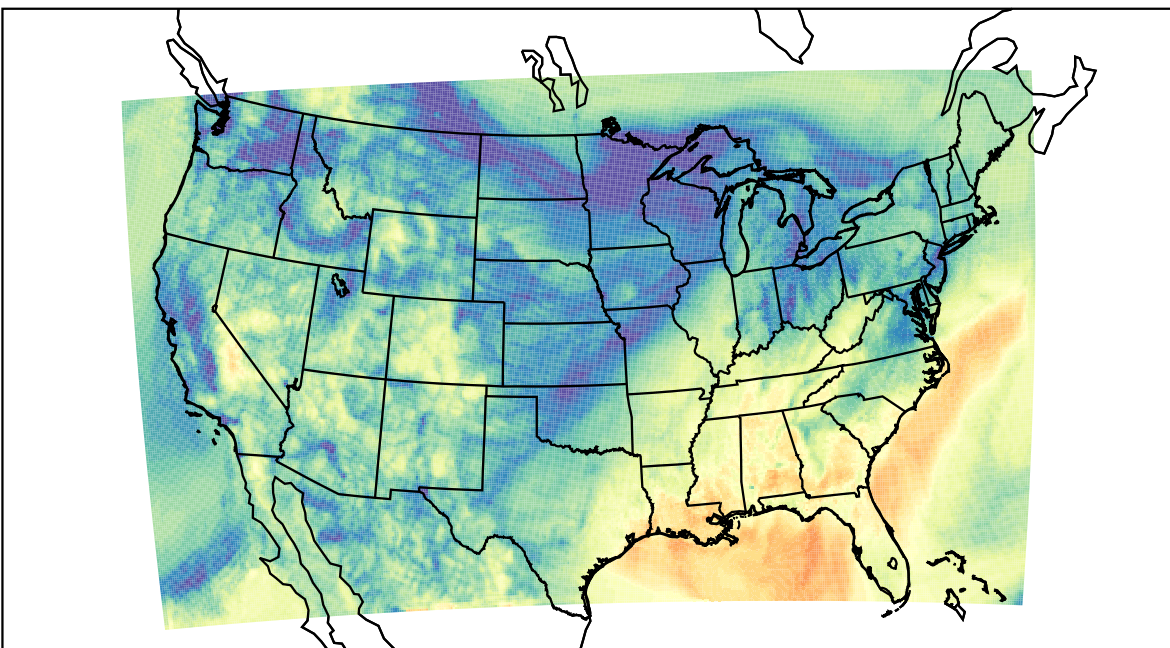
WRF (2023-11-06_16:00:00)
