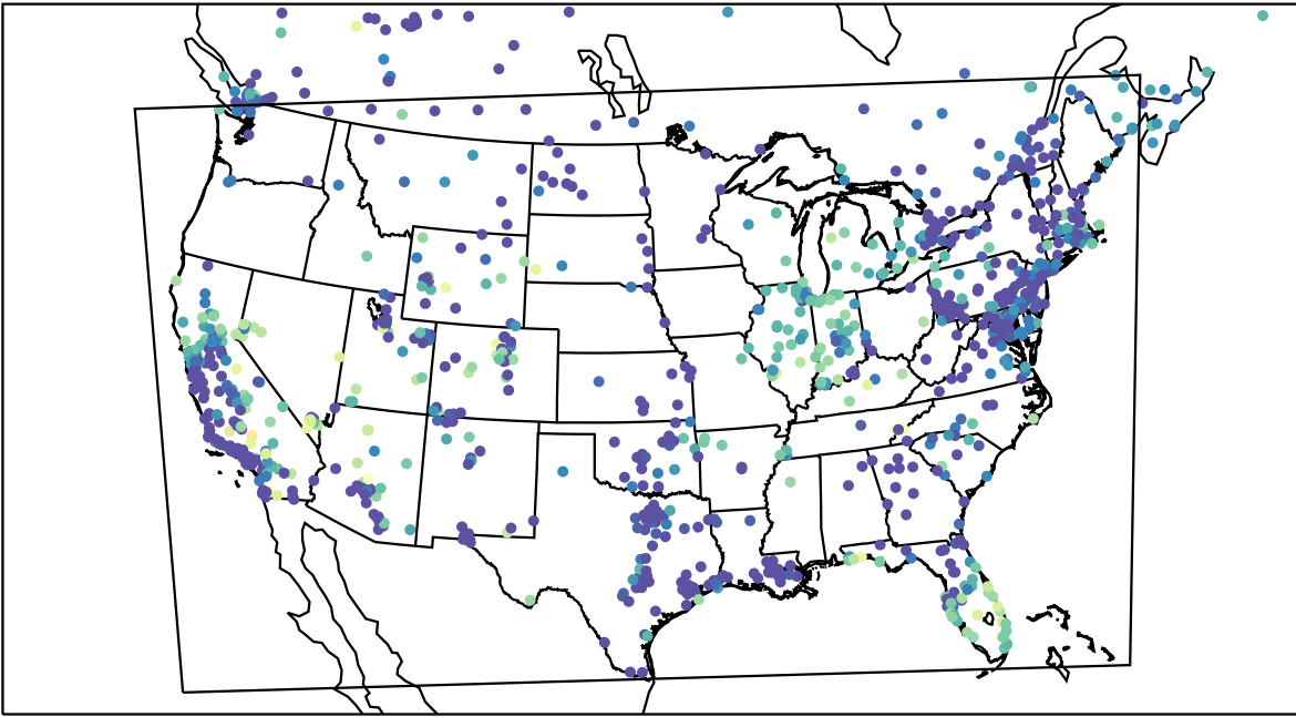
AirNOW (2023-11-06_13:00:00)
