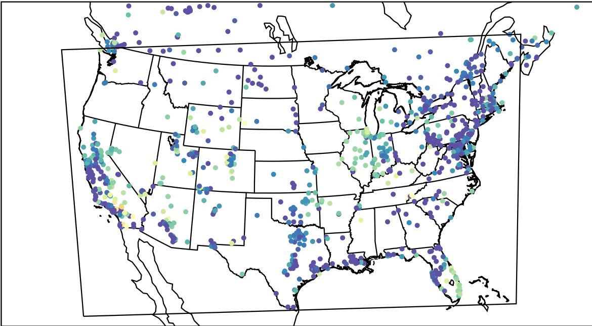
AirNOW (2023-11-06_09:00:00)
