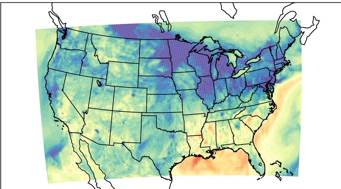
WRF (2023-11-06_02:00:00)
