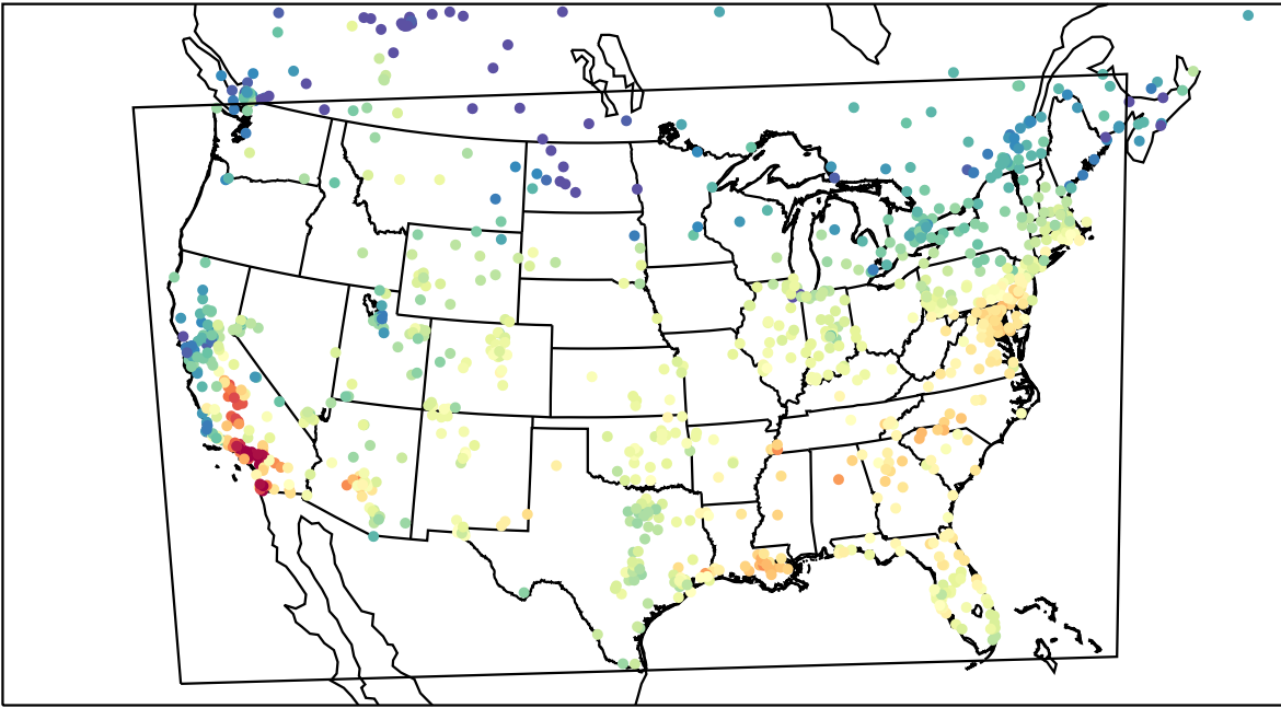
AirNOW (2023-11-05_20:00:00)
