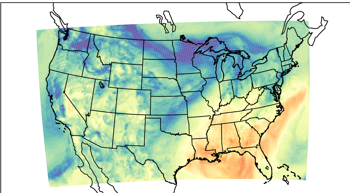
WRF (2023-11-06_17:00:00)
