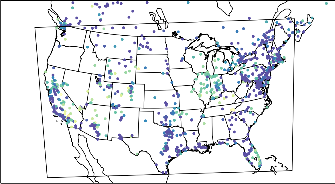
AirNOW (2023-11-06_11:00:00)
