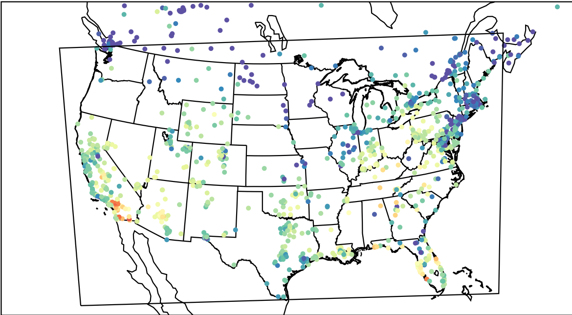
AirNOW (2023-11-06_23:00:00)
