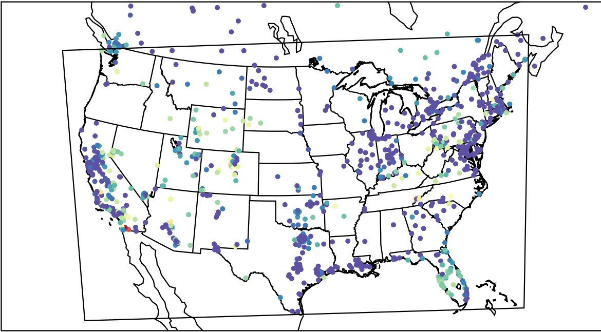
AirNOW (2023-11-05_08:00:00)
