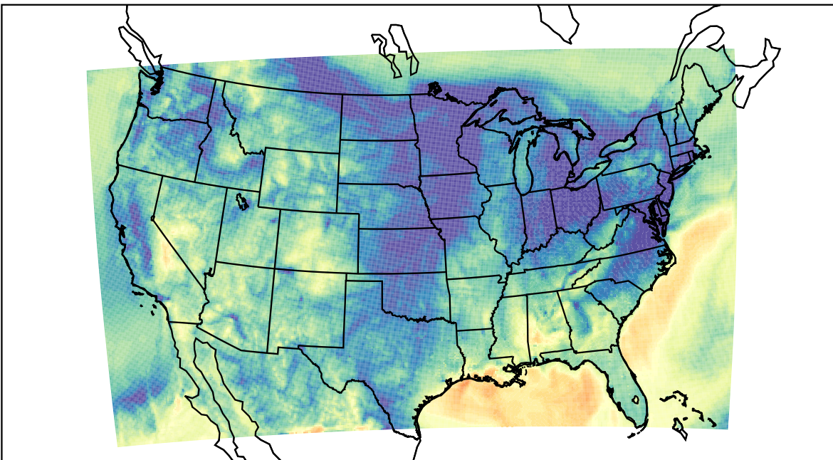
WRF (2023-11-06_11:00:00)
