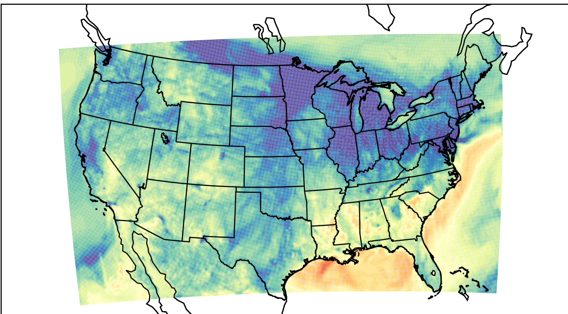
WRF (2023-11-06_04:00:00)
