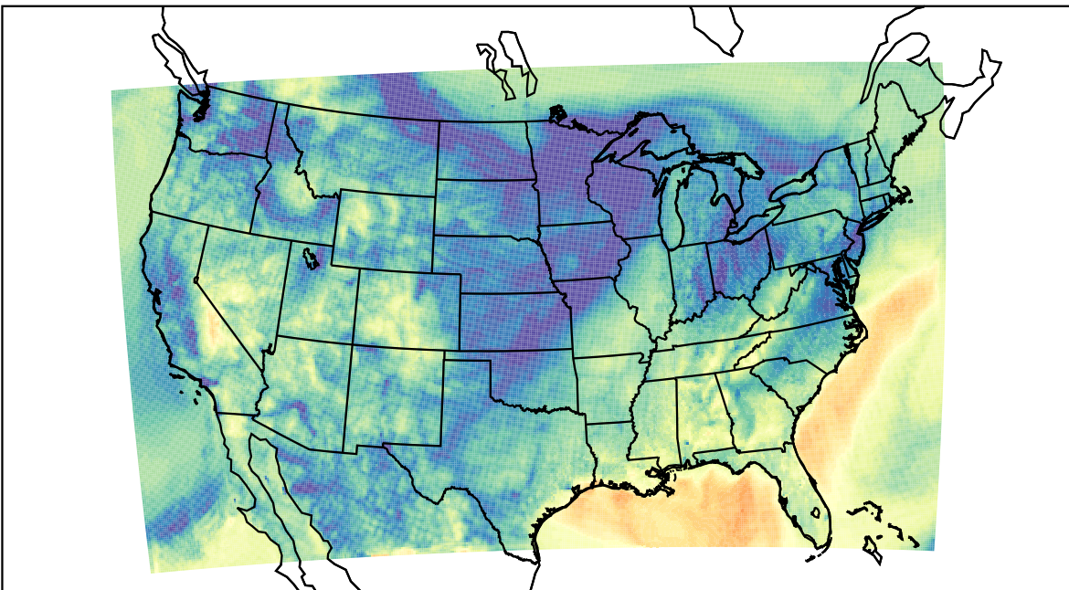
WRF (2023-11-06_15:00:00)
