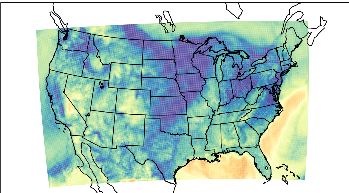
WRF (2023-11-06_14:00:00)
