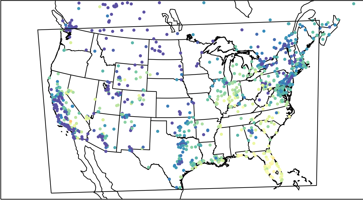
AirNOW (2023-11-06_15:00:00)
