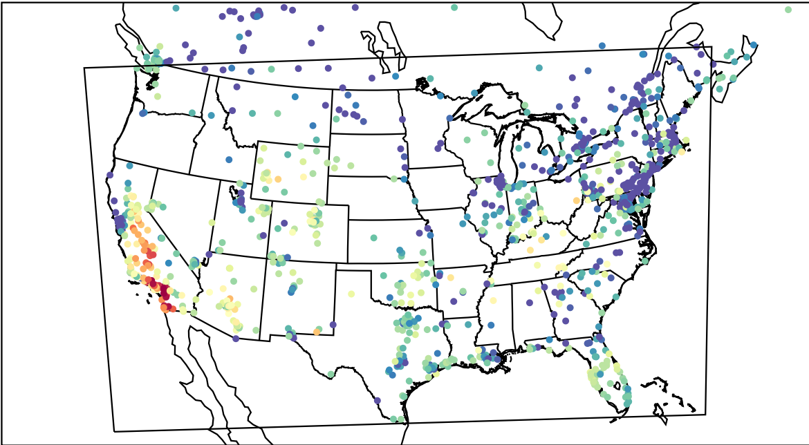
AirNOW (2023-11-05_00:00:00)
