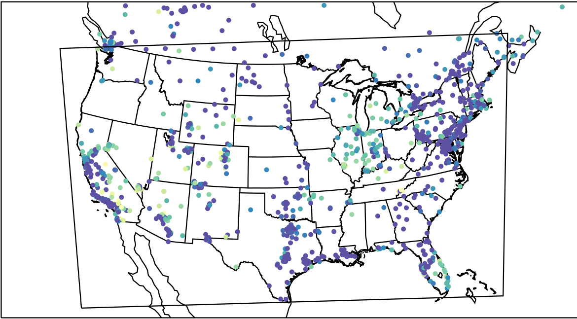
AirNOW (2023-11-06_12:00:00)
