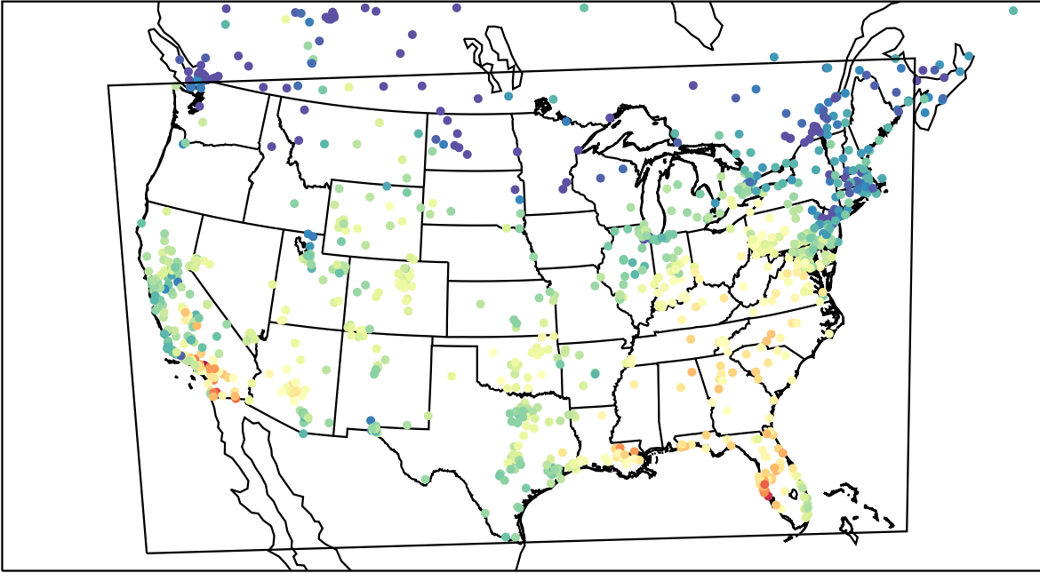
AirNOW (2023-11-06_21:00:00)
