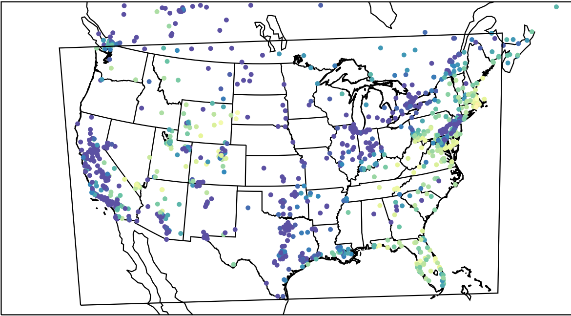
AirNOW (2023-11-07_14:00:00)
