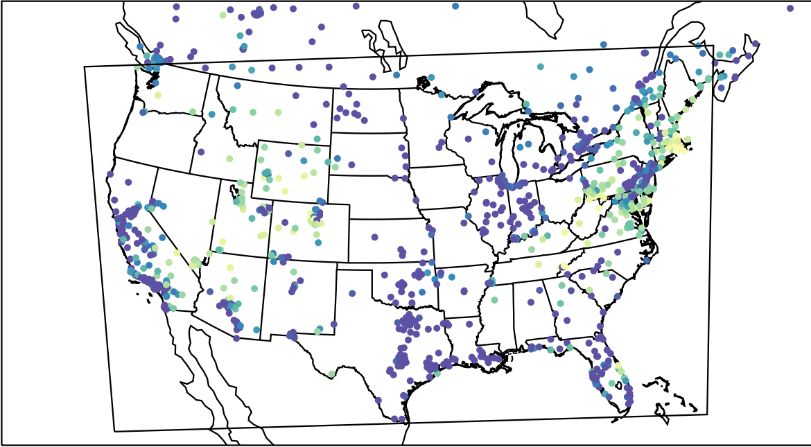
AirNOW (2023-11-07_12:00:00)
