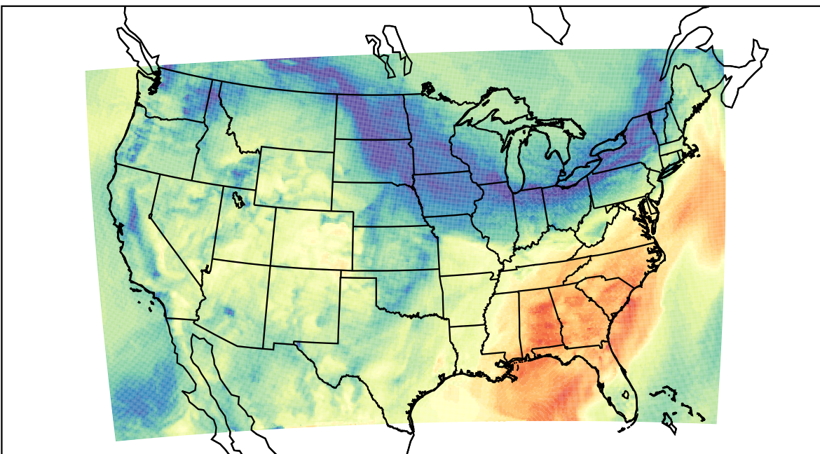
WRF (2023-11-07_18:00:00)
