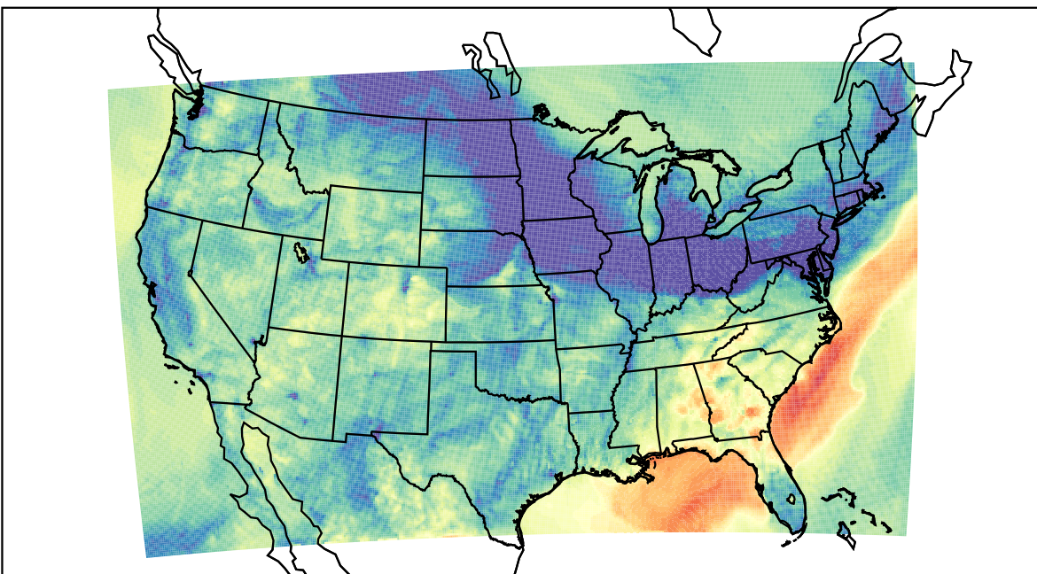
WRF (2023-11-08_03:00:00)
