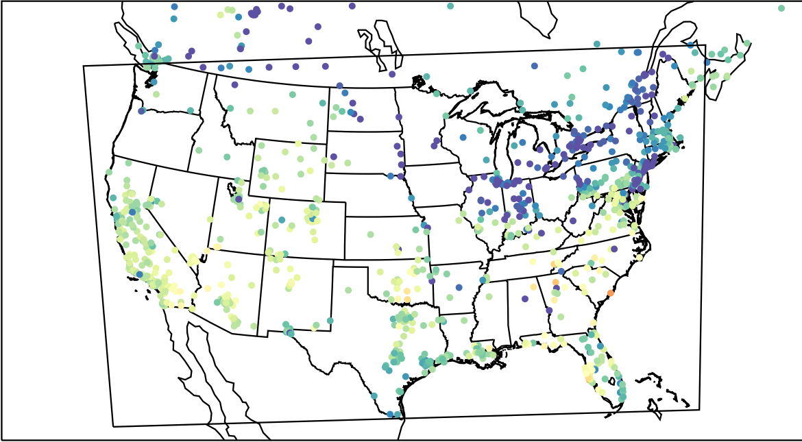
AirNOW (2023-11-07_23:00:00)
