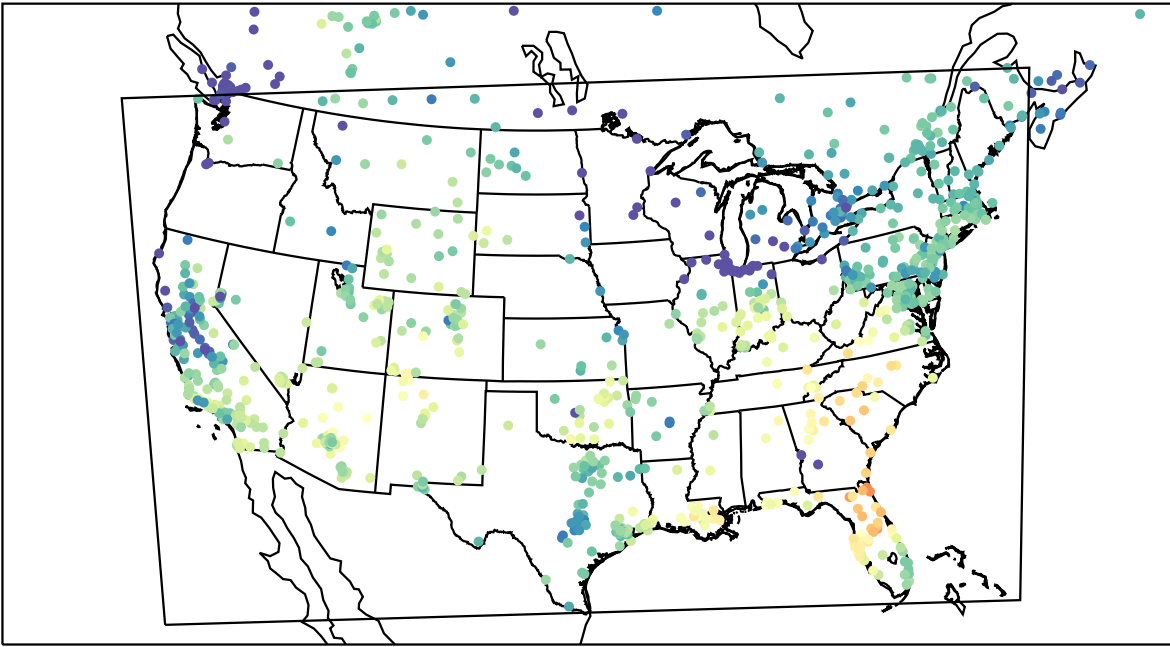
AirNOW (2023-11-08_18:00:00)
