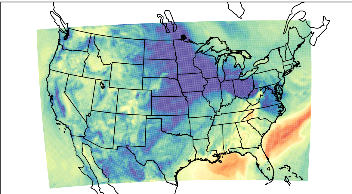
WRF (2023-11-08_15:00:00)
