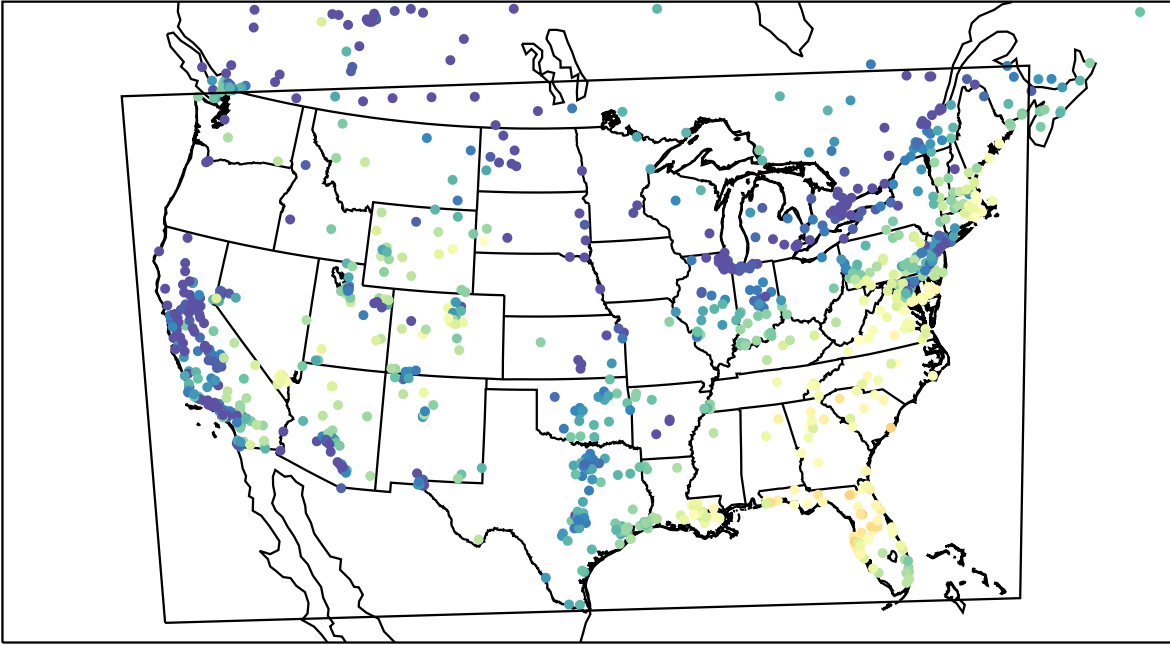
AirNOW (2023-11-07_16:00:00)
