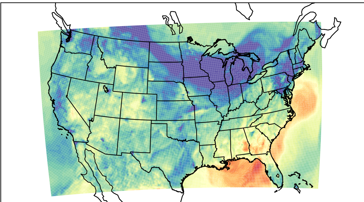
WRF (2023-11-07_03:00:00)
