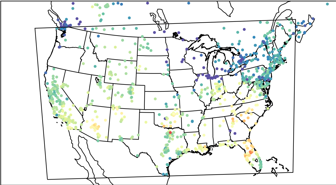
AirNOW (2023-11-08_21:00:00)
