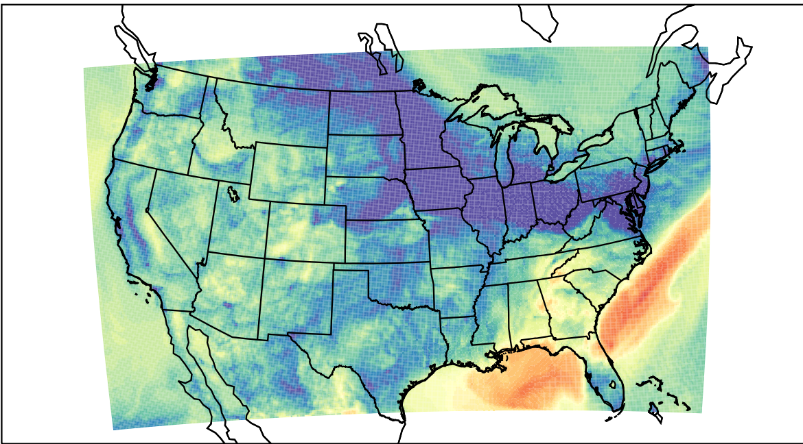
WRF (2023-11-08_07:00:00)
