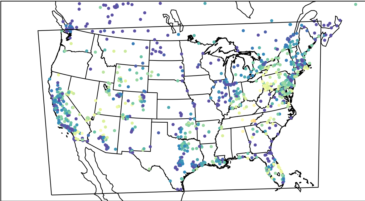
AirNOW (2023-11-07_04:00:00)
