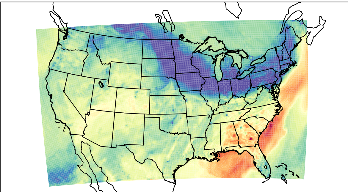
WRF (2023-11-07_23:00:00)
