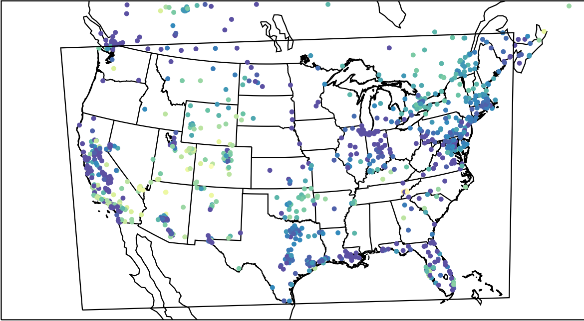
AirNOW (2023-11-08_08:00:00)
