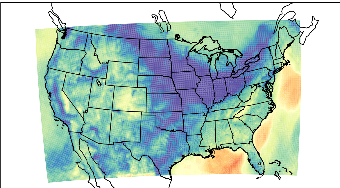
WRF (2023-11-07_14:00:00)
