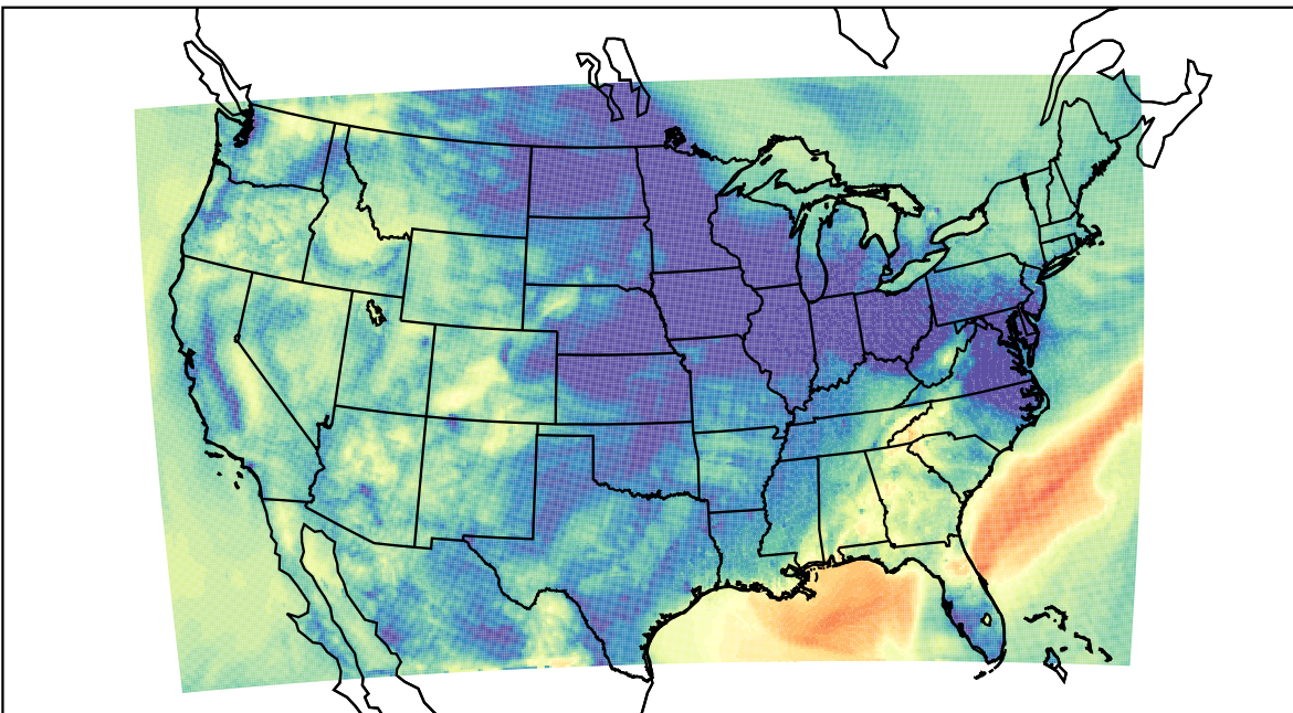
WRF (2023-11-08_12:00:00)
