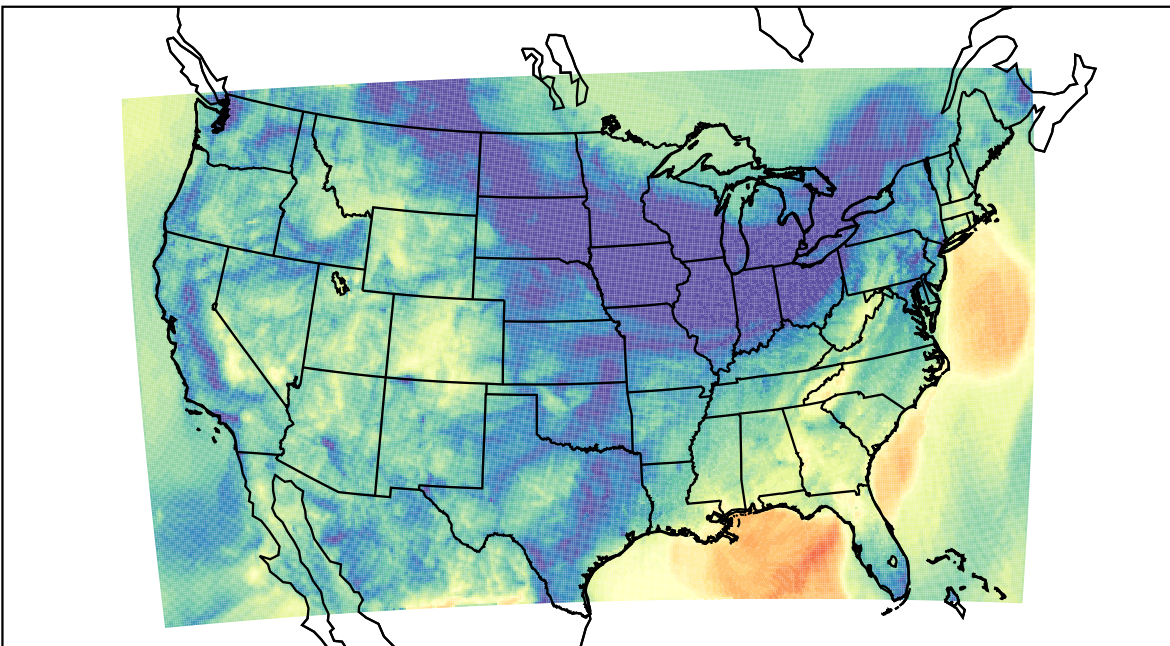
WRF (2023-11-07_10:00:00)
