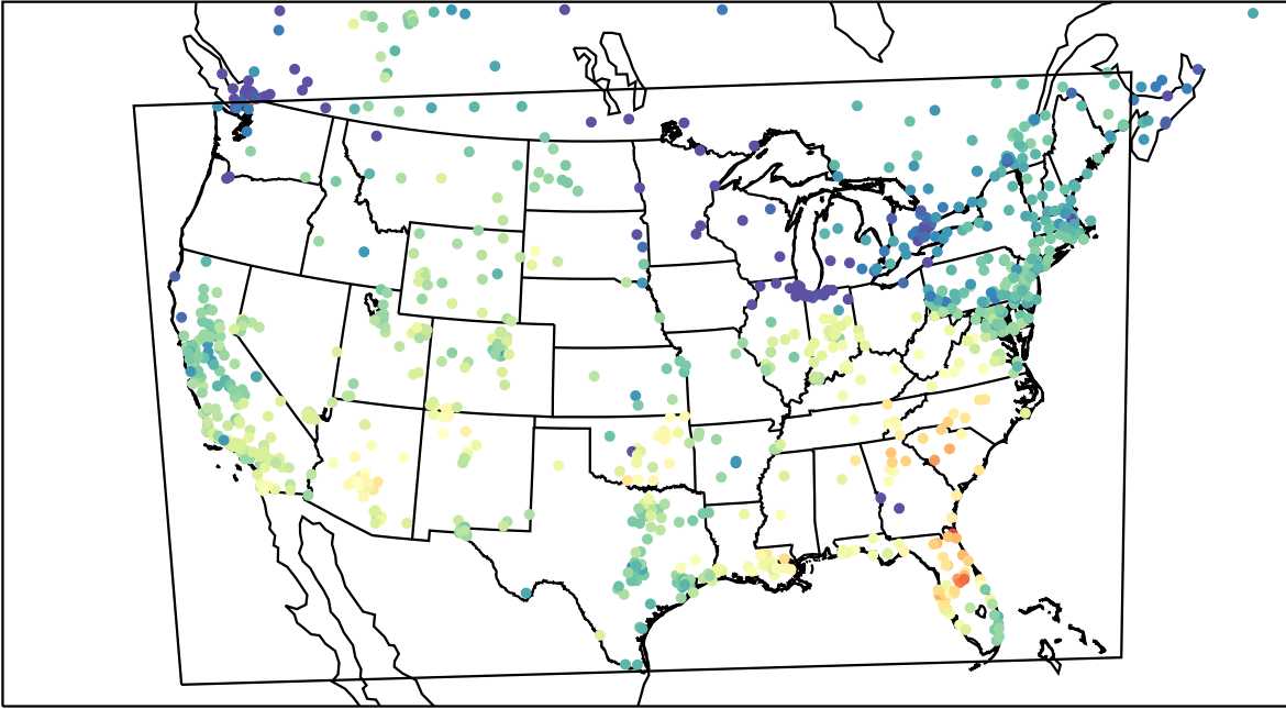
AirNOW (2023-11-08_20:00:00)
