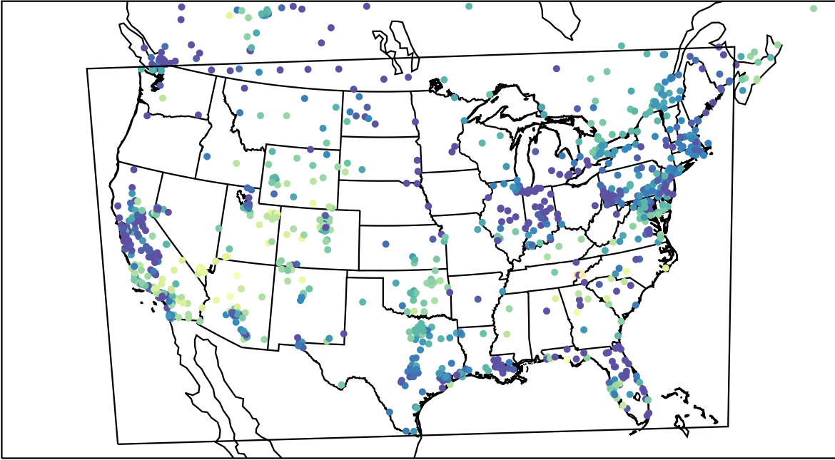
AirNOW (2023-11-08_05:00:00)
