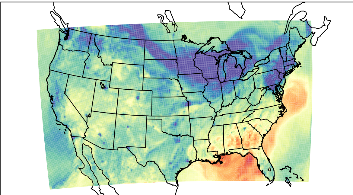
WRF (2023-11-07_01:00:00)
