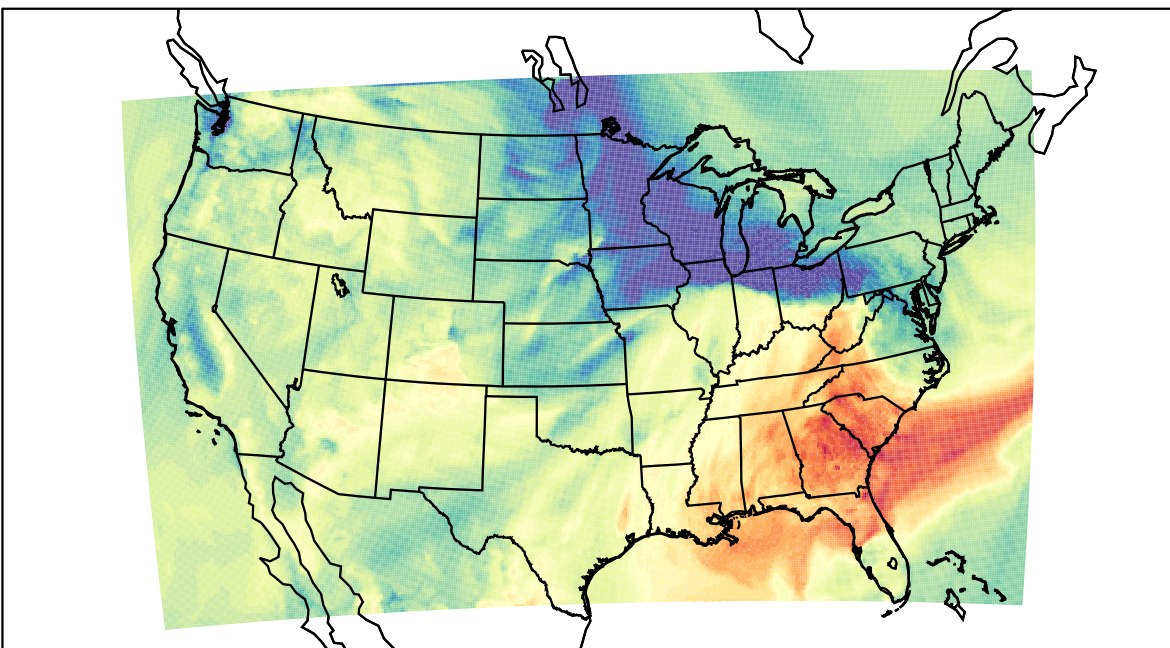
WRF (2023-11-08_19:00:00)
