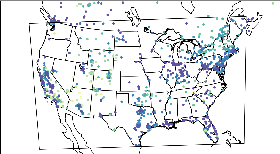
AirNOW (2023-11-08_09:00:00)
