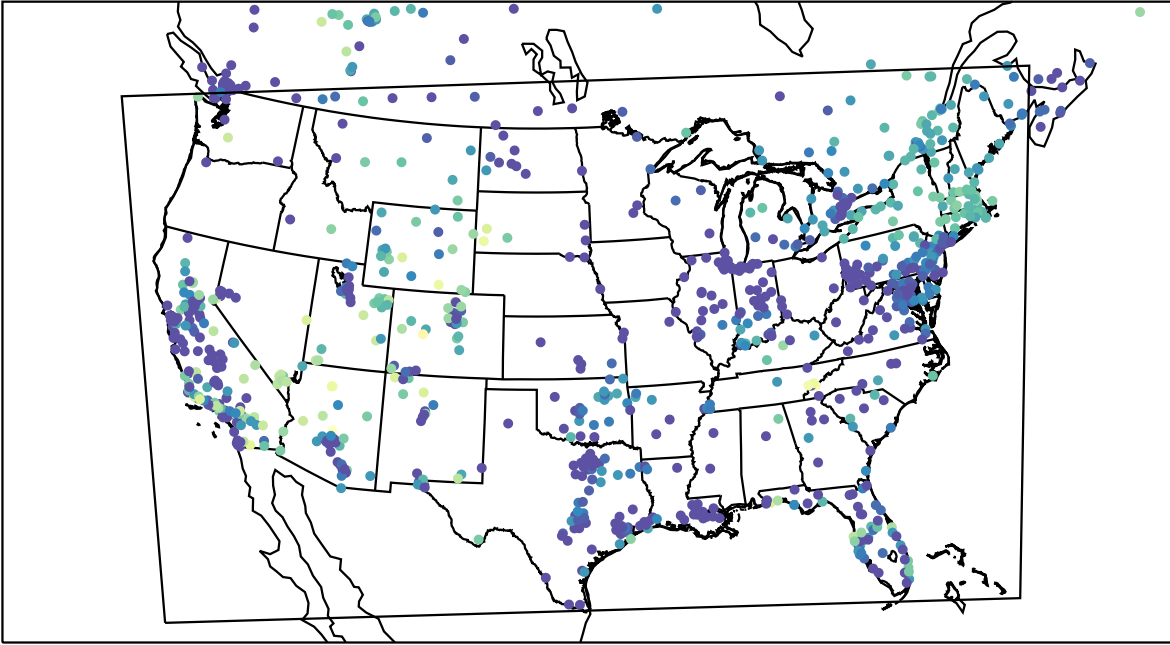
AirNOW (2023-11-08_13:00:00)
