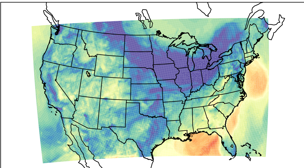
WRF (2023-11-07_09:00:00)
