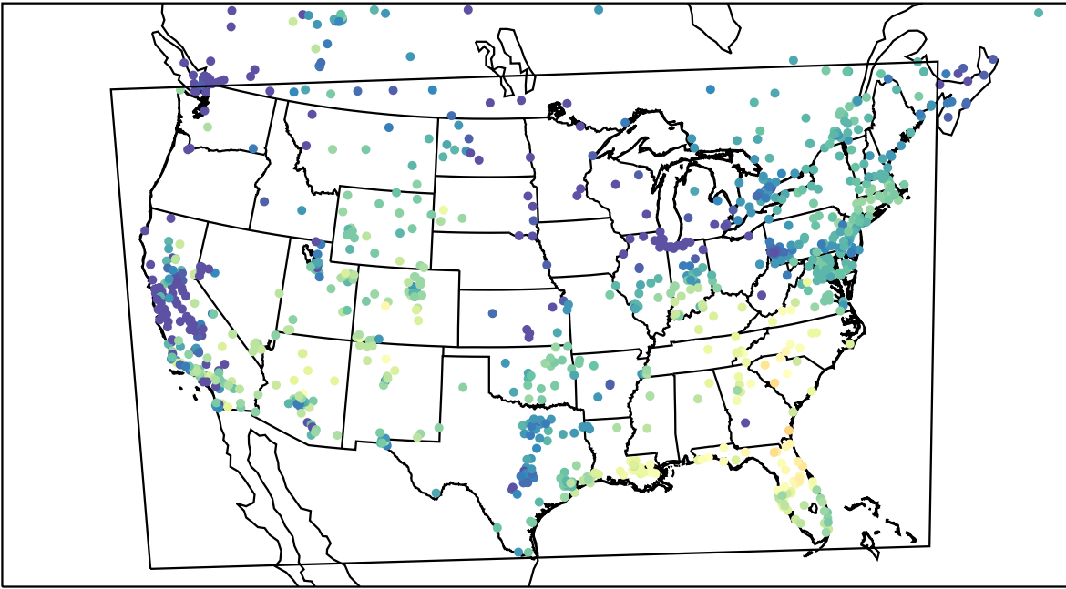
AirNOW (2023-11-08_16:00:00)
