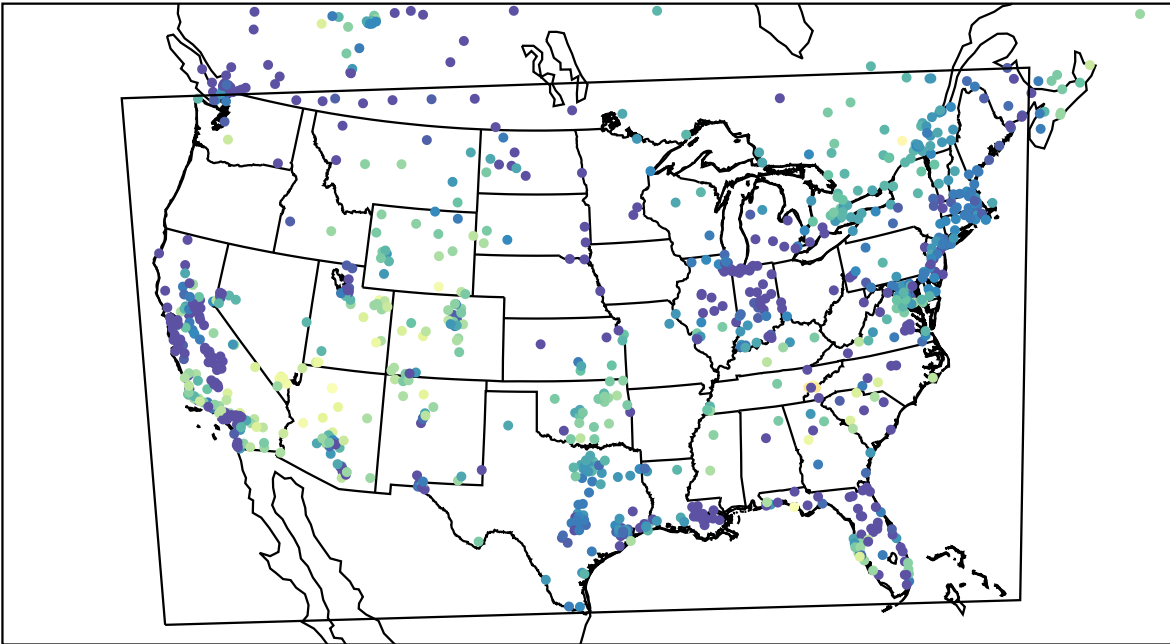
AirNOW (2023-11-08_06:00:00)
