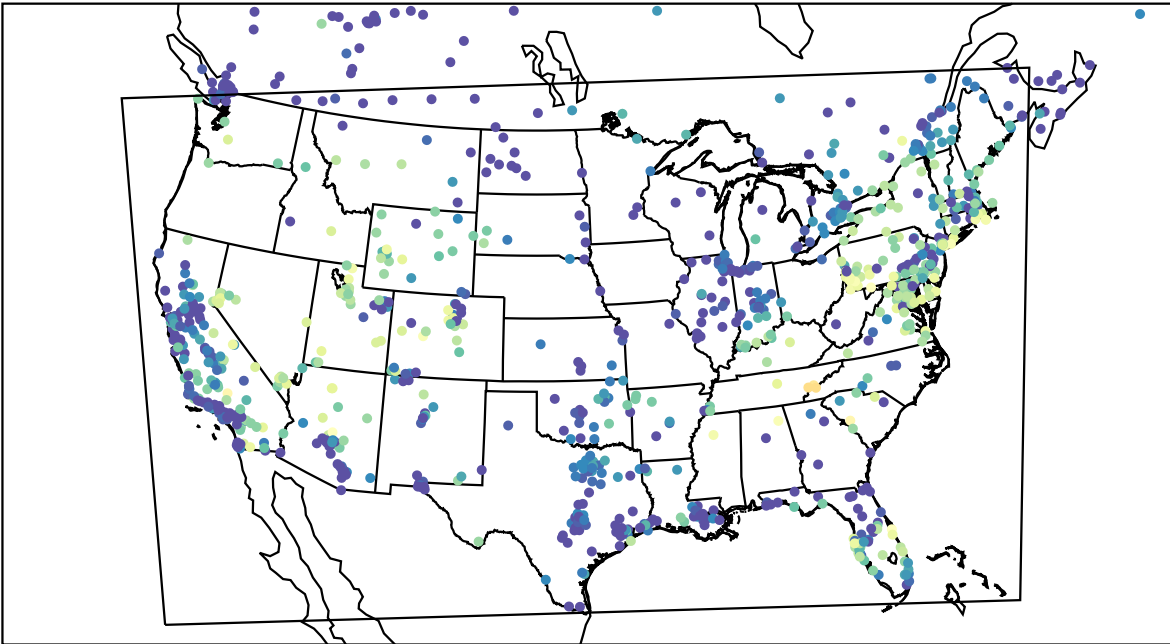
AirNOW (2023-11-07_07:00:00)
