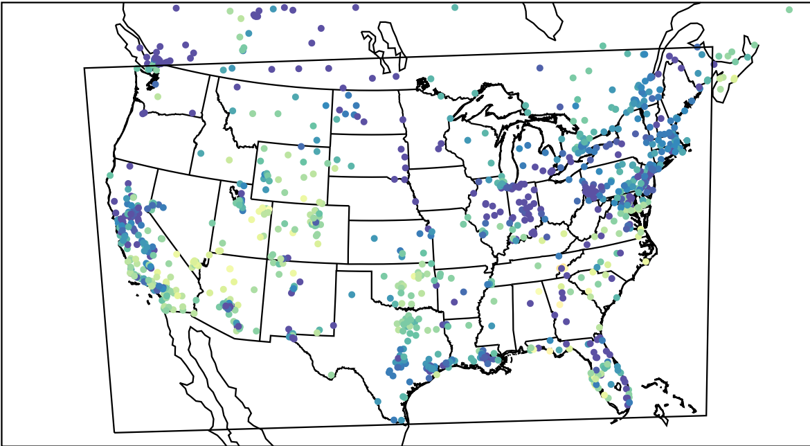
AirNOW (2023-11-08_03:00:00)
