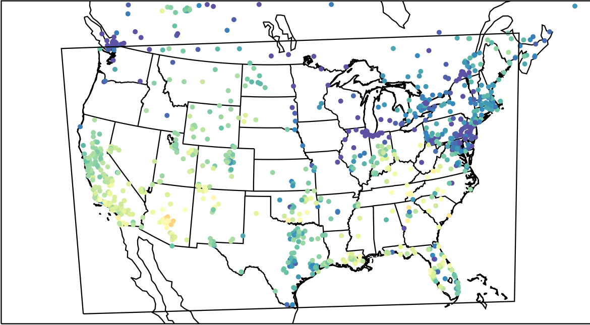
AirNOW (2023-11-08_23:00:00)
