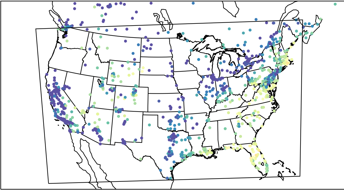
AirNOW (2023-11-07_15:00:00)
