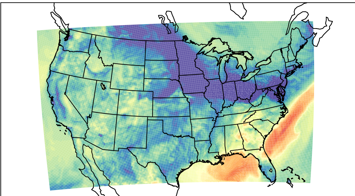
WRF (2023-11-08_06:00:00)
