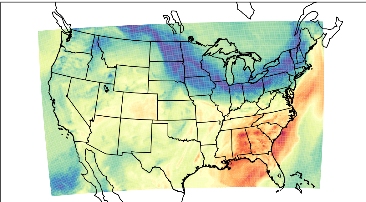
WRF (2023-11-07_21:00:00)
