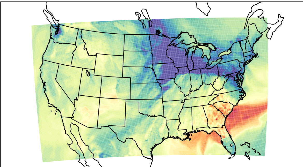
WRF (2023-11-08_23:00:00)
