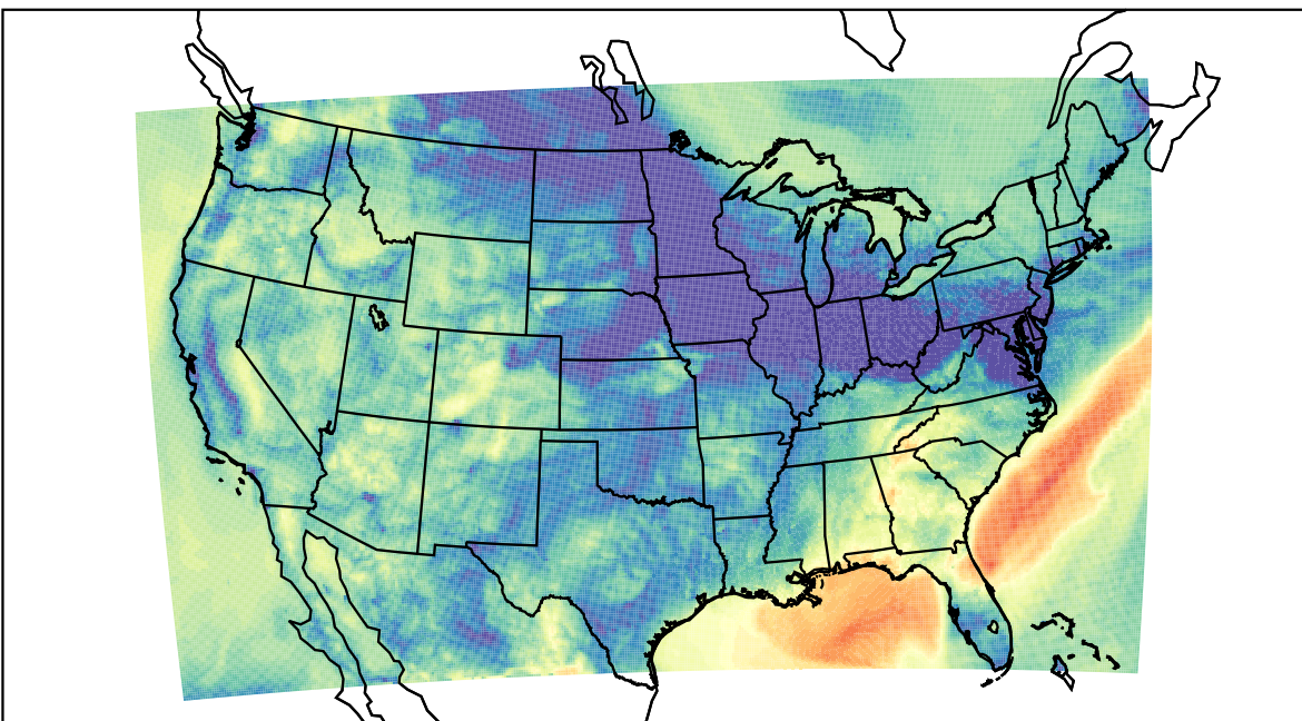
WRF (2023-11-08_08:00:00)
