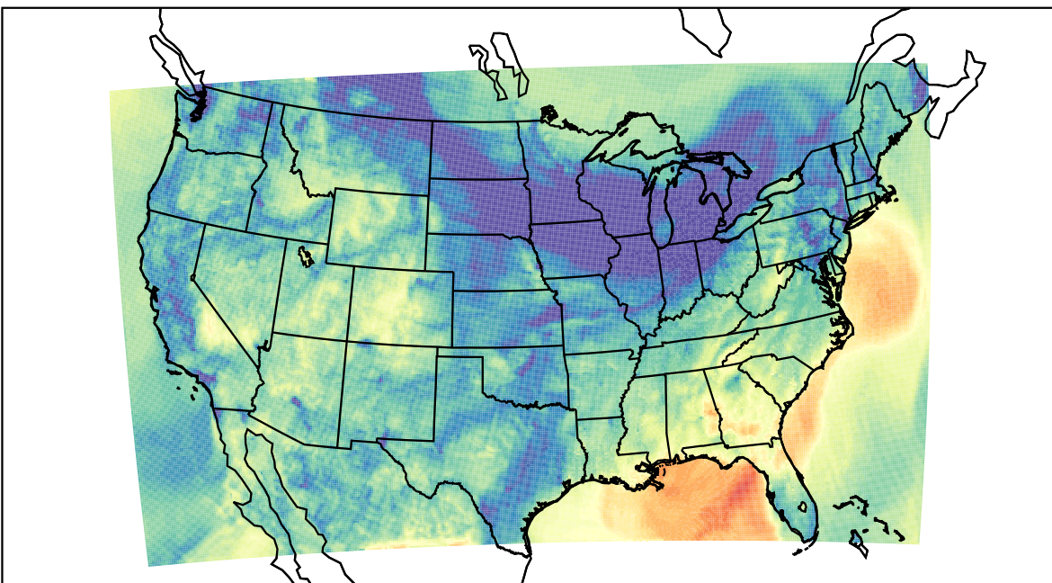
WRF (2023-11-07_06:00:00)
