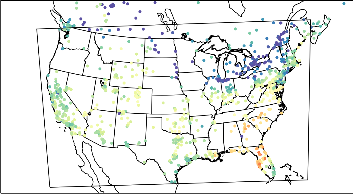
AirNOW (2023-11-07_20:00:00)
