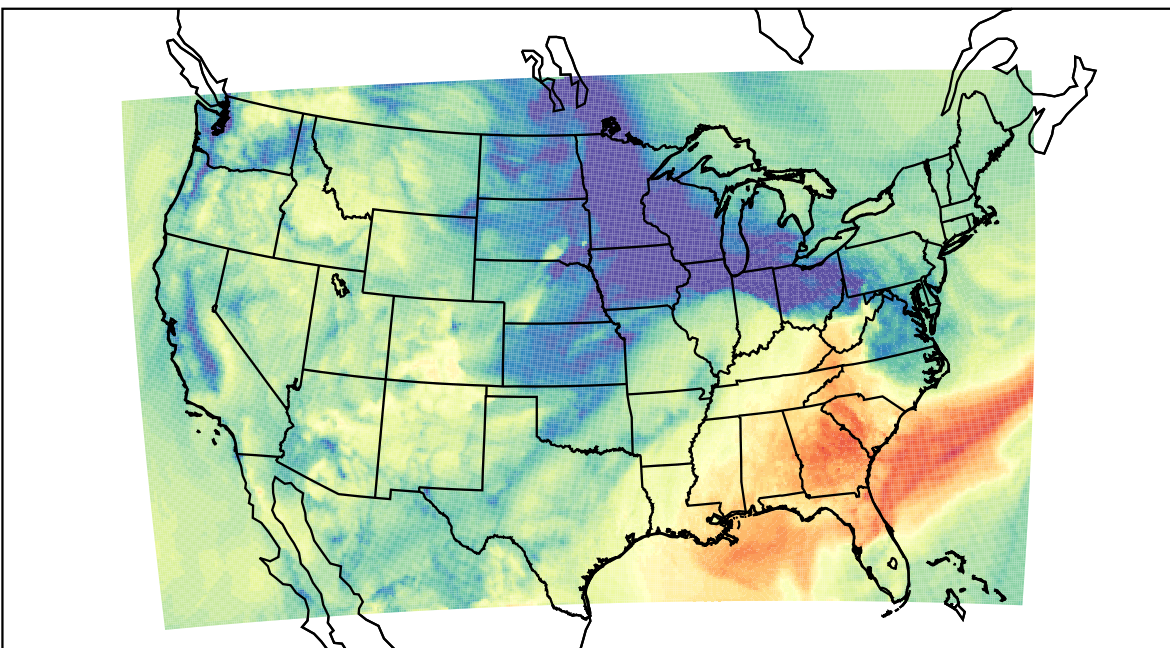
WRF (2023-11-08_17:00:00)
