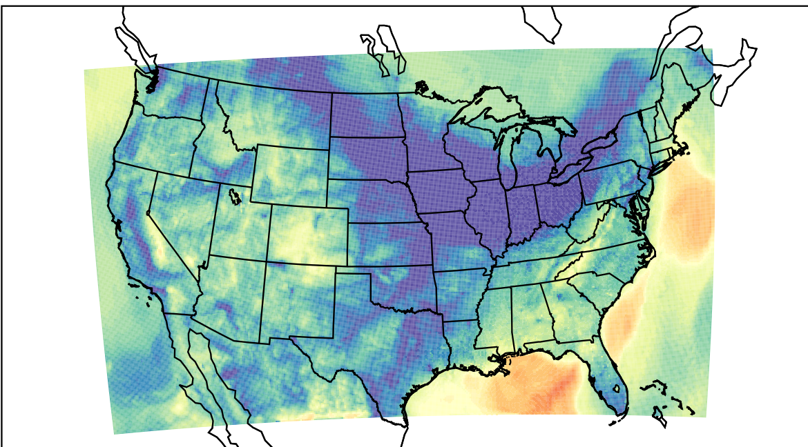
WRF (2023-11-07_13:00:00)
