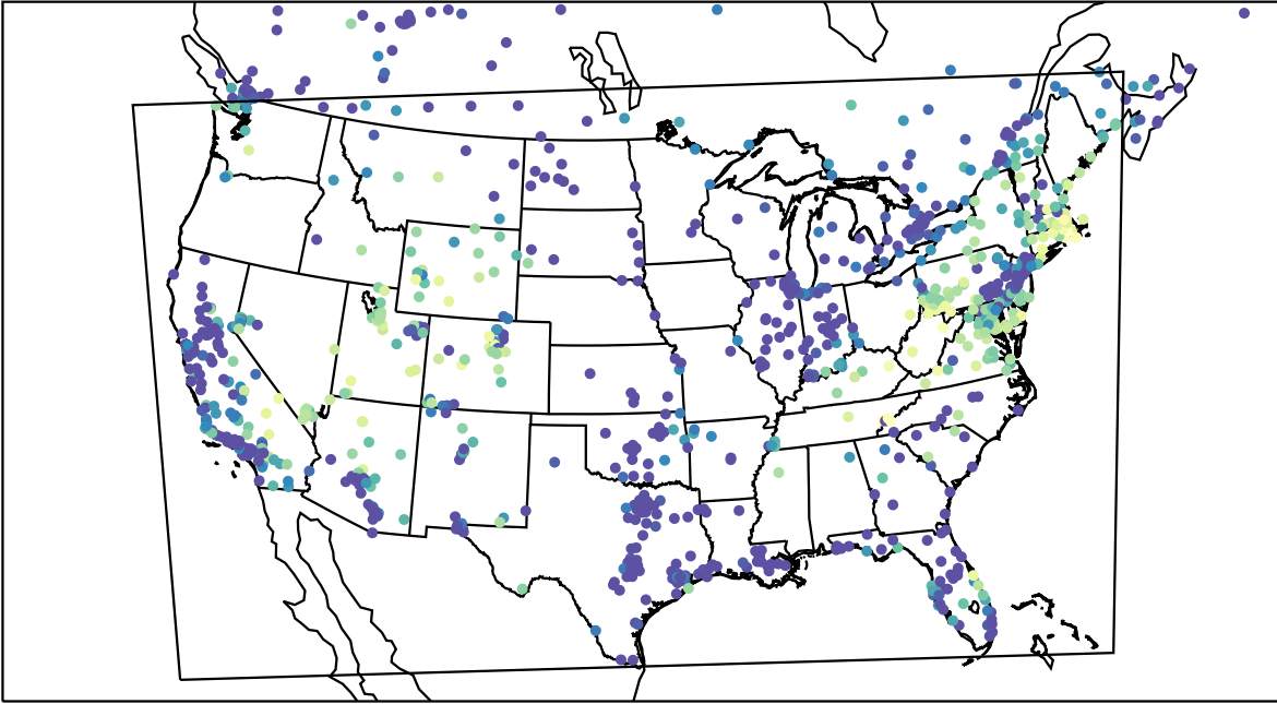
AirNOW (2023-11-07_11:00:00)
