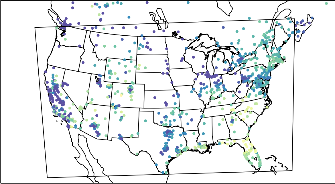
AirNOW (2023-11-08_15:00:00)
