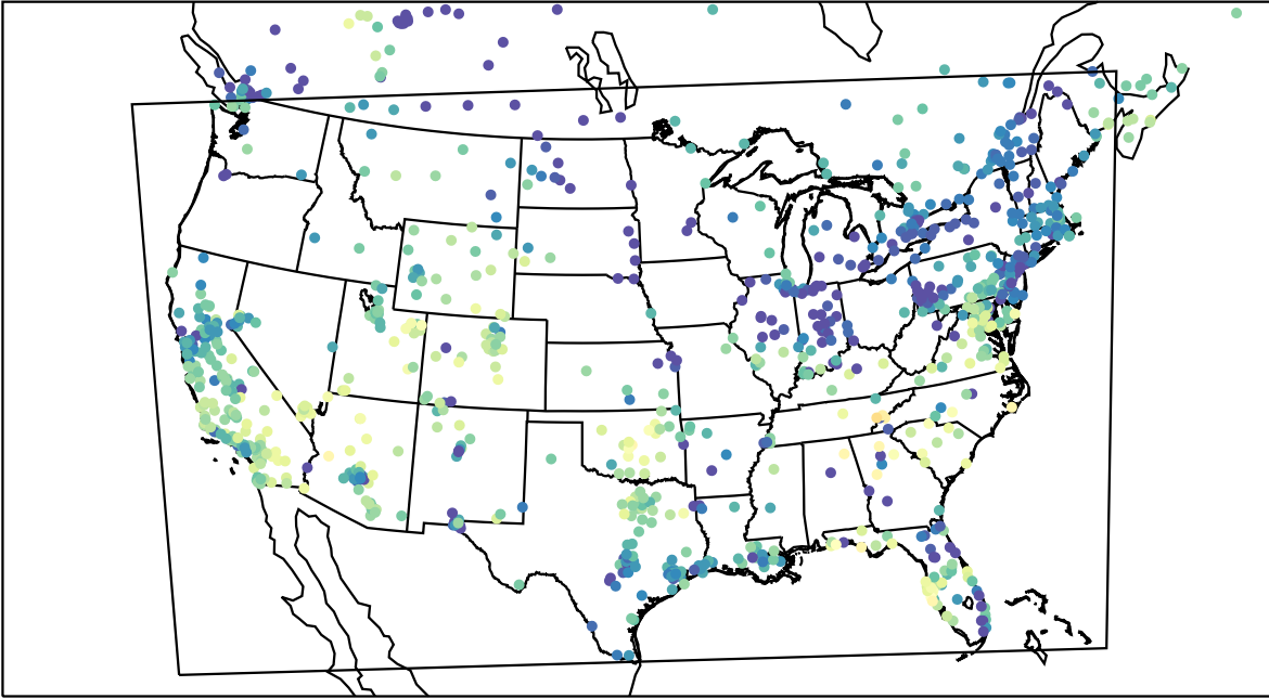
AirNOW (2023-11-08_01:00:00)
