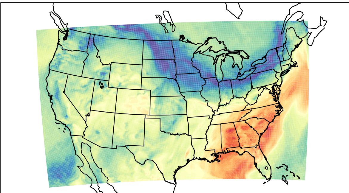
WRF (2023-11-07_19:00:00)
