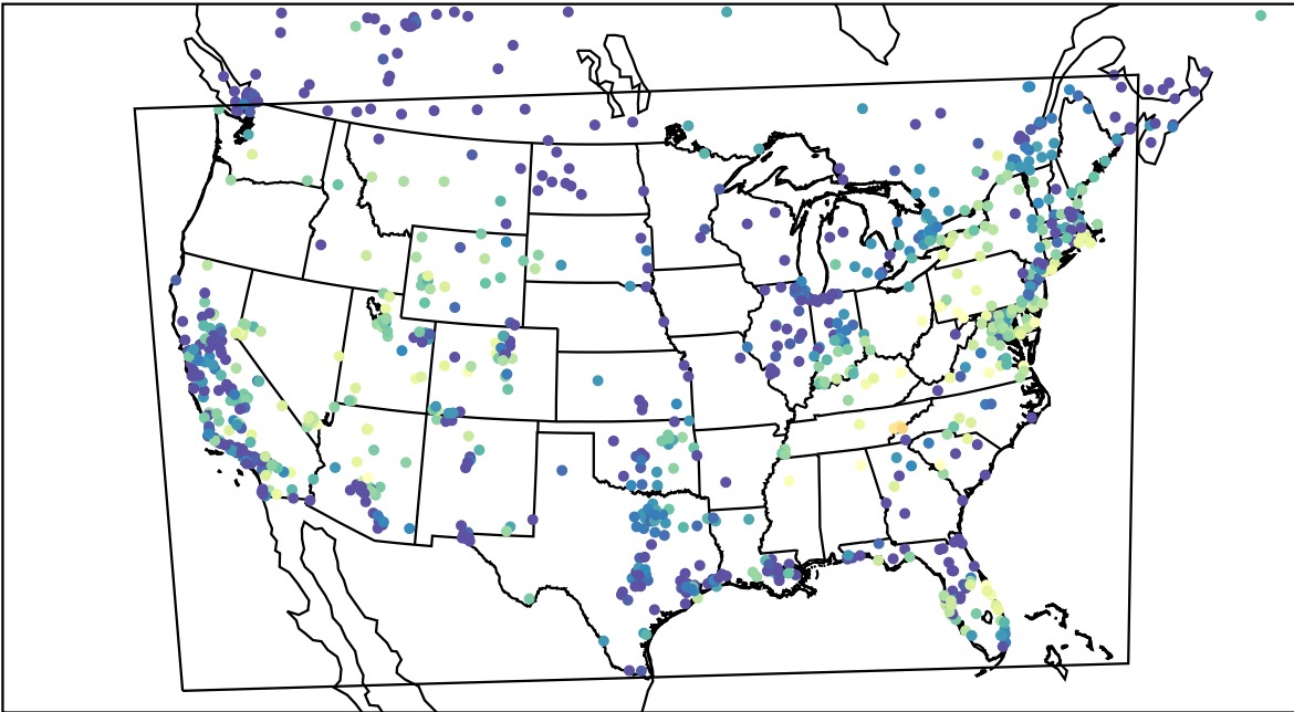
AirNOW (2023-11-07_06:00:00)
