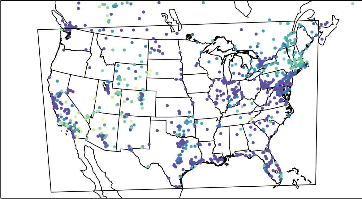
AirNOW (2023-11-08_12:00:00)
