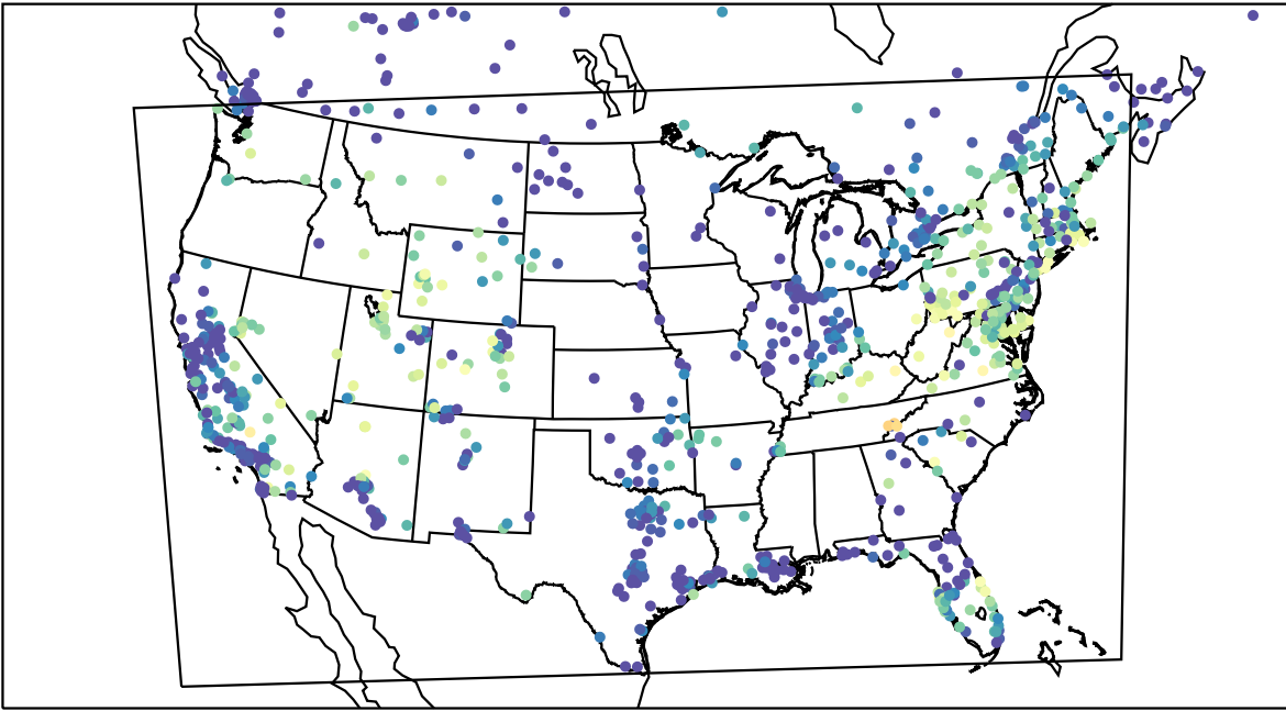
AirNOW (2023-11-07_08:00:00)
