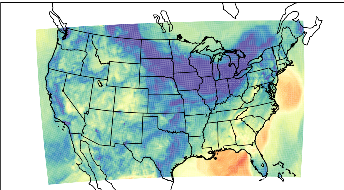
WRF (2023-11-07_08:00:00)
