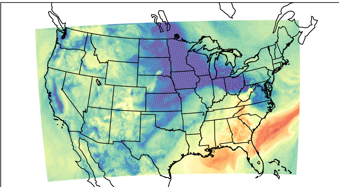
WRF (2023-11-08_16:00:00)
