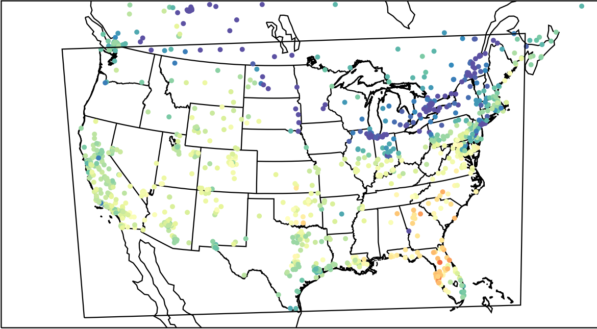
AirNOW (2023-11-07_21:00:00)
