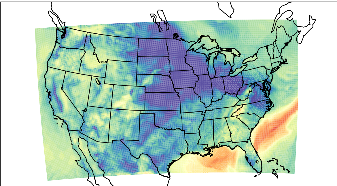
WRF (2023-11-08_14:00:00)
