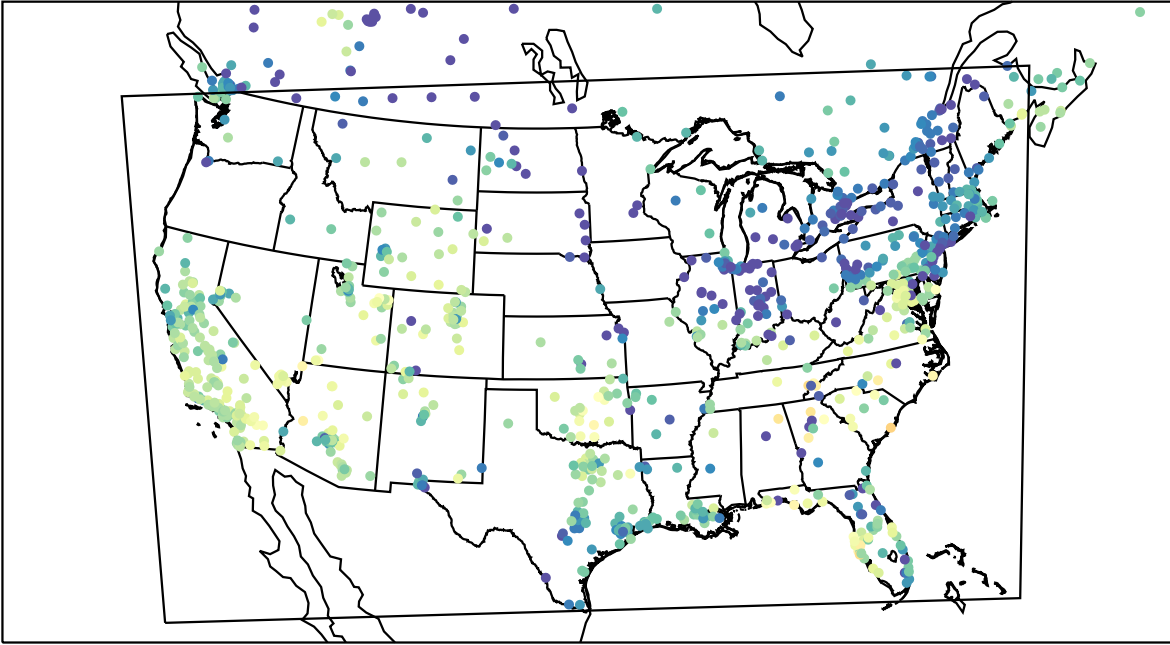
AirNOW (2023-11-08_00:00:00)
