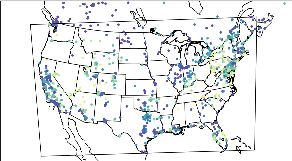
AirNOW (2023-11-07_05:00:00)
