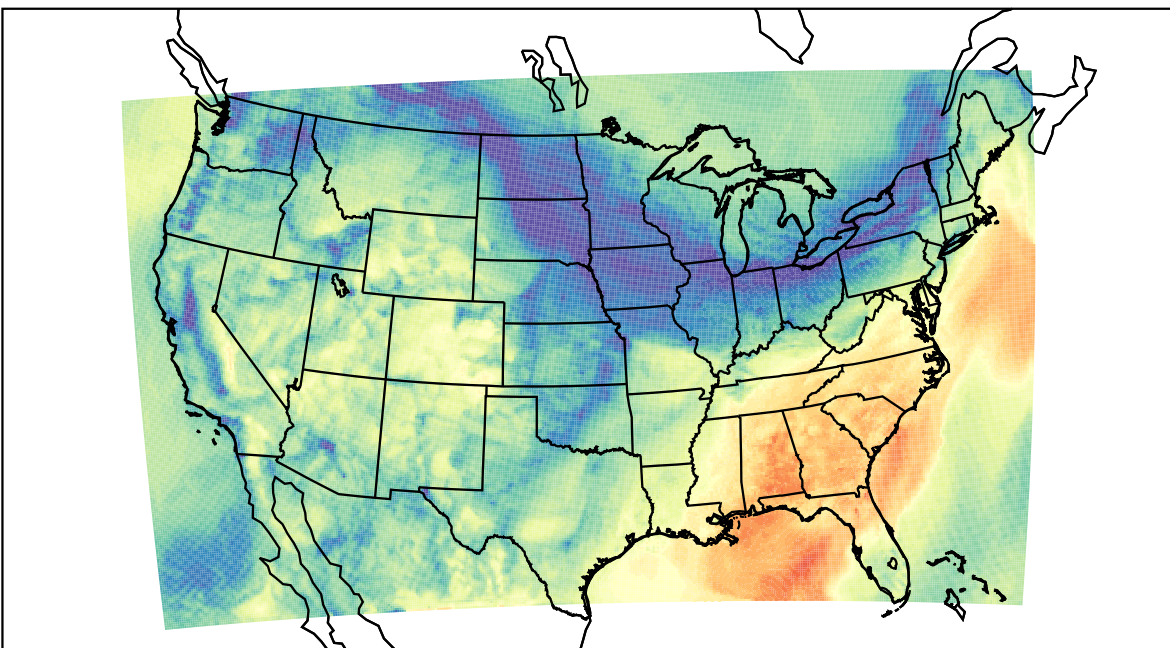
WRF (2023-11-07_17:00:00)
