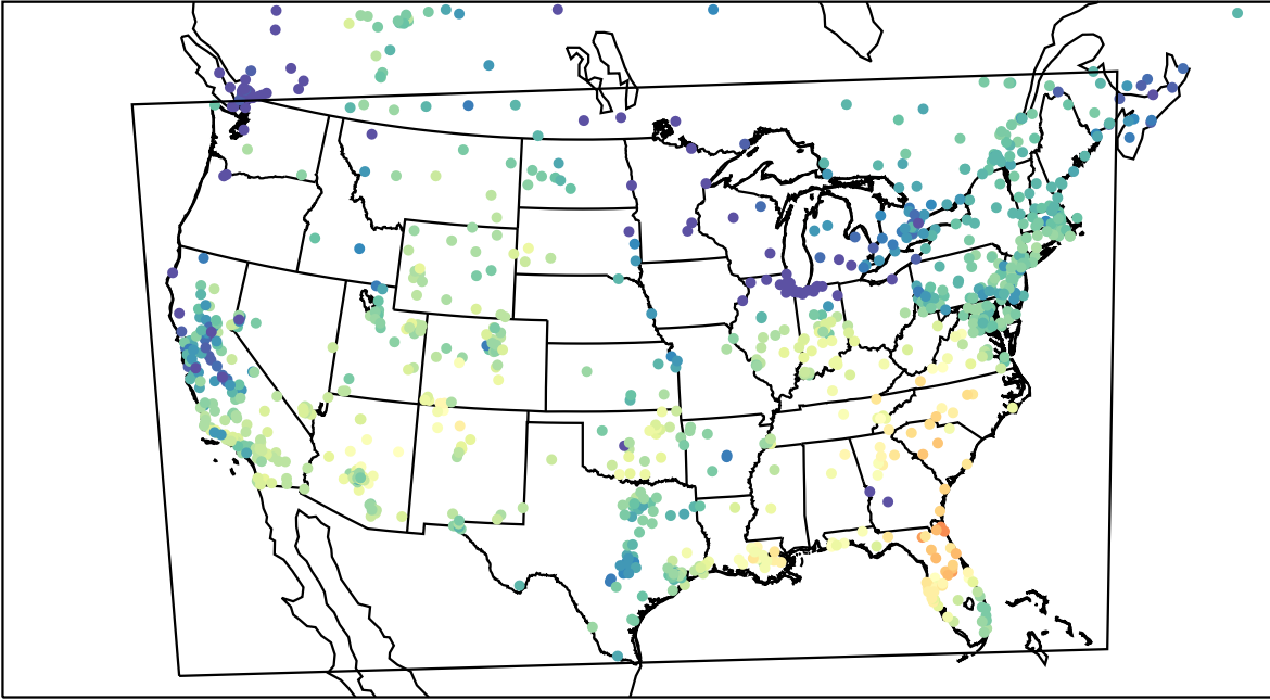
AirNOW (2023-11-08_18:00:00)
