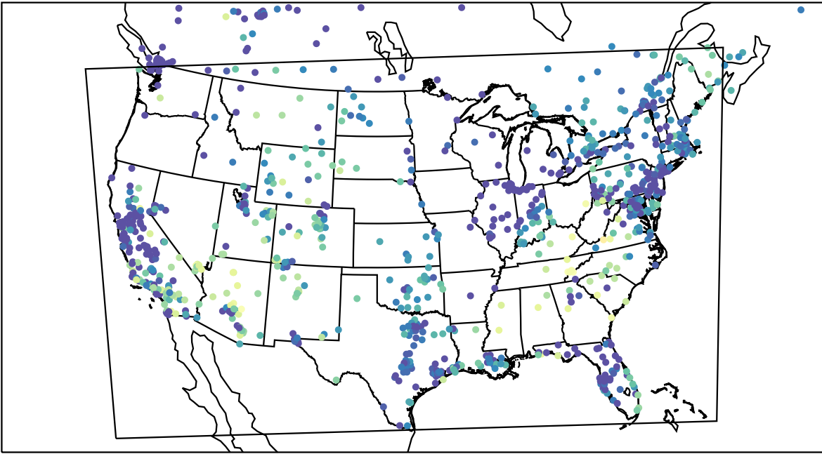
AirNOW (2023-11-09_05:00:00)
