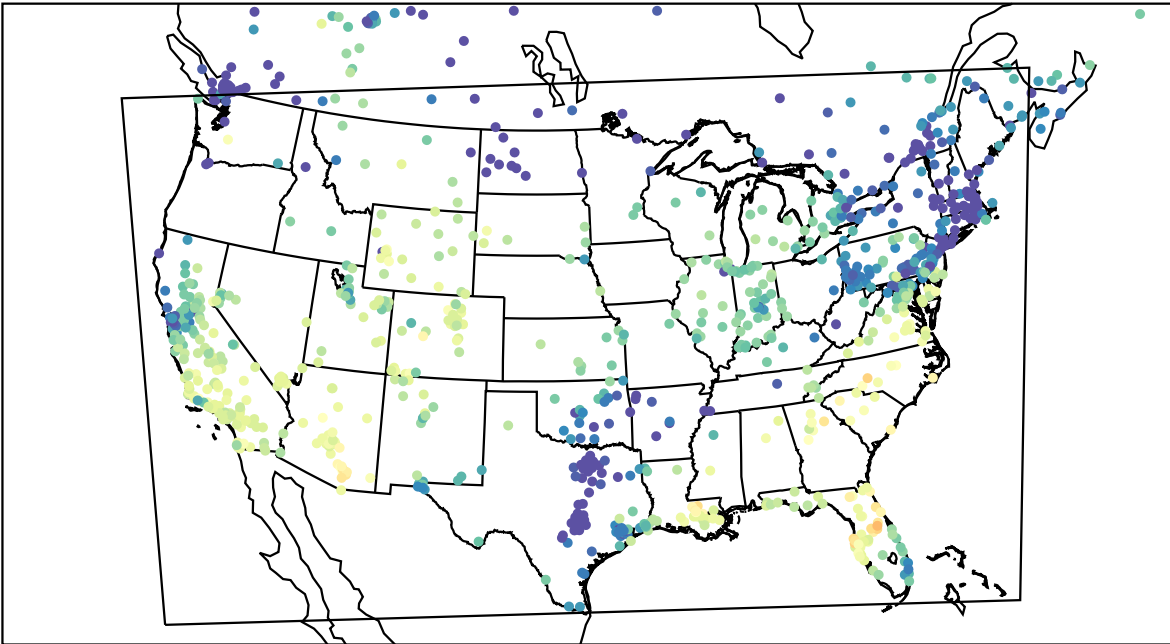
AirNOW (2023-11-09_20:00:00)
