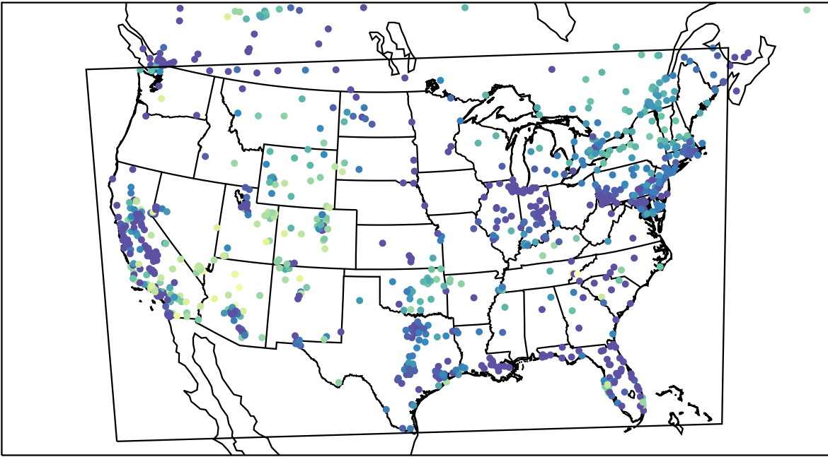
AirNOW (2023-11-08_09:00:00)
