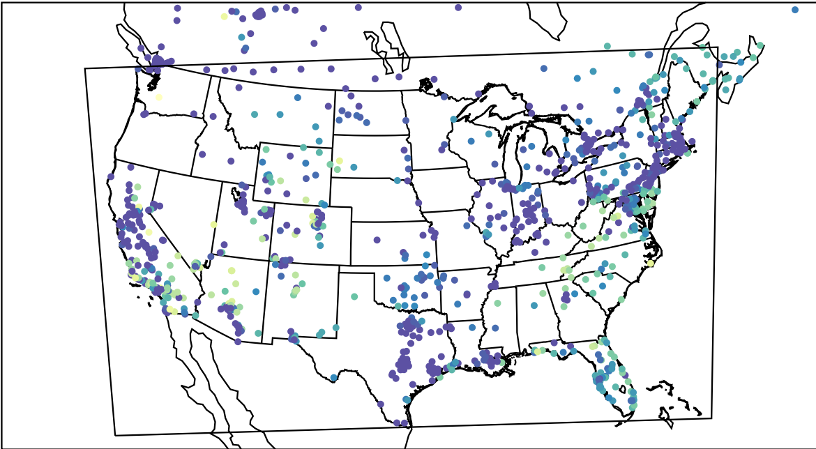
AirNOW (2023-11-09_14:00:00)
