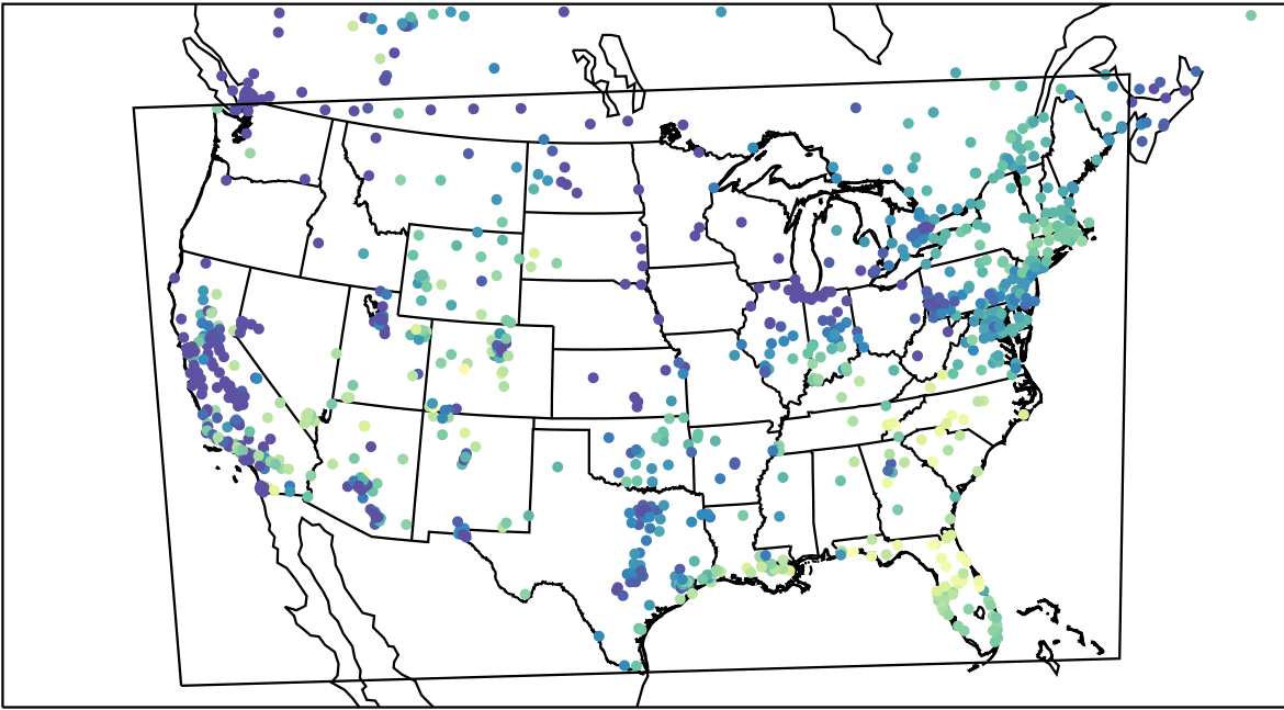
AirNOW (2023-11-08_15:00:00)
