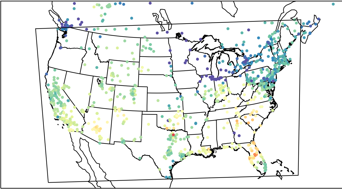
AirNOW (2023-11-08_21:00:00)
