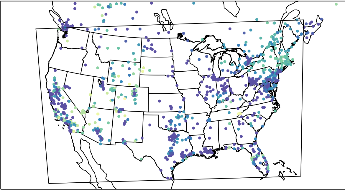
AirNOW (2023-11-08_13:00:00)
