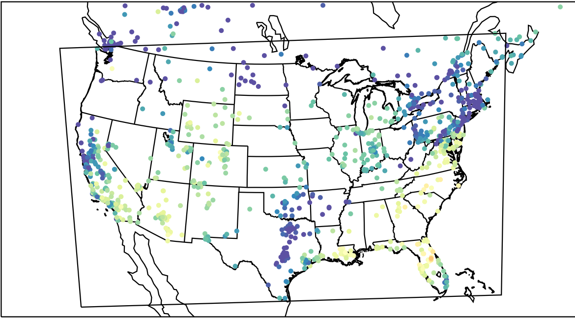
AirNOW (2023-11-09_18:00:00)
