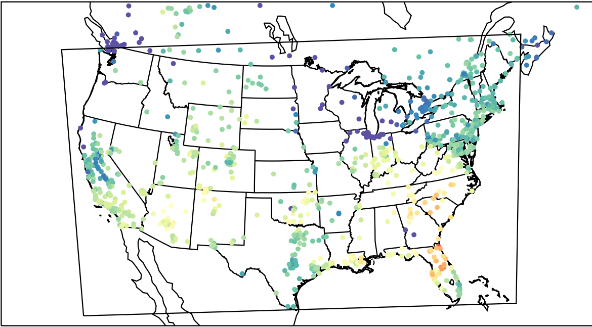
AirNOW (2023-11-08_19:00:00)
