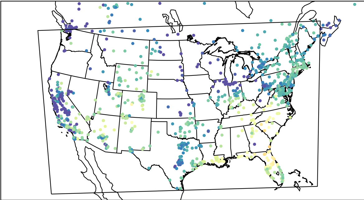
AirNOW (2023-11-08_16:00:00)
