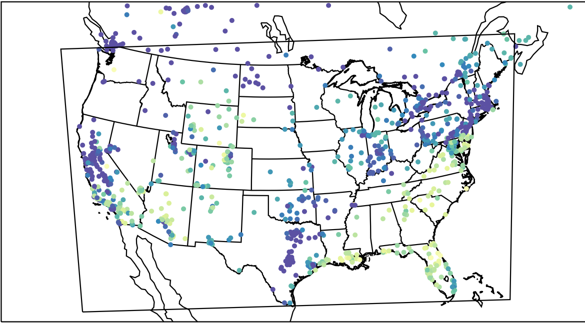
AirNOW (2023-11-09_16:00:00)
