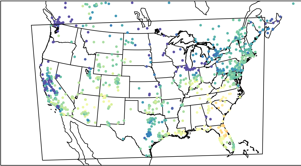
AirNOW (2023-11-08_17:00:00)
