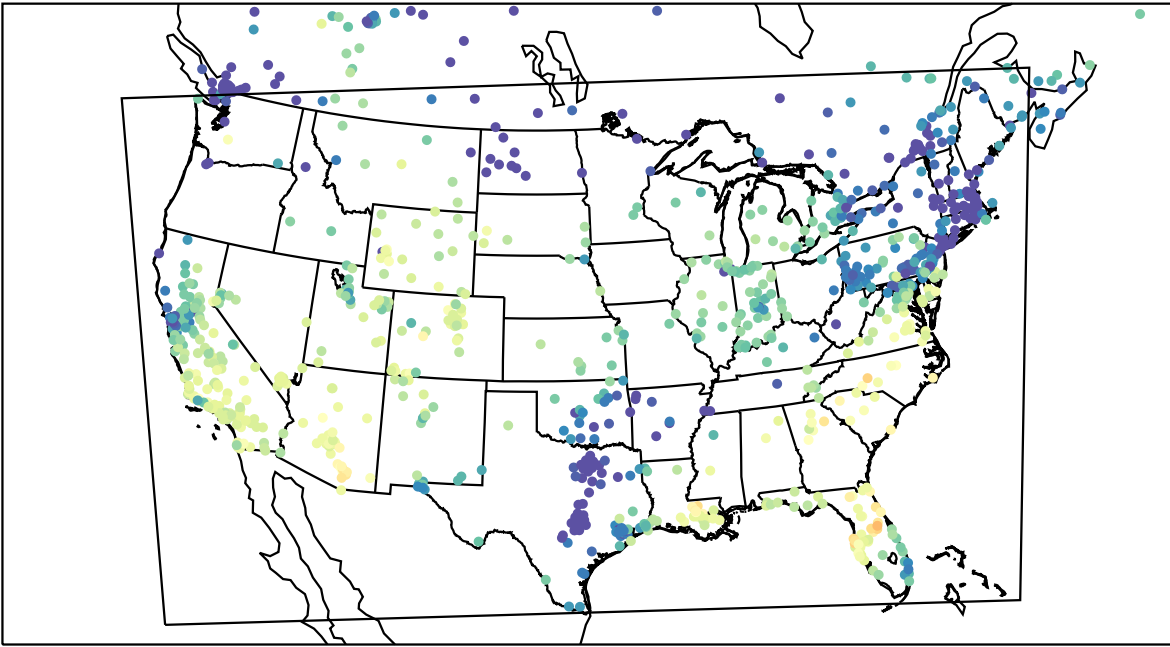
AirNOW (2023-11-09_20:00:00)
