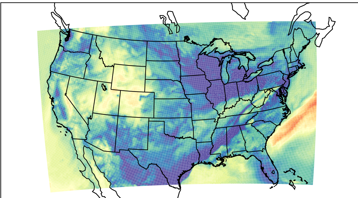
WRF (2023-11-10_14:00:00)
