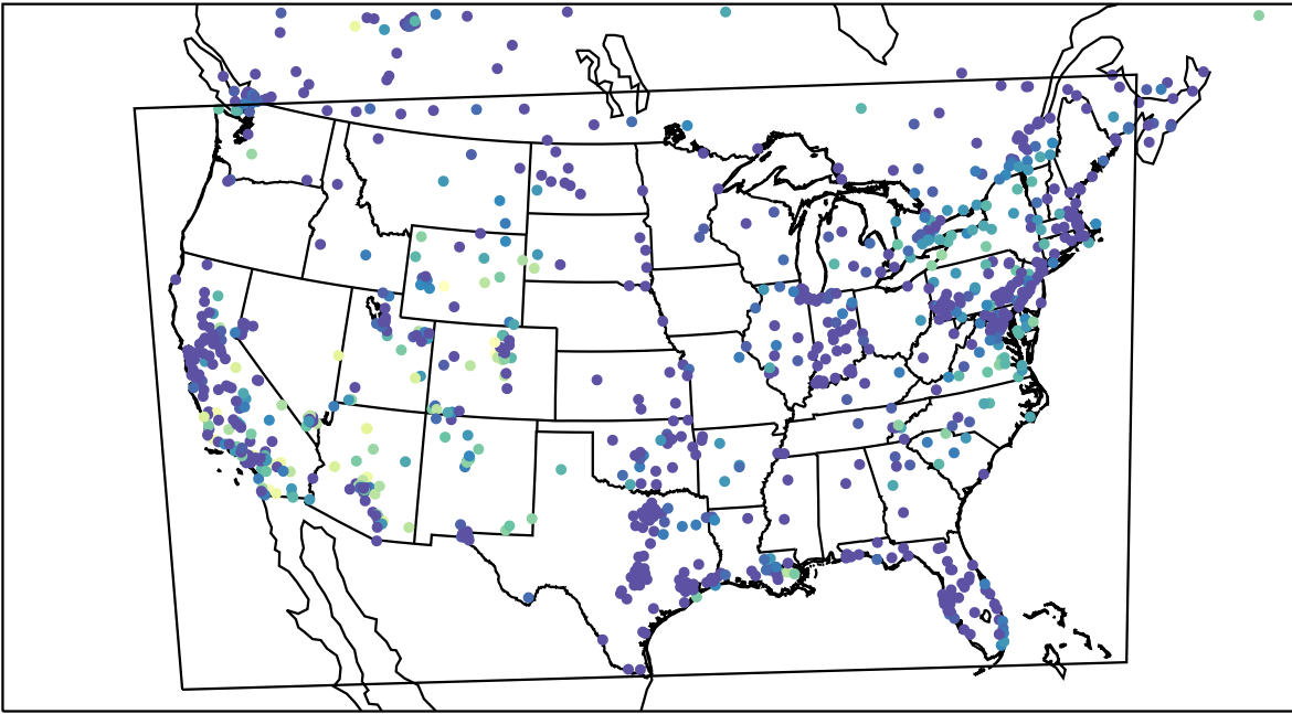
AirNOW (2023-11-10_09:00:00)
