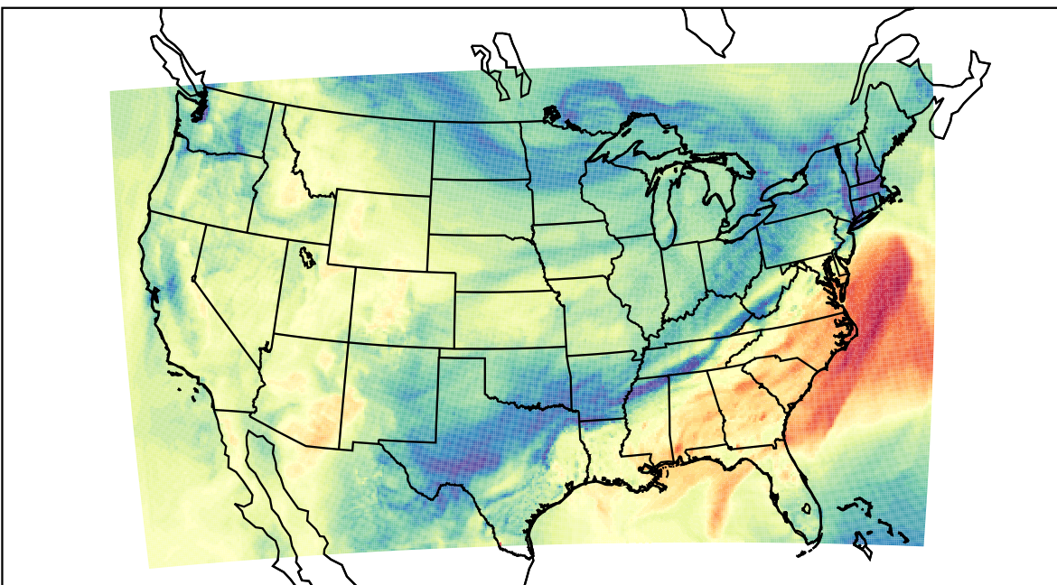
WRF (2023-11-09_20:00:00)
