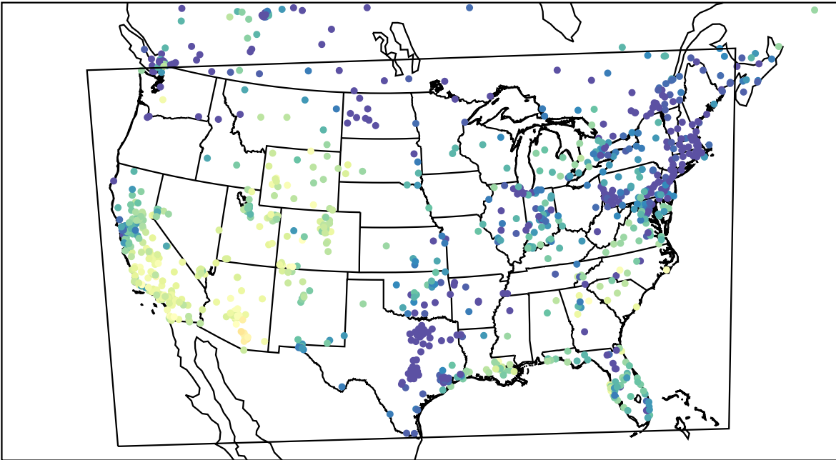
AirNOW (2023-11-09_23:00:00)
