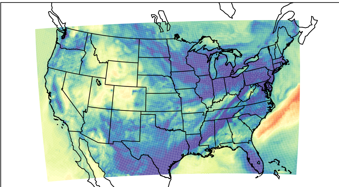
WRF (2023-11-10_12:00:00)
