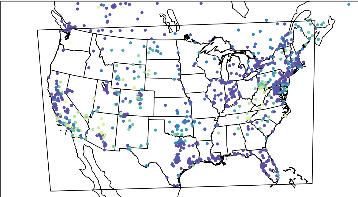
AirNOW (2023-11-09_11:00:00)
