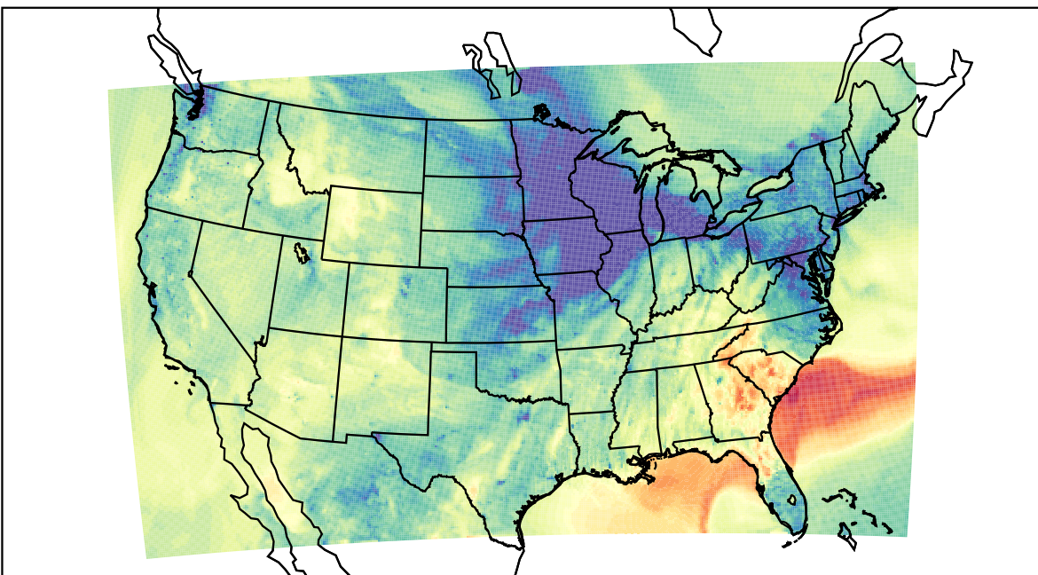
WRF (2023-11-09_00:00:00)
