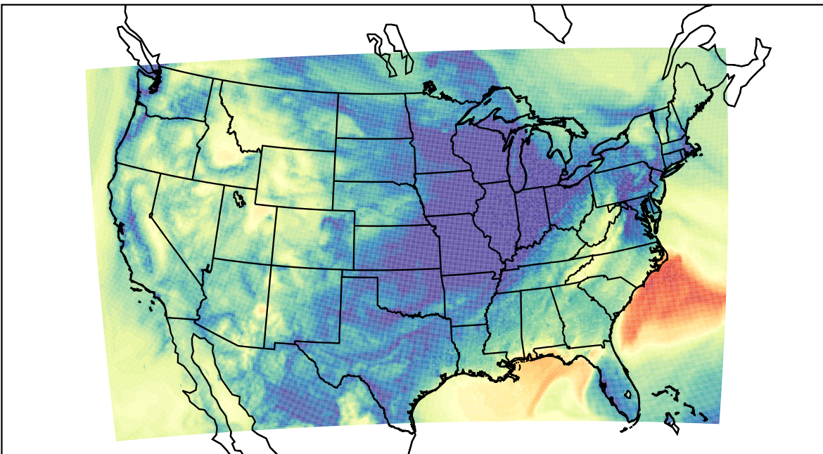
WRF (2023-11-09_10:00:00)
