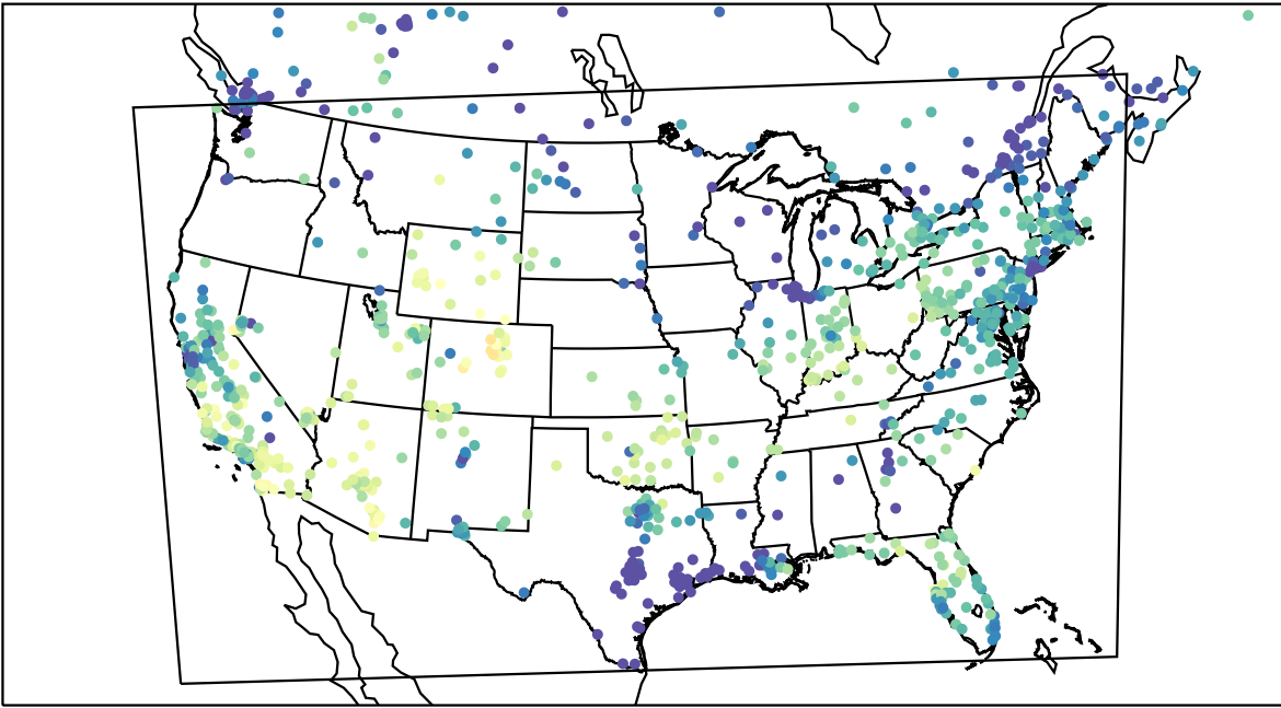
AirNOW (2023-11-10_19:00:00)
