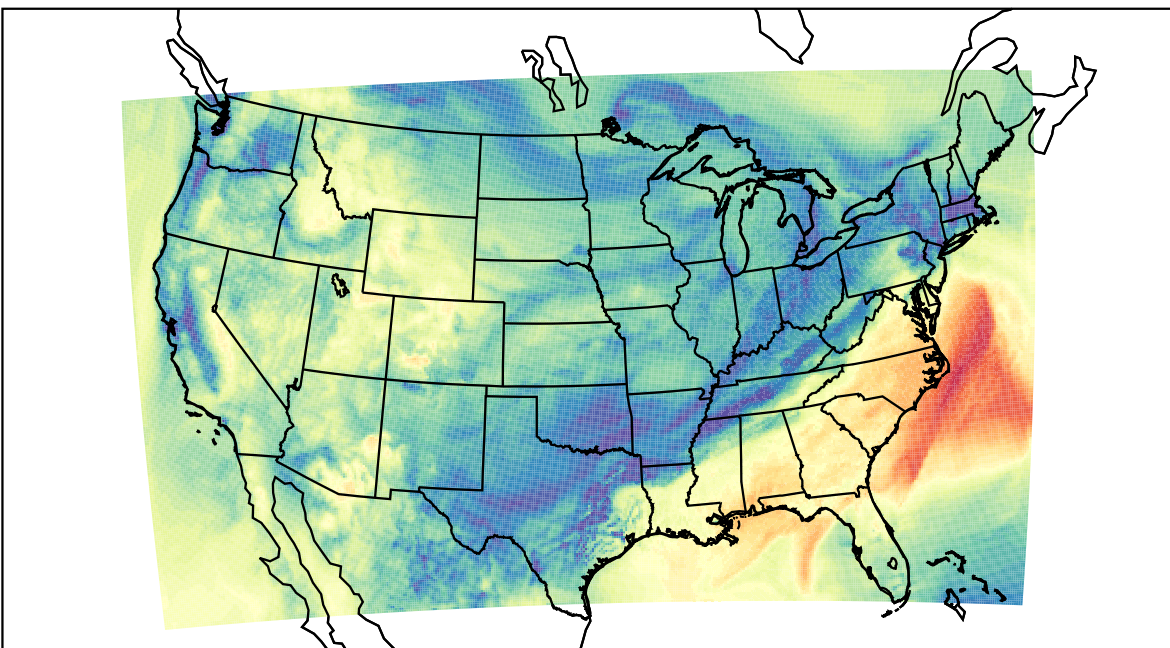
WRF (2023-11-09_17:00:00)
