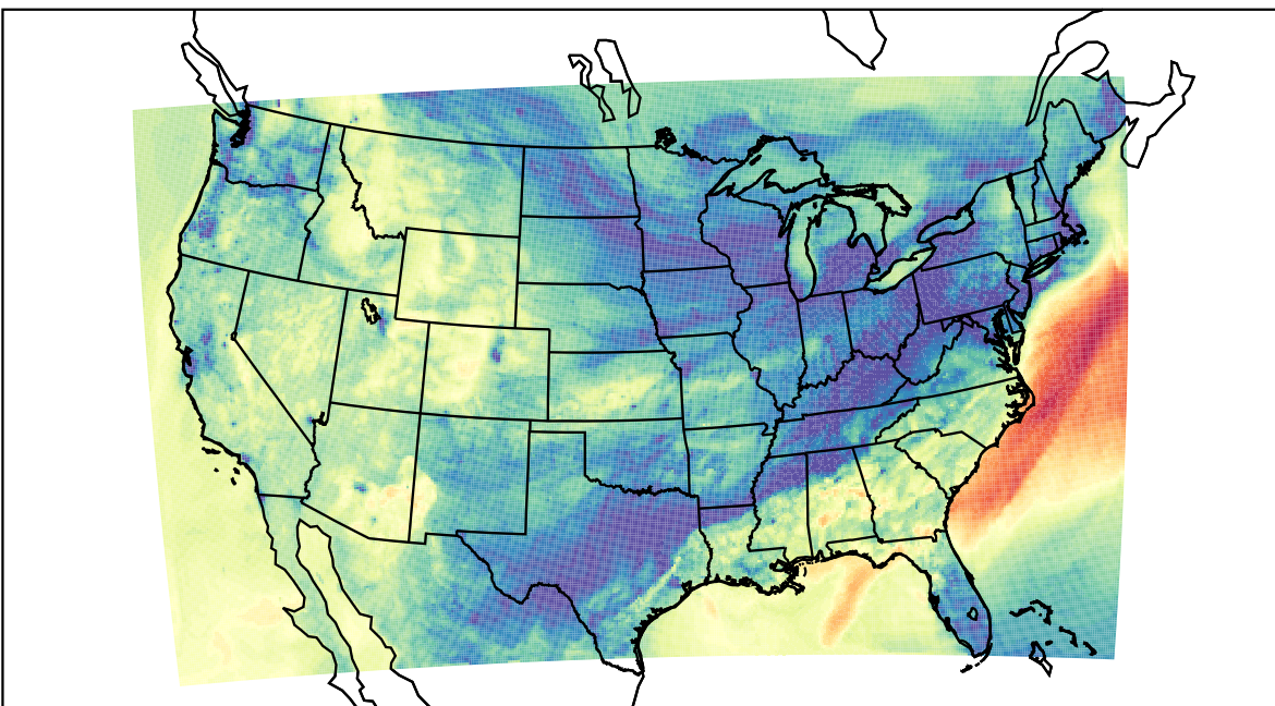
WRF (2023-11-10_01:00:00)
