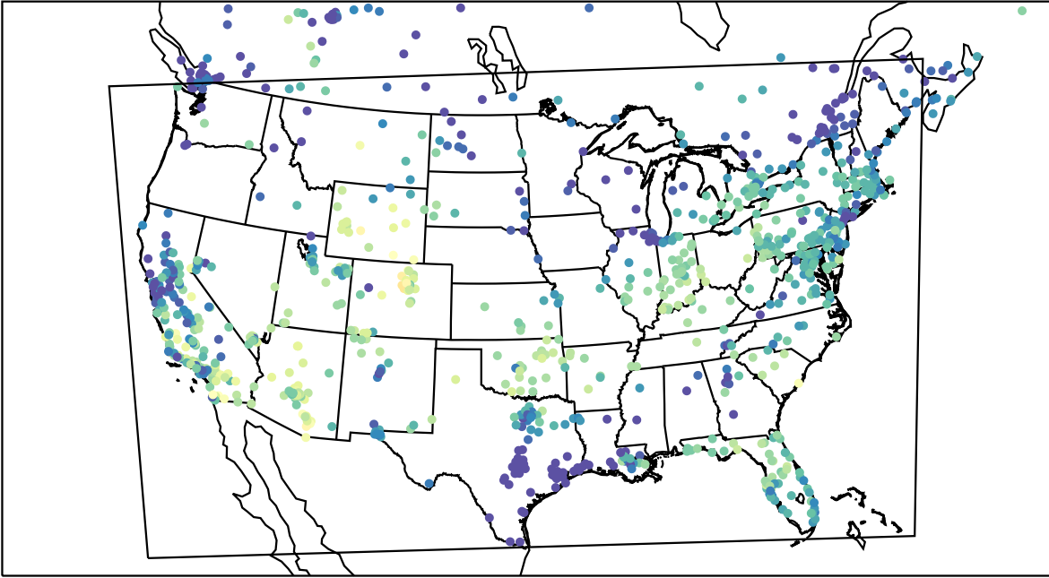
AirNOW (2023-11-10_18:00:00)
