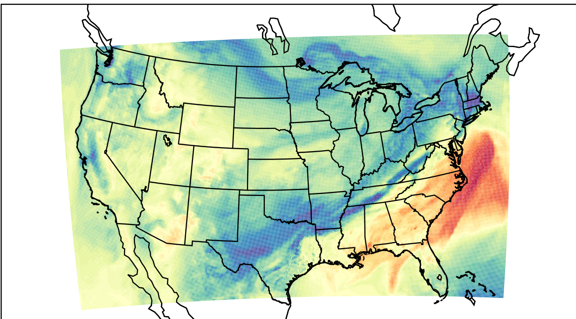
WRF (2023-11-09_19:00:00)
