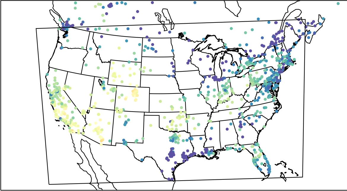
AirNOW (2023-11-10_21:00:00)
