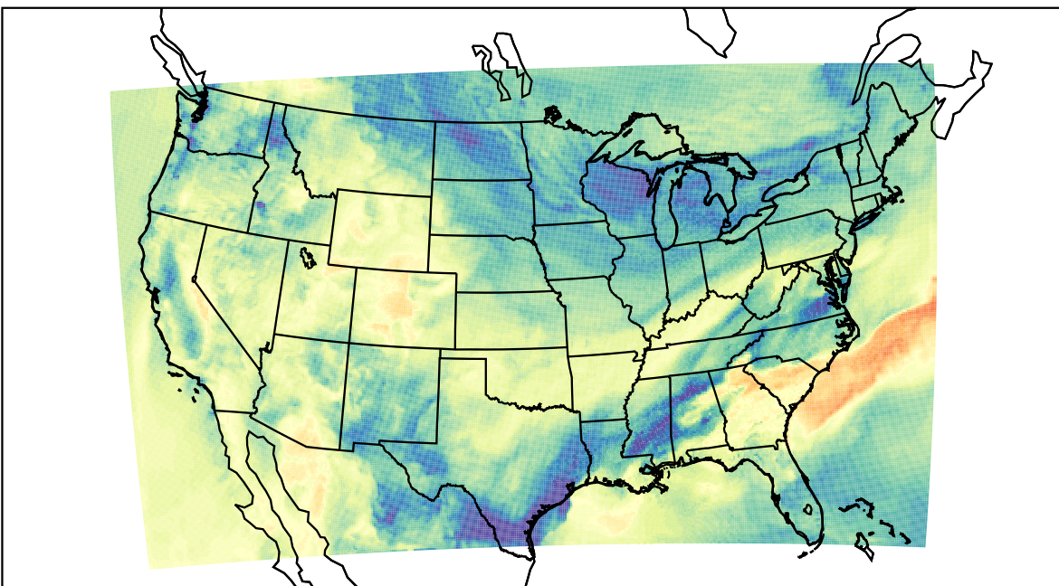
WRF (2023-11-10_19:00:00)
