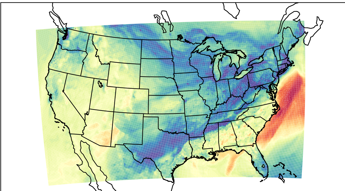
WRF (2023-11-09_23:00:00)
