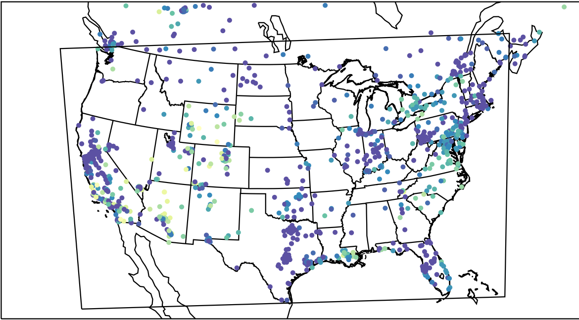
AirNOW (2023-11-10_05:00:00)
