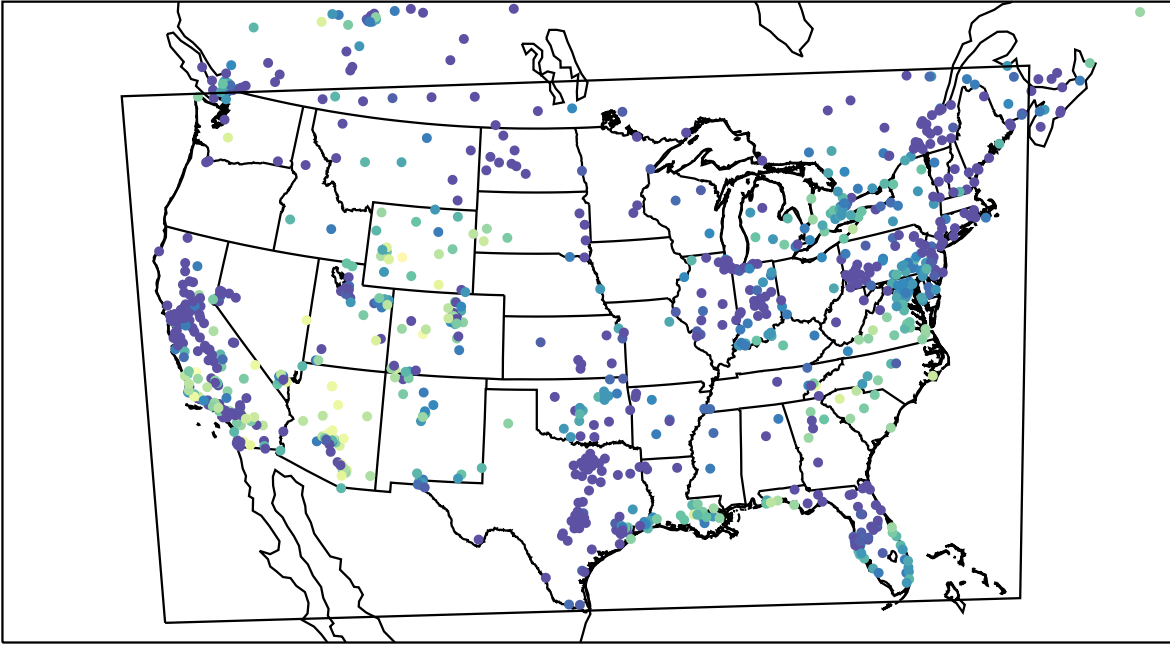
AirNOW (2023-11-10_03:00:00)
