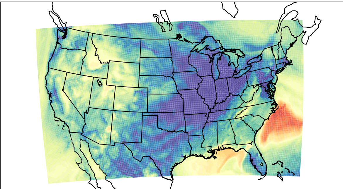
WRF (2023-11-09_12:00:00)
