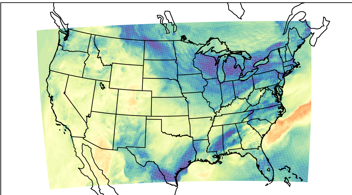
WRF (2023-11-10_22:00:00)
