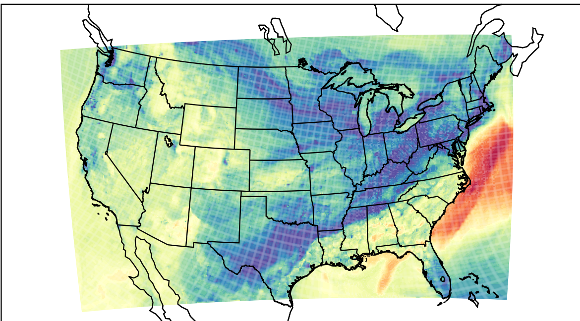
WRF (2023-11-10_00:00:00)
