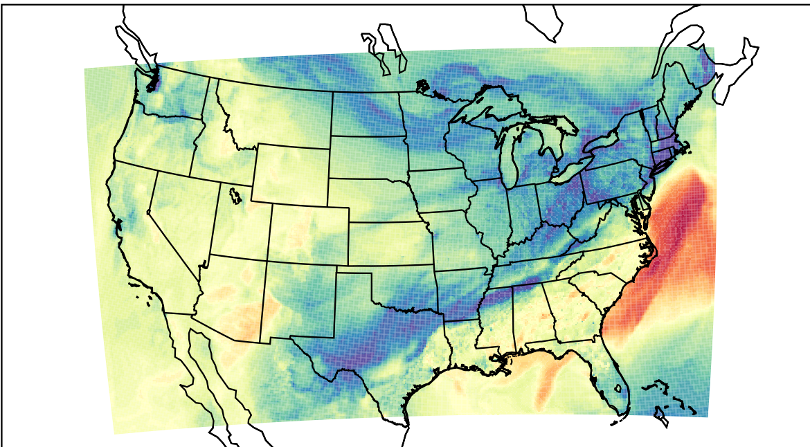
WRF (2023-11-09_22:00:00)
