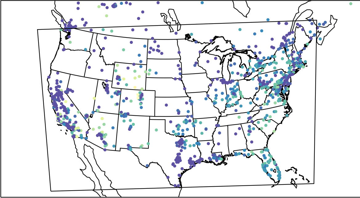
AirNOW (2023-11-10_15:00:00)
