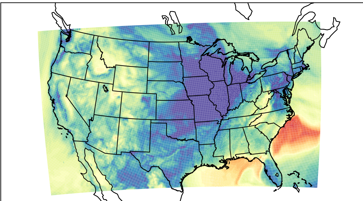
WRF (2023-11-09_08:00:00)
