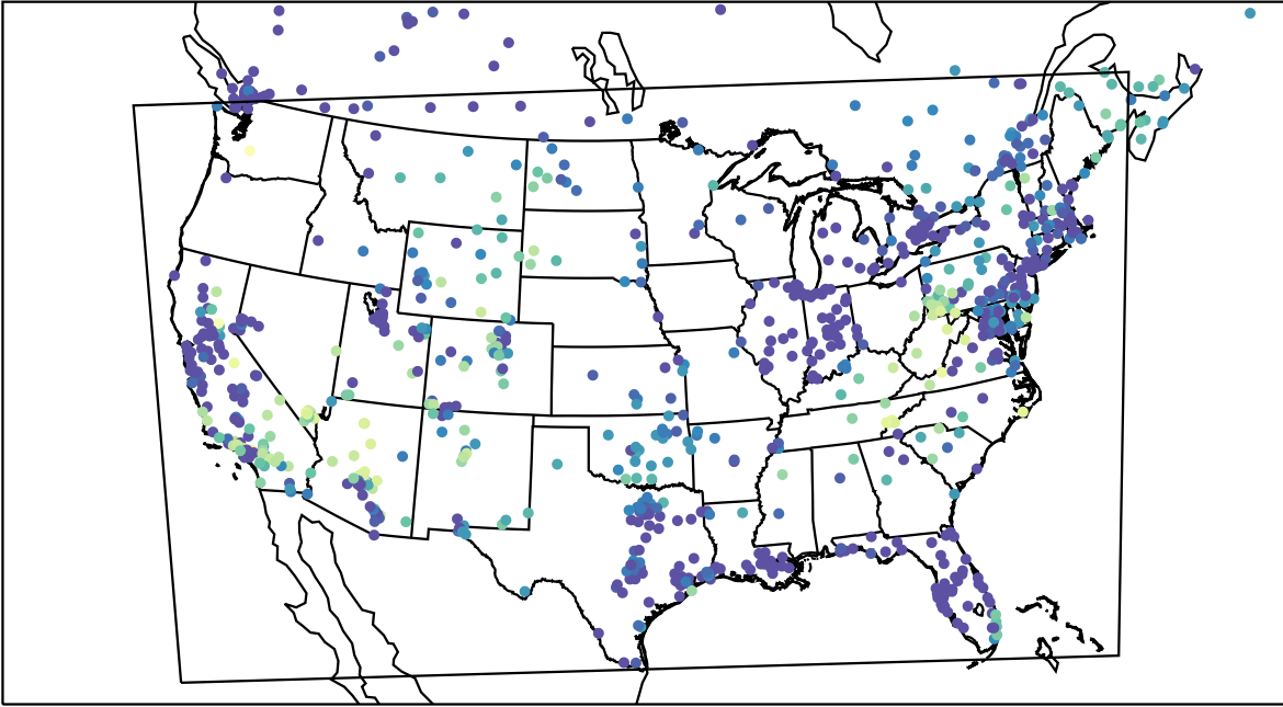
AirNOW (2023-11-09_10:00:00)
