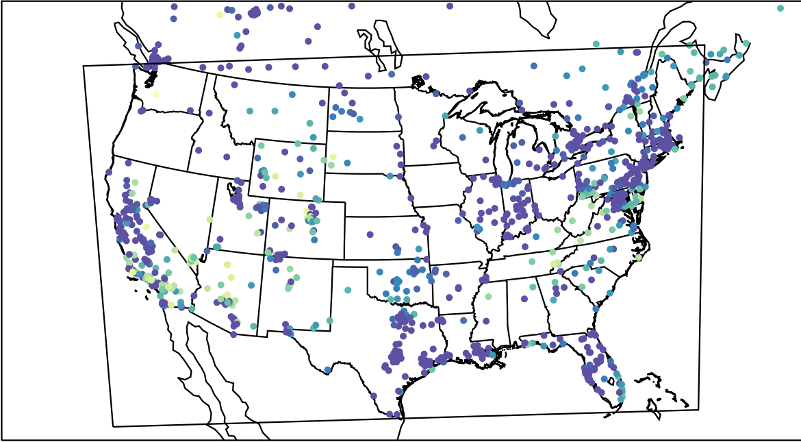
AirNOW (2023-11-09_13:00:00)
