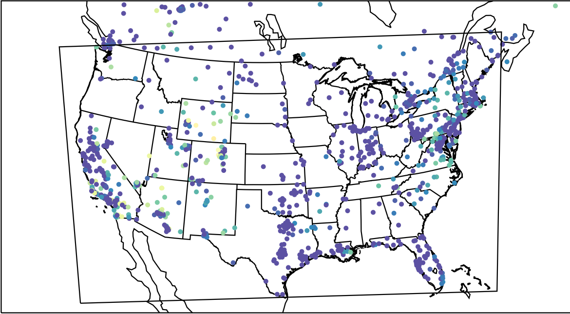
AirNOW (2023-11-10_13:00:00)
