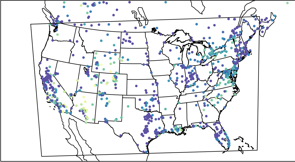
AirNOW (2023-11-10_06:00:00)
