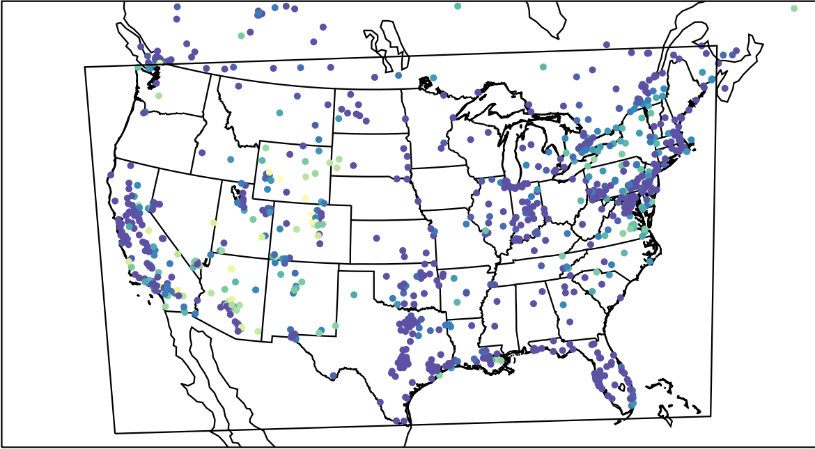
AirNOW (2023-11-10_10:00:00)
