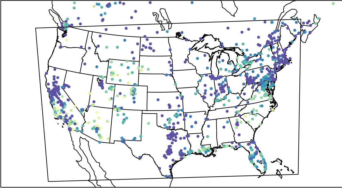
AirNOW (2023-11-10_02:00:00)
