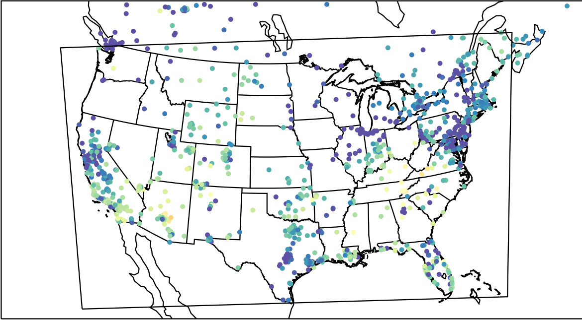
AirNOW (2023-11-09_01:00:00)
