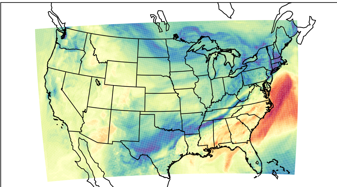
WRF (2023-11-09_21:00:00)
