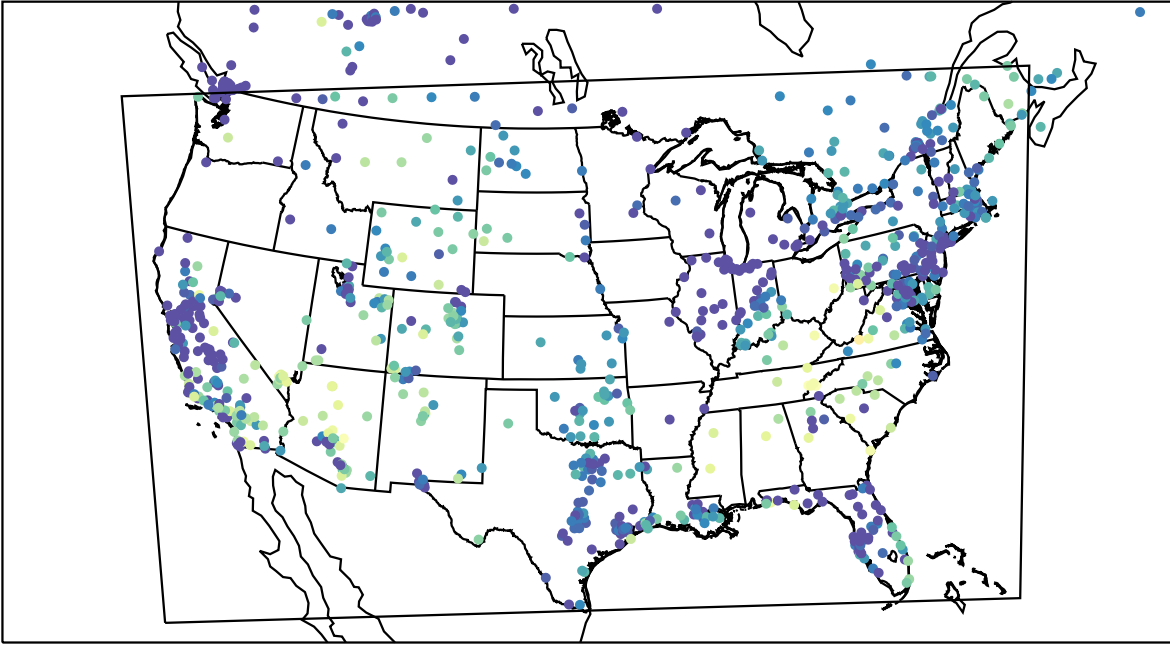
AirNOW (2023-11-09_05:00:00)
