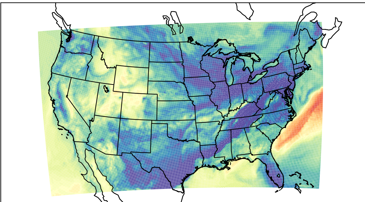
WRF (2023-11-10_09:00:00)
