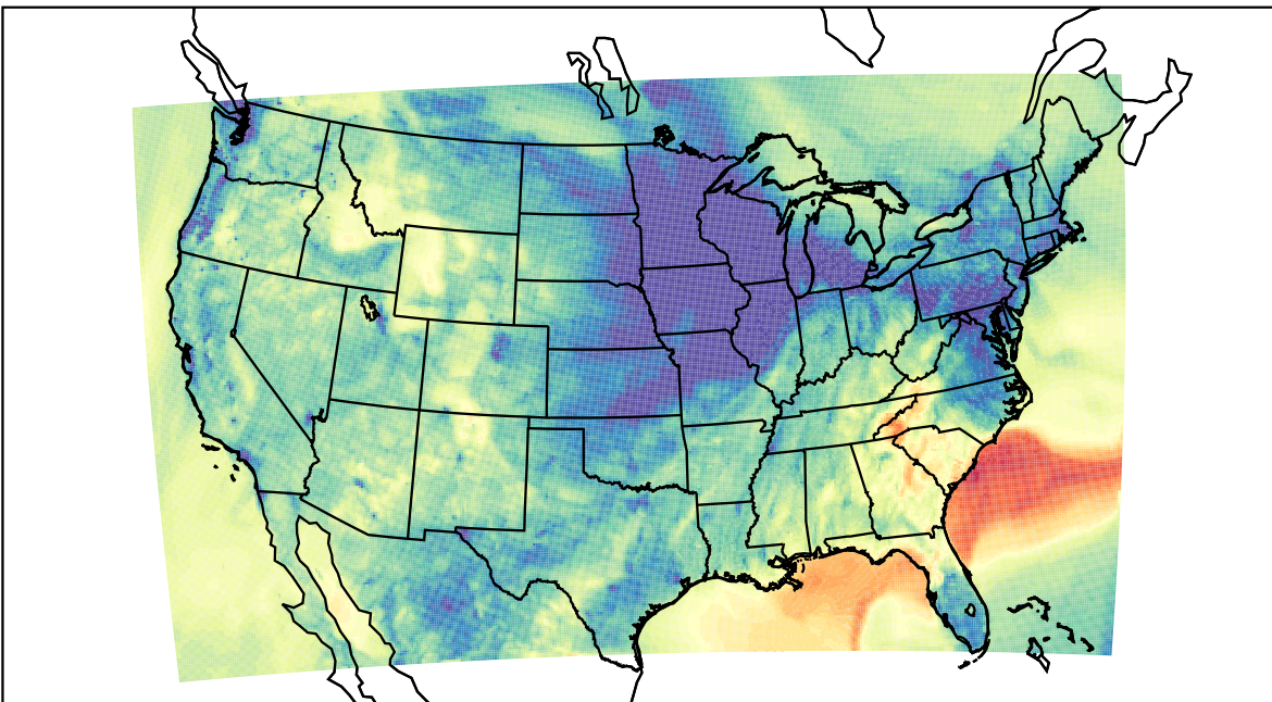
WRF (2023-11-09_02:00:00)
