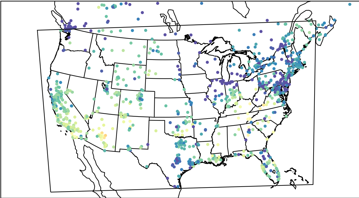
AirNOW (2023-11-09_00:00:00)
