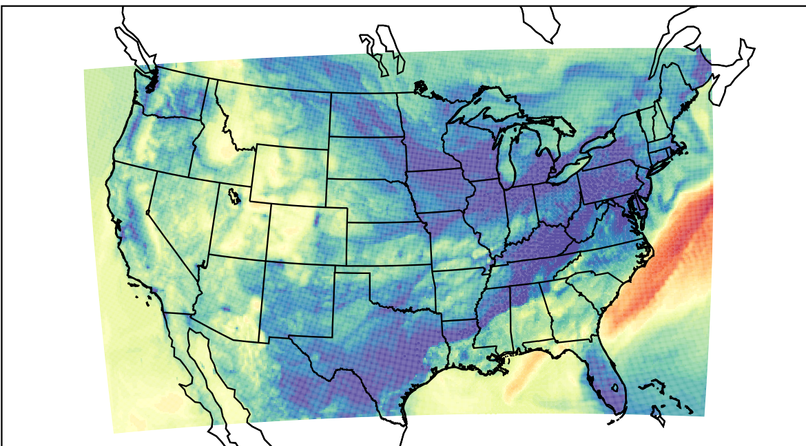
WRF (2023-11-10_05:00:00)
