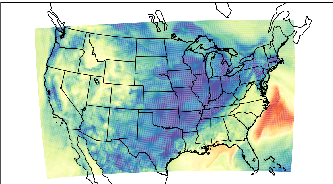
WRF (2023-11-09_15:00:00)
