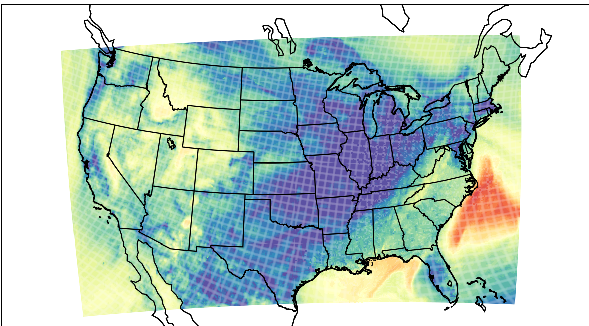
WRF (2023-11-09_14:00:00)
