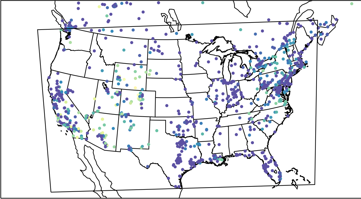
AirNOW (2023-11-10_11:00:00)
