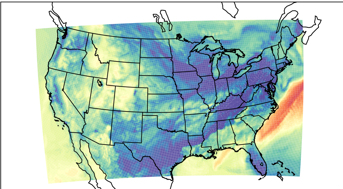
WRF (2023-11-10_06:00:00)
