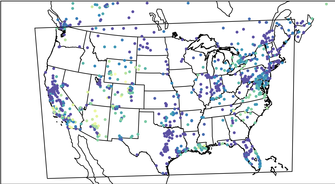
AirNOW (2023-11-10_04:00:00)
