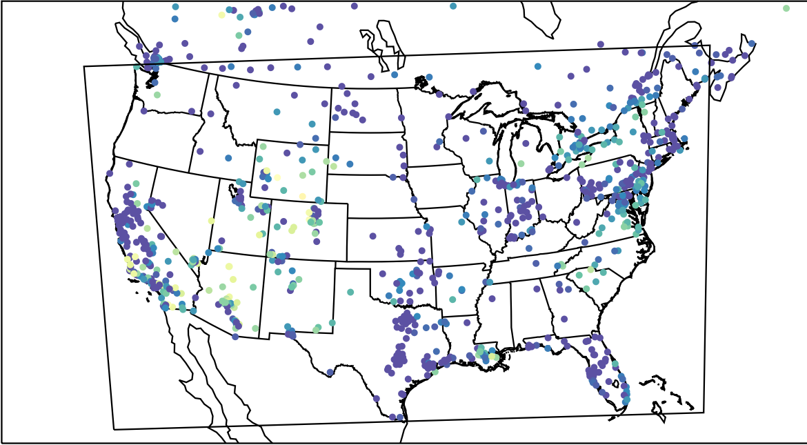
AirNOW (2023-11-10_07:00:00)
