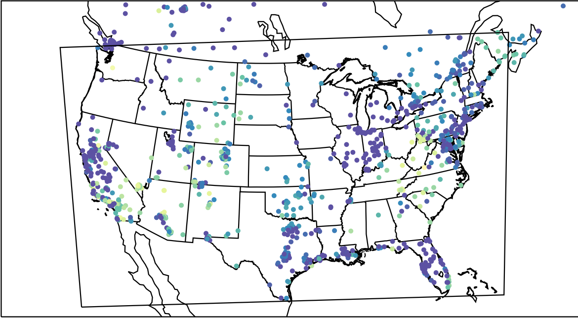
AirNOW (2023-11-09_08:00:00)
