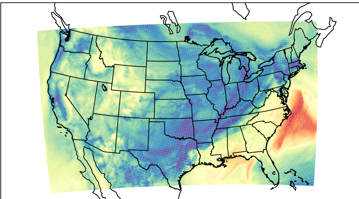
WRF (2023-11-09_16:00:00)
