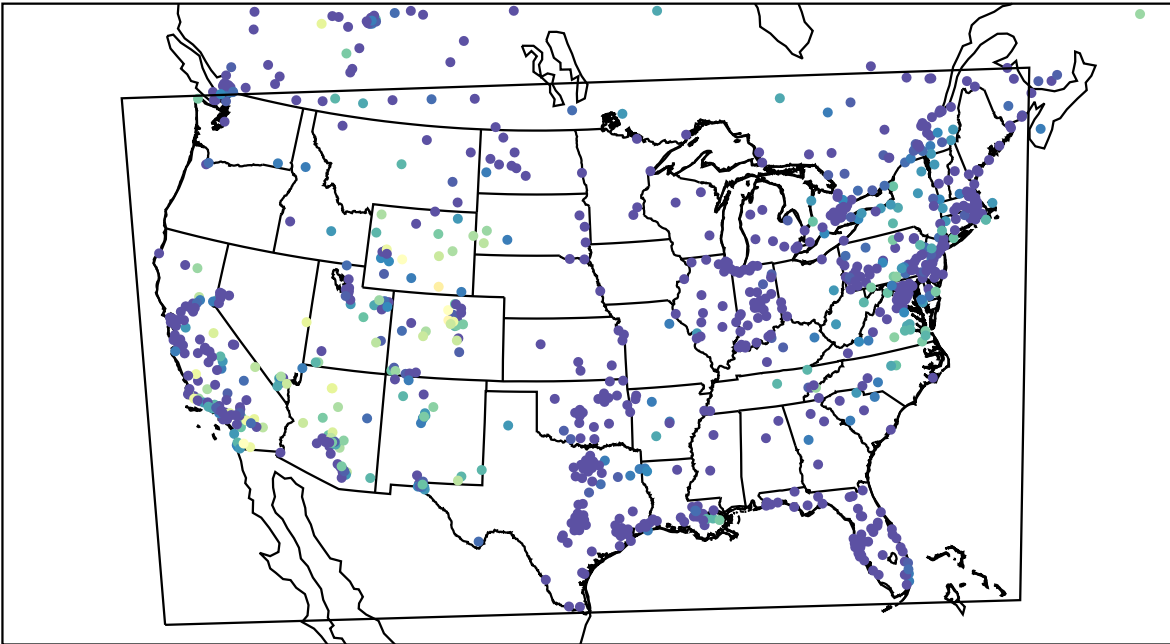
AirNOW (2023-11-10_12:00:00)
