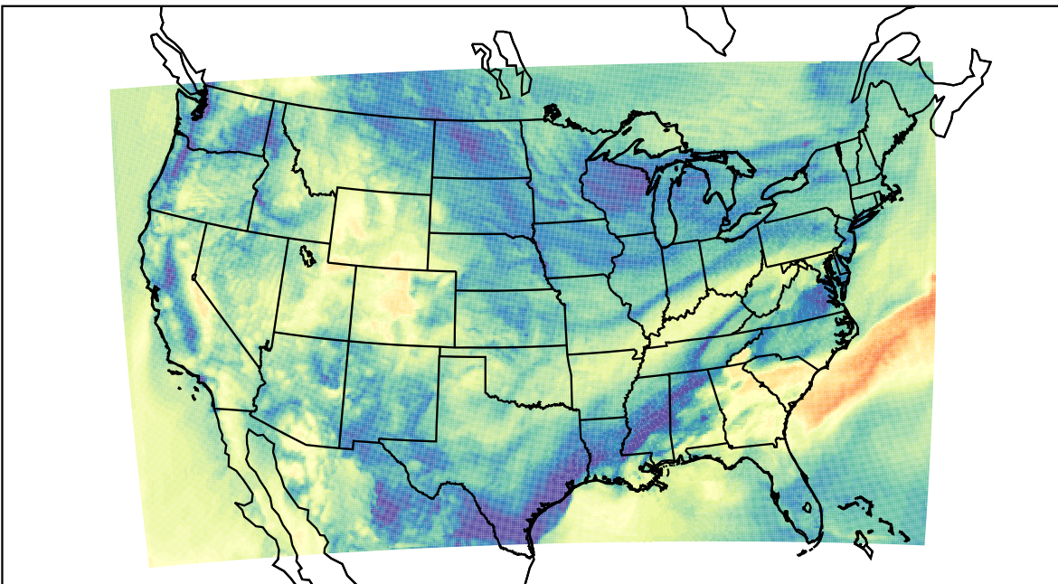
WRF (2023-11-10_17:00:00)
