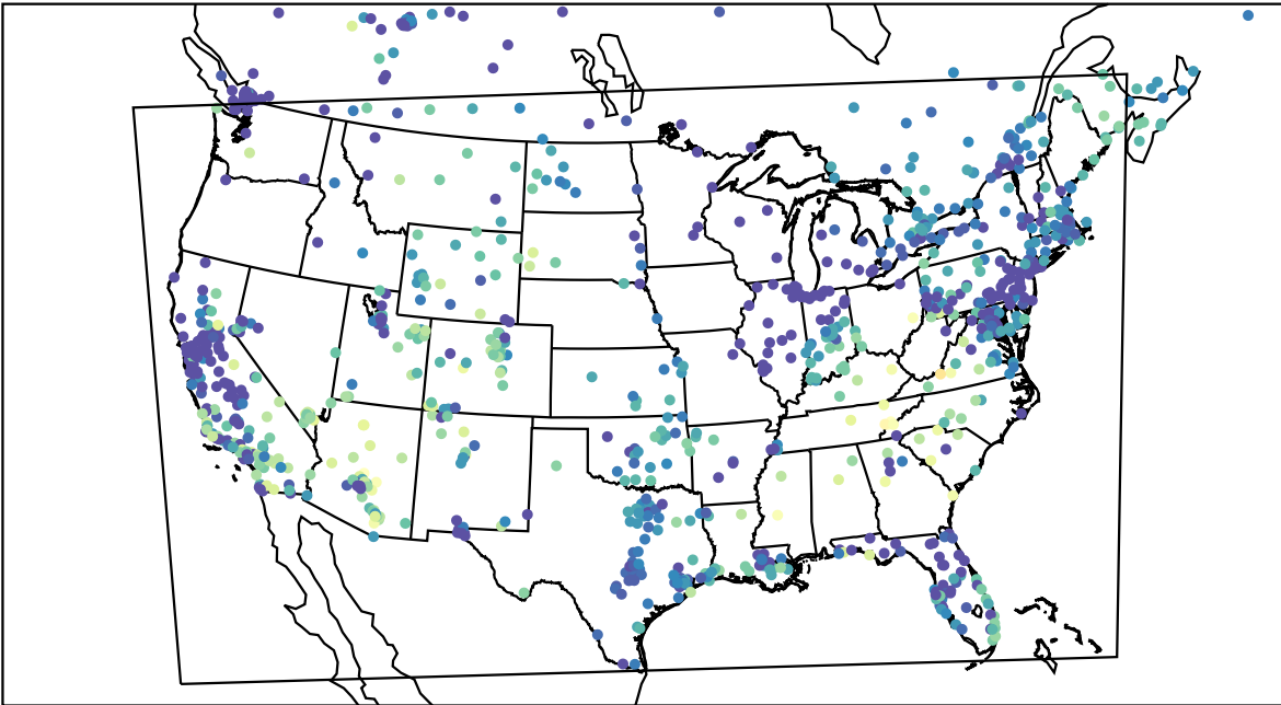
AirNOW (2023-11-09_04:00:00)
