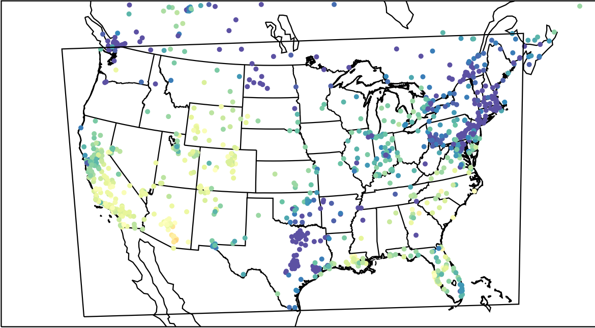
AirNOW (2023-11-09_22:00:00)
