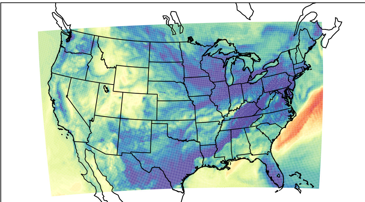
WRF (2023-11-10_08:00:00)
