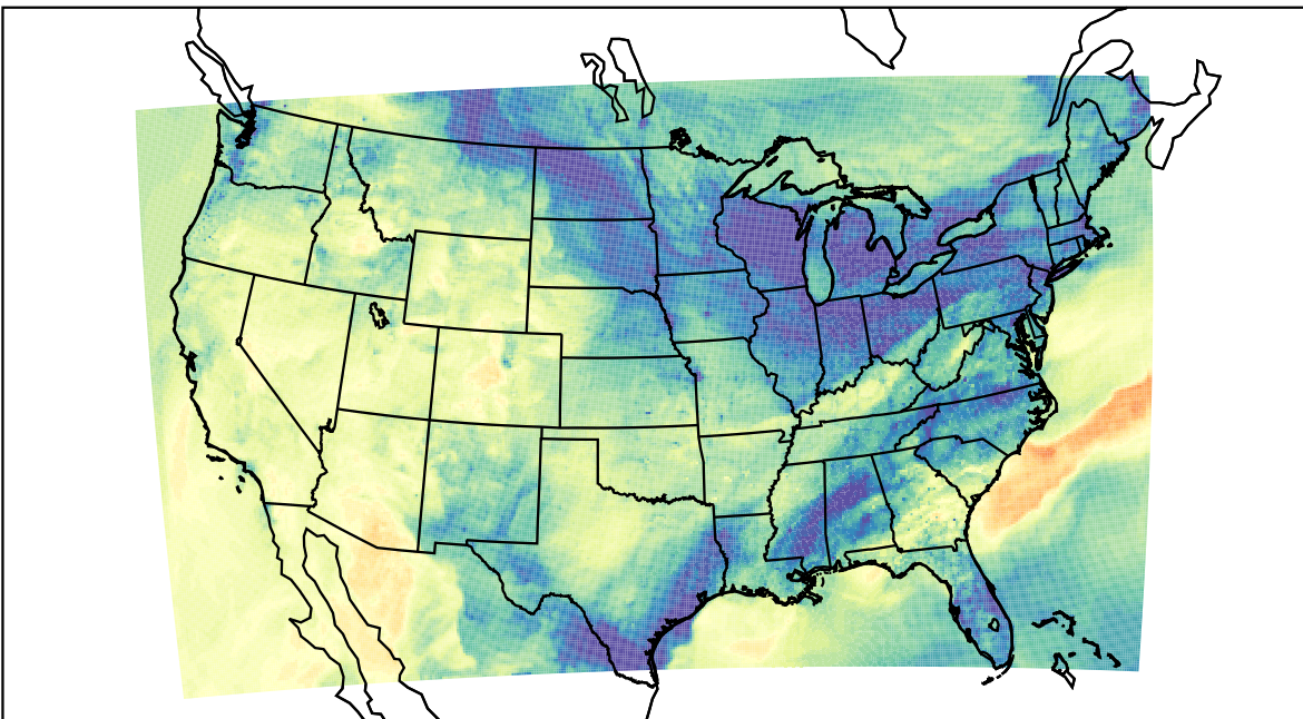
WRF (2023-11-10_23:00:00)
