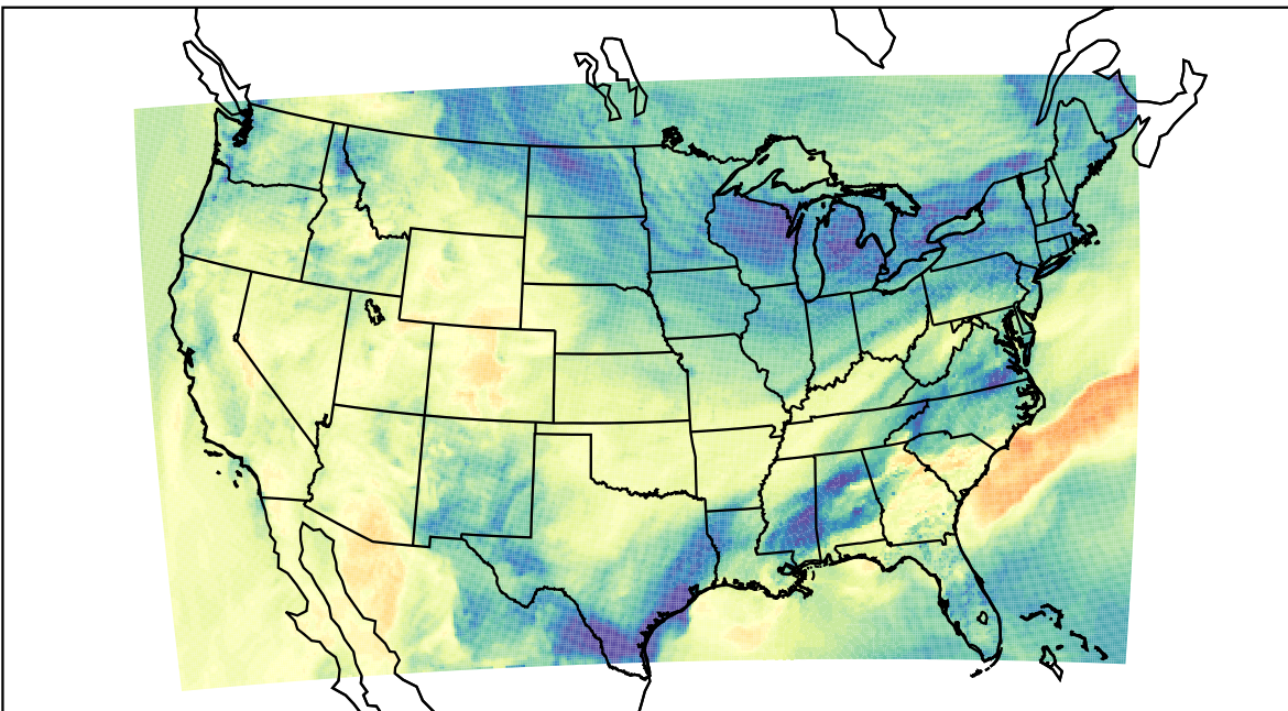
WRF (2023-11-10_21:00:00)
