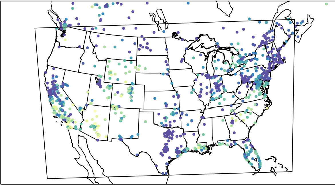
AirNOW (2023-11-10_01:00:00)
