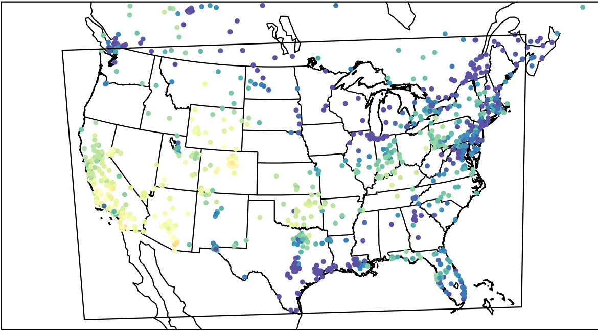
AirNOW (2023-11-10_22:00:00)
