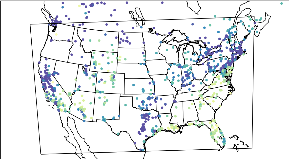
AirNOW (2023-11-09_16:00:00)
