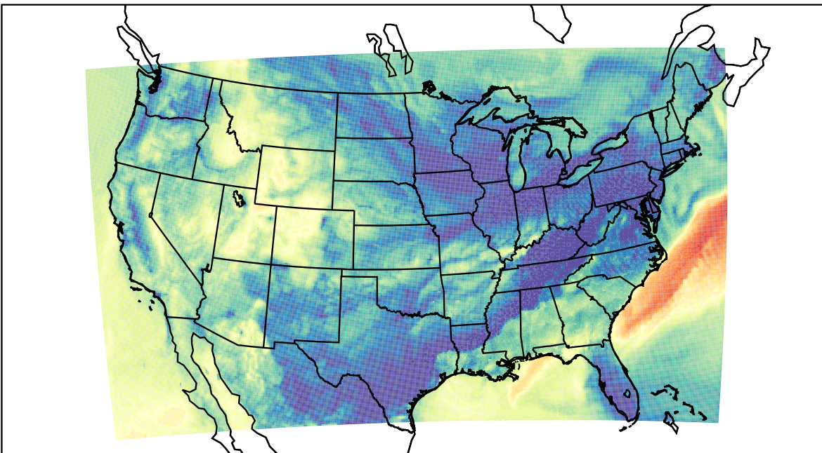
WRF (2023-11-10_07:00:00)
