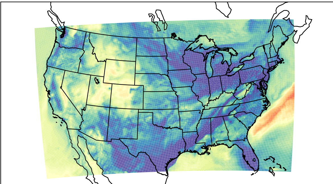
WRF (2023-11-10_13:00:00)
