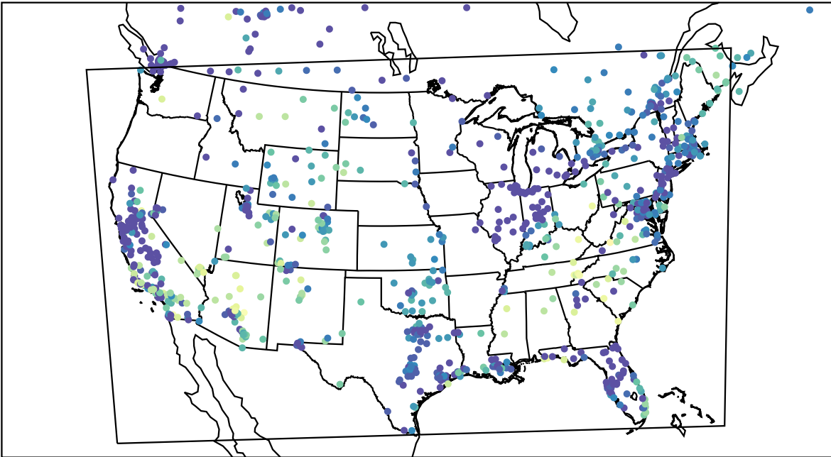
AirNOW (2023-11-09_06:00:00)
