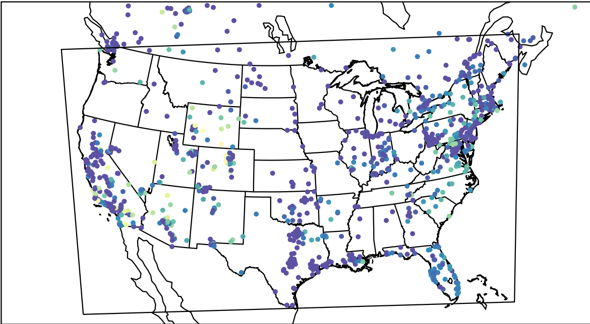
AirNOW (2023-11-10_14:00:00)
