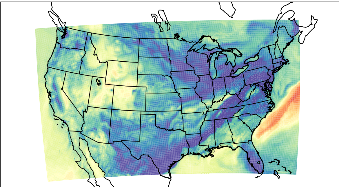
WRF (2023-11-10_10:00:00)
