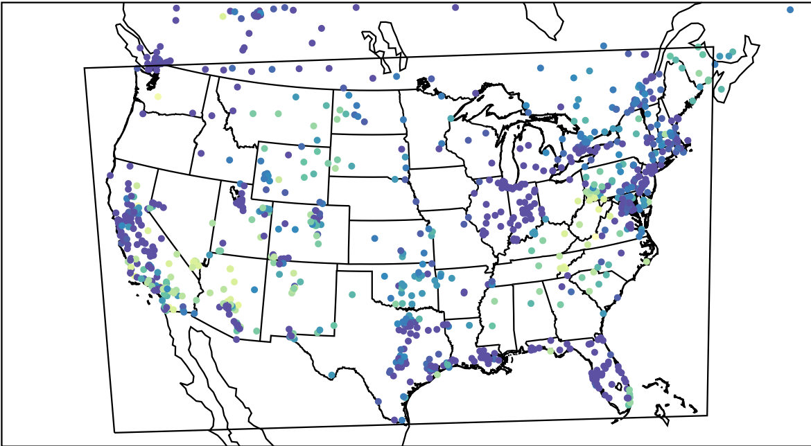
AirNOW (2023-11-09_09:00:00)
