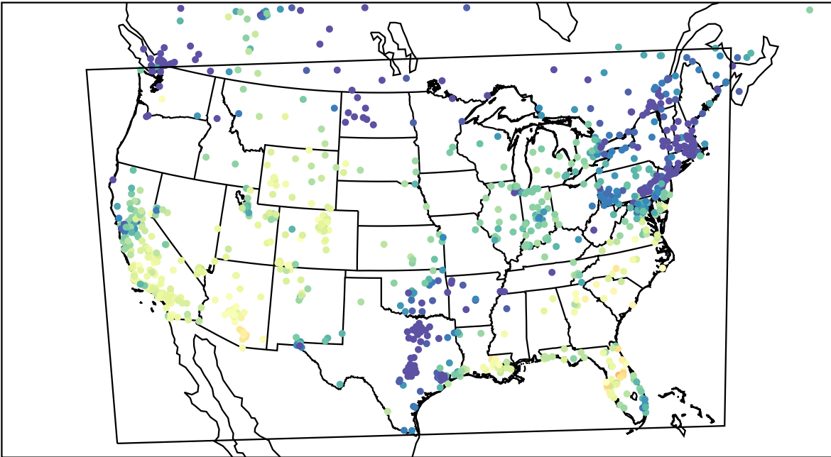
AirNOW (2023-11-09_21:00:00)
