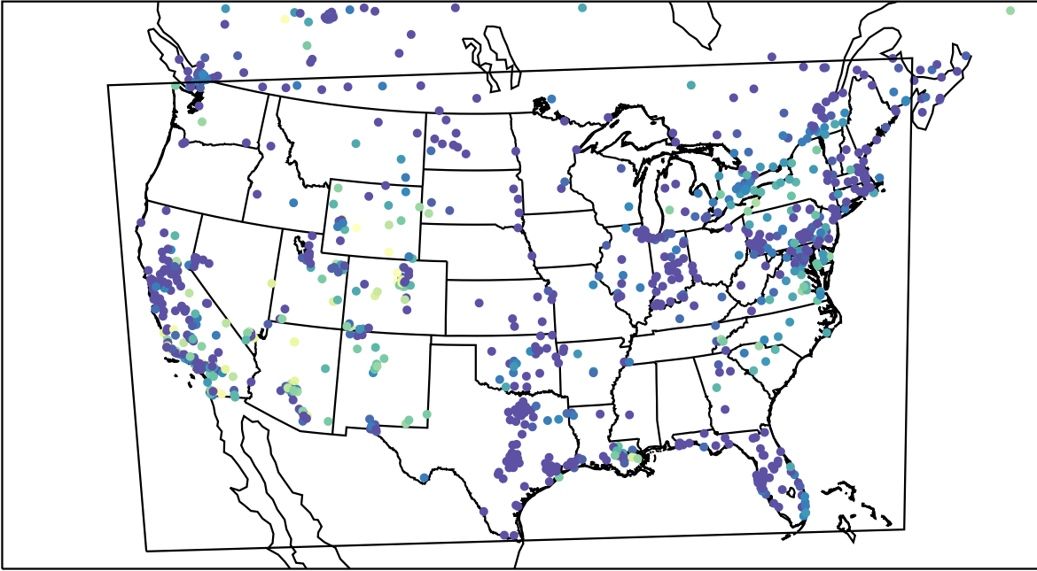
AirNOW (2023-11-10_08:00:00)
