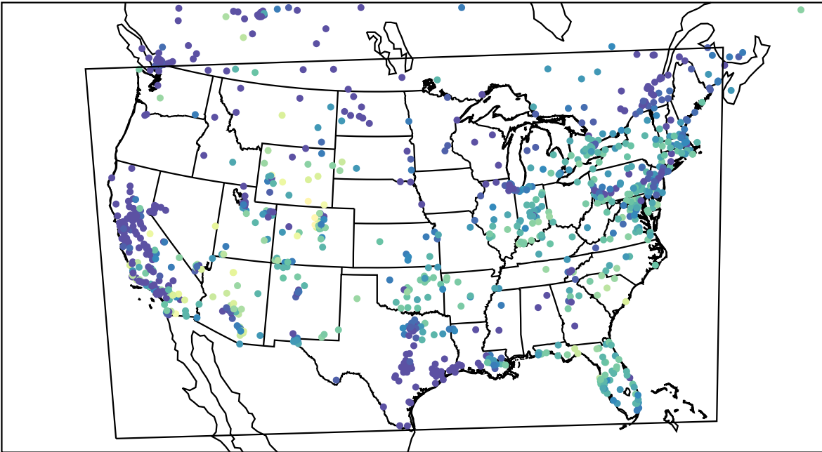
AirNOW (2023-11-10_16:00:00)
