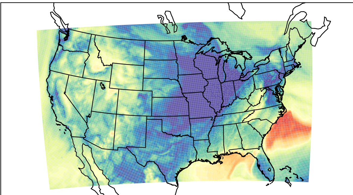
WRF (2023-11-09_09:00:00)
