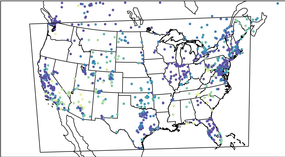
AirNOW (2023-11-09_07:00:00)
