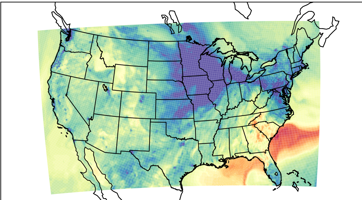
WRF (2023-11-09_01:00:00)
