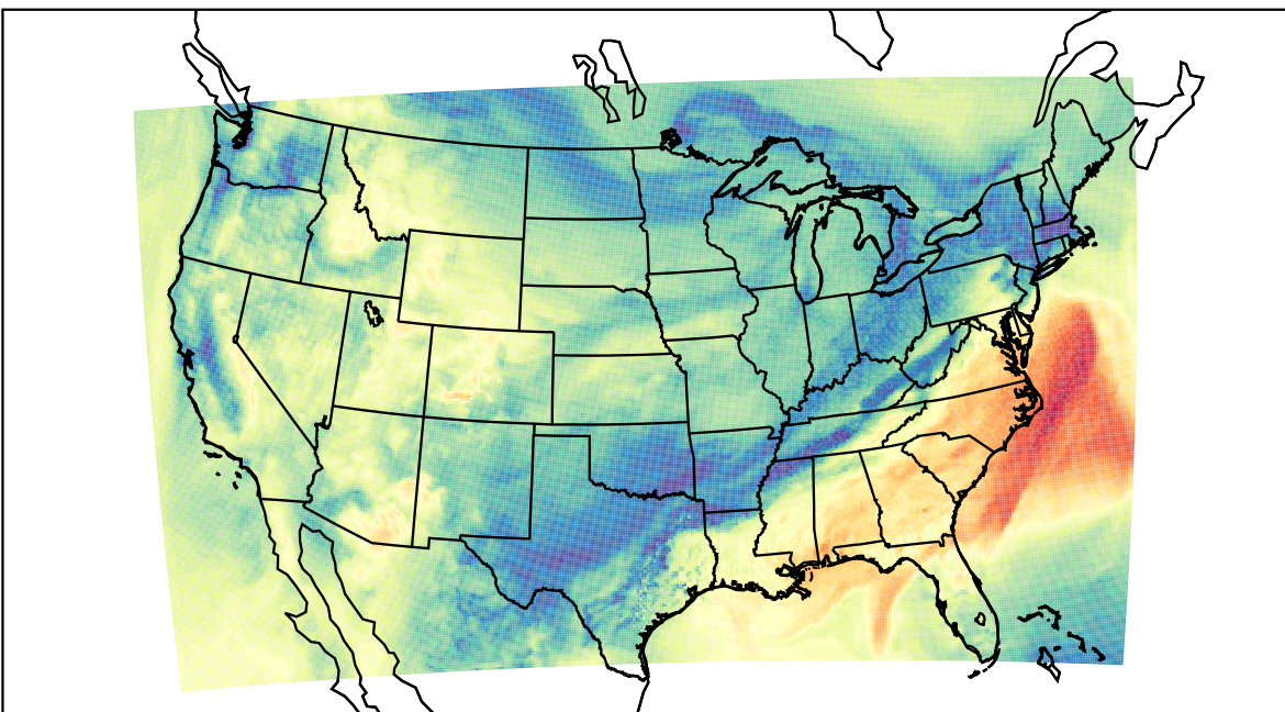
WRF (2023-11-09_18:00:00)
