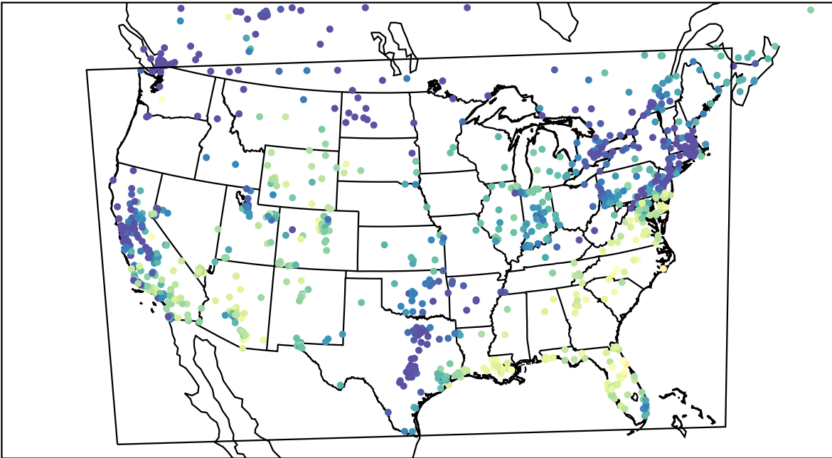
AirNOW (2023-11-09_17:00:00)
