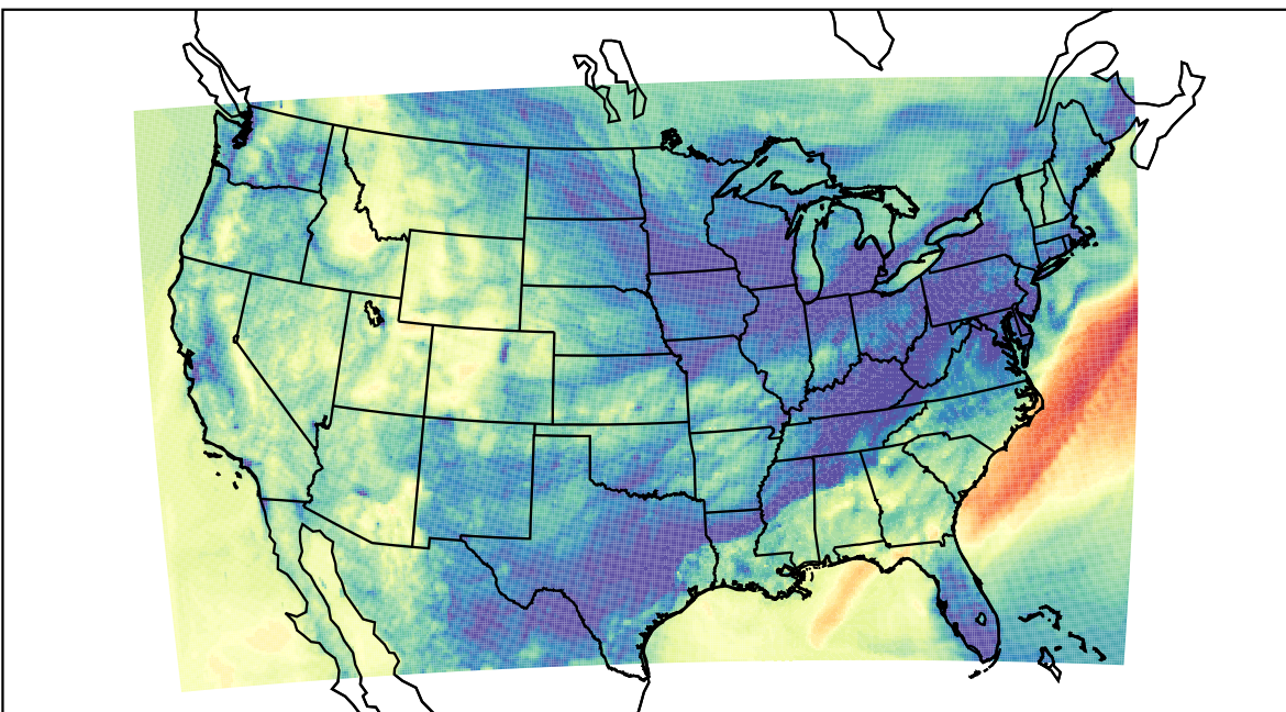
WRF (2023-11-10_04:00:00)
