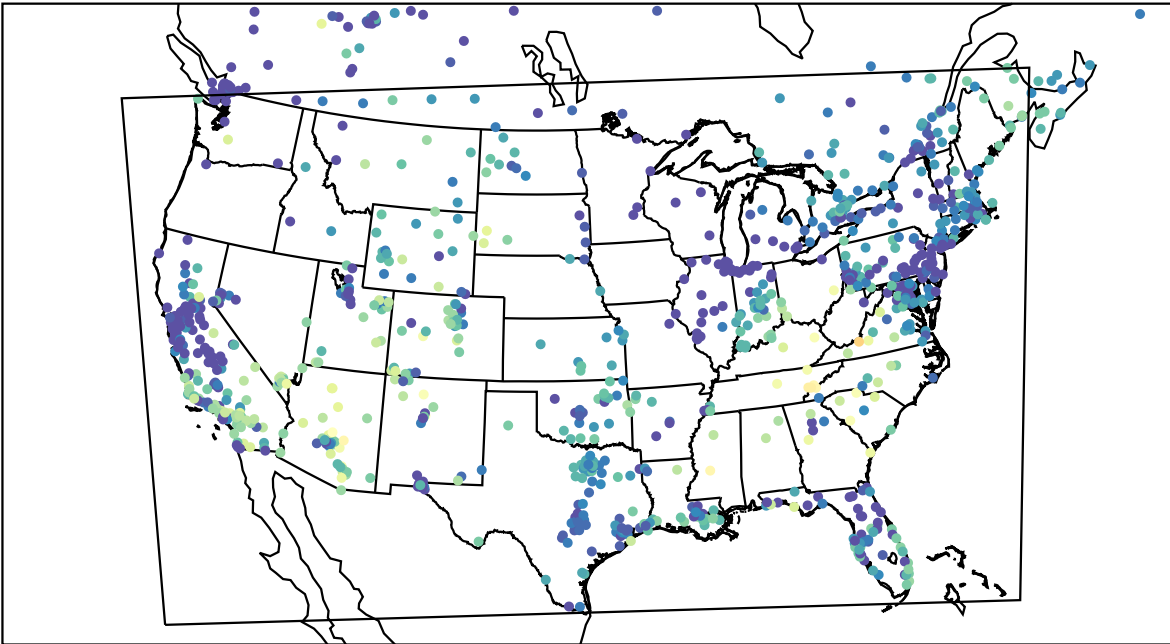
AirNOW (2023-11-09_03:00:00)
