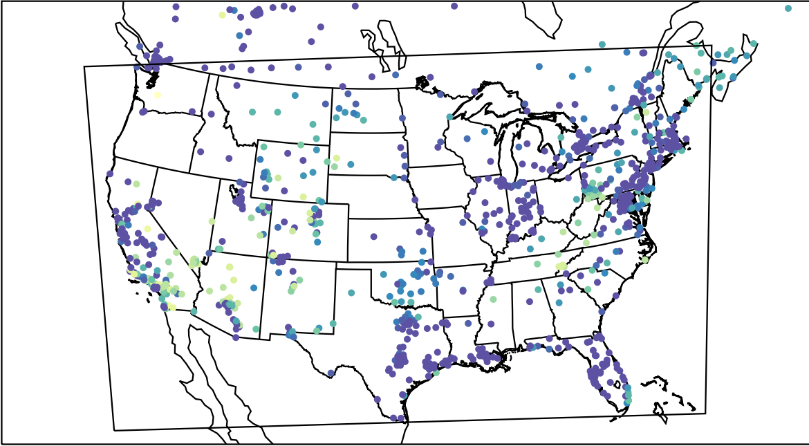
AirNOW (2023-11-09_12:00:00)
