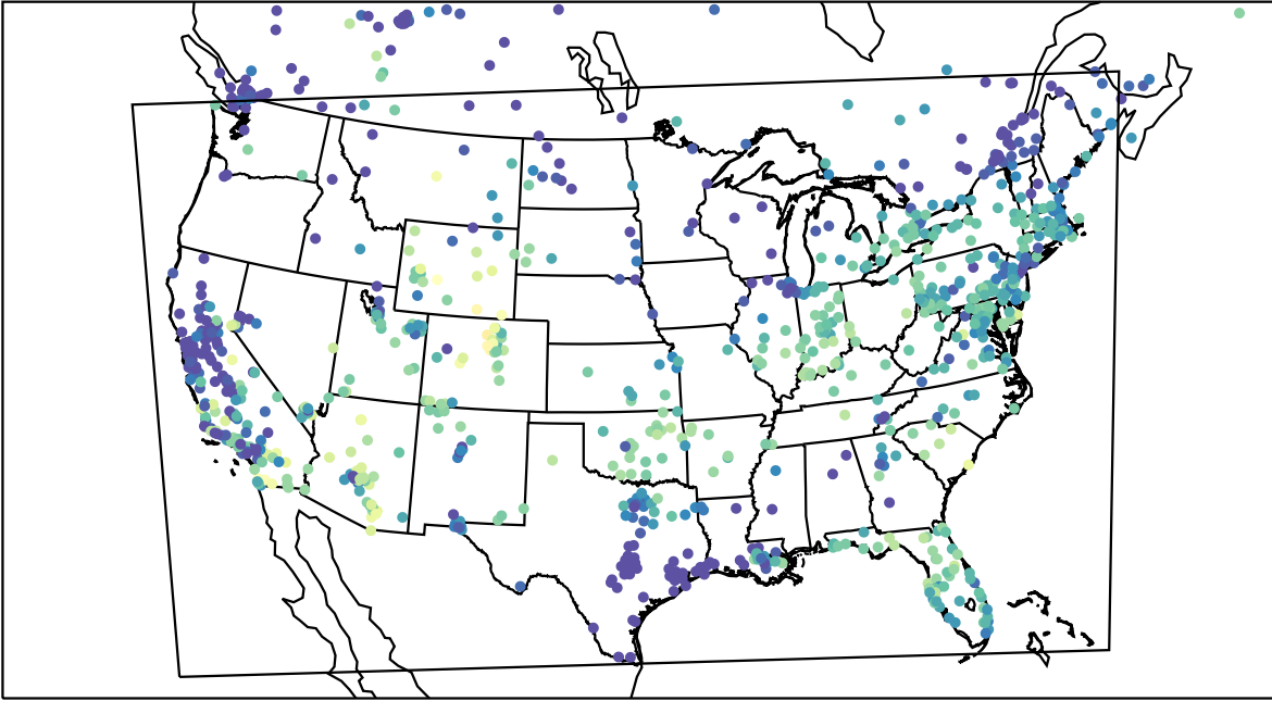
AirNOW (2023-11-10_17:00:00)
