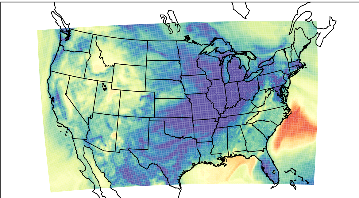
WRF (2023-11-09_13:00:00)
