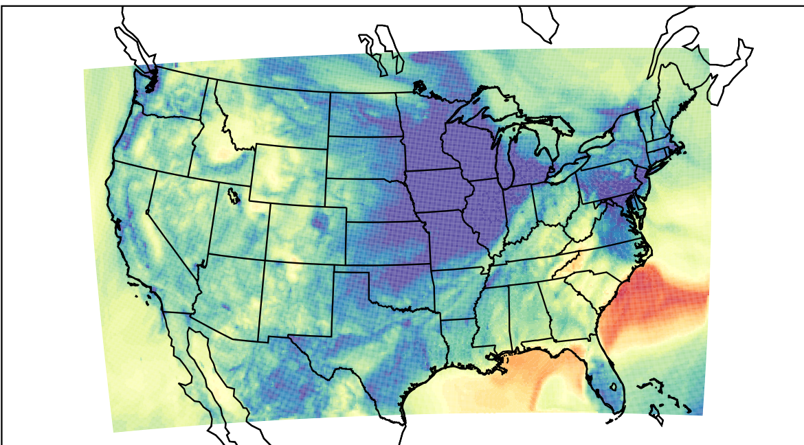
WRF (2023-11-09_05:00:00)
