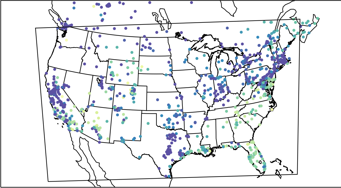
AirNOW (2023-11-09_15:00:00)
