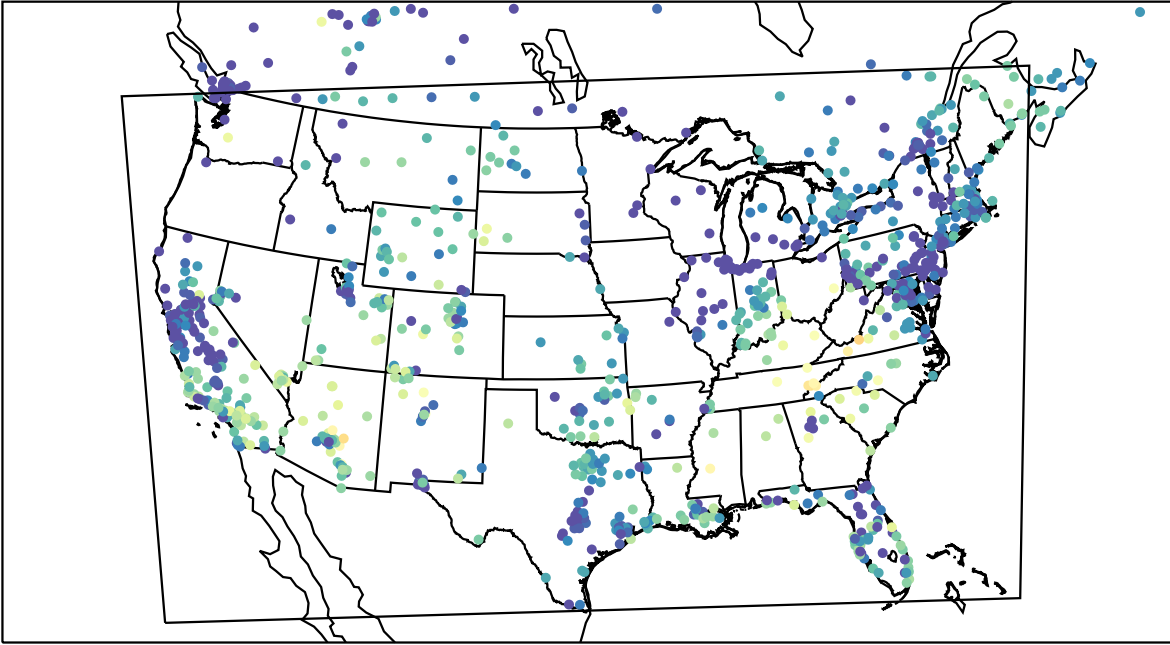
AirNOW (2023-11-09_02:00:00)
