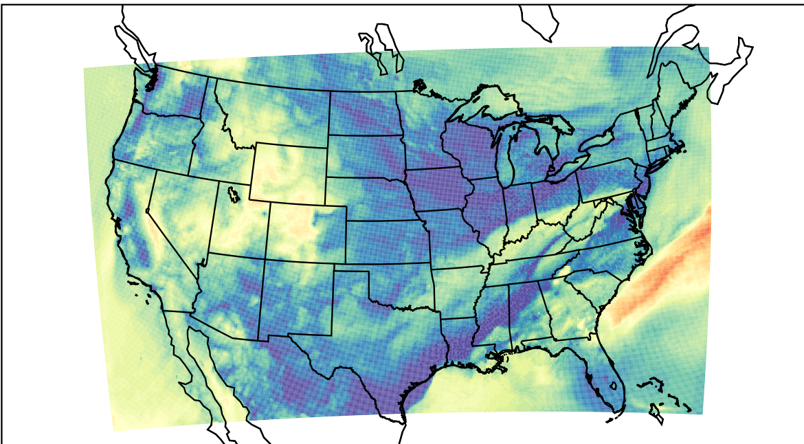
WRF (2023-11-10_15:00:00)
