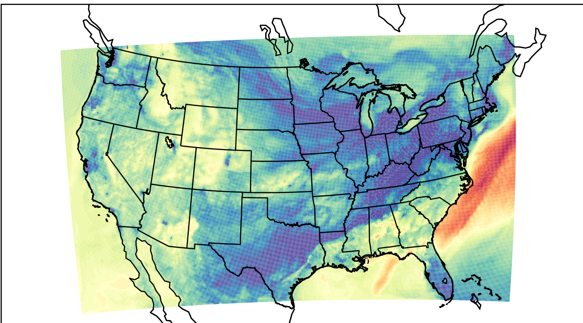
WRF (2023-11-10_02:00:00)
