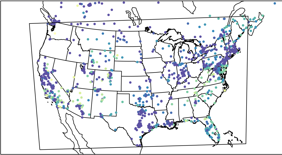
AirNOW (2023-11-09_14:00:00)
