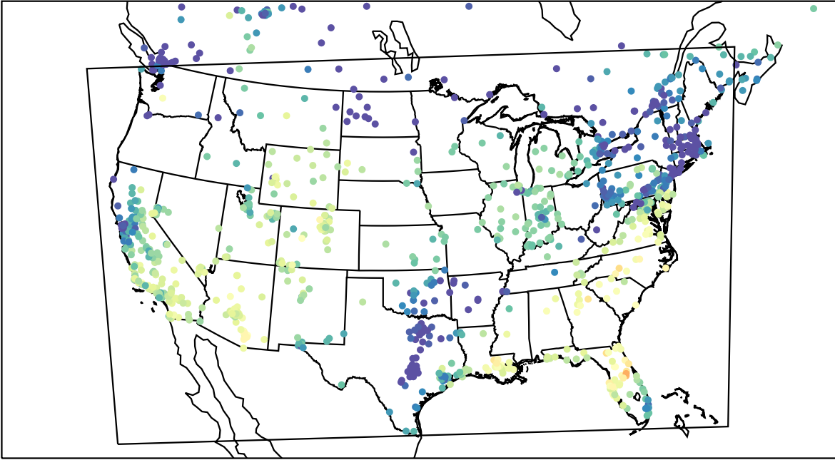
AirNOW (2023-11-09_19:00:00)
