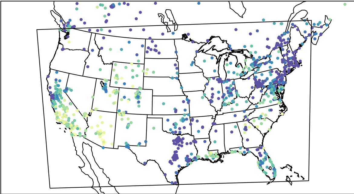
AirNOW (2023-11-10_00:00:00)
