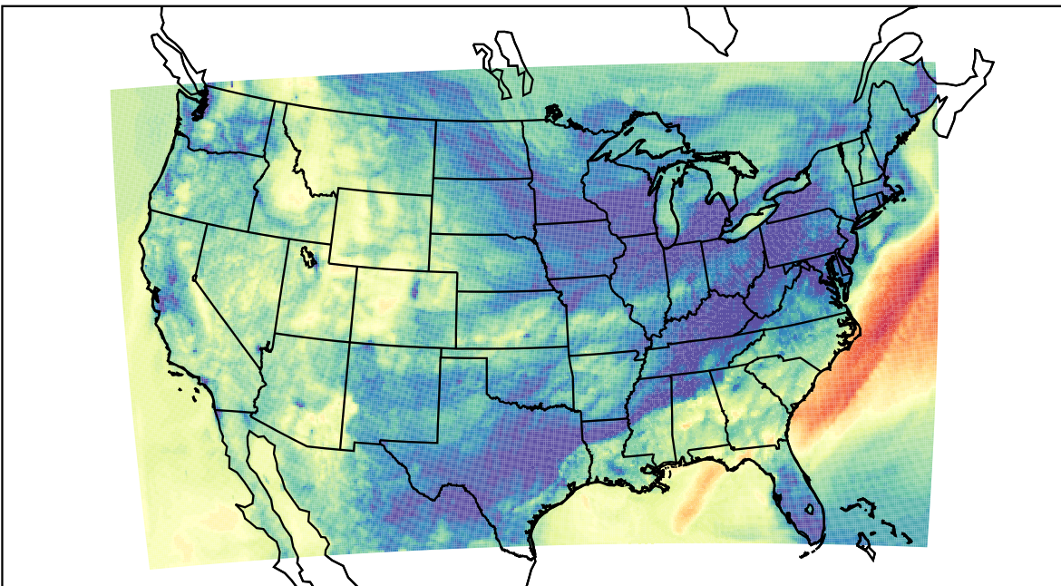
WRF (2023-11-10_03:00:00)
