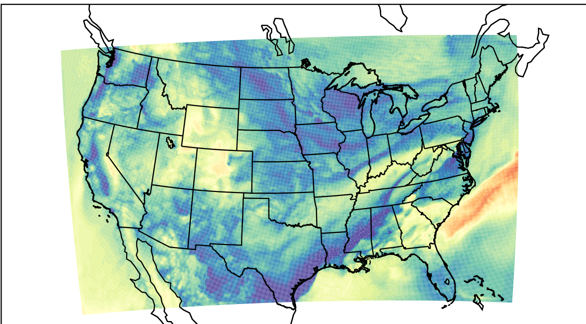
WRF (2023-11-10_16:00:00)
