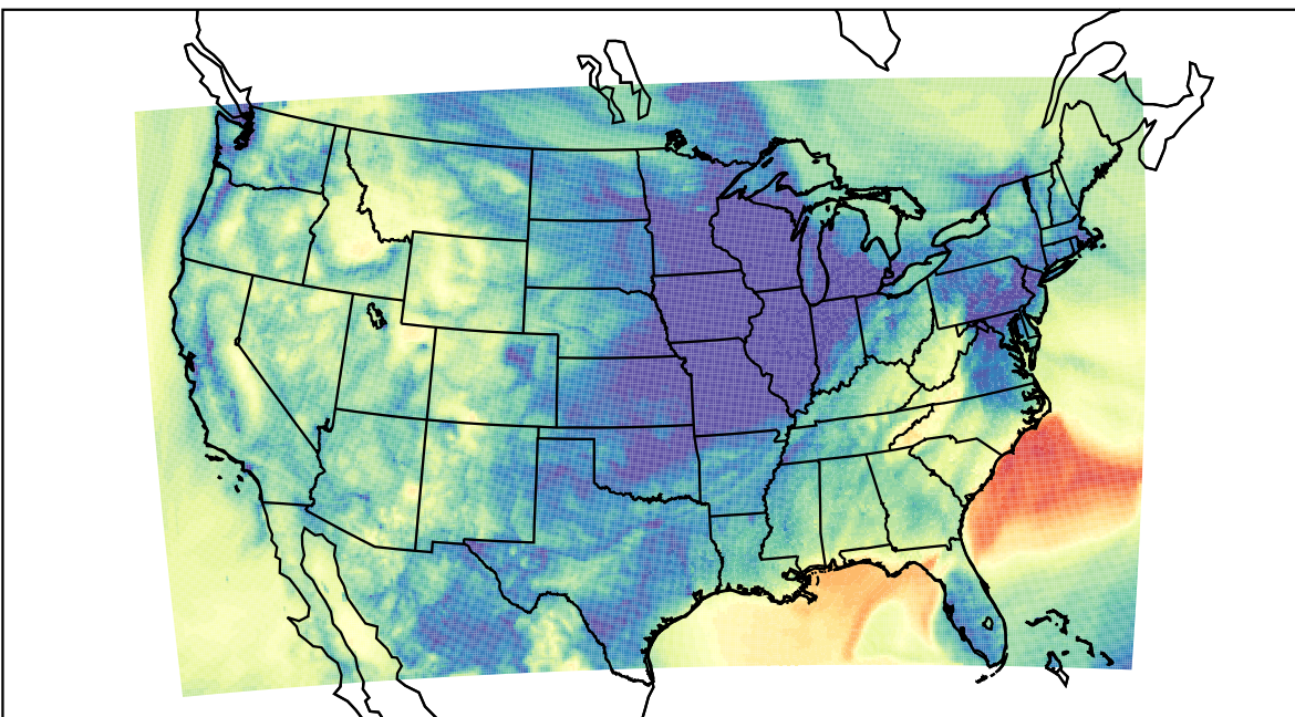
WRF (2023-11-09_07:00:00)
