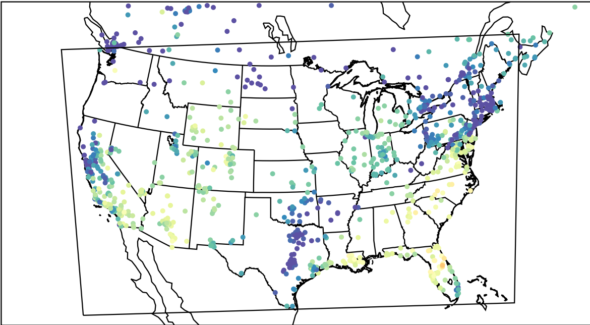
AirNOW (2023-11-09_18:00:00)
