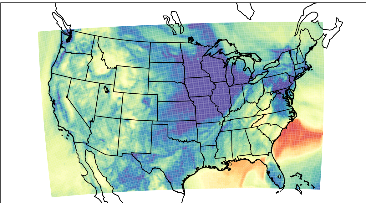
WRF (2023-11-09_06:00:00)
