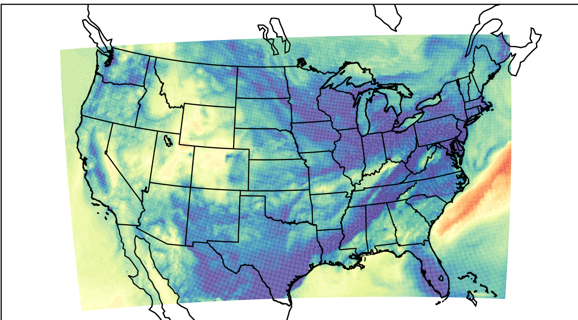
WRF (2023-11-10_11:00:00)
