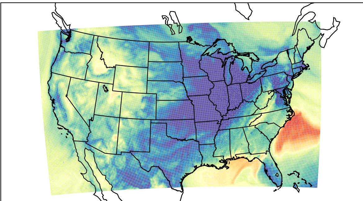
WRF (2023-11-09_11:00:00)
