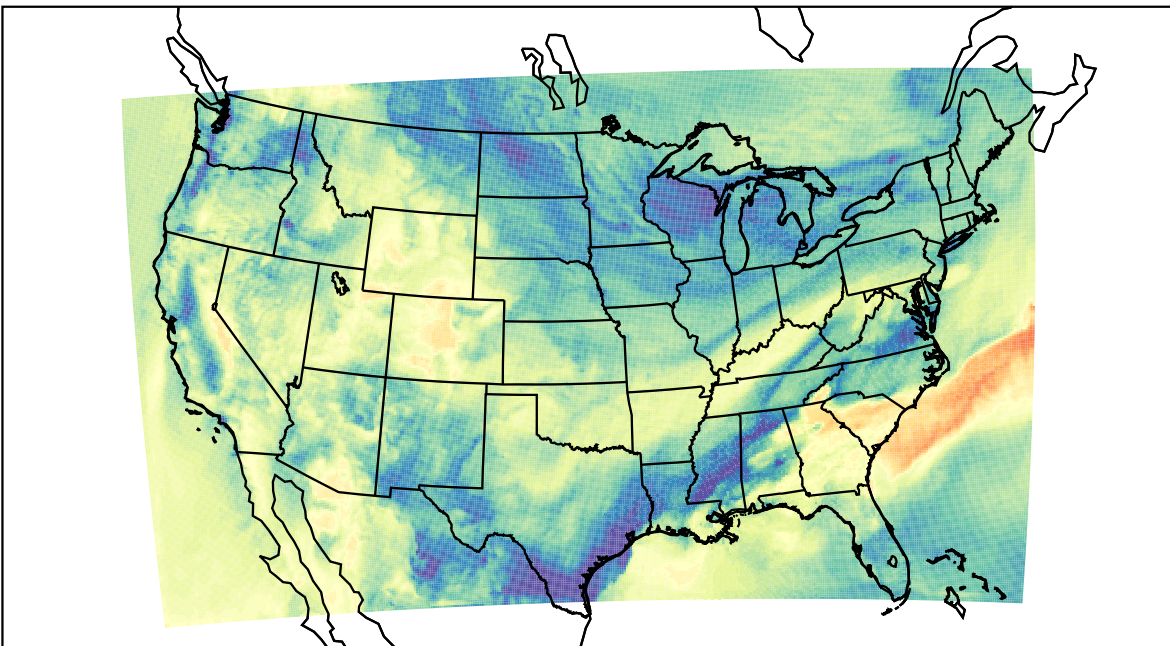
WRF (2023-11-10_18:00:00)
