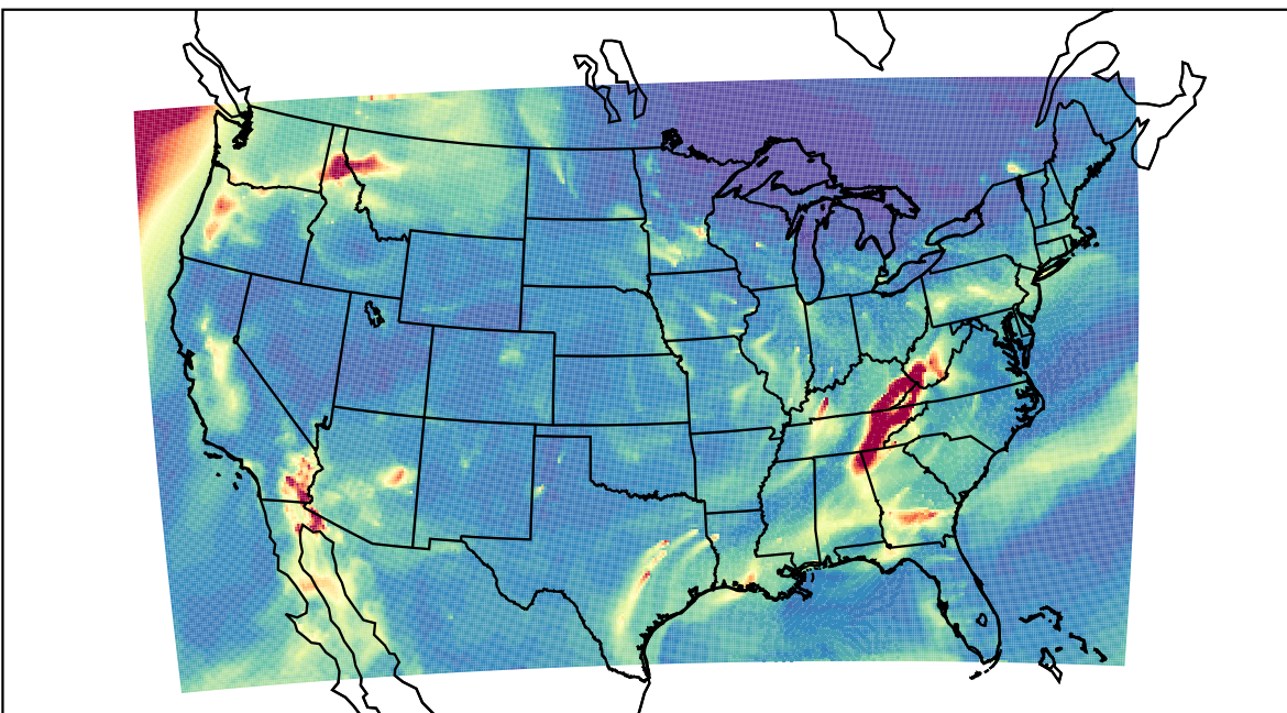
WRF 2023-11-11_08:00:00
