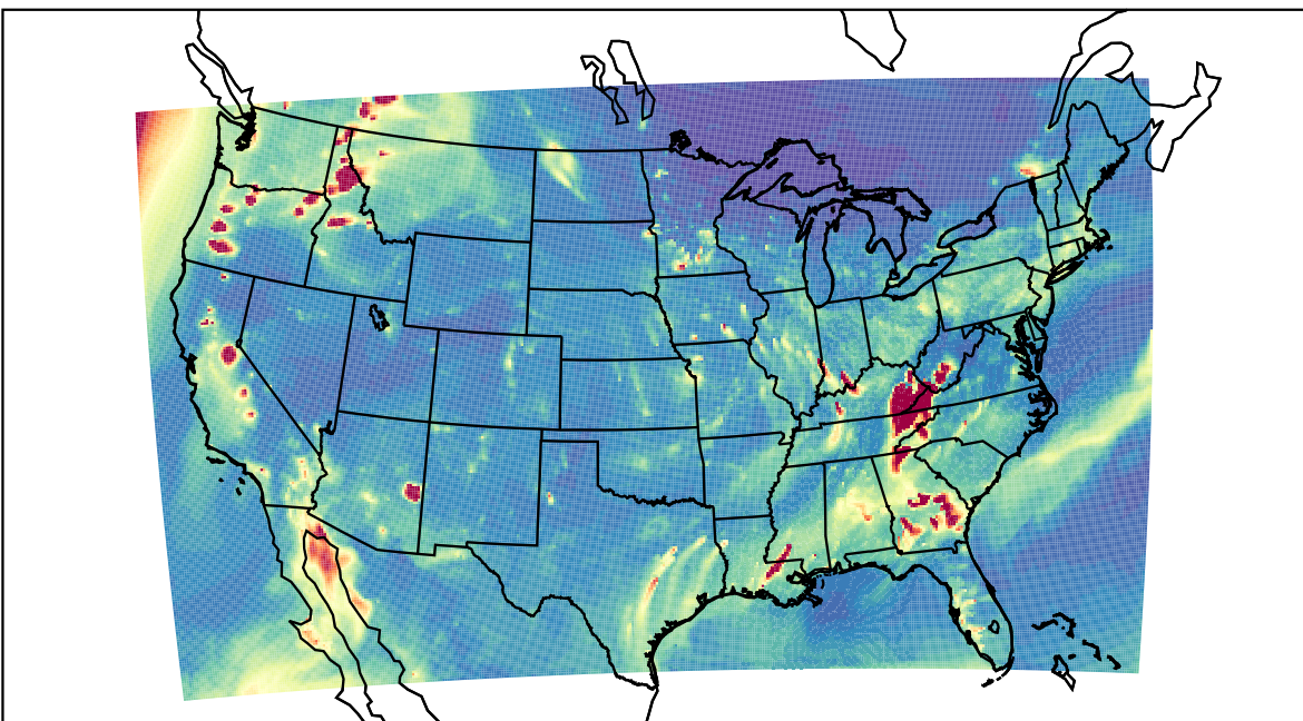
WRF 2023-11-11_02:00:00
