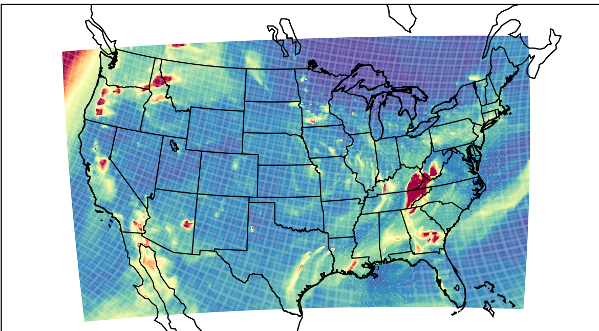
WRF 2023-11-11_05:00:00
