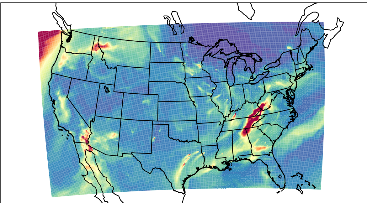
WRF 2023-11-11_09:00:00
