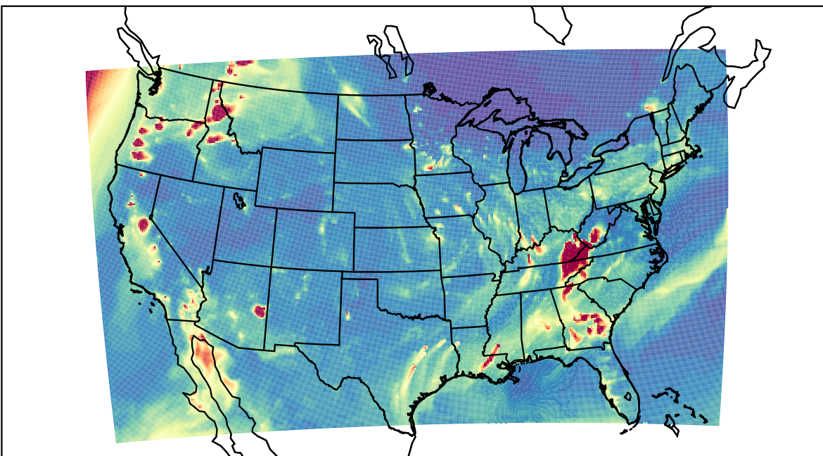
WRF 2023-11-11_03:00:00
