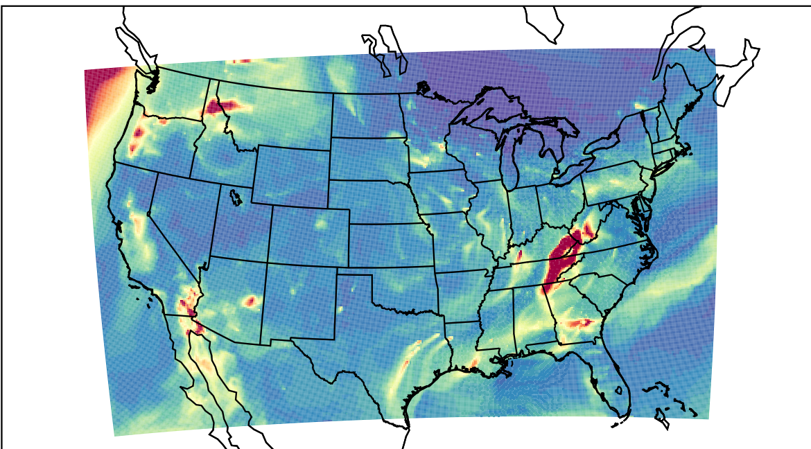
WRF 2023-11-11_07:00:00
