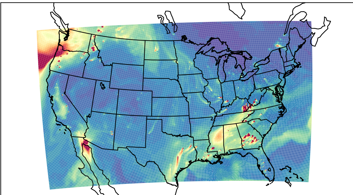
WRF 2023-11-11_21:00:00
