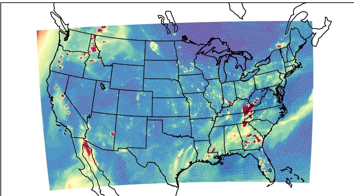
WRF 2023-11-11_00:00:00
