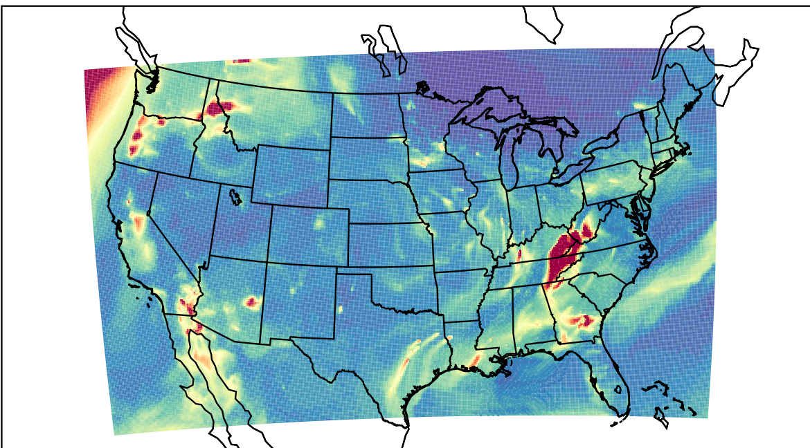
WRF 2023-11-11_06:00:00
