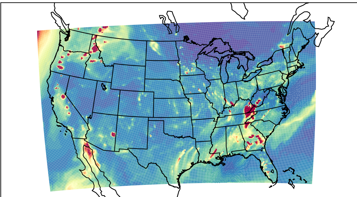
WRF 2023-11-11_01:00:00
