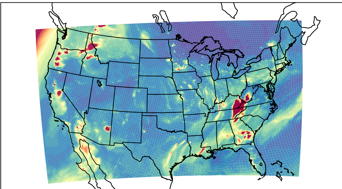
WRF 2023-11-11_04:00:00
