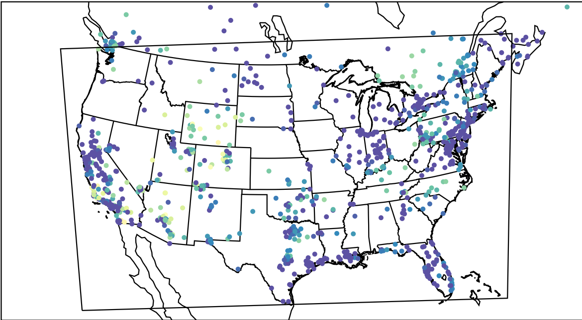
AirNOW (2023-11-11_04:00:00)
