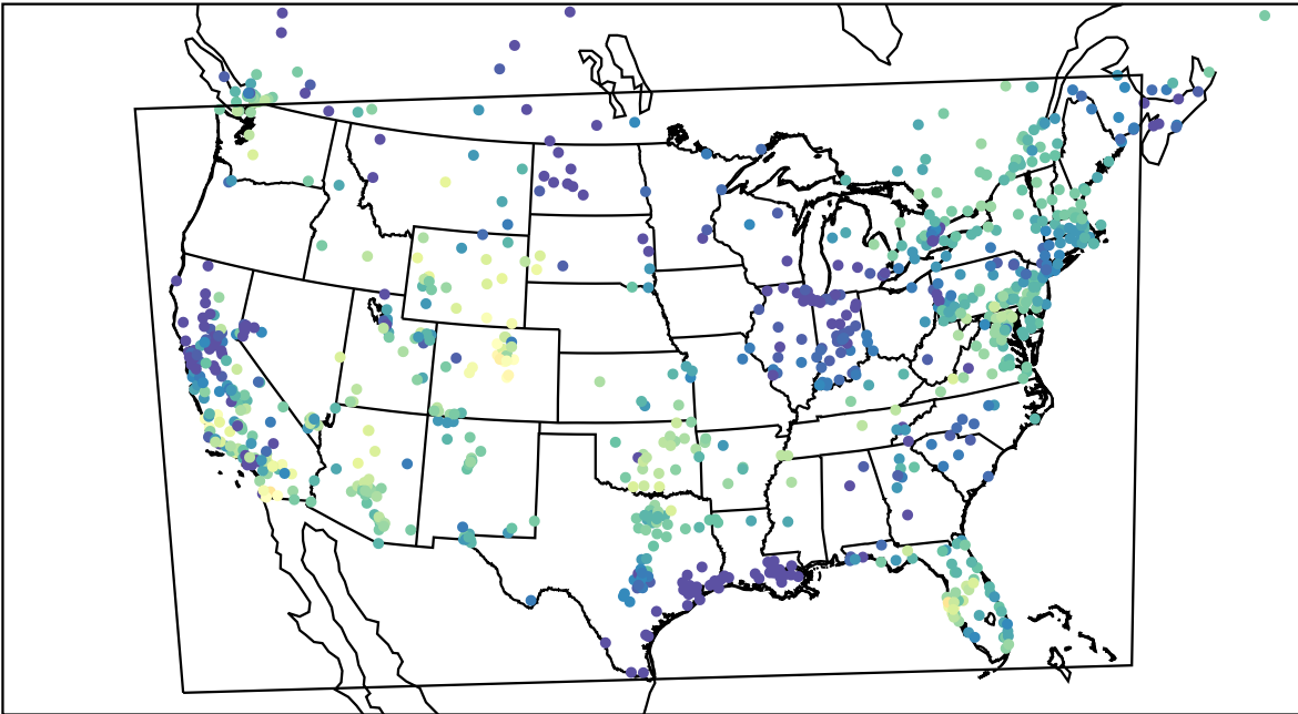
AirNOW (2023-11-11_17:00:00)
