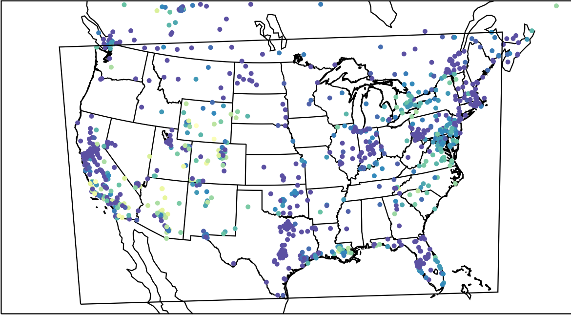
AirNOW (2023-11-10_05:00:00)
