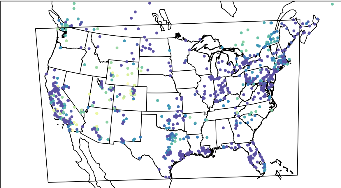
AirNOW (2023-11-11_08:00:00)
