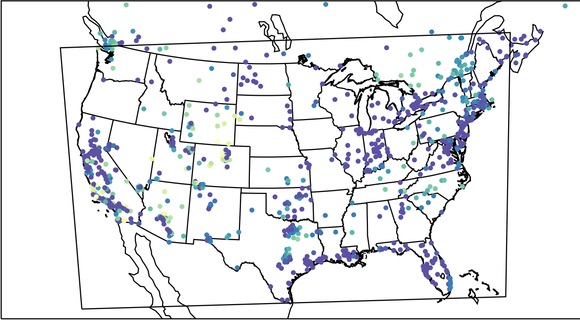
AirNOW (2023-11-11_06:00:00)
