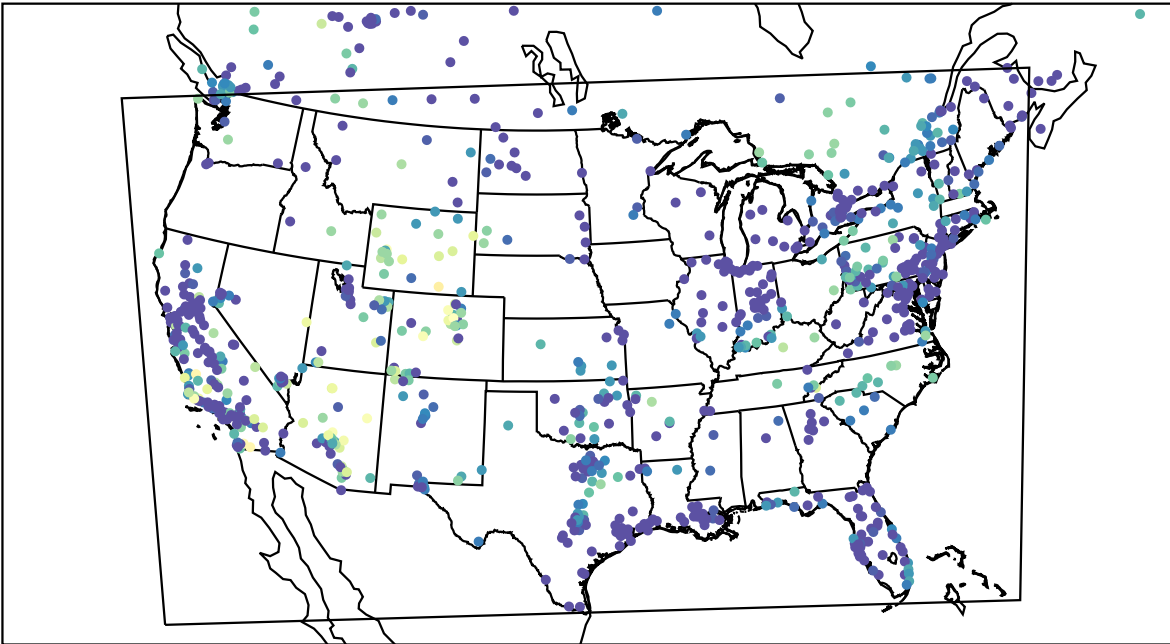
AirNOW (2023-11-11_03:00:00)
