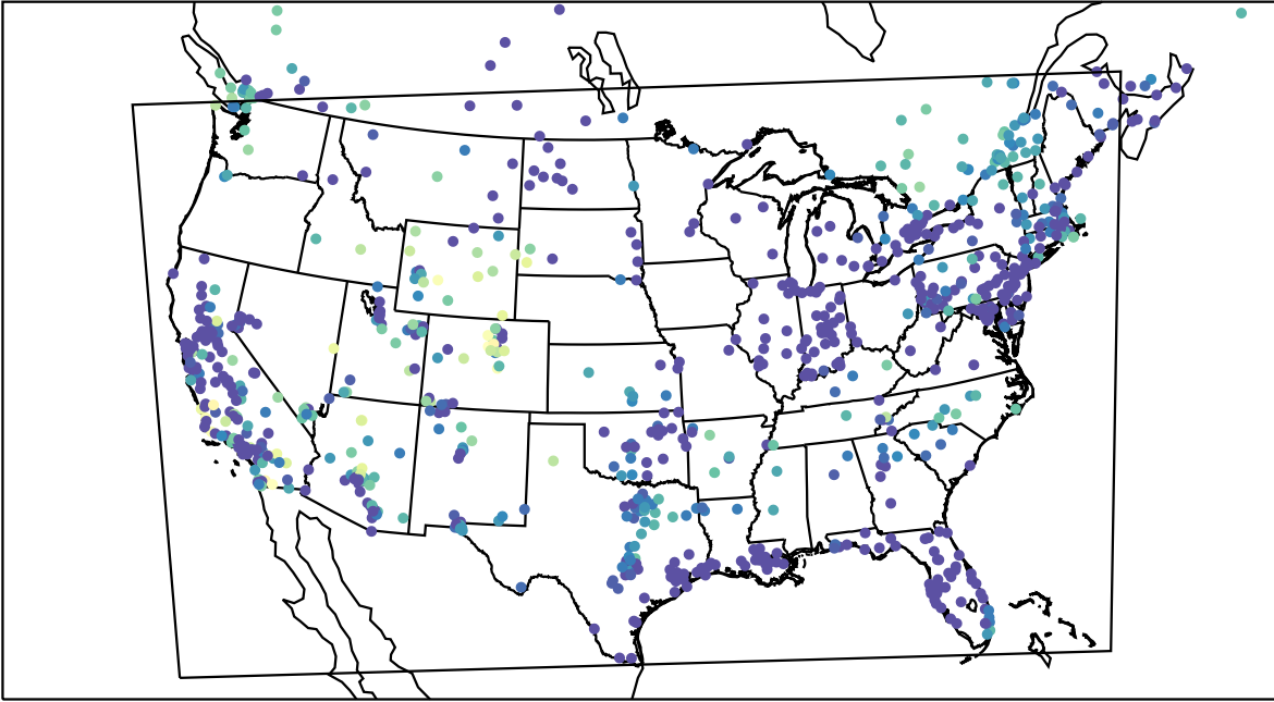
AirNOW (2023-11-11_09:00:00)
