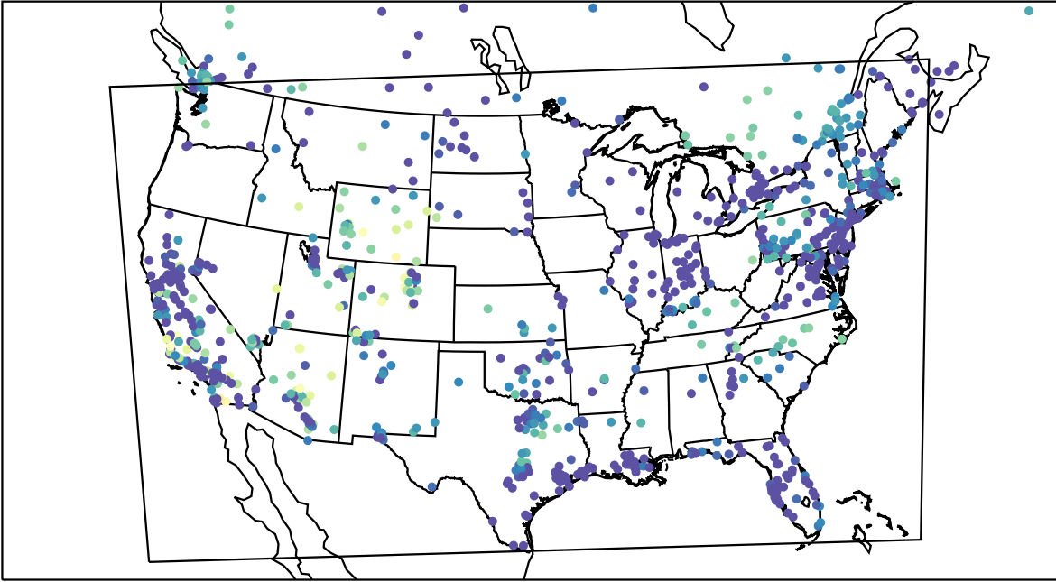
AirNOW (2023-11-11_05:00:00)
