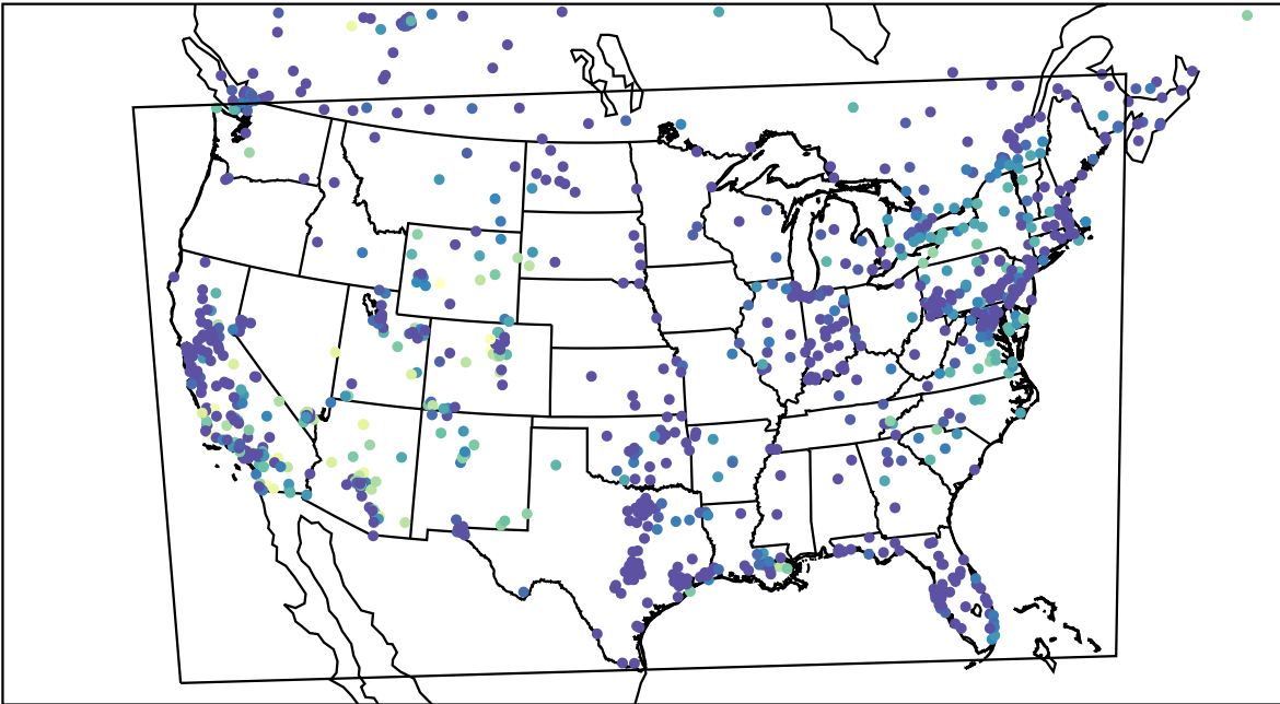
AirNOW (2023-11-10_09:00:00)
