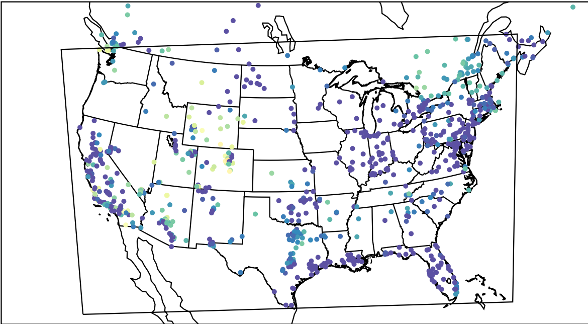
AirNOW (2023-11-11_11:00:00)
