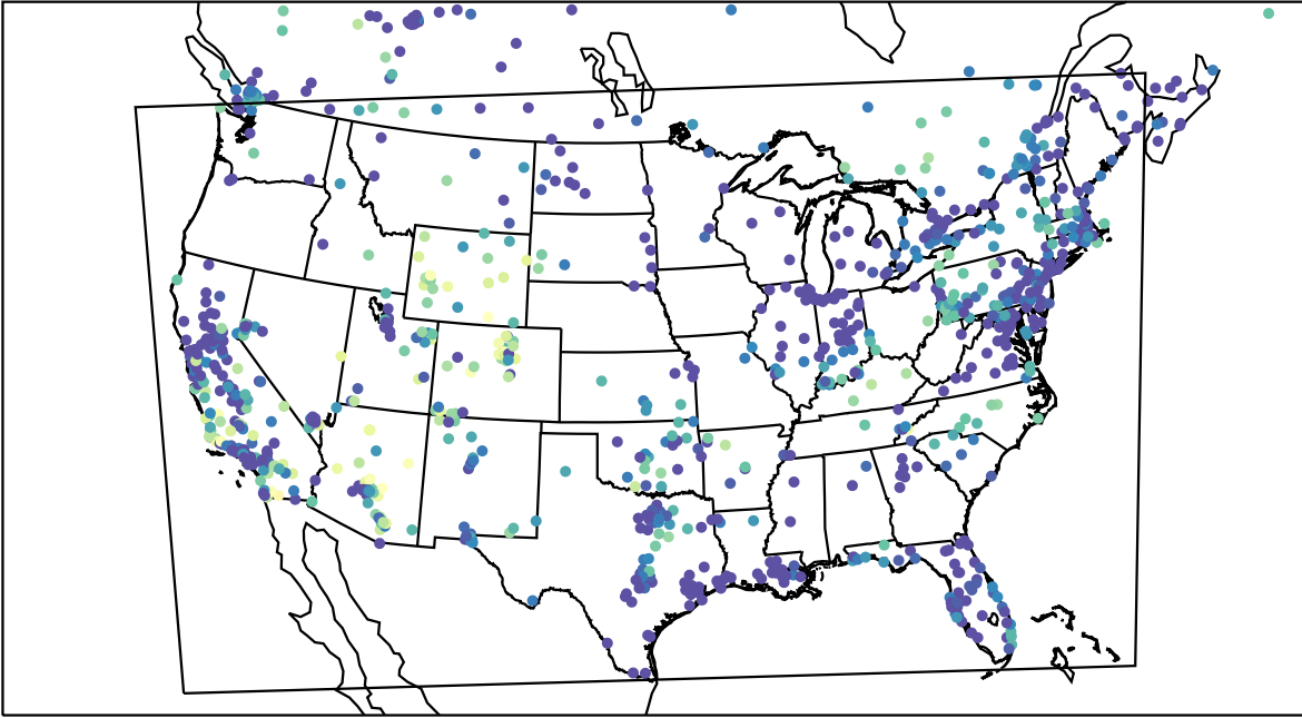
AirNOW (2023-11-11_02:00:00)
