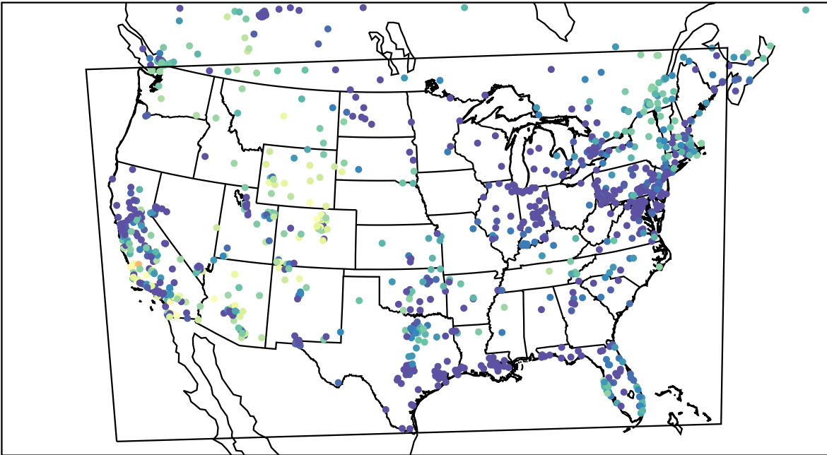
AirNOW (2023-11-12_02:00:00)
