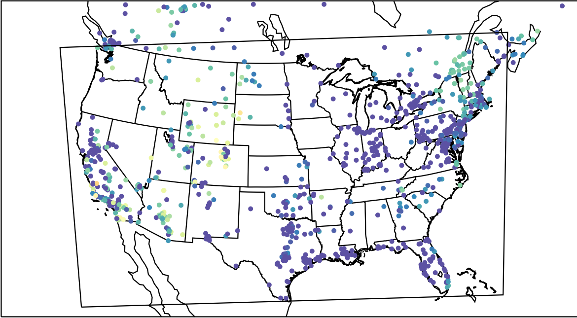
AirNOW (2023-11-12_11:00:00)
