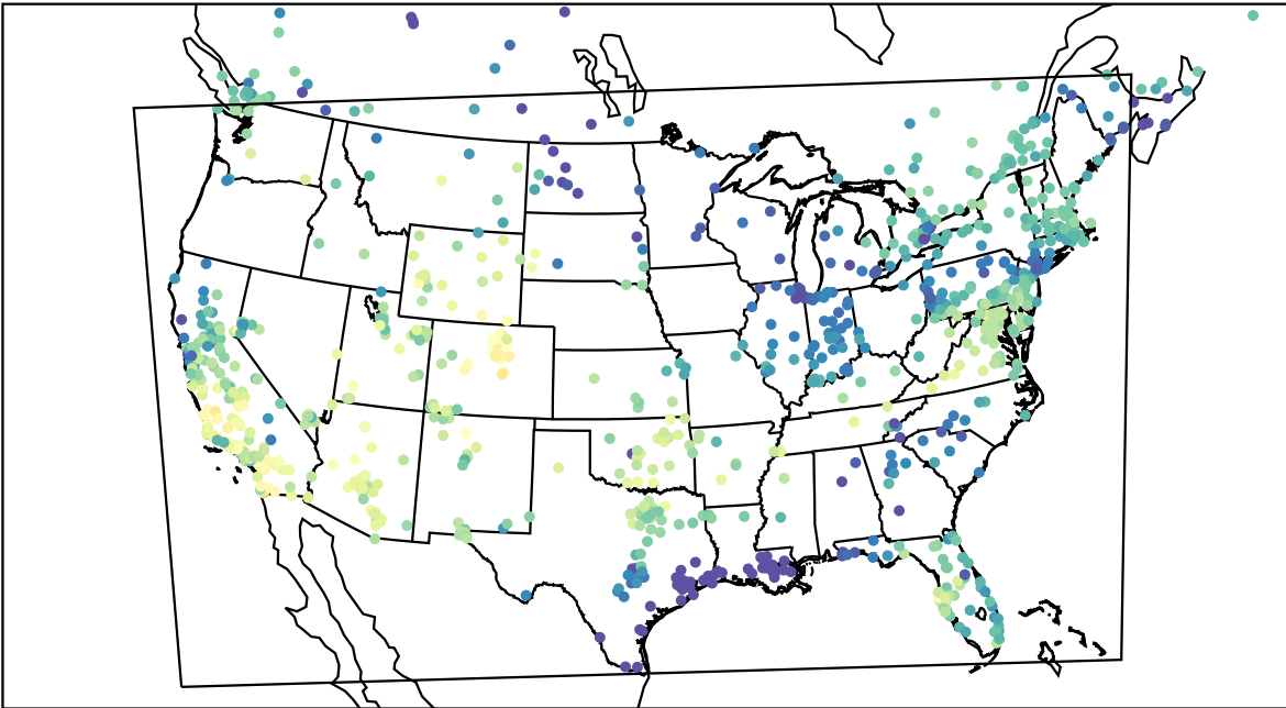
AirNOW (2023-11-11_19:00:00)
