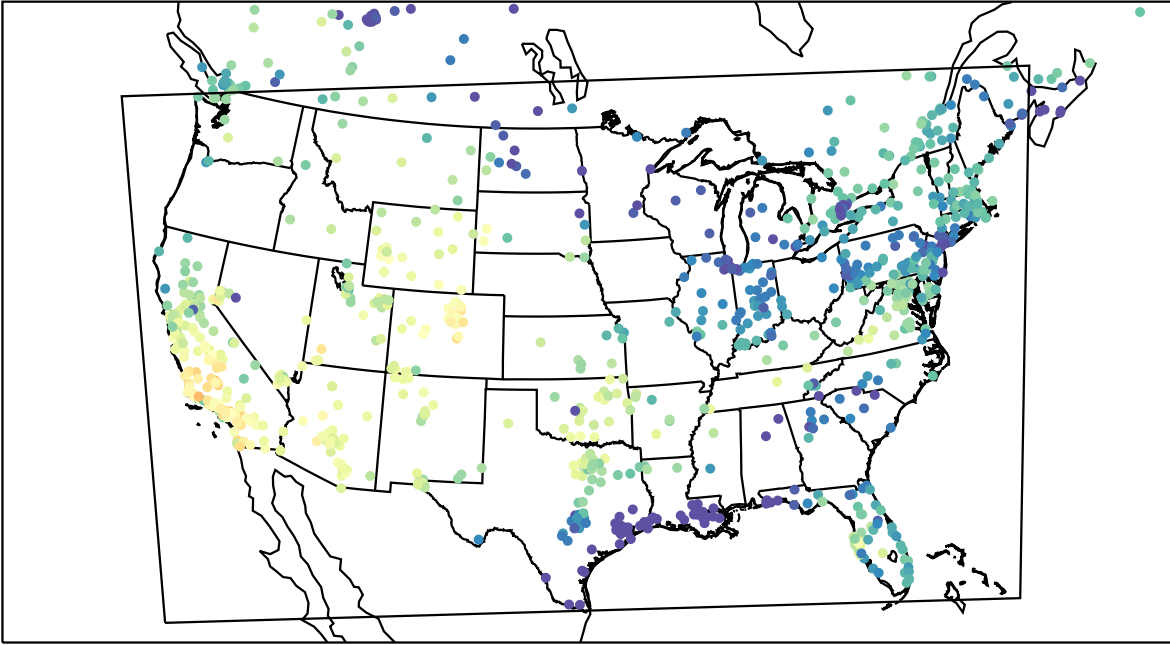
AirNOW (2023-11-11_21:00:00)
