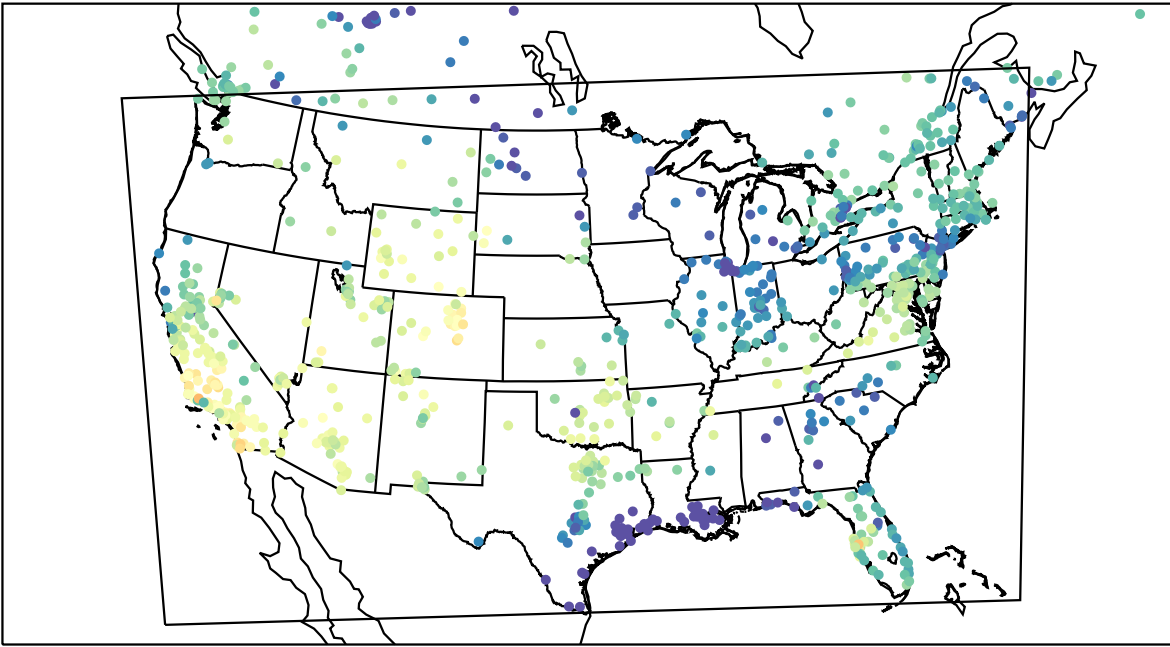
AirNOW (2023-11-11_20:00:00)
