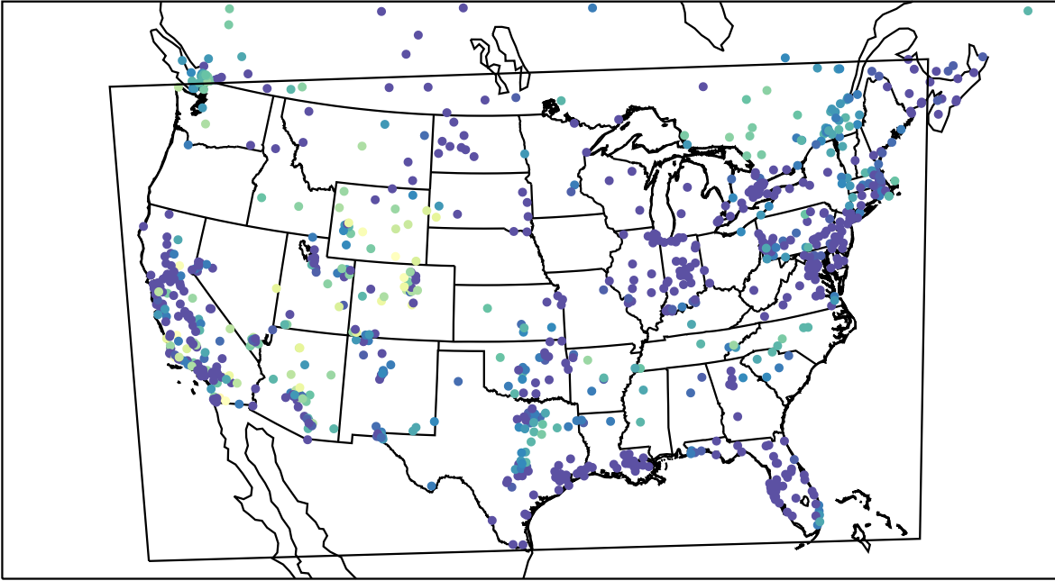
AirNOW (2023-11-11_07:00:00)
