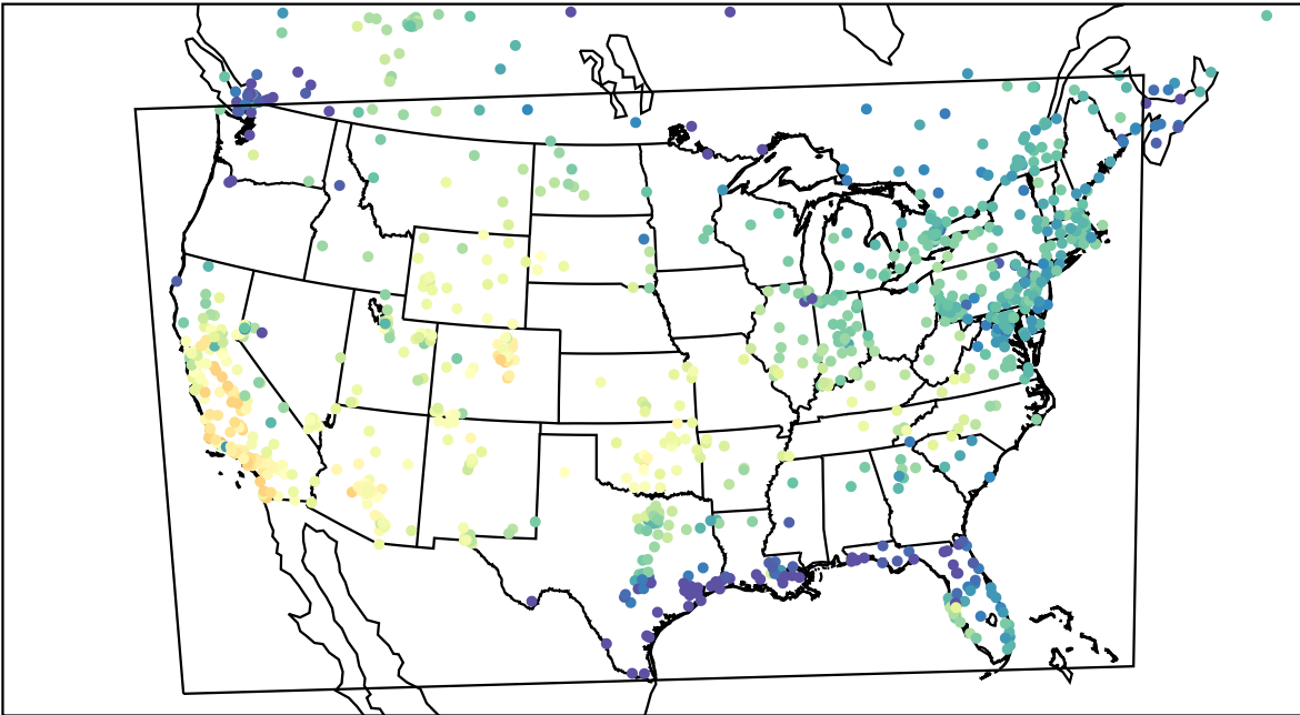
AirNOW (2023-11-12_21:00:00)
