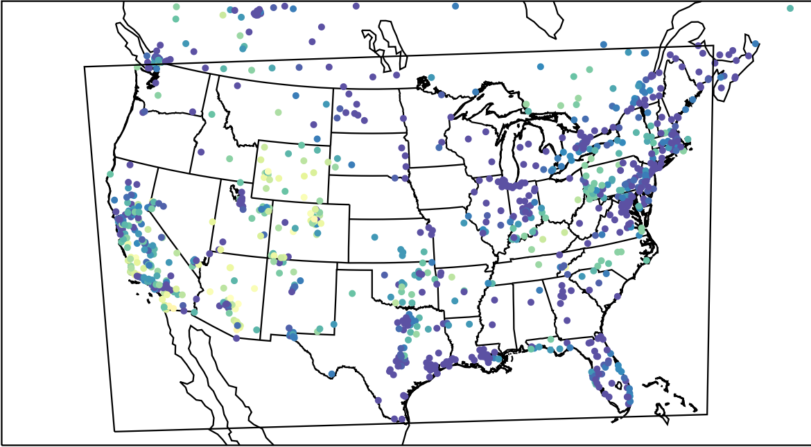
AirNOW (2023-11-11_01:00:00)
