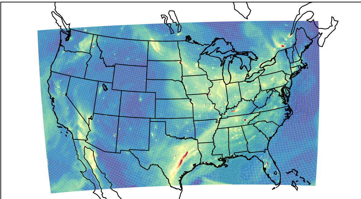
WRF 2023-11-13_22:00:00
