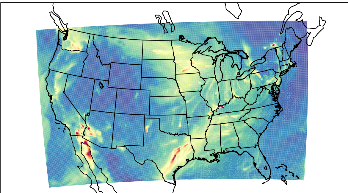
WRF 2023-11-13_06:00:00
