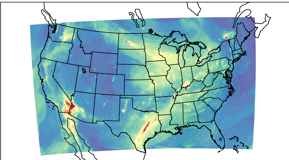
WRF 2023-11-13_15:00:00
