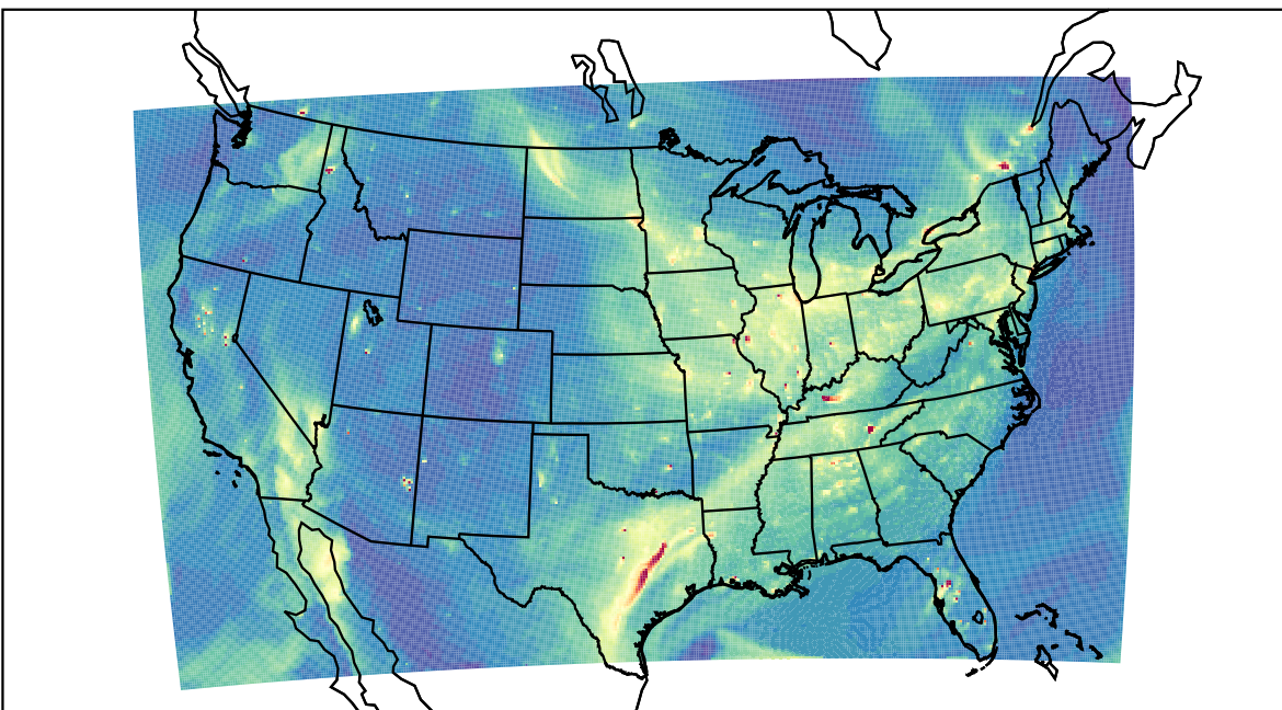
WRF 2023-11-13_23:00:00
