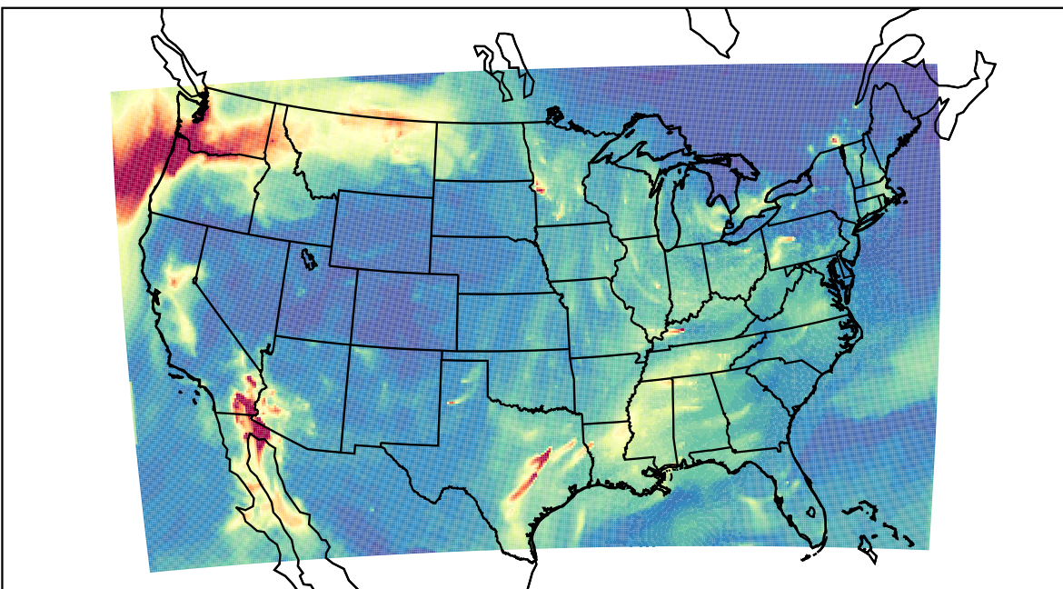
WRF 2023-11-12_11:00:00
