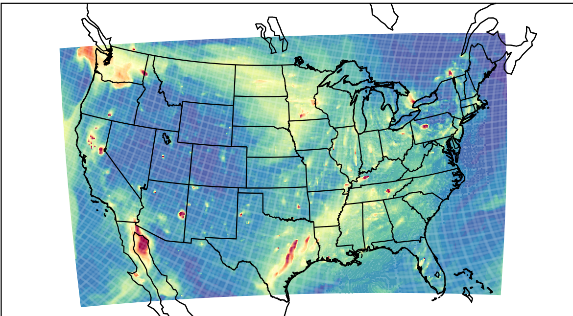
WRF 2023-11-13_01:00:00
