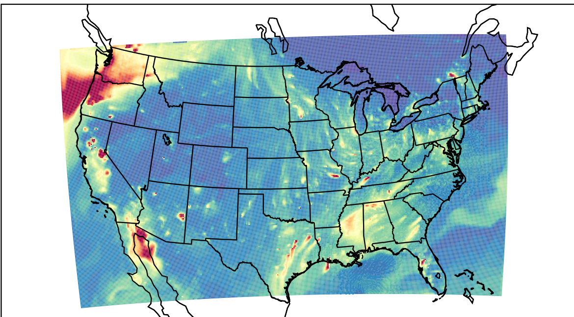
WRF 2023-11-12_02:00:00
