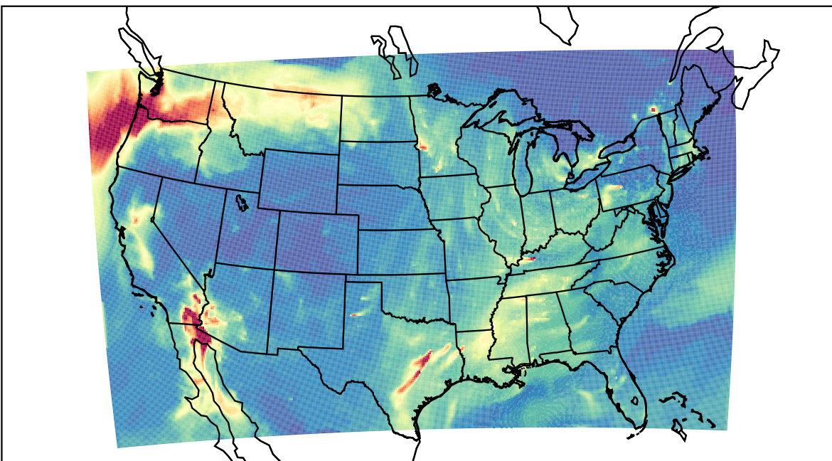
WRF 2023-11-12_12:00:00
