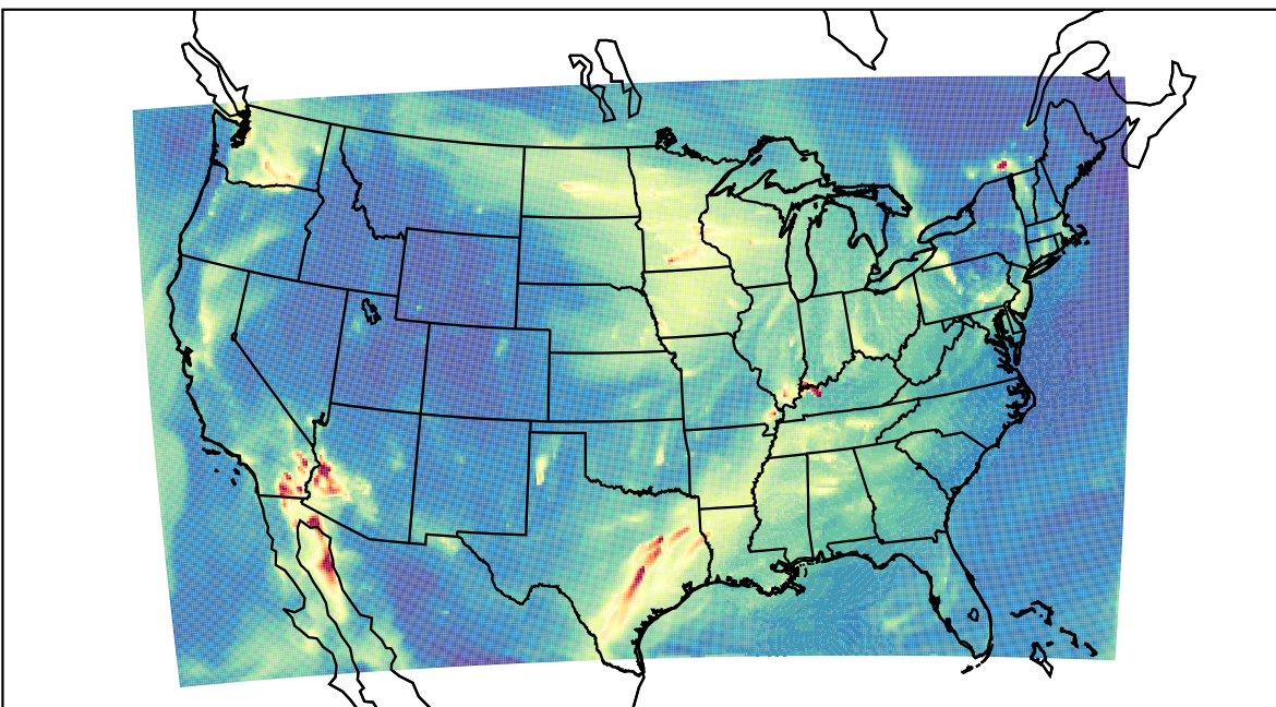
WRF 2023-11-13_07:00:00
