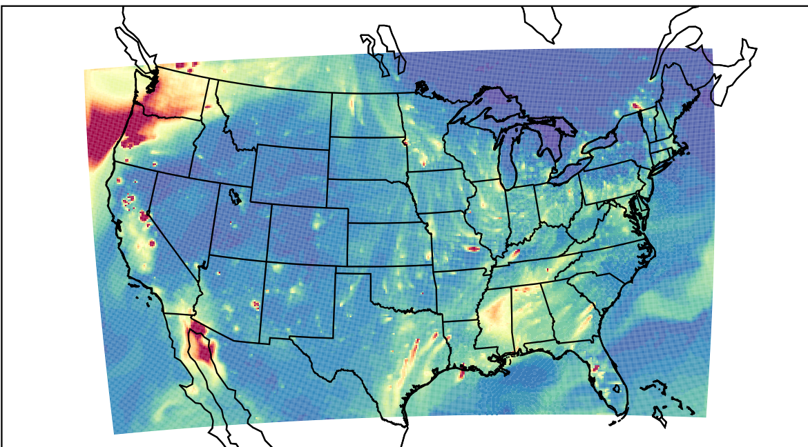
WRF 2023-11-12_01:00:00
