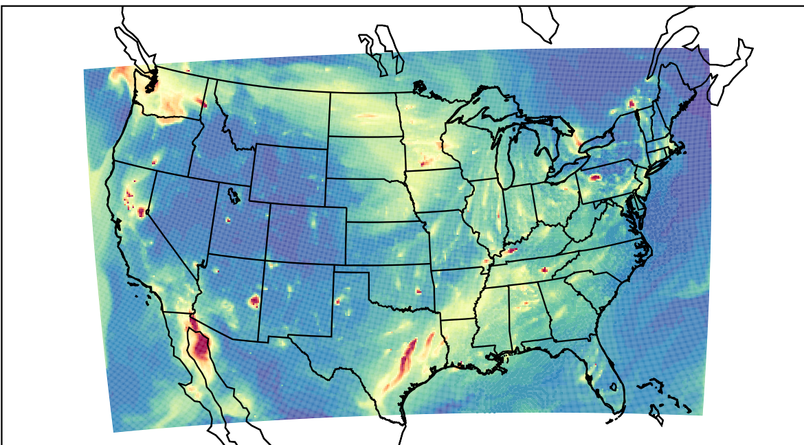
WRF 2023-11-13_02:00:00
