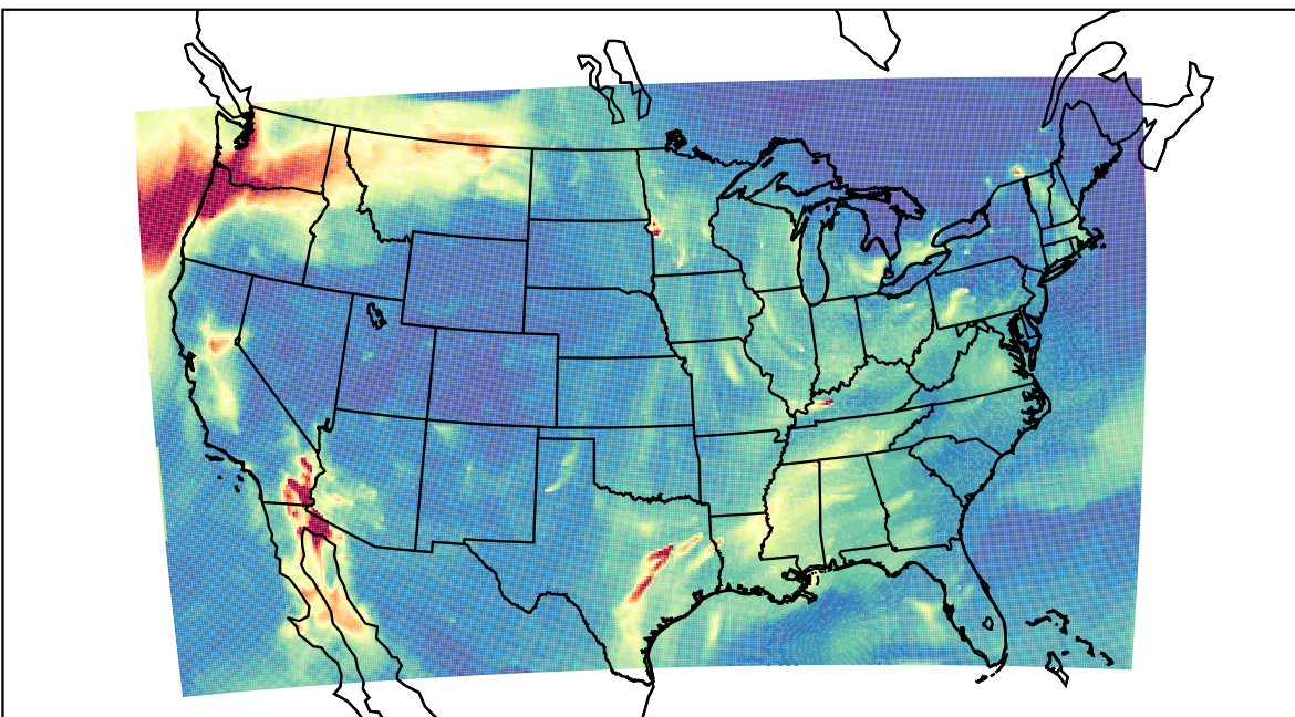
WRF 2023-11-12_09:00:00
