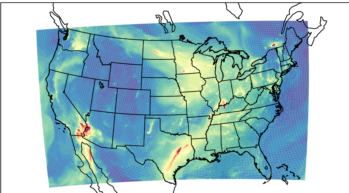
WRF 2023-11-13_12:00:00
