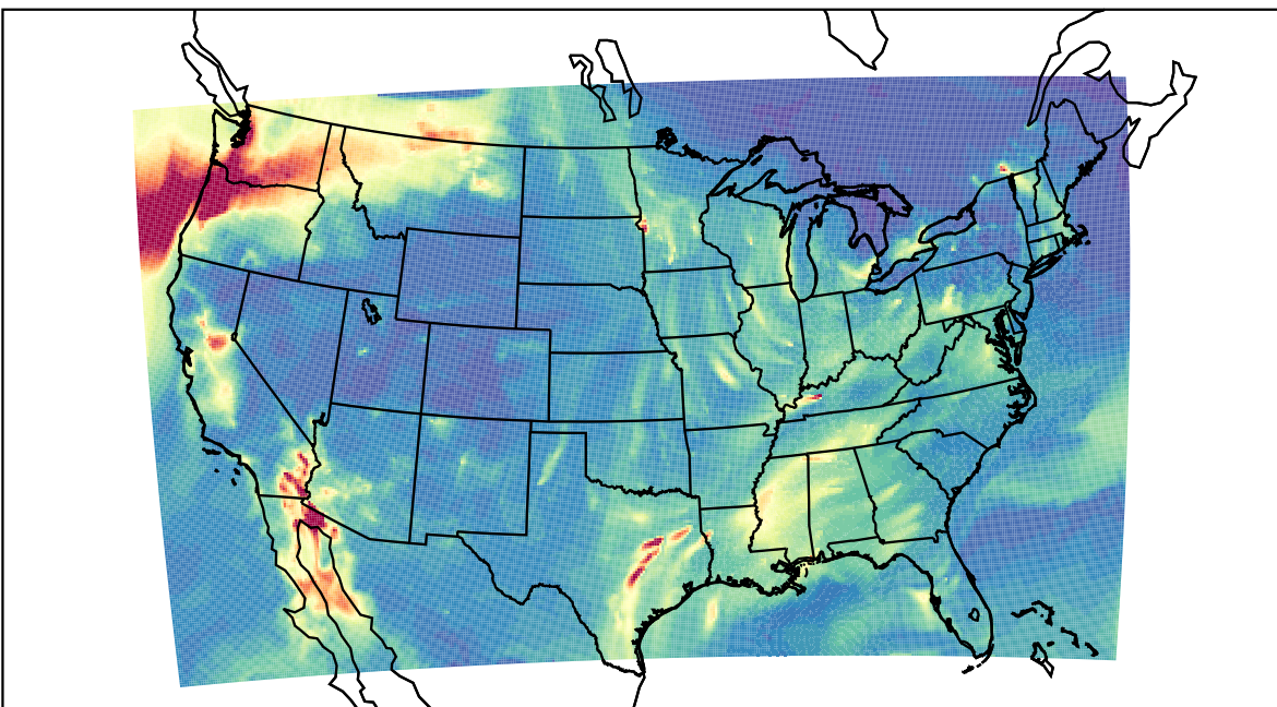
WRF 2023-11-12_07:00:00
