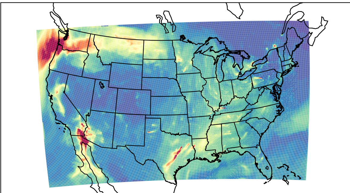
WRF 2023-11-12_14:00:00
