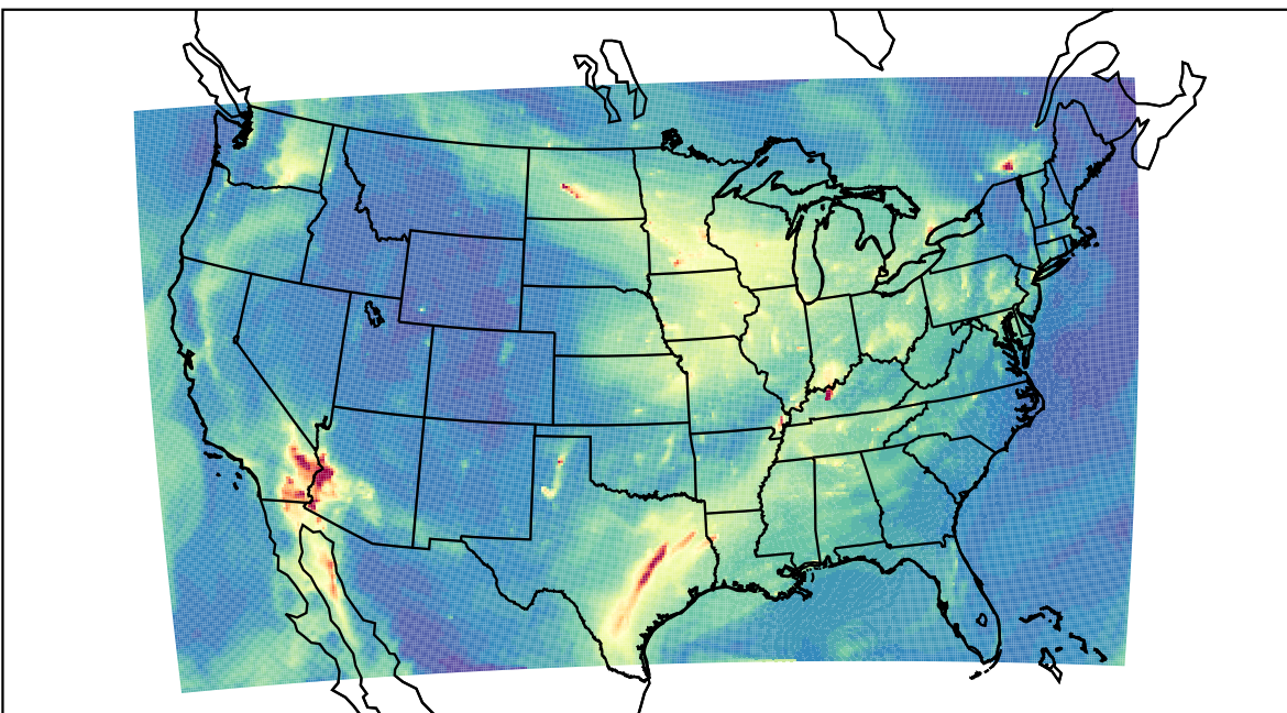
WRF 2023-11-13_14:00:00
