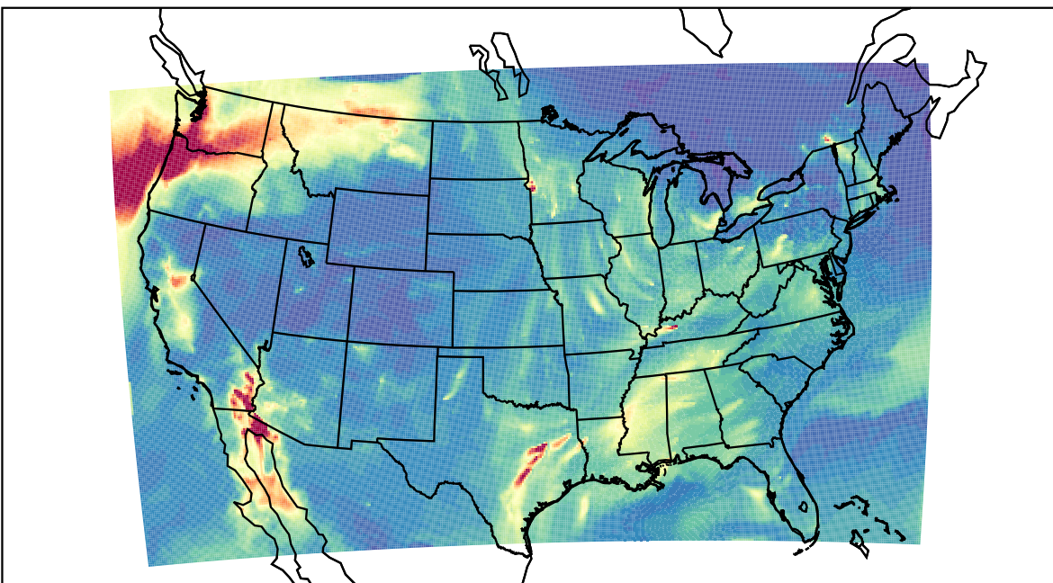
WRF 2023-11-12_08:00:00
