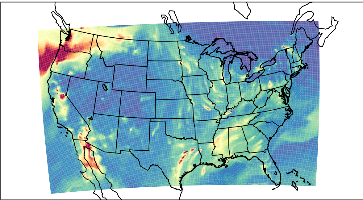
WRF 2023-11-12_05:00:00
