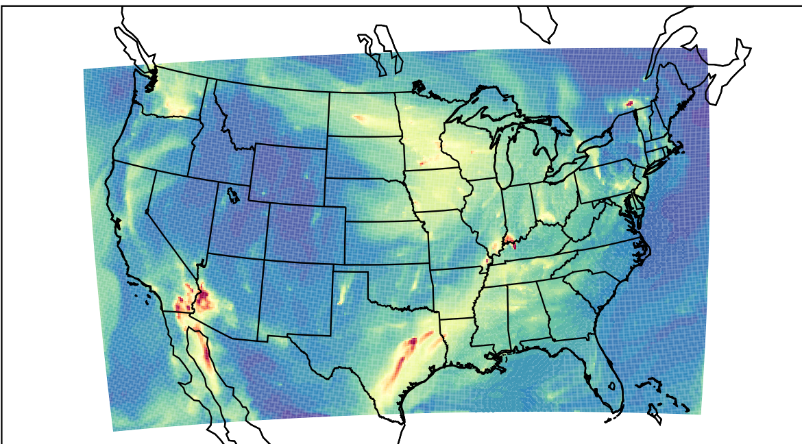
WRF 2023-11-13_09:00:00
