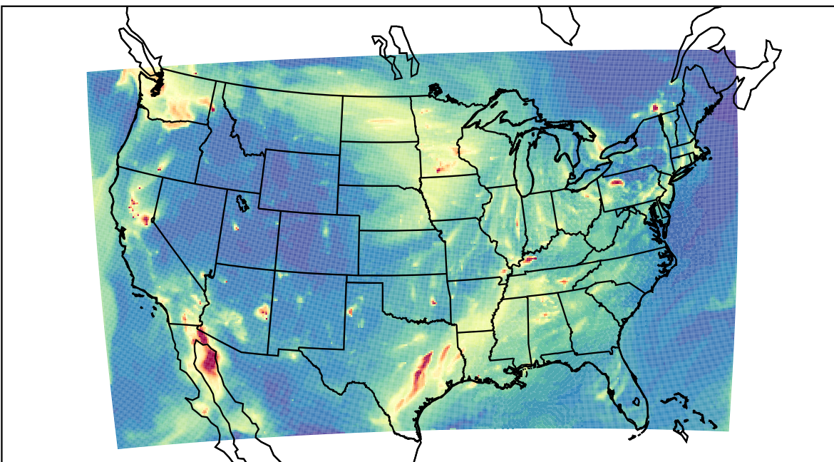
WRF 2023-11-13_03:00:00
