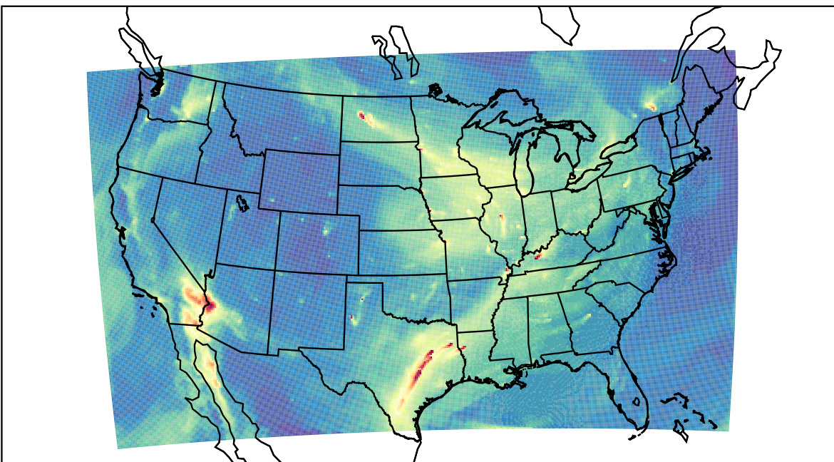
WRF 2023-11-13_17:00:00
