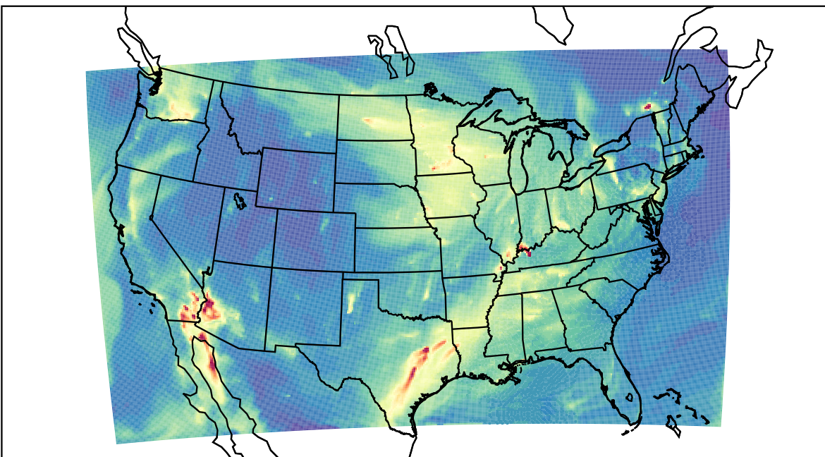
WRF 2023-11-13_08:00:00
