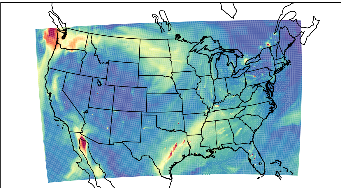
WRF 2023-11-12_21:00:00
