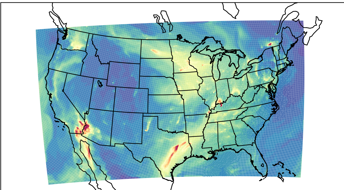
WRF 2023-11-13_11:00:00
