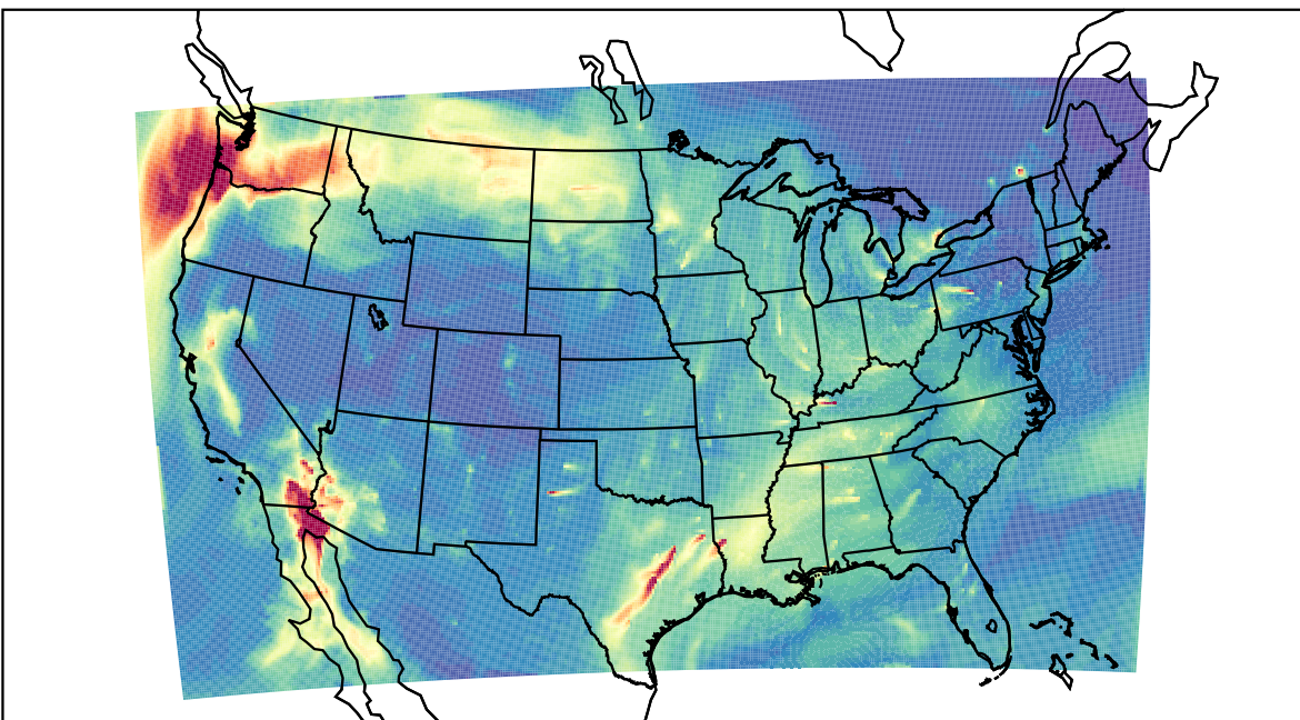
WRF 2023-11-12_15:00:00
