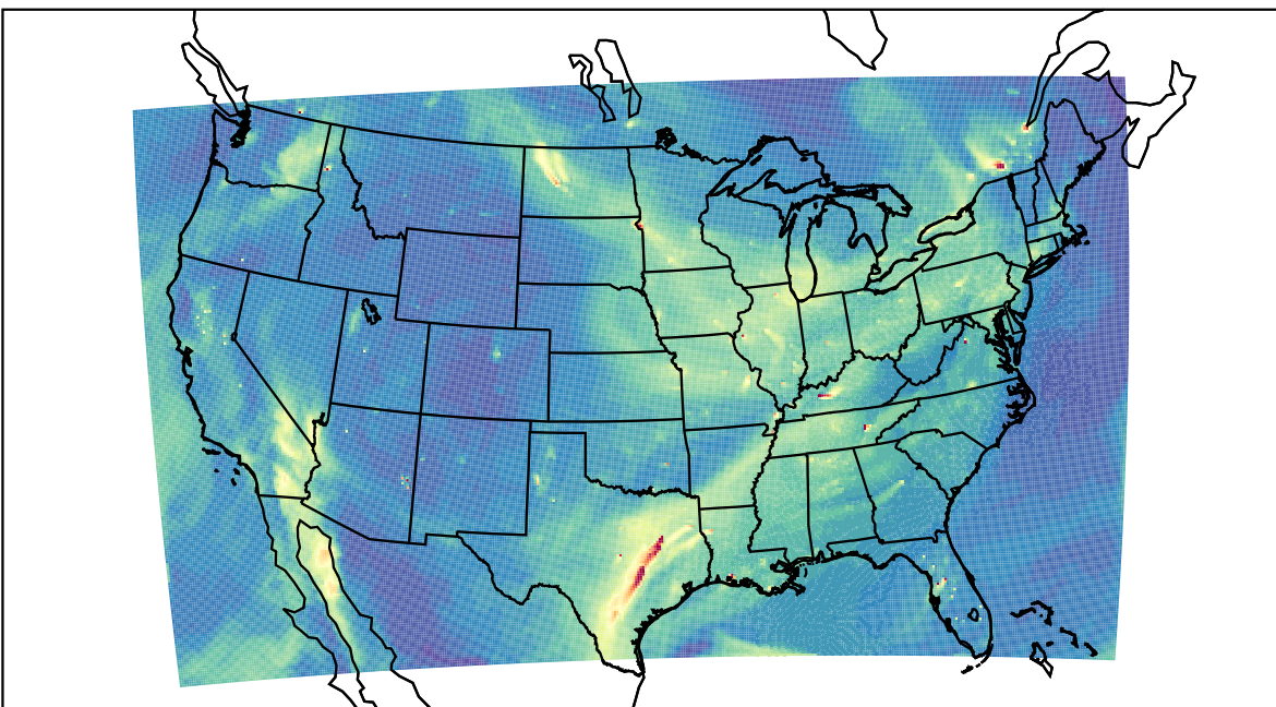
WRF 2023-11-13_21:00:00
