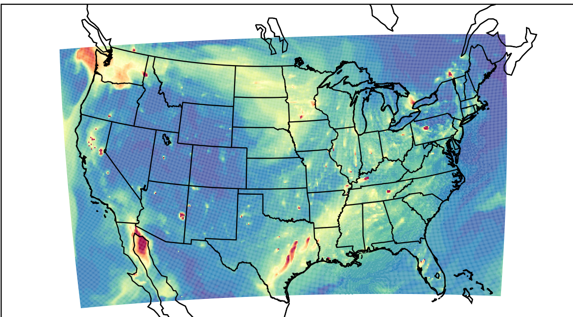
WRF 2023-11-13_00:00:00
