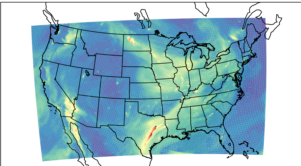
WRF 2023-11-13_19:00:00
