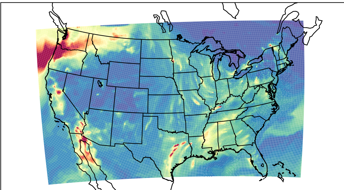
WRF 2023-11-12_06:00:00
