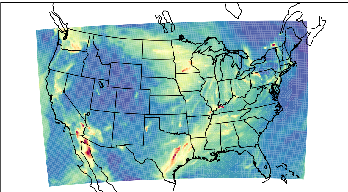
WRF 2023-11-13_05:00:00
