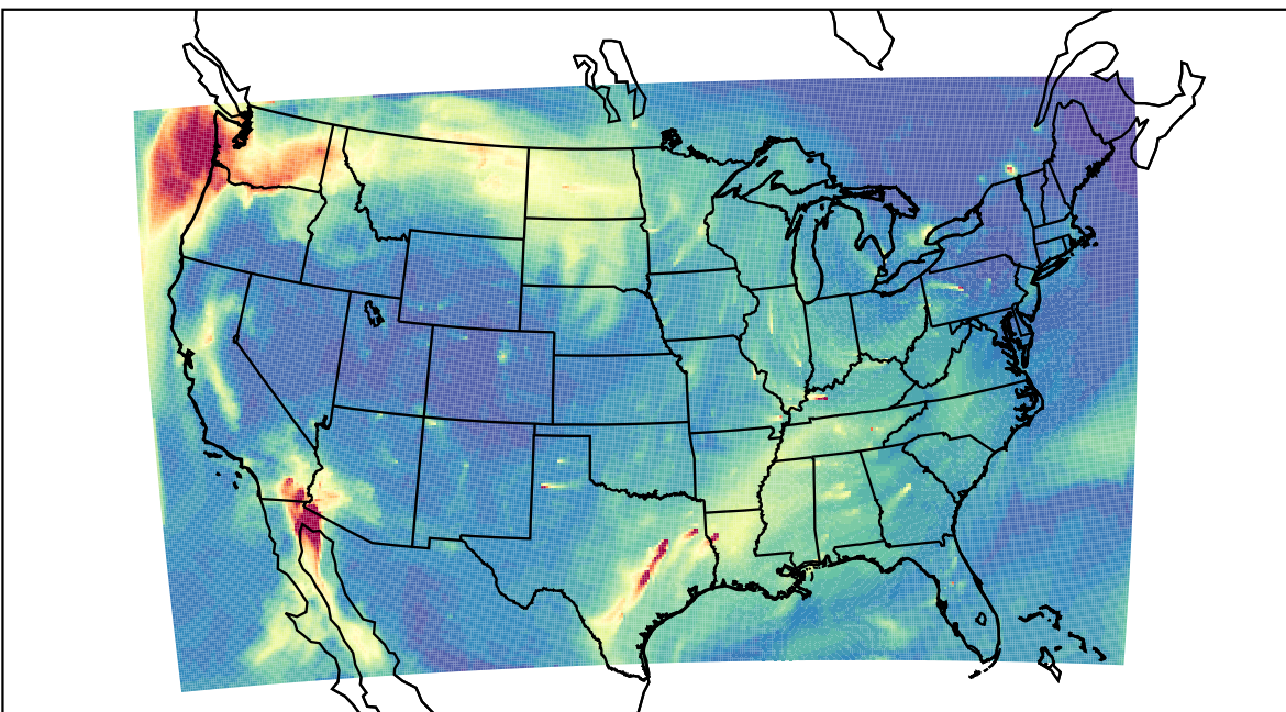
WRF 2023-11-12_17:00:00
