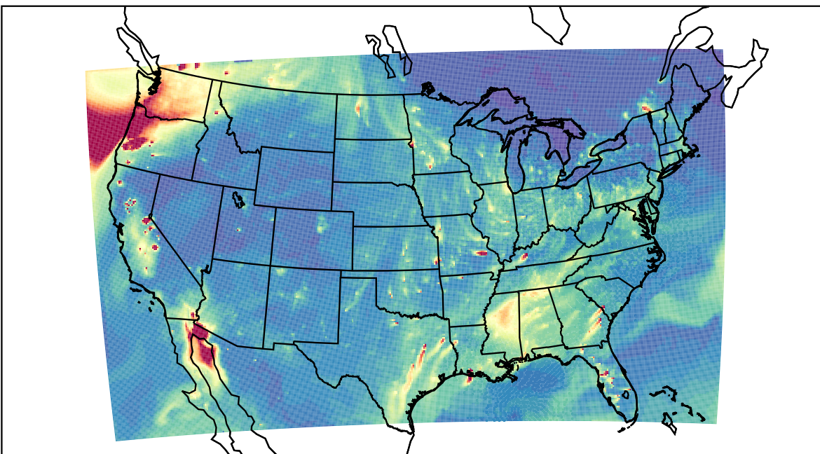
WRF 2023-11-12_00:00:00
