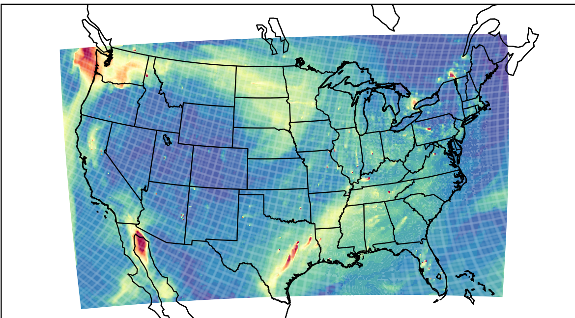
WRF 2023-11-12_22:00:00
