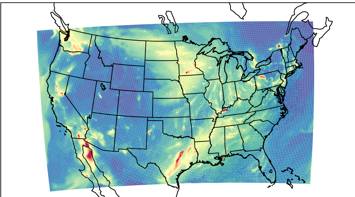
WRF 2023-11-13_04:00:00
